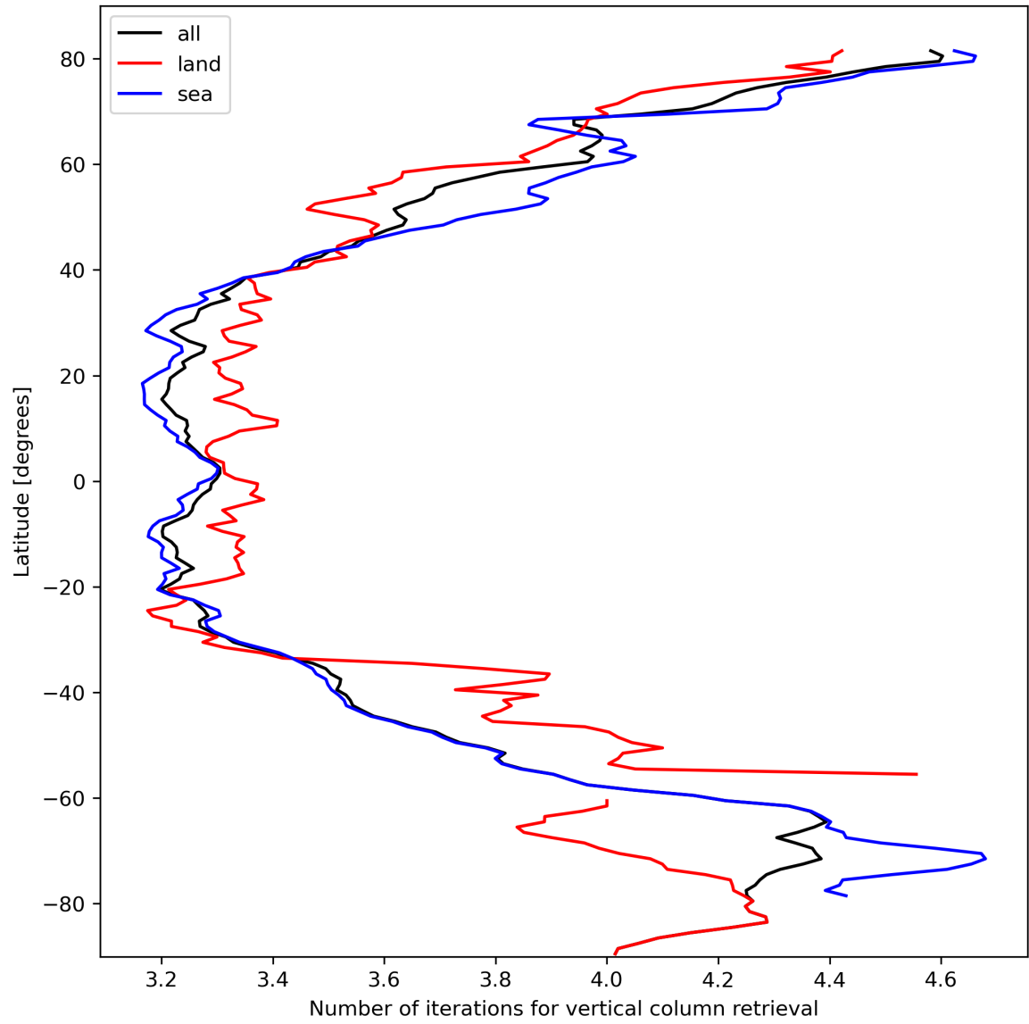
Figure 19: Zonal average of “Number of iterations for vertical column retrieval” for 2023-10-12 to 2023-10-13.
