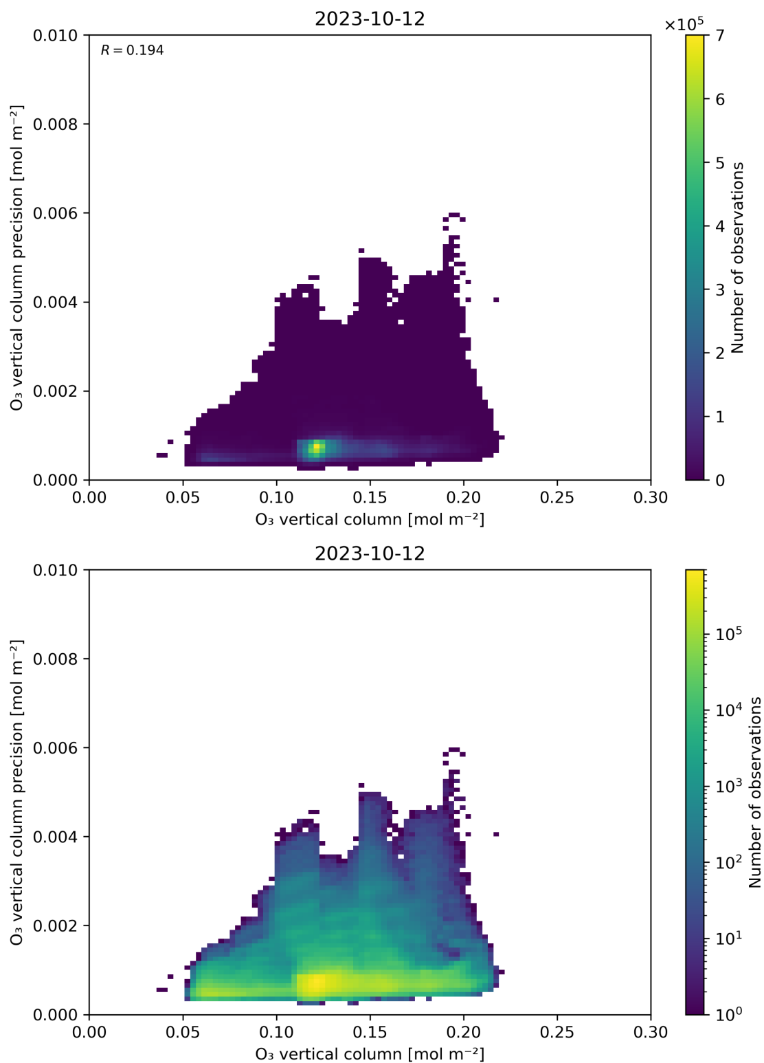
Figure 41: Scatter density plot of “O 3 vertical column” against “O 3 vertical column precision” for 2023-10-12 to 2023-10-13.
