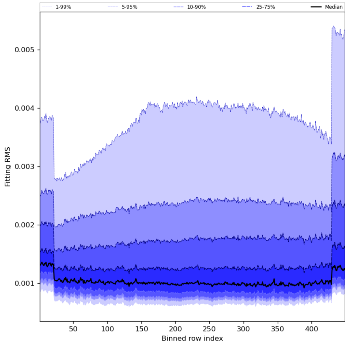
Figure 30: Along track statistics of “Fitting RMS” for 2023-10-12 to 2023-10-13
