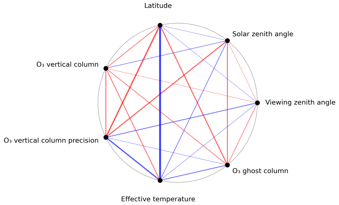
Figure 1: Map of correlation graph for 2023-10-12 to 2023-10-13.
