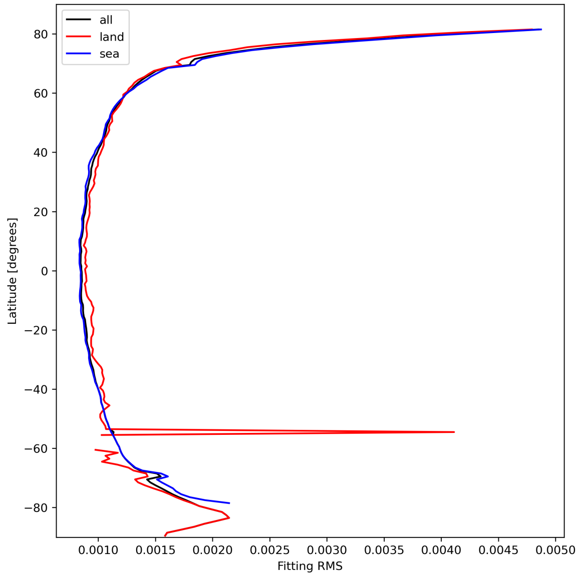
Figure 16: Zonal average of “Fitting RMS” for 2023-10-12 to 2023-10-13.
