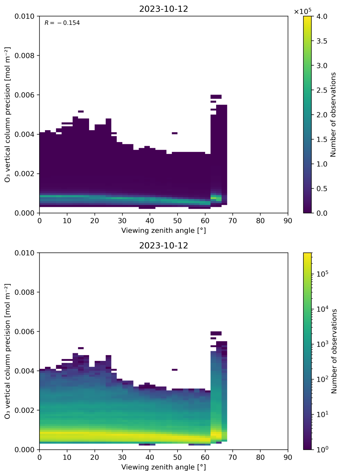
Figure 53: Scatter density plot of “Viewing zenith angle” against “O 3 vertical column precision” for 2023-10-12 to 2023-10-13.
