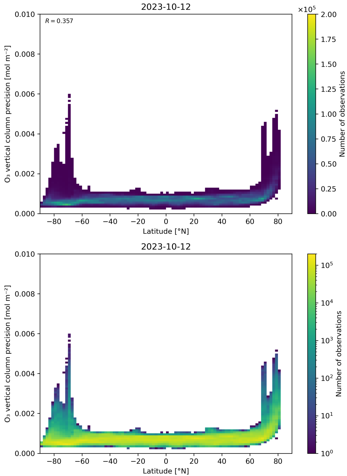
Figure 37: Scatter density plot of “Latitude” against “O 3 vertical column precision” for 2023-10-12 to 2023-10-13.
