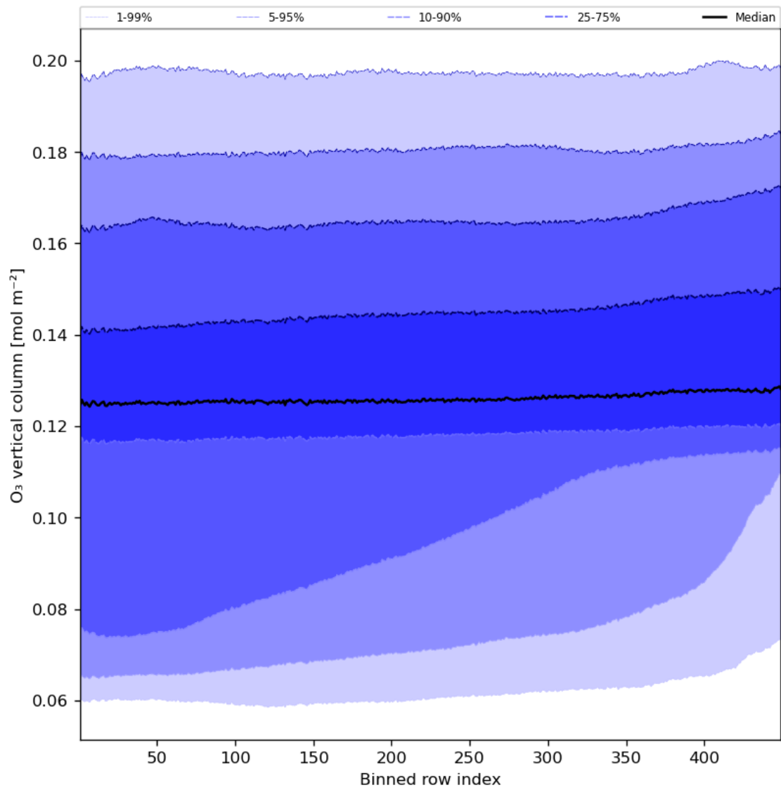
Figure 28: Along track statistics of “O 3 vertical column” for 2023-10-12 to 2023-10-13
