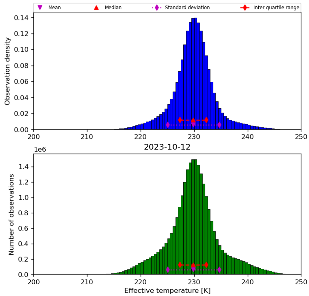
Figure 24: Histogram of “Effective temperature” for 2023-10-12 to 2023-10-13
