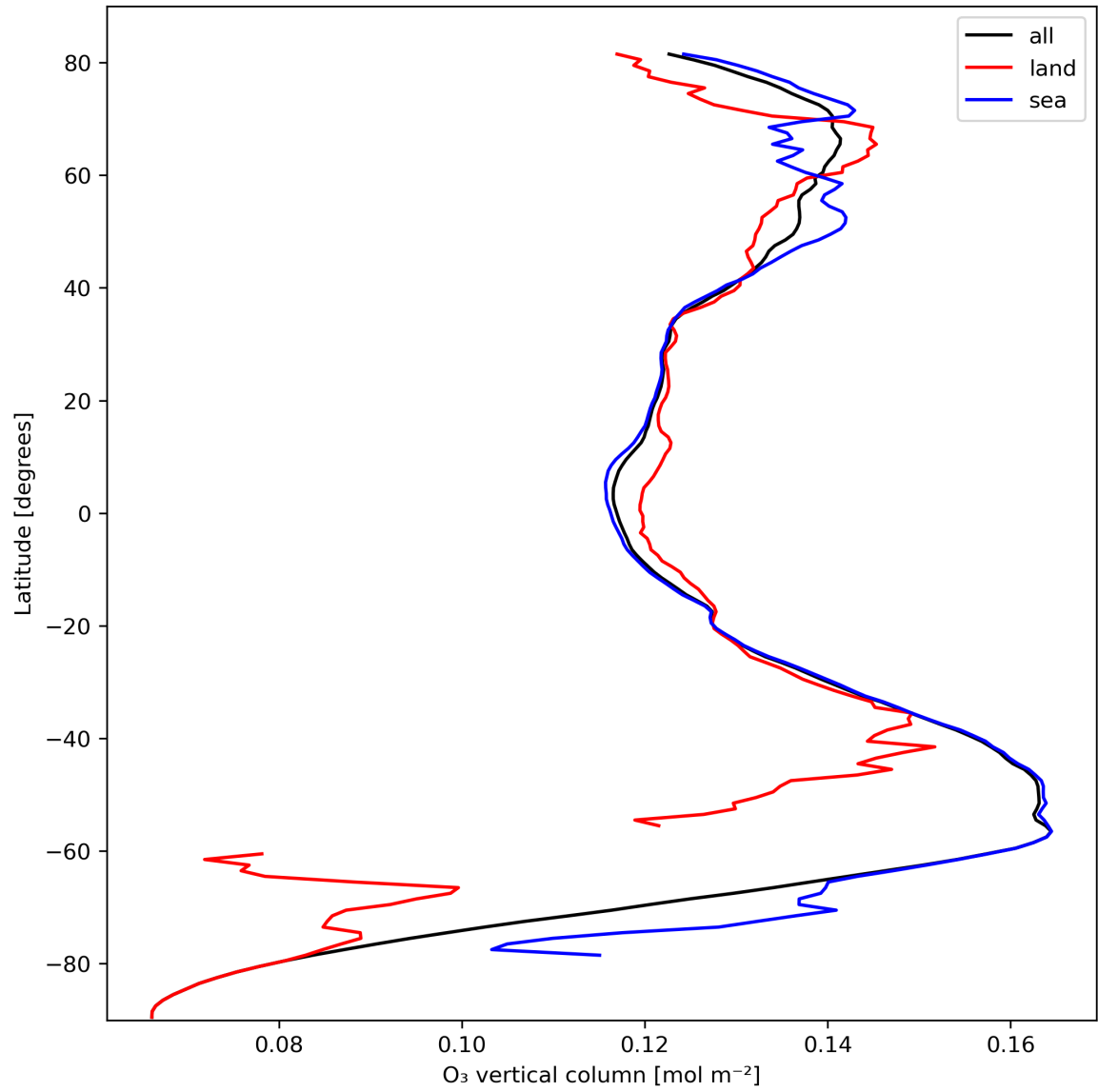
Figure 14: Zonal average of “O 3 vertical column” for 2023-10-12 to 2023-10-13.
