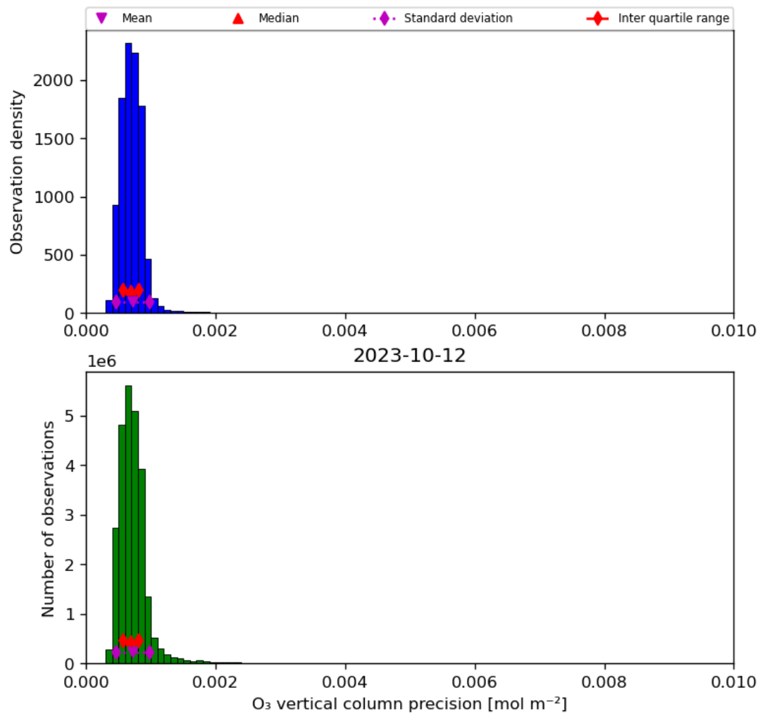
Figure 22: Histogram of “O 3 vertical column precision” for 2023-10-12 to 2023-10-13
