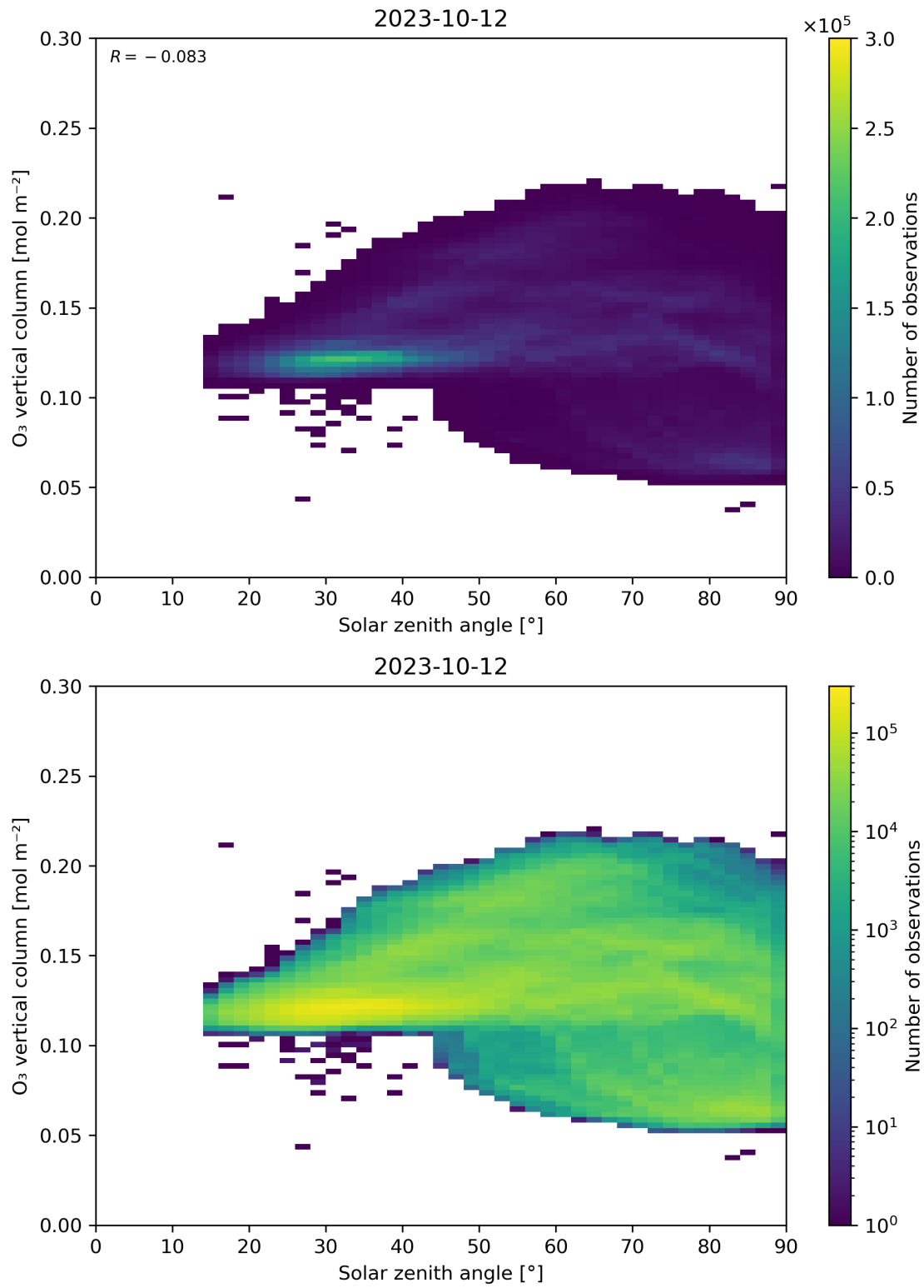
Figure 47: Scatter density plot of “Solar zenith angle” against “O 3 vertical column” for 2023-10-12 to 2023-10-13.
