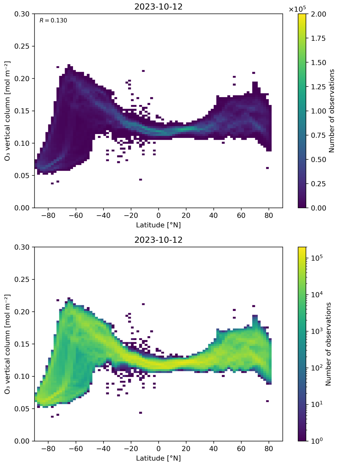
Figure 36: Scatter density plot of “Latitude” against “O 3 vertical column” for 2023-10-12 to 2023-10-13.
