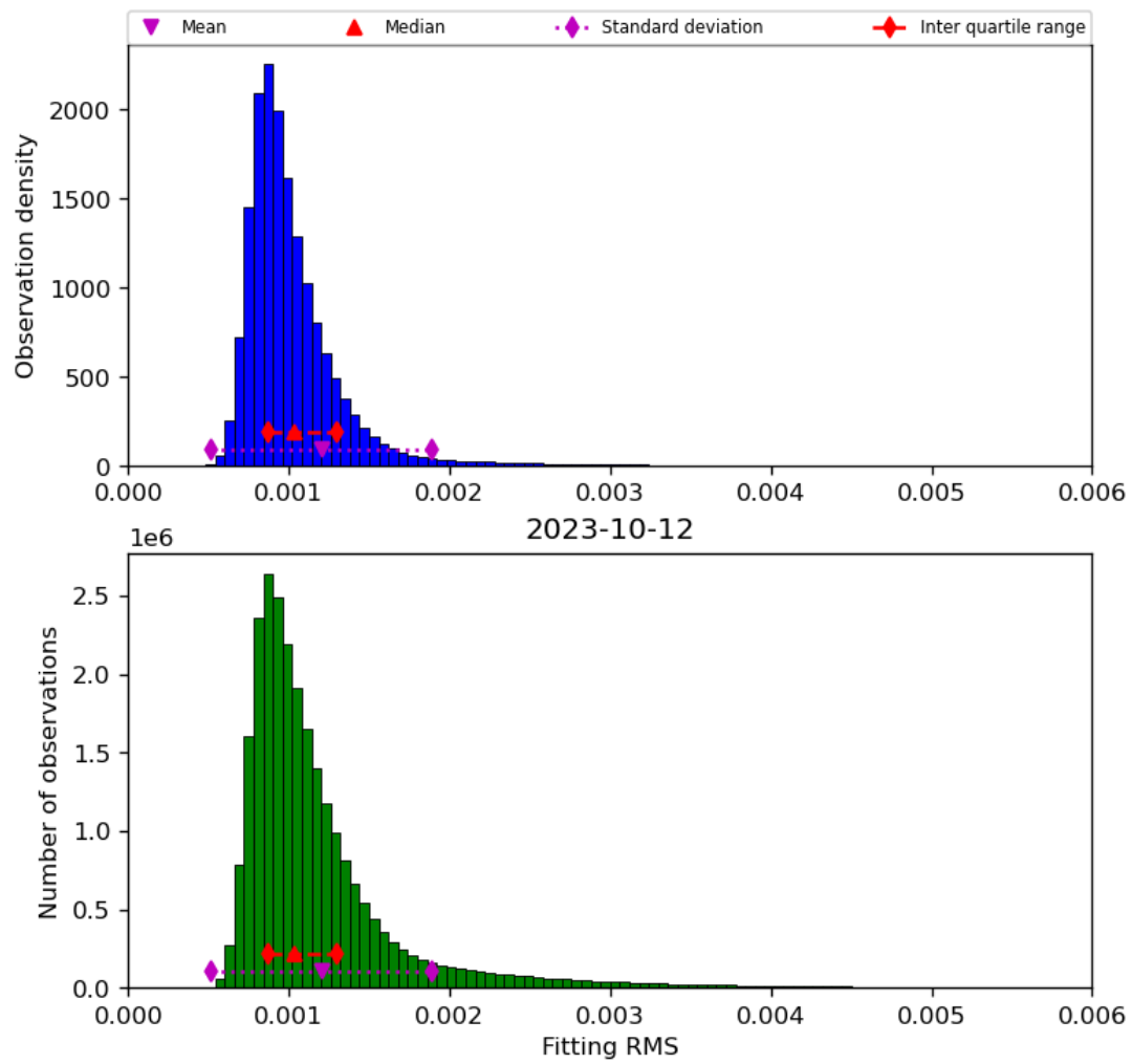
Figure 23: Histogram of “Fitting RMS” for 2023-10-12 to 2023-10-13
