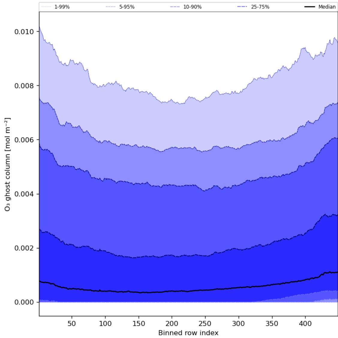
Figure 32: Along track statistics of “O 3 ghost column” for 2023-10-12 to 2023-10-13
