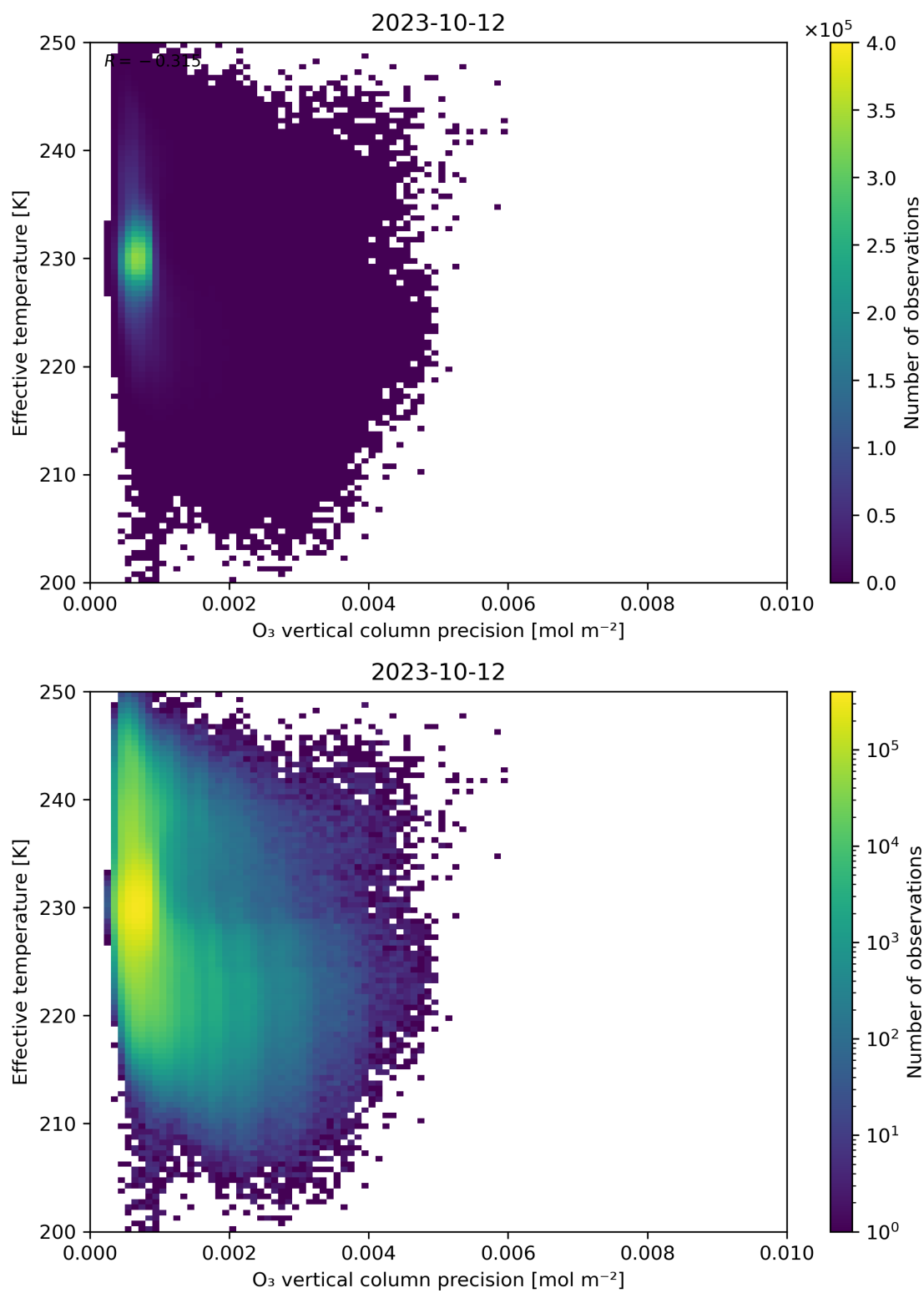
Figure 42: Scatter density plot of “ O_3 vertical column precision” against “Effective temperature” for 2023-10-12 to 2023-10-13.
