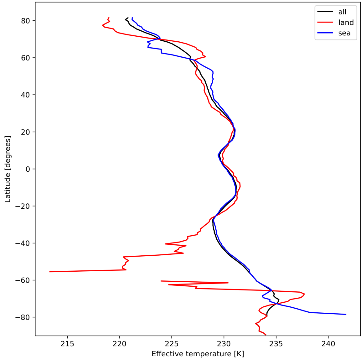
Figure 17: Zonal average of “Effective temperature” for 2023-10-12 to 2023-10-13.
