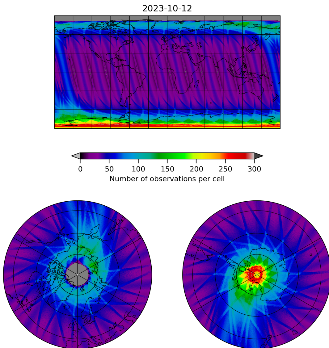
Figure 12: Map of the number of observations for 2023-10-12 to 2023-10-13
