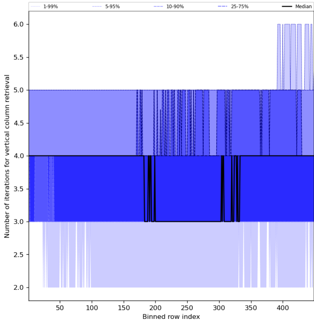
Figure 33: Along track statistics of “Number of iterations for vertical column retrieval” for 2023-10-12 to 2023-10-13
