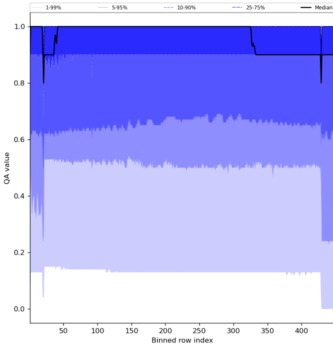
Figure 27: Along track statistics of “QA value” for 2023-10-12 to 2023-10-13
