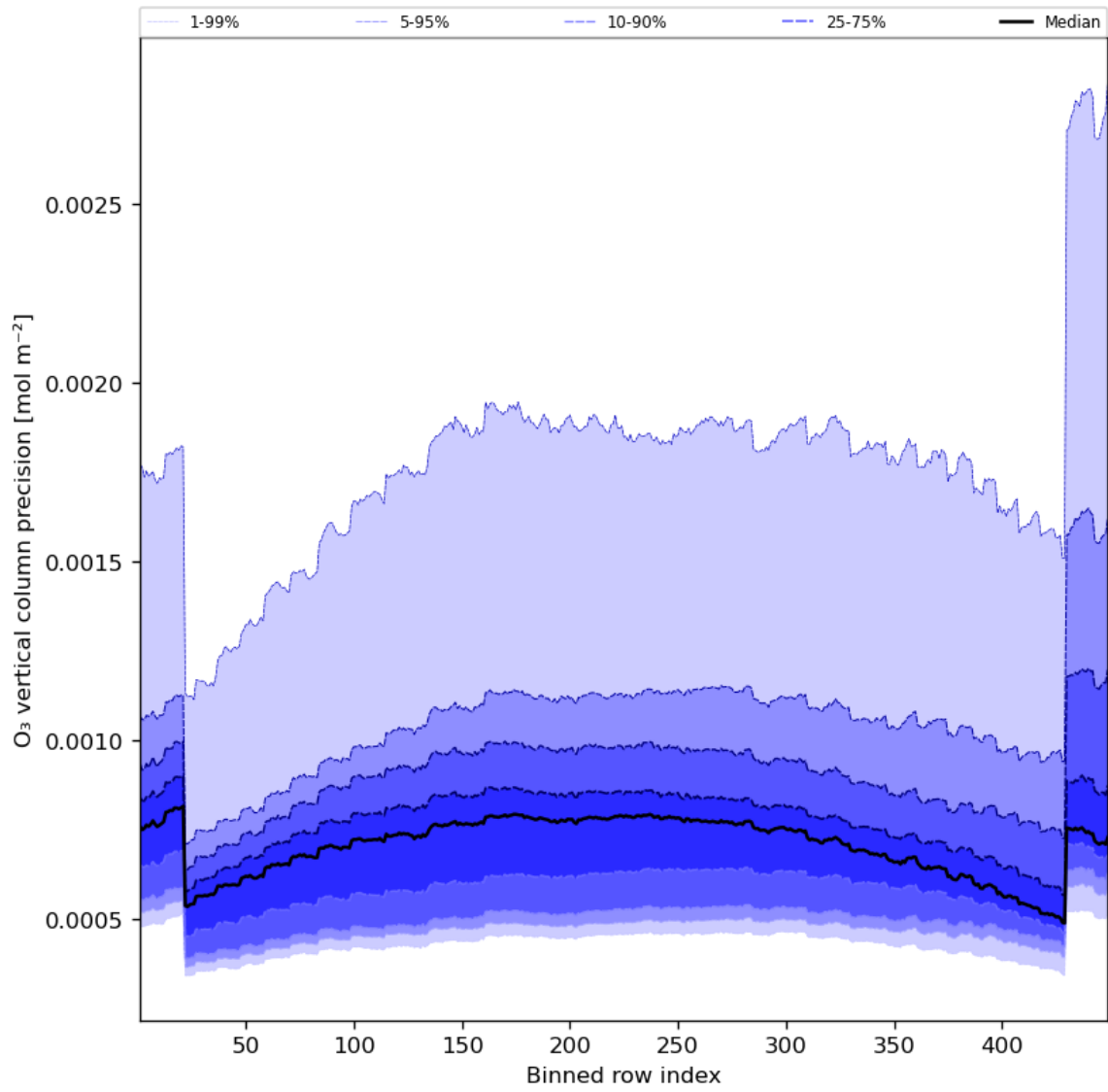
Figure 29: Along track statistics of “O 3 vertical column precision” for 2023-10-12 to 2023-10-13
