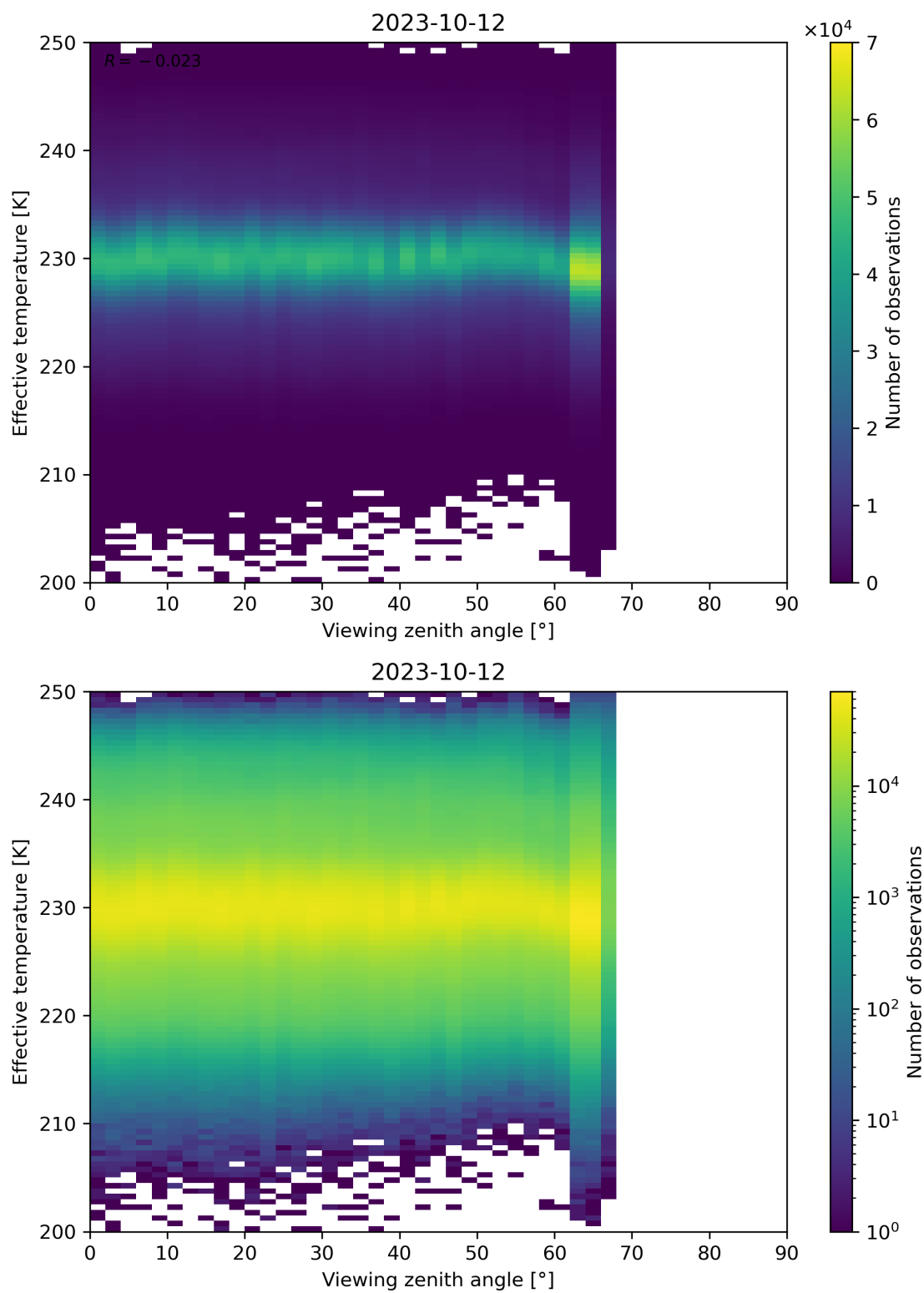
Figure 50: Scatter density plot of “Viewing zenith angle” against “Effective temperature” for 2023-10-12 to 2023-10-13.
