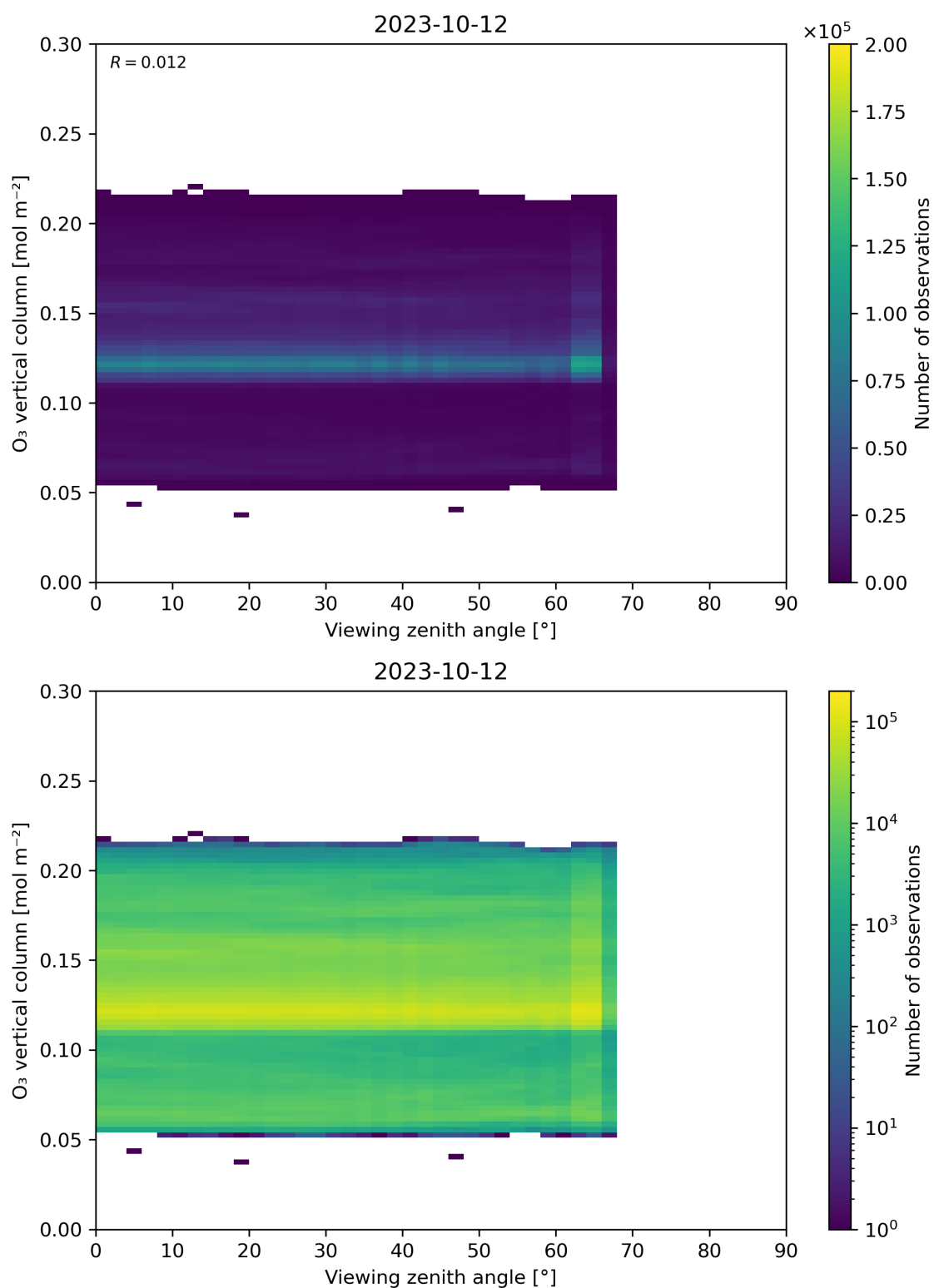
Figure 52: Scatter density plot of “Viewing zenith angle” against “O 3 vertical column” for 2023-10-12 to 2023-10-13.
