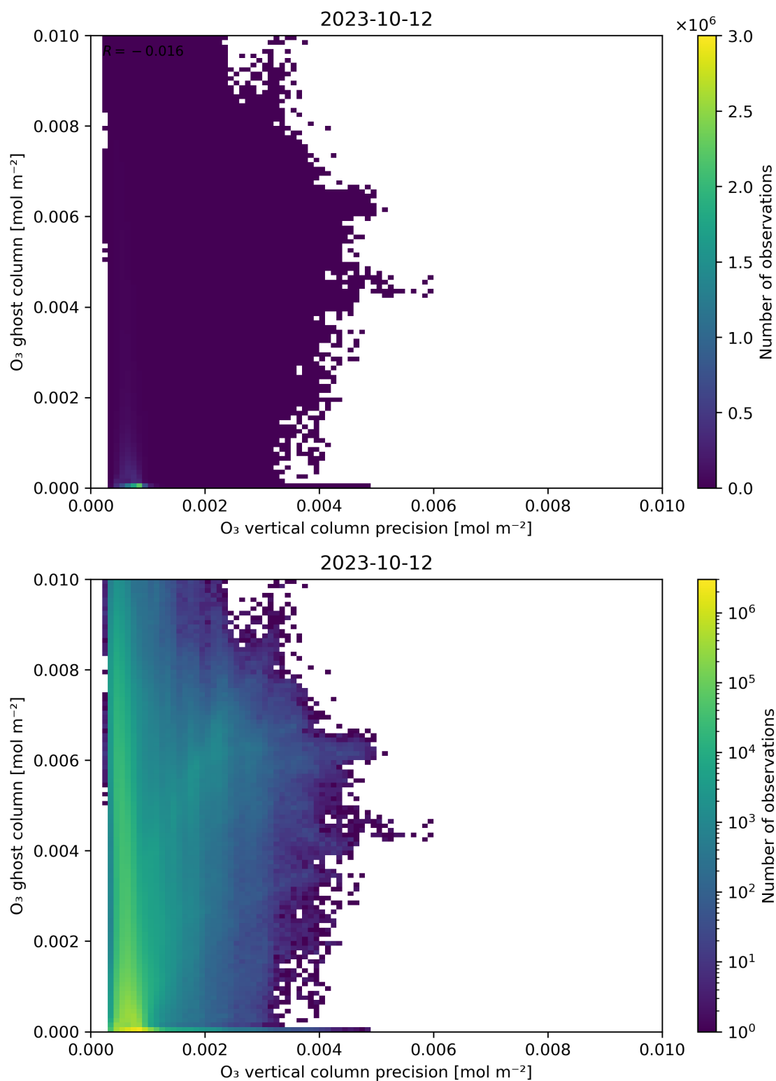
Figure 43: Scatter density plot of “ O_3 vertical column precision” against “ O_3 ghost column” for 2023-10-12 to 2023-10-13.
