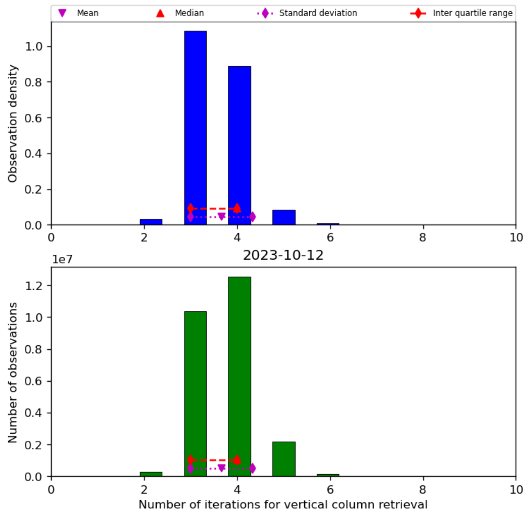
Figure 26: Histogram of “Number of iterations for vertical column retrieval” for 2023-10-12 to 2023-10-13
