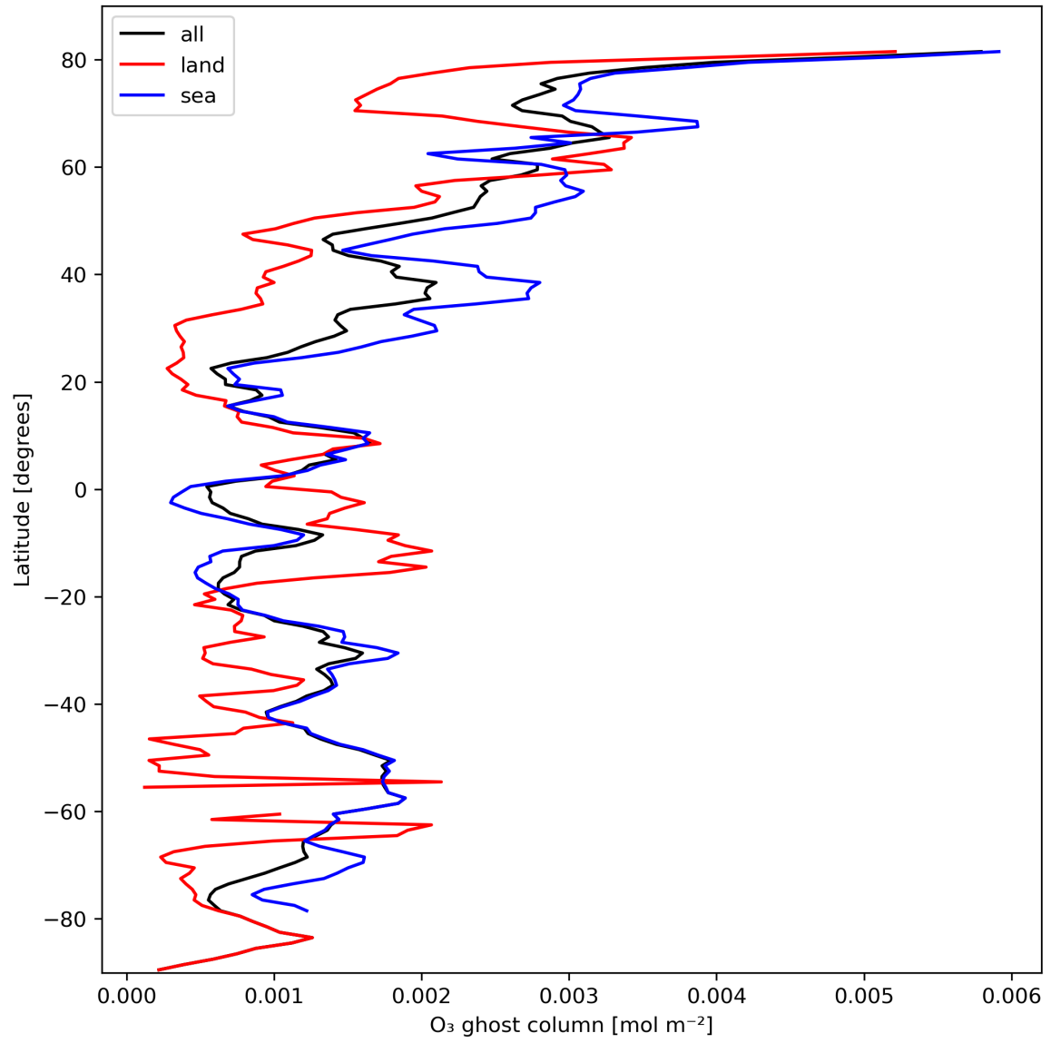
Figure 18: Zonal average of "O 3 ghost column" for 2023-10-12 to 2023-10-13.
