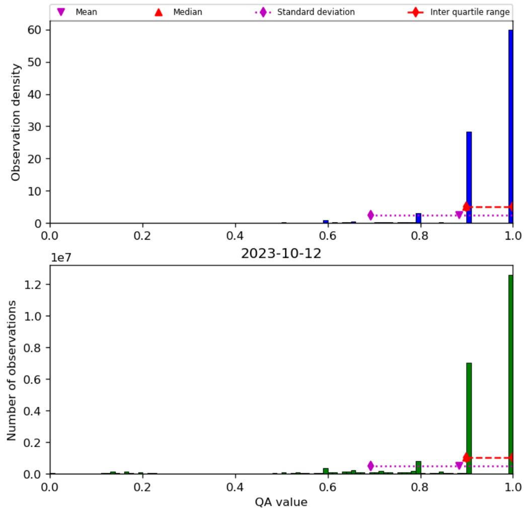
Figure 20: Histogram of “QA value” for 2023-10-12 to 2023-10-13
