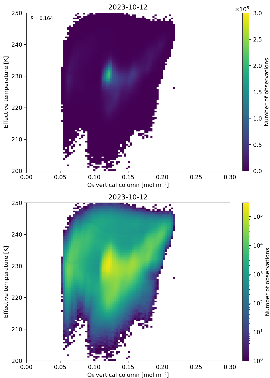
Figure 39: Scatter density plot of “O 3 vertical column” against “Effective temperature” for 2023-10-12 to 2023-10-13.
