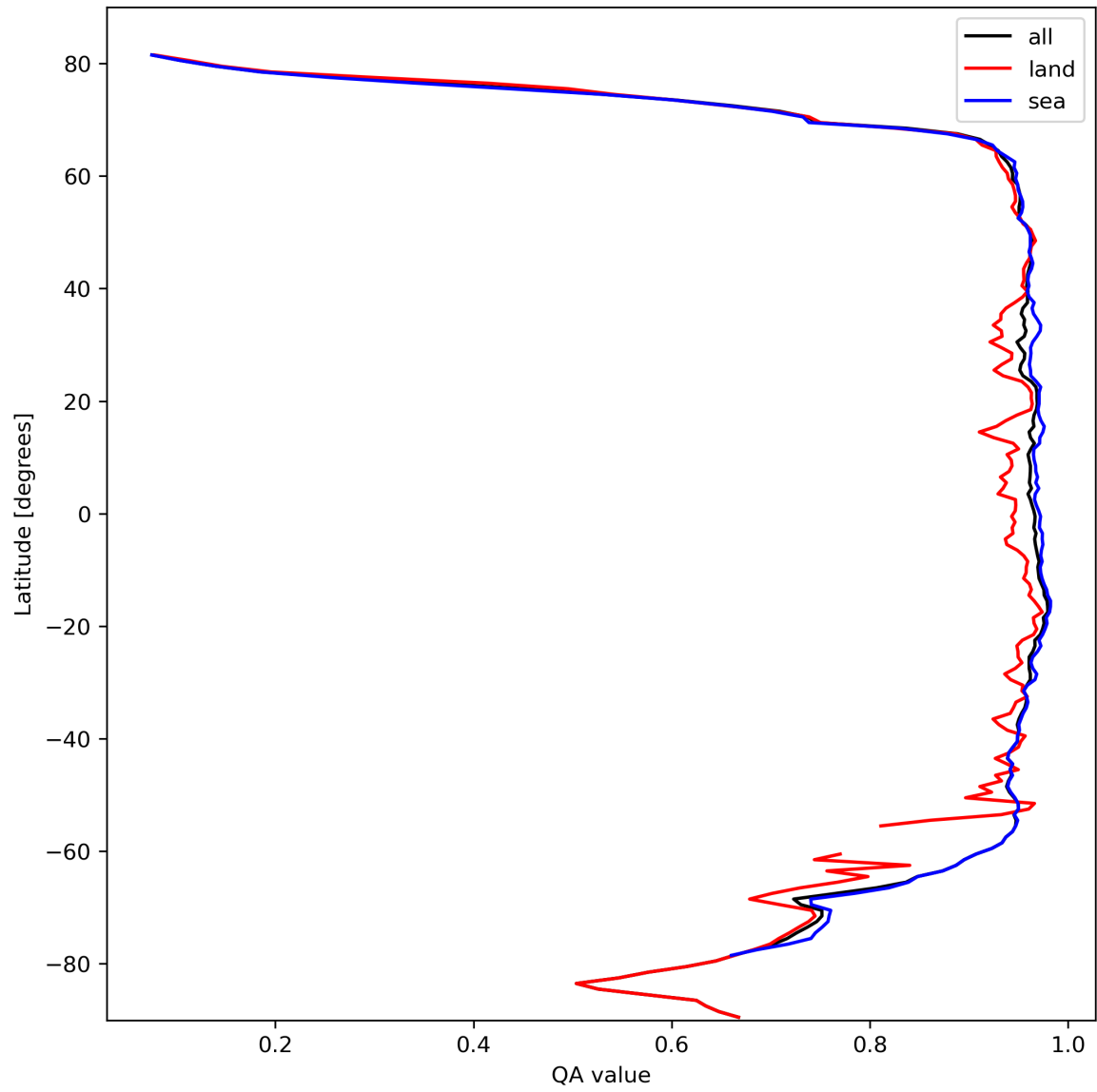
Figure 13: Zonal average of “QA value” for 2023-10-12 to 2023-10-13.
