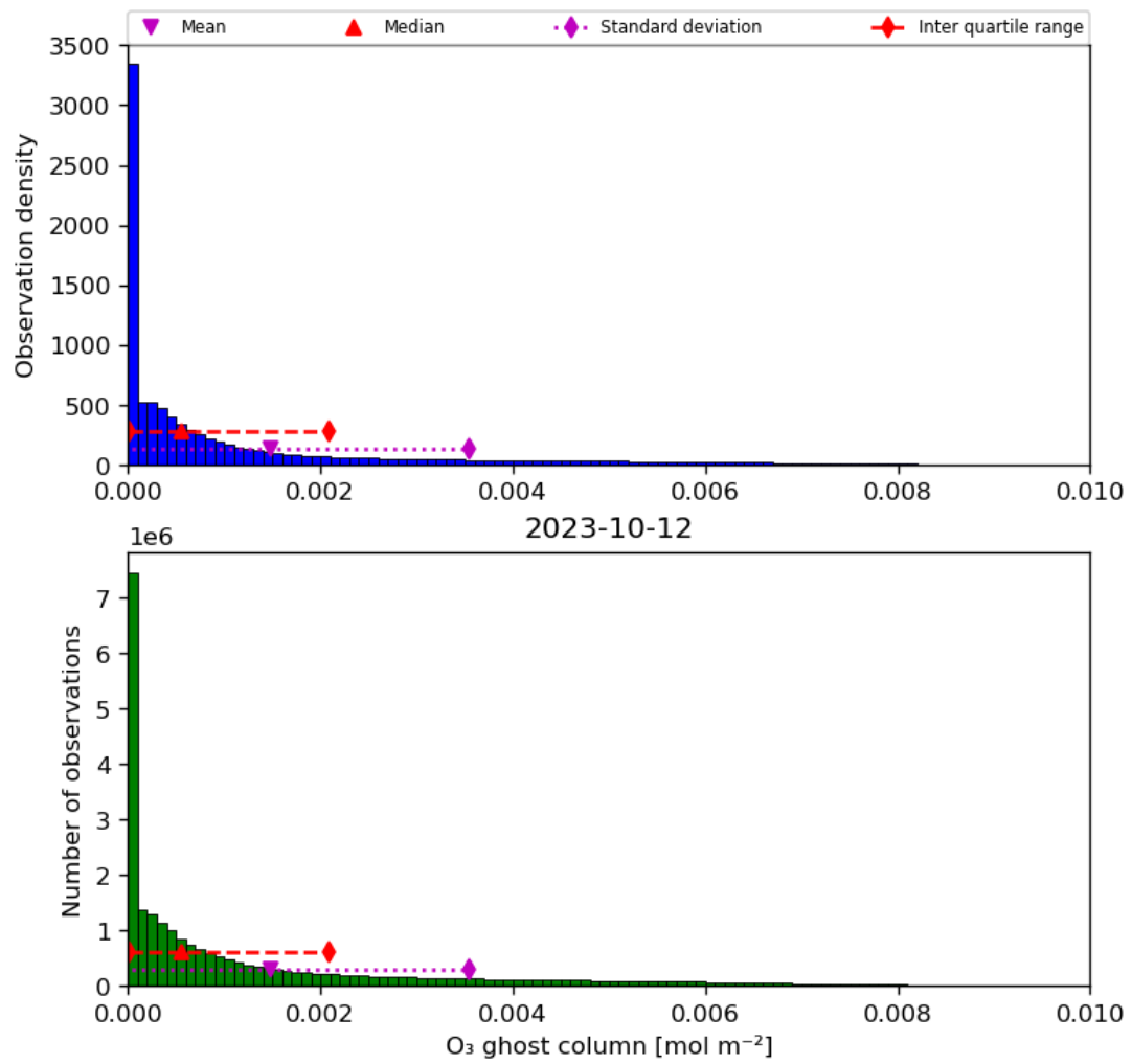
Figure 25: Histogram of “O 3 ghost column” for 2023-10-12 to 2023-10-13
