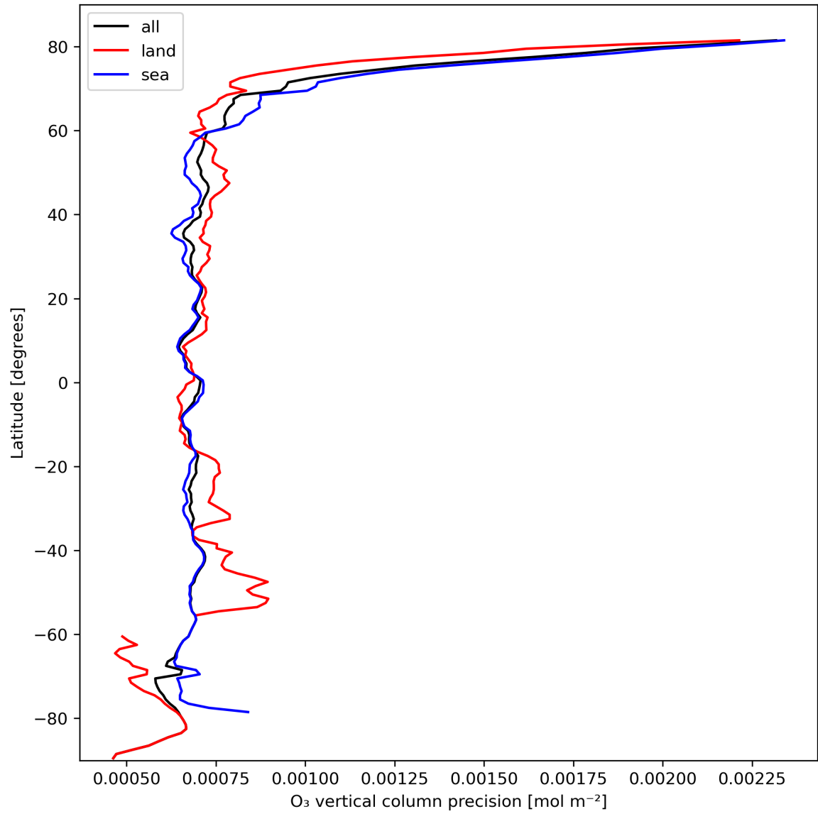
Figure 15: Zonal average of "O 3 vertical column precision" for 2023-10-12 to 2023-10-13.
