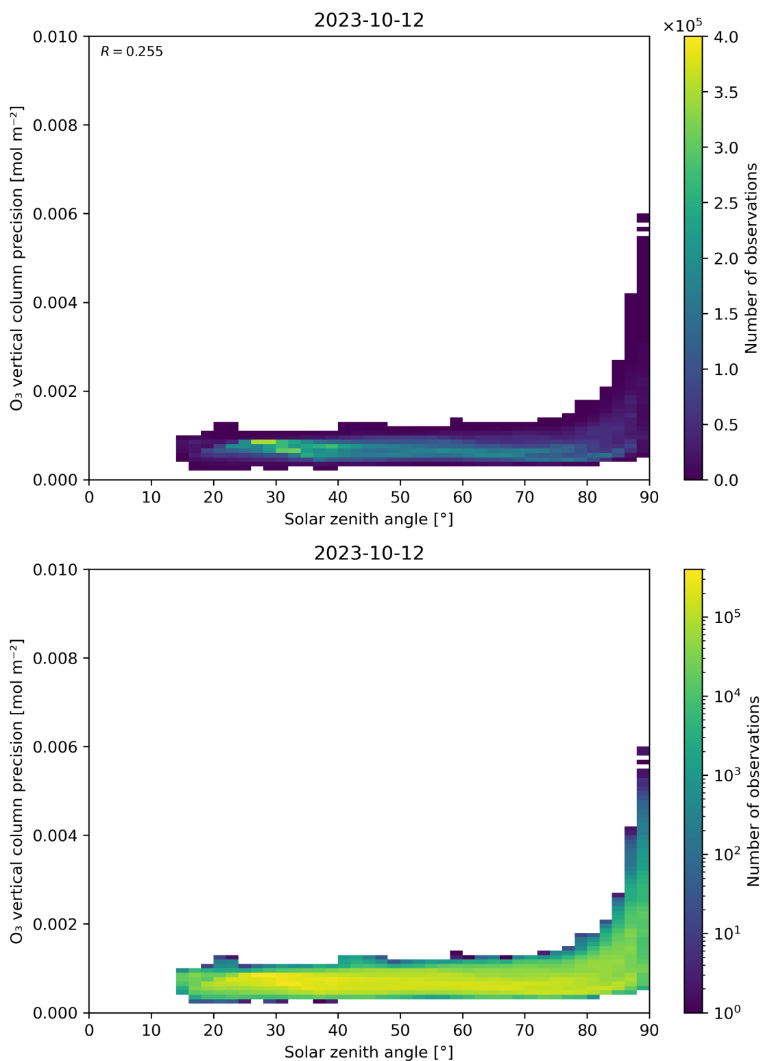
Figure 48: Scatter density plot of “Solar zenith angle” against “O 3 vertical column precision” for 2023-10-12 to 2023-10-13.
