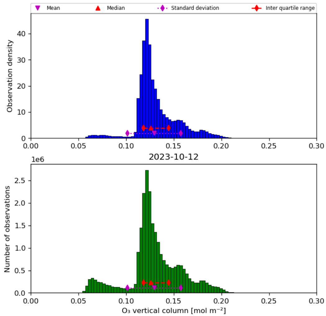
Figure 21: Histogram of “O 3 vertical column” for 2023-10-12 to 2023-10-13
