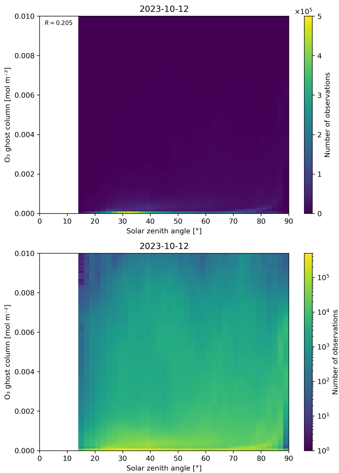
Figure 46: Scatter density plot of “Solar zenith angle” against “O 3 ghost column” for 2023-10-12 to 2023-10-13.
