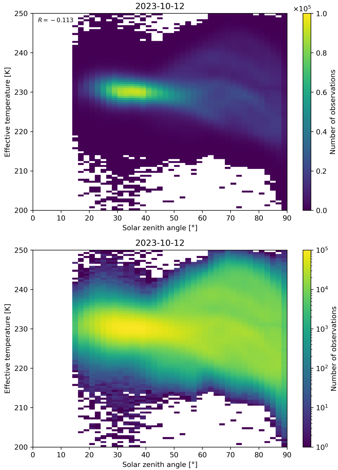
Figure 45: Scatter density plot of “Solar zenith angle” against “Effective temperature” for 2023-10-12 to 2023-10-13.
