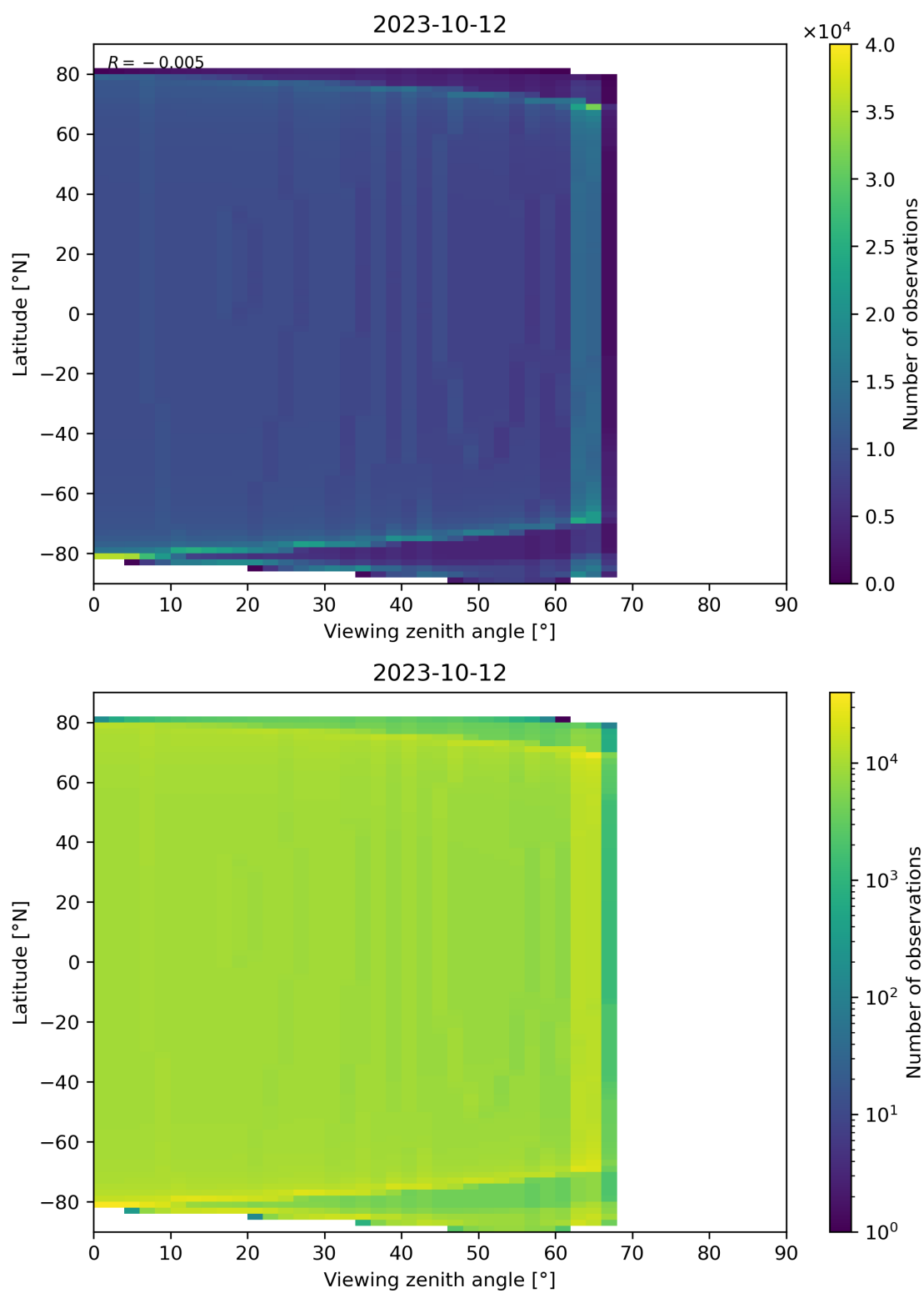
Figure 49: Scatter density plot of “Viewing zenith angle” against “Latitude” for 2023-10-12 to 2023-10-13.
