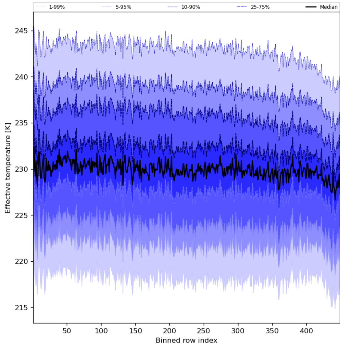
Figure 31: Along track statistics of “Effective temperature” for 2023-10-12 to 2023-10-13
