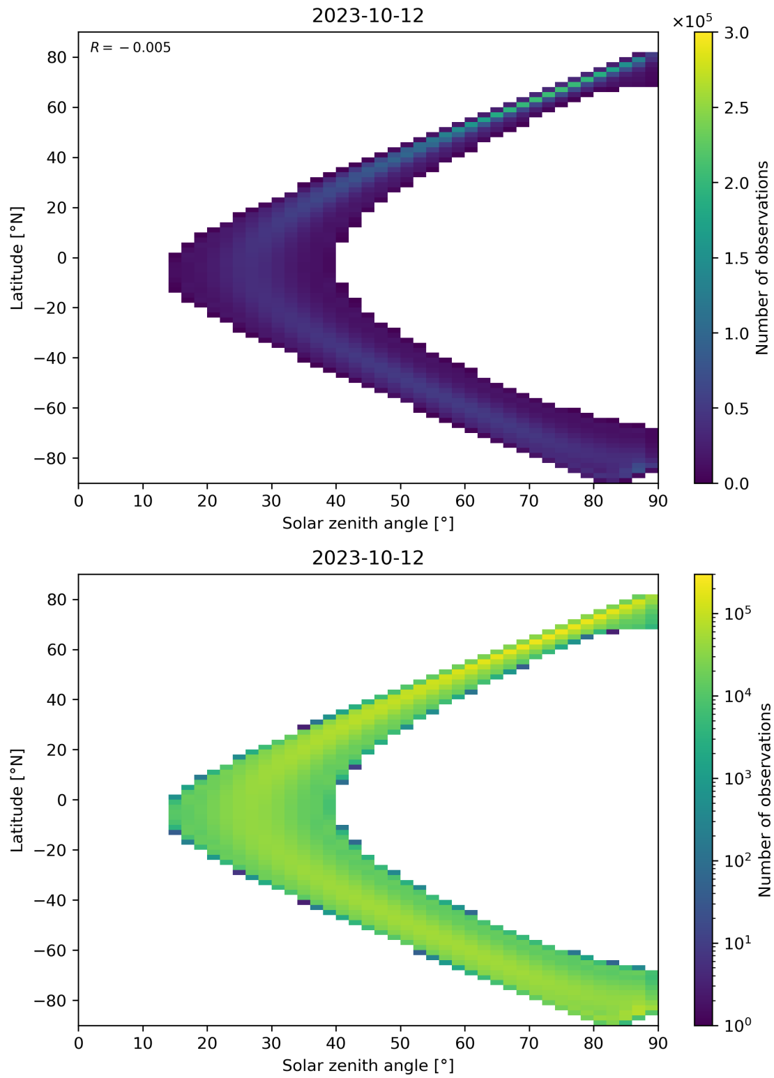
Figure 44: Scatter density plot of “Solar zenith angle” against “Latitude” for 2023-10-12 to 2023-10-13.
