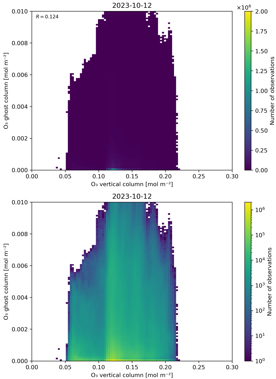
Figure 40: Scatter density plot of “O 3 vertical column” against “O 3 ghost column” for 2023-10-12 to 2023-10-13.
