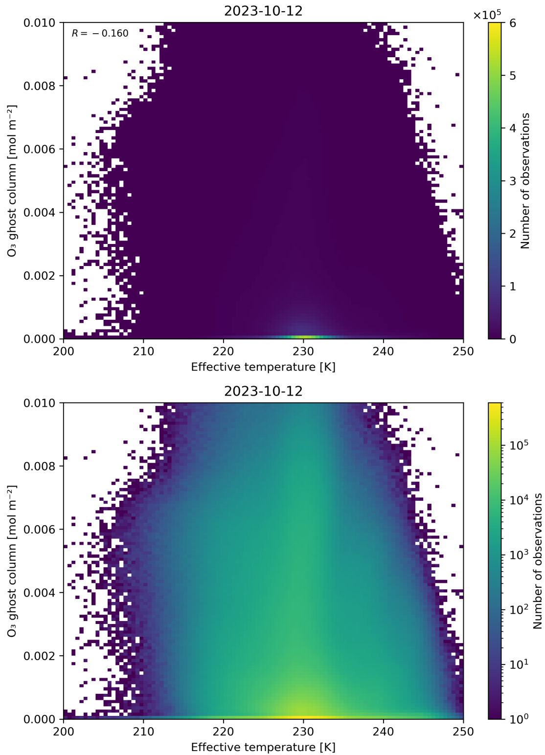
Figure 38: Scatter density plot of “Effective temperature” against “O 3 ghost column” for 2023-10-12 to 2023-10-13.
