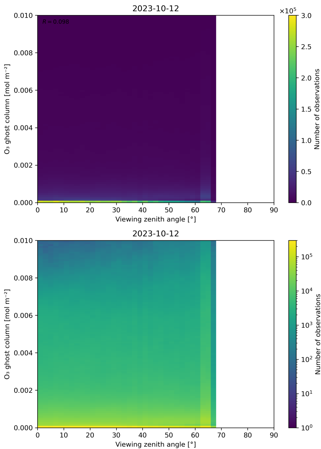
Figure 51: Scatter density plot of “Viewing zenith angle” against “O 3 ghost column” for 2023-10-12 to 2023-10-13.
