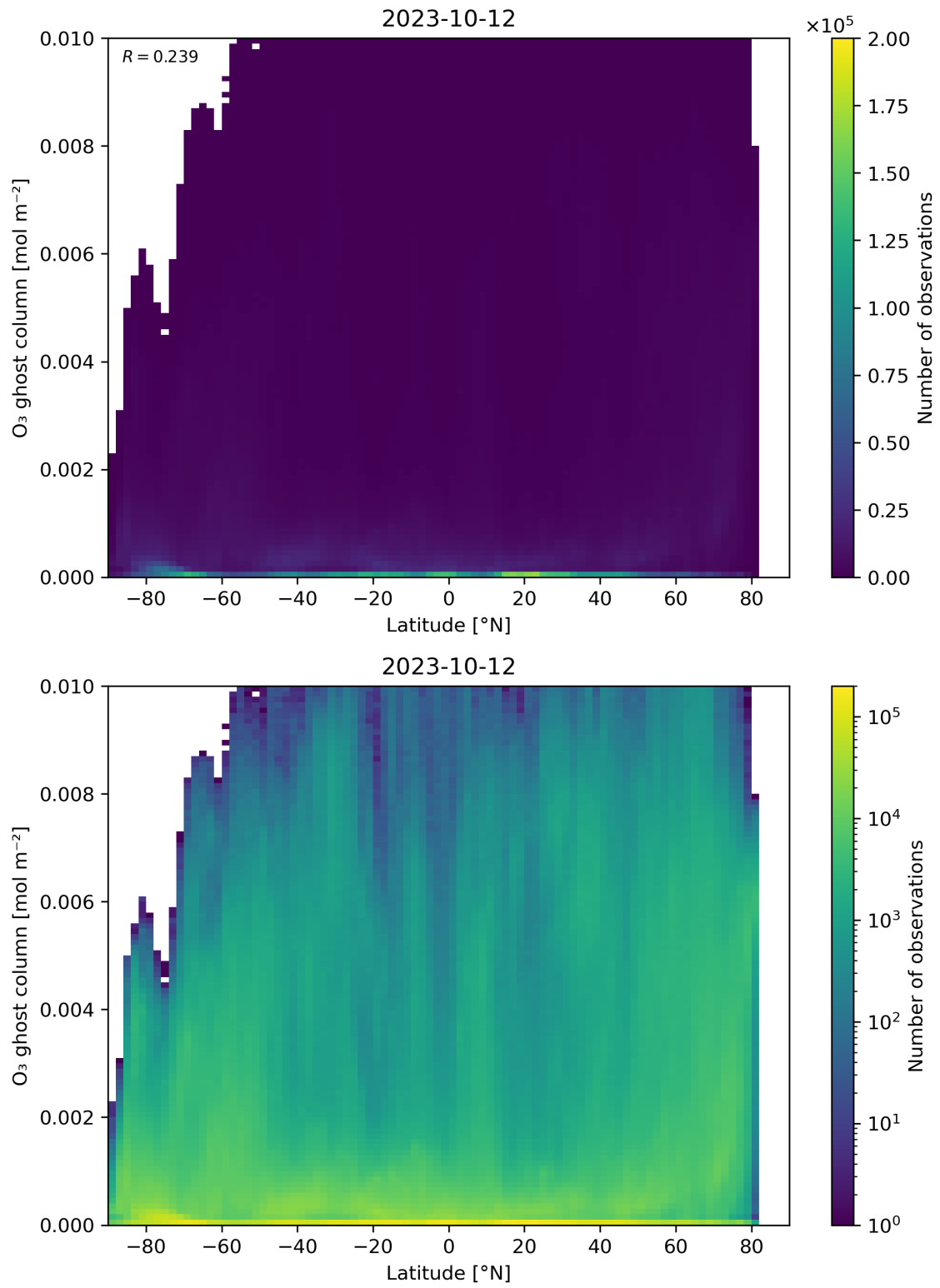
Figure 35: Scatter density plot of “Latitude” against “O 3 ghost column” for 2023-10-12 to 2023-10-13.
