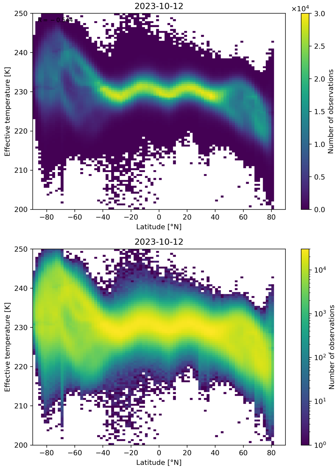
Figure 34: Scatter density plot of “Latitude” against “Effective temperature” for 2023-10-12 to 2023-10-13.
