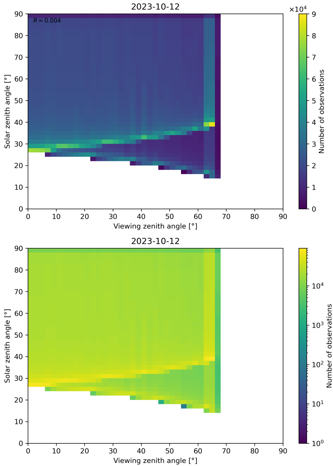
Figure 54: Scatter density plot of “Viewing zenith angle” against “Solar zenith angle” for 2023-10-12 to 2023-10-13.
