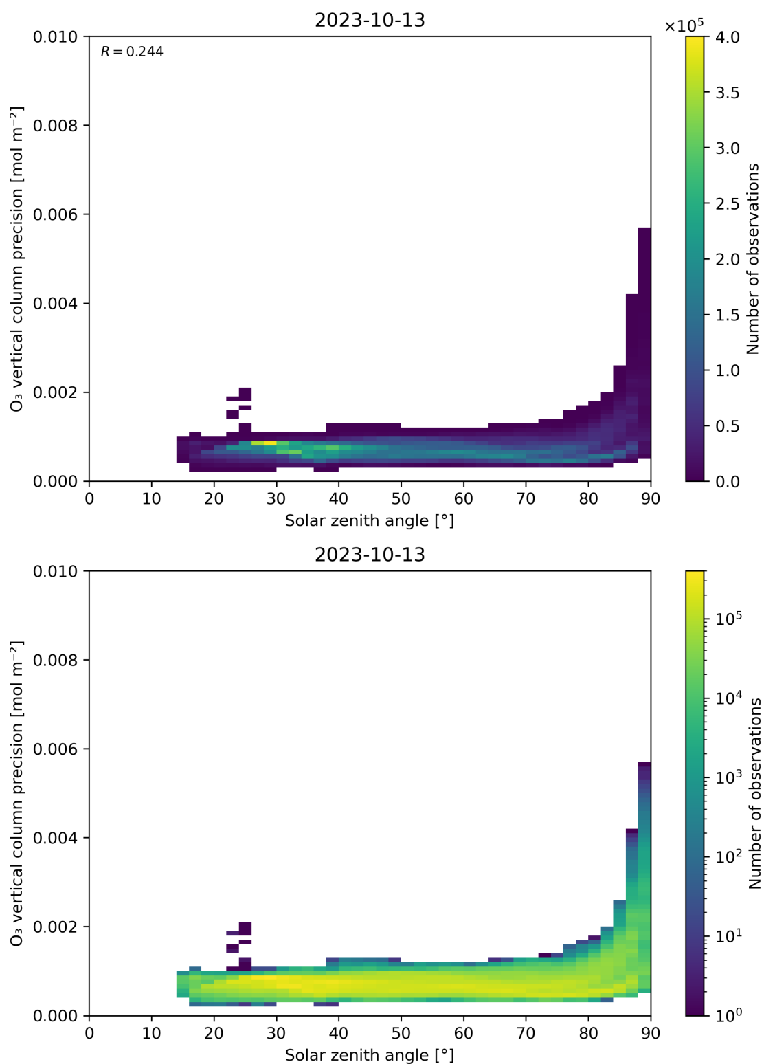
Figure 48: Scatter density plot of “Solar zenith angle” against “O 3 vertical column precision” for 2023-10-12 to 2023-10-14.
