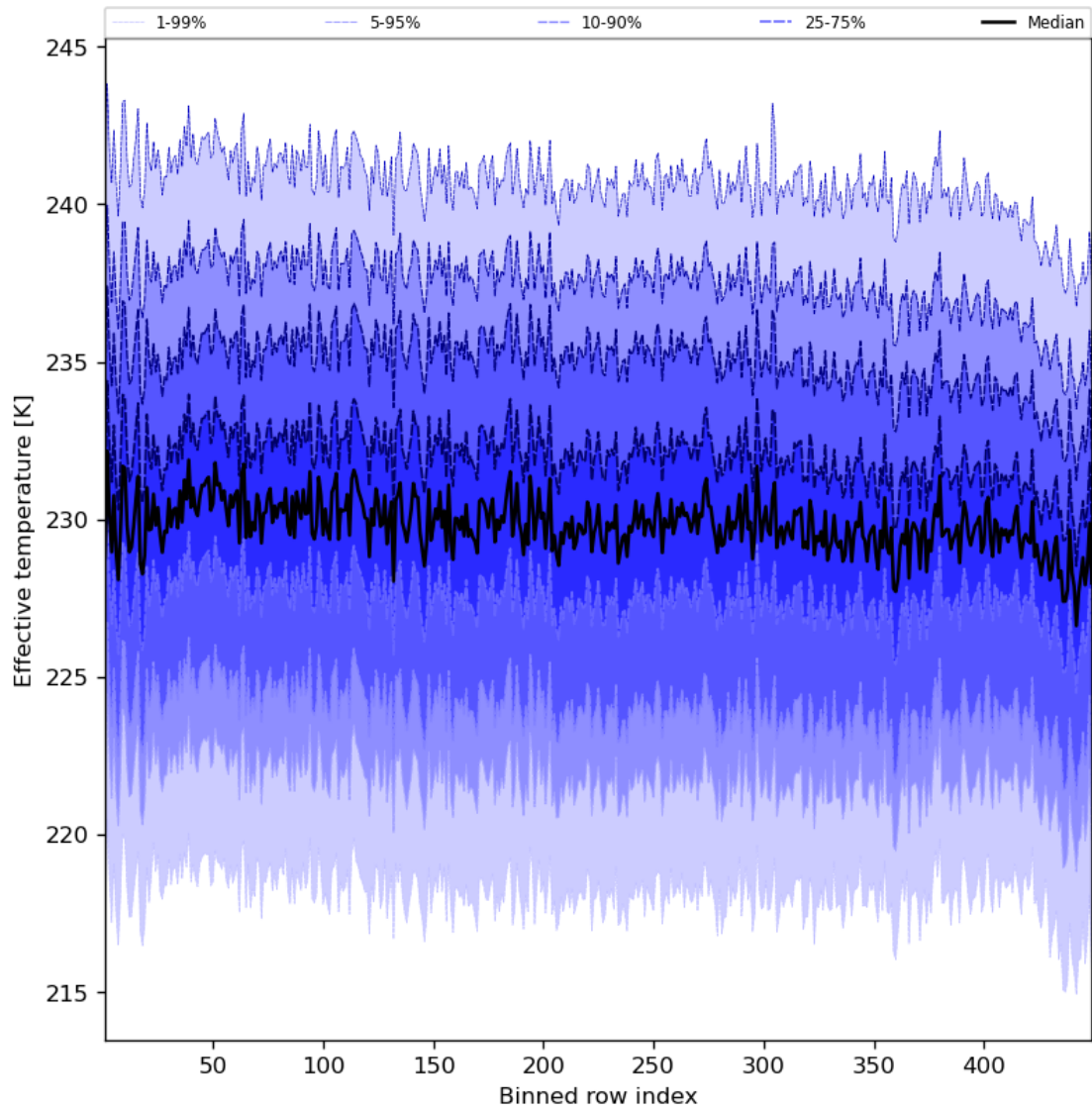
Figure 31: Along track statistics of “Effective temperature” for 2023-10-12 to 2023-10-14
