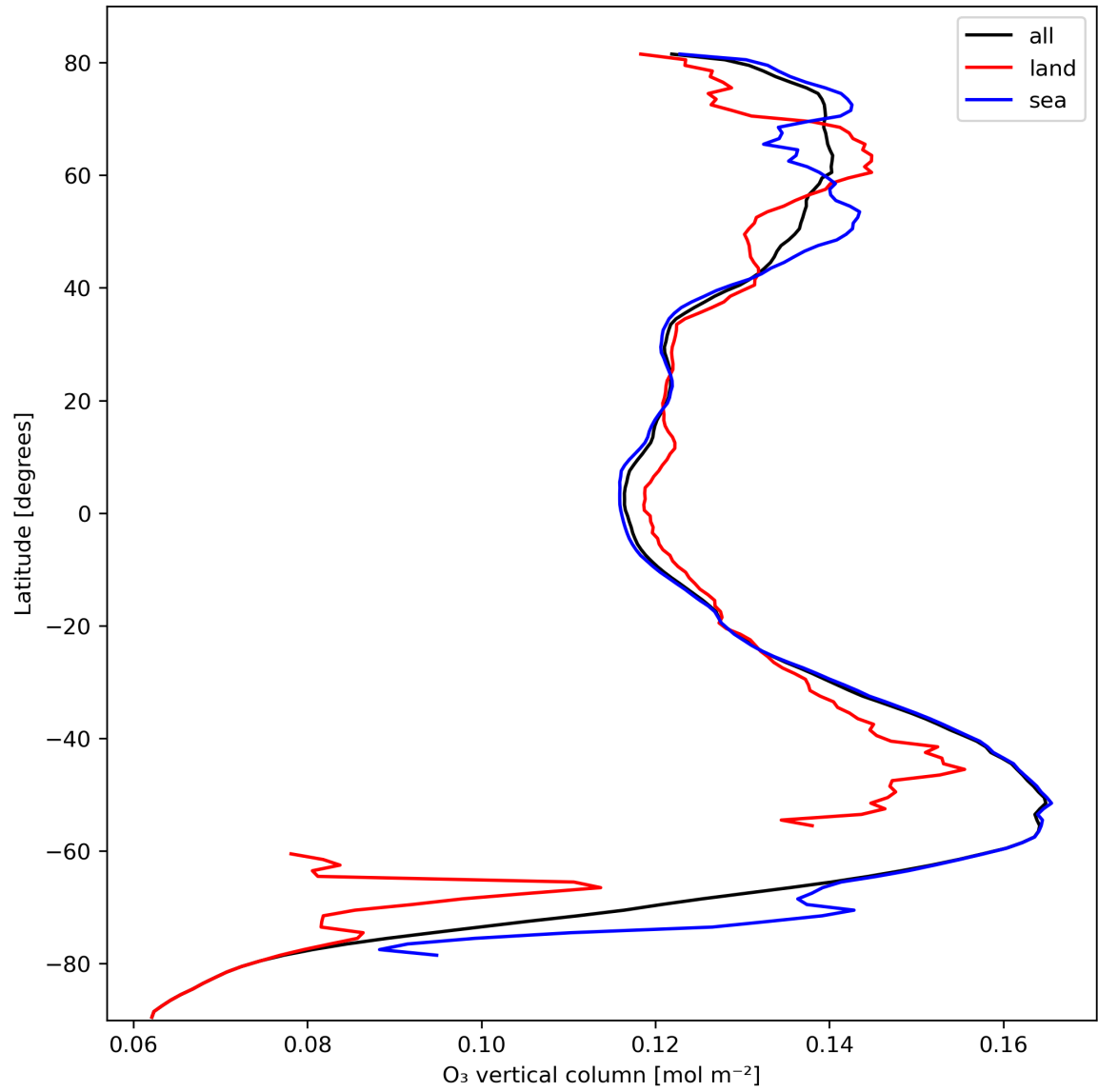
Figure 14: Zonal average of “O 3 vertical column” for 2023-10-12 to 2023-10-14.
