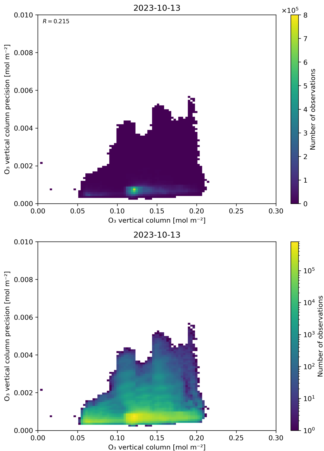
Figure 41: Scatter density plot of “O 3 vertical column” against “O 3 vertical column precision” for 2023-10-12 to 2023-10-14.
