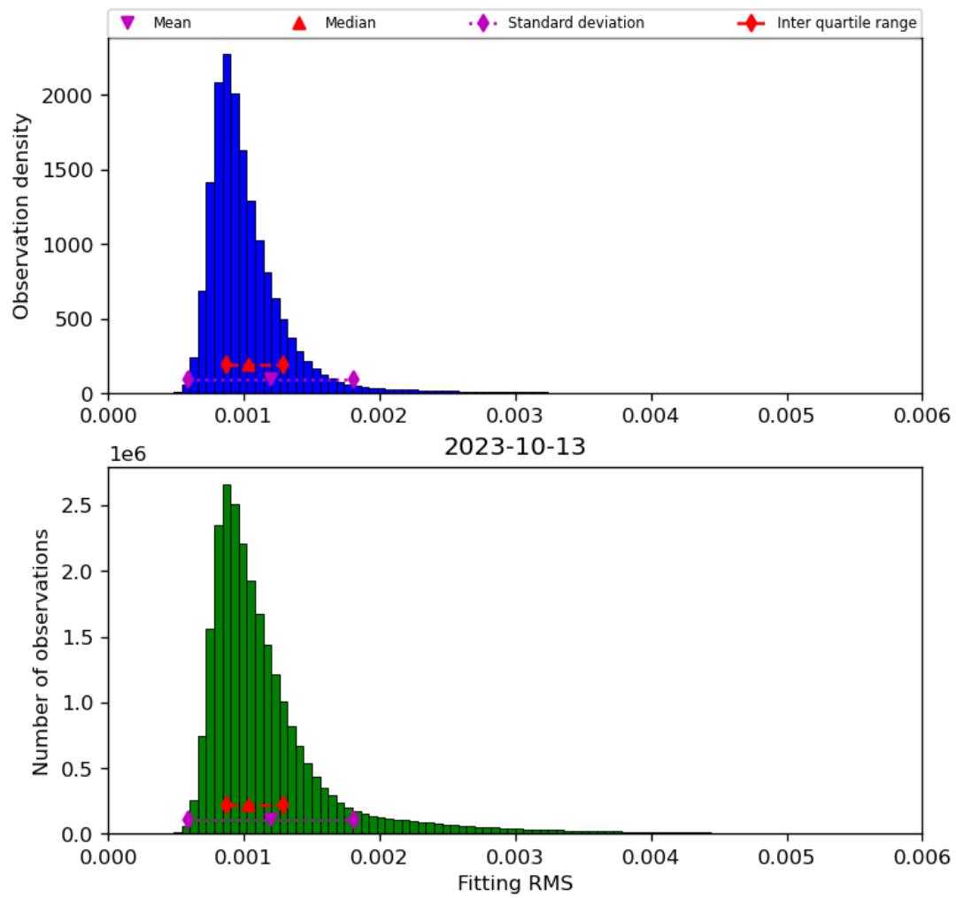
Figure 23: Histogram of “Fitting RMS” for 2023-10-12 to 2023-10-14
