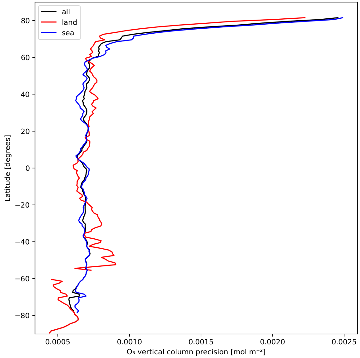
Figure 15: Zonal average of “O 3 vertical column precision” for 2023-10-12 to 2023-10-14.
