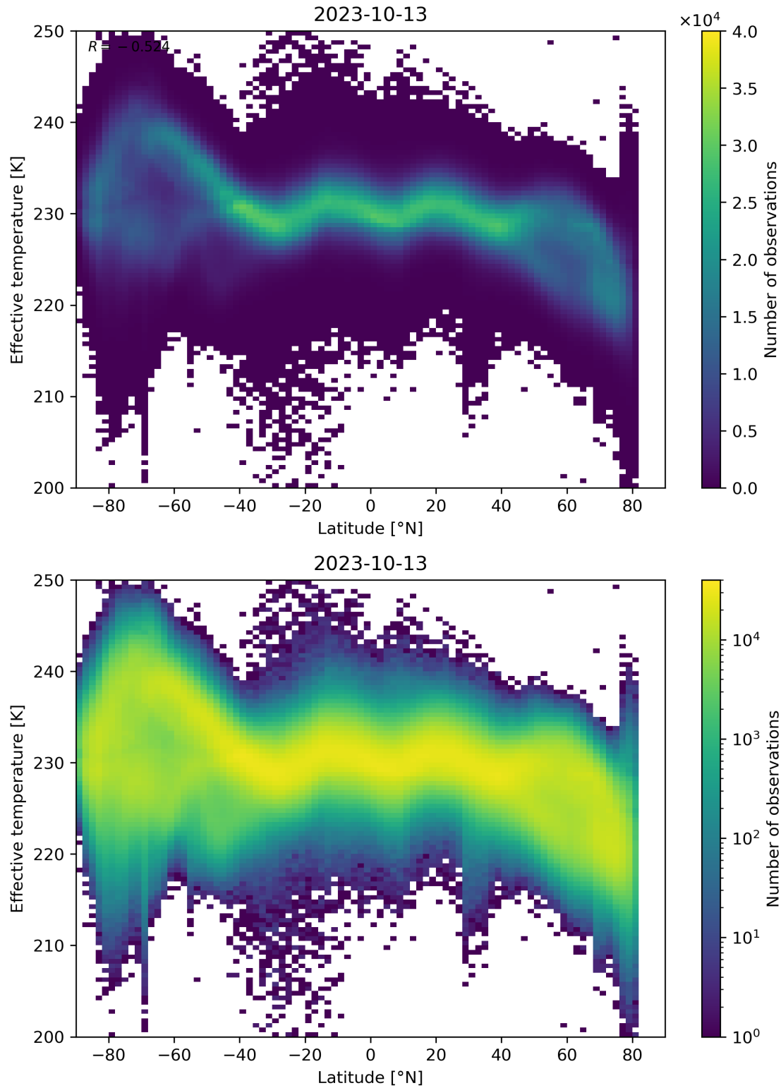
Figure 34: Scatter density plot of “Latitude” against “Effective temperature” for 2023-10-12 to 2023-10-14.
