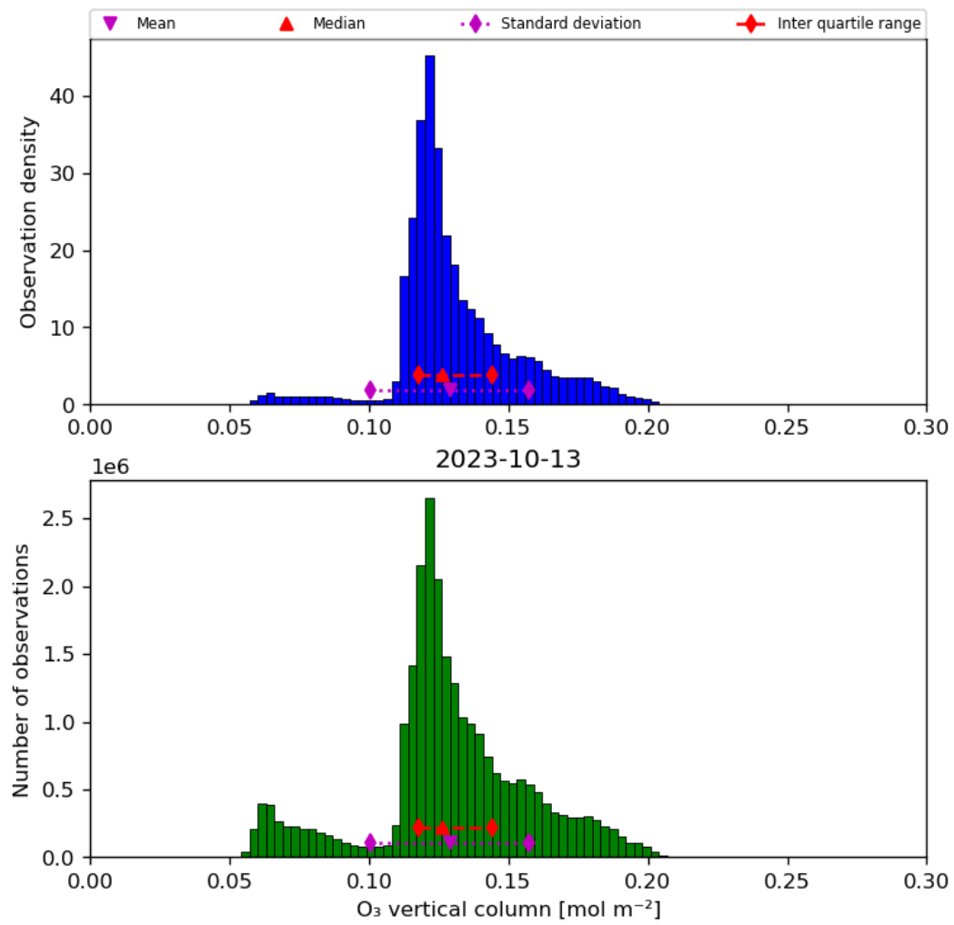
Figure 21: Histogram of “O 3 vertical column” for 2023-10-12 to 2023-10-14
