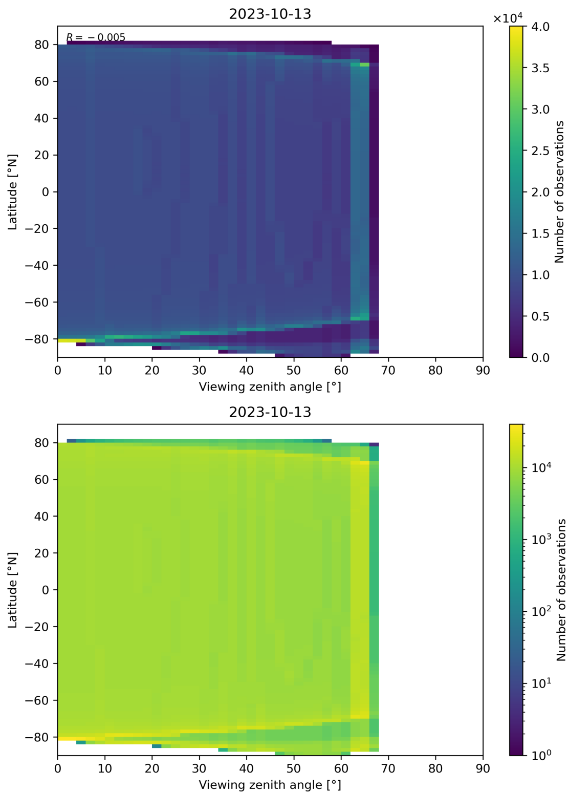
Figure 49: Scatter density plot of “Viewing zenith angle” against “Latitude” for 2023-10-12 to 2023-10-14.
