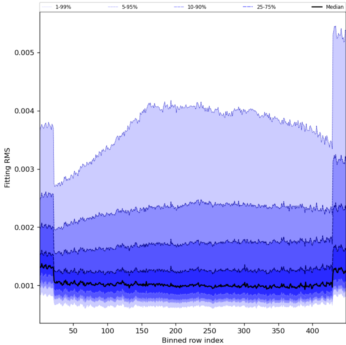
Figure 30: Along track statistics of “Fitting RMS” for 2023-10-12 to 2023-10-14
