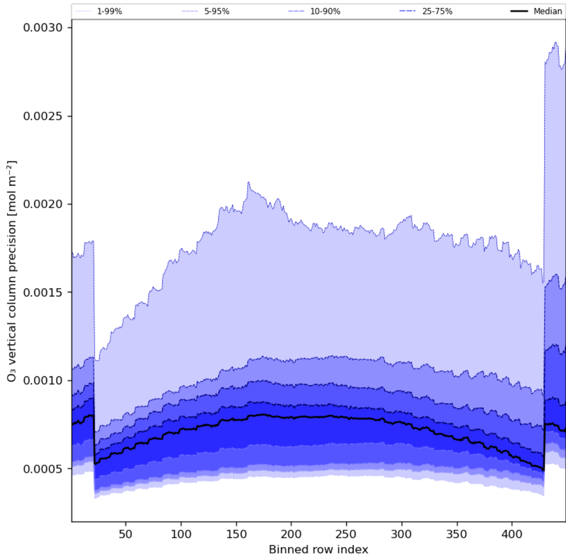
Figure 29: Along track statistics of “O 3 vertical column precision” for 2023-10-12 to 2023-10-14
