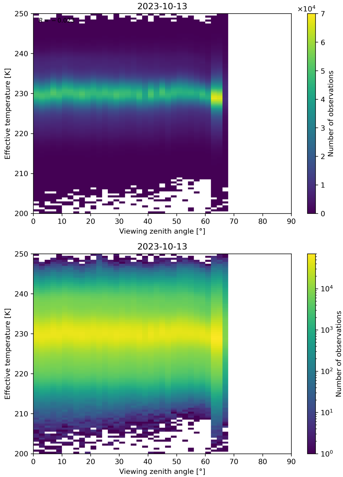
Figure 50: Scatter density plot of “Viewing zenith angle” against “Effective temperature” for 2023-10-12 to 2023-10-14.
