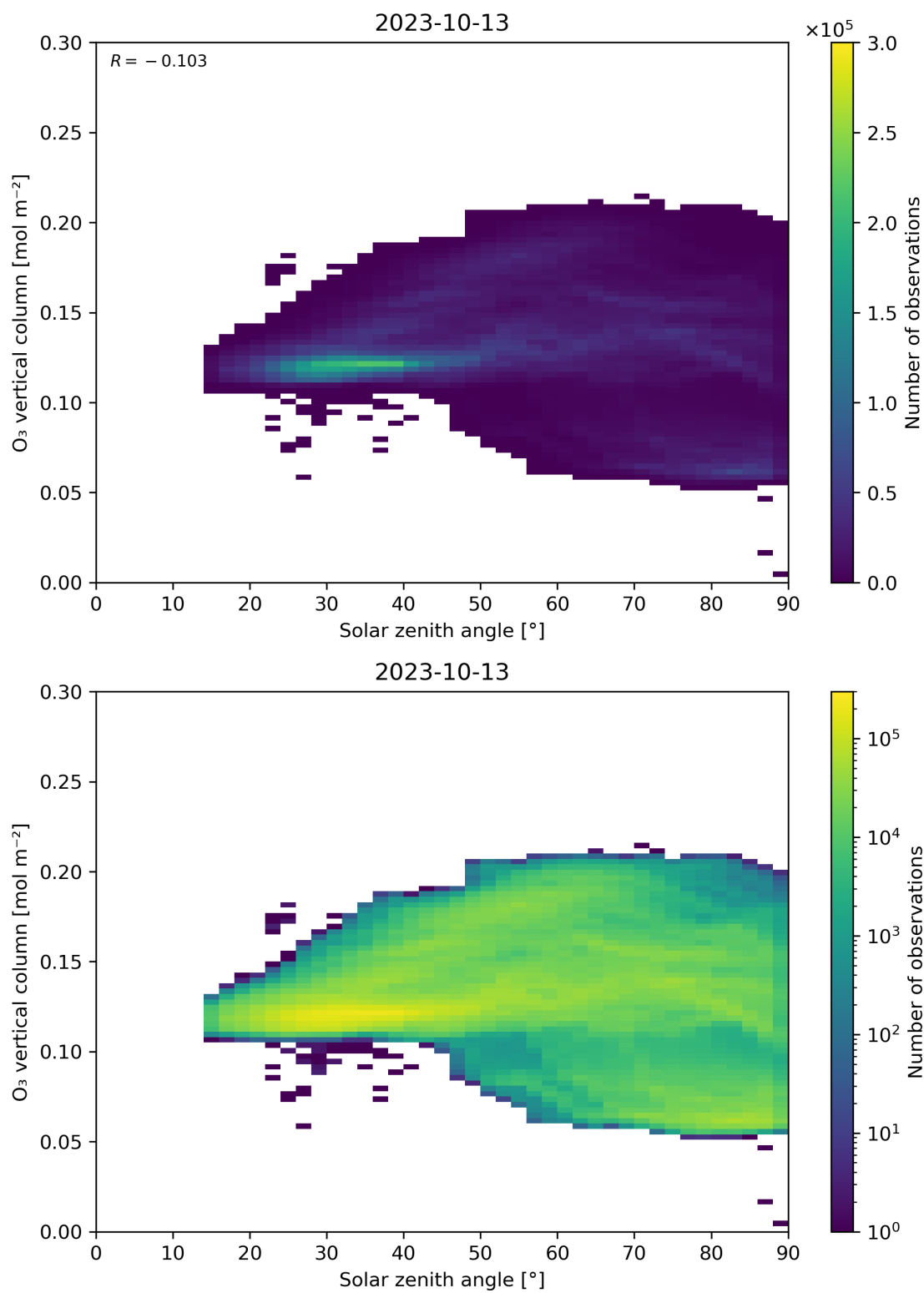
Figure 47: Scatter density plot of “Solar zenith angle” against “O 3 vertical column” for 2023-10-12 to 2023-10-14.
