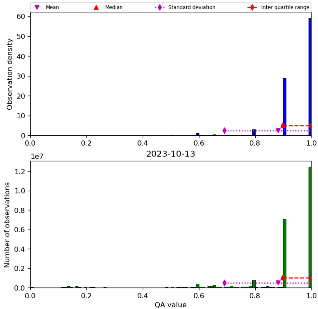
Figure 20: Histogram of “QA value” for 2023-10-12 to 2023-10-14
