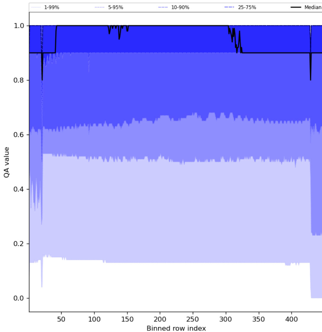
Figure 27: Along track statistics of “QA value” for 2023-10-12 to 2023-10-14
