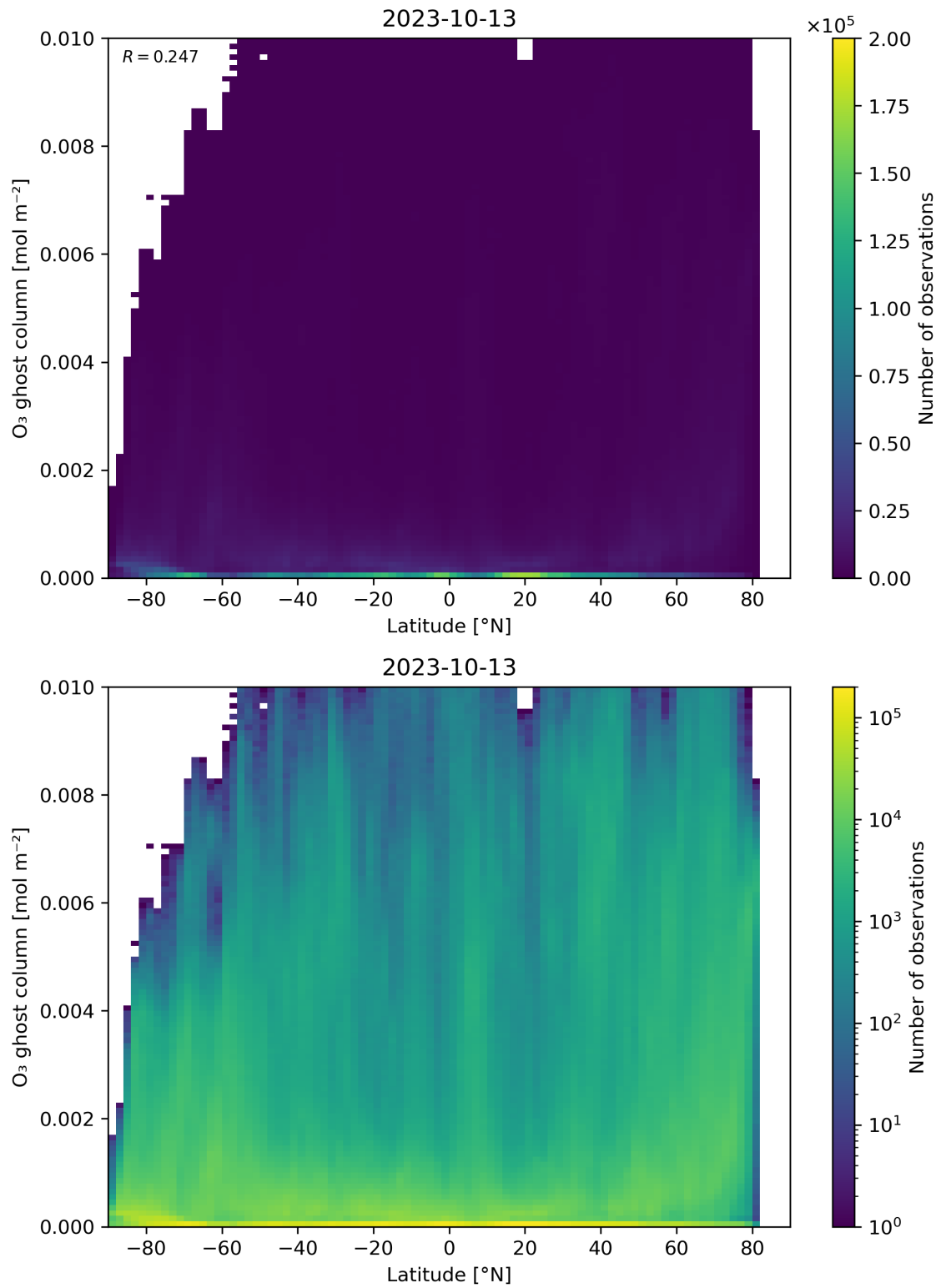
Figure 35: Scatter density plot of “Latitude” against “O 3 ghost column” for 2023-10-12 to 2023-10-14.
