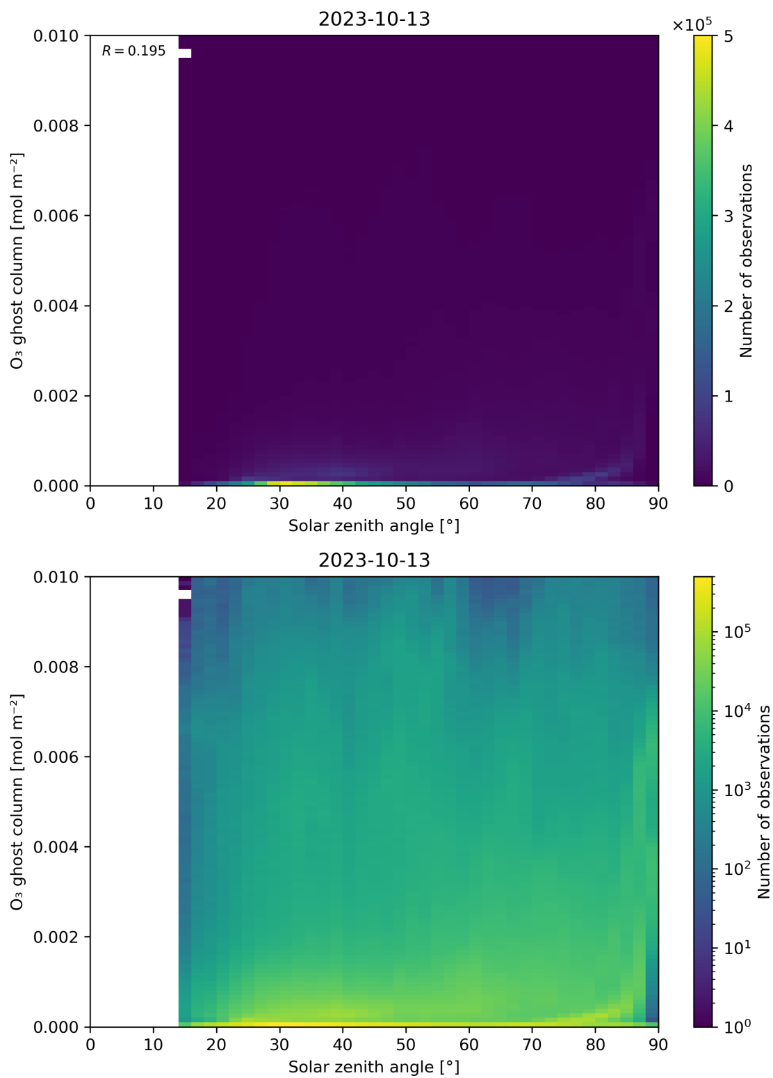
Figure 46: Scatter density plot of “Solar zenith angle” against “O 3 ghost column” for 2023-10-12 to 2023-10-14.
