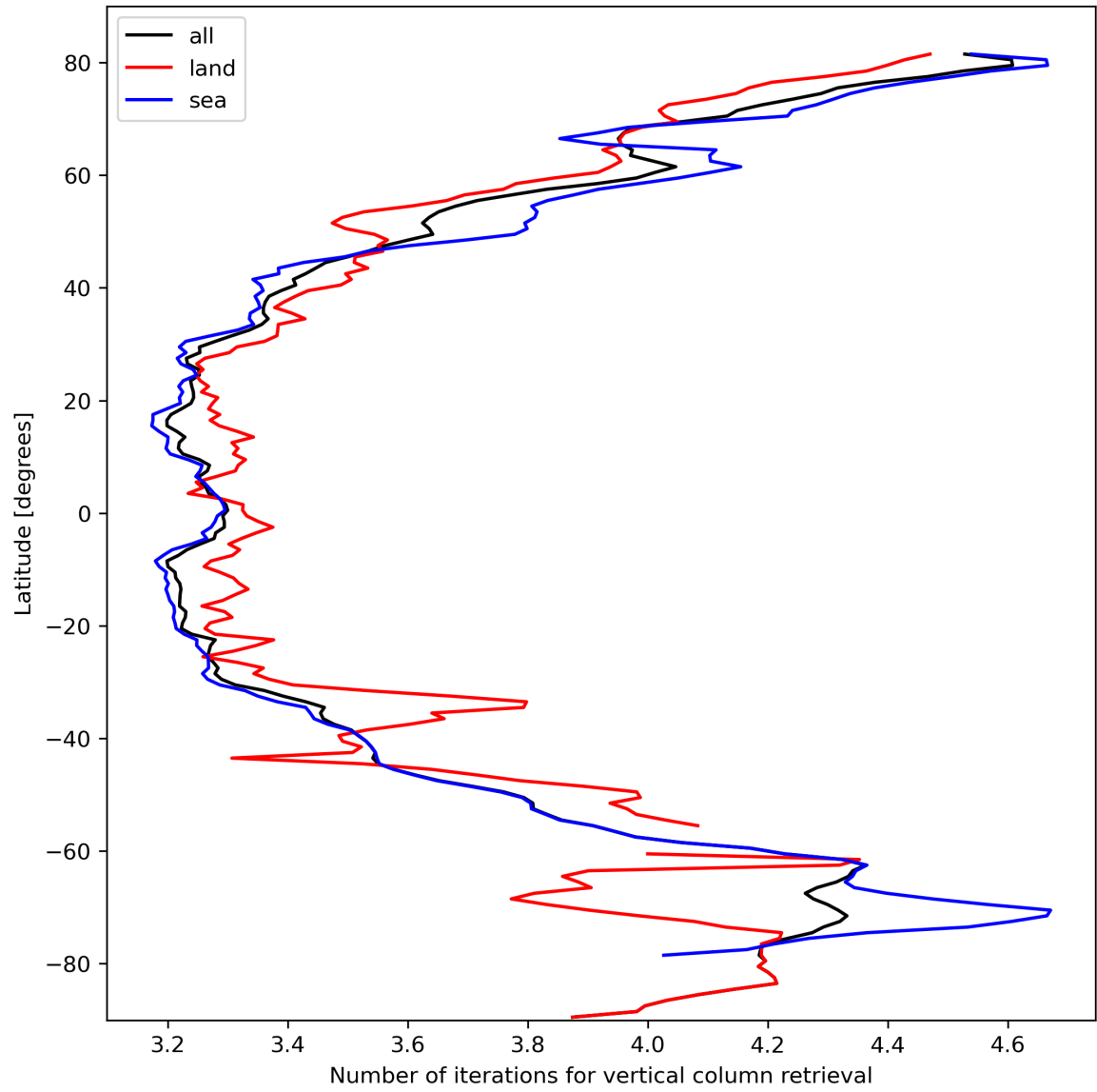
Figure 19: Zonal average of “Number of iterations for vertical column retrieval” for 2023-10-12 to 2023-10-14.
