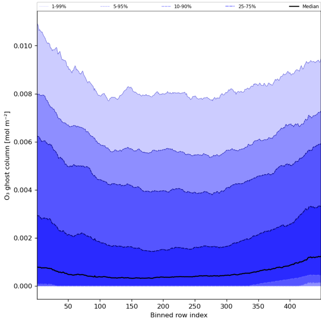
Figure 32: Along track statistics of “O 3 ghost column” for 2023-10-12 to 2023-10-14
