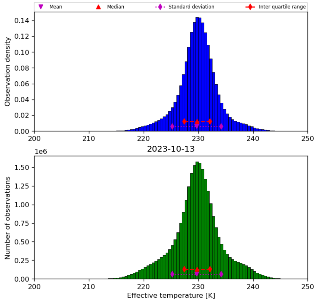
Figure 24: Histogram of “Effective temperature” for 2023-10-12 to 2023-10-14
