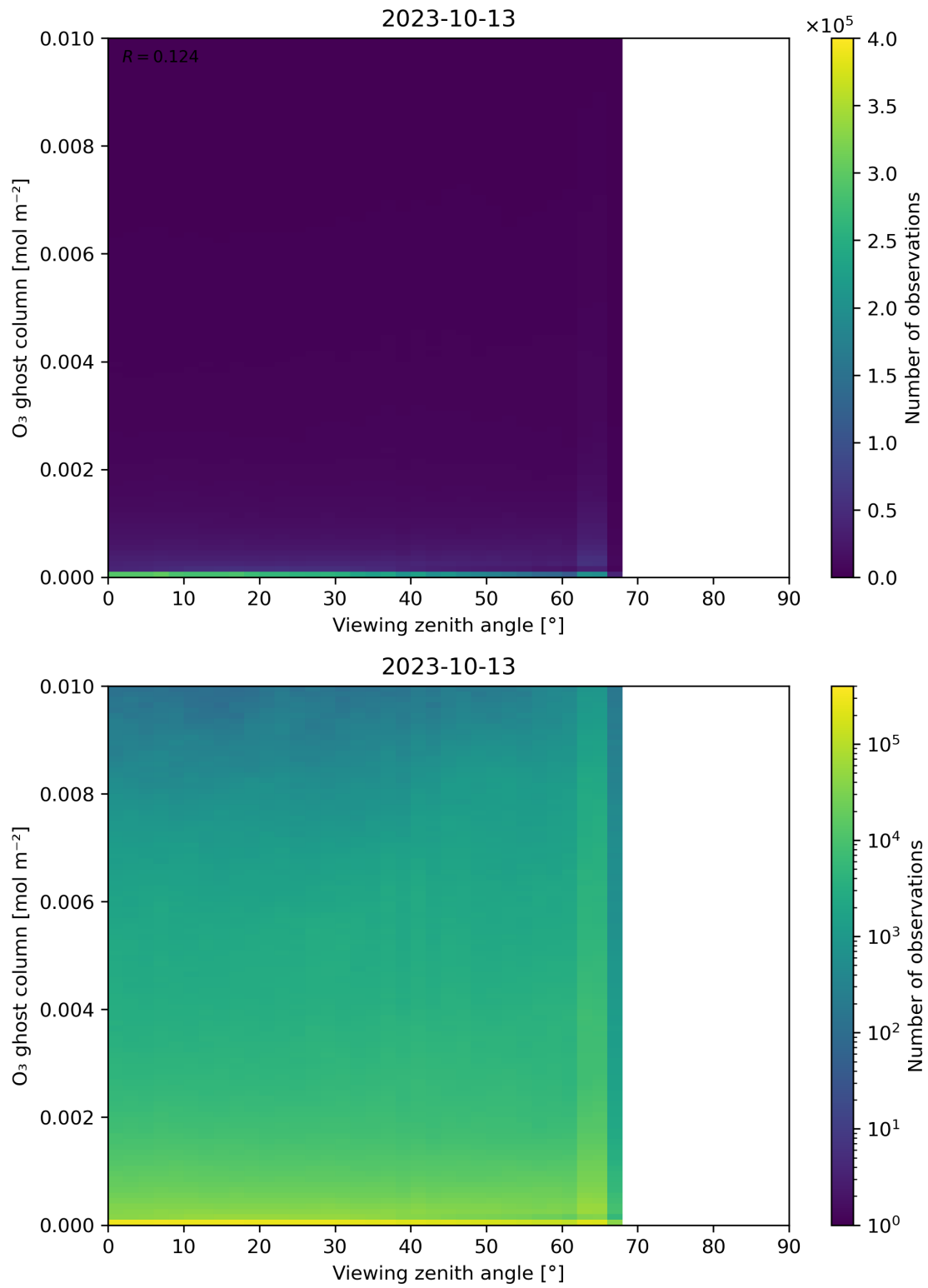
Figure 51: Scatter density plot of “Viewing zenith angle” against “O 3 ghost column” for 2023-10-12 to 2023-10-14.
