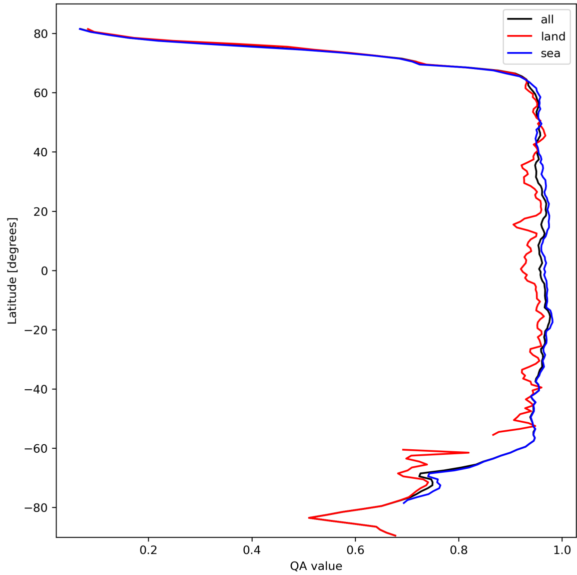
Figure 13: Zonal average of “QA value” for 2023-10-12 to 2023-10-14.
