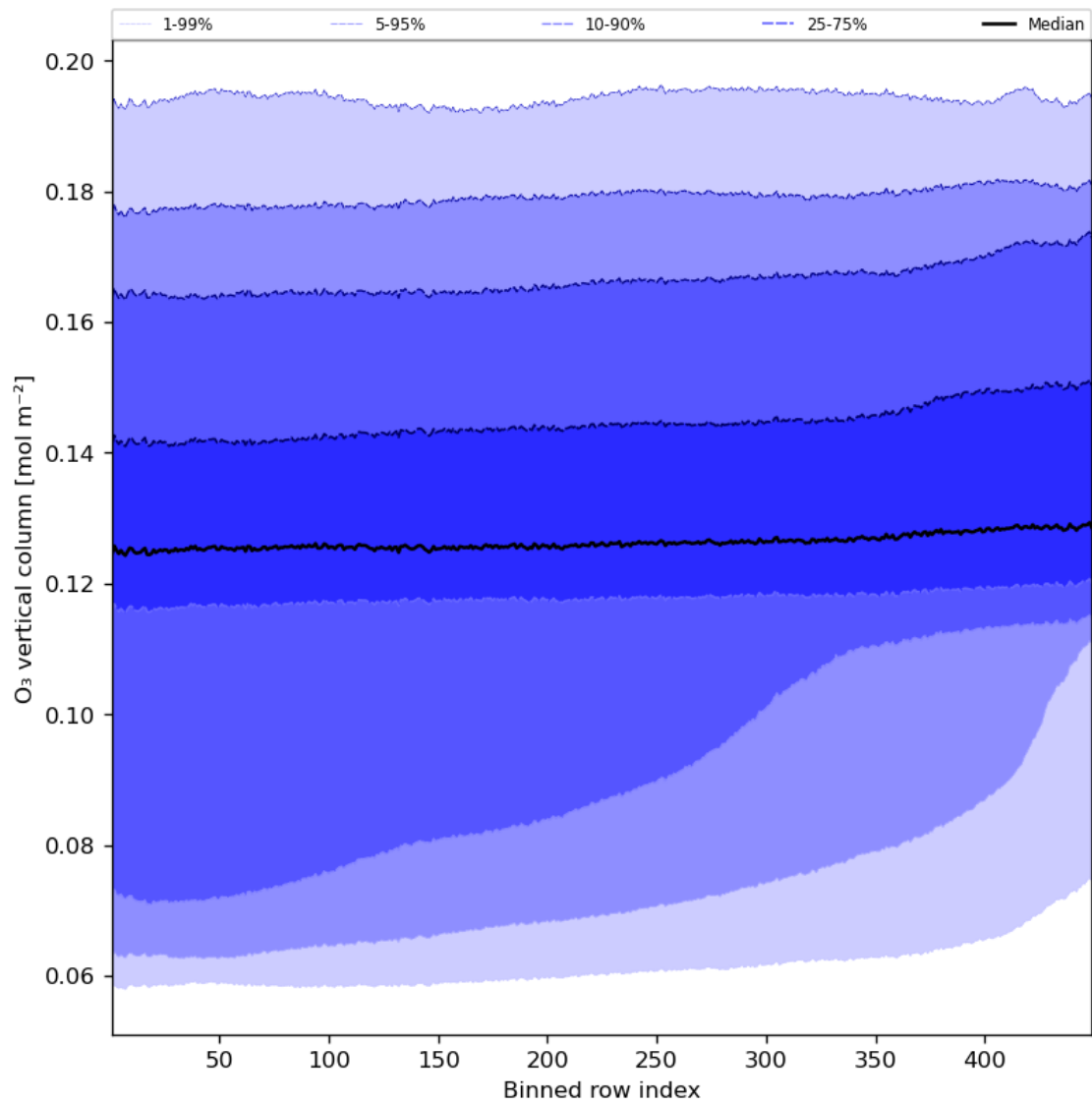
Figure 28: Along track statistics of “O 3 vertical column” for 2023-10-12 to 2023-10-14
