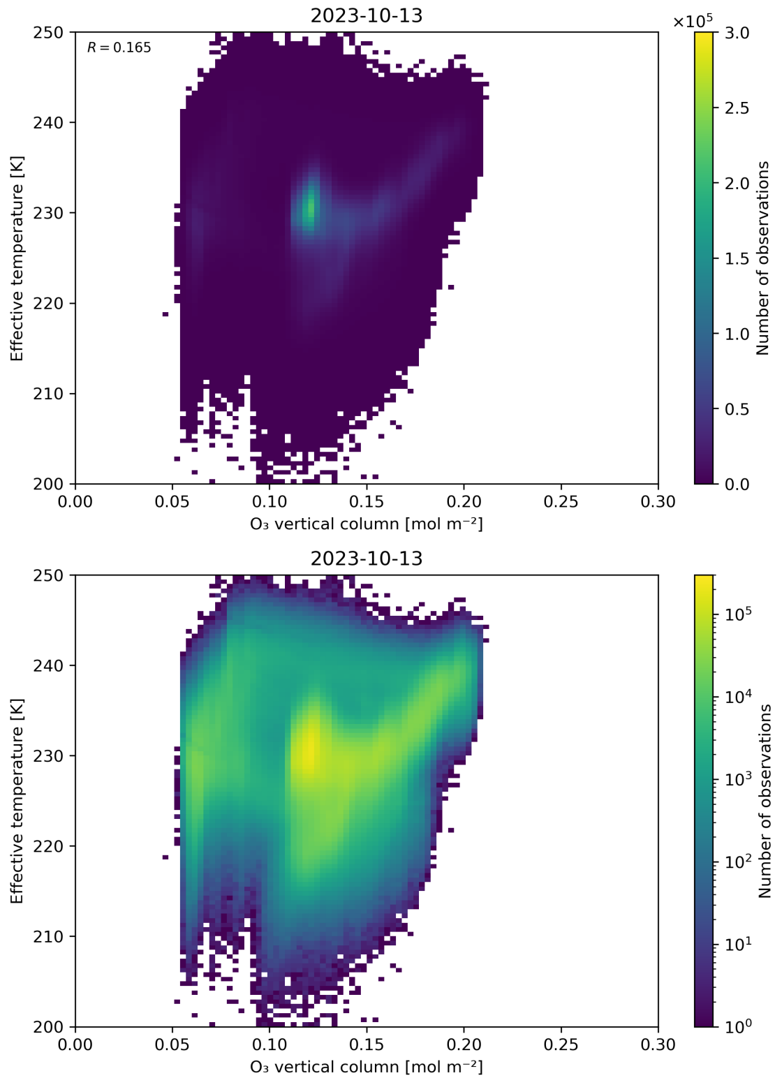
Figure 39: Scatter density plot of “O 3 vertical column” against “Effective temperature” for 2023-10-12 to 2023-10-14.
