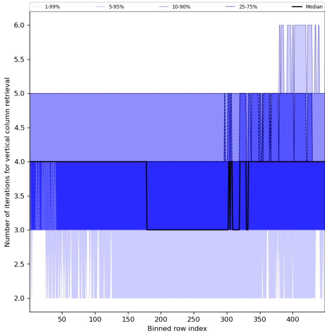
Figure 33: Along track statistics of “Number of iterations for vertical column retrieval” for 2023-10-12 to 2023-10-14
