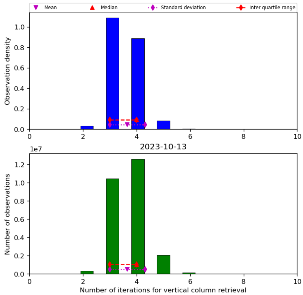
Figure 26: Histogram of “Number of iterations for vertical column retrieval” for 2023-10-12 to 2023-10-14
