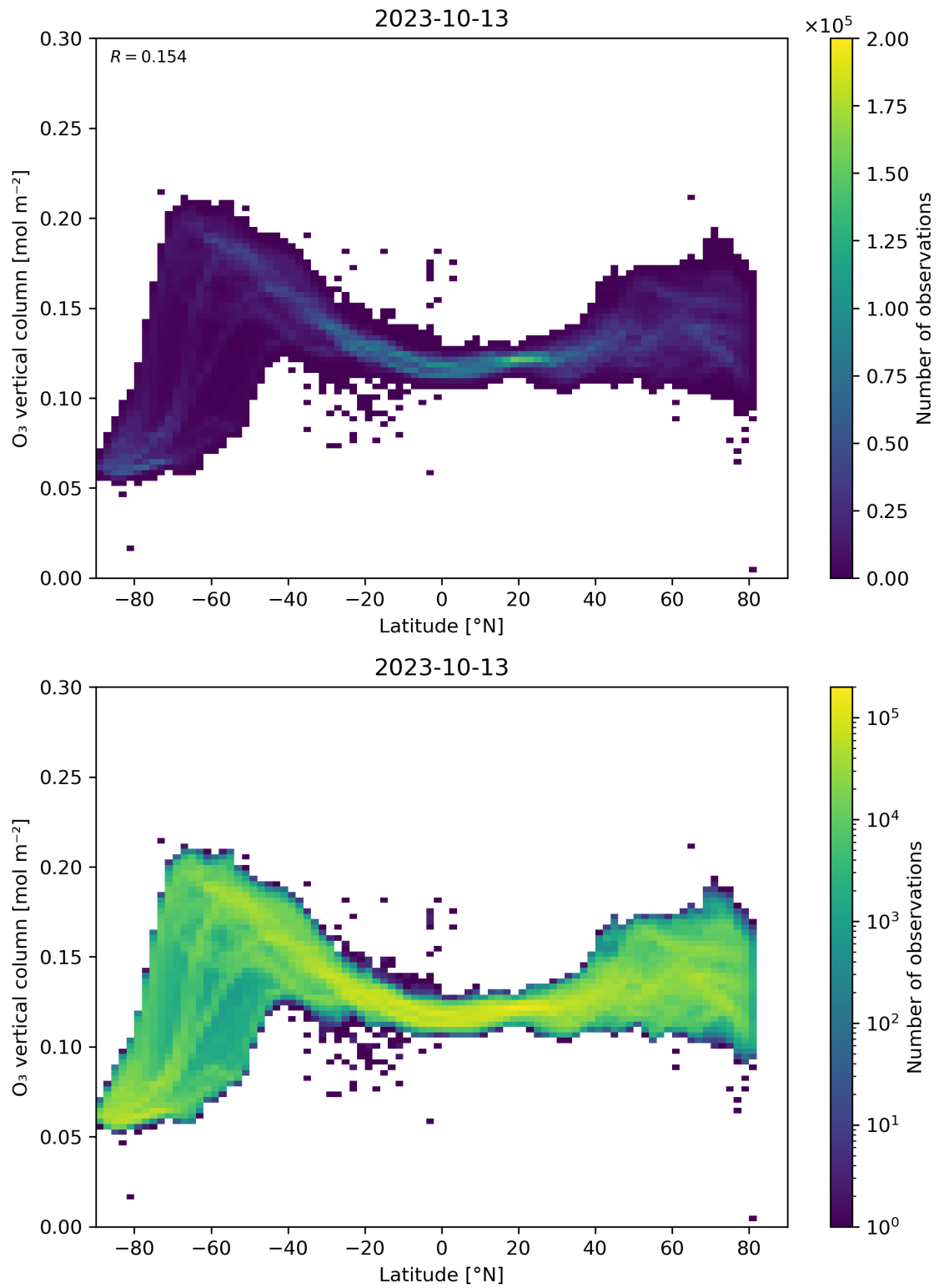
Figure 36: Scatter density plot of “Latitude” against “O 3 vertical column” for 2023-10-12 to 2023-10-14.
