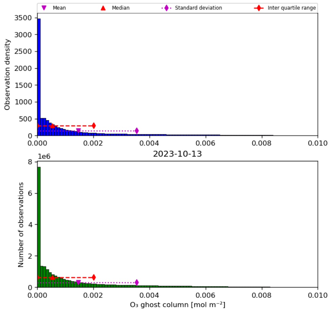
Figure 25: Histogram of “O 3 ghost column” for 2023-10-12 to 2023-10-14
