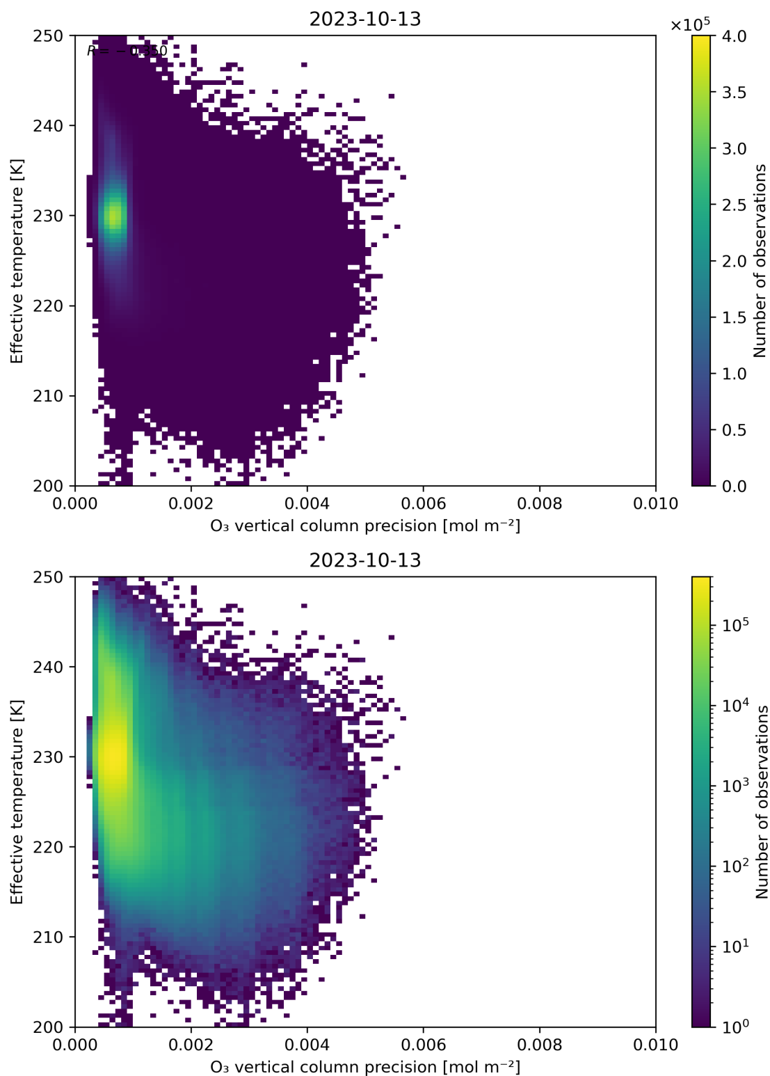
Figure 42: Scatter density plot of “ O_3 vertical column precision” against “Effective temperature” for 2023-10-12 to 2023-10-14.
