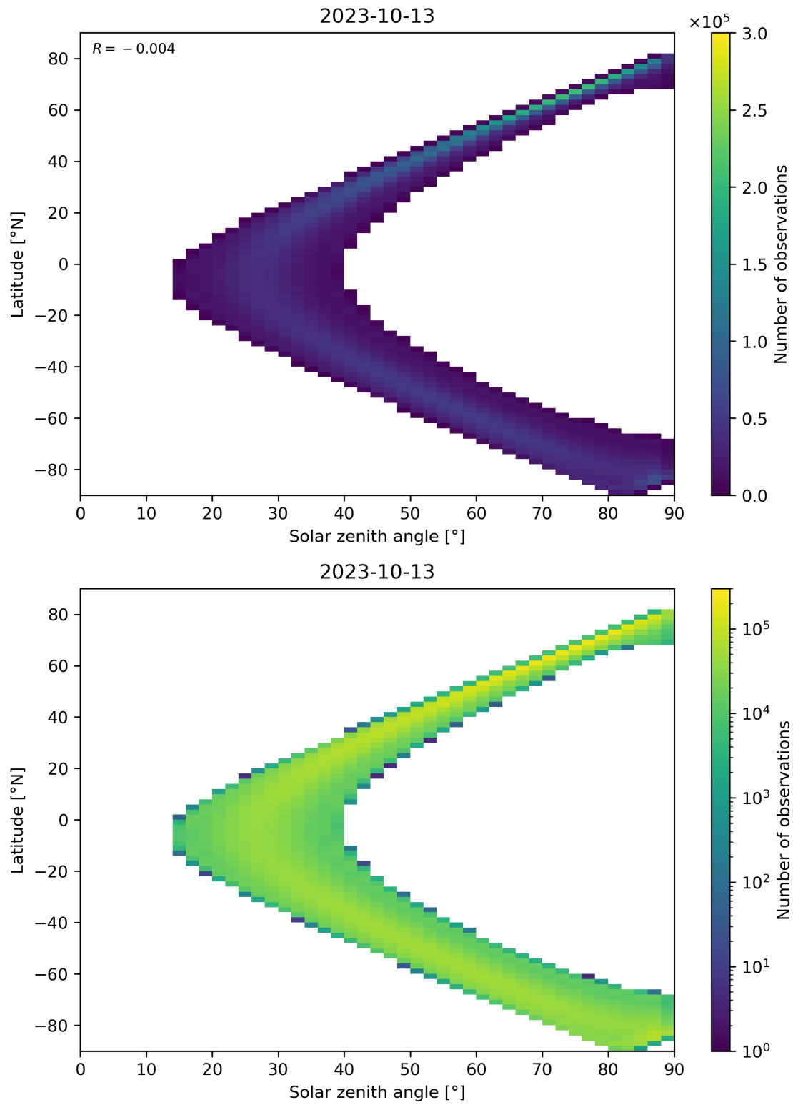
Figure 44: Scatter density plot of “Solar zenith angle” against “Latitude” for 2023-10-12 to 2023-10-14.
