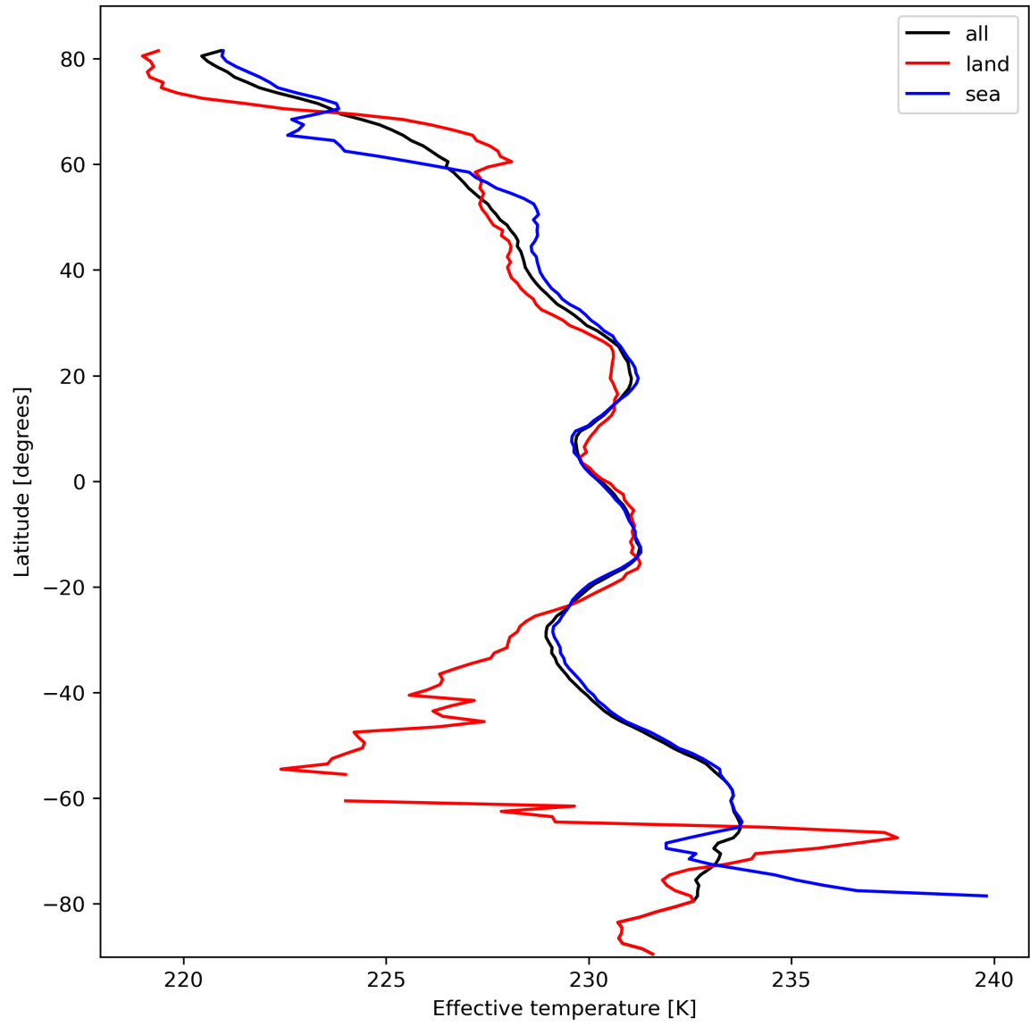
Figure 17: Zonal average of “Effective temperature” for 2023-10-12 to 2023-10-14.
