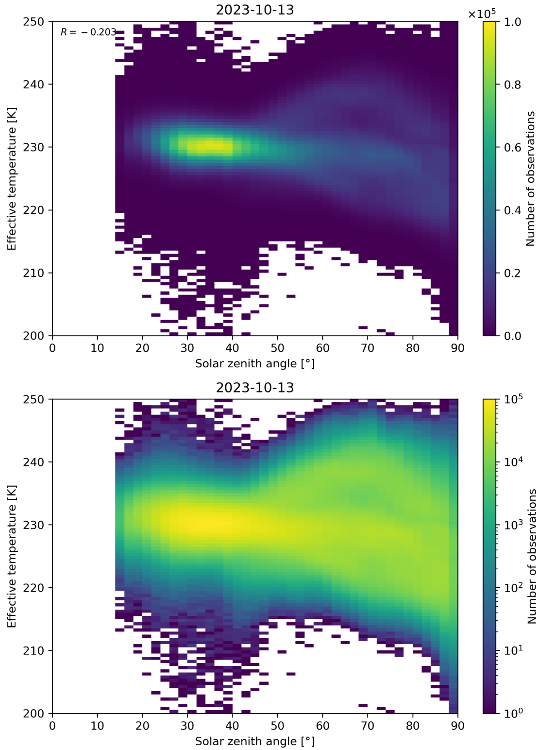
Figure 45: Scatter density plot of “Solar zenith angle” against “Effective temperature” for 2023-10-12 to 2023-10-14.
