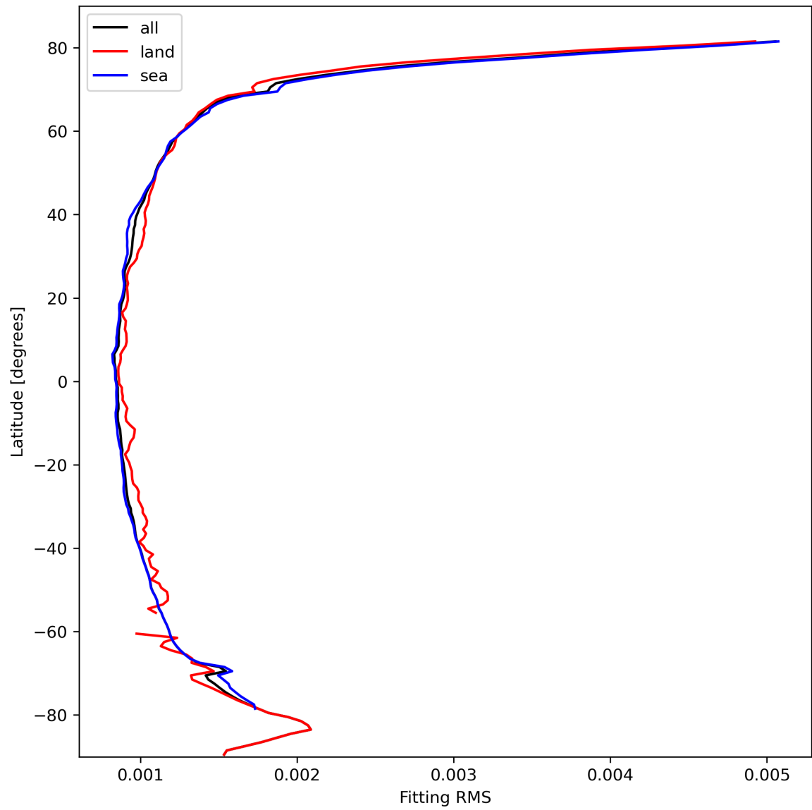
Figure 16: Zonal average of “Fitting RMS” for 2023-10-12 to 2023-10-14.
