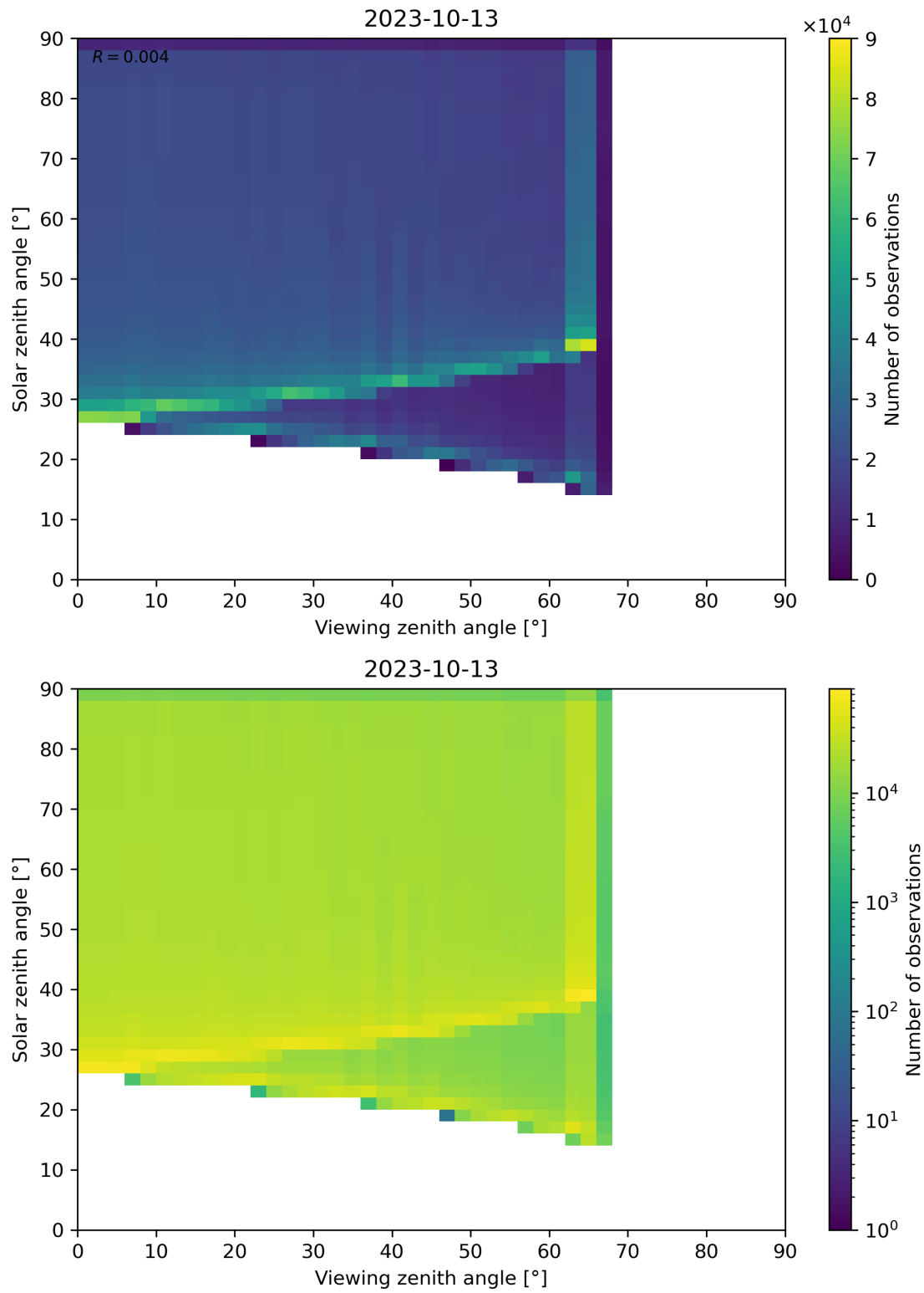
Figure 54: Scatter density plot of “Viewing zenith angle” against “Solar zenith angle” for 2023-10-12 to 2023-10-14.
