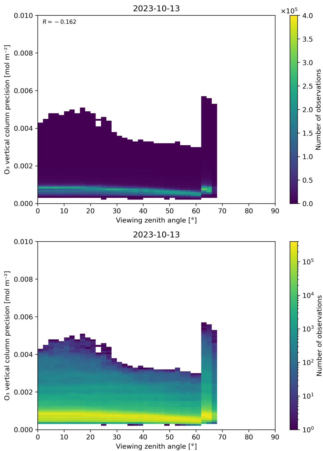
Figure 53: Scatter density plot of “Viewing zenith angle” against “O 3 vertical column precision” for 2023-10-12 to 2023-10-14.
