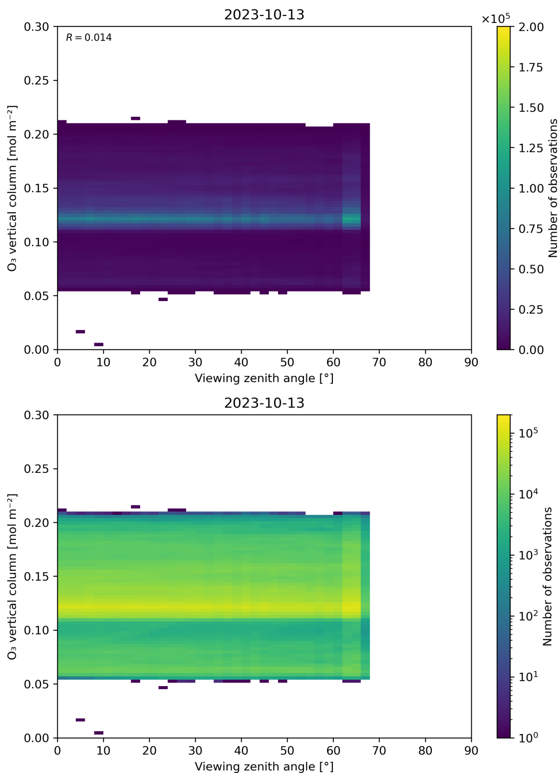
Figure 52: Scatter density plot of “Viewing zenith angle” against “O 3 vertical column” for 2023-10-12 to 2023-10-14.
