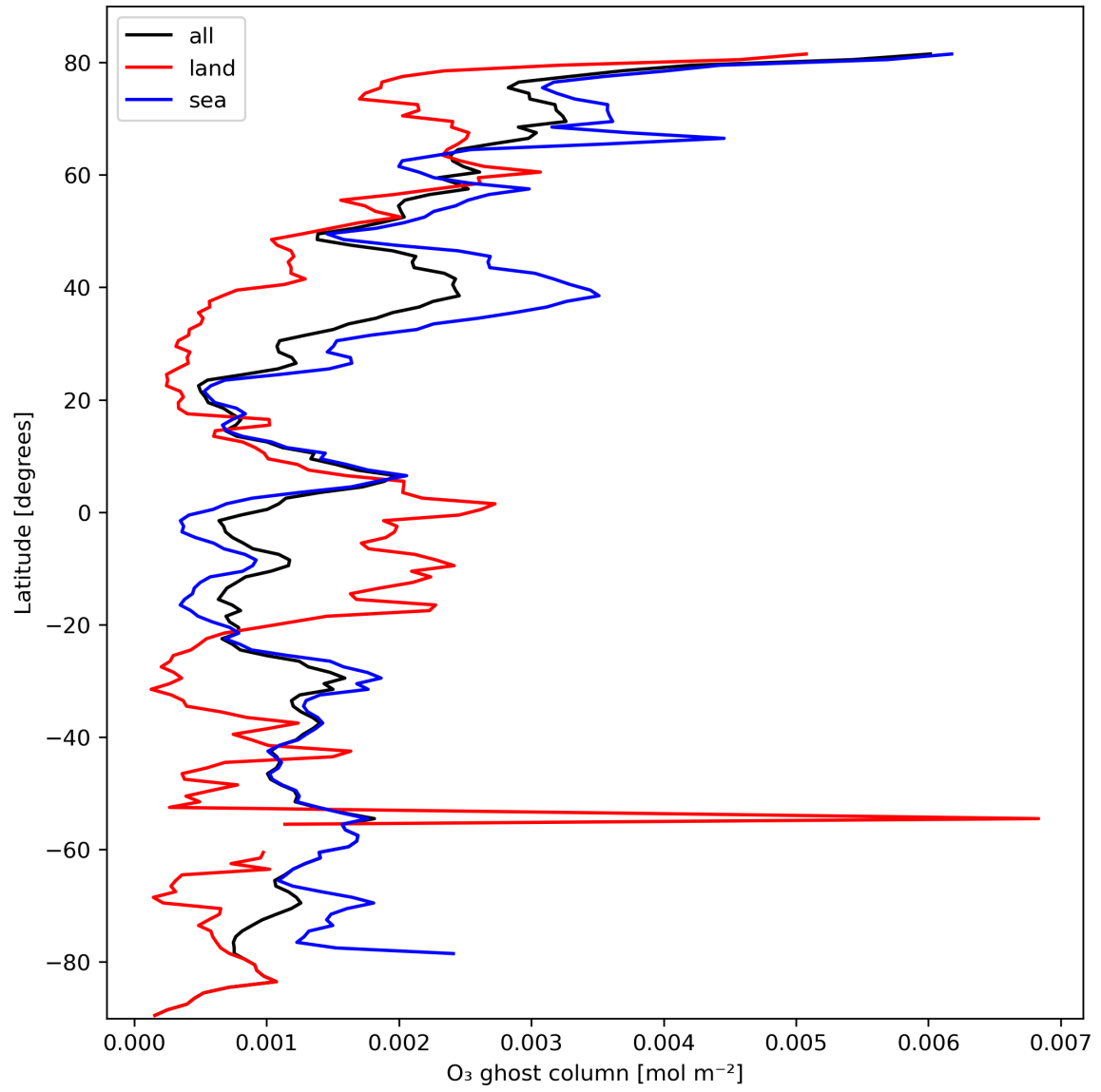
Figure 18: Zonal average of "O 3 ghost column" for 2023-10-12 to 2023-10-14.
