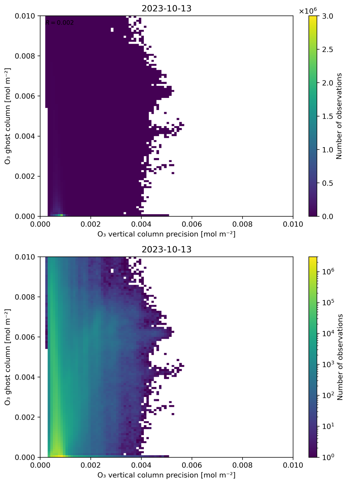
Figure 43: Scatter density plot of “O 3 vertical column precision” against “O 3 ghost column” for 2023-10-12 to 2023-10-14.
