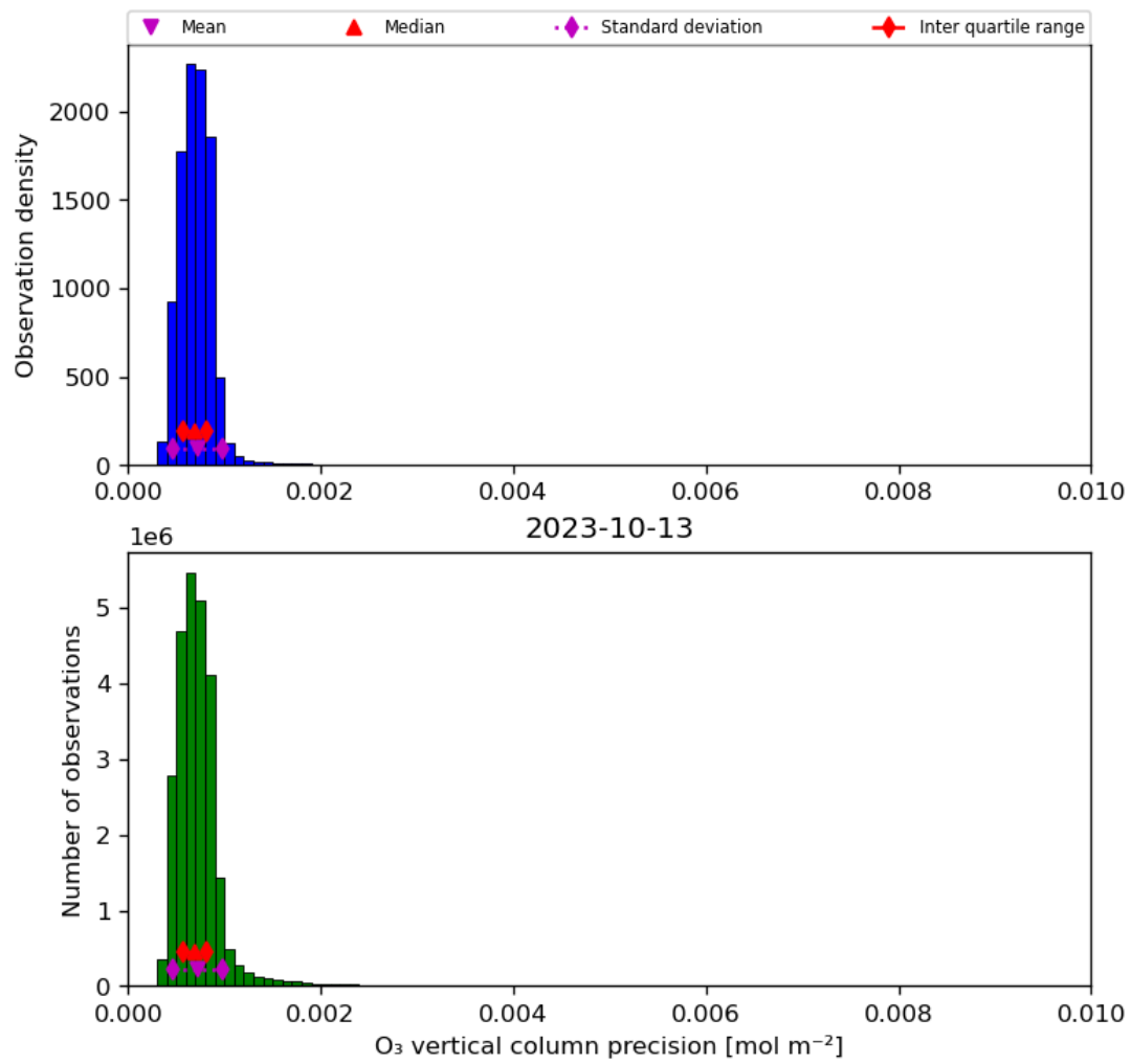
Figure 22: Histogram of “O 3 vertical column precision” for 2023-10-12 to 2023-10-14
