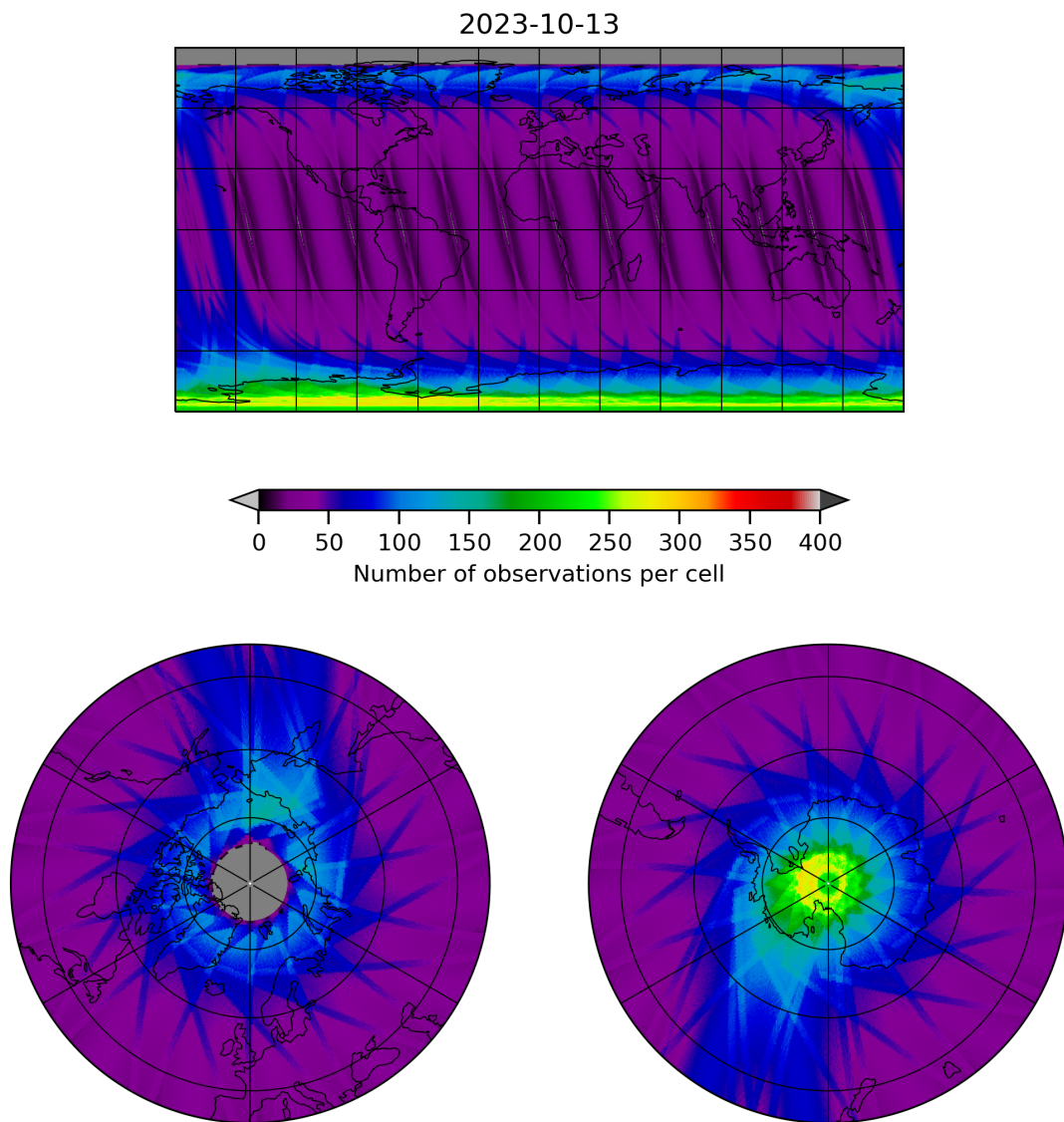
Figure 12: Map of the number of observations for 2023-10-12 to 2023-10-14
