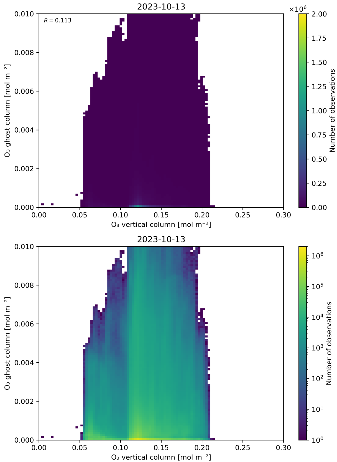
Figure 40: Scatter density plot of “O 3 vertical column” against “O 3 ghost column” for 2023-10-12 to 2023-10-14.
