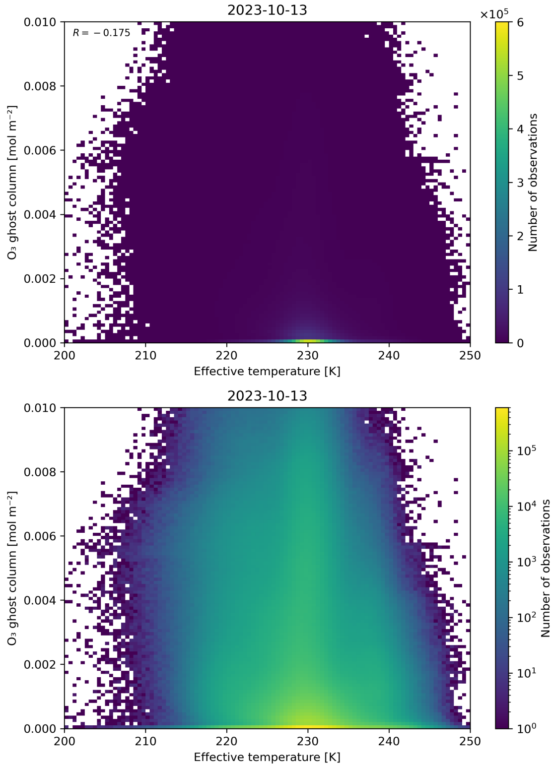
Figure 38: Scatter density plot of “Effective temperature” against “O 3 ghost column” for 2023-10-12 to 2023-10-14.
