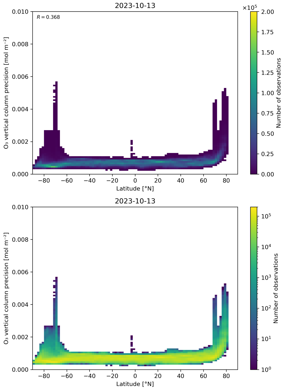
Figure 37: Scatter density plot of “Latitude” against “O 3 vertical column precision” for 2023-10-12 to 2023-10-14.
