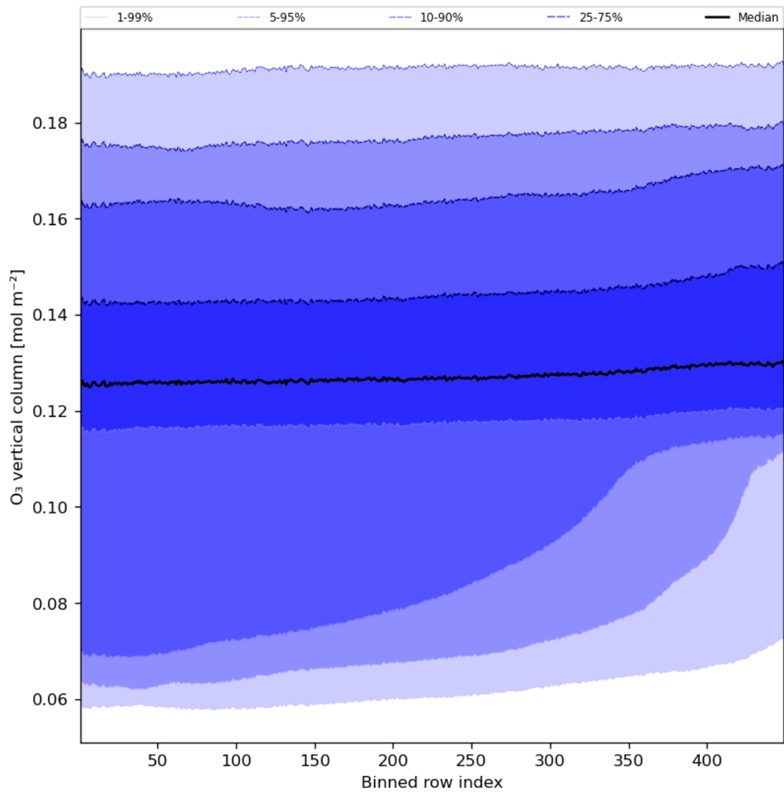
Figure 28: Along track statistics of “O 3 vertical column” for 2023-10-13 to 2023-10-15
