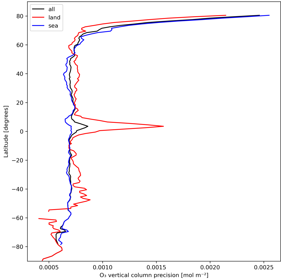
Figure 15: Zonal average of “O 3 vertical column precision” for 2023-10-13 to 2023-10-15.
