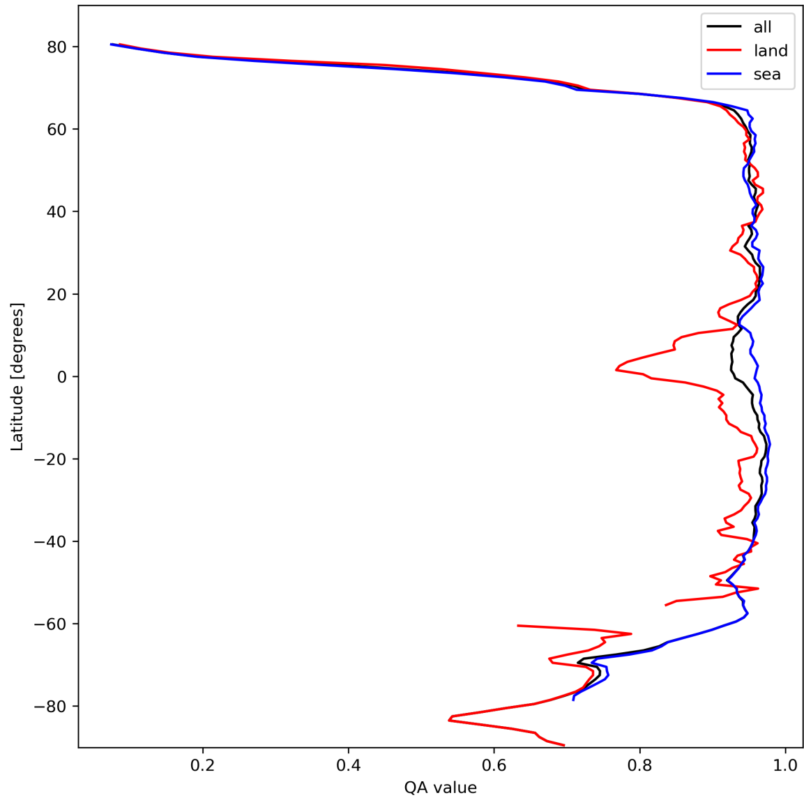
Figure 13: Zonal average of “QA value” for 2023-10-13 to 2023-10-15.
