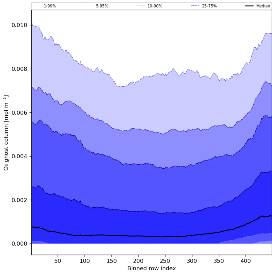
Figure 32: Along track statistics of “O 3 ghost column” for 2023-10-13 to 2023-10-15
