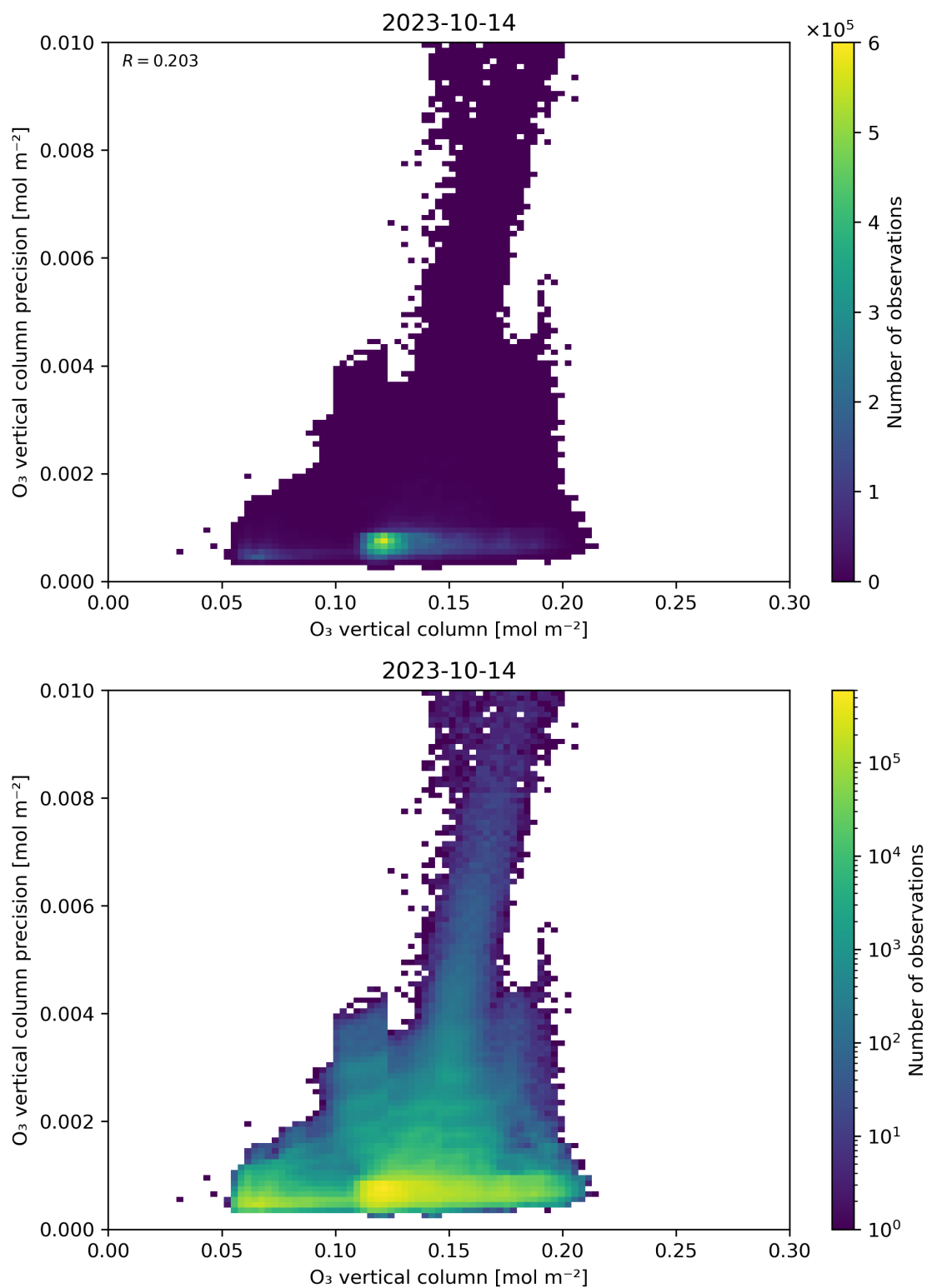
Figure 41: Scatter density plot of “O 3 vertical column” against “O 3 vertical column precision” for 2023-10-13 to 2023-10-15.
