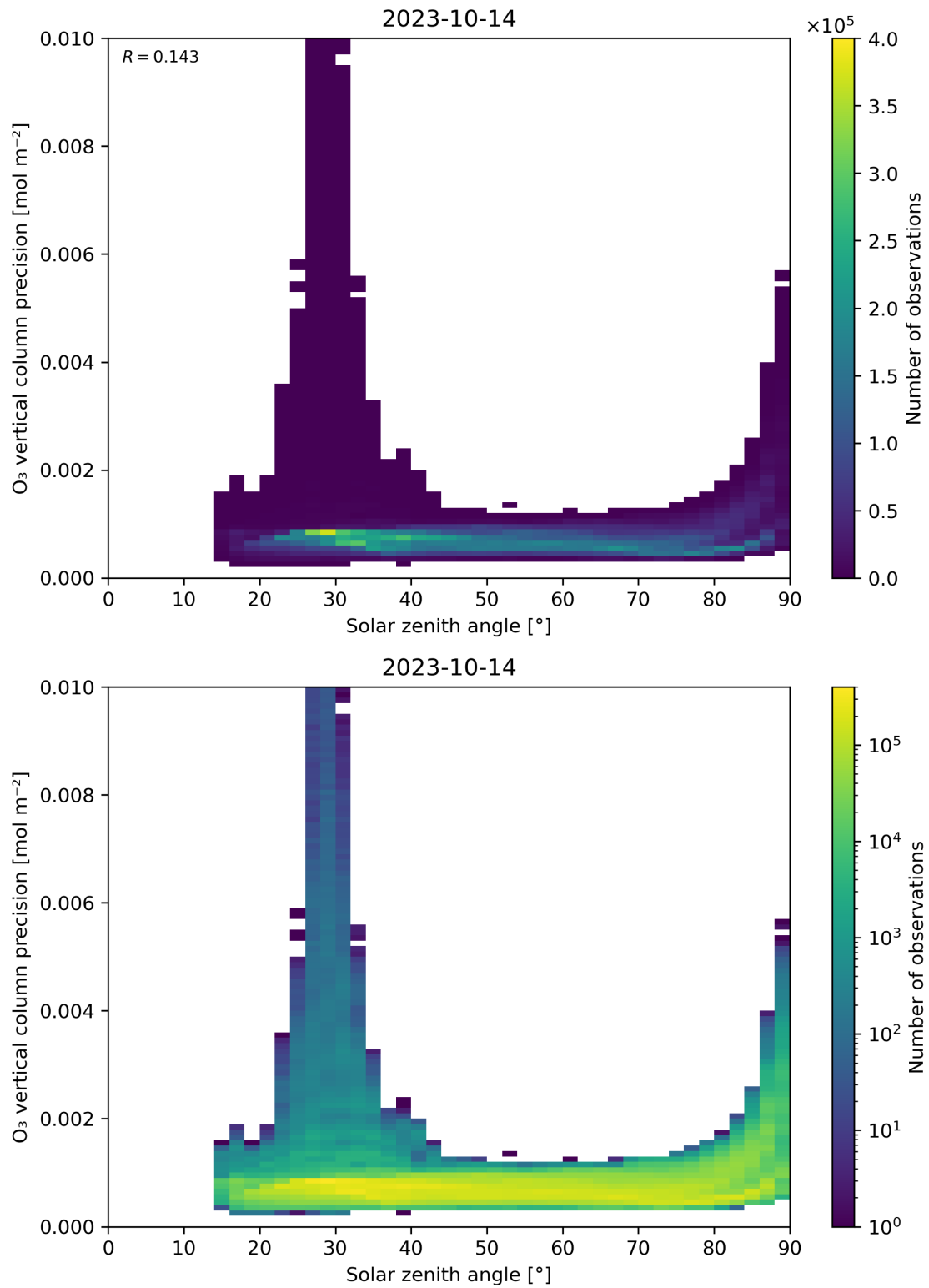
Figure 48: Scatter density plot of “Solar zenith angle” against “O 3 vertical column precision” for 2023-10-13 to 2023-10-15.
