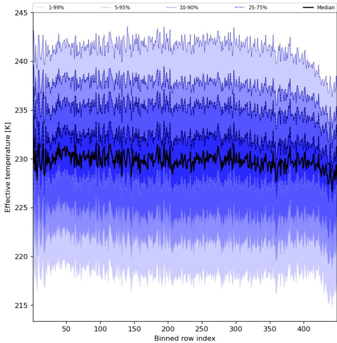
Figure 31: Along track statistics of “Effective temperature” for 2023-10-13 to 2023-10-15
