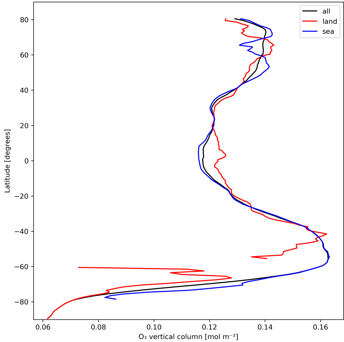
Figure 14: Zonal average of “O 3 vertical column” for 2023-10-13 to 2023-10-15.
