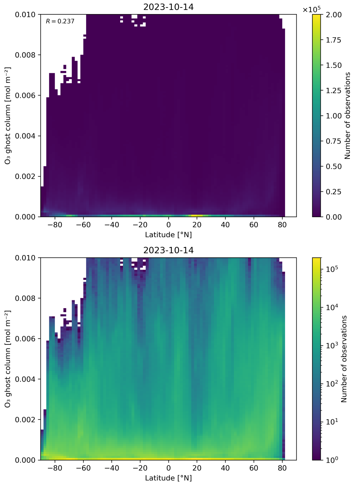
Figure 35: Scatter density plot of “Latitude” against “O 3 ghost column” for 2023-10-13 to 2023-10-15.
