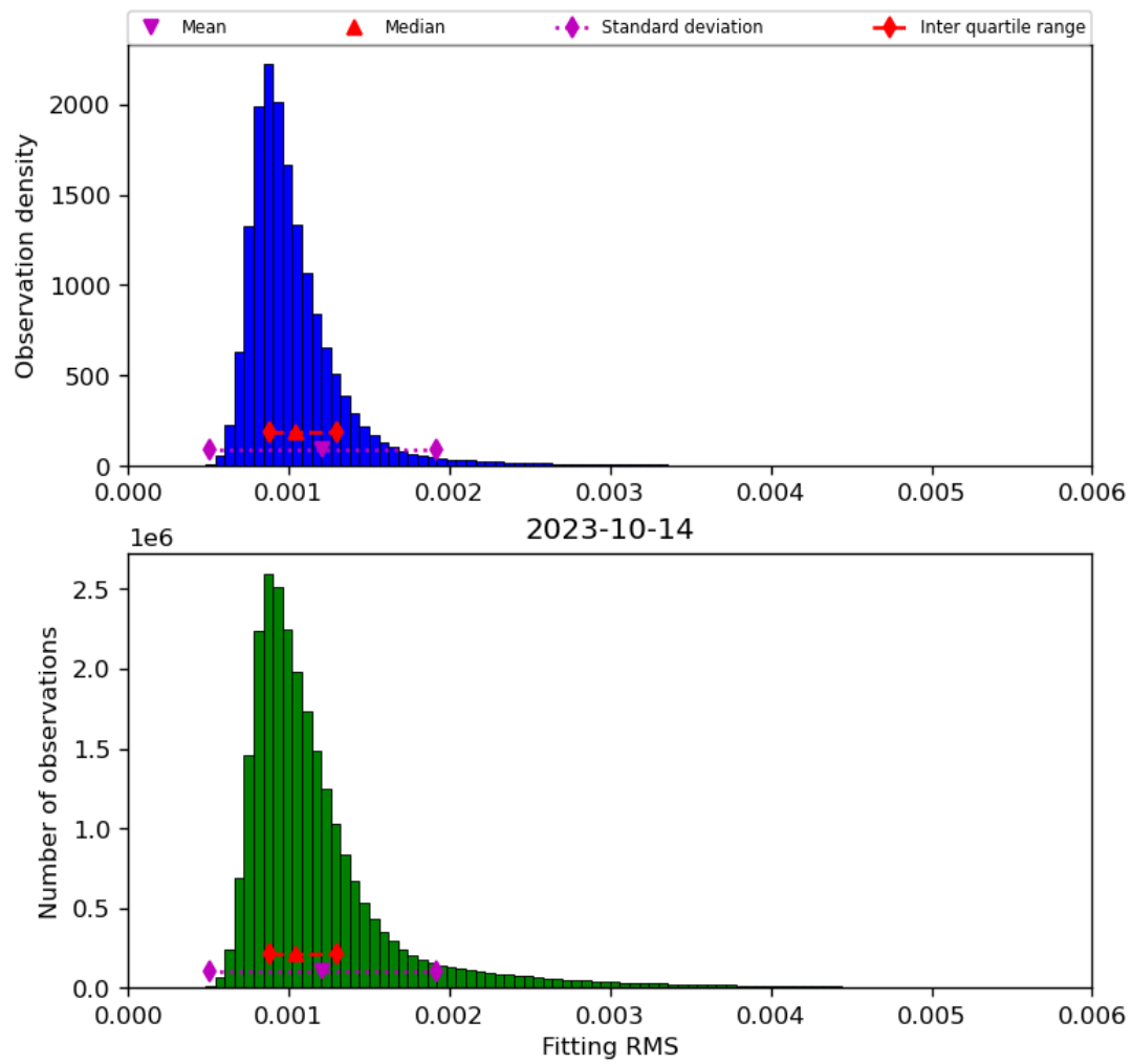
Figure 23: Histogram of “Fitting RMS” for 2023-10-13 to 2023-10-15
