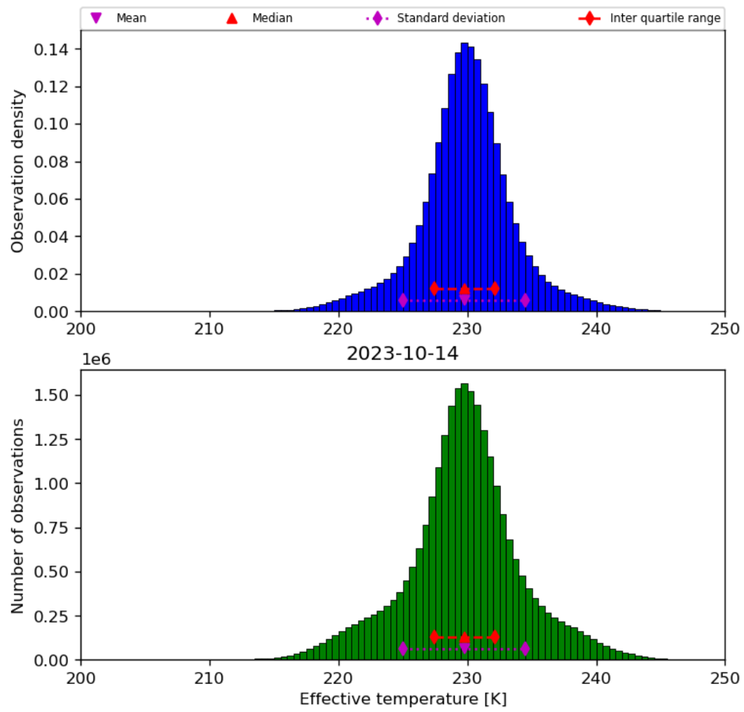
Figure 24: Histogram of “Effective temperature” for 2023-10-13 to 2023-10-15
