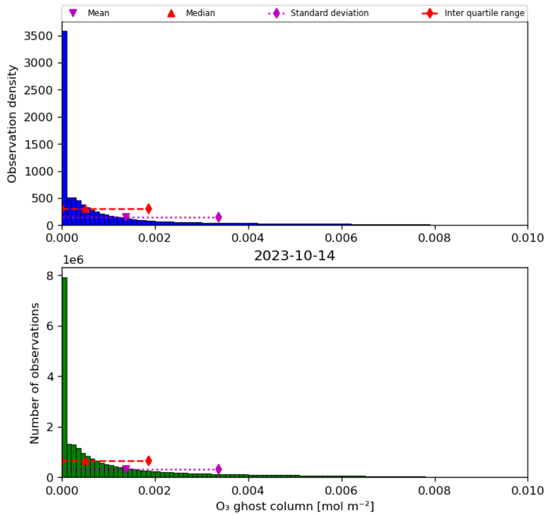
Figure 25: Histogram of “O 3 ghost column” for 2023-10-13 to 2023-10-15
