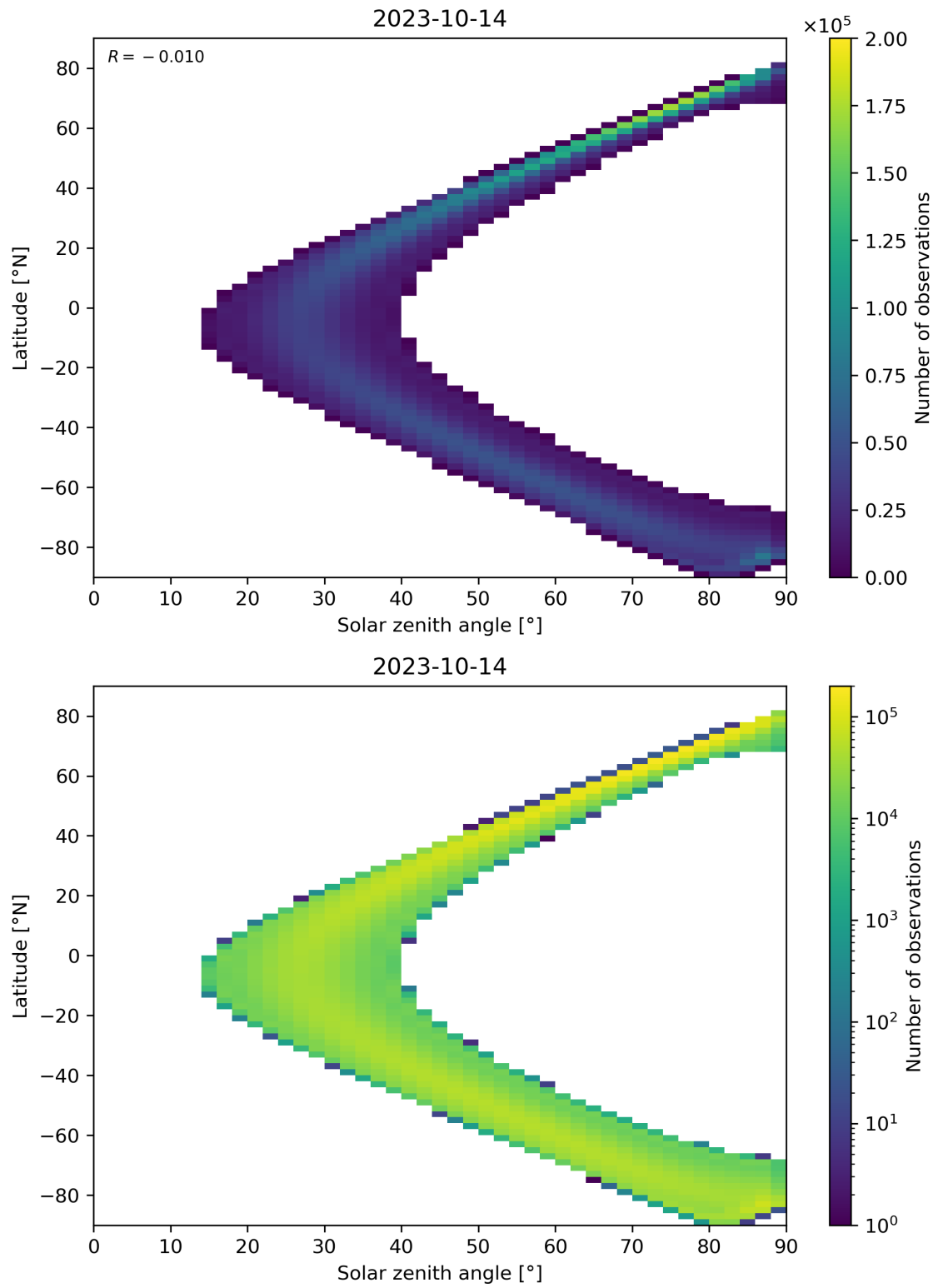
Figure 44: Scatter density plot of “Solar zenith angle” against “Latitude” for 2023-10-13 to 2023-10-15.
