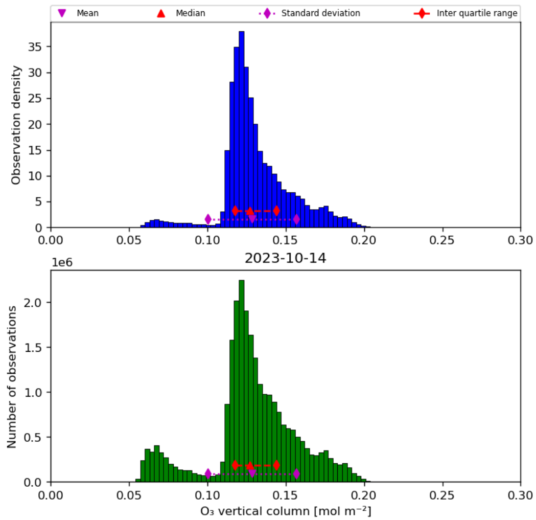
Figure 21: Histogram of “O 3 vertical column” for 2023-10-13 to 2023-10-15
