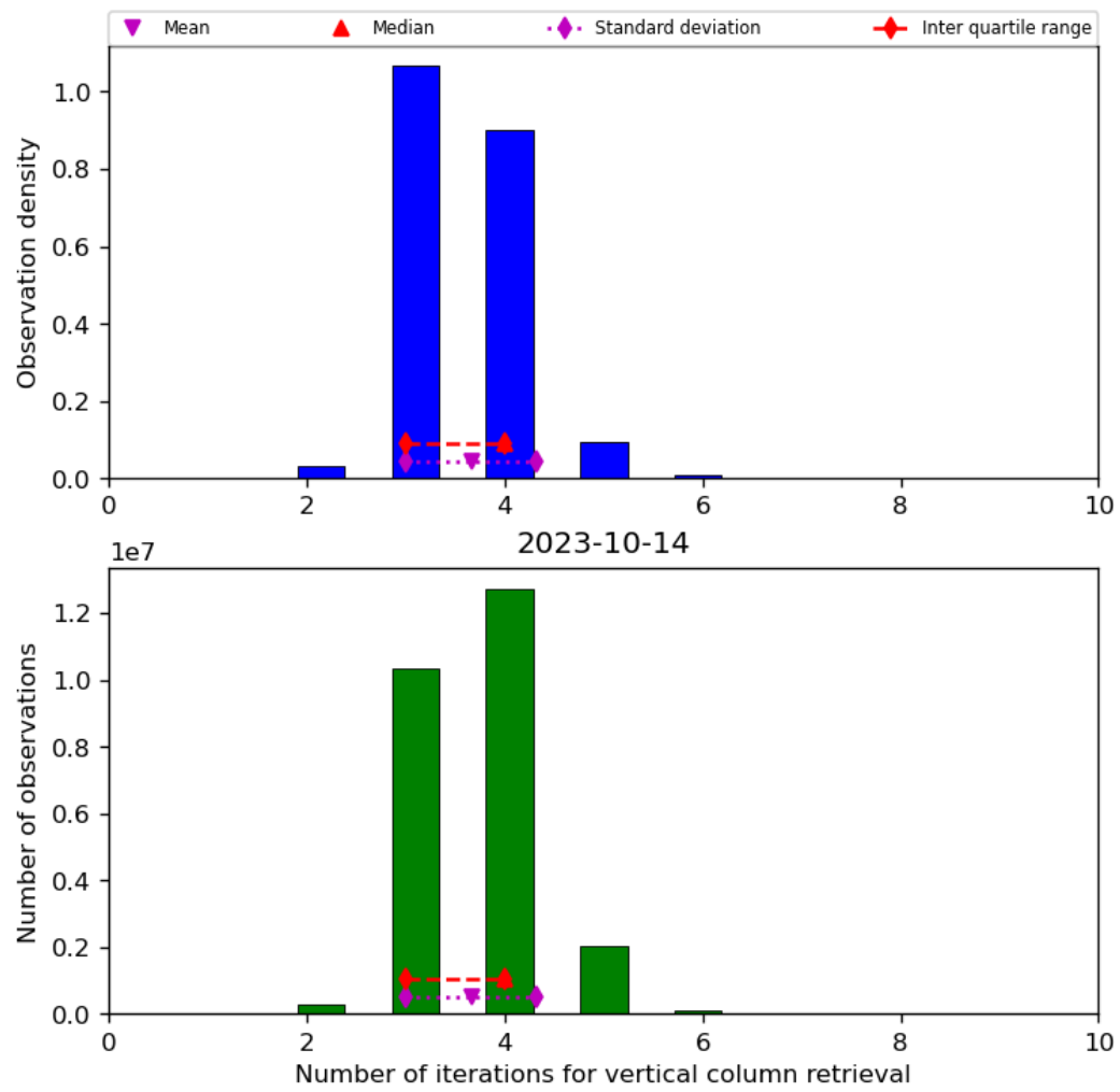
Figure 26: Histogram of “Number of iterations for vertical column retrieval” for 2023-10-13 to 2023-10-15
