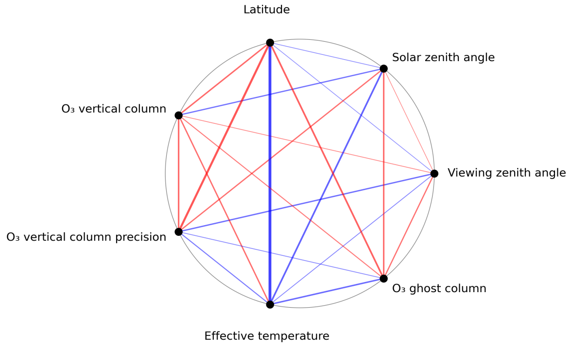
Figure 1: Map of correlation graph for 2023-10-13 to 2023-10-15.
