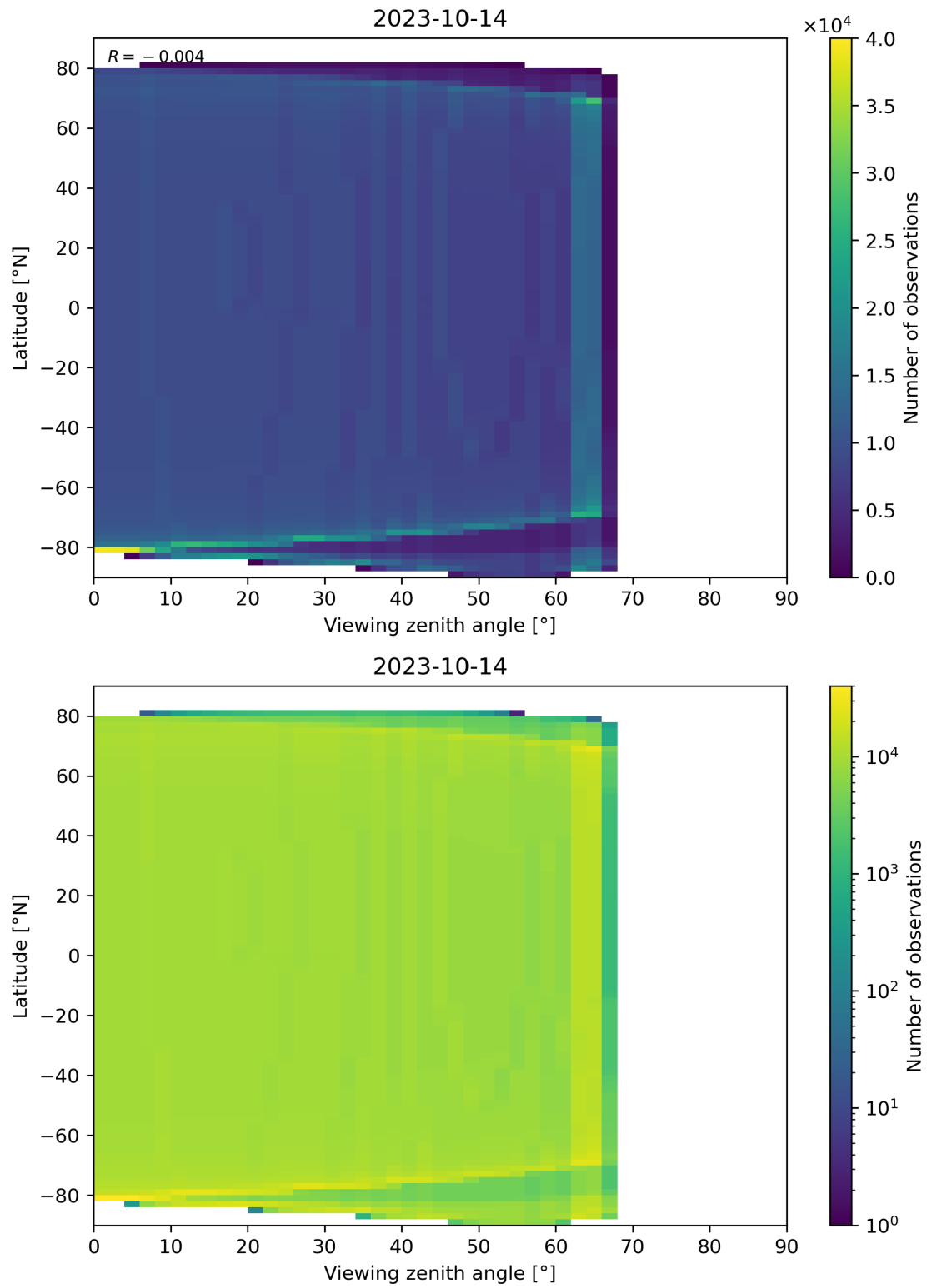
Figure 49: Scatter density plot of “Viewing zenith angle” against “Latitude” for 2023-10-13 to 2023-10-15.
