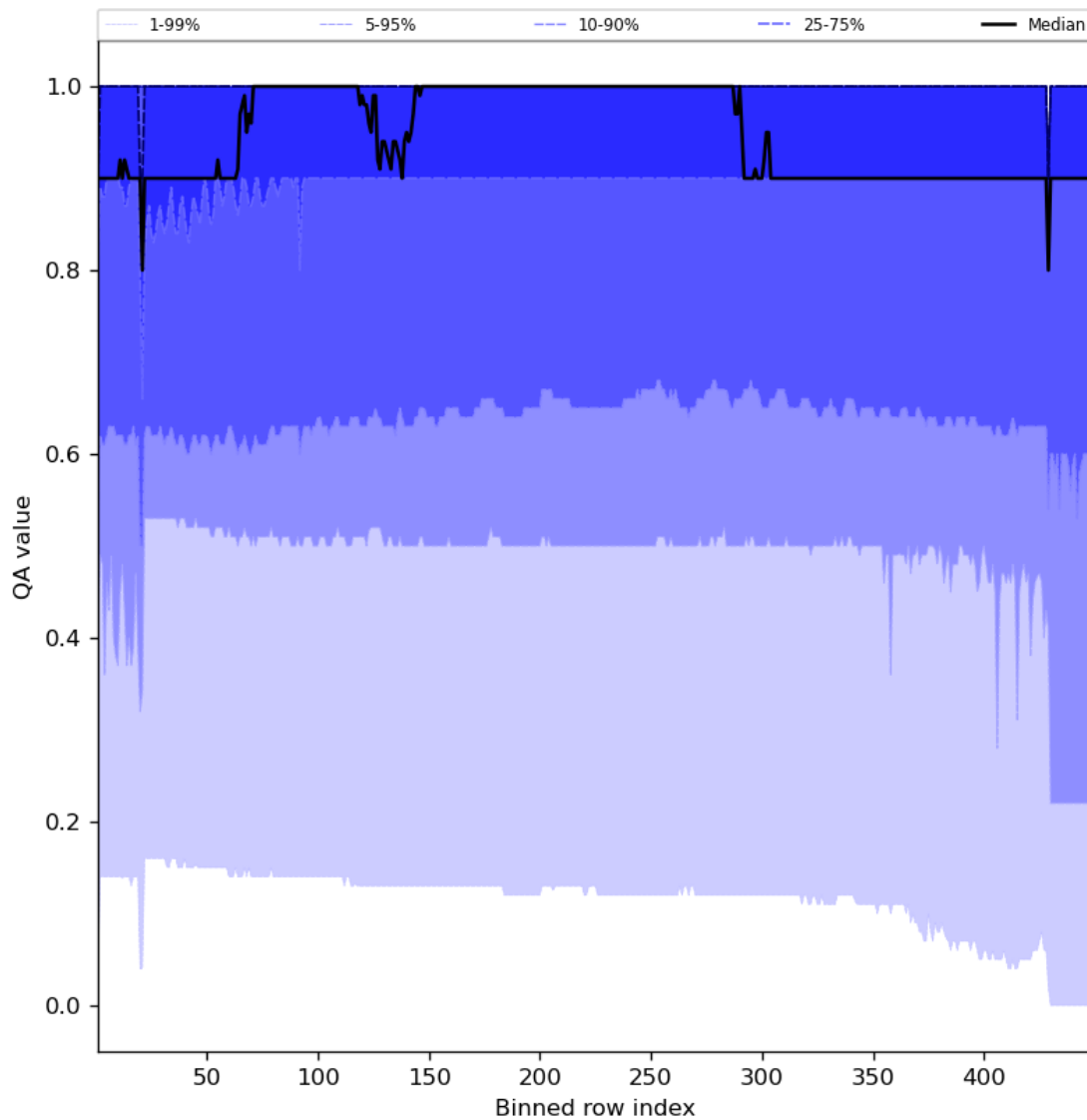
Figure 27: Along track statistics of “QA value” for 2023-10-13 to 2023-10-15
