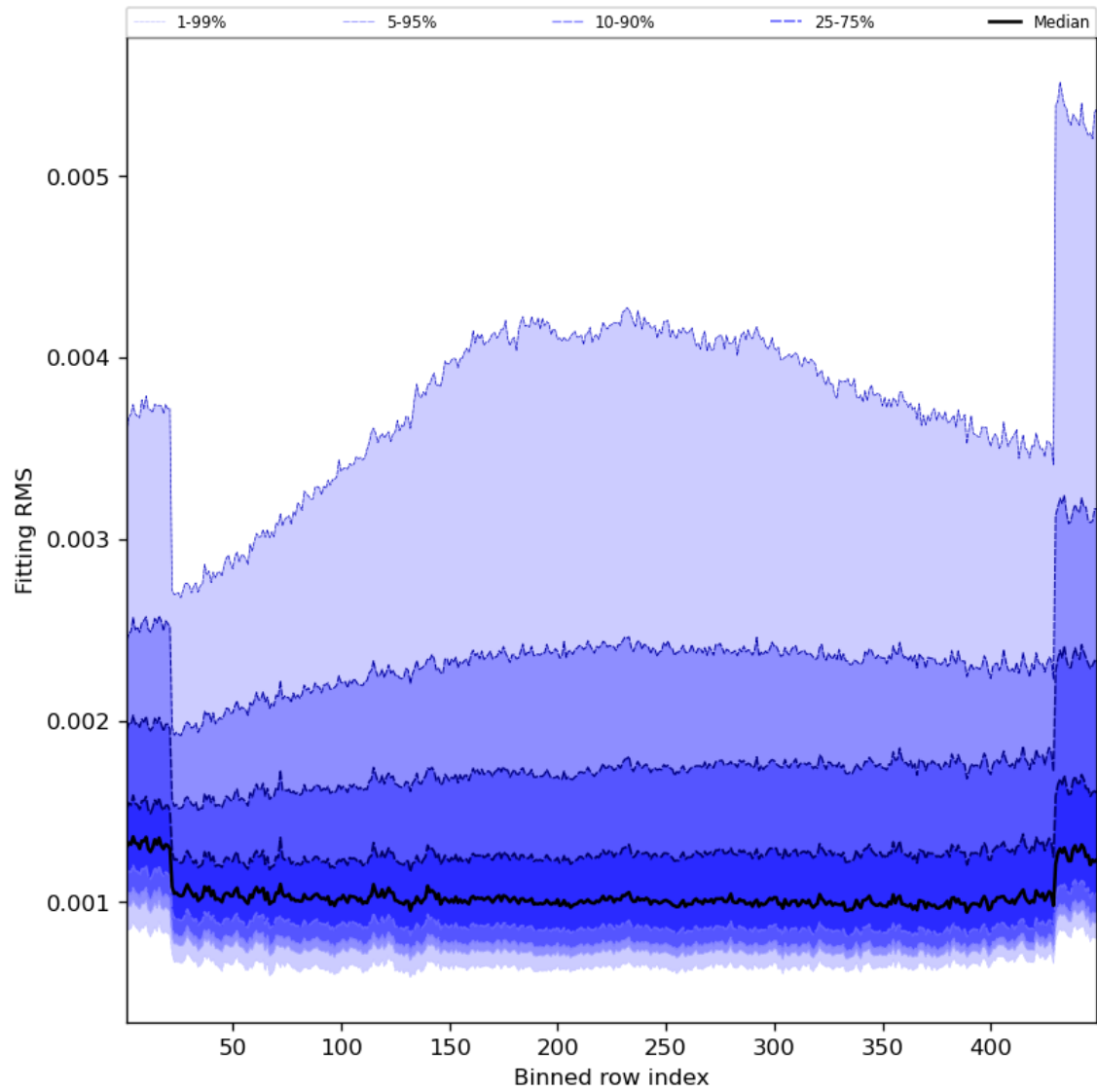
Figure 30: Along track statistics of “Fitting RMS” for 2023-10-13 to 2023-10-15
