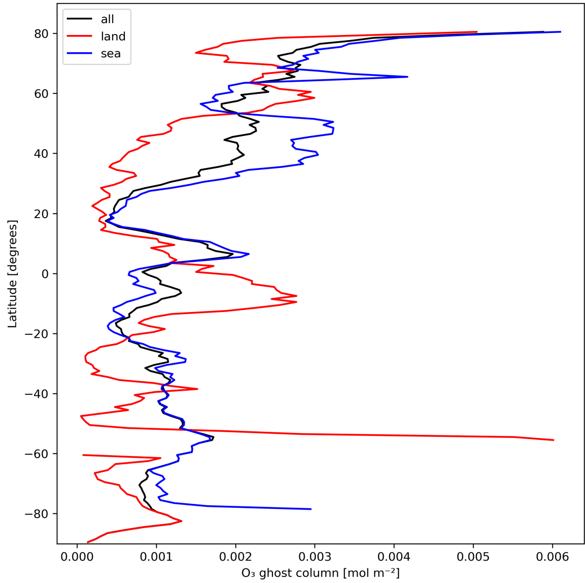
Figure 18: Zonal average of “O 3 ghost column” for 2023-10-13 to 2023-10-15.
