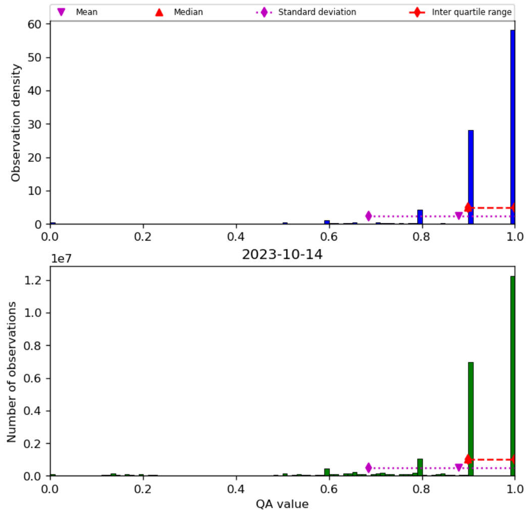
Figure 20: Histogram of “QA value” for 2023-10-13 to 2023-10-15
