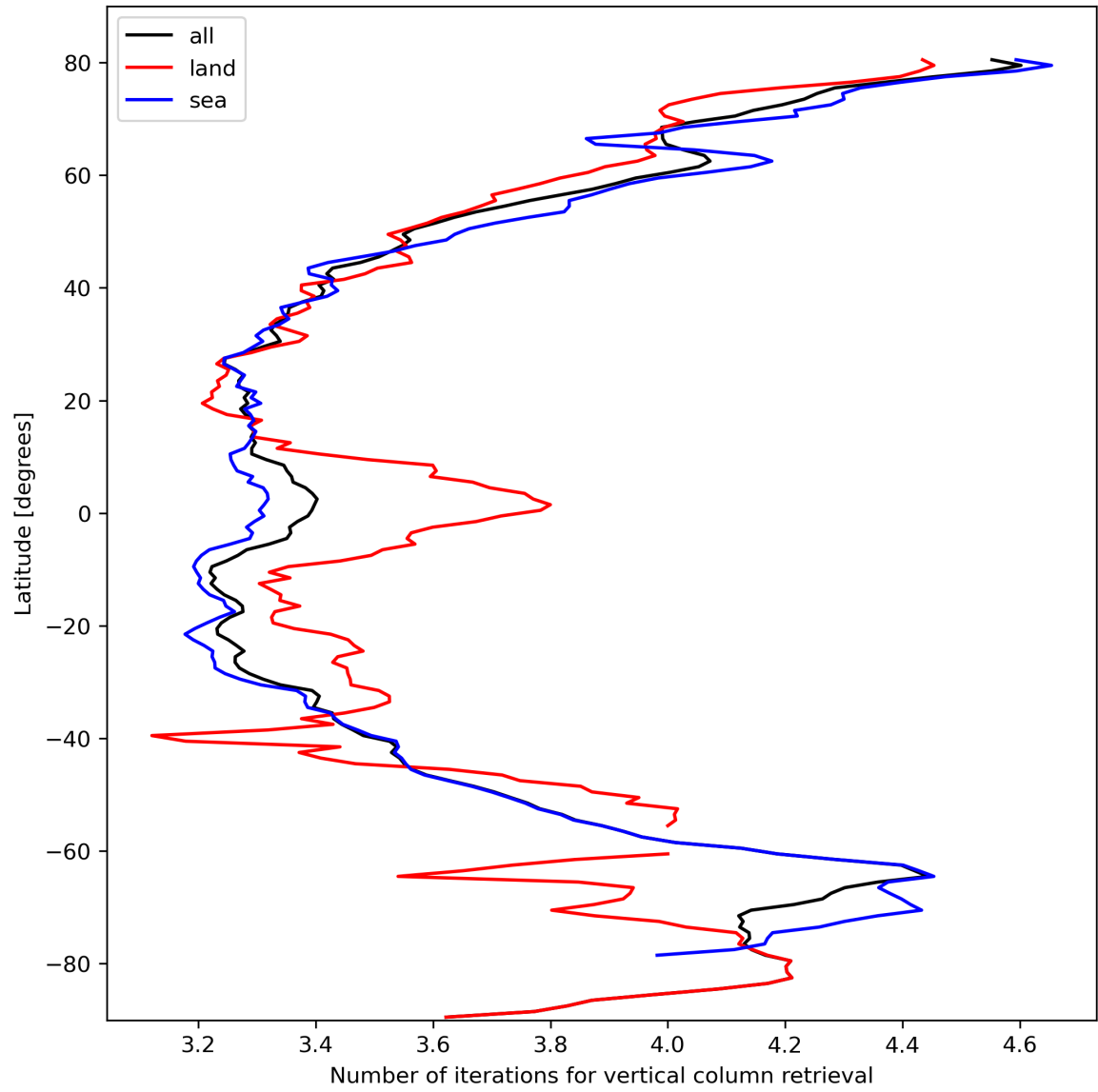
Figure 19: Zonal average of “Number of iterations for vertical column retrieval” for 2023-10-13 to 2023-10-15.
