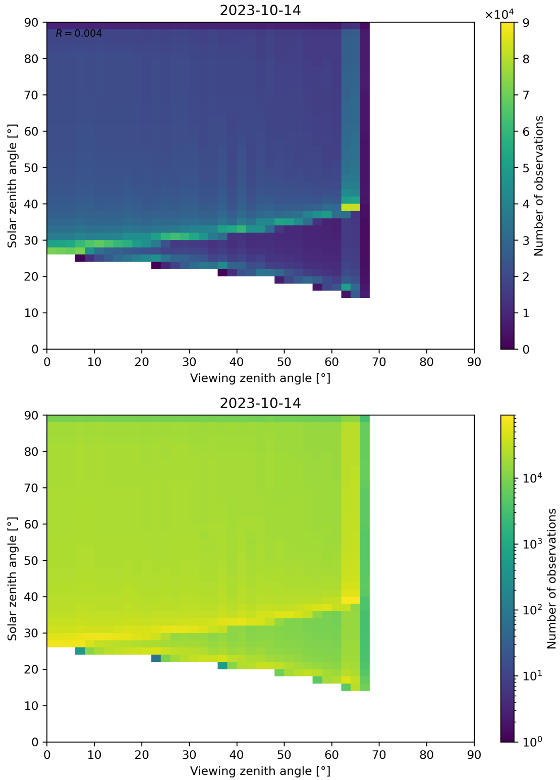
Figure 54: Scatter density plot of “Viewing zenith angle” against “Solar zenith angle” for 2023-10-13 to 2023-10-15.
