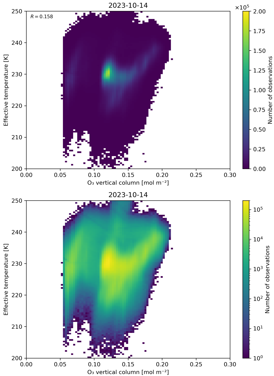
Figure 39: Scatter density plot of “O 3 vertical column” against “Effective temperature” for 2023-10-13 to 2023-10-15.
