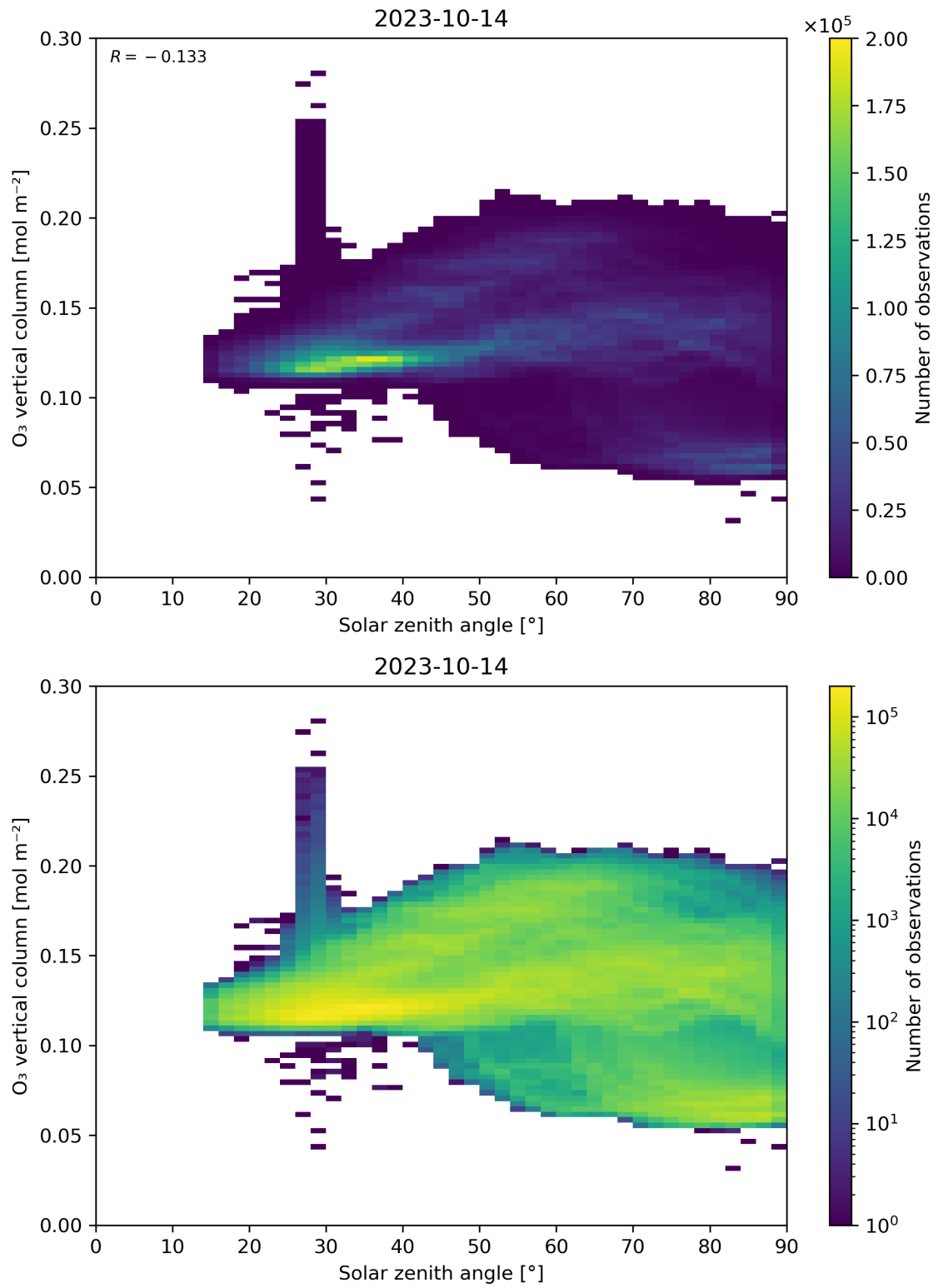
Figure 47: Scatter density plot of “Solar zenith angle” against “O 3 vertical column” for 2023-10-13 to 2023-10-15.
