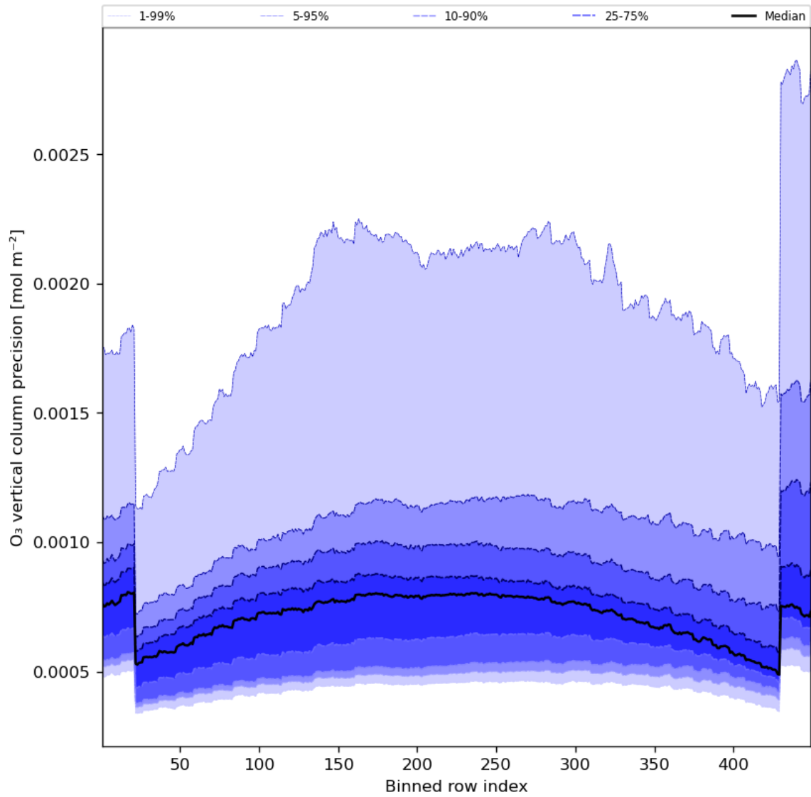
Figure 29: Along track statistics of “O 3 vertical column precision” for 2023-10-13 to 2023-10-15
