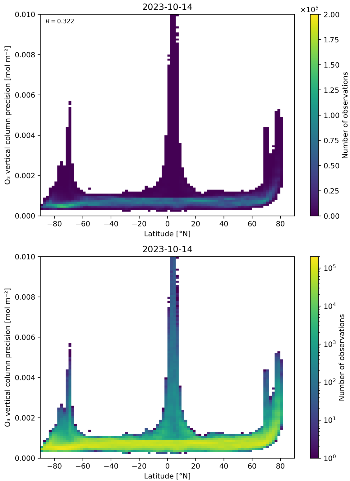
Figure 37: Scatter density plot of “Latitude” against “O 3 vertical column precision” for 2023-10-13 to 2023-10-15.
