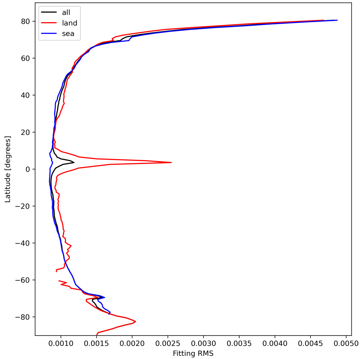
Figure 16: Zonal average of “Fitting RMS” for 2023-10-13 to 2023-10-15.
