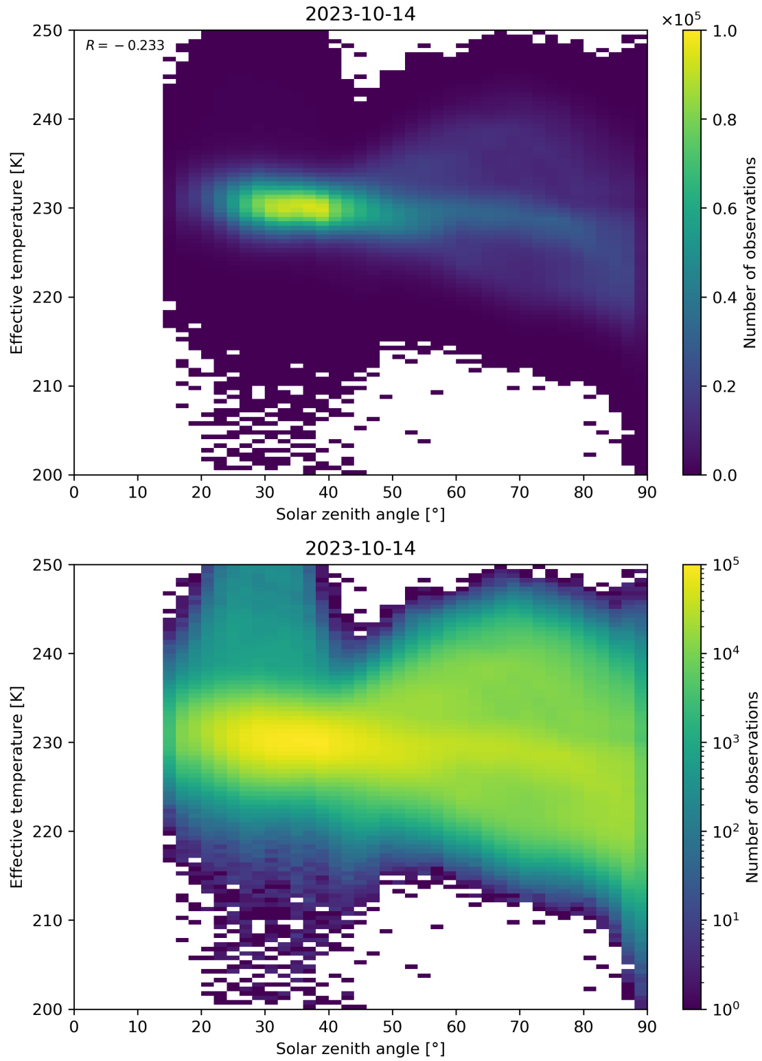
Figure 45: Scatter density plot of “Solar zenith angle” against “Effective temperature” for 2023-10-13 to 2023-10-15.
