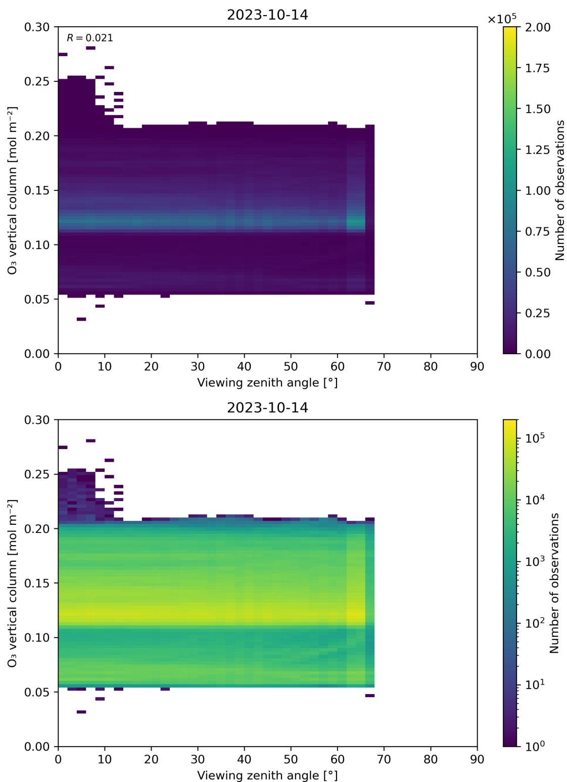
Figure 52: Scatter density plot of “Viewing zenith angle” against “O 3 vertical column” for 2023-10-13 to 2023-10-15.
