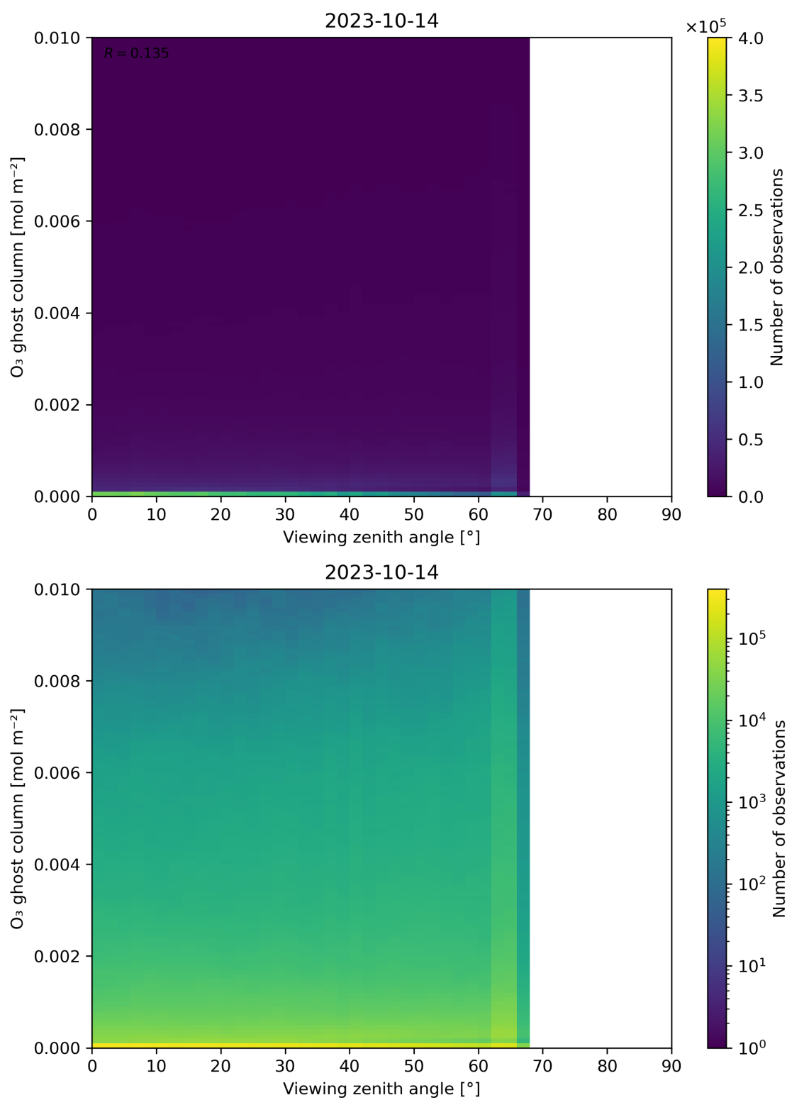
Figure 51: Scatter density plot of “Viewing zenith angle” against “O 3 ghost column” for 2023-10-13 to 2023-10-15.
