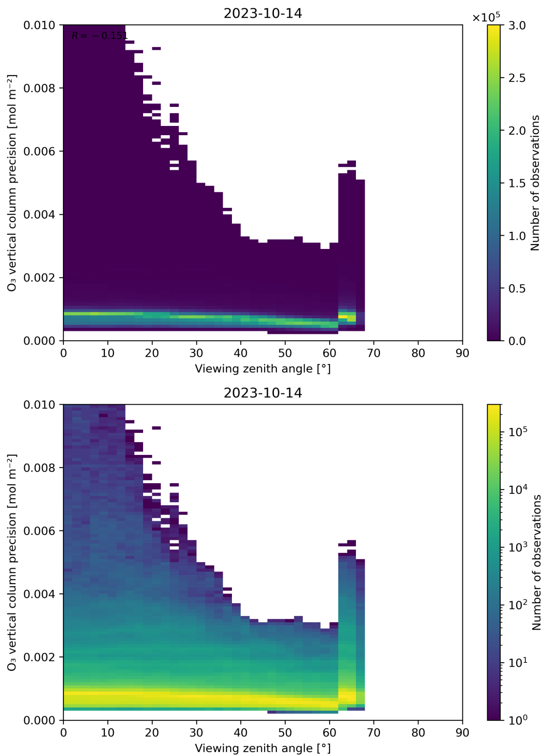
Figure 53: Scatter density plot of “Viewing zenith angle” against “O 3 vertical column precision” for 2023-10-13 to 2023-10-15.
