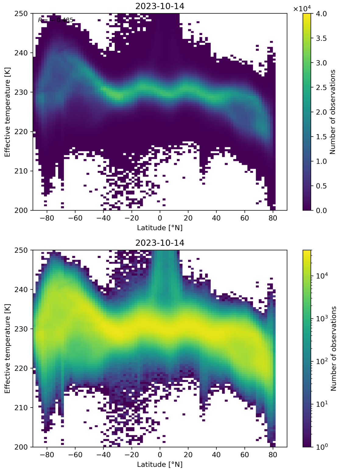
Figure 34: Scatter density plot of “Latitude” against “Effective temperature” for 2023-10-13 to 2023-10-15.
