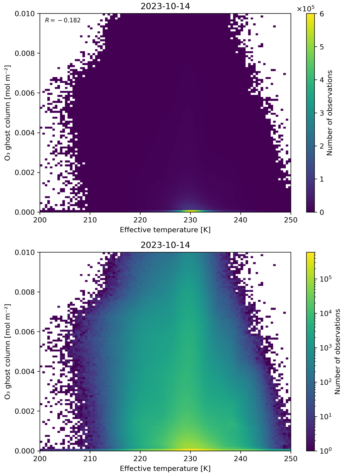
Figure 38: Scatter density plot of “Effective temperature” against “O 3 ghost column” for 2023-10-13 to 2023-10-15.
