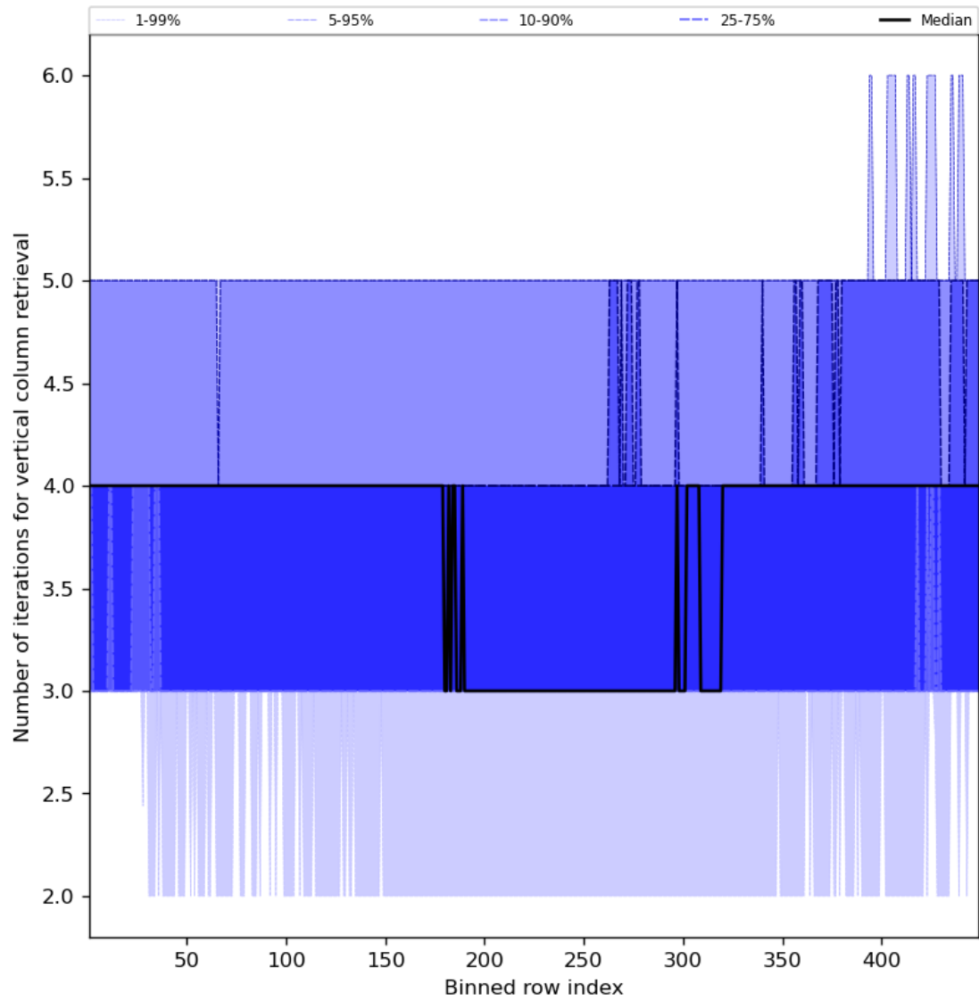
Figure 33: Along track statistics of “Number of iterations for vertical column retrieval” for 2023-10-13 to 2023-10-15
