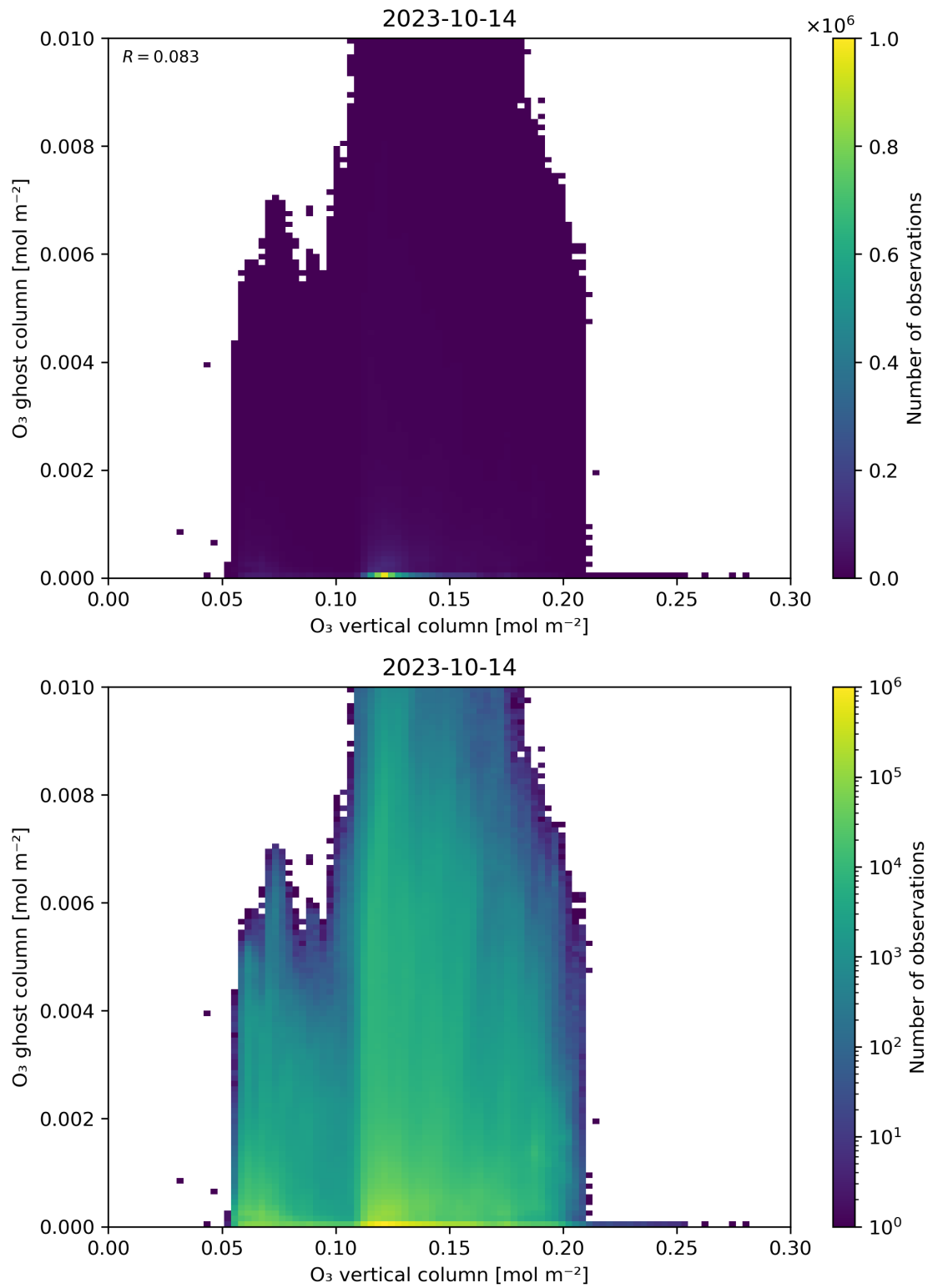
Figure 40: Scatter density plot of “O 3 vertical column” against “O 3 ghost column” for 2023-10-13 to 2023-10-15.
