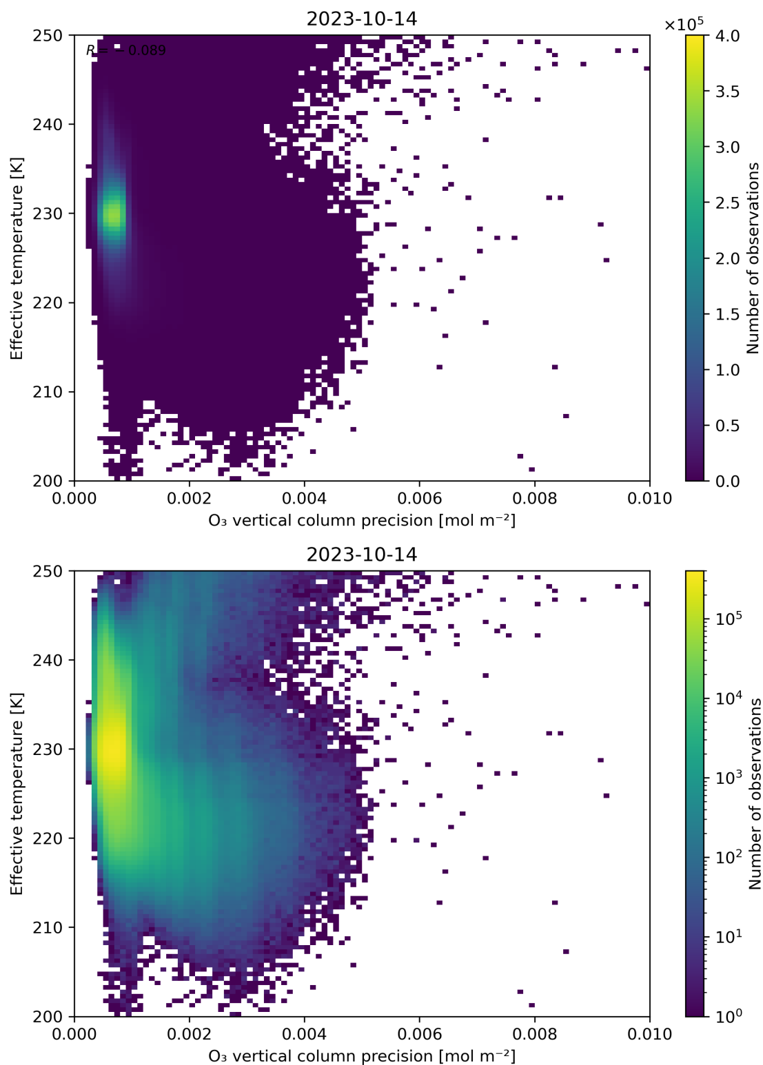
Figure 42: Scatter density plot of “O 3 vertical column precision” against “Effective temperature” for 2023-10-13 to 2023-10-15.
