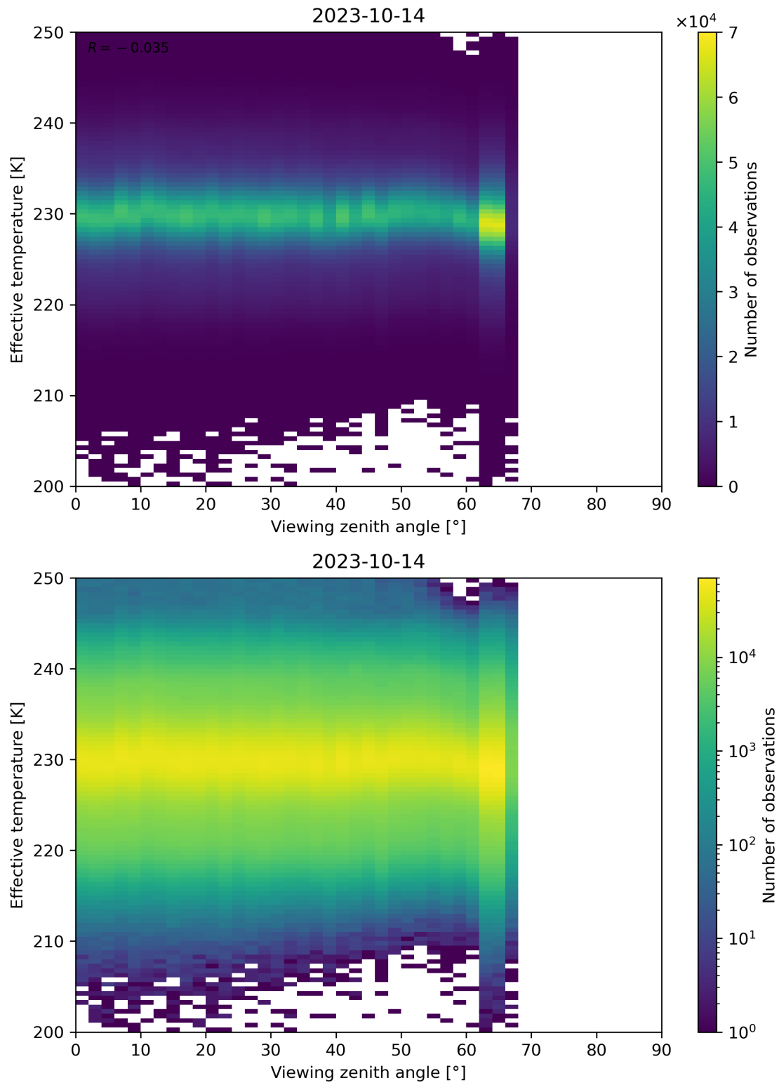
Figure 50: Scatter density plot of “Viewing zenith angle” against “Effective temperature” for 2023-10-13 to 2023-10-15.
