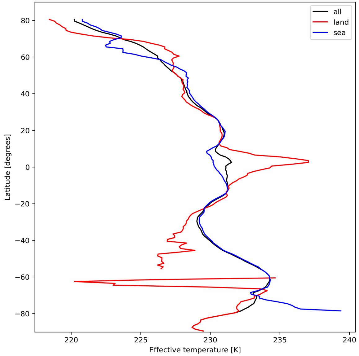
Figure 17: Zonal average of “Effective temperature” for 2023-10-13 to 2023-10-15.
