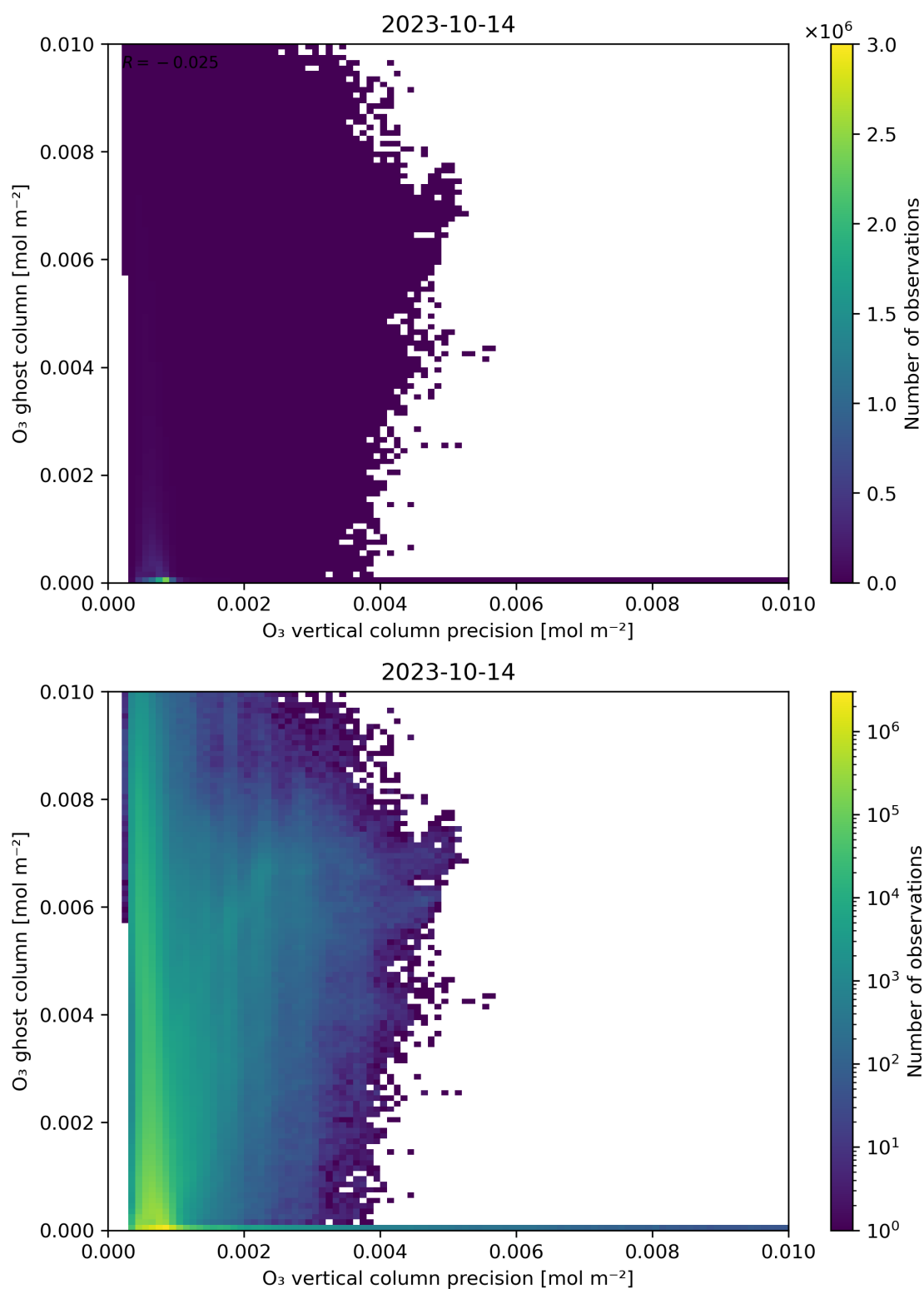
Figure 43: Scatter density plot of “ \text{O}_3 vertical column precision” against “ \text{O}_3 ghost column” for 2023-10-13 to 2023-10-15.
