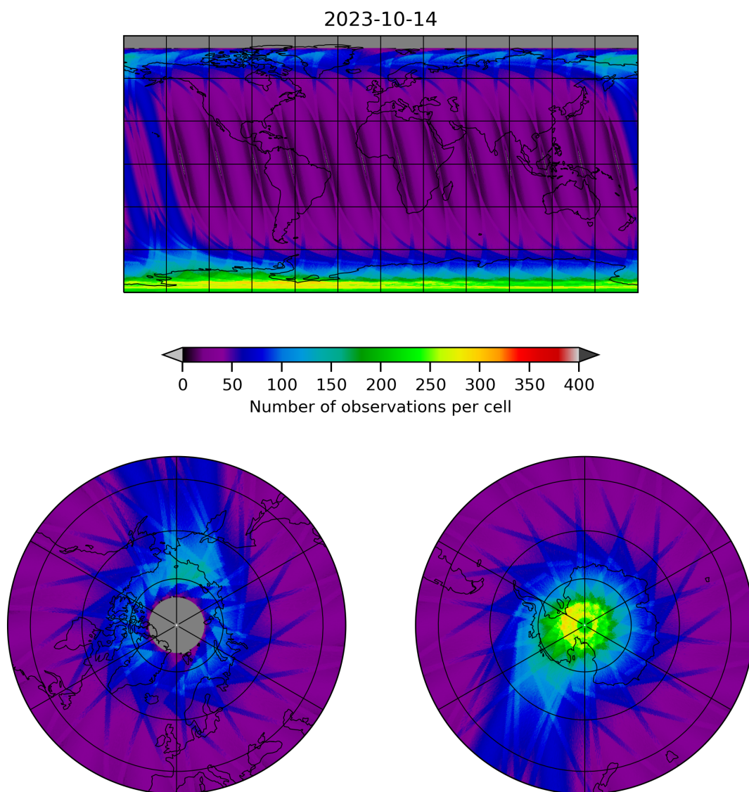
Figure 12: Map of the number of observations for 2023-10-13 to 2023-10-15
