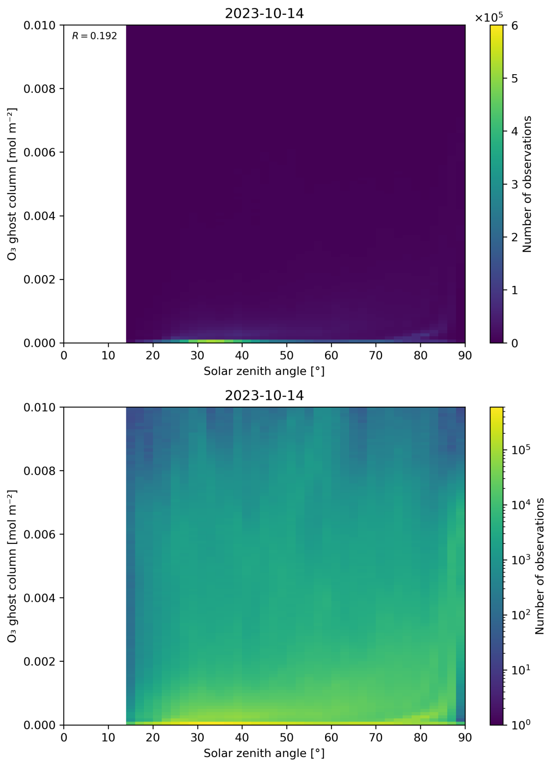
Figure 46: Scatter density plot of “Solar zenith angle” against “O 3 ghost column” for 2023-10-13 to 2023-10-15.
