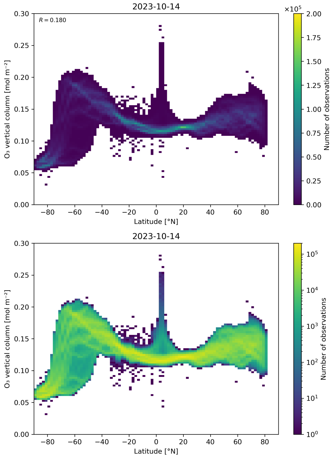
Figure 36: Scatter density plot of “Latitude” against “O 3 vertical column” for 2023-10-13 to 2023-10-15.
