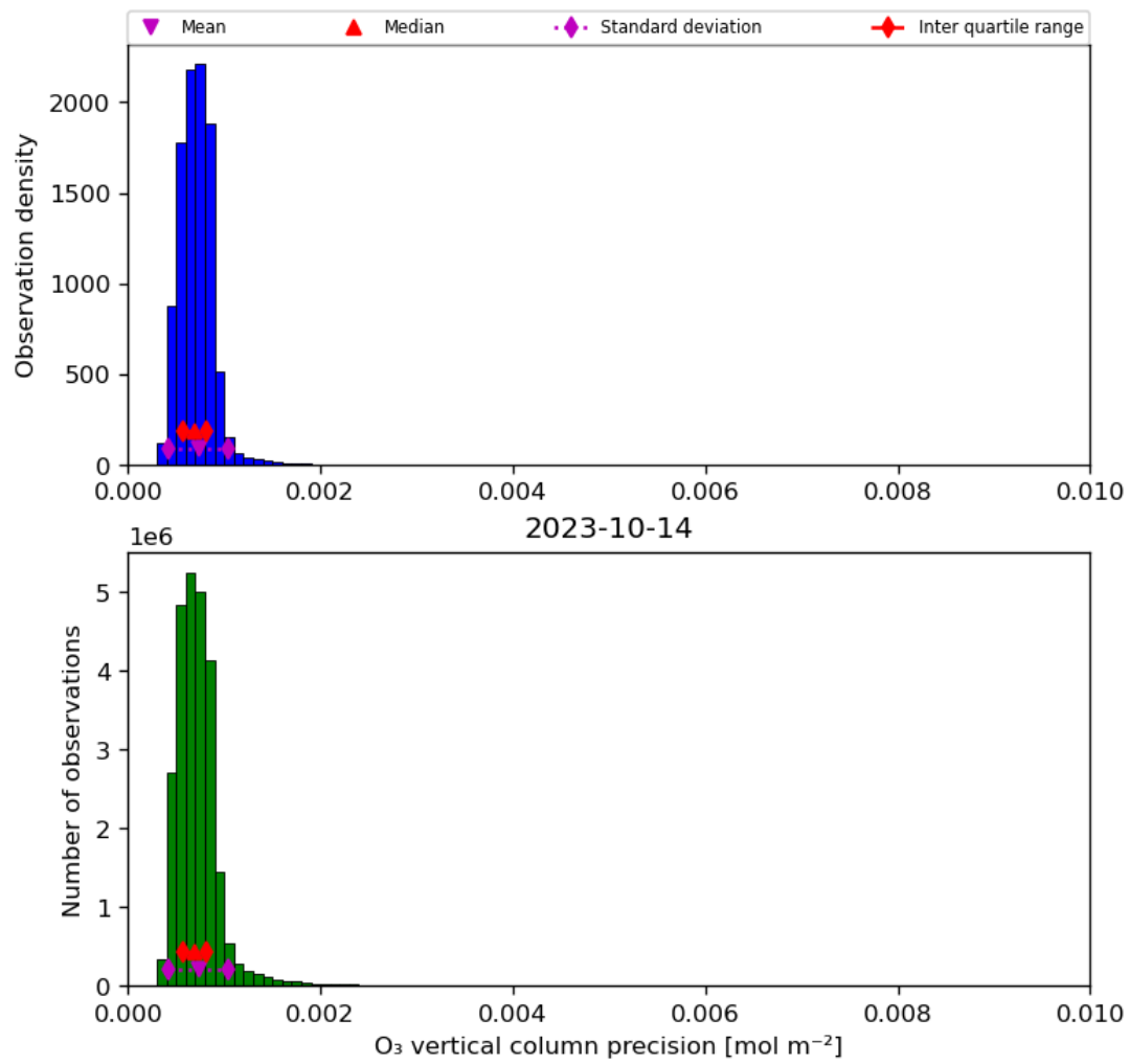
Figure 22: Histogram of “O 3 vertical column precision” for 2023-10-13 to 2023-10-15
