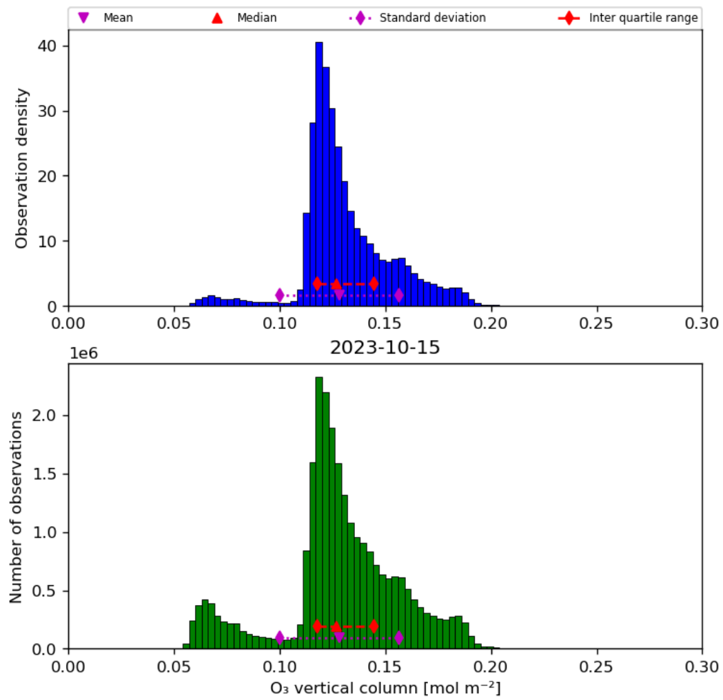
Figure 21: Histogram of “O 3 vertical column” for 2023-10-14 to 2023-10-16
