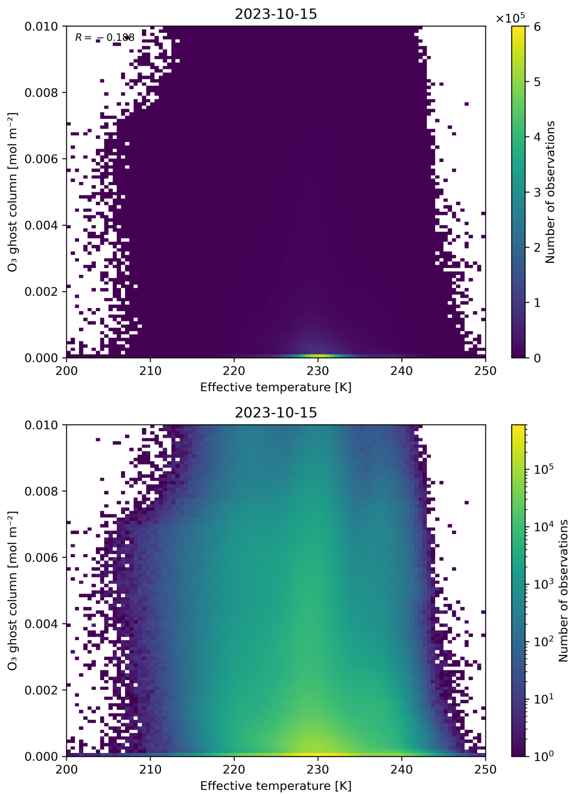
Figure 38: Scatter density plot of “Effective temperature” against “O 3 ghost column” for 2023-10-14 to 2023-10-16.
