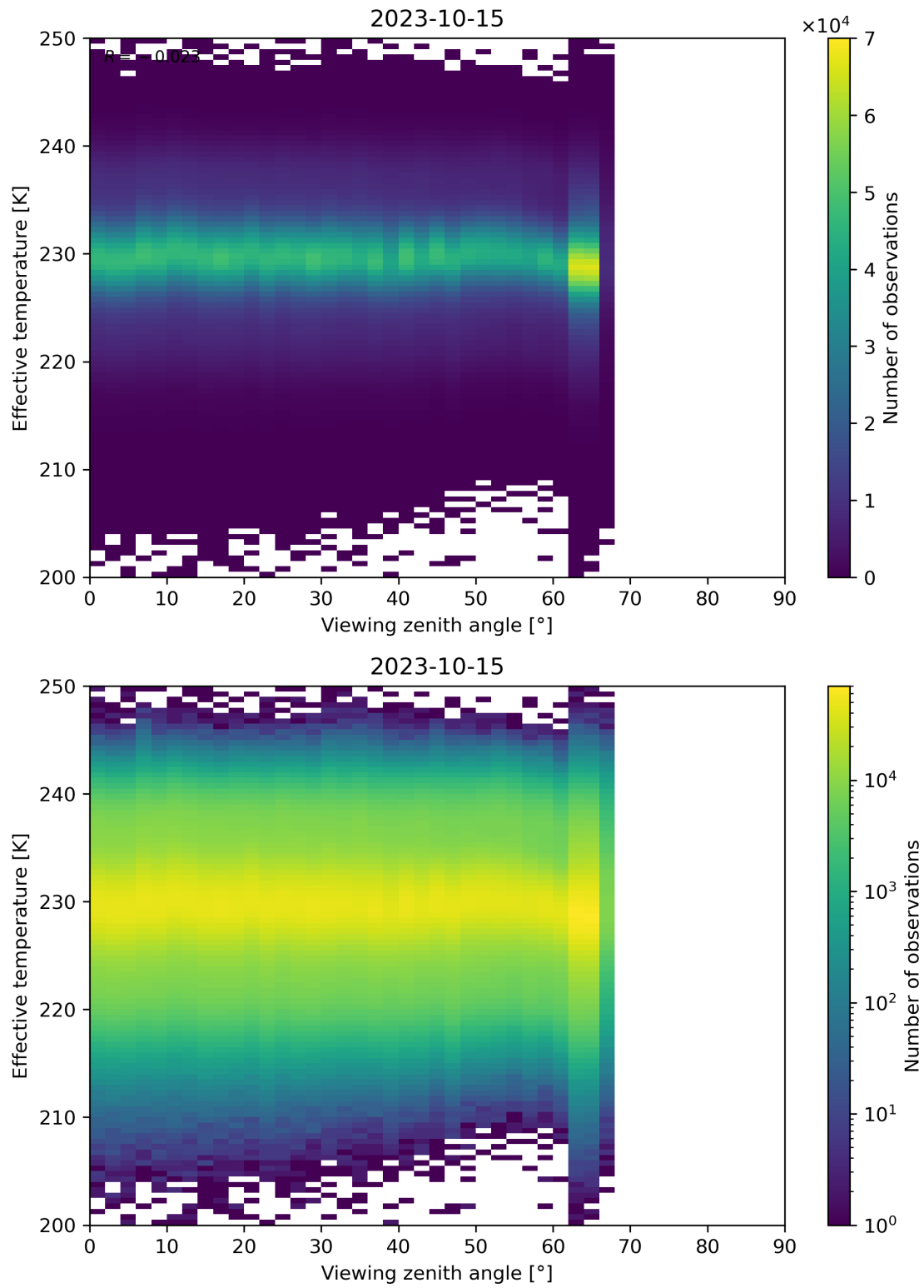
Figure 50: Scatter density plot of “Viewing zenith angle” against “Effective temperature” for 2023-10-14 to 2023-10-16.
