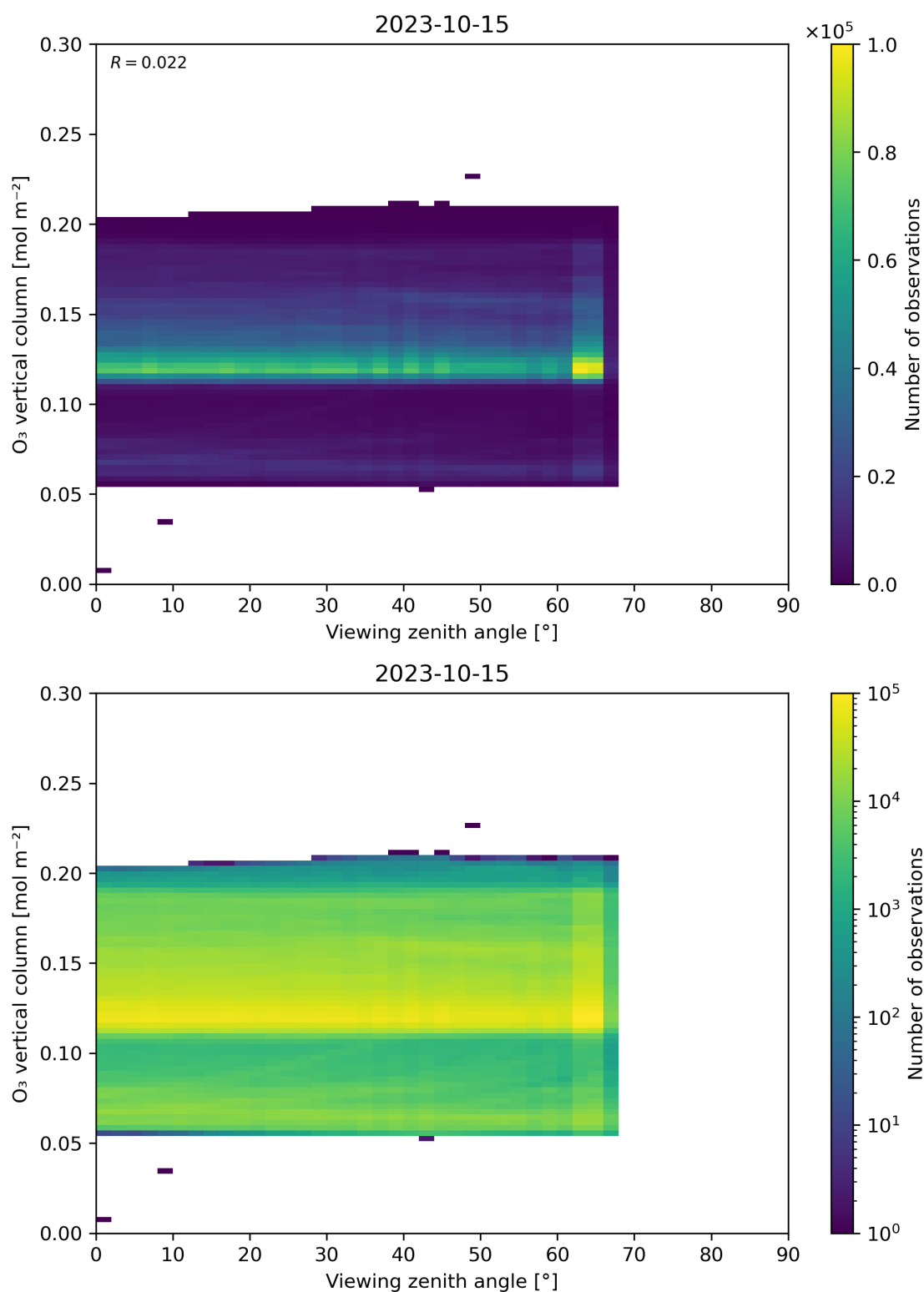
Figure 52: Scatter density plot of “Viewing zenith angle” against “O 3 vertical column” for 2023-10-14 to 2023-10-16.
