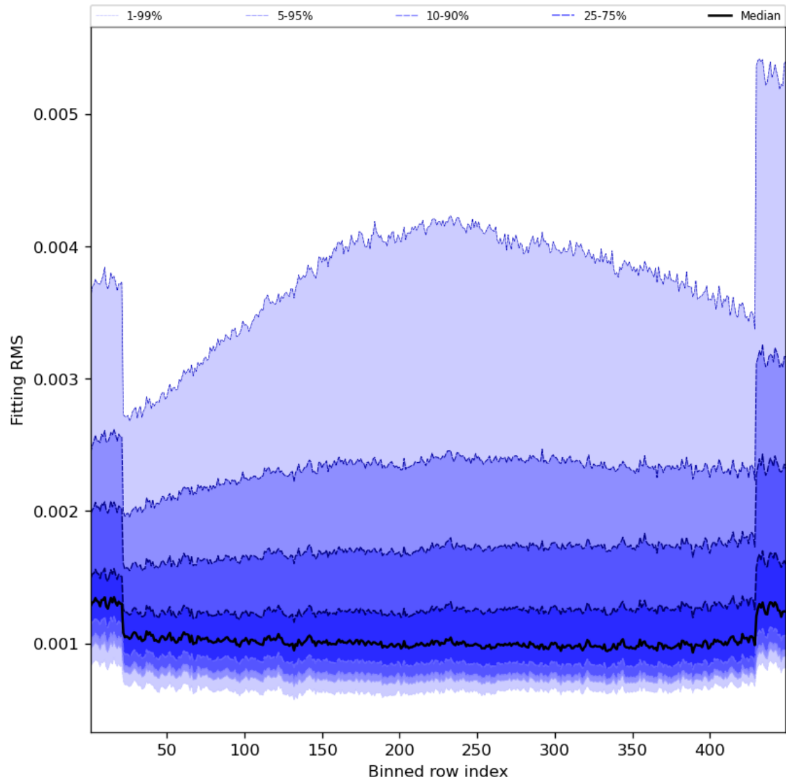
Figure 30: Along track statistics of “Fitting RMS” for 2023-10-14 to 2023-10-16
