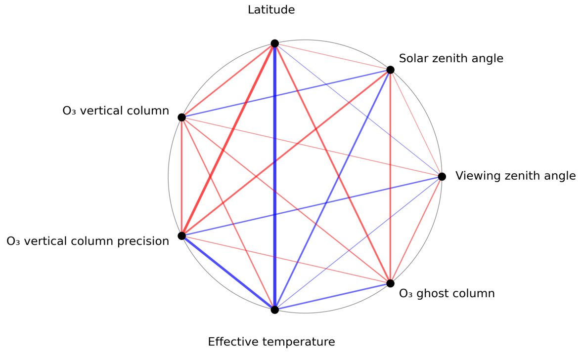
Figure 1: Map of correlation graph for 2023-10-14 to 2023-10-16.
