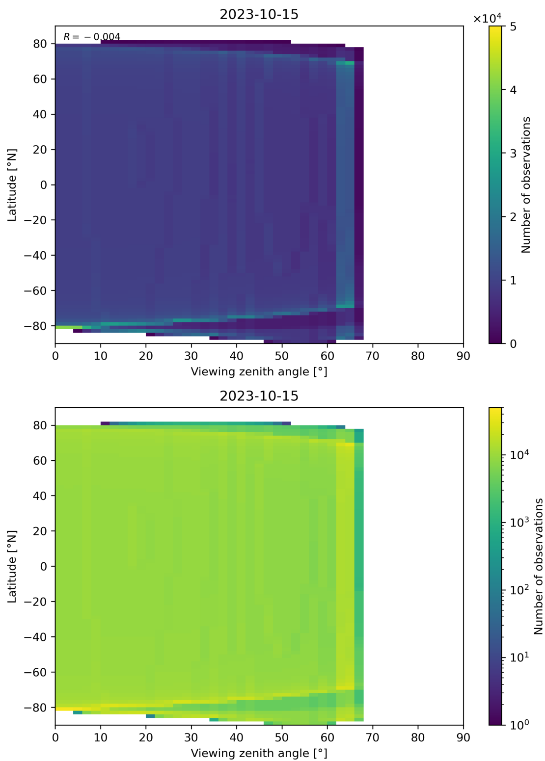
Figure 49: Scatter density plot of “Viewing zenith angle” against “Latitude” for 2023-10-14 to 2023-10-16.
