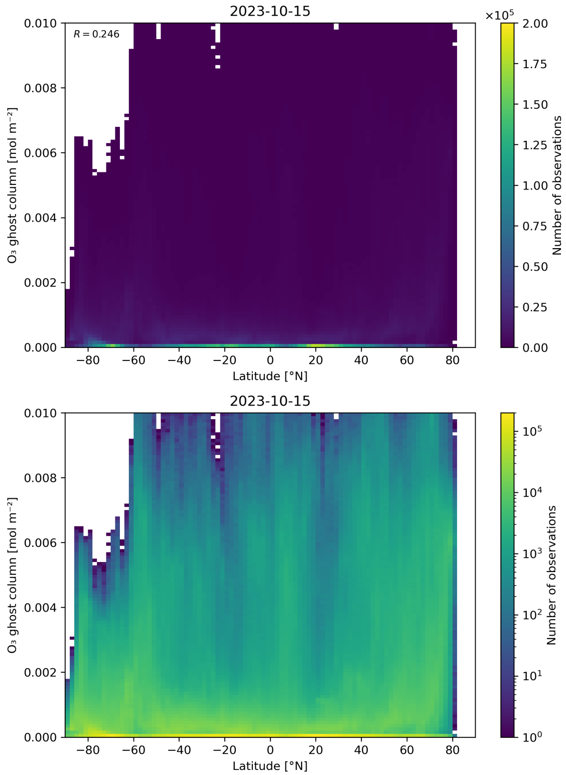
Figure 35: Scatter density plot of “Latitude” against “O 3 ghost column” for 2023-10-14 to 2023-10-16.
