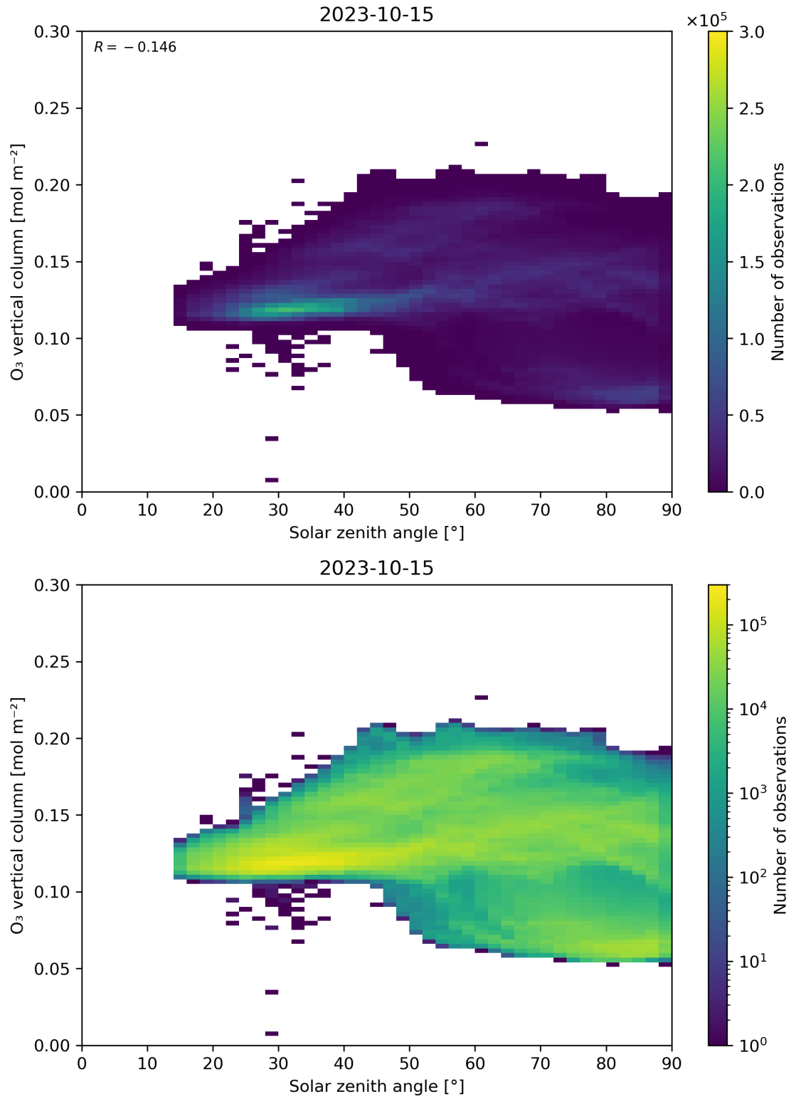
Figure 47: Scatter density plot of “Solar zenith angle” against “O 3 vertical column” for 2023-10-14 to 2023-10-16.
