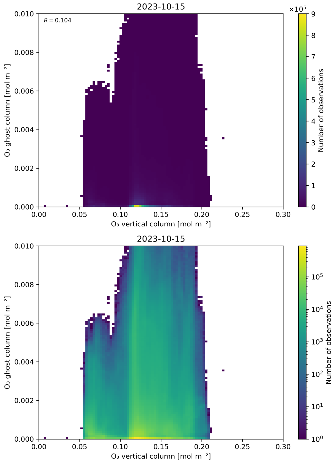
Figure 40: Scatter density plot of “O 3 vertical column” against “O 3 ghost column” for 2023-10-14 to 2023-10-16.
