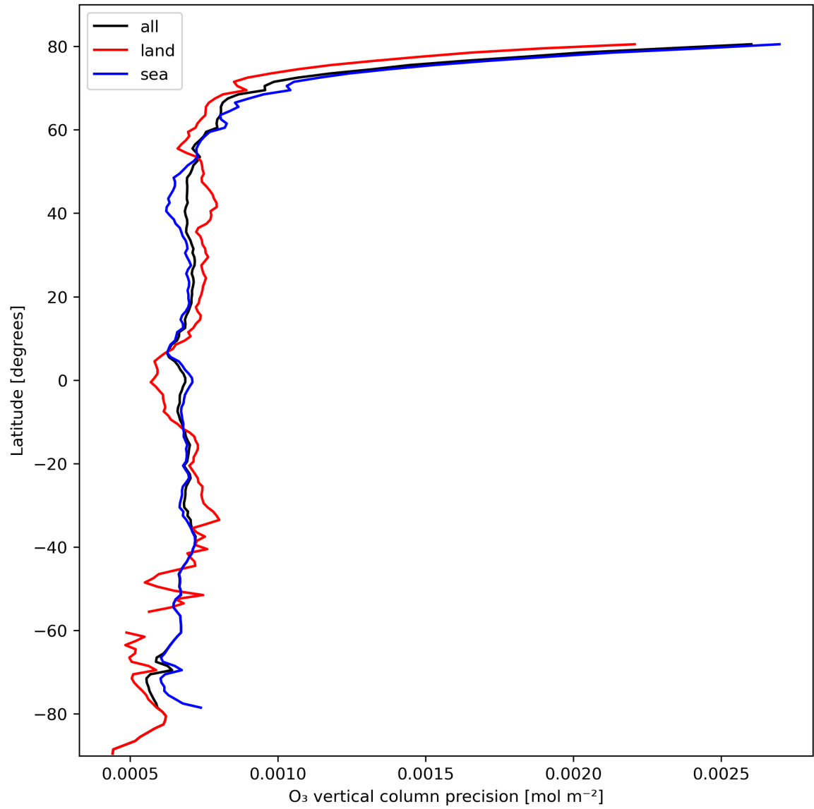
Figure 15: Zonal average of “O 3 vertical column precision” for 2023-10-14 to 2023-10-16.
