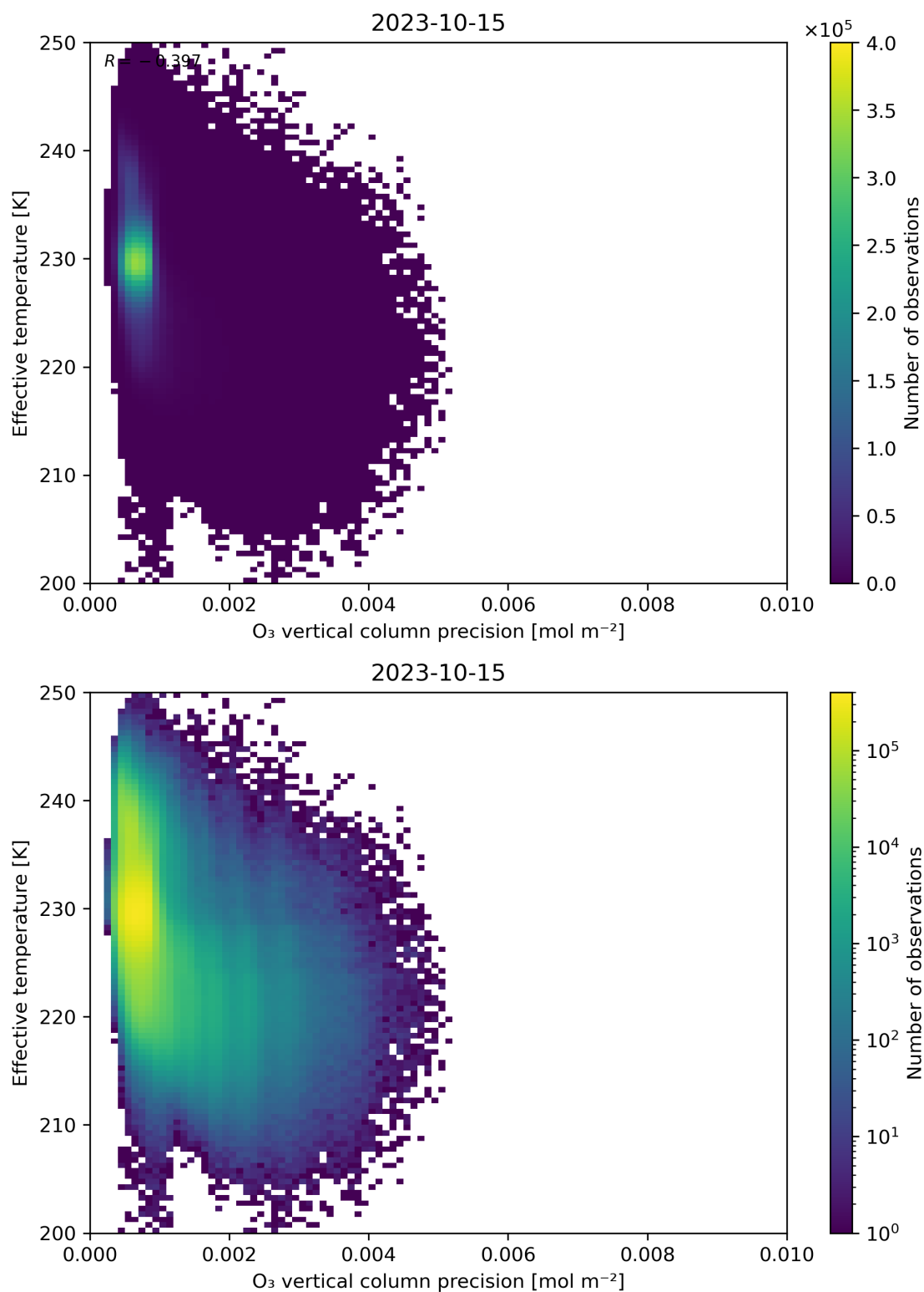
Figure 42: Scatter density plot of “O 3 vertical column precision” against “Effective temperature” for 2023-10-14 to 2023-10-16.
