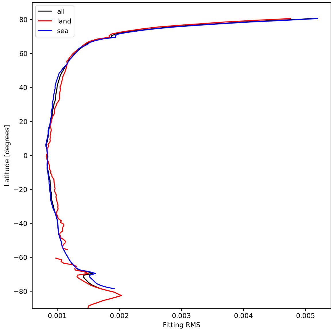
Figure 16: Zonal average of “Fitting RMS” for 2023-10-14 to 2023-10-16.
