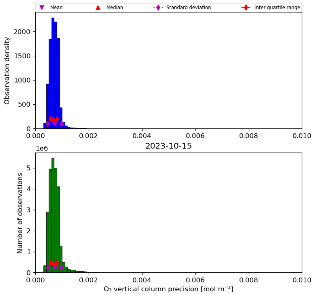
Figure 22: Histogram of “O 3 vertical column precision” for 2023-10-14 to 2023-10-16
