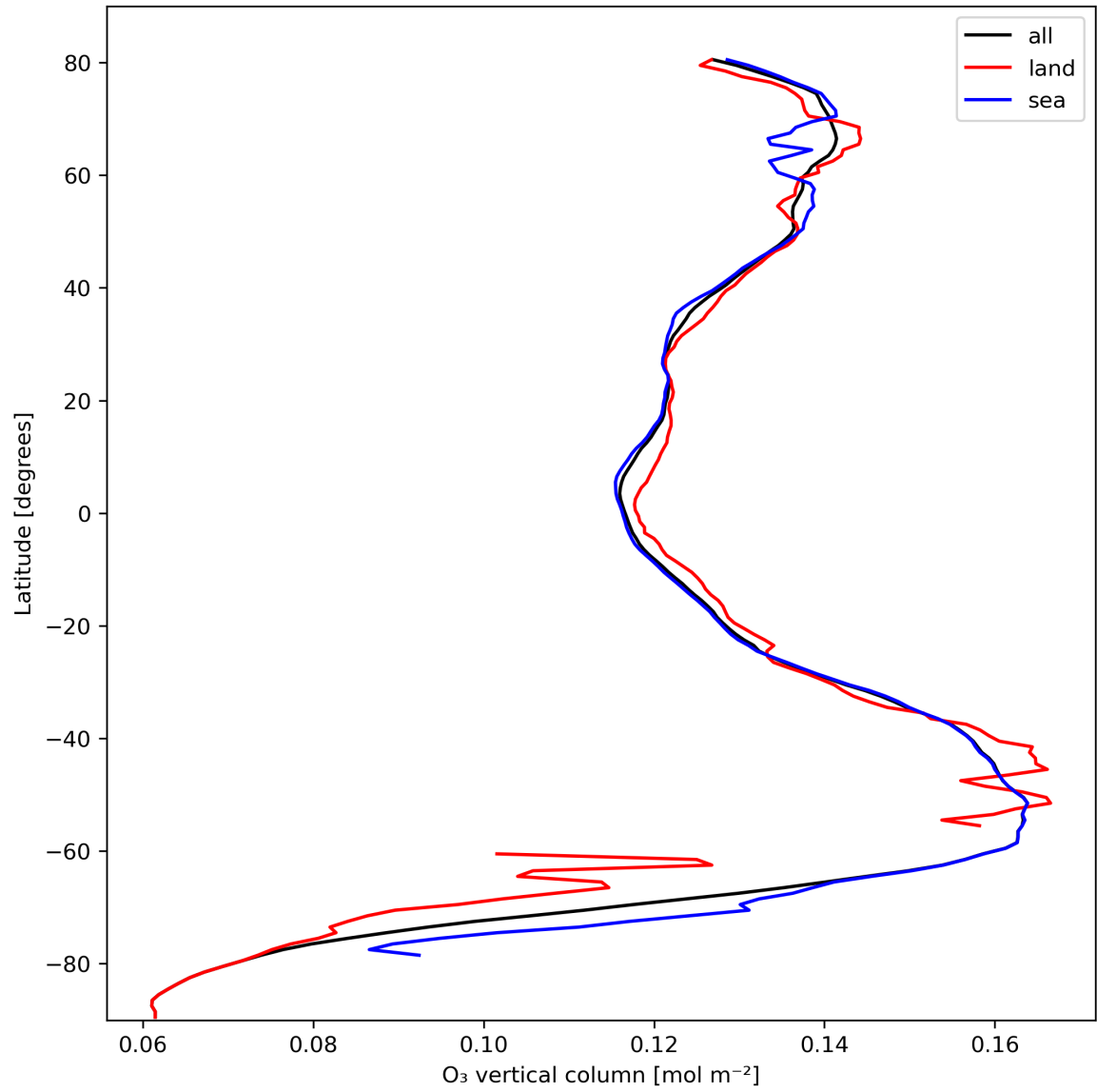
Figure 14: Zonal average of “O 3 vertical column” for 2023-10-14 to 2023-10-16.
