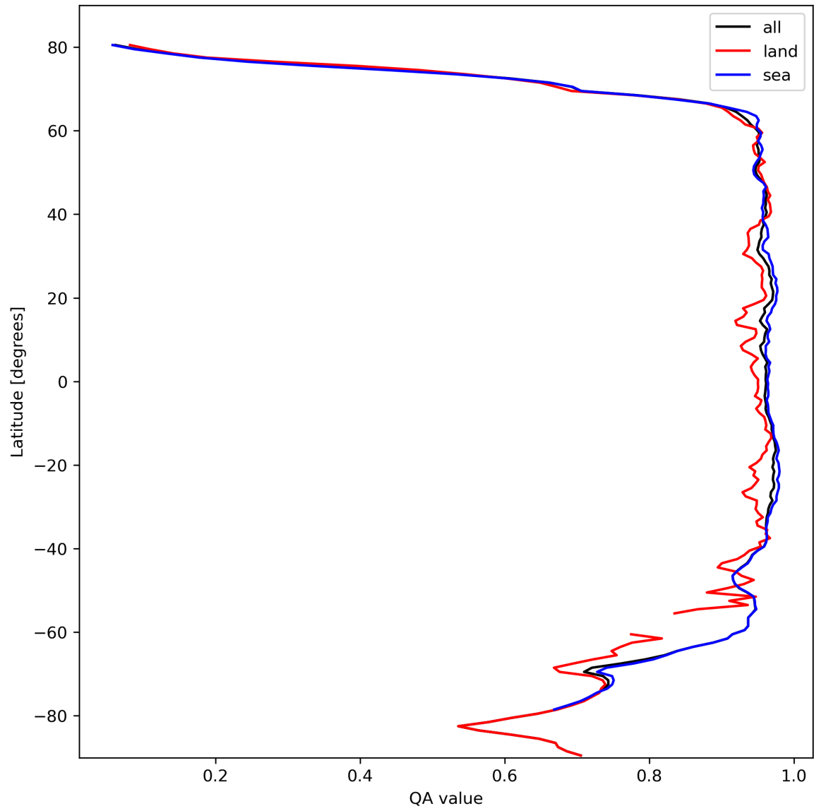
Figure 13: Zonal average of “QA value” for 2023-10-14 to 2023-10-16.
