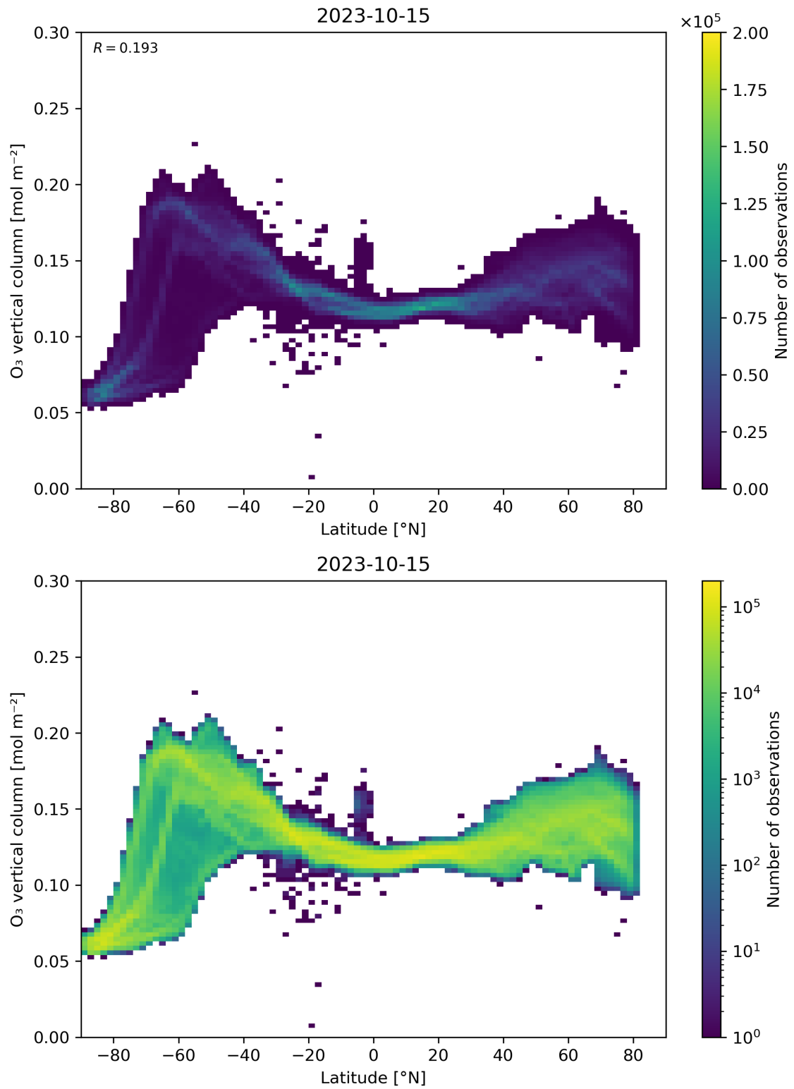
Figure 36: Scatter density plot of “Latitude” against “O 3 vertical column” for 2023-10-14 to 2023-10-16.
