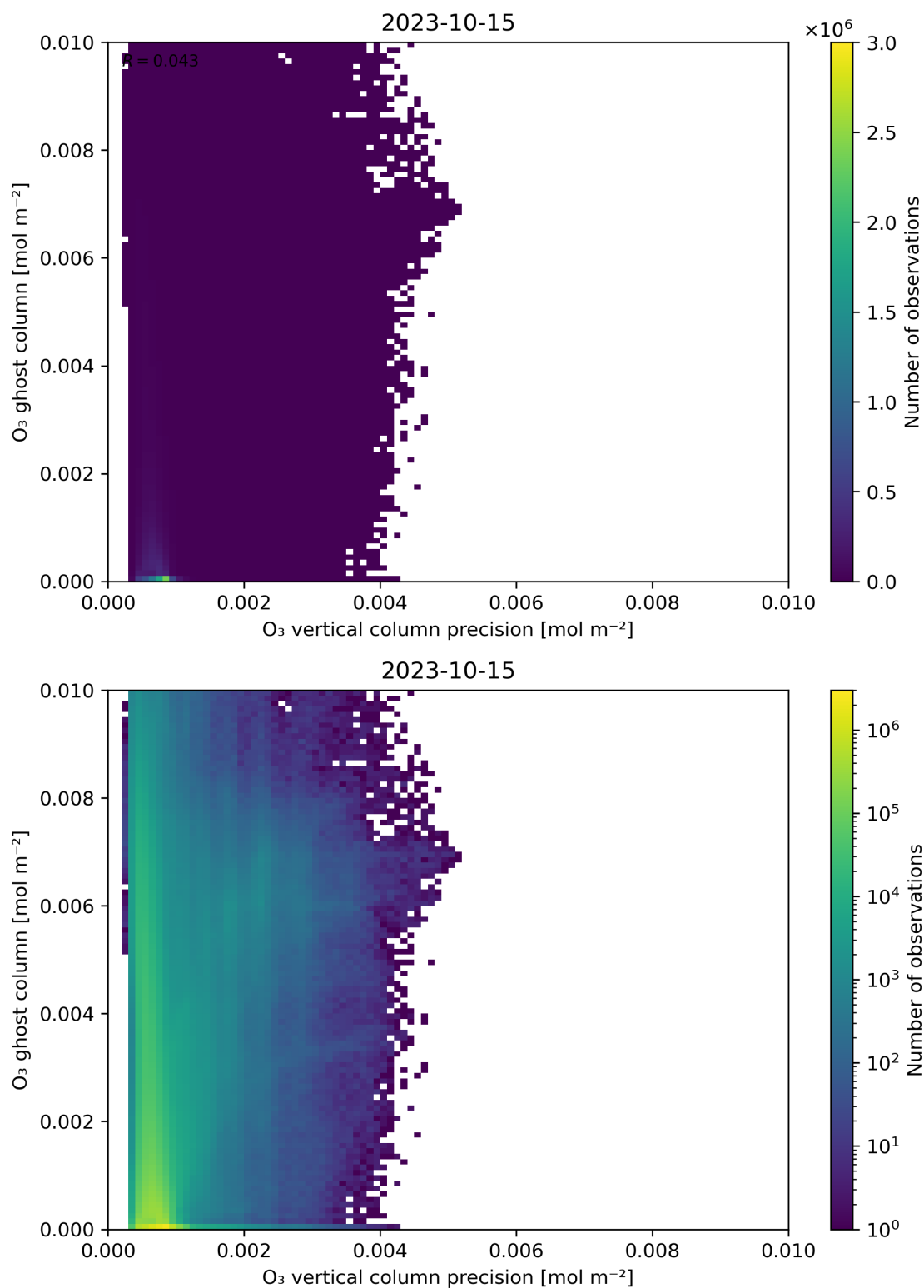
Figure 43: Scatter density plot of “O 3 vertical column precision” against “O 3 ghost column” for 2023-10-14 to 2023-10-16.
