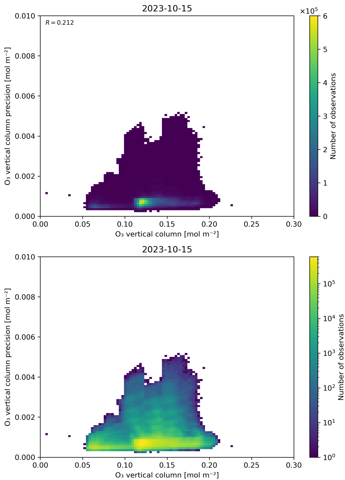
Figure 41: Scatter density plot of “O 3 vertical column” against “O 3 vertical column precision” for 2023-10-14 to 2023-10-16.
