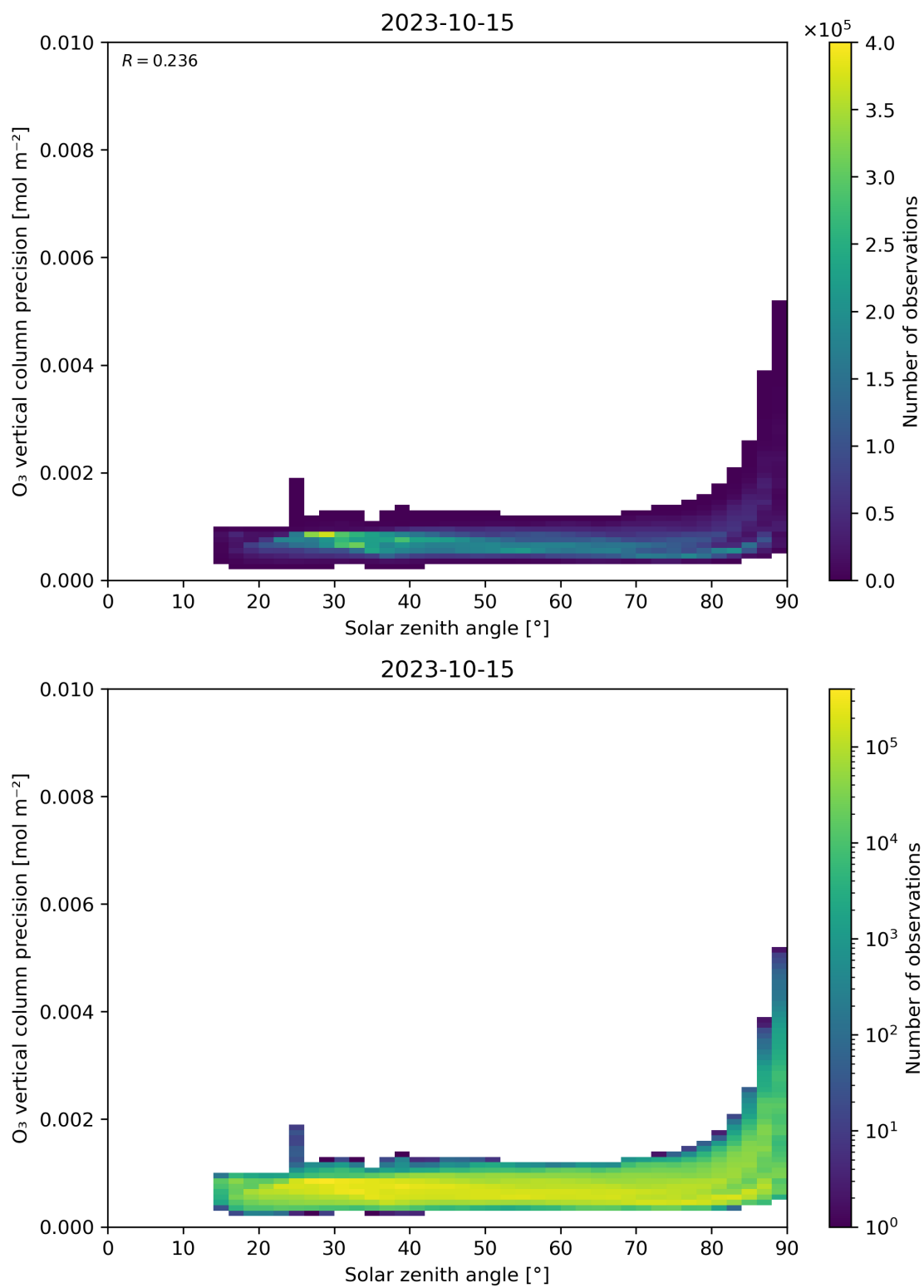
Figure 48: Scatter density plot of “Solar zenith angle” against “O 3 vertical column precision” for 2023-10-14 to 2023-10-16.
