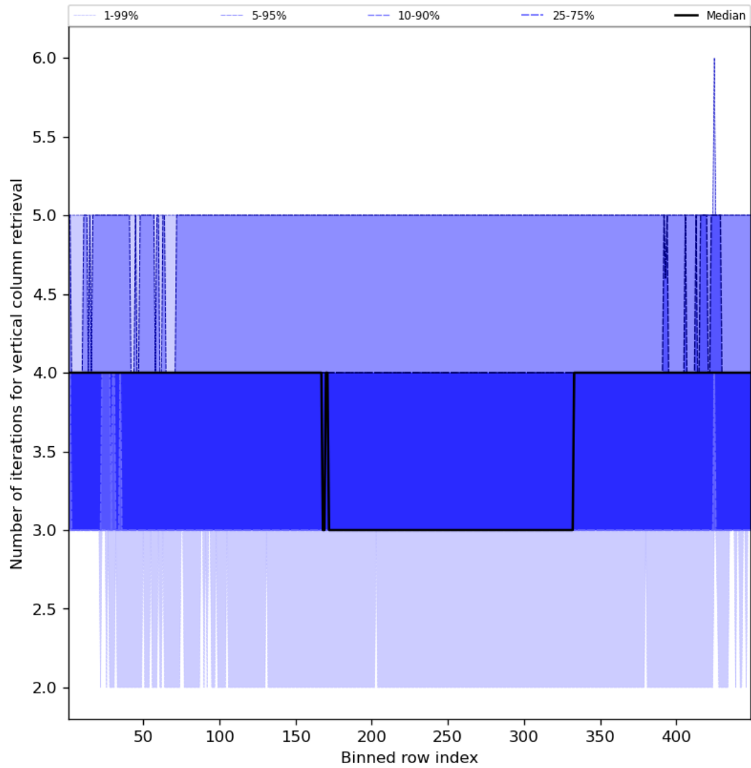
Figure 33: Along track statistics of “Number of iterations for vertical column retrieval” for 2023-10-14 to 2023-10-16
