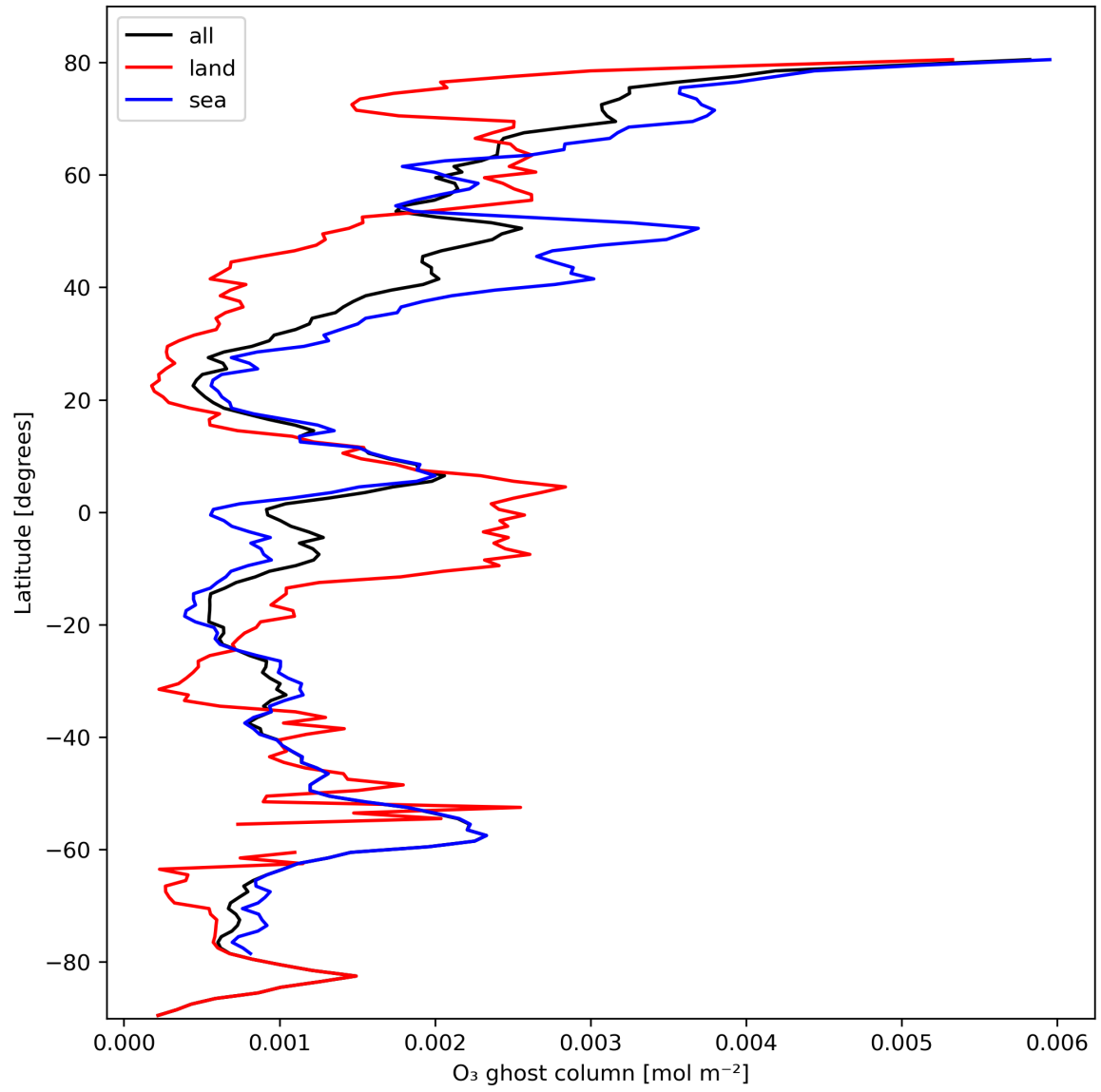
Figure 18: Zonal average of "O 3 ghost column" for 2023-10-14 to 2023-10-16.
