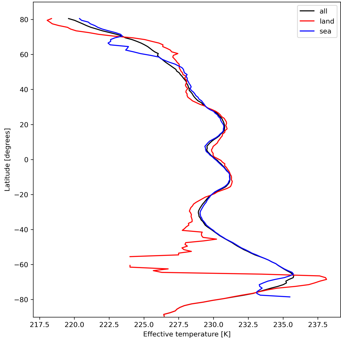
Figure 17: Zonal average of “Effective temperature” for 2023-10-14 to 2023-10-16.
