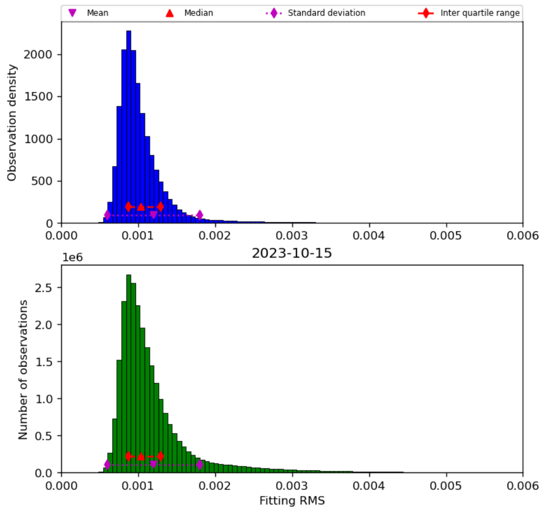
Figure 23: Histogram of “Fitting RMS” for 2023-10-14 to 2023-10-16
