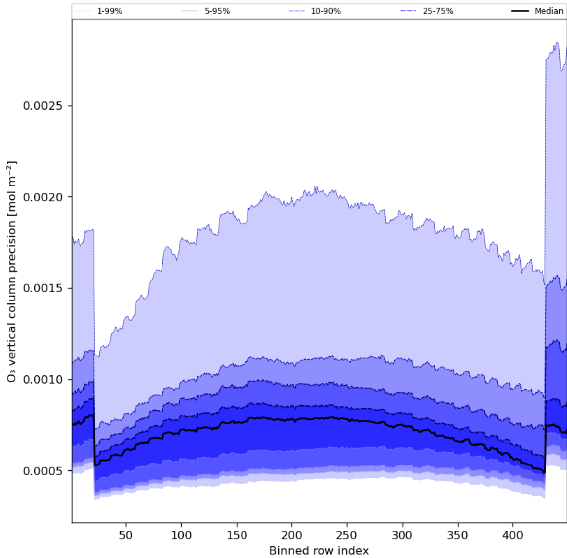
Figure 29: Along track statistics of “O 3 vertical column precision” for 2023-10-14 to 2023-10-16
