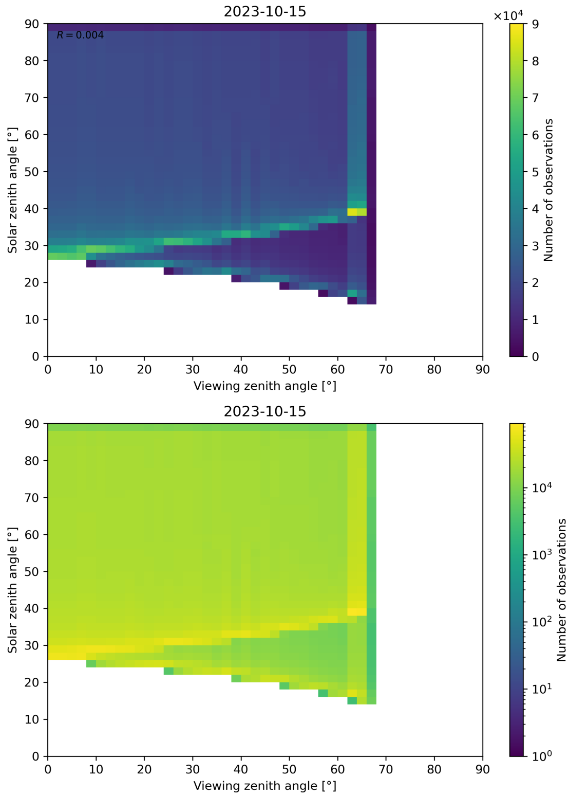
Figure 54: Scatter density plot of “Viewing zenith angle” against “Solar zenith angle” for 2023-10-14 to 2023-10-16.
