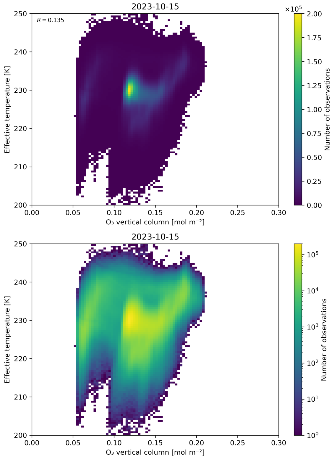
Figure 39: Scatter density plot of “O 3 vertical column” against “Effective temperature” for 2023-10-14 to 2023-10-16.
