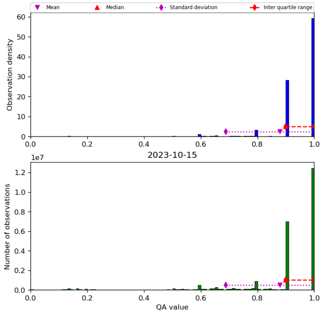
Figure 20: Histogram of “QA value” for 2023-10-14 to 2023-10-16
