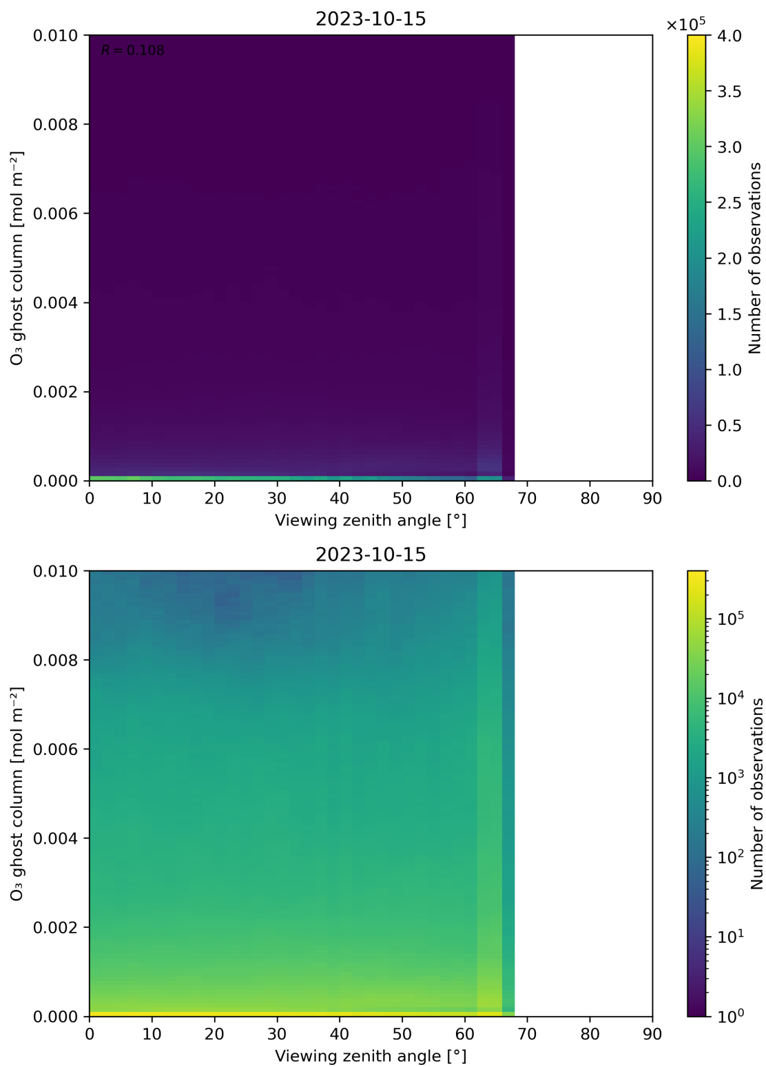
Figure 51: Scatter density plot of “Viewing zenith angle” against “O 3 ghost column” for 2023-10-14 to 2023-10-16.
