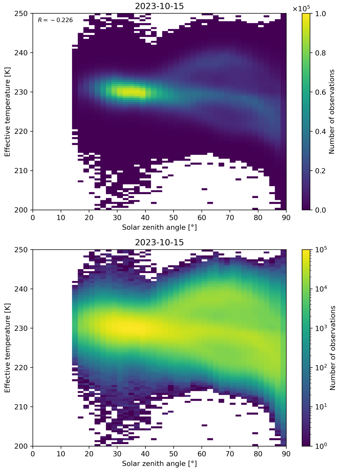
Figure 45: Scatter density plot of “Solar zenith angle” against “Effective temperature” for 2023-10-14 to 2023-10-16.
