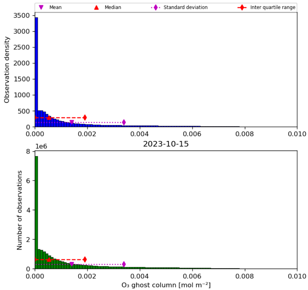
Figure 25: Histogram of “O 3 ghost column” for 2023-10-14 to 2023-10-16
