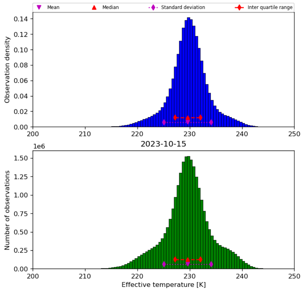
Figure 24: Histogram of “Effective temperature” for 2023-10-14 to 2023-10-16
