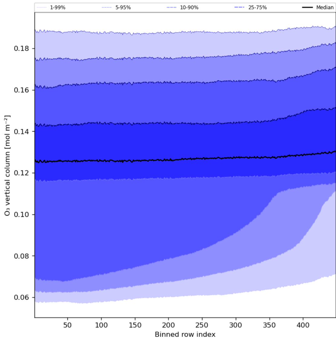
Figure 28: Along track statistics of “O 3 vertical column” for 2023-10-14 to 2023-10-16
