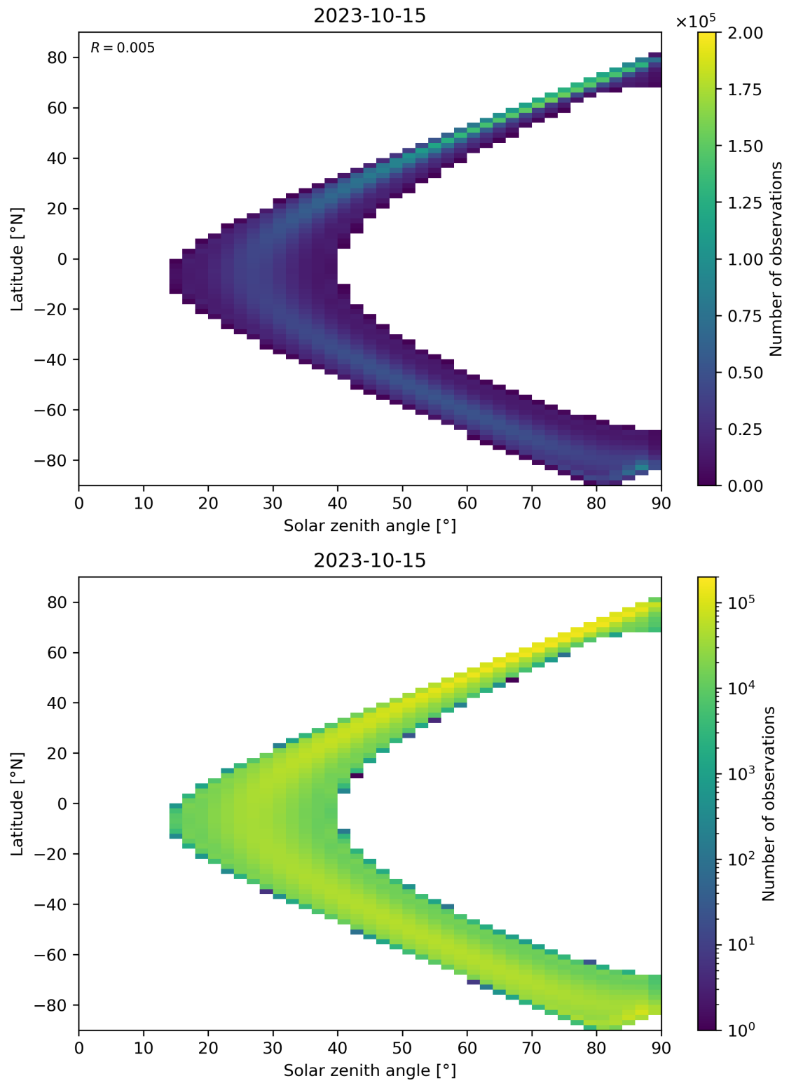
Figure 44: Scatter density plot of “Solar zenith angle” against “Latitude” for 2023-10-14 to 2023-10-16.
