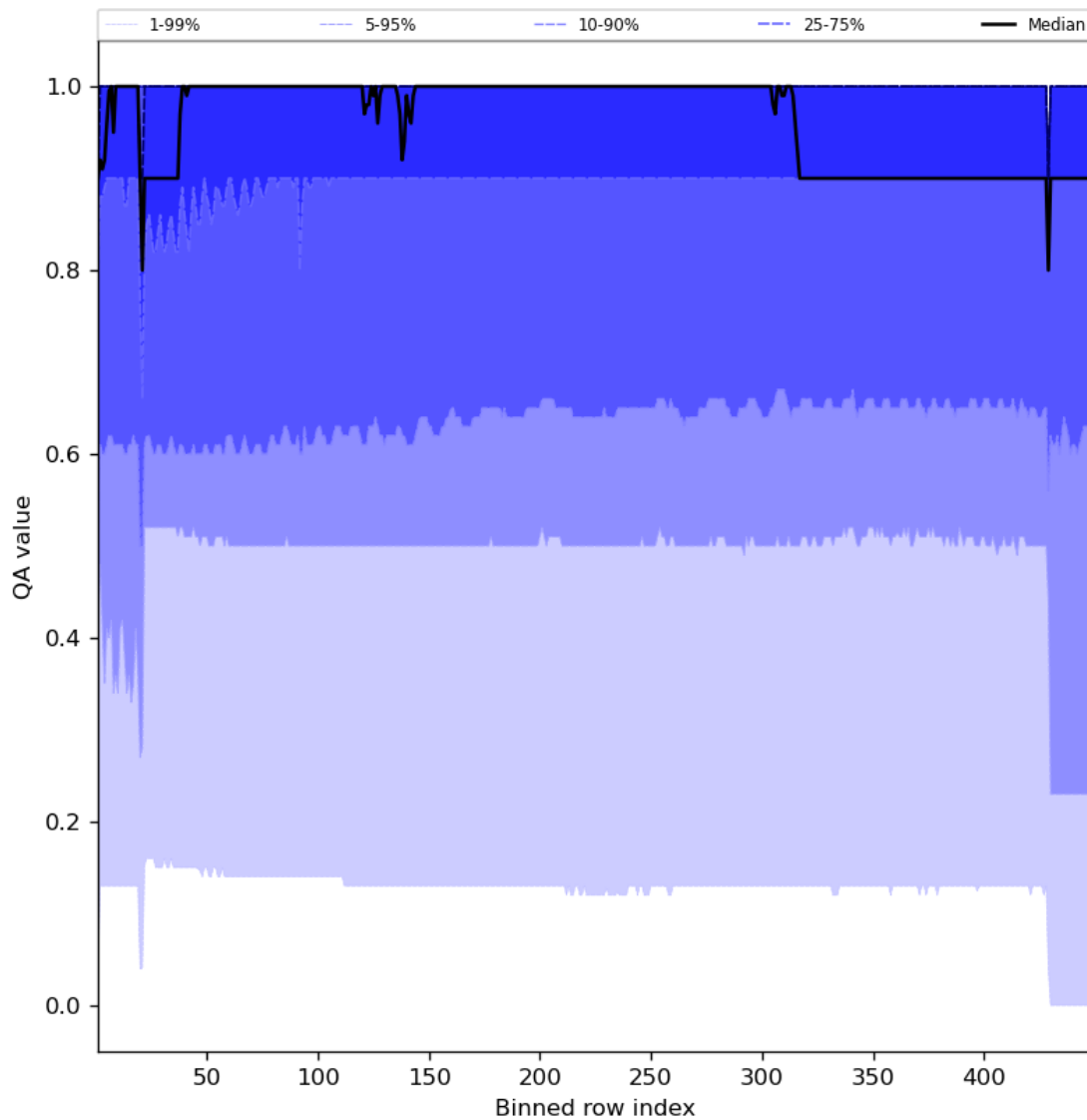
Figure 27: Along track statistics of “QA value” for 2023-10-14 to 2023-10-16
