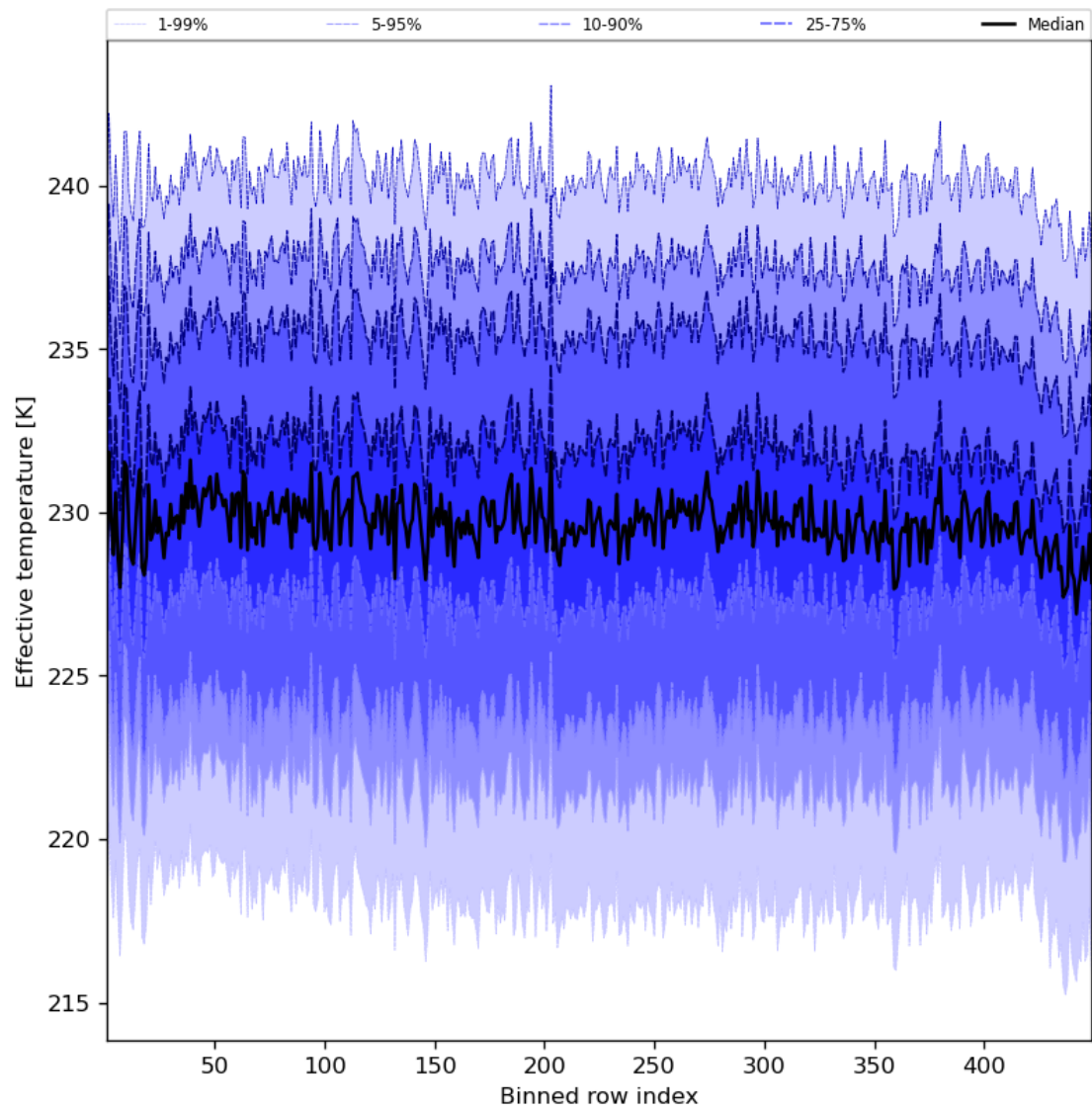
Figure 31: Along track statistics of “Effective temperature” for 2023-10-14 to 2023-10-16
