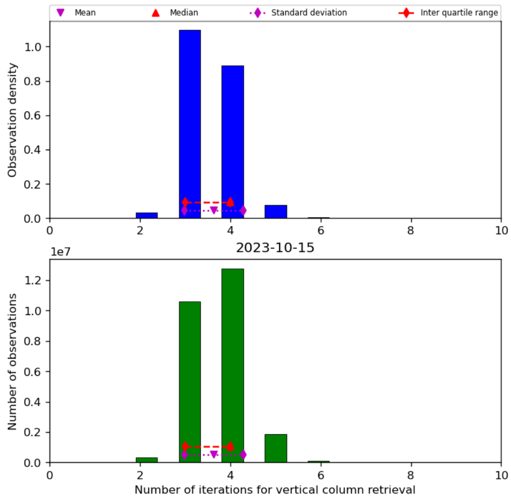
Figure 26: Histogram of “Number of iterations for vertical column retrieval” for 2023-10-14 to 2023-10-16
