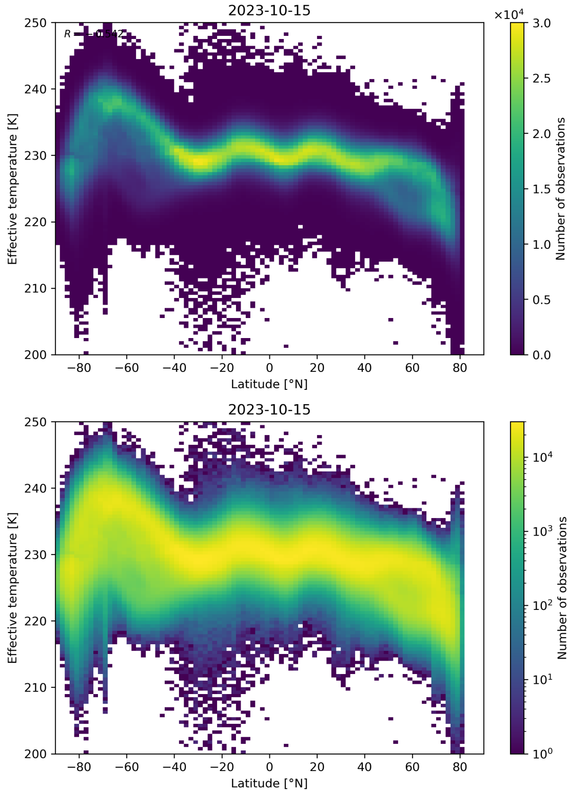
Figure 34: Scatter density plot of “Latitude” against “Effective temperature” for 2023-10-14 to 2023-10-16.
