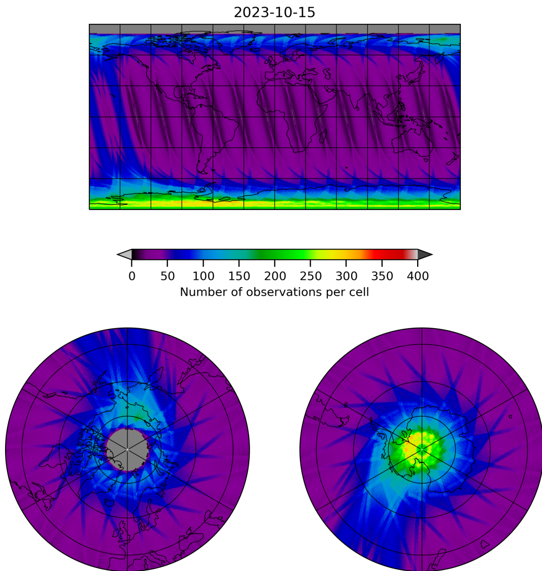
Figure 12: Map of the number of observations for 2023-10-14 to 2023-10-16
