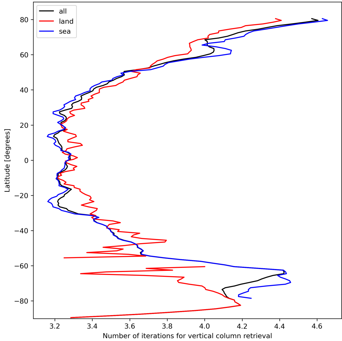
Figure 19: Zonal average of “Number of iterations for vertical column retrieval” for 2023-10-14 to 2023-10-16.
