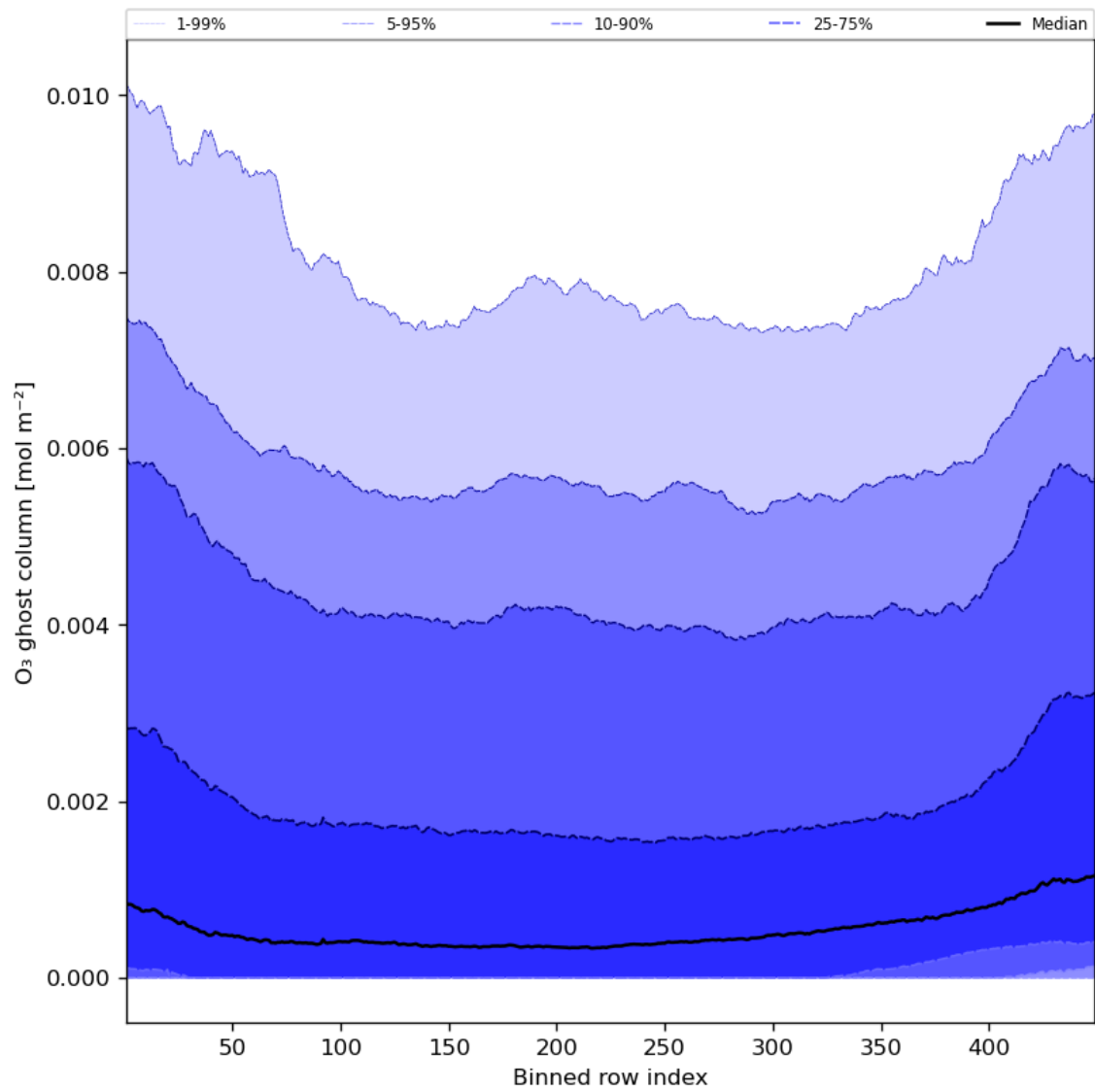
Figure 32: Along track statistics of “O 3 ghost column” for 2023-10-14 to 2023-10-16
