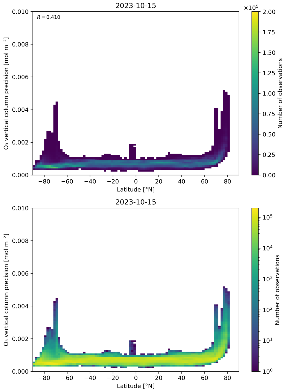
Figure 37: Scatter density plot of “Latitude” against “O 3 vertical column precision” for 2023-10-14 to 2023-10-16.
