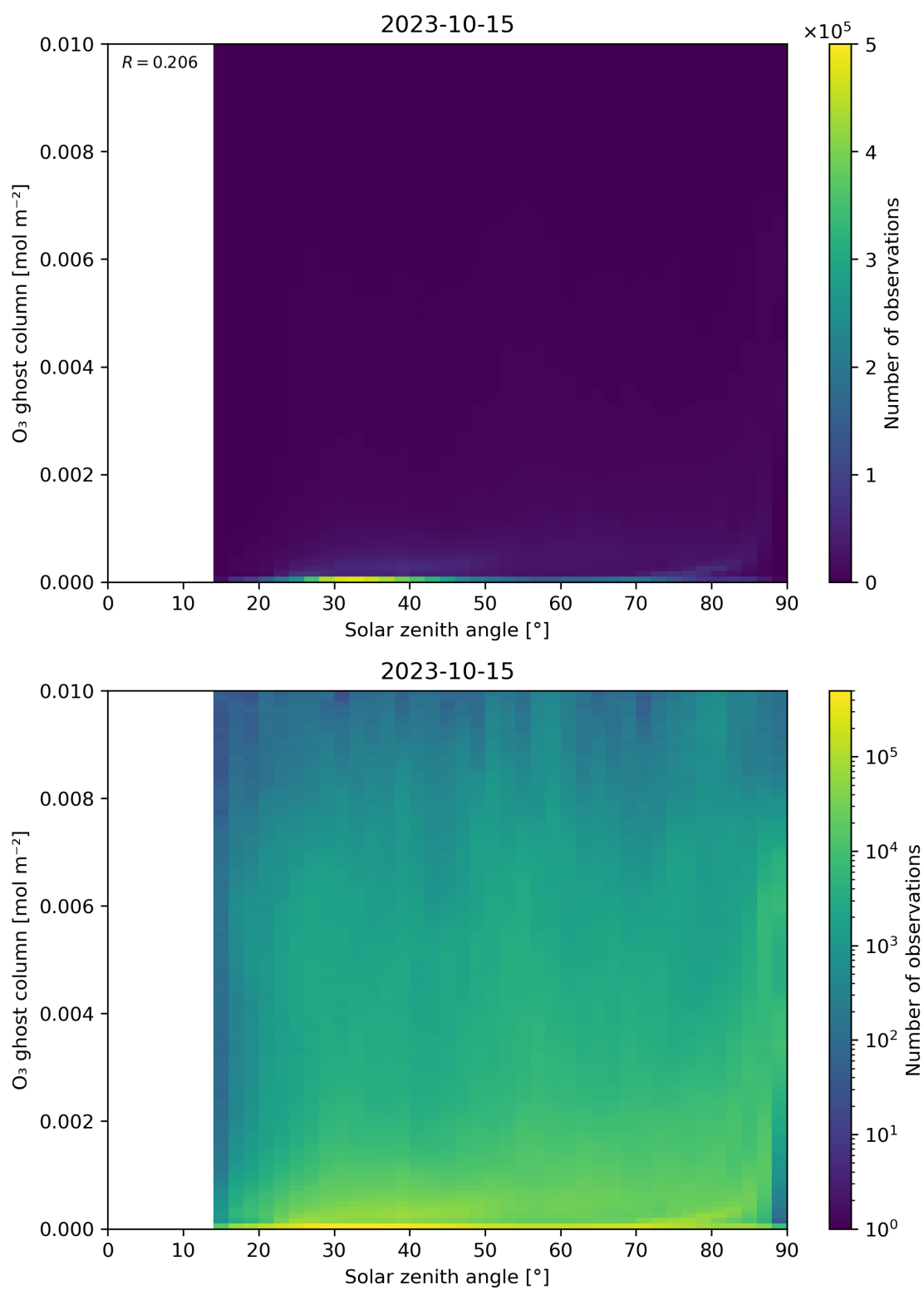
Figure 46: Scatter density plot of “Solar zenith angle” against “O 3 ghost column” for 2023-10-14 to 2023-10-16.
