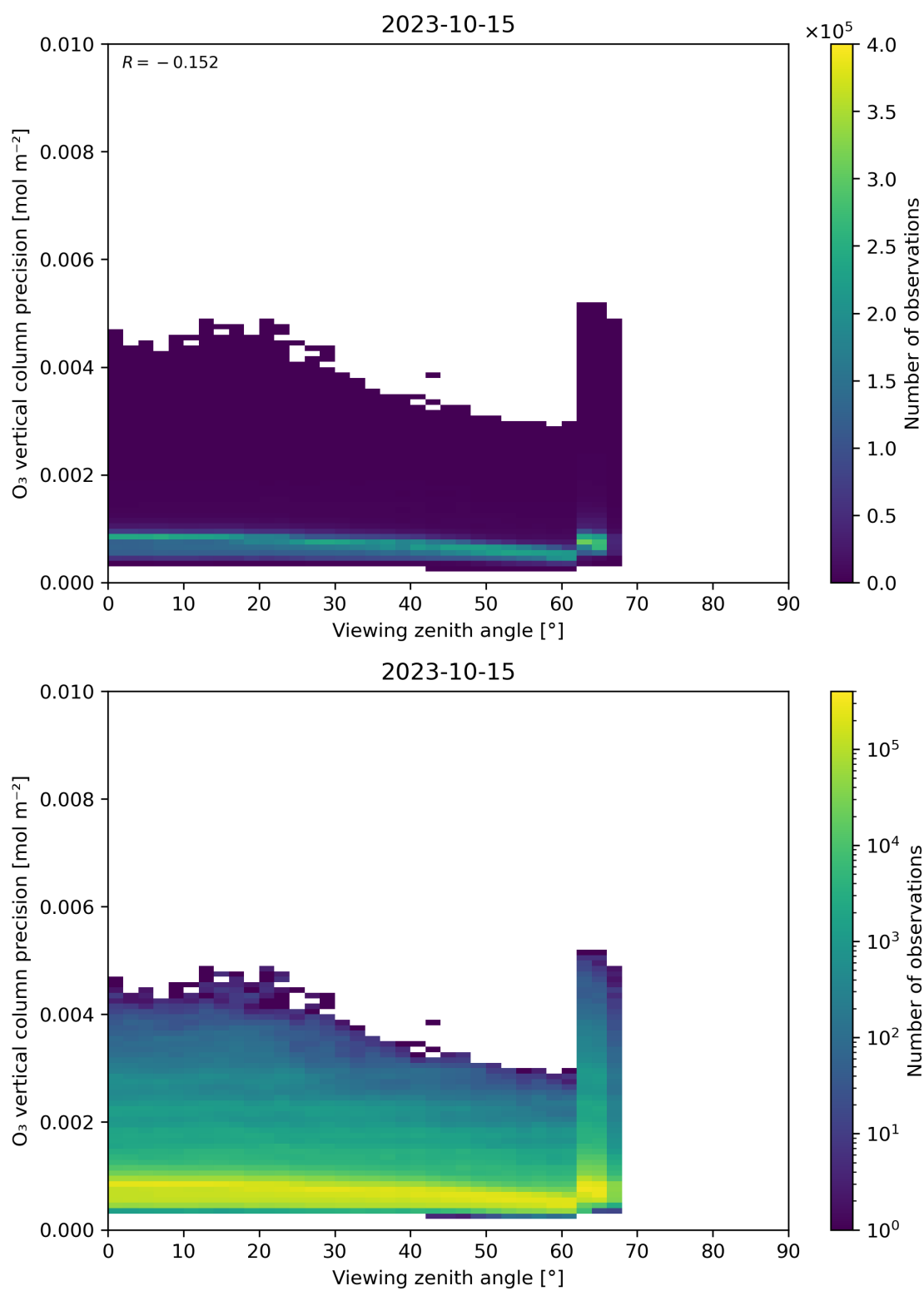
Figure 53: Scatter density plot of “Viewing zenith angle” against “O 3 vertical column precision” for 2023-10-14 to 2023-10-16.
