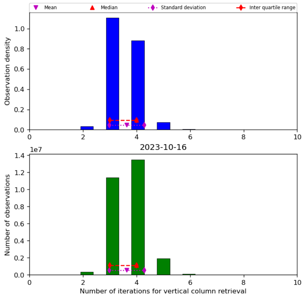
Figure 26: Histogram of “Number of iterations for vertical column retrieval” for 2023-10-15 to 2023-10-17
