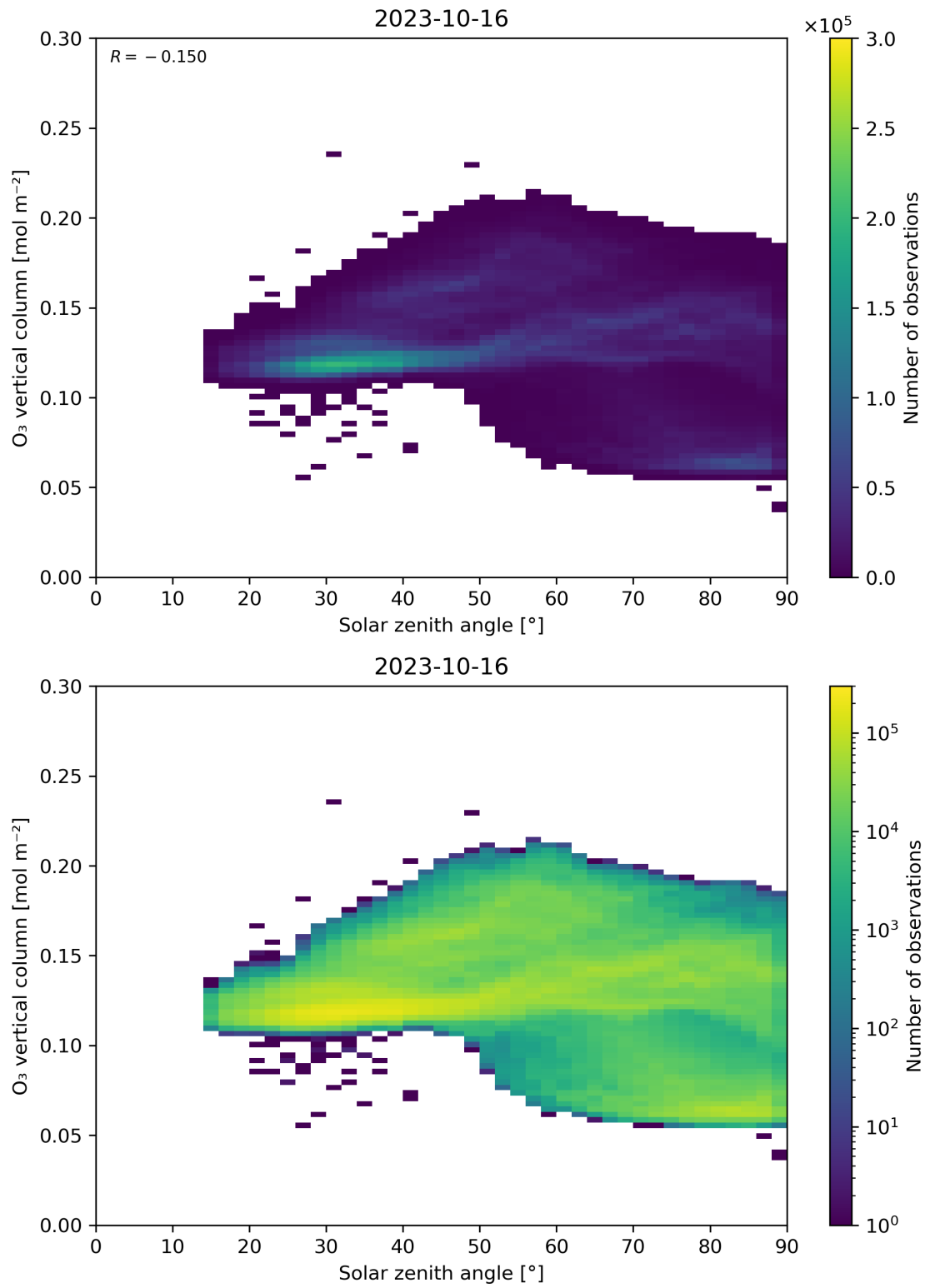
Figure 47: Scatter density plot of “Solar zenith angle” against “O 3 vertical column” for 2023-10-15 to 2023-10-17.
