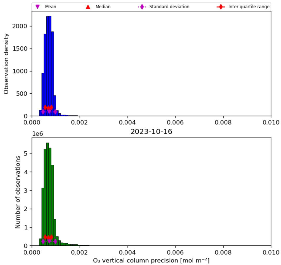
Figure 22: Histogram of “O 3 vertical column precision” for 2023-10-15 to 2023-10-17
