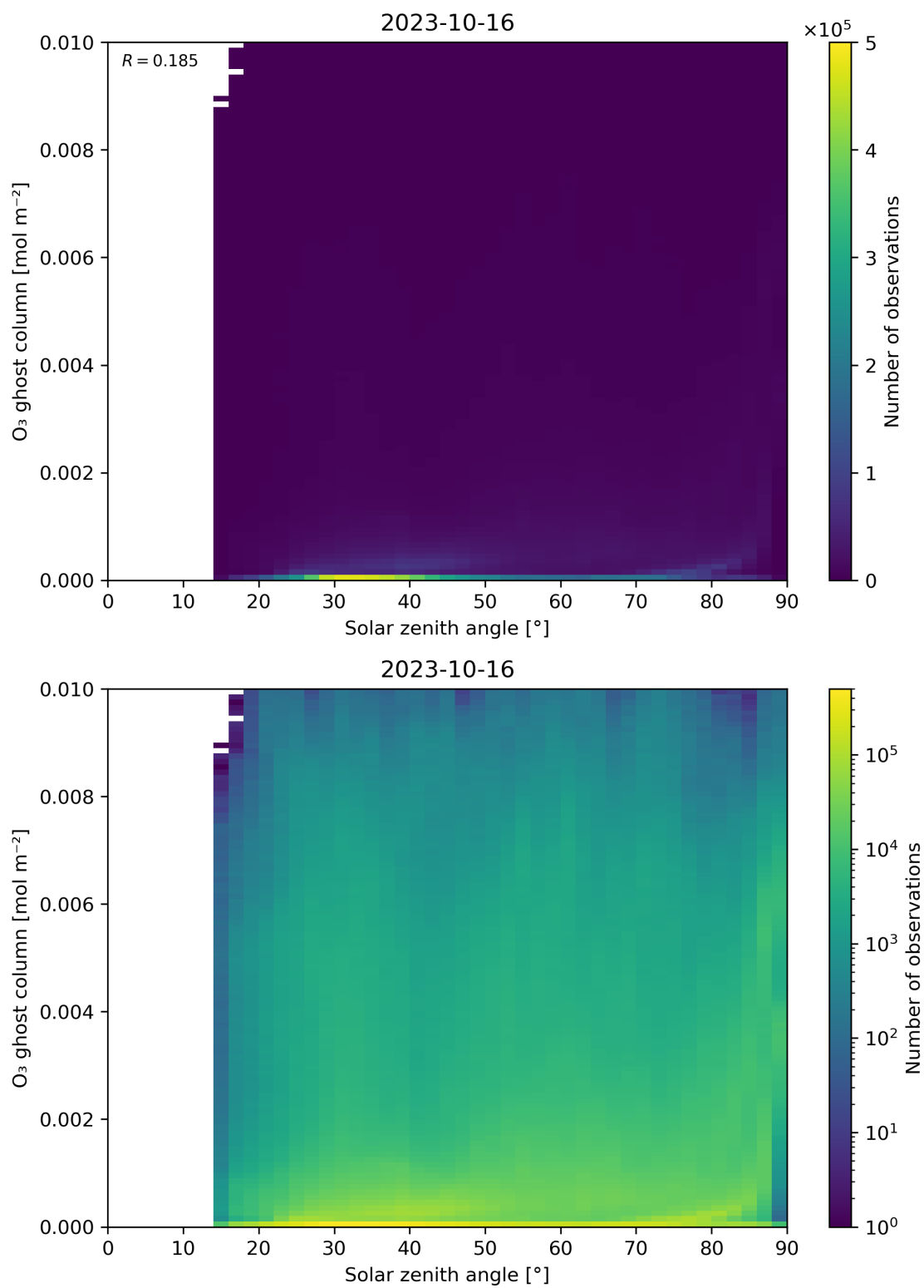
Figure 46: Scatter density plot of “Solar zenith angle” against “O 3 ghost column” for 2023-10-15 to 2023-10-17.
