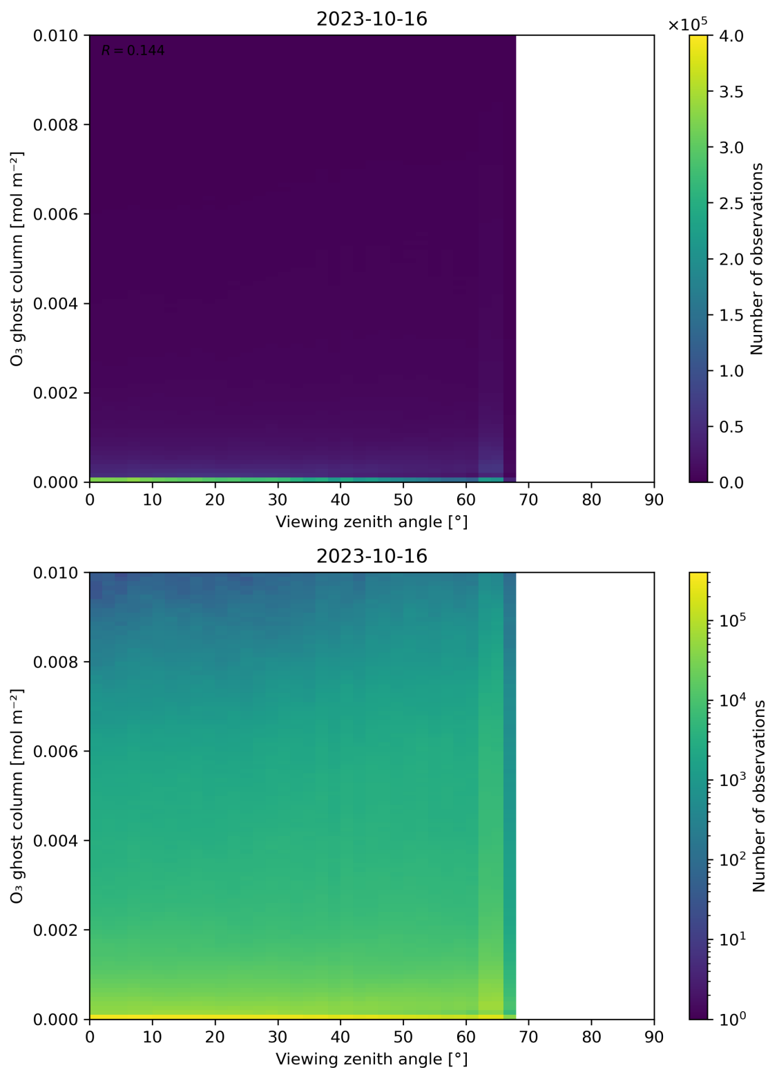
Figure 51: Scatter density plot of “Viewing zenith angle” against “O 3 ghost column” for 2023-10-15 to 2023-10-17.
