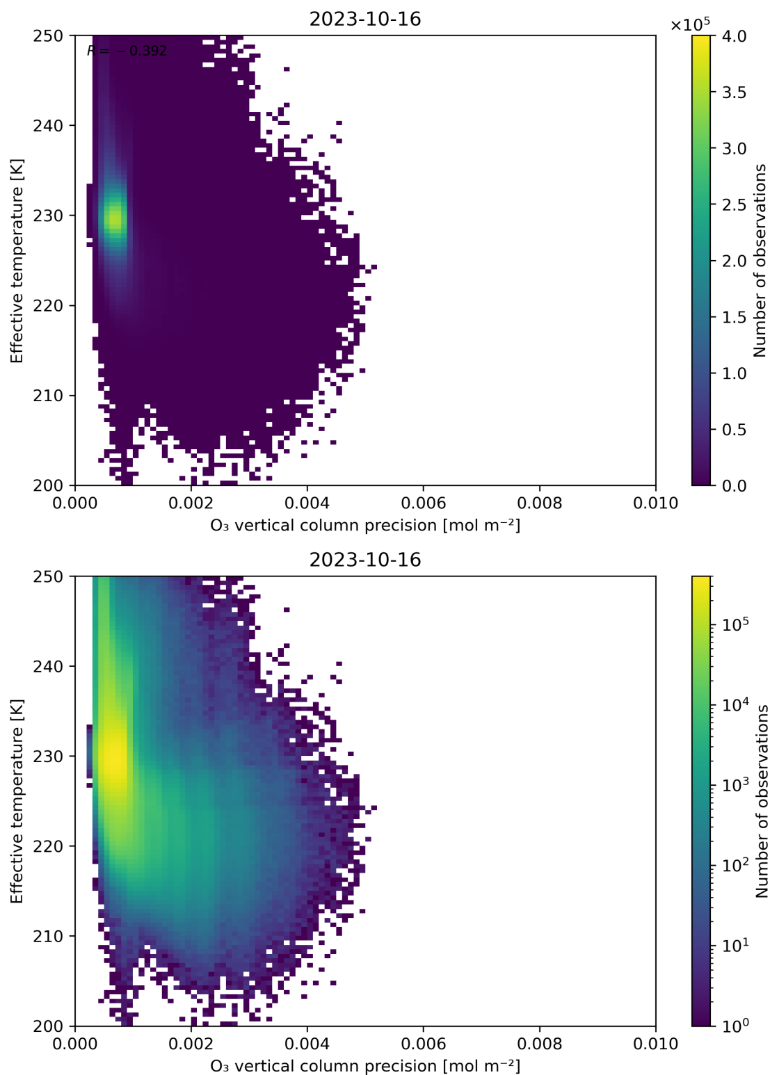
Figure 42: Scatter density plot of “O 3 vertical column precision” against “Effective temperature” for 2023-10-15 to 2023-10-17.
