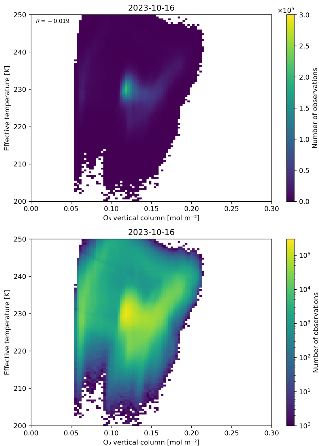
Figure 39: Scatter density plot of “O 3 vertical column” against “Effective temperature” for 2023-10-15 to 2023-10-17.
