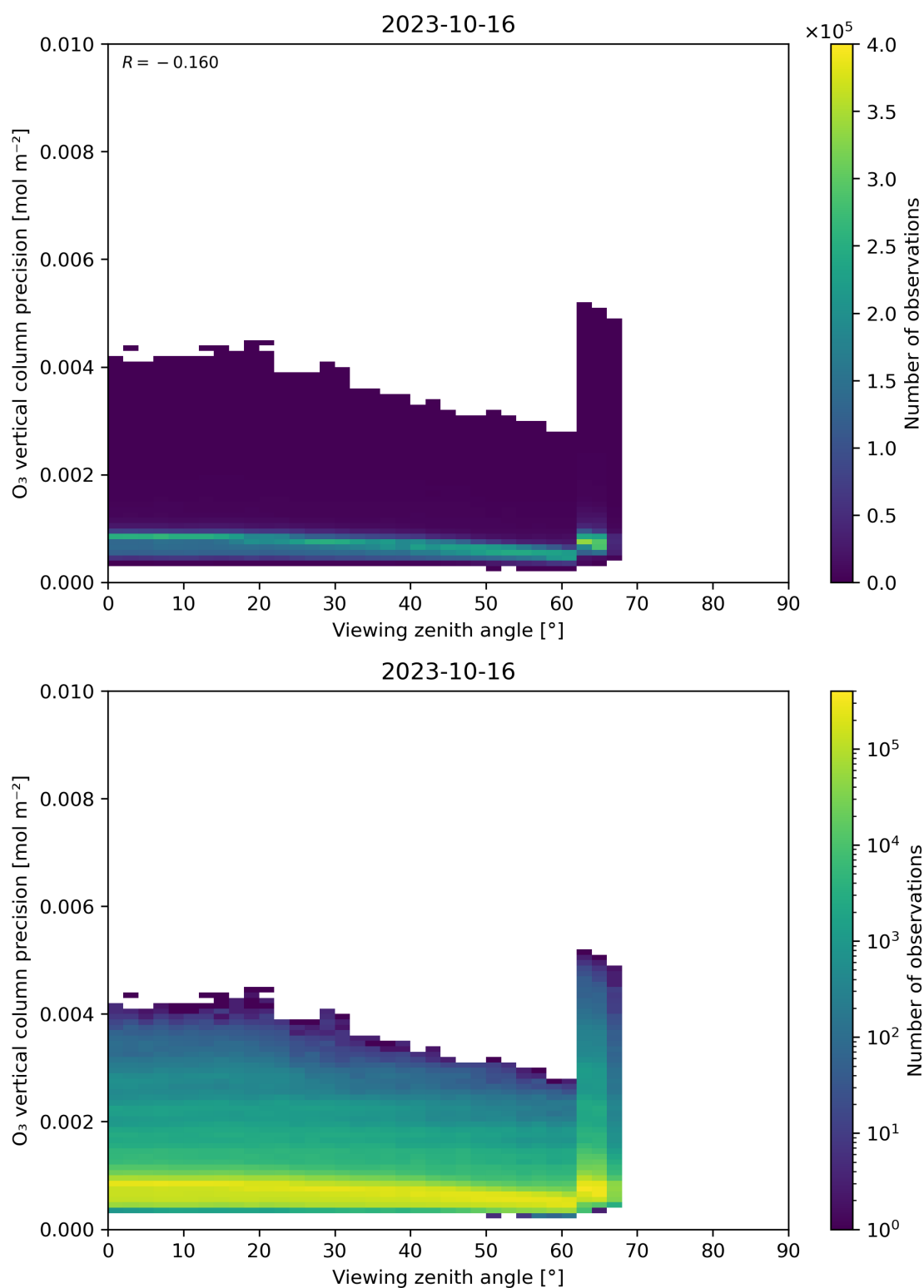
Figure 53: Scatter density plot of “Viewing zenith angle” against “O 3 vertical column precision” for 2023-10-15 to 2023-10-17.
