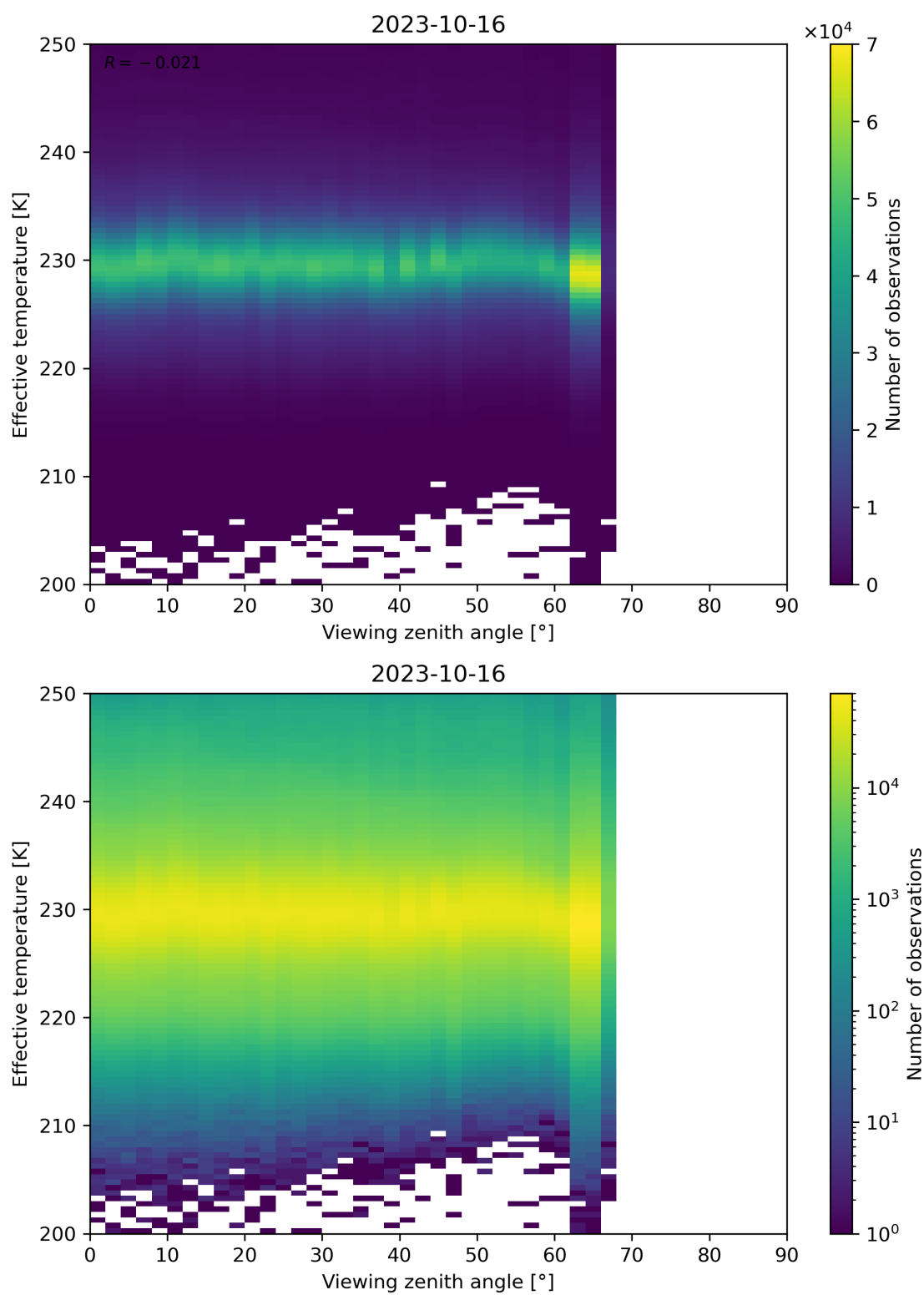
Figure 50: Scatter density plot of “Viewing zenith angle” against “Effective temperature” for 2023-10-15 to 2023-10-17.
