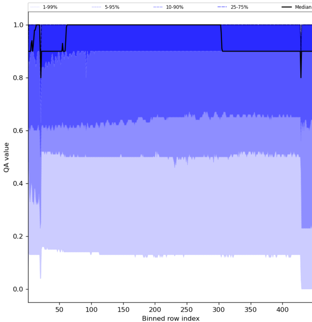
Figure 27: Along track statistics of “QA value” for 2023-10-15 to 2023-10-17
