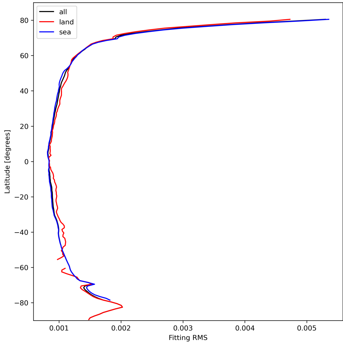
Figure 16: Zonal average of “Fitting RMS” for 2023-10-15 to 2023-10-17.
