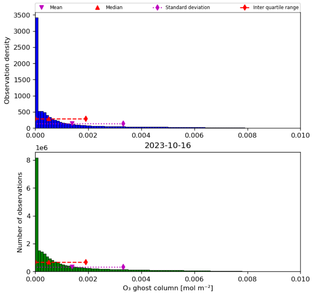
Figure 25: Histogram of “O 3 ghost column” for 2023-10-15 to 2023-10-17
