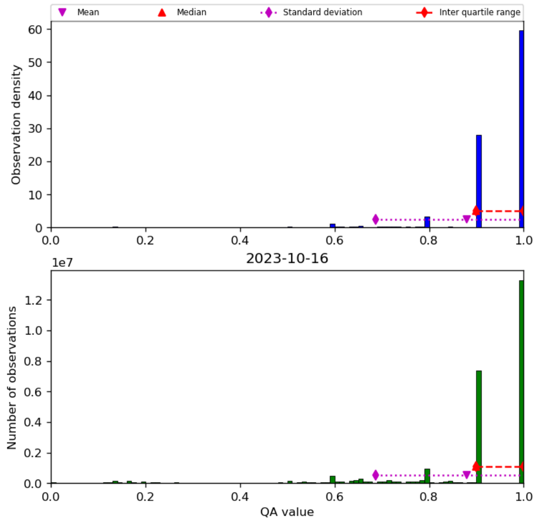
Figure 20: Histogram of “QA value” for 2023-10-15 to 2023-10-17
