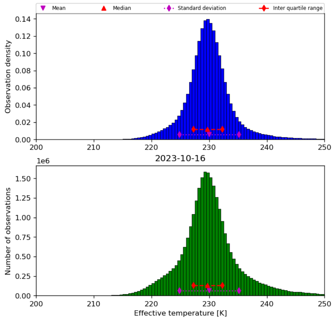
Figure 24: Histogram of “Effective temperature” for 2023-10-15 to 2023-10-17
