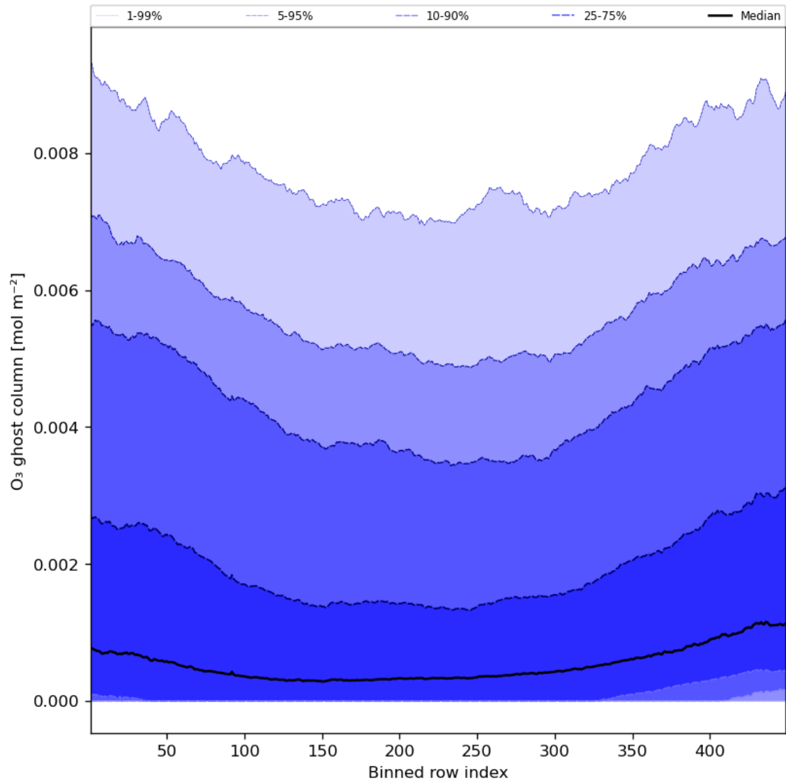
Figure 32: Along track statistics of “O 3 ghost column” for 2023-10-15 to 2023-10-17
