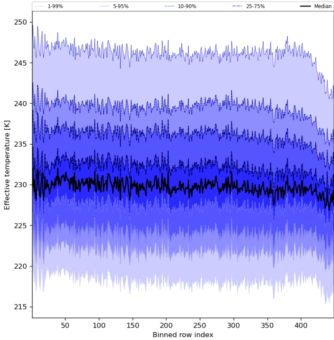
Figure 31: Along track statistics of “Effective temperature” for 2023-10-15 to 2023-10-17
