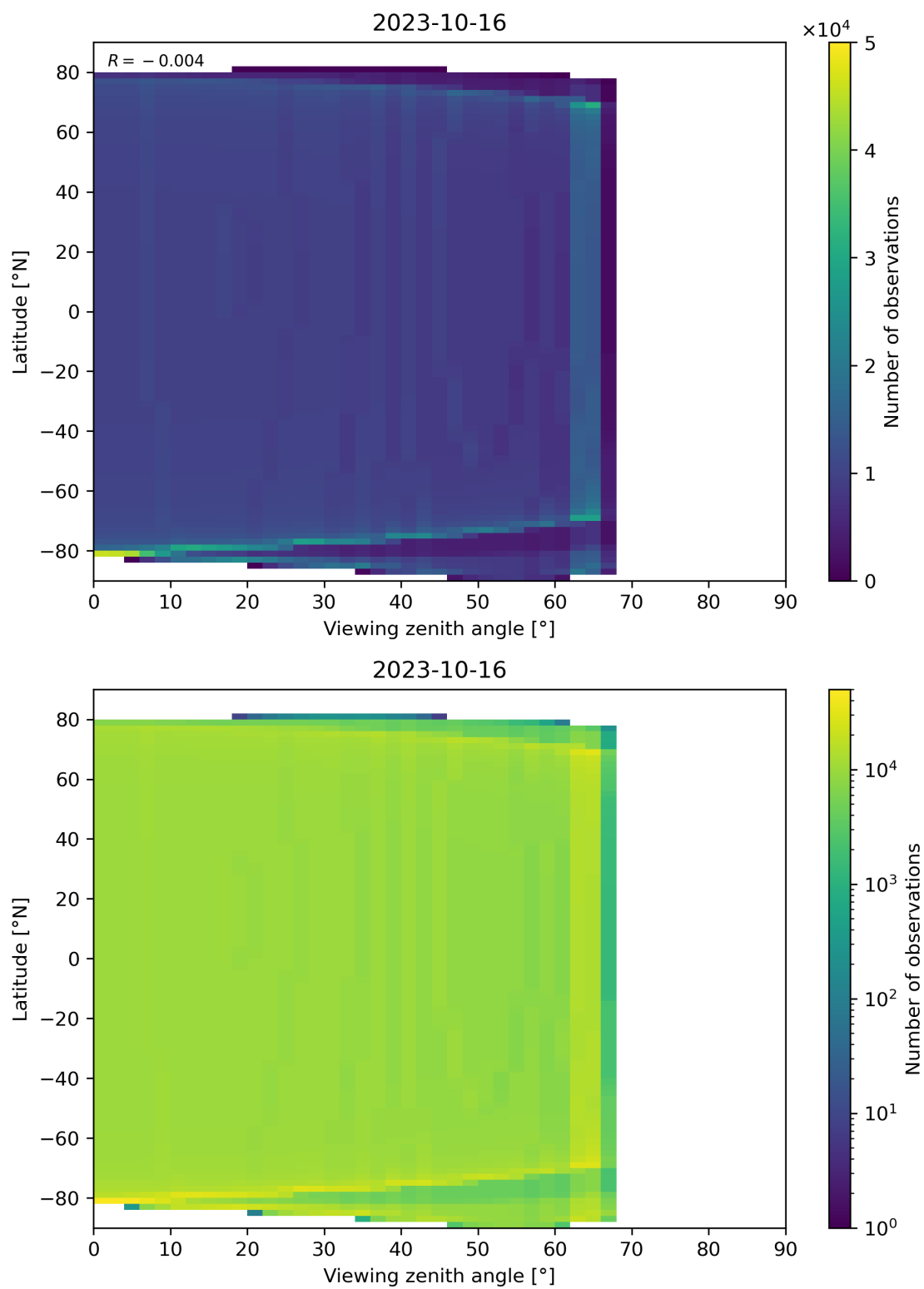
Figure 49: Scatter density plot of “Viewing zenith angle” against “Latitude” for 2023-10-15 to 2023-10-17.
