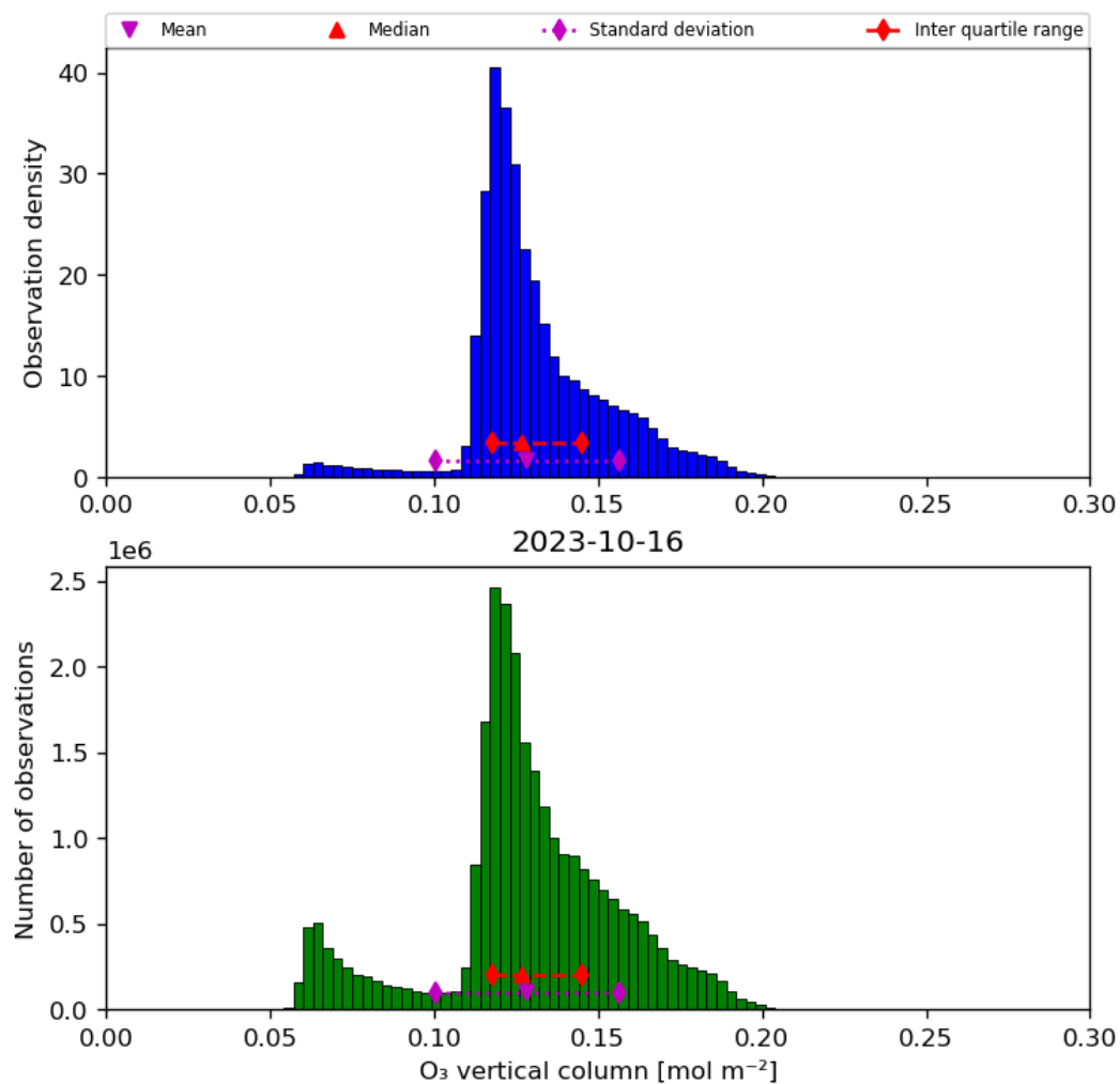
Figure 21: Histogram of “O 3 vertical column” for 2023-10-15 to 2023-10-17
