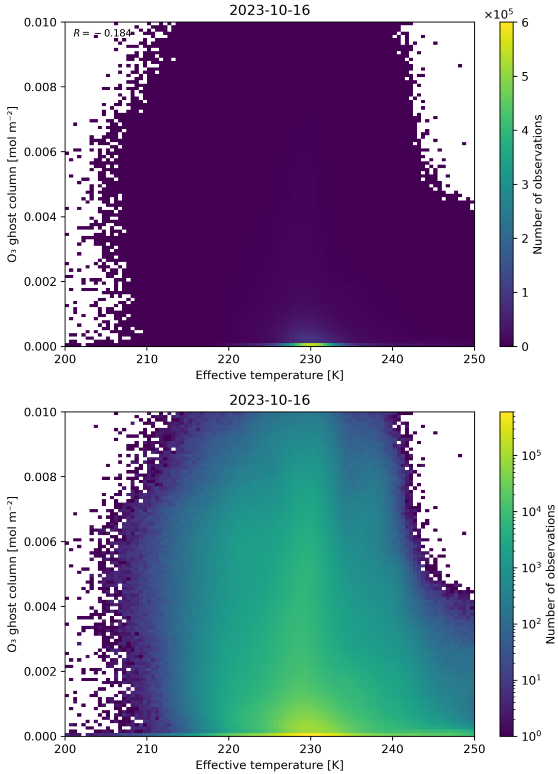
Figure 38: Scatter density plot of “Effective temperature” against “O 3 ghost column” for 2023-10-15 to 2023-10-17.
