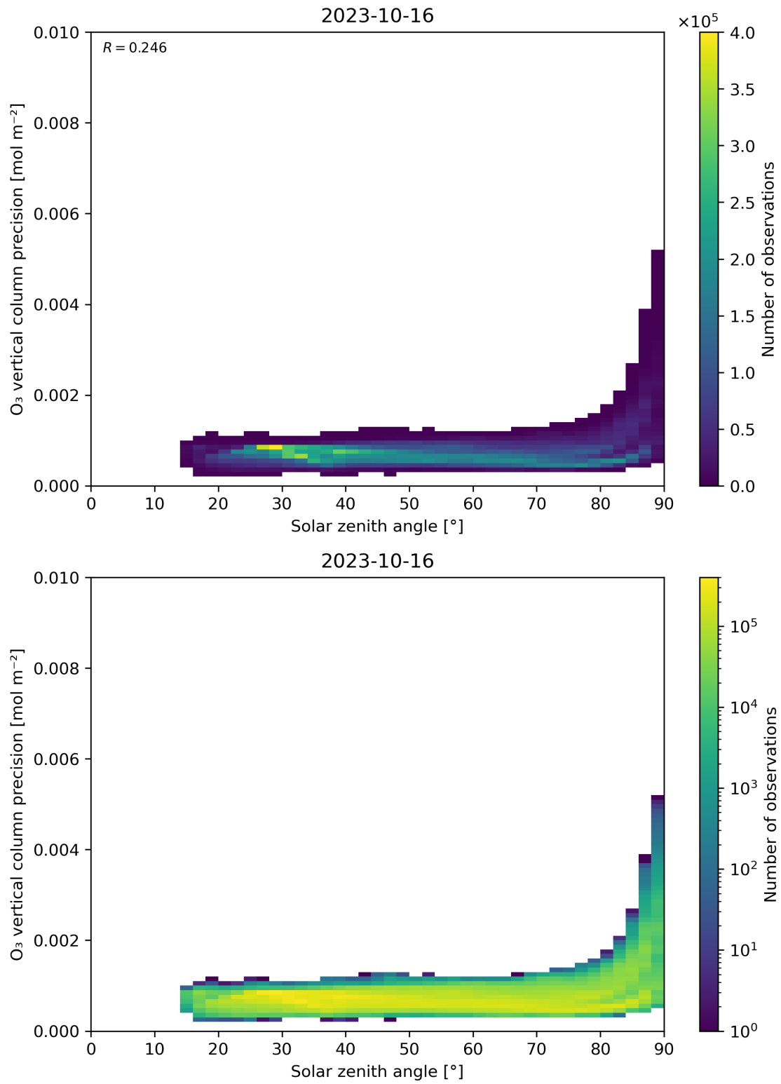
Figure 48: Scatter density plot of “Solar zenith angle” against “O 3 vertical column precision” for 2023-10-15 to 2023-10-17.
