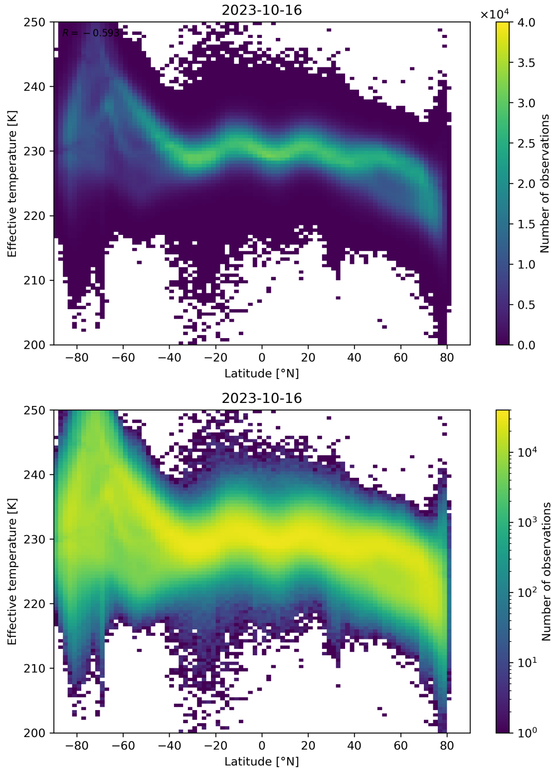
Figure 34: Scatter density plot of “Latitude” against “Effective temperature” for 2023-10-15 to 2023-10-17.
