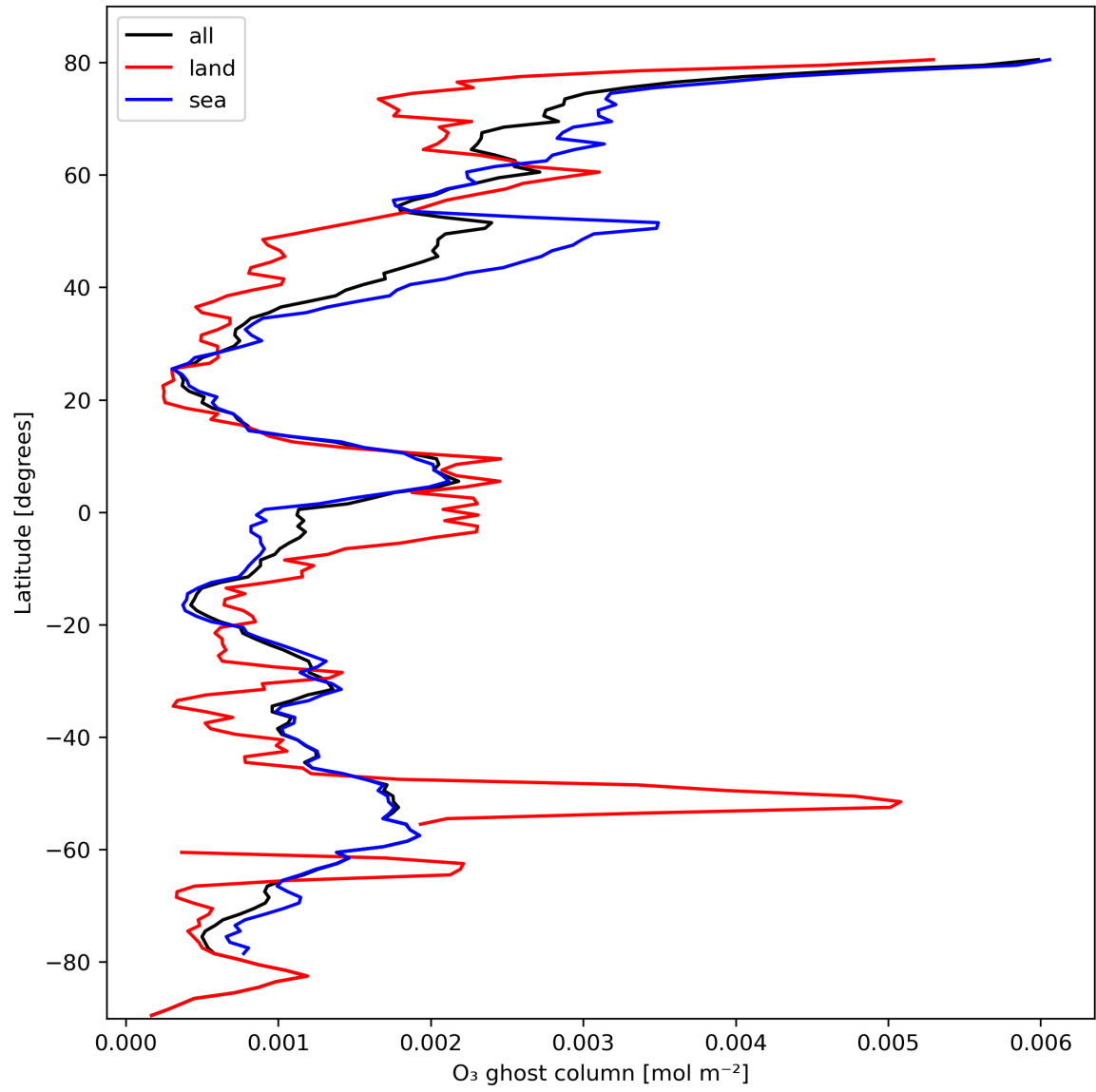
Figure 18: Zonal average of “O 3 ghost column” for 2023-10-15 to 2023-10-17.
