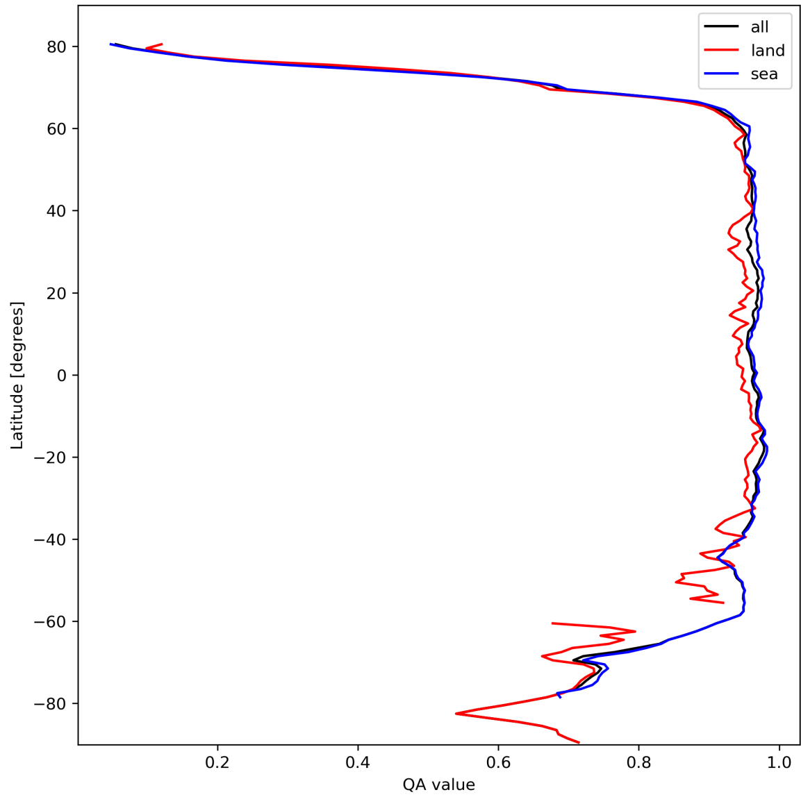
Figure 13: Zonal average of “QA value” for 2023-10-15 to 2023-10-17.
