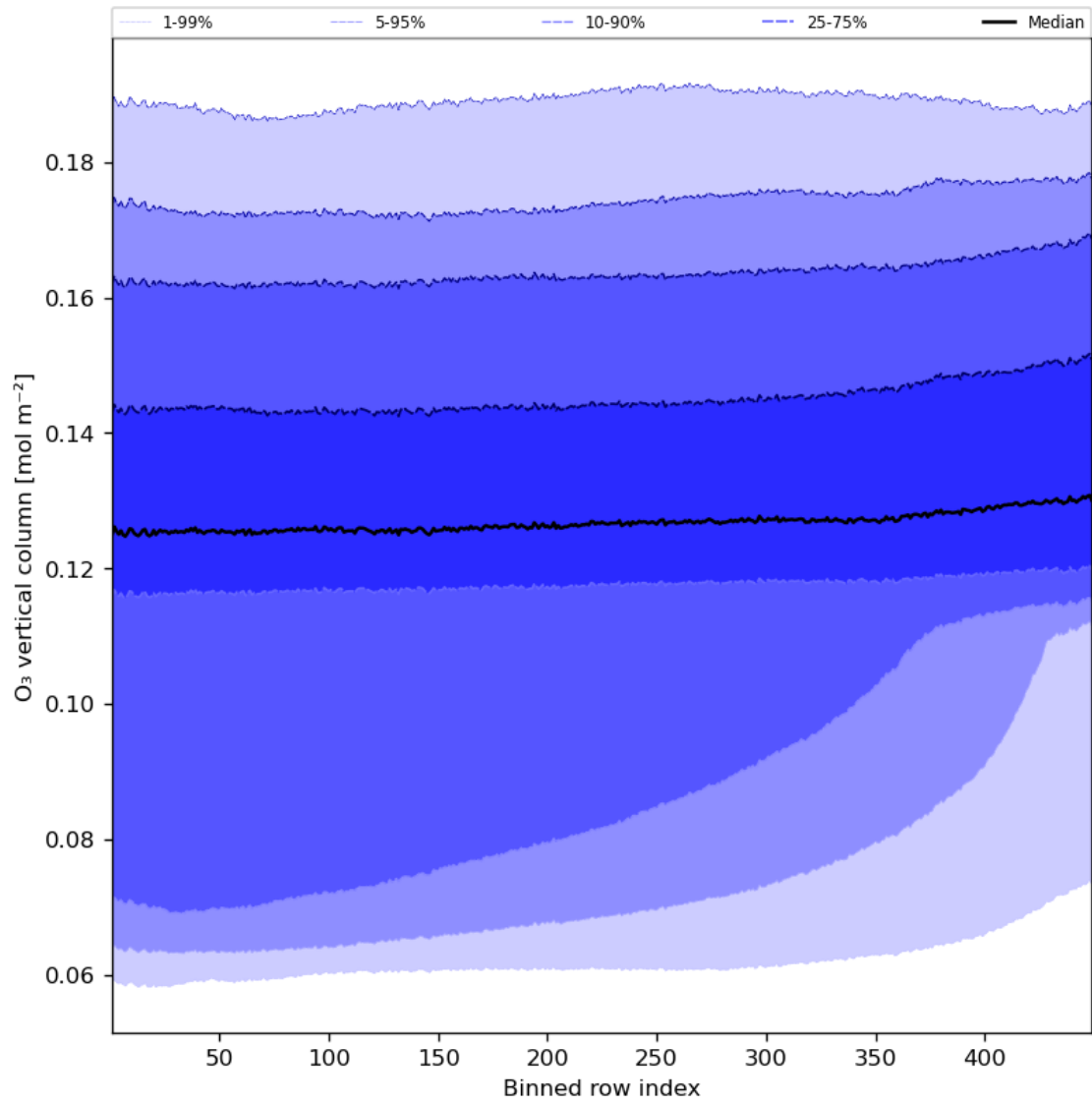
Figure 28: Along track statistics of “O 3 vertical column” for 2023-10-15 to 2023-10-17
