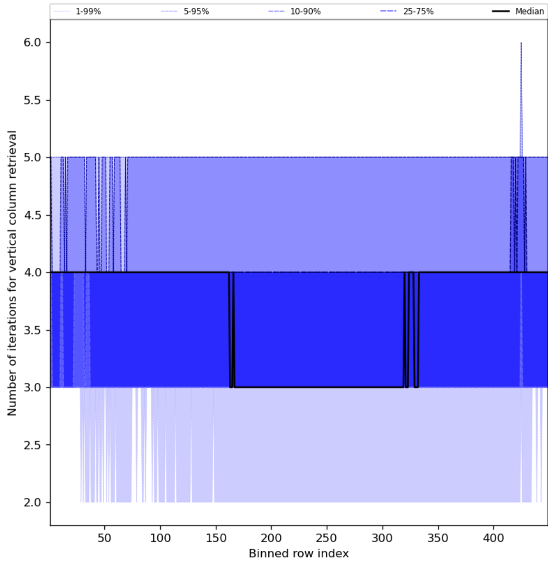
Figure 33: Along track statistics of “Number of iterations for vertical column retrieval” for 2023-10-15 to 2023-10-17
