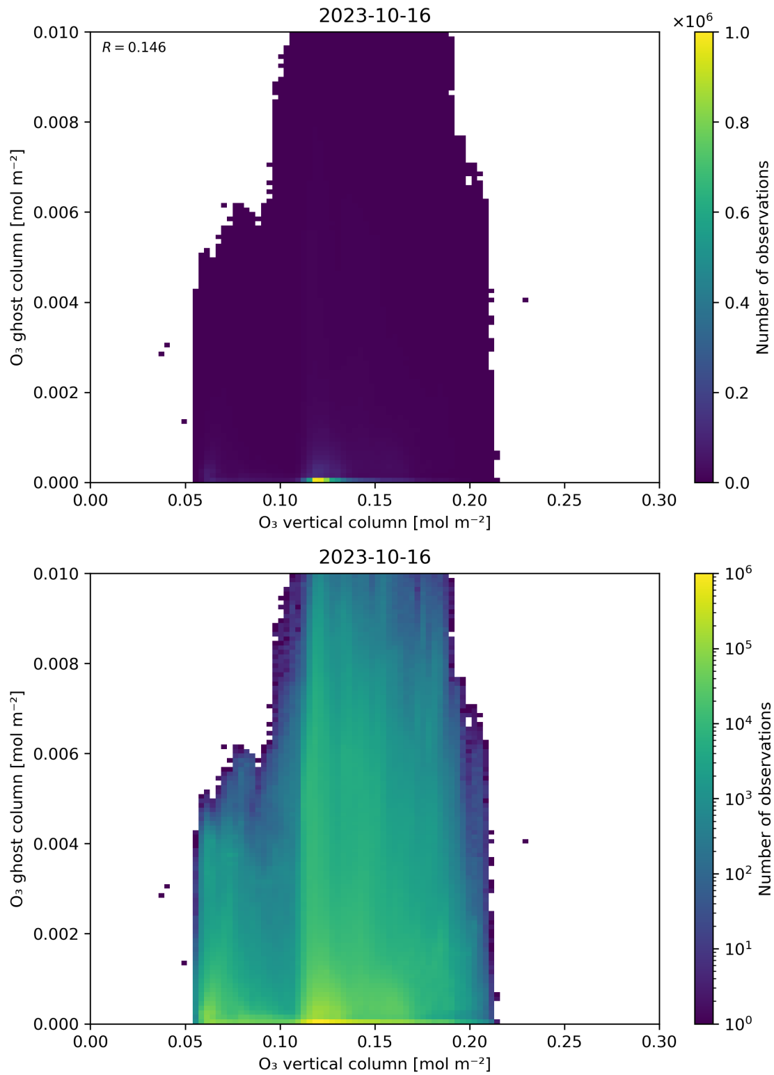
Figure 40: Scatter density plot of “O 3 vertical column” against “O 3 ghost column” for 2023-10-15 to 2023-10-17.
