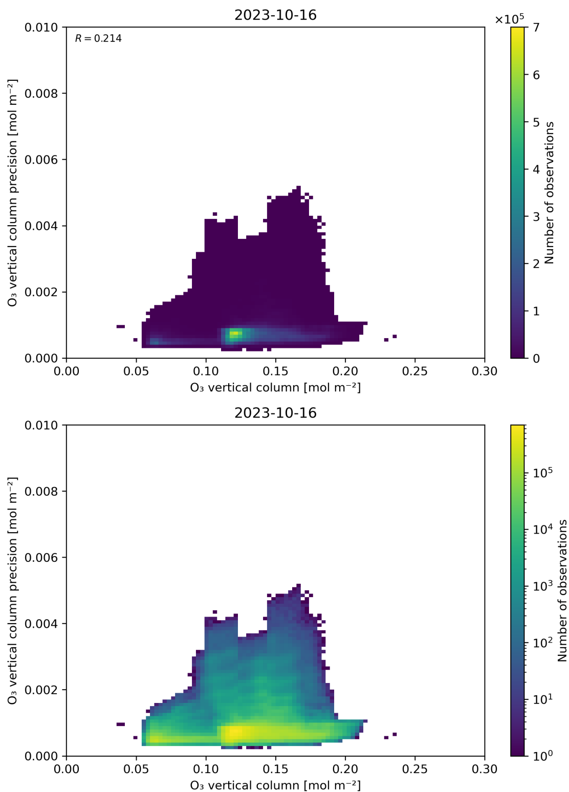
Figure 41: Scatter density plot of “O 3 vertical column” against “O 3 vertical column precision” for 2023-10-15 to 2023-10-17.
