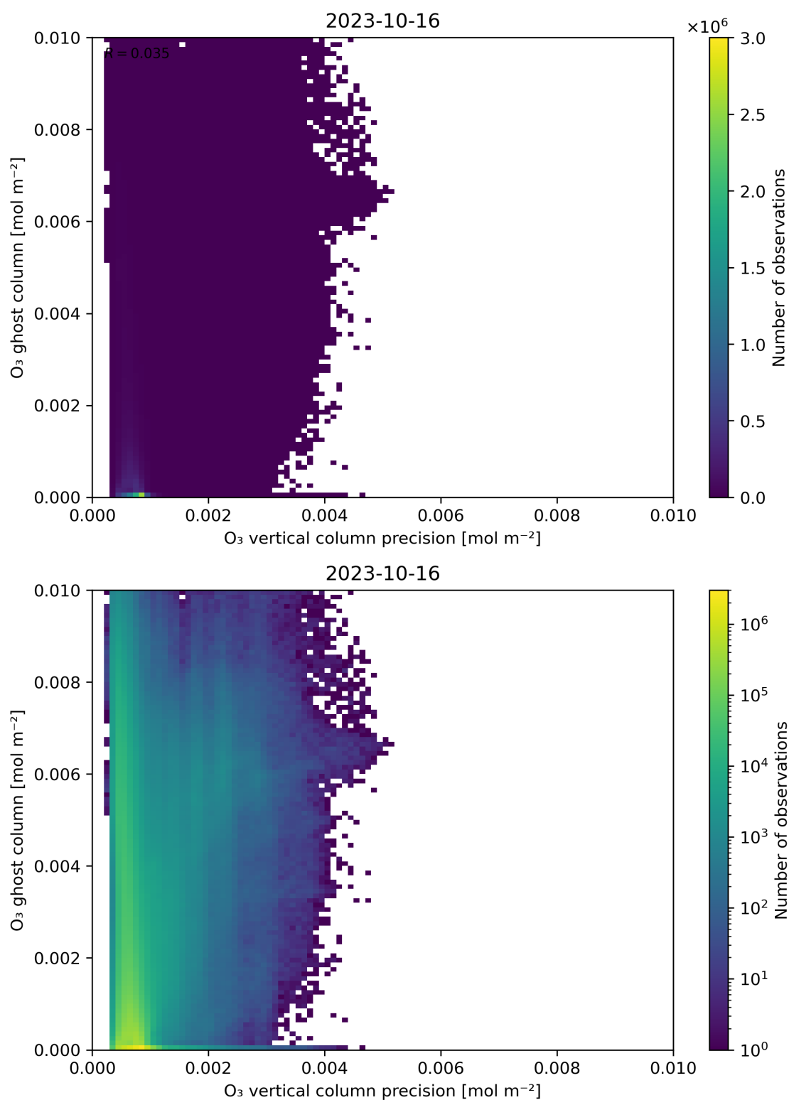
Figure 43: Scatter density plot of “O 3 vertical column precision” against “O 3 ghost column” for 2023-10-15 to 2023-10-17.
