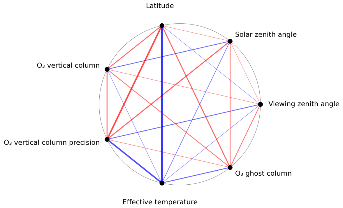
Figure 1: Map of correlation graph for 2023-10-15 to 2023-10-17.
