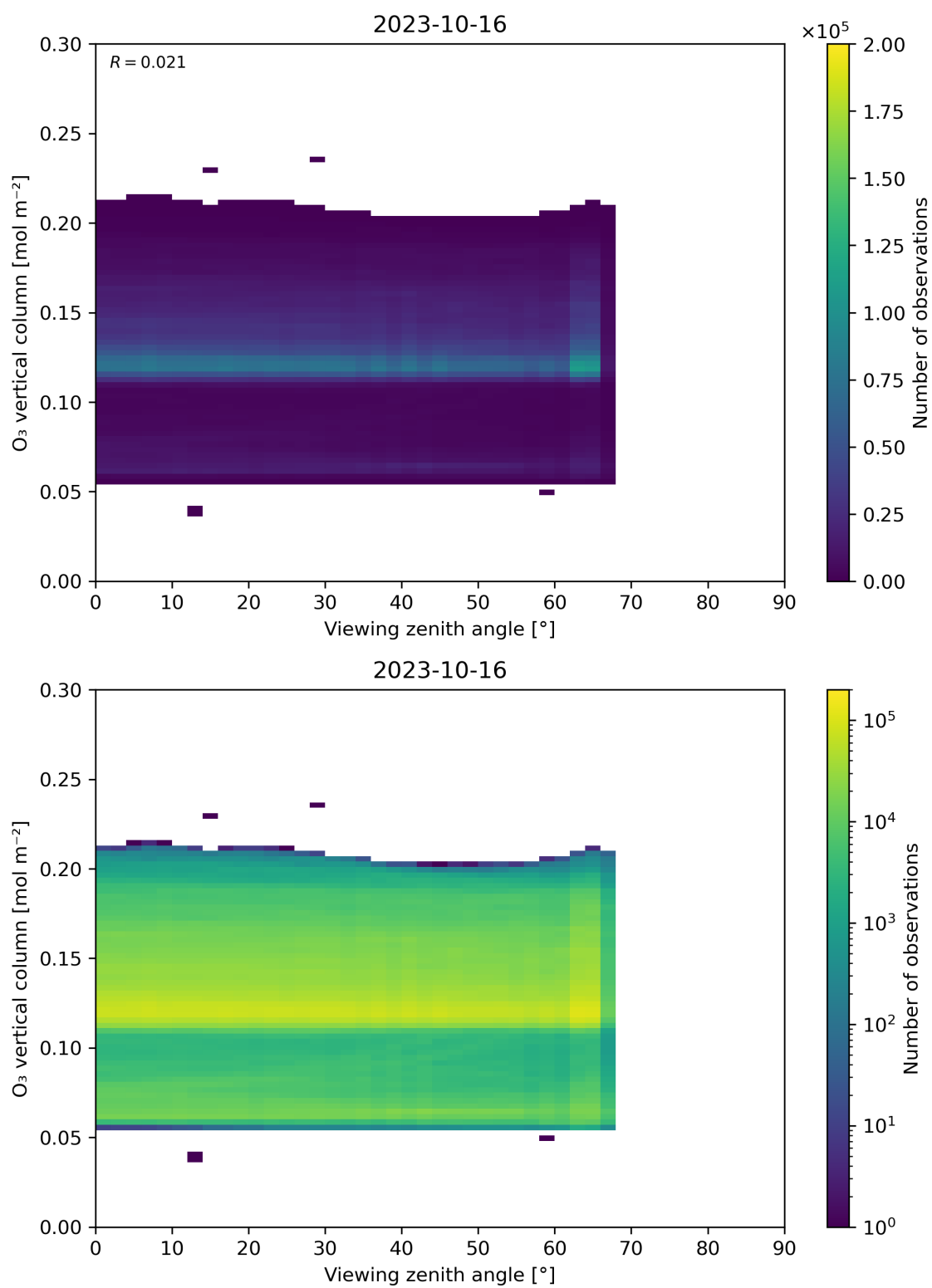
Figure 52: Scatter density plot of “Viewing zenith angle” against “O 3 vertical column” for 2023-10-15 to 2023-10-17.
