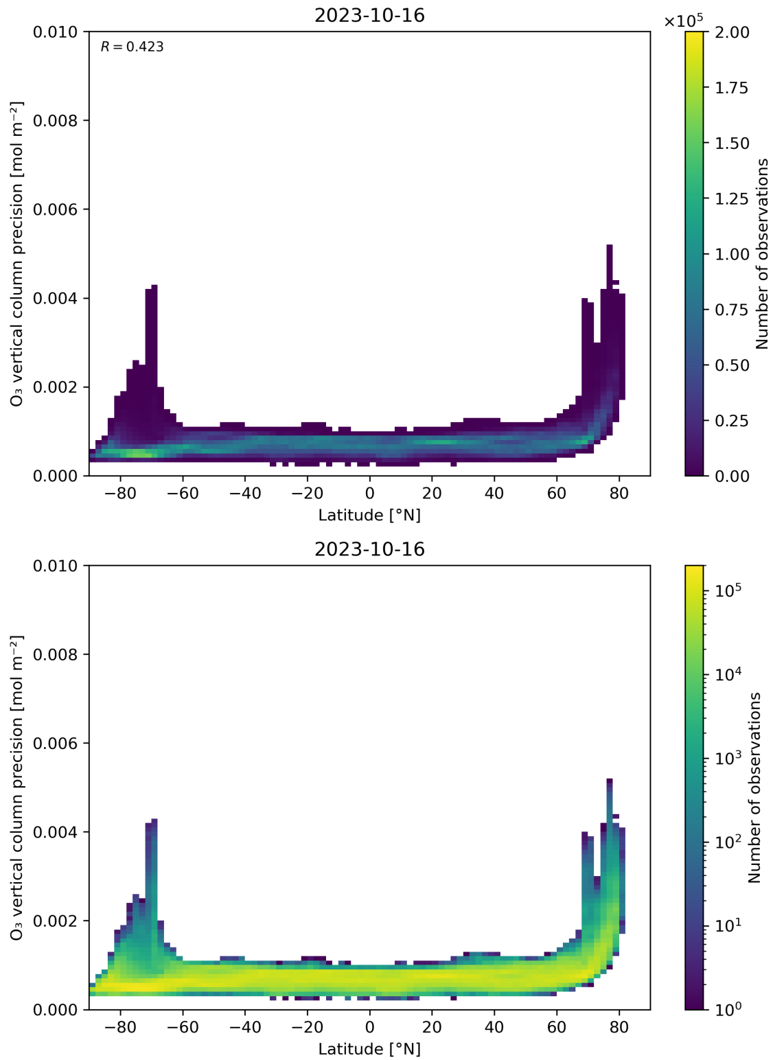
Figure 37: Scatter density plot of “Latitude” against “O 3 vertical column precision” for 2023-10-15 to 2023-10-17.
