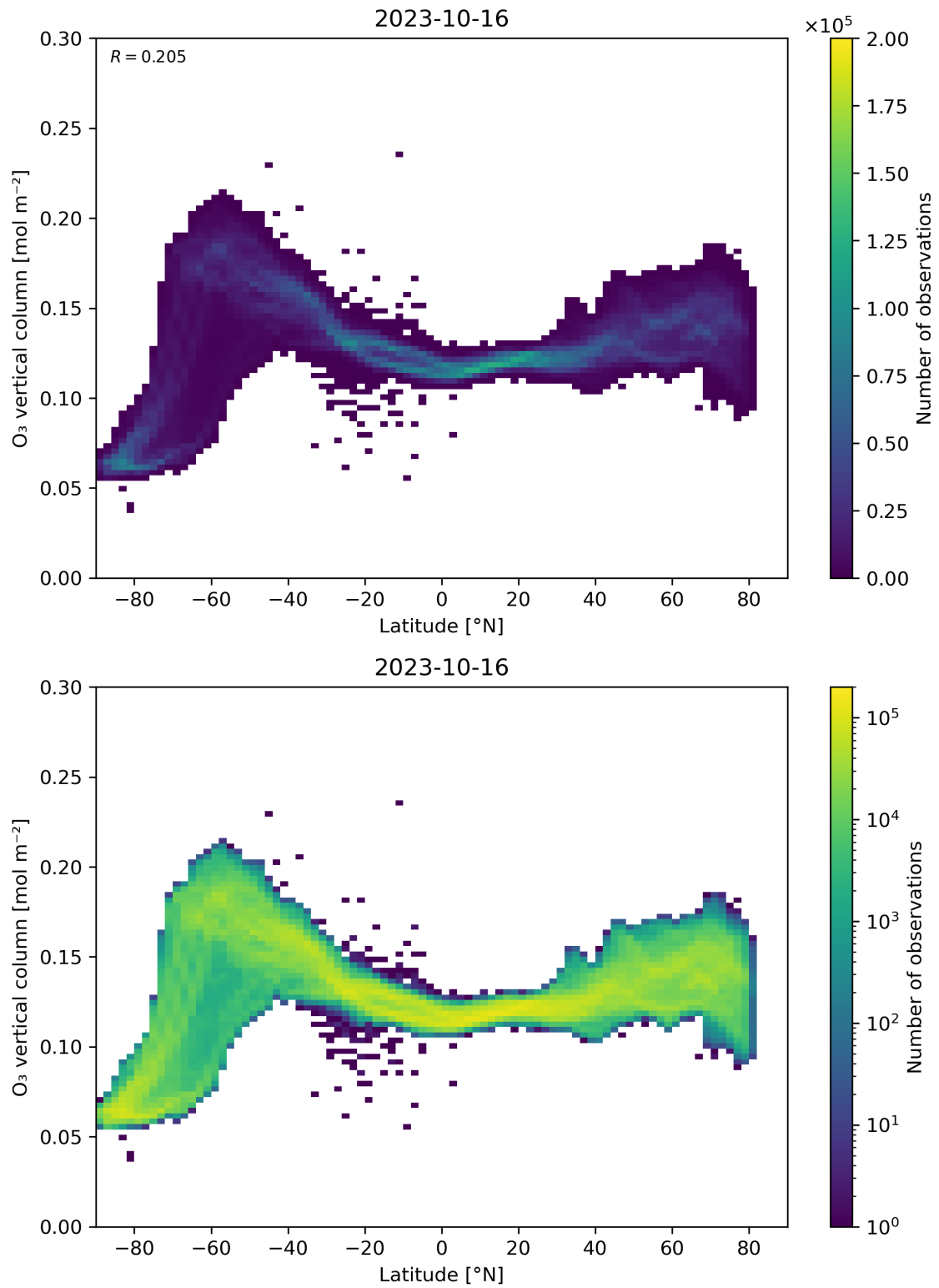
Figure 36: Scatter density plot of “Latitude” against “O 3 vertical column” for 2023-10-15 to 2023-10-17.
