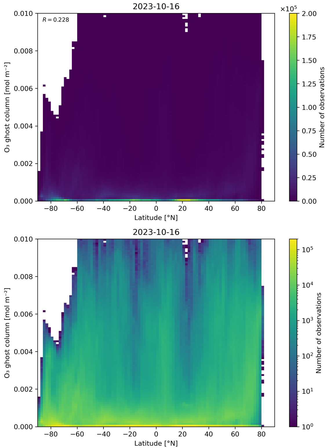
Figure 35: Scatter density plot of “Latitude” against “O 3 ghost column” for 2023-10-15 to 2023-10-17.
