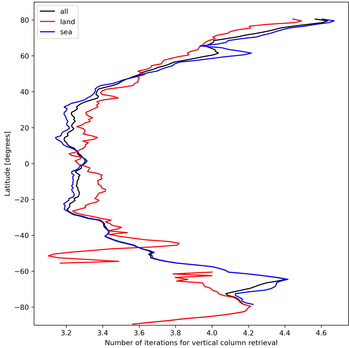
Figure 19: Zonal average of “Number of iterations for vertical column retrieval” for 2023-10-15 to 2023-10-17.
