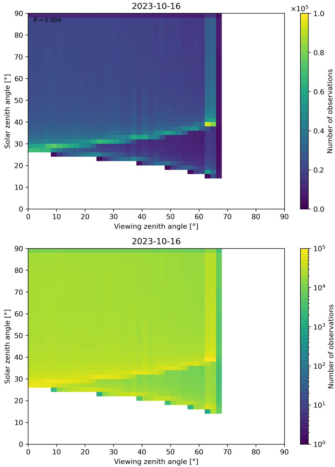
Figure 54: Scatter density plot of “Viewing zenith angle” against “Solar zenith angle” for 2023-10-15 to 2023-10-17.
