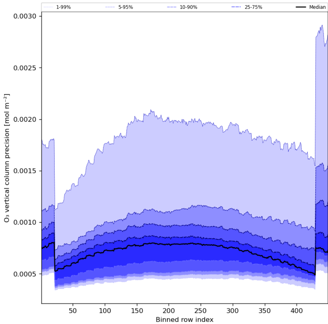
Figure 29: Along track statistics of “O 3 vertical column precision” for 2023-10-15 to 2023-10-17
