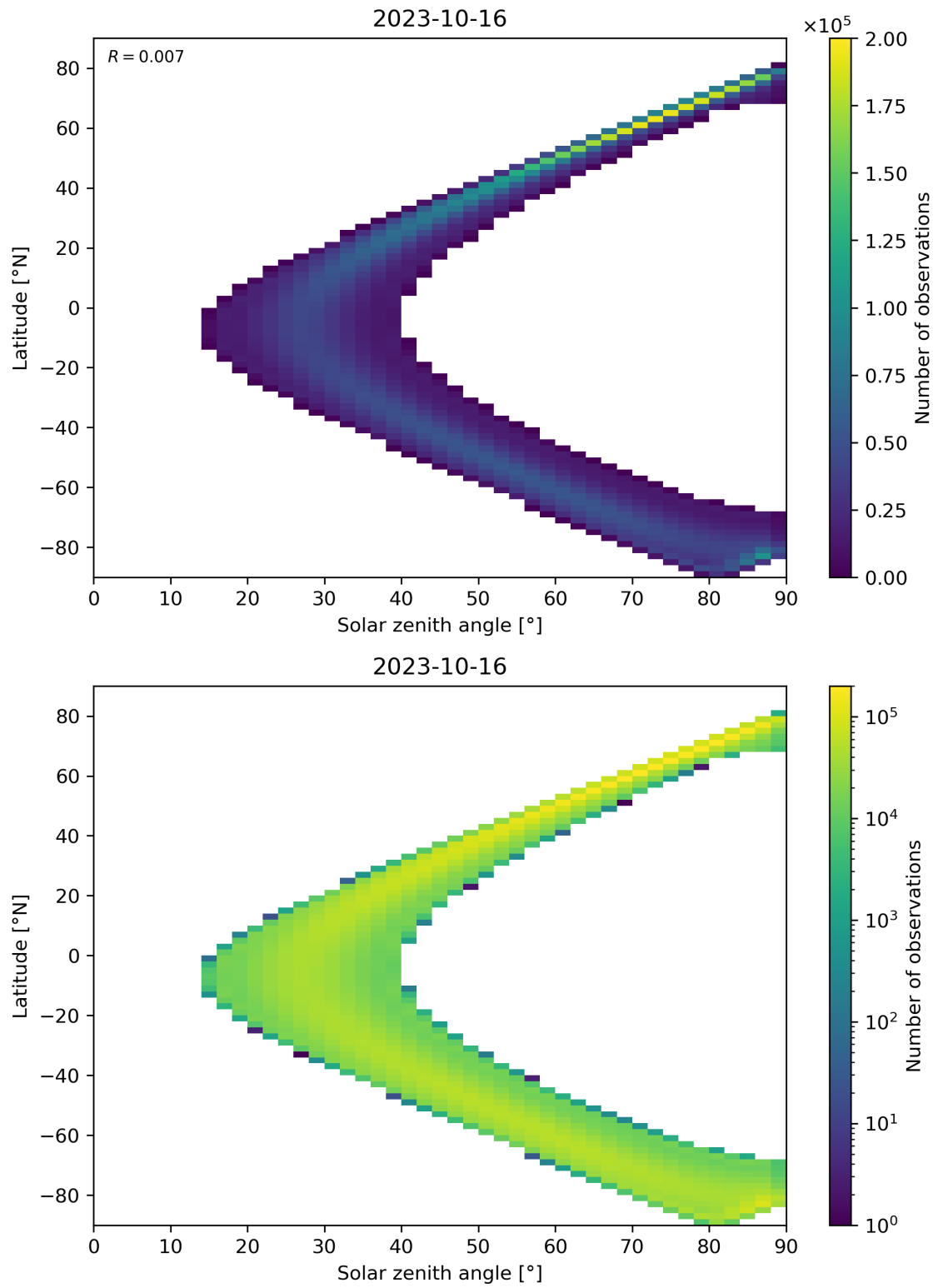
Figure 44: Scatter density plot of “Solar zenith angle” against “Latitude” for 2023-10-15 to 2023-10-17.
