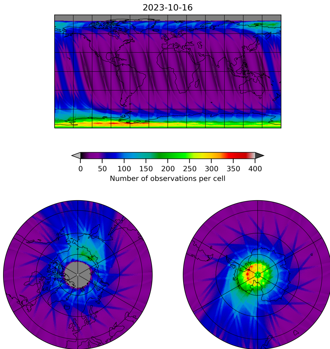
Figure 12: Map of the number of observations for 2023-10-15 to 2023-10-17
