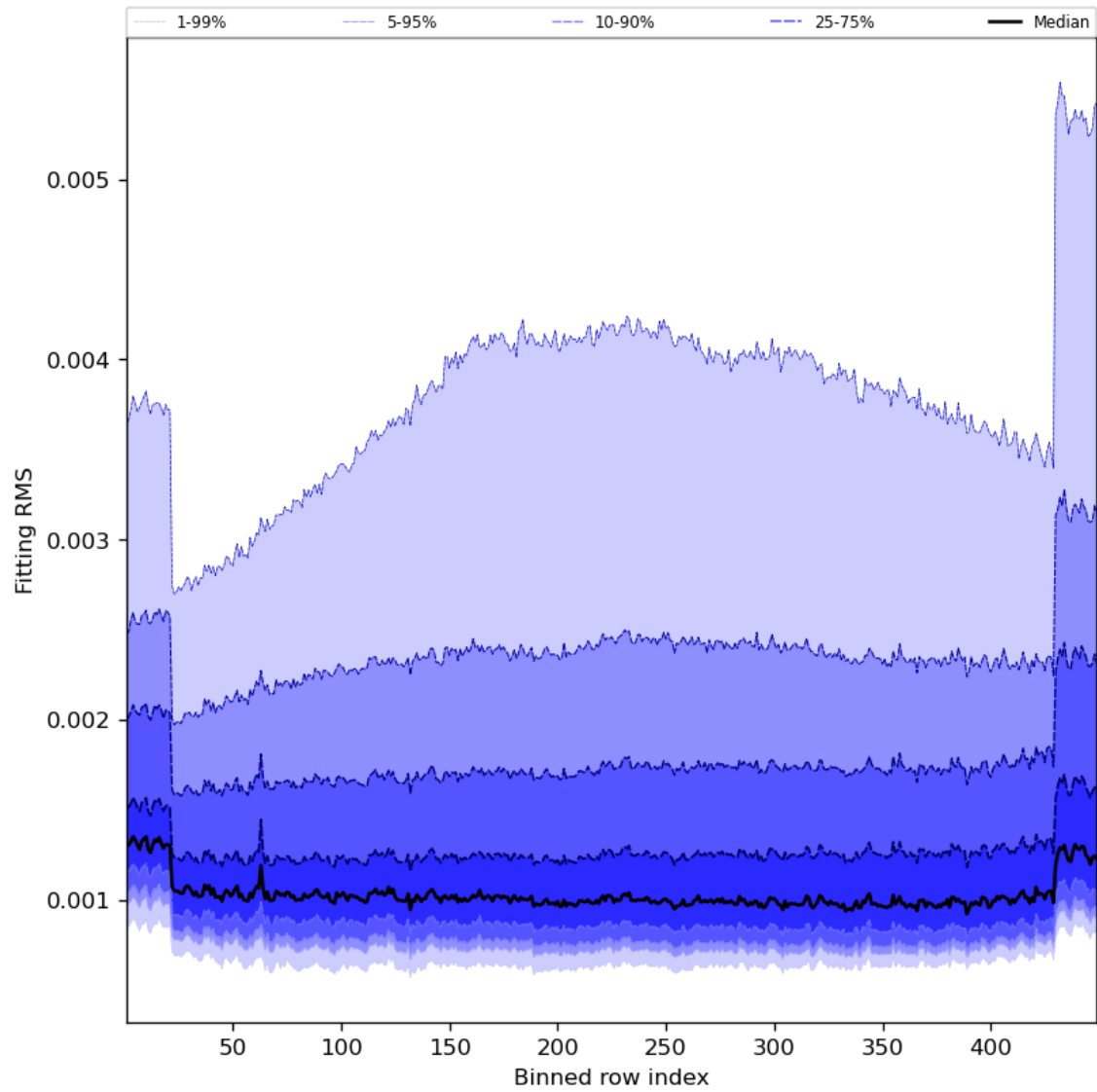
Figure 30: Along track statistics of “Fitting RMS” for 2023-10-15 to 2023-10-17
