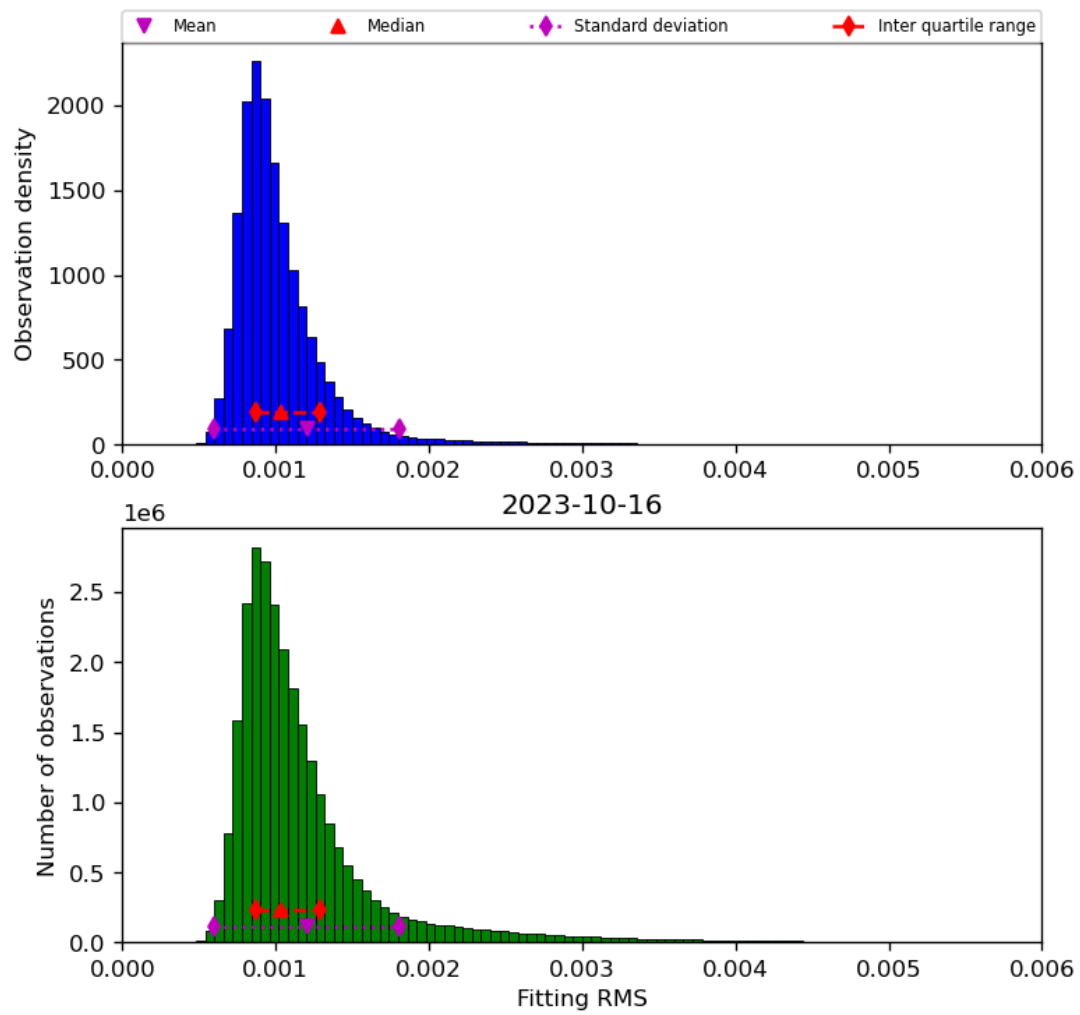
Figure 23: Histogram of “Fitting RMS” for 2023-10-15 to 2023-10-17
