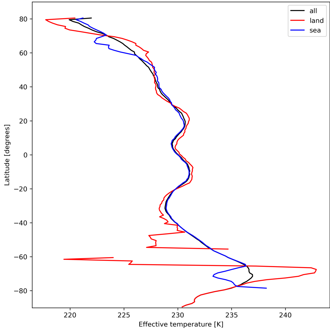
Figure 17: Zonal average of "Effective temperature" for 2023-10-15 to 2023-10-17.
