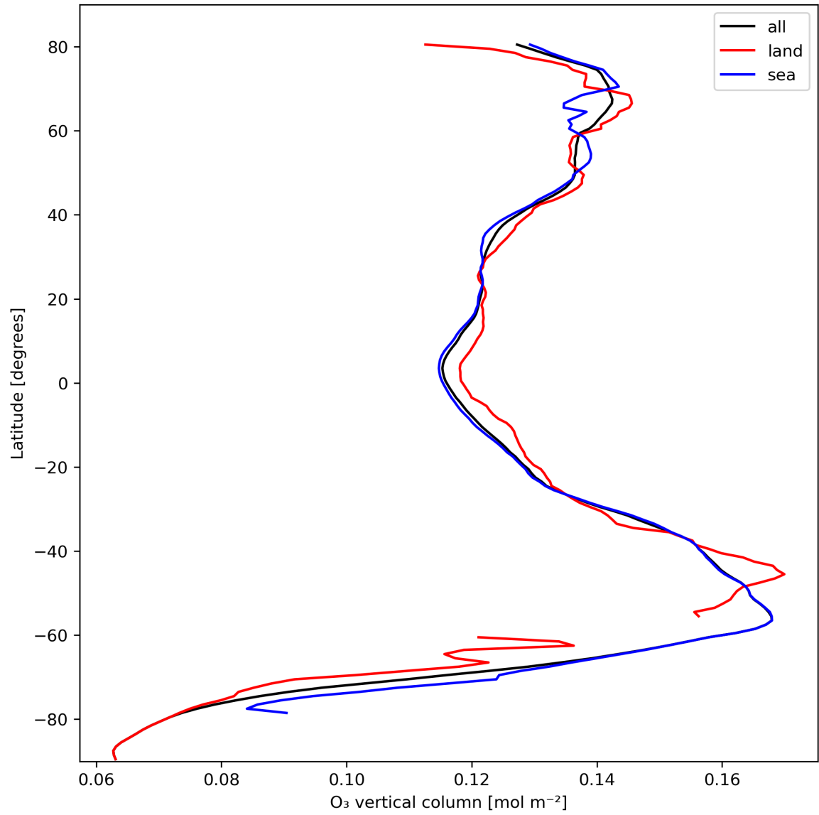
Figure 14: Zonal average of “O 3 vertical column” for 2023-10-15 to 2023-10-17.
