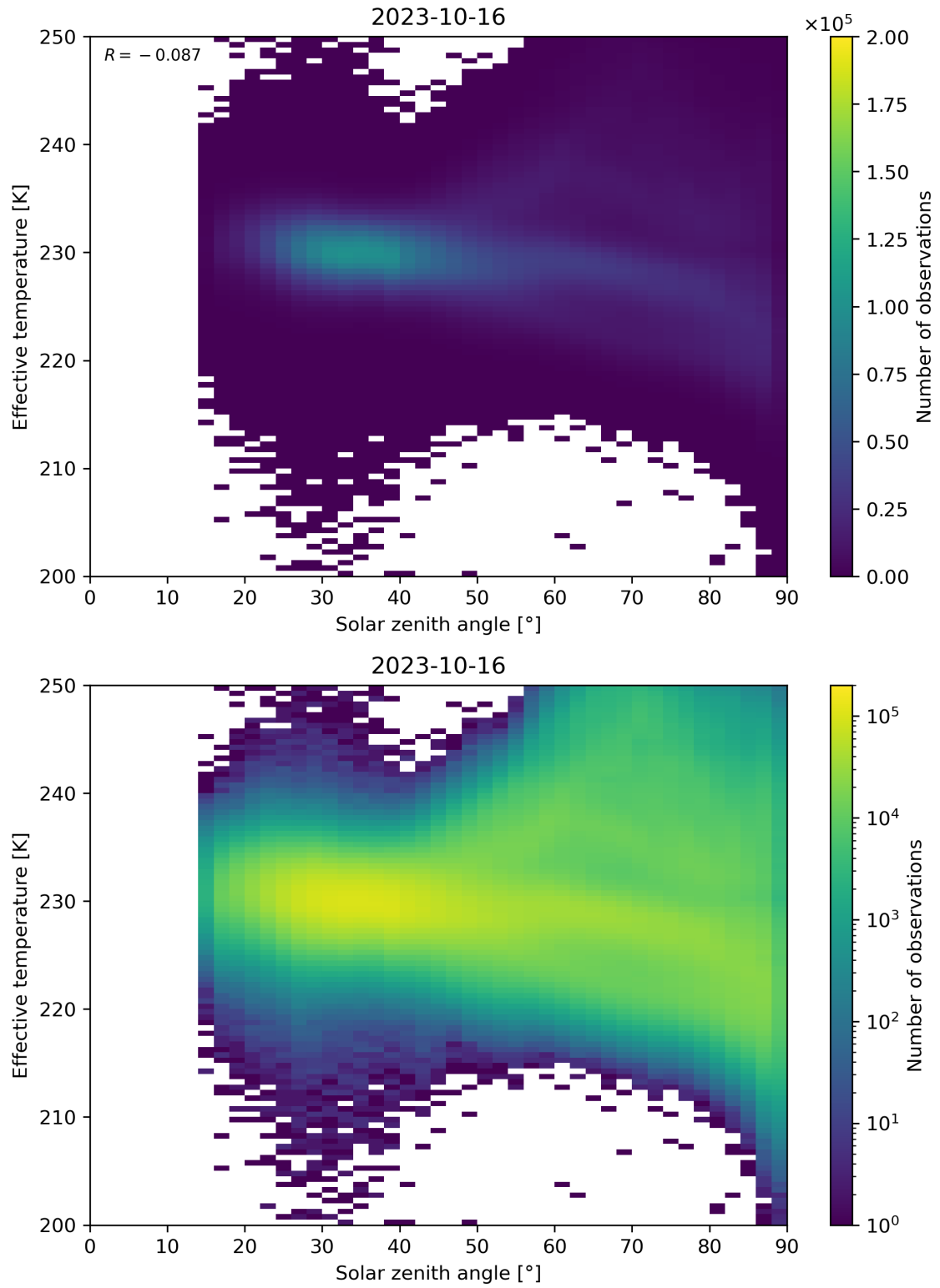
Figure 45: Scatter density plot of “Solar zenith angle” against “Effective temperature” for 2023-10-15 to 2023-10-17.
