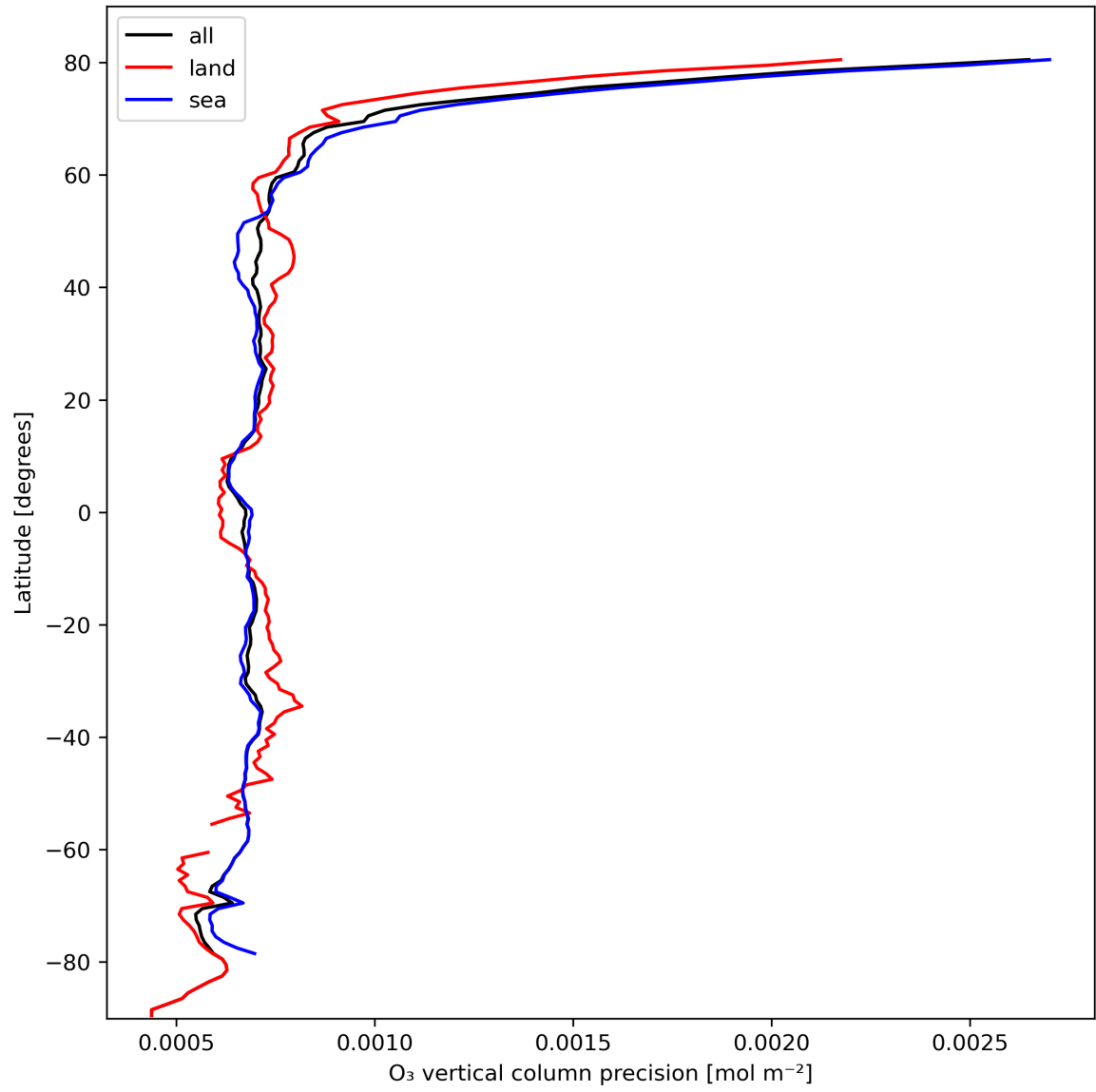
Figure 15: Zonal average of “O 3 vertical column precision” for 2023-10-15 to 2023-10-17.
