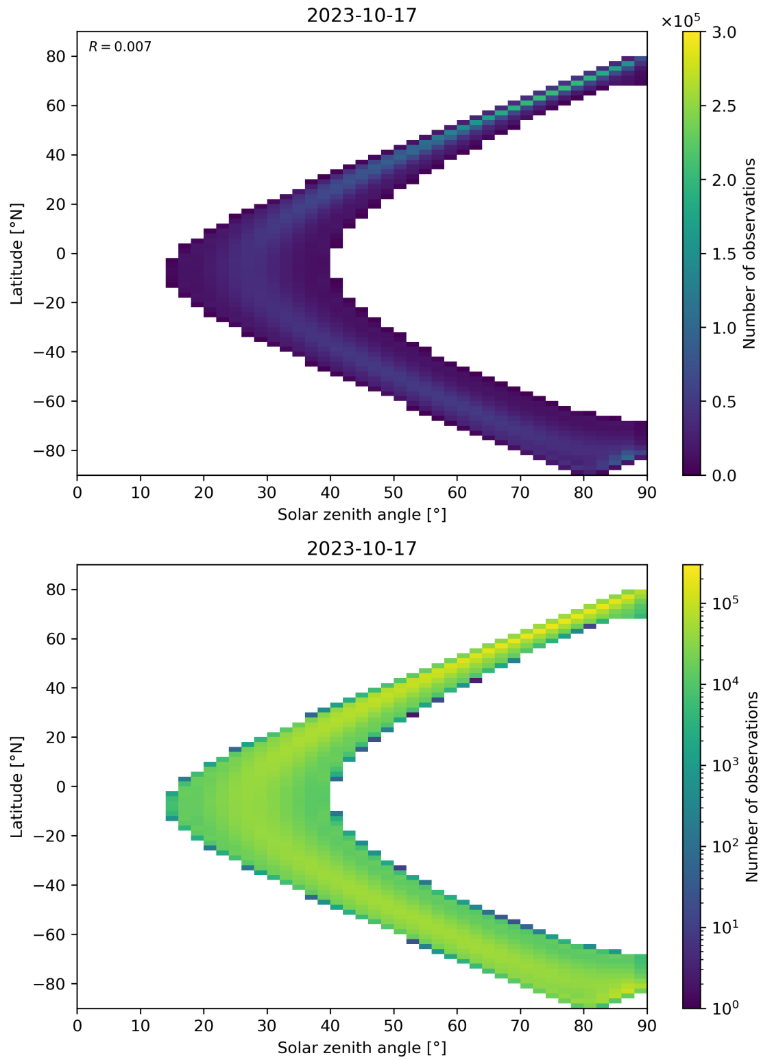
Figure 44: Scatter density plot of “Solar zenith angle” against “Latitude” for 2023-10-17 to 2023-10-18.
