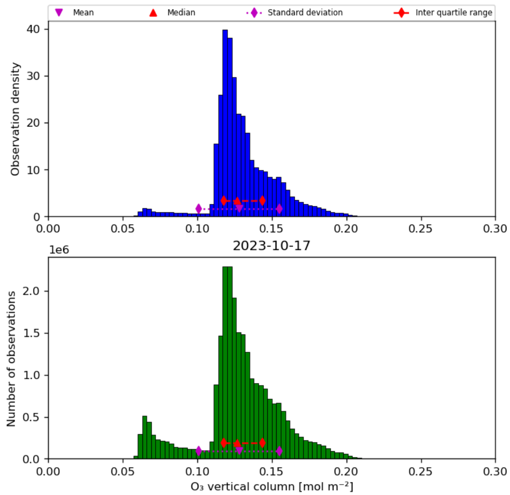
Figure 21: Histogram of “O 3 vertical column” for 2023-10-17 to 2023-10-18
