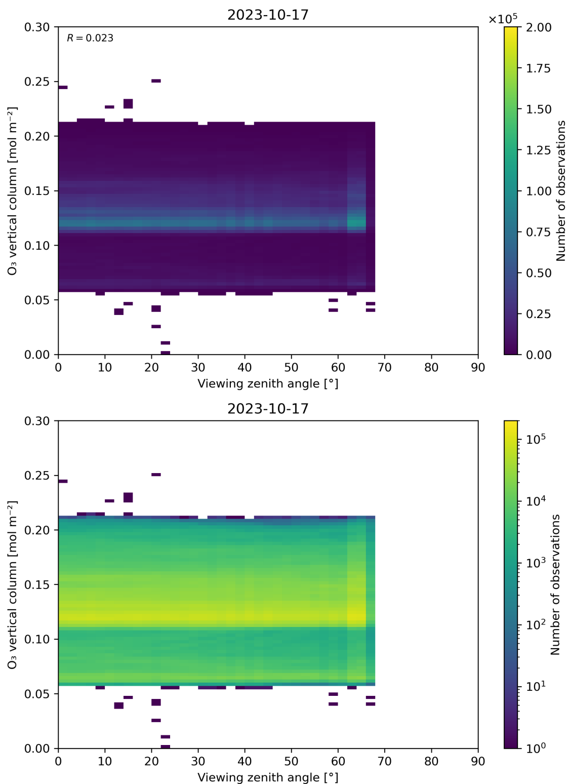
Figure 52: Scatter density plot of “Viewing zenith angle” against “O 3 vertical column” for 2023-10-17 to 2023-10-18.
