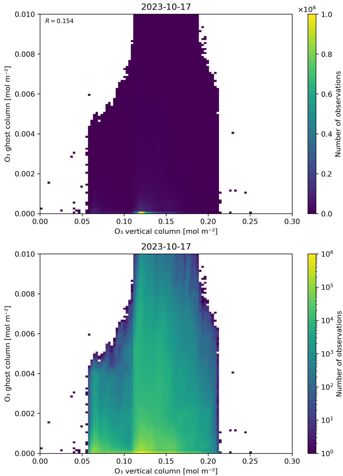
Figure 40: Scatter density plot of “O 3 vertical column” against “O 3 ghost column” for 2023-10-17 to 2023-10-18.
