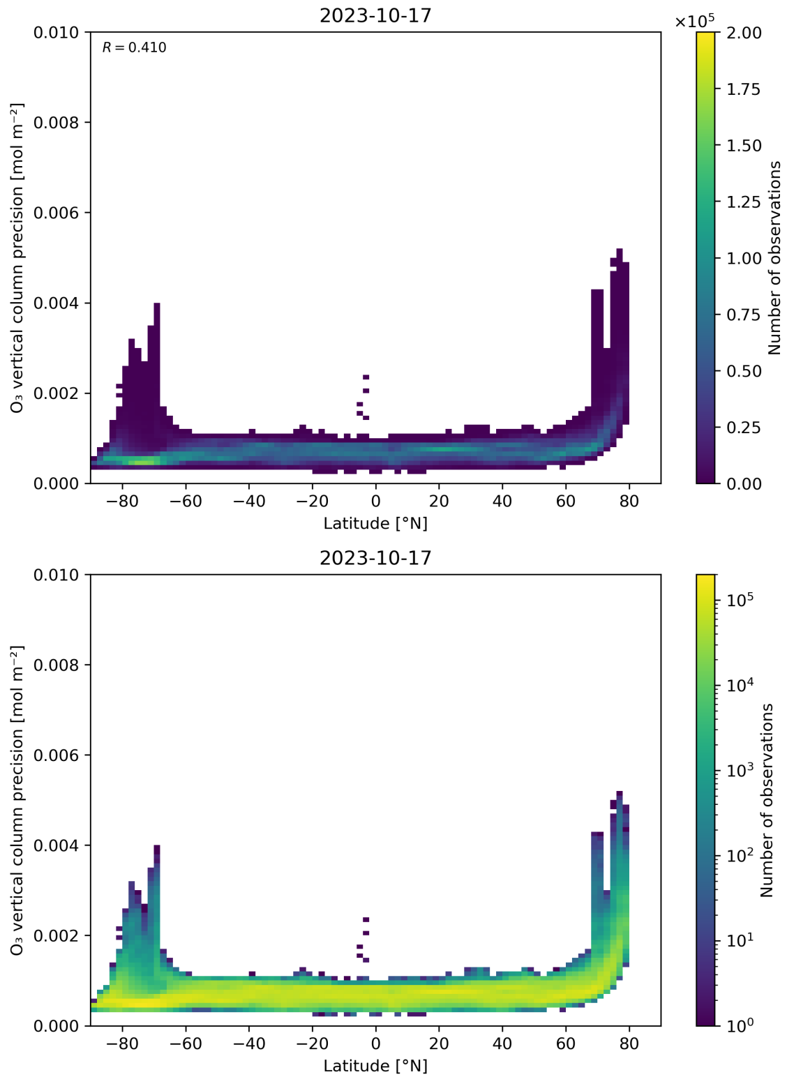
Figure 37: Scatter density plot of “Latitude” against “O 3 vertical column precision” for 2023-10-17 to 2023-10-18.
