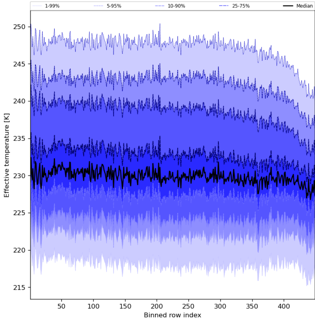
Figure 31: Along track statistics of “Effective temperature” for 2023-10-17 to 2023-10-18
