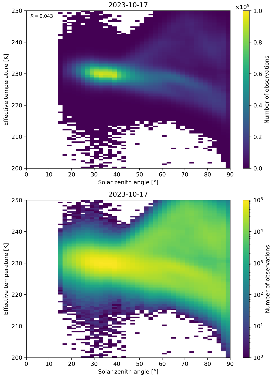
Figure 45: Scatter density plot of “Solar zenith angle” against “Effective temperature” for 2023-10-17 to 2023-10-18.
