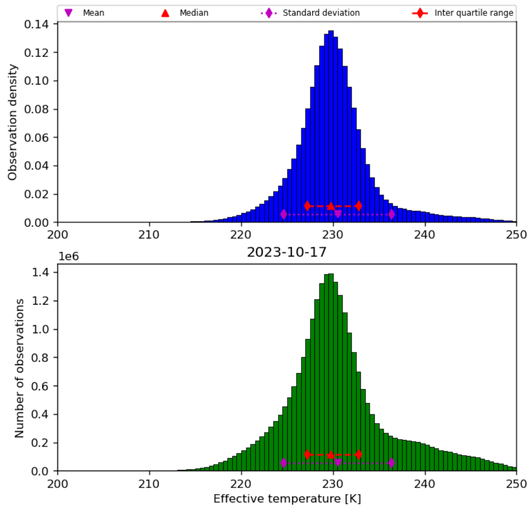
Figure 24: Histogram of “Effective temperature” for 2023-10-17 to 2023-10-18
