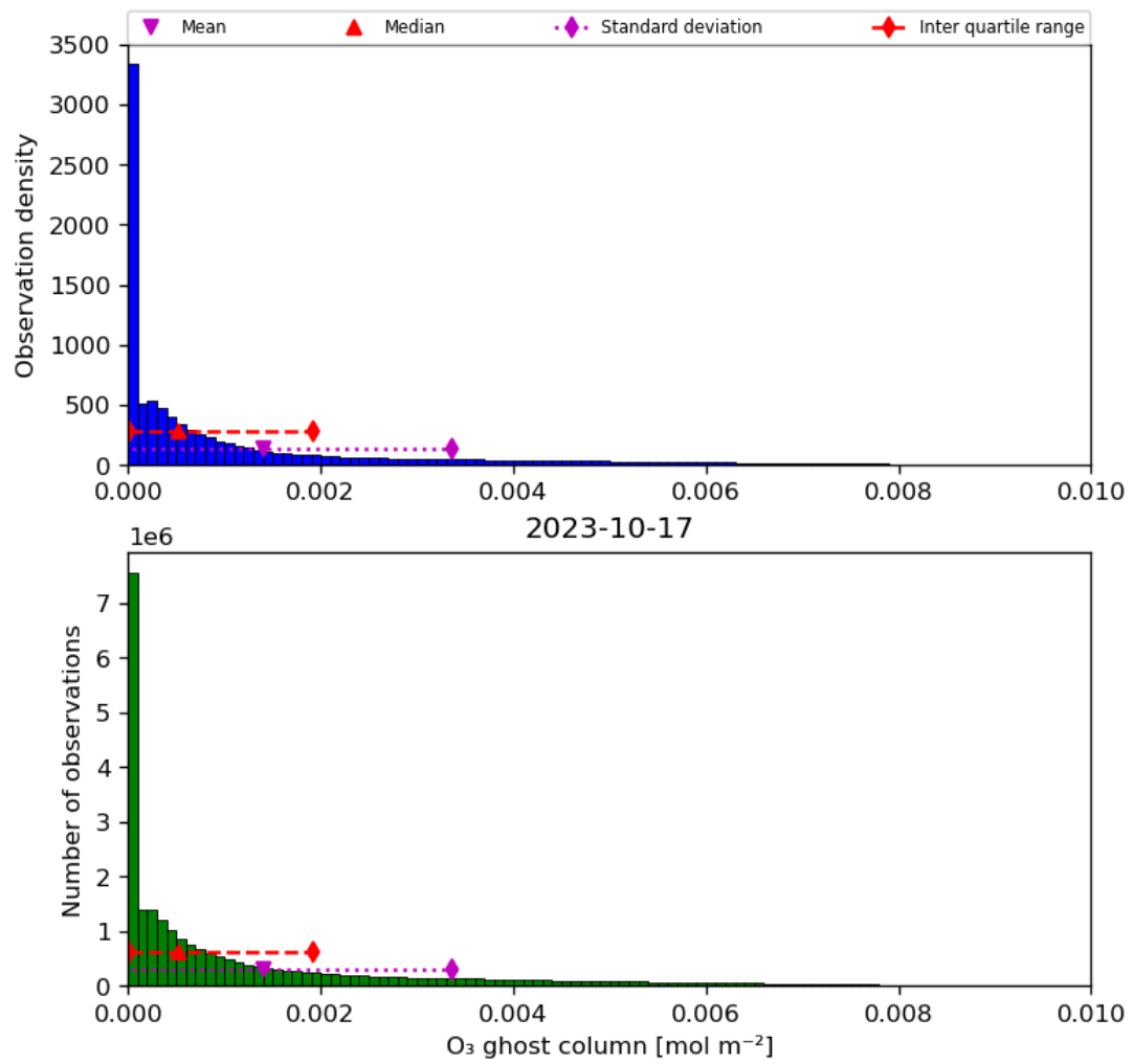
Figure 25: Histogram of “O 3 ghost column” for 2023-10-17 to 2023-10-18
