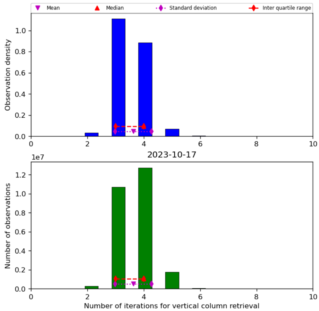
Figure 26: Histogram of “Number of iterations for vertical column retrieval” for 2023-10-17 to 2023-10-18
