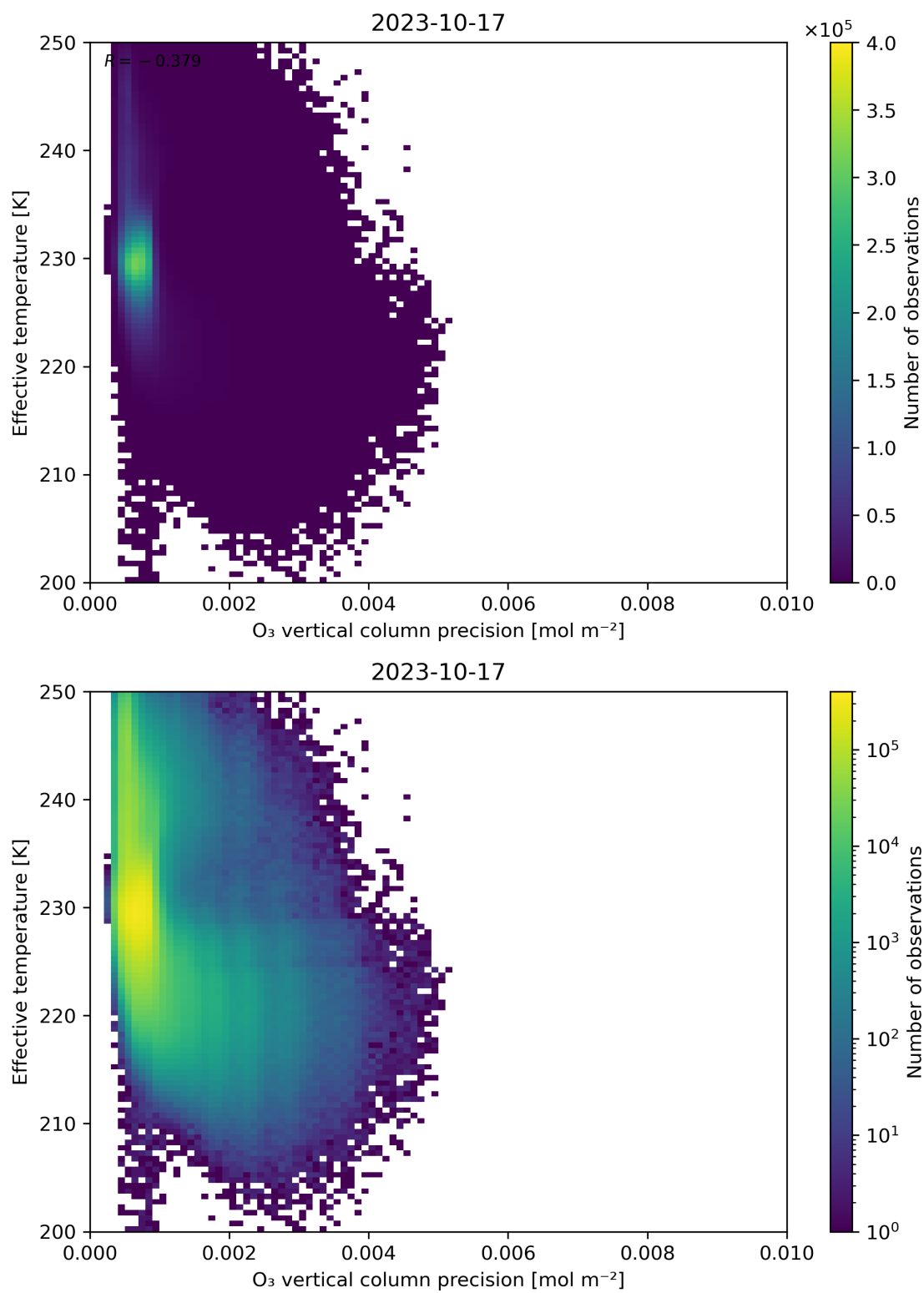
Figure 42: Scatter density plot of “O 3 vertical column precision” against “Effective temperature” for 2023-10-17 to 2023-10-18.
