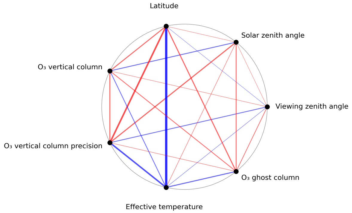
Figure 1: Map of correlation graph for 2023-10-17 to 2023-10-18.
