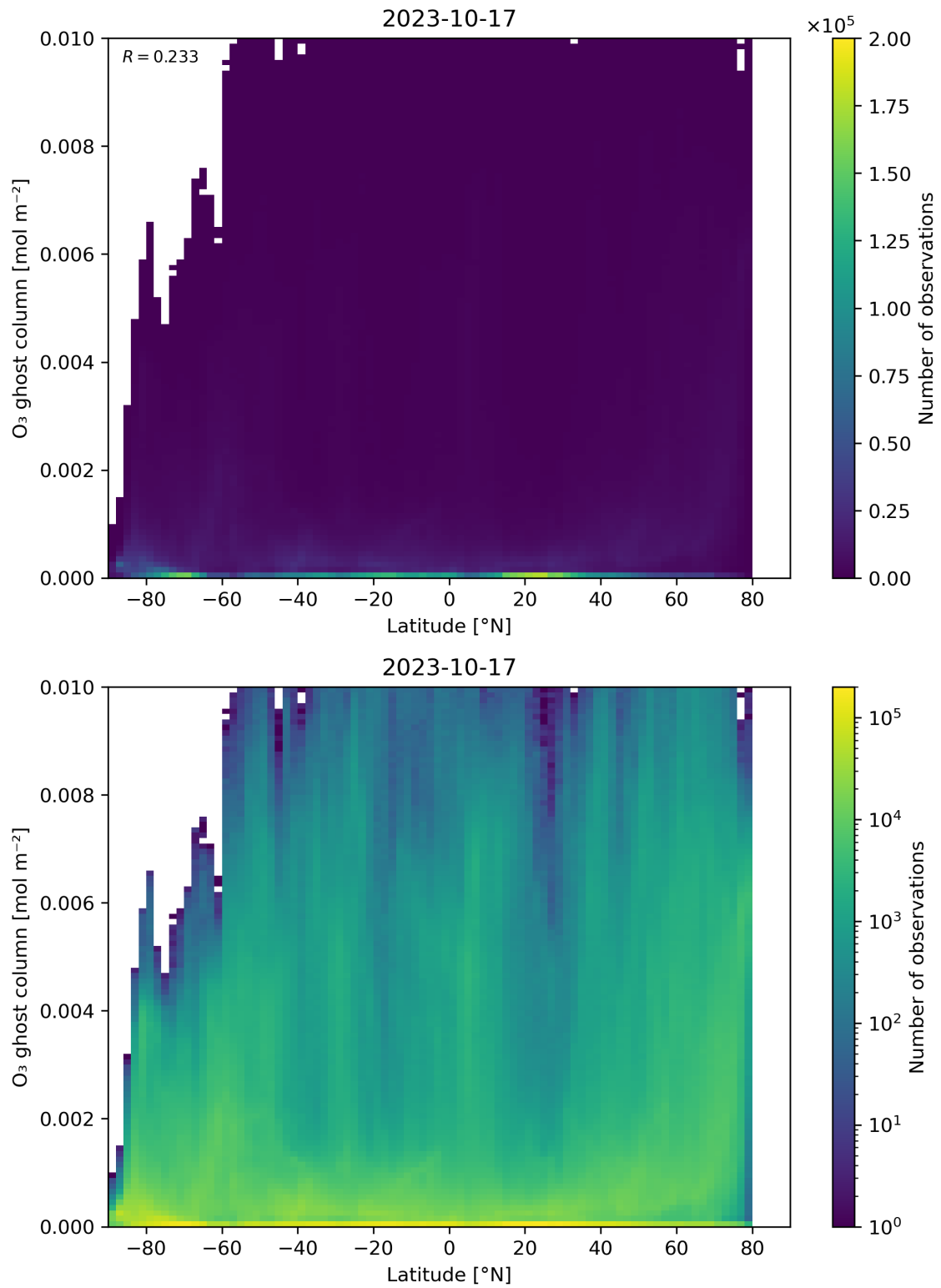
Figure 35: Scatter density plot of “Latitude” against “O 3 ghost column” for 2023-10-17 to 2023-10-18.
