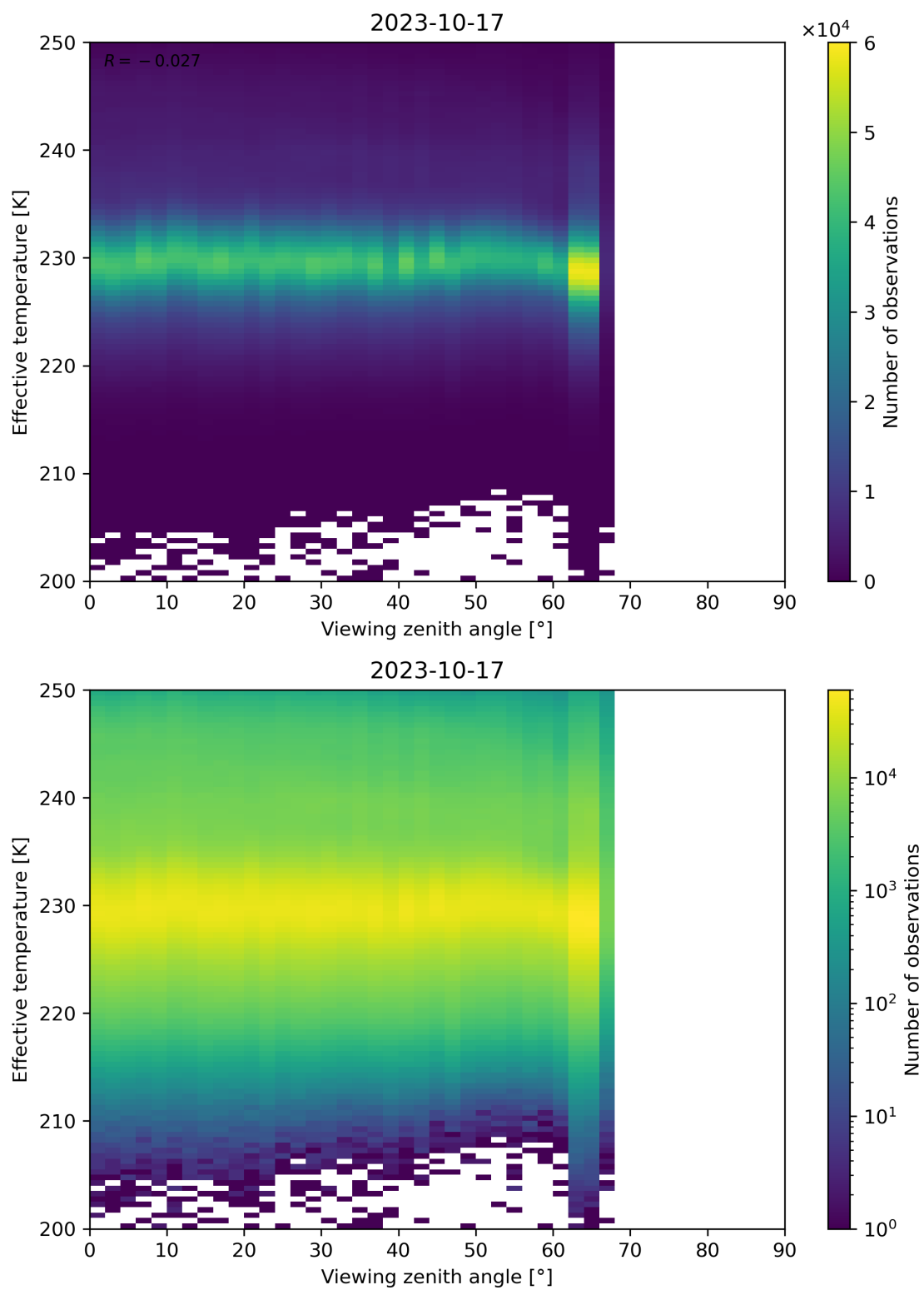
Figure 50: Scatter density plot of “Viewing zenith angle” against “Effective temperature” for 2023-10-17 to 2023-10-18.
