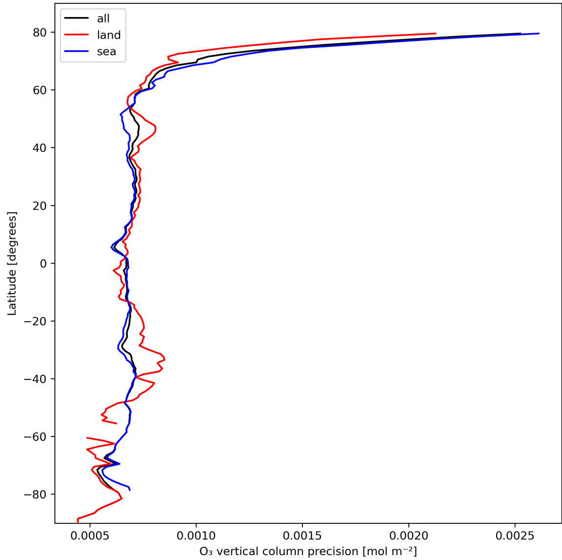
Figure 15: Zonal average of “O 3 vertical column precision” for 2023-10-17 to 2023-10-18.
