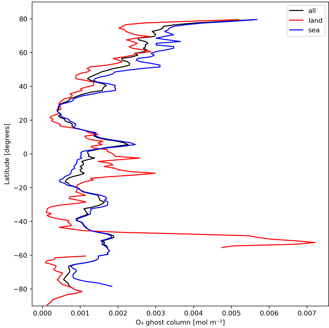
Figure 18: Zonal average of “O 3 ghost column” for 2023-10-17 to 2023-10-18.
