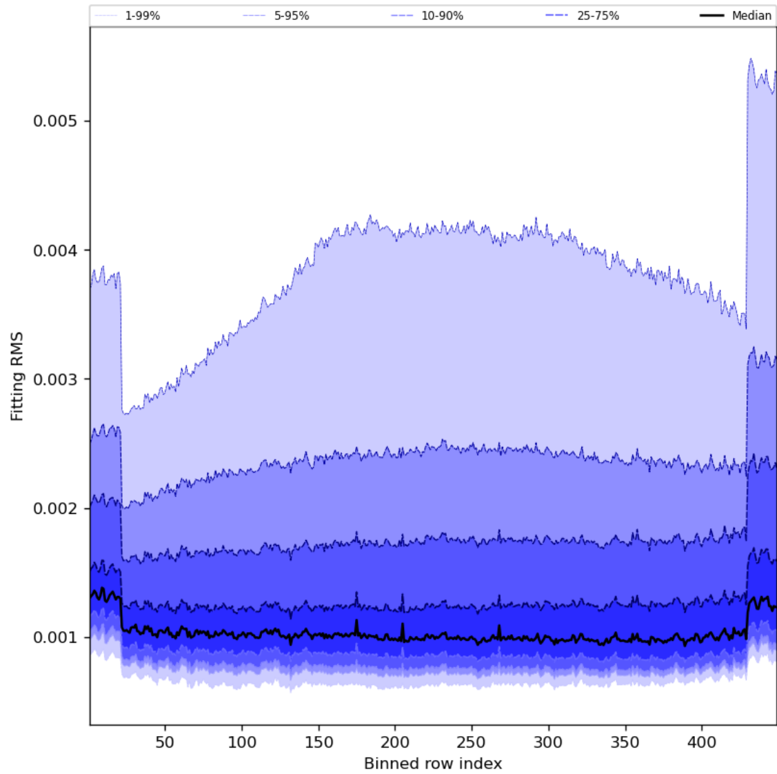
Figure 30: Along track statistics of “Fitting RMS” for 2023-10-17 to 2023-10-18
