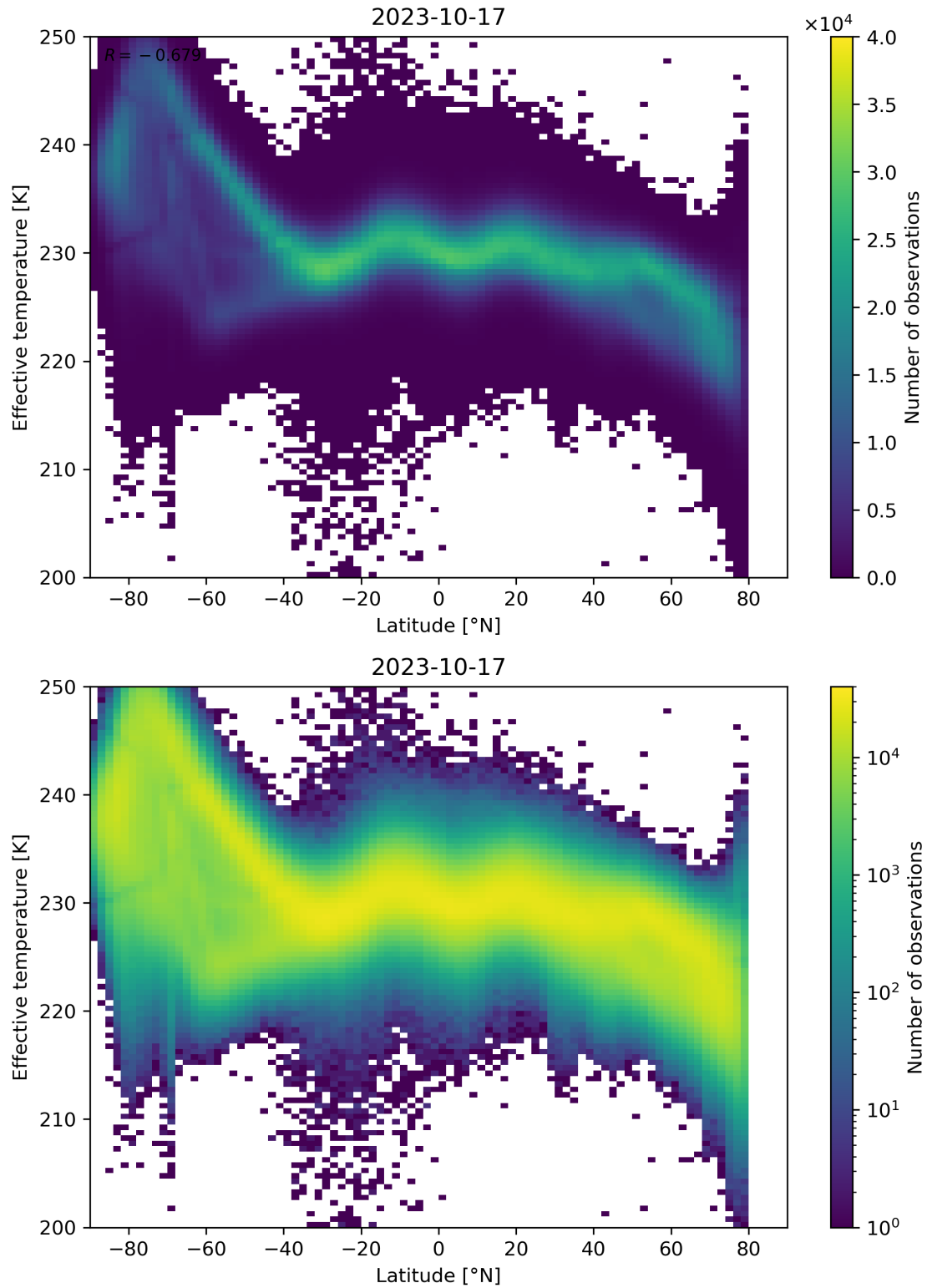
Figure 34: Scatter density plot of “Latitude” against “Effective temperature” for 2023-10-17 to 2023-10-18.
