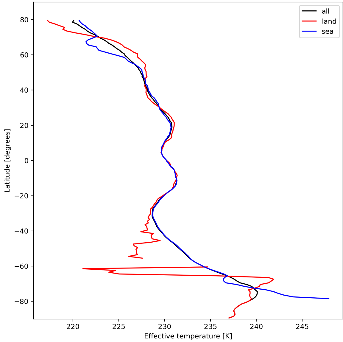
Figure 17: Zonal average of “Effective temperature” for 2023-10-17 to 2023-10-18.
