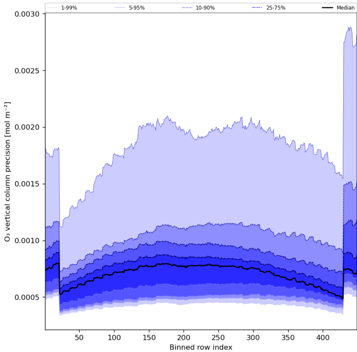
Figure 29: Along track statistics of “O 3 vertical column precision” for 2023-10-17 to 2023-10-18
