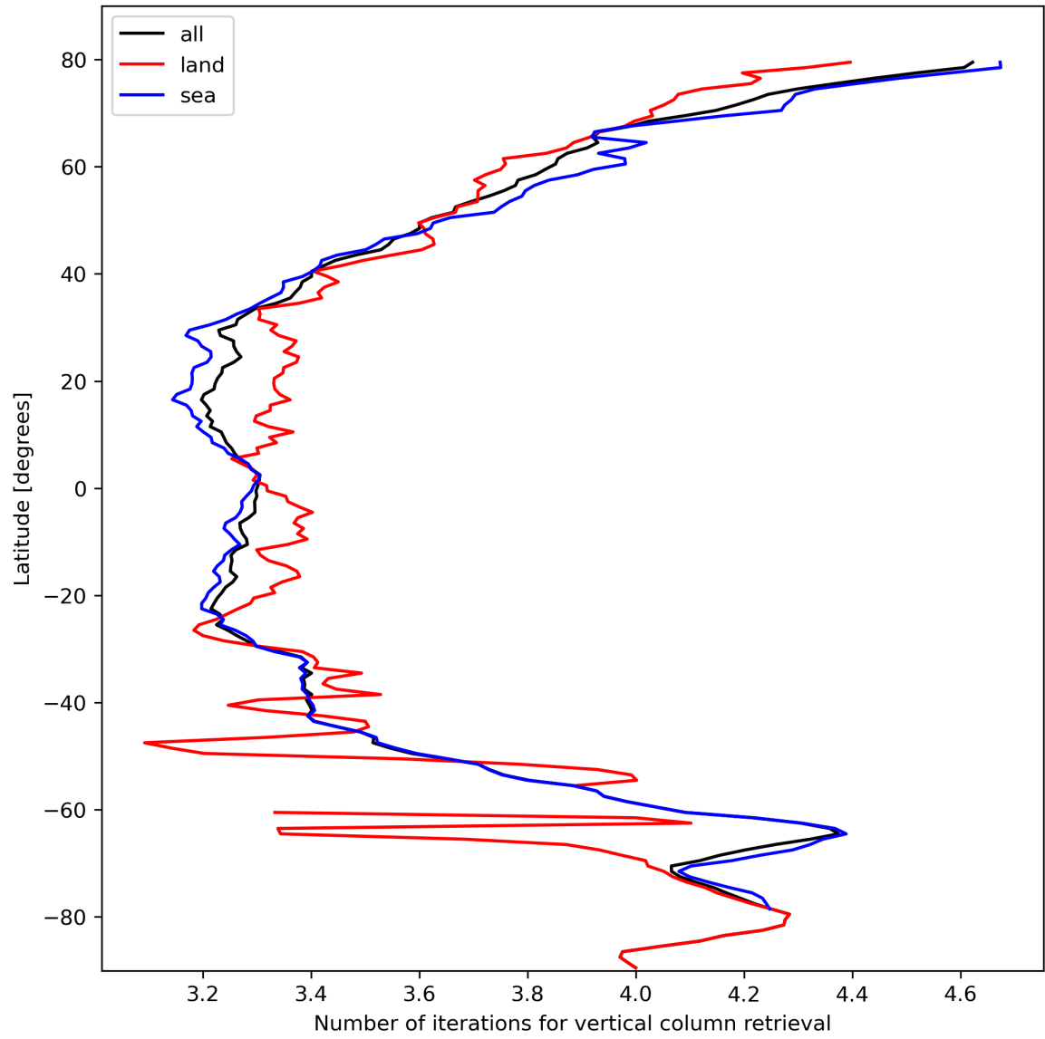
Figure 19: Zonal average of “Number of iterations for vertical column retrieval” for 2023-10-17 to 2023-10-18.
