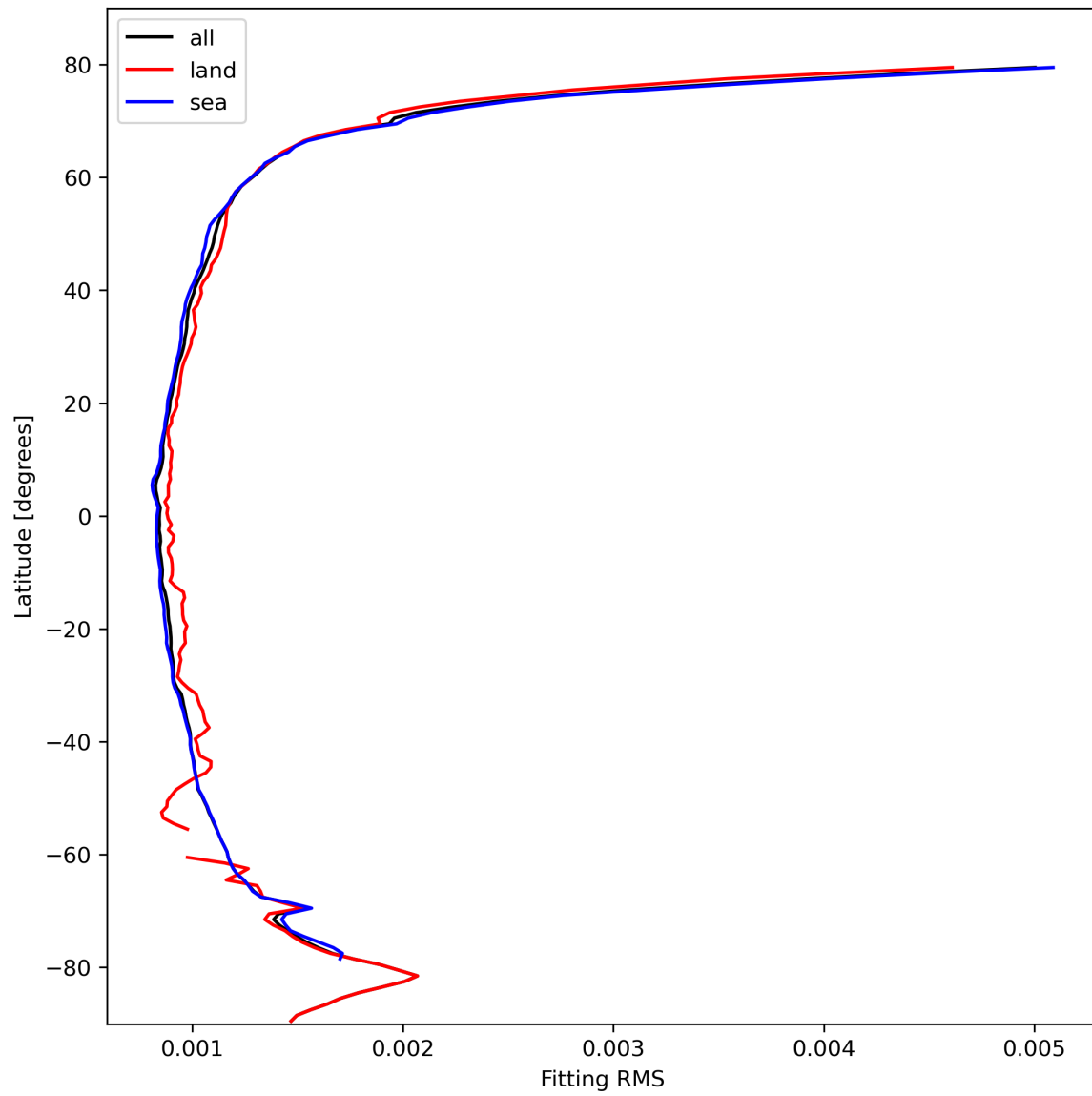
Figure 16: Zonal average of “Fitting RMS” for 2023-10-17 to 2023-10-18.
