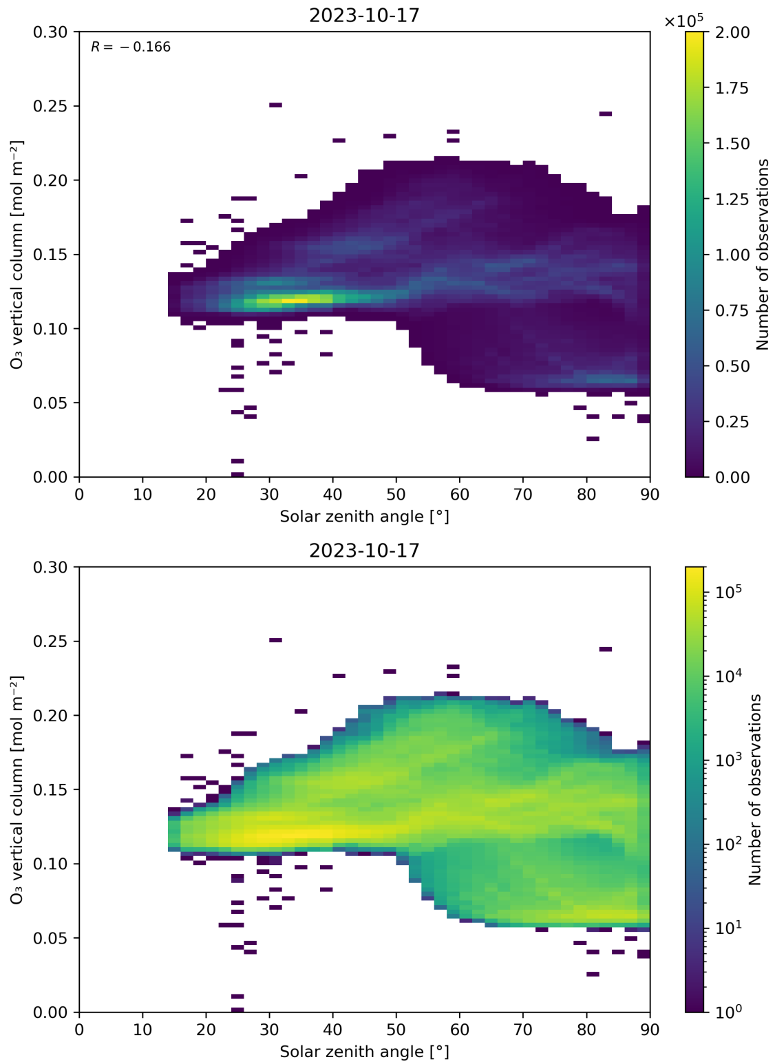
Figure 47: Scatter density plot of “Solar zenith angle” against “O 3 vertical column” for 2023-10-17 to 2023-10-18.
