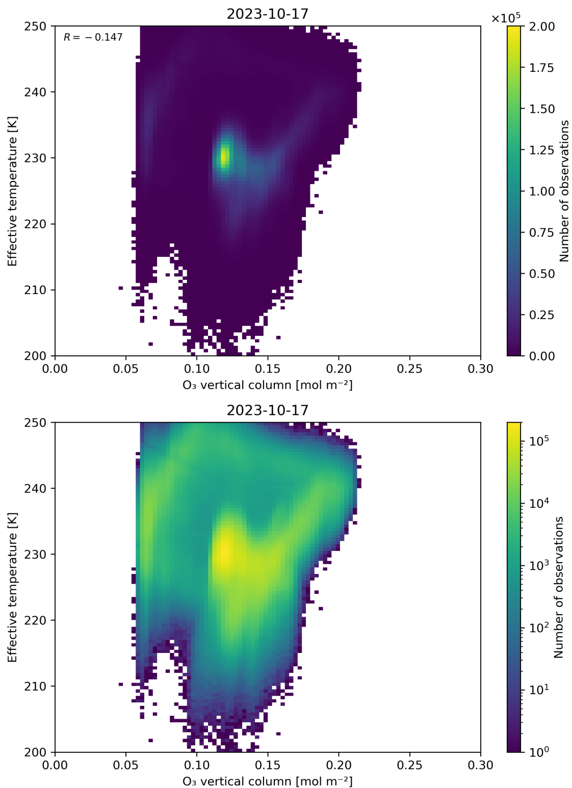
Figure 39: Scatter density plot of “O 3 vertical column” against “Effective temperature” for 2023-10-17 to 2023-10-18.
