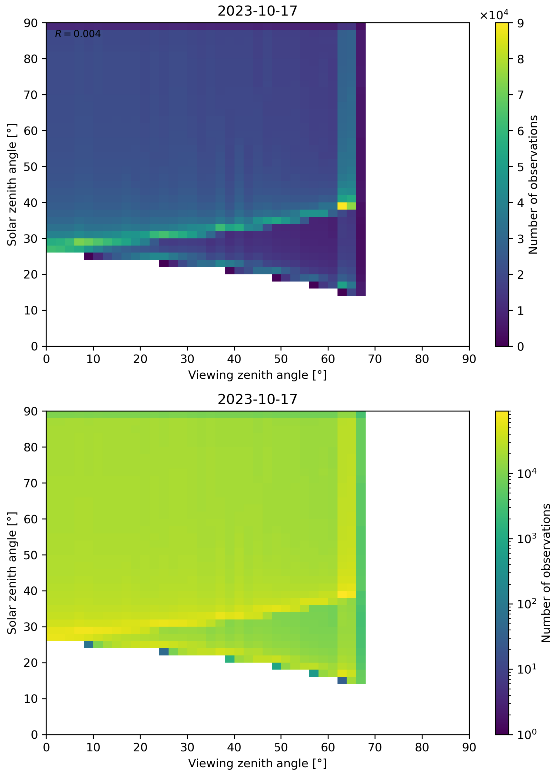
Figure 54: Scatter density plot of “Viewing zenith angle” against “Solar zenith angle” for 2023-10-17 to 2023-10-18.
