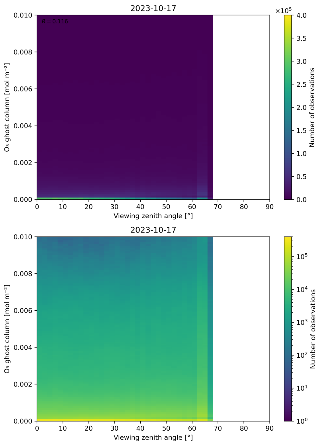
Figure 51: Scatter density plot of “Viewing zenith angle” against “O 3 ghost column” for 2023-10-17 to 2023-10-18.
