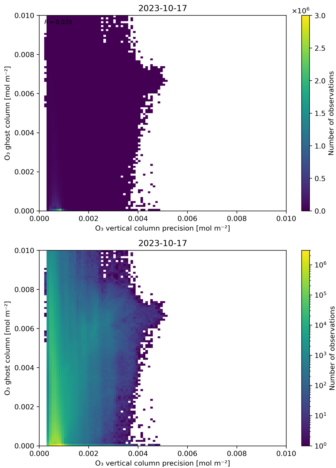
Figure 43: Scatter density plot of “O 3 vertical column precision” against “O 3 ghost column” for 2023-10-17 to 2023-10-18.
