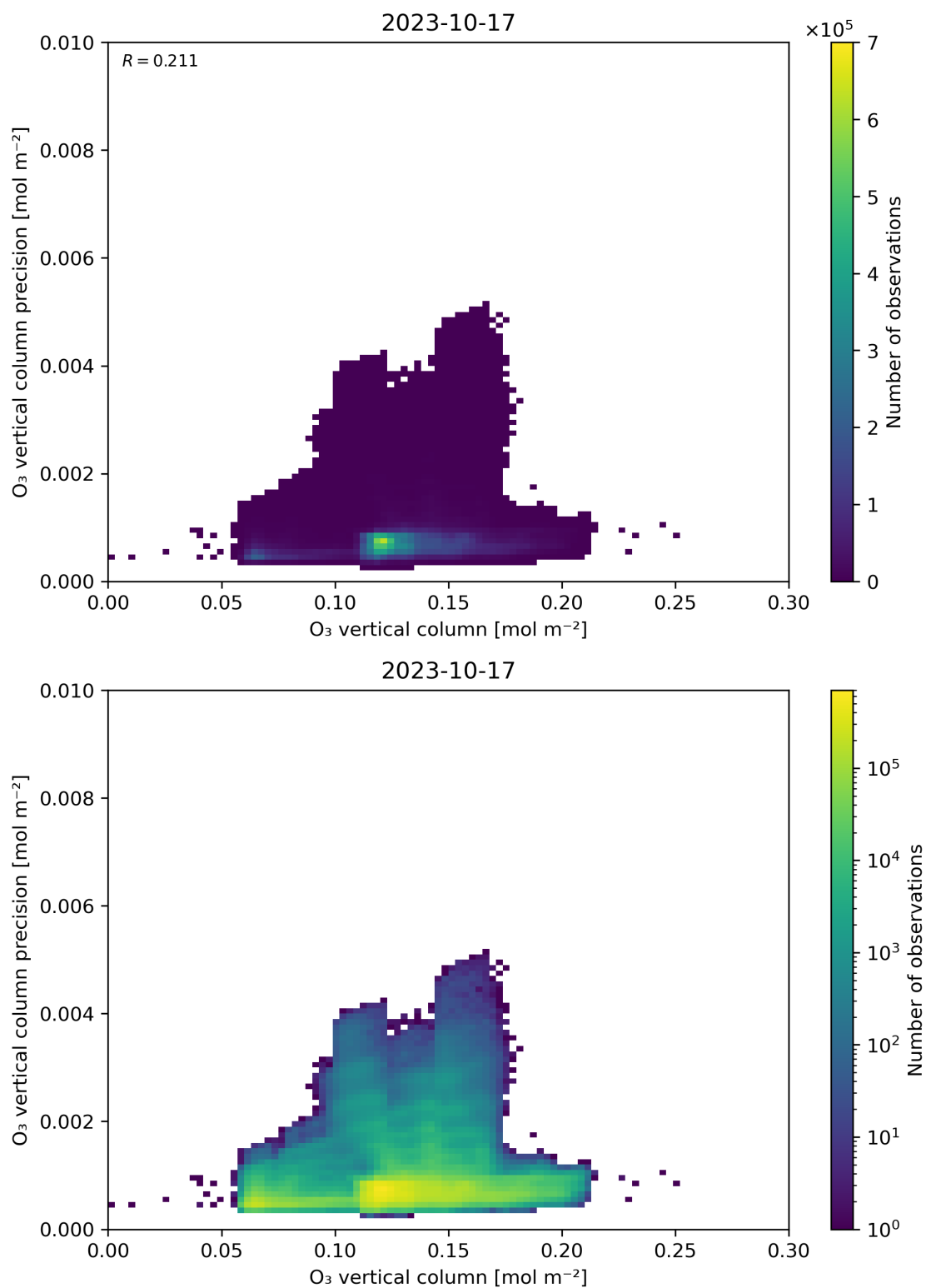
Figure 41: Scatter density plot of “O 3 vertical column” against “O 3 vertical column precision” for 2023-10-17 to 2023-10-18.
