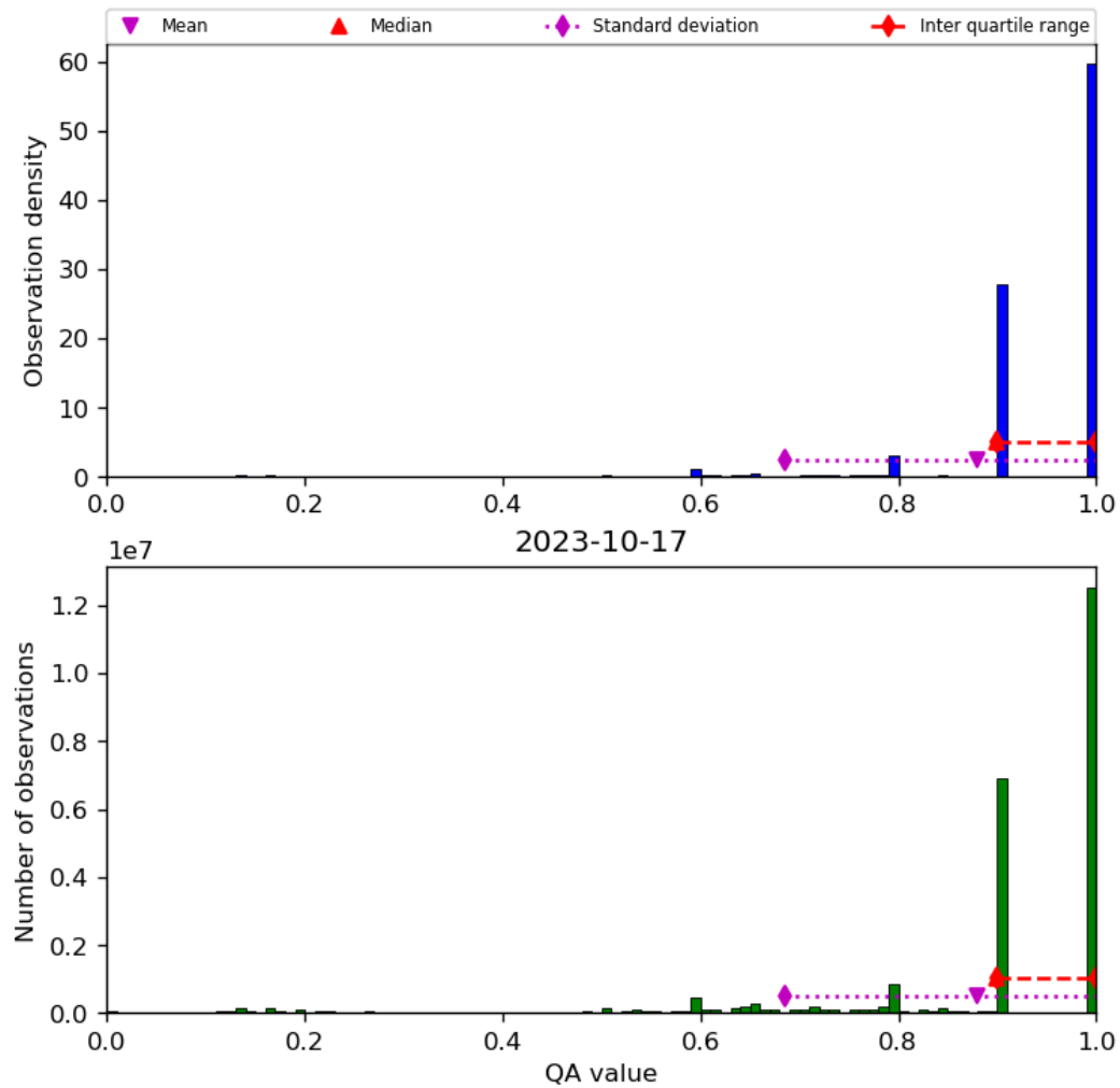
Figure 20: Histogram of “QA value” for 2023-10-17 to 2023-10-18
