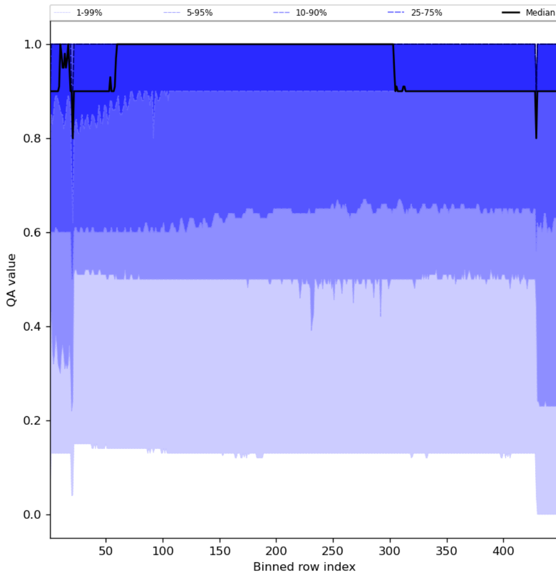
Figure 27: Along track statistics of “QA value” for 2023-10-17 to 2023-10-18
