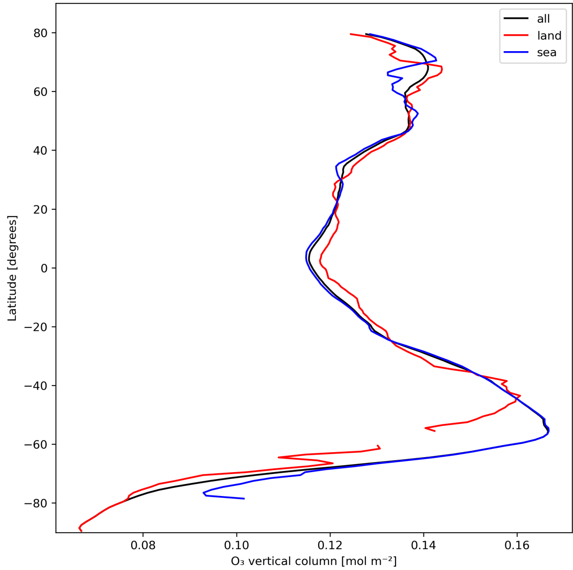
Figure 14: Zonal average of “O 3 vertical column” for 2023-10-17 to 2023-10-18.
