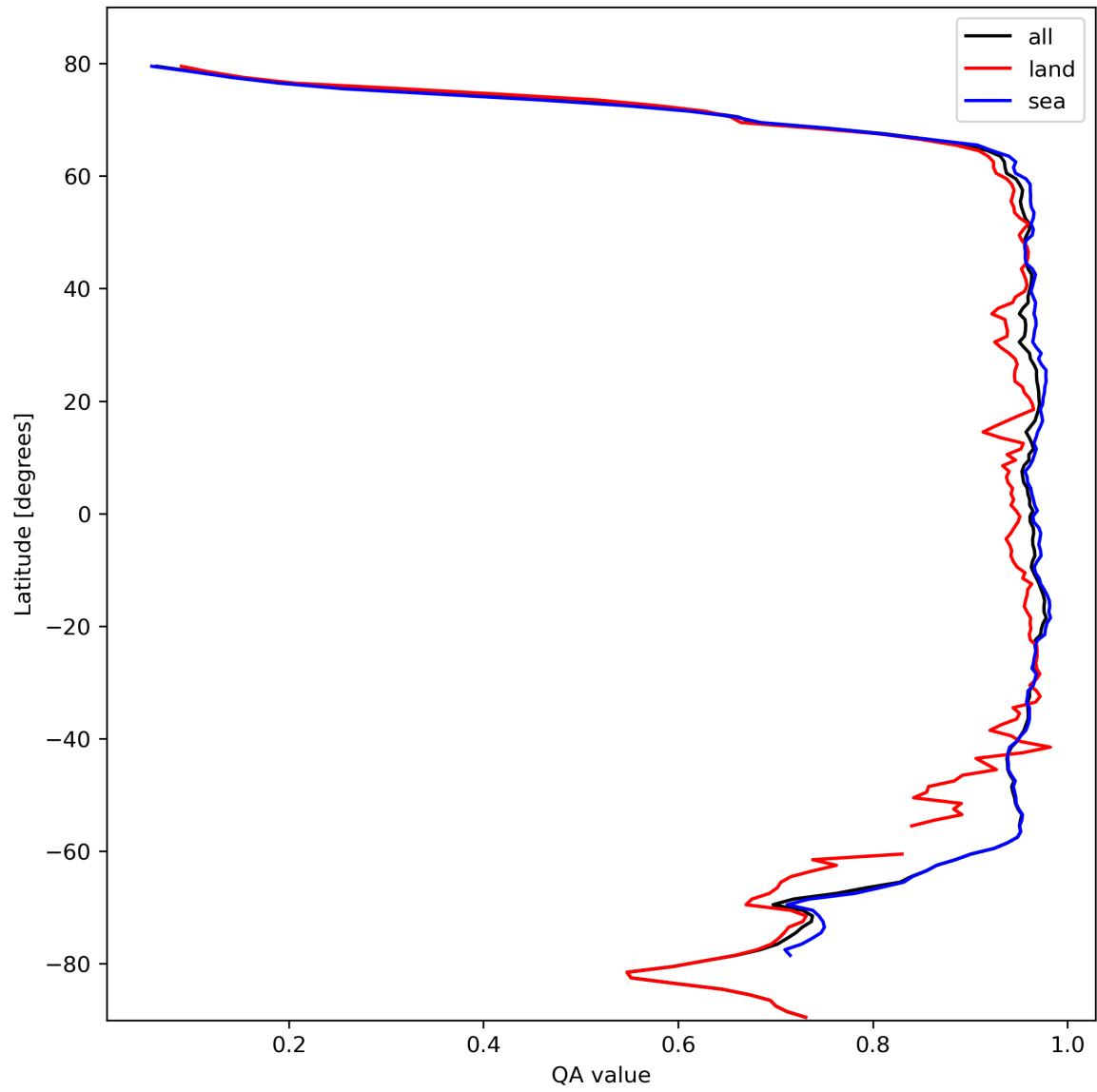
Figure 13: Zonal average of “QA value” for 2023-10-17 to 2023-10-18.
