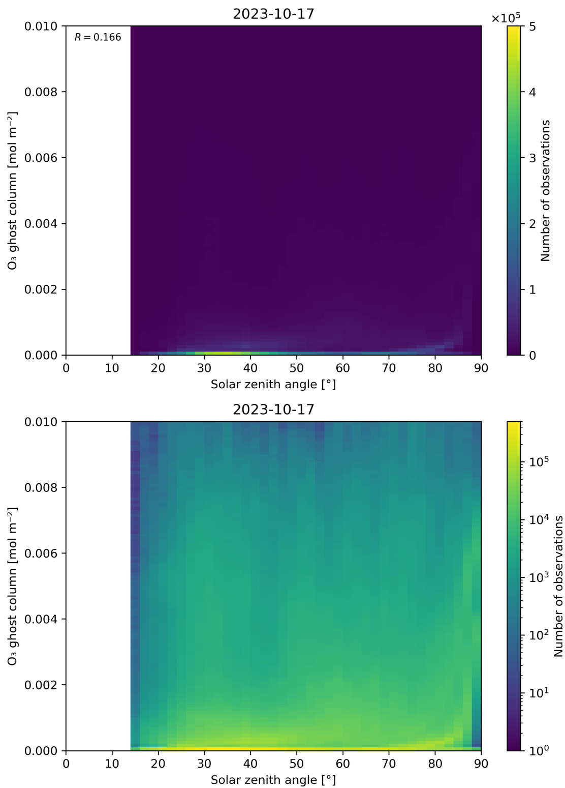
Figure 46: Scatter density plot of “Solar zenith angle” against “O 3 ghost column” for 2023-10-17 to 2023-10-18.
