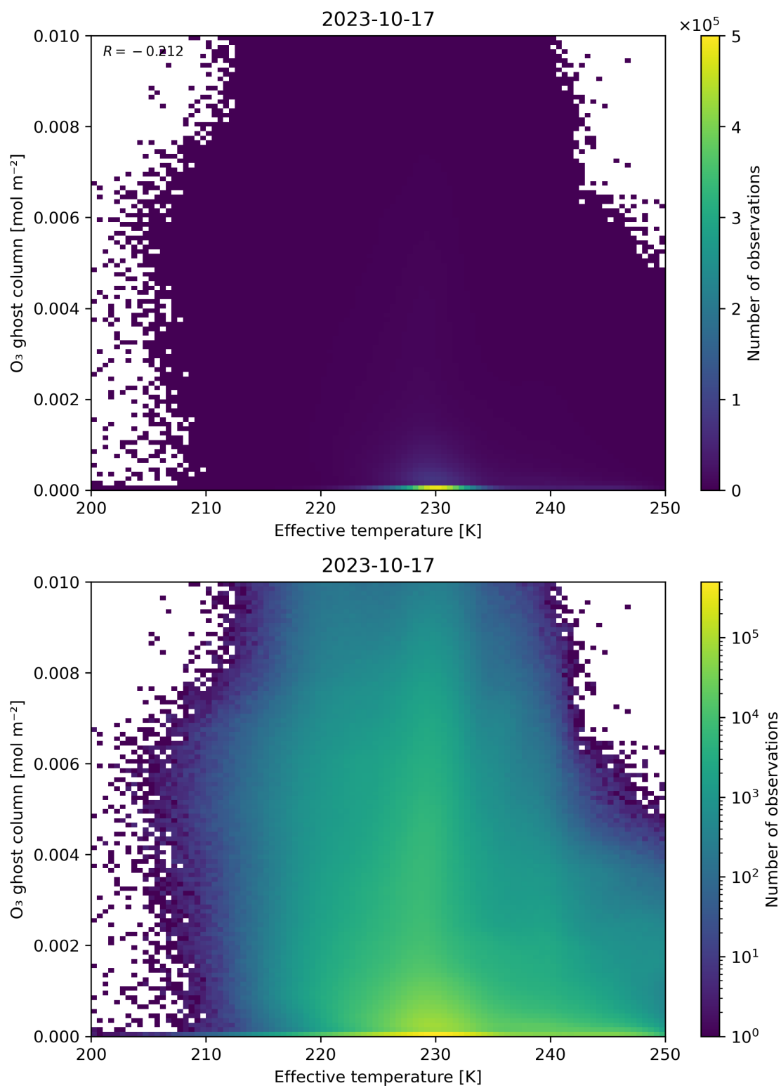
Figure 38: Scatter density plot of “Effective temperature” against “O 3 ghost column” for 2023-10-17 to 2023-10-18.
