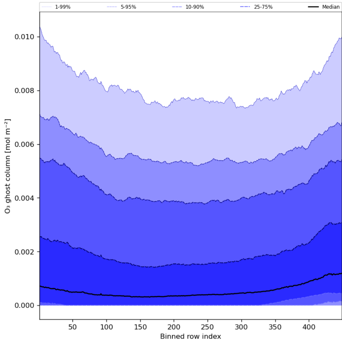
Figure 32: Along track statistics of “O 3 ghost column” for 2023-10-17 to 2023-10-18
