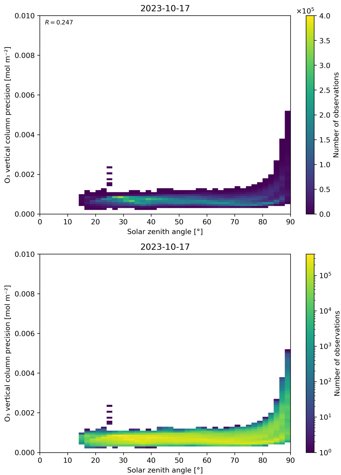
Figure 48: Scatter density plot of “Solar zenith angle” against “O 3 vertical column precision” for 2023-10-17 to 2023-10-18.
