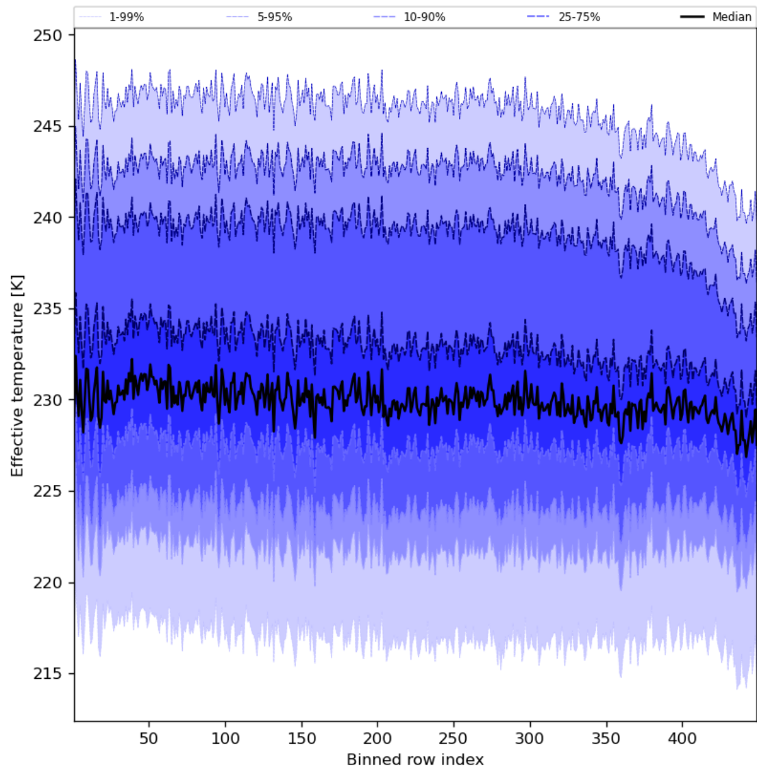
Figure 31: Along track statistics of “Effective temperature” for 2023-10-17 to 2023-10-19
