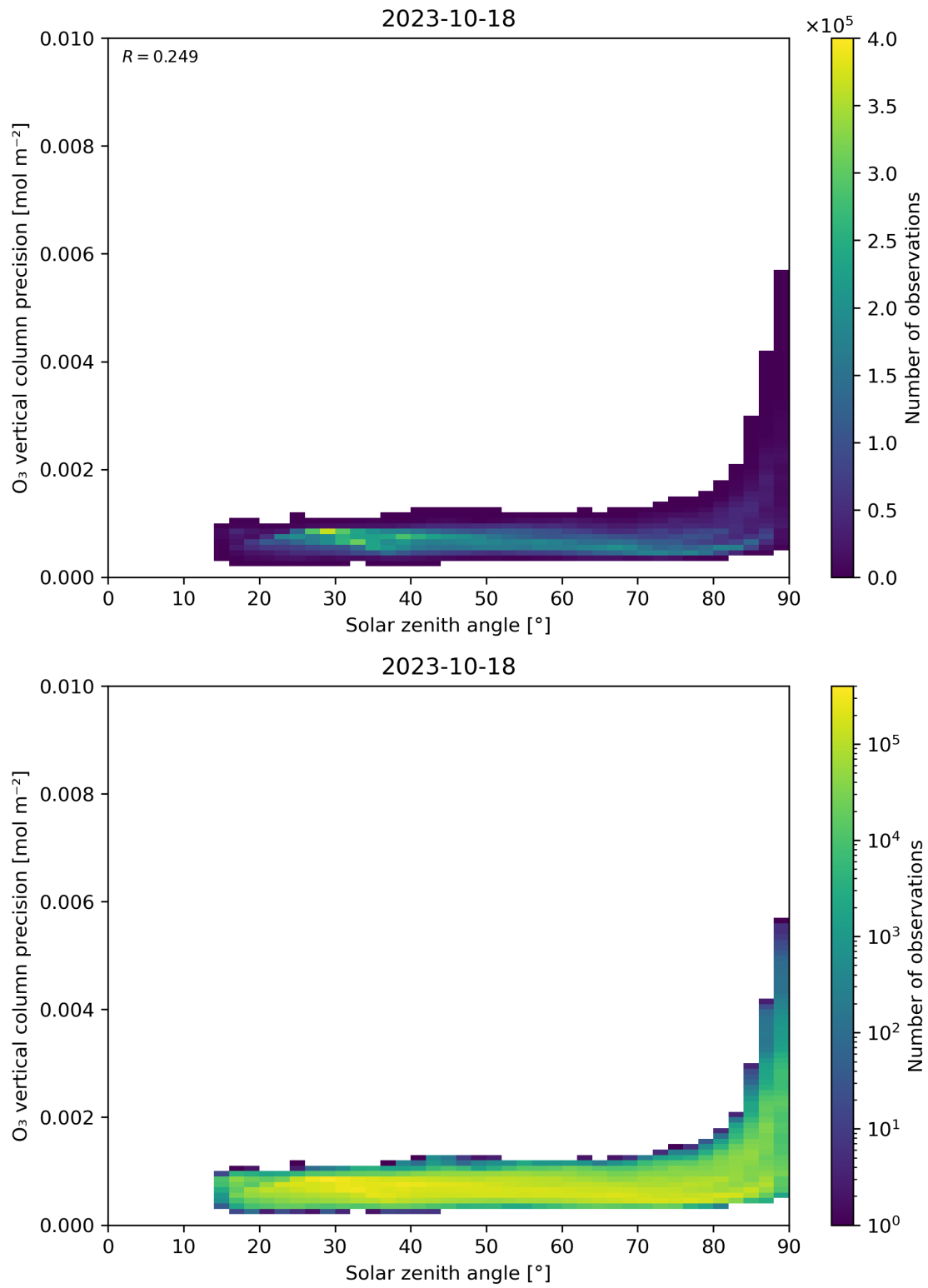
Figure 48: Scatter density plot of “Solar zenith angle” against “O 3 vertical column precision” for 2023-10-17 to 2023-10-19.
