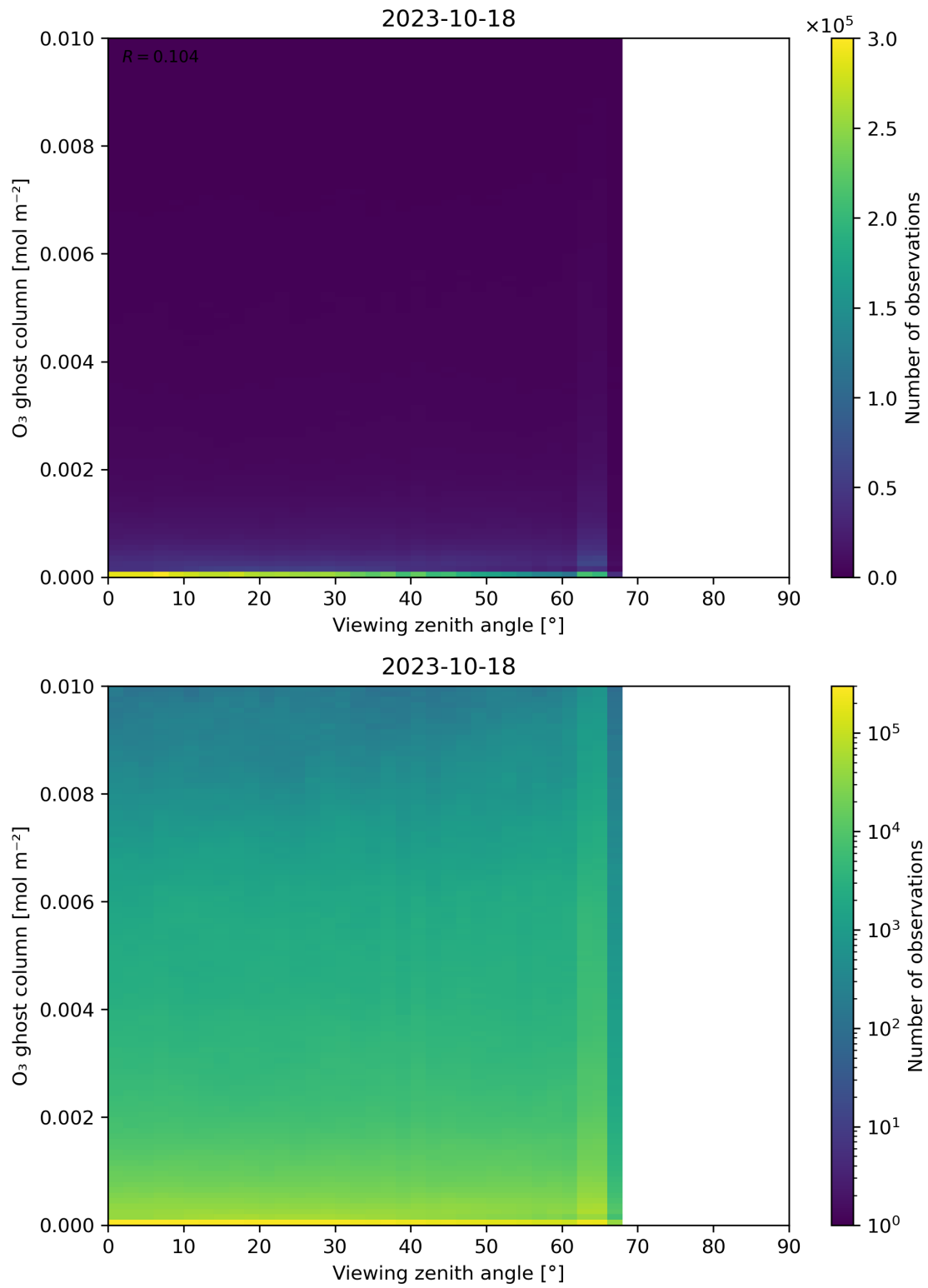
Figure 51: Scatter density plot of “Viewing zenith angle” against “O 3 ghost column” for 2023-10-17 to 2023-10-19.
