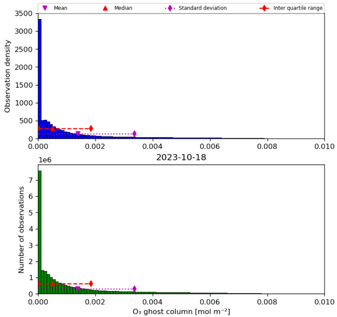
Figure 25: Histogram of “O 3 ghost column” for 2023-10-17 to 2023-10-19
