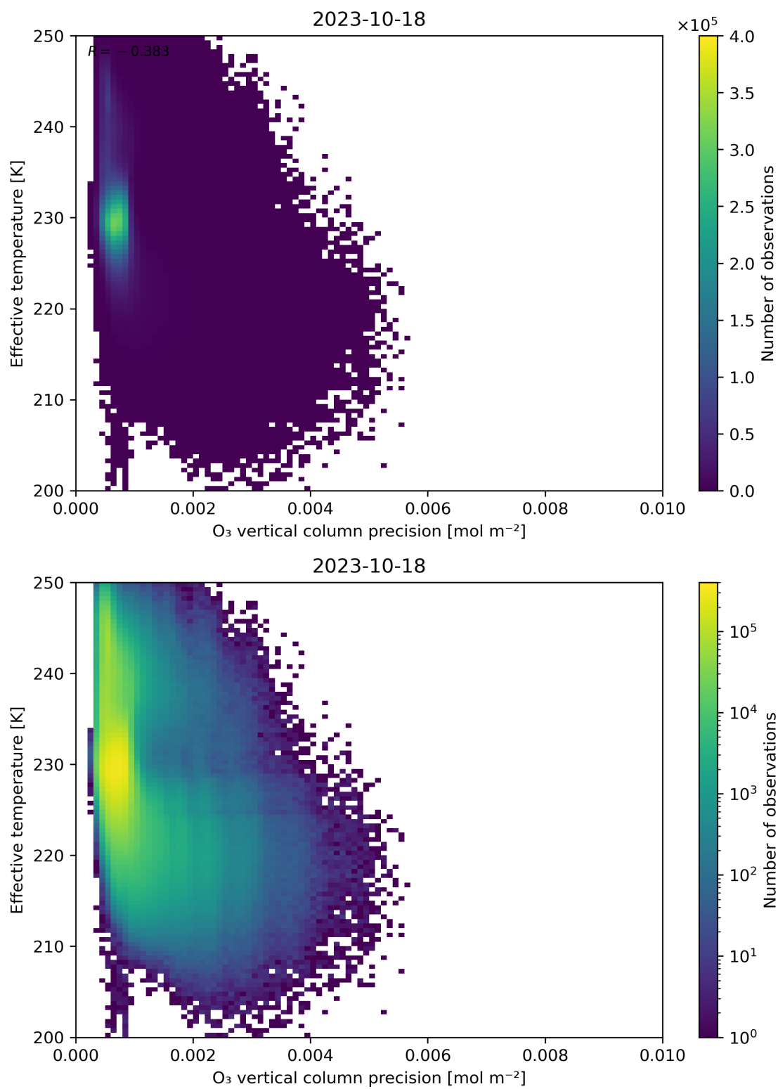
Figure 42: Scatter density plot of “O 3 vertical column precision” against “Effective temperature” for 2023-10-17 to 2023-10-19.
