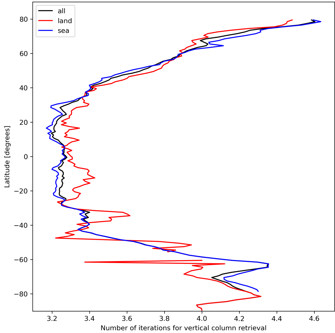
Figure 19: Zonal average of “Number of iterations for vertical column retrieval” for 2023-10-17 to 2023-10-19.
