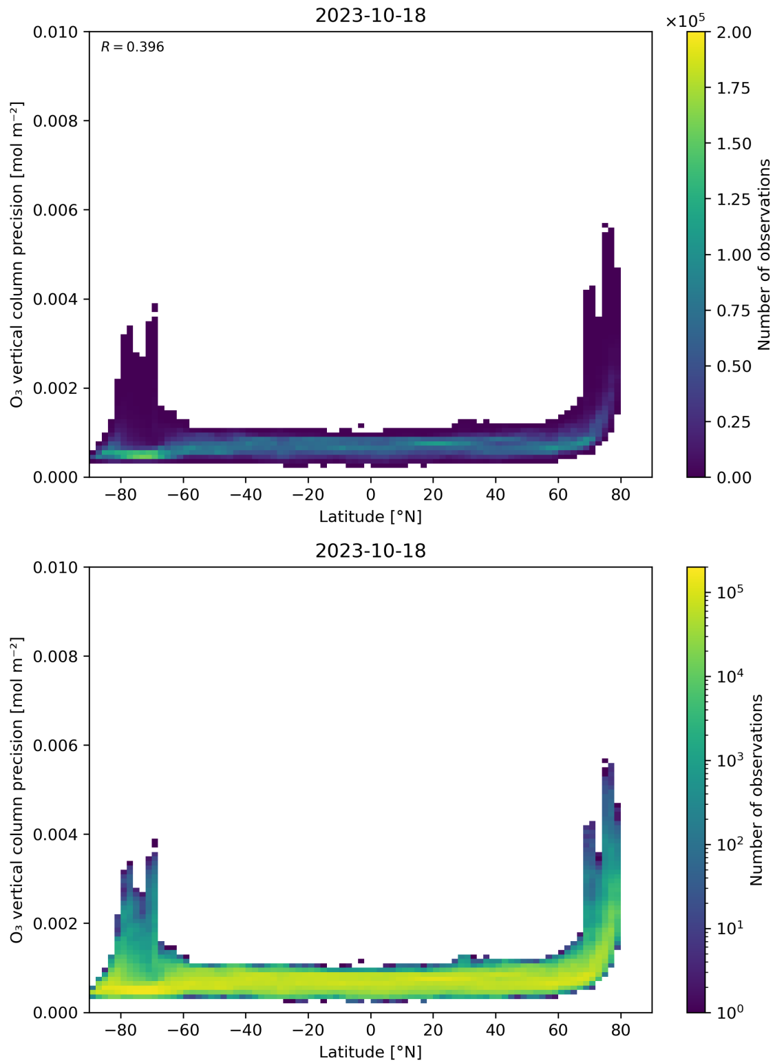
Figure 37: Scatter density plot of “Latitude” against “O 3 vertical column precision” for 2023-10-17 to 2023-10-19.
