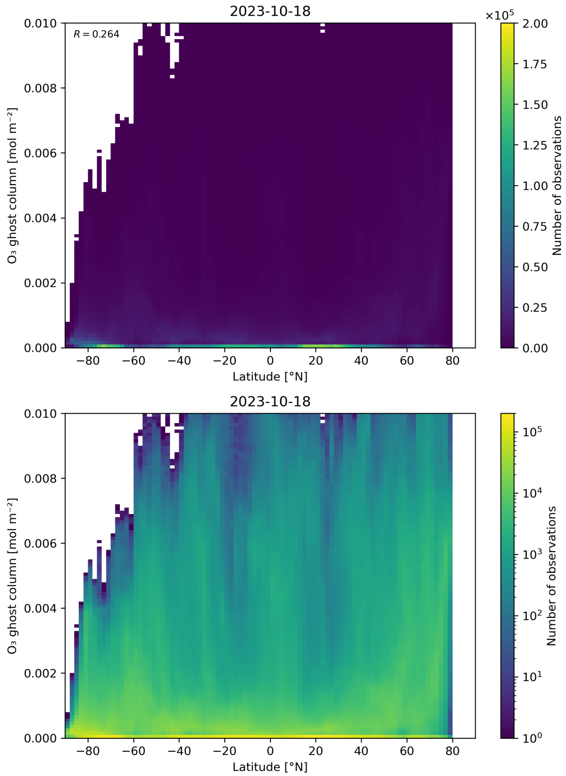
Figure 35: Scatter density plot of “Latitude” against “O 3 ghost column” for 2023-10-17 to 2023-10-19.
