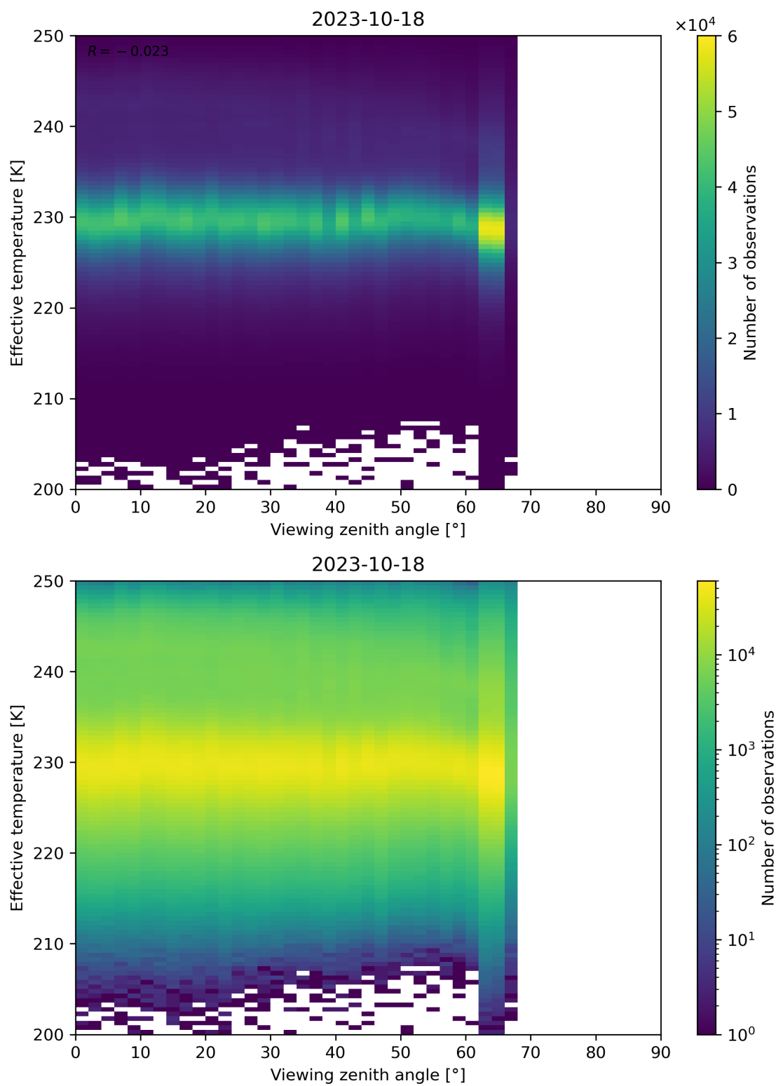
Figure 50: Scatter density plot of “Viewing zenith angle” against “Effective temperature” for 2023-10-17 to 2023-10-19.
