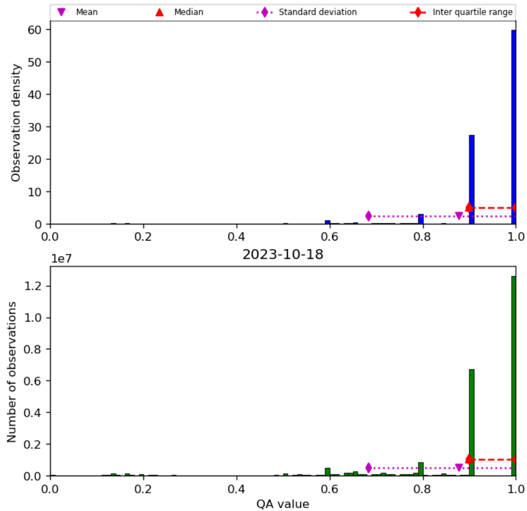
Figure 20: Histogram of “QA value” for 2023-10-17 to 2023-10-19
