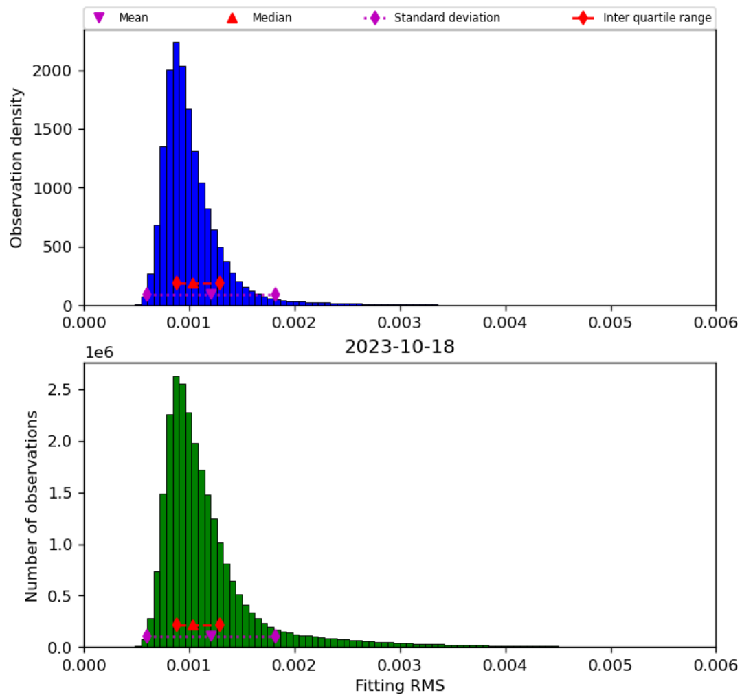
Figure 23: Histogram of “Fitting RMS” for 2023-10-17 to 2023-10-19
