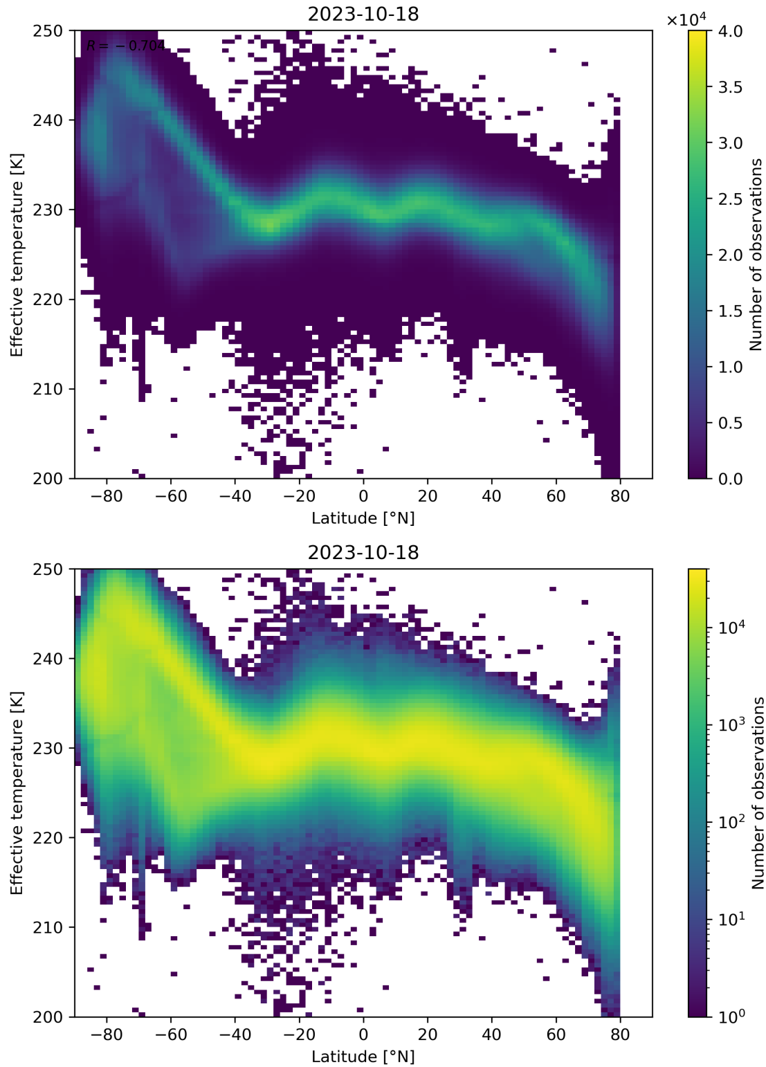
Figure 34: Scatter density plot of “Latitude” against “Effective temperature” for 2023-10-17 to 2023-10-19.
