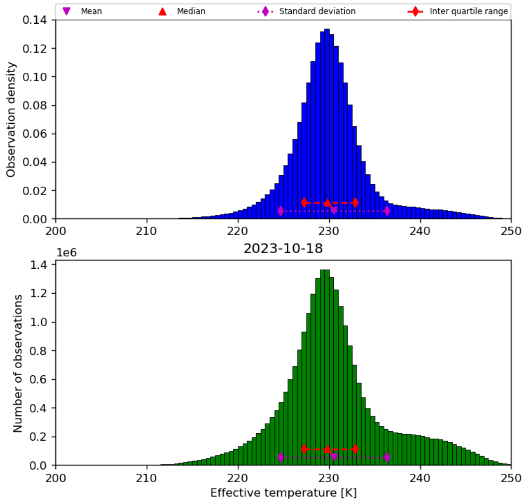
Figure 24: Histogram of “Effective temperature” for 2023-10-17 to 2023-10-19
