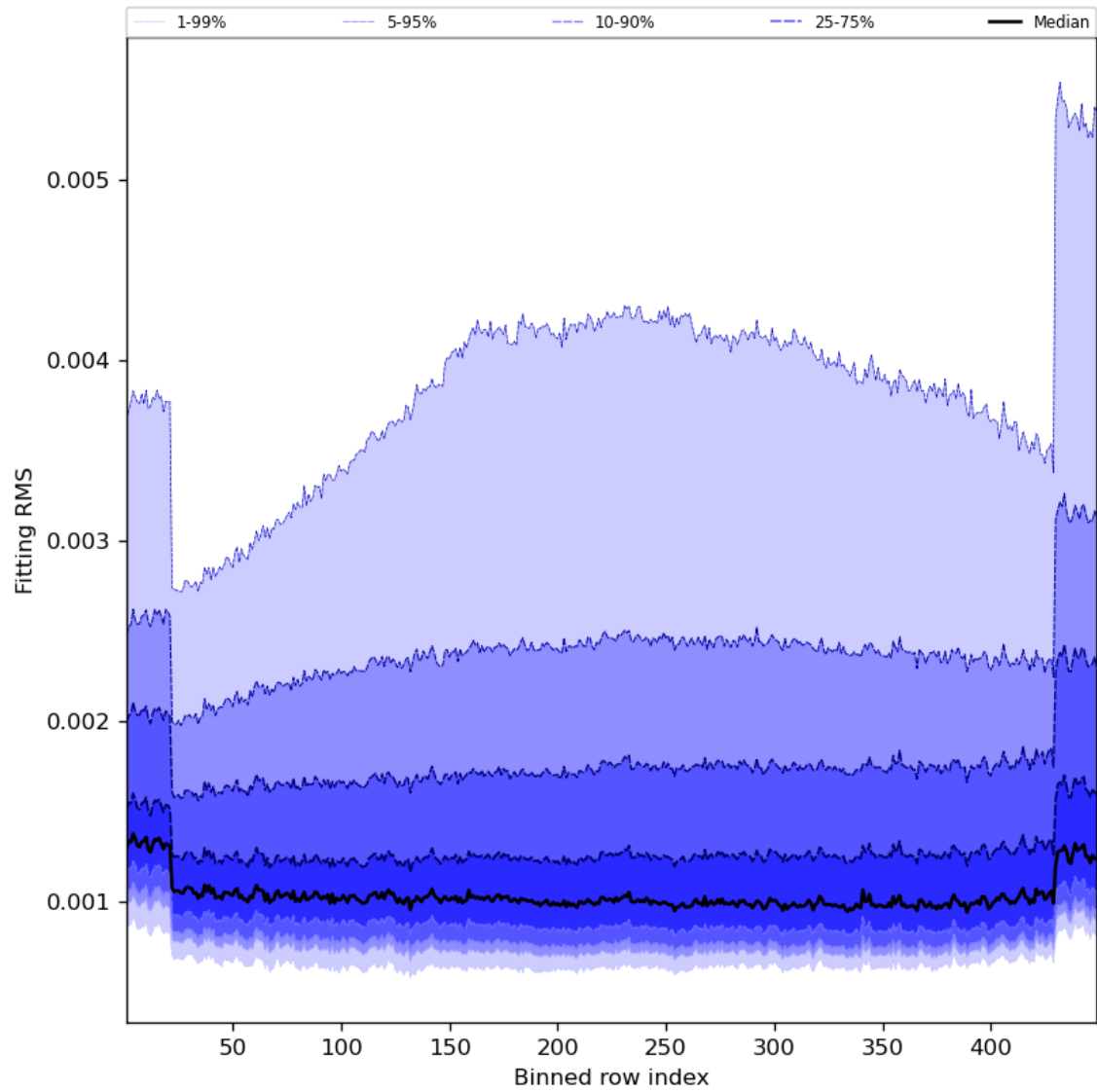
Figure 30: Along track statistics of “Fitting RMS” for 2023-10-17 to 2023-10-19
