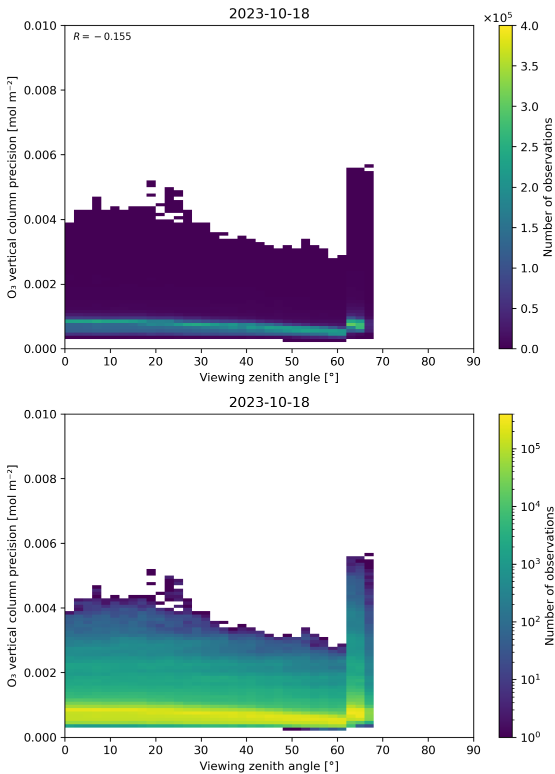
Figure 53: Scatter density plot of “Viewing zenith angle” against “O 3 vertical column precision” for 2023-10-17 to 2023-10-19.
