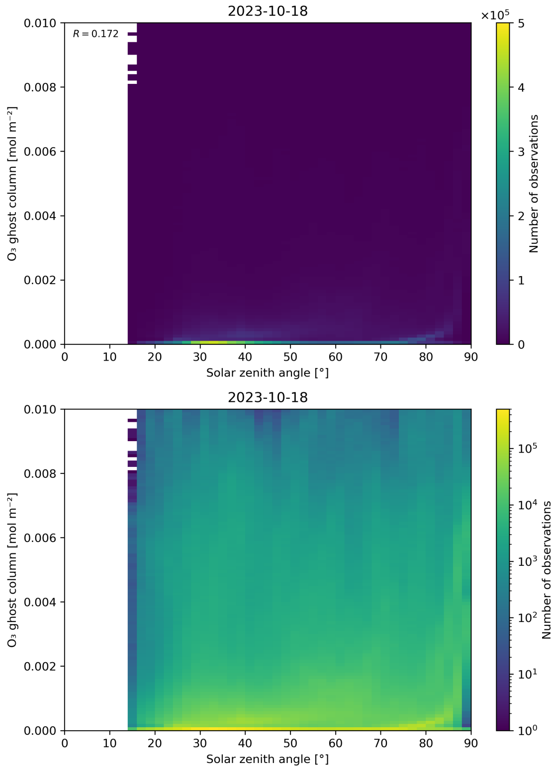
Figure 46: Scatter density plot of “Solar zenith angle” against “O 3 ghost column” for 2023-10-17 to 2023-10-19.
