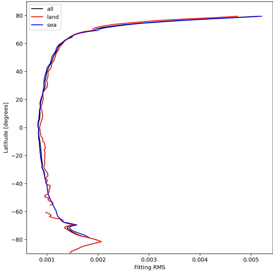
Figure 16: Zonal average of “Fitting RMS” for 2023-10-17 to 2023-10-19.
