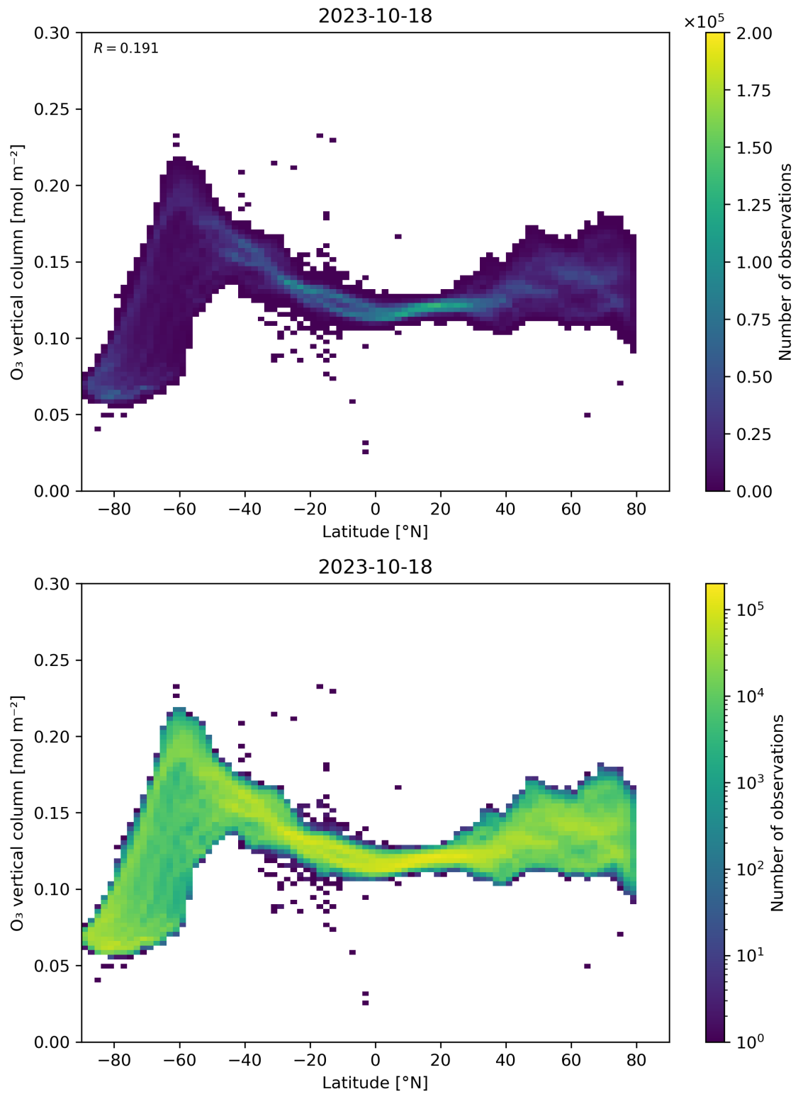
Figure 36: Scatter density plot of “Latitude” against “O 3 vertical column” for 2023-10-17 to 2023-10-19.
