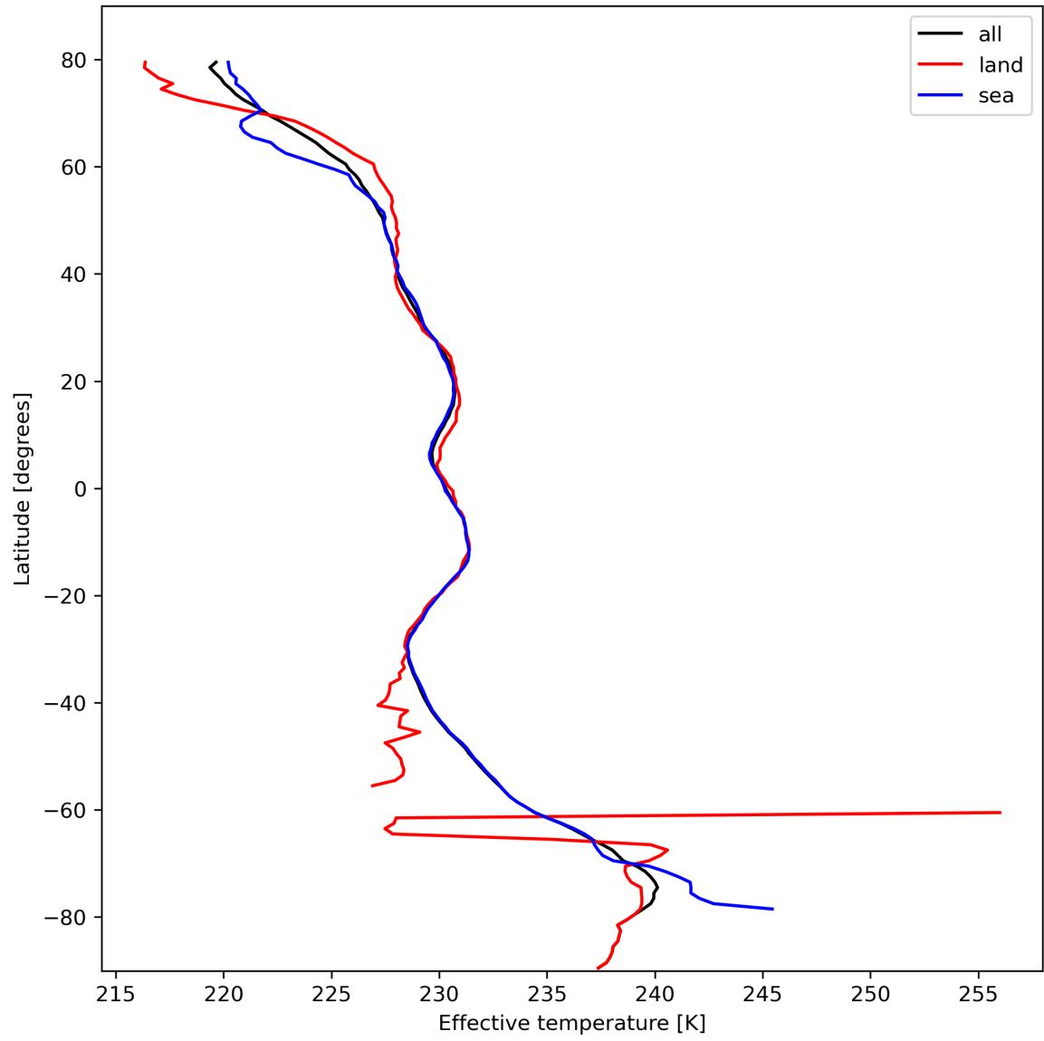
Figure 17: Zonal average of "Effective temperature" for 2023-10-17 to 2023-10-19.
