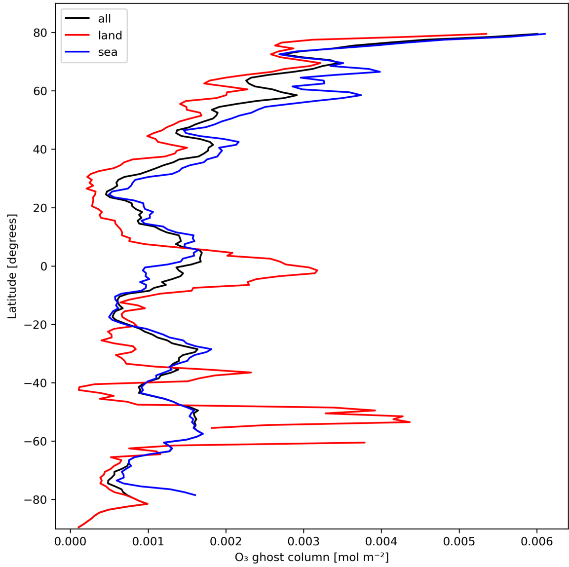
Figure 18: Zonal average of “O 3 ghost column” for 2023-10-17 to 2023-10-19.
