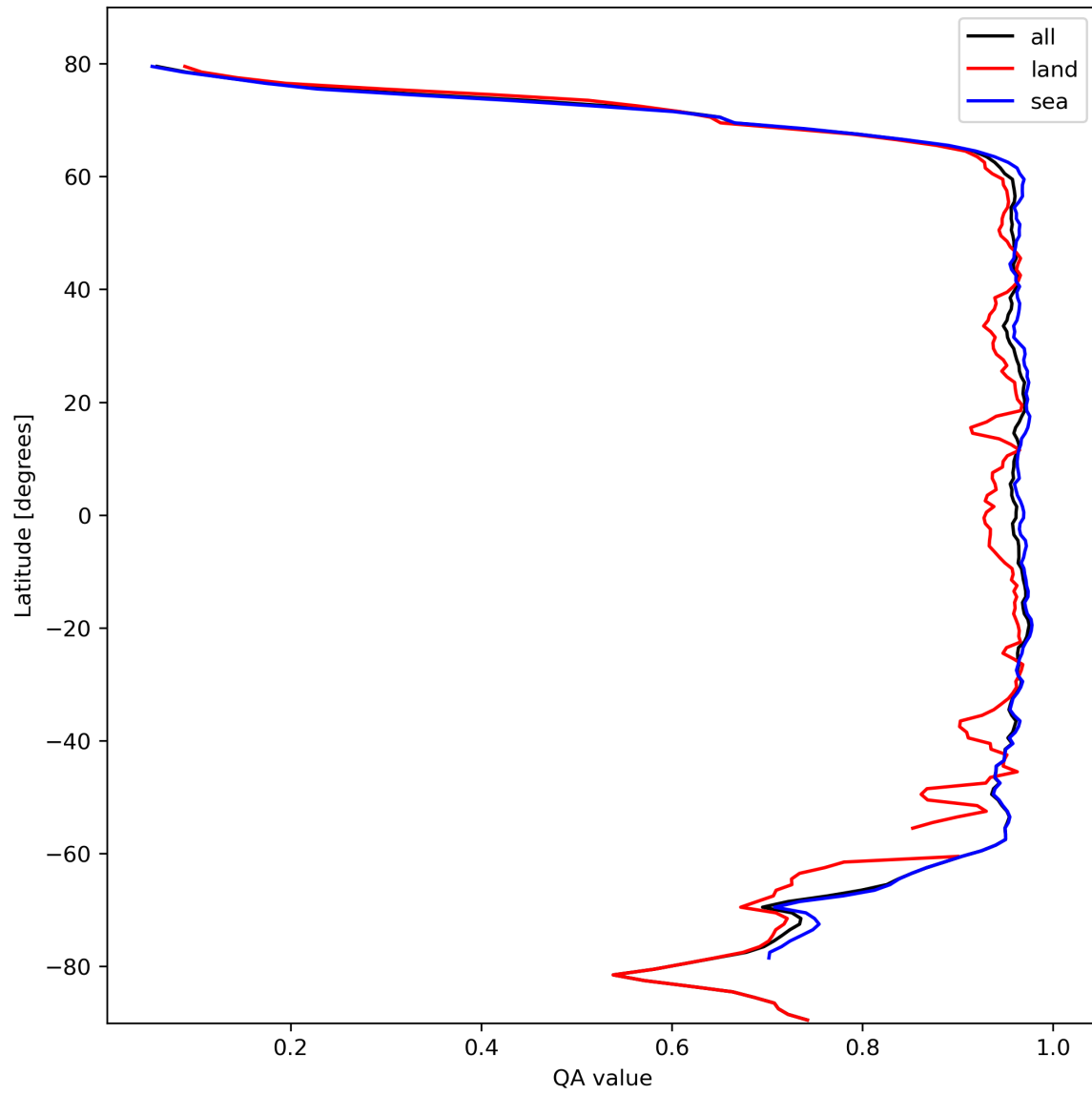
Figure 13: Zonal average of “QA value” for 2023-10-17 to 2023-10-19.
