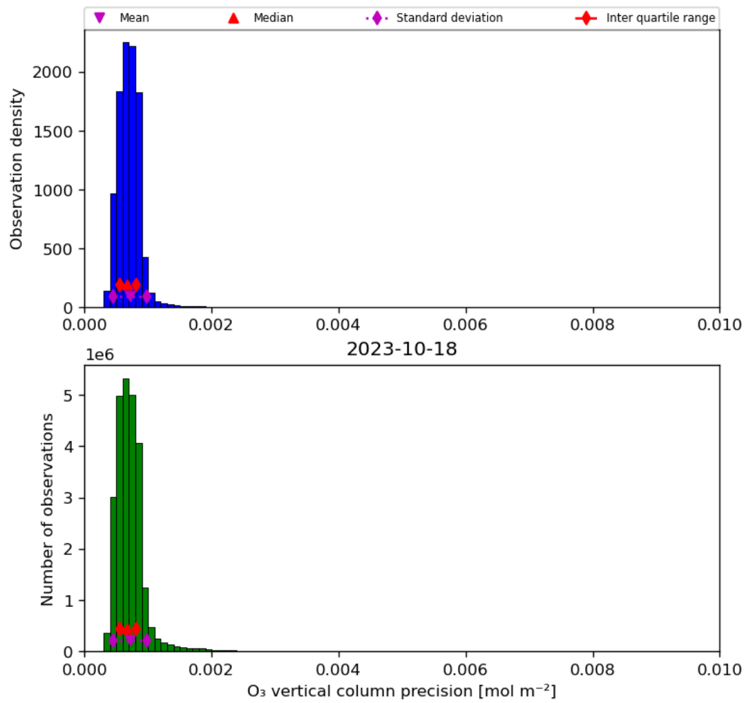
Figure 22: Histogram of “O 3 vertical column precision” for 2023-10-17 to 2023-10-19
