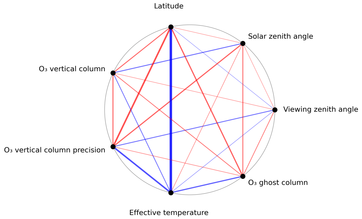
Figure 1: Map of correlation graph for 2023-10-17 to 2023-10-19.
