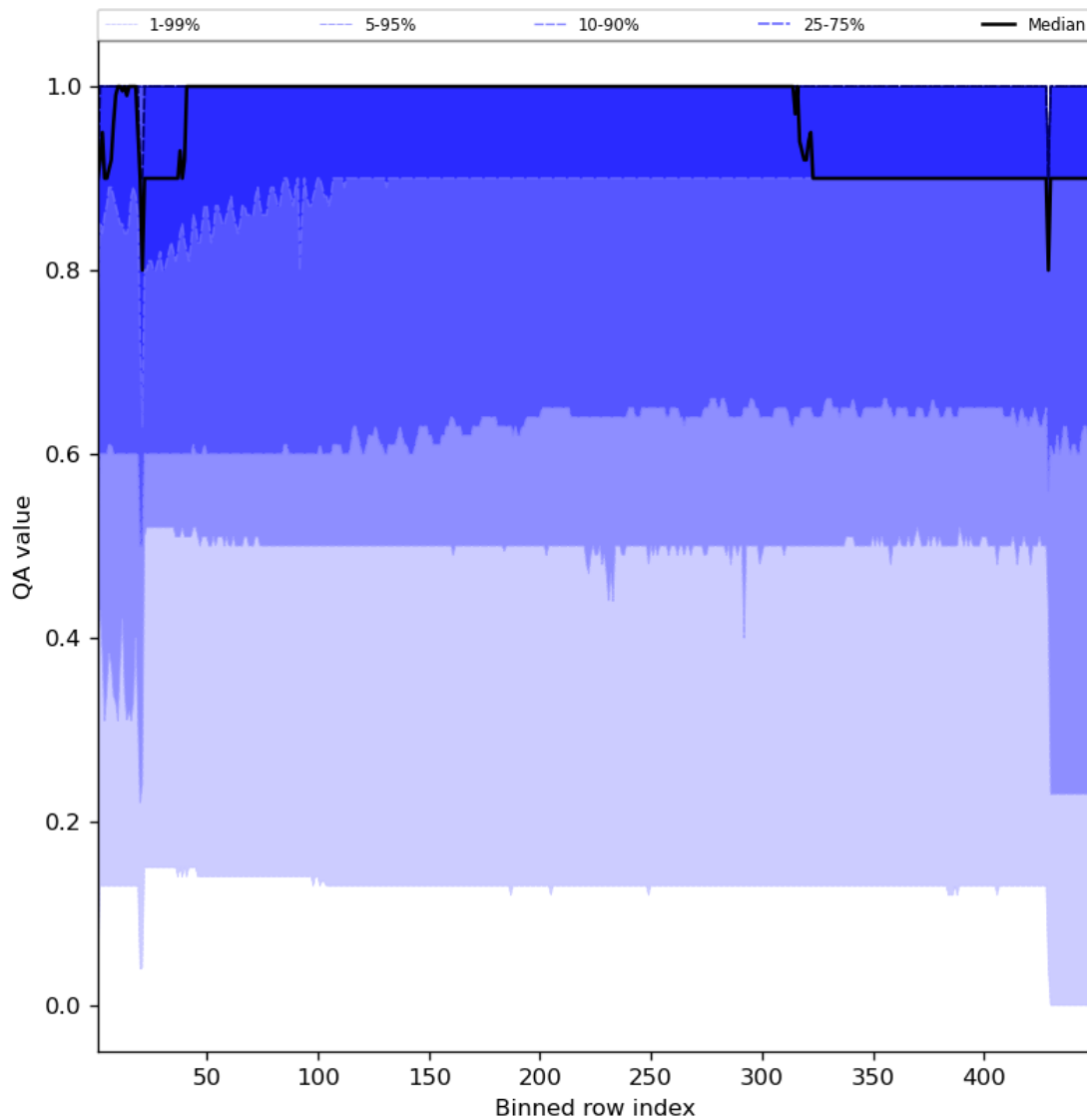
Figure 27: Along track statistics of “QA value” for 2023-10-17 to 2023-10-19
