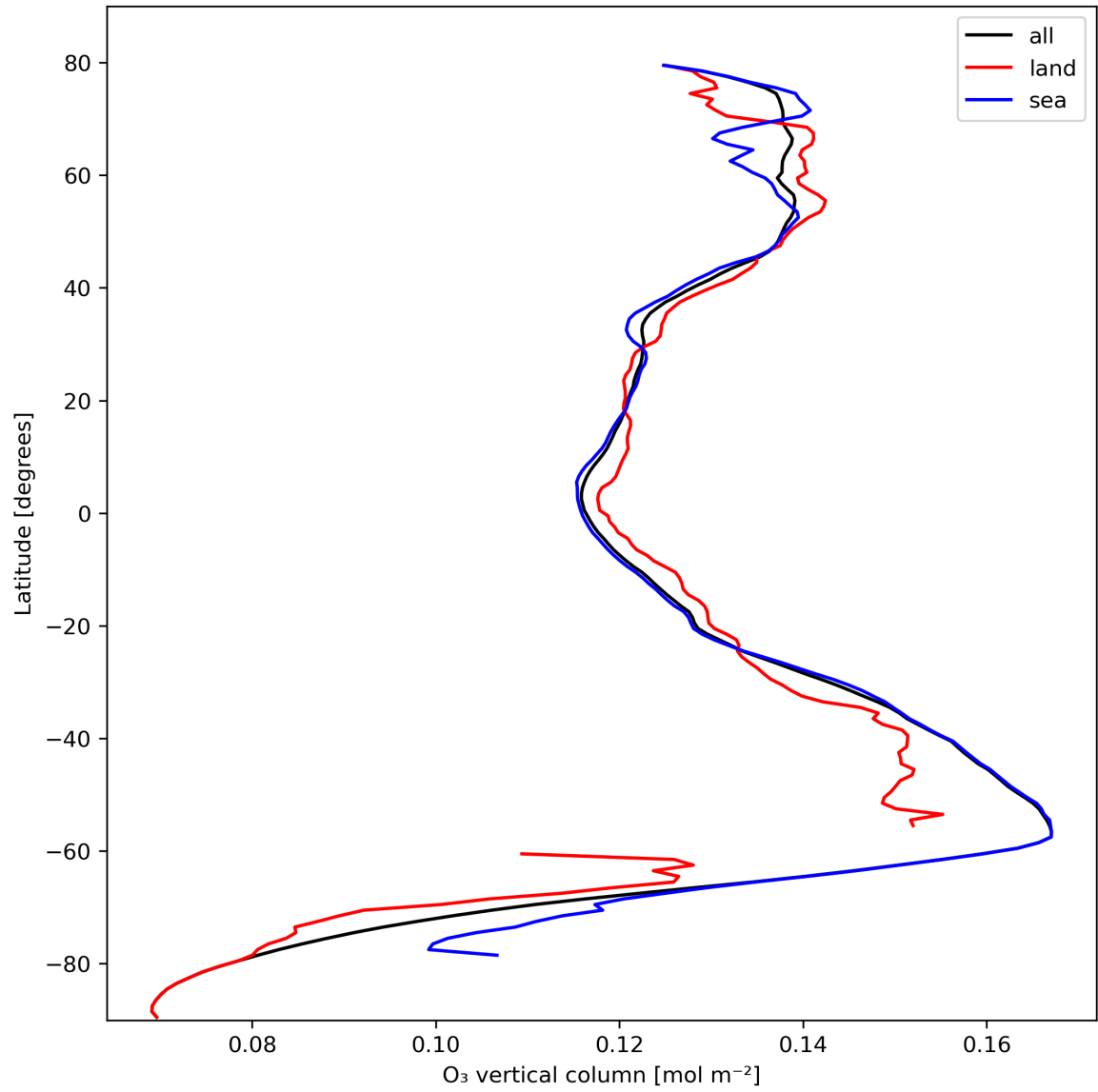
Figure 14: Zonal average of “O 3 vertical column” for 2023-10-17 to 2023-10-19.
