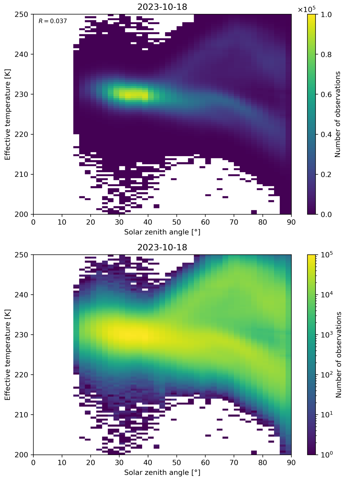
Figure 45: Scatter density plot of “Solar zenith angle” against “Effective temperature” for 2023-10-17 to 2023-10-19.
