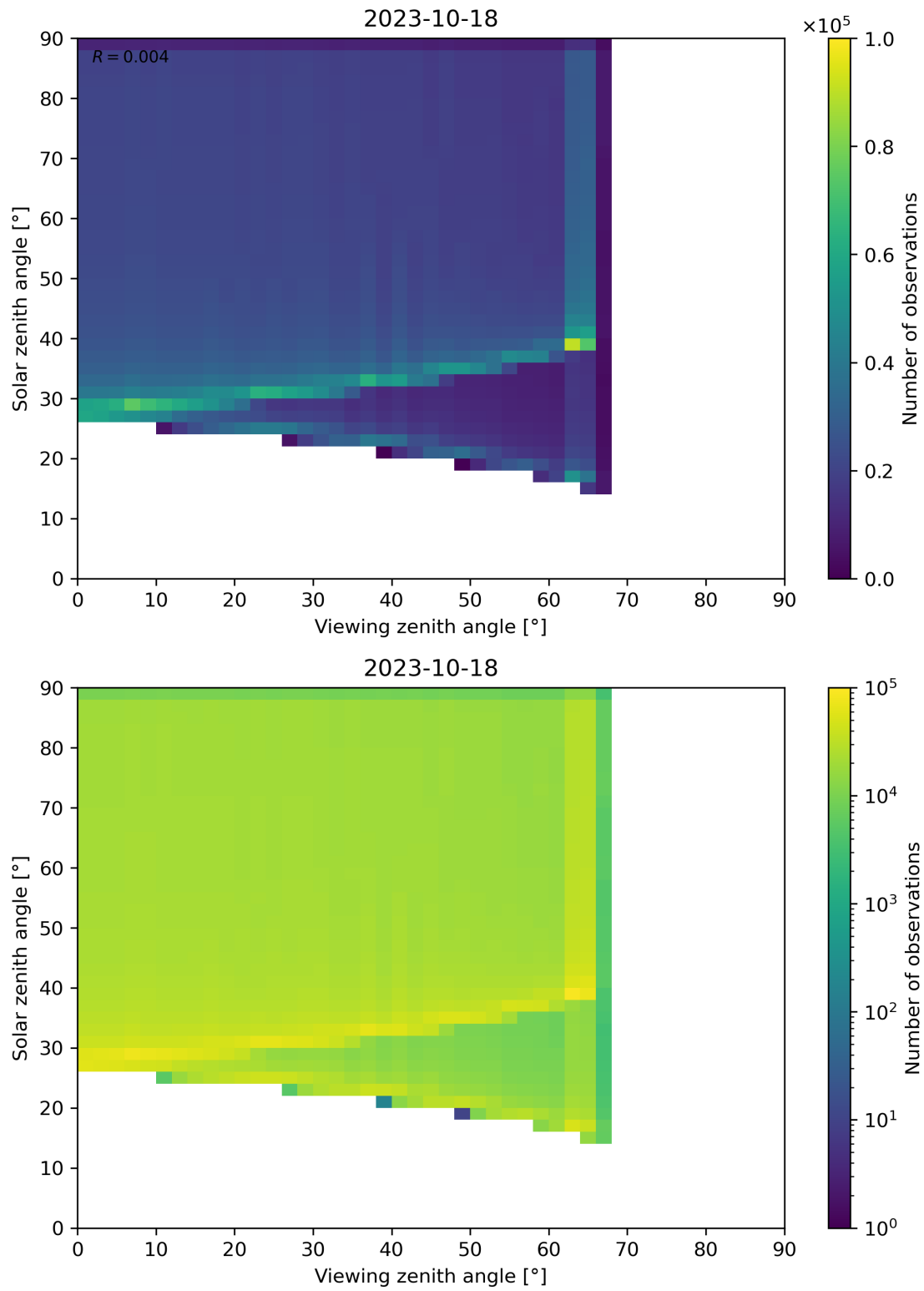
Figure 54: Scatter density plot of “Viewing zenith angle” against “Solar zenith angle” for 2023-10-17 to 2023-10-19.
