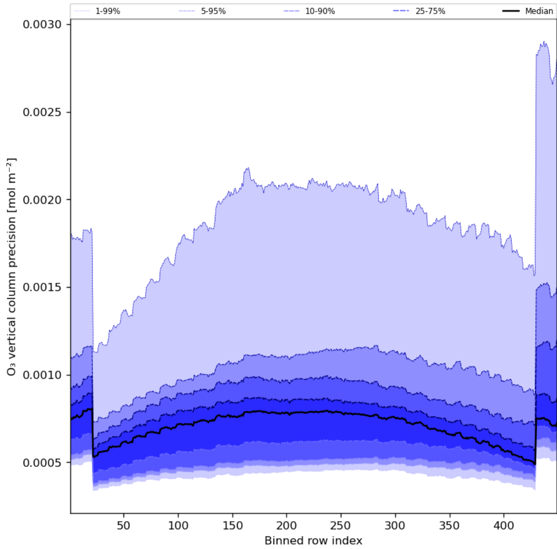
Figure 29: Along track statistics of “O 3 vertical column precision” for 2023-10-17 to 2023-10-19
