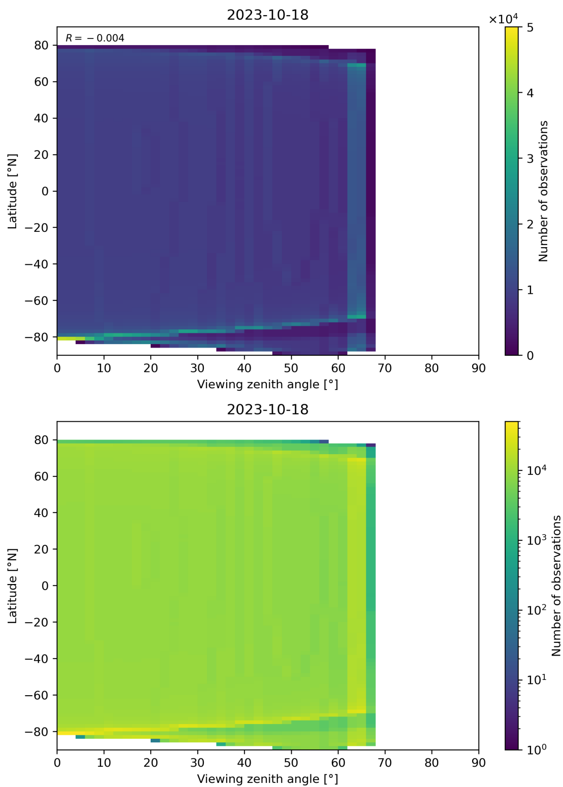
Figure 49: Scatter density plot of “Viewing zenith angle” against “Latitude” for 2023-10-17 to 2023-10-19.
