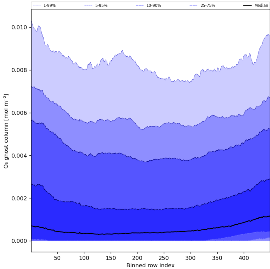
Figure 32: Along track statistics of “O 3 ghost column” for 2023-10-17 to 2023-10-19
