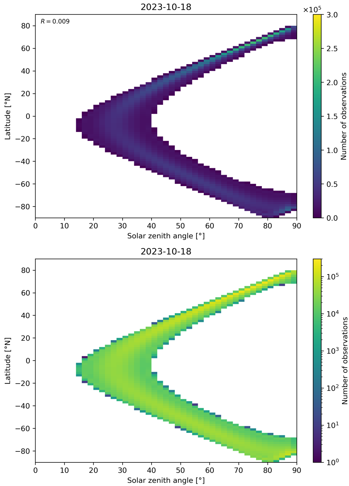
Figure 44: Scatter density plot of “Solar zenith angle” against “Latitude” for 2023-10-17 to 2023-10-19.
