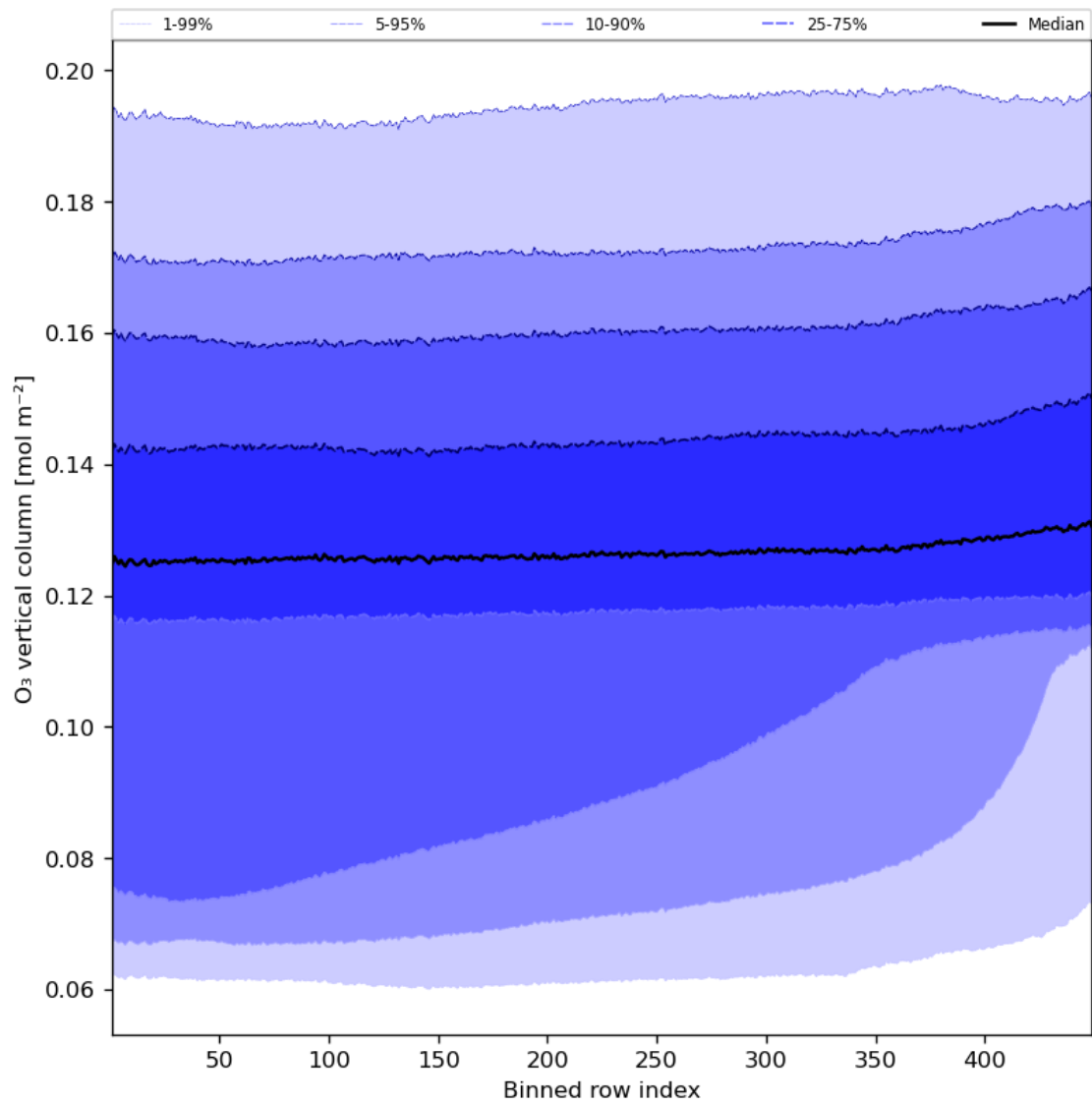
Figure 28: Along track statistics of “O 3 vertical column” for 2023-10-17 to 2023-10-19
