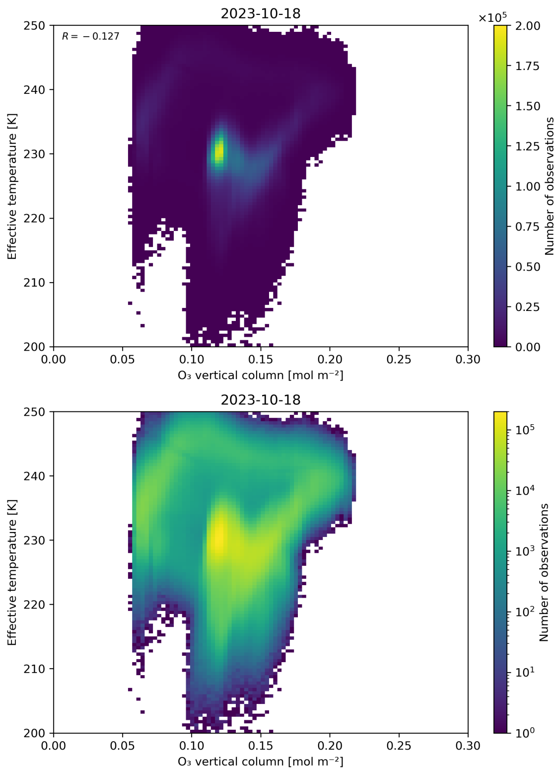
Figure 39: Scatter density plot of “O 3 vertical column” against “Effective temperature” for 2023-10-17 to 2023-10-19.
