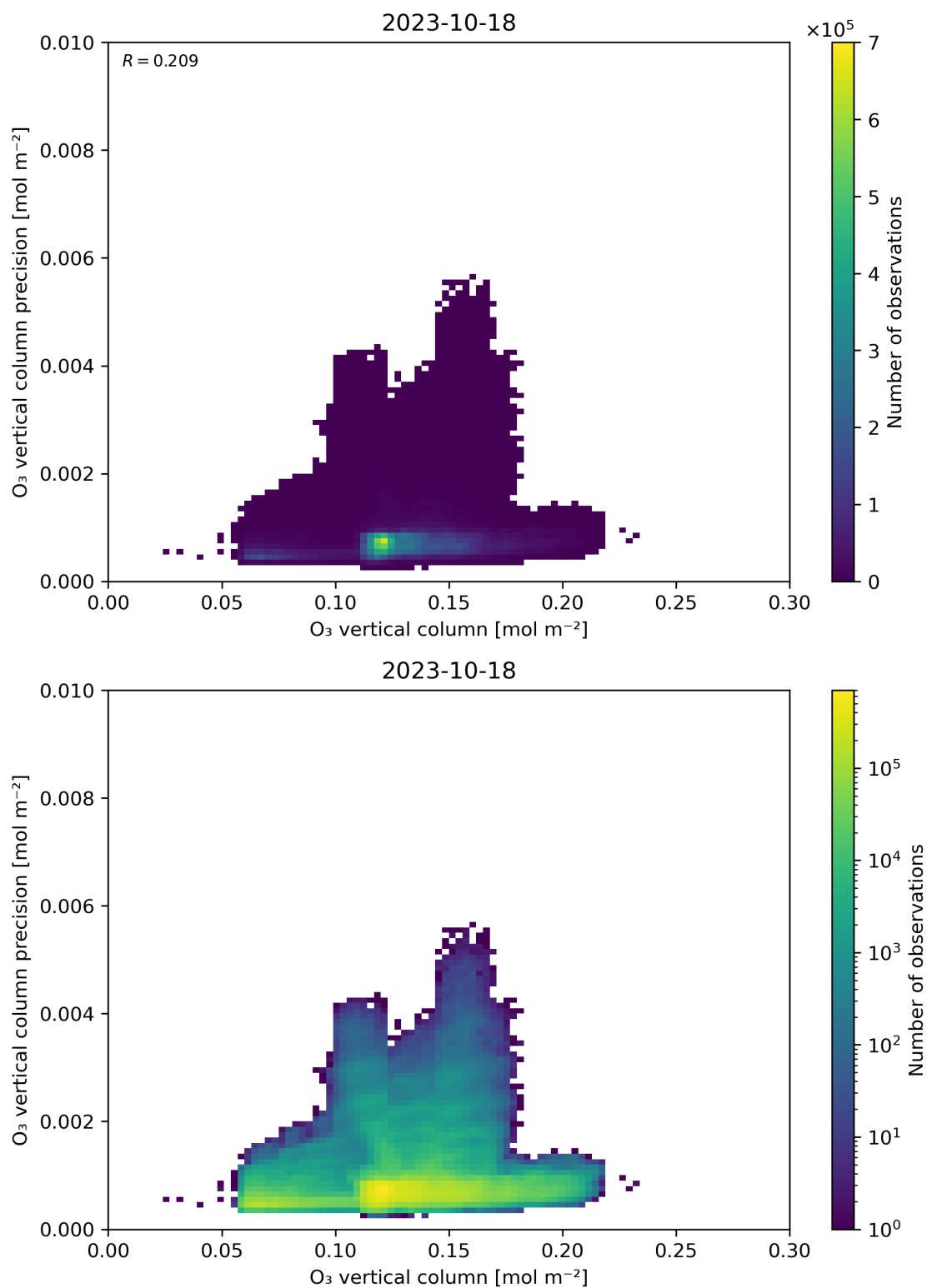
Figure 41: Scatter density plot of “O 3 vertical column” against “O 3 vertical column precision” for 2023-10-17 to 2023-10-19.
