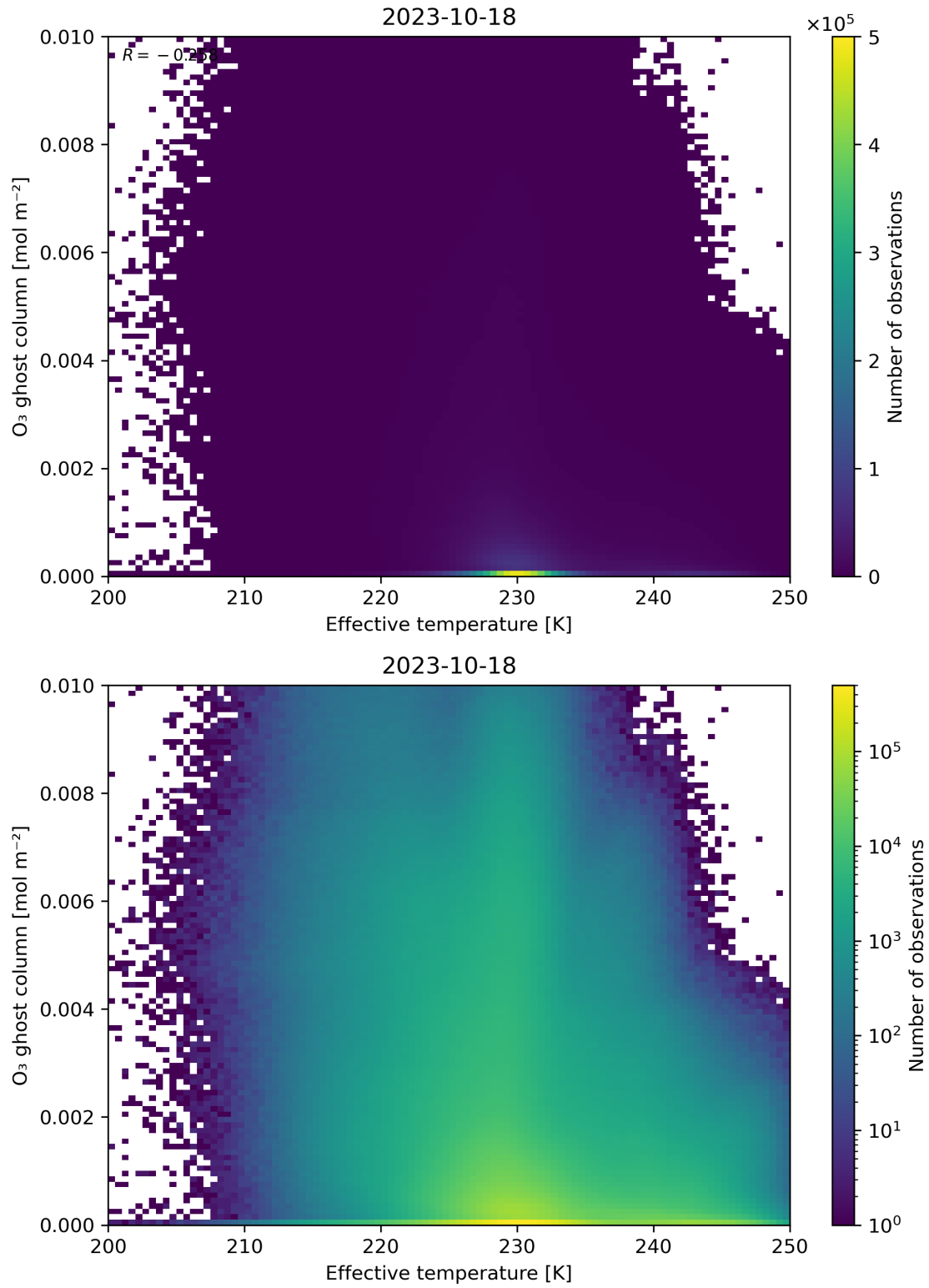
Figure 38: Scatter density plot of “Effective temperature” against “O 3 ghost column” for 2023-10-17 to 2023-10-19.
