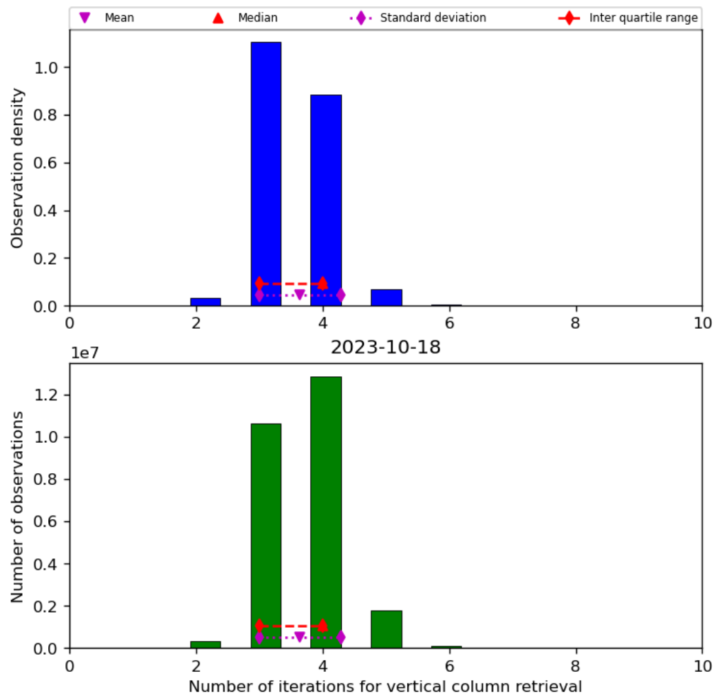
Figure 26: Histogram of “Number of iterations for vertical column retrieval” for 2023-10-17 to 2023-10-19
