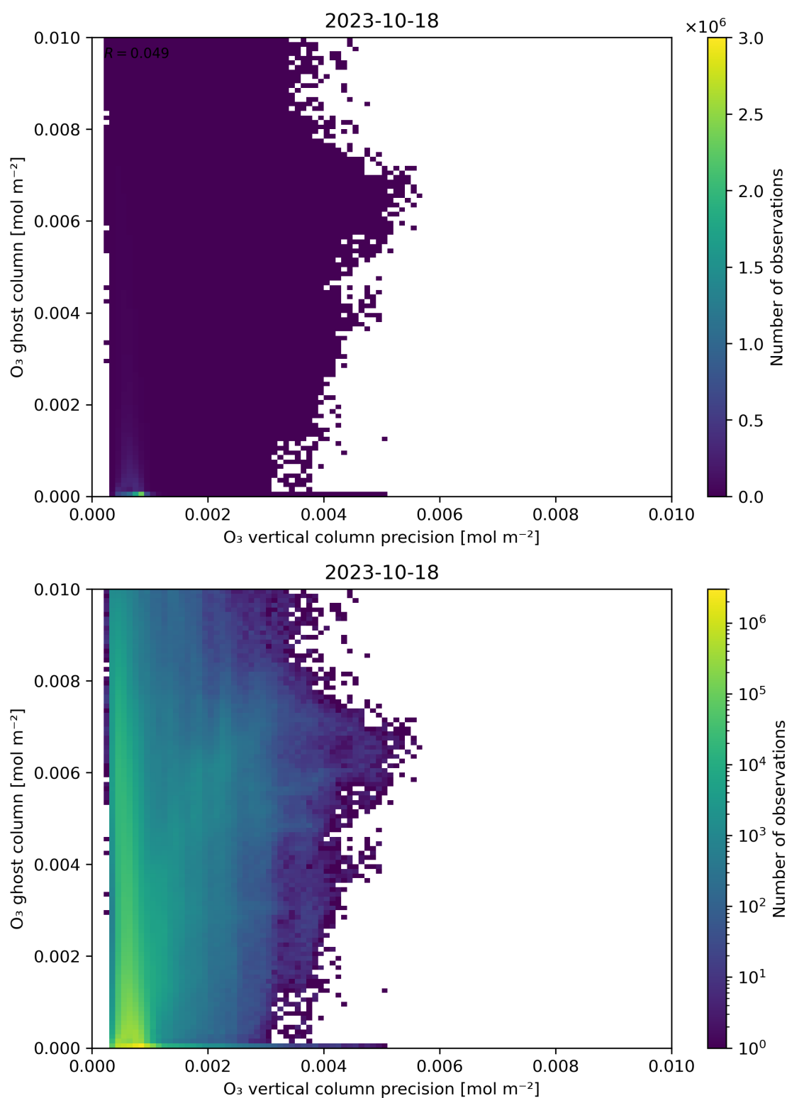
Figure 43: Scatter density plot of “ O_3 vertical column precision” against “ O_3 ghost column” for 2023-10-17 to 2023-10-19.
