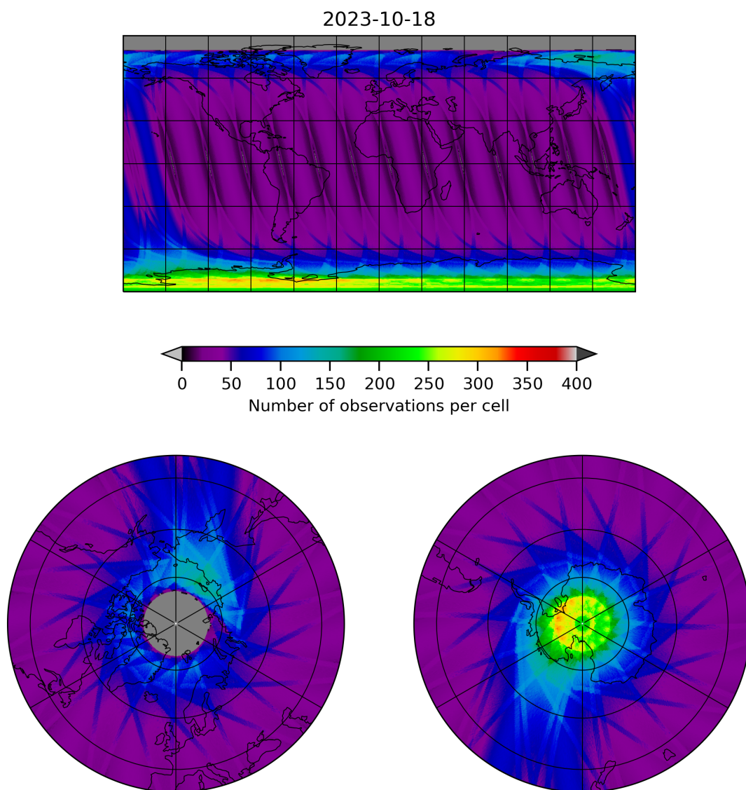
Figure 12: Map of the number of observations for 2023-10-17 to 2023-10-19
