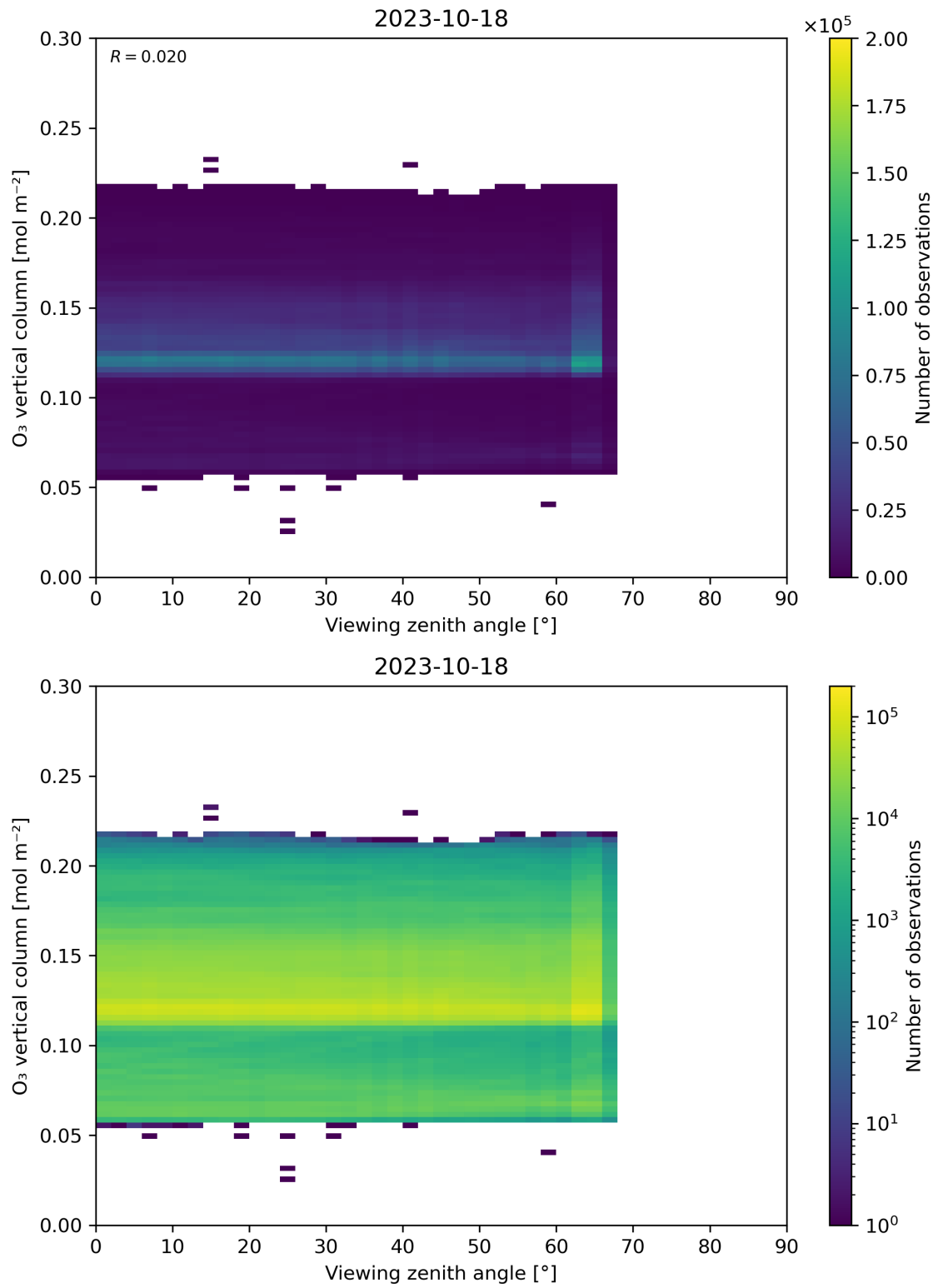
Figure 52: Scatter density plot of “Viewing zenith angle” against “O 3 vertical column” for 2023-10-17 to 2023-10-19.
