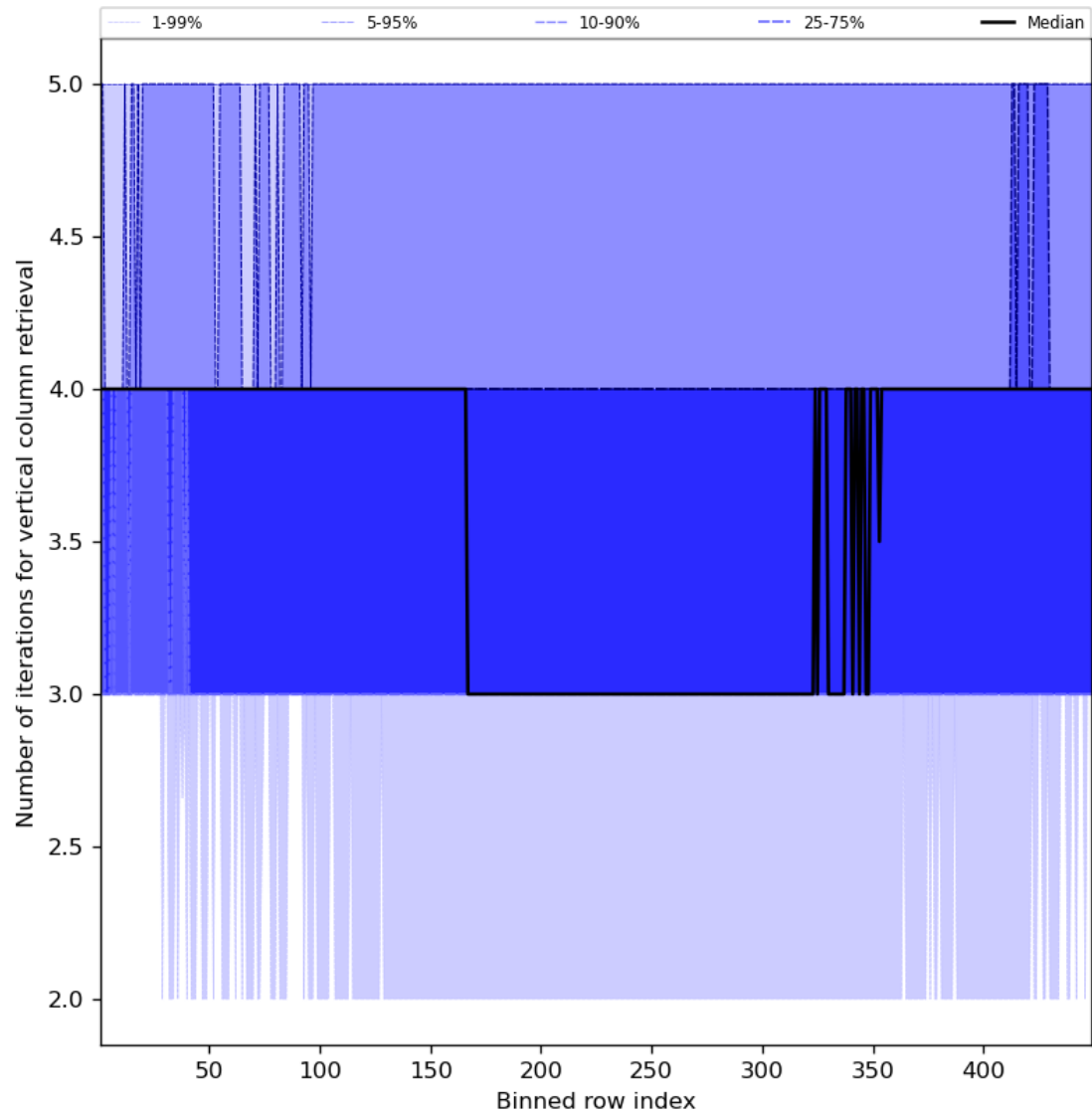
Figure 33: Along track statistics of “Number of iterations for vertical column retrieval” for 2023-10-17 to 2023-10-19
