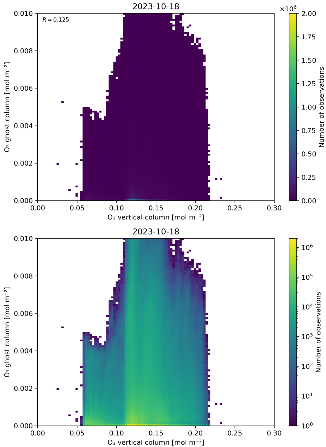
Figure 40: Scatter density plot of “O 3 vertical column” against “O 3 ghost column” for 2023-10-17 to 2023-10-19.
