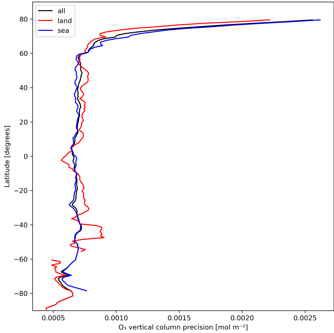
Figure 15: Zonal average of “O 3 vertical column precision” for 2023-10-17 to 2023-10-19.
