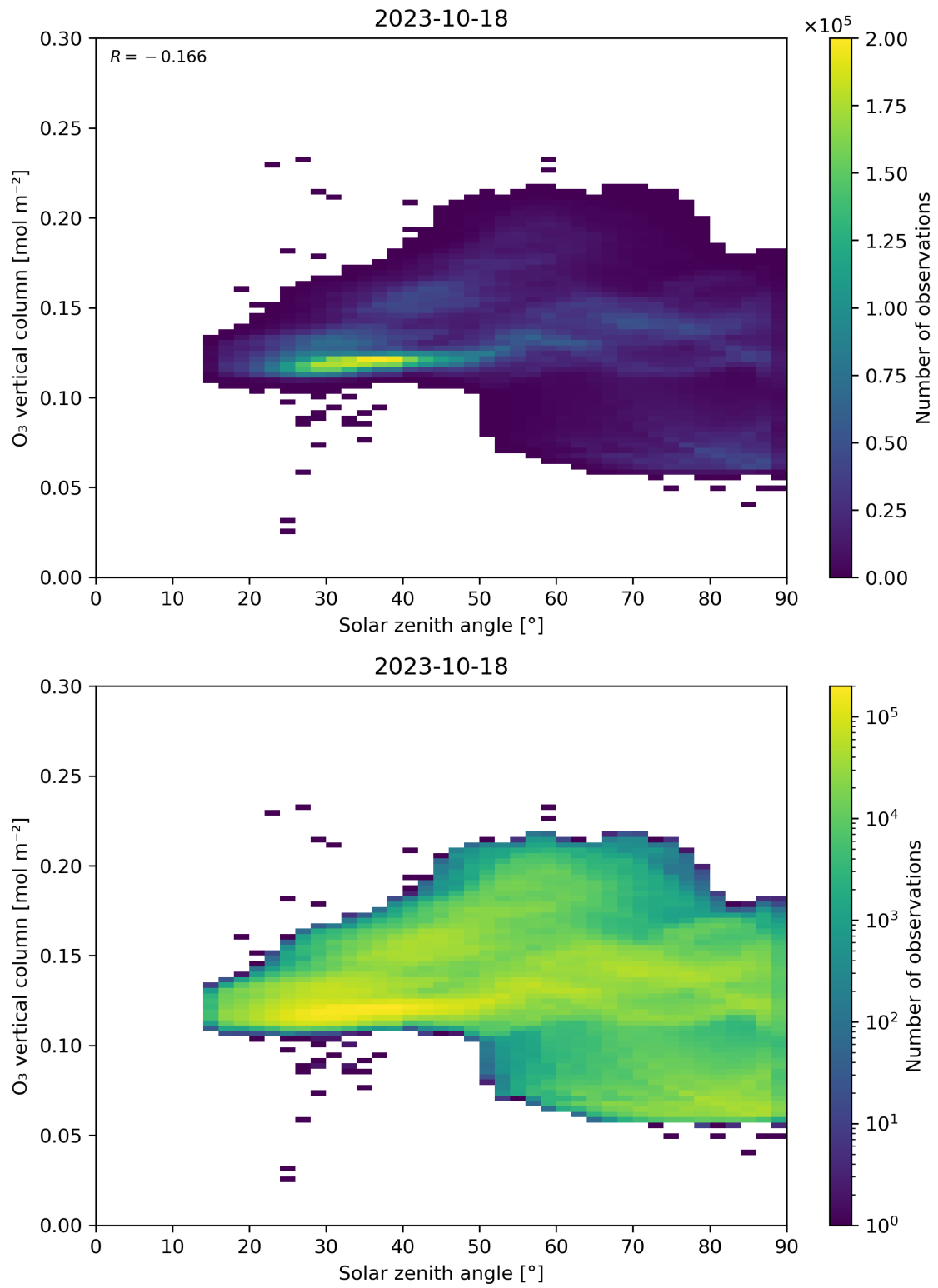
Figure 47: Scatter density plot of “Solar zenith angle” against “O 3 vertical column” for 2023-10-17 to 2023-10-19.
