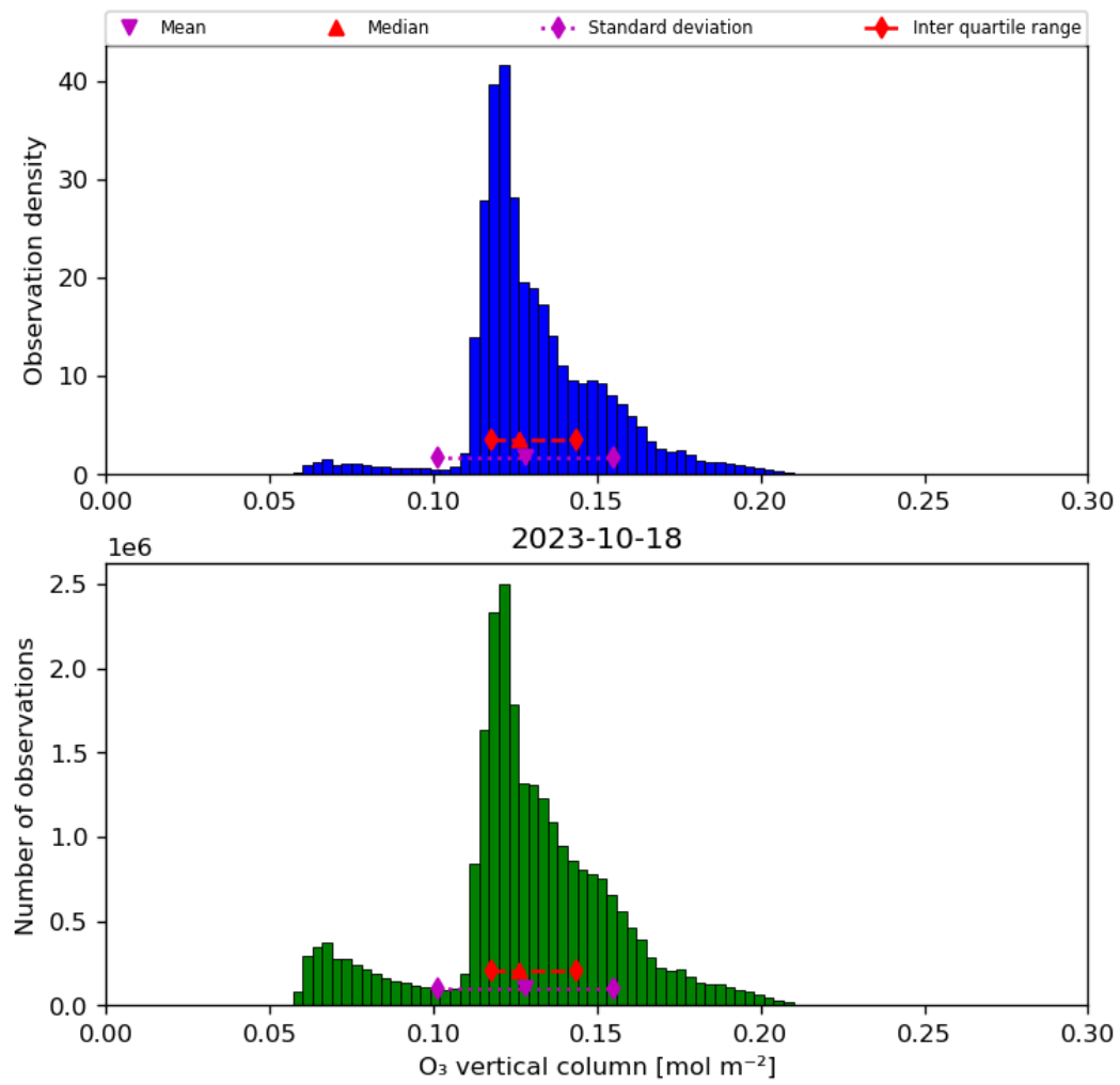
Figure 21: Histogram of “O 3 vertical column” for 2023-10-17 to 2023-10-19
