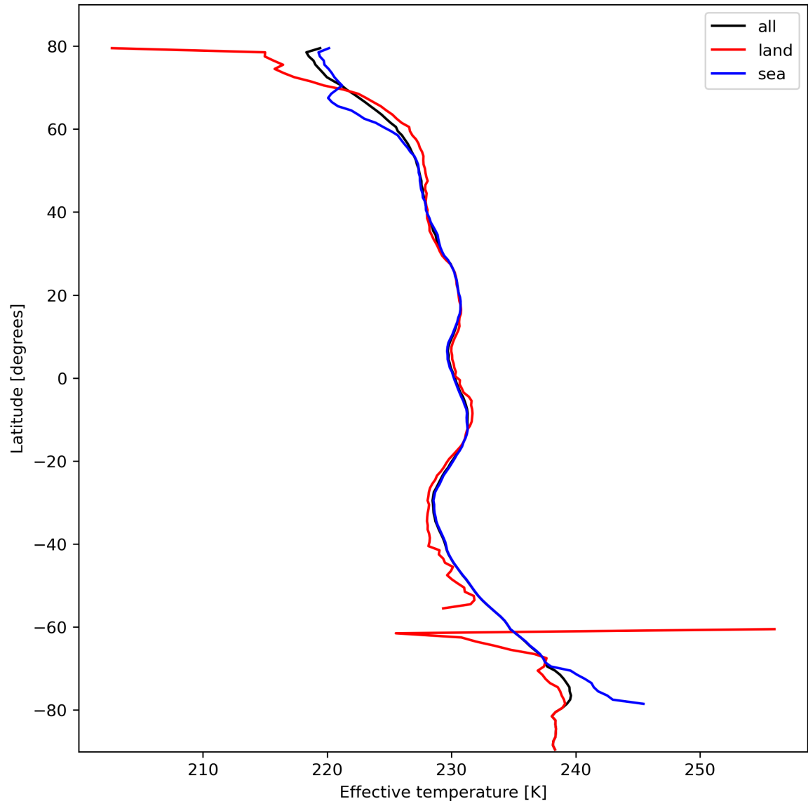
Figure 17: Zonal average of "Effective temperature" for 2023-10-18 to 2023-10-20.
