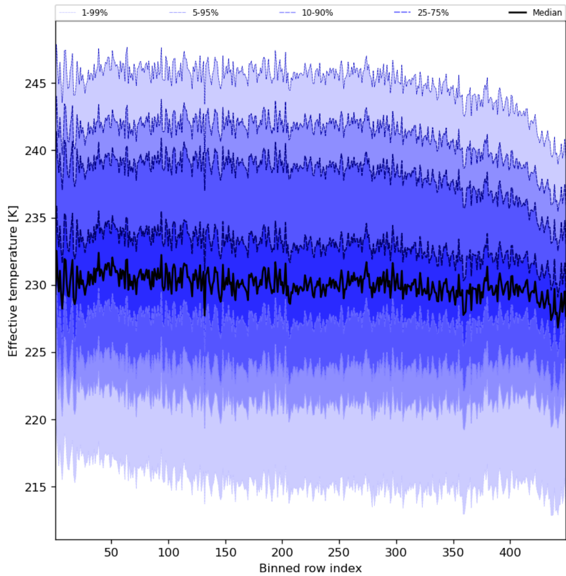
Figure 31: Along track statistics of “Effective temperature” for 2023-10-19 to 2023-10-21
