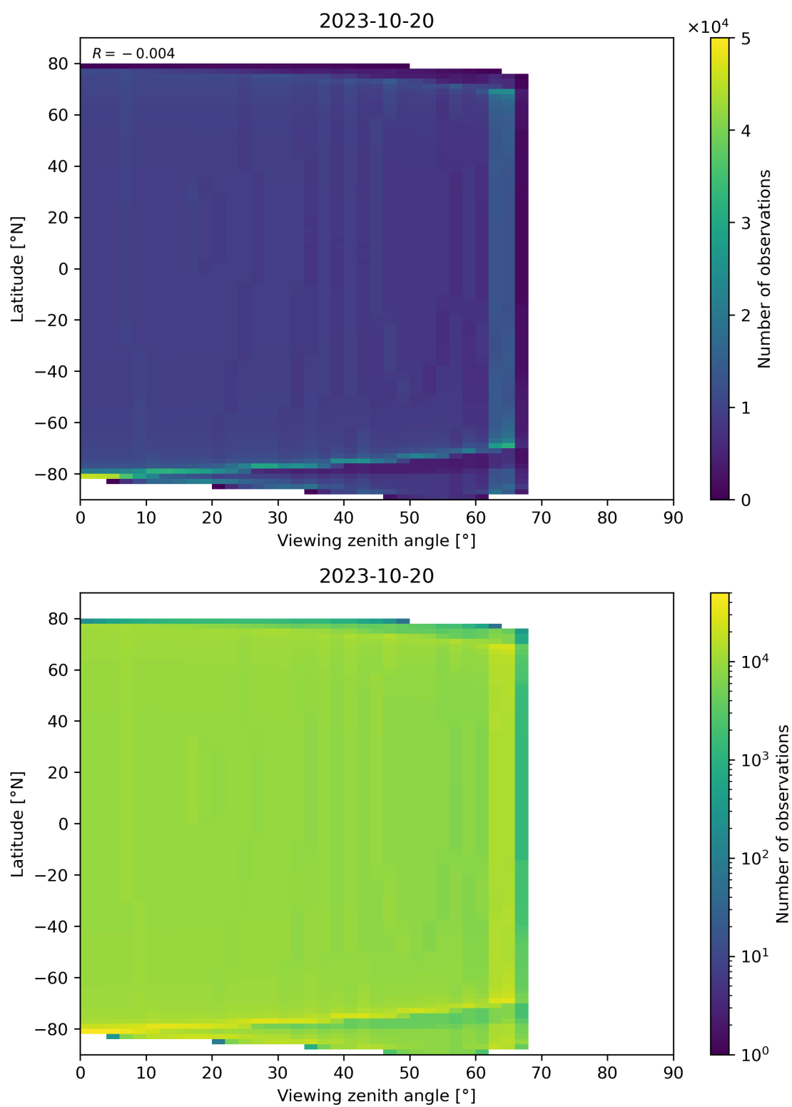
Figure 49: Scatter density plot of “Viewing zenith angle” against “Latitude” for 2023-10-19 to 2023-10-21.
