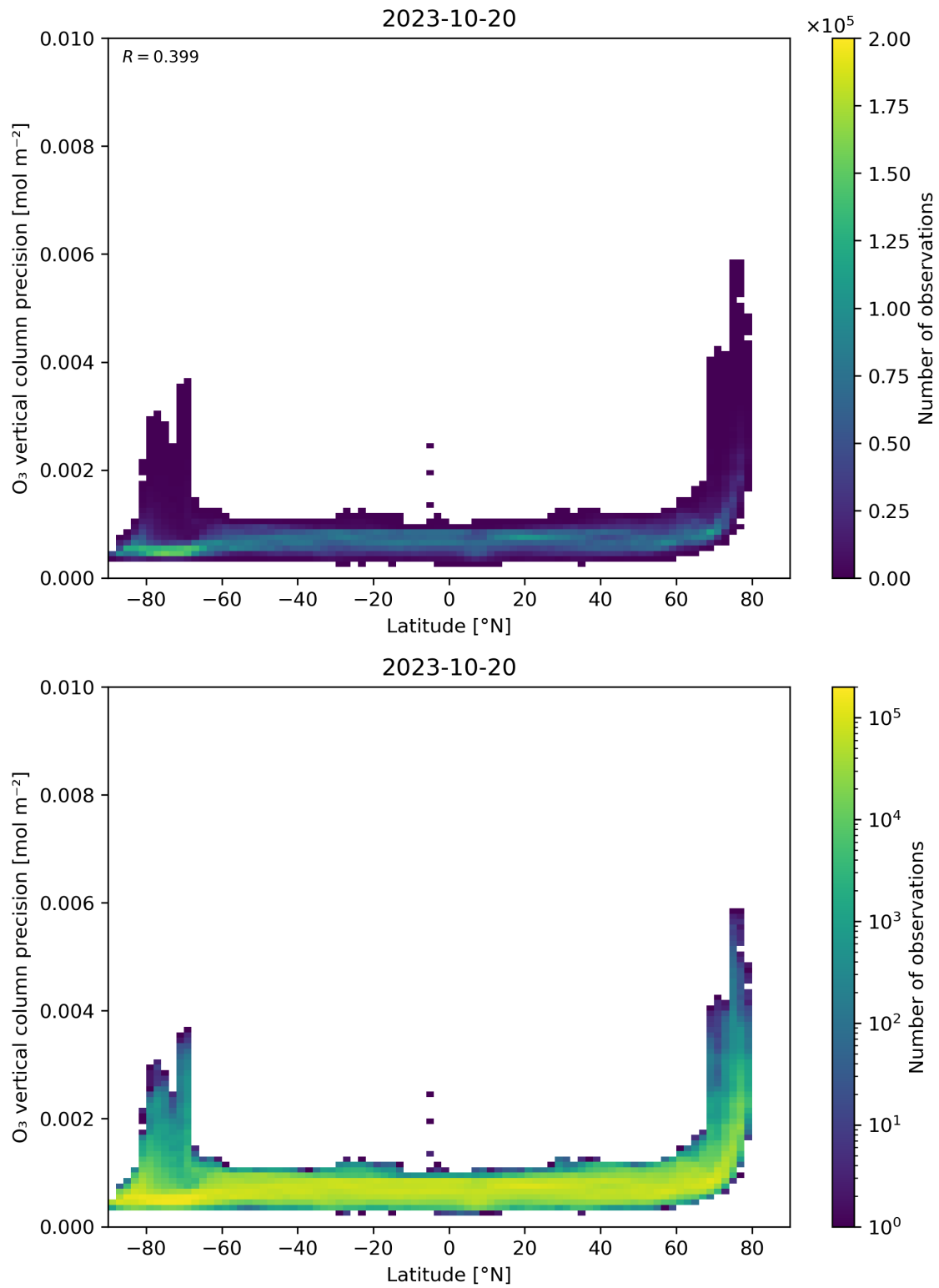
Figure 37: Scatter density plot of “Latitude” against “O 3 vertical column precision” for 2023-10-19 to 2023-10-21.
