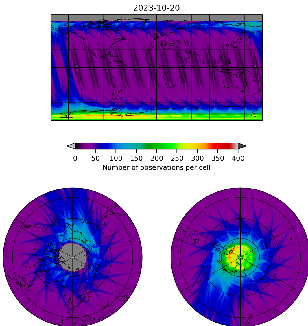
Figure 12: Map of the number of observations for 2023-10-19 to 2023-10-21
