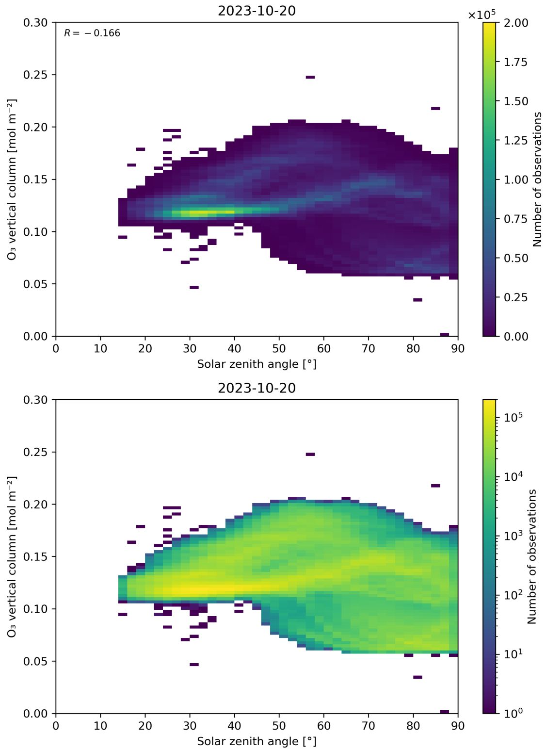
Figure 47: Scatter density plot of “Solar zenith angle” against “O 3 vertical column” for 2023-10-19 to 2023-10-21.
