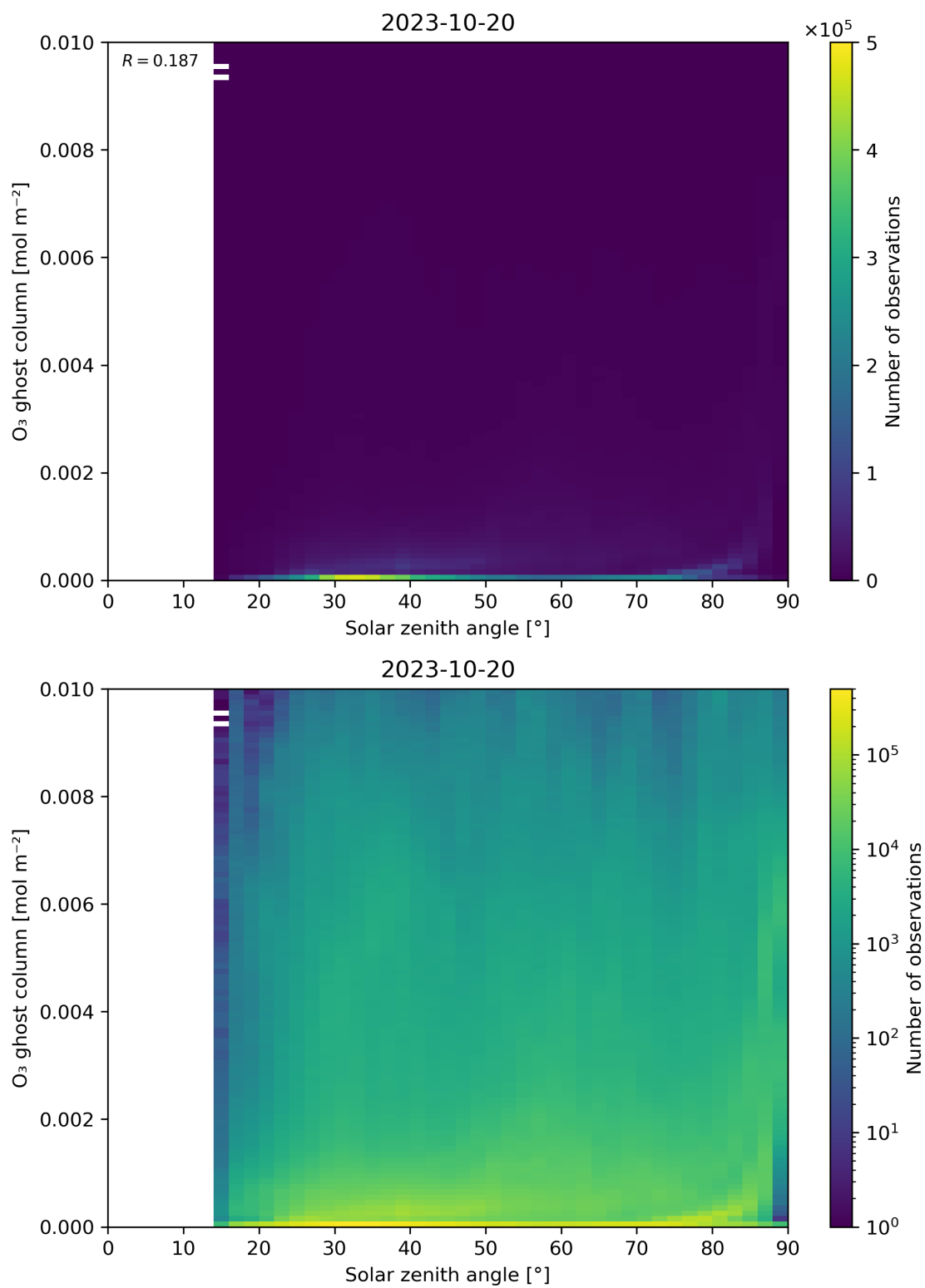
Figure 46: Scatter density plot of “Solar zenith angle” against “O 3 ghost column” for 2023-10-19 to 2023-10-21.
