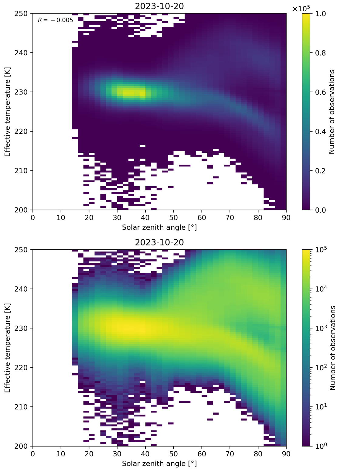
Figure 45: Scatter density plot of “Solar zenith angle” against “Effective temperature” for 2023-10-19 to 2023-10-21.
