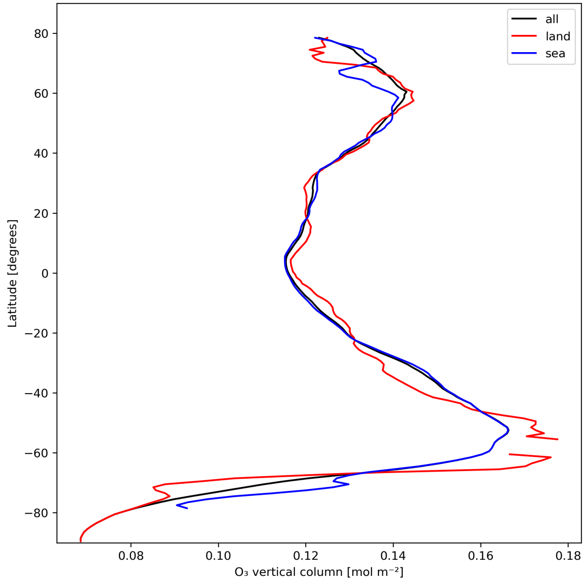
Figure 14: Zonal average of “O 3 vertical column” for 2023-10-19 to 2023-10-21.
