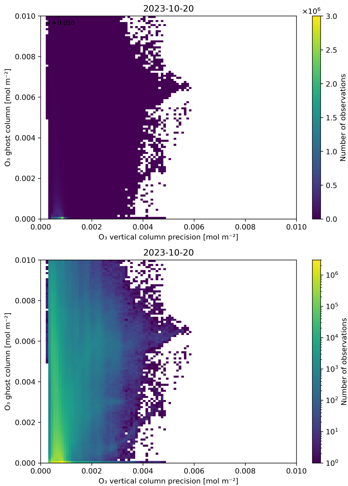
Figure 43: Scatter density plot of “O 3 vertical column precision” against “O 3 ghost column” for 2023-10-19 to 2023-10-21.
