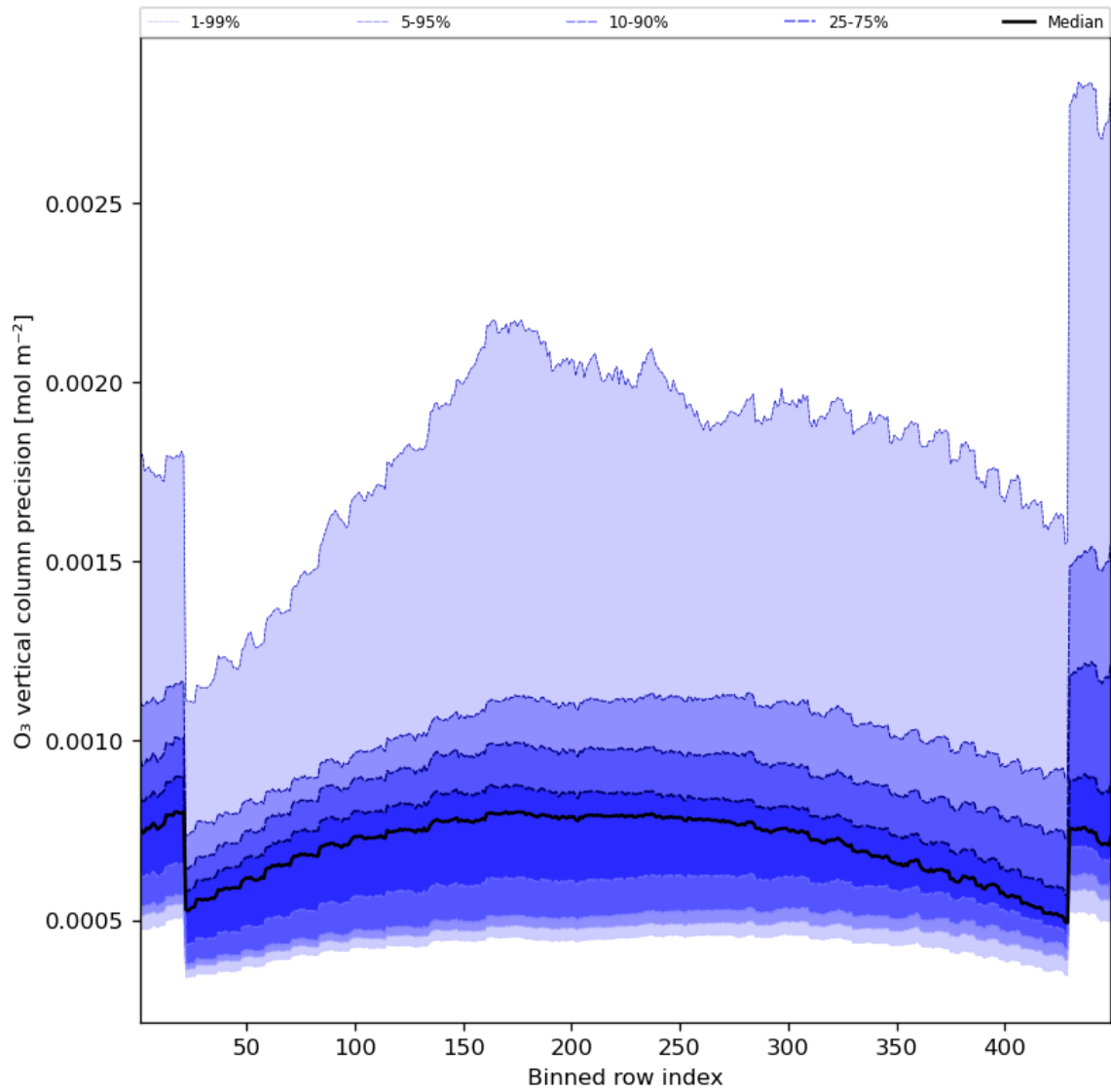
Figure 29: Along track statistics of “O 3 vertical column precision” for 2023-10-19 to 2023-10-21
