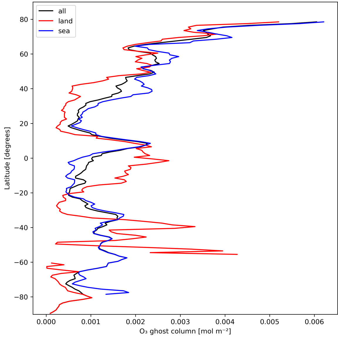
Figure 18: Zonal average of "O 3 ghost column" for 2023-10-19 to 2023-10-21.
