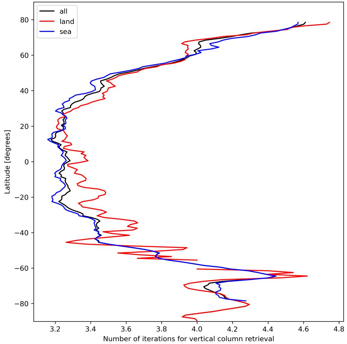
Figure 19: Zonal average of “Number of iterations for vertical column retrieval” for 2023-10-19 to 2023-10-21.
