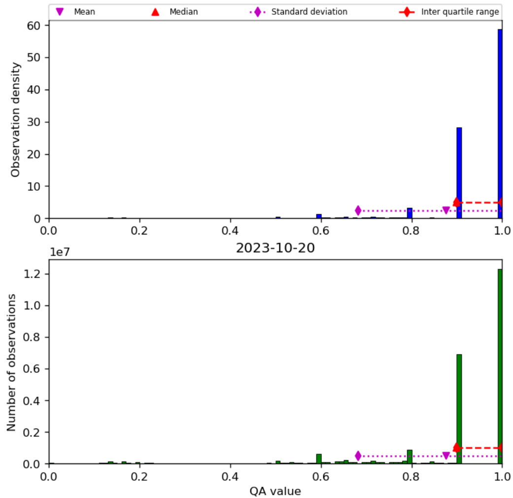
Figure 20: Histogram of “QA value” for 2023-10-19 to 2023-10-21
