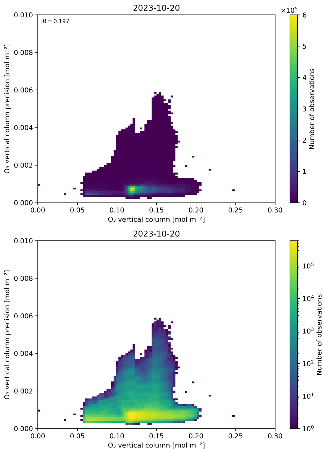
Figure 41: Scatter density plot of “O 3 vertical column” against “O 3 vertical column precision” for 2023-10-19 to 2023-10-21.
