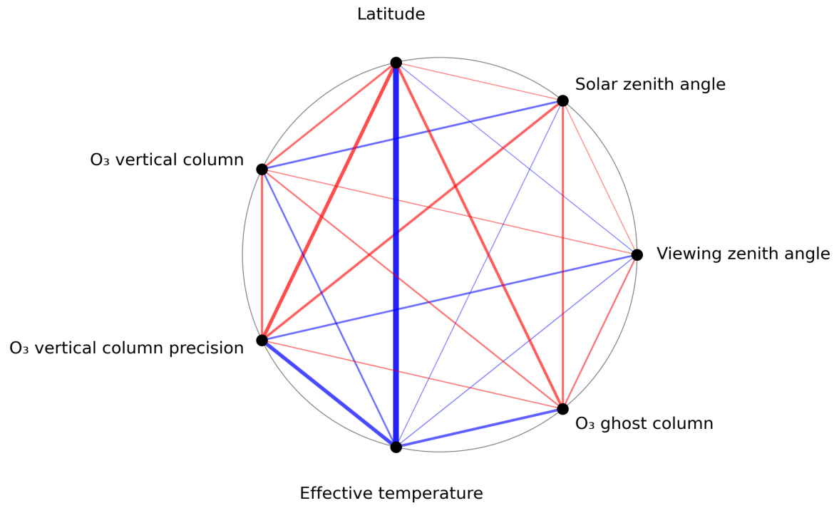
Figure 1: Map of correlation graph for 2023-10-19 to 2023-10-21.
