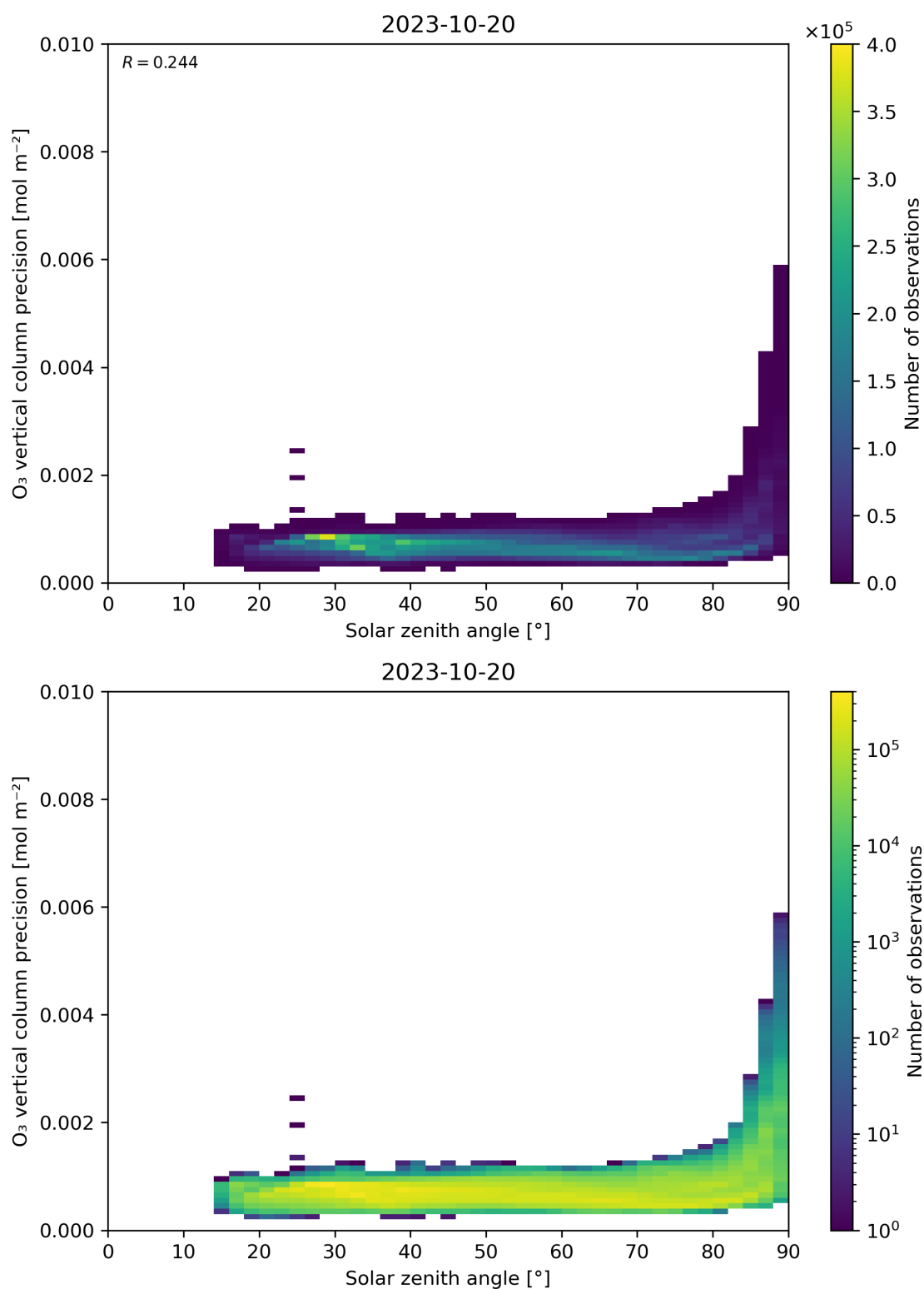
Figure 48: Scatter density plot of “Solar zenith angle” against “O 3 vertical column precision” for 2023-10-19 to 2023-10-21.
