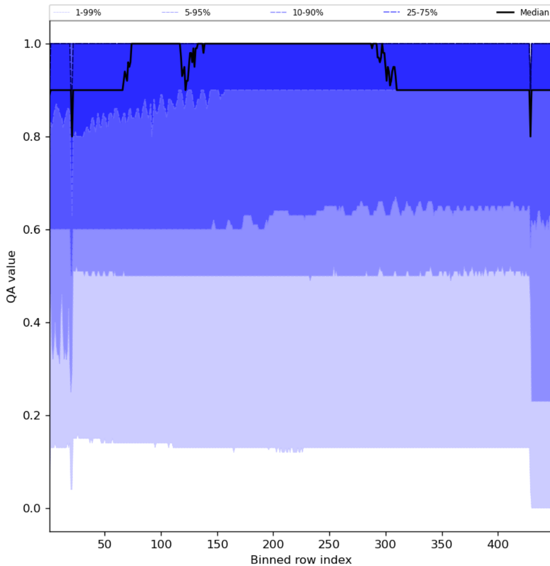
Figure 27: Along track statistics of “QA value” for 2023-10-19 to 2023-10-21
