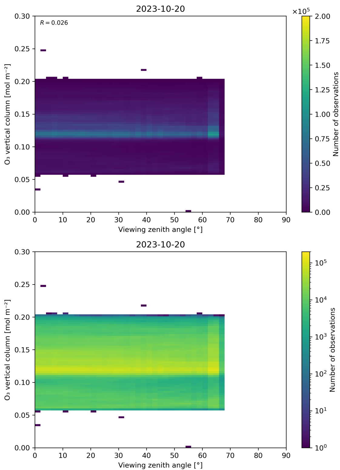
Figure 52: Scatter density plot of “Viewing zenith angle” against “O 3 vertical column” for 2023-10-19 to 2023-10-21.
