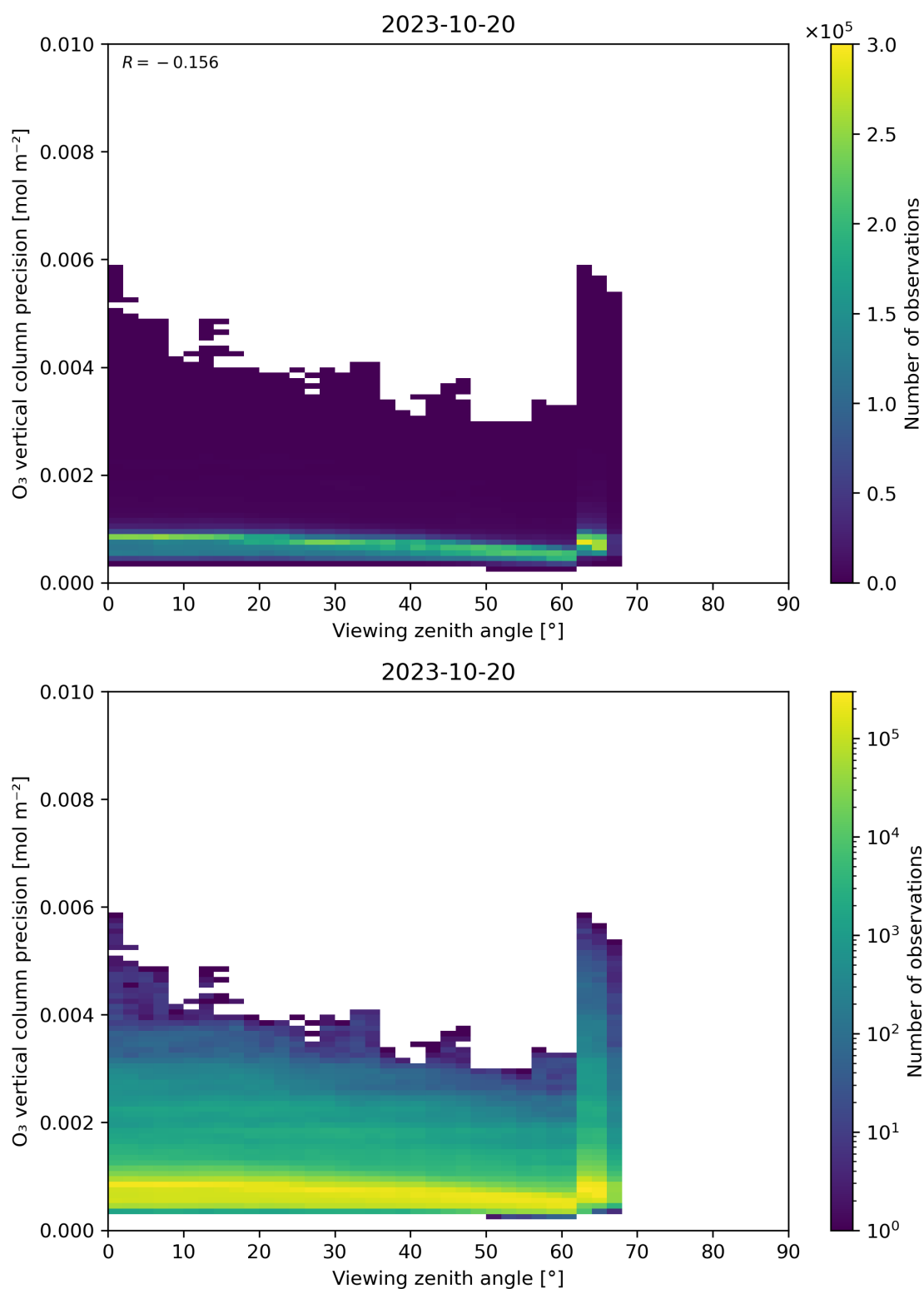
Figure 53: Scatter density plot of “Viewing zenith angle” against “O 3 vertical column precision” for 2023-10-19 to 2023-10-21.
