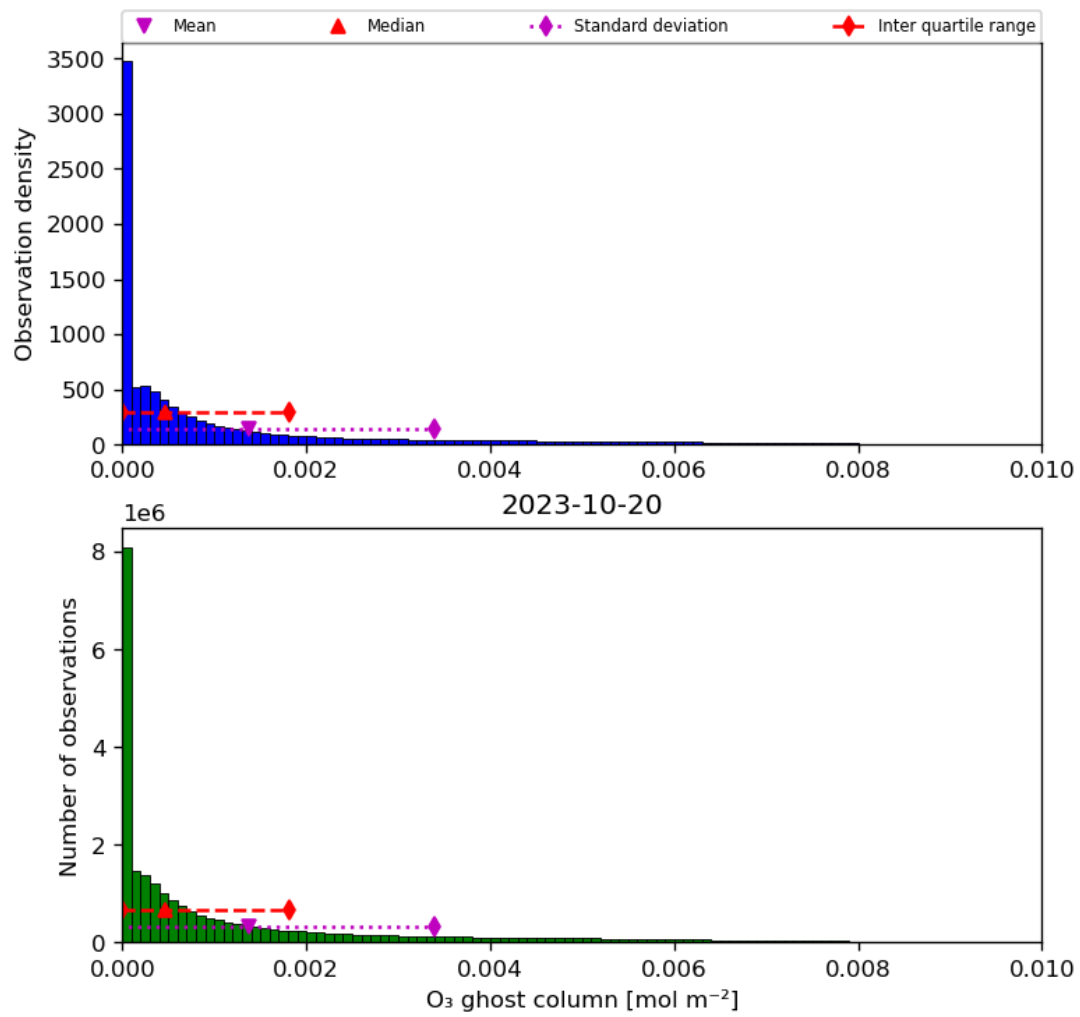
Figure 25: Histogram of “O 3 ghost column” for 2023-10-19 to 2023-10-21
