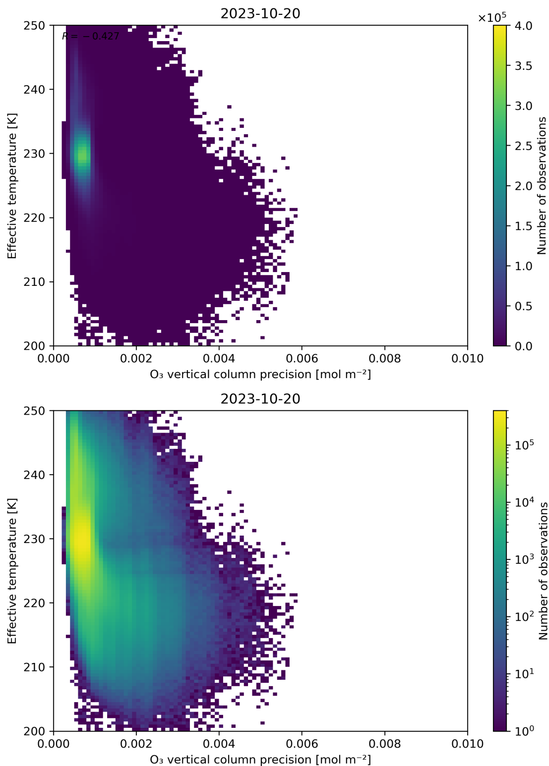
Figure 42: Scatter density plot of “O 3 vertical column precision” against “Effective temperature” for 2023-10-19 to 2023-10-21.
