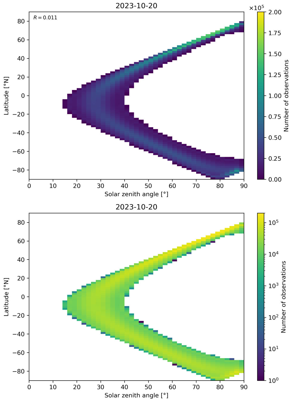
Figure 44: Scatter density plot of “Solar zenith angle” against “Latitude” for 2023-10-19 to 2023-10-21.
