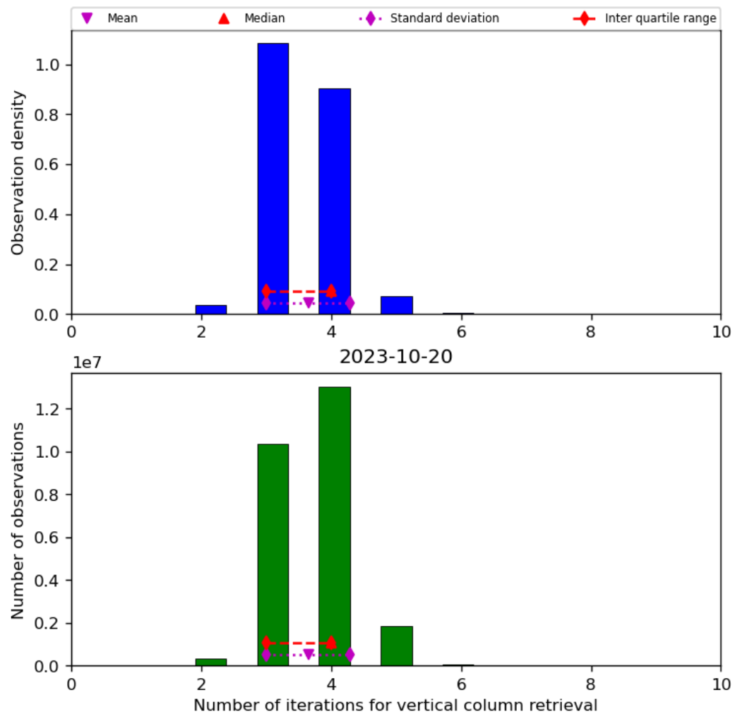
Figure 26: Histogram of “Number of iterations for vertical column retrieval” for 2023-10-19 to 2023-10-21
