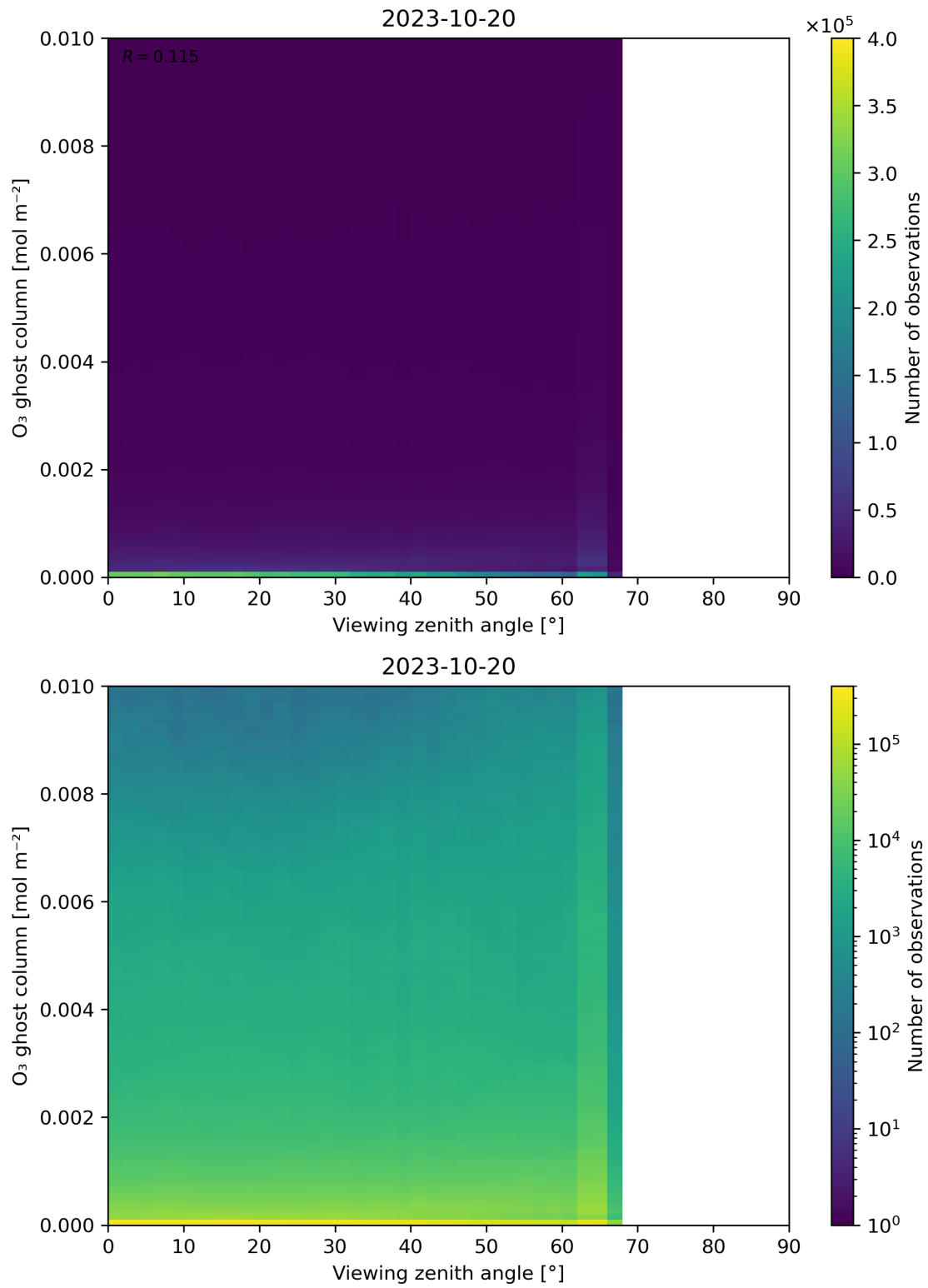
Figure 51: Scatter density plot of “Viewing zenith angle” against “O 3 ghost column” for 2023-10-19 to 2023-10-21.
