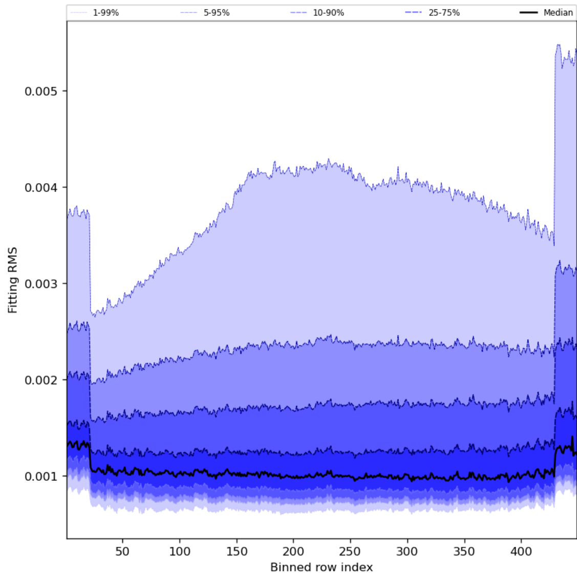
Figure 30: Along track statistics of “Fitting RMS” for 2023-10-19 to 2023-10-21
