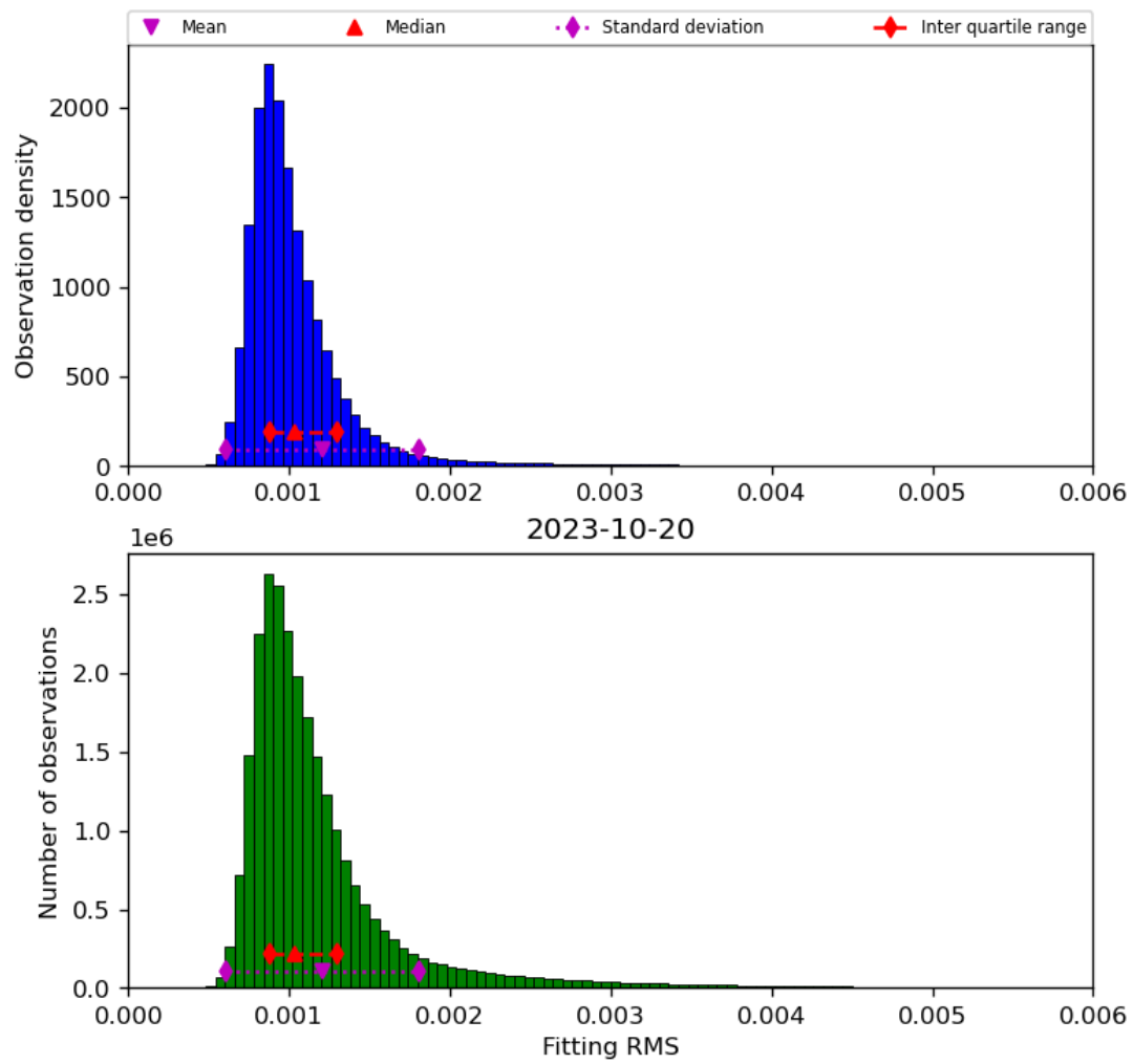
Figure 23: Histogram of “Fitting RMS” for 2023-10-19 to 2023-10-21
