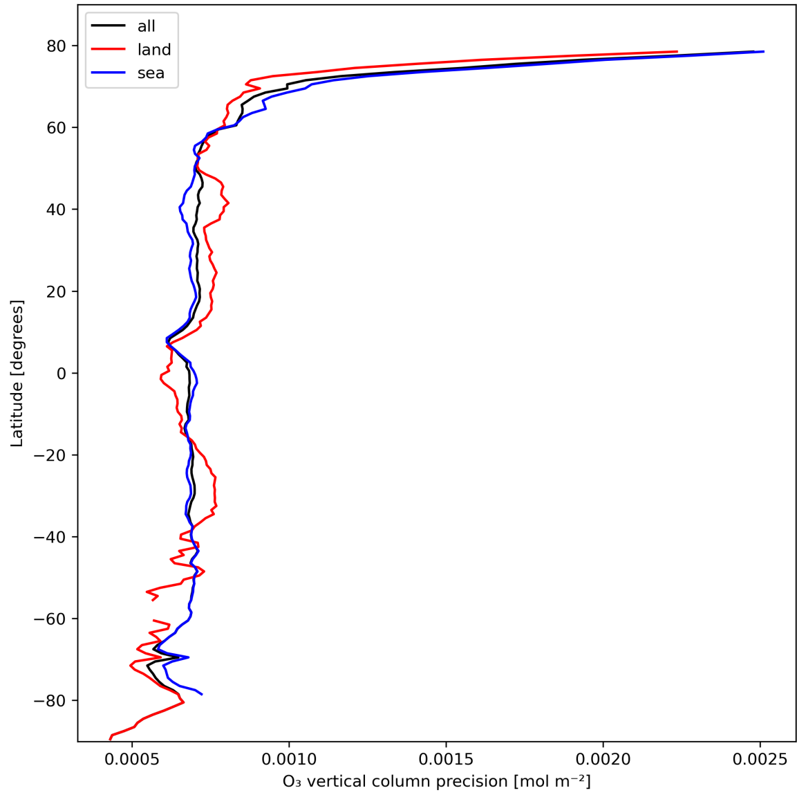
Figure 15: Zonal average of “O 3 vertical column precision” for 2023-10-19 to 2023-10-21.
