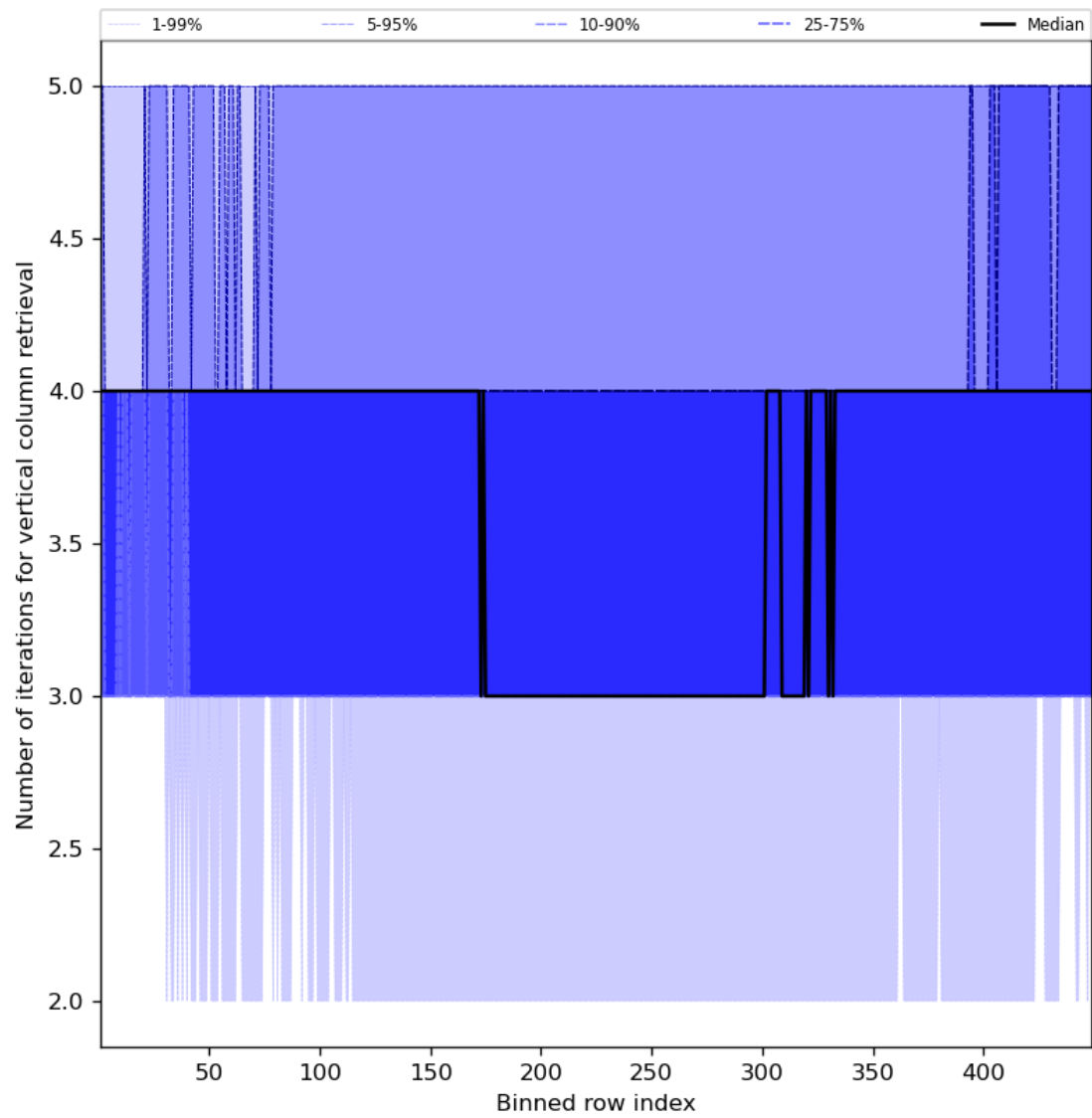
Figure 33: Along track statistics of “Number of iterations for vertical column retrieval” for 2023-10-19 to 2023-10-21
