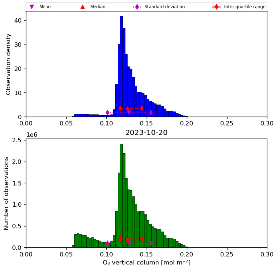
Figure 21: Histogram of “O 3 vertical column” for 2023-10-19 to 2023-10-21
