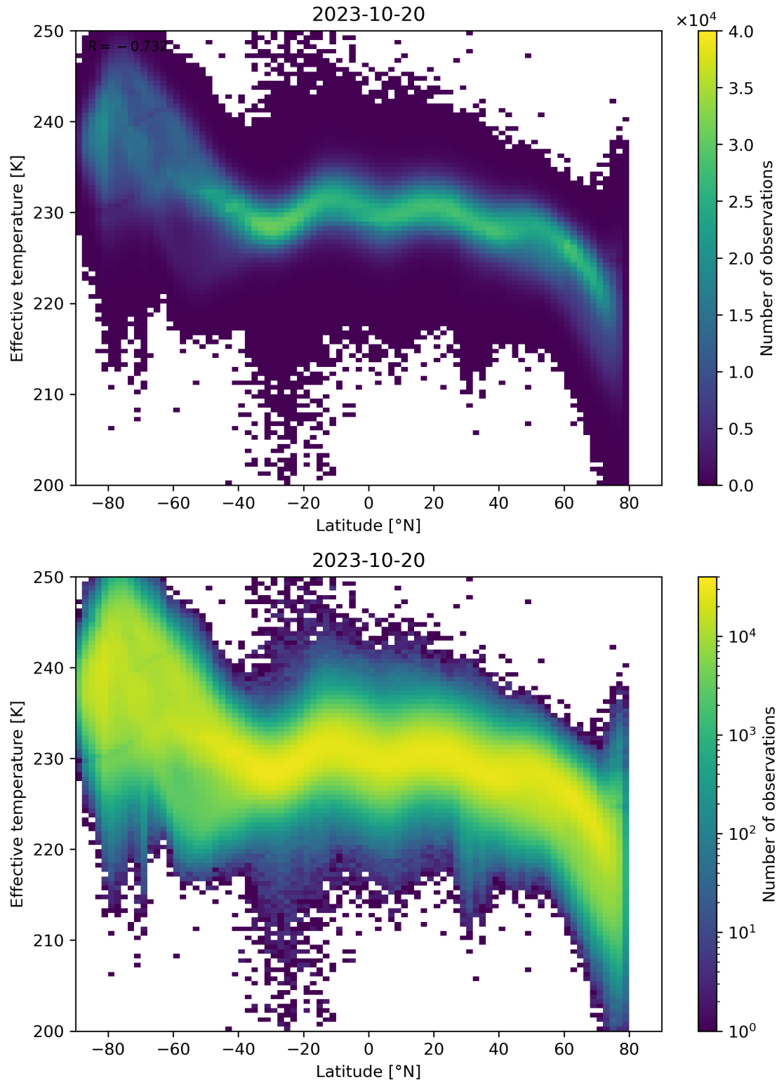
Figure 34: Scatter density plot of “Latitude” against “Effective temperature” for 2023-10-19 to 2023-10-21.
