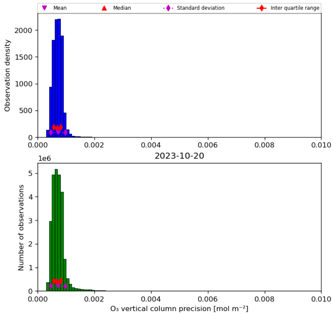
Figure 22: Histogram of “O 3 vertical column precision” for 2023-10-19 to 2023-10-21
