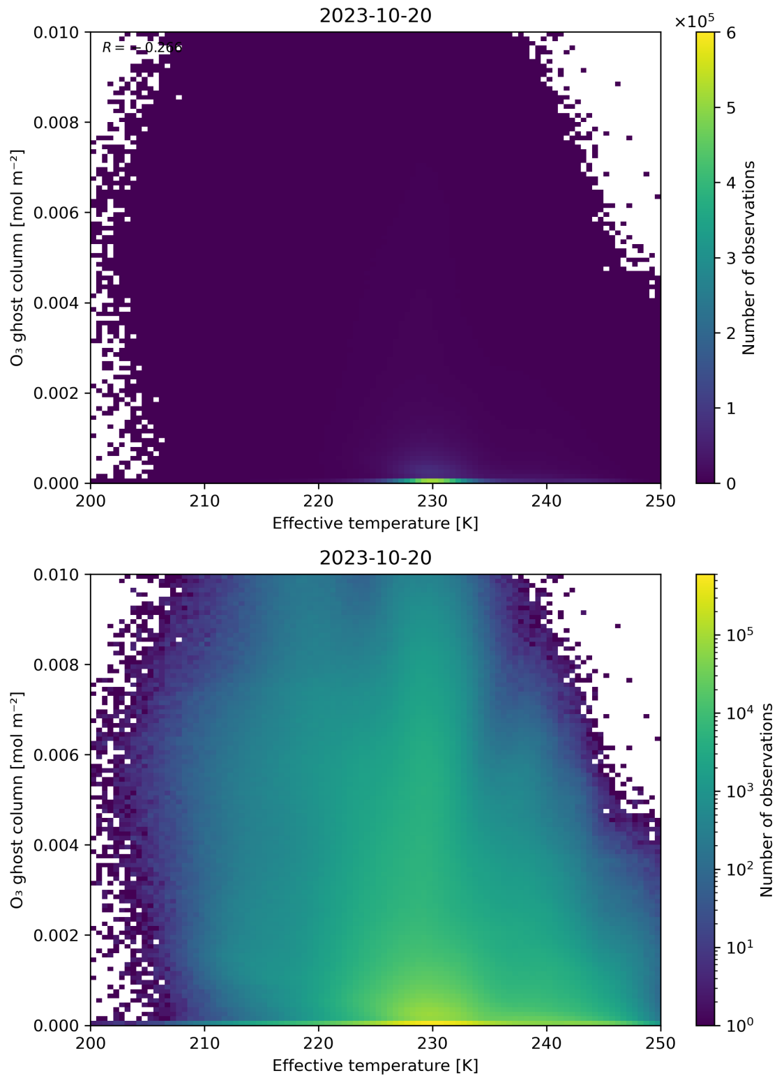
Figure 38: Scatter density plot of “Effective temperature” against “O 3 ghost column” for 2023-10-19 to 2023-10-21.
