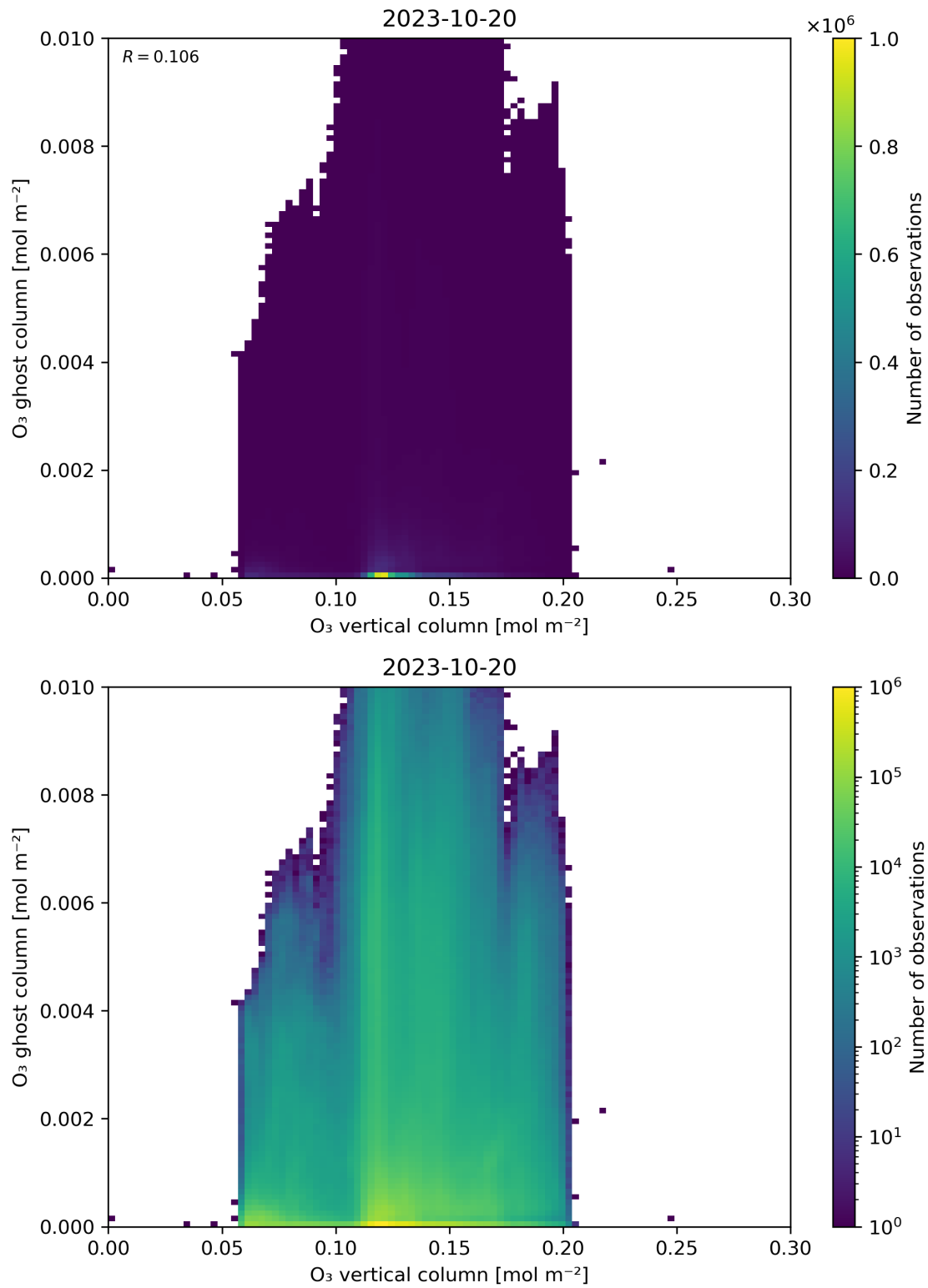
Figure 40: Scatter density plot of “O 3 vertical column” against “O 3 ghost column” for 2023-10-19 to 2023-10-21.
