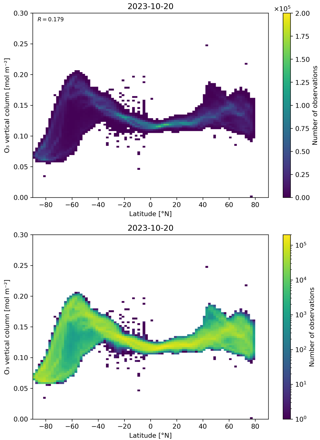
Figure 36: Scatter density plot of “Latitude” against “O 3 vertical column” for 2023-10-19 to 2023-10-21.
