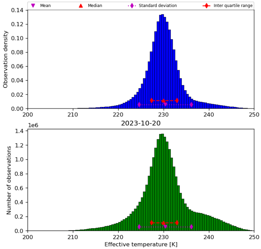
Figure 24: Histogram of “Effective temperature” for 2023-10-19 to 2023-10-21
