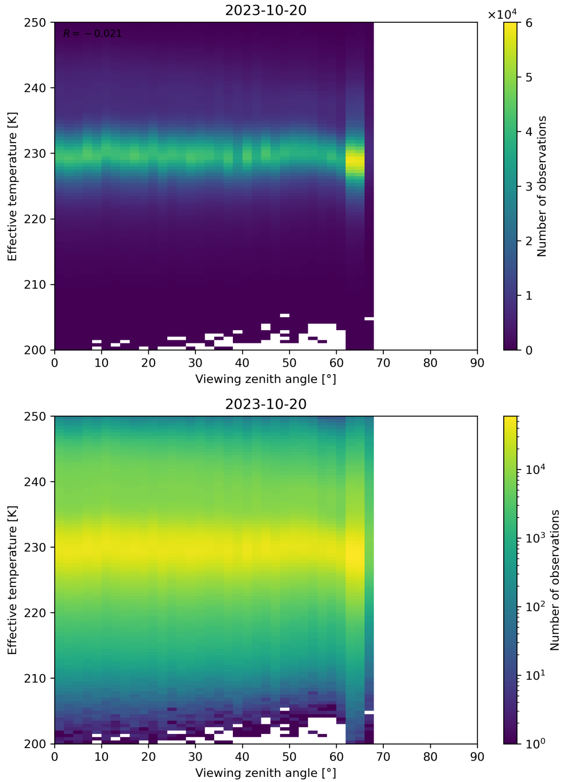
Figure 50: Scatter density plot of “Viewing zenith angle” against “Effective temperature” for 2023-10-19 to 2023-10-21.
