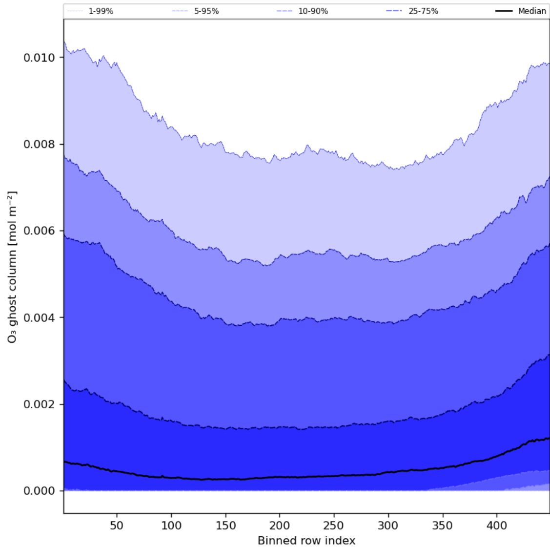
Figure 32: Along track statistics of “O 3 ghost column” for 2023-10-19 to 2023-10-21
