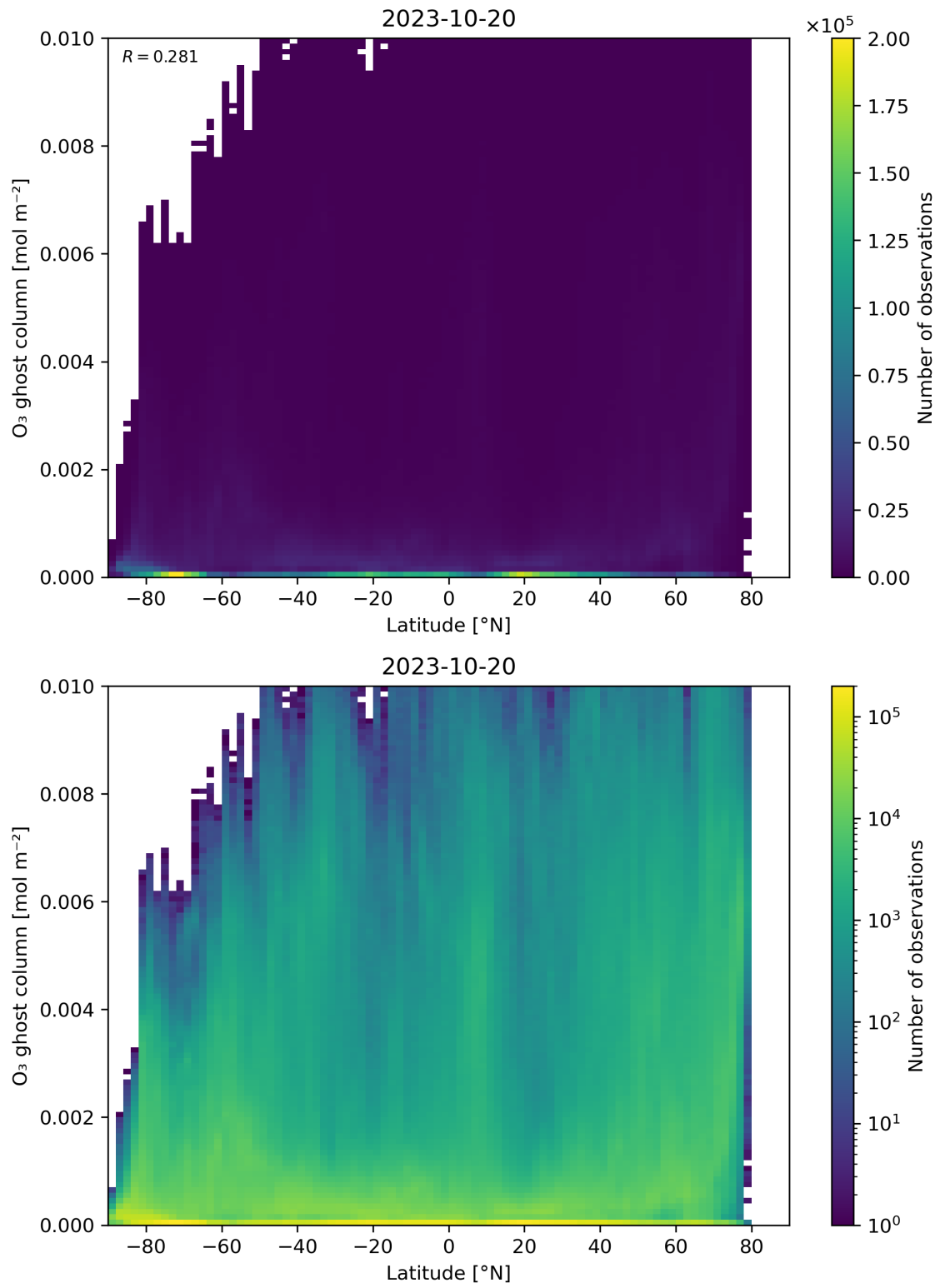
Figure 35: Scatter density plot of “Latitude” against “O 3 ghost column” for 2023-10-19 to 2023-10-21.
