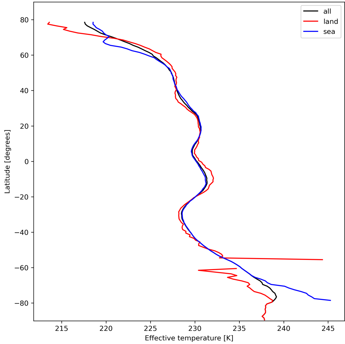
Figure 17: Zonal average of “Effective temperature” for 2023-10-19 to 2023-10-21.
