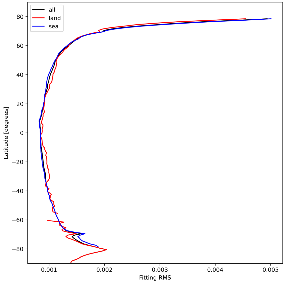
Figure 16: Zonal average of “Fitting RMS” for 2023-10-19 to 2023-10-21.
