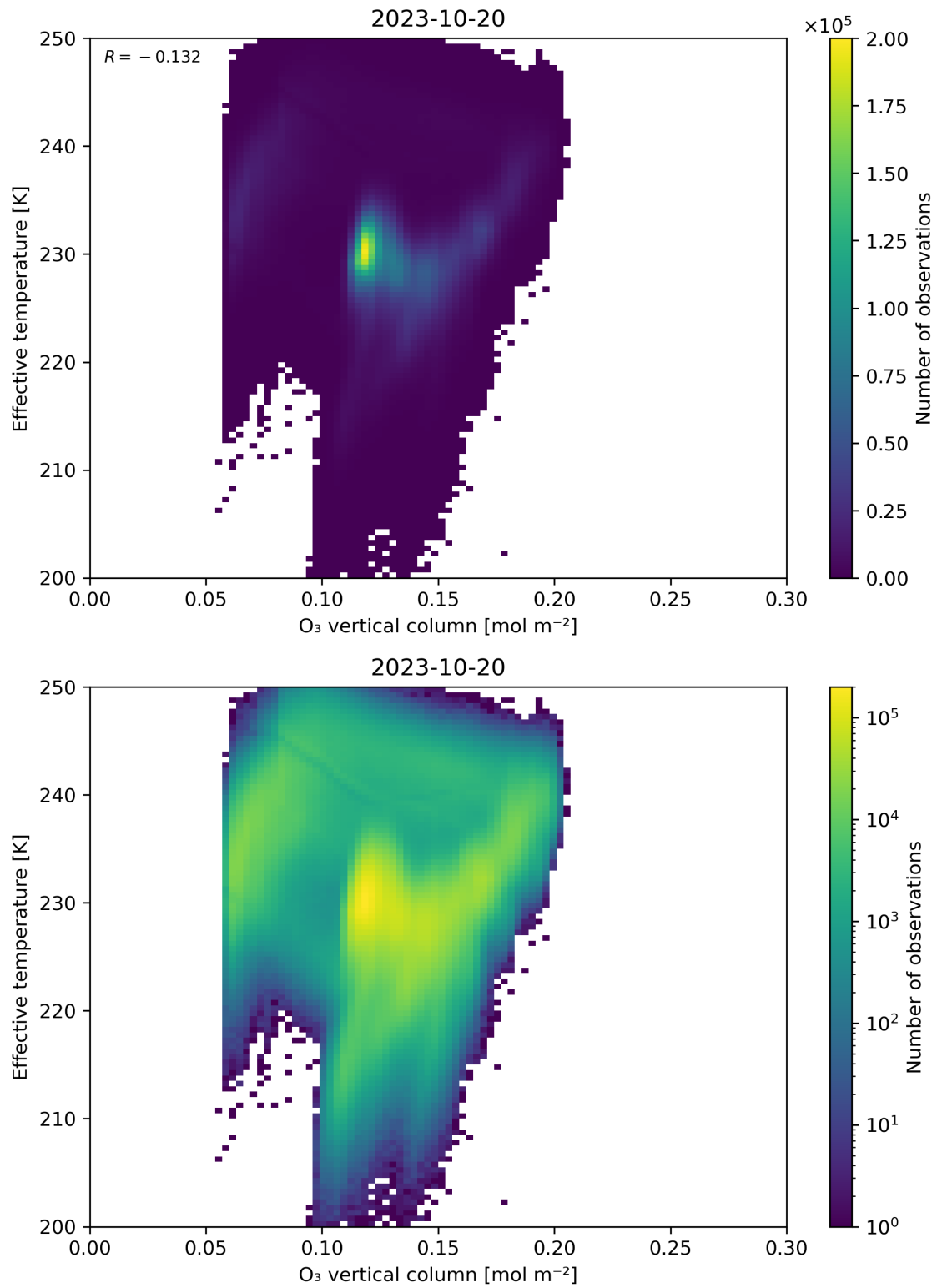
Figure 39: Scatter density plot of “O 3 vertical column” against “Effective temperature” for 2023-10-19 to 2023-10-21.
