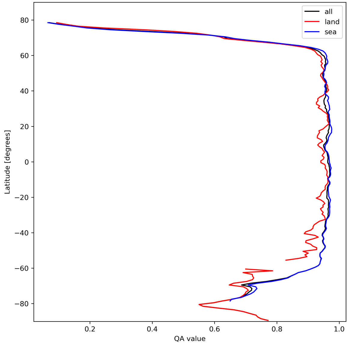
Figure 13: Zonal average of “QA value” for 2023-10-19 to 2023-10-21.
