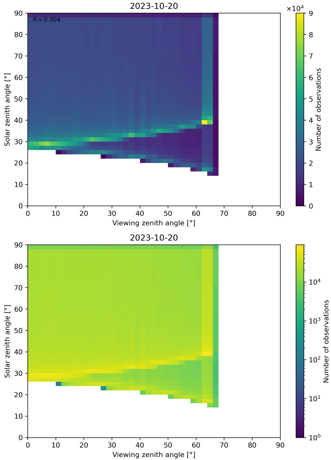
Figure 54: Scatter density plot of “Viewing zenith angle” against “Solar zenith angle” for 2023-10-19 to 2023-10-21.
