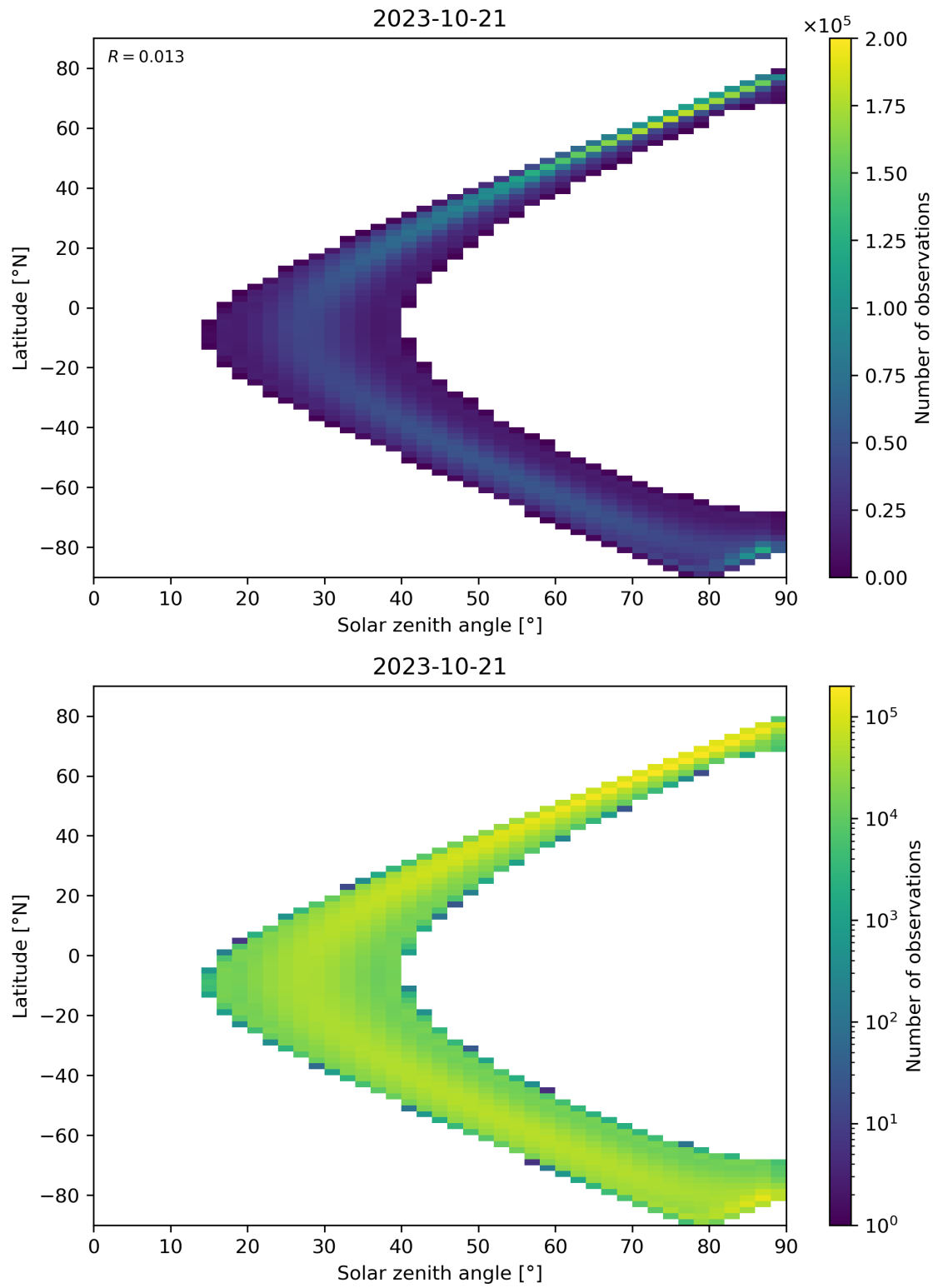
Figure 44: Scatter density plot of “Solar zenith angle” against “Latitude” for 2023-10-20 to 2023-10-22.
