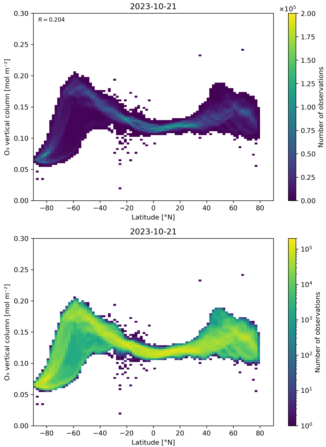
Figure 36: Scatter density plot of “Latitude” against “O 3 vertical column” for 2023-10-20 to 2023-10-22.
