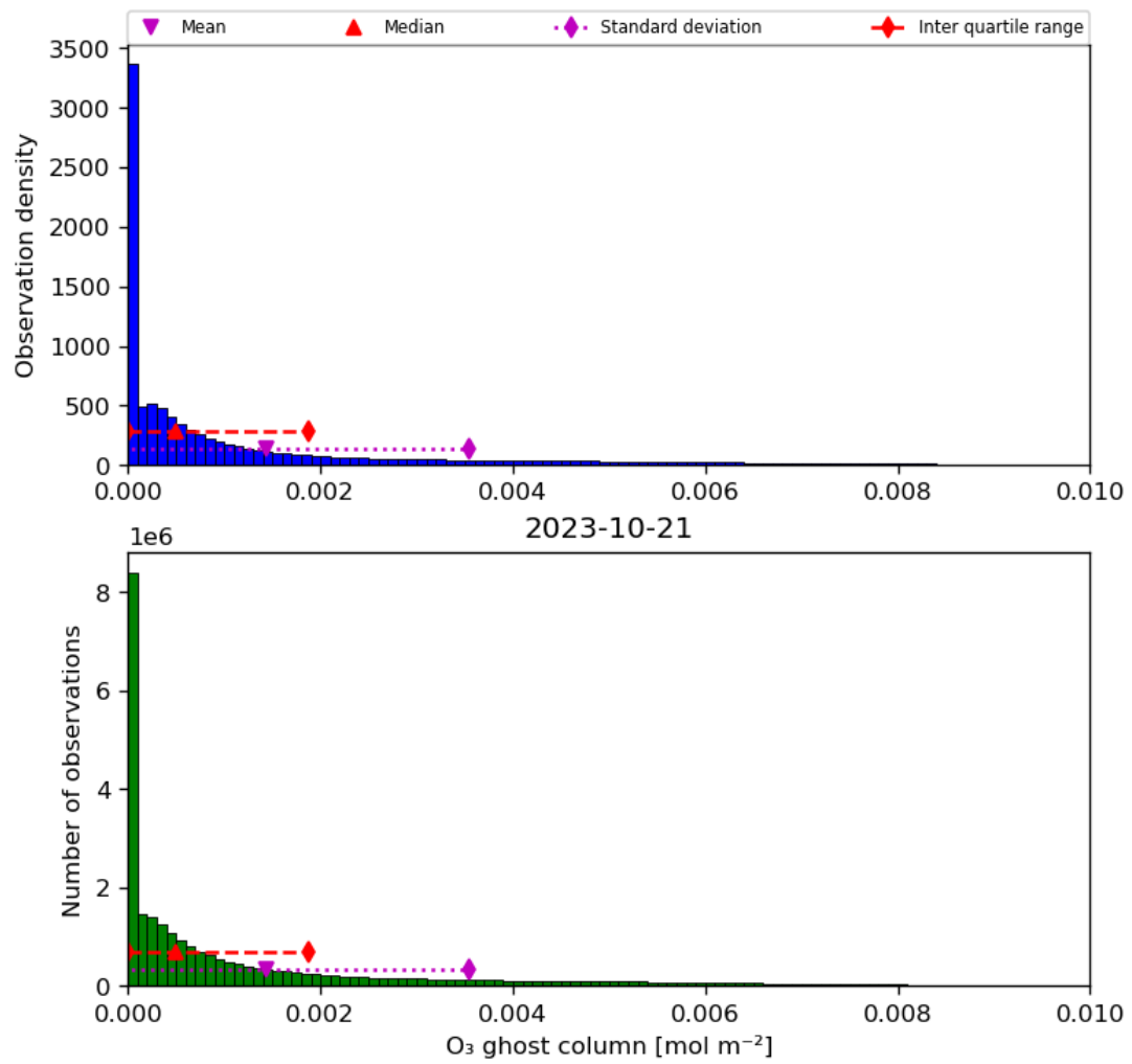
Figure 25: Histogram of “O 3 ghost column” for 2023-10-20 to 2023-10-22
