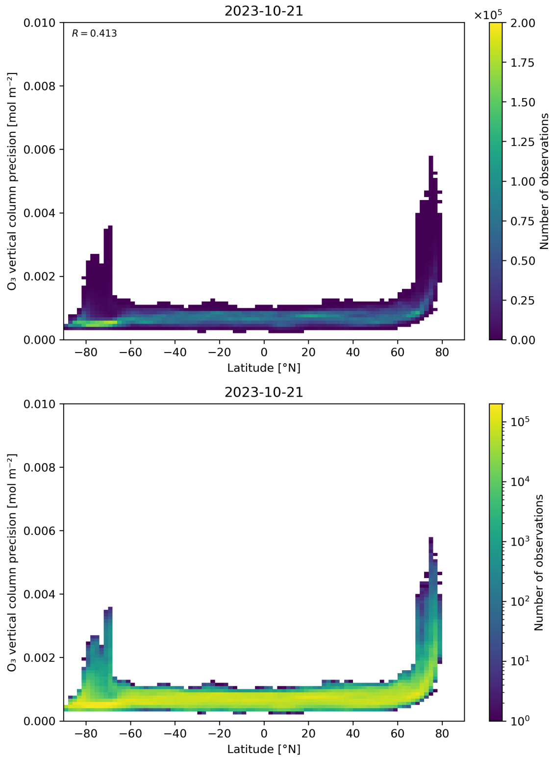
Figure 37: Scatter density plot of “Latitude” against “O 3 vertical column precision” for 2023-10-20 to 2023-10-22.
