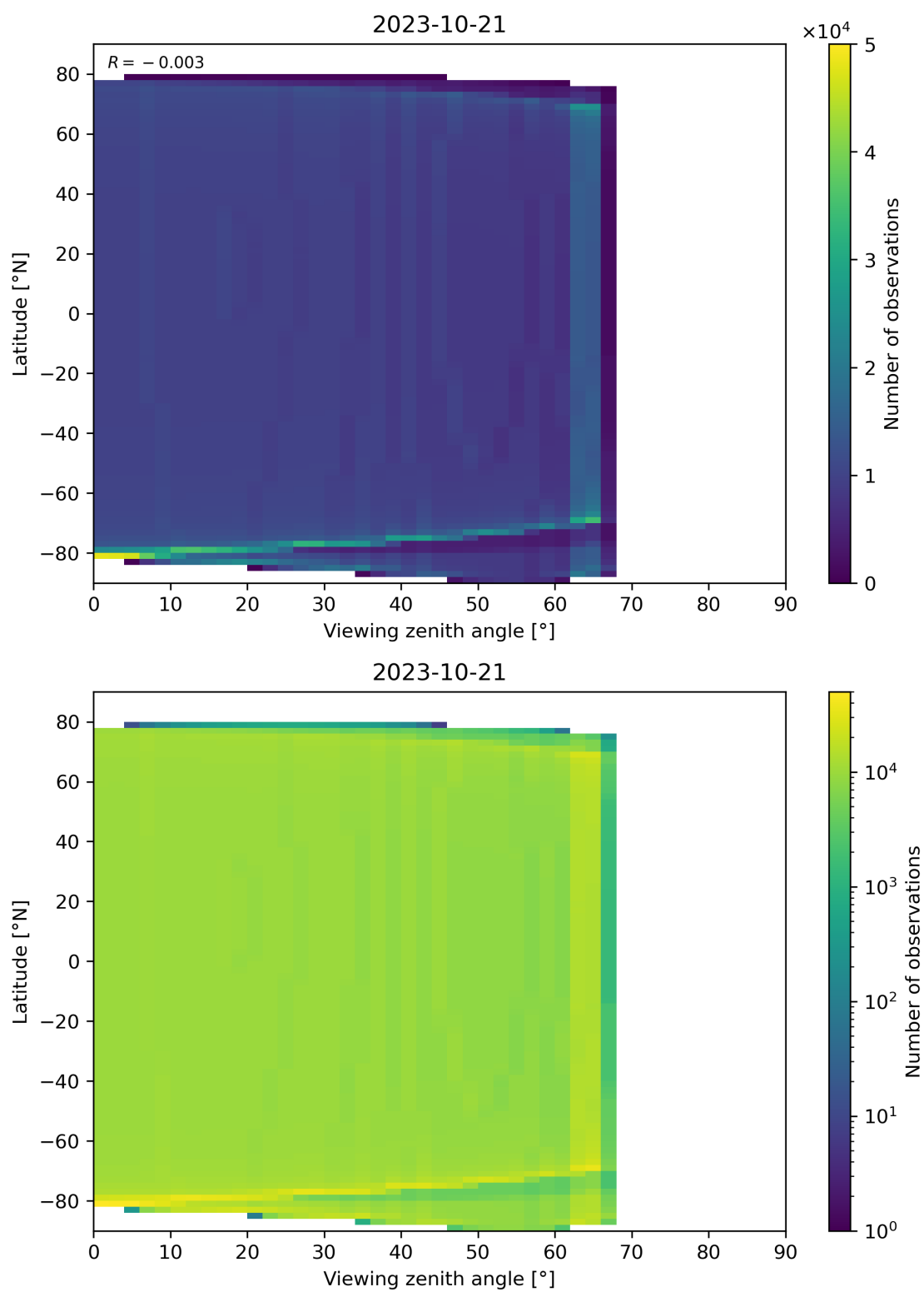
Figure 49: Scatter density plot of “Viewing zenith angle” against “Latitude” for 2023-10-20 to 2023-10-22.
