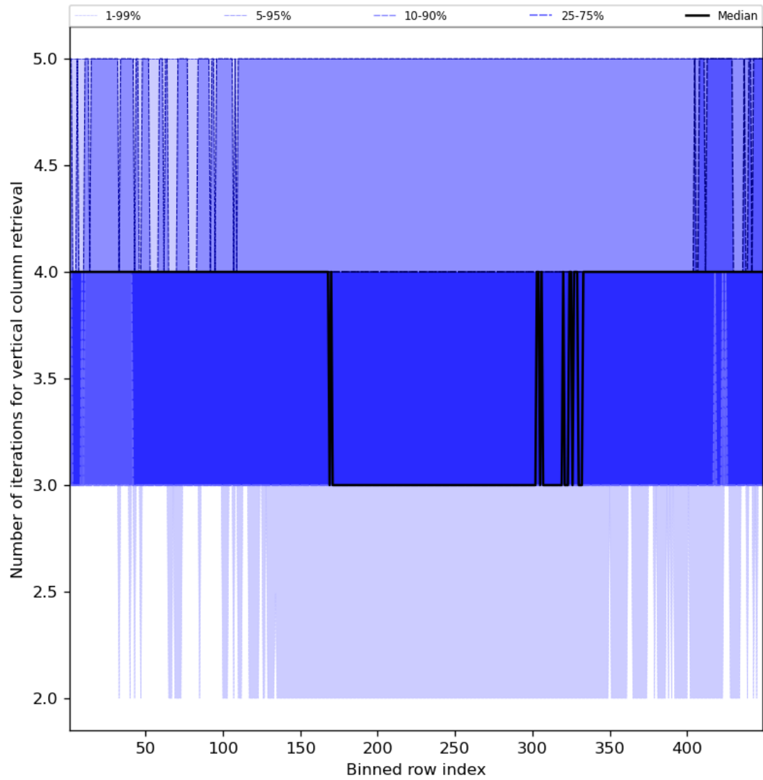
Figure 33: Along track statistics of “Number of iterations for vertical column retrieval” for 2023-10-20 to 2023-10-22
