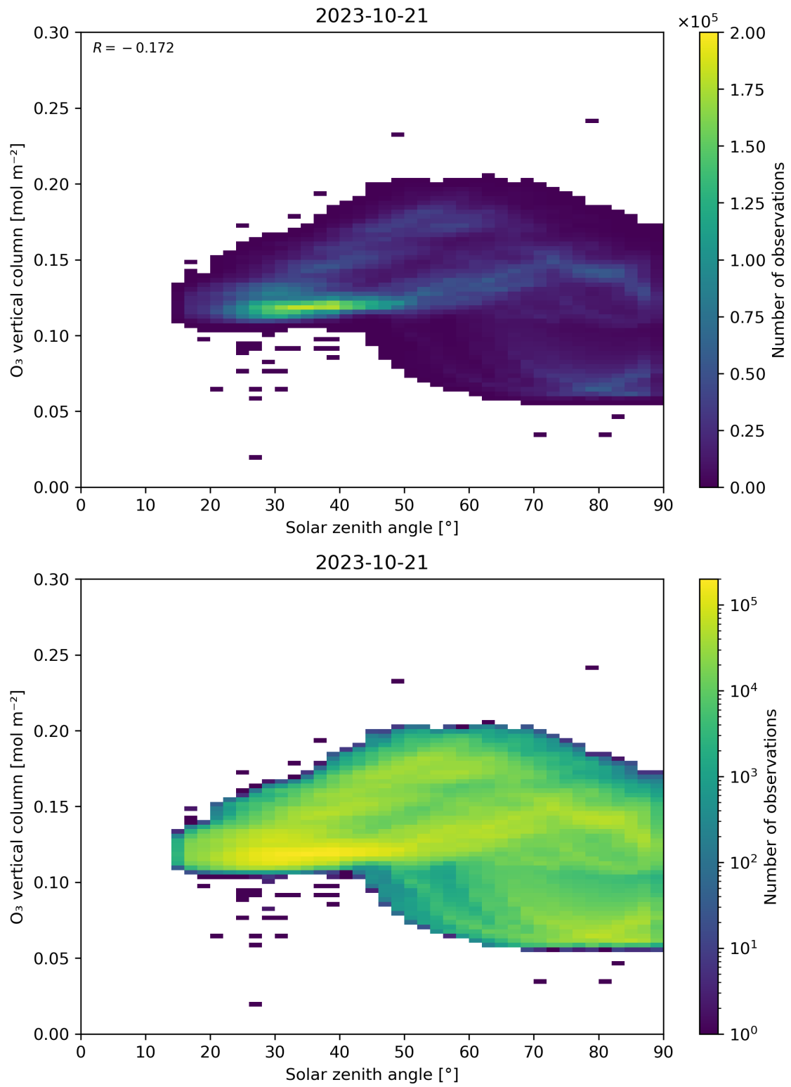
Figure 47: Scatter density plot of “Solar zenith angle” against “O 3 vertical column” for 2023-10-20 to 2023-10-22.
