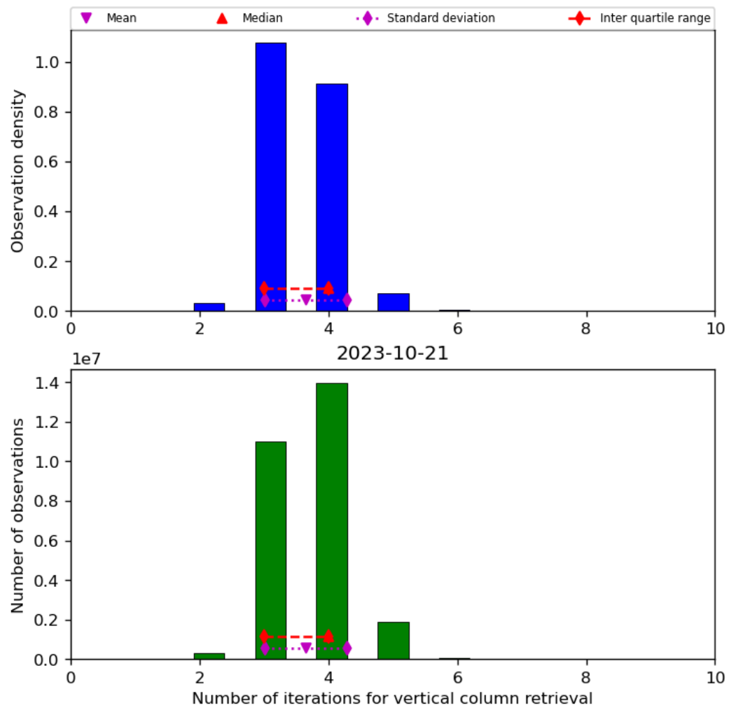
Figure 26: Histogram of “Number of iterations for vertical column retrieval” for 2023-10-20 to 2023-10-22
