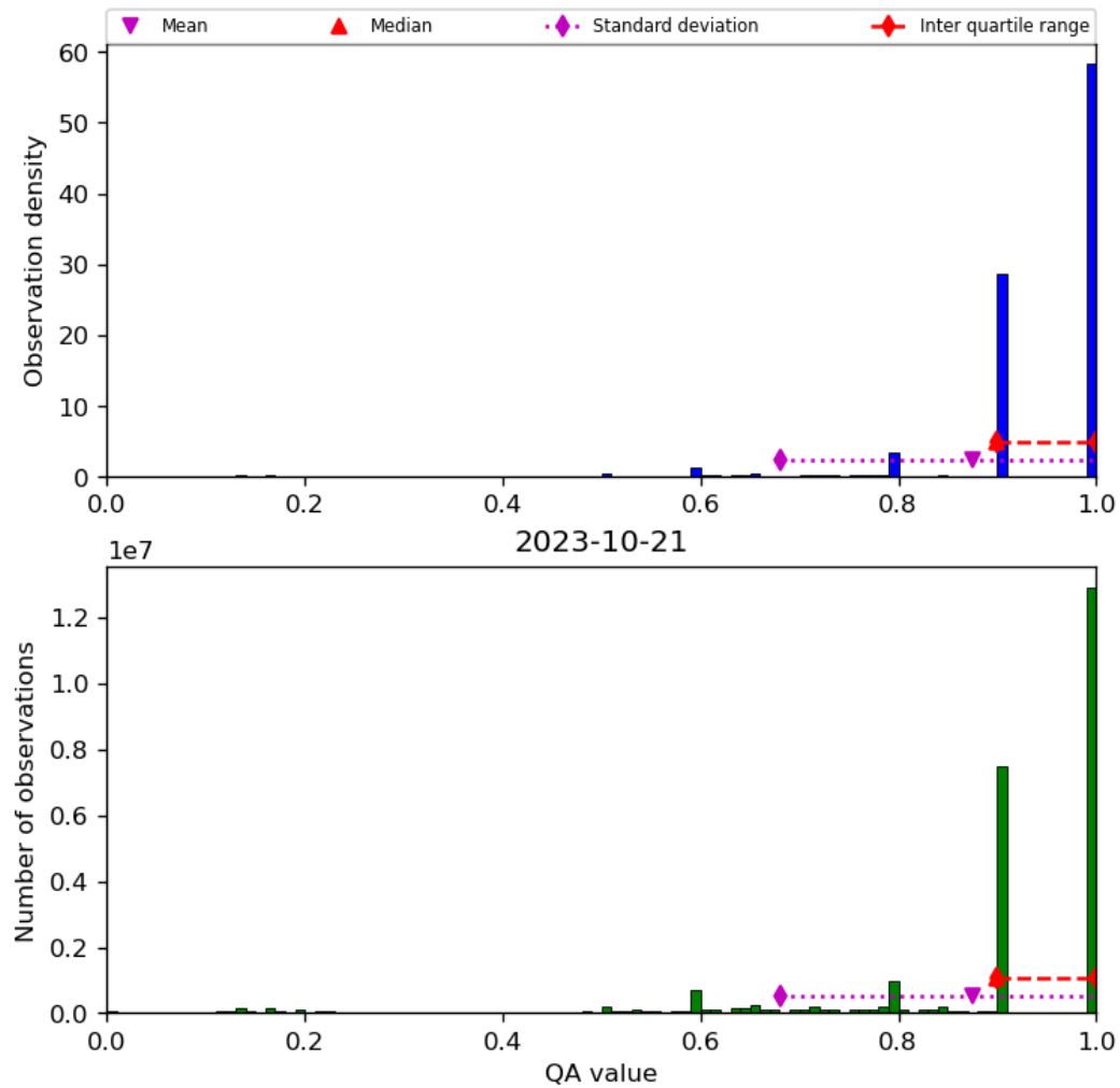
Figure 20: Histogram of “QA value” for 2023-10-20 to 2023-10-22
