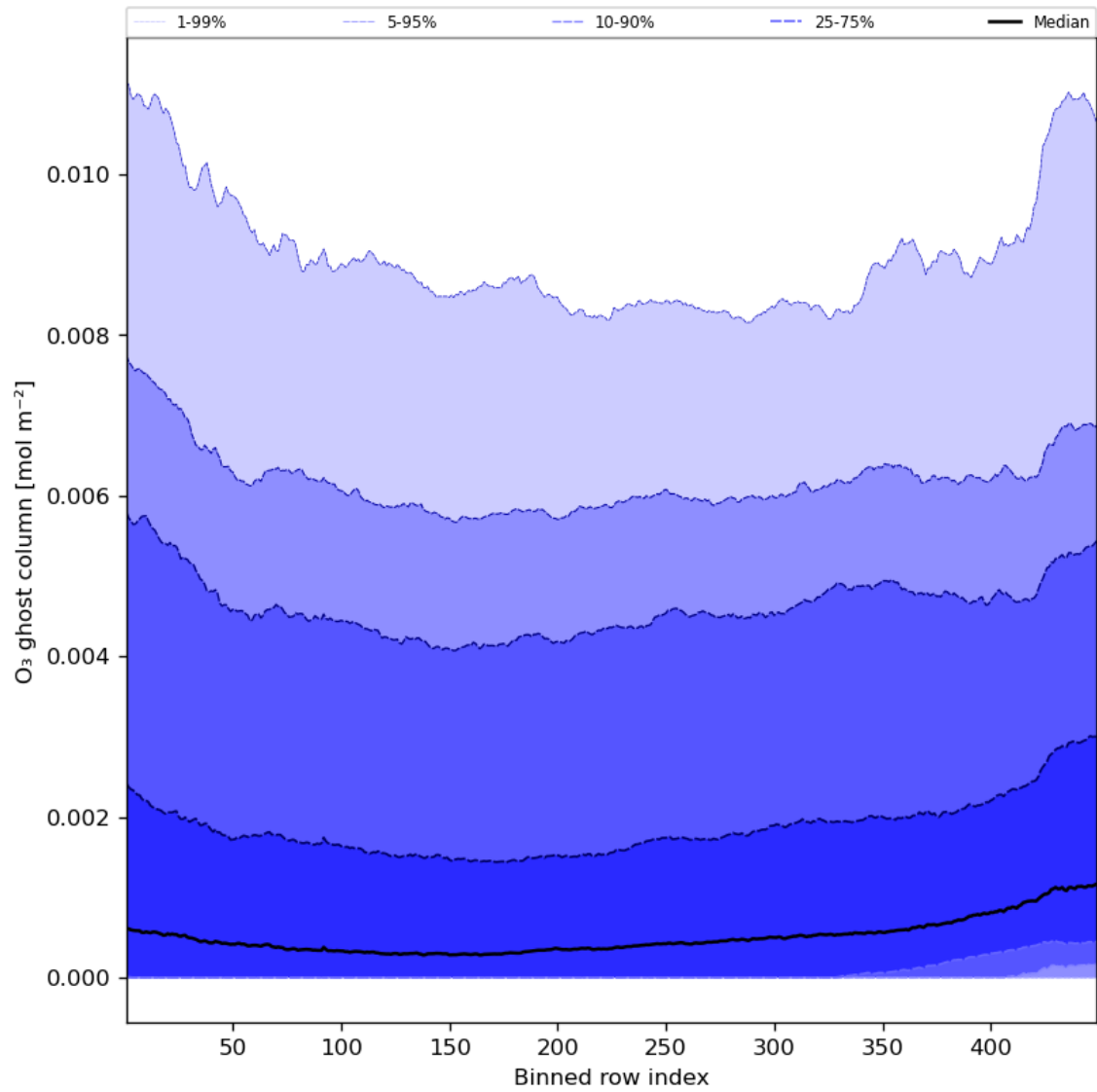
Figure 32: Along track statistics of “O 3 ghost column” for 2023-10-20 to 2023-10-22
