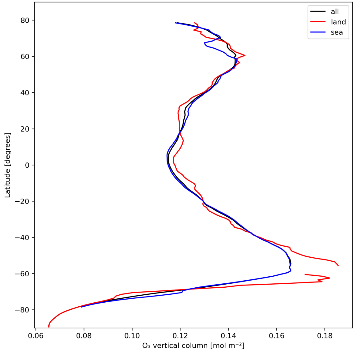
Figure 14: Zonal average of “O 3 vertical column” for 2023-10-20 to 2023-10-22.
