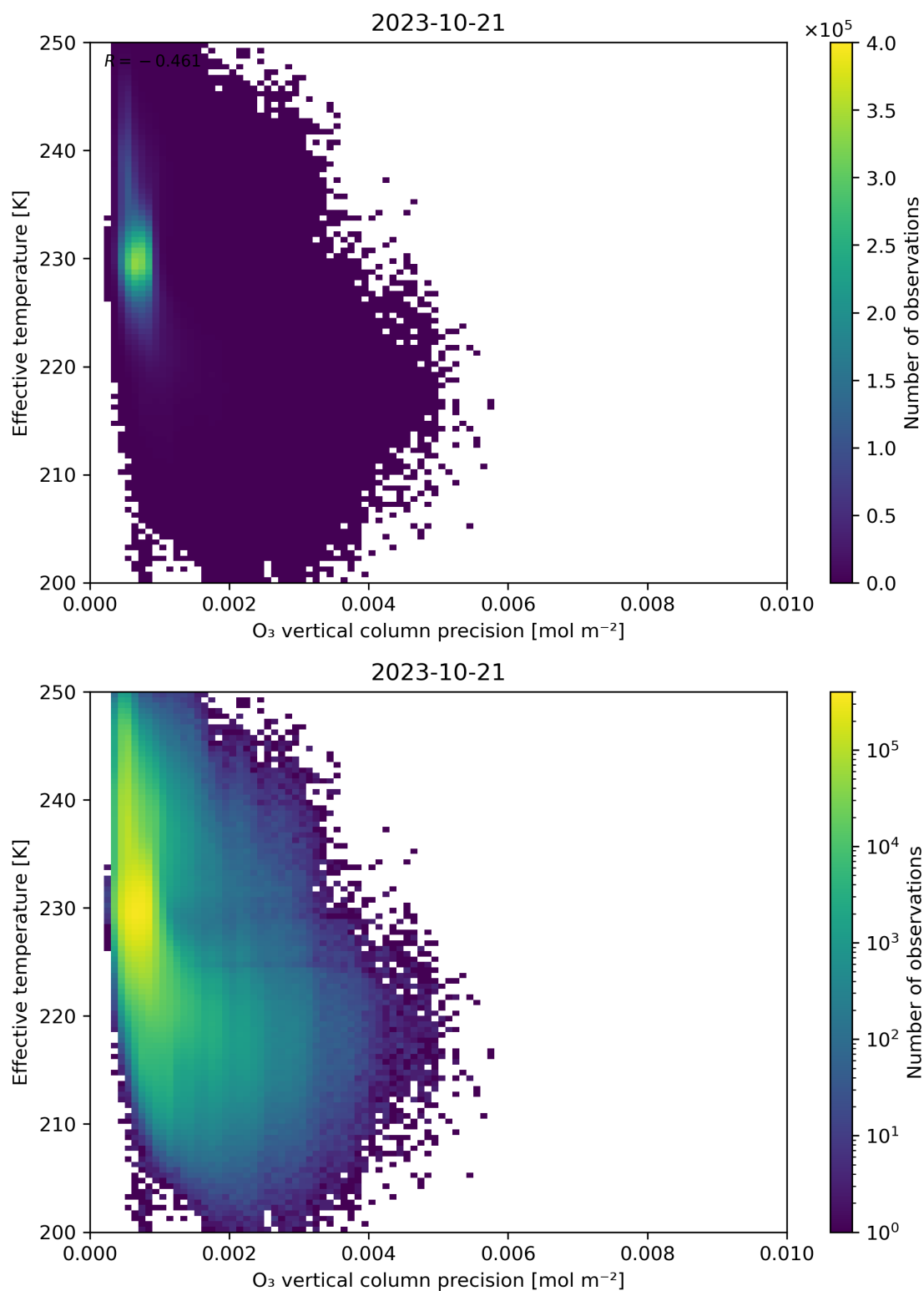
Figure 42: Scatter density plot of “O 3 vertical column precision” against “Effective temperature” for 2023-10-20 to 2023-10-22.
