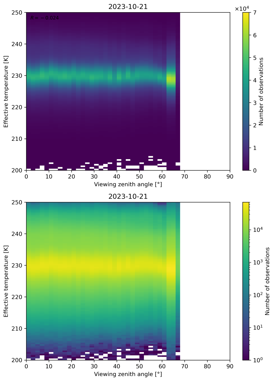
Figure 50: Scatter density plot of “Viewing zenith angle” against “Effective temperature” for 2023-10-20 to 2023-10-22.
