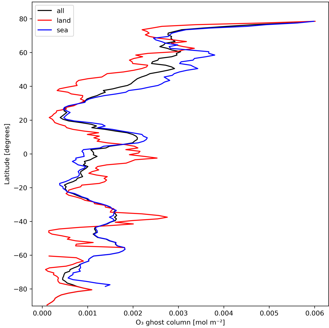
Figure 18: Zonal average of "O 3 ghost column" for 2023-10-20 to 2023-10-22.
