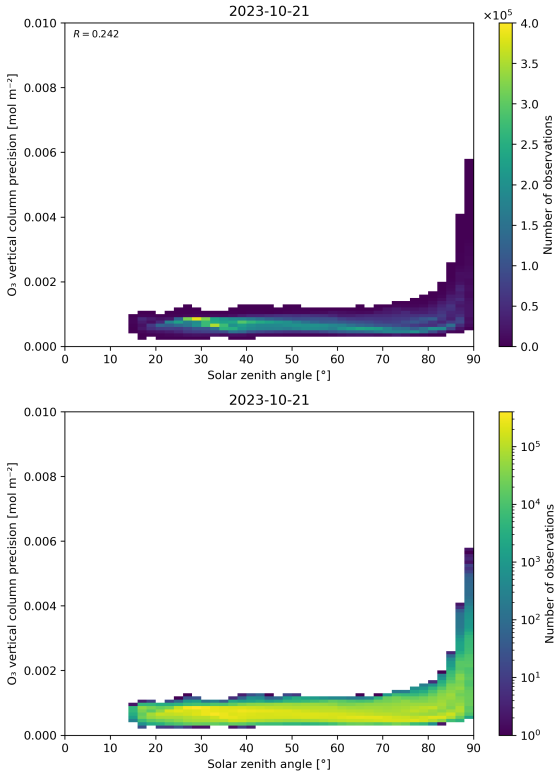
Figure 48: Scatter density plot of “Solar zenith angle” against “O 3 vertical column precision” for 2023-10-20 to 2023-10-22.
