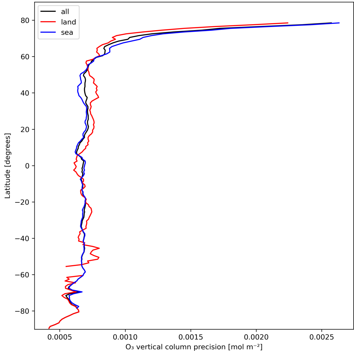
Figure 15: Zonal average of “O 3 vertical column precision” for 2023-10-20 to 2023-10-22.
