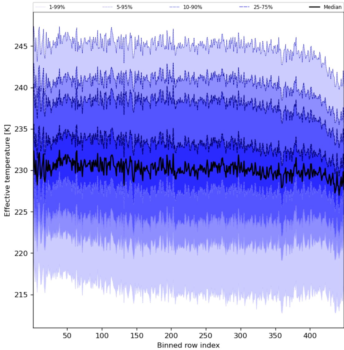
Figure 31: Along track statistics of “Effective temperature” for 2023-10-20 to 2023-10-22
