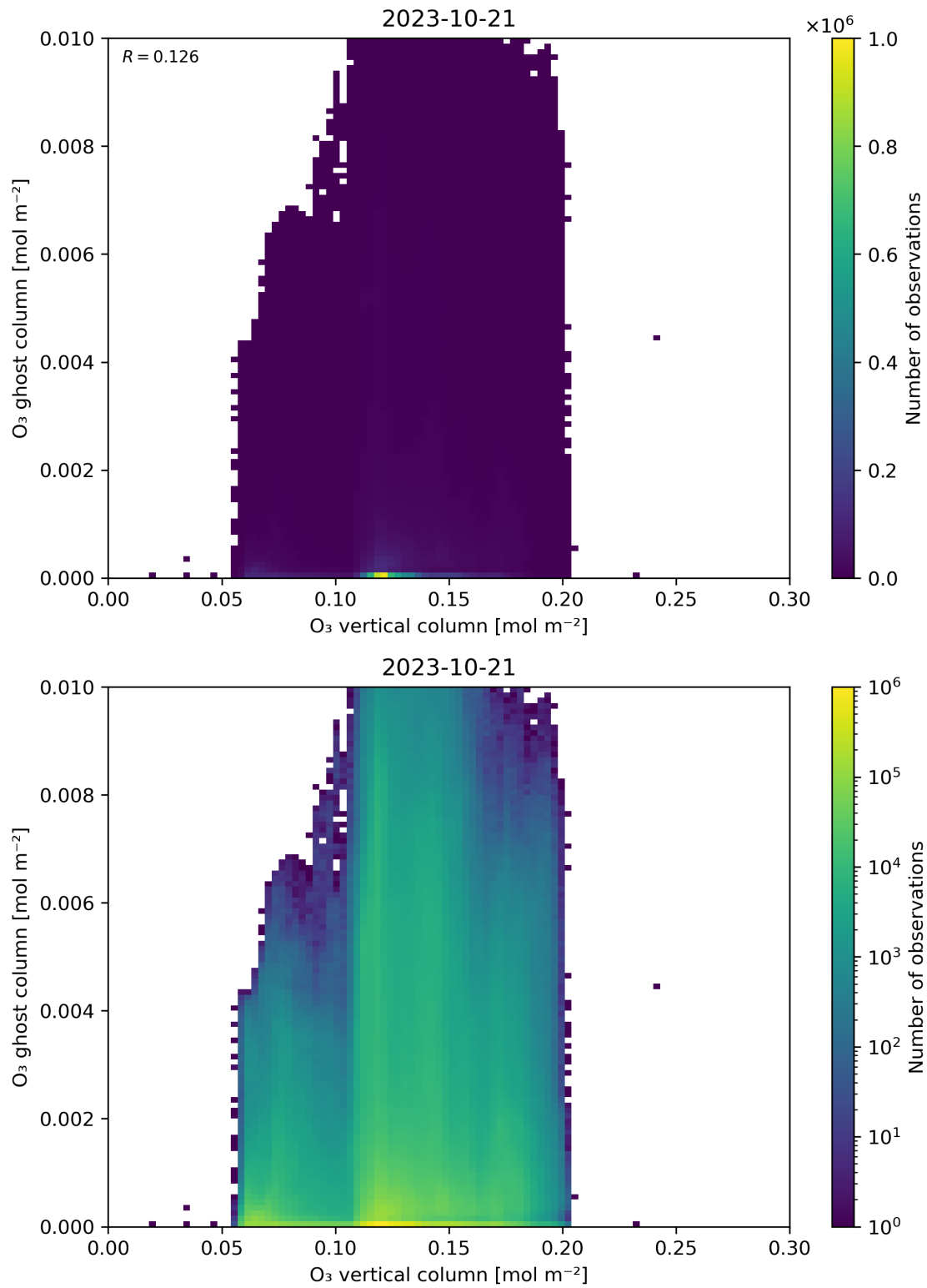
Figure 40: Scatter density plot of “O 3 vertical column” against “O 3 ghost column” for 2023-10-20 to 2023-10-22.
