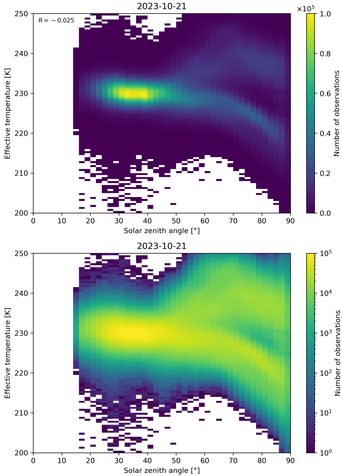
Figure 45: Scatter density plot of “Solar zenith angle” against “Effective temperature” for 2023-10-20 to 2023-10-22.
