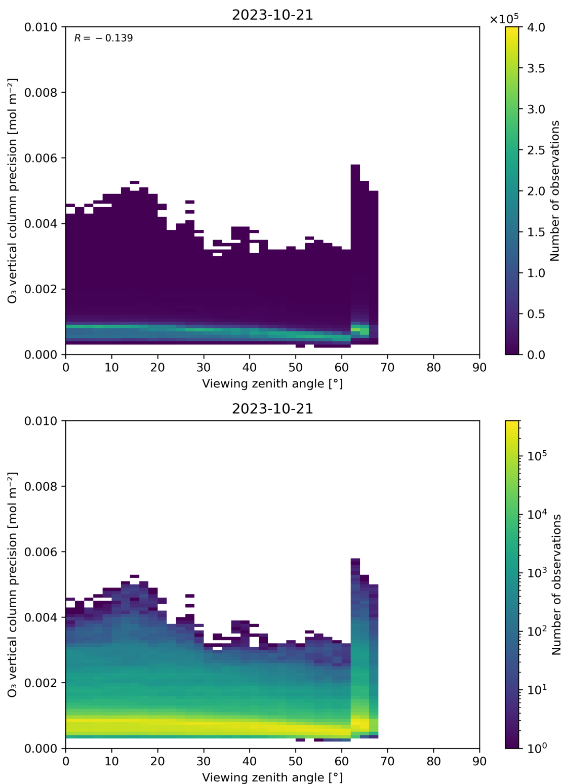
Figure 53: Scatter density plot of “Viewing zenith angle” against “O 3 vertical column precision” for 2023-10-20 to 2023-10-22.
