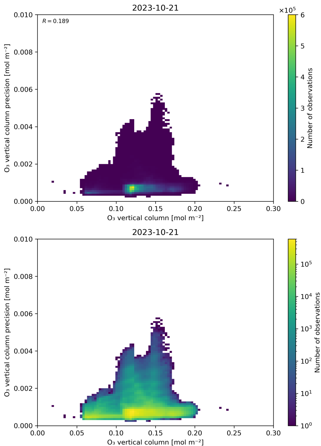
Figure 41: Scatter density plot of “O 3 vertical column” against “O 3 vertical column precision” for 2023-10-20 to 2023-10-22.
