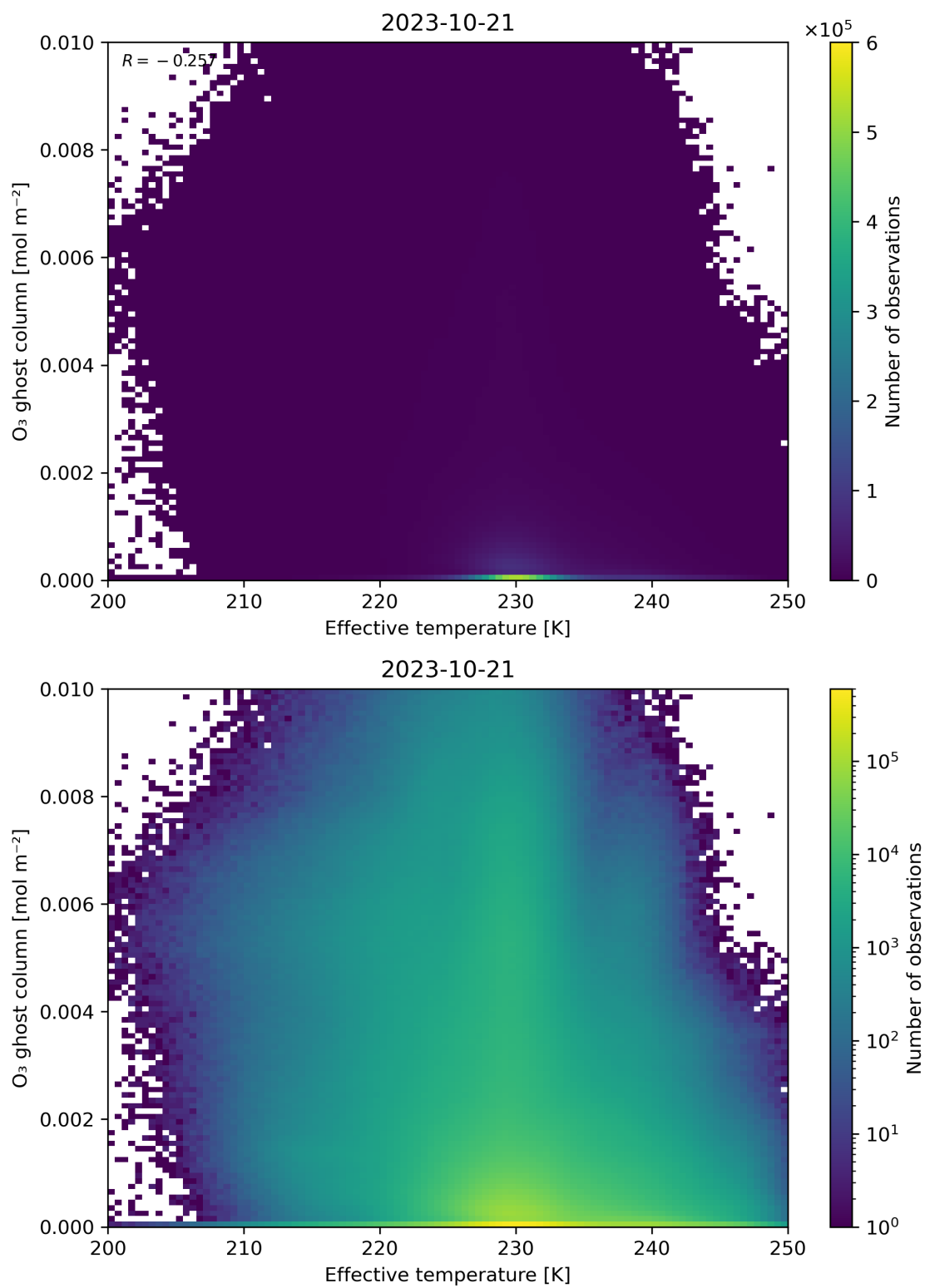
Figure 38: Scatter density plot of “Effective temperature” against “O 3 ghost column” for 2023-10-20 to 2023-10-22.
