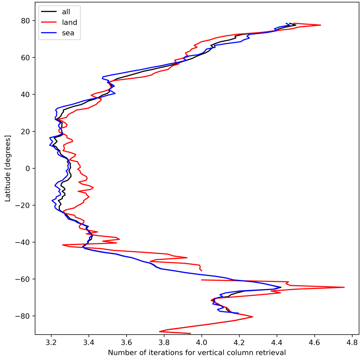
Figure 19: Zonal average of “Number of iterations for vertical column retrieval” for 2023-10-20 to 2023-10-22.
