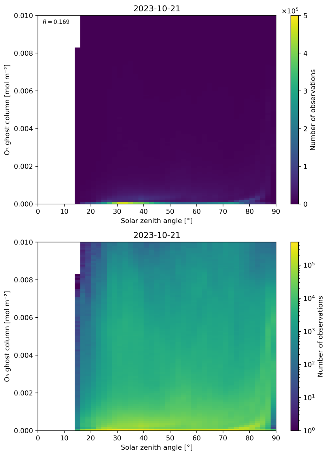
Figure 46: Scatter density plot of “Solar zenith angle” against “O 3 ghost column” for 2023-10-20 to 2023-10-22.
