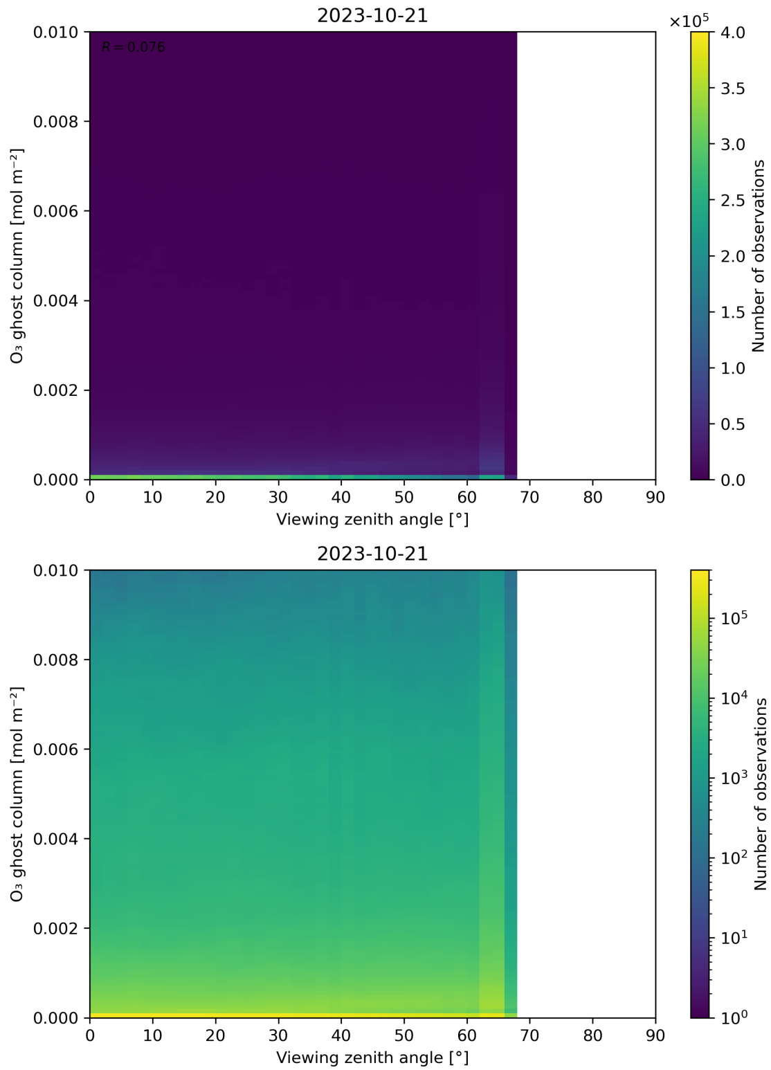
Figure 51: Scatter density plot of “Viewing zenith angle” against “O 3 ghost column” for 2023-10-20 to 2023-10-22.
