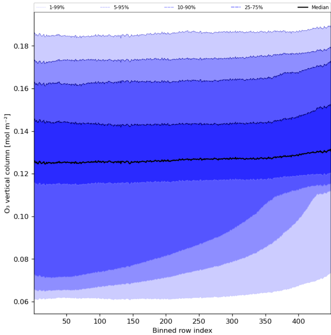
Figure 28: Along track statistics of “O 3 vertical column” for 2023-10-20 to 2023-10-22
