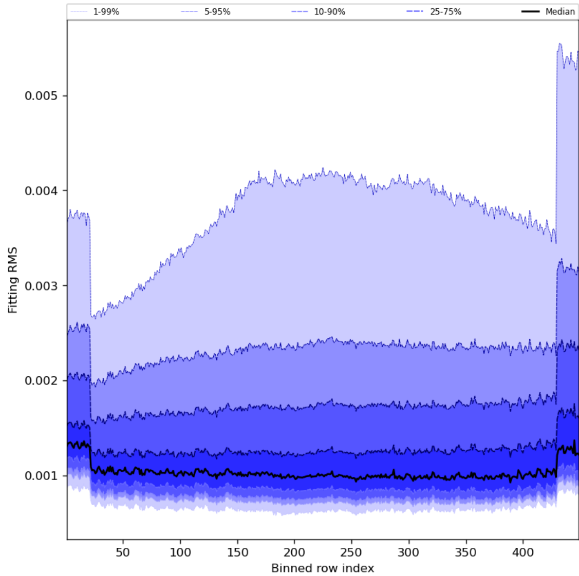
Figure 30: Along track statistics of “Fitting RMS” for 2023-10-20 to 2023-10-22
