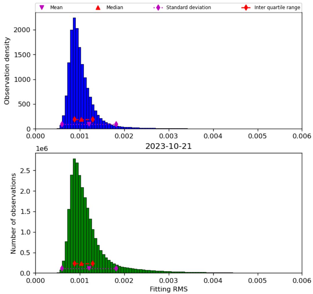
Figure 23: Histogram of “Fitting RMS” for 2023-10-20 to 2023-10-22
