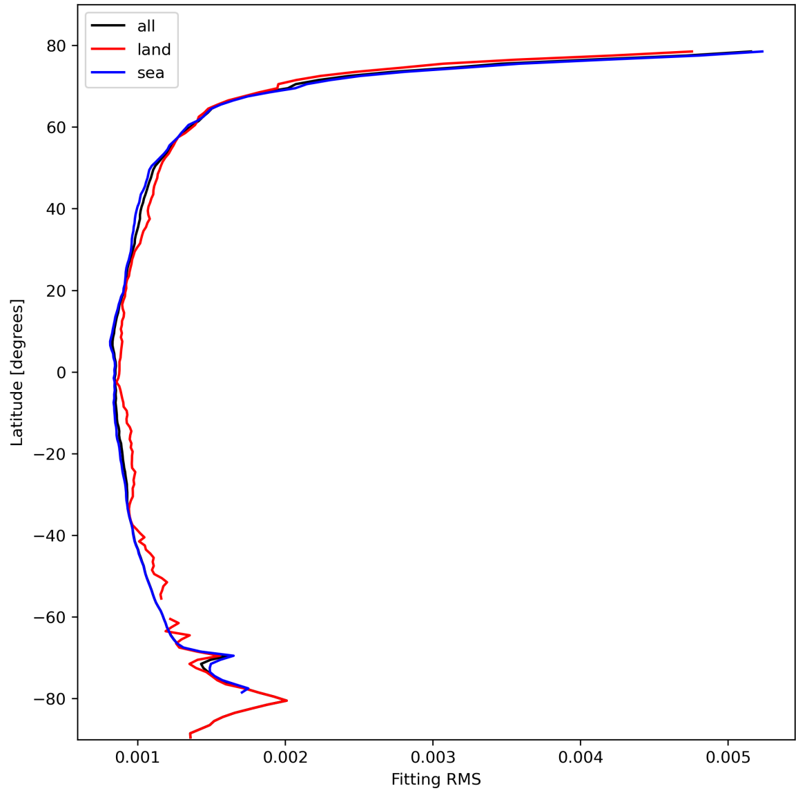
Figure 16: Zonal average of “Fitting RMS” for 2023-10-20 to 2023-10-22.
