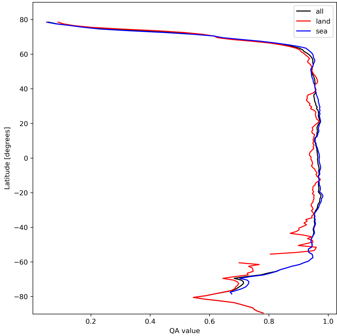
Figure 13: Zonal average of “QA value” for 2023-10-20 to 2023-10-22.
