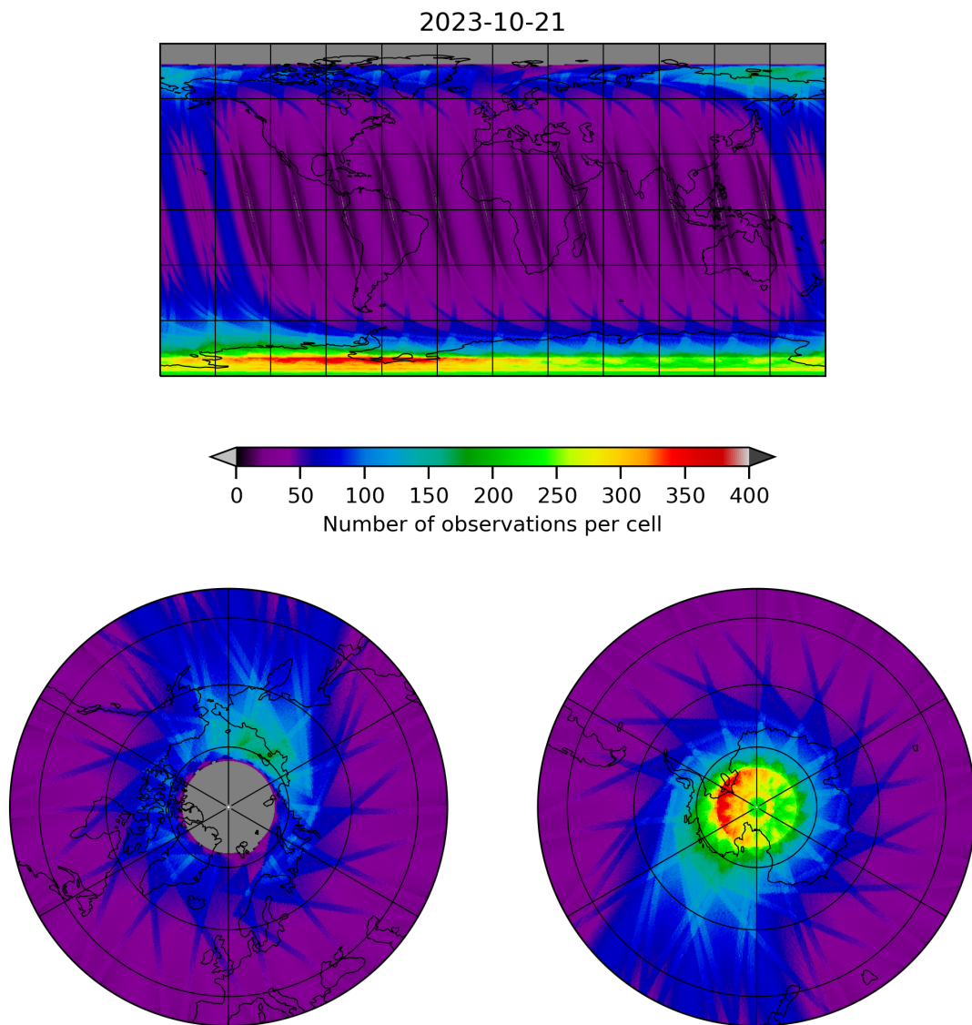
Figure 12: Map of the number of observations for 2023-10-20 to 2023-10-22
