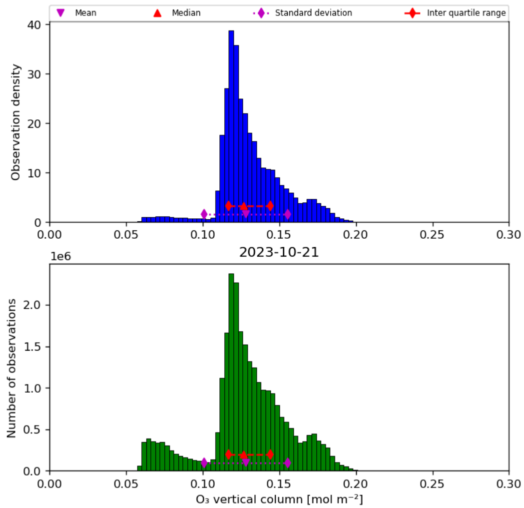
Figure 21: Histogram of “O 3 vertical column” for 2023-10-20 to 2023-10-22
