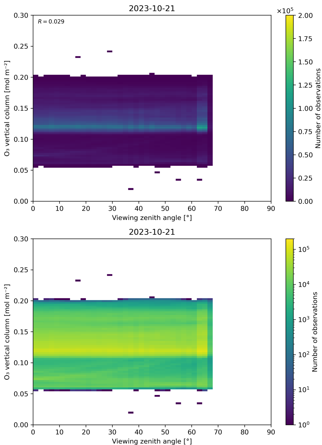
Figure 52: Scatter density plot of “Viewing zenith angle” against “O 3 vertical column” for 2023-10-20 to 2023-10-22.
