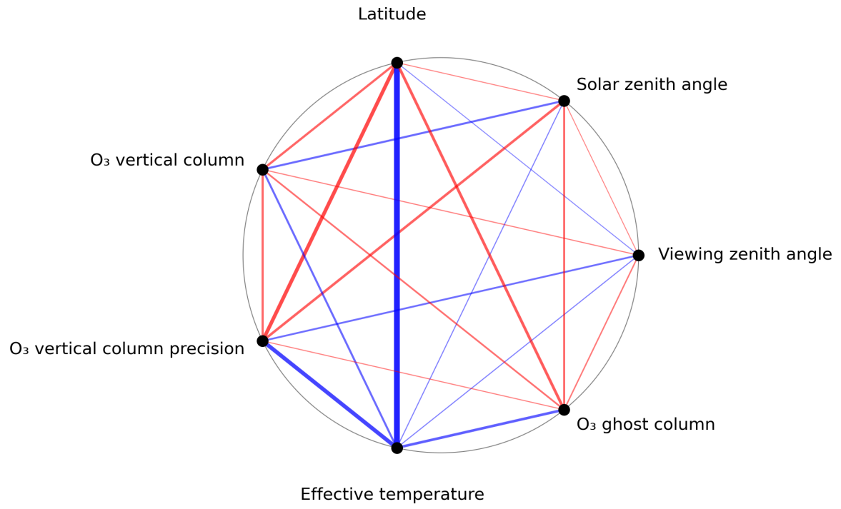
Figure 1: Map of correlation graph for 2023-10-20 to 2023-10-22.
