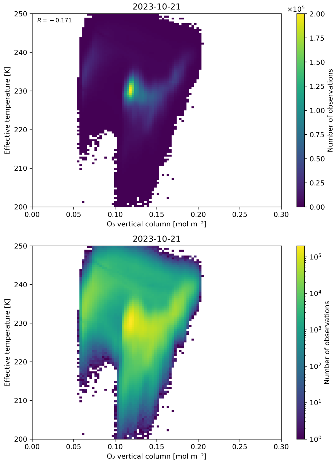
Figure 39: Scatter density plot of “O 3 vertical column” against “Effective temperature” for 2023-10-20 to 2023-10-22.
