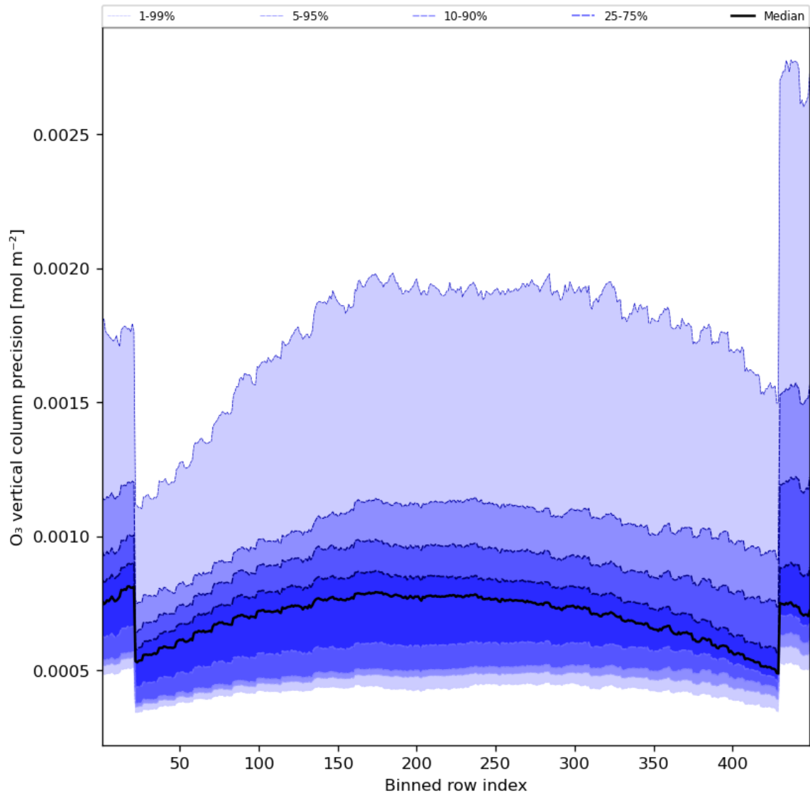
Figure 29: Along track statistics of “O 3 vertical column precision” for 2023-10-20 to 2023-10-22
