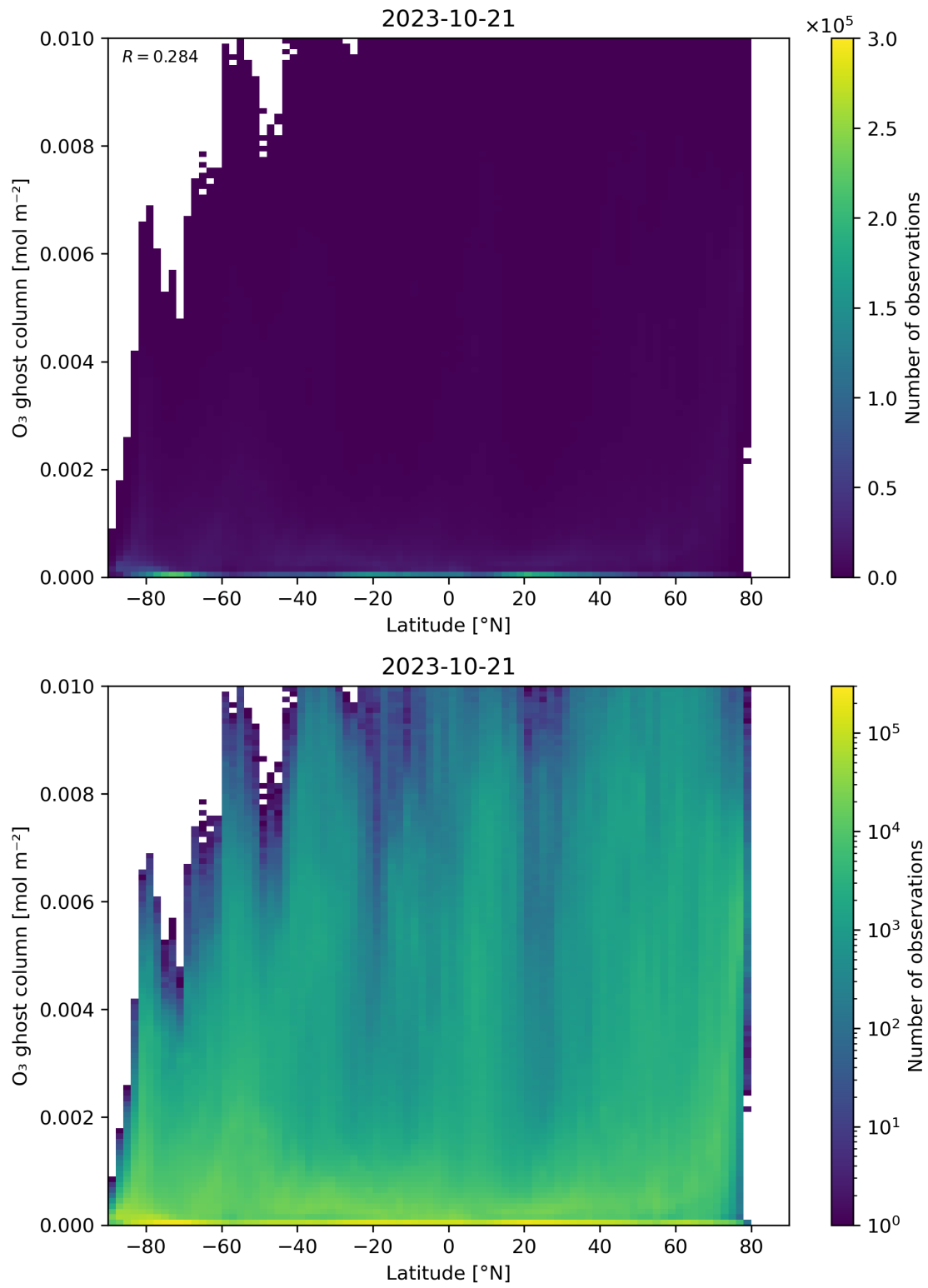
Figure 35: Scatter density plot of “Latitude” against “O 3 ghost column” for 2023-10-20 to 2023-10-22.
