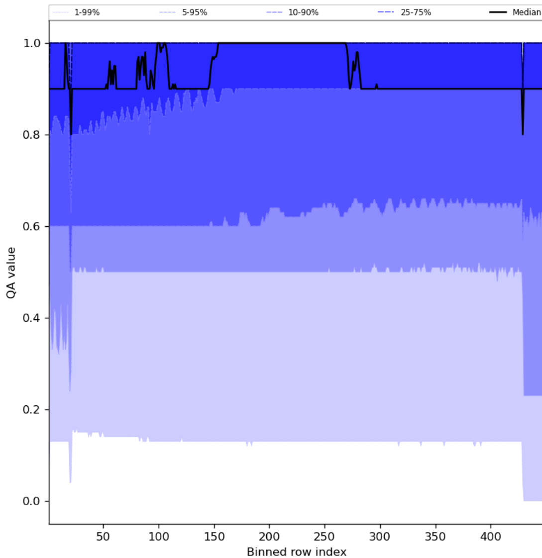
Figure 27: Along track statistics of “QA value” for 2023-10-20 to 2023-10-22
