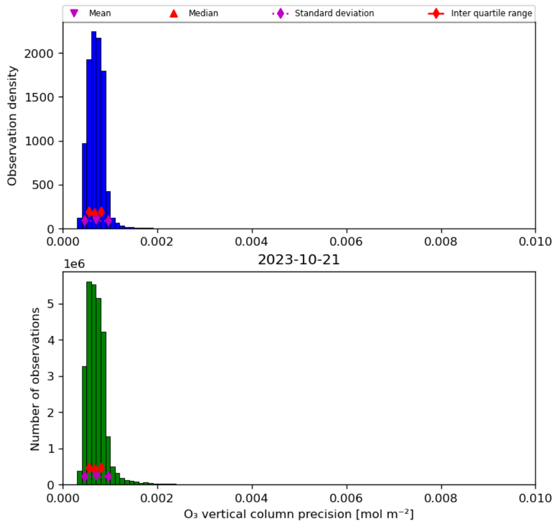
Figure 22: Histogram of “O 3 vertical column precision” for 2023-10-20 to 2023-10-22
