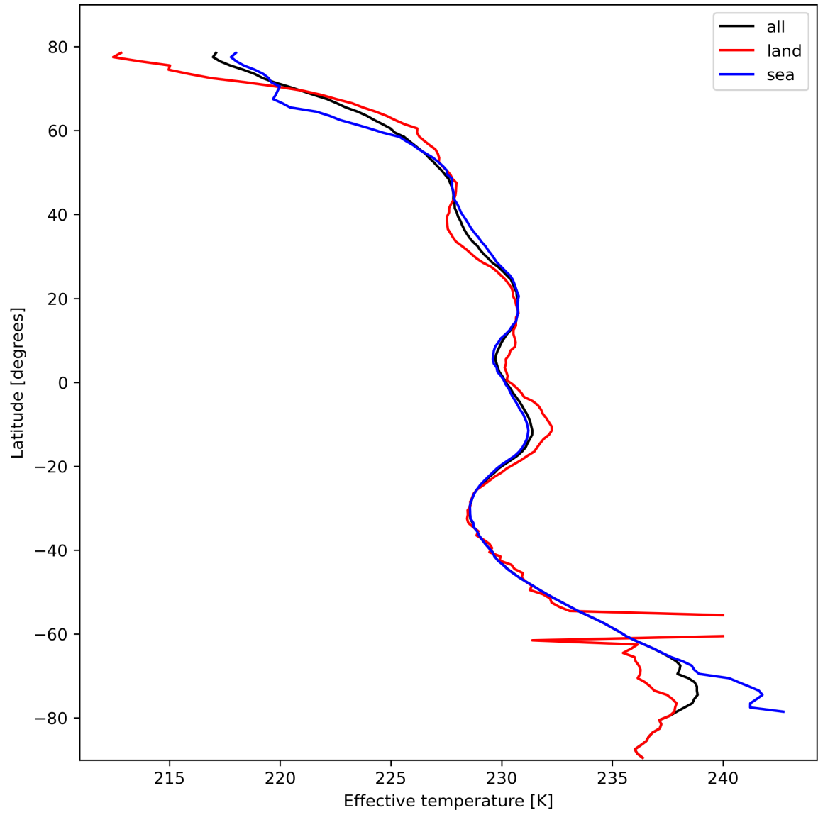
Figure 17: Zonal average of "Effective temperature" for 2023-10-20 to 2023-10-22.
