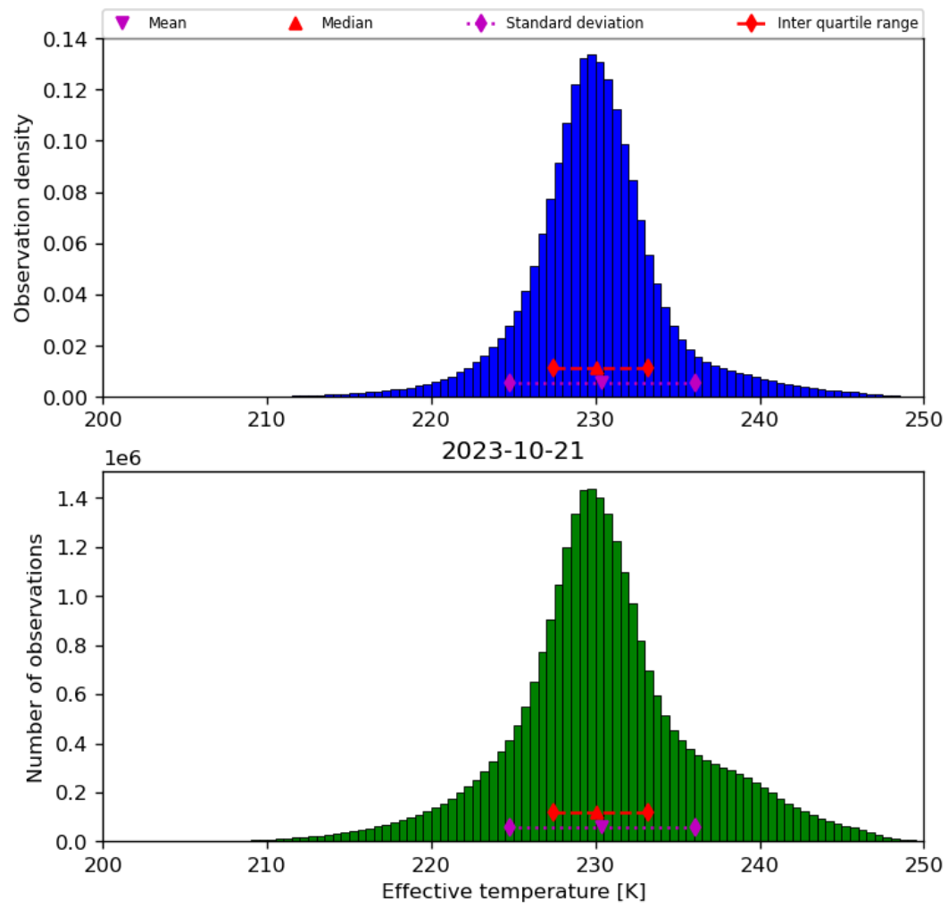
Figure 24: Histogram of “Effective temperature” for 2023-10-20 to 2023-10-22
