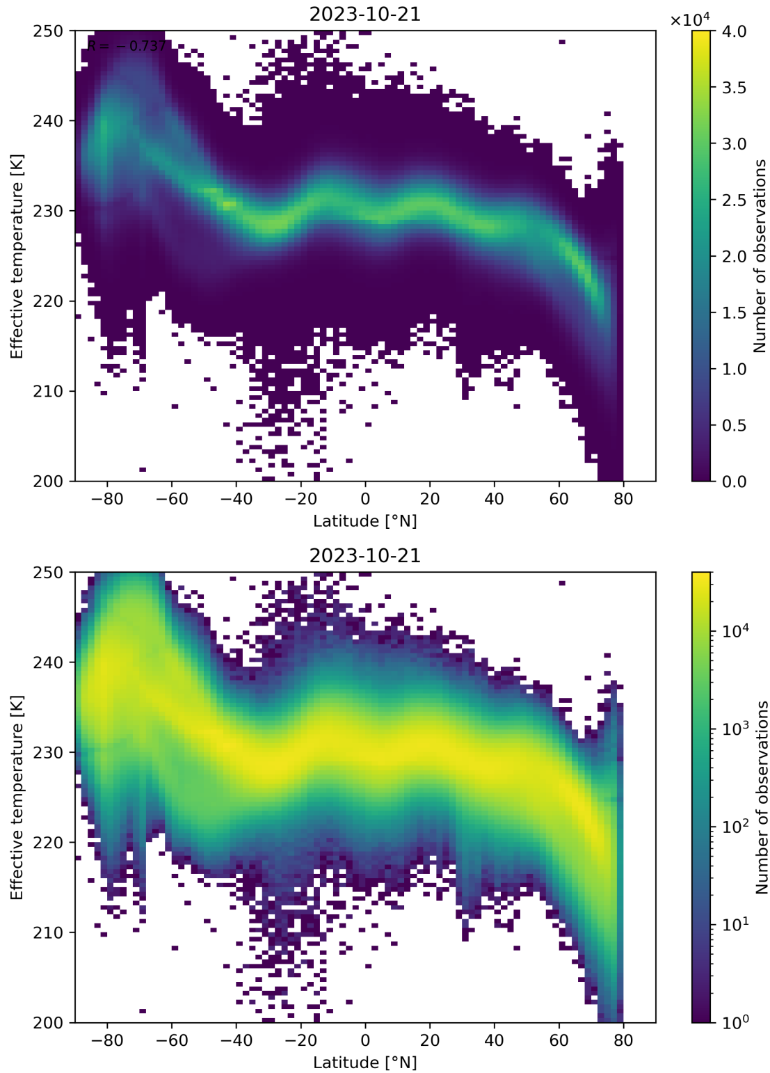
Figure 34: Scatter density plot of “Latitude” against “Effective temperature” for 2023-10-20 to 2023-10-22.
