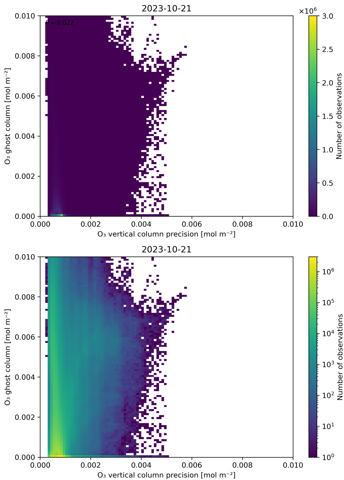
Figure 43: Scatter density plot of “O 3 vertical column precision” against “O 3 ghost column” for 2023-10-20 to 2023-10-22.
