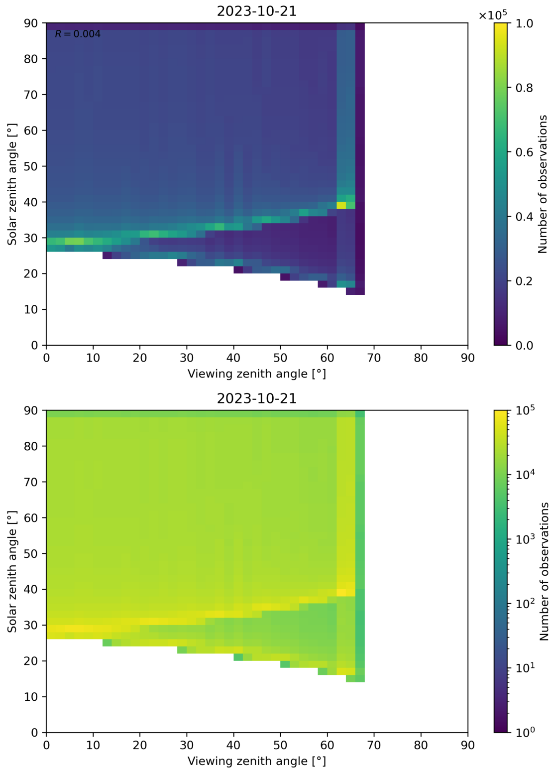
Figure 54: Scatter density plot of “Viewing zenith angle” against “Solar zenith angle” for 2023-10-20 to 2023-10-22.
