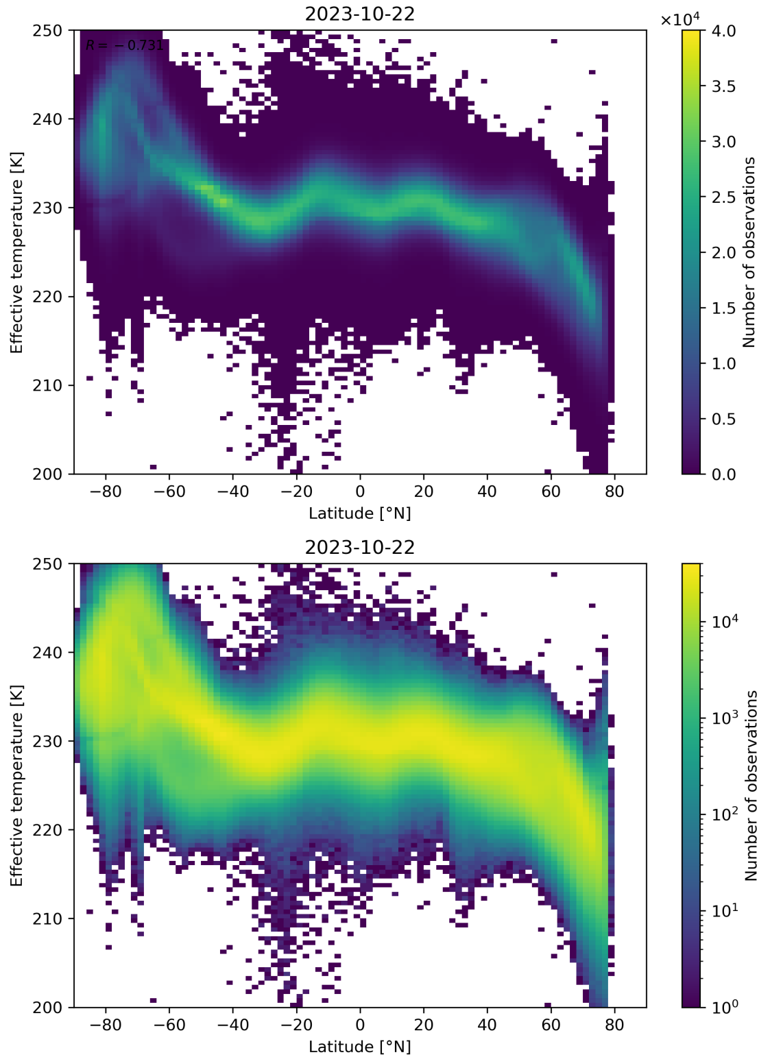
Figure 34: Scatter density plot of “Latitude” against “Effective temperature” for 2023-10-22 to 2023-10-23.
