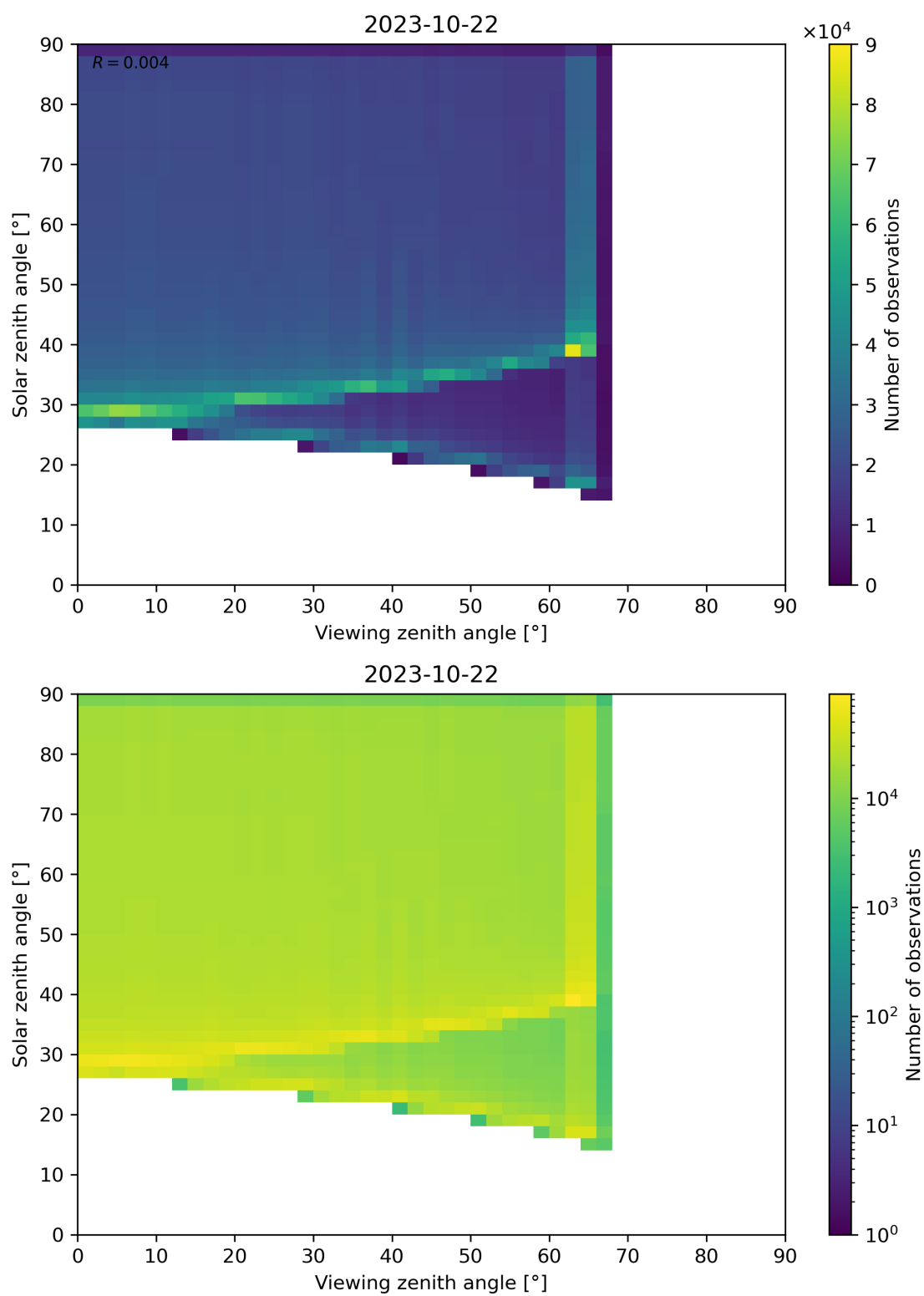
Figure 54: Scatter density plot of “Viewing zenith angle” against “Solar zenith angle” for 2023-10-22 to 2023-10-23.
