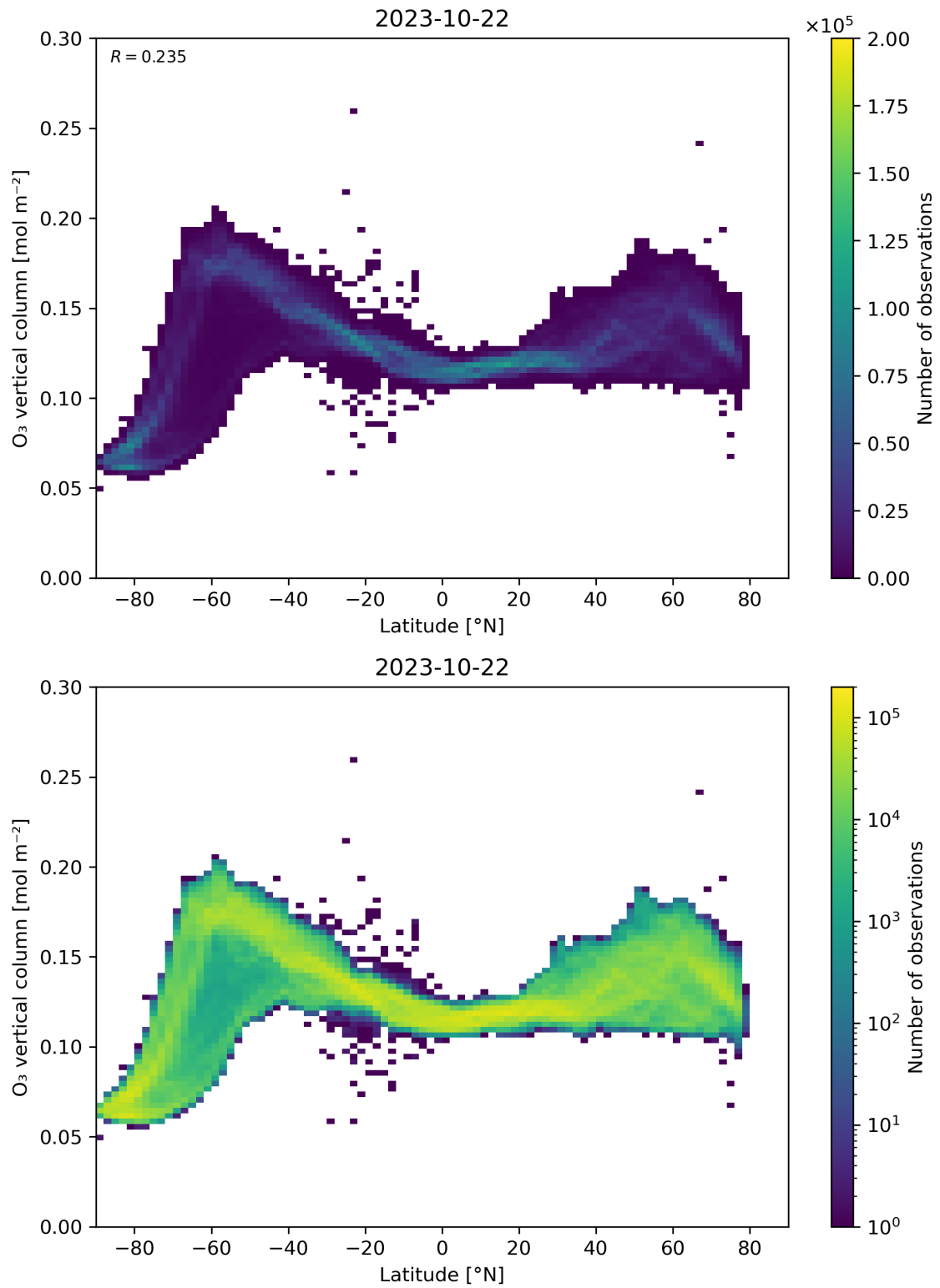
Figure 36: Scatter density plot of “Latitude” against “O 3 vertical column” for 2023-10-22 to 2023-10-23.
