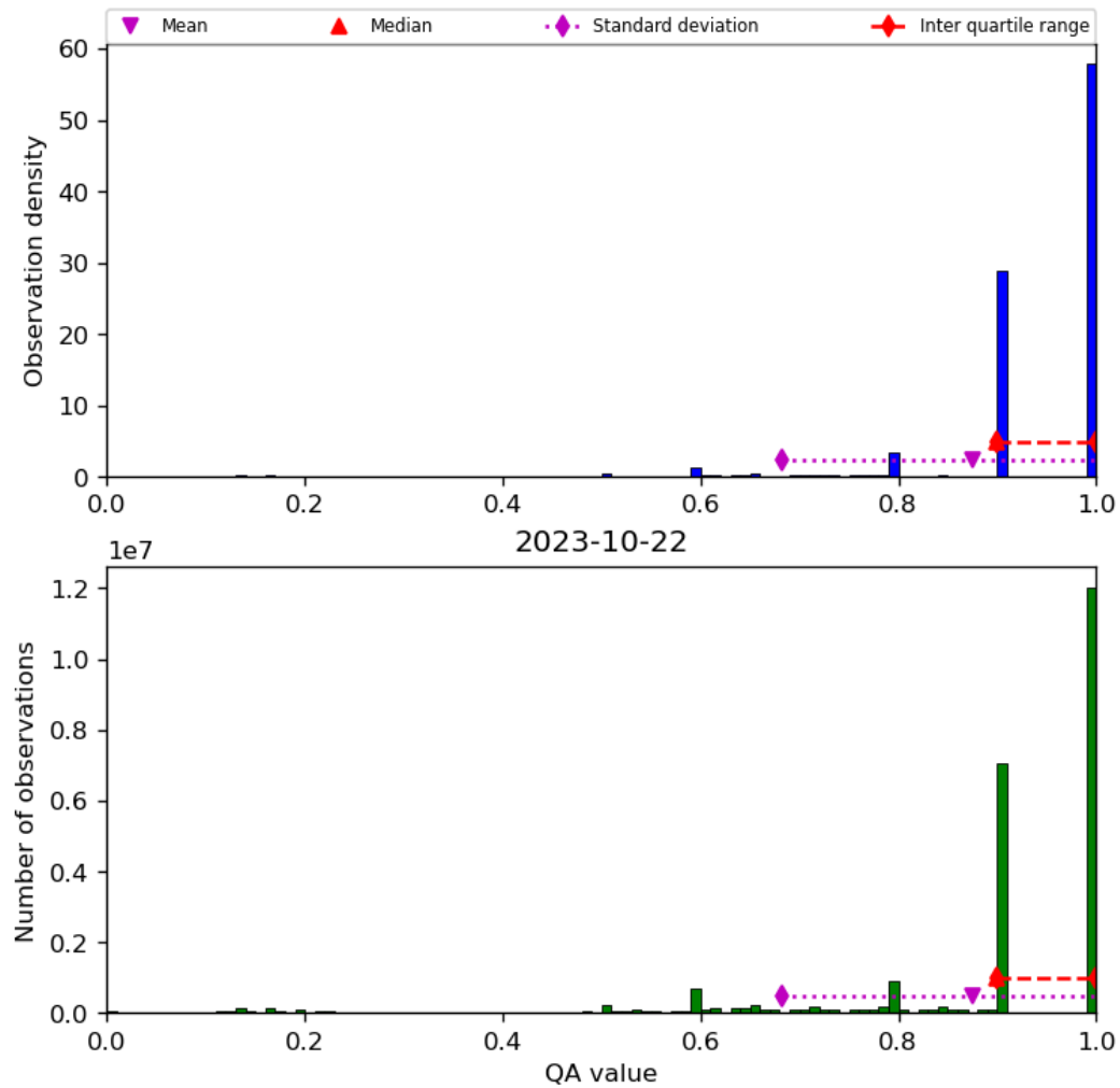
Figure 20: Histogram of “QA value” for 2023-10-22 to 2023-10-23
