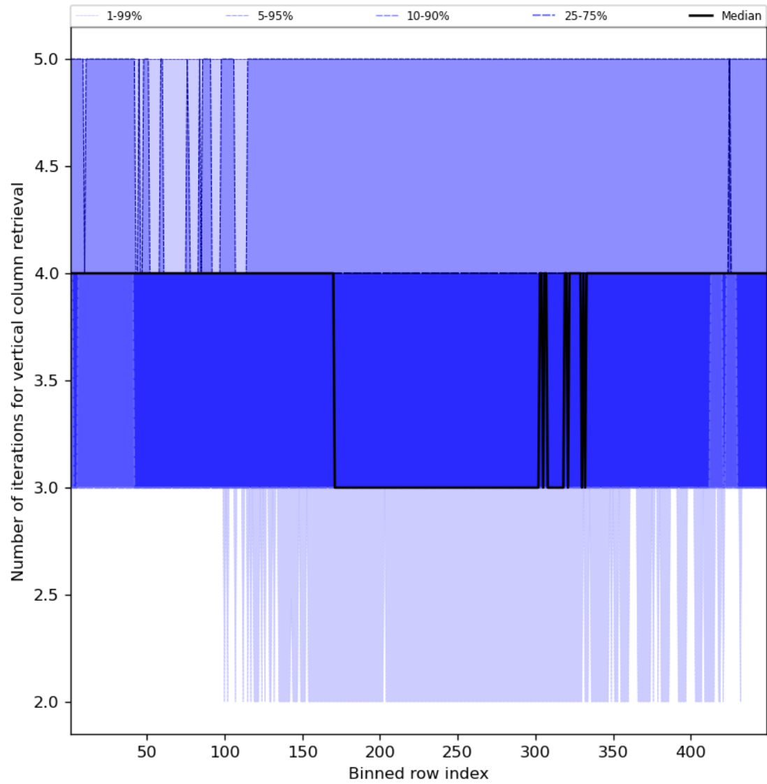
Figure 33: Along track statistics of “Number of iterations for vertical column retrieval” for 2023-10-22 to 2023-10-23
