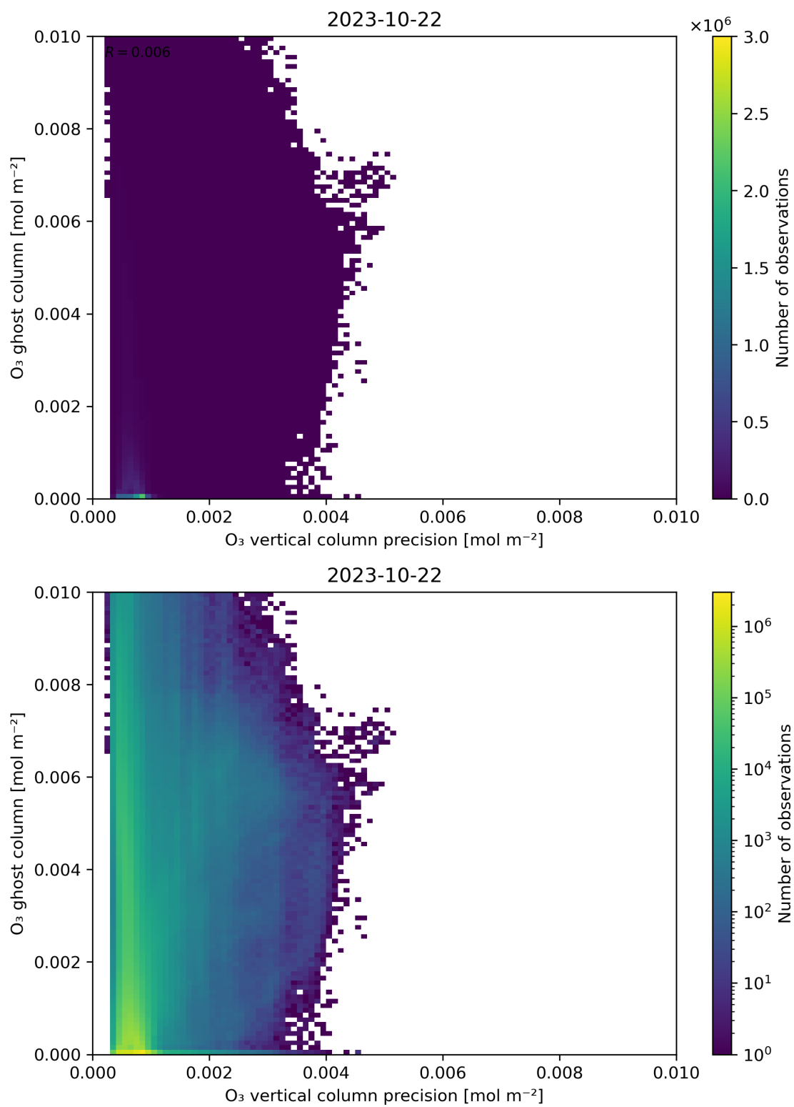
Figure 43: Scatter density plot of “O 3 vertical column precision” against “O 3 ghost column” for 2023-10-22 to 2023-10-23.
