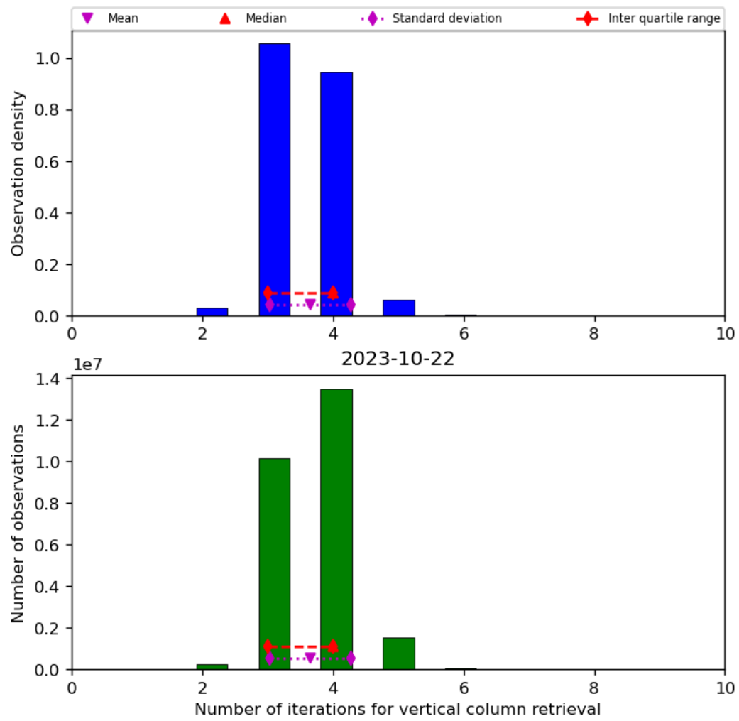
Figure 26: Histogram of “Number of iterations for vertical column retrieval” for 2023-10-22 to 2023-10-23
