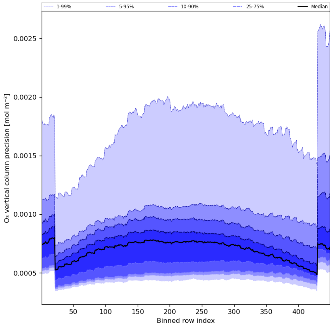
Figure 29: Along track statistics of “O 3 vertical column precision” for 2023-10-22 to 2023-10-23
