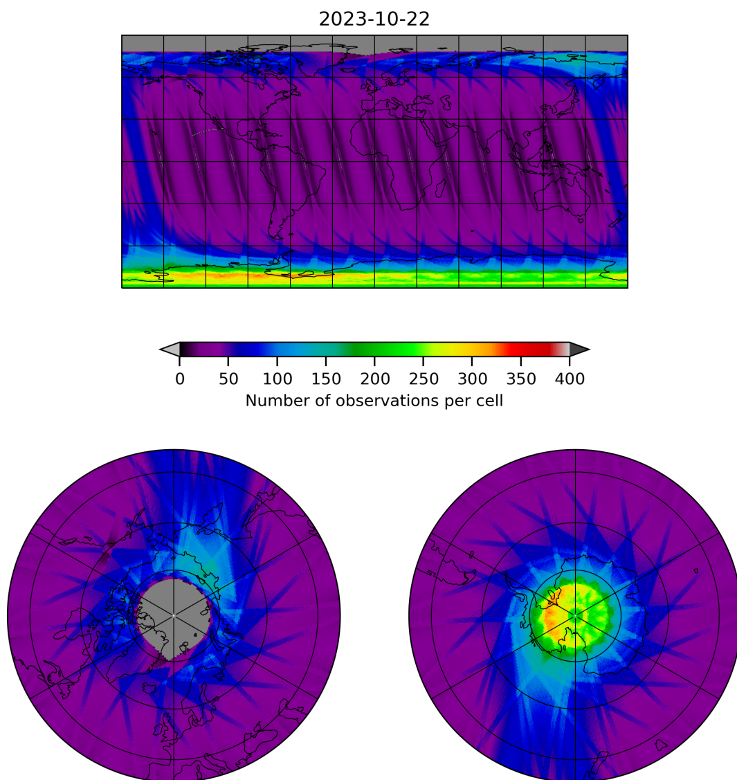
Figure 12: Map of the number of observations for 2023-10-22 to 2023-10-23
