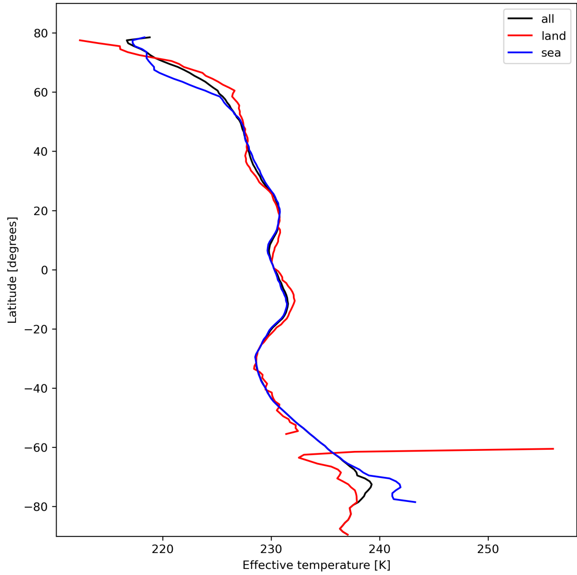
Figure 17: Zonal average of “Effective temperature” for 2023-10-22 to 2023-10-23.
