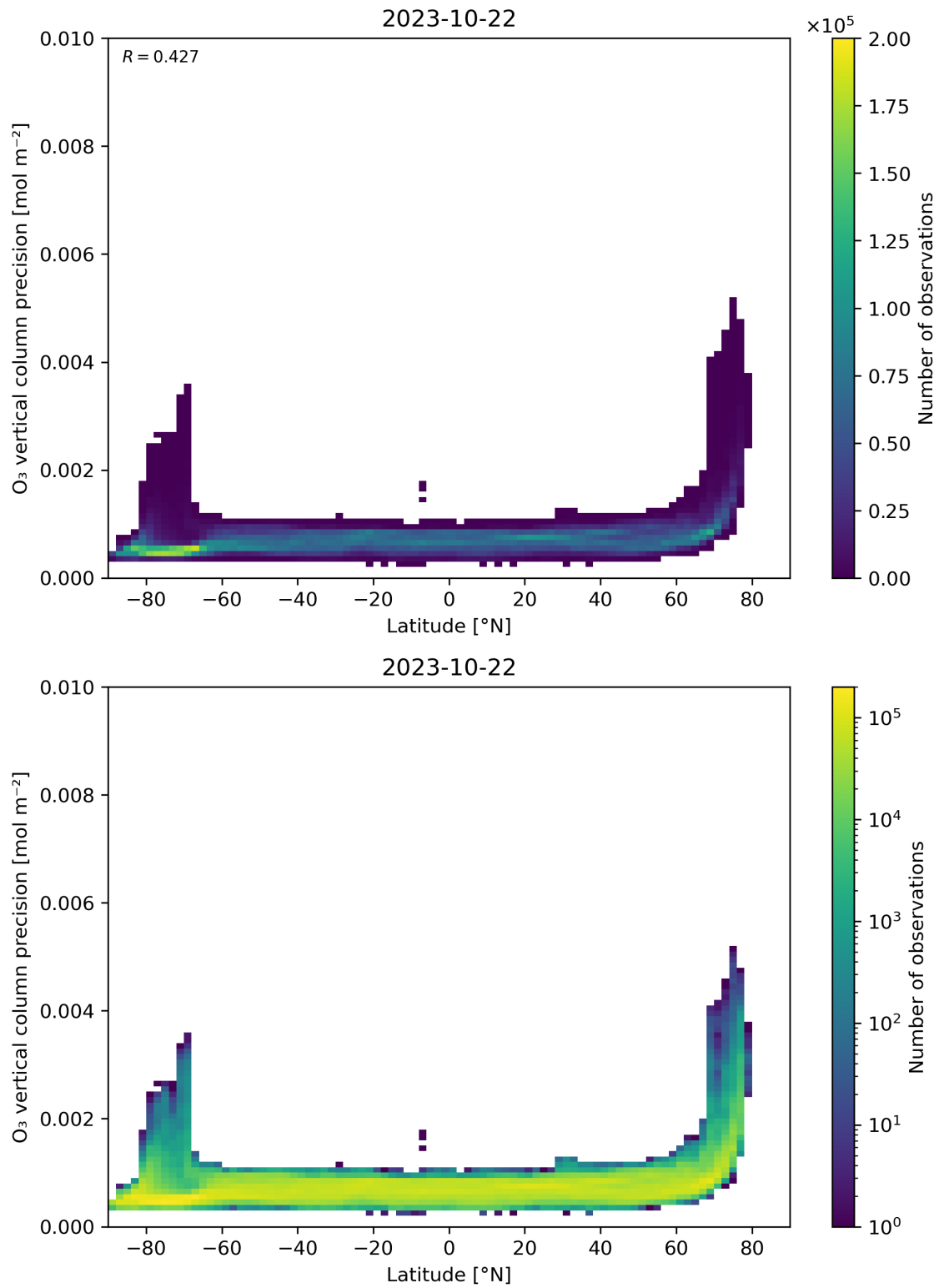
Figure 37: Scatter density plot of “Latitude” against “O 3 vertical column precision” for 2023-10-22 to 2023-10-23.
