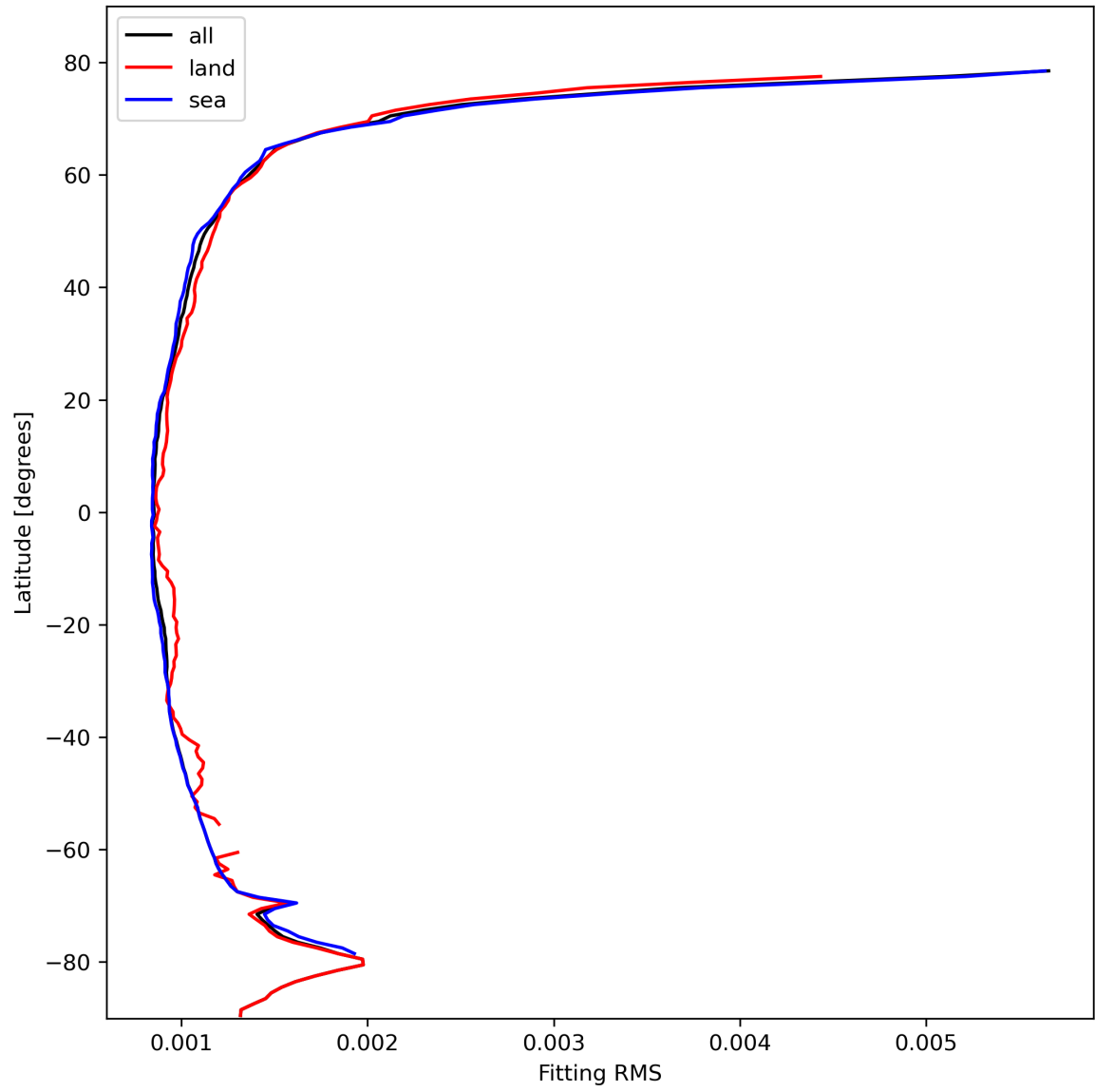
Figure 16: Zonal average of “Fitting RMS” for 2023-10-22 to 2023-10-23.
