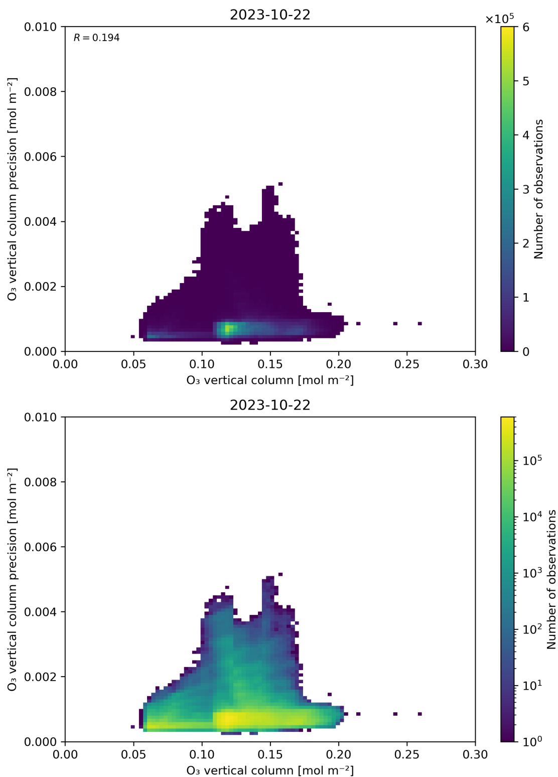
Figure 41: Scatter density plot of “O 3 vertical column” against “O 3 vertical column precision” for 2023-10-22 to 2023-10-23.
