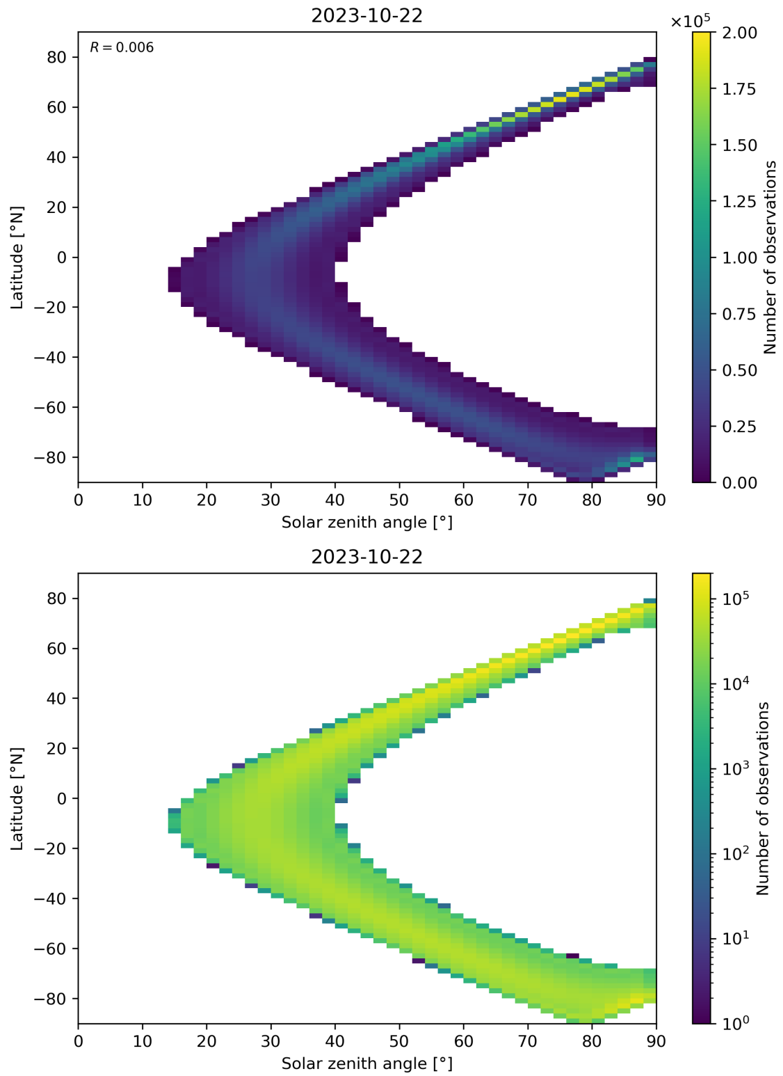
Figure 44: Scatter density plot of “Solar zenith angle” against “Latitude” for 2023-10-22 to 2023-10-23.
