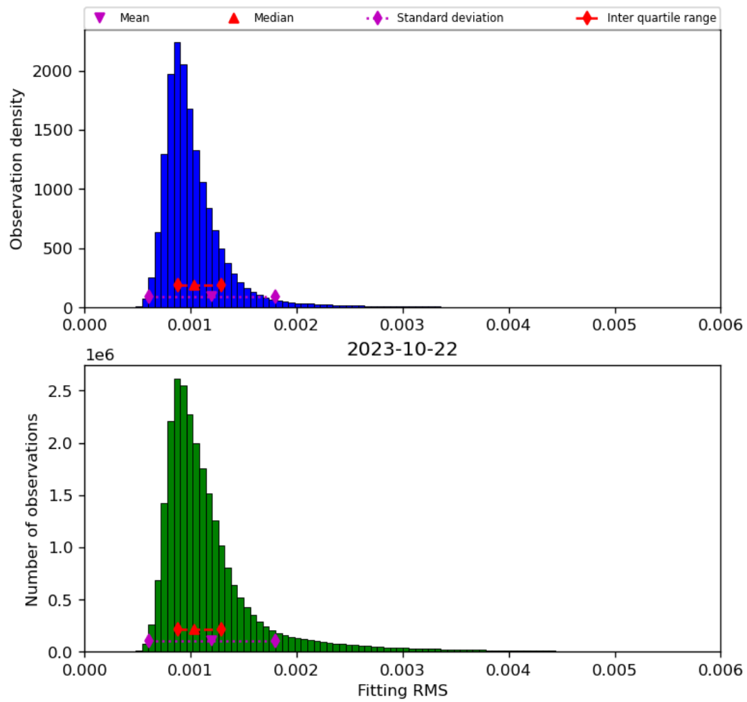
Figure 23: Histogram of “Fitting RMS” for 2023-10-22 to 2023-10-23
