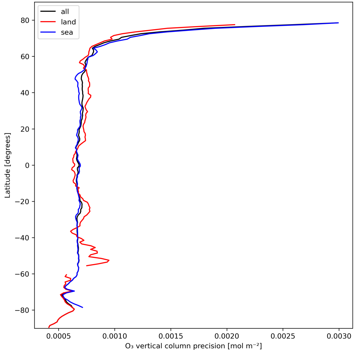
Figure 15: Zonal average of “O 3 vertical column precision” for 2023-10-22 to 2023-10-23.
