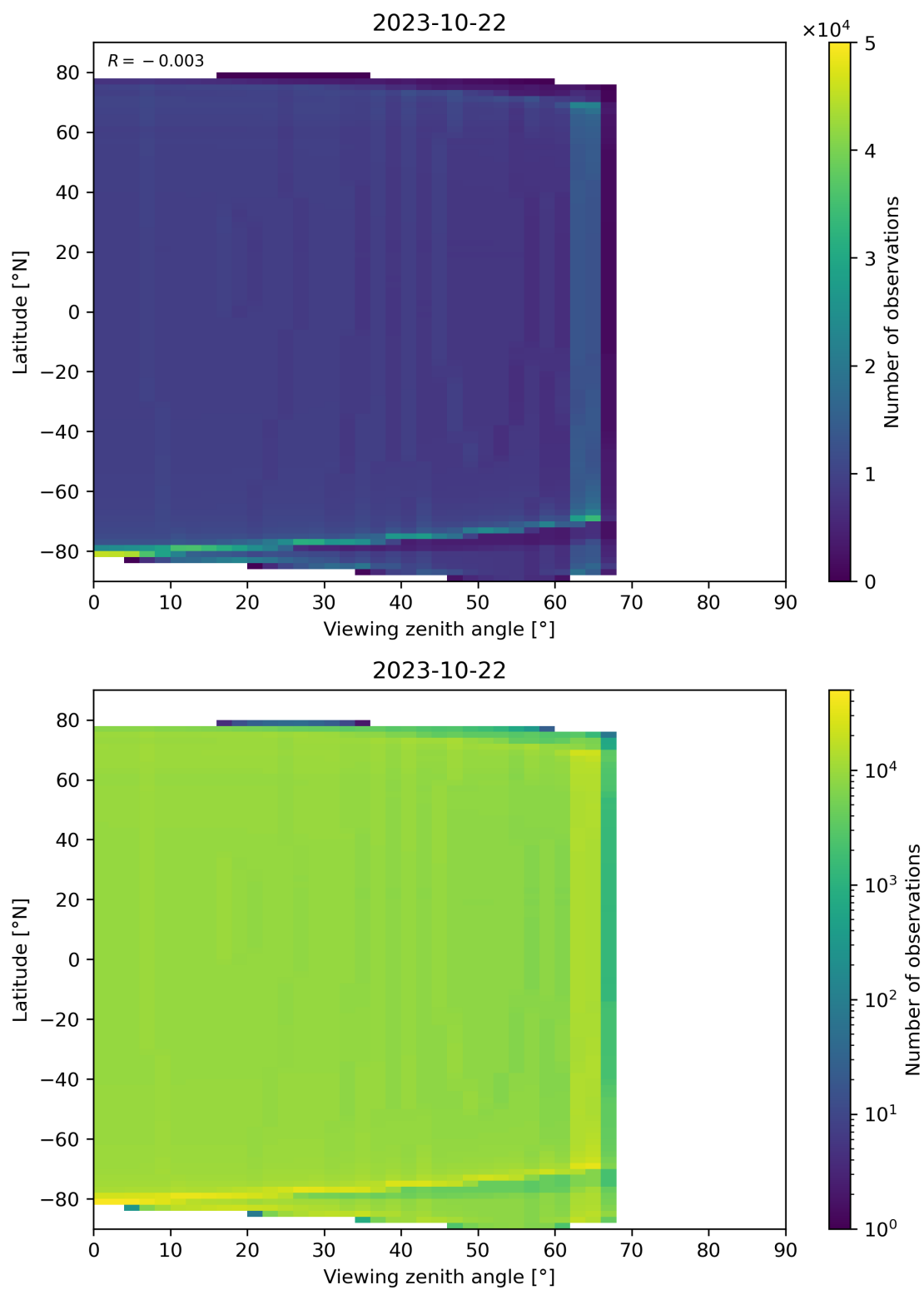
Figure 49: Scatter density plot of “Viewing zenith angle” against “Latitude” for 2023-10-22 to 2023-10-23.
