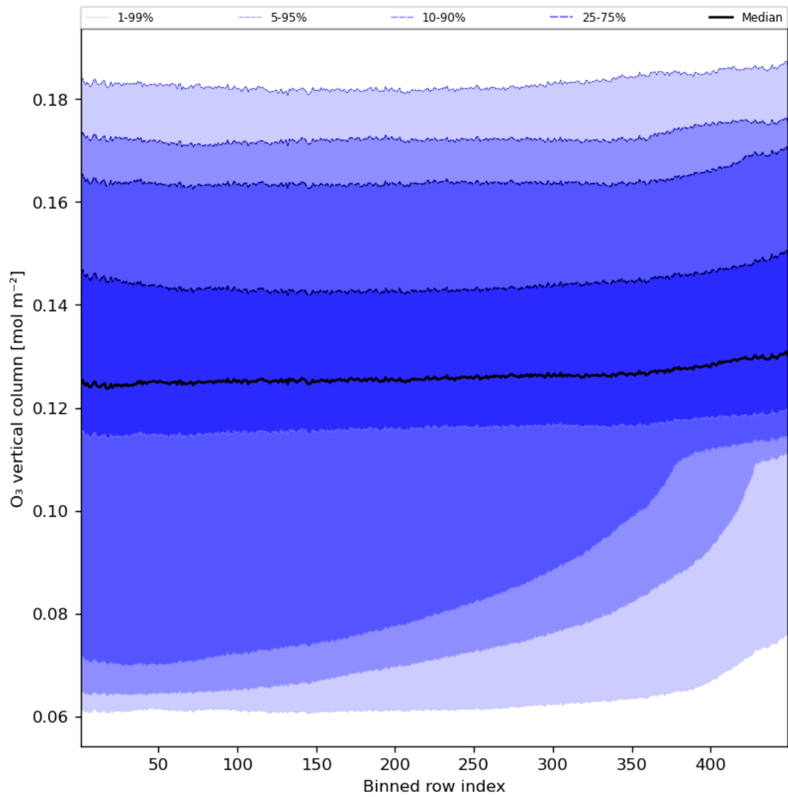
Figure 28: Along track statistics of “O 3 vertical column” for 2023-10-22 to 2023-10-23
