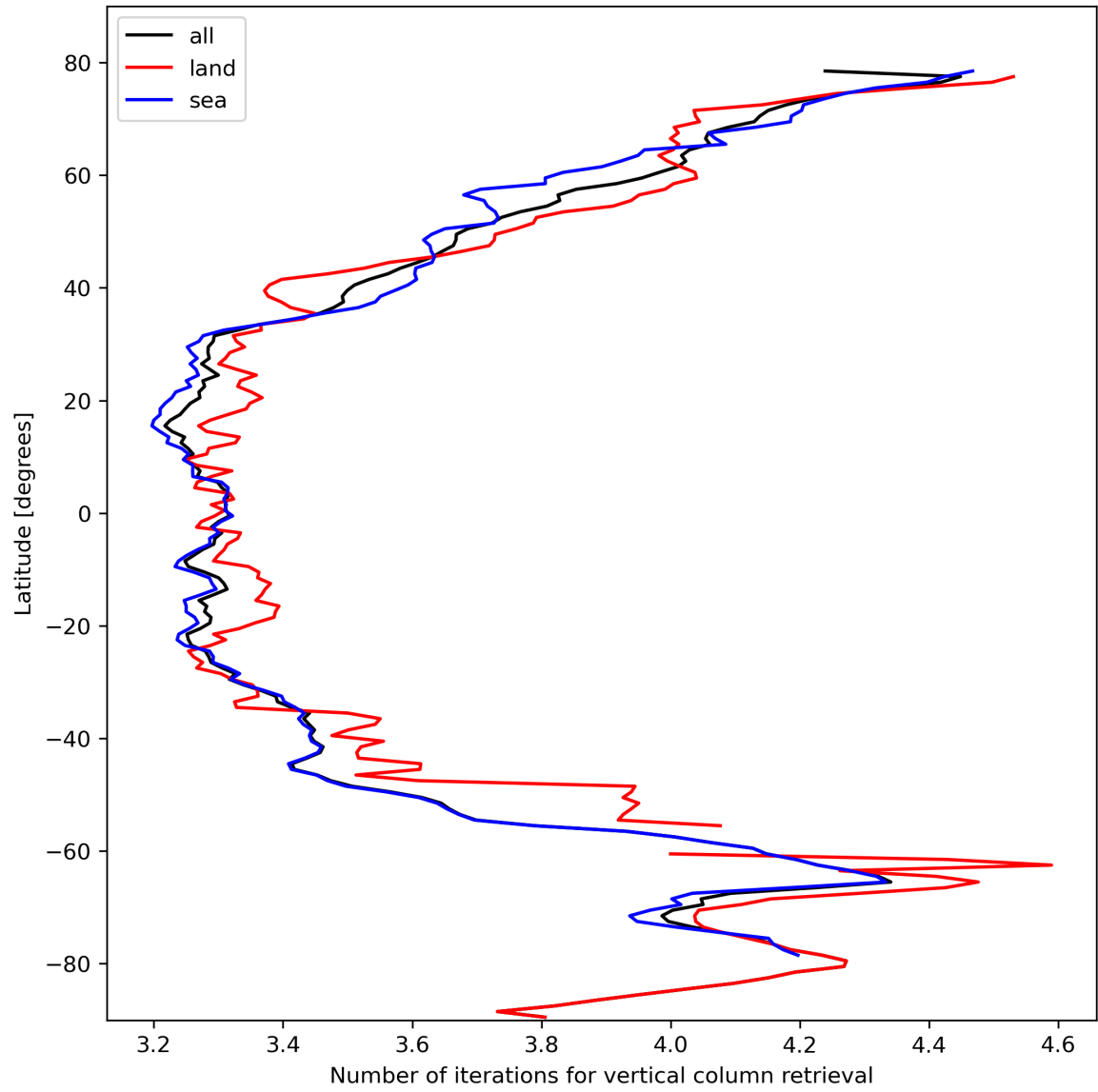
Figure 19: Zonal average of “Number of iterations for vertical column retrieval” for 2023-10-22 to 2023-10-23.
