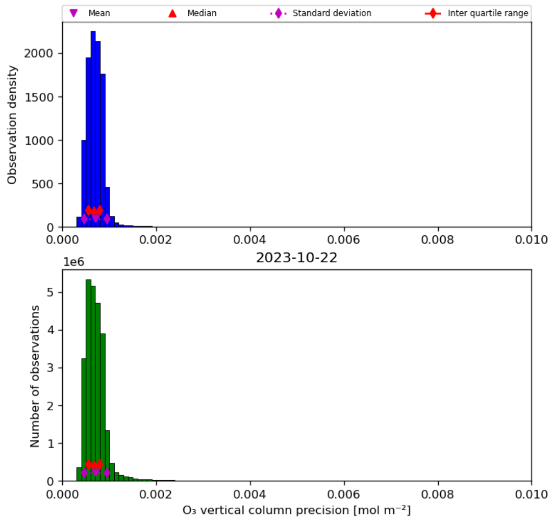
Figure 22: Histogram of “O 3 vertical column precision” for 2023-10-22 to 2023-10-23
