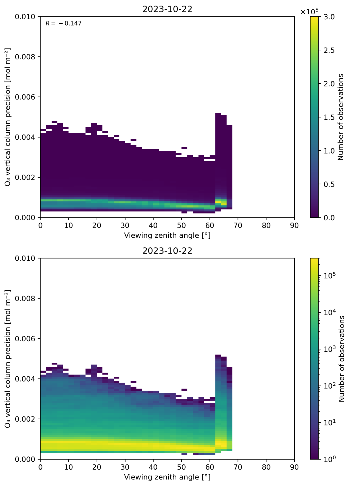
Figure 53: Scatter density plot of “Viewing zenith angle” against “O 3 vertical column precision” for 2023-10-22 to 2023-10-23.
