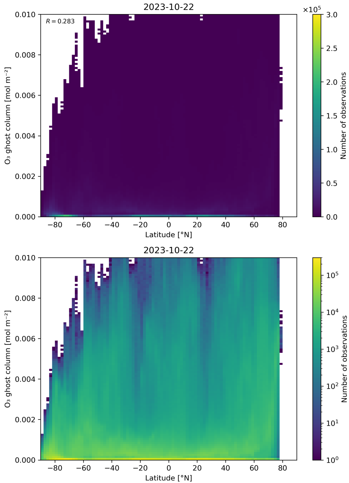
Figure 35: Scatter density plot of “Latitude” against “O 3 ghost column” for 2023-10-22 to 2023-10-23.
