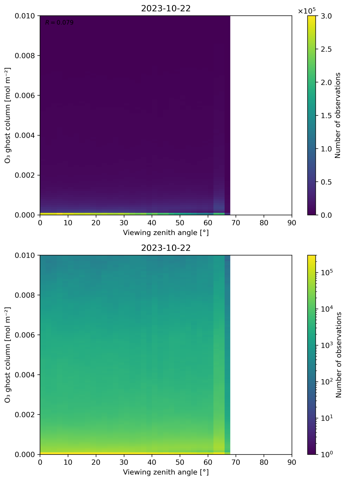
Figure 51: Scatter density plot of “Viewing zenith angle” against “O 3 ghost column” for 2023-10-22 to 2023-10-23.
