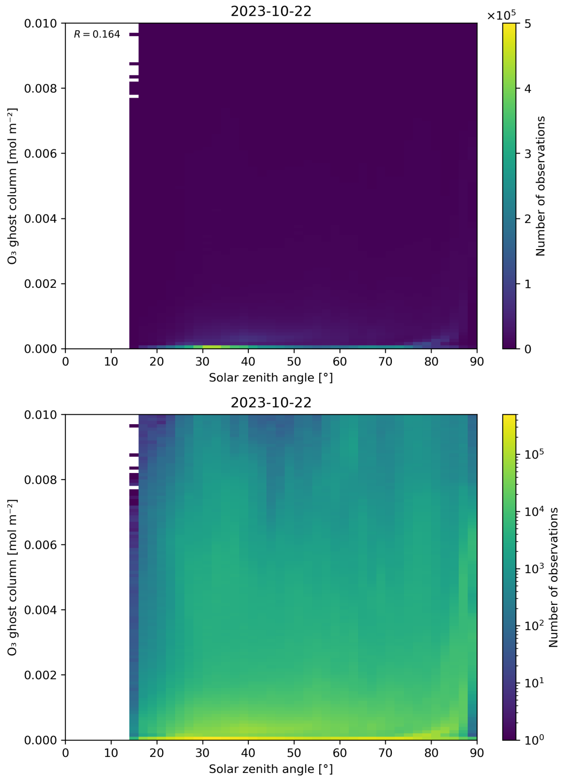
Figure 46: Scatter density plot of “Solar zenith angle” against “O 3 ghost column” for 2023-10-22 to 2023-10-23.
