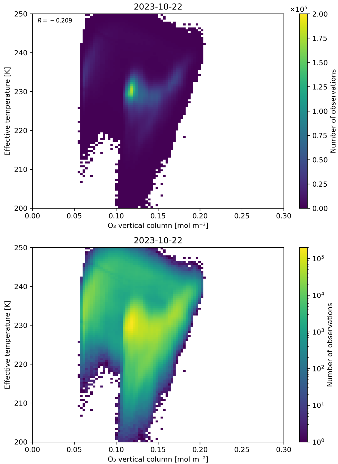
Figure 39: Scatter density plot of “O 3 vertical column” against “Effective temperature” for 2023-10-22 to 2023-10-23.
