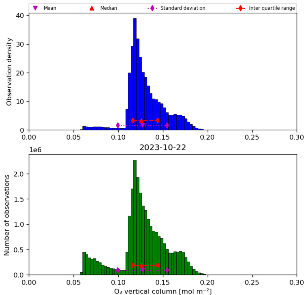
Figure 21: Histogram of “O 3 vertical column” for 2023-10-22 to 2023-10-23
