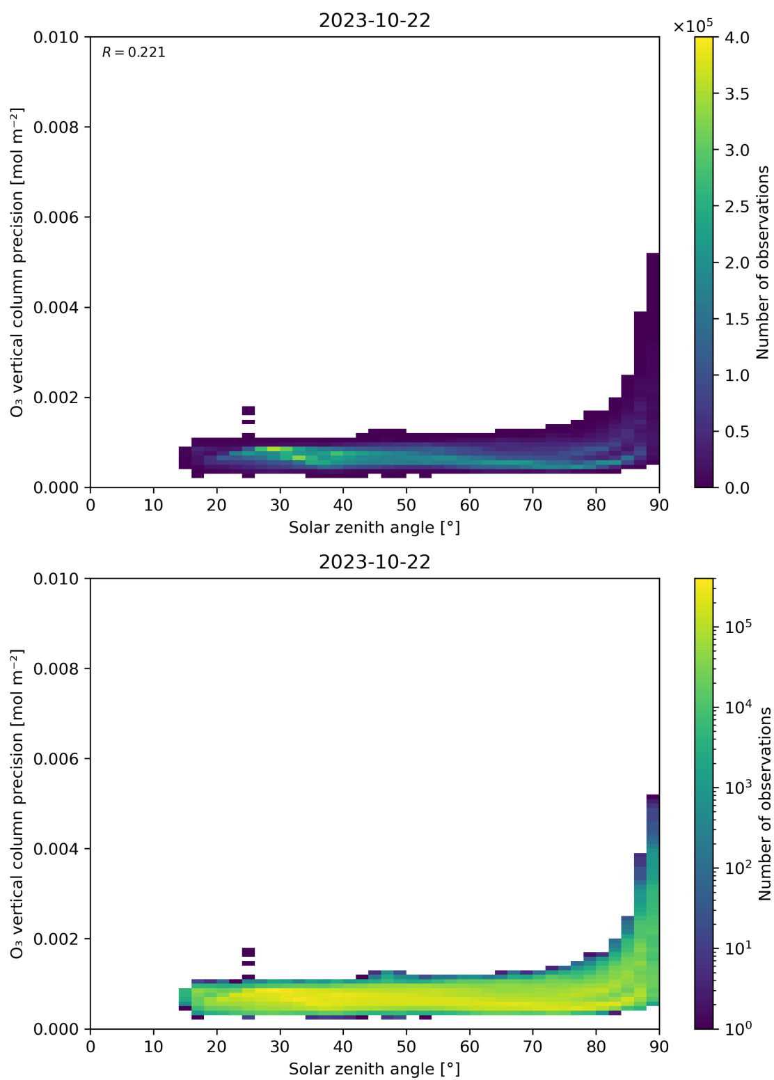
Figure 48: Scatter density plot of “Solar zenith angle” against “O 3 vertical column precision” for 2023-10-22 to 2023-10-23.
