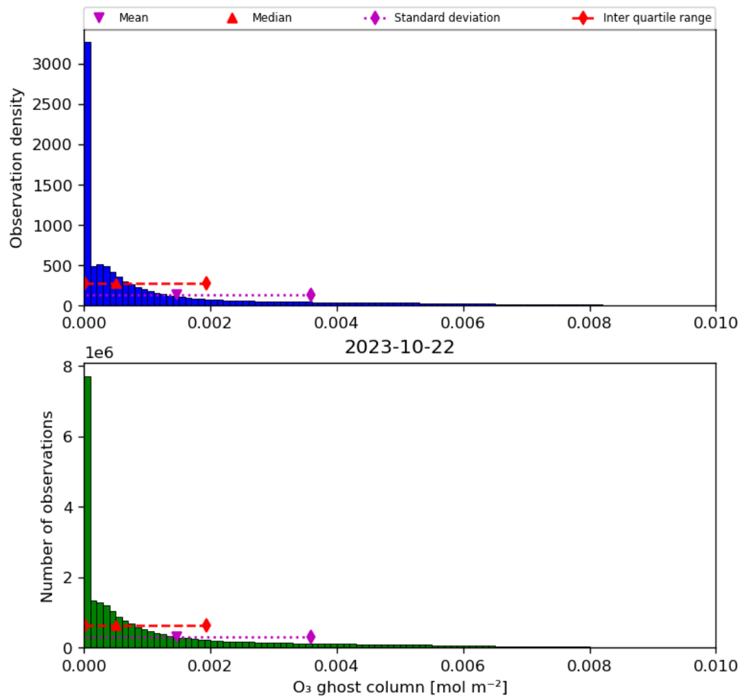
Figure 25: Histogram of “O 3 ghost column” for 2023-10-22 to 2023-10-23
