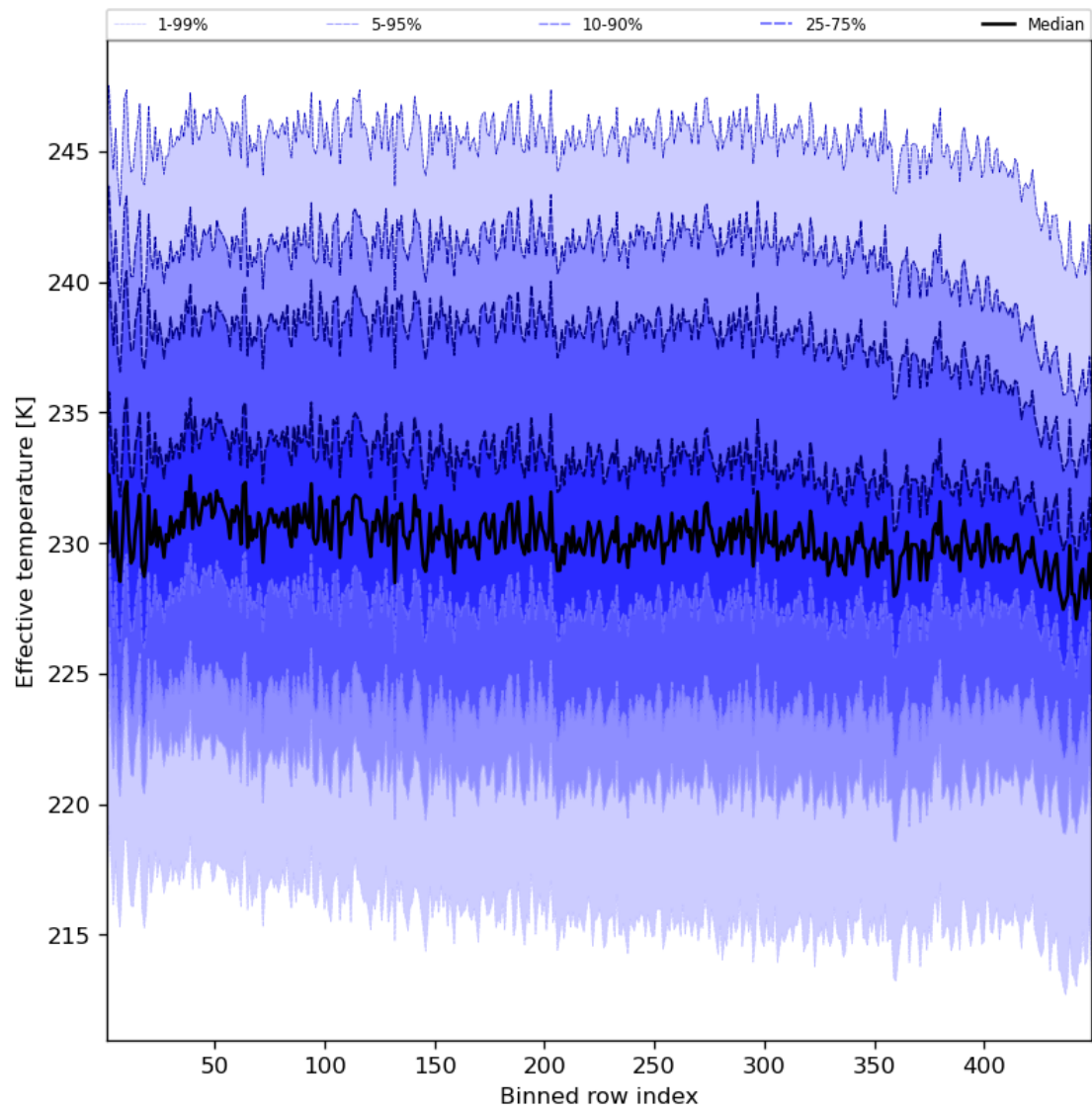
Figure 31: Along track statistics of “Effective temperature” for 2023-10-22 to 2023-10-23
