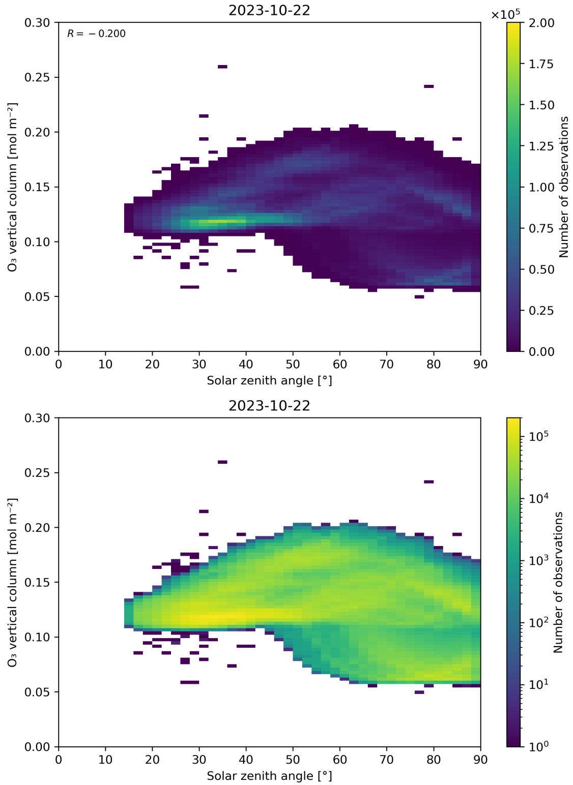
Figure 47: Scatter density plot of “Solar zenith angle” against “O 3 vertical column” for 2023-10-22 to 2023-10-23.
