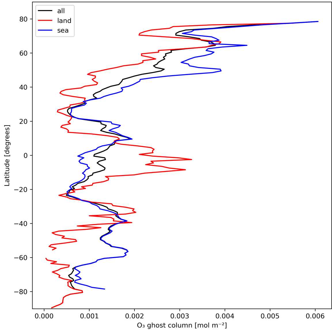
Figure 18: Zonal average of "O 3 ghost column" for 2023-10-22 to 2023-10-23.
