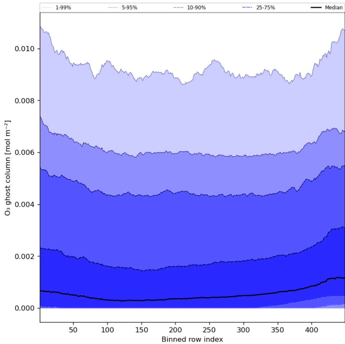
Figure 32: Along track statistics of “O 3 ghost column” for 2023-10-22 to 2023-10-23
