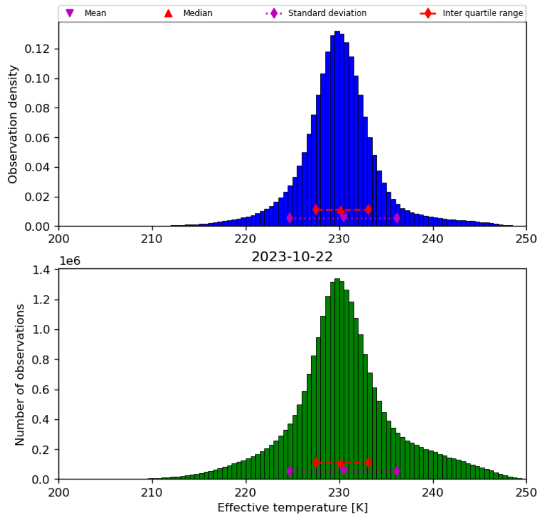
Figure 24: Histogram of “Effective temperature” for 2023-10-22 to 2023-10-23
