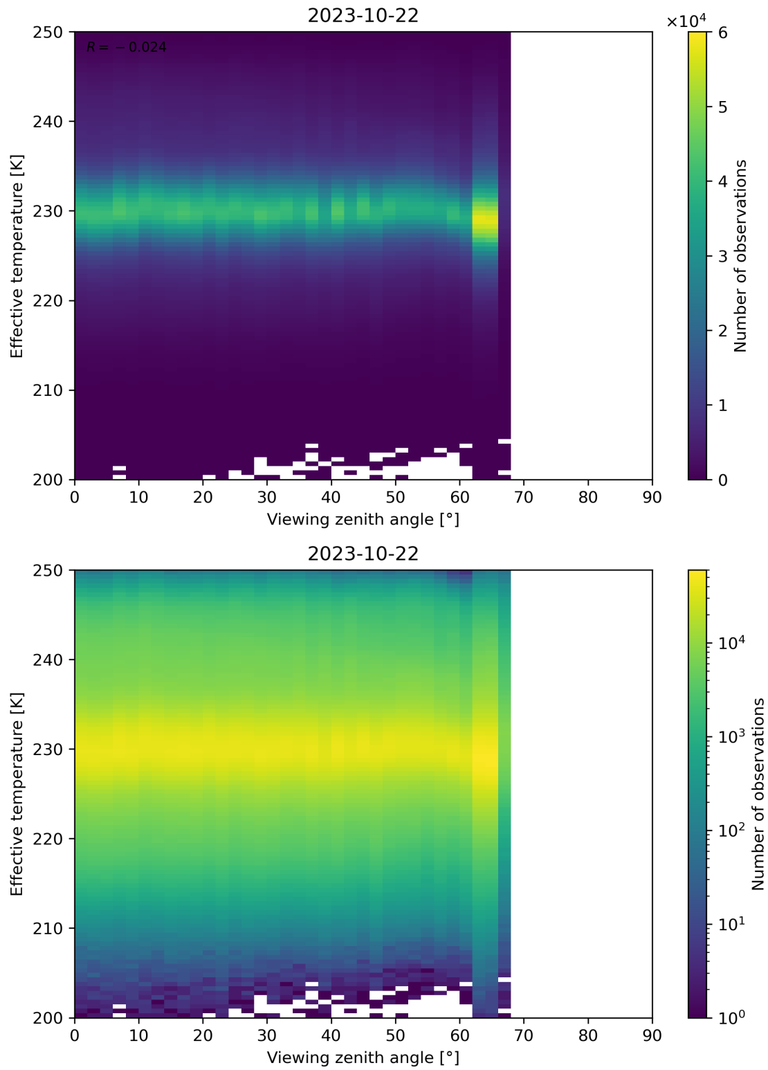
Figure 50: Scatter density plot of “Viewing zenith angle” against “Effective temperature” for 2023-10-22 to 2023-10-23.
