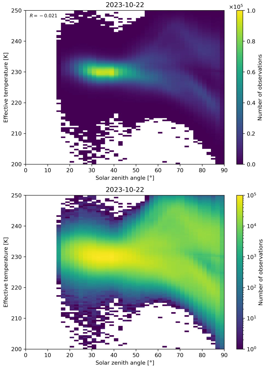
Figure 45: Scatter density plot of “Solar zenith angle” against “Effective temperature” for 2023-10-22 to 2023-10-23.
