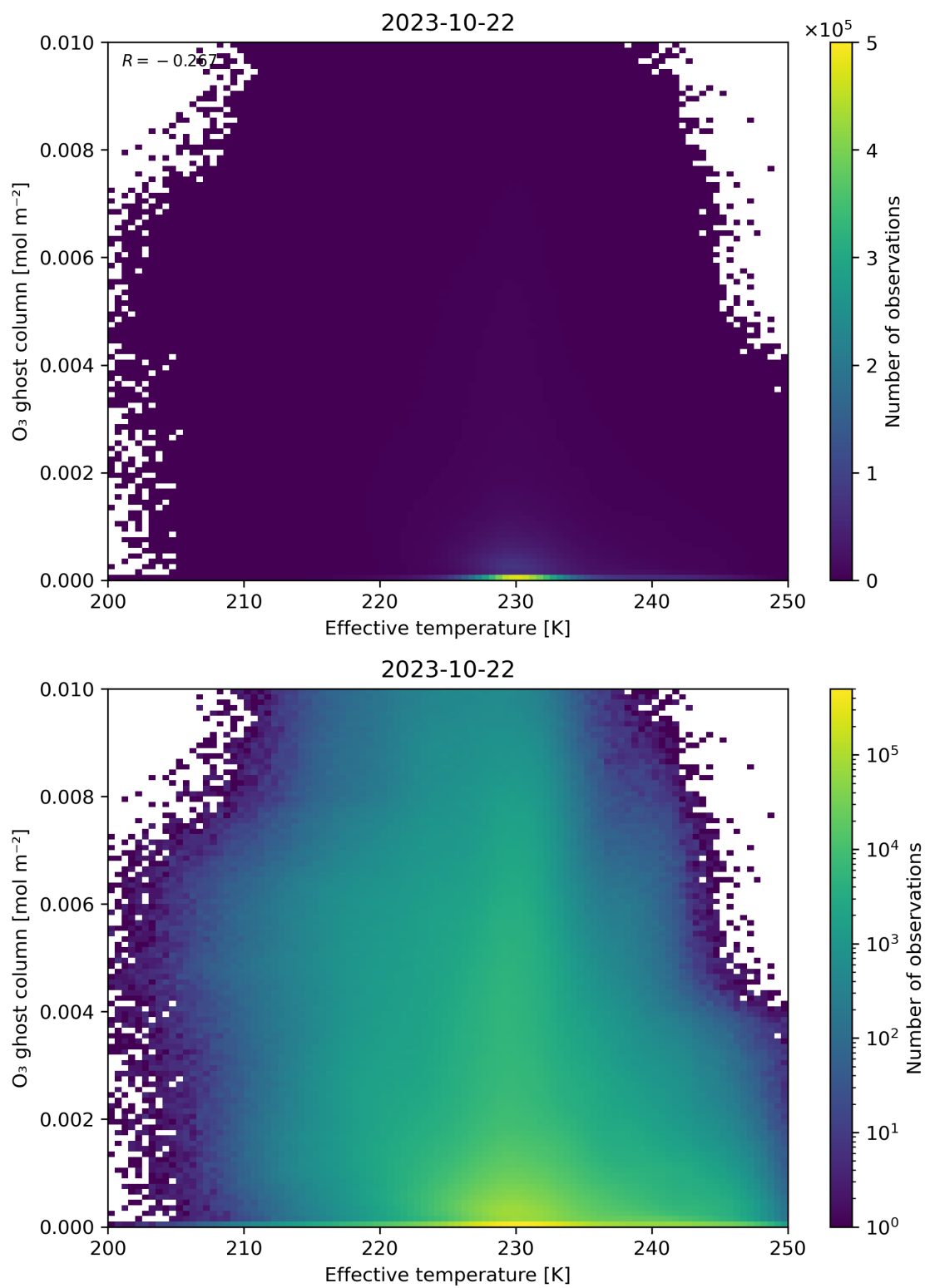
Figure 38: Scatter density plot of “Effective temperature” against “O 3 ghost column” for 2023-10-22 to 2023-10-23.
