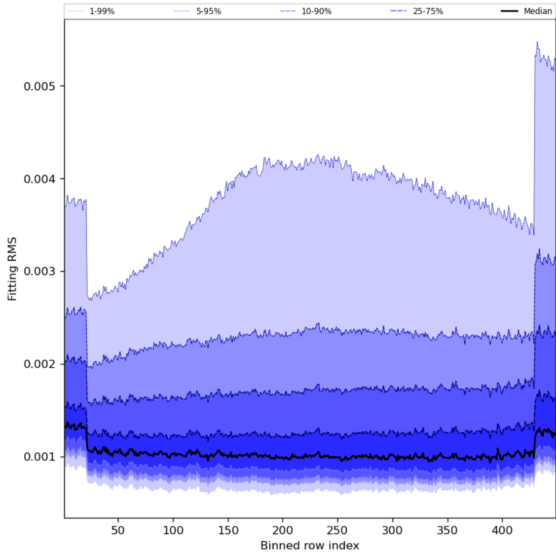
Figure 30: Along track statistics of “Fitting RMS” for 2023-10-22 to 2023-10-23
