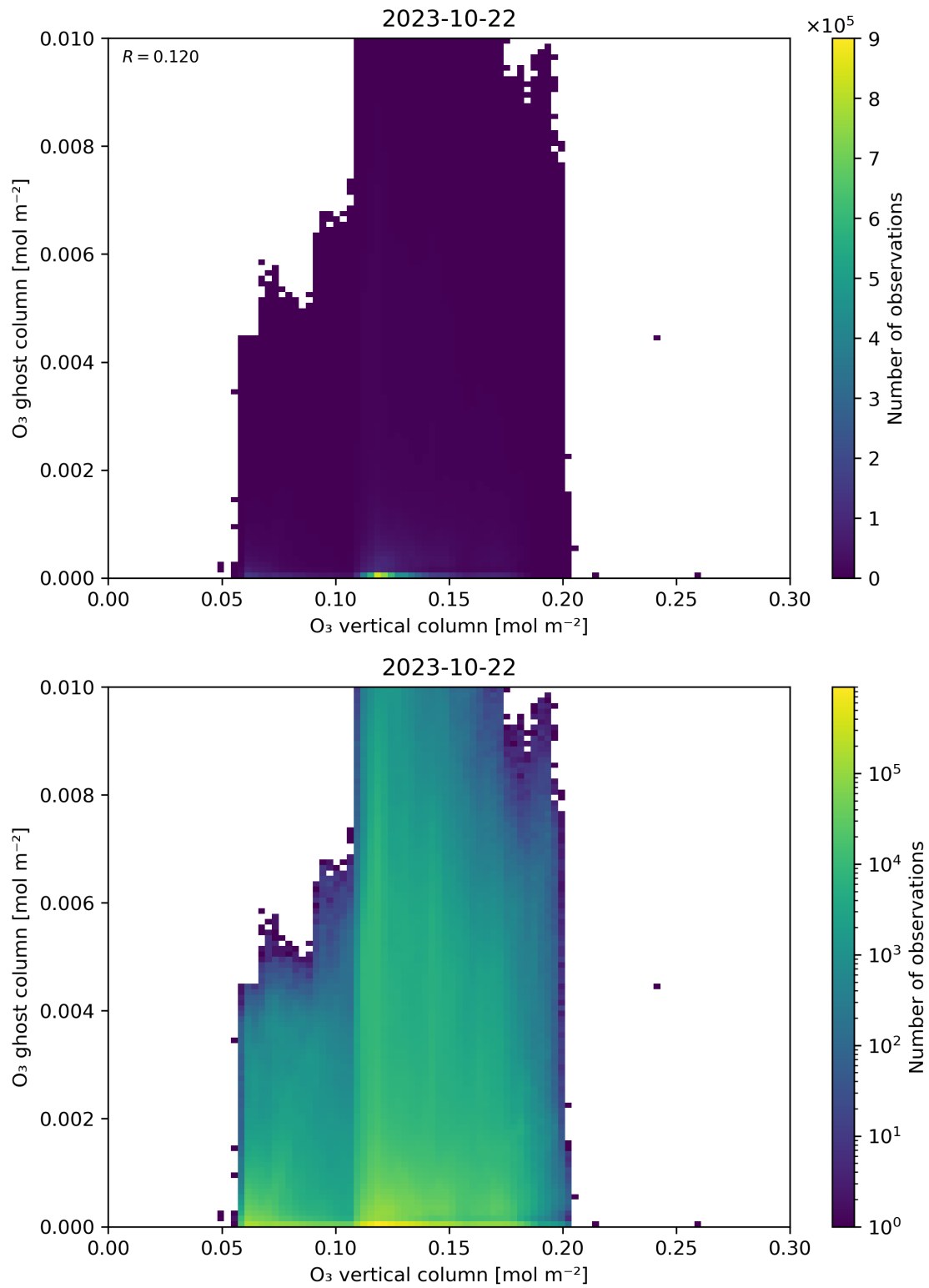
Figure 40: Scatter density plot of “O 3 vertical column” against “O 3 ghost column” for 2023-10-22 to 2023-10-23.
