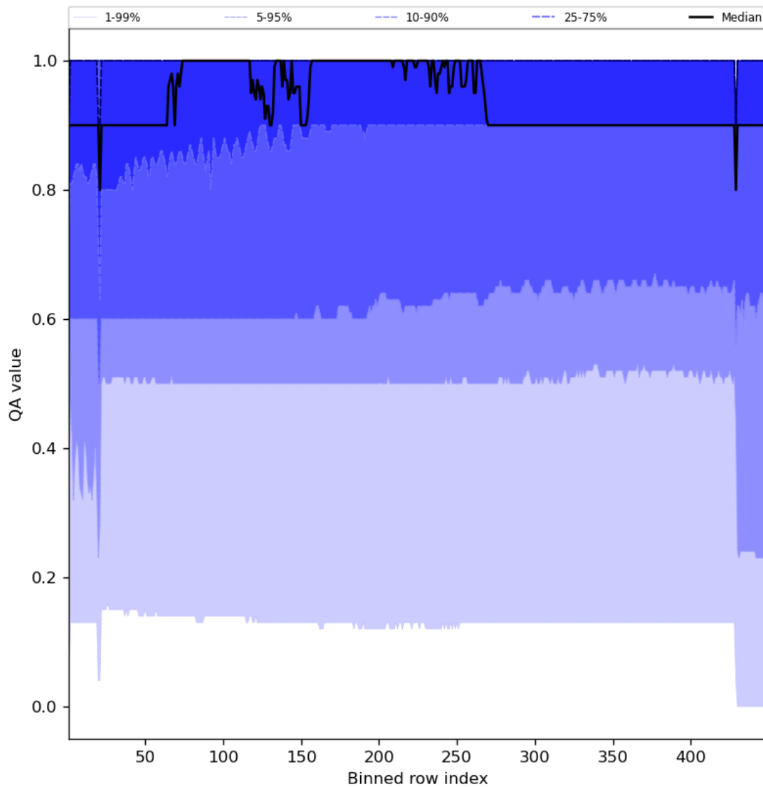
Figure 27: Along track statistics of “QA value” for 2023-10-22 to 2023-10-23
