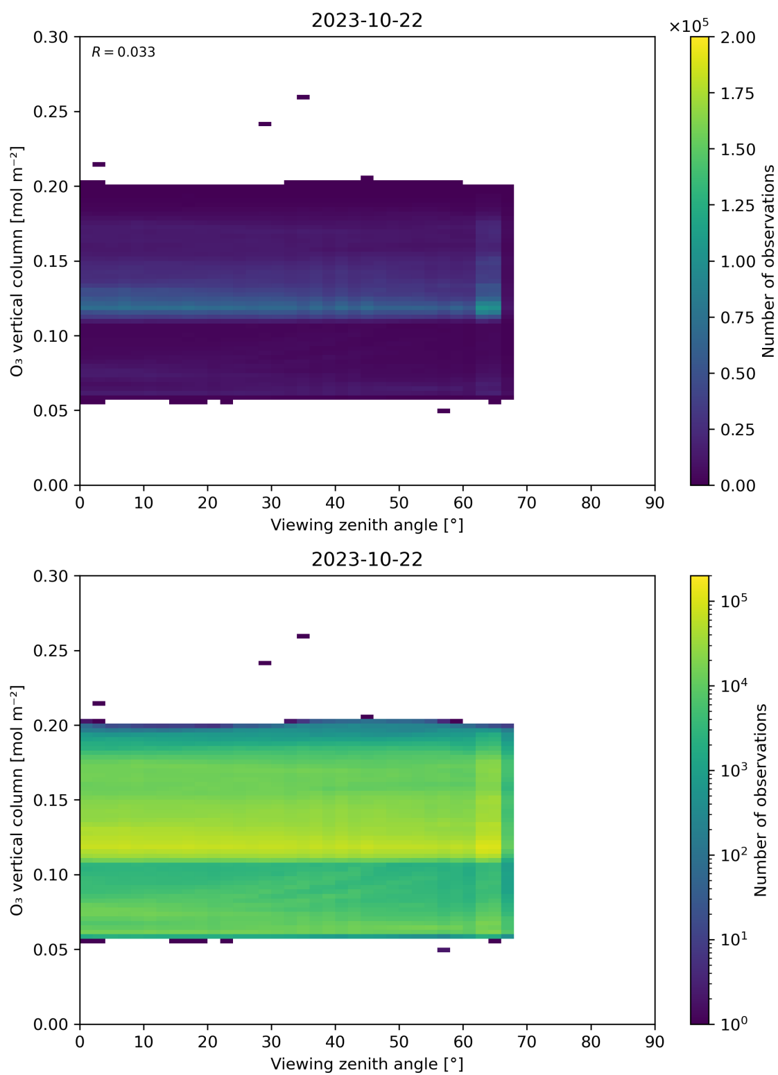
Figure 52: Scatter density plot of “Viewing zenith angle” against “O 3 vertical column” for 2023-10-22 to 2023-10-23.
