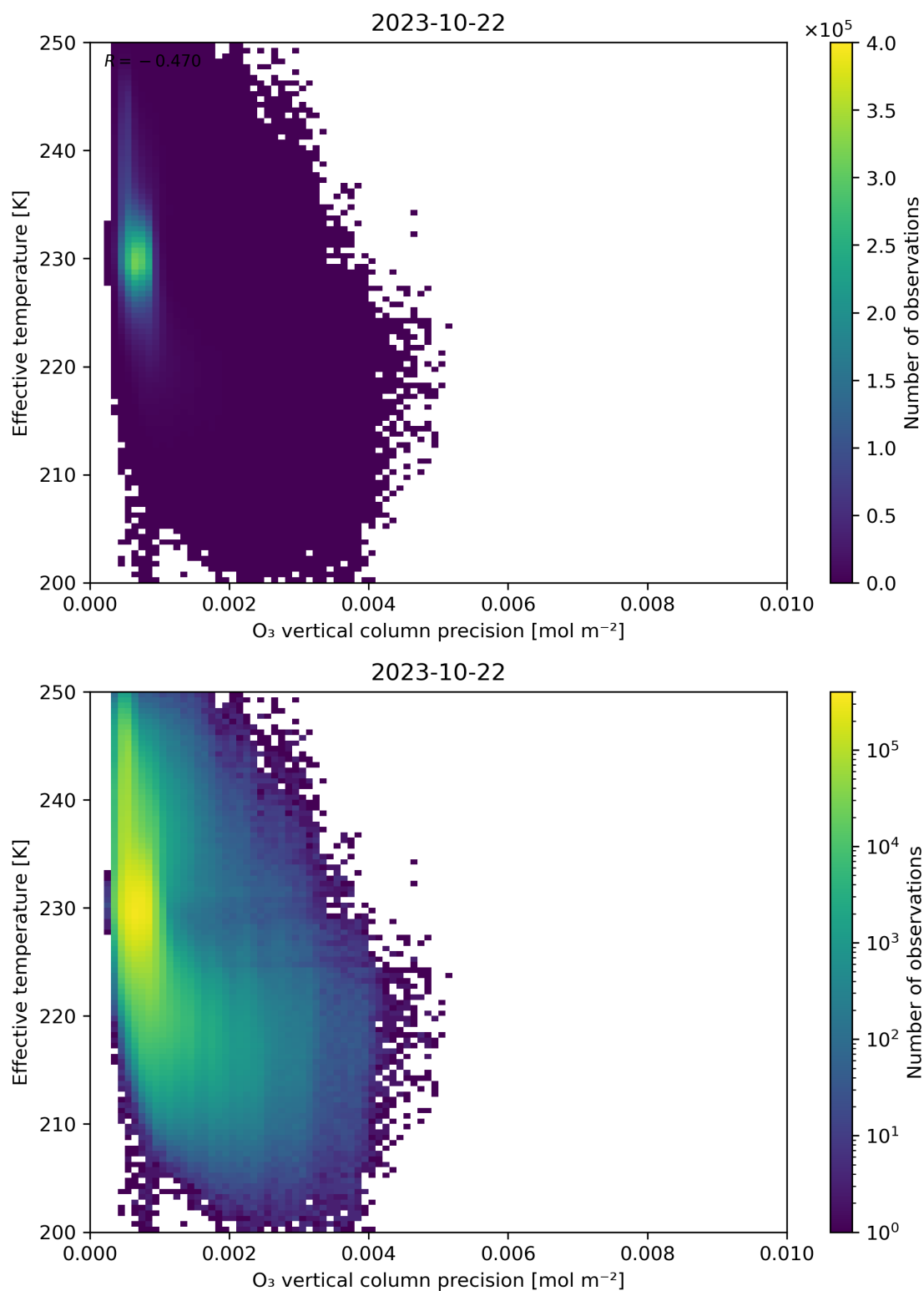
Figure 42: Scatter density plot of “O 3 vertical column precision” against “Effective temperature” for 2023-10-22 to 2023-10-23.
