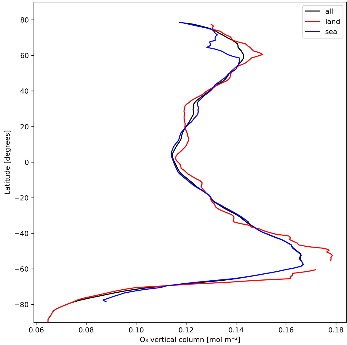
Figure 14: Zonal average of “O 3 vertical column” for 2023-10-22 to 2023-10-23.
