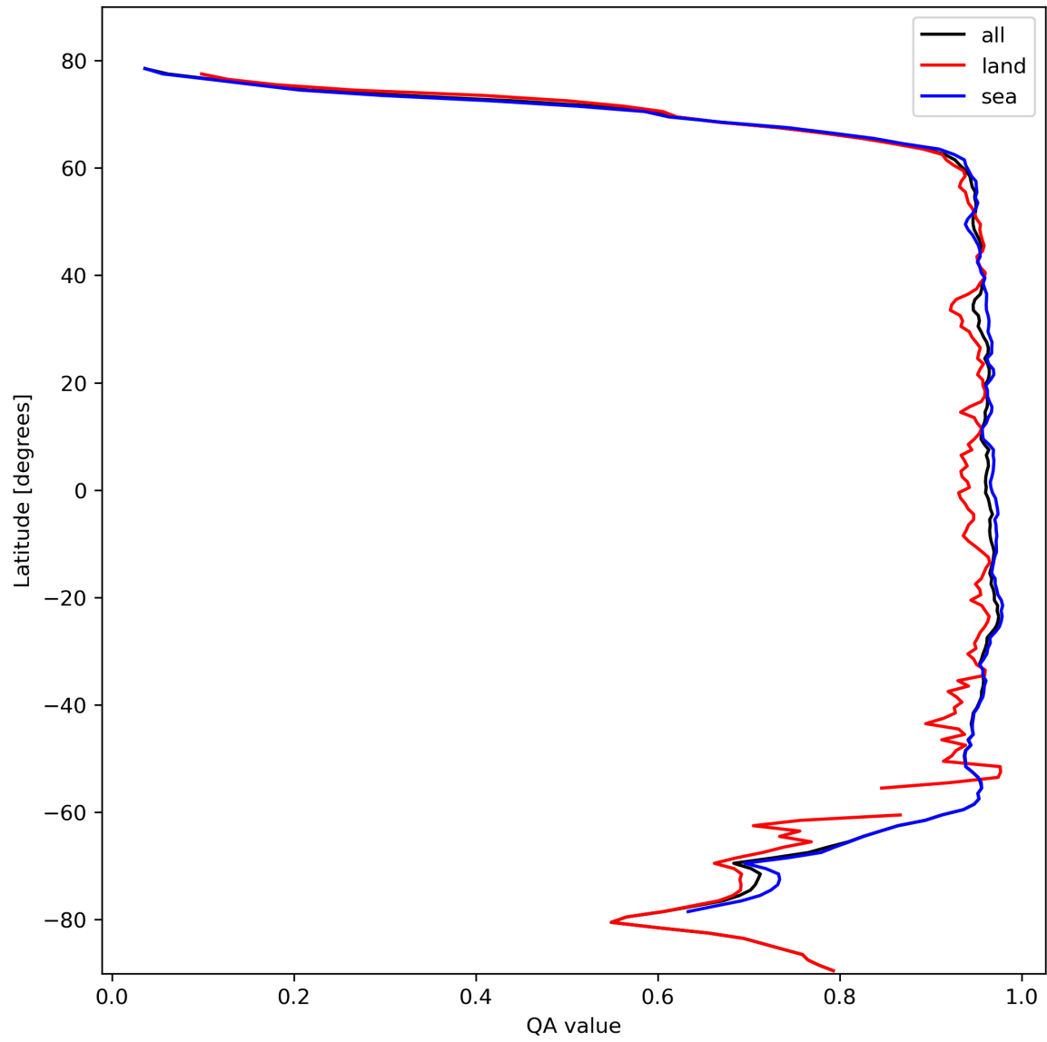
Figure 13: Zonal average of “QA value” for 2023-10-22 to 2023-10-23.
