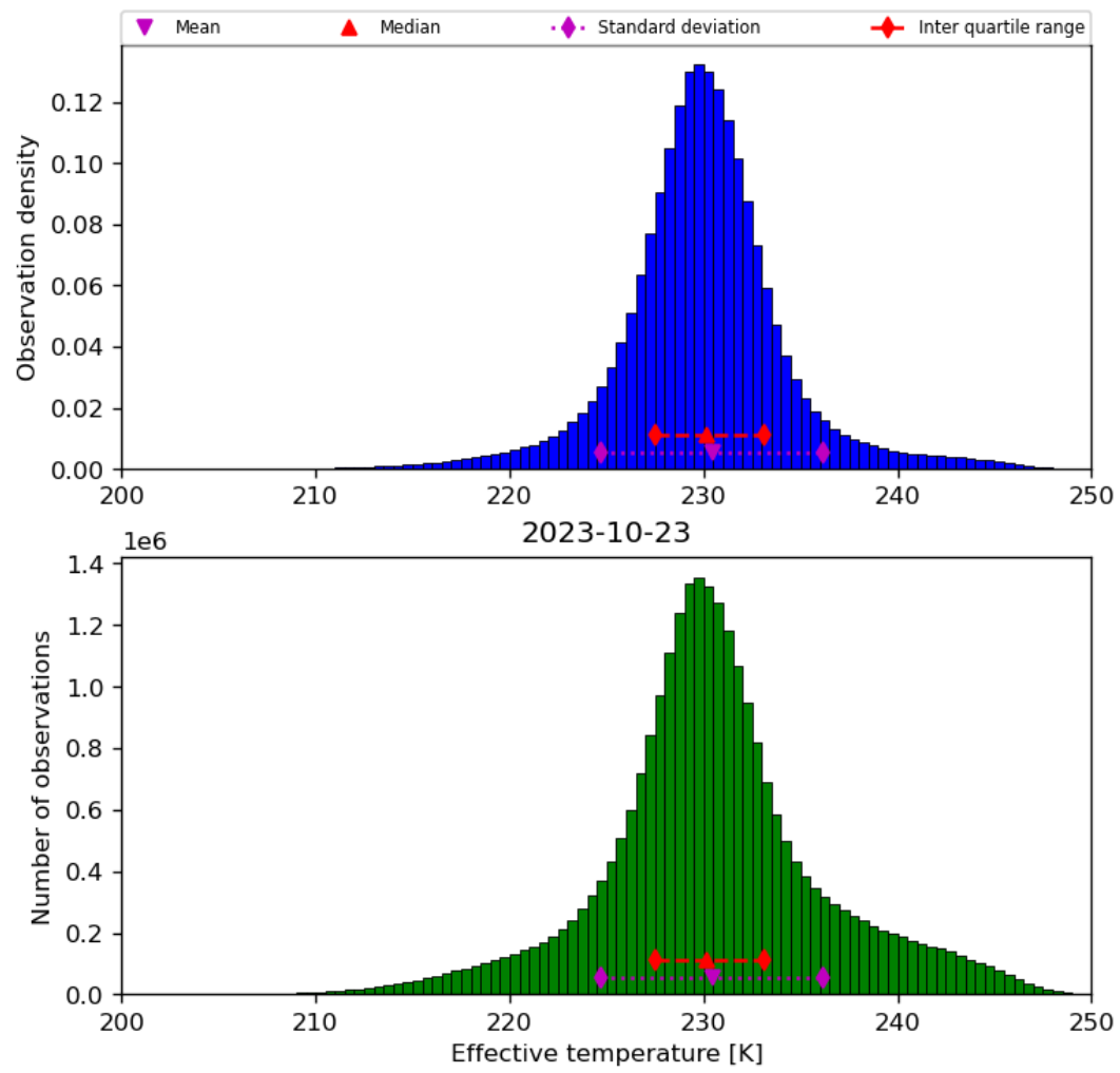
Figure 24: Histogram of “Effective temperature” for 2023-10-22 to 2023-10-24
