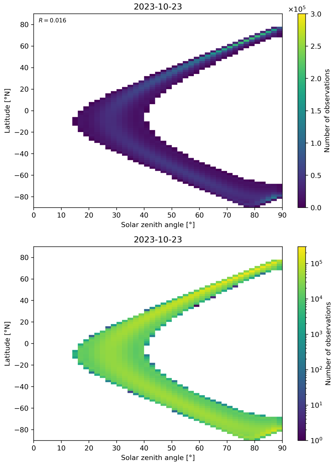
Figure 44: Scatter density plot of “Solar zenith angle” against “Latitude” for 2023-10-22 to 2023-10-24.
