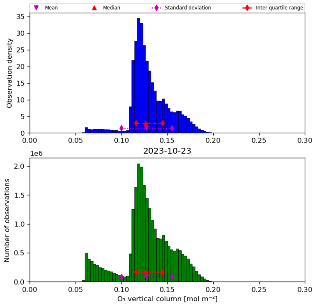
Figure 21: Histogram of “O 3 vertical column” for 2023-10-22 to 2023-10-24
