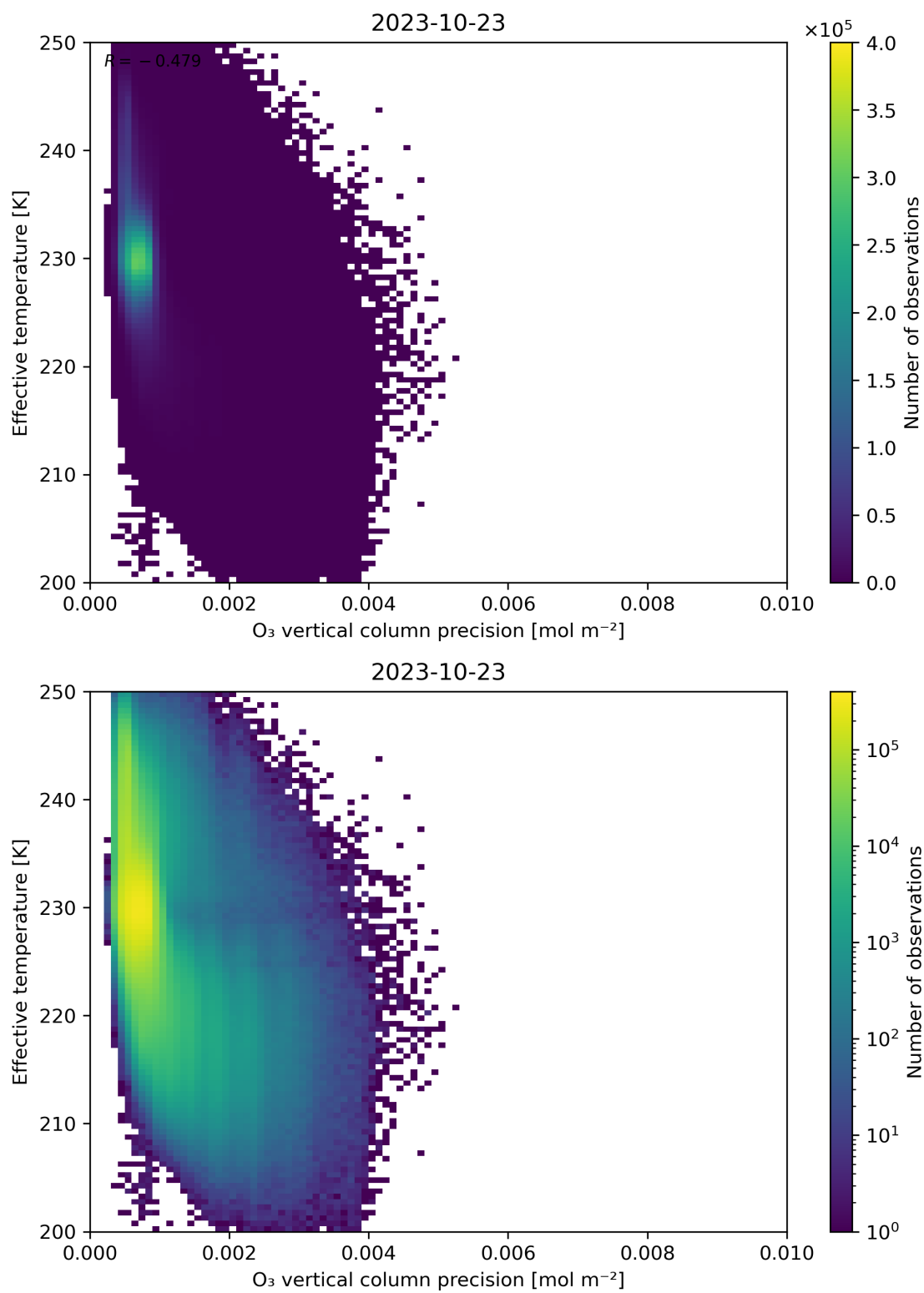
Figure 42: Scatter density plot of “O 3 vertical column precision” against “Effective temperature” for 2023-10-22 to 2023-10-24.
