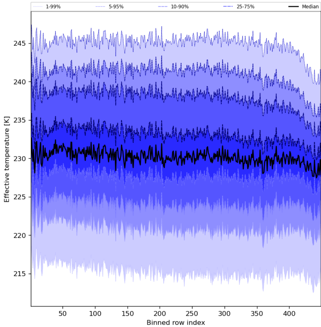
Figure 31: Along track statistics of “Effective temperature” for 2023-10-22 to 2023-10-24
