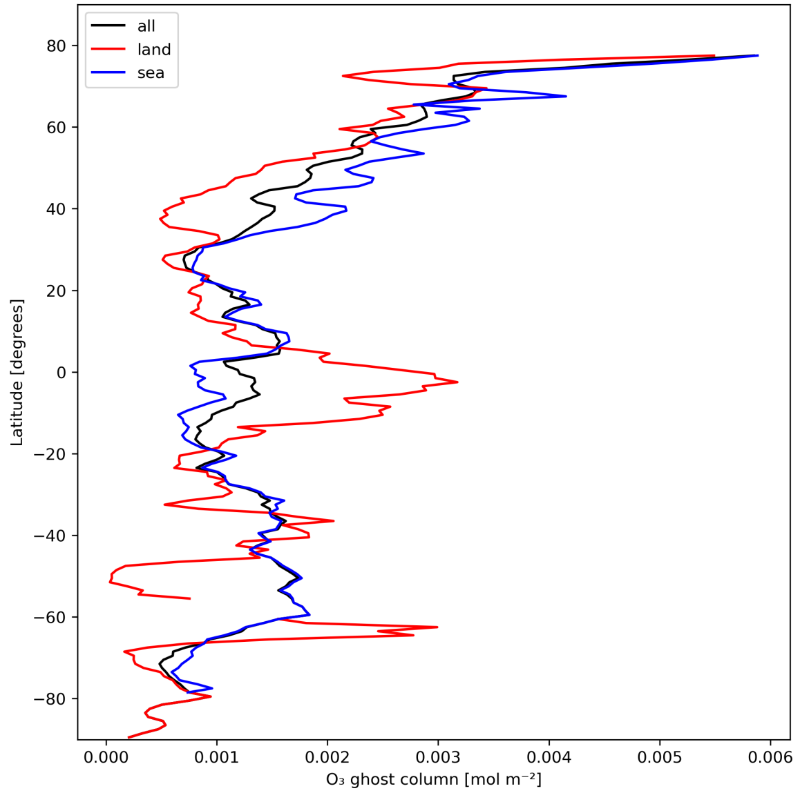
Figure 18: Zonal average of “O 3 ghost column” for 2023-10-22 to 2023-10-24.
