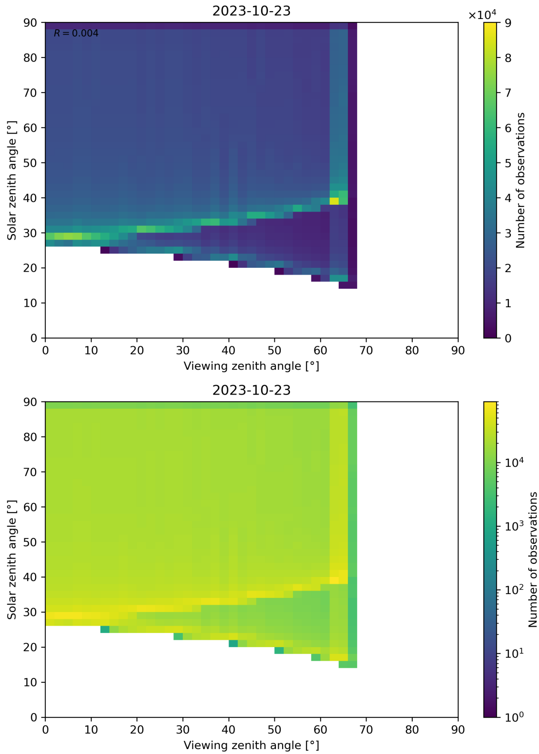
Figure 54: Scatter density plot of “Viewing zenith angle” against “Solar zenith angle” for 2023-10-22 to 2023-10-24.
