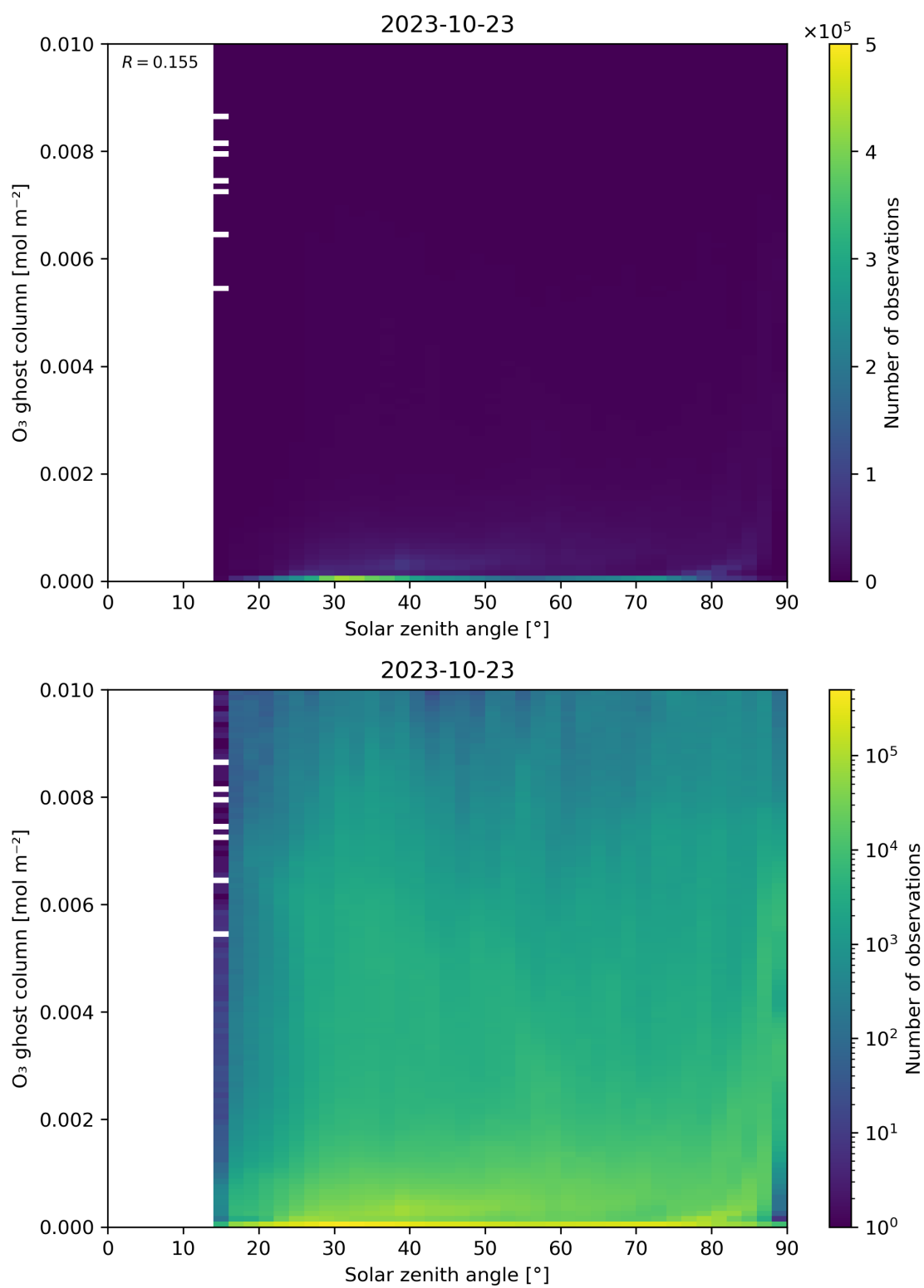
Figure 46: Scatter density plot of “Solar zenith angle” against “O 3 ghost column” for 2023-10-22 to 2023-10-24.
