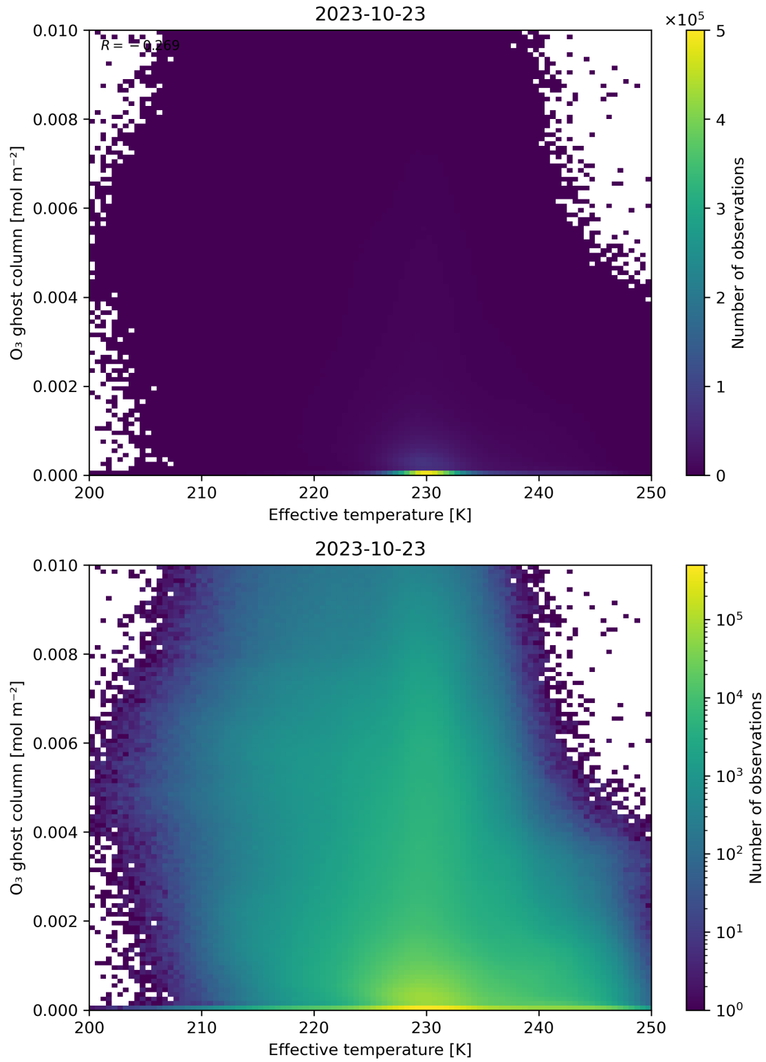
Figure 38: Scatter density plot of “Effective temperature” against “O 3 ghost column” for 2023-10-22 to 2023-10-24.
