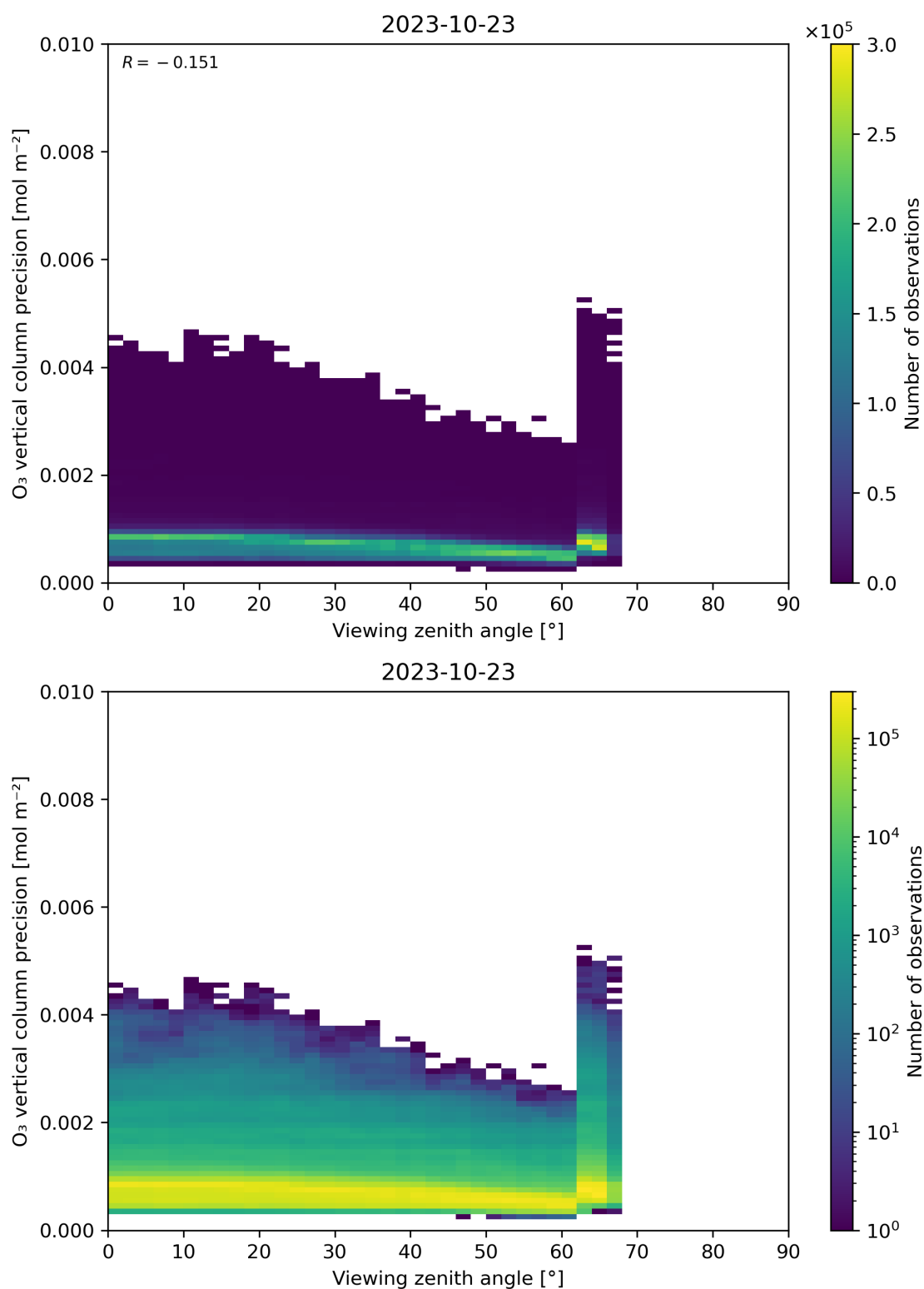
Figure 53: Scatter density plot of “Viewing zenith angle” against “O 3 vertical column precision” for 2023-10-22 to 2023-10-24.
