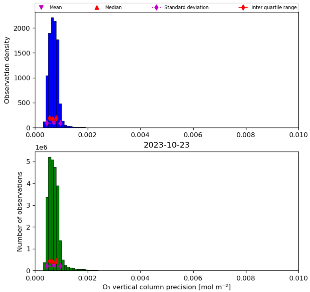
Figure 22: Histogram of “O 3 vertical column precision” for 2023-10-22 to 2023-10-24
