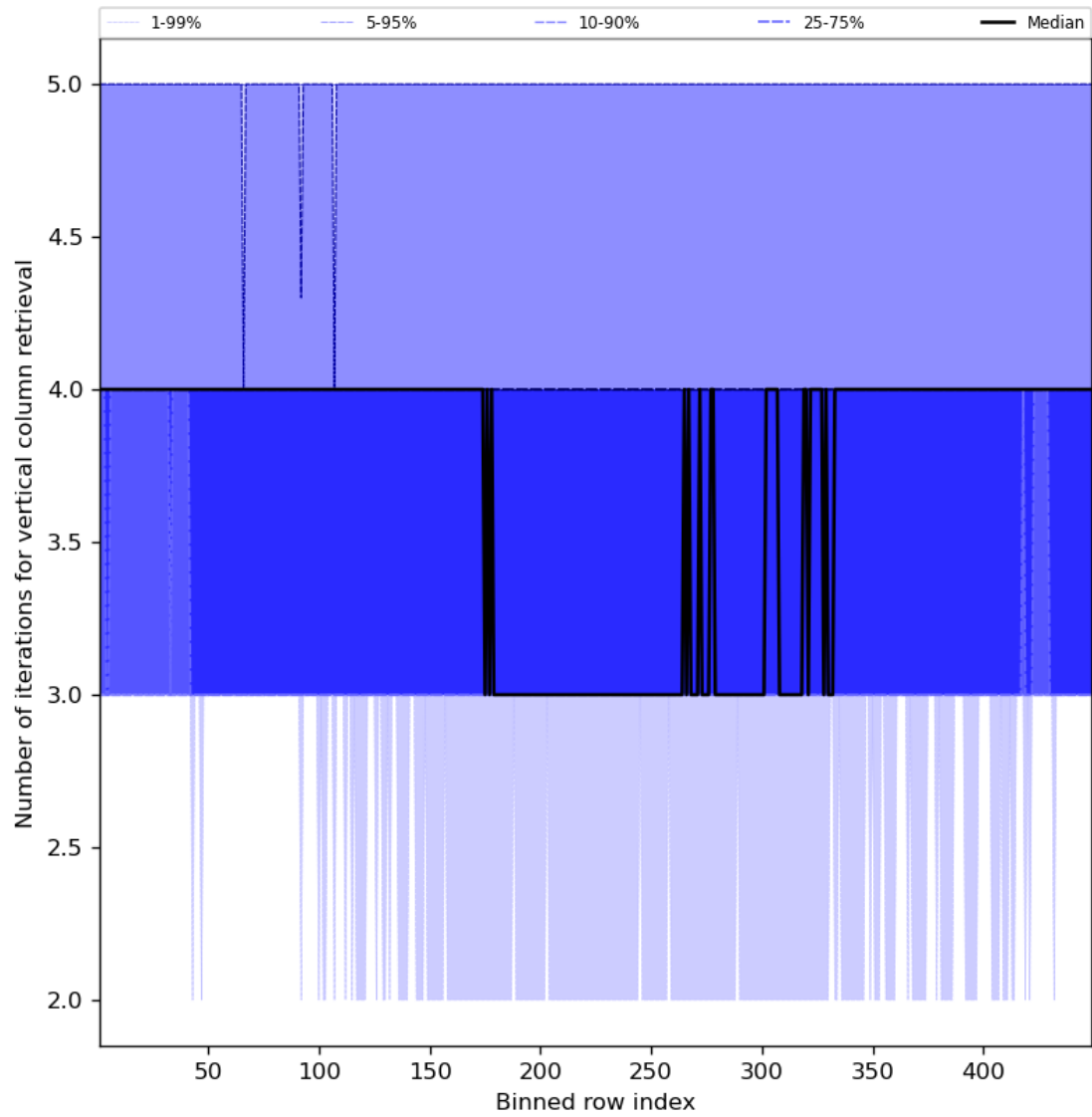
Figure 33: Along track statistics of “Number of iterations for vertical column retrieval” for 2023-10-22 to 2023-10-24
