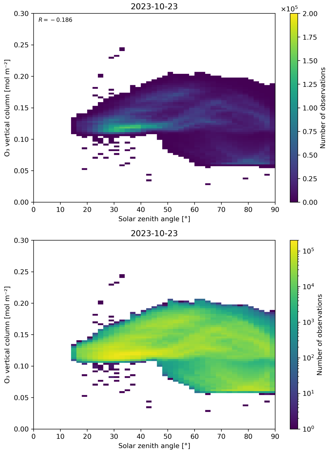
Figure 47: Scatter density plot of “Solar zenith angle” against “O 3 vertical column” for 2023-10-22 to 2023-10-24.
