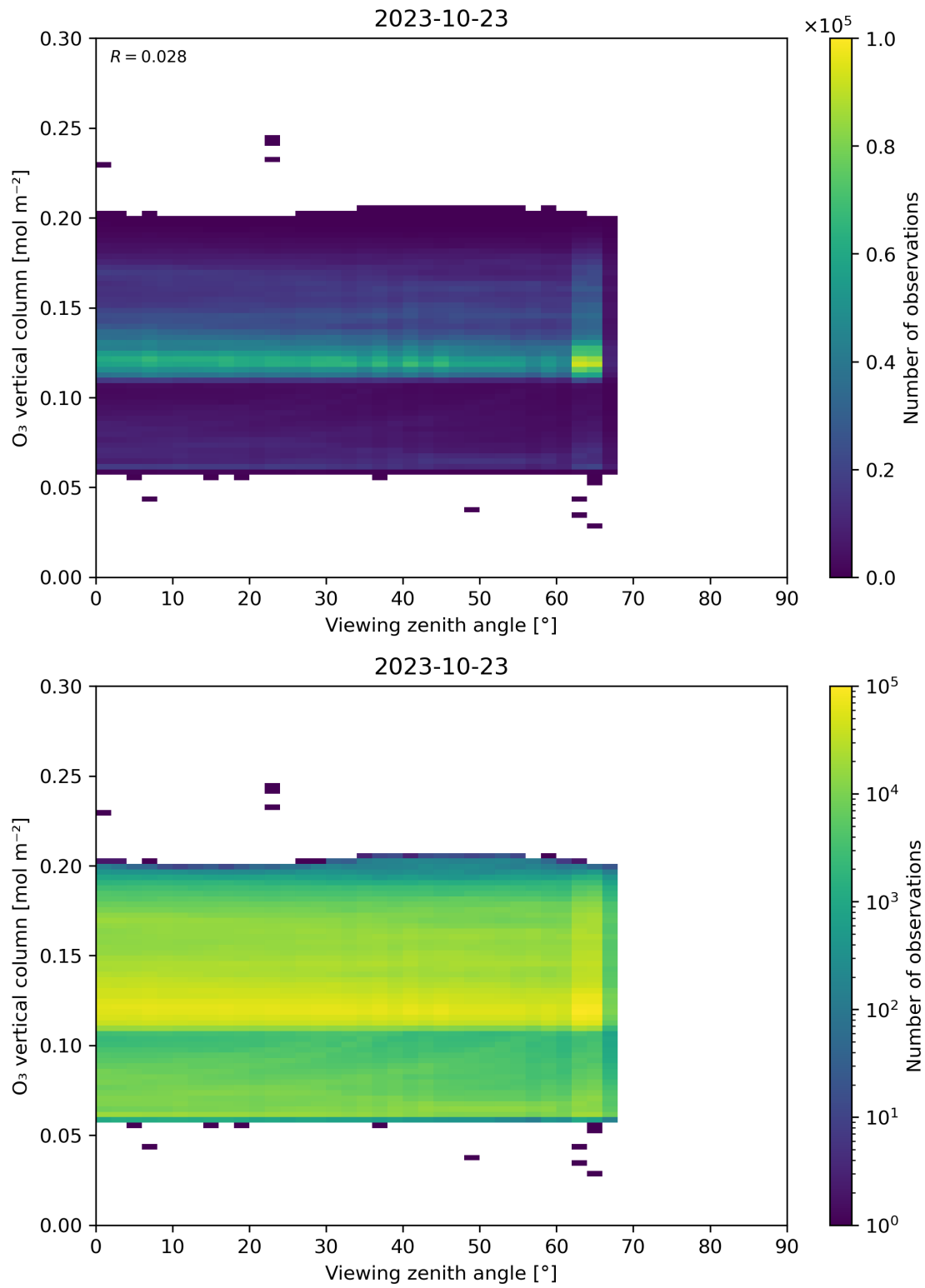
Figure 52: Scatter density plot of “Viewing zenith angle” against “O 3 vertical column” for 2023-10-22 to 2023-10-24.
