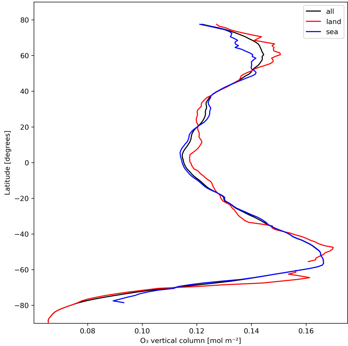
Figure 14: Zonal average of “O 3 vertical column” for 2023-10-22 to 2023-10-24.
