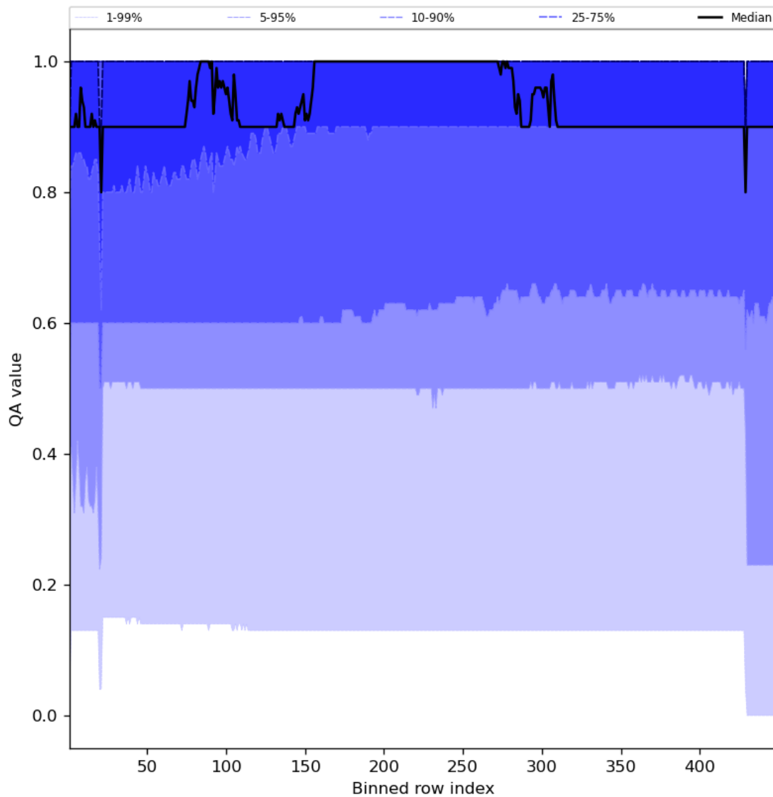
Figure 27: Along track statistics of “QA value” for 2023-10-22 to 2023-10-24
