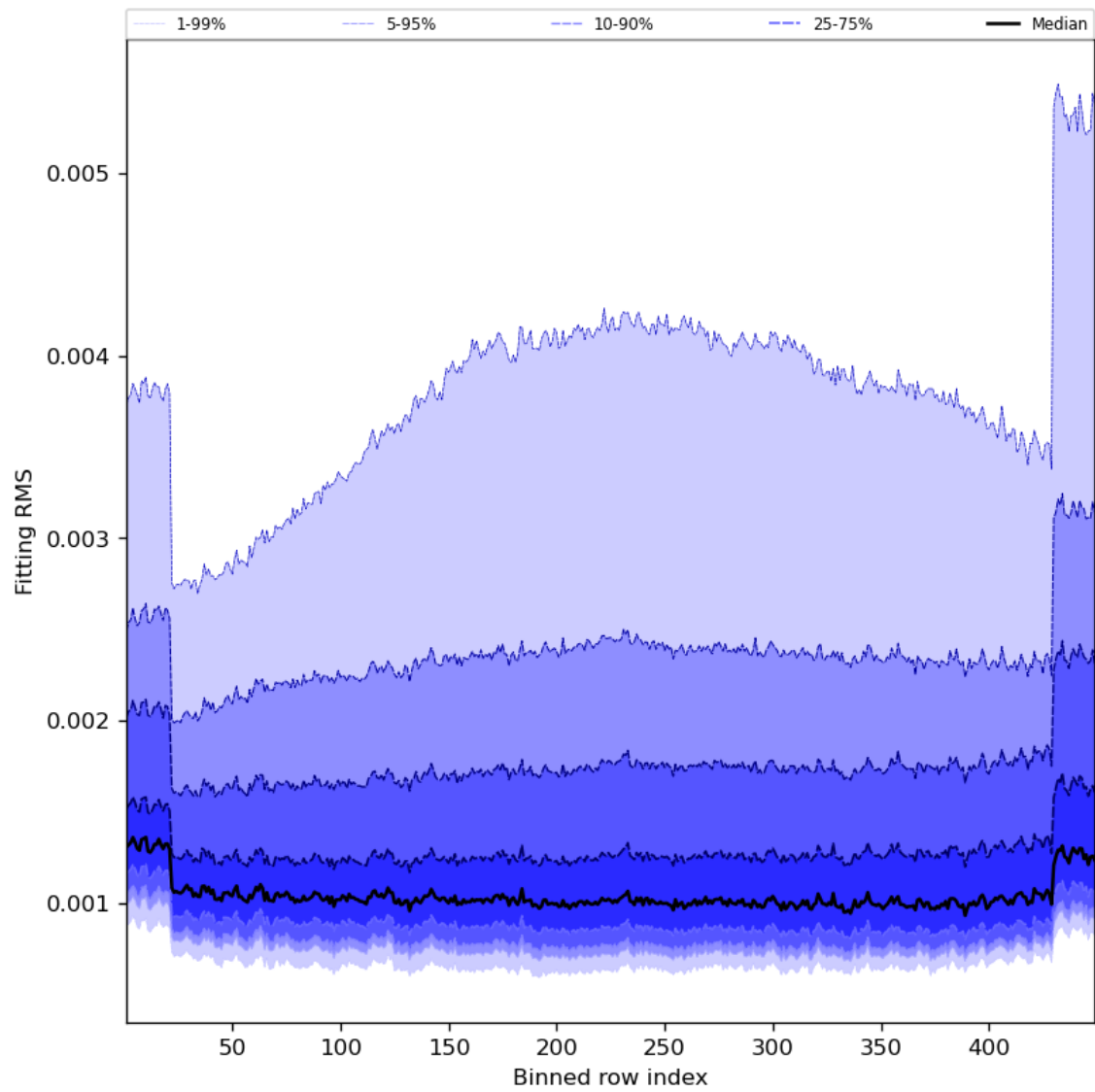
Figure 30: Along track statistics of “Fitting RMS” for 2023-10-22 to 2023-10-24
