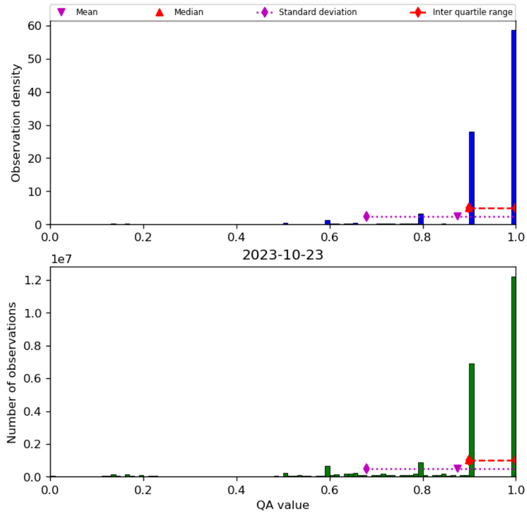
Figure 20: Histogram of “QA value” for 2023-10-22 to 2023-10-24
