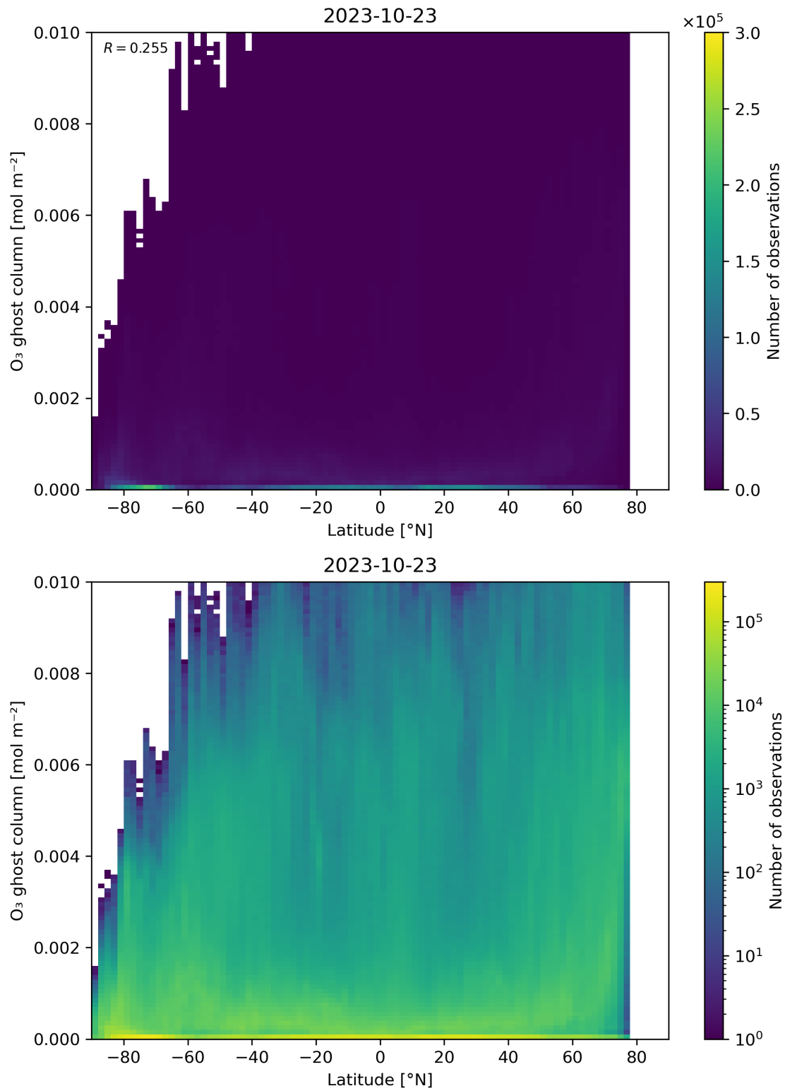
Figure 35: Scatter density plot of “Latitude” against “O 3 ghost column” for 2023-10-22 to 2023-10-24.
