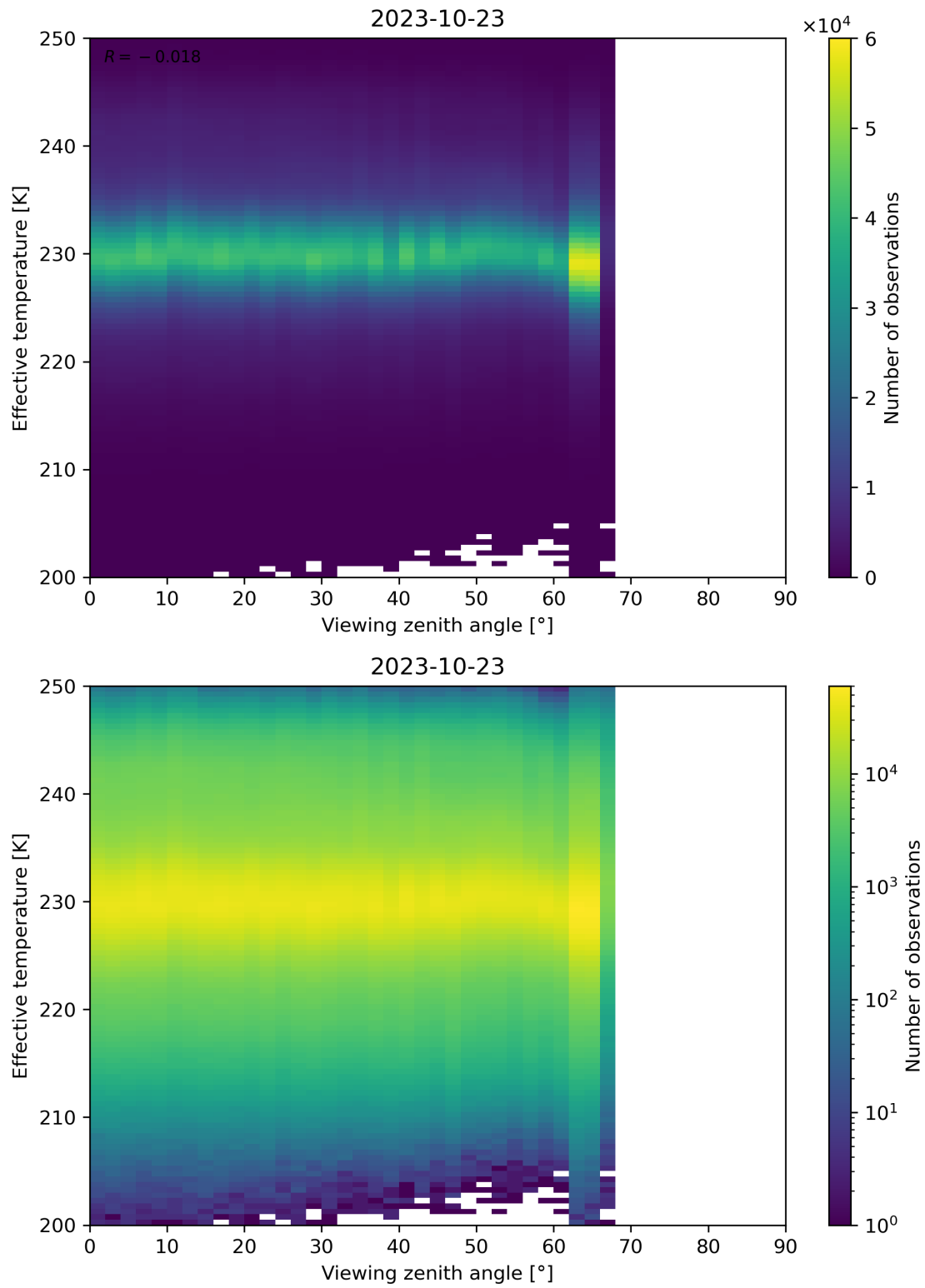
Figure 50: Scatter density plot of “Viewing zenith angle” against “Effective temperature” for 2023-10-22 to 2023-10-24.
