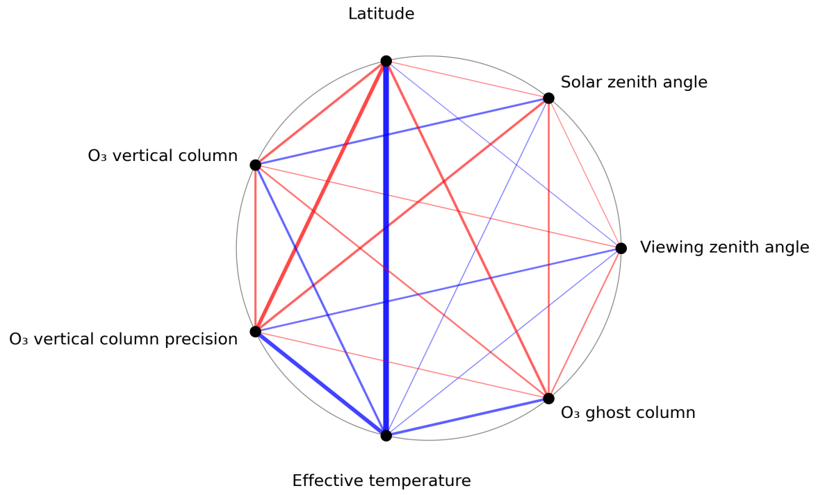
Figure 1: Map of correlation graph for 2023-10-22 to 2023-10-24.
