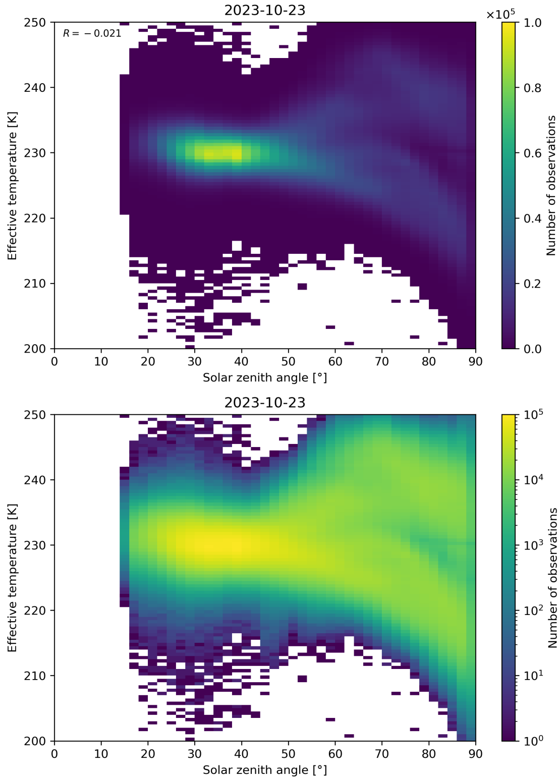
Figure 45: Scatter density plot of “Solar zenith angle” against “Effective temperature” for 2023-10-22 to 2023-10-24.
