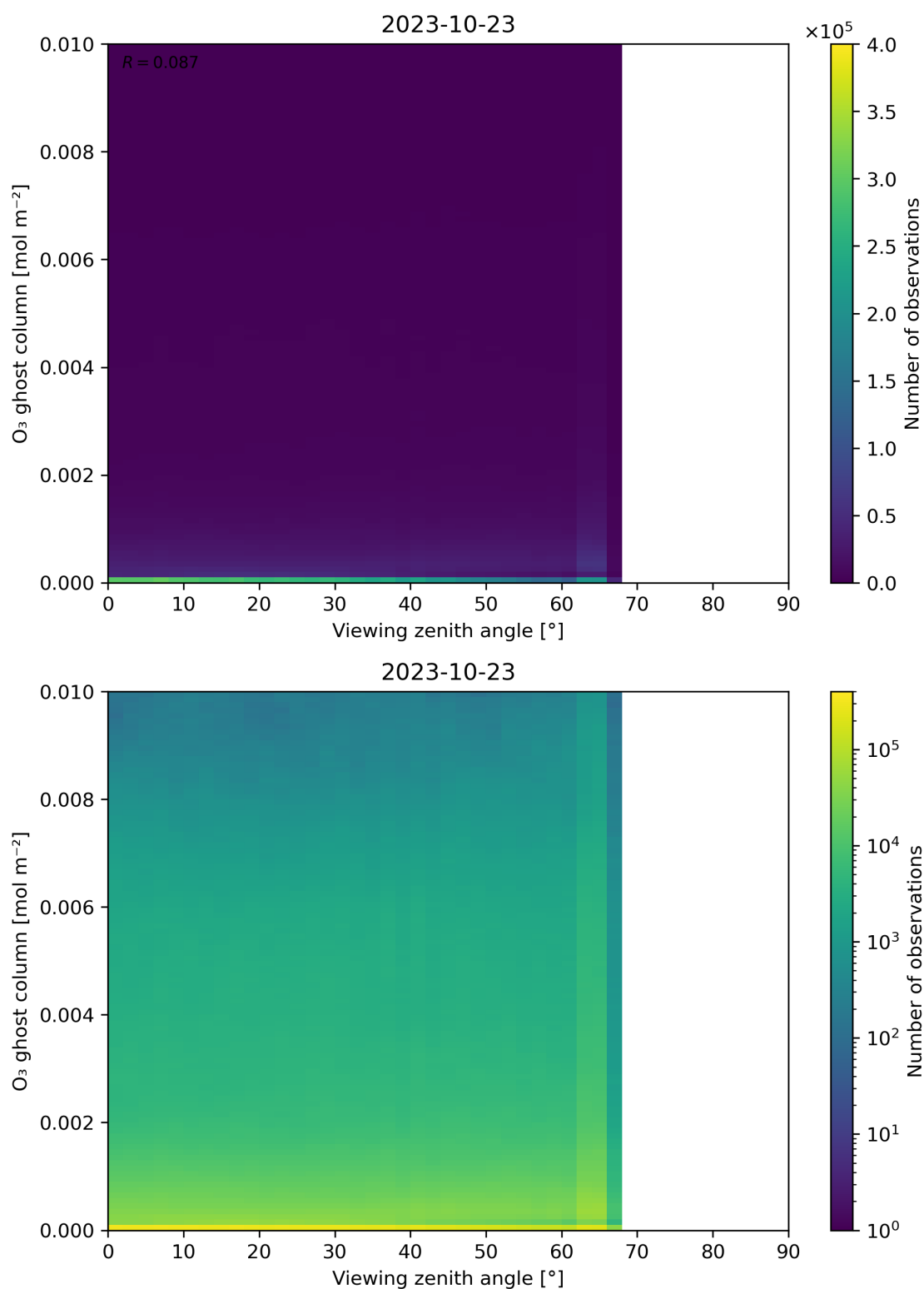
Figure 51: Scatter density plot of “Viewing zenith angle” against “O 3 ghost column” for 2023-10-22 to 2023-10-24.
