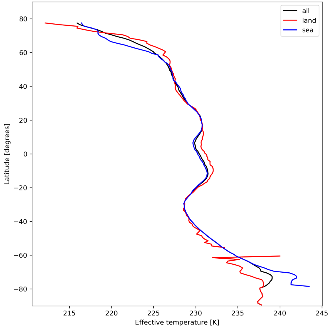
Figure 17: Zonal average of "Effective temperature" for 2023-10-22 to 2023-10-24.
