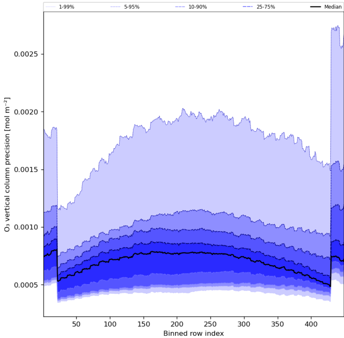
Figure 29: Along track statistics of “O 3 vertical column precision” for 2023-10-22 to 2023-10-24
