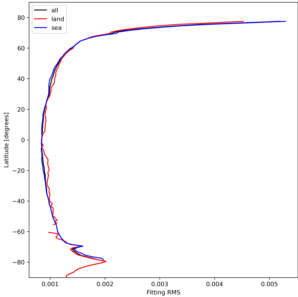
Figure 16: Zonal average of “Fitting RMS” for 2023-10-22 to 2023-10-24.
