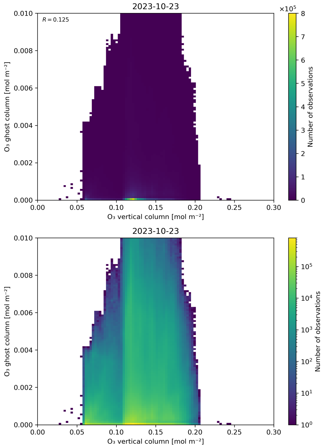
Figure 40: Scatter density plot of “O 3 vertical column” against “O 3 ghost column” for 2023-10-22 to 2023-10-24.
