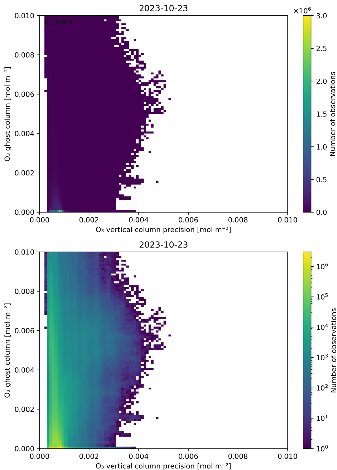
Figure 43: Scatter density plot of “O 3 vertical column precision” against “O 3 ghost column” for 2023-10-22 to 2023-10-24.
