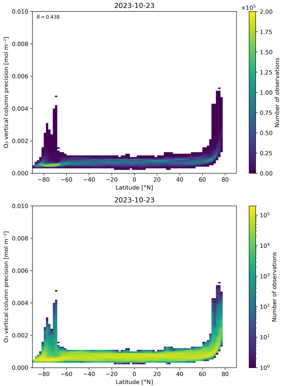
Figure 37: Scatter density plot of “Latitude” against “O 3 vertical column precision” for 2023-10-22 to 2023-10-24.
