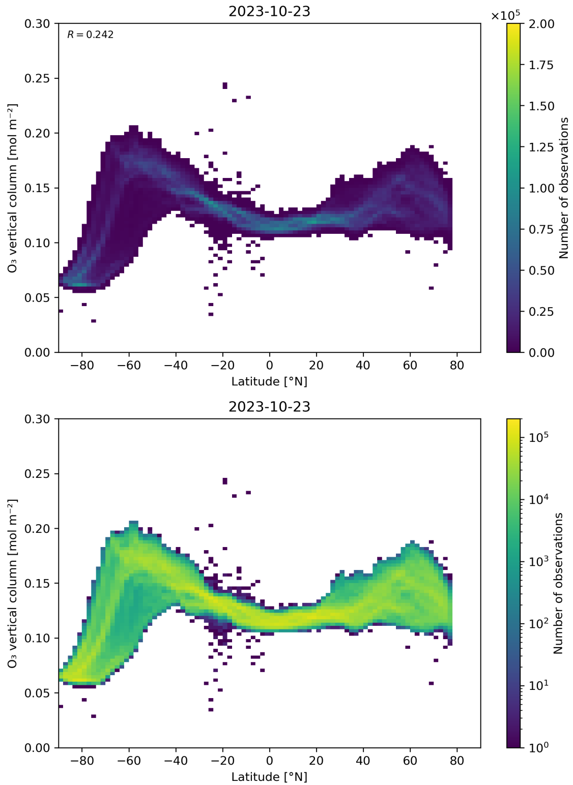
Figure 36: Scatter density plot of “Latitude” against “O 3 vertical column” for 2023-10-22 to 2023-10-24.
