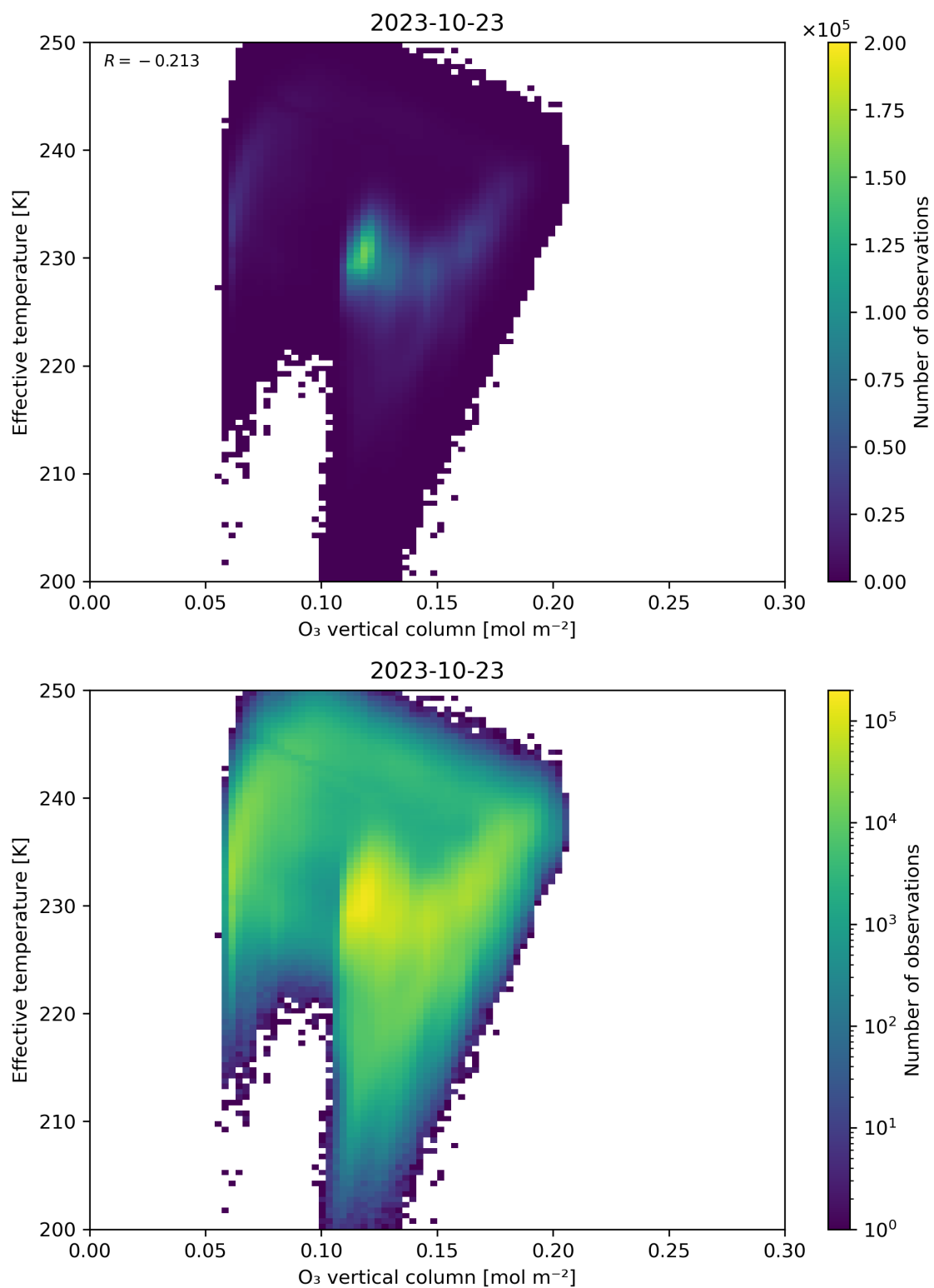
Figure 39: Scatter density plot of “O 3 vertical column” against “Effective temperature” for 2023-10-22 to 2023-10-24.
