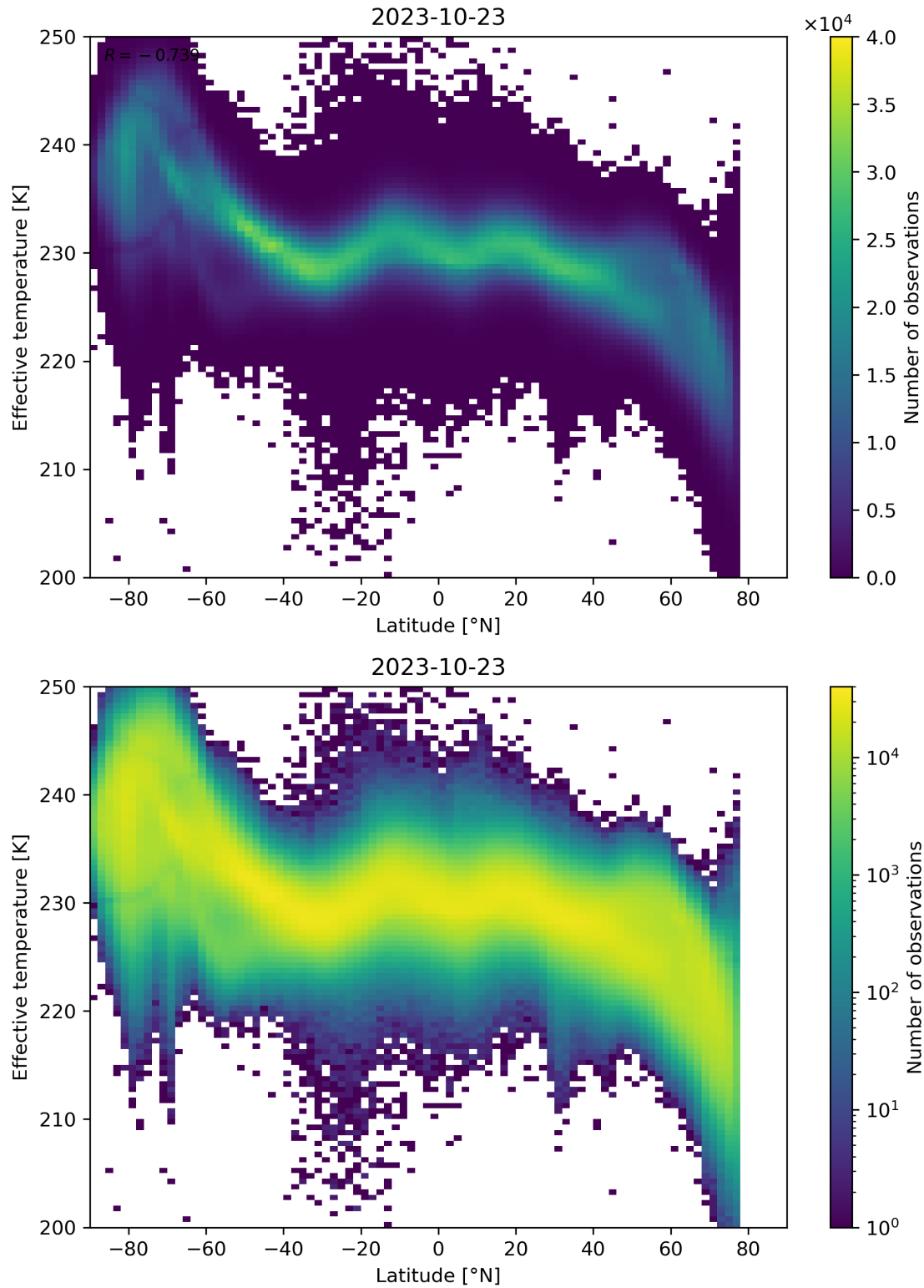
Figure 34: Scatter density plot of “Latitude” against “Effective temperature” for 2023-10-22 to 2023-10-24.
