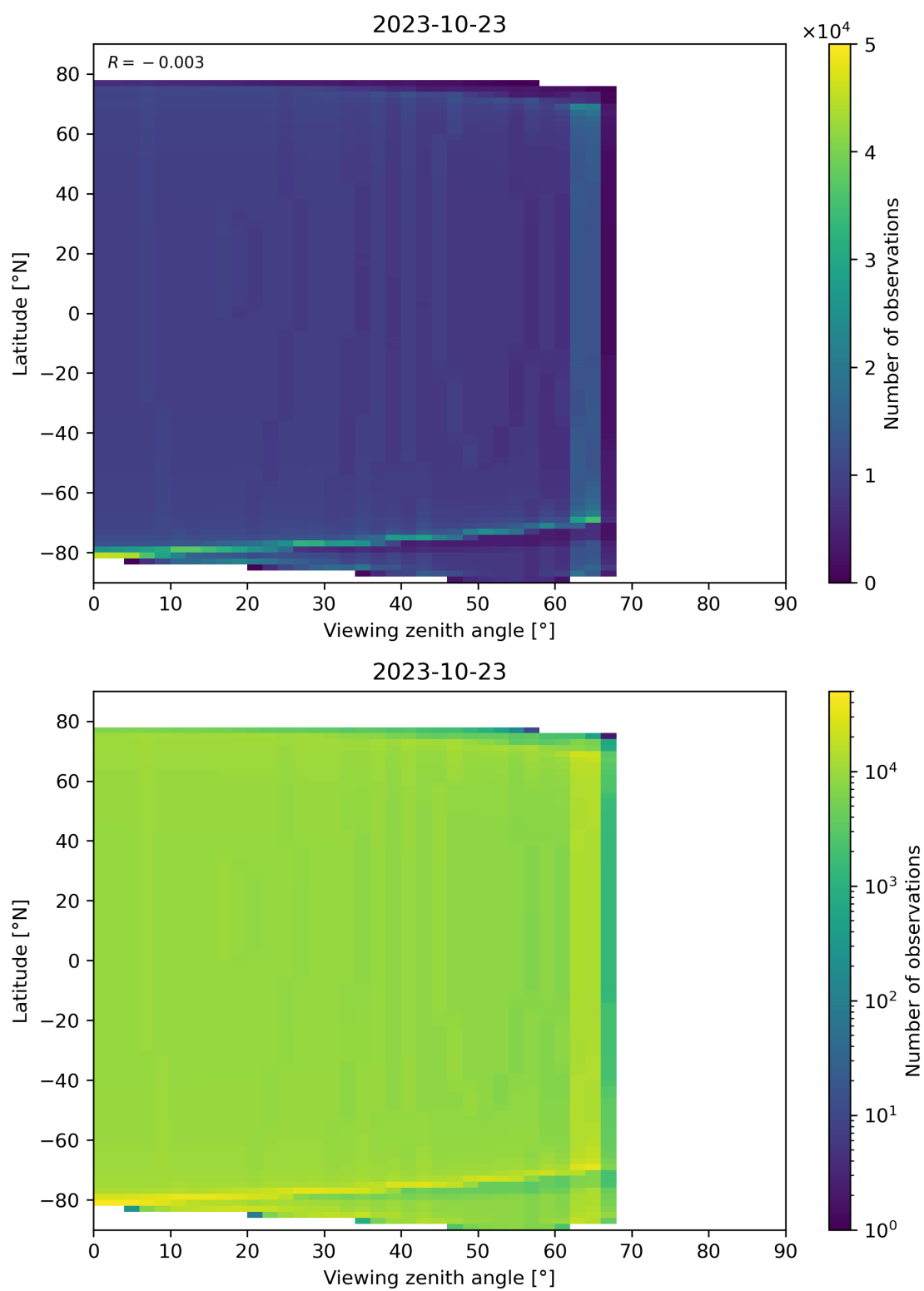
Figure 49: Scatter density plot of “Viewing zenith angle” against “Latitude” for 2023-10-22 to 2023-10-24.
