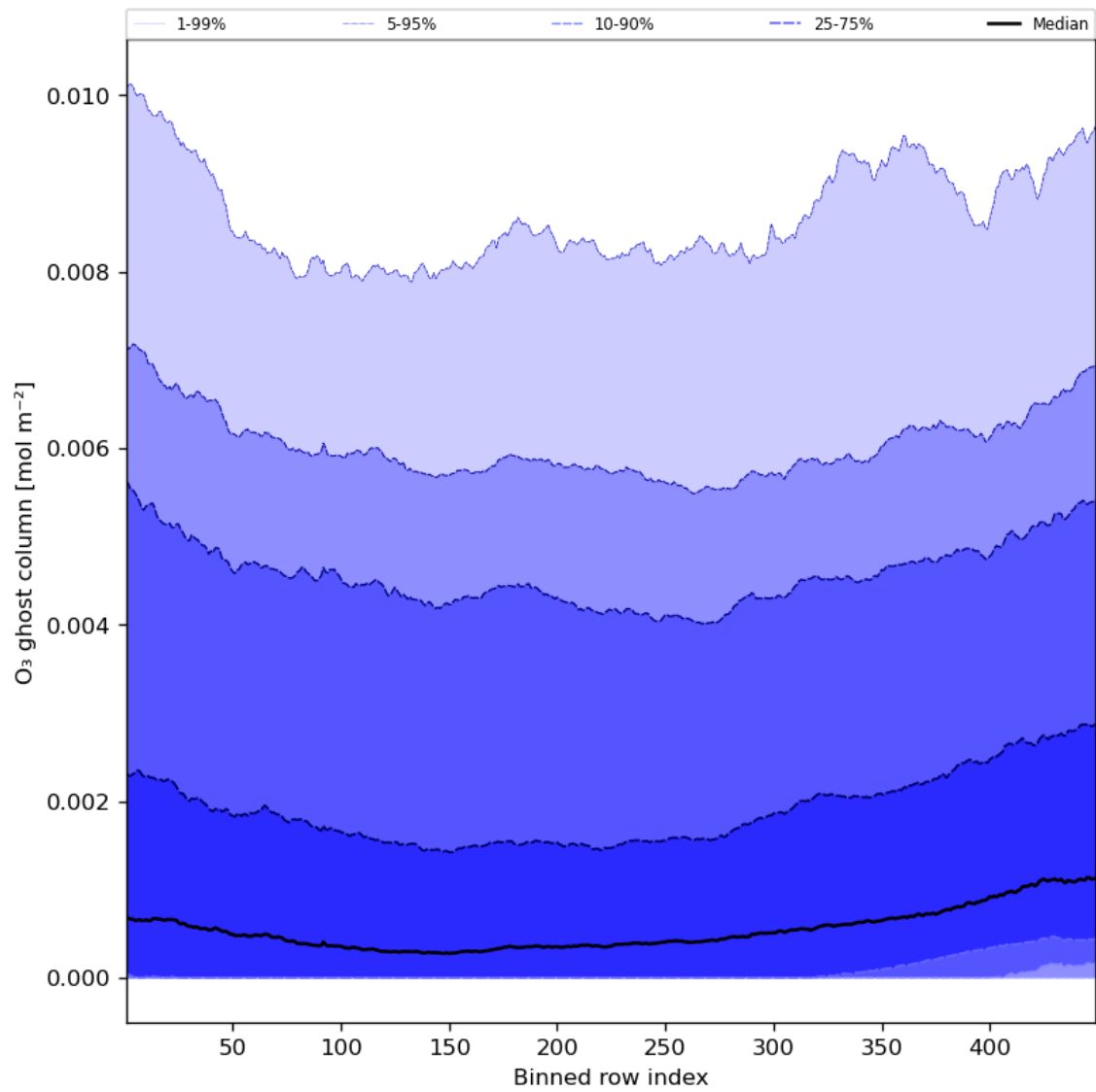
Figure 32: Along track statistics of “O 3 ghost column” for 2023-10-22 to 2023-10-24
