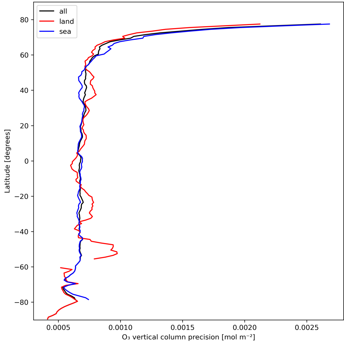
Figure 15: Zonal average of “O 3 vertical column precision” for 2023-10-22 to 2023-10-24.
