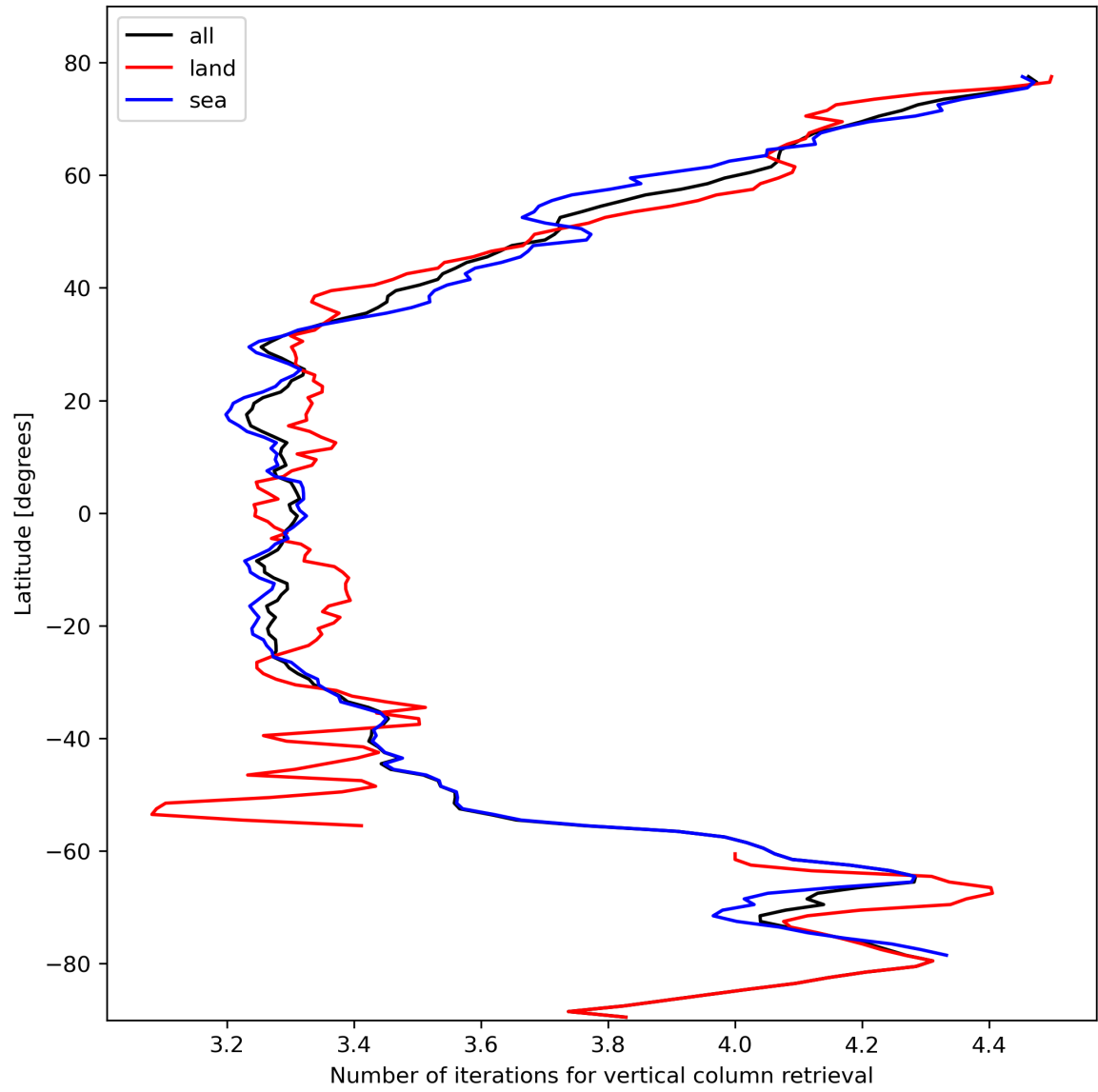
Figure 19: Zonal average of “Number of iterations for vertical column retrieval” for 2023-10-22 to 2023-10-24.
