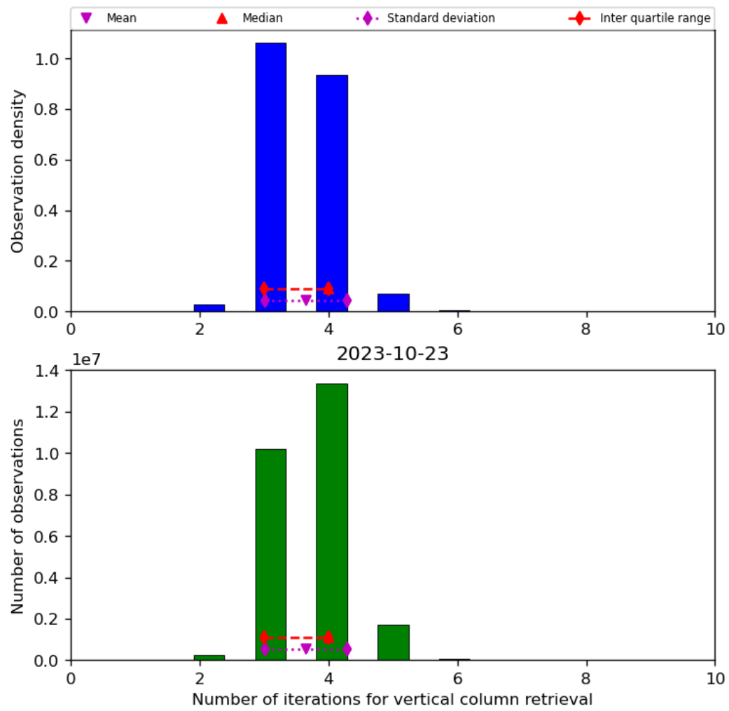
Figure 26: Histogram of “Number of iterations for vertical column retrieval” for 2023-10-22 to 2023-10-24
