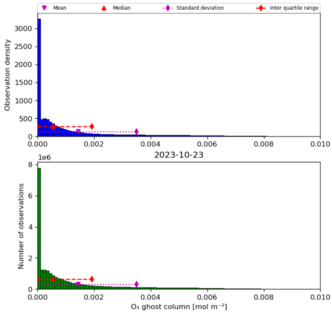
Figure 25: Histogram of “O 3 ghost column” for 2023-10-22 to 2023-10-24
