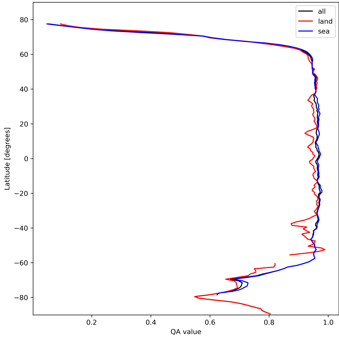
Figure 13: Zonal average of “QA value” for 2023-10-22 to 2023-10-24.
