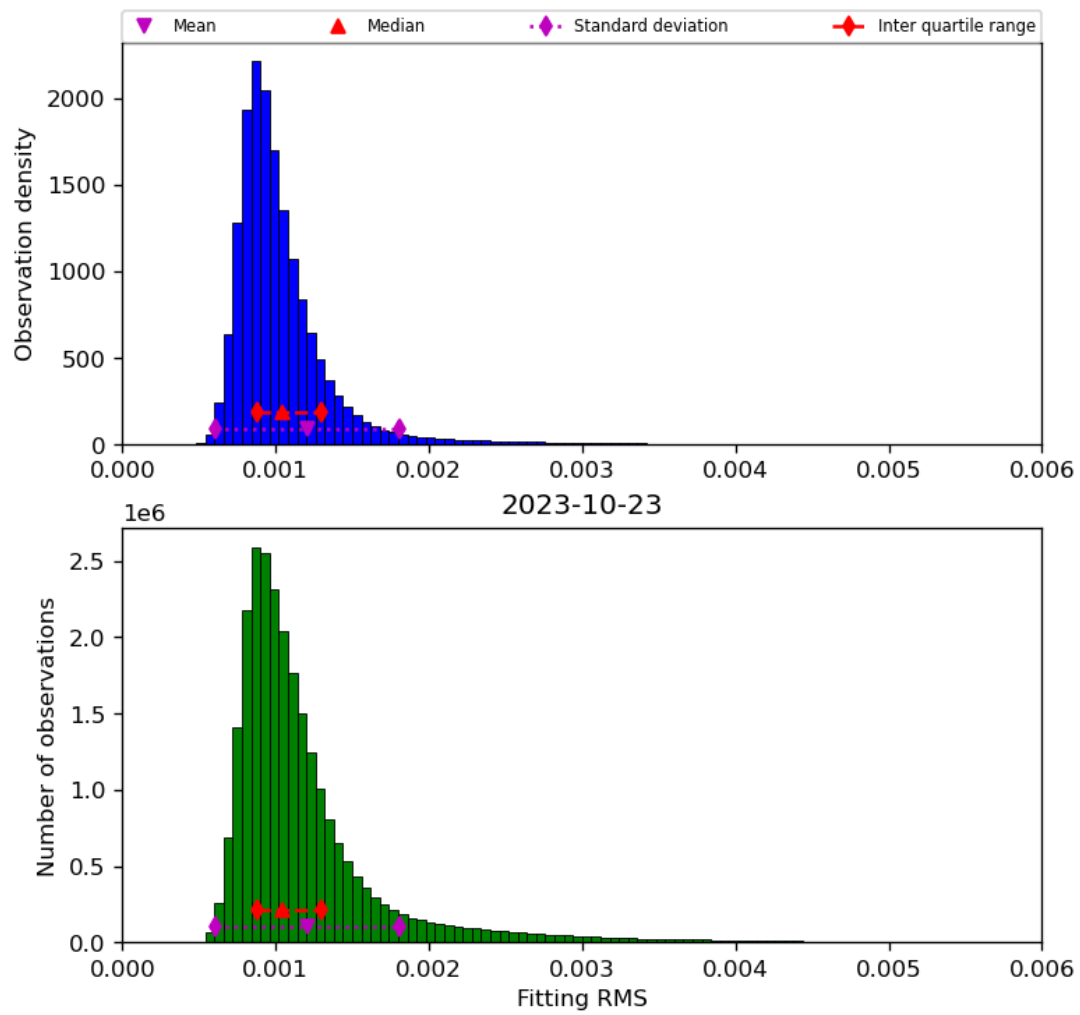
Figure 23: Histogram of “Fitting RMS” for 2023-10-22 to 2023-10-24
