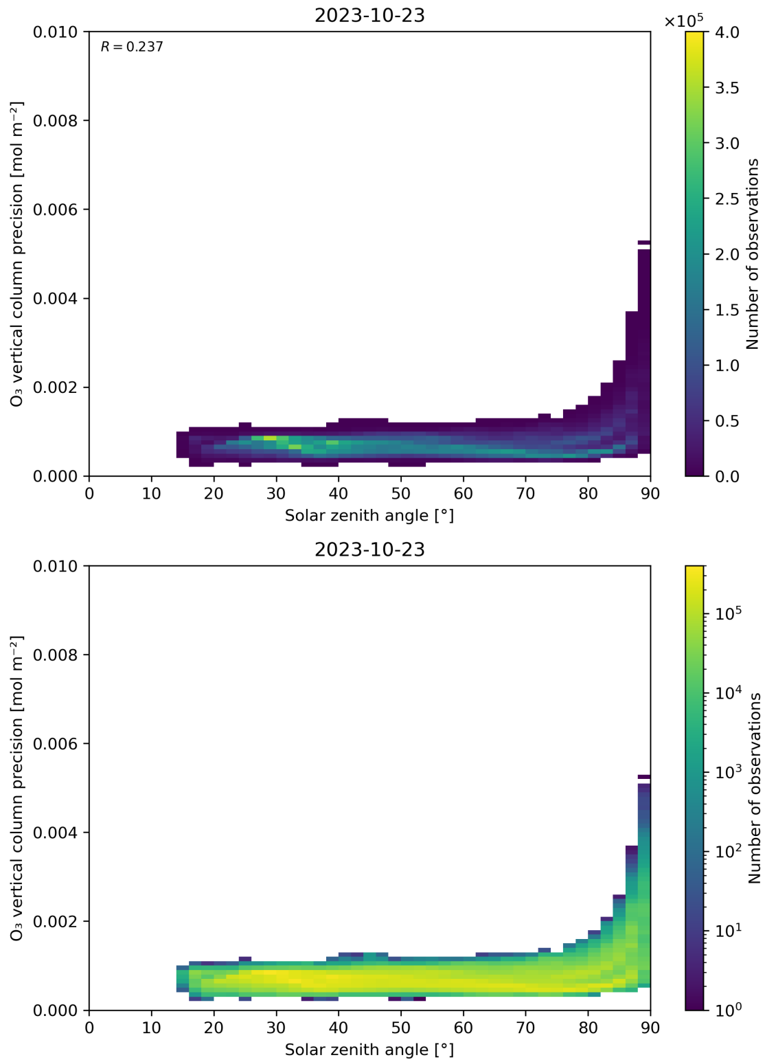
Figure 48: Scatter density plot of “Solar zenith angle” against “O 3 vertical column precision” for 2023-10-22 to 2023-10-24.
