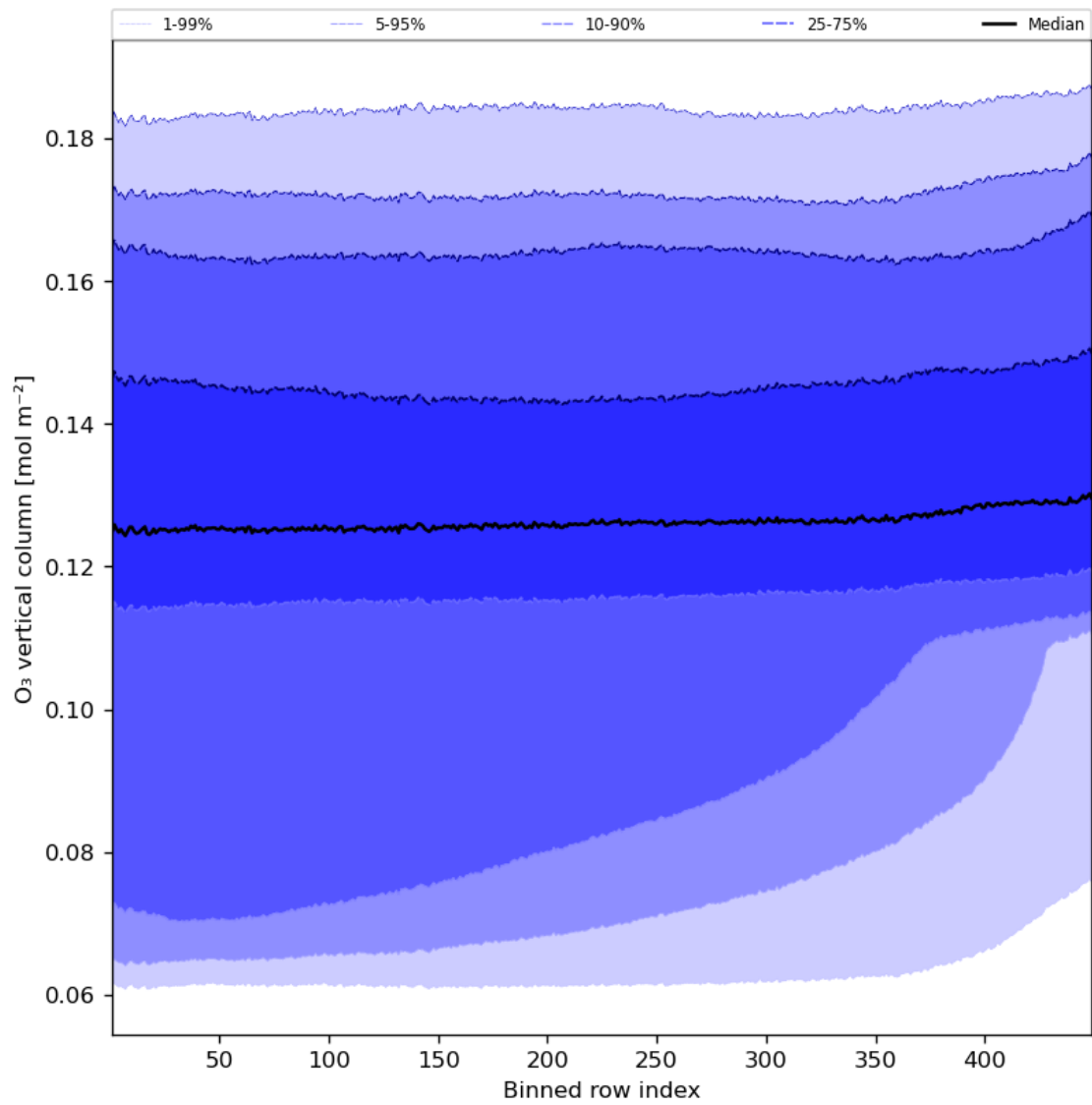
Figure 28: Along track statistics of “O 3 vertical column” for 2023-10-22 to 2023-10-24
