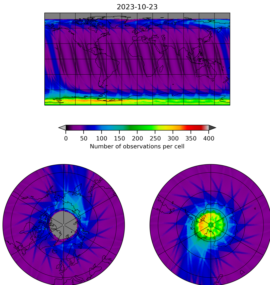
Figure 12: Map of the number of observations for 2023-10-22 to 2023-10-24
