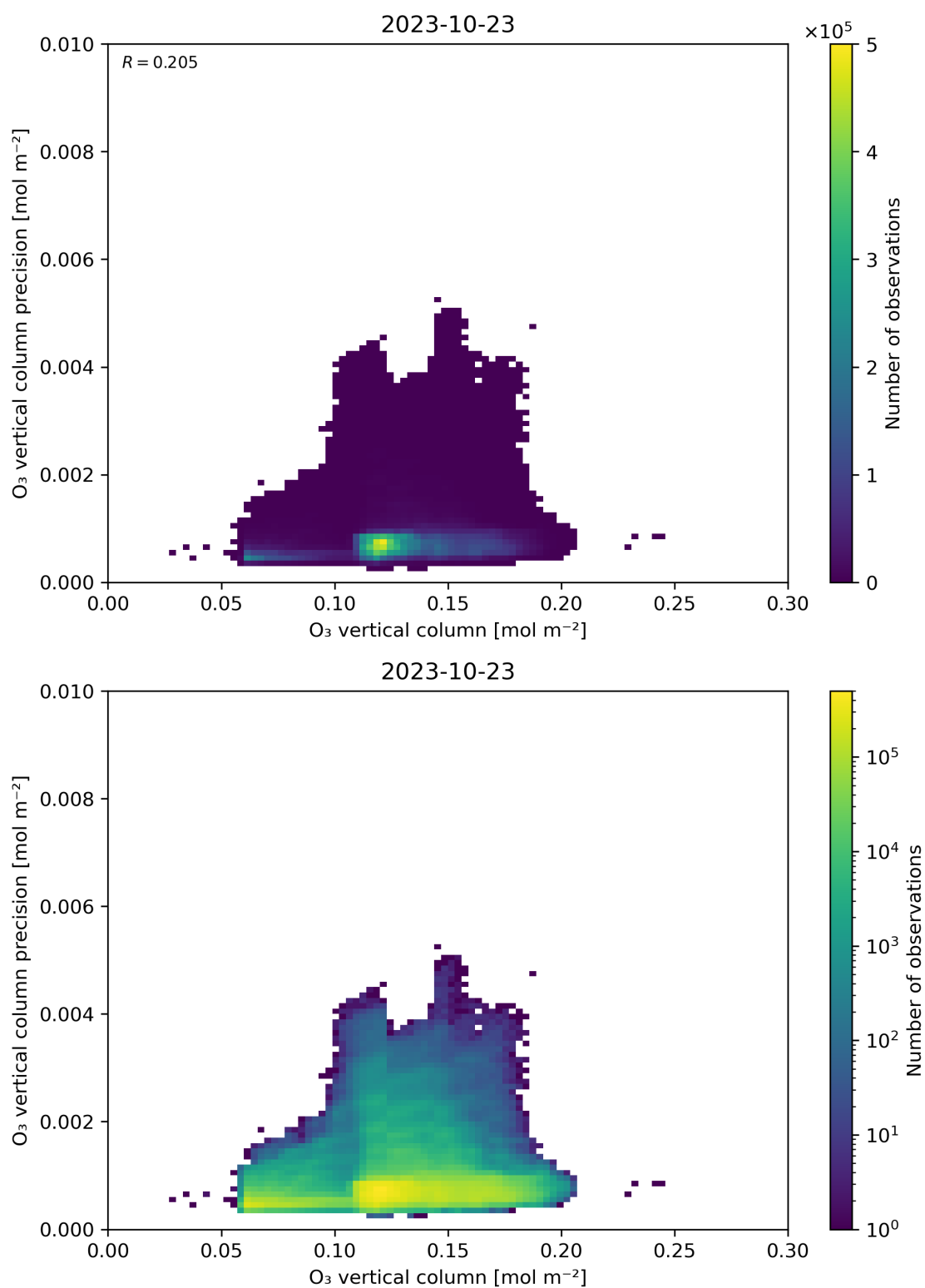
Figure 41: Scatter density plot of “O 3 vertical column” against “O 3 vertical column precision” for 2023-10-22 to 2023-10-24.
