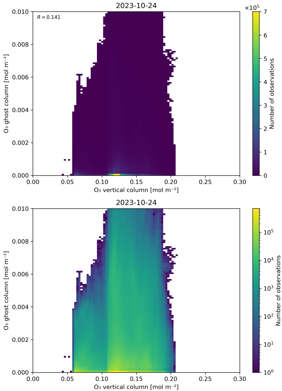
Figure 40: Scatter density plot of “O 3 vertical column” against “O 3 ghost column” for 2023-10-23 to 2023-10-25.
