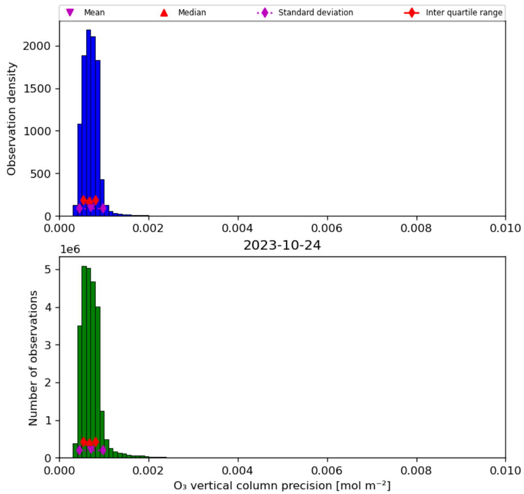
Figure 22: Histogram of “O 3 vertical column precision” for 2023-10-23 to 2023-10-25
