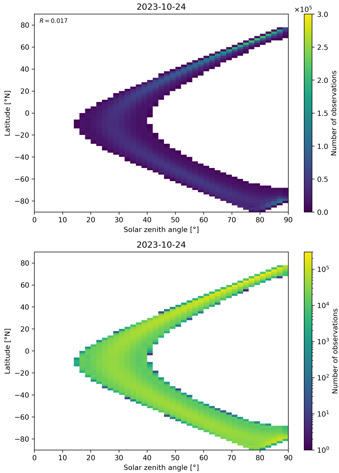
Figure 44: Scatter density plot of “Solar zenith angle” against “Latitude” for 2023-10-23 to 2023-10-25.
