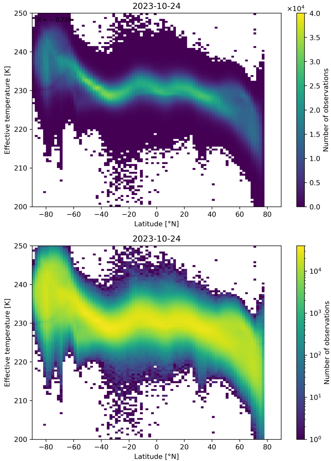
Figure 34: Scatter density plot of “Latitude” against “Effective temperature” for 2023-10-23 to 2023-10-25.
