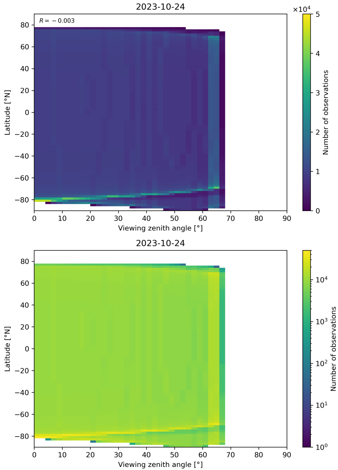
Figure 49: Scatter density plot of “Viewing zenith angle” against “Latitude” for 2023-10-23 to 2023-10-25.
