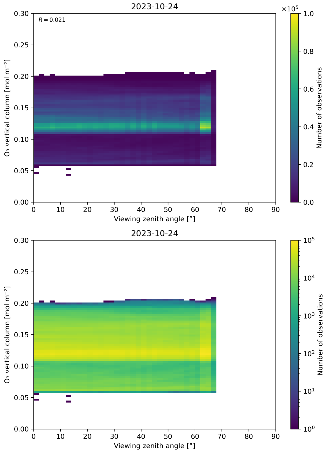
Figure 52: Scatter density plot of “Viewing zenith angle” against “O 3 vertical column” for 2023-10-23 to 2023-10-25.
