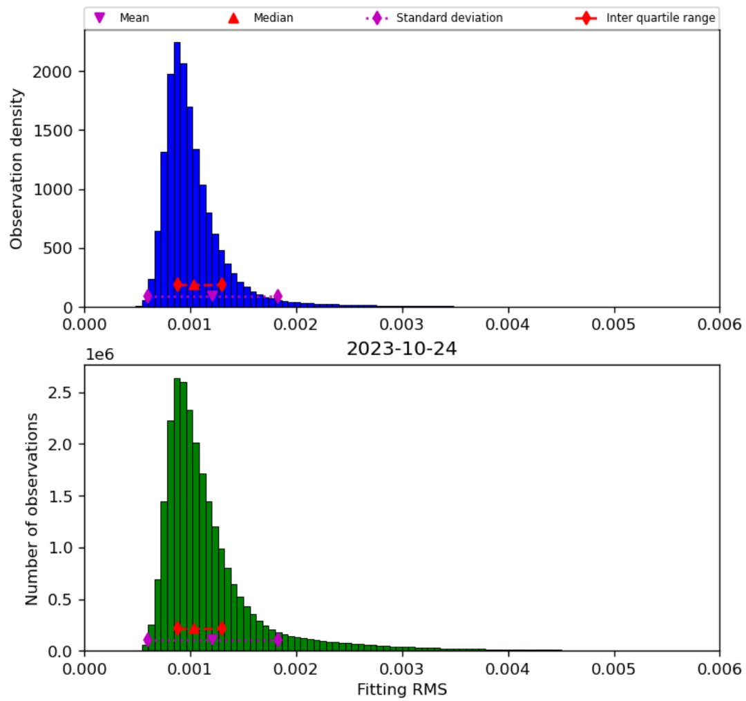
Figure 23: Histogram of “Fitting RMS” for 2023-10-23 to 2023-10-25
