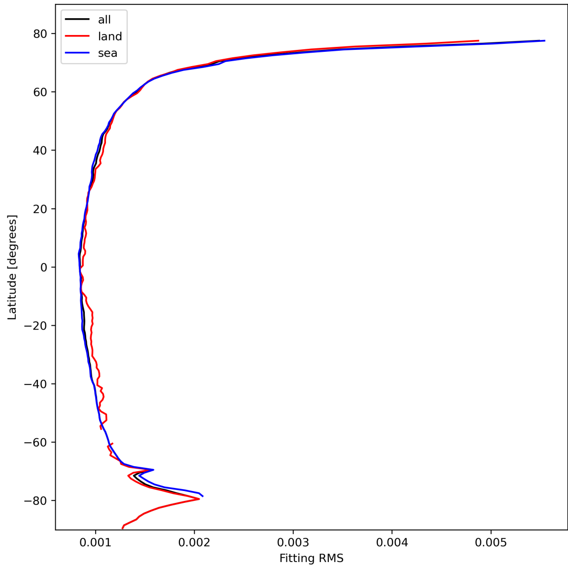
Figure 16: Zonal average of “Fitting RMS” for 2023-10-23 to 2023-10-25.
