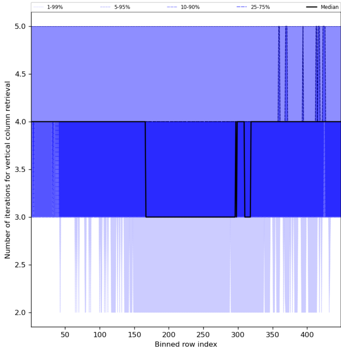
Figure 33: Along track statistics of “Number of iterations for vertical column retrieval” for 2023-10-23 to 2023-10-25
