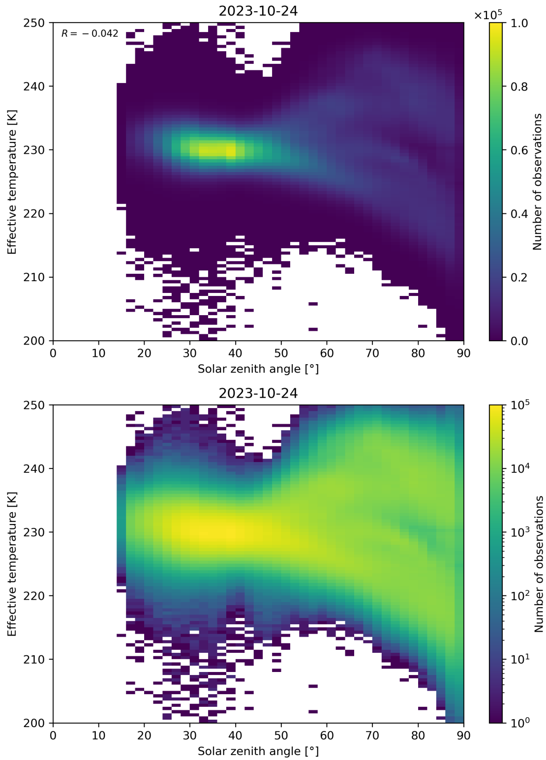
Figure 45: Scatter density plot of “Solar zenith angle” against “Effective temperature” for 2023-10-23 to 2023-10-25.
