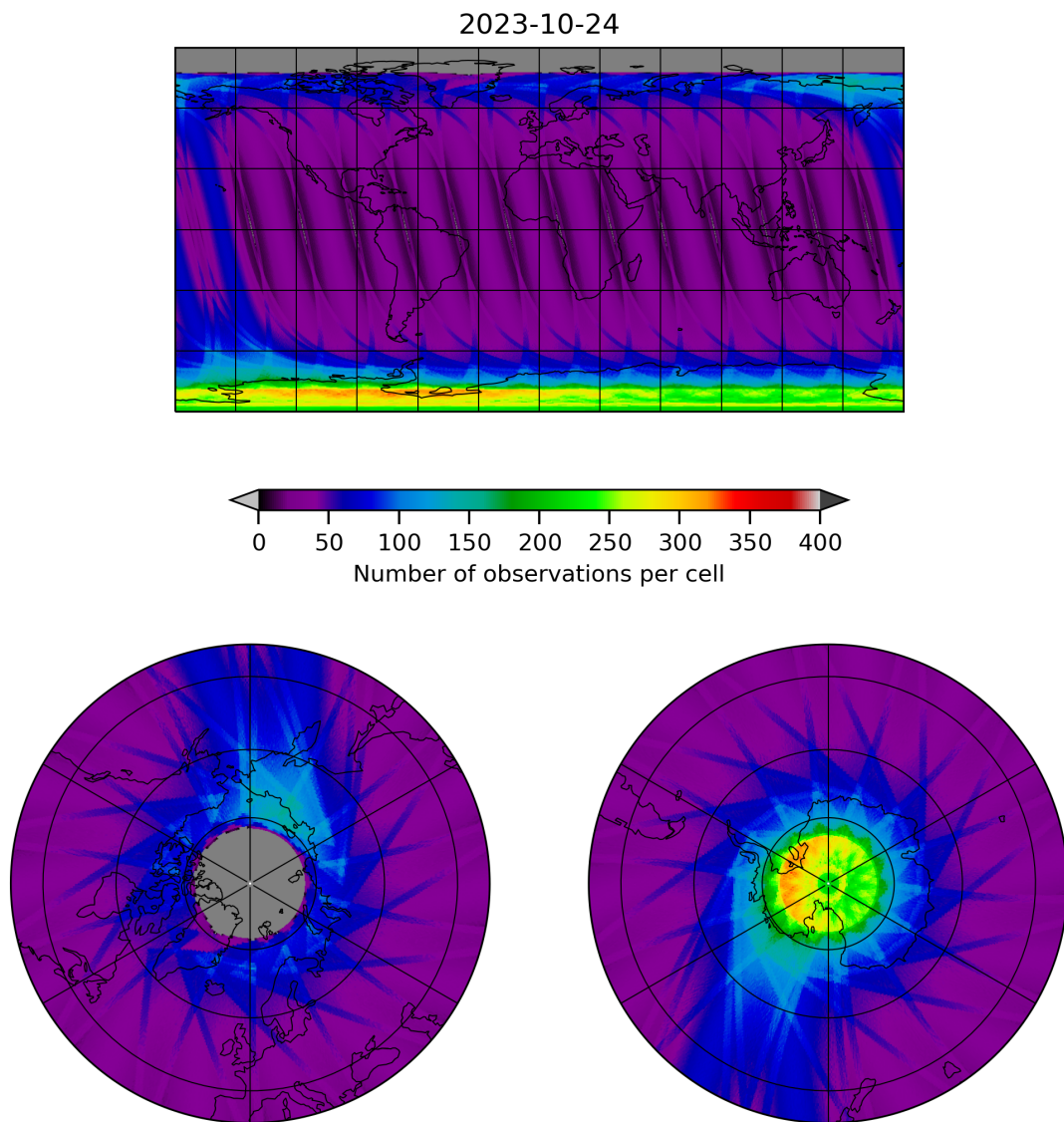
Figure 12: Map of the number of observations for 2023-10-23 to 2023-10-25
