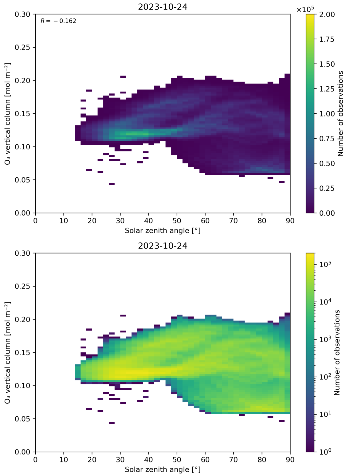
Figure 47: Scatter density plot of “Solar zenith angle” against “O 3 vertical column” for 2023-10-23 to 2023-10-25.
