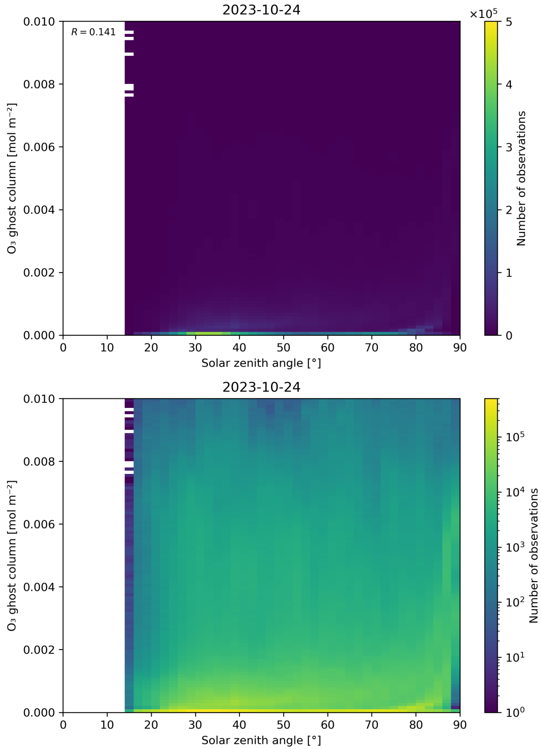
Figure 46: Scatter density plot of “Solar zenith angle” against “O 3 ghost column” for 2023-10-23 to 2023-10-25.
