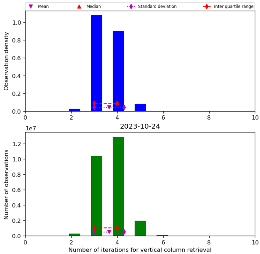
Figure 26: Histogram of “Number of iterations for vertical column retrieval” for 2023-10-23 to 2023-10-25
