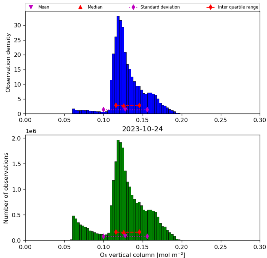
Figure 21: Histogram of “O 3 vertical column” for 2023-10-23 to 2023-10-25
