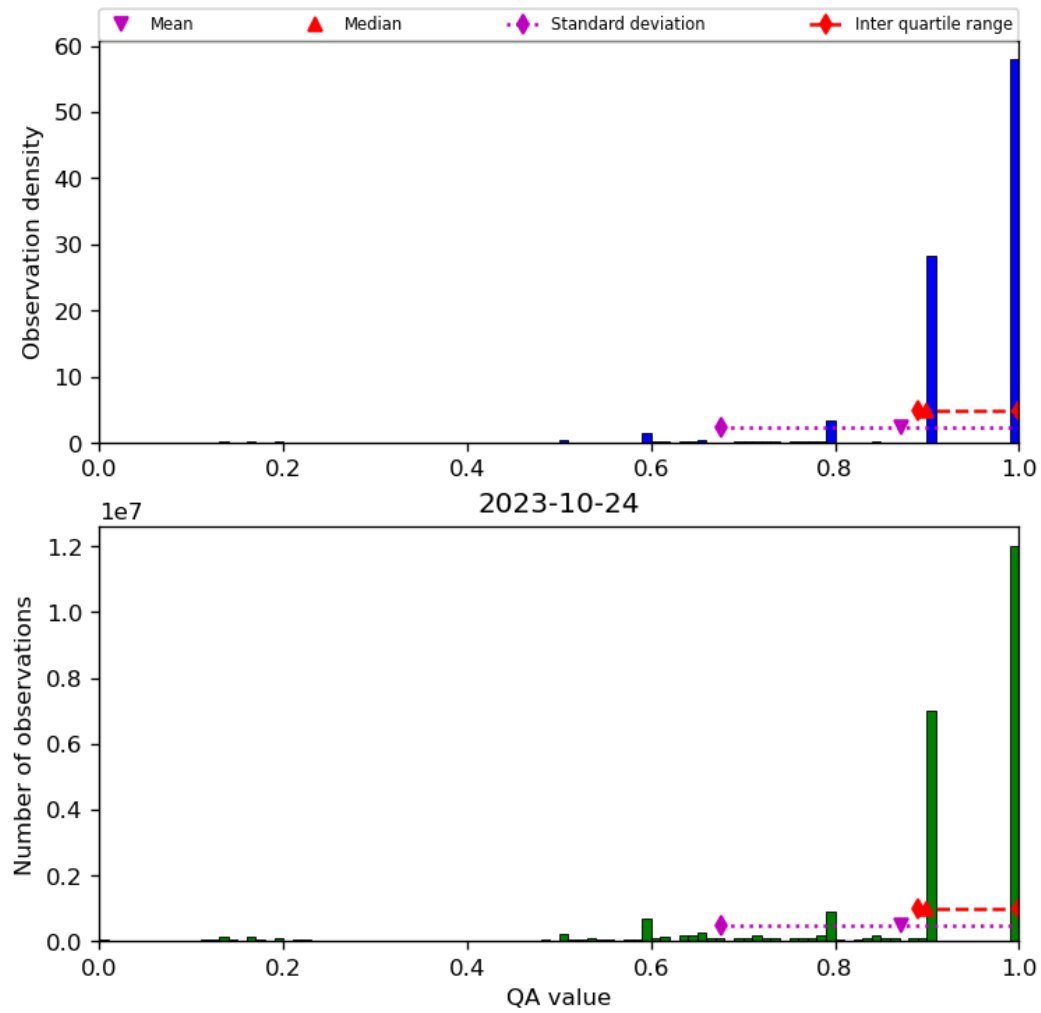
Figure 20: Histogram of “QA value” for 2023-10-23 to 2023-10-25
