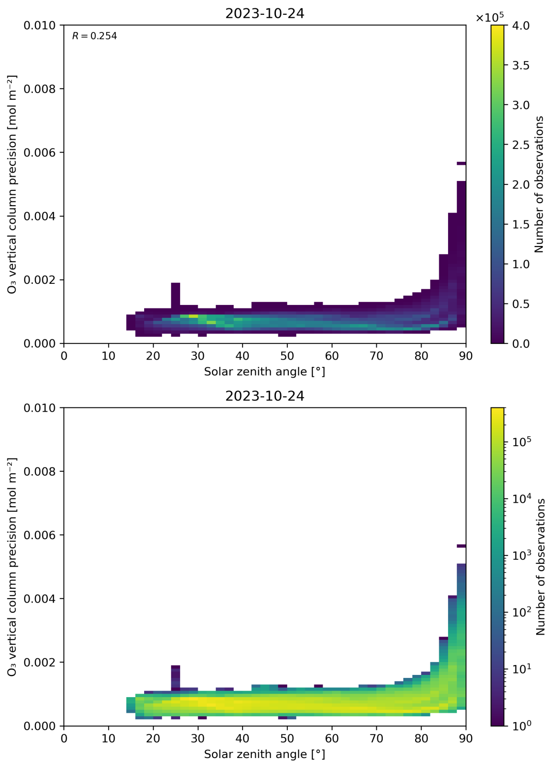
Figure 48: Scatter density plot of “Solar zenith angle” against “O 3 vertical column precision” for 2023-10-23 to 2023-10-25.
