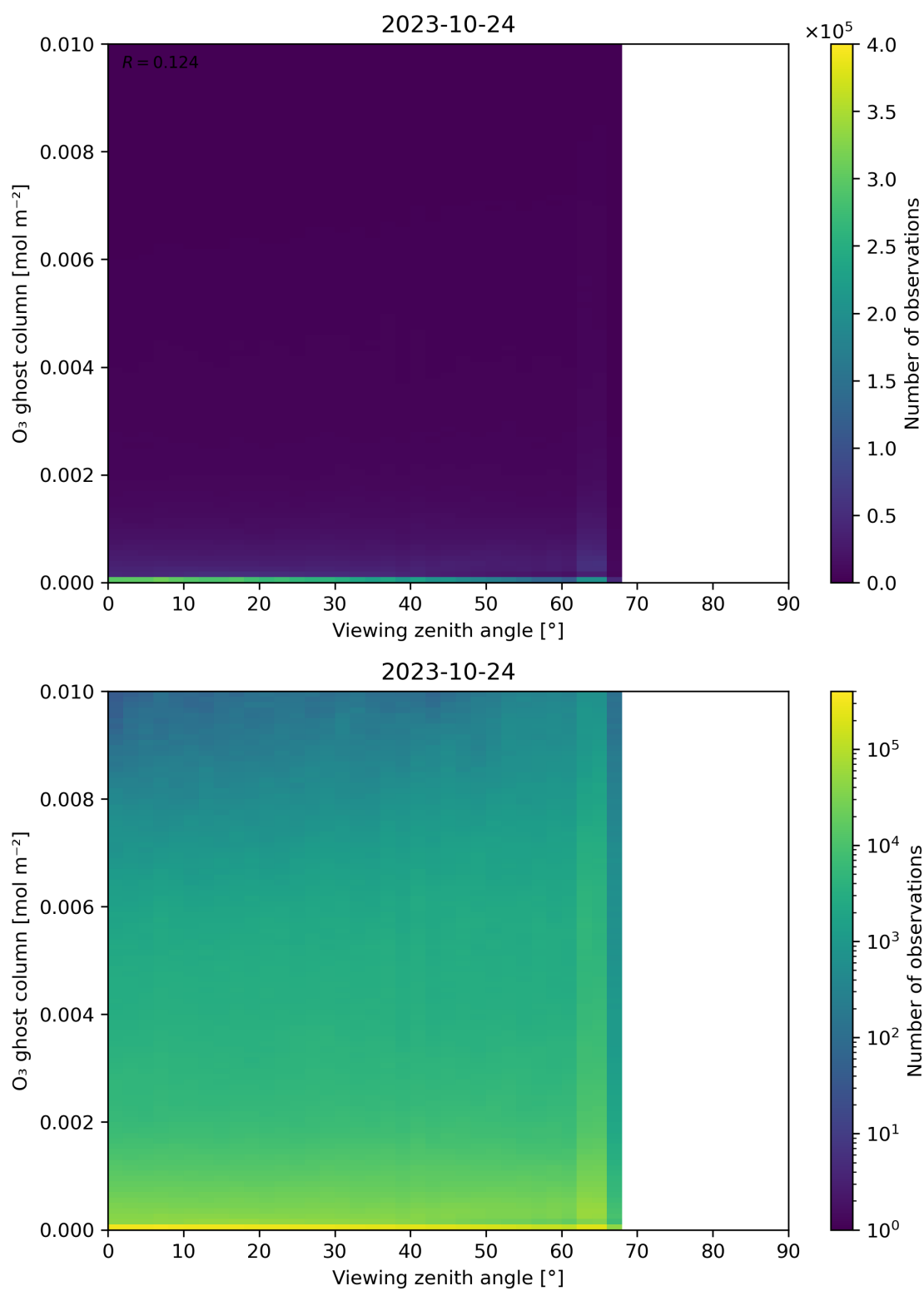
Figure 51: Scatter density plot of “Viewing zenith angle” against “O 3 ghost column” for 2023-10-23 to 2023-10-25.
