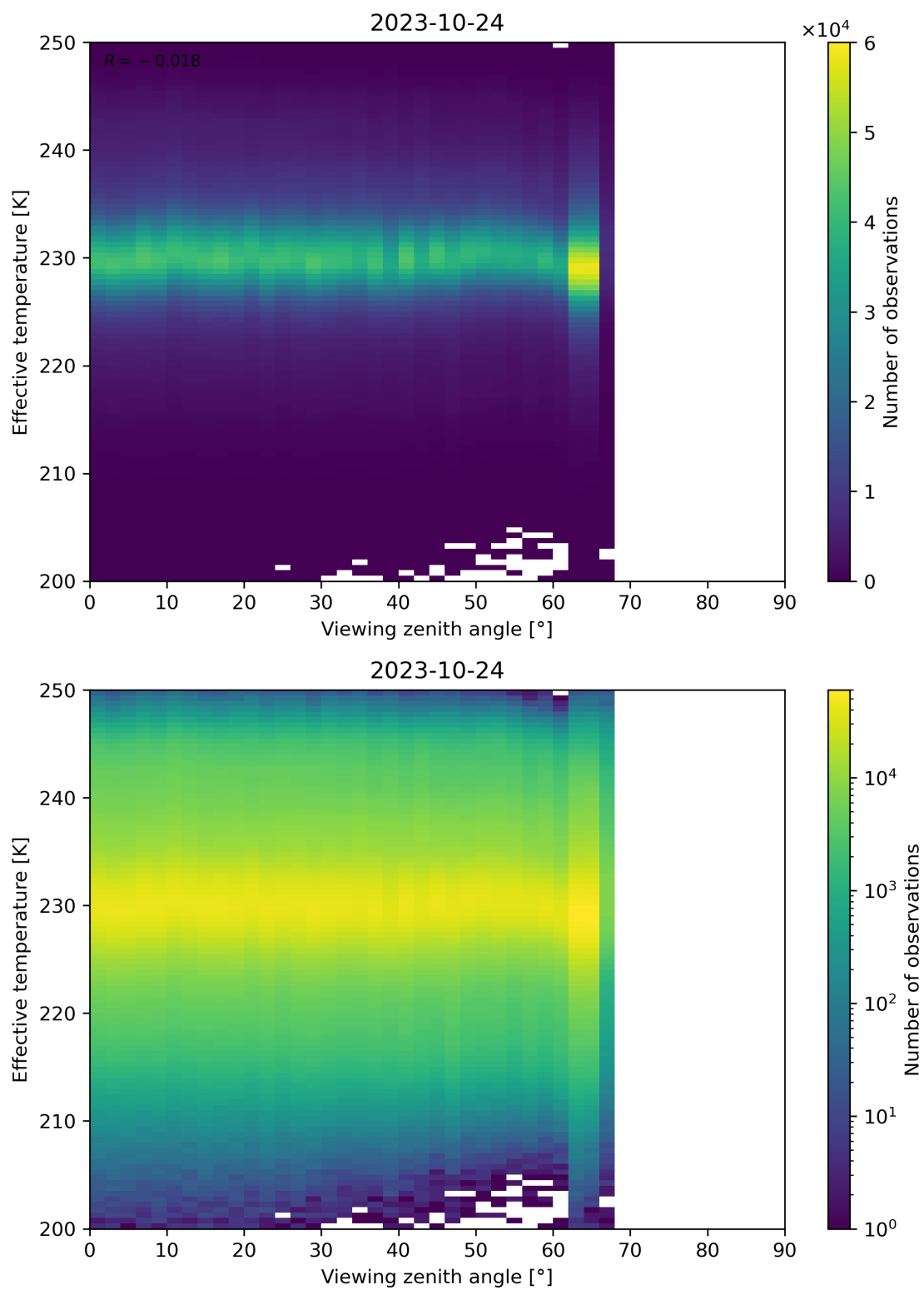
Figure 50: Scatter density plot of “Viewing zenith angle” against “Effective temperature” for 2023-10-23 to 2023-10-25.
