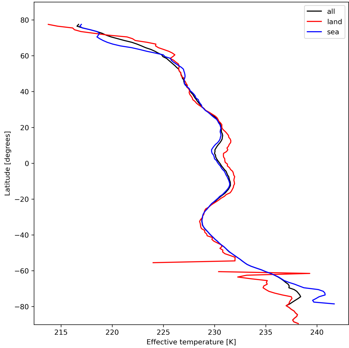
Figure 17: Zonal average of "Effective temperature" for 2023-10-23 to 2023-10-25.
