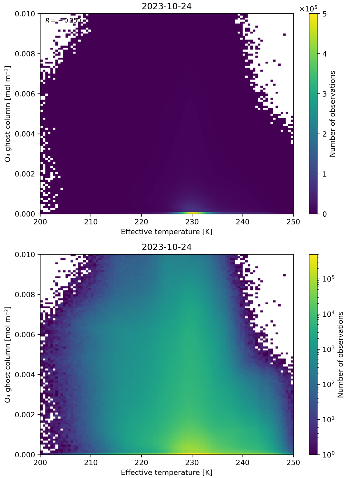
Figure 38: Scatter density plot of “Effective temperature” against “O 3 ghost column” for 2023-10-23 to 2023-10-25.
