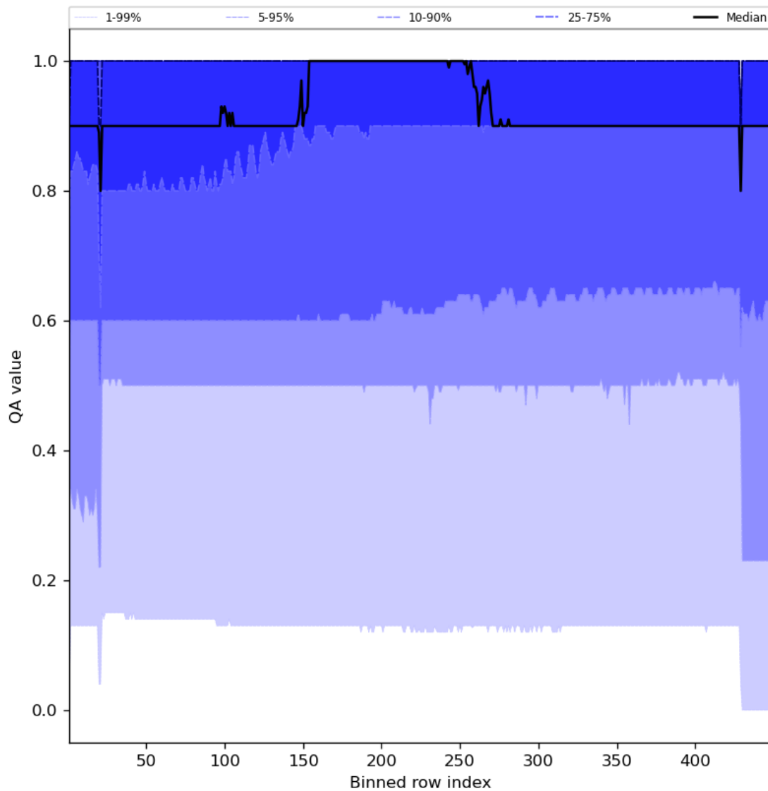
Figure 27: Along track statistics of “QA value” for 2023-10-23 to 2023-10-25
