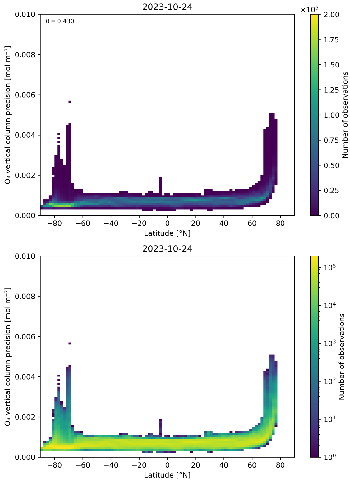
Figure 37: Scatter density plot of “Latitude” against “O 3 vertical column precision” for 2023-10-23 to 2023-10-25.
