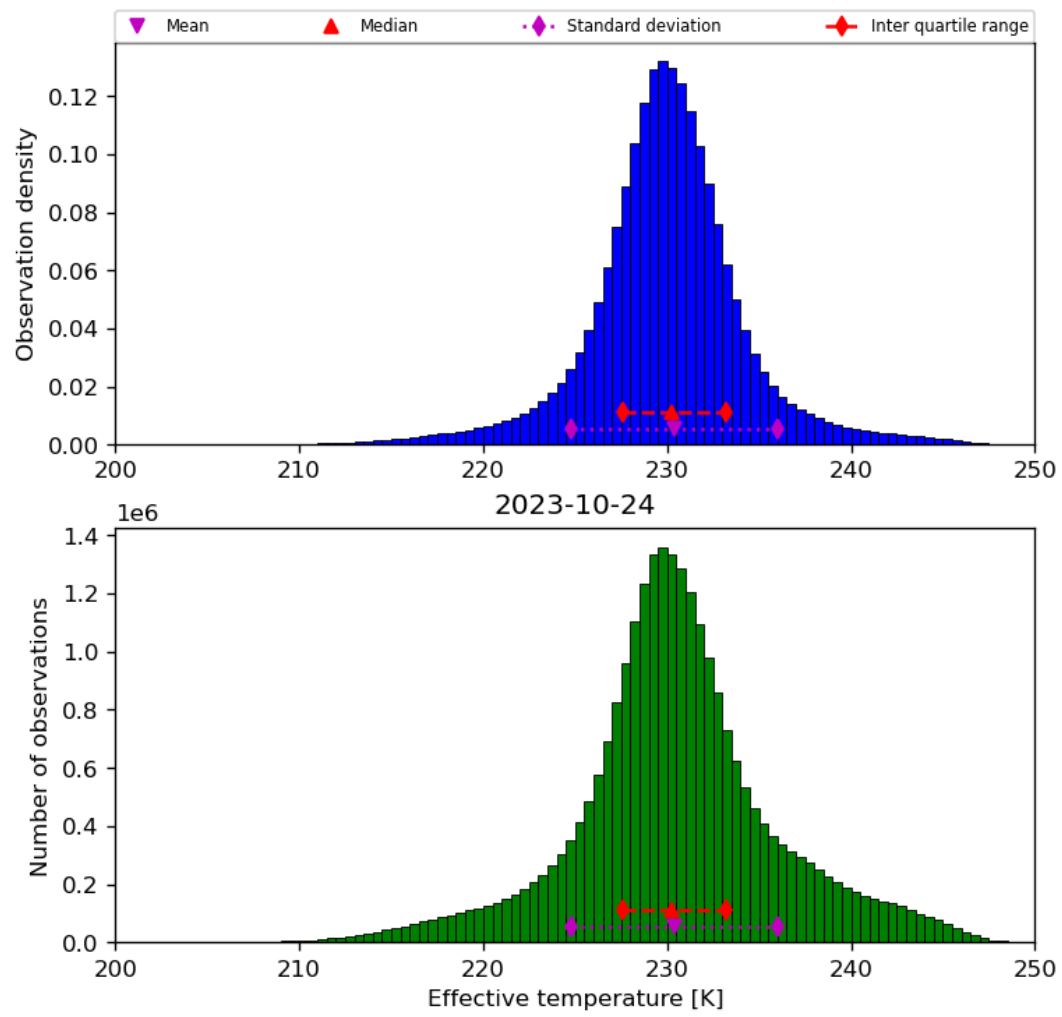
Figure 24: Histogram of “Effective temperature” for 2023-10-23 to 2023-10-25
