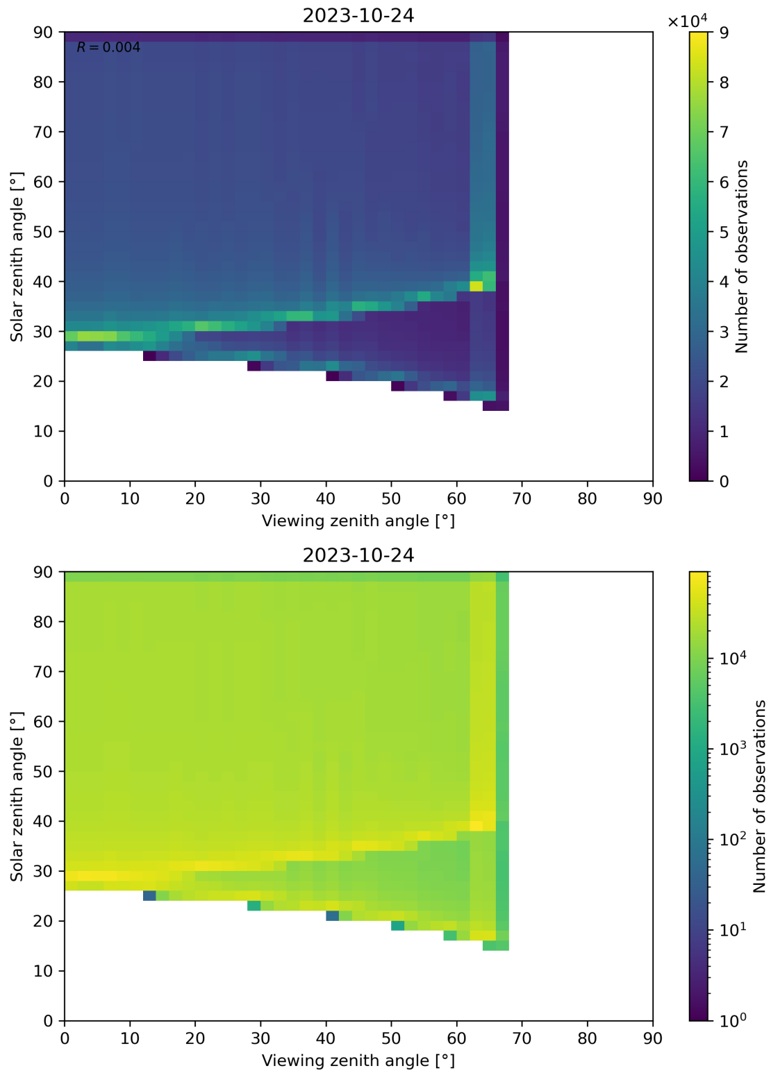
Figure 54: Scatter density plot of “Viewing zenith angle” against “Solar zenith angle” for 2023-10-23 to 2023-10-25.
