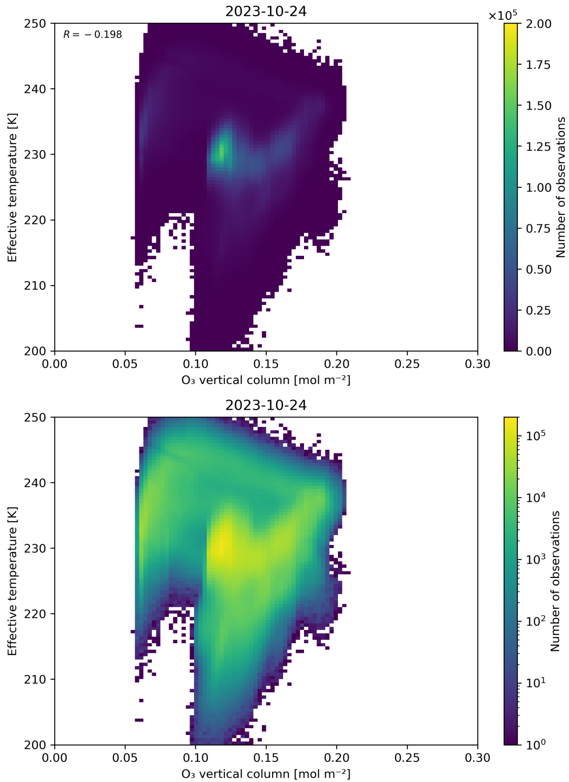
Figure 39: Scatter density plot of “O 3 vertical column” against “Effective temperature” for 2023-10-23 to 2023-10-25.
