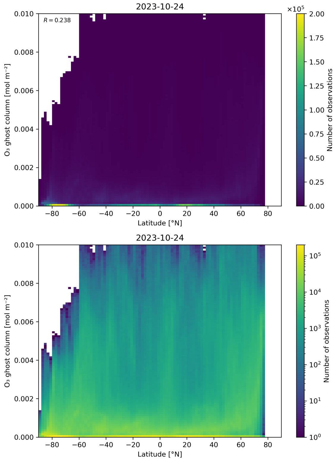
Figure 35: Scatter density plot of “Latitude” against “O 3 ghost column” for 2023-10-23 to 2023-10-25.
