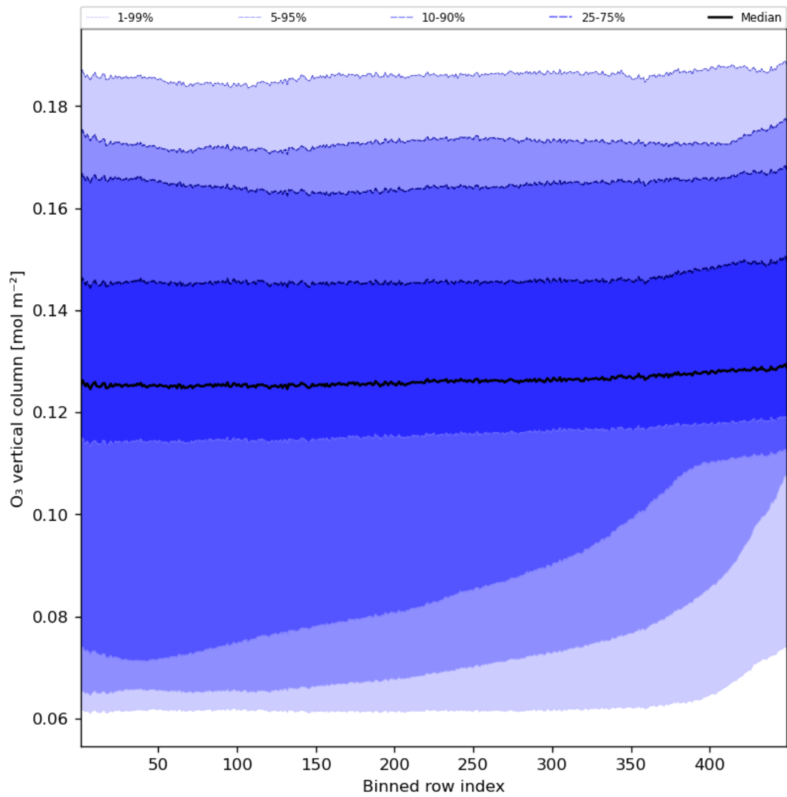
Figure 28: Along track statistics of “O 3 vertical column” for 2023-10-23 to 2023-10-25
