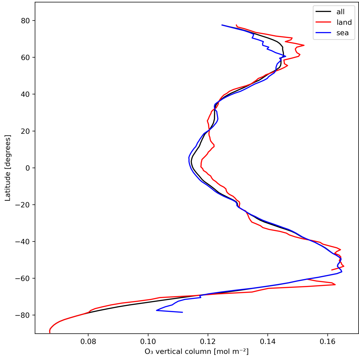
Figure 14: Zonal average of “O 3 vertical column” for 2023-10-23 to 2023-10-25.
