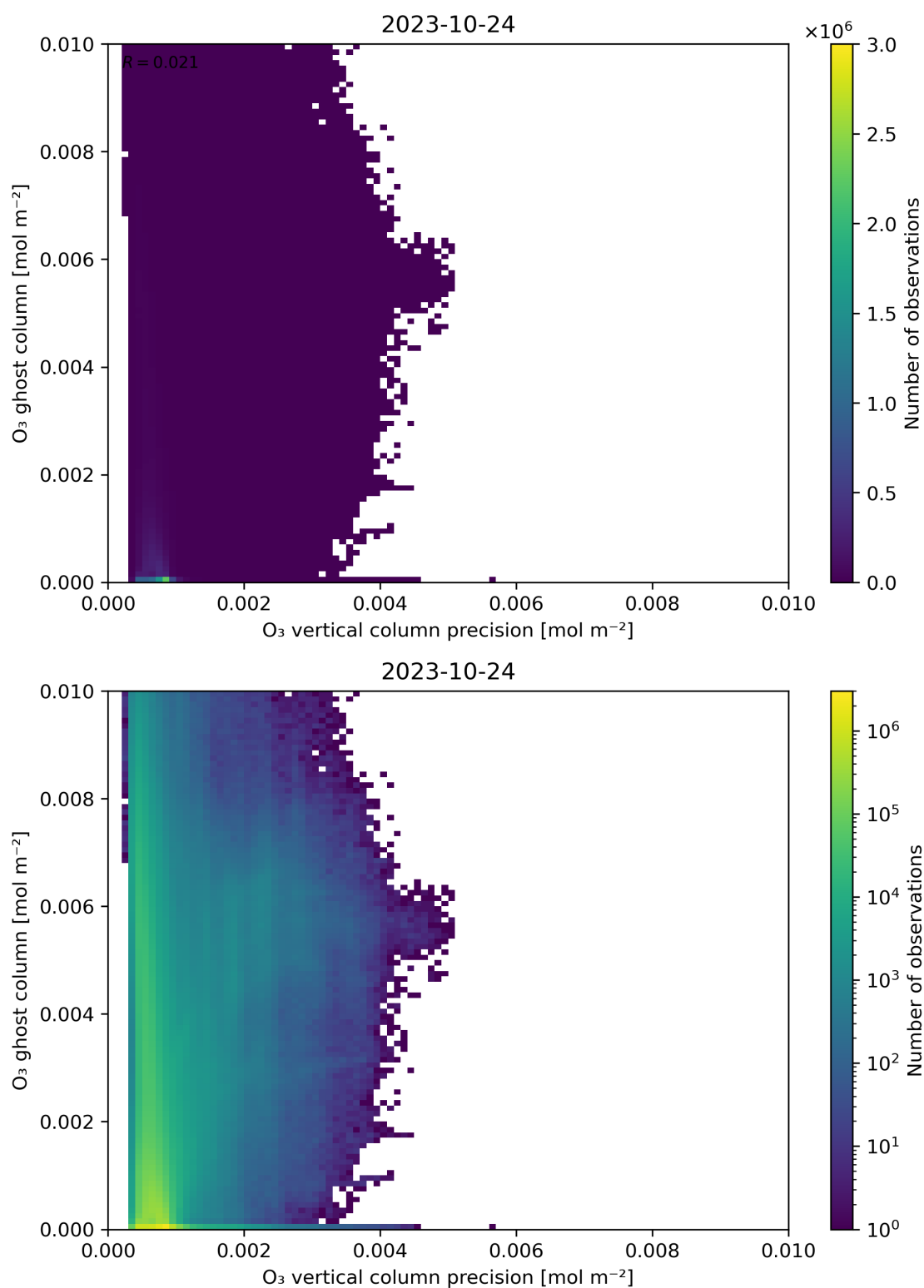
Figure 43: Scatter density plot of “ \text{O}_3 vertical column precision” against “ \text{O}_3 ghost column” for 2023-10-23 to 2023-10-25.
