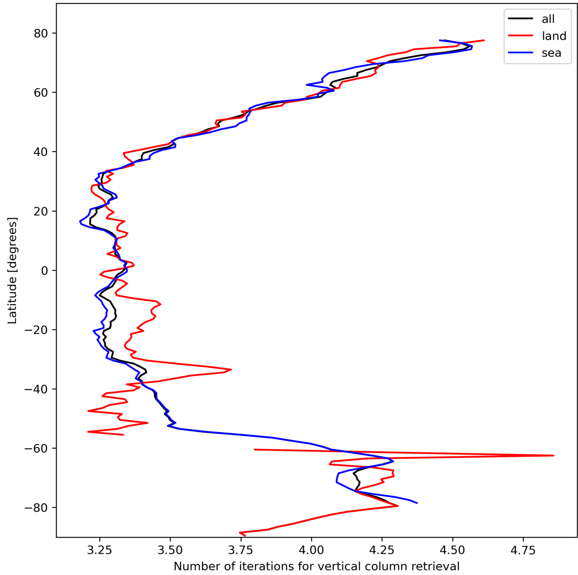
Figure 19: Zonal average of “Number of iterations for vertical column retrieval” for 2023-10-23 to 2023-10-25.
