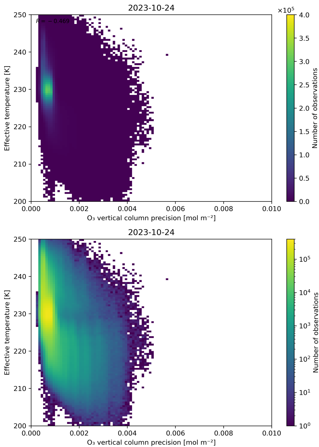
Figure 42: Scatter density plot of “O 3 vertical column precision” against “Effective temperature” for 2023-10-23 to 2023-10-25.
