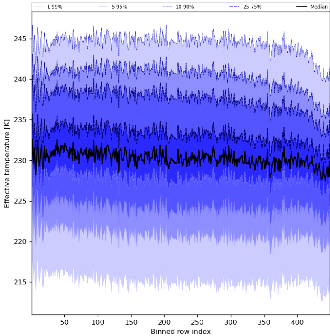
Figure 31: Along track statistics of “Effective temperature” for 2023-10-23 to 2023-10-25
