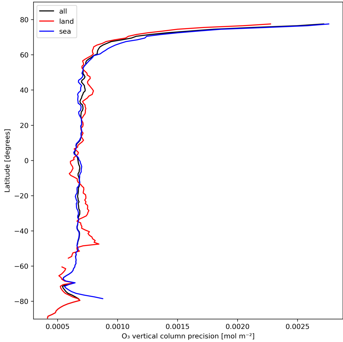
Figure 15: Zonal average of “O 3 vertical column precision” for 2023-10-23 to 2023-10-25.
