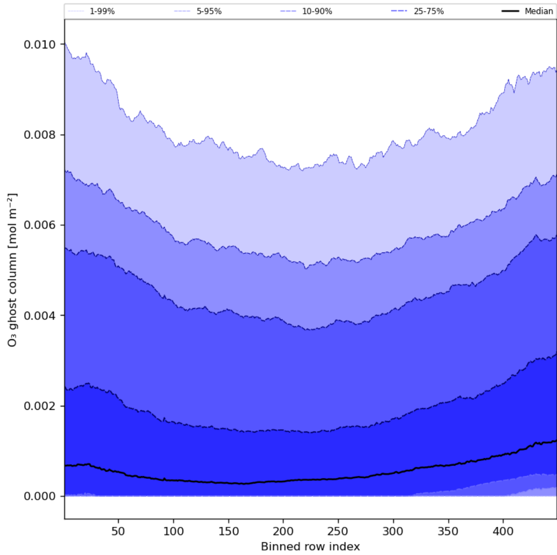
Figure 32: Along track statistics of “O 3 ghost column” for 2023-10-23 to 2023-10-25
