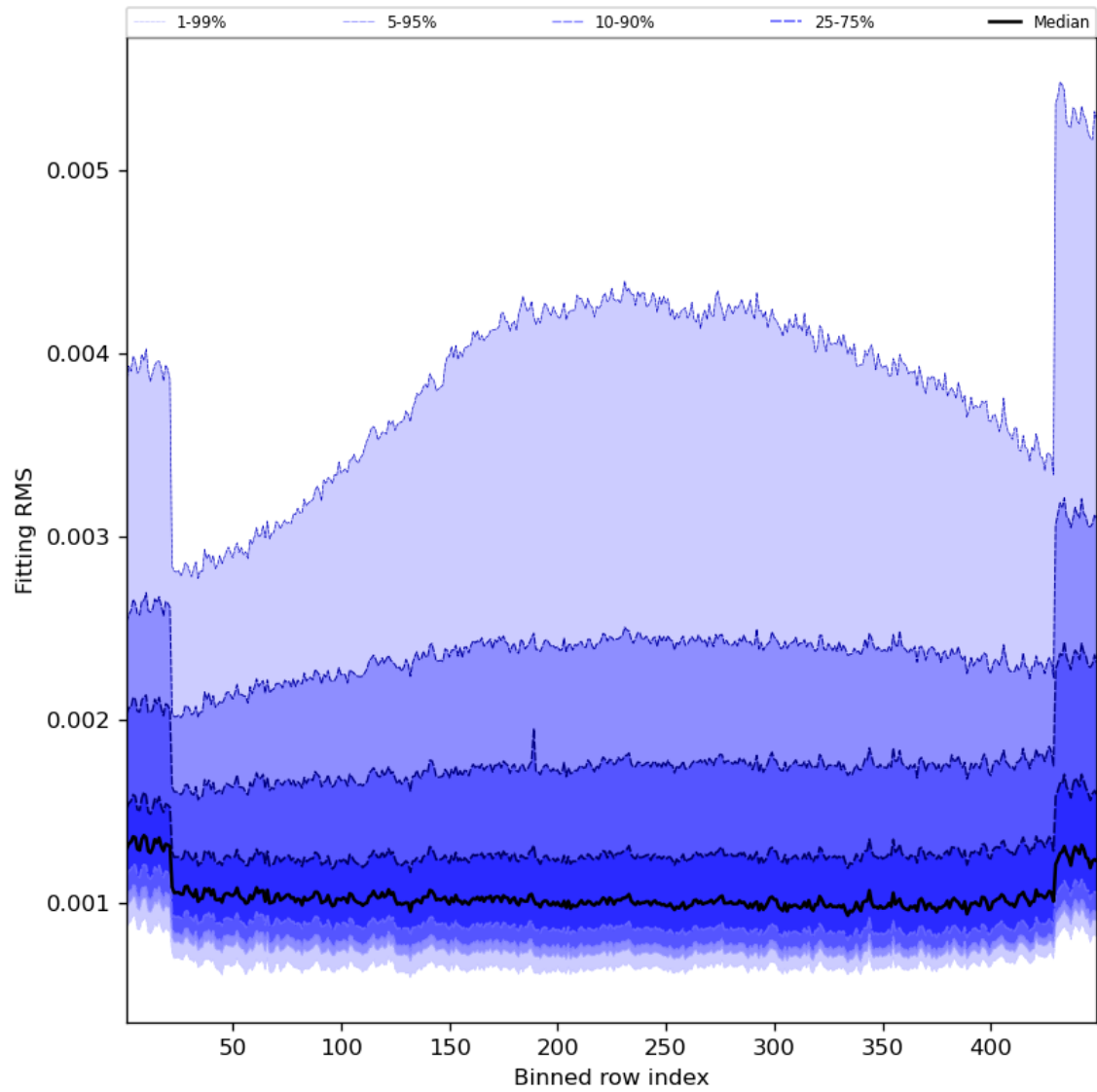
Figure 30: Along track statistics of “Fitting RMS” for 2023-10-23 to 2023-10-25
