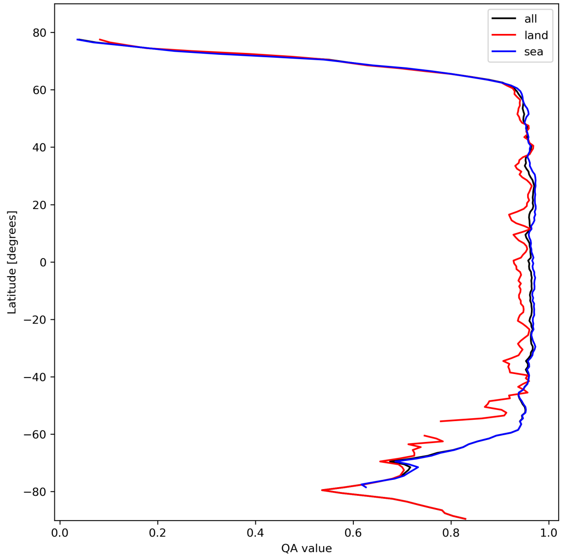
Figure 13: Zonal average of “QA value” for 2023-10-23 to 2023-10-25.
