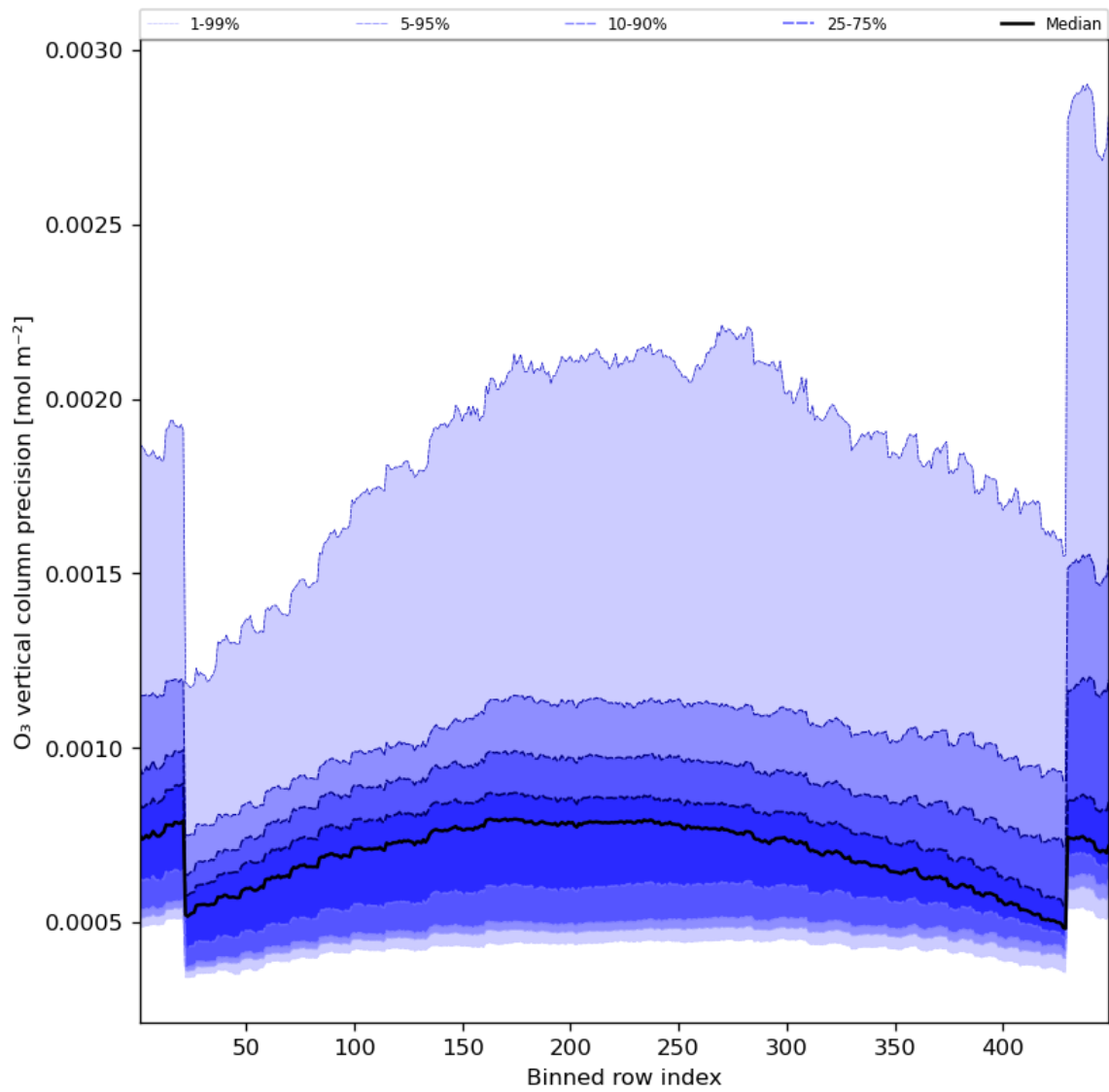
Figure 29: Along track statistics of “O 3 vertical column precision” for 2023-10-23 to 2023-10-25
