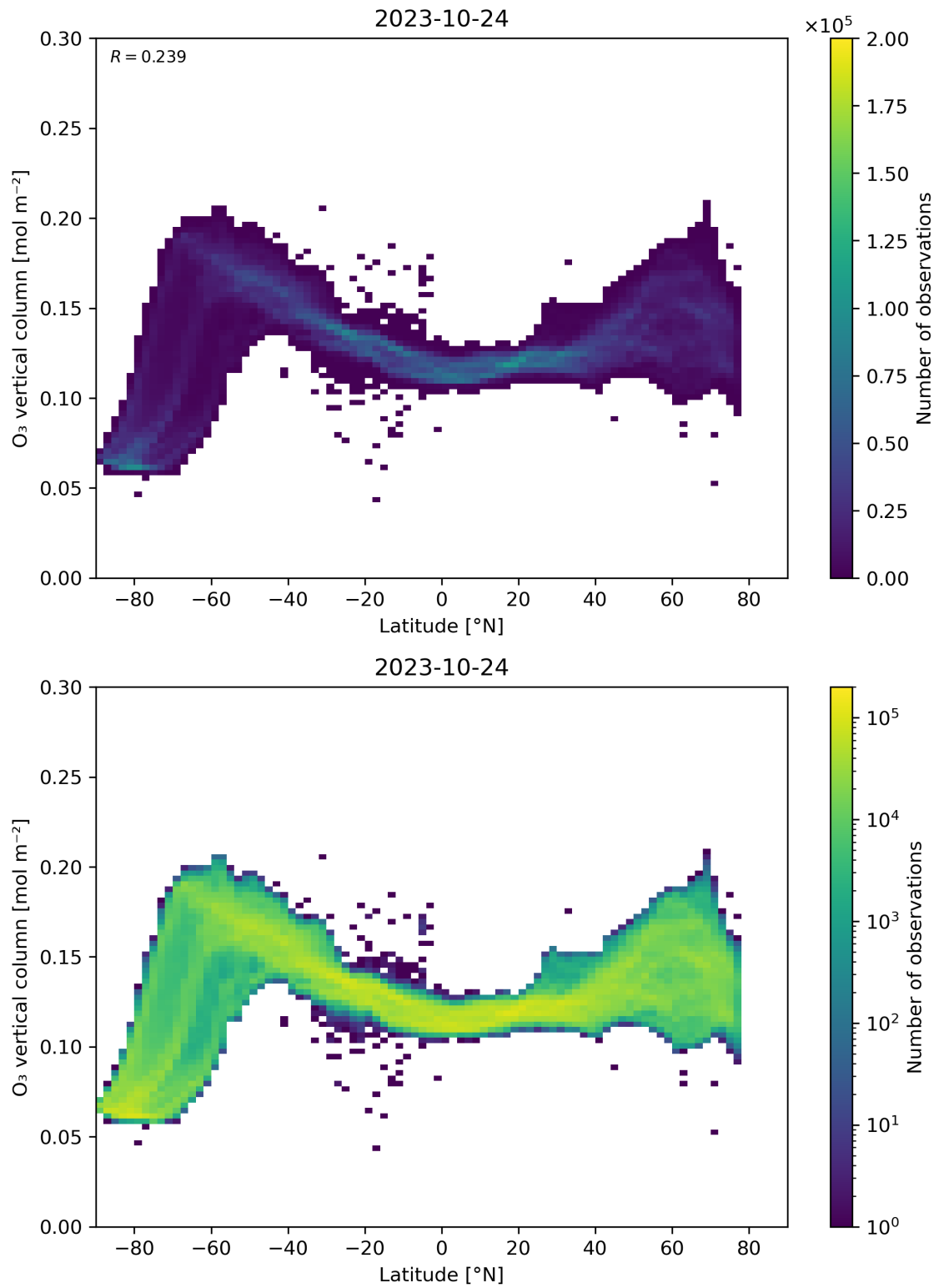
Figure 36: Scatter density plot of “Latitude” against “O 3 vertical column” for 2023-10-23 to 2023-10-25.
