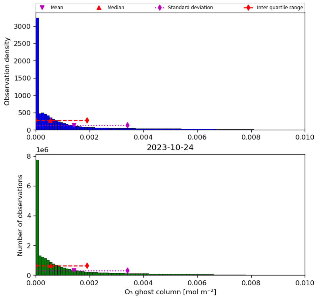
Figure 25: Histogram of “O 3 ghost column” for 2023-10-23 to 2023-10-25
