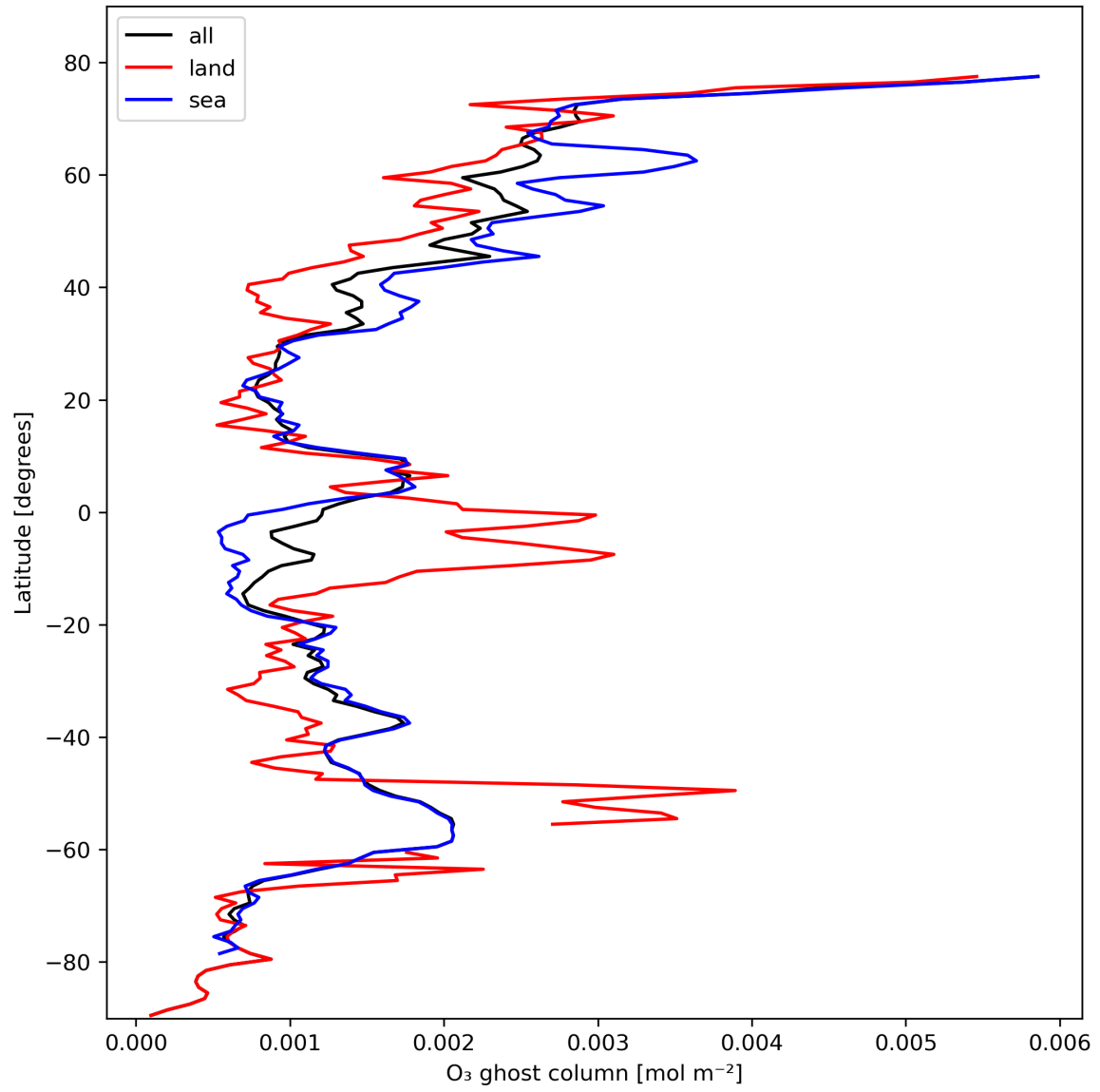
Figure 18: Zonal average of “O 3 ghost column” for 2023-10-23 to 2023-10-25.
