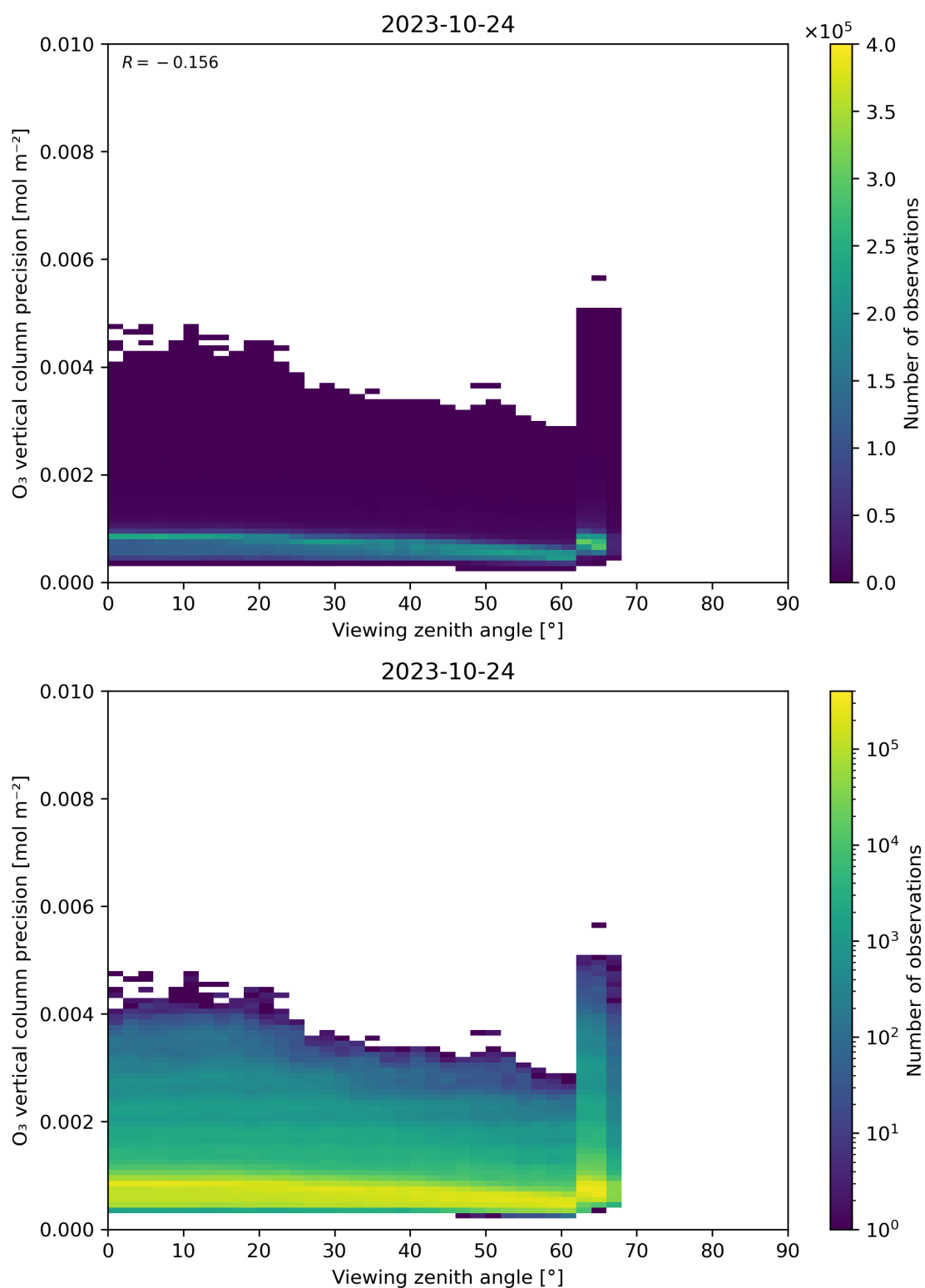
Figure 53: Scatter density plot of “Viewing zenith angle” against “O 3 vertical column precision” for 2023-10-23 to 2023-10-25.
