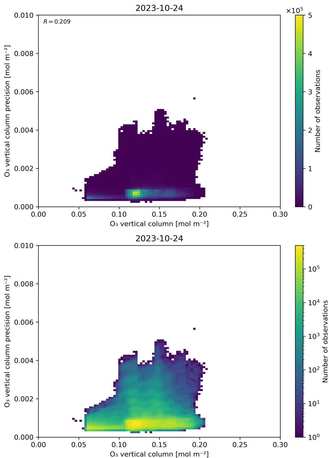
Figure 41: Scatter density plot of “O 3 vertical column” against “O 3 vertical column precision” for 2023-10-23 to 2023-10-25.
