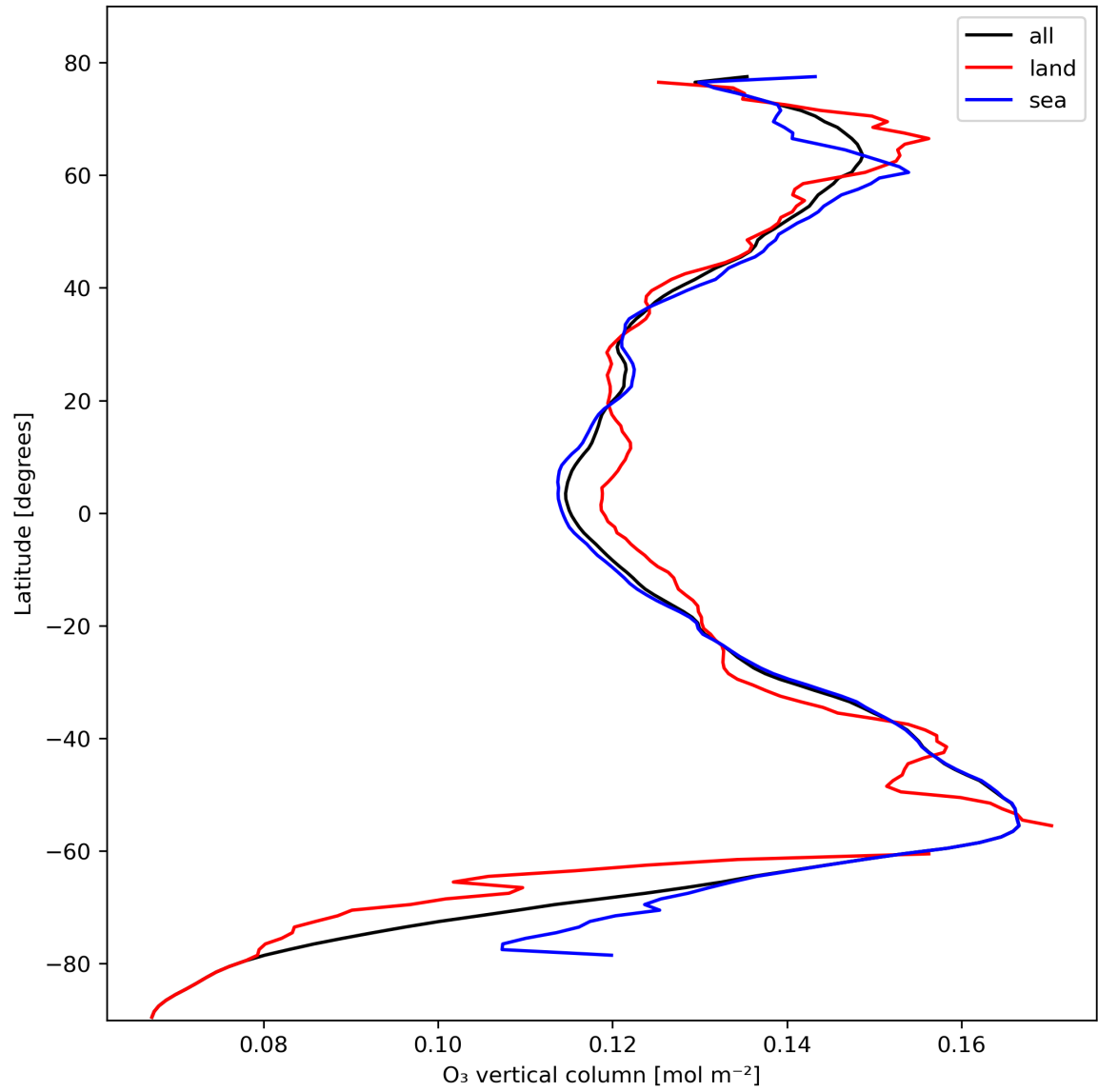
Figure 14: Zonal average of “O 3 vertical column” for 2023-10-24 to 2023-10-26.
