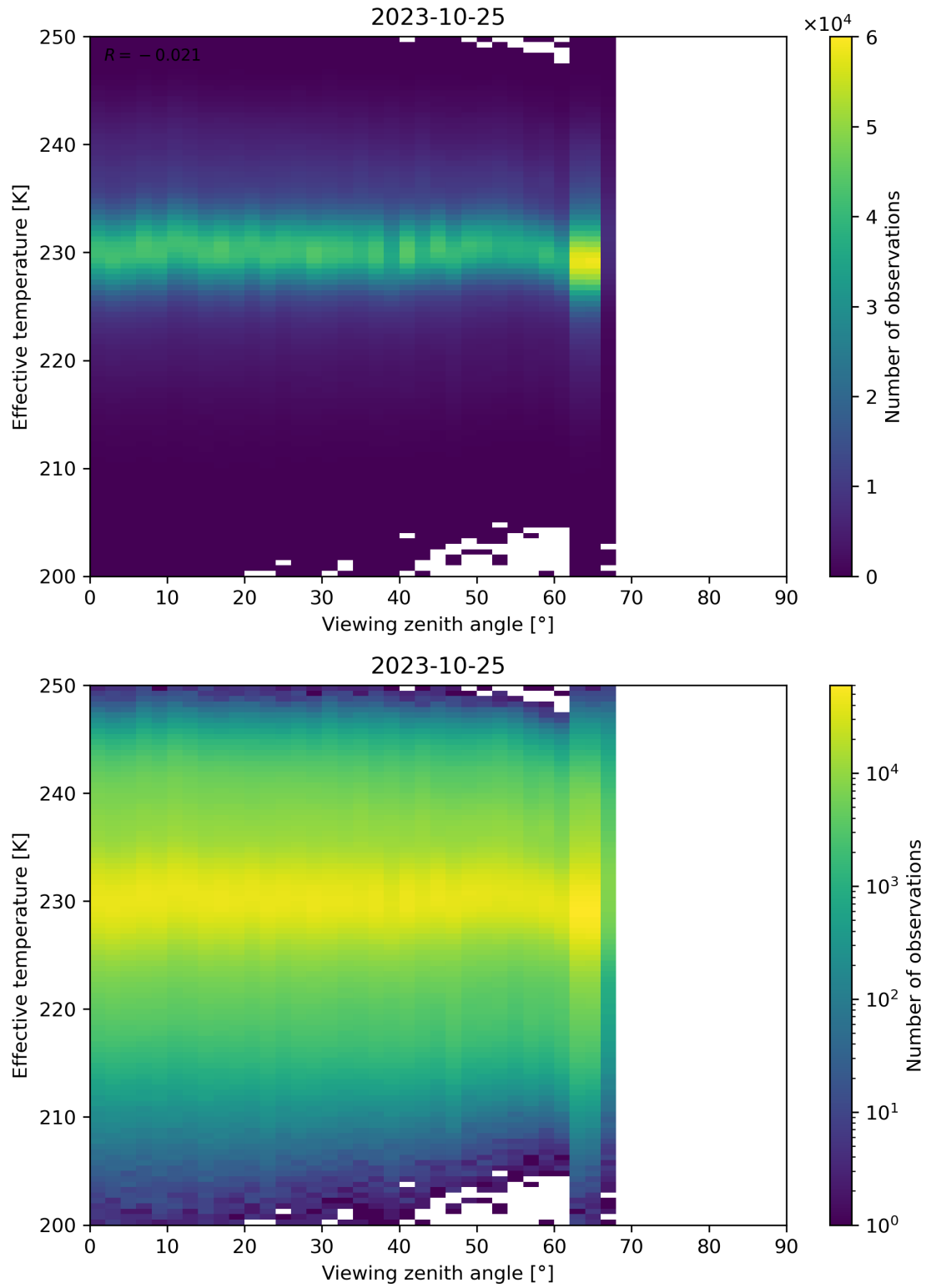
Figure 50: Scatter density plot of “Viewing zenith angle” against “Effective temperature” for 2023-10-24 to 2023-10-26.
