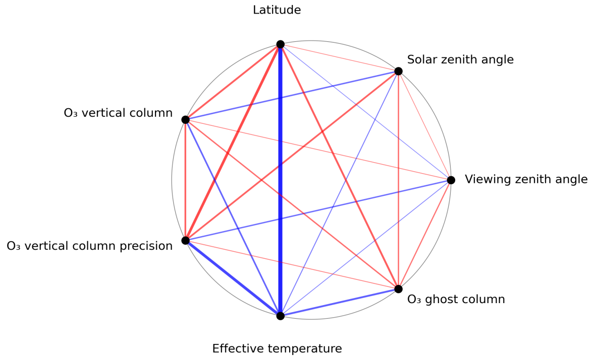
Figure 1: Map of correlation graph for 2023-10-24 to 2023-10-26.
