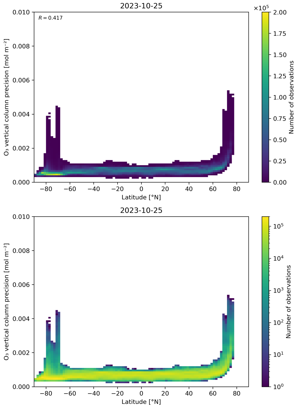
Figure 37: Scatter density plot of “Latitude” against “O 3 vertical column precision” for 2023-10-24 to 2023-10-26.
