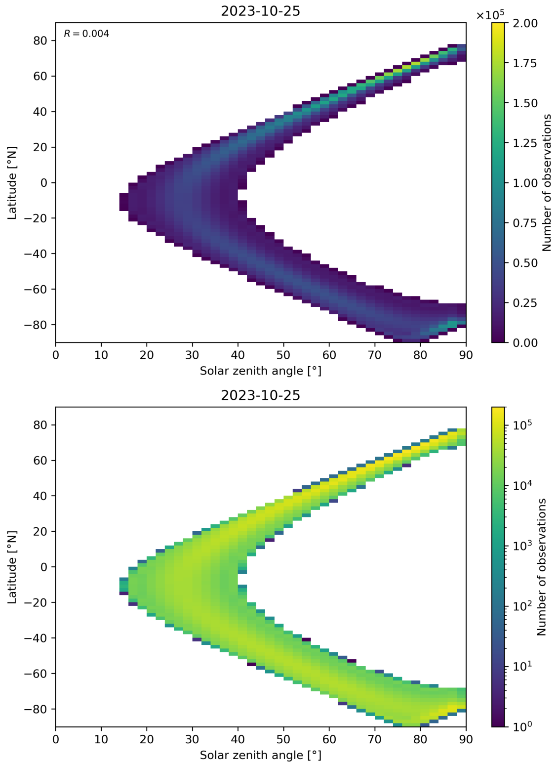
Figure 44: Scatter density plot of “Solar zenith angle” against “Latitude” for 2023-10-24 to 2023-10-26.
