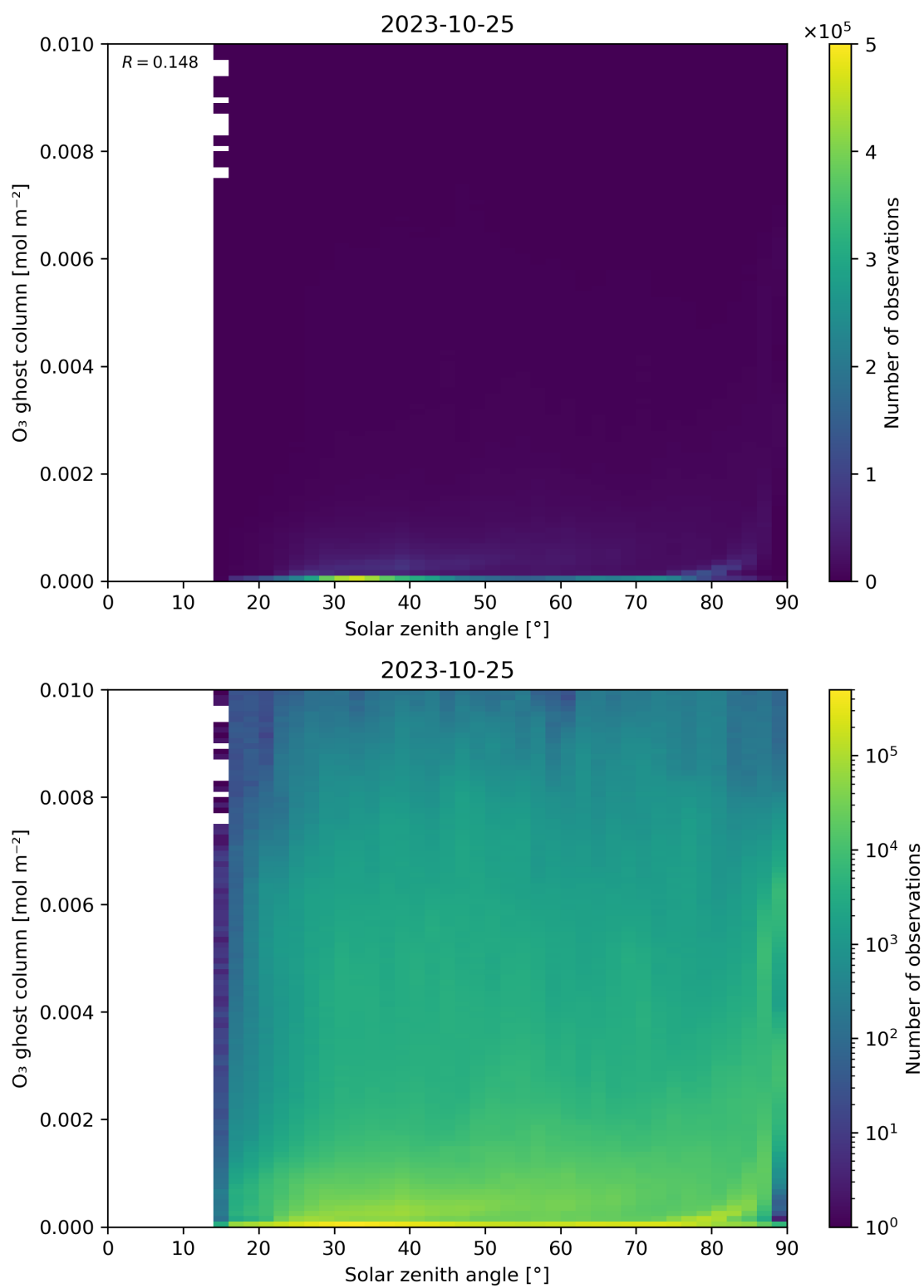
Figure 46: Scatter density plot of “Solar zenith angle” against “O 3 ghost column” for 2023-10-24 to 2023-10-26.
