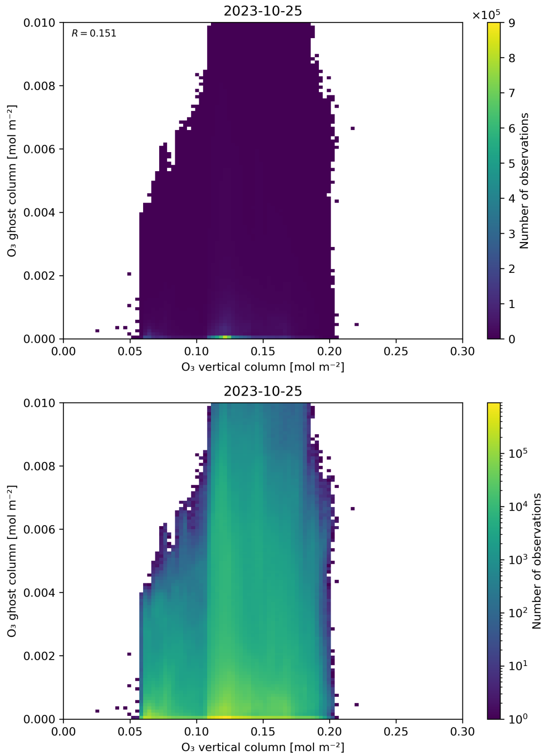
Figure 40: Scatter density plot of “O 3 vertical column” against “O 3 ghost column” for 2023-10-24 to 2023-10-26.
