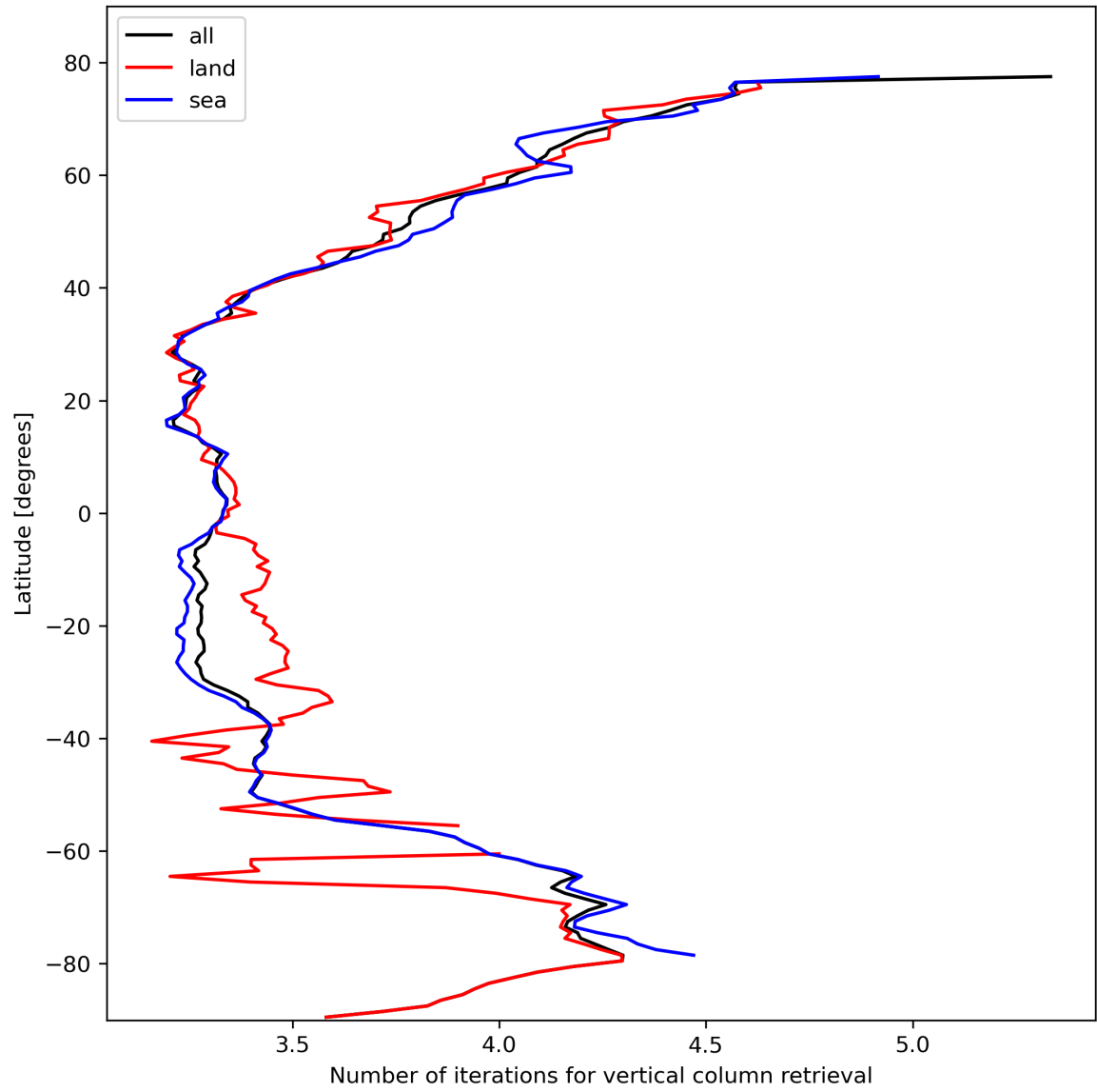
Figure 19: Zonal average of “Number of iterations for vertical column retrieval” for 2023-10-24 to 2023-10-26.
