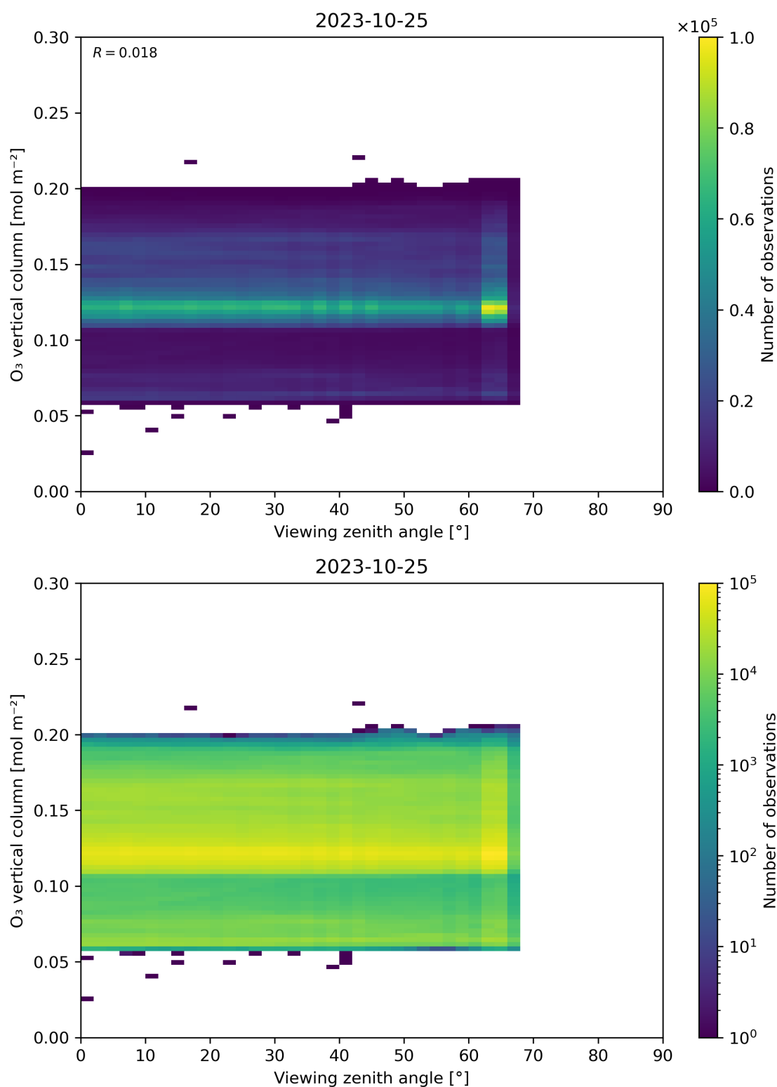
Figure 52: Scatter density plot of “Viewing zenith angle” against “O 3 vertical column” for 2023-10-24 to 2023-10-26.
