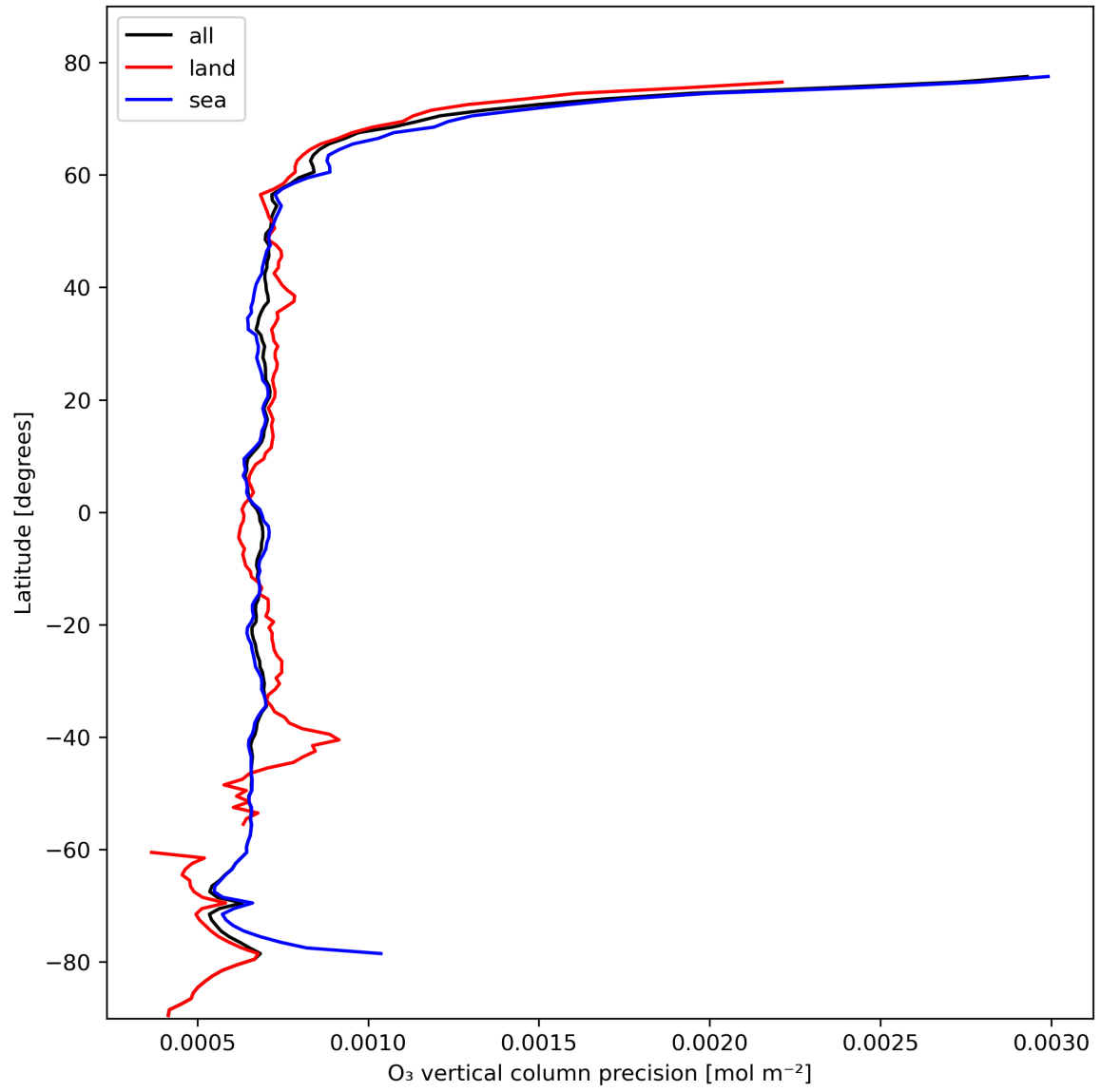
Figure 15: Zonal average of "O 3 vertical column precision" for 2023-10-24 to 2023-10-26.
