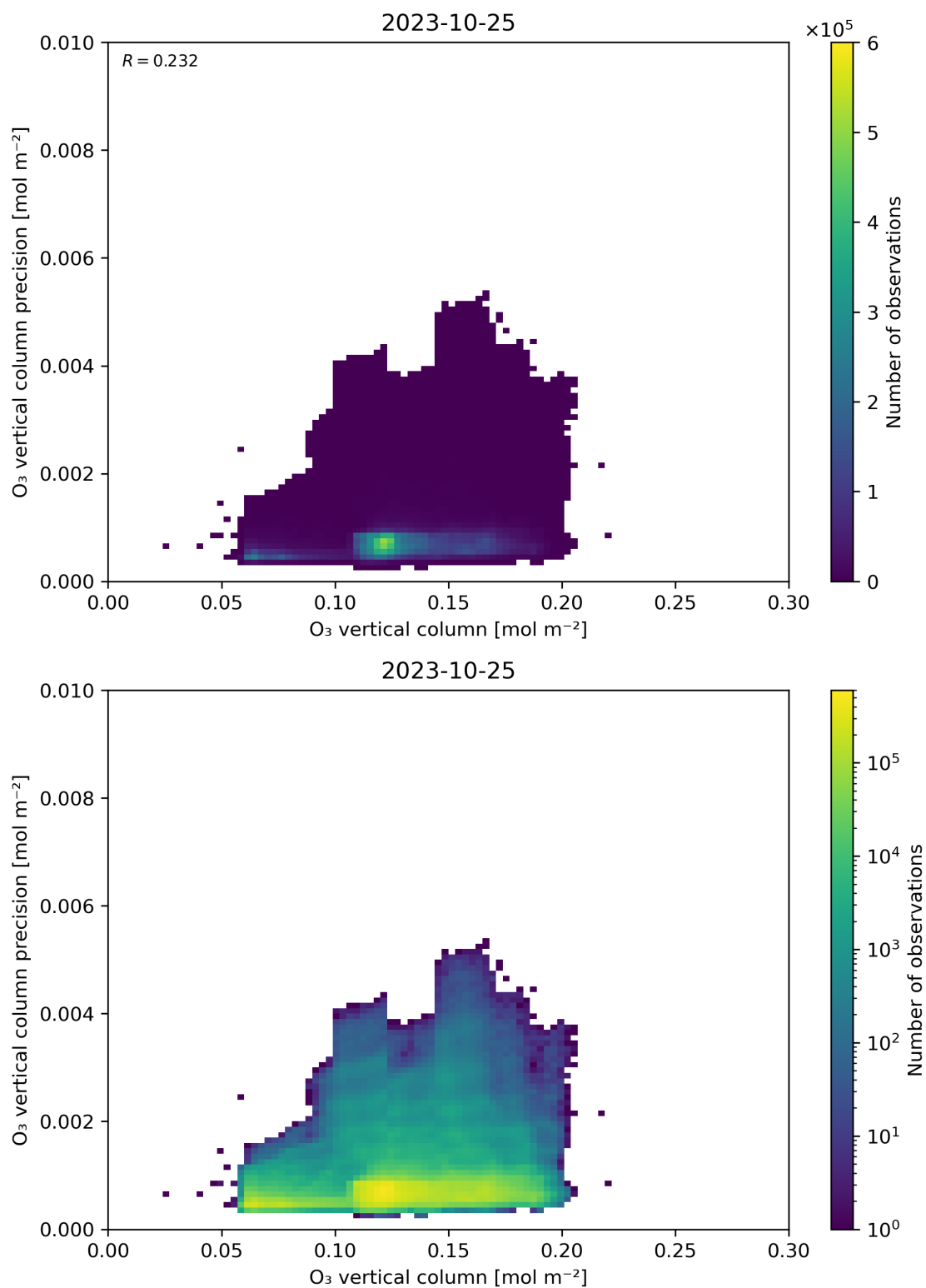
Figure 41: Scatter density plot of “O 3 vertical column” against “O 3 vertical column precision” for 2023-10-24 to 2023-10-26.
