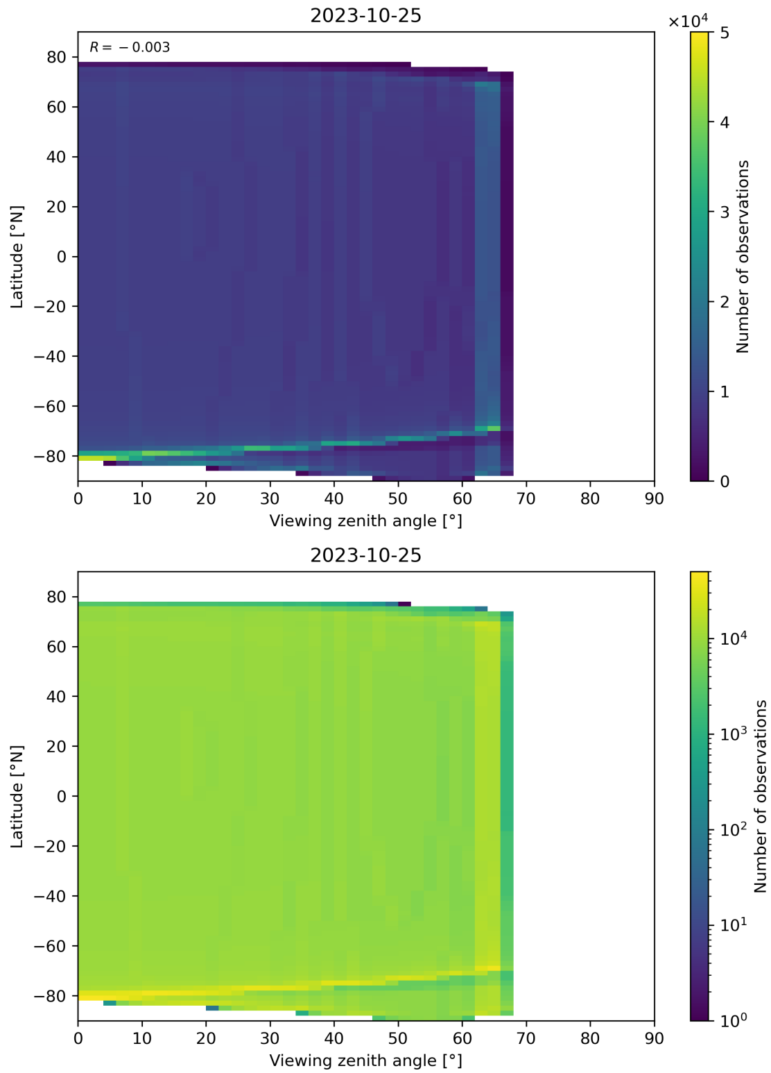
Figure 49: Scatter density plot of “Viewing zenith angle” against “Latitude” for 2023-10-24 to 2023-10-26.
