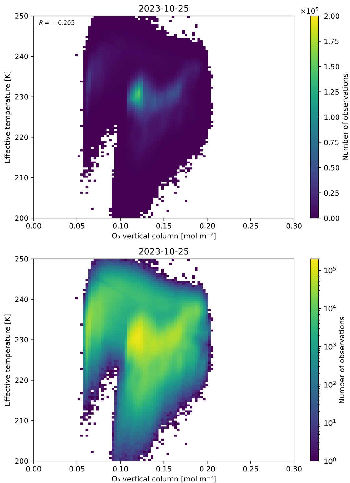
Figure 39: Scatter density plot of “O 3 vertical column” against “Effective temperature” for 2023-10-24 to 2023-10-26.
