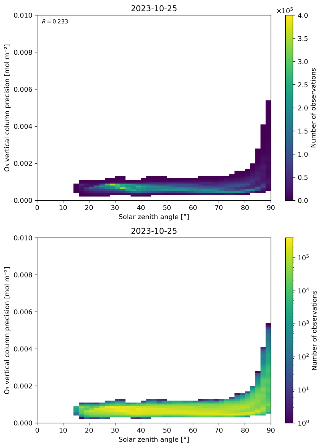
Figure 48: Scatter density plot of “Solar zenith angle” against “O 3 vertical column precision” for 2023-10-24 to 2023-10-26.
