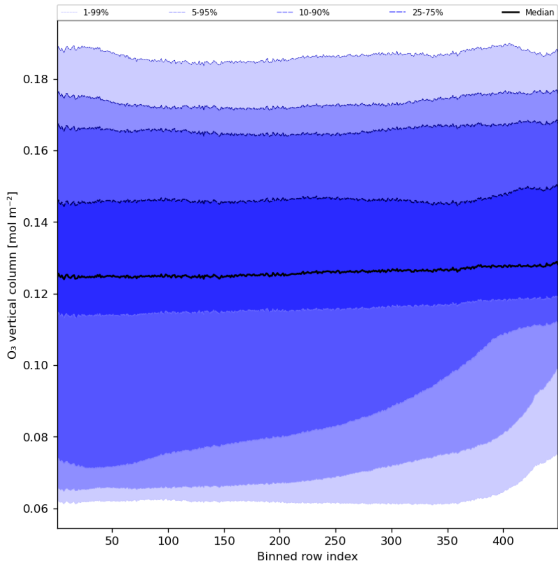
Figure 28: Along track statistics of “O 3 vertical column” for 2023-10-24 to 2023-10-26
