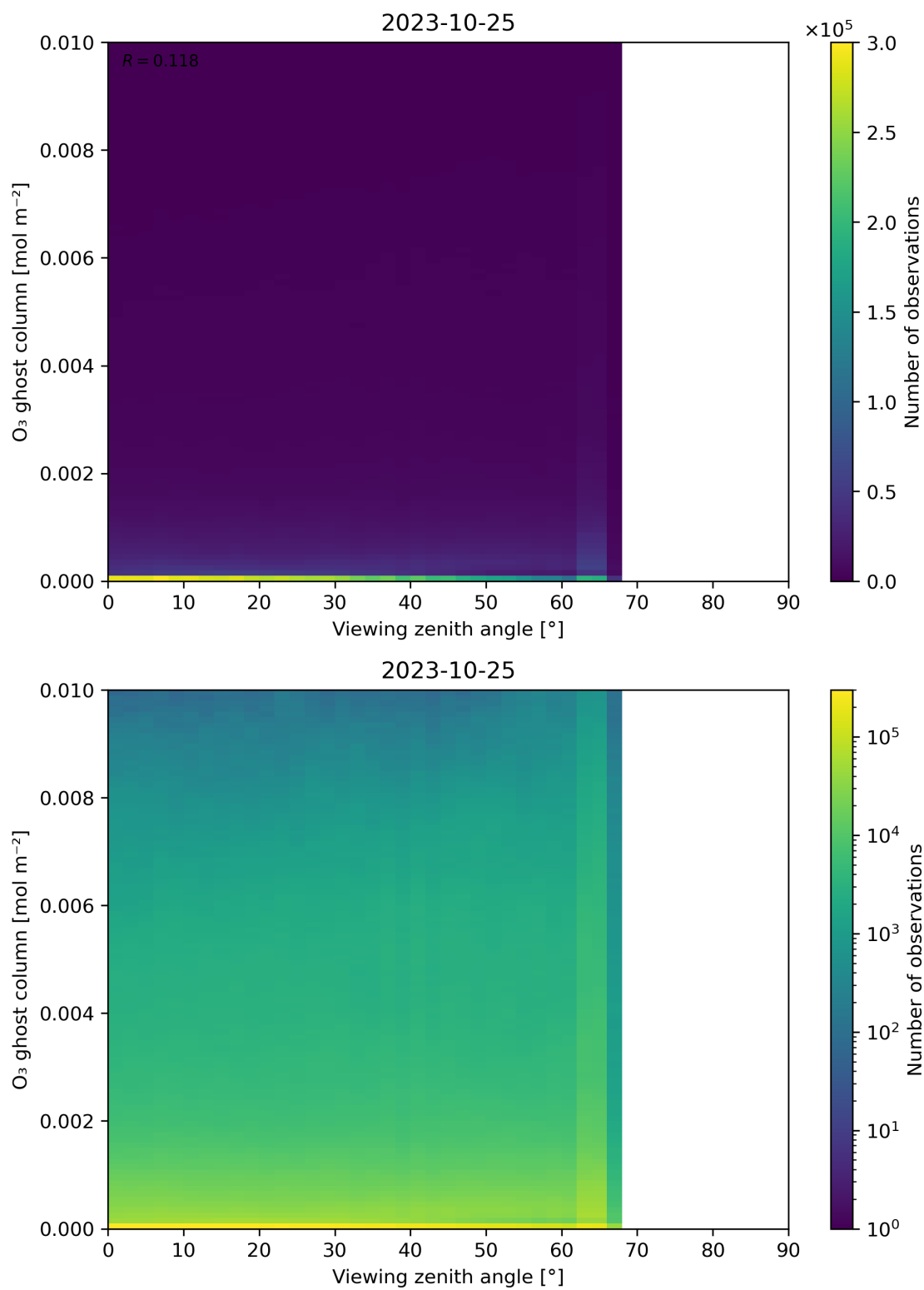
Figure 51: Scatter density plot of “Viewing zenith angle” against “O 3 ghost column” for 2023-10-24 to 2023-10-26.
