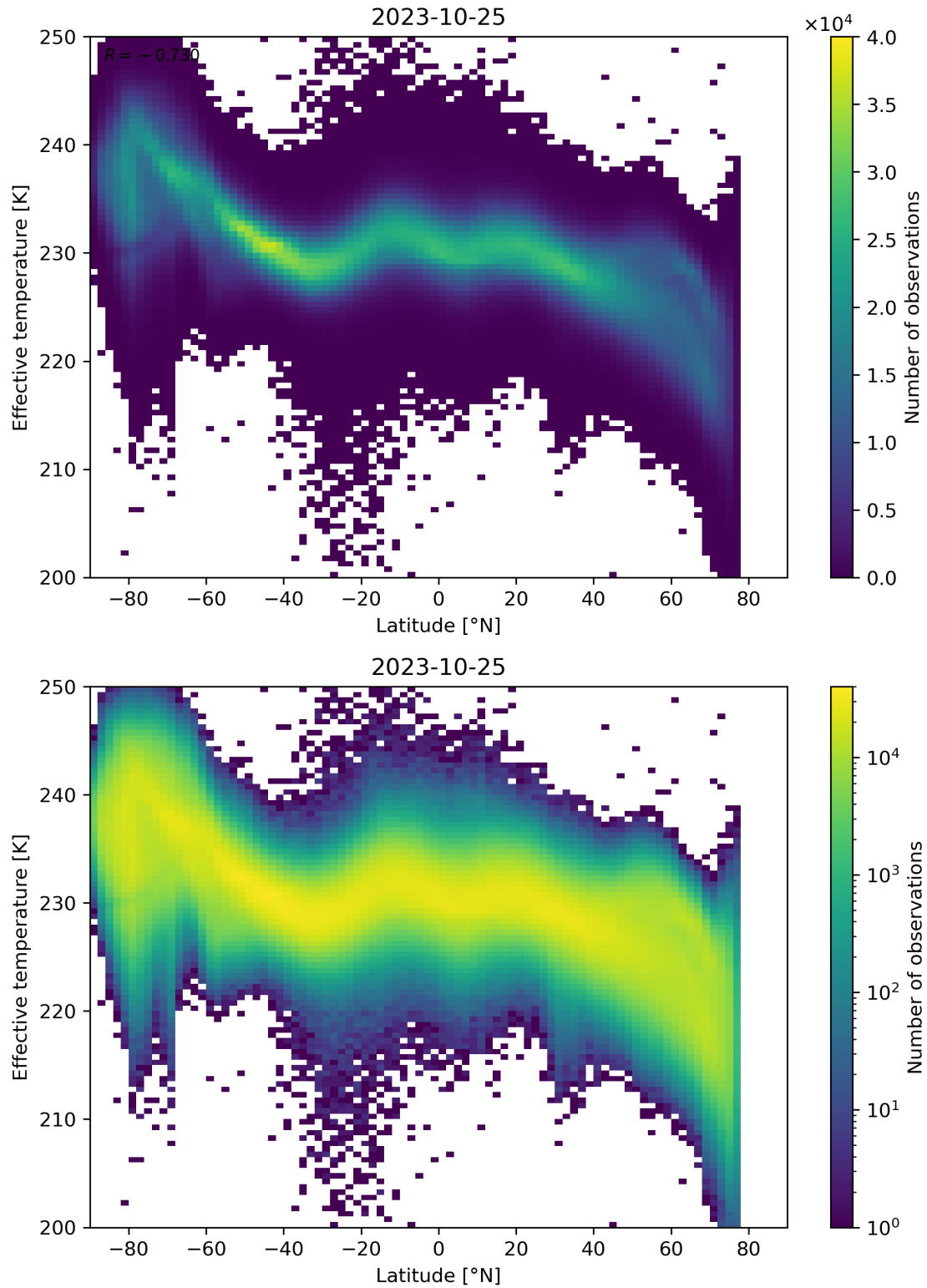
Figure 34: Scatter density plot of “Latitude” against “Effective temperature” for 2023-10-24 to 2023-10-26.
