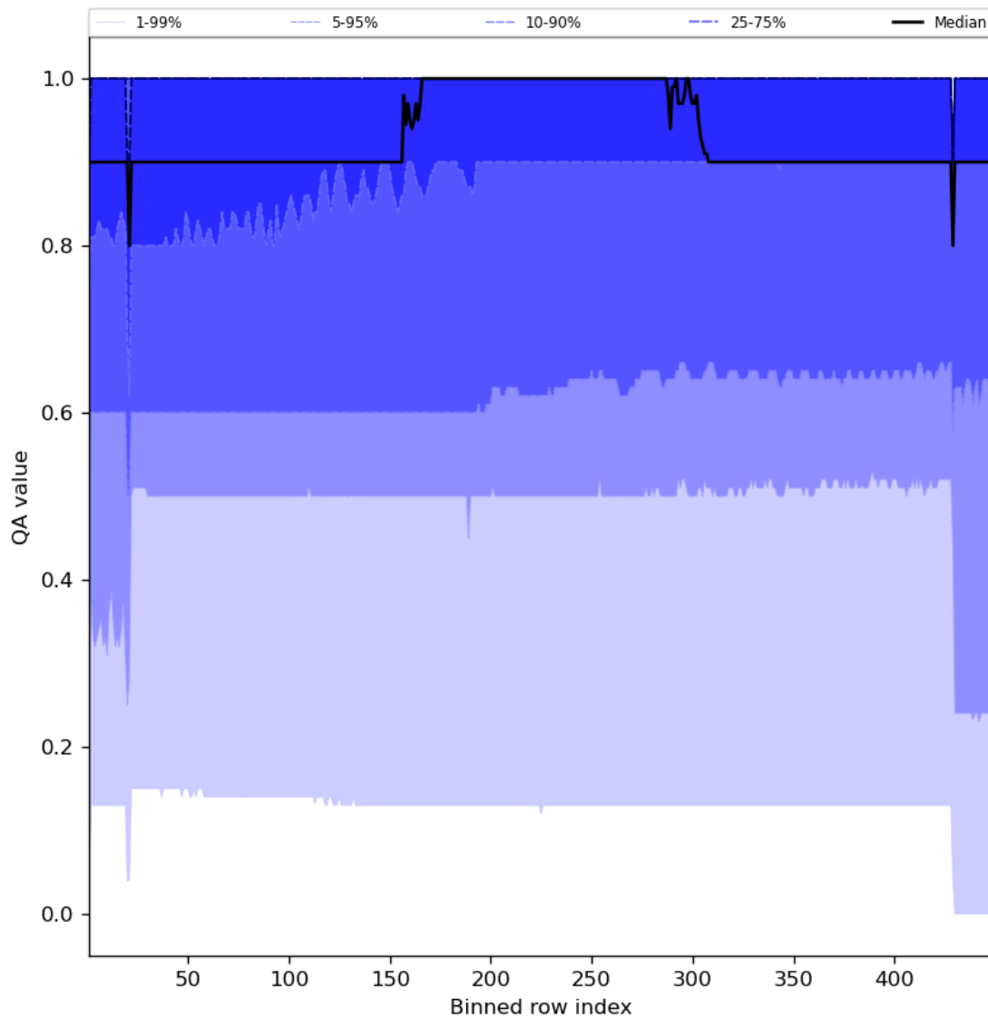
Figure 27: Along track statistics of “QA value” for 2023-10-24 to 2023-10-26
