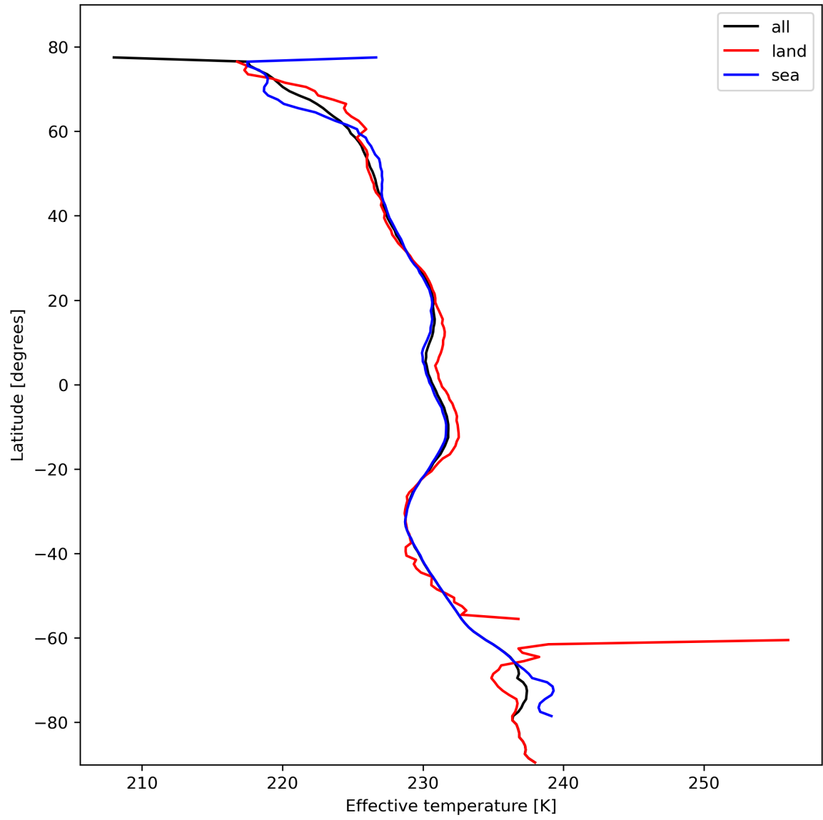
Figure 17: Zonal average of “Effective temperature” for 2023-10-24 to 2023-10-26.
