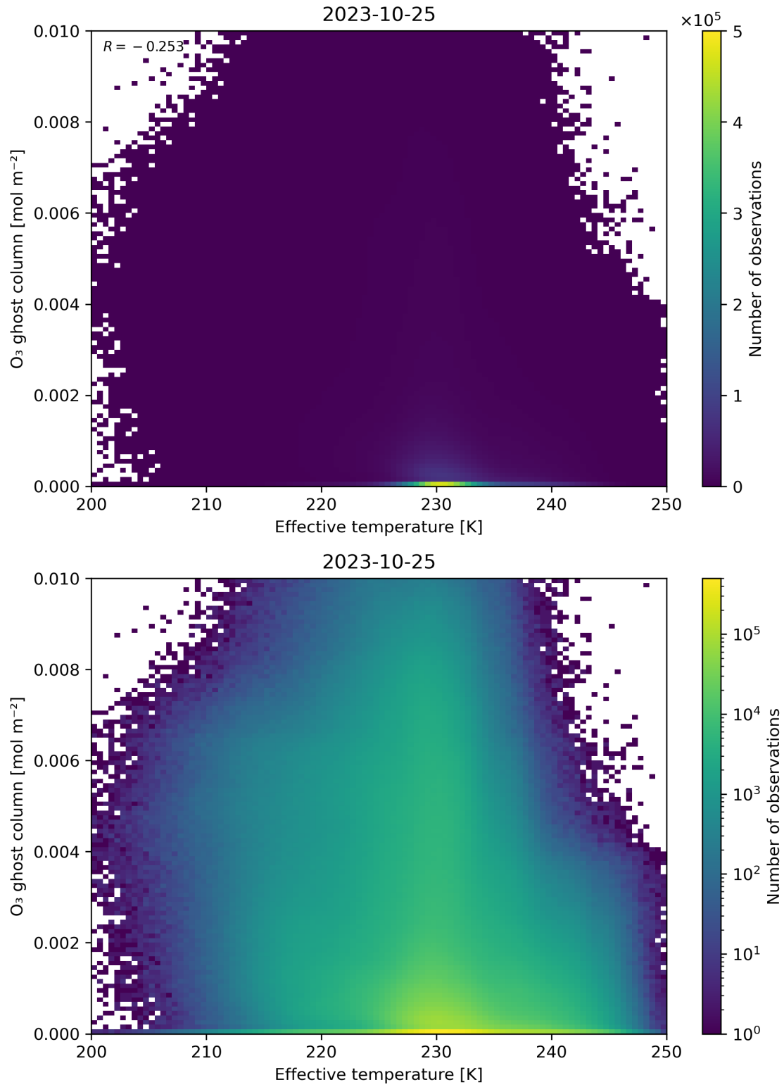
Figure 38: Scatter density plot of “Effective temperature” against “O 3 ghost column” for 2023-10-24 to 2023-10-26.
