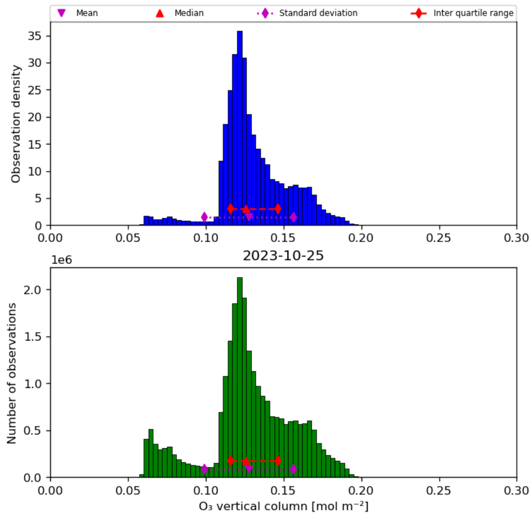
Figure 21: Histogram of “O 3 vertical column” for 2023-10-24 to 2023-10-26
