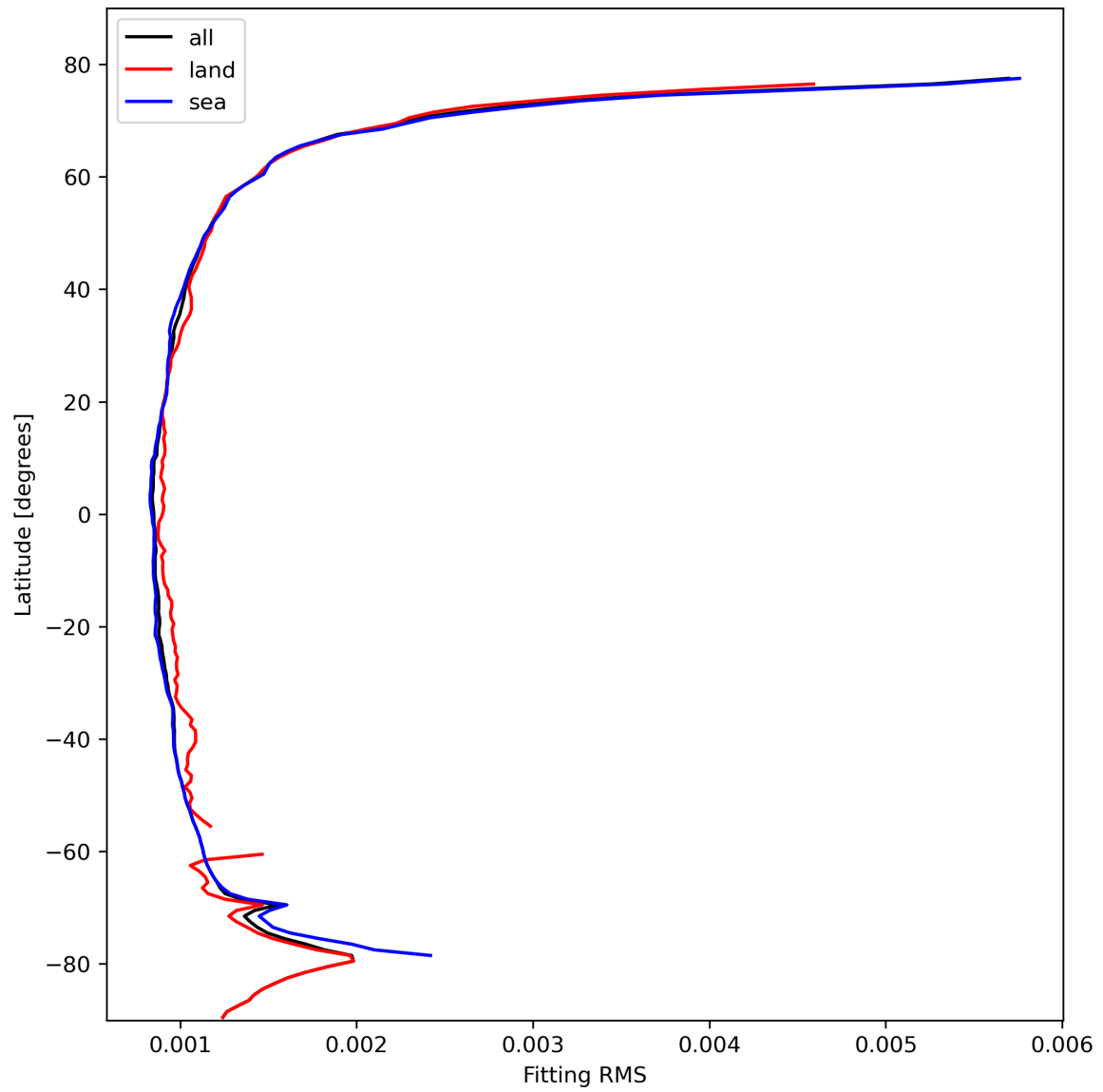
Figure 16: Zonal average of “Fitting RMS” for 2023-10-24 to 2023-10-26.
