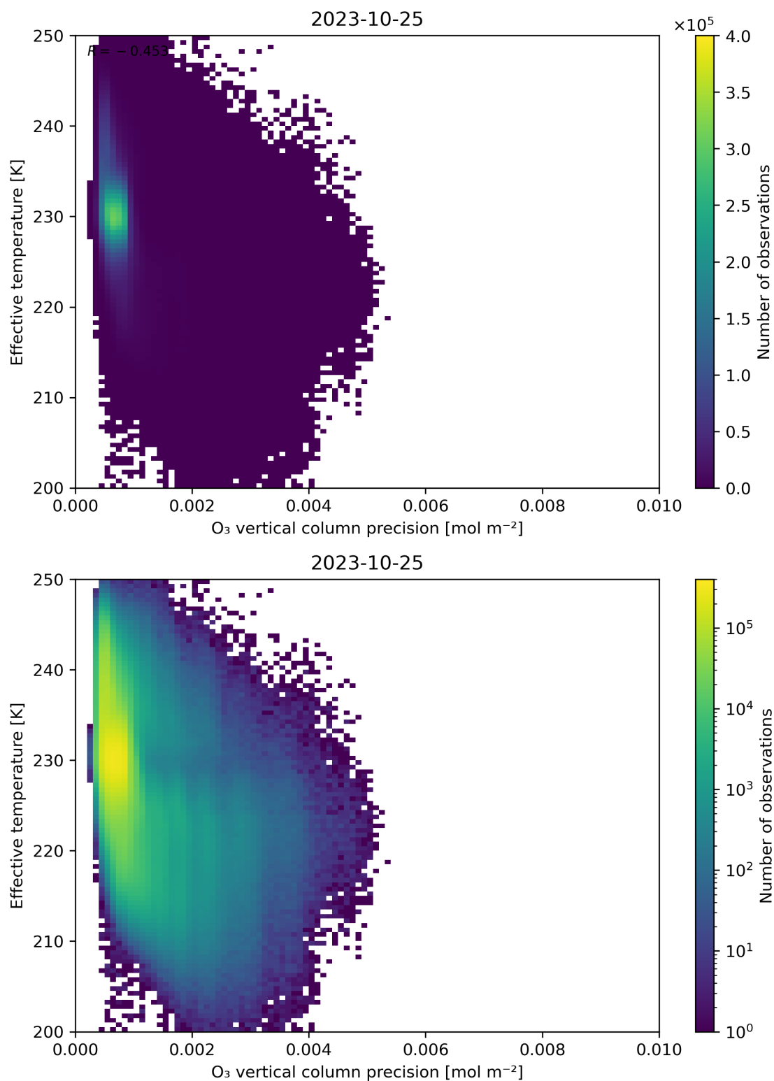
Figure 42: Scatter density plot of “O 3 vertical column precision” against “Effective temperature” for 2023-10-24 to 2023-10-26.
