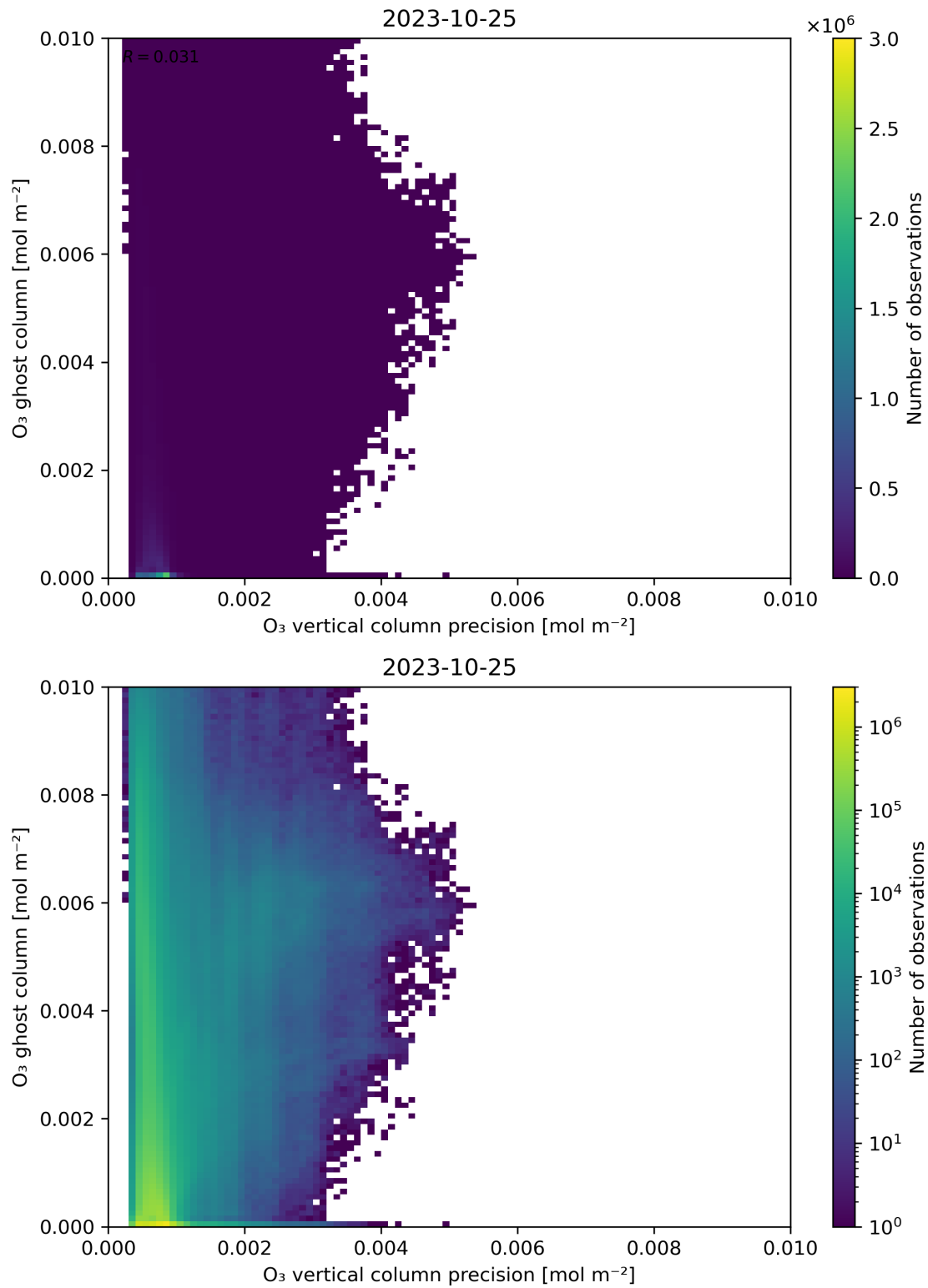
Figure 43: Scatter density plot of “O 3 vertical column precision” against “O 3 ghost column” for 2023-10-24 to 2023-10-26.
