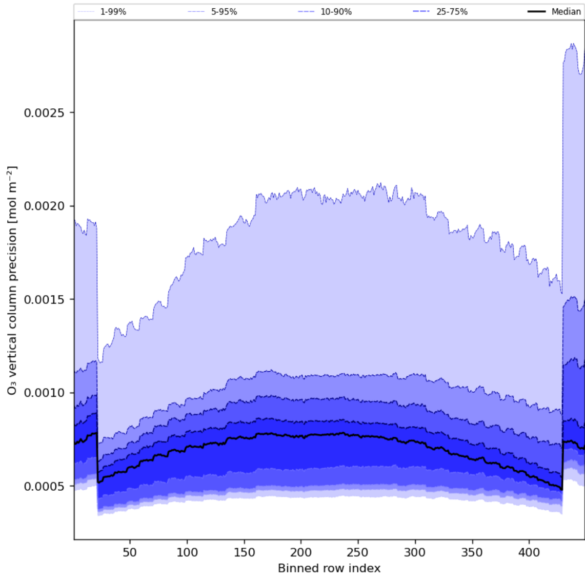
Figure 29: Along track statistics of “O 3 vertical column precision” for 2023-10-24 to 2023-10-26
