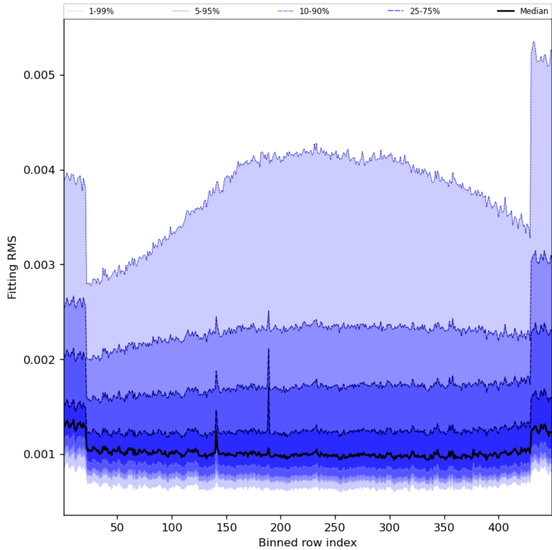
Figure 30: Along track statistics of “Fitting RMS” for 2023-10-24 to 2023-10-26
