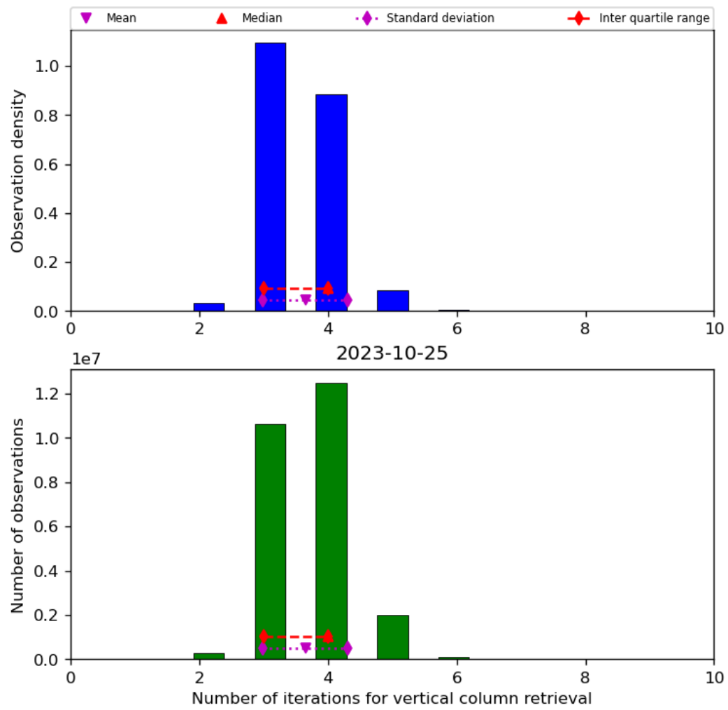
Figure 26: Histogram of “Number of iterations for vertical column retrieval” for 2023-10-24 to 2023-10-26
