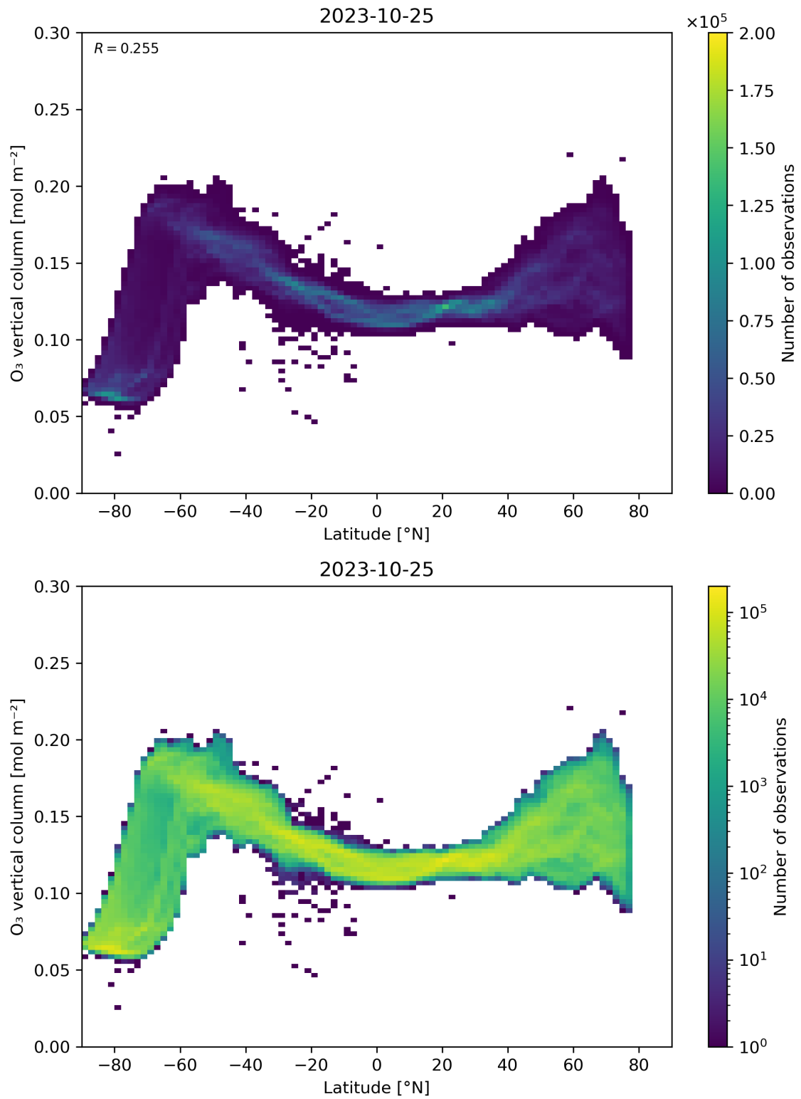
Figure 36: Scatter density plot of “Latitude” against “O 3 vertical column” for 2023-10-24 to 2023-10-26.
