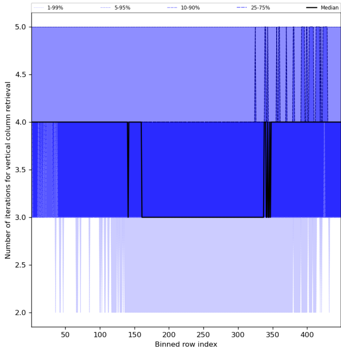
Figure 33: Along track statistics of “Number of iterations for vertical column retrieval” for 2023-10-24 to 2023-10-26
