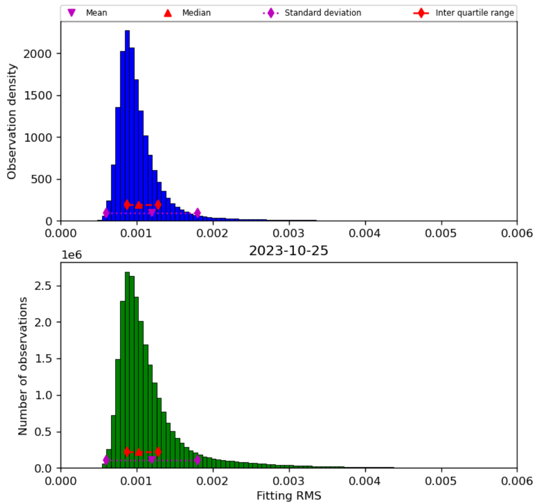
Figure 23: Histogram of “Fitting RMS” for 2023-10-24 to 2023-10-26
