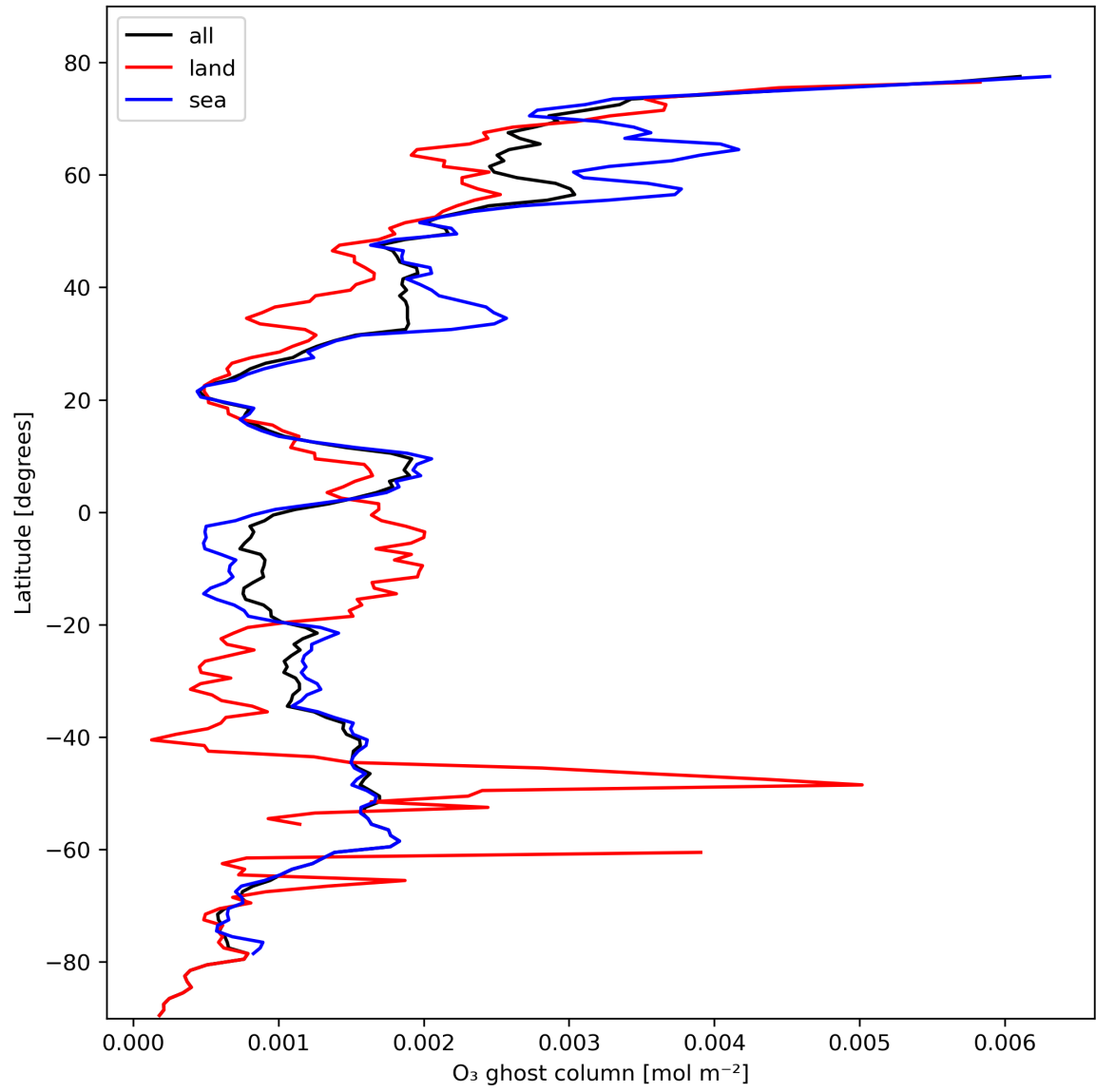
Figure 18: Zonal average of “O 3 ghost column” for 2023-10-24 to 2023-10-26.
