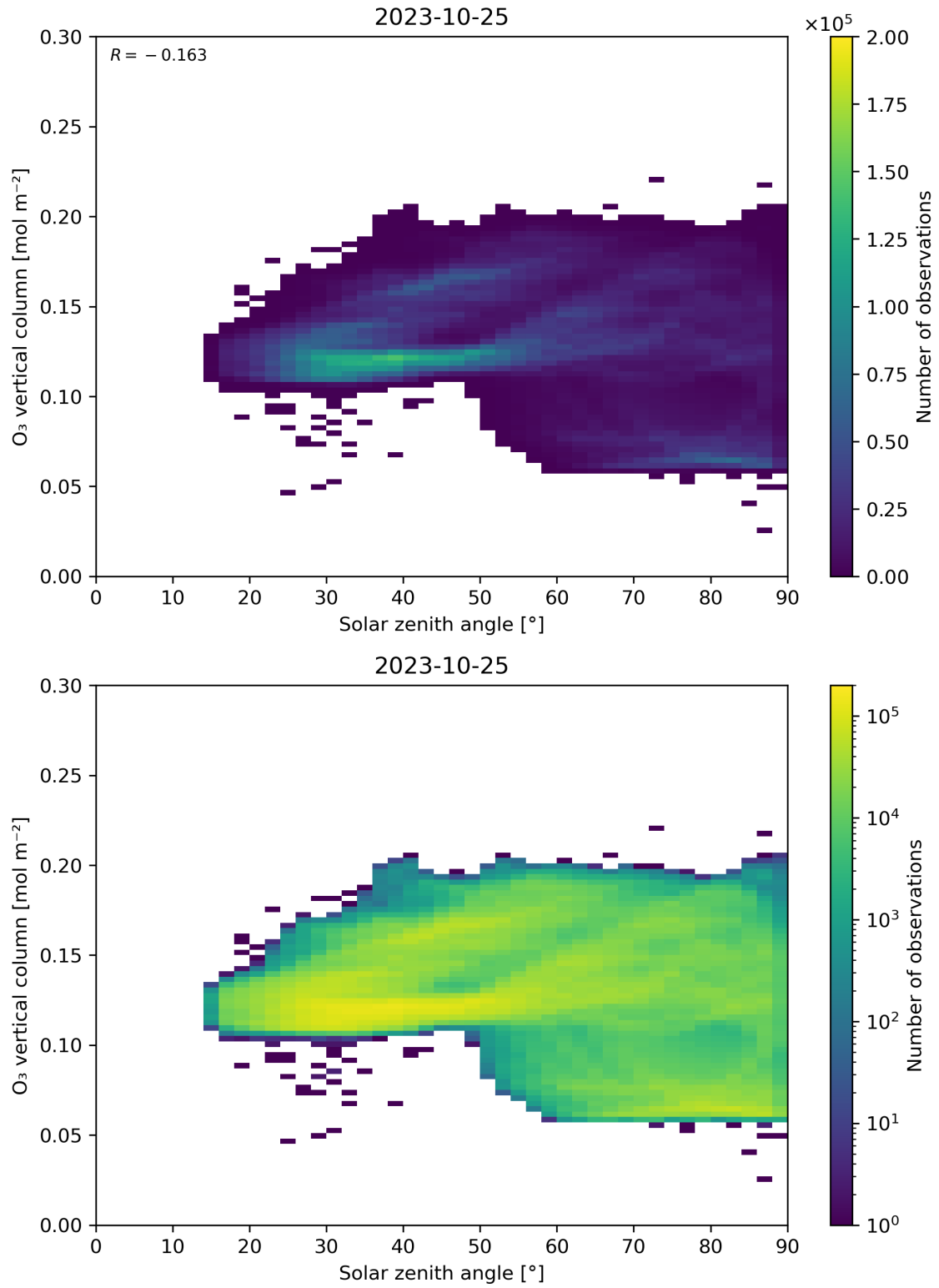
Figure 47: Scatter density plot of “Solar zenith angle” against “O 3 vertical column” for 2023-10-24 to 2023-10-26.
