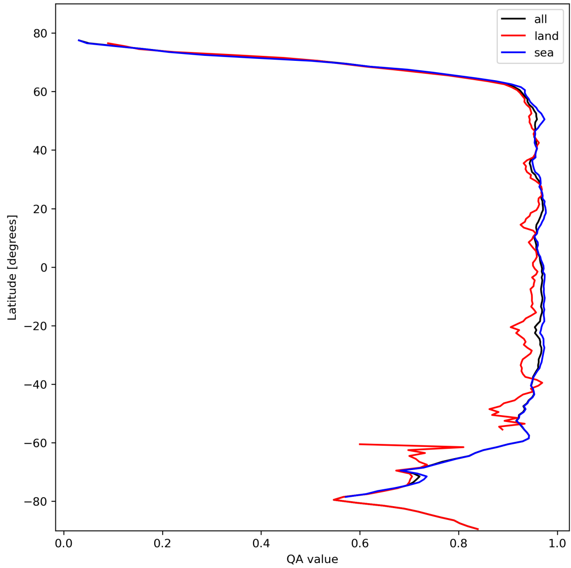
Figure 13: Zonal average of “QA value” for 2023-10-24 to 2023-10-26.
