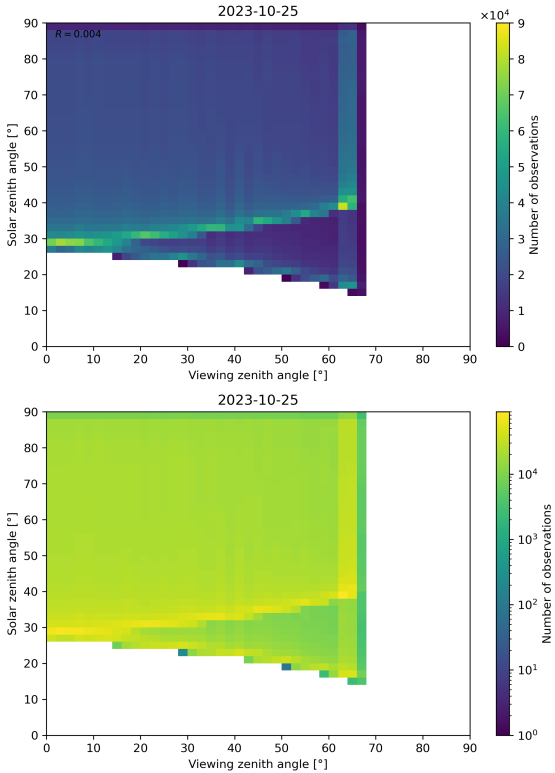
Figure 54: Scatter density plot of “Viewing zenith angle” against “Solar zenith angle” for 2023-10-24 to 2023-10-26.
