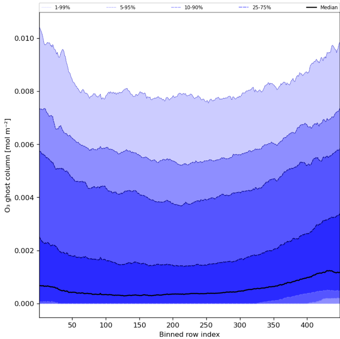
Figure 32: Along track statistics of “O 3 ghost column” for 2023-10-24 to 2023-10-26
