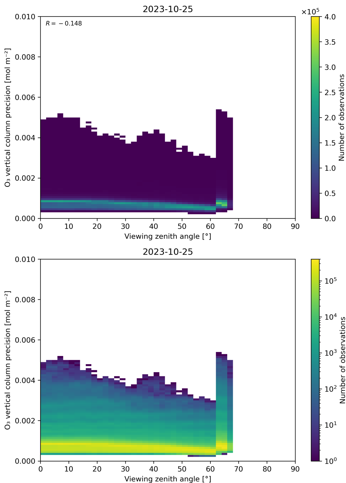
Figure 53: Scatter density plot of “Viewing zenith angle” against “O 3 vertical column precision” for 2023-10-24 to 2023-10-26.
