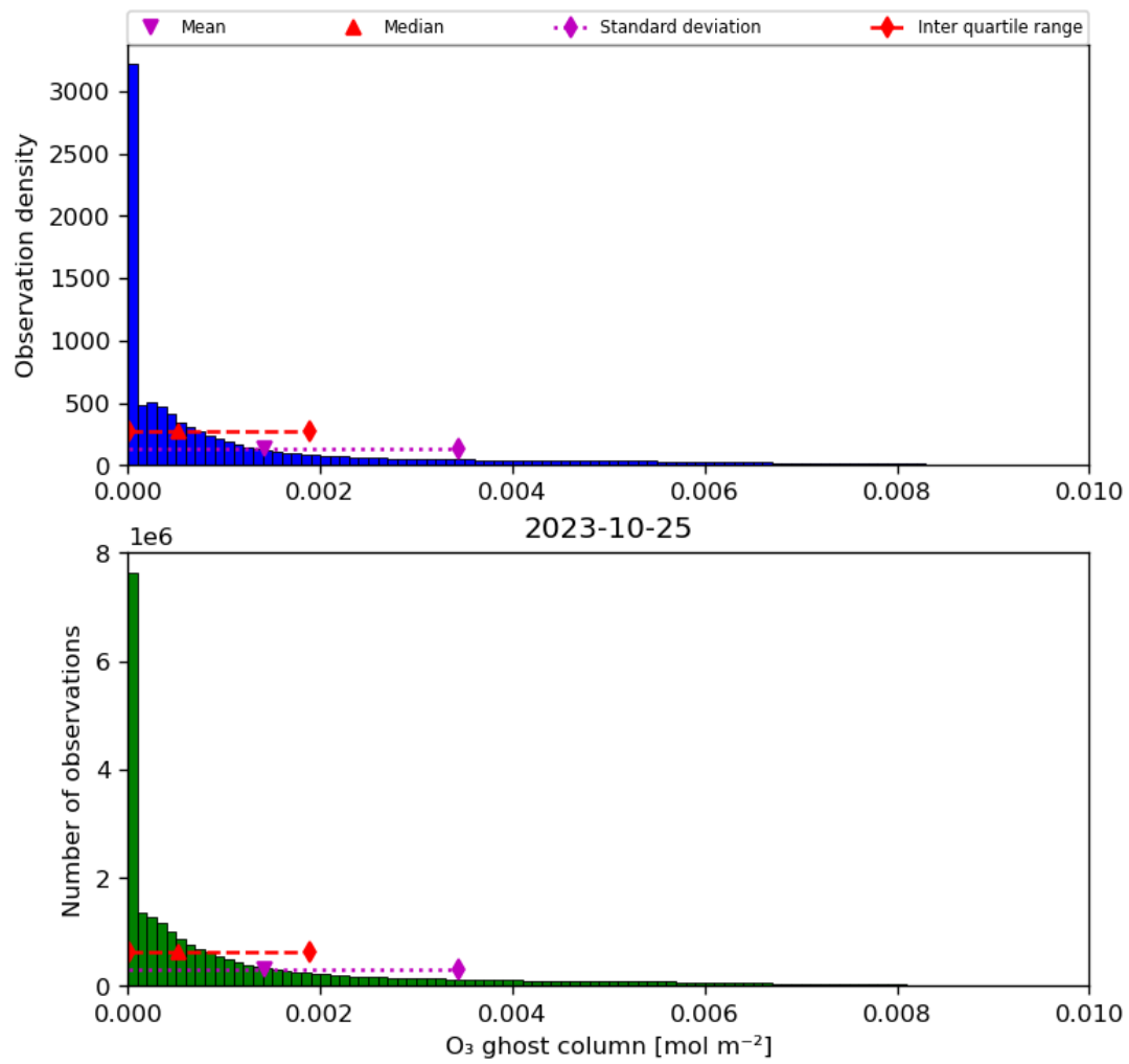
Figure 25: Histogram of “O 3 ghost column” for 2023-10-24 to 2023-10-26
