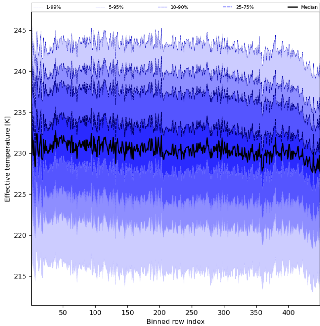
Figure 31: Along track statistics of “Effective temperature” for 2023-10-24 to 2023-10-26
