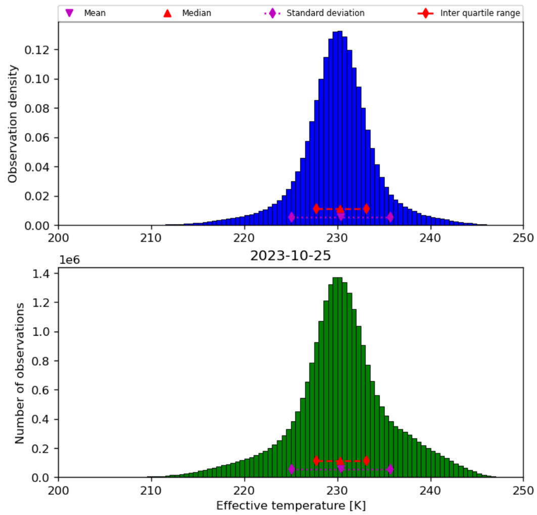
Figure 24: Histogram of “Effective temperature” for 2023-10-24 to 2023-10-26
