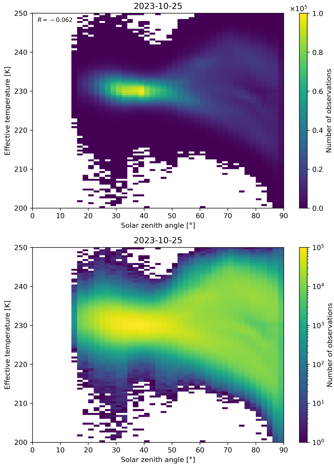
Figure 45: Scatter density plot of “Solar zenith angle” against “Effective temperature” for 2023-10-24 to 2023-10-26.
