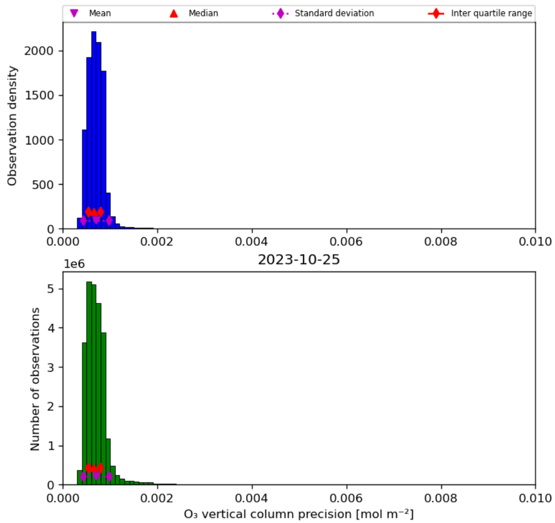
Figure 22: Histogram of “O 3 vertical column precision” for 2023-10-24 to 2023-10-26
