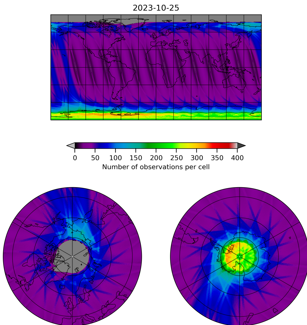
Figure 12: Map of the number of observations for 2023-10-24 to 2023-10-26
