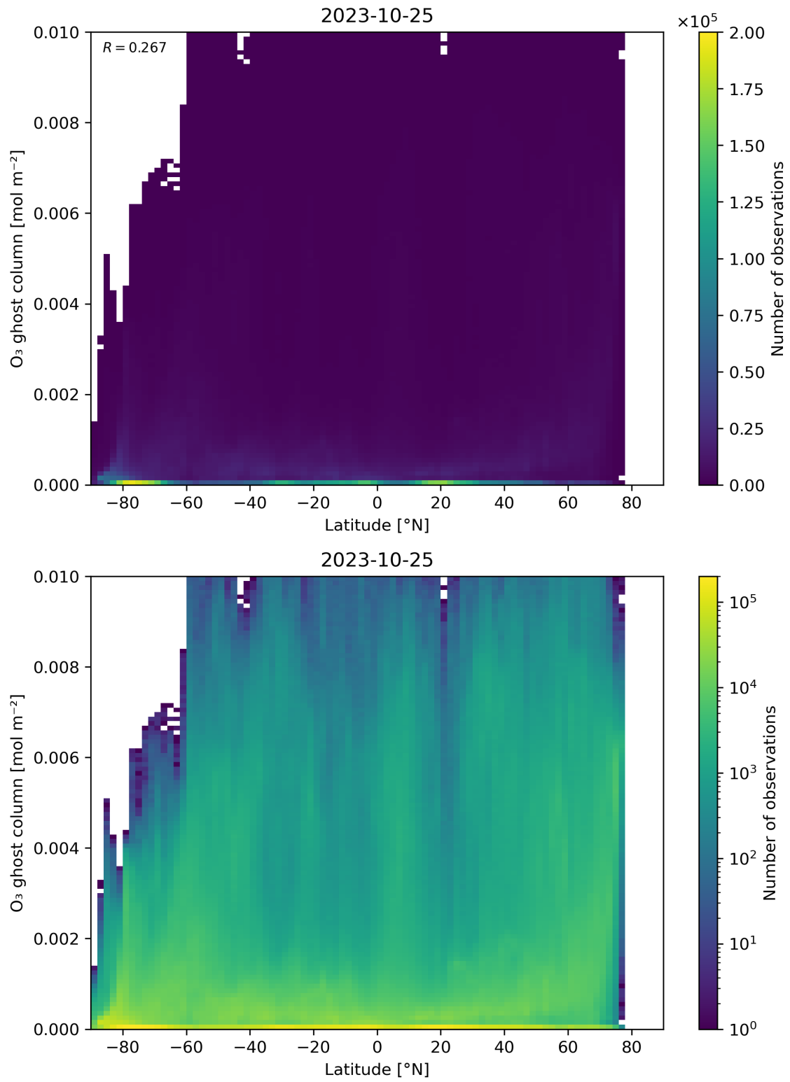
Figure 35: Scatter density plot of “Latitude” against “O 3 ghost column” for 2023-10-24 to 2023-10-26.
