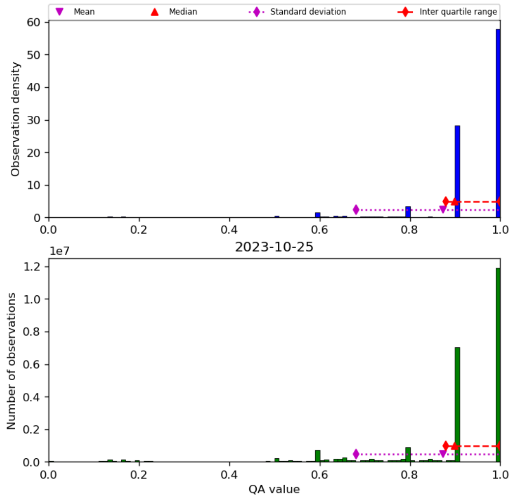
Figure 20: Histogram of “QA value” for 2023-10-24 to 2023-10-26
