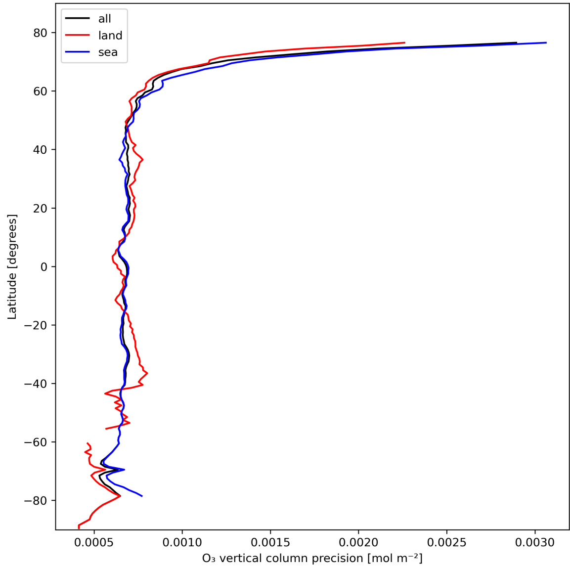
Figure 15: Zonal average of “O 3 vertical column precision” for 2023-10-25 to 2023-10-27.
