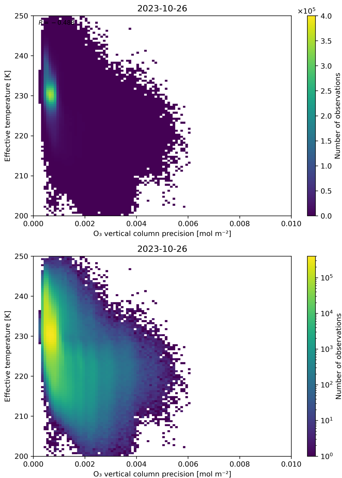
Figure 42: Scatter density plot of “O 3 vertical column precision” against “Effective temperature” for 2023-10-25 to 2023-10-27.
