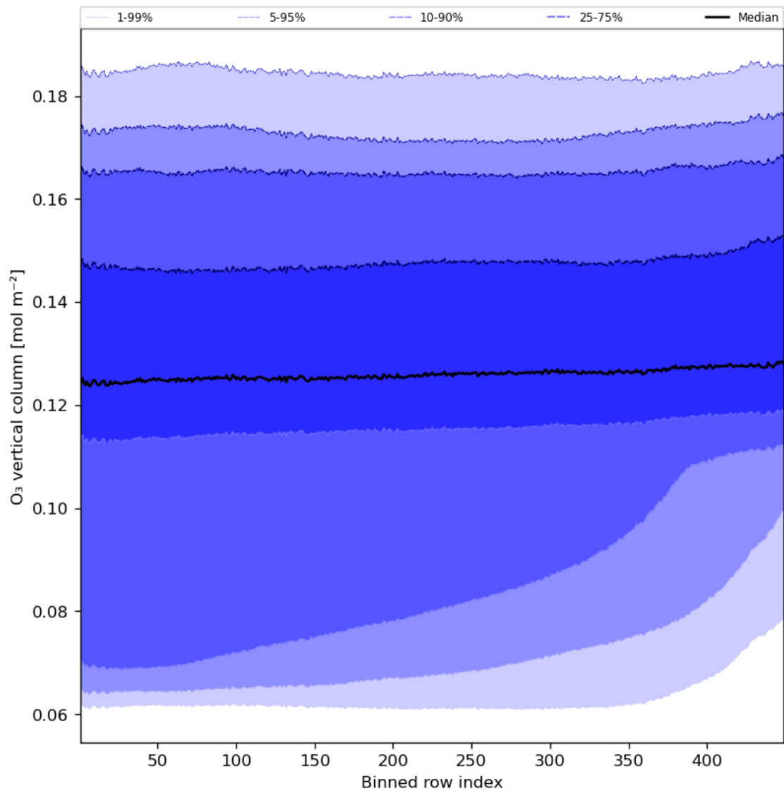
Figure 28: Along track statistics of “O 3 vertical column” for 2023-10-25 to 2023-10-27
