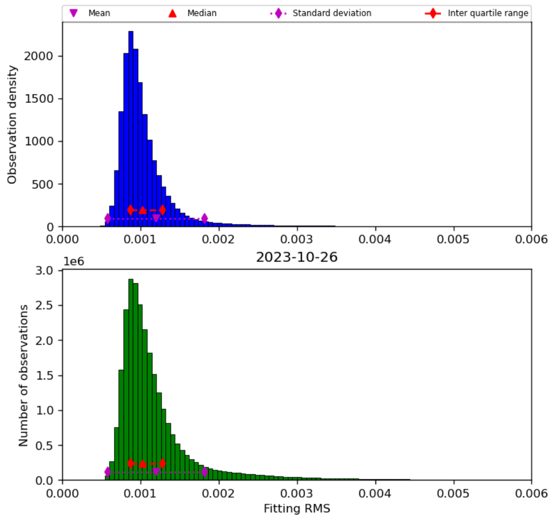
Figure 23: Histogram of “Fitting RMS” for 2023-10-25 to 2023-10-27
