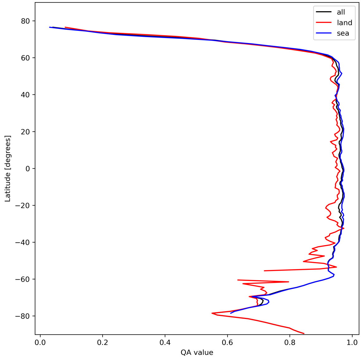
Figure 13: Zonal average of “QA value” for 2023-10-25 to 2023-10-27.
