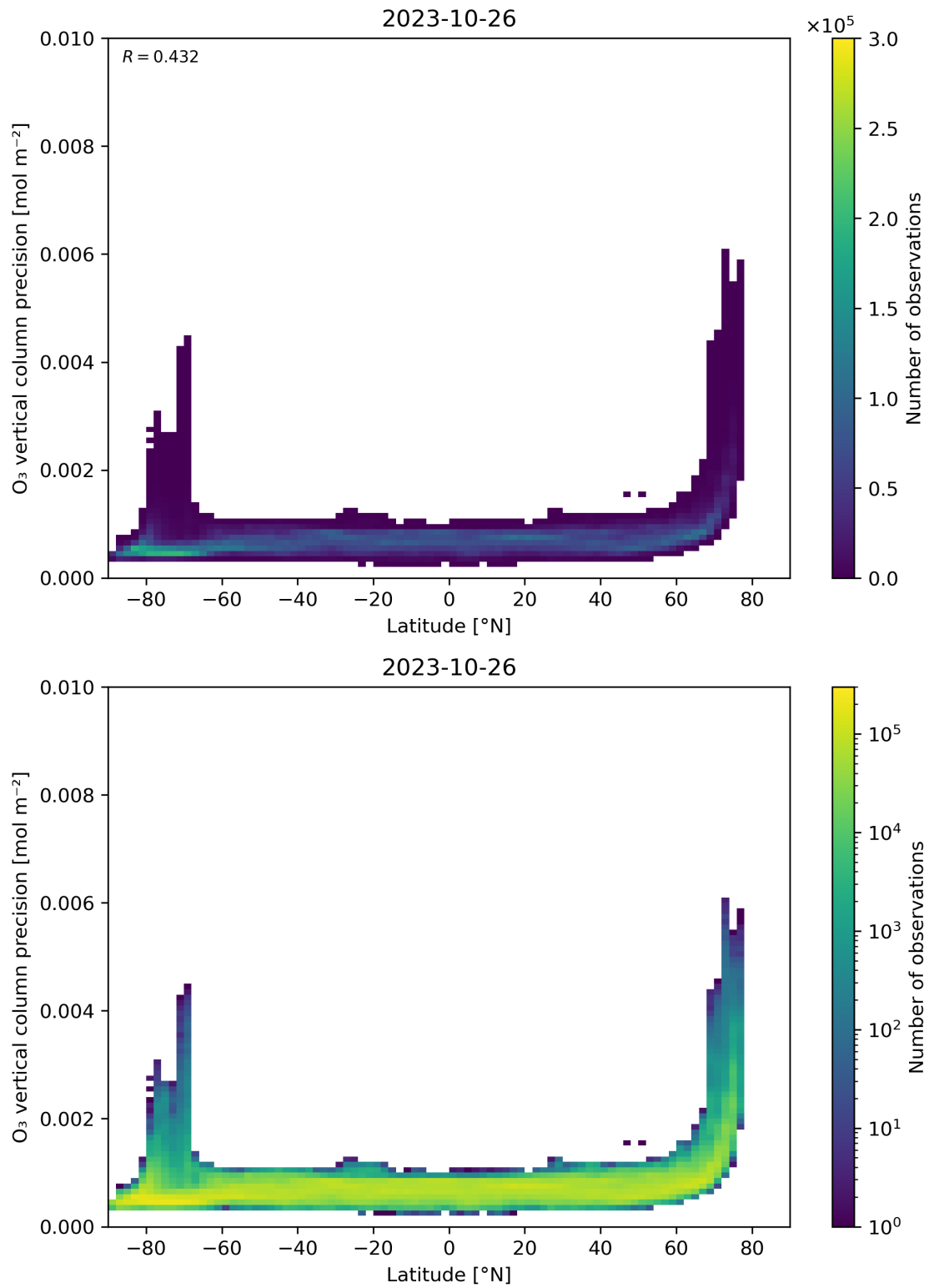
Figure 37: Scatter density plot of “Latitude” against “O 3 vertical column precision” for 2023-10-25 to 2023-10-27.
