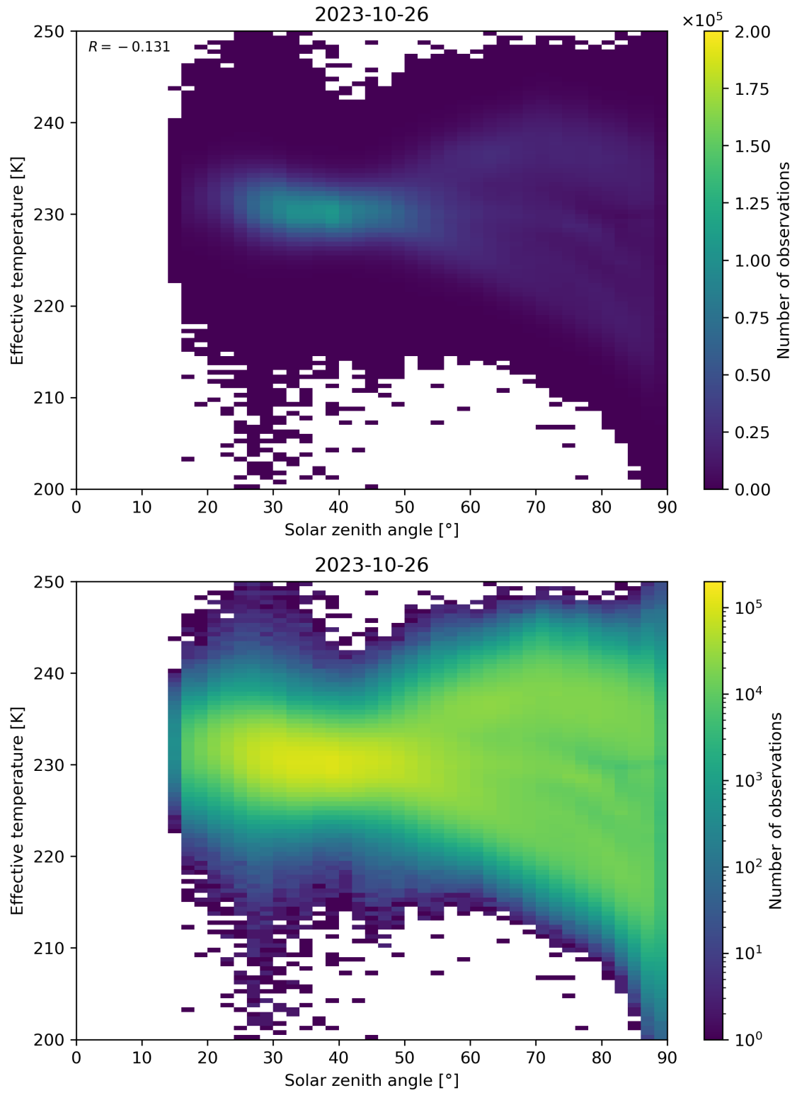
Figure 45: Scatter density plot of “Solar zenith angle” against “Effective temperature” for 2023-10-25 to 2023-10-27.
