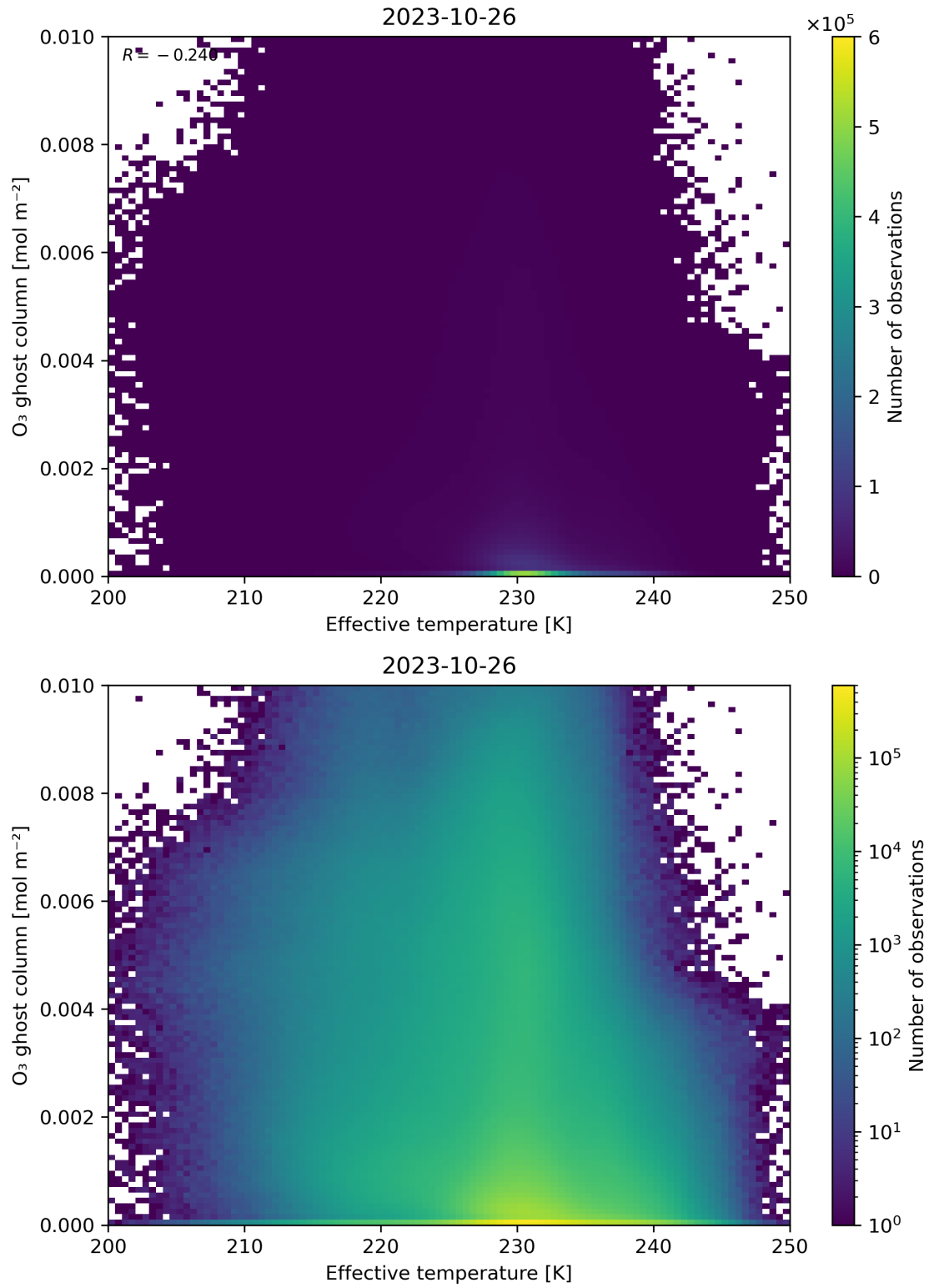
Figure 38: Scatter density plot of “Effective temperature” against “O 3 ghost column” for 2023-10-25 to 2023-10-27.
