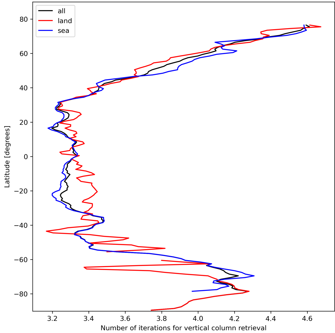
Figure 19: Zonal average of “Number of iterations for vertical column retrieval” for 2023-10-25 to 2023-10-27.
