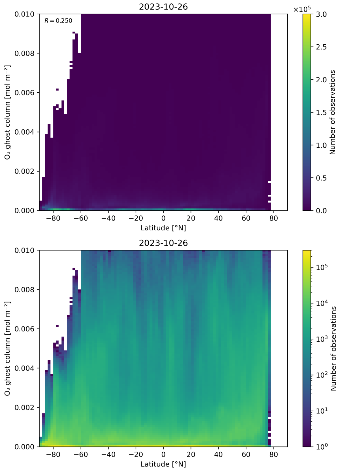
Figure 35: Scatter density plot of “Latitude” against “O 3 ghost column” for 2023-10-25 to 2023-10-27.
