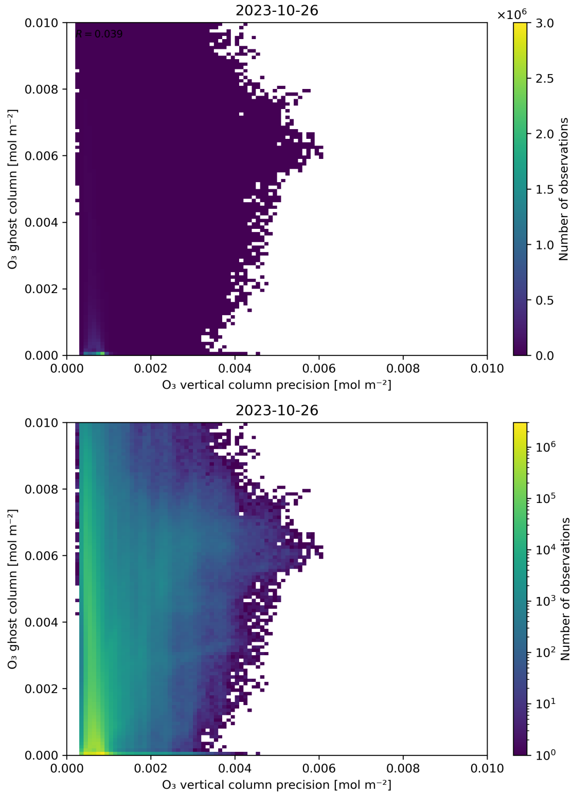
Figure 43: Scatter density plot of “ \text{O}_3 vertical column precision” against “ \text{O}_3 ghost column” for 2023-10-25 to 2023-10-27.
