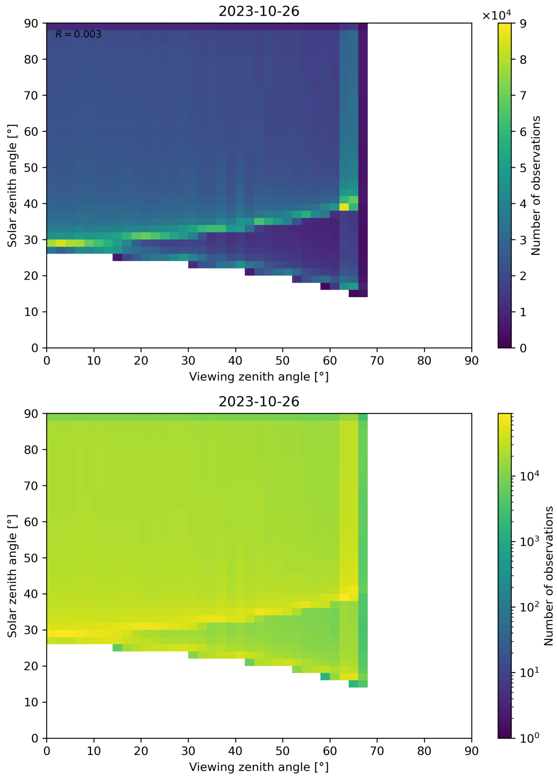
Figure 54: Scatter density plot of “Viewing zenith angle” against “Solar zenith angle” for 2023-10-25 to 2023-10-27.
