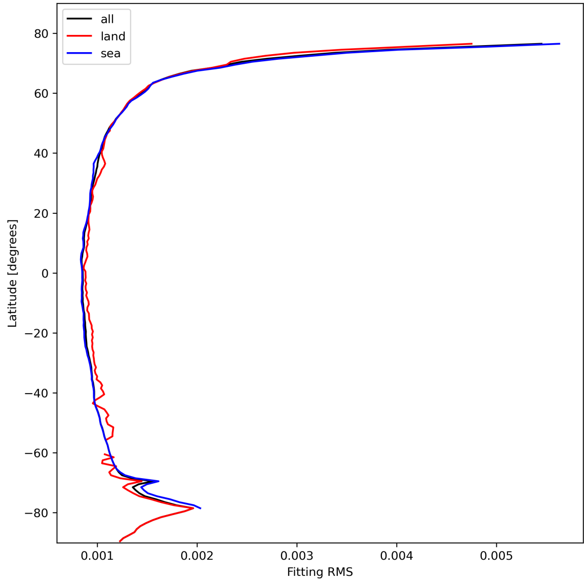
Figure 16: Zonal average of “Fitting RMS” for 2023-10-25 to 2023-10-27.
