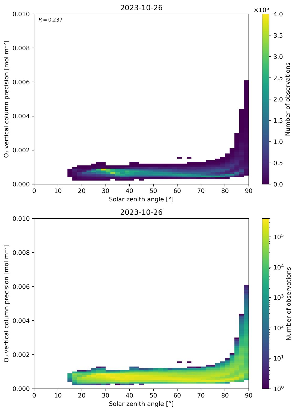
Figure 48: Scatter density plot of “Solar zenith angle” against “O 3 vertical column precision” for 2023-10-25 to 2023-10-27.
