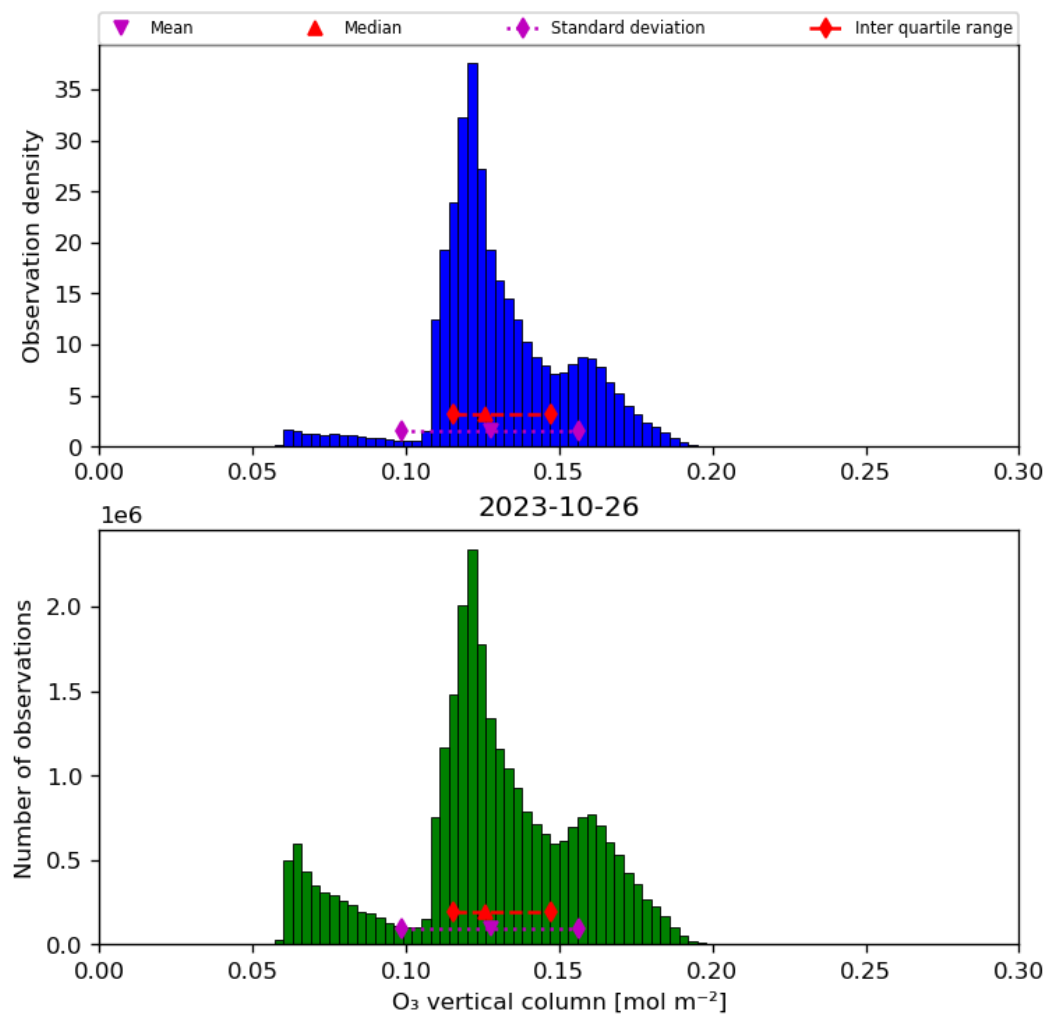
Figure 21: Histogram of “O 3 vertical column” for 2023-10-25 to 2023-10-27
