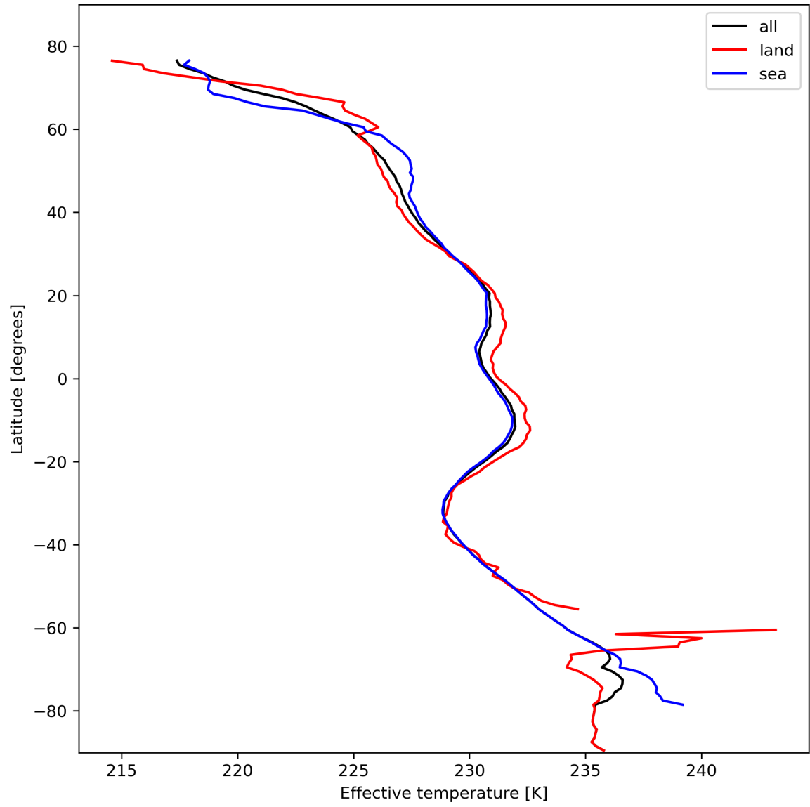
Figure 17: Zonal average of “Effective temperature” for 2023-10-25 to 2023-10-27.
