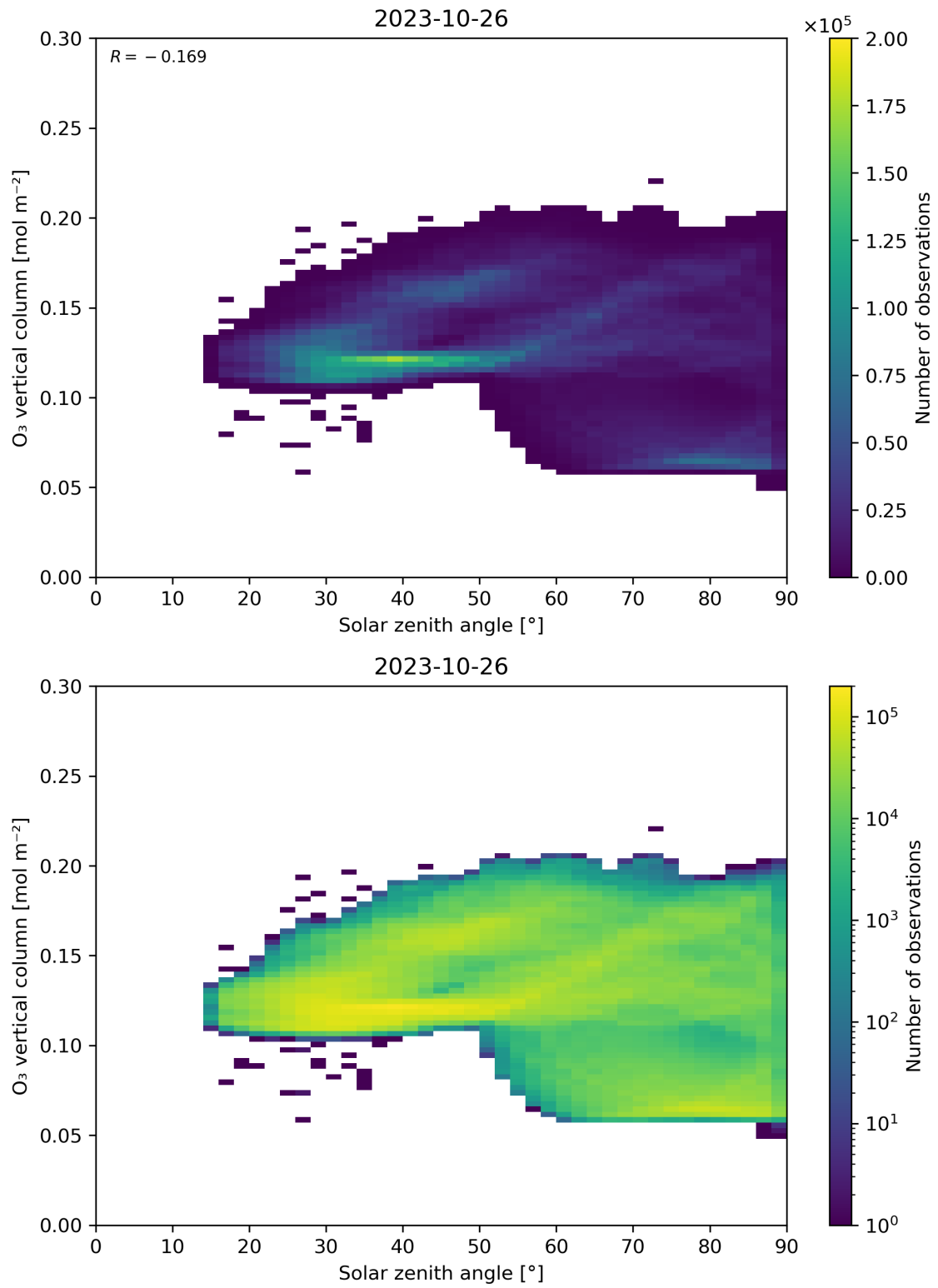
Figure 47: Scatter density plot of “Solar zenith angle” against “O 3 vertical column” for 2023-10-25 to 2023-10-27.
