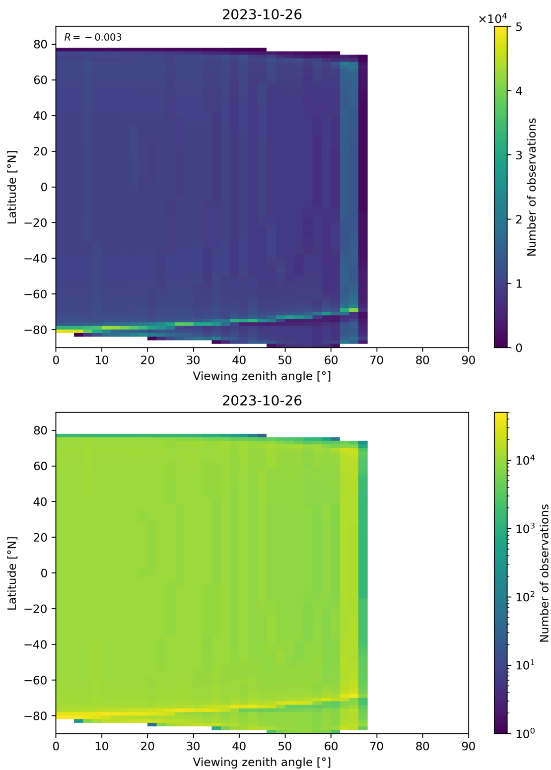
Figure 49: Scatter density plot of “Viewing zenith angle” against “Latitude” for 2023-10-25 to 2023-10-27.
