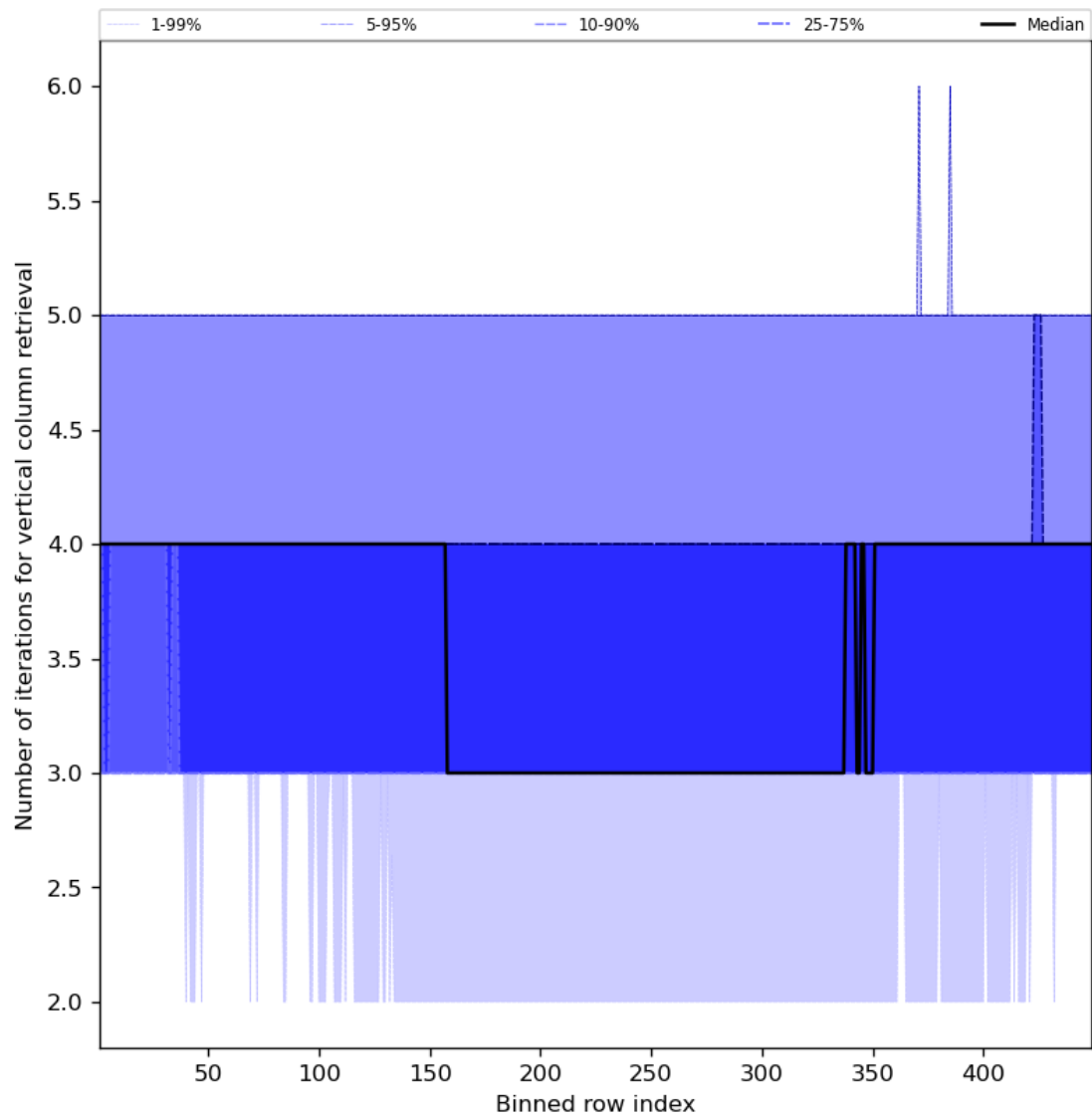
Figure 33: Along track statistics of “Number of iterations for vertical column retrieval” for 2023-10-27 to 2023-10-28
