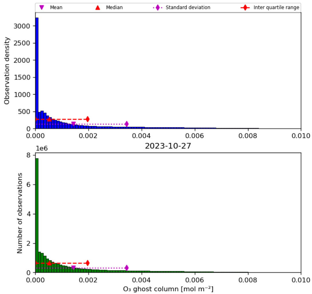
Figure 25: Histogram of “O 3 ghost column” for 2023-10-27 to 2023-10-28
