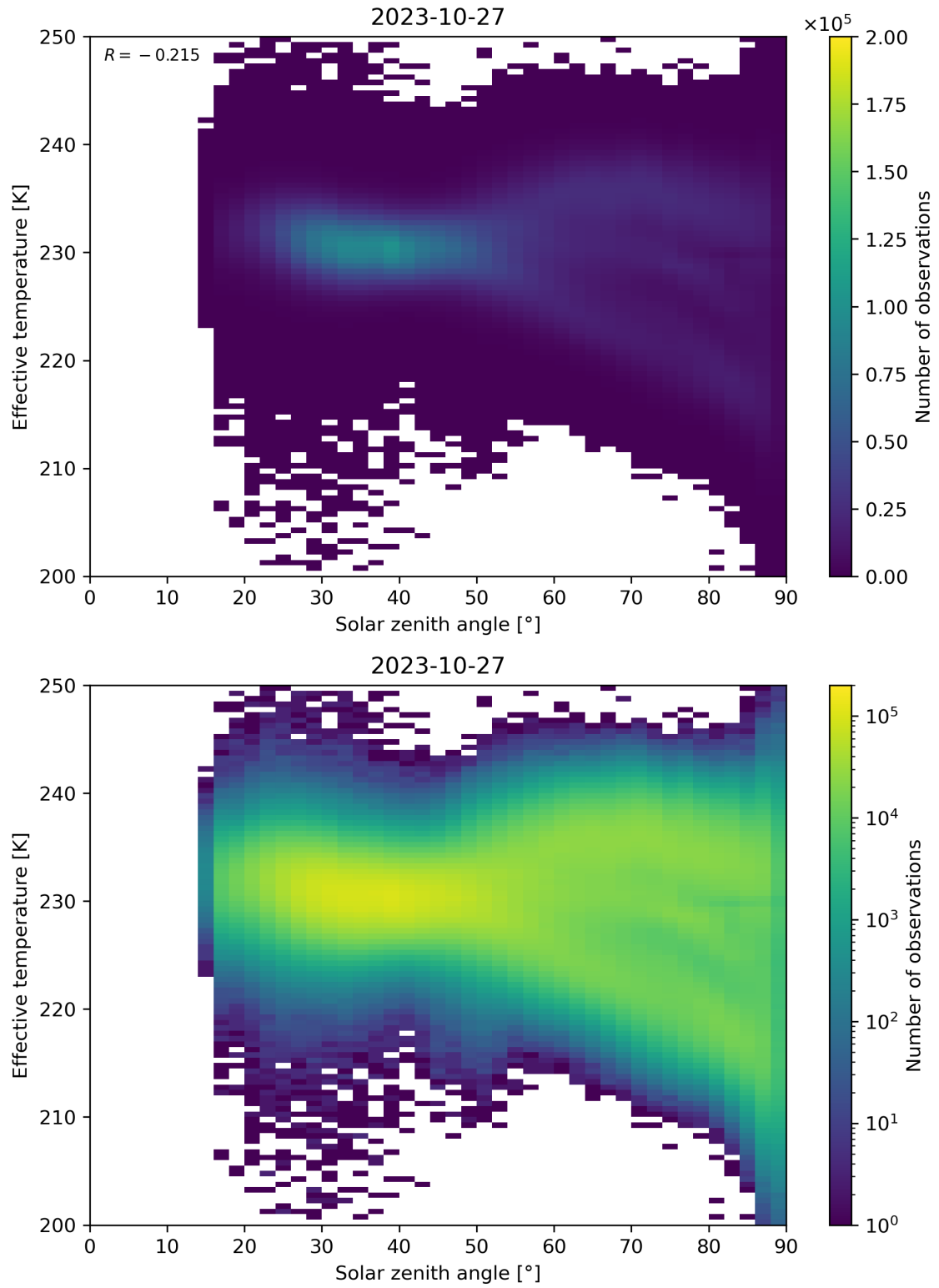
Figure 45: Scatter density plot of “Solar zenith angle” against “Effective temperature” for 2023-10-27 to 2023-10-28.
