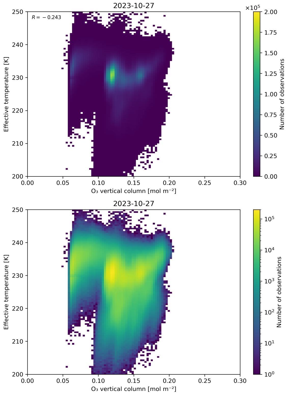
Figure 39: Scatter density plot of “O 3 vertical column” against “Effective temperature” for 2023-10-27 to 2023-10-28.
