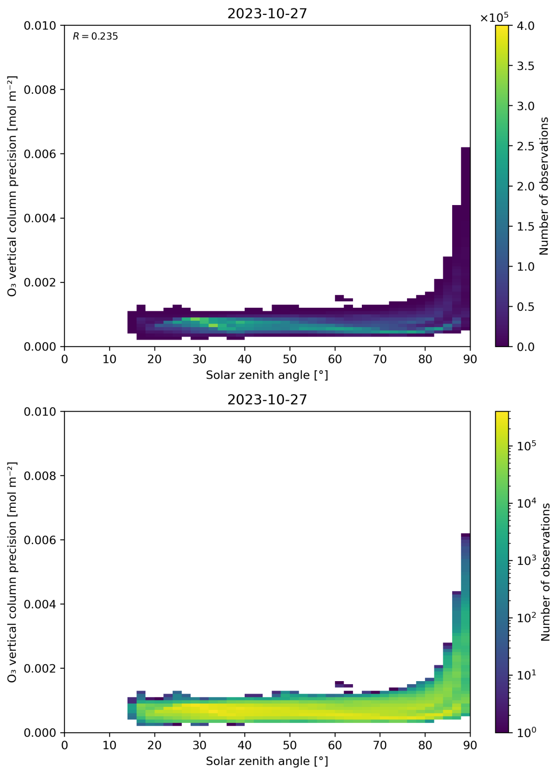
Figure 48: Scatter density plot of “Solar zenith angle” against “O 3 vertical column precision” for 2023-10-27 to 2023-10-28.
