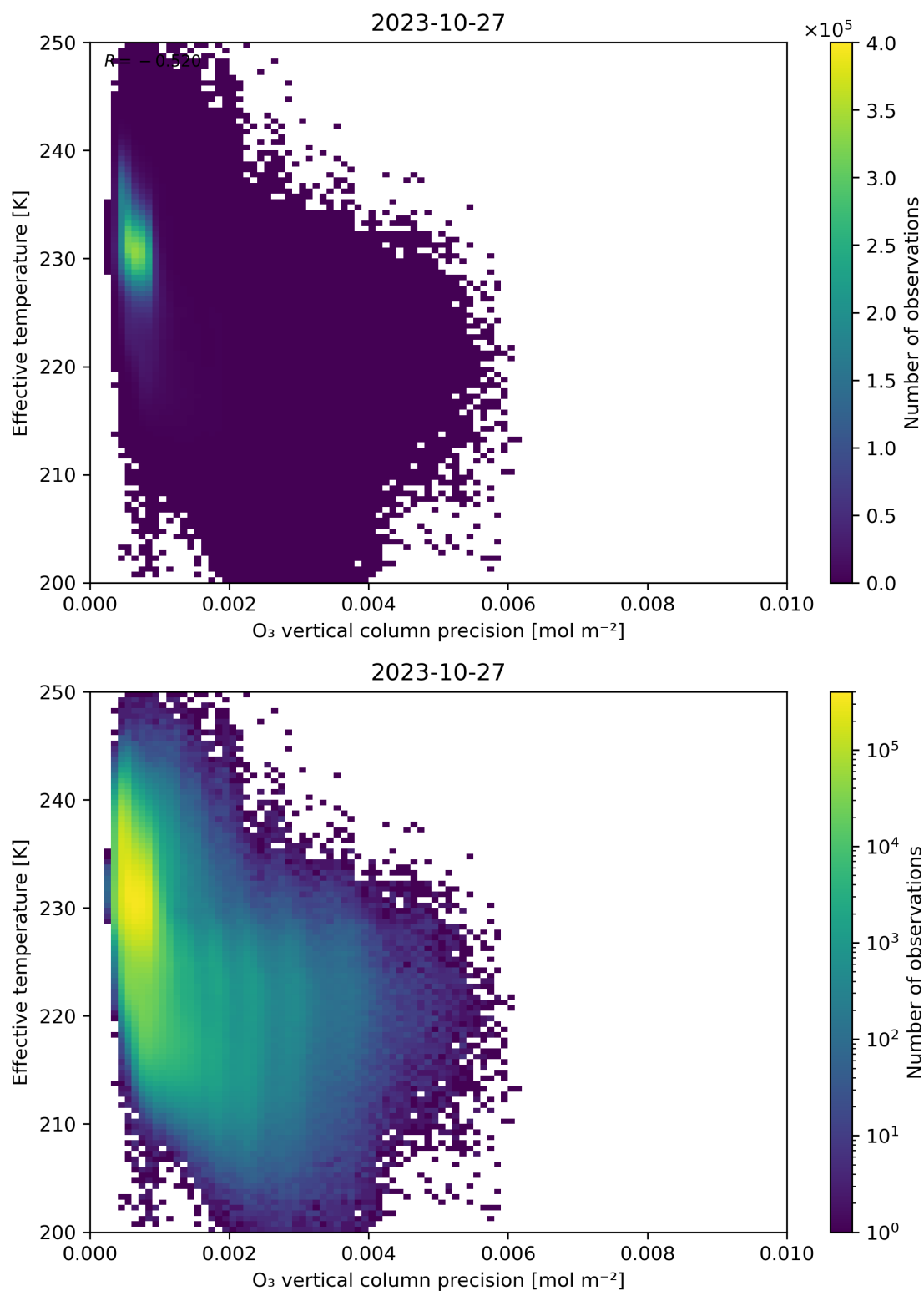
Figure 42: Scatter density plot of “O 3 vertical column precision” against “Effective temperature” for 2023-10-27 to 2023-10-28.
