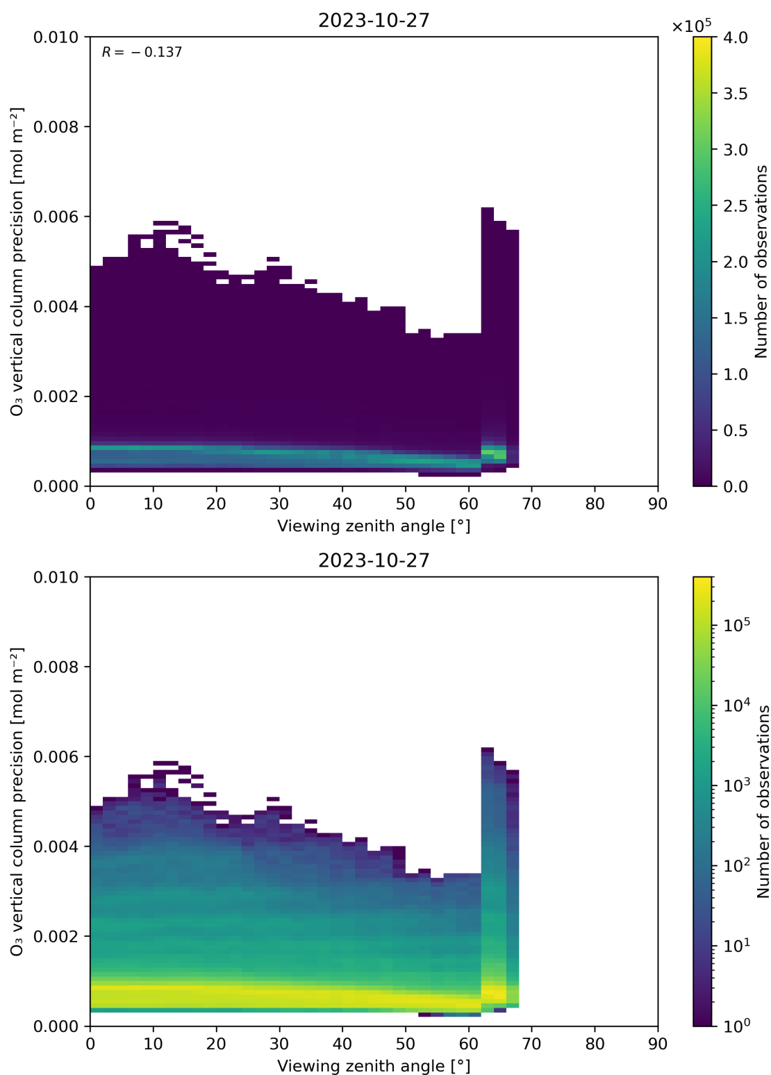
Figure 53: Scatter density plot of “Viewing zenith angle” against “O 3 vertical column precision” for 2023-10-27 to 2023-10-28.
