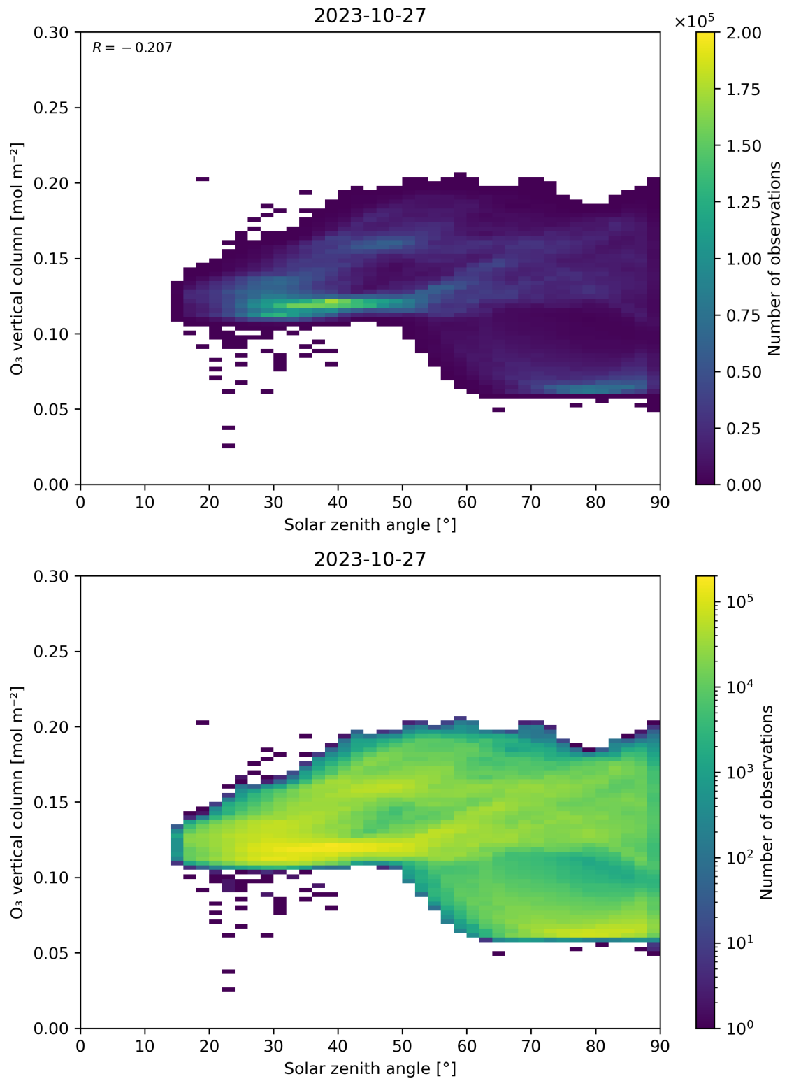
Figure 47: Scatter density plot of “Solar zenith angle” against “O 3 vertical column” for 2023-10-27 to 2023-10-28.
