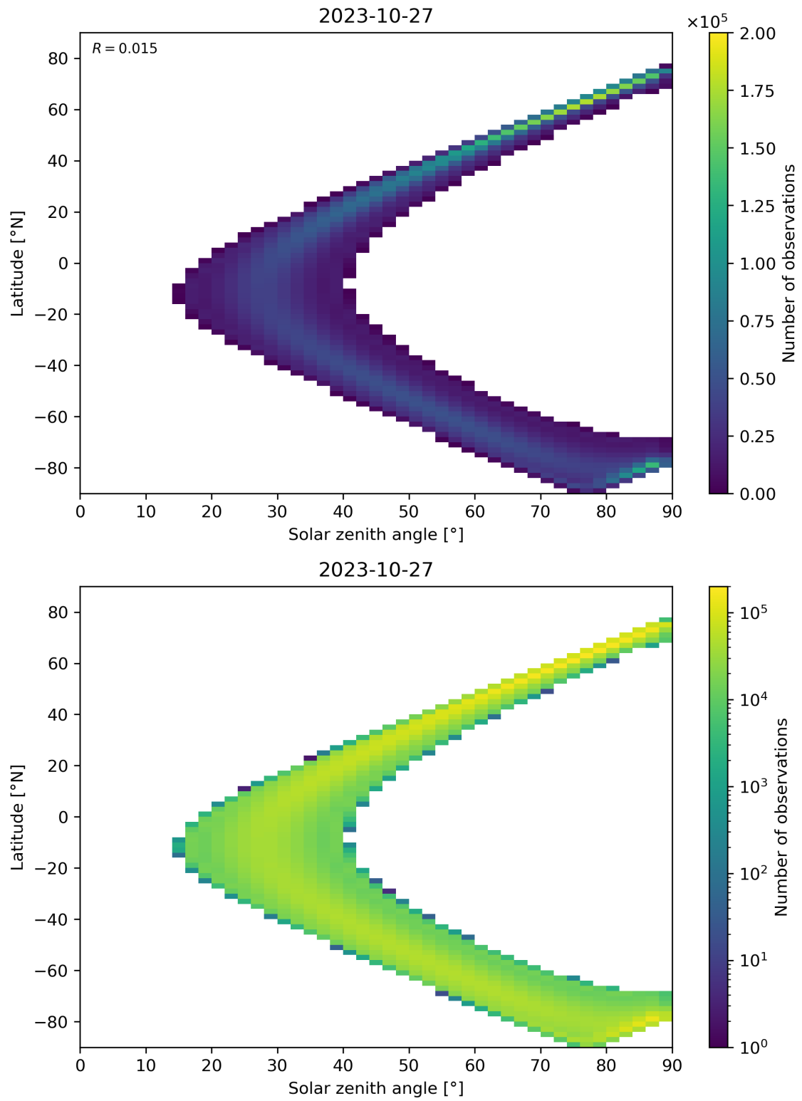
Figure 44: Scatter density plot of “Solar zenith angle” against “Latitude” for 2023-10-27 to 2023-10-28.
