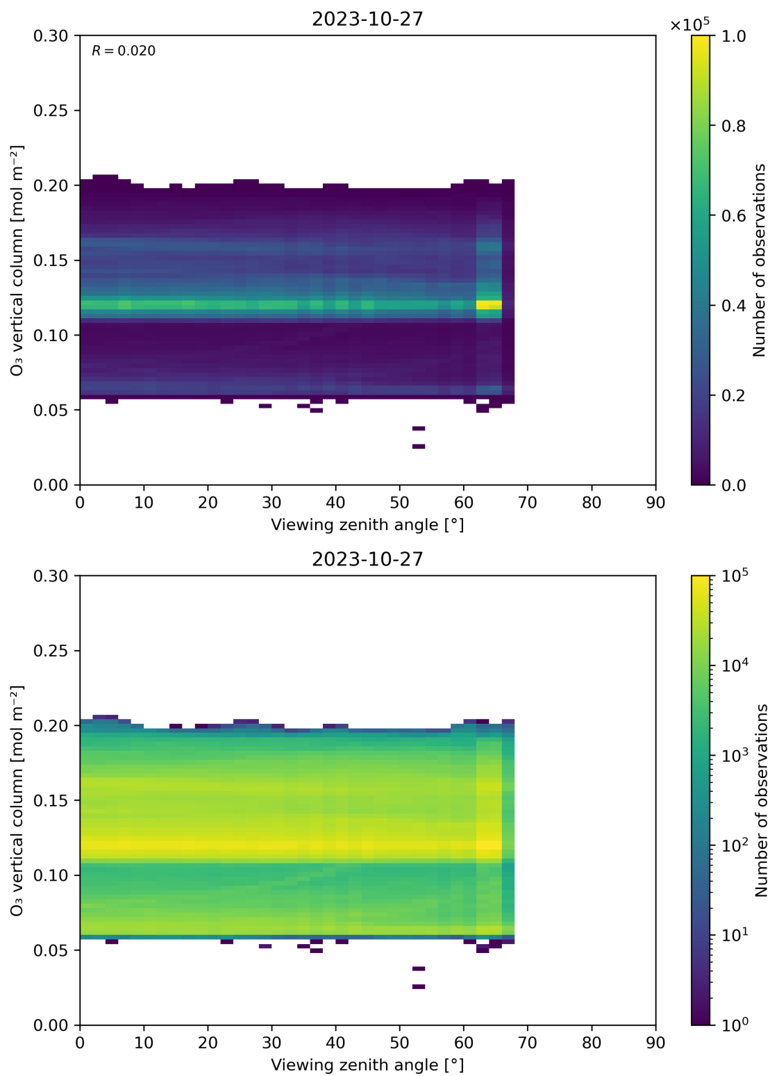
Figure 52: Scatter density plot of “Viewing zenith angle” against “O 3 vertical column” for 2023-10-27 to 2023-10-28.
