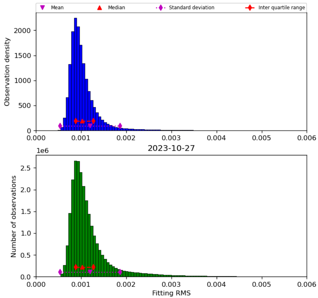
Figure 23: Histogram of “Fitting RMS” for 2023-10-27 to 2023-10-28
