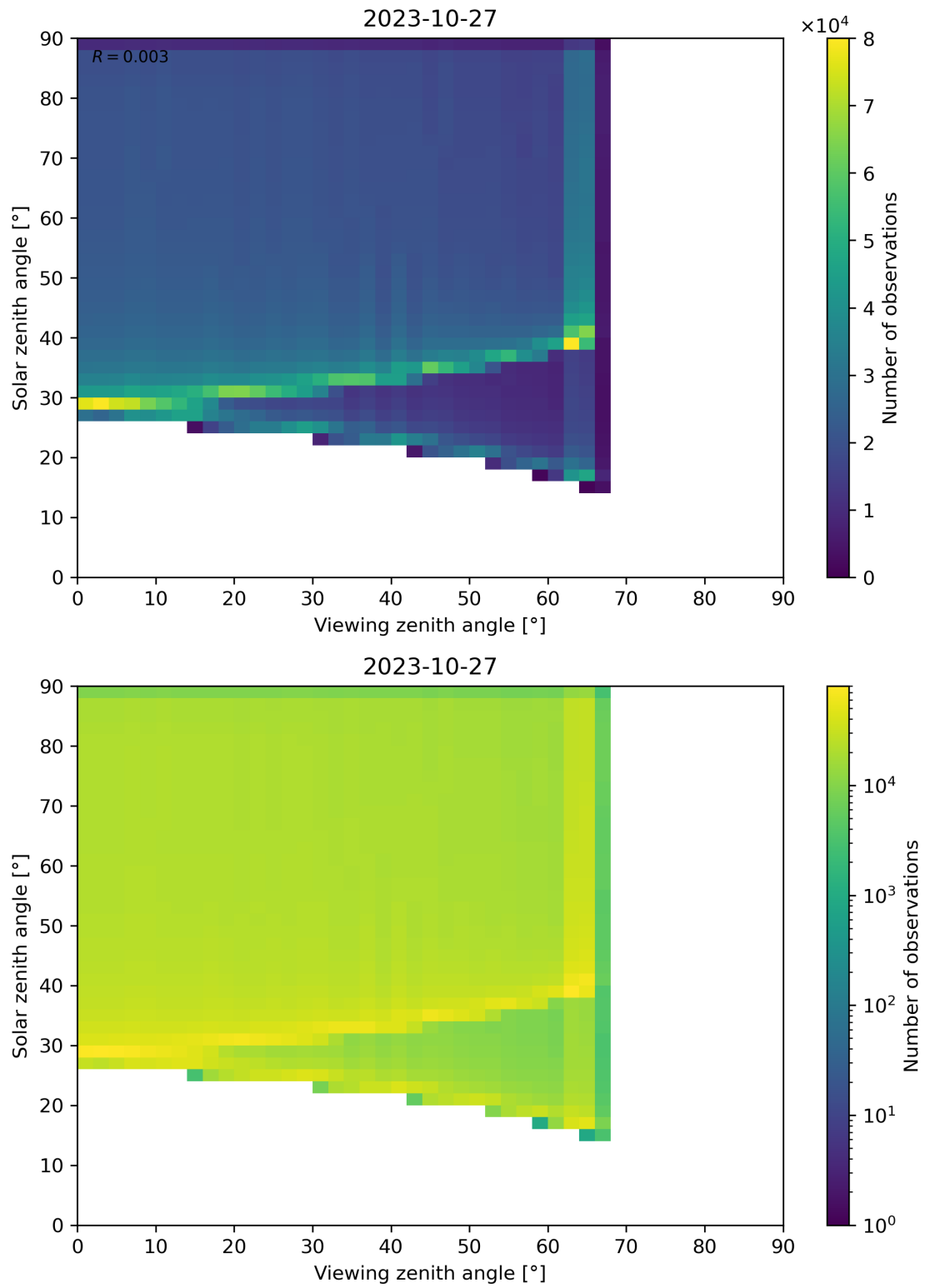
Figure 54: Scatter density plot of “Viewing zenith angle” against “Solar zenith angle” for 2023-10-27 to 2023-10-28.
