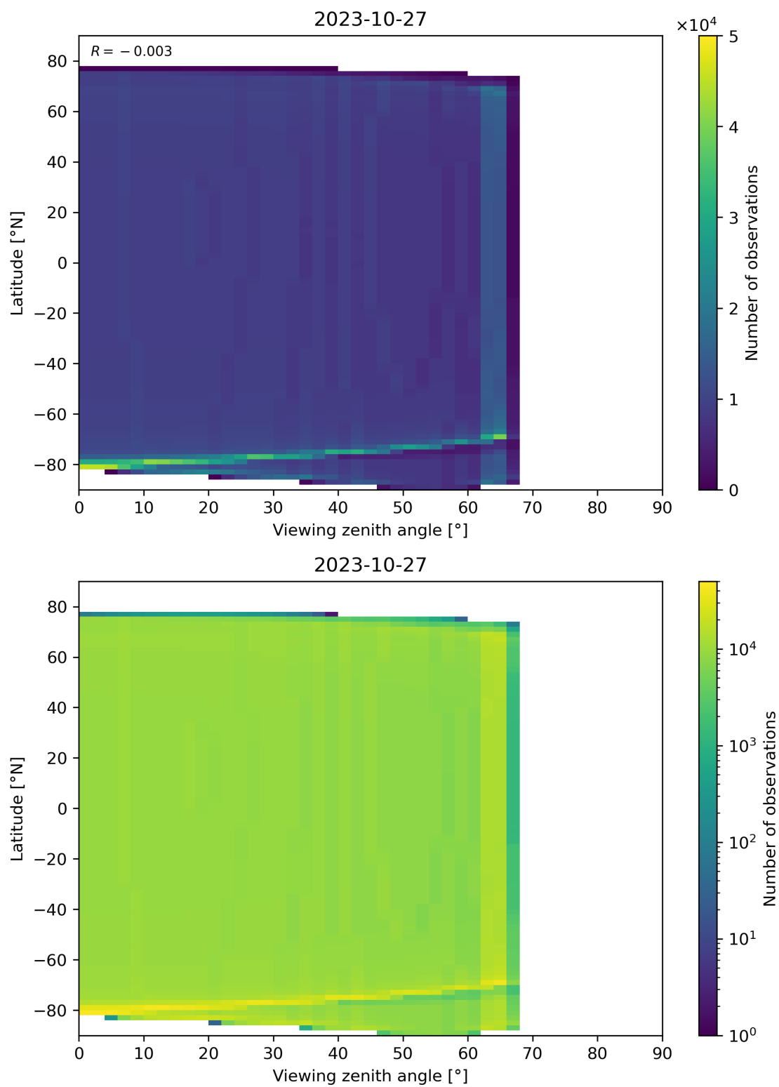
Figure 49: Scatter density plot of “Viewing zenith angle” against “Latitude” for 2023-10-27 to 2023-10-28.
