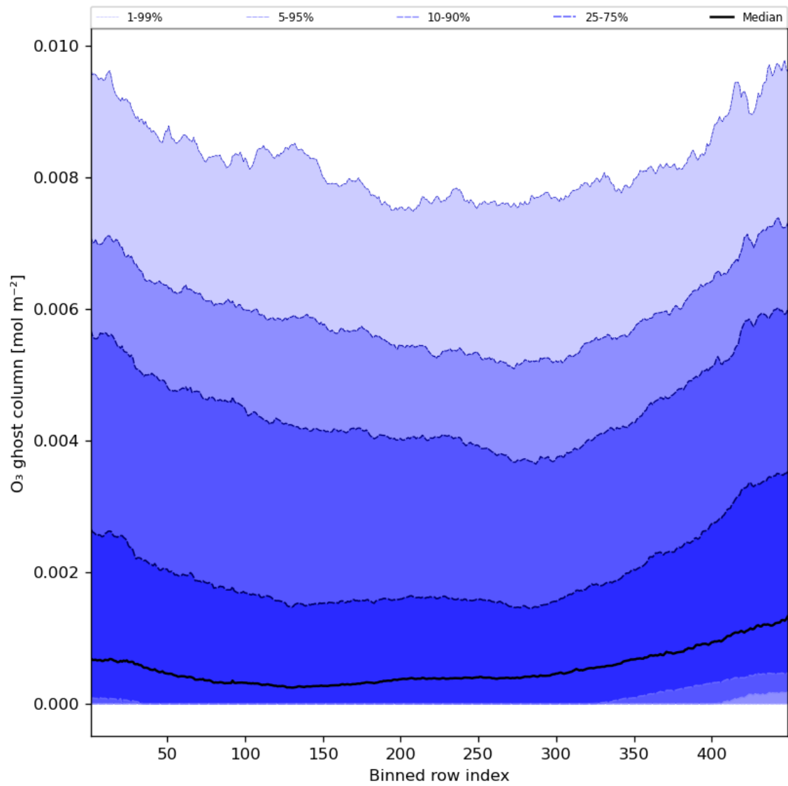
Figure 32: Along track statistics of “O 3 ghost column” for 2023-10-27 to 2023-10-28
