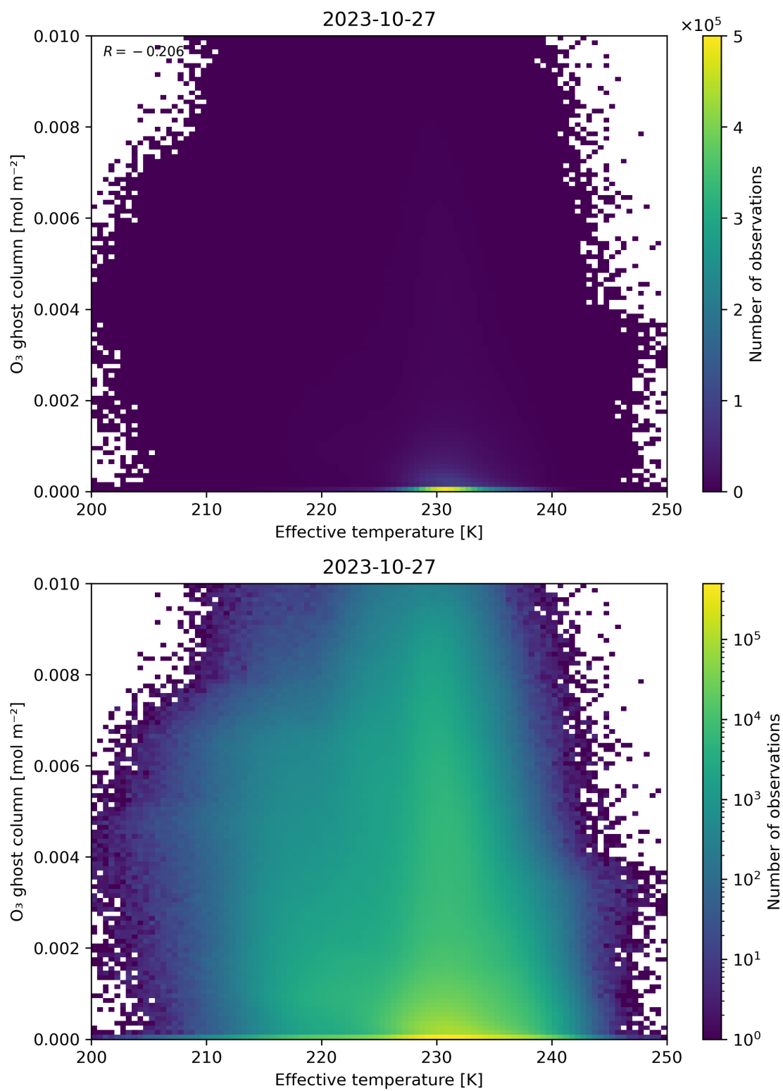
Figure 38: Scatter density plot of “Effective temperature” against “O 3 ghost column” for 2023-10-27 to 2023-10-28.
