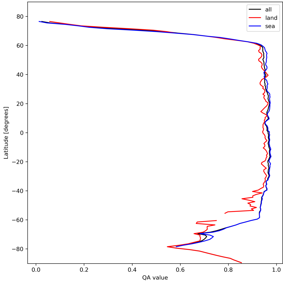
Figure 13: Zonal average of “QA value” for 2023-10-27 to 2023-10-28.
