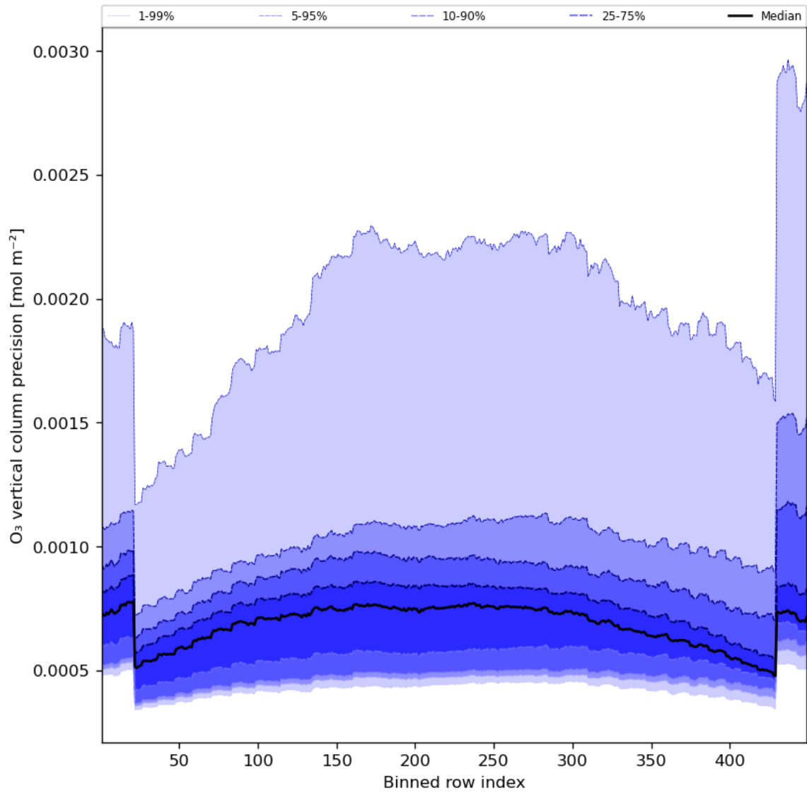
Figure 29: Along track statistics of “O 3 vertical column precision” for 2023-10-27 to 2023-10-28
