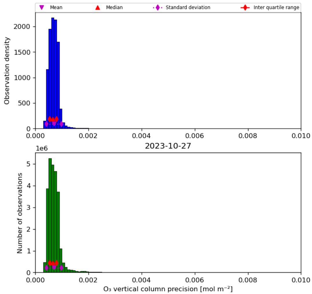
Figure 22: Histogram of “O 3 vertical column precision” for 2023-10-27 to 2023-10-28
