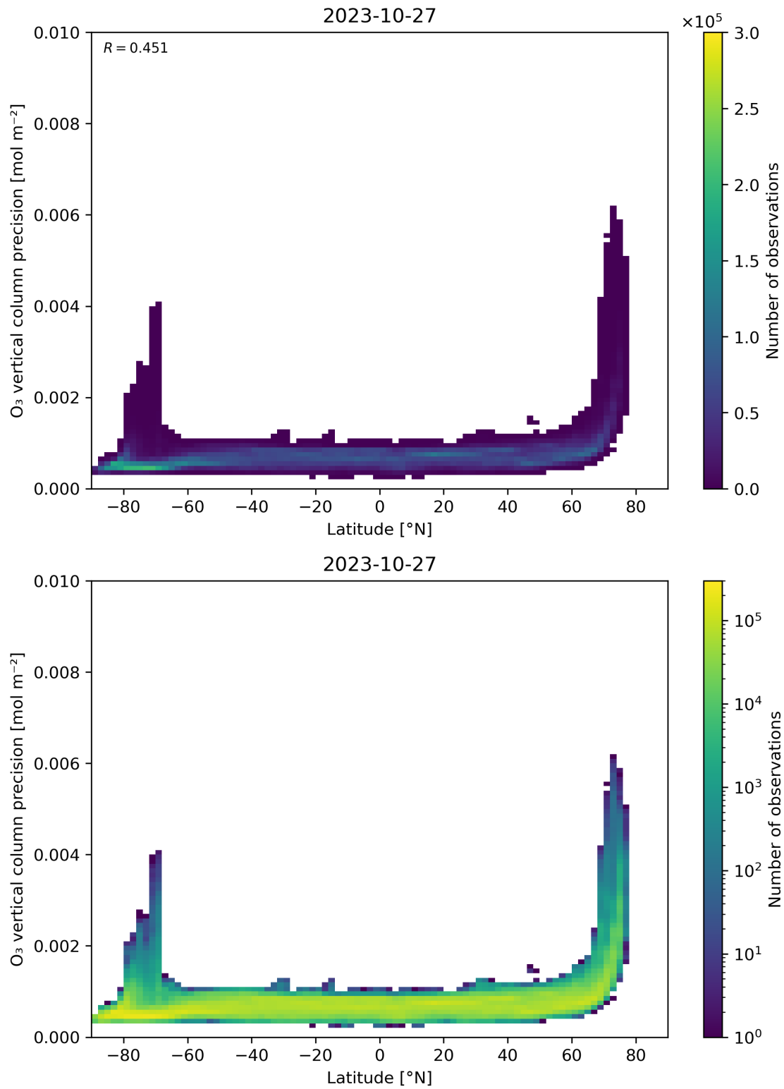
Figure 37: Scatter density plot of “Latitude” against “O 3 vertical column precision” for 2023-10-27 to 2023-10-28.
