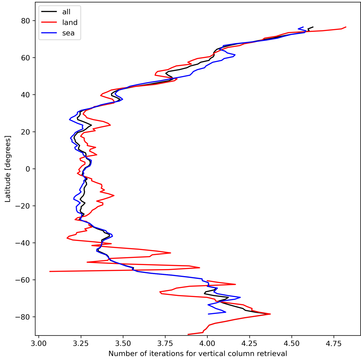
Figure 19: Zonal average of “Number of iterations for vertical column retrieval” for 2023-10-27 to 2023-10-28.
