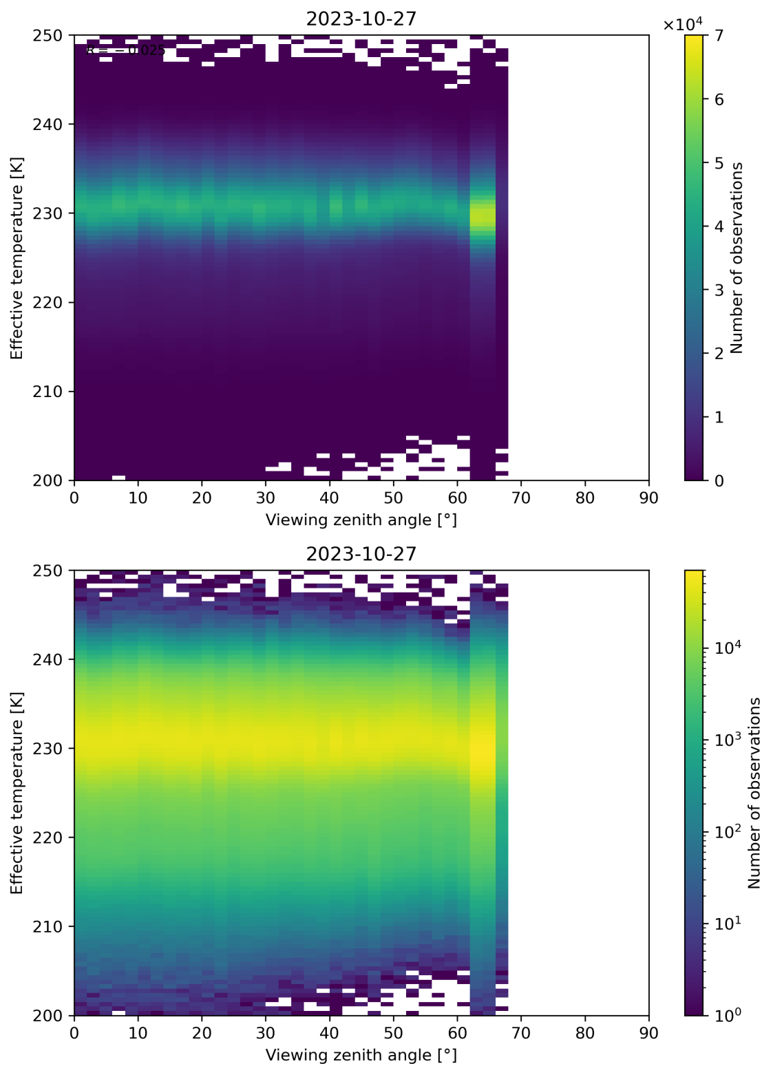
Figure 50: Scatter density plot of “Viewing zenith angle” against “Effective temperature” for 2023-10-27 to 2023-10-28.
