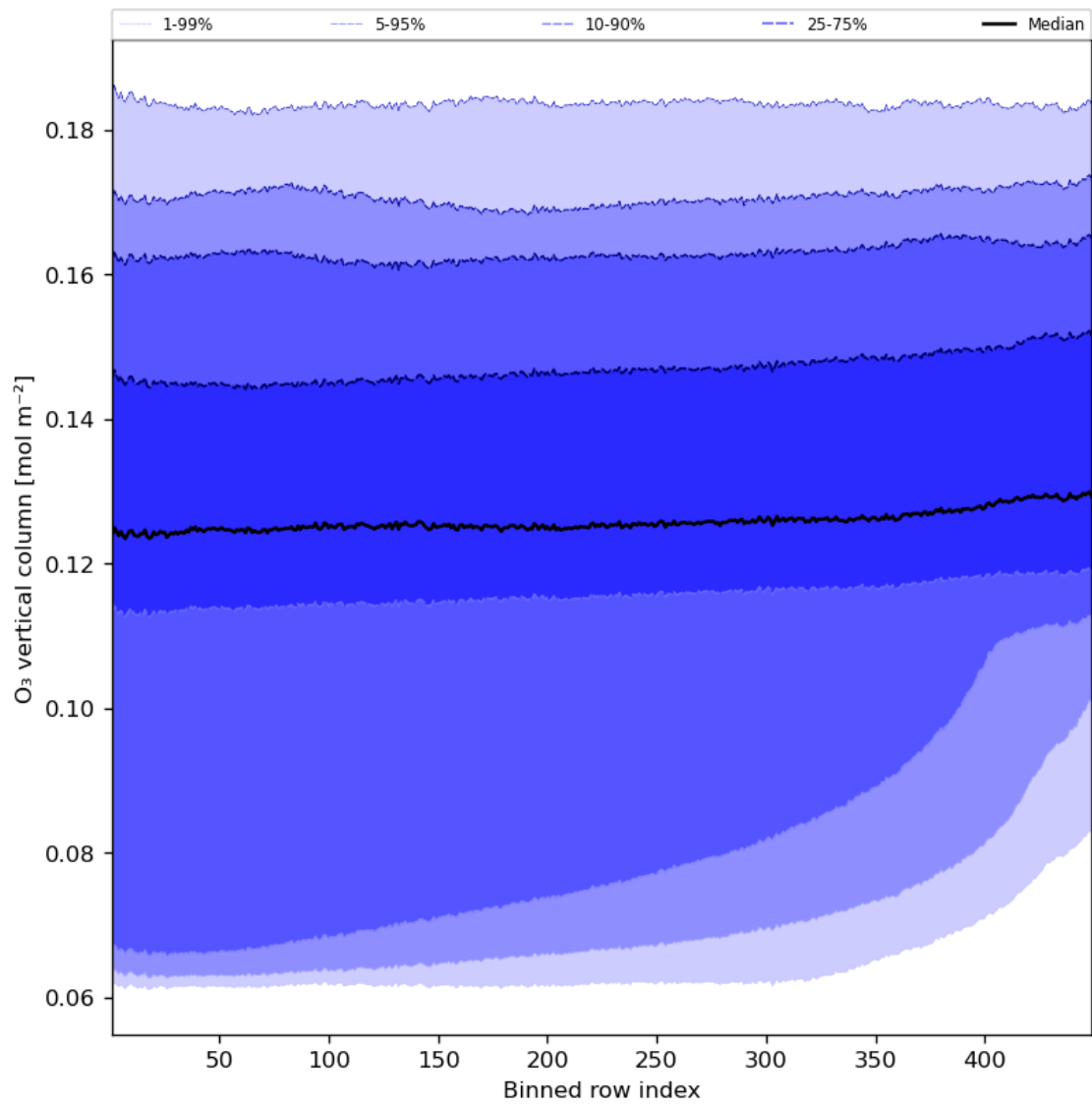
Figure 28: Along track statistics of “O 3 vertical column” for 2023-10-27 to 2023-10-28
