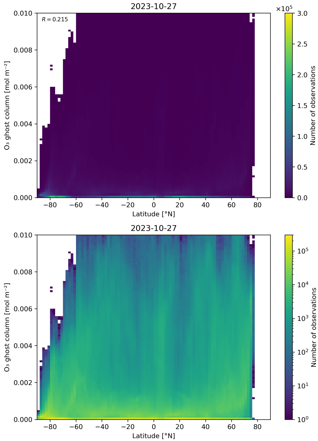
Figure 35: Scatter density plot of “Latitude” against “O 3 ghost column” for 2023-10-27 to 2023-10-28.
