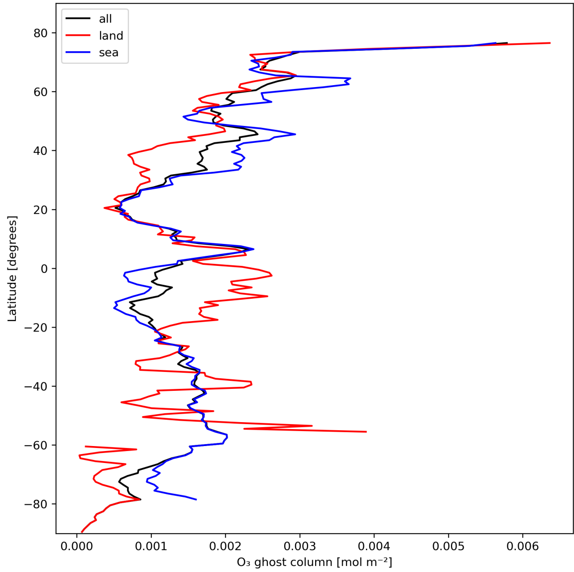
Figure 18: Zonal average of "O 3 ghost column" for 2023-10-27 to 2023-10-28.
