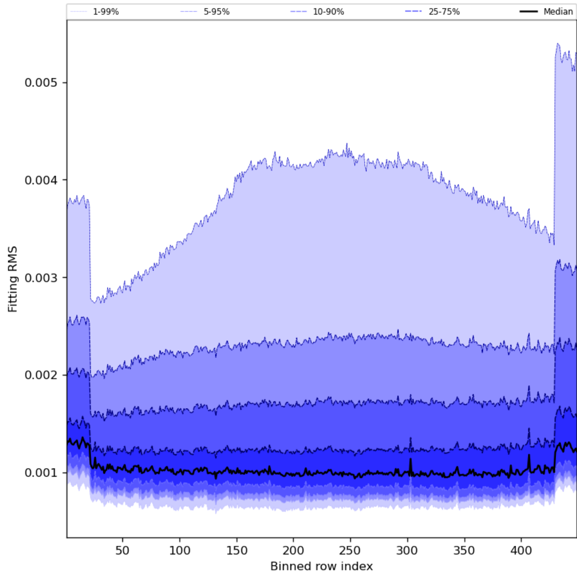
Figure 30: Along track statistics of “Fitting RMS” for 2023-10-27 to 2023-10-28
