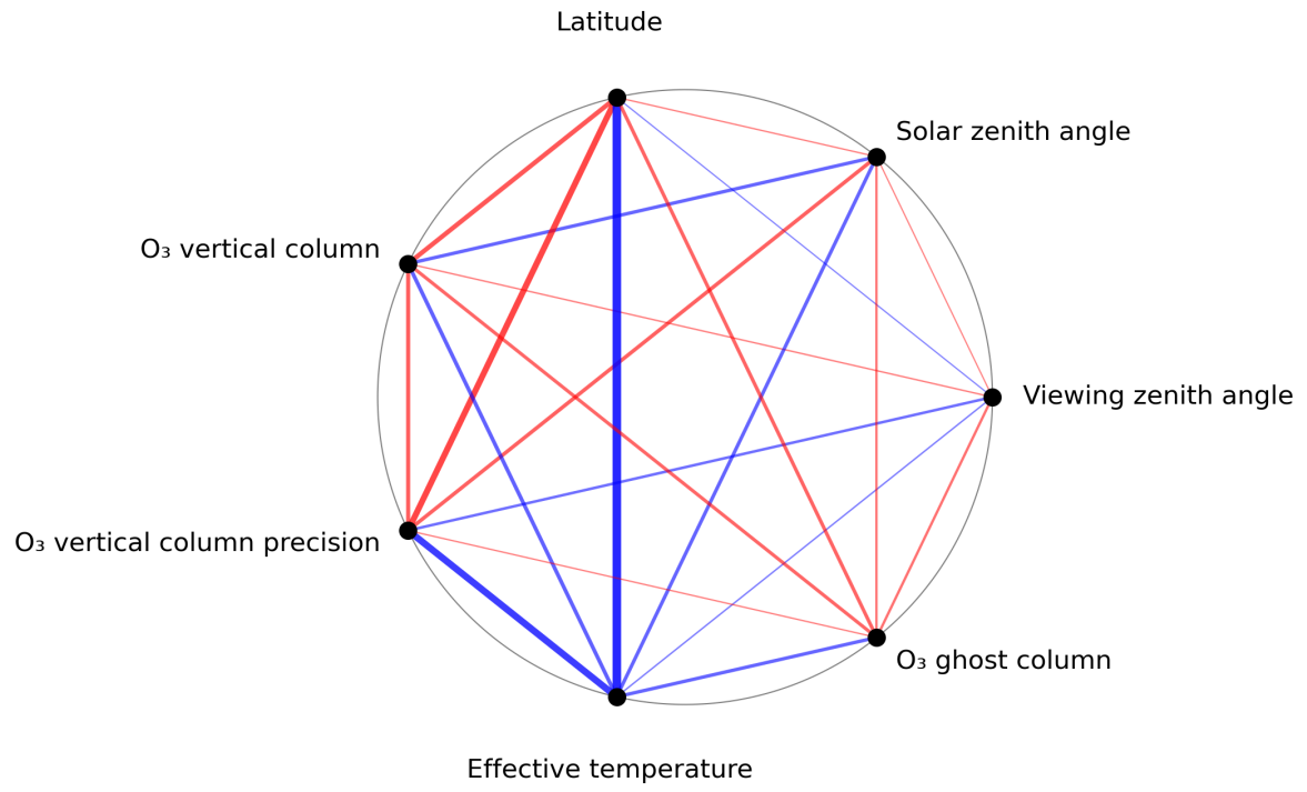
Figure 1: Map of correlation graph for 2023-10-27 to 2023-10-28.
