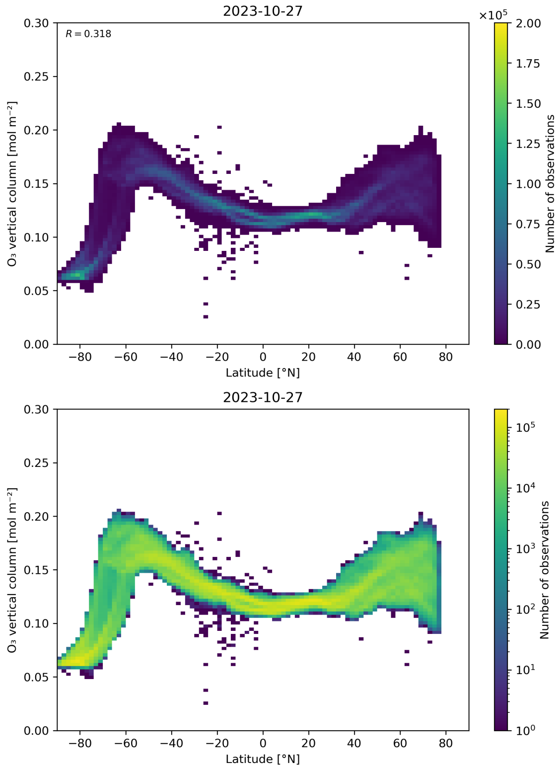
Figure 36: Scatter density plot of “Latitude” against “O 3 vertical column” for 2023-10-27 to 2023-10-28.
