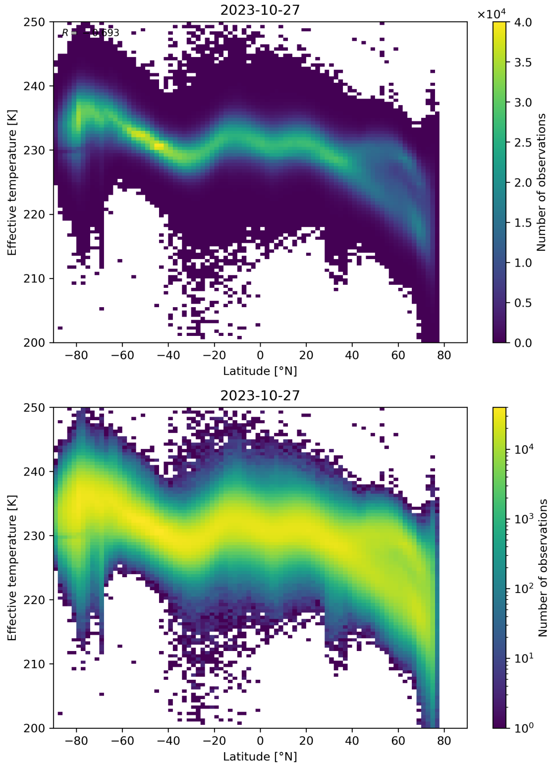
Figure 34: Scatter density plot of “Latitude” against “Effective temperature” for 2023-10-27 to 2023-10-28.
