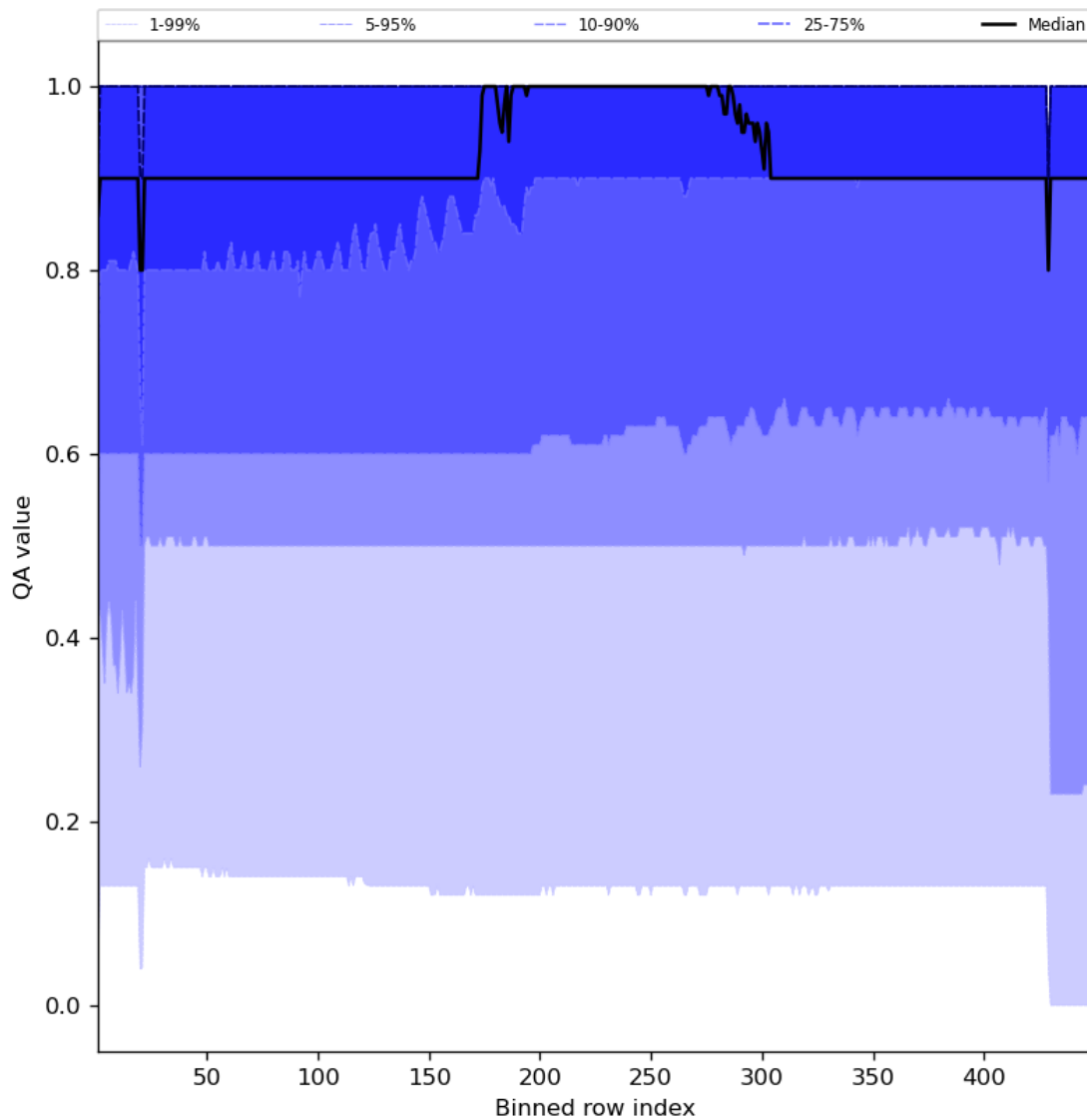
Figure 27: Along track statistics of “QA value” for 2023-10-27 to 2023-10-28
