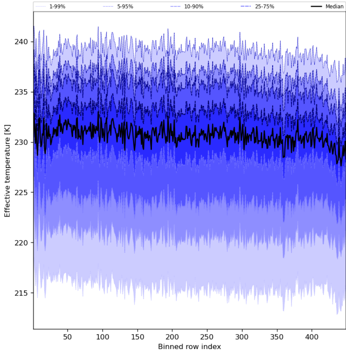
Figure 31: Along track statistics of “Effective temperature” for 2023-10-27 to 2023-10-28
