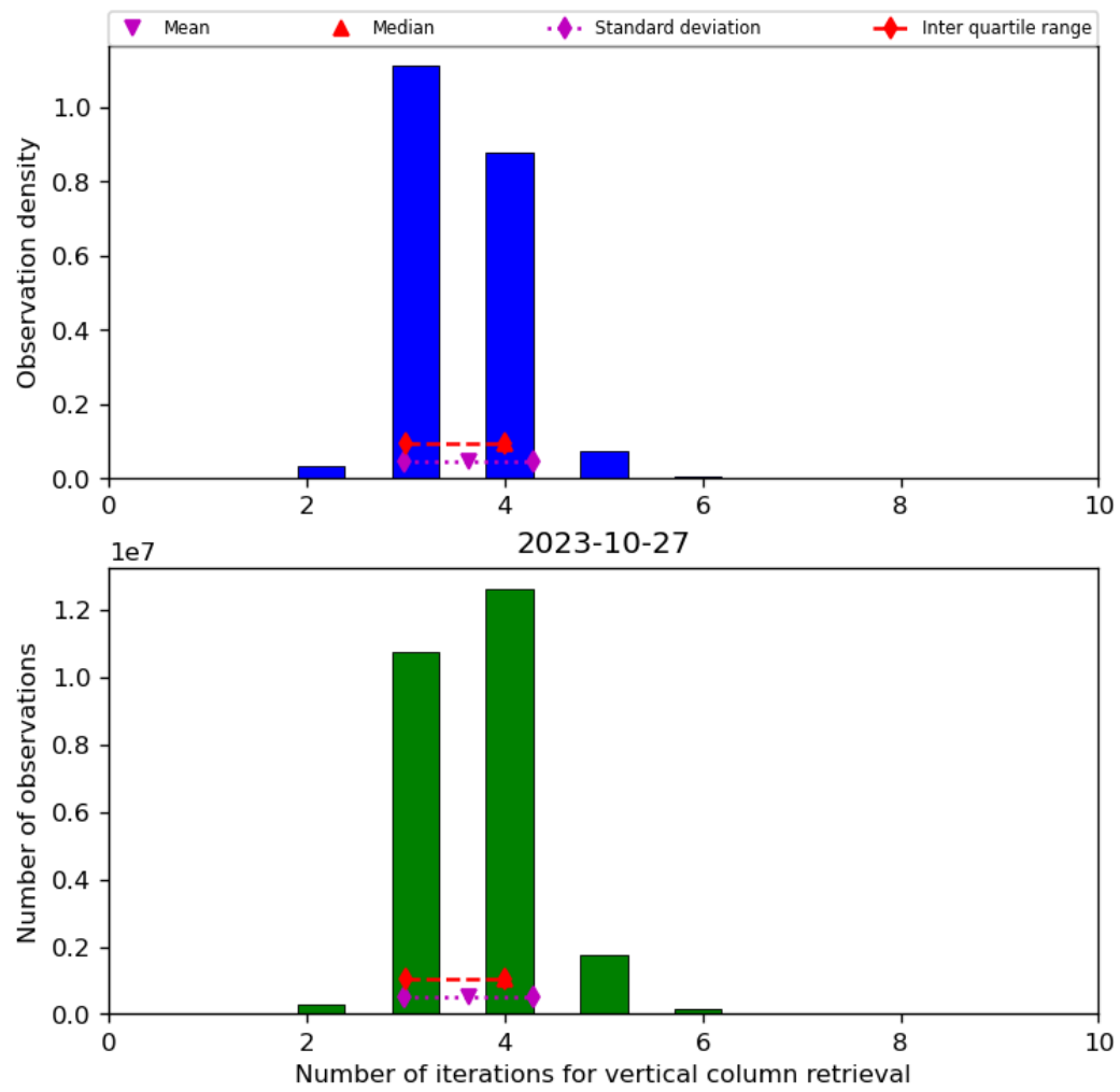
Figure 26: Histogram of "Number of iterations for vertical column retrieval" for 2023-10-27 to 2023-10-28
