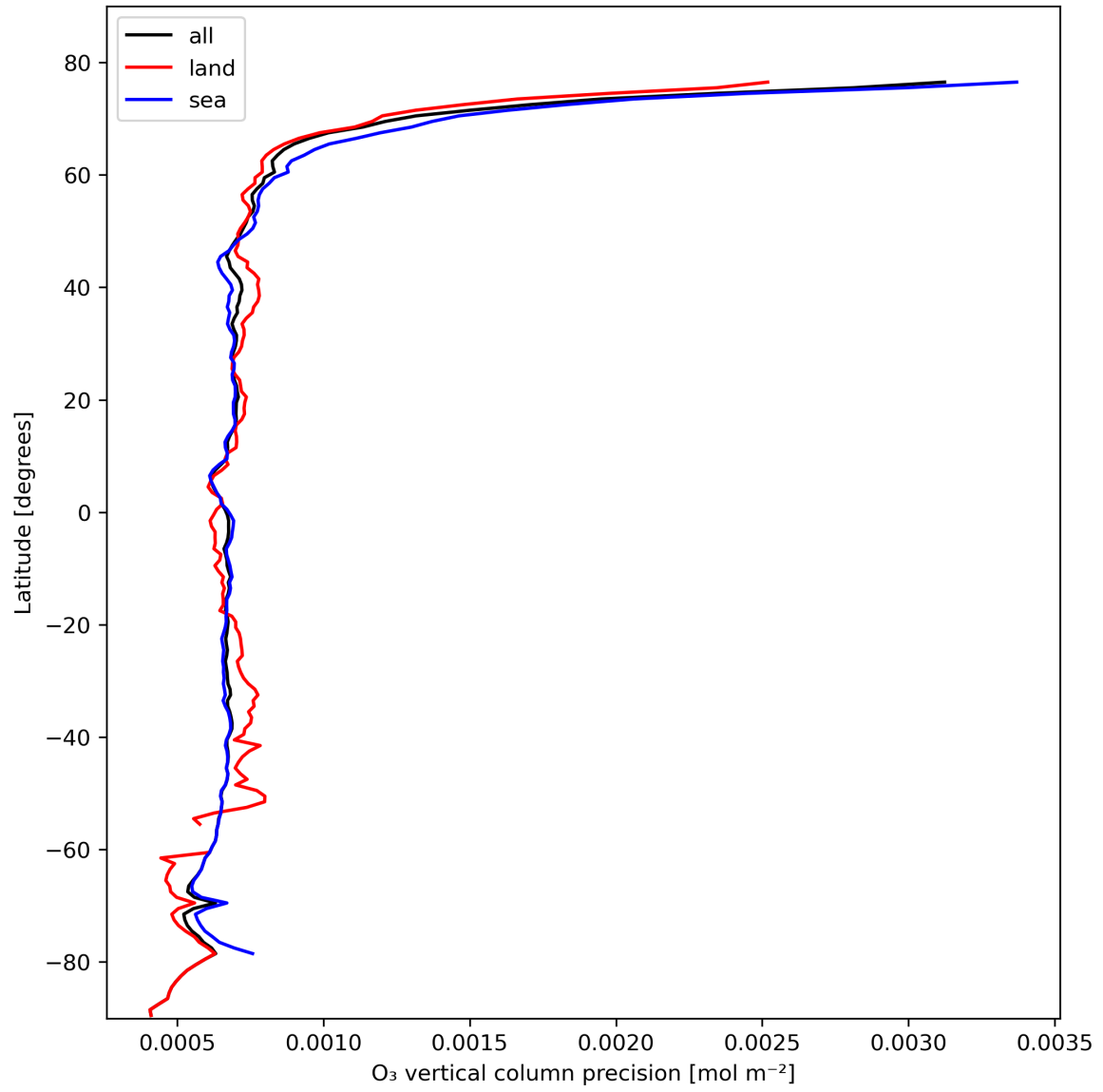
Figure 15: Zonal average of "O 3 vertical column precision" for 2023-10-27 to 2023-10-28.
