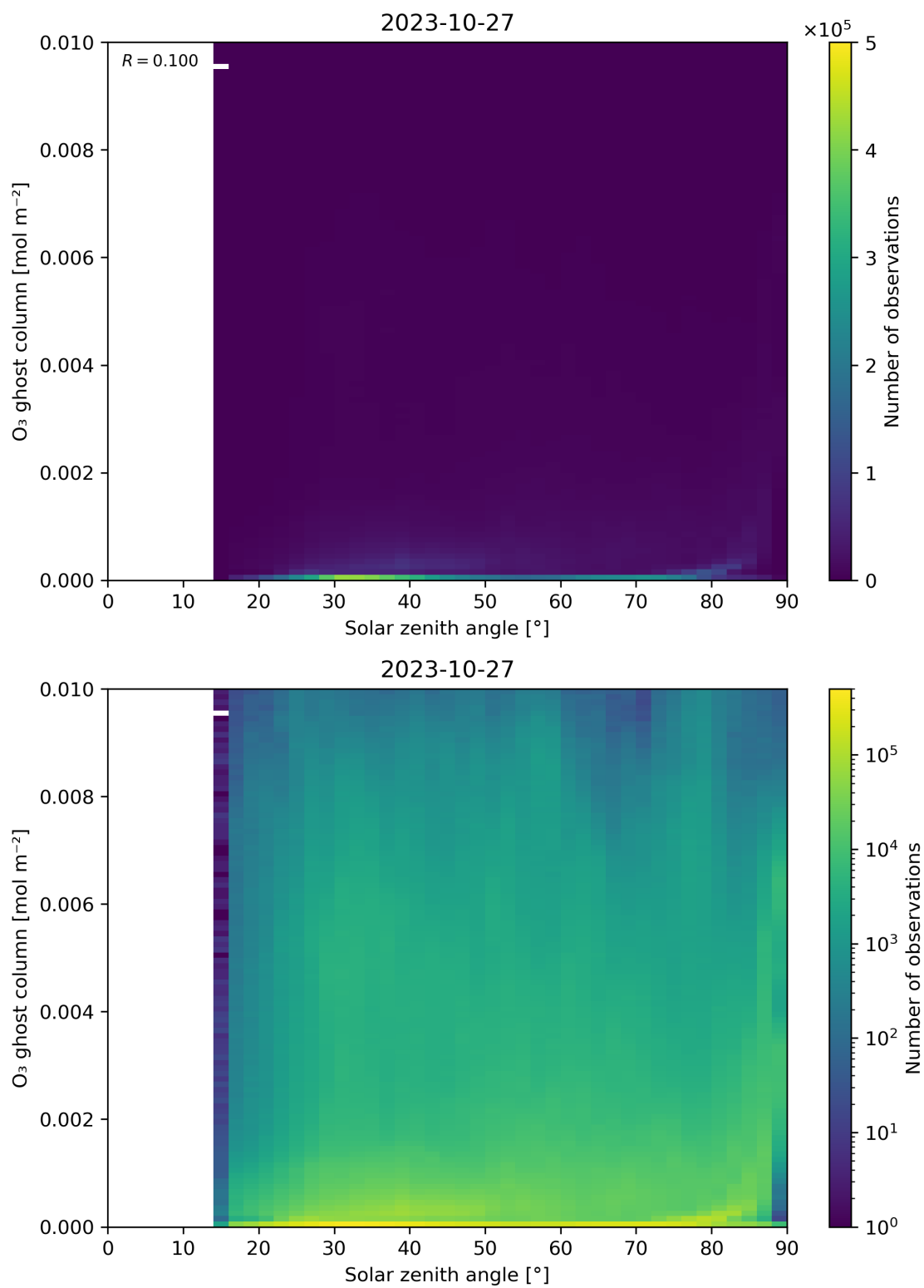
Figure 46: Scatter density plot of “Solar zenith angle” against “O 3 ghost column” for 2023-10-27 to 2023-10-28.
