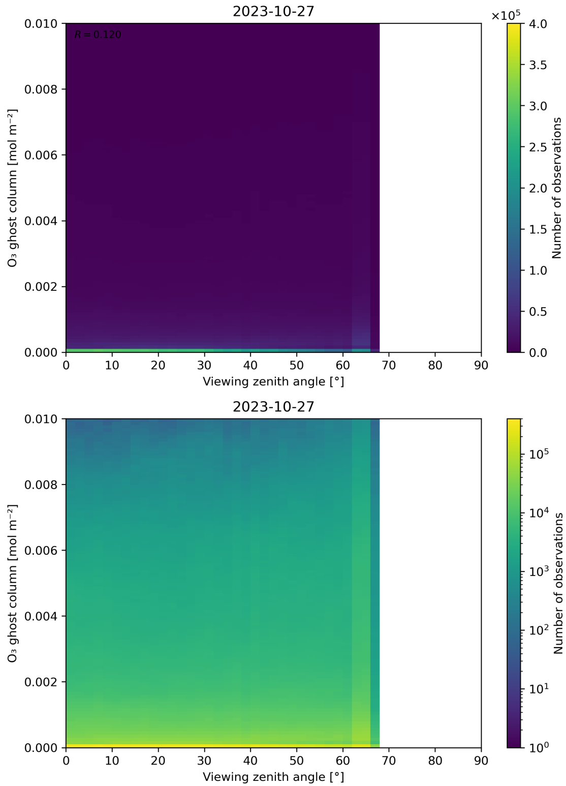
Figure 51: Scatter density plot of “Viewing zenith angle” against “O 3 ghost column” for 2023-10-27 to 2023-10-28.
