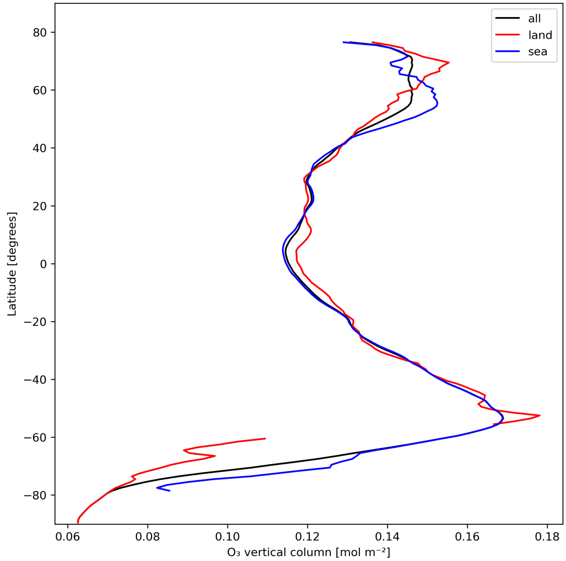
Figure 14: Zonal average of “O 3 vertical column” for 2023-10-27 to 2023-10-28.
