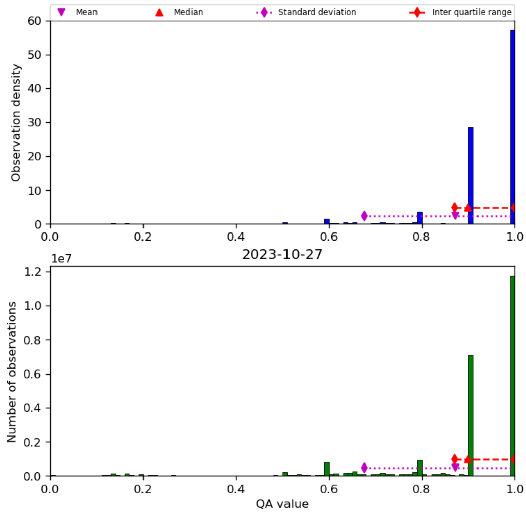
Figure 20: Histogram of “QA value” for 2023-10-27 to 2023-10-28
