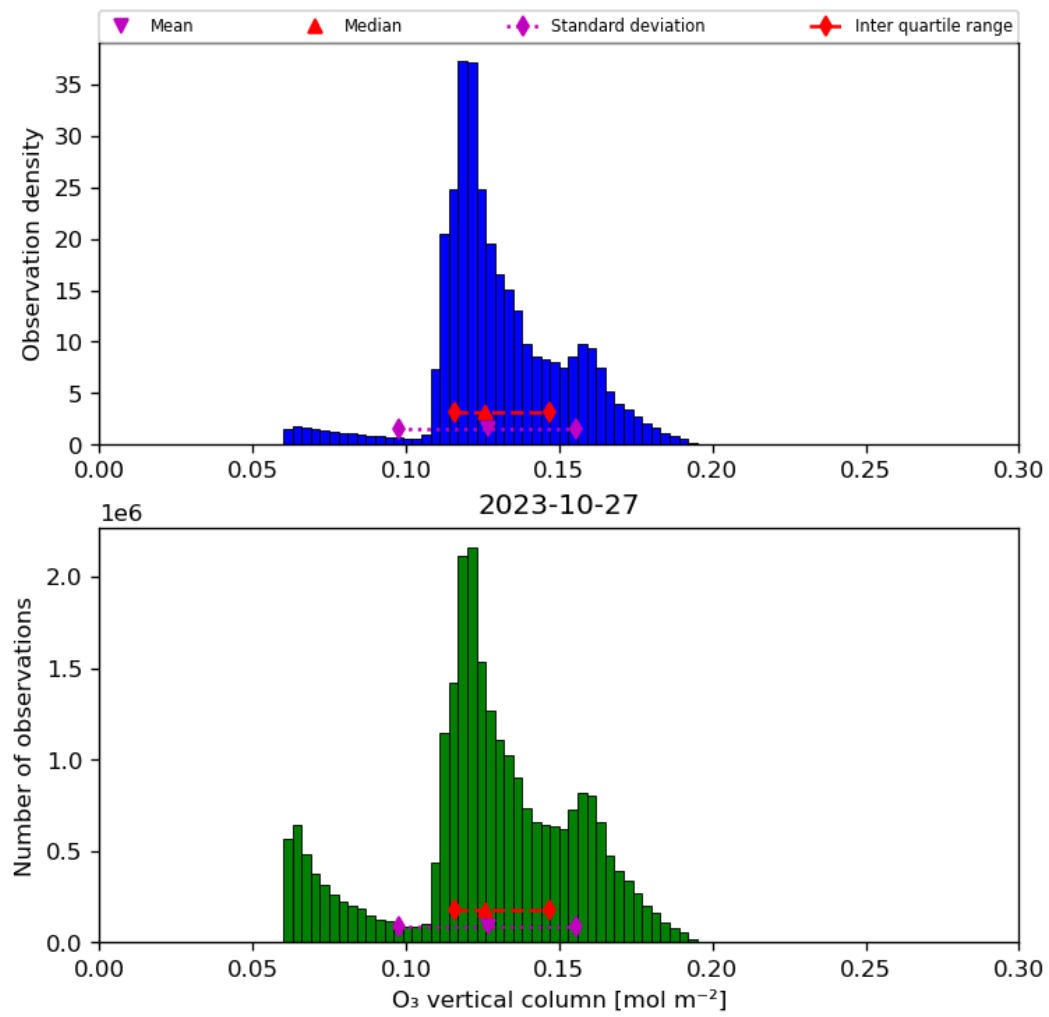
Figure 21: Histogram of “O 3 vertical column” for 2023-10-27 to 2023-10-28
