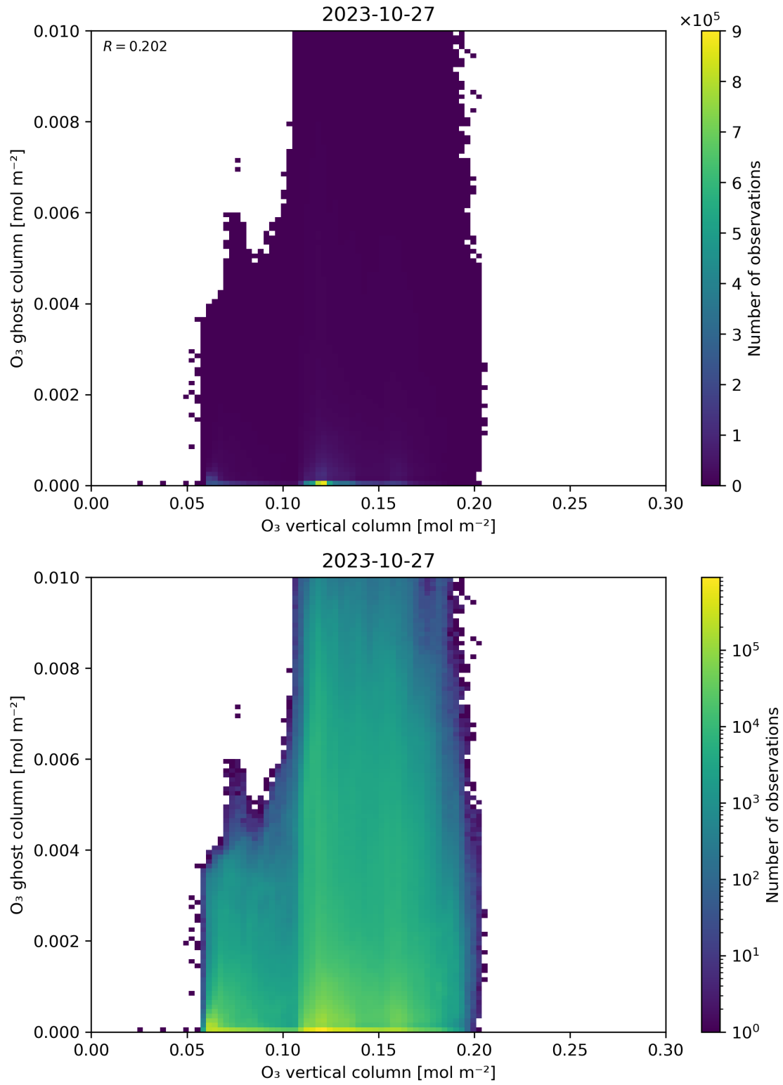
Figure 40: Scatter density plot of “O 3 vertical column” against “O 3 ghost column” for 2023-10-27 to 2023-10-28.
