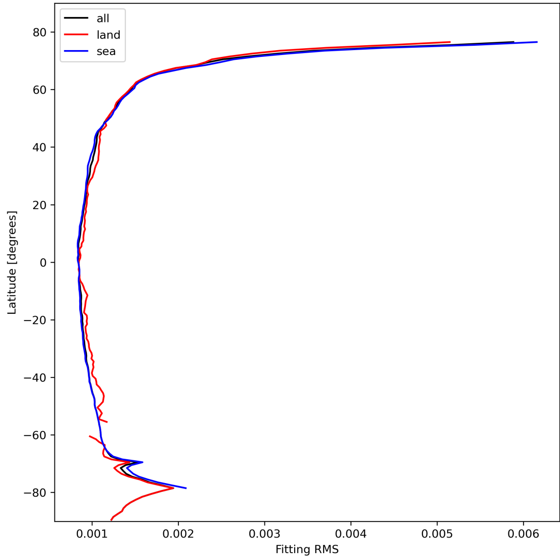
Figure 16: Zonal average of “Fitting RMS” for 2023-10-27 to 2023-10-28.
