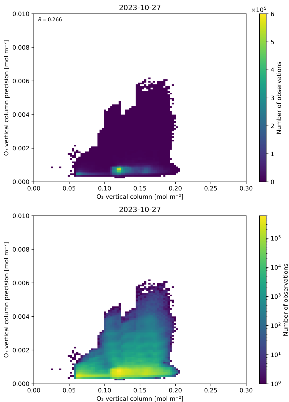
Figure 41: Scatter density plot of “O 3 vertical column” against “O 3 vertical column precision” for 2023-10-27 to 2023-10-28.
