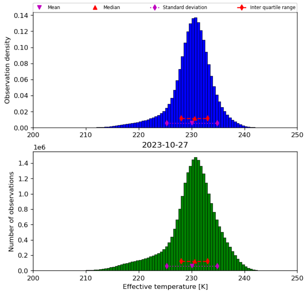
Figure 24: Histogram of “Effective temperature” for 2023-10-27 to 2023-10-28
