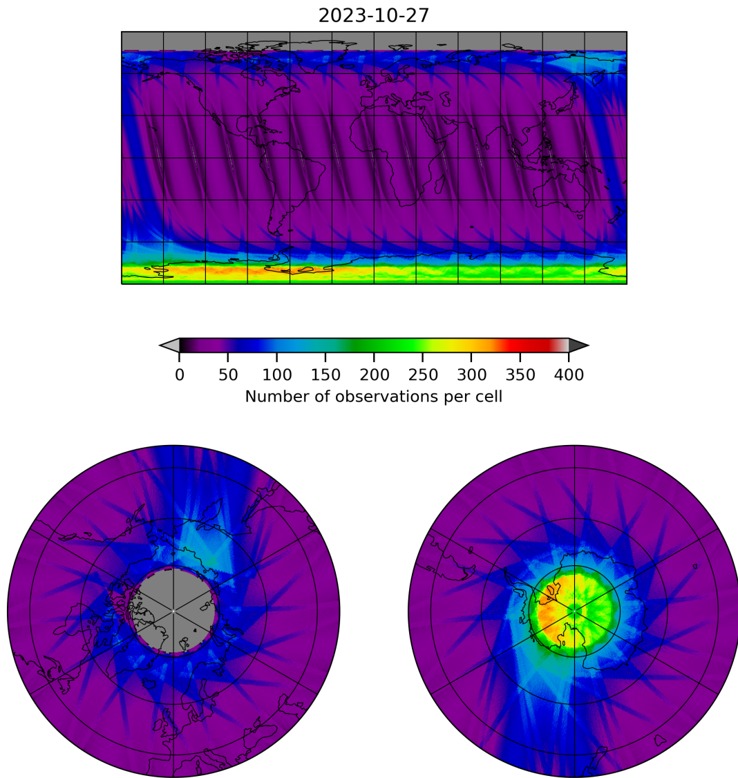
Figure 12: Map of the number of observations for 2023-10-27 to 2023-10-28
