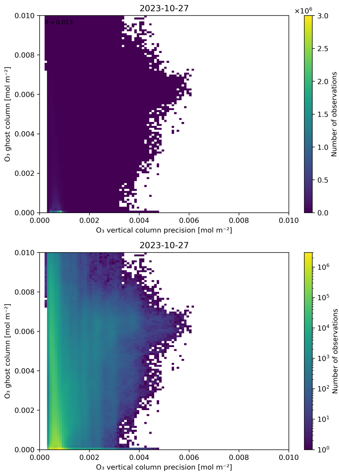
Figure 43: Scatter density plot of “ \text{O}_3 vertical column precision” against “ \text{O}_3 ghost column” for 2023-10-27 to 2023-10-28.
