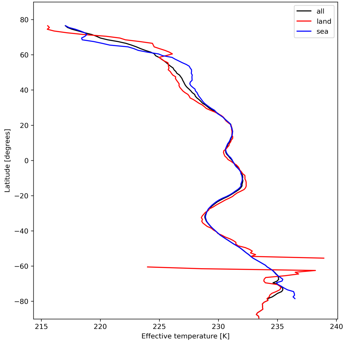
Figure 17: Zonal average of "Effective temperature" for 2023-10-27 to 2023-10-28.
