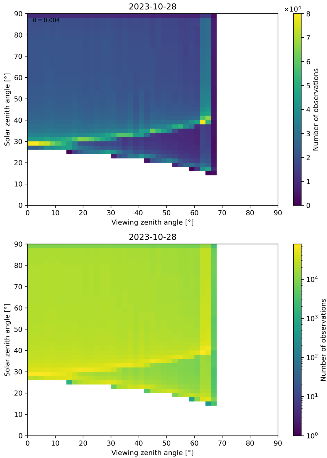
Figure 54: Scatter density plot of “Viewing zenith angle” against “Solar zenith angle” for 2023-10-28 to 2023-10-29.
