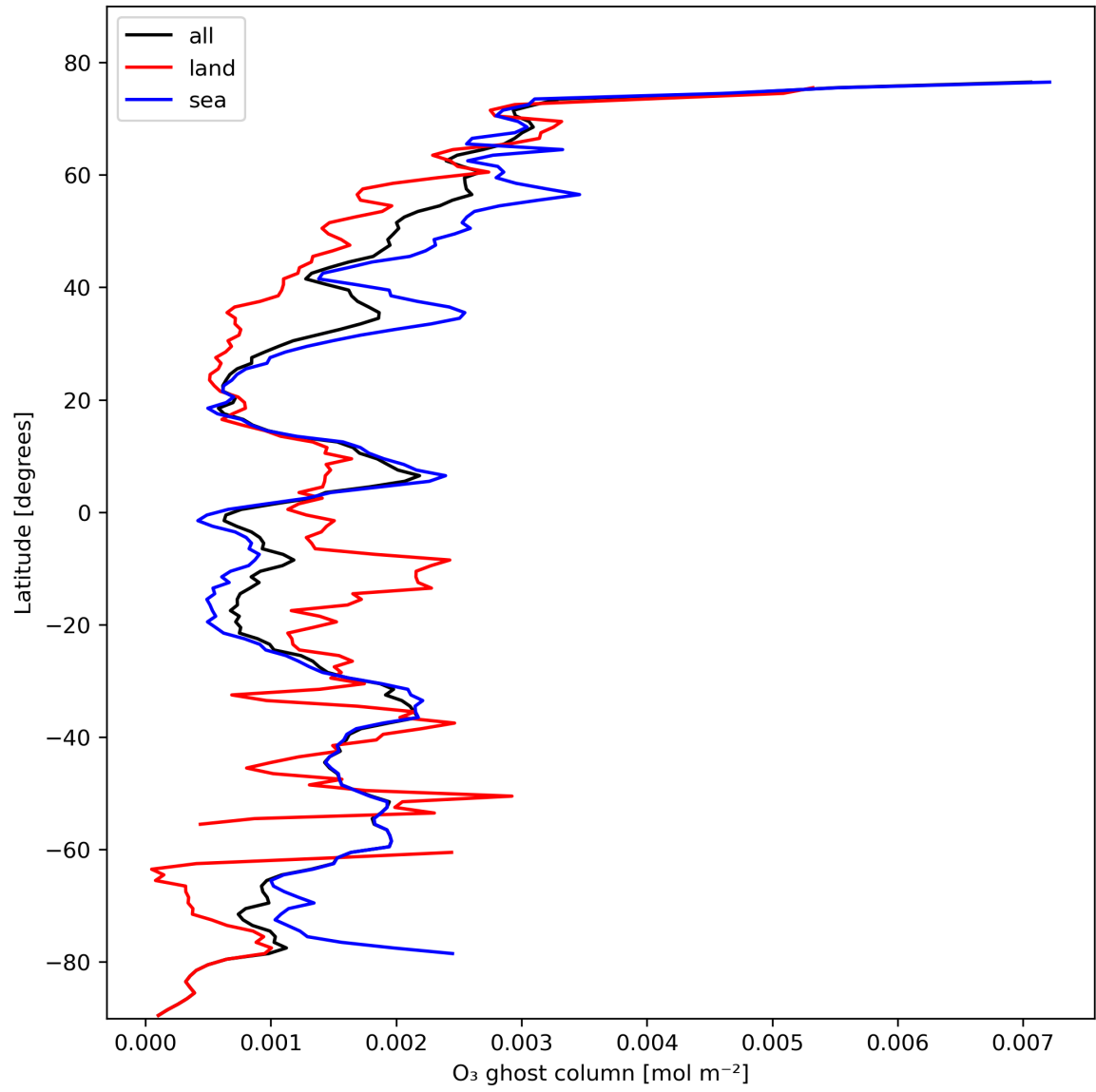
Figure 18: Zonal average of "O 3 ghost column" for 2023-10-28 to 2023-10-29.
