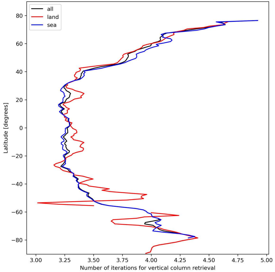
Figure 19: Zonal average of “Number of iterations for vertical column retrieval” for 2023-10-28 to 2023-10-29.
