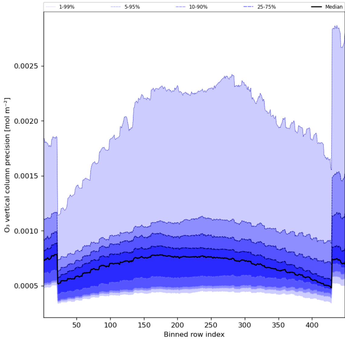
Figure 29: Along track statistics of “O 3 vertical column precision” for 2023-10-28 to 2023-10-29
