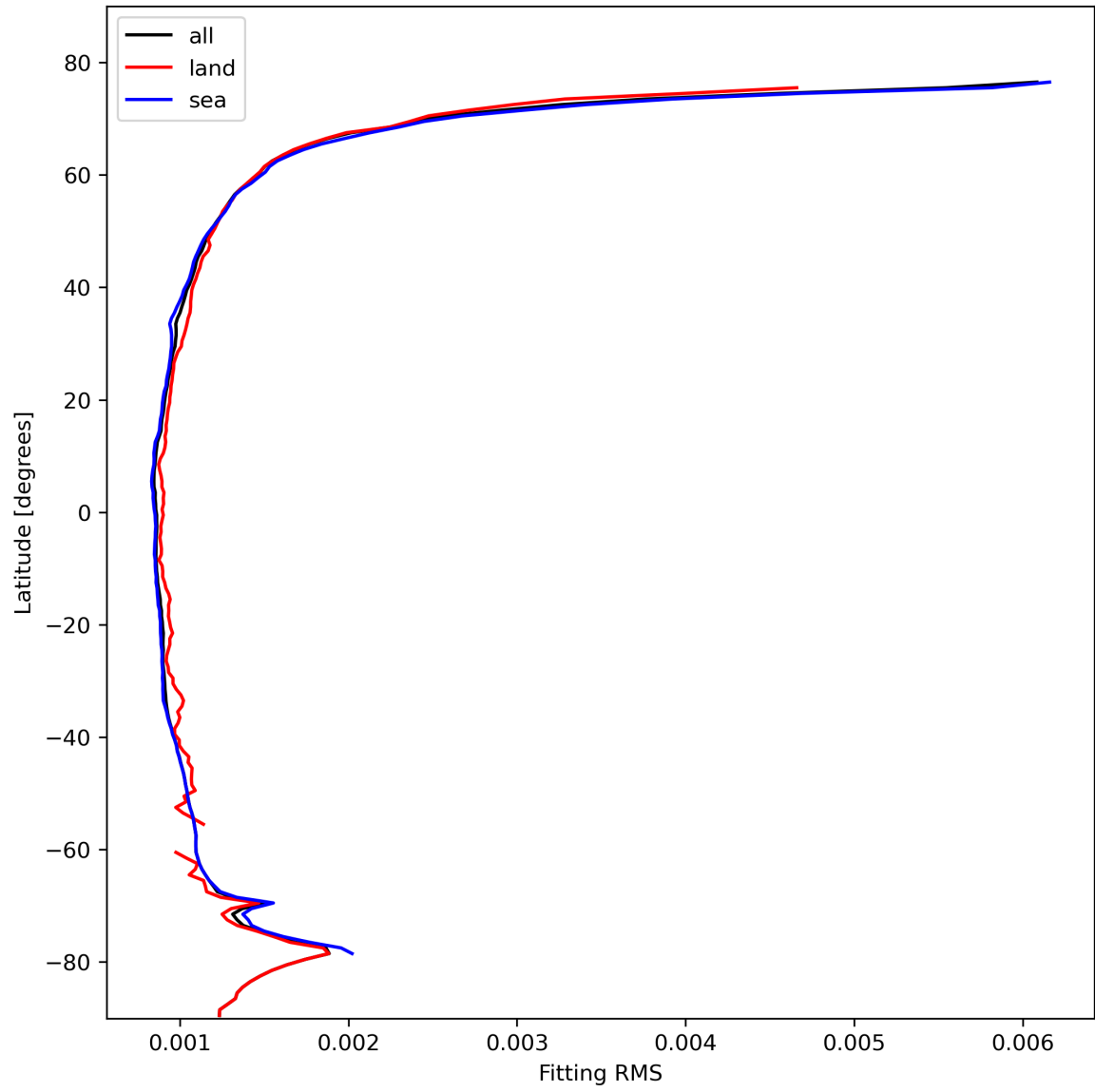
Figure 16: Zonal average of “Fitting RMS” for 2023-10-28 to 2023-10-29.
