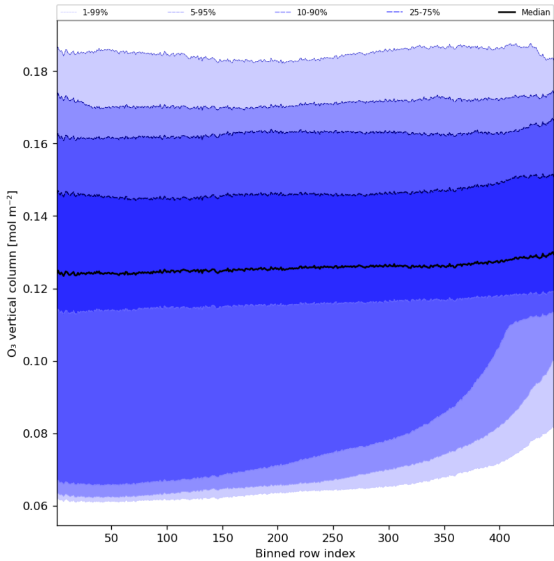
Figure 28: Along track statistics of “O 3 vertical column” for 2023-10-28 to 2023-10-29
