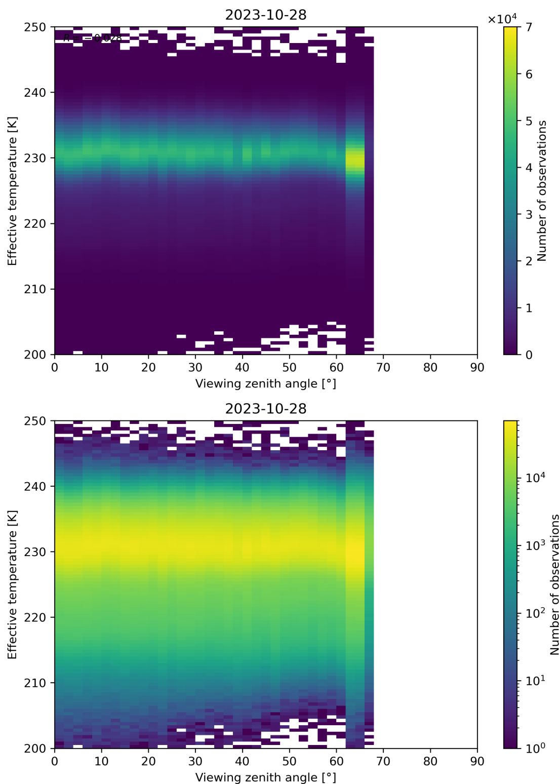
Figure 50: Scatter density plot of “Viewing zenith angle” against “Effective temperature” for 2023-10-28 to 2023-10-29.
