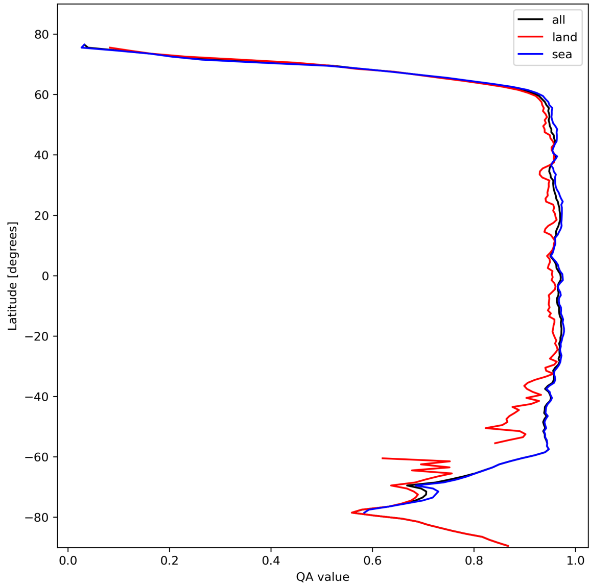
Figure 13: Zonal average of “QA value” for 2023-10-28 to 2023-10-29.
