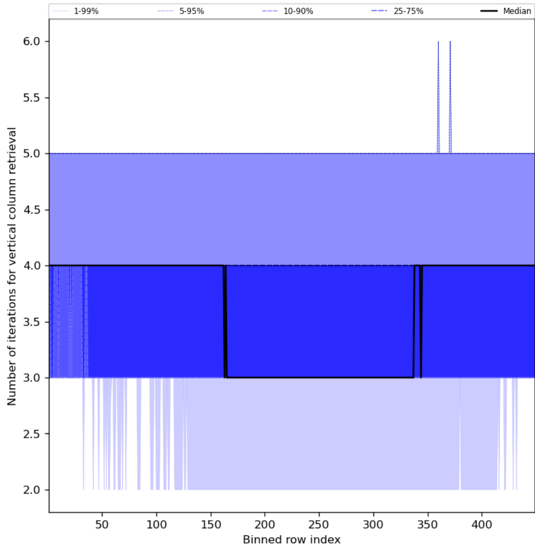
Figure 33: Along track statistics of “Number of iterations for vertical column retrieval” for 2023-10-28 to 2023-10-29
