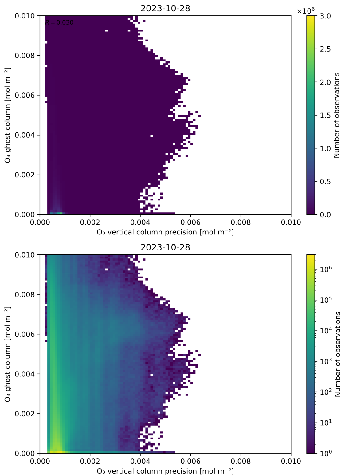
Figure 43: Scatter density plot of “O 3 vertical column precision” against “O 3 ghost column” for 2023-10-28 to 2023-10-29.
