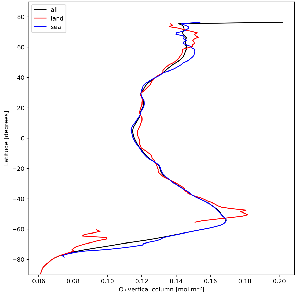
Figure 14: Zonal average of “O 3 vertical column” for 2023-10-28 to 2023-10-29.
