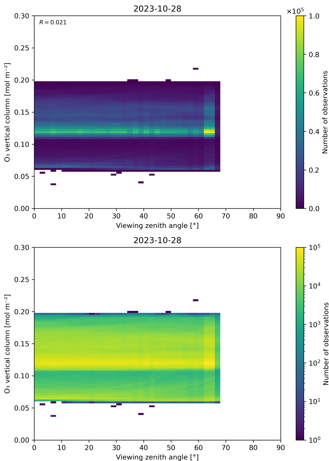
Figure 52: Scatter density plot of “Viewing zenith angle” against “O 3 vertical column” for 2023-10-28 to 2023-10-29.
