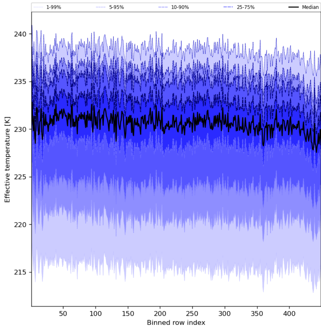
Figure 31: Along track statistics of “Effective temperature” for 2023-10-28 to 2023-10-29
