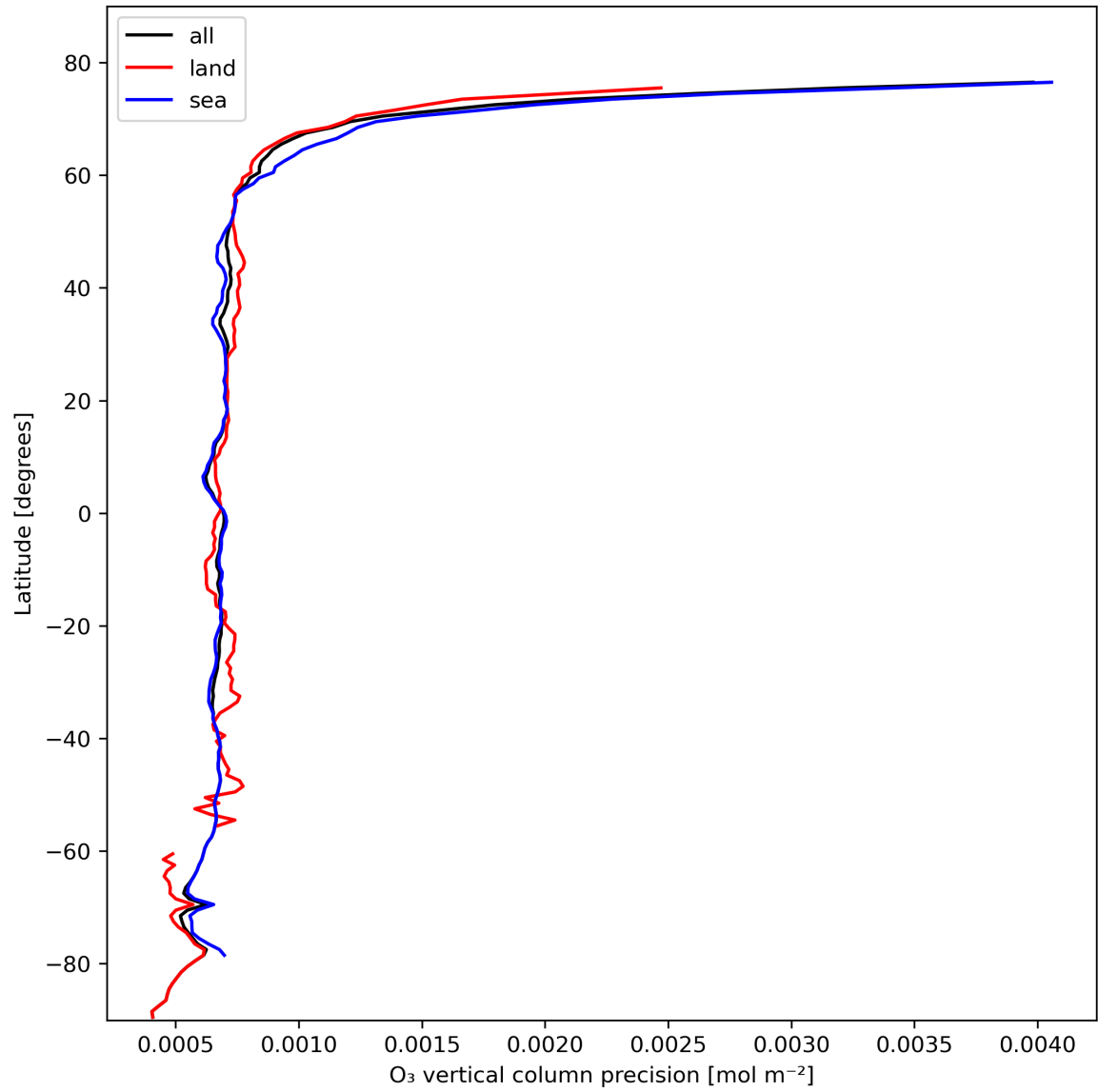
Figure 15: Zonal average of “O 3 vertical column precision” for 2023-10-28 to 2023-10-29.
