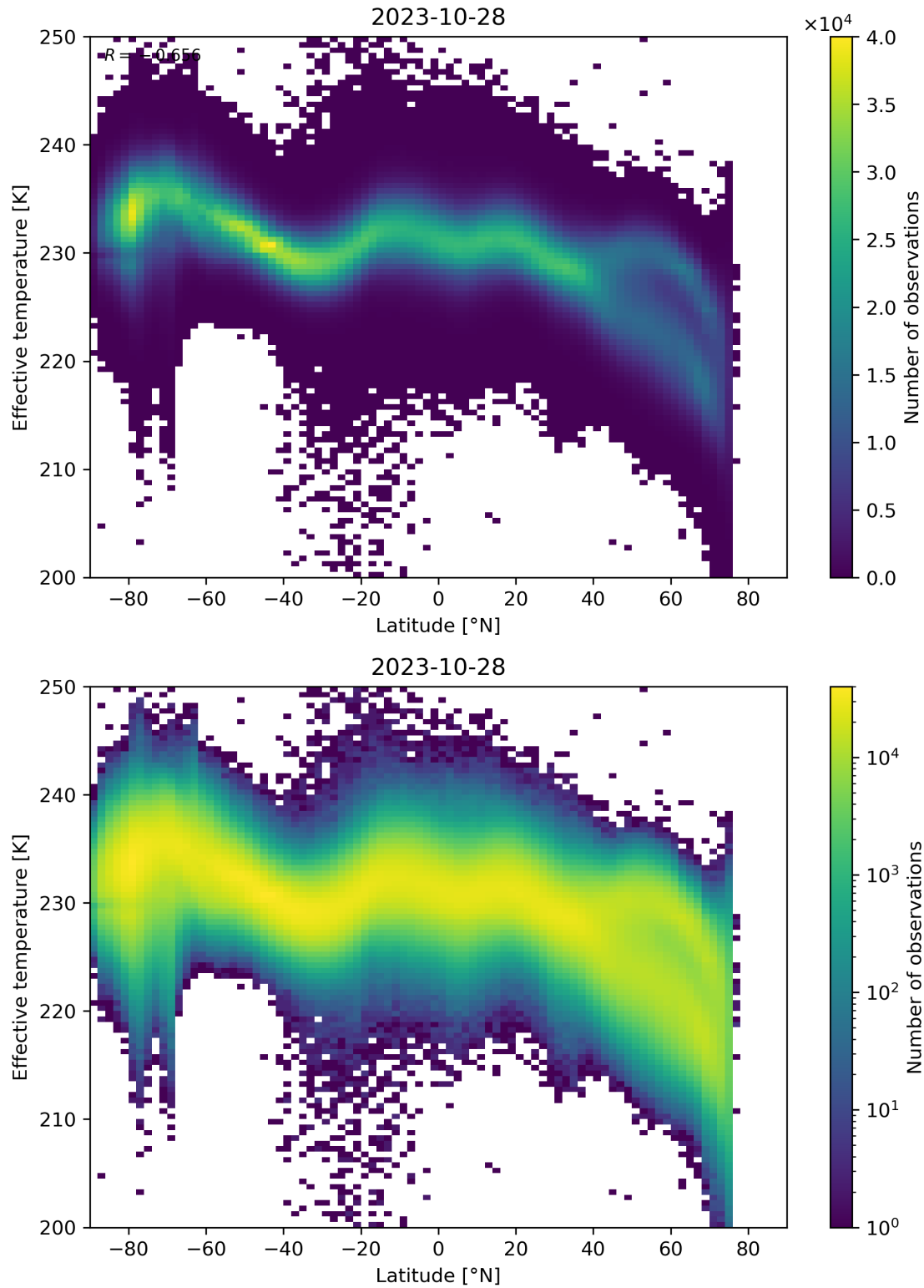
Figure 34: Scatter density plot of “Latitude” against “Effective temperature” for 2023-10-28 to 2023-10-29.
