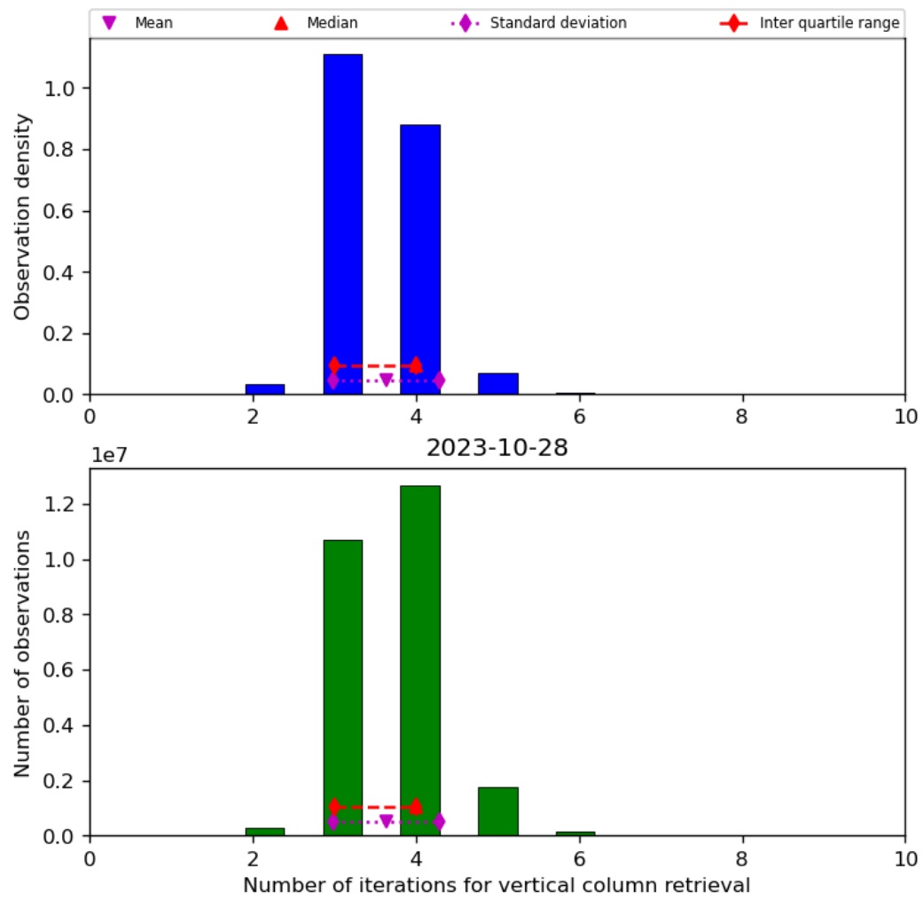
Figure 26: Histogram of “Number of iterations for vertical column retrieval” for 2023-10-28 to 2023-10-29
