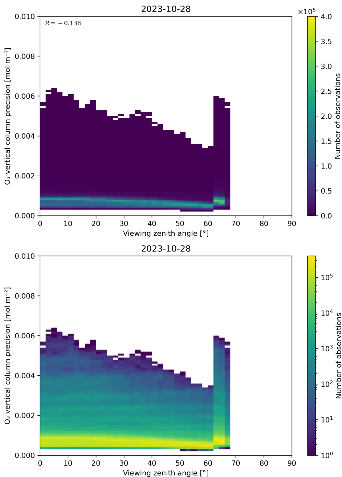
Figure 53: Scatter density plot of “Viewing zenith angle” against “O 3 vertical column precision” for 2023-10-28 to 2023-10-29.
