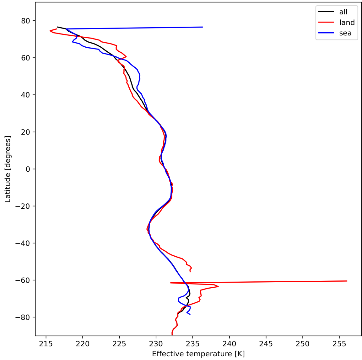
Figure 17: Zonal average of “Effective temperature” for 2023-10-28 to 2023-10-29.
