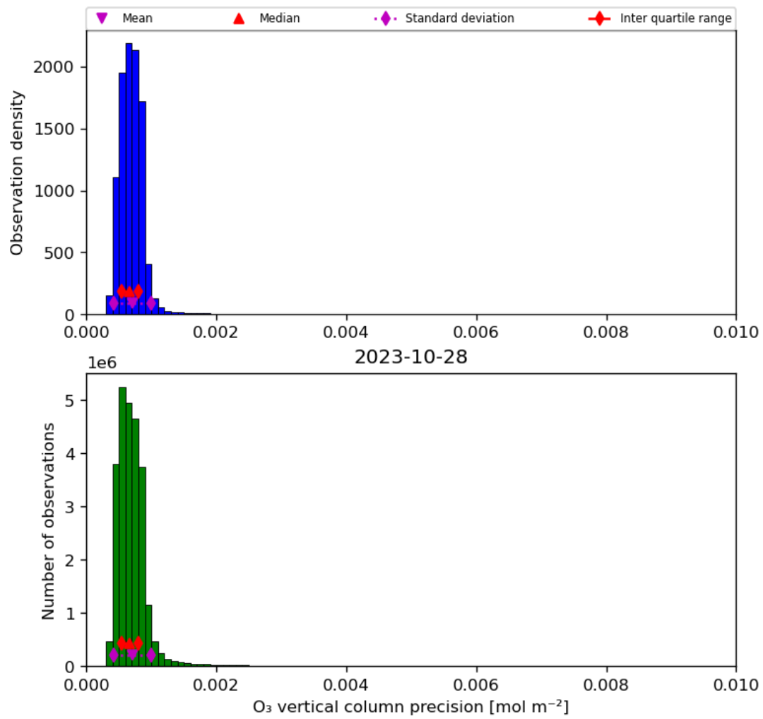
Figure 22: Histogram of “O 3 vertical column precision” for 2023-10-28 to 2023-10-29
