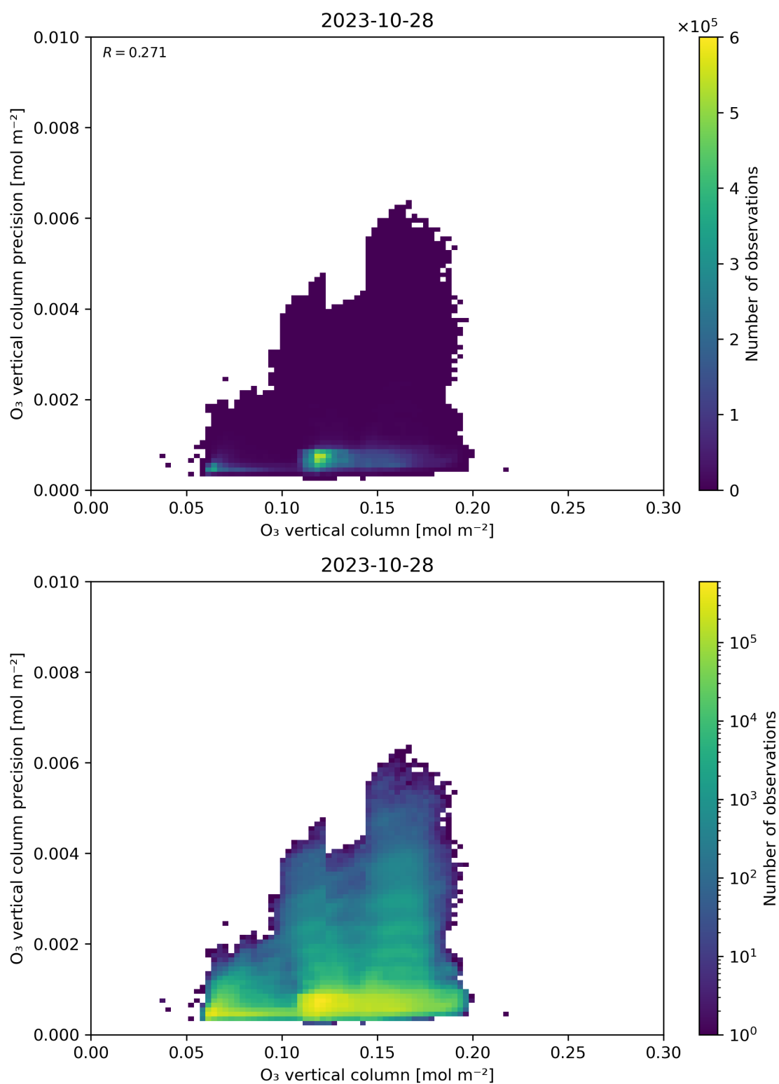
Figure 41: Scatter density plot of “O 3 vertical column” against “O 3 vertical column precision” for 2023-10-28 to 2023-10-29.
