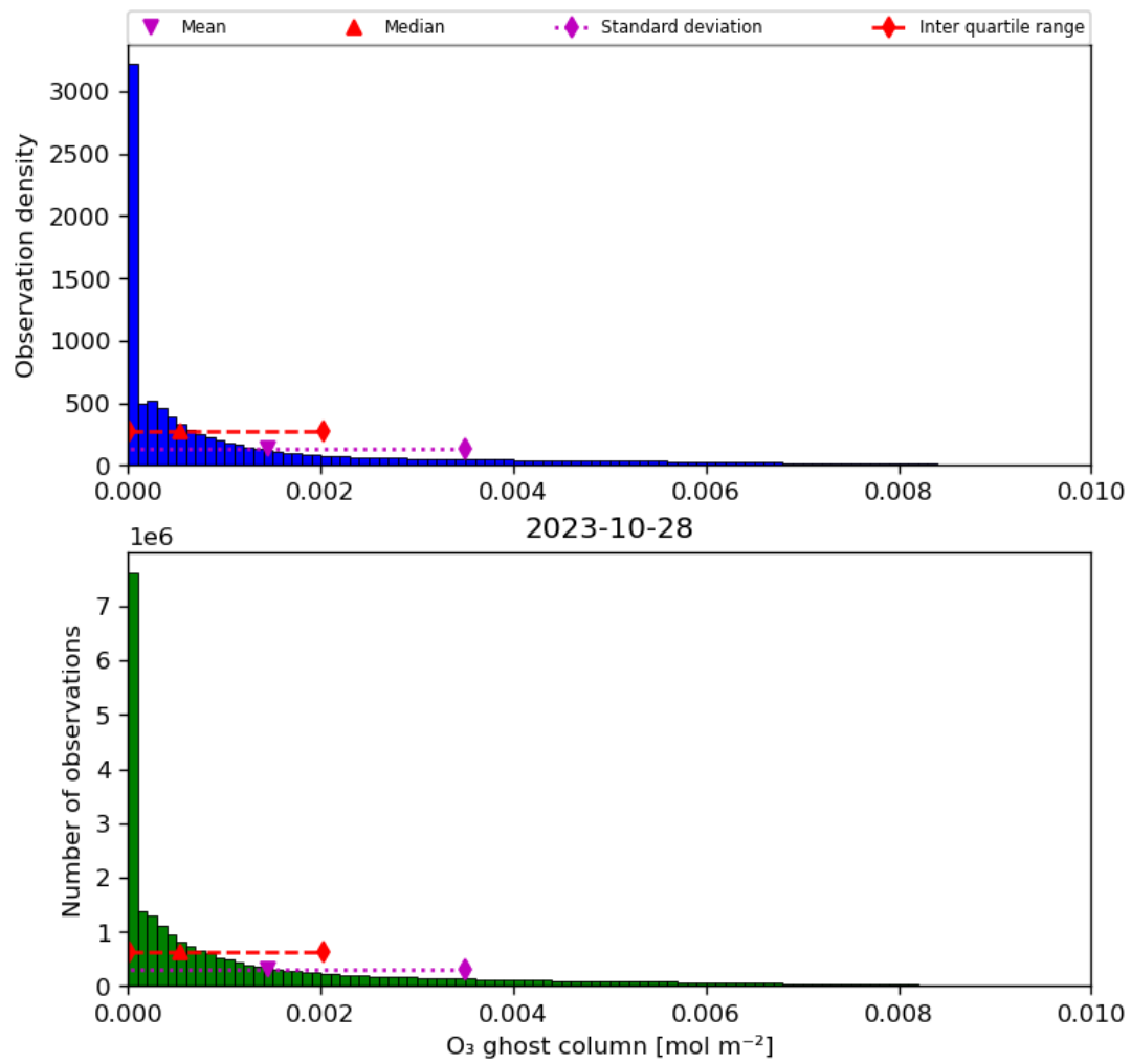
Figure 25: Histogram of “O 3 ghost column” for 2023-10-28 to 2023-10-29
