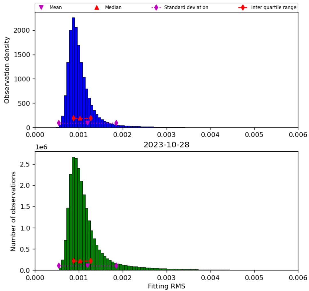
Figure 23: Histogram of “Fitting RMS” for 2023-10-28 to 2023-10-29
