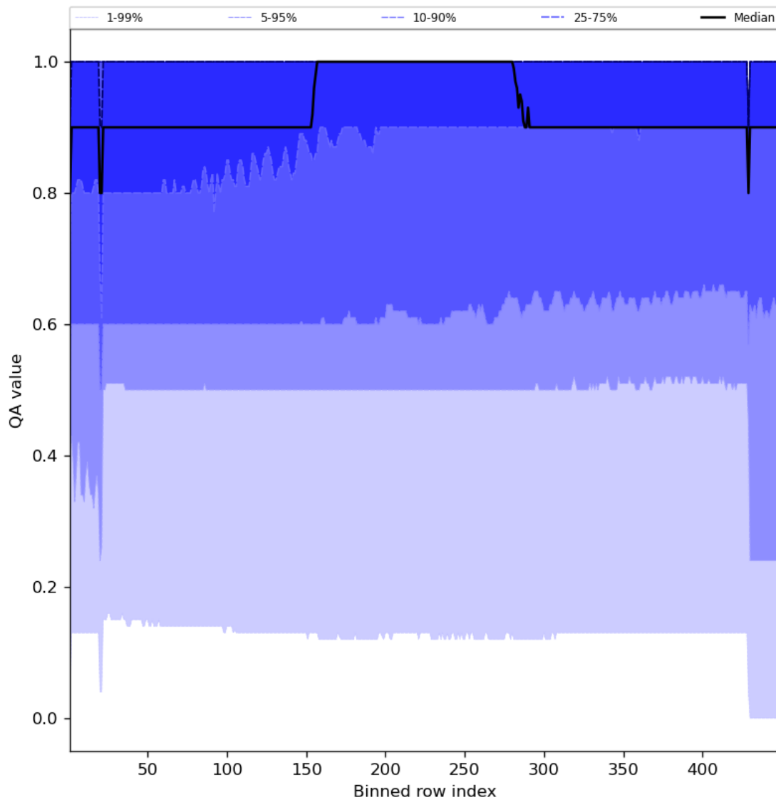
Figure 27: Along track statistics of “QA value” for 2023-10-28 to 2023-10-29
