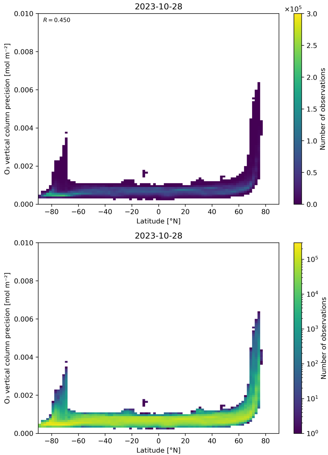
Figure 37: Scatter density plot of “Latitude” against “O 3 vertical column precision” for 2023-10-28 to 2023-10-29.
