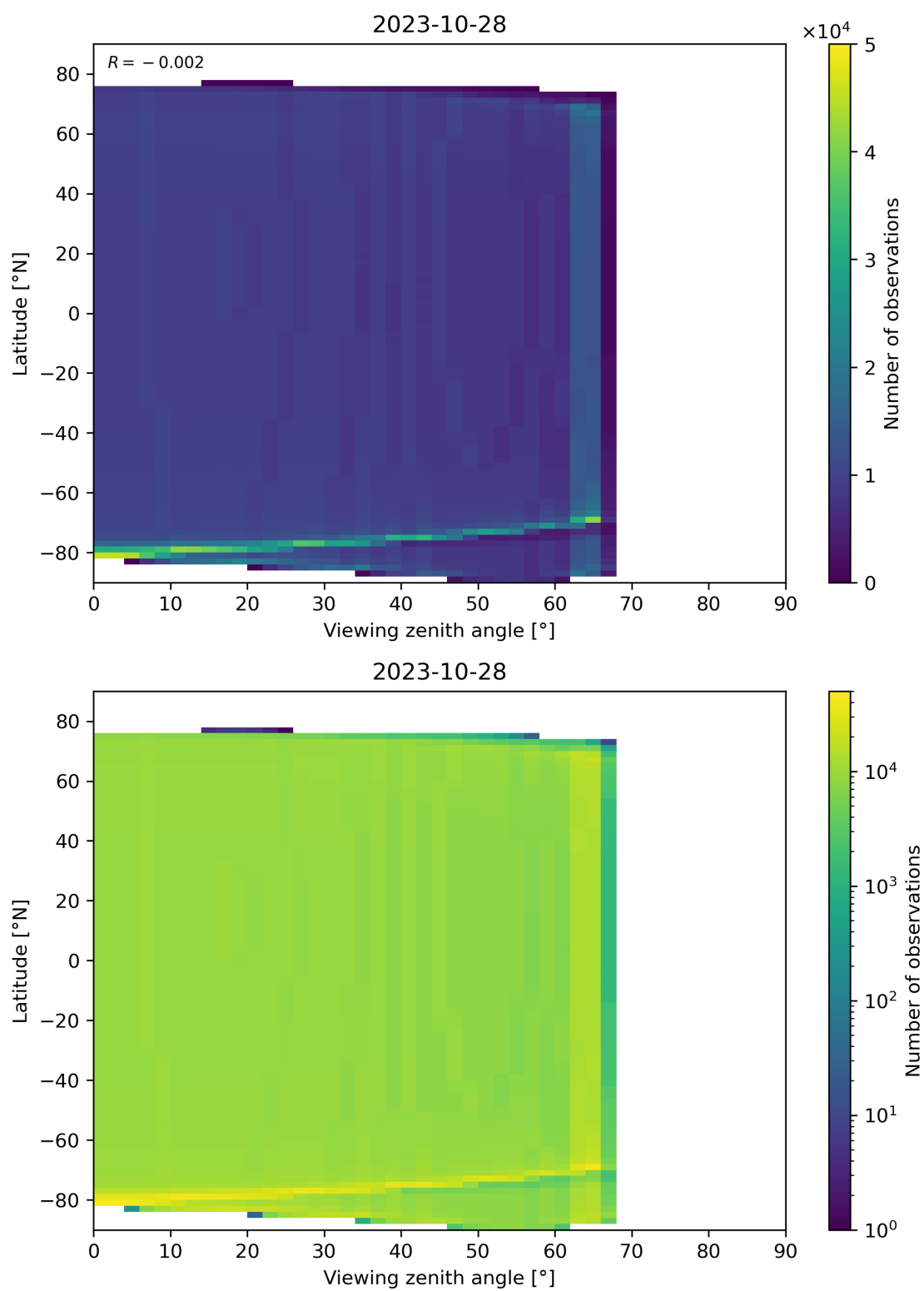
Figure 49: Scatter density plot of “Viewing zenith angle” against “Latitude” for 2023-10-28 to 2023-10-29.
