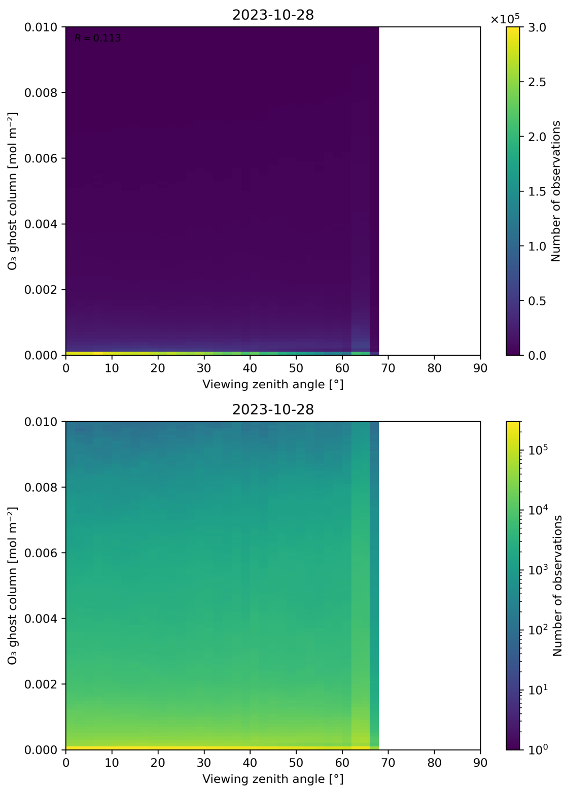
Figure 51: Scatter density plot of “Viewing zenith angle” against “O 3 ghost column” for 2023-10-28 to 2023-10-29.
