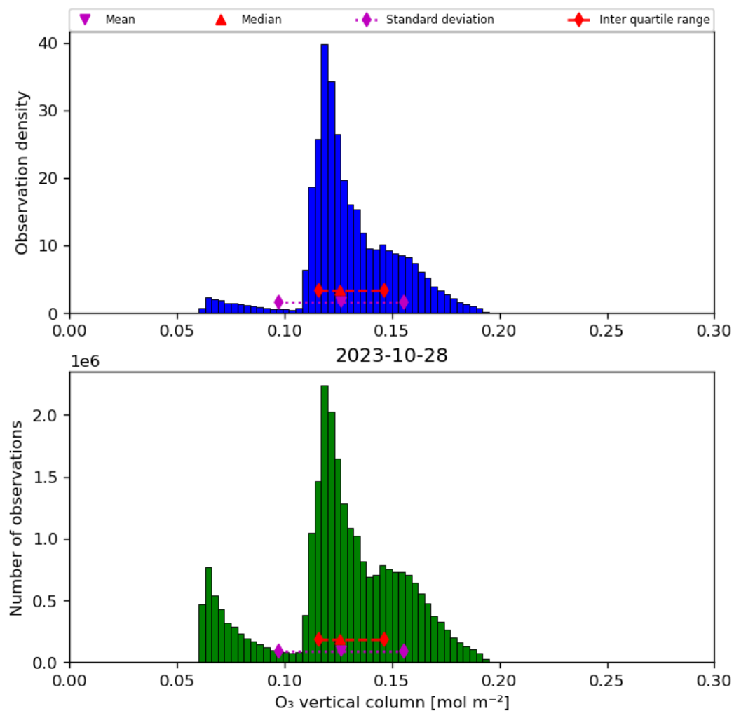
Figure 21: Histogram of “O 3 vertical column” for 2023-10-28 to 2023-10-29
