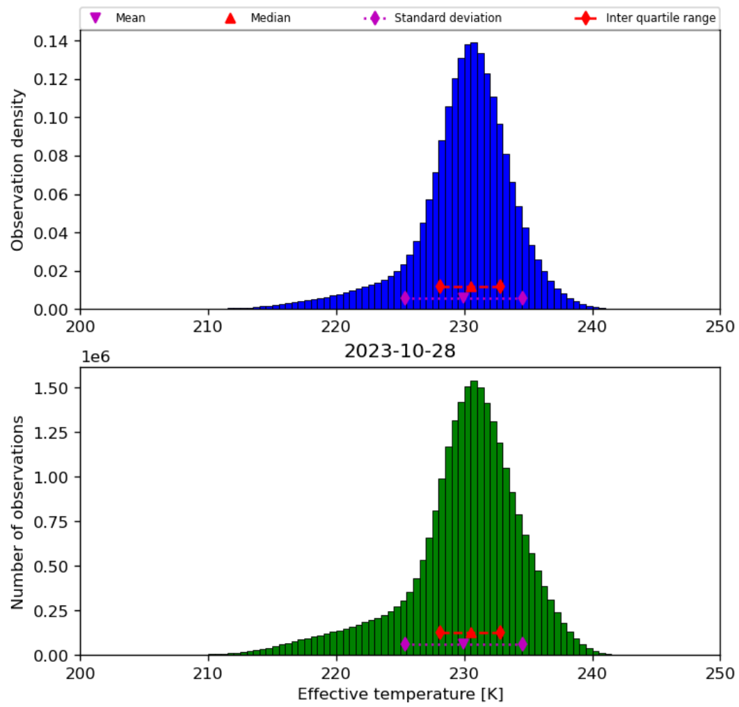
Figure 24: Histogram of “Effective temperature” for 2023-10-28 to 2023-10-29
