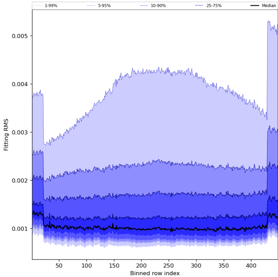
Figure 30: Along track statistics of “Fitting RMS” for 2023-10-28 to 2023-10-29
