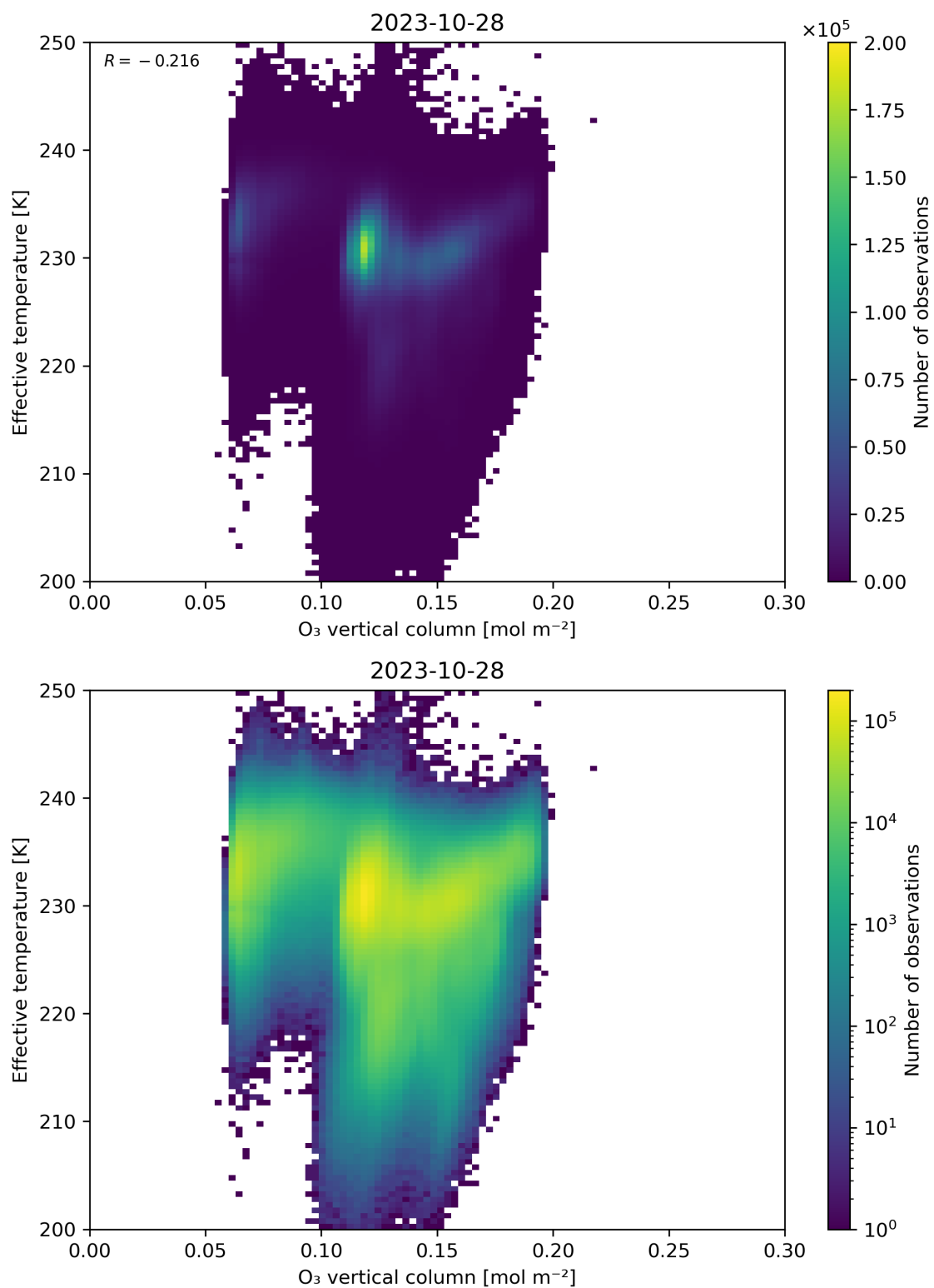
Figure 39: Scatter density plot of “O 3 vertical column” against “Effective temperature” for 2023-10-28 to 2023-10-29.
