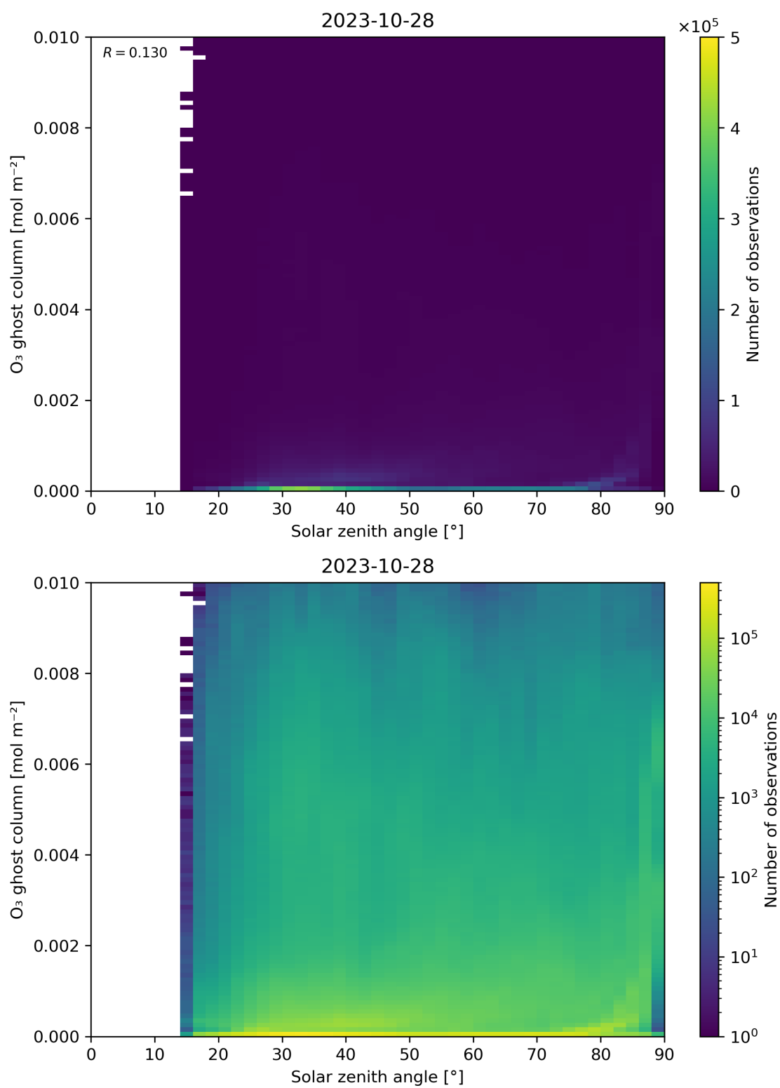
Figure 46: Scatter density plot of “Solar zenith angle” against “O 3 ghost column” for 2023-10-28 to 2023-10-29.
