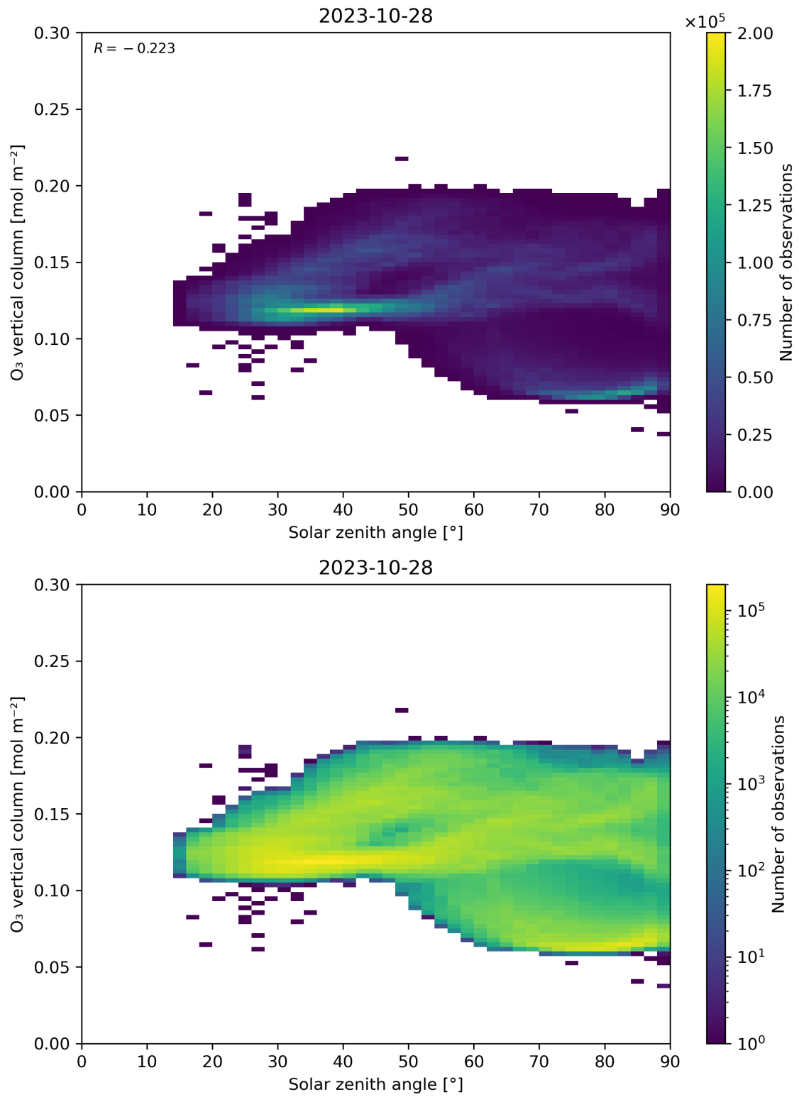
Figure 47: Scatter density plot of “Solar zenith angle” against “O 3 vertical column” for 2023-10-28 to 2023-10-29.
