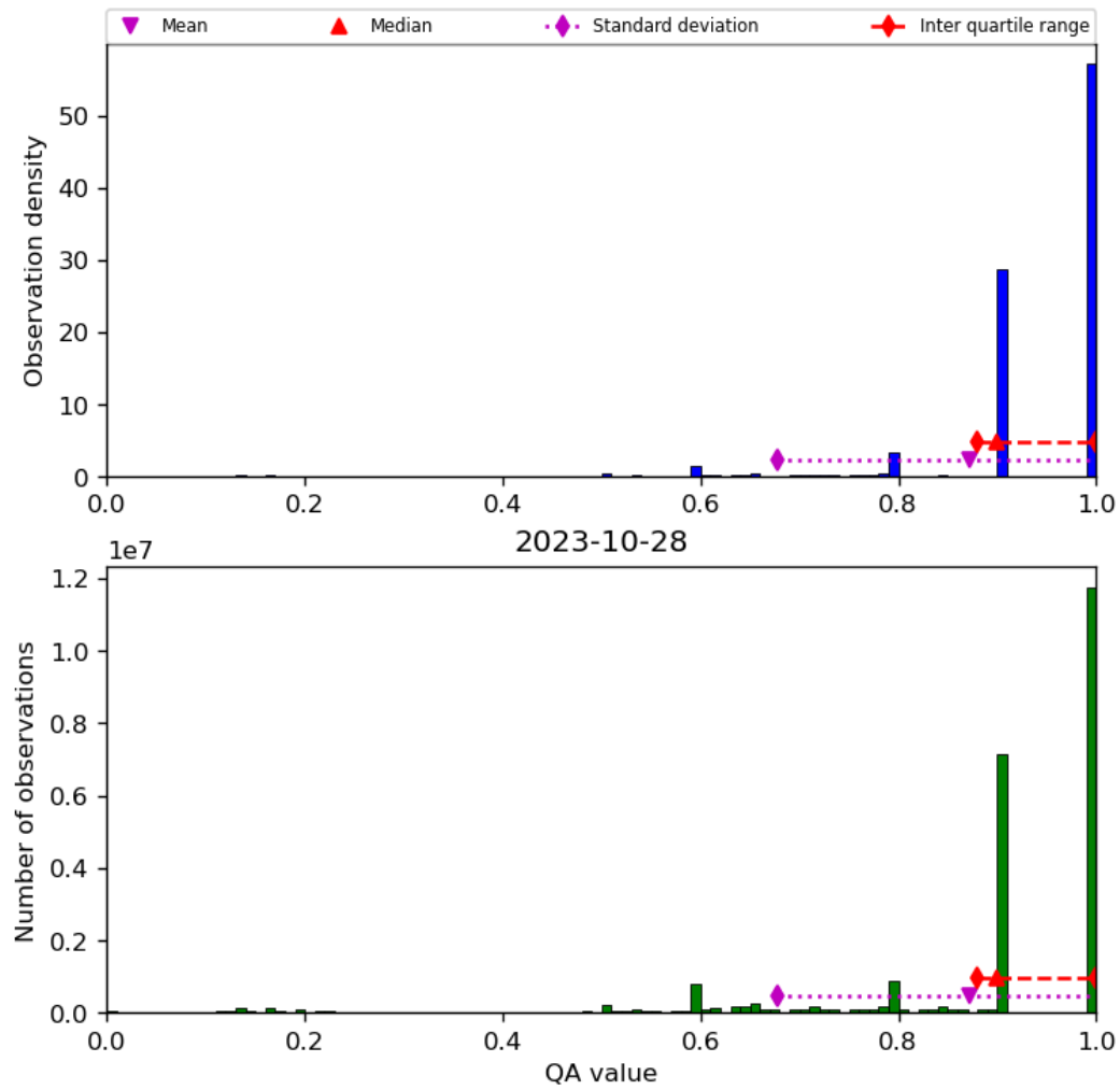
Figure 20: Histogram of “QA value” for 2023-10-28 to 2023-10-29
