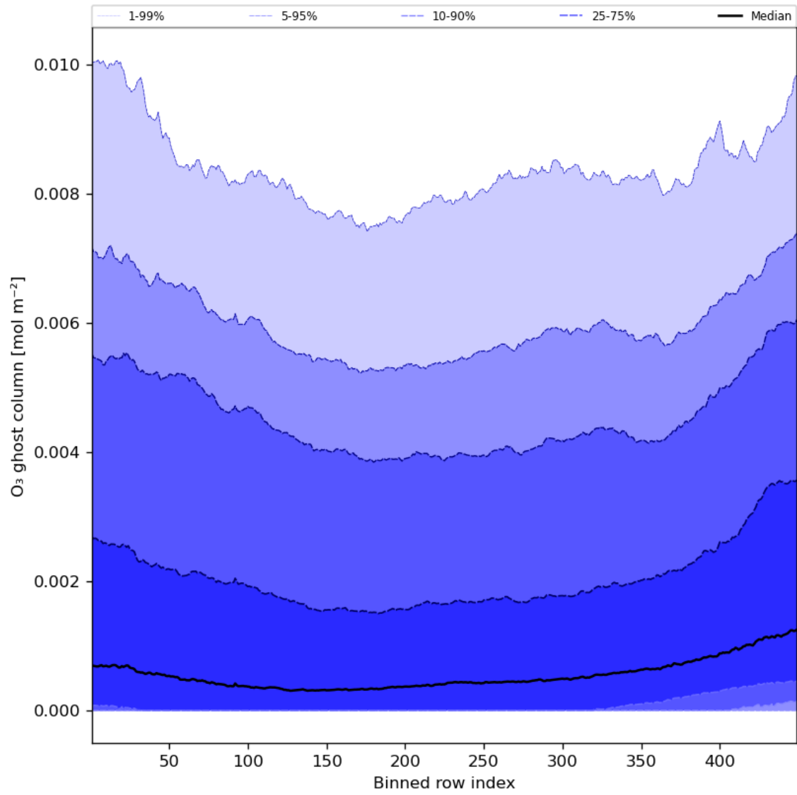
Figure 32: Along track statistics of "O 3 ghost column" for 2023-10-28 to 2023-10-29
