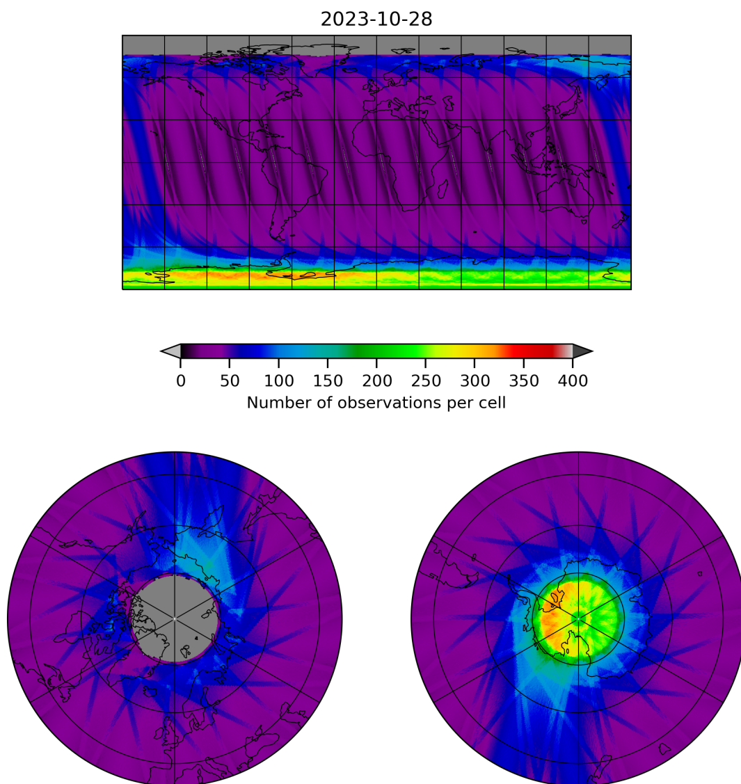
Figure 12: Map of the number of observations for 2023-10-28 to 2023-10-29
