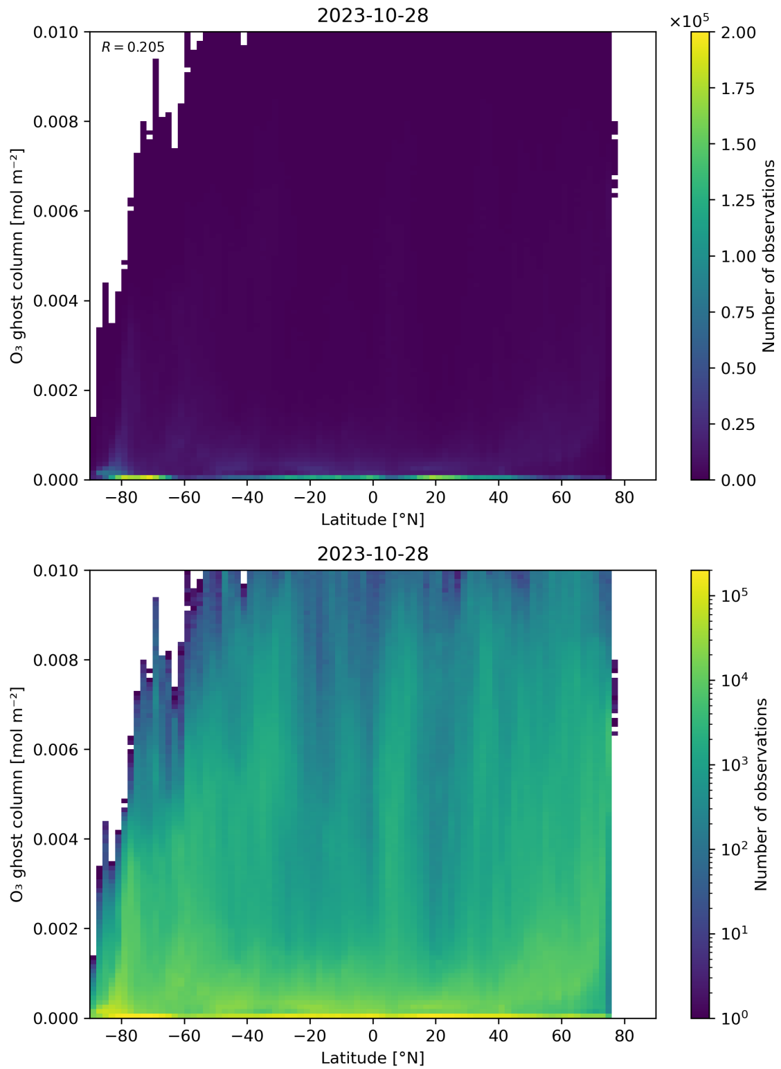
Figure 35: Scatter density plot of “Latitude” against “O 3 ghost column” for 2023-10-28 to 2023-10-29.
