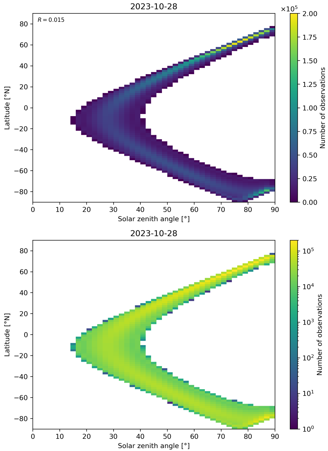
Figure 44: Scatter density plot of “Solar zenith angle” against “Latitude” for 2023-10-28 to 2023-10-29.
