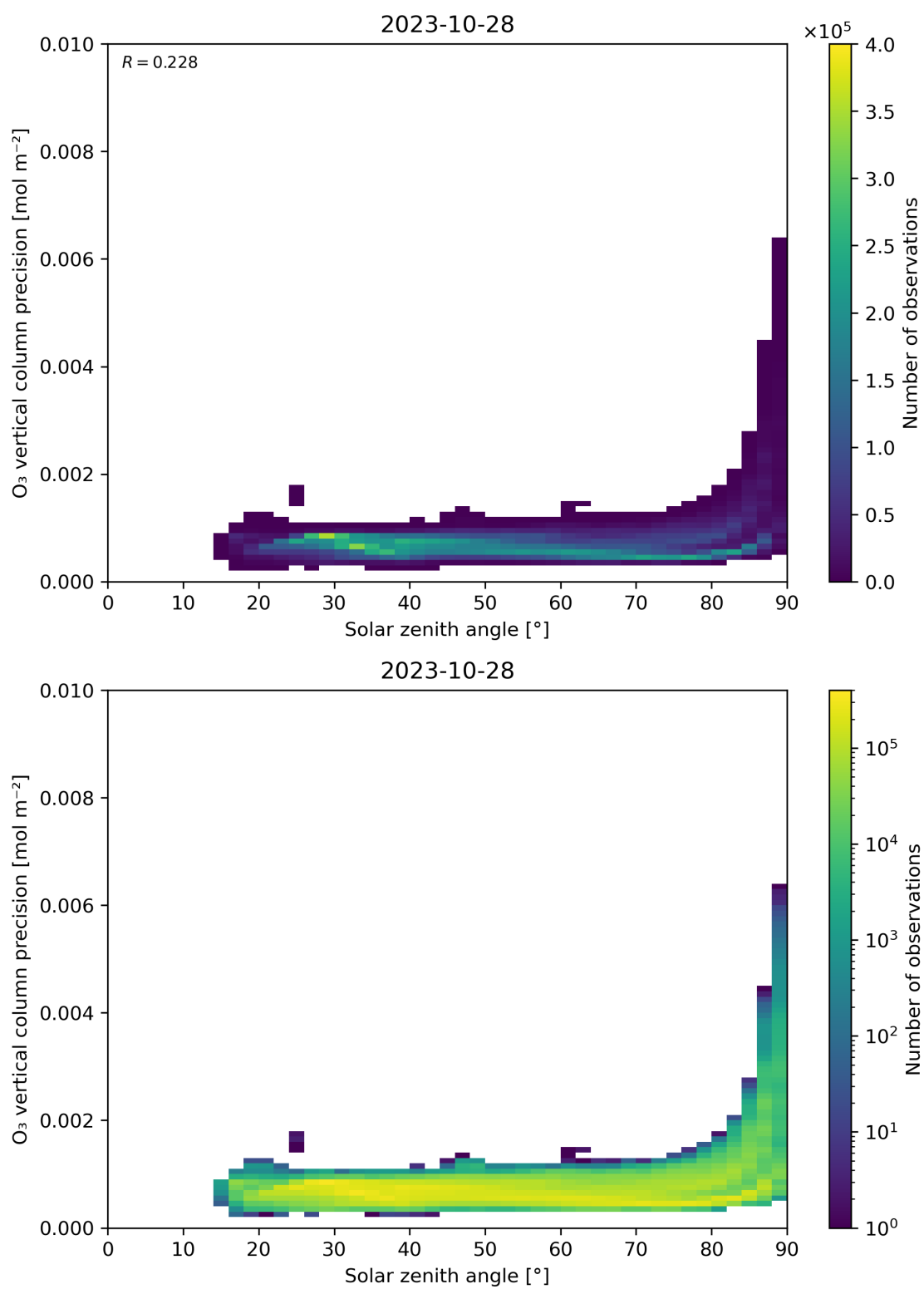
Figure 48: Scatter density plot of “Solar zenith angle” against “O 3 vertical column precision” for 2023-10-28 to 2023-10-29.
