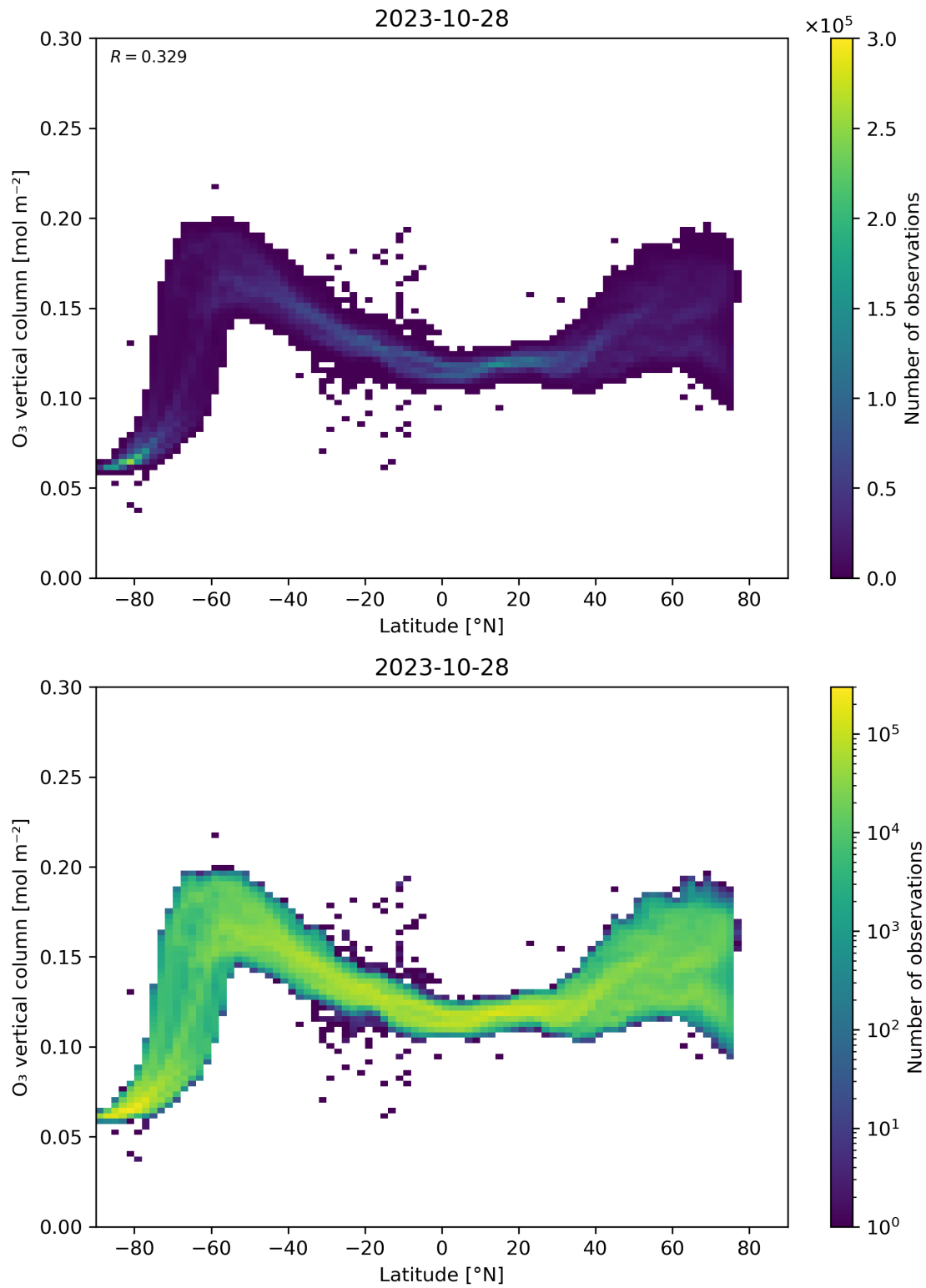
Figure 36: Scatter density plot of “Latitude” against “O 3 vertical column” for 2023-10-28 to 2023-10-29.
