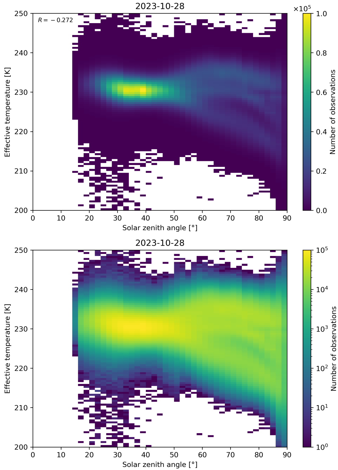
Figure 45: Scatter density plot of “Solar zenith angle” against “Effective temperature” for 2023-10-28 to 2023-10-29.
