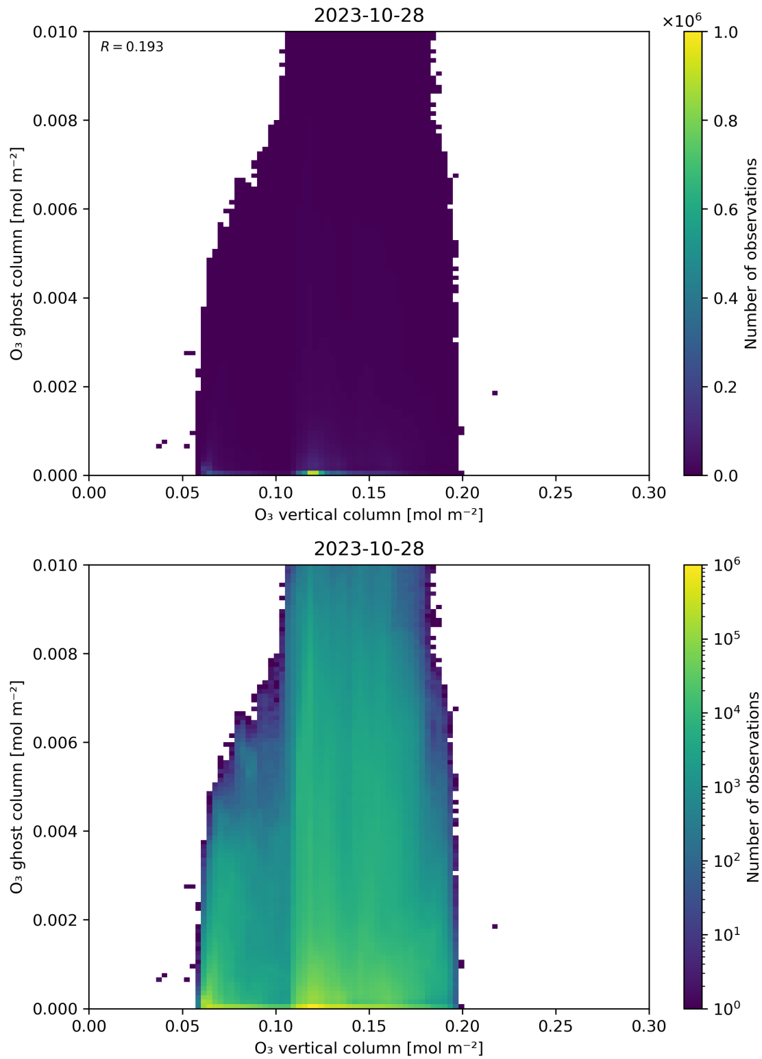
Figure 40: Scatter density plot of “O 3 vertical column” against “O 3 ghost column” for 2023-10-28 to 2023-10-29.
