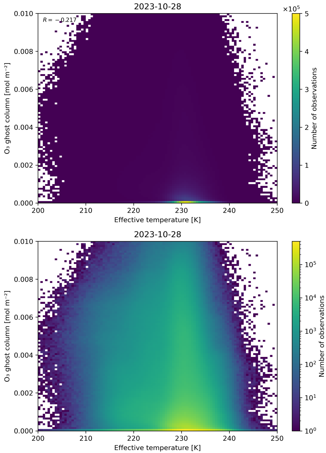
Figure 38: Scatter density plot of “Effective temperature” against “O 3 ghost column” for 2023-10-28 to 2023-10-29.
