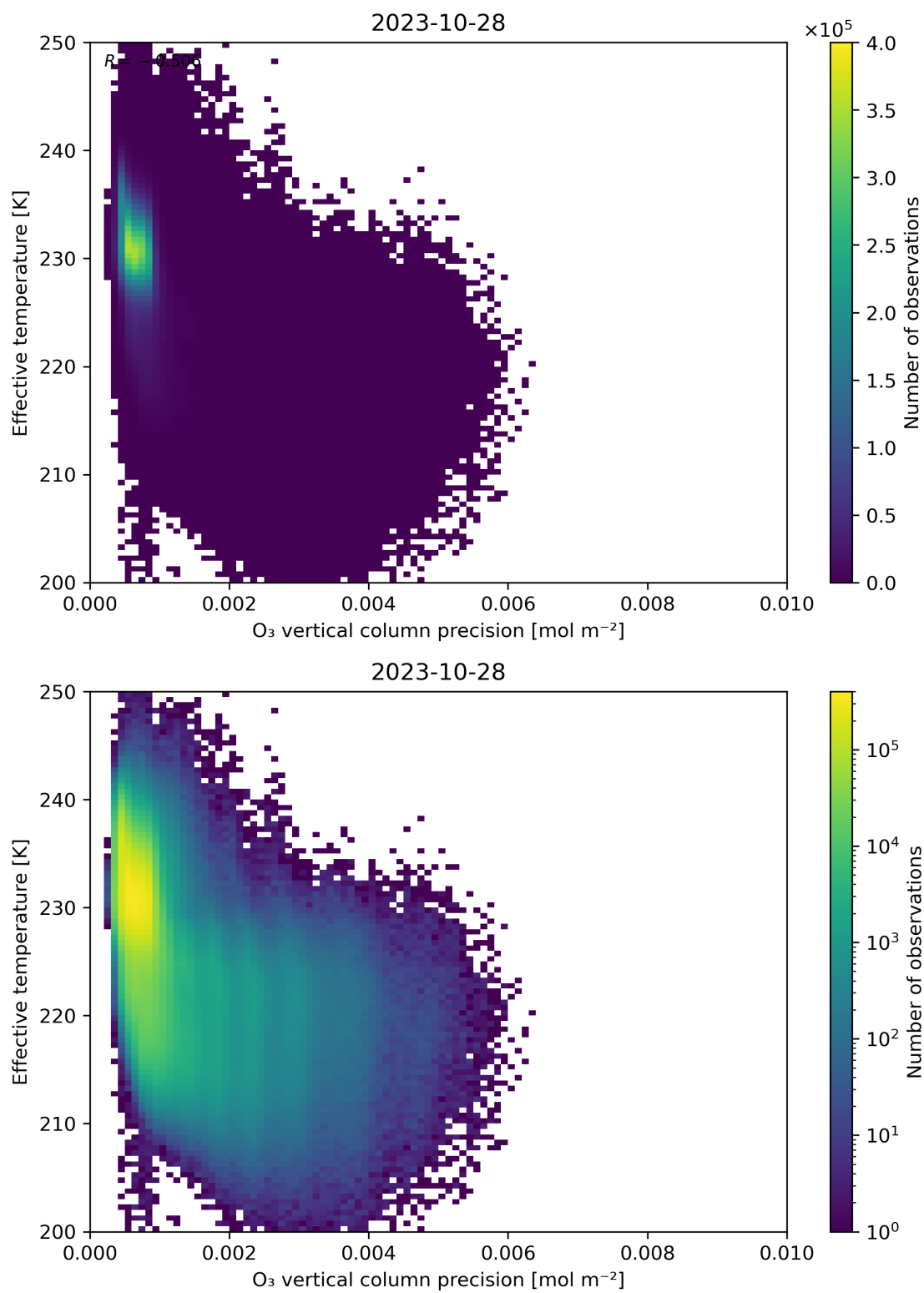
Figure 42: Scatter density plot of “O 3 vertical column precision” against “Effective temperature” for 2023-10-28 to 2023-10-29.
