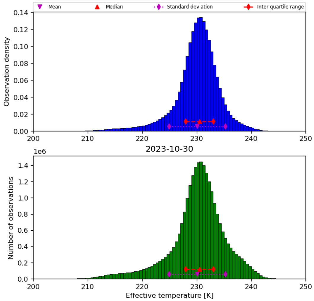
Figure 24: Histogram of “Effective temperature” for 2023-10-29 to 2023-10-31
