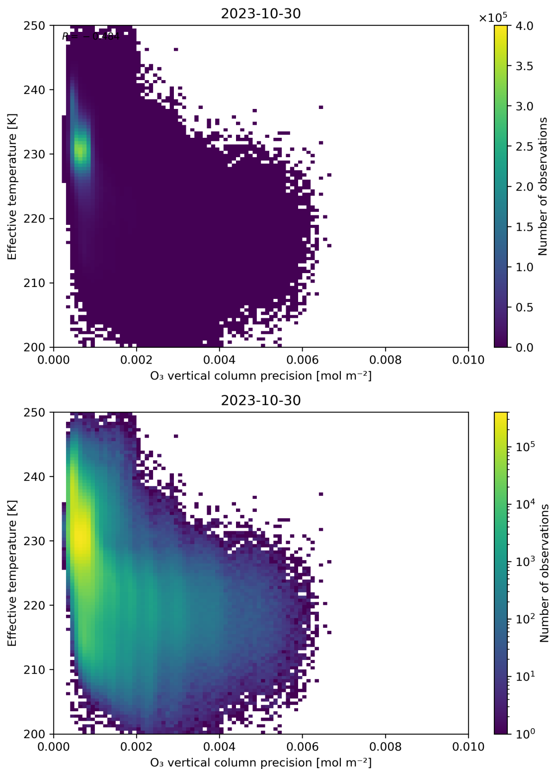
Figure 42: Scatter density plot of “O 3 vertical column precision” against “Effective temperature” for 2023-10-29 to 2023-10-31.
