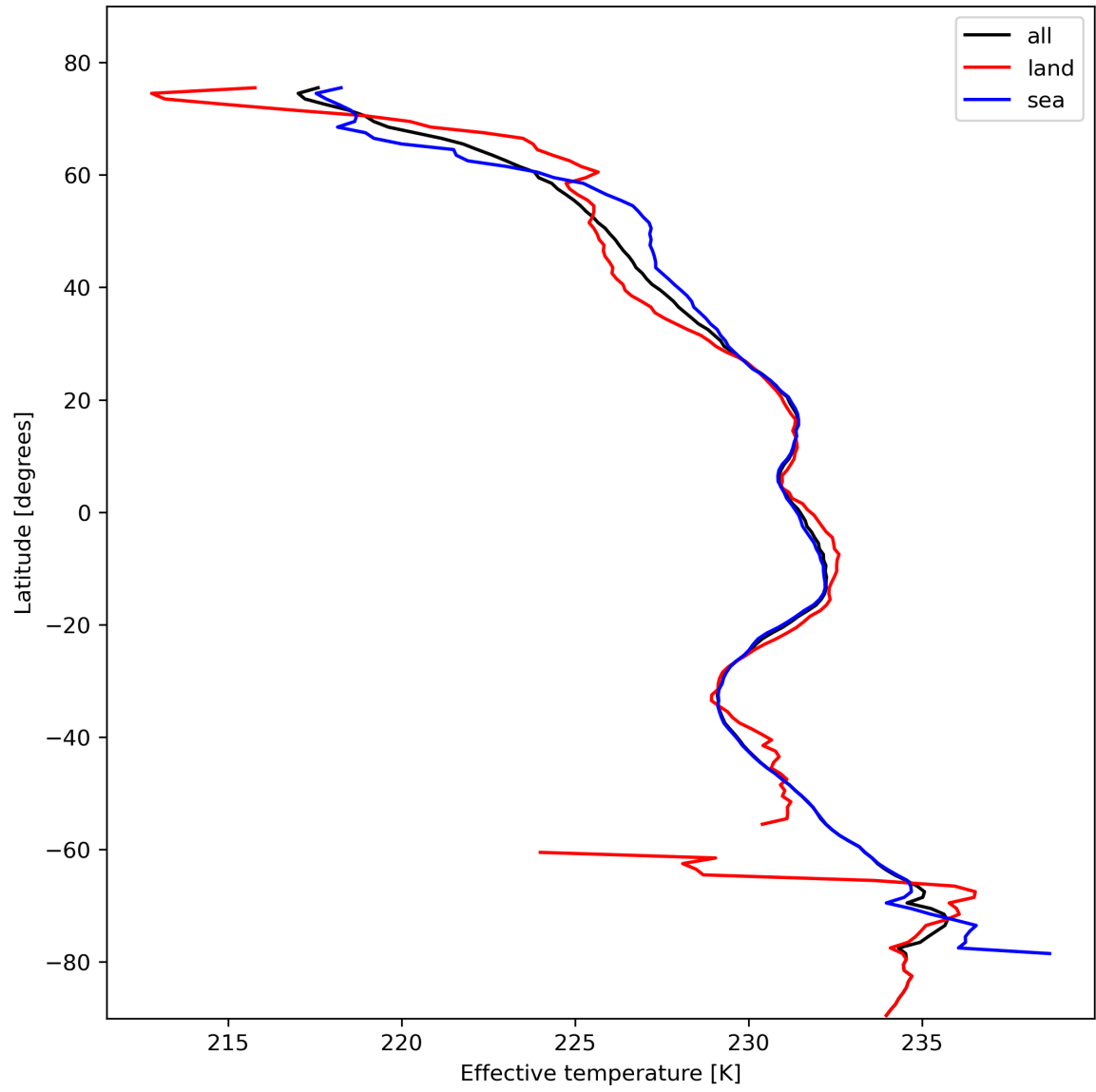
Figure 17: Zonal average of “Effective temperature” for 2023-10-29 to 2023-10-31.
