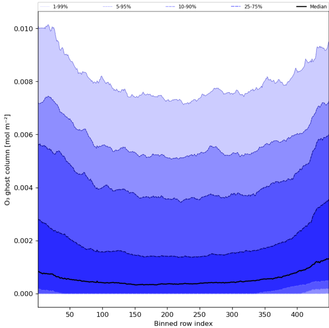
Figure 32: Along track statistics of “O 3 ghost column” for 2023-10-29 to 2023-10-31
