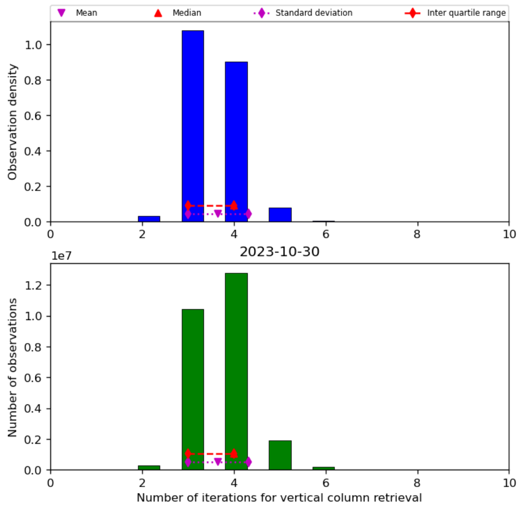
Figure 26: Histogram of “Number of iterations for vertical column retrieval” for 2023-10-29 to 2023-10-31
