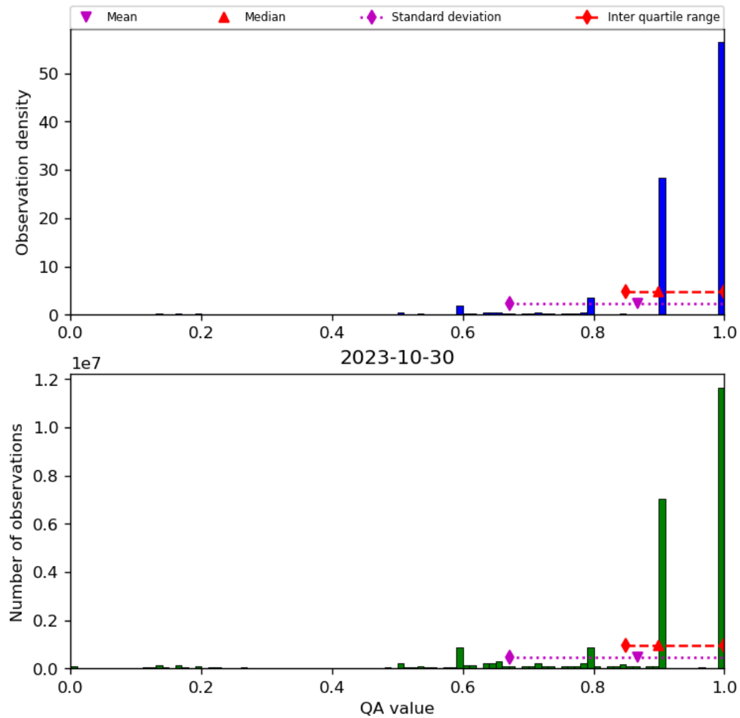
Figure 20: Histogram of “QA value” for 2023-10-29 to 2023-10-31
