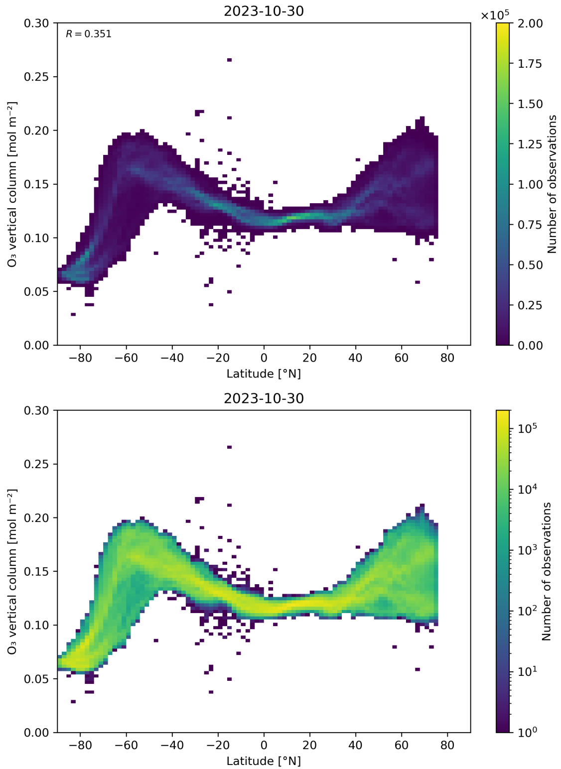
Figure 36: Scatter density plot of “Latitude” against “O 3 vertical column” for 2023-10-29 to 2023-10-31.
