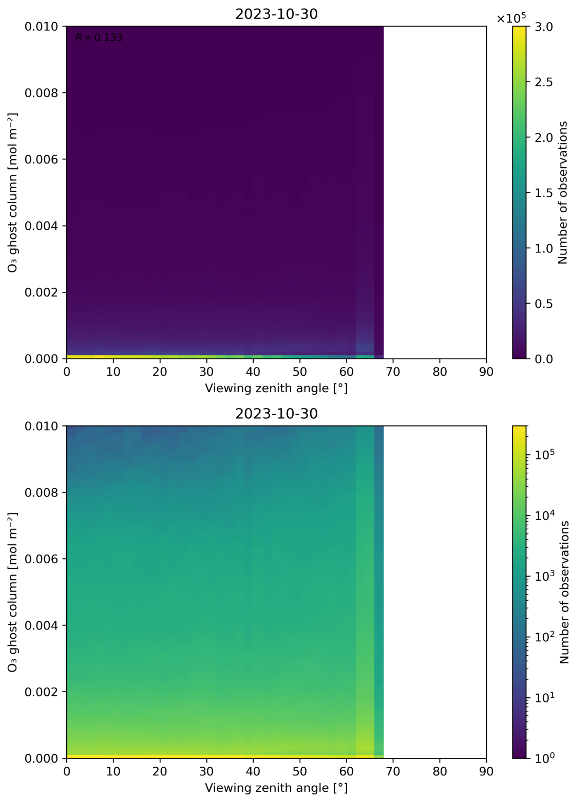
Figure 51: Scatter density plot of “Viewing zenith angle” against “O 3 ghost column” for 2023-10-29 to 2023-10-31.
