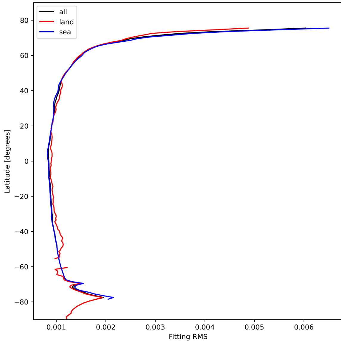
Figure 16: Zonal average of “Fitting RMS” for 2023-10-29 to 2023-10-31.
