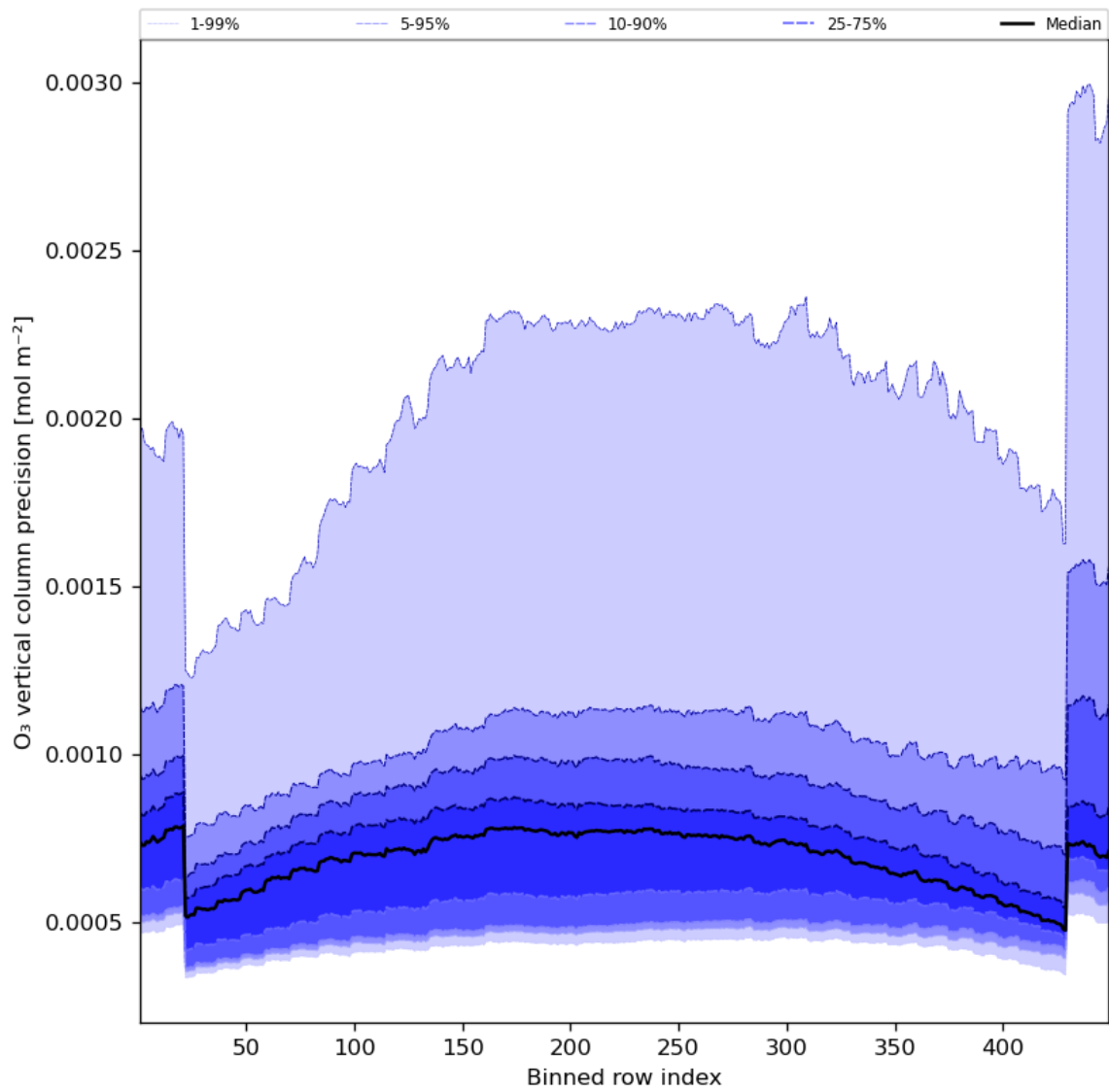
Figure 29: Along track statistics of “O 3 vertical column precision” for 2023-10-29 to 2023-10-31
