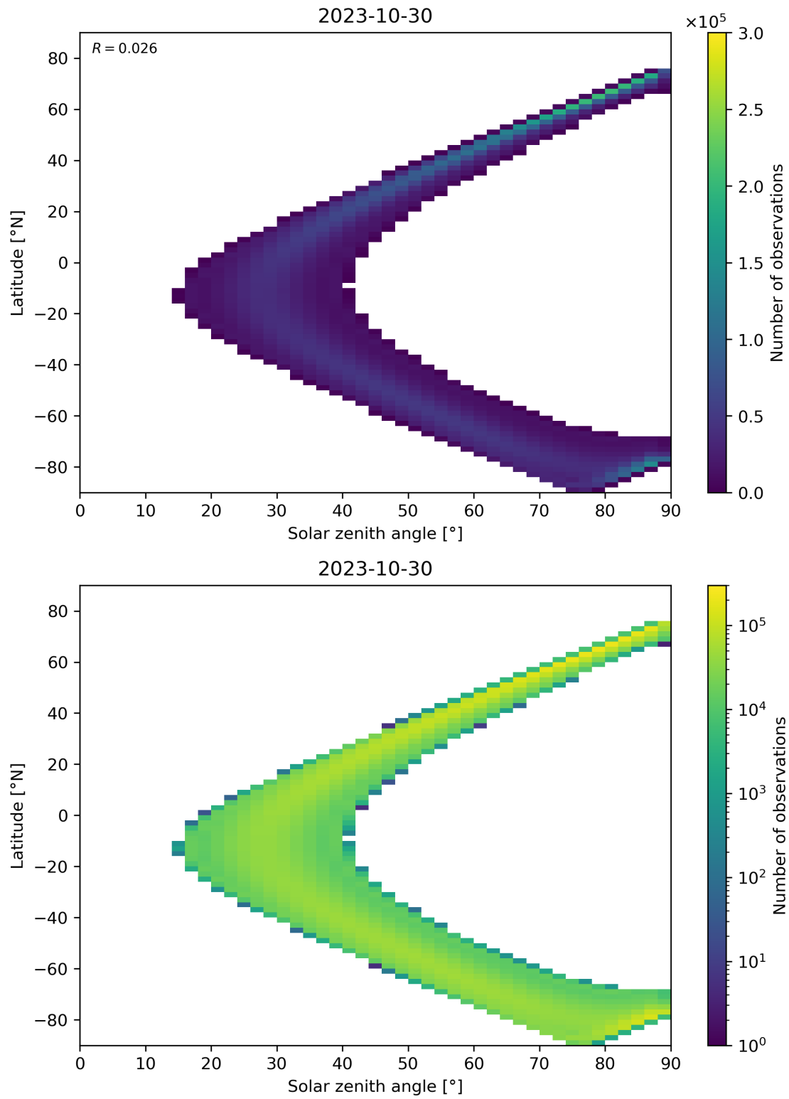
Figure 44: Scatter density plot of “Solar zenith angle” against “Latitude” for 2023-10-29 to 2023-10-31.
