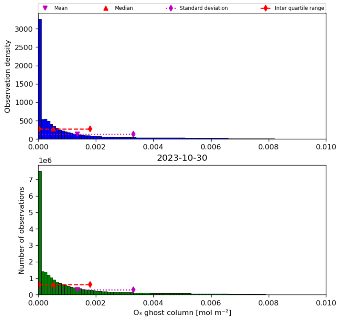
Figure 25: Histogram of “O 3 ghost column” for 2023-10-29 to 2023-10-31
