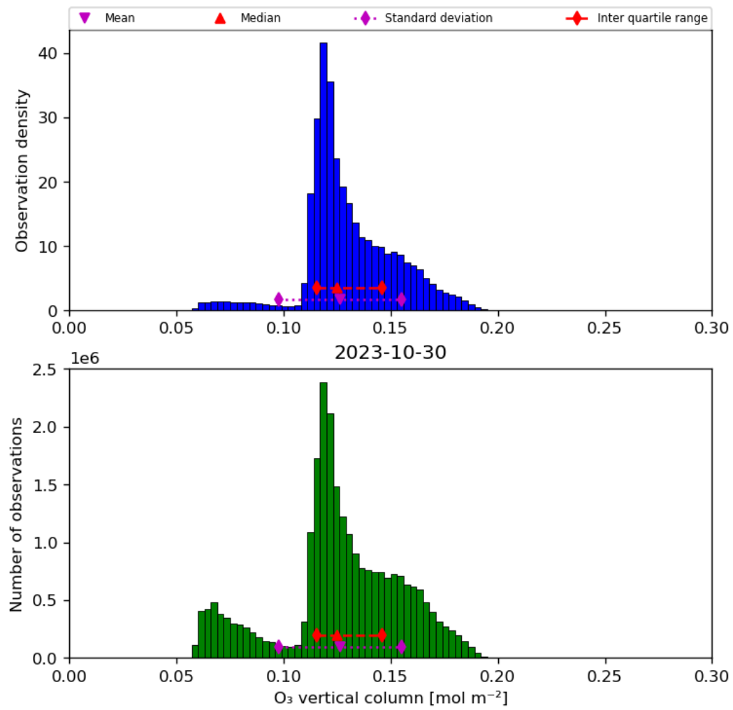
Figure 21: Histogram of “O 3 vertical column” for 2023-10-29 to 2023-10-31
