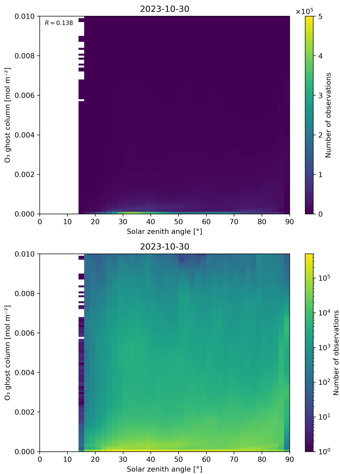
Figure 46: Scatter density plot of “Solar zenith angle” against “O 3 ghost column” for 2023-10-29 to 2023-10-31.
