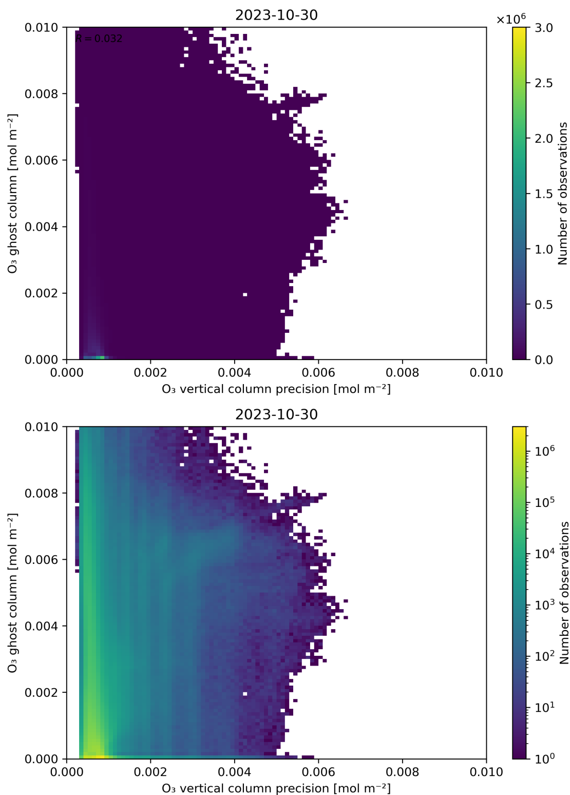
Figure 43: Scatter density plot of “O 3 vertical column precision” against “O 3 ghost column” for 2023-10-29 to 2023-10-31.
