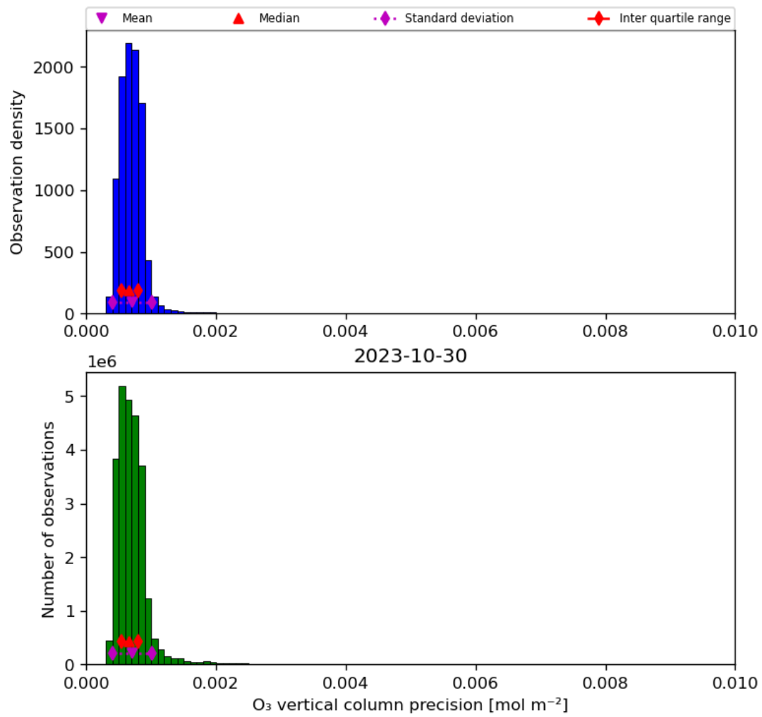
Figure 22: Histogram of “O 3 vertical column precision” for 2023-10-29 to 2023-10-31
