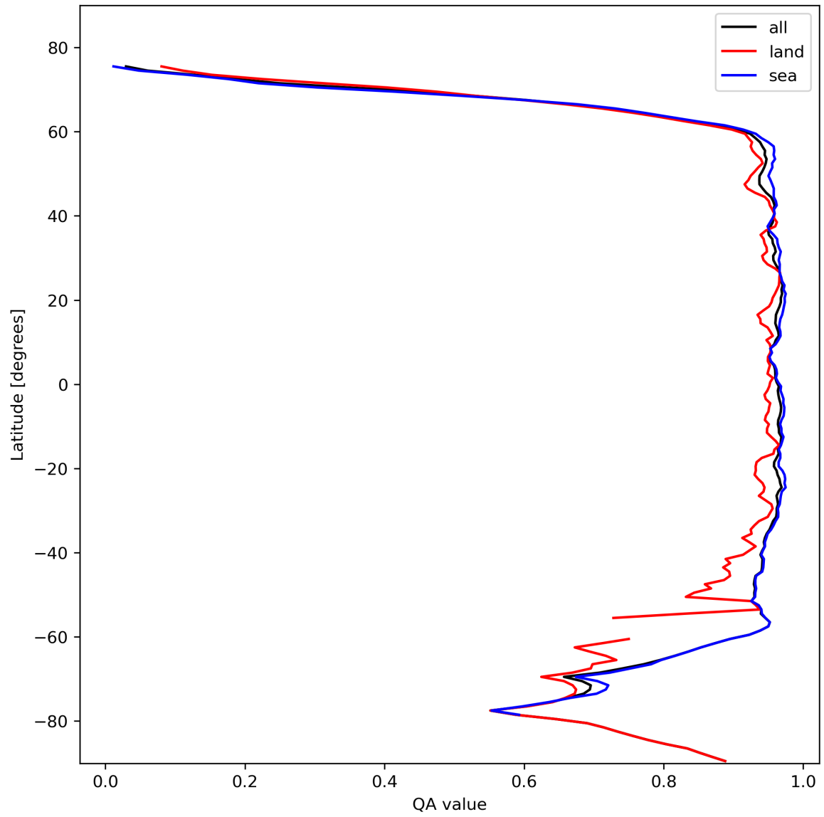
Figure 13: Zonal average of “QA value” for 2023-10-29 to 2023-10-31.
