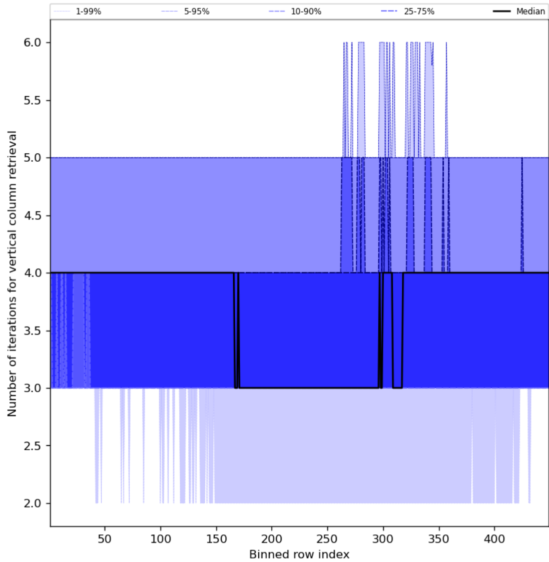
Figure 33: Along track statistics of “Number of iterations for vertical column retrieval” for 2023-10-29 to 2023-10-31
