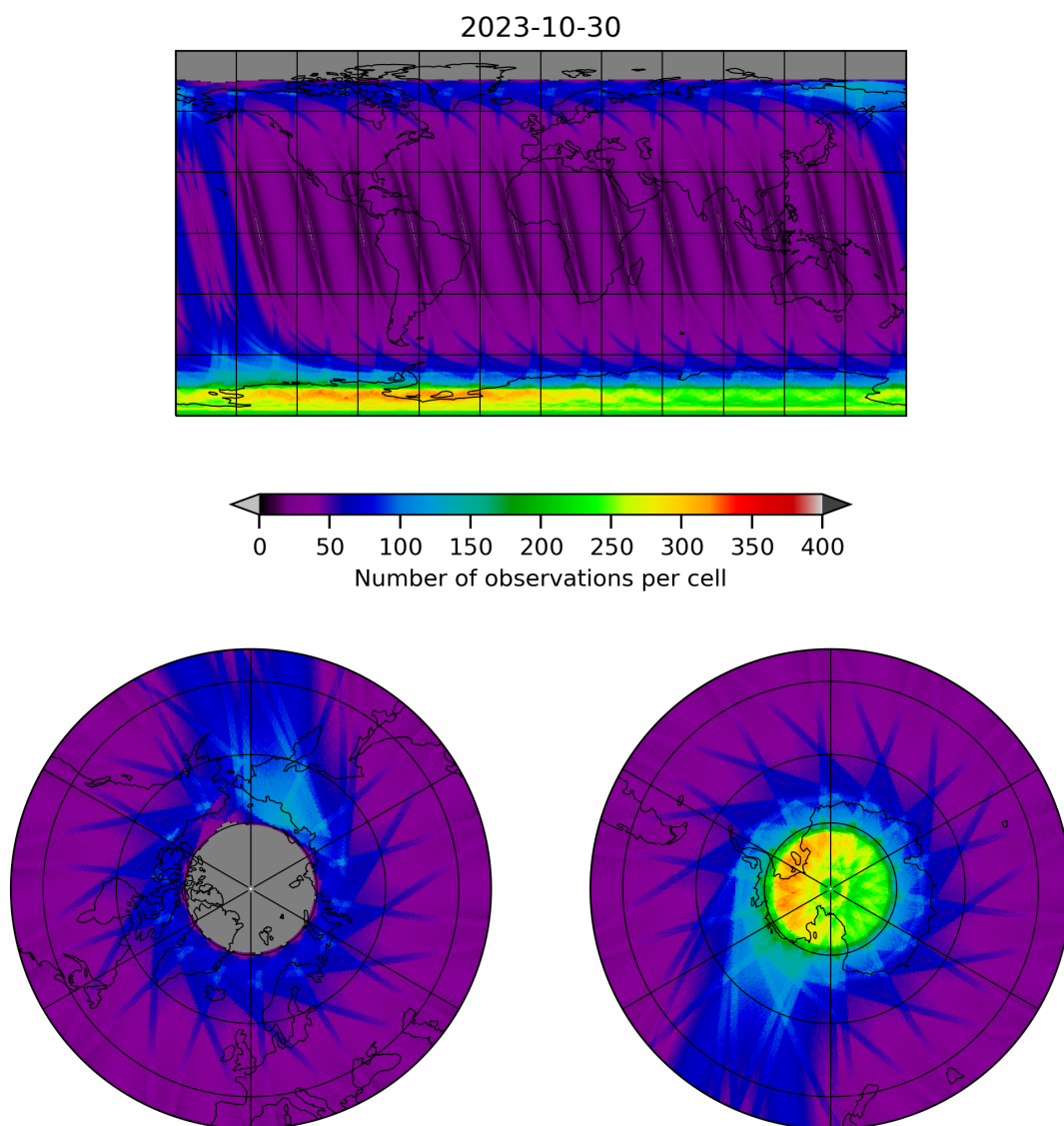
Figure 12: Map of the number of observations for 2023-10-29 to 2023-10-31
