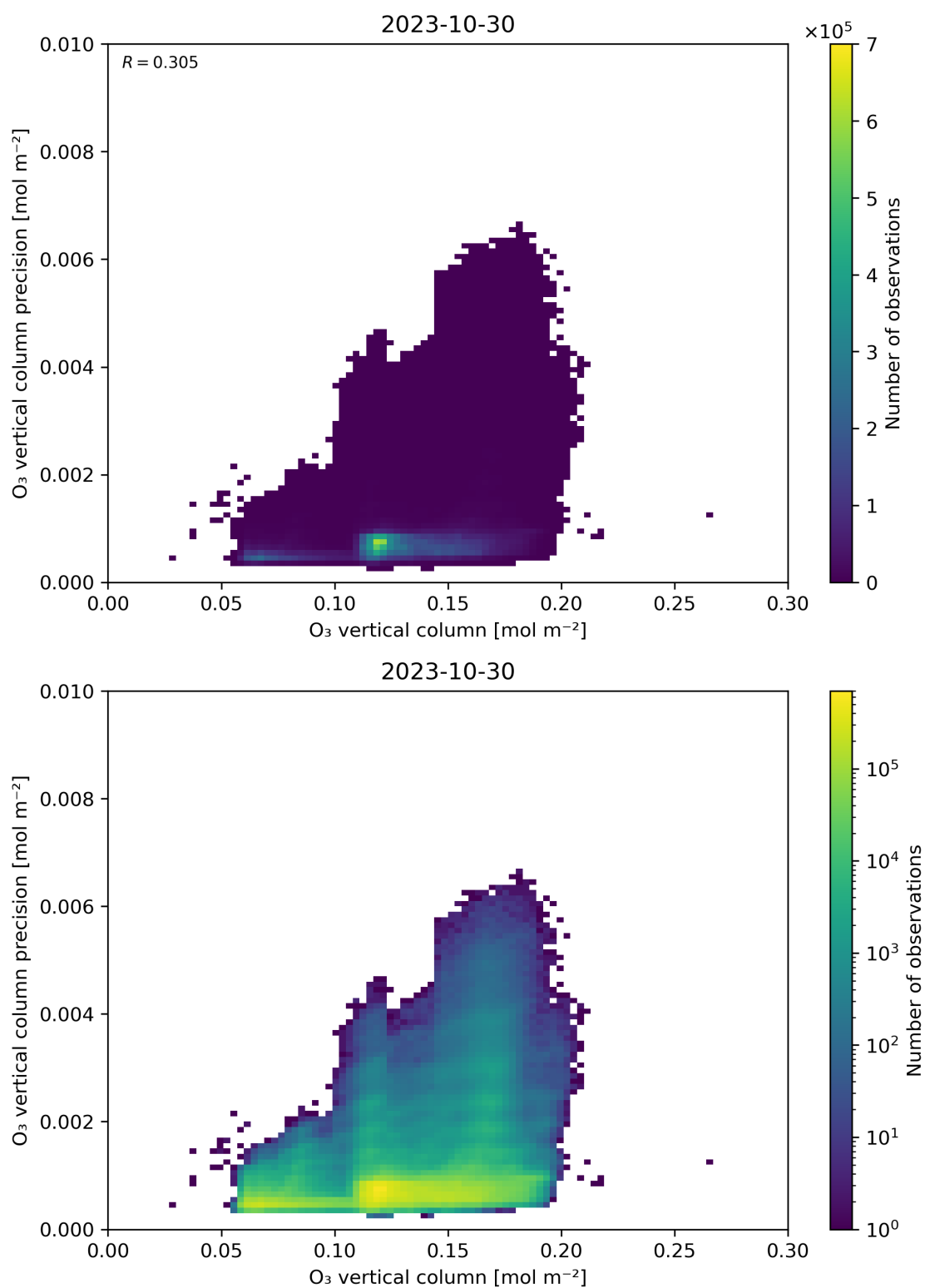
Figure 41: Scatter density plot of “O 3 vertical column” against “O 3 vertical column precision” for 2023-10-29 to 2023-10-31.
