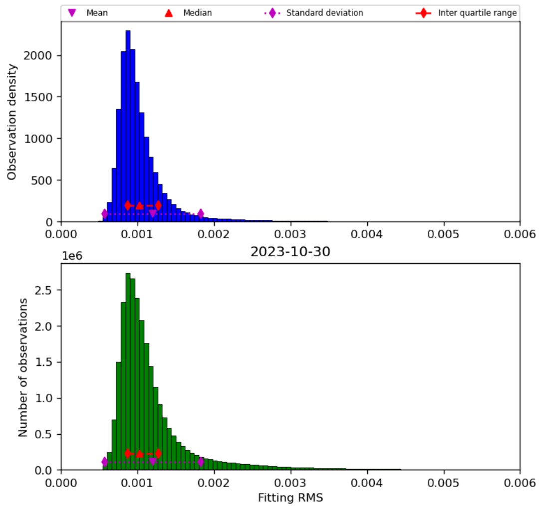
Figure 23: Histogram of “Fitting RMS” for 2023-10-29 to 2023-10-31
