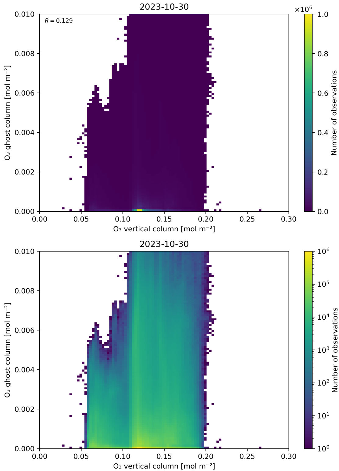
Figure 40: Scatter density plot of “O 3 vertical column” against “O 3 ghost column” for 2023-10-29 to 2023-10-31.
