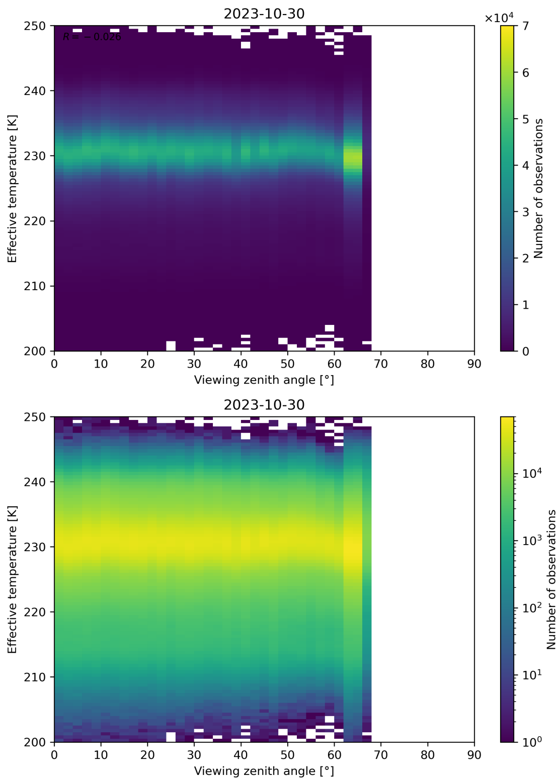
Figure 50: Scatter density plot of “Viewing zenith angle” against “Effective temperature” for 2023-10-29 to 2023-10-31.
