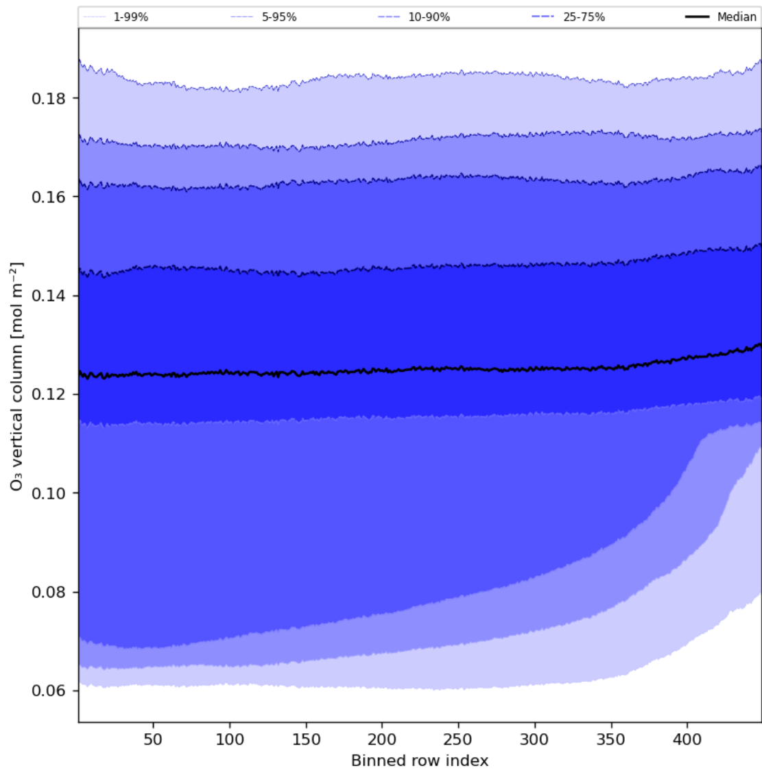
Figure 28: Along track statistics of “O 3 vertical column” for 2023-10-29 to 2023-10-31
