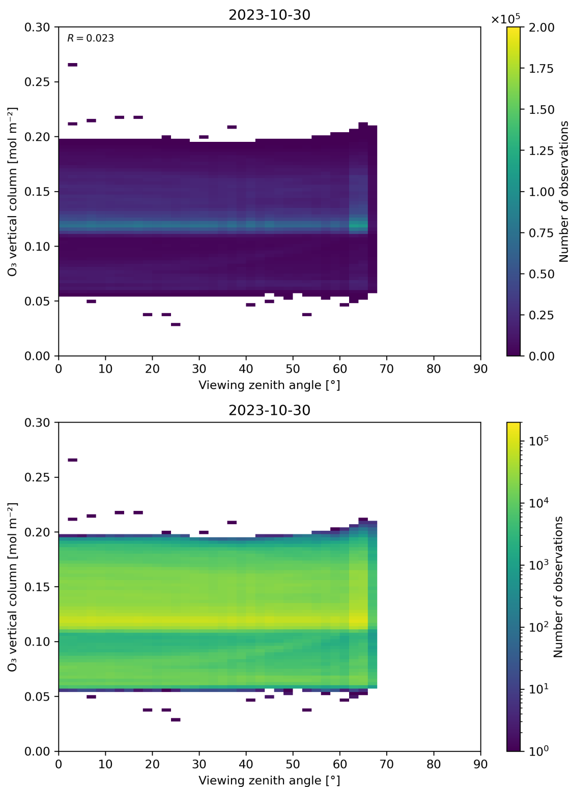
Figure 52: Scatter density plot of “Viewing zenith angle” against “O 3 vertical column” for 2023-10-29 to 2023-10-31.
