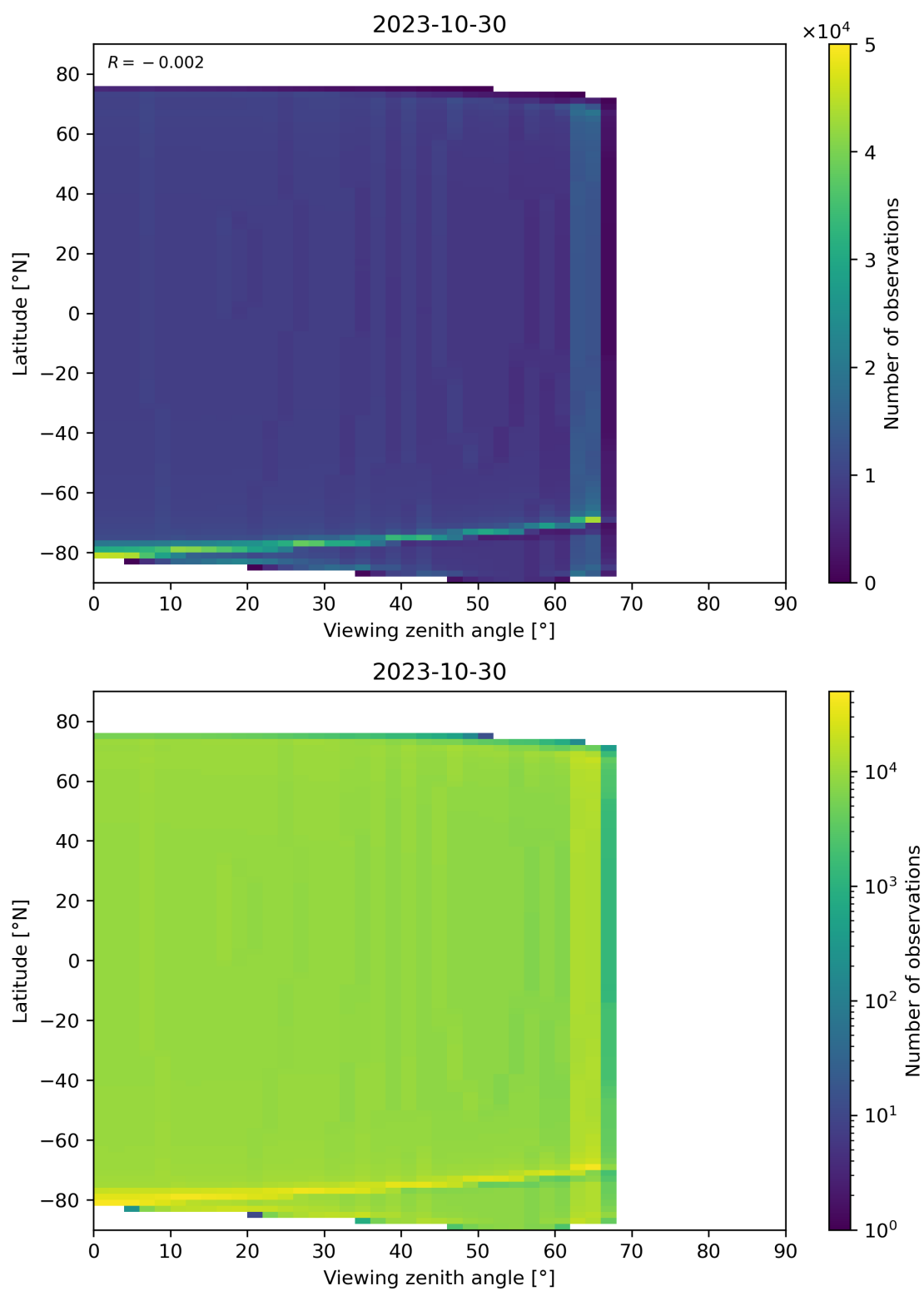
Figure 49: Scatter density plot of “Viewing zenith angle” against “Latitude” for 2023-10-29 to 2023-10-31.
