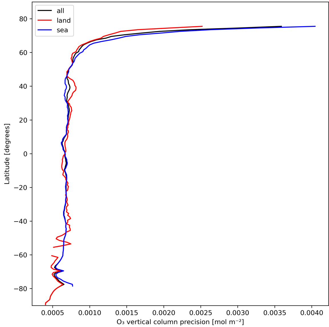
Figure 15: Zonal average of “O 3 vertical column precision” for 2023-10-29 to 2023-10-31.
