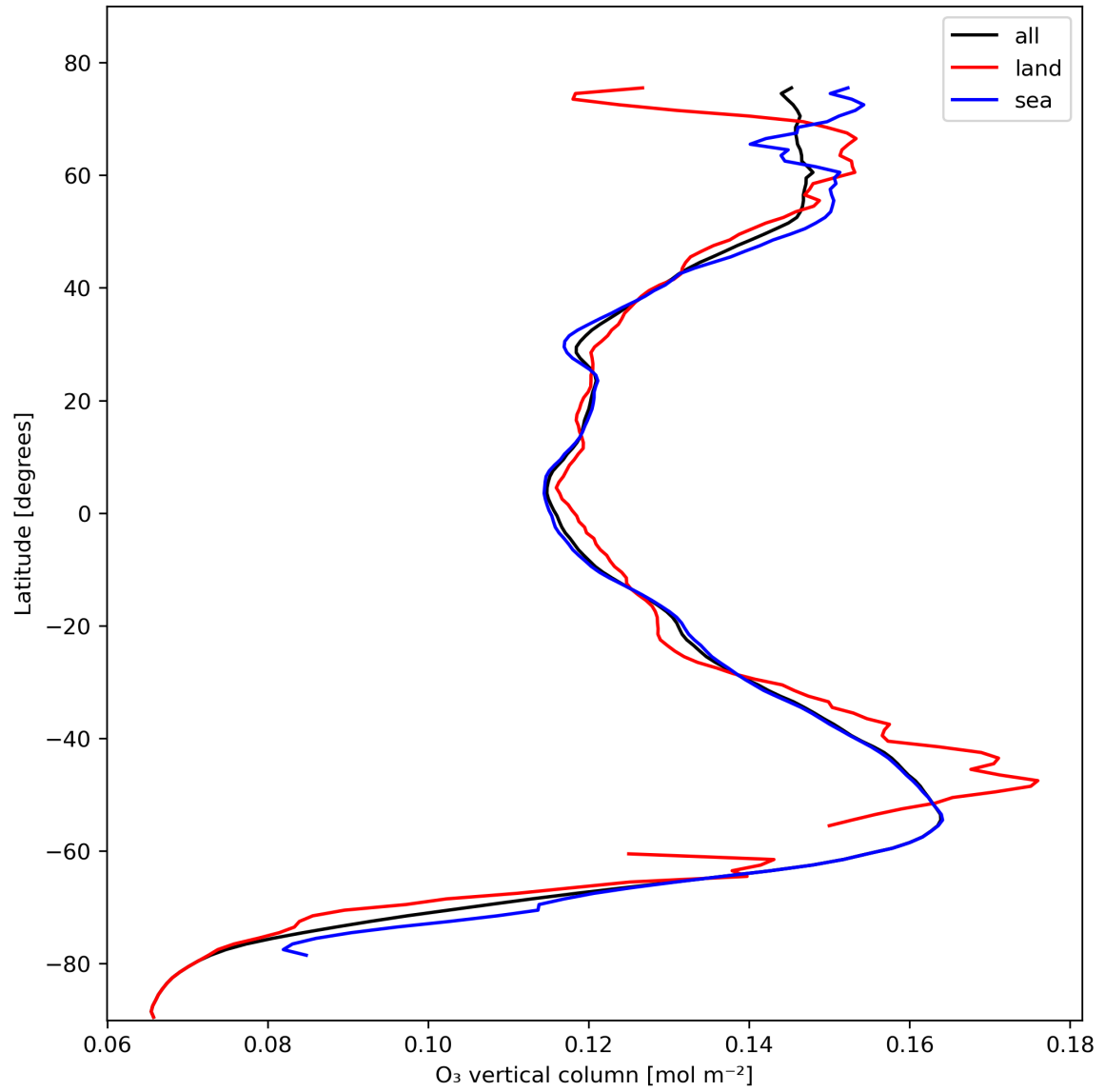
Figure 14: Zonal average of “O 3 vertical column” for 2023-10-29 to 2023-10-31.
