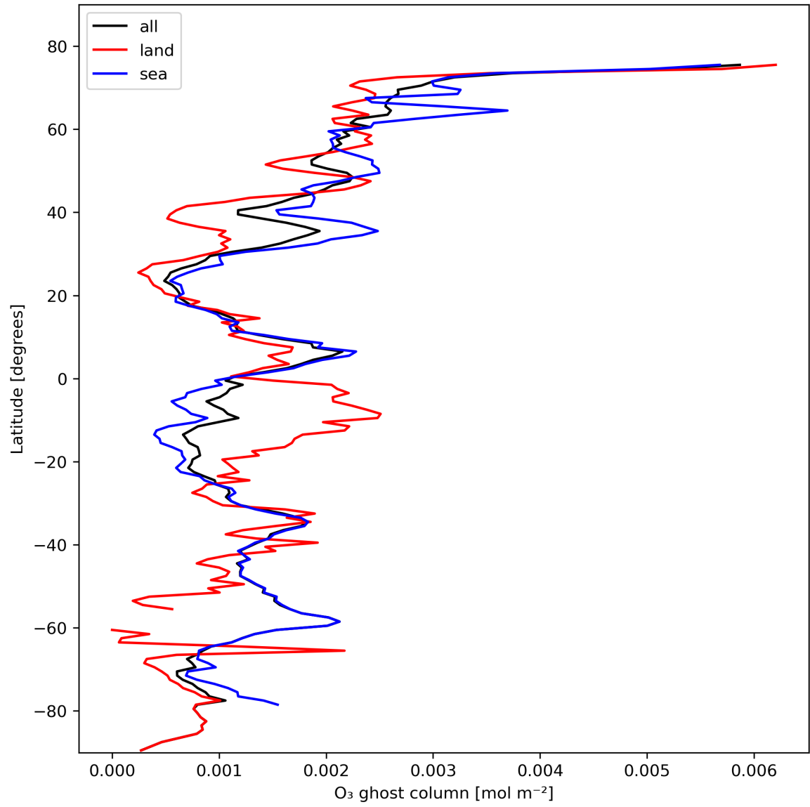
Figure 18: Zonal average of “O 3 ghost column” for 2023-10-29 to 2023-10-31.
