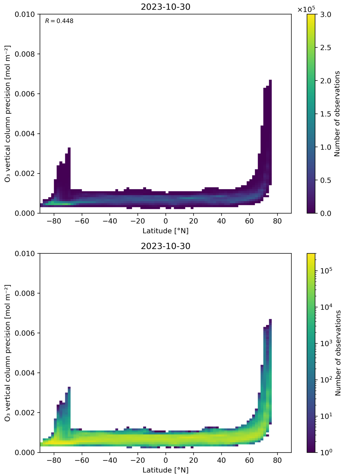
Figure 37: Scatter density plot of “Latitude” against “O 3 vertical column precision” for 2023-10-29 to 2023-10-31.
