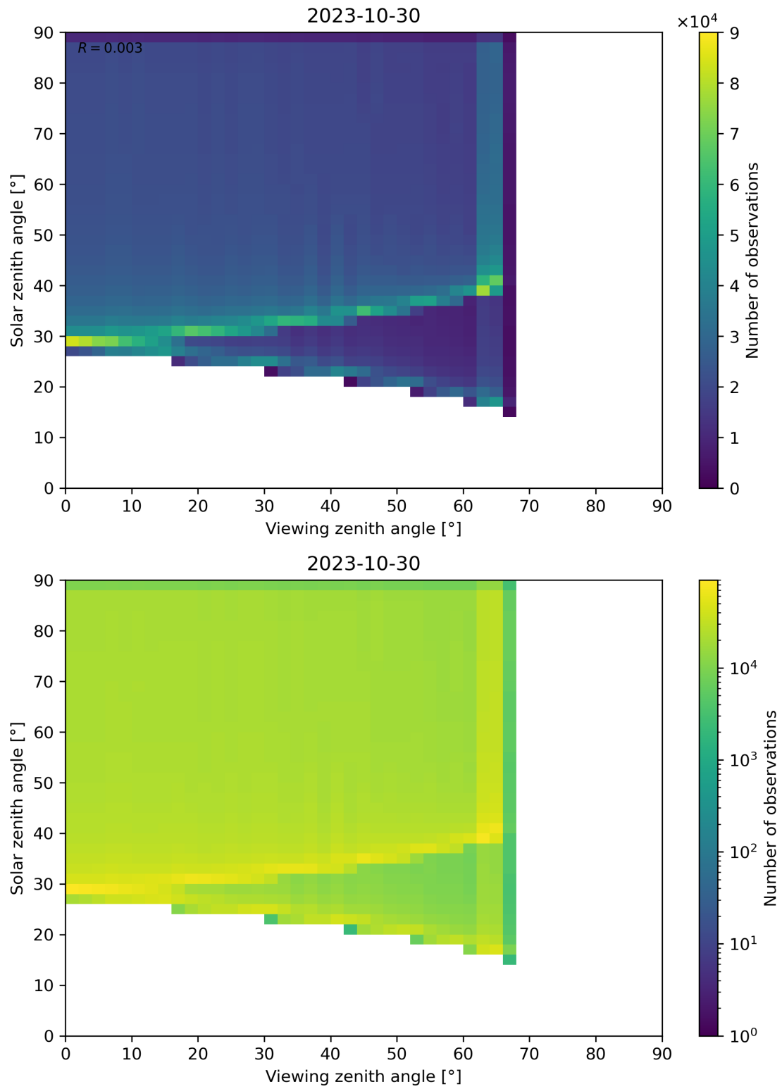
Figure 54: Scatter density plot of “Viewing zenith angle” against “Solar zenith angle” for 2023-10-29 to 2023-10-31.
