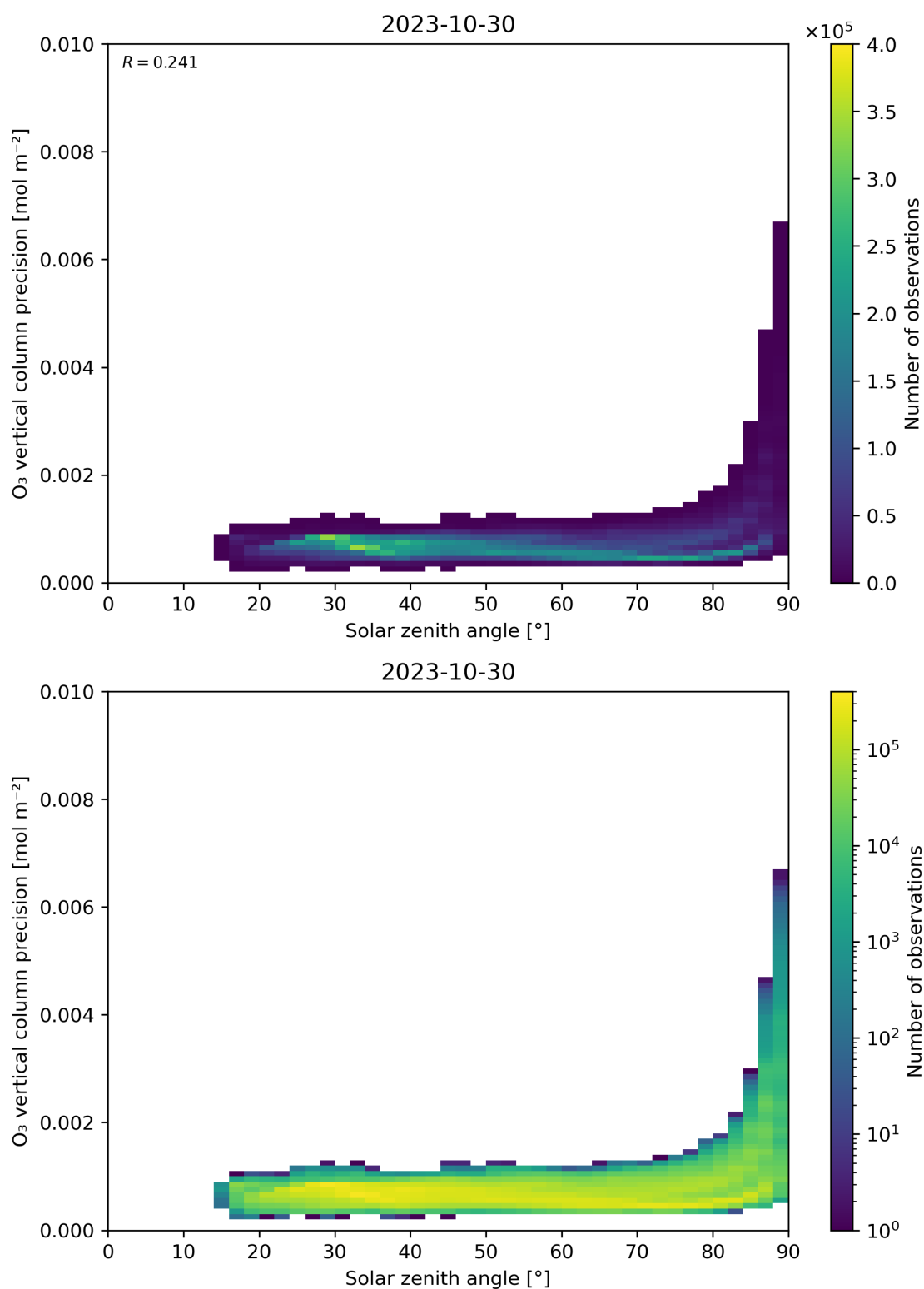
Figure 48: Scatter density plot of “Solar zenith angle” against “O 3 vertical column precision” for 2023-10-29 to 2023-10-31.
