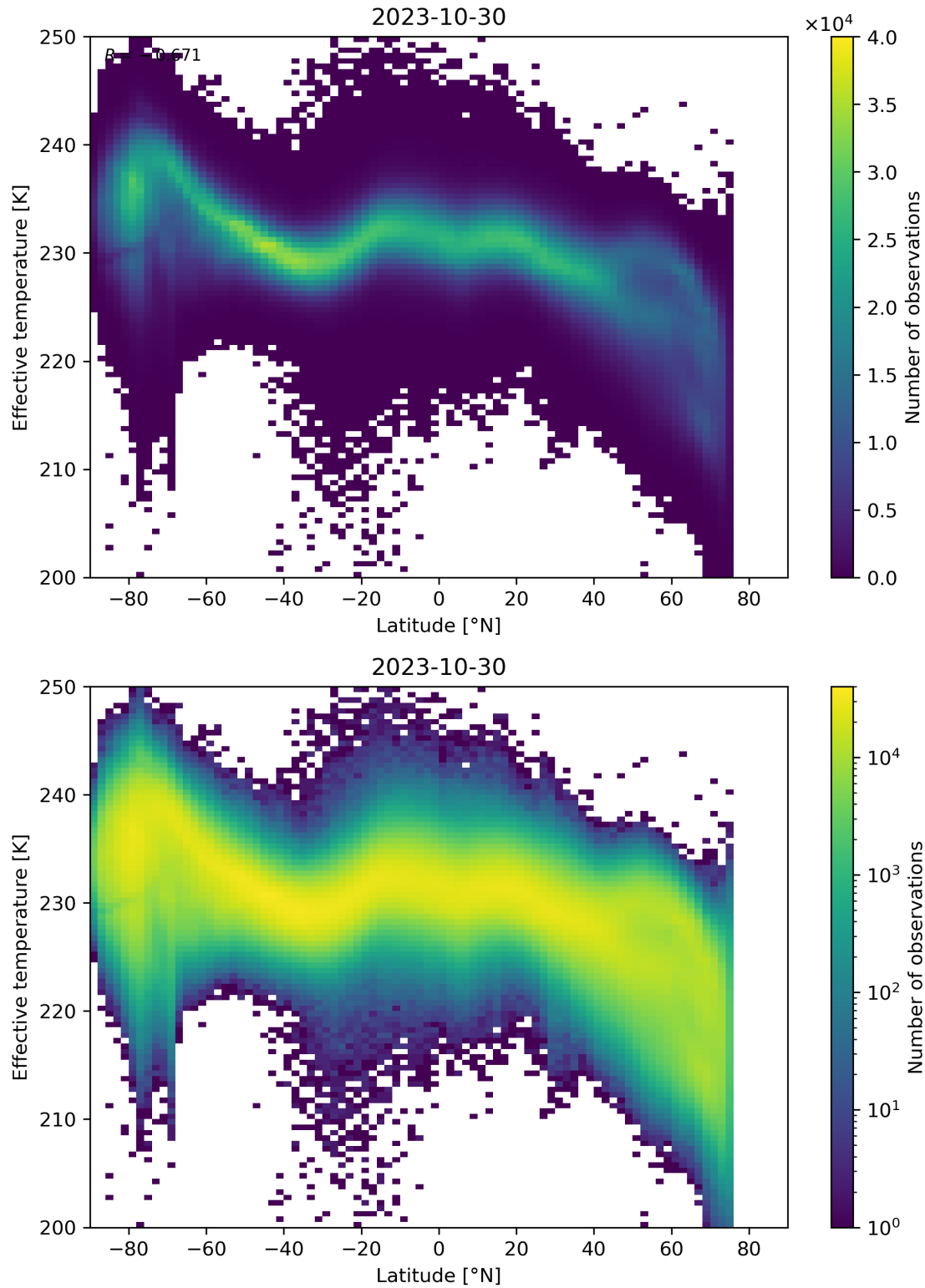
Figure 34: Scatter density plot of “Latitude” against “Effective temperature” for 2023-10-29 to 2023-10-31.
