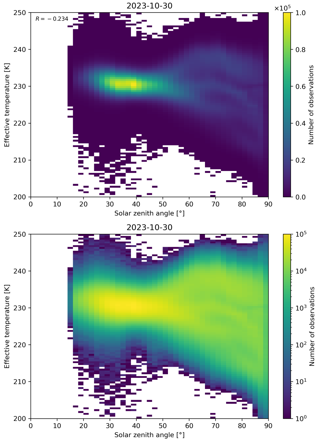
Figure 45: Scatter density plot of “Solar zenith angle” against “Effective temperature” for 2023-10-29 to 2023-10-31.
