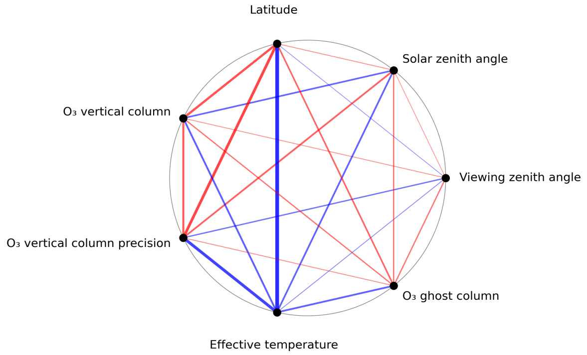
Figure 1: Map of correlation graph for 2023-10-29 to 2023-10-31.
