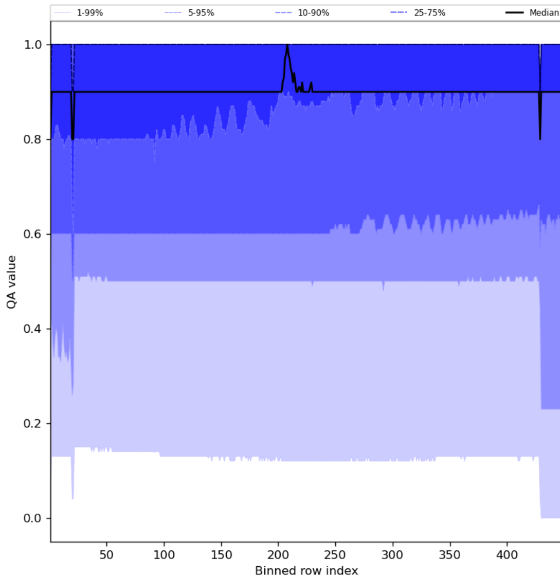
Figure 27: Along track statistics of “QA value” for 2023-10-29 to 2023-10-31
