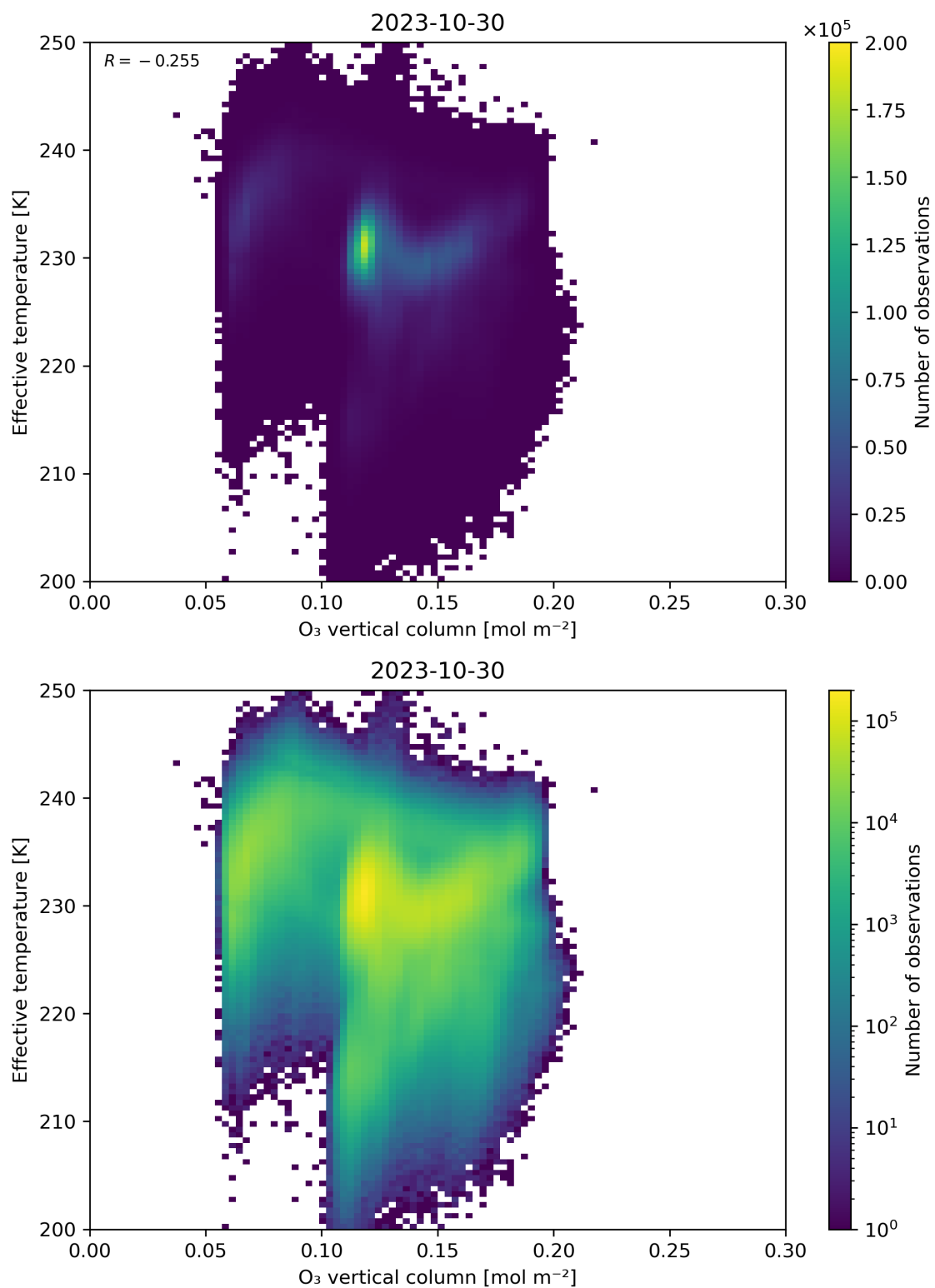
Figure 39: Scatter density plot of “O 3 vertical column” against “Effective temperature” for 2023-10-29 to 2023-10-31.
