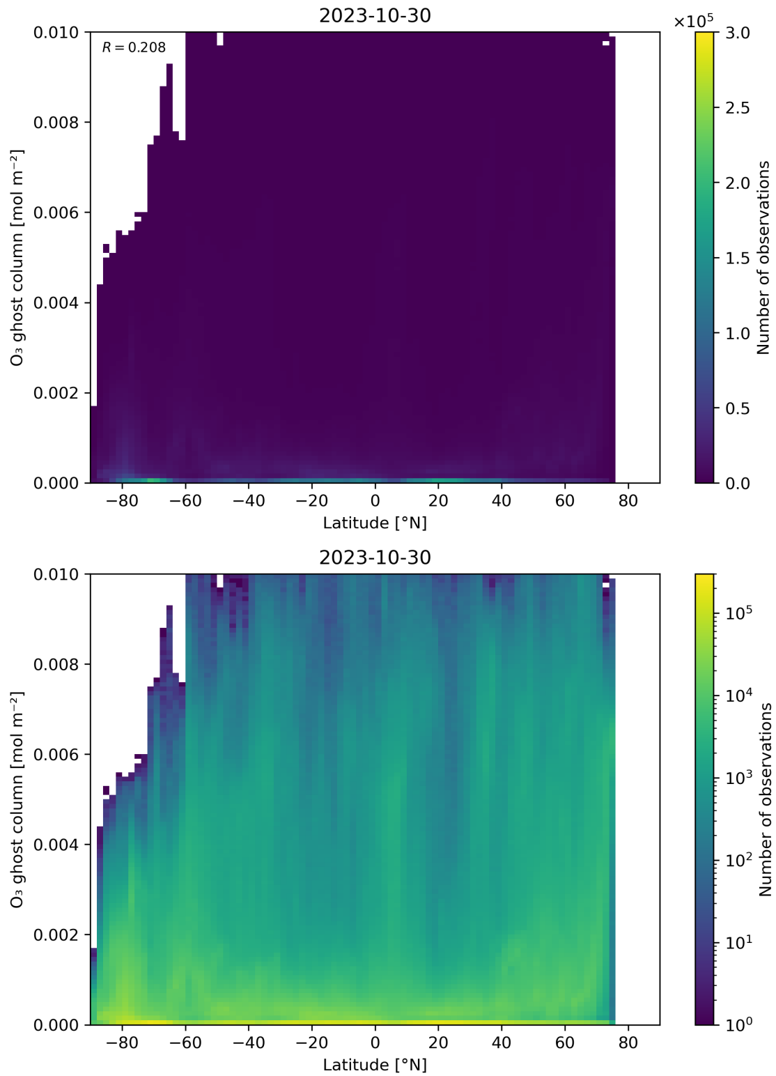
Figure 35: Scatter density plot of “Latitude” against “O 3 ghost column” for 2023-10-29 to 2023-10-31.
