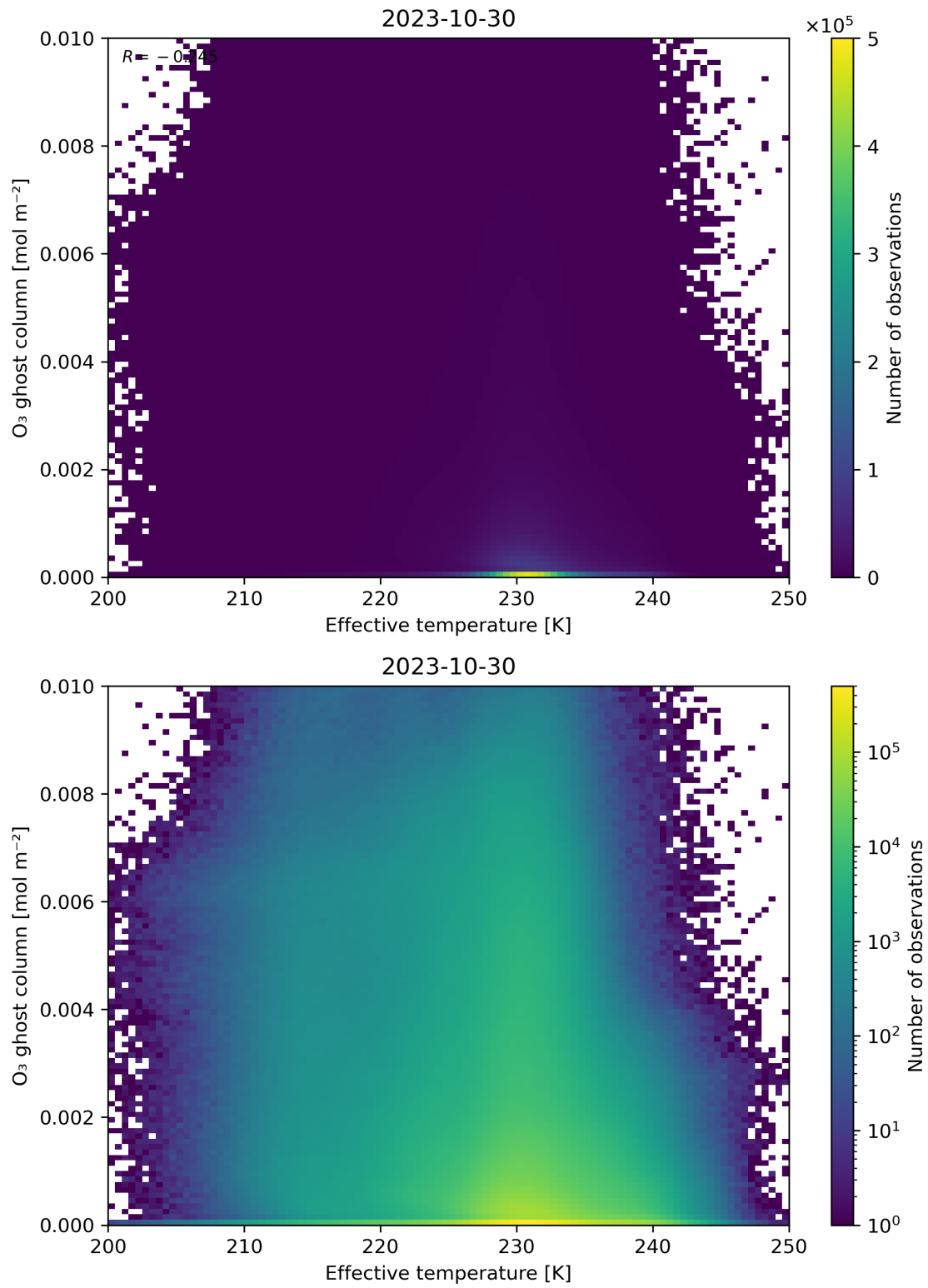
Figure 38: Scatter density plot of “Effective temperature” against “O 3 ghost column” for 2023-10-29 to 2023-10-31.
