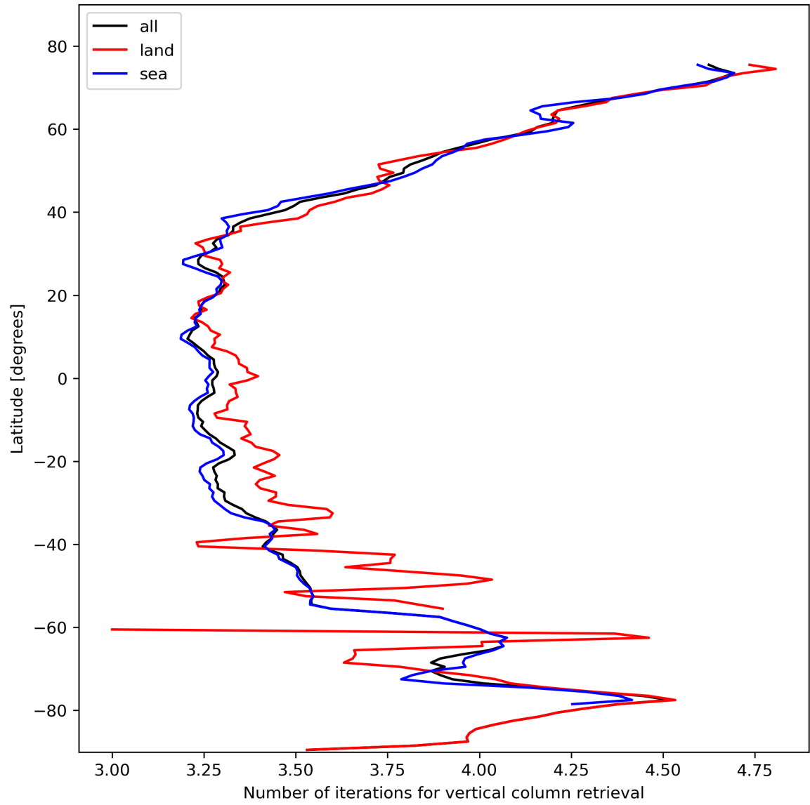
Figure 19: Zonal average of “Number of iterations for vertical column retrieval” for 2023-10-29 to 2023-10-31.
