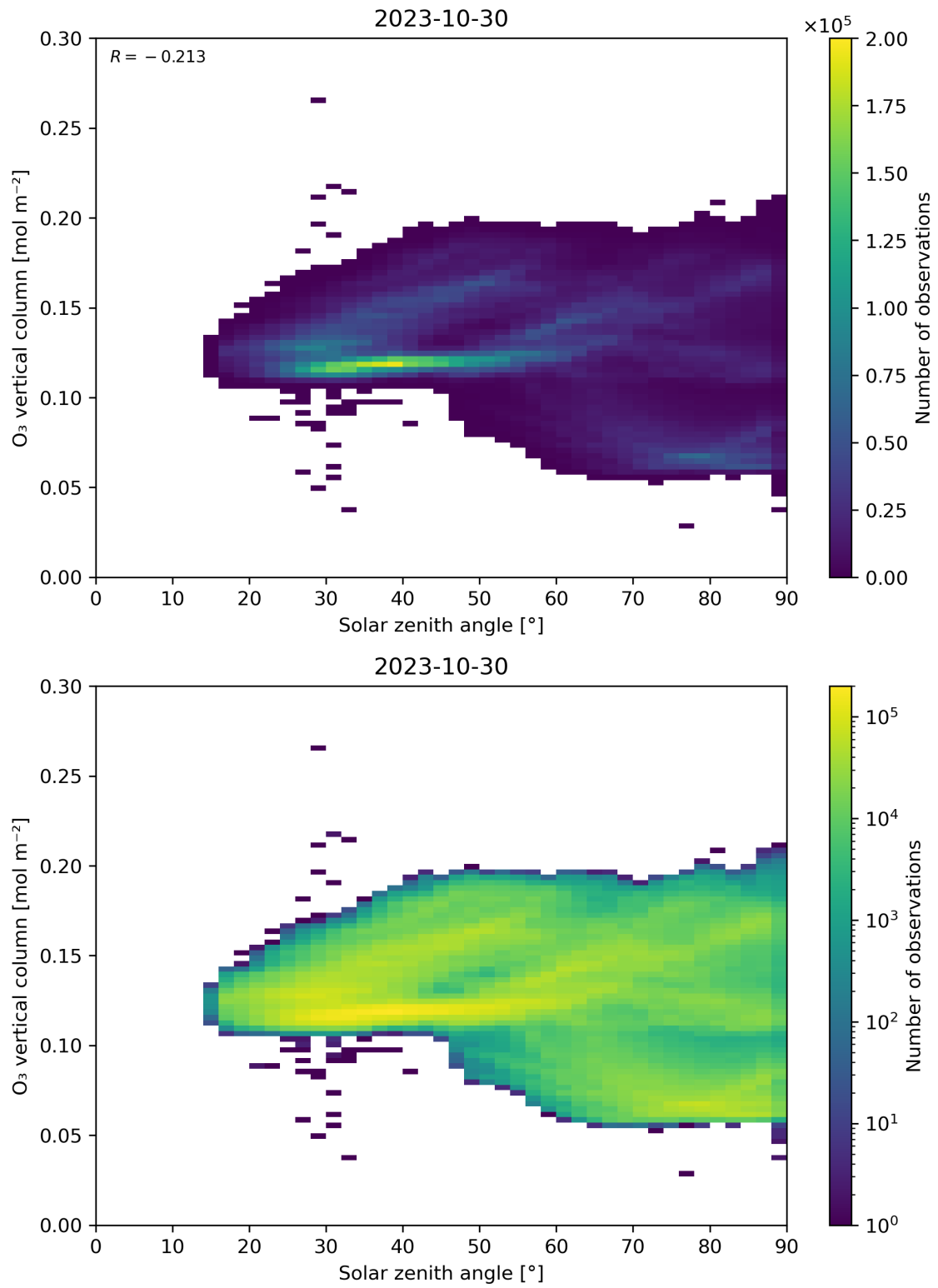
Figure 47: Scatter density plot of “Solar zenith angle” against “O 3 vertical column” for 2023-10-29 to 2023-10-31.
