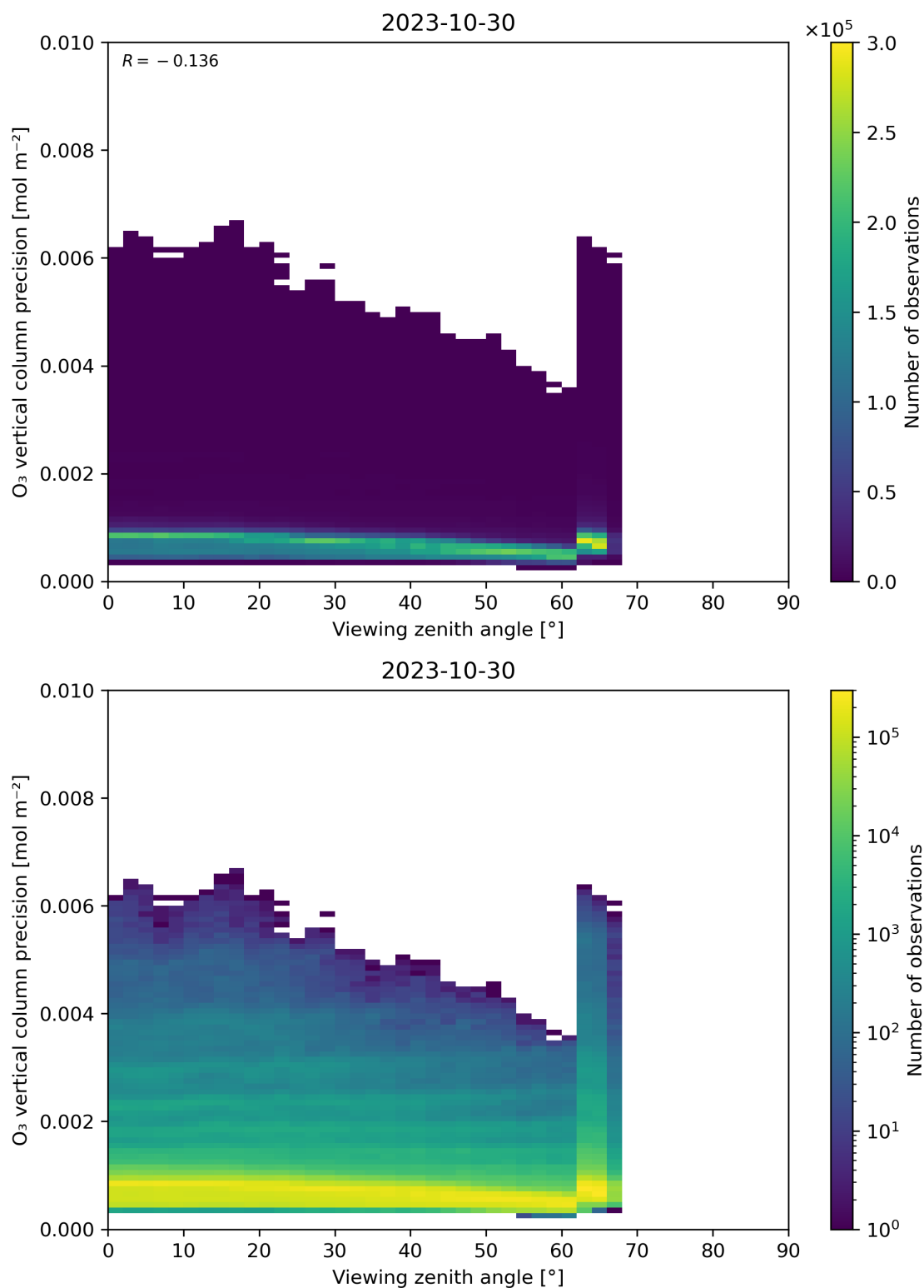
Figure 53: Scatter density plot of “Viewing zenith angle” against “O 3 vertical column precision” for 2023-10-29 to 2023-10-31.
