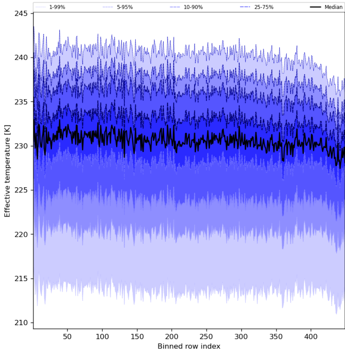
Figure 31: Along track statistics of “Effective temperature” for 2023-10-29 to 2023-10-31
