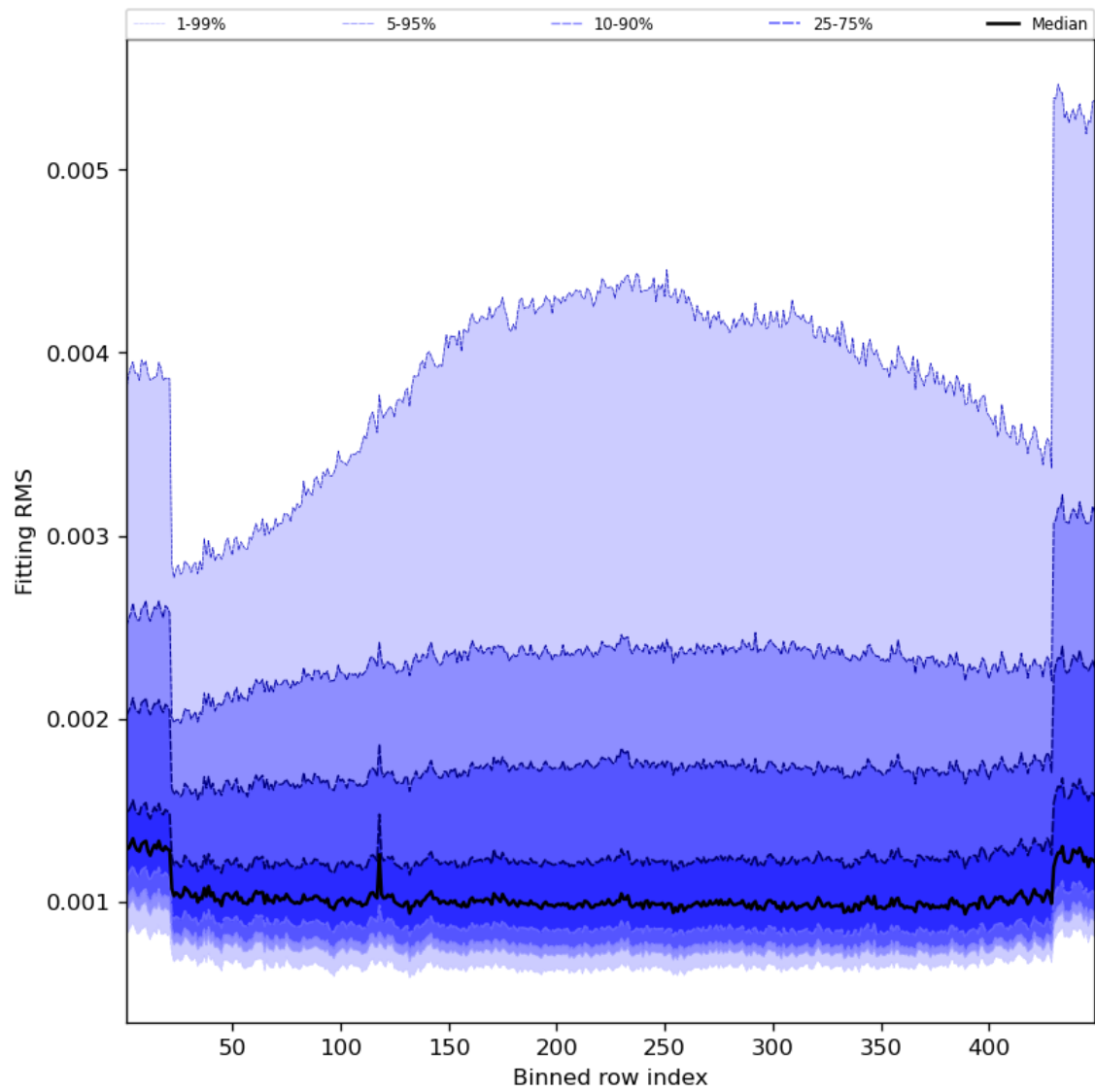
Figure 30: Along track statistics of “Fitting RMS” for 2023-10-29 to 2023-10-31
