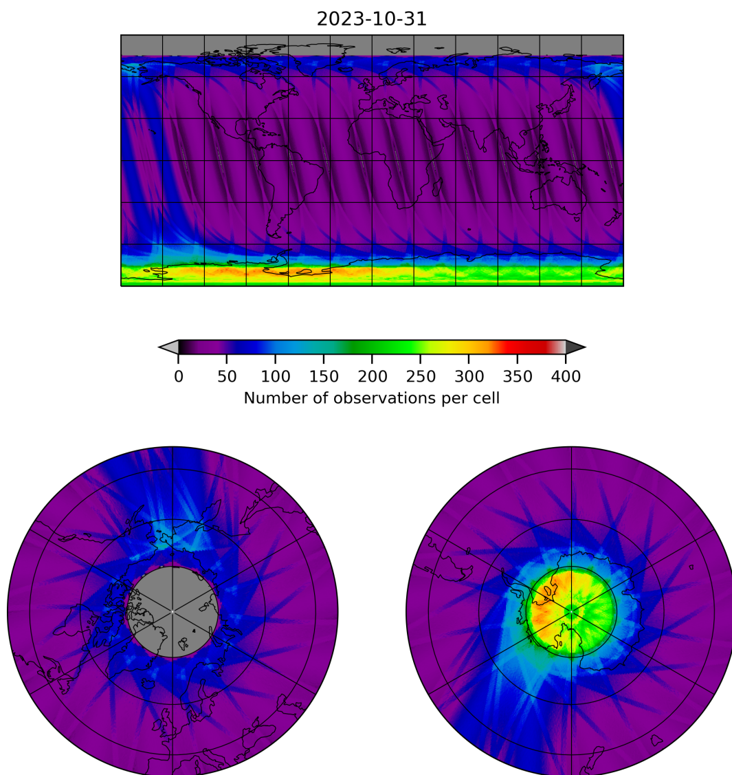
Figure 12: Map of the number of observations for 2023-10-30 to 2023-11-01
