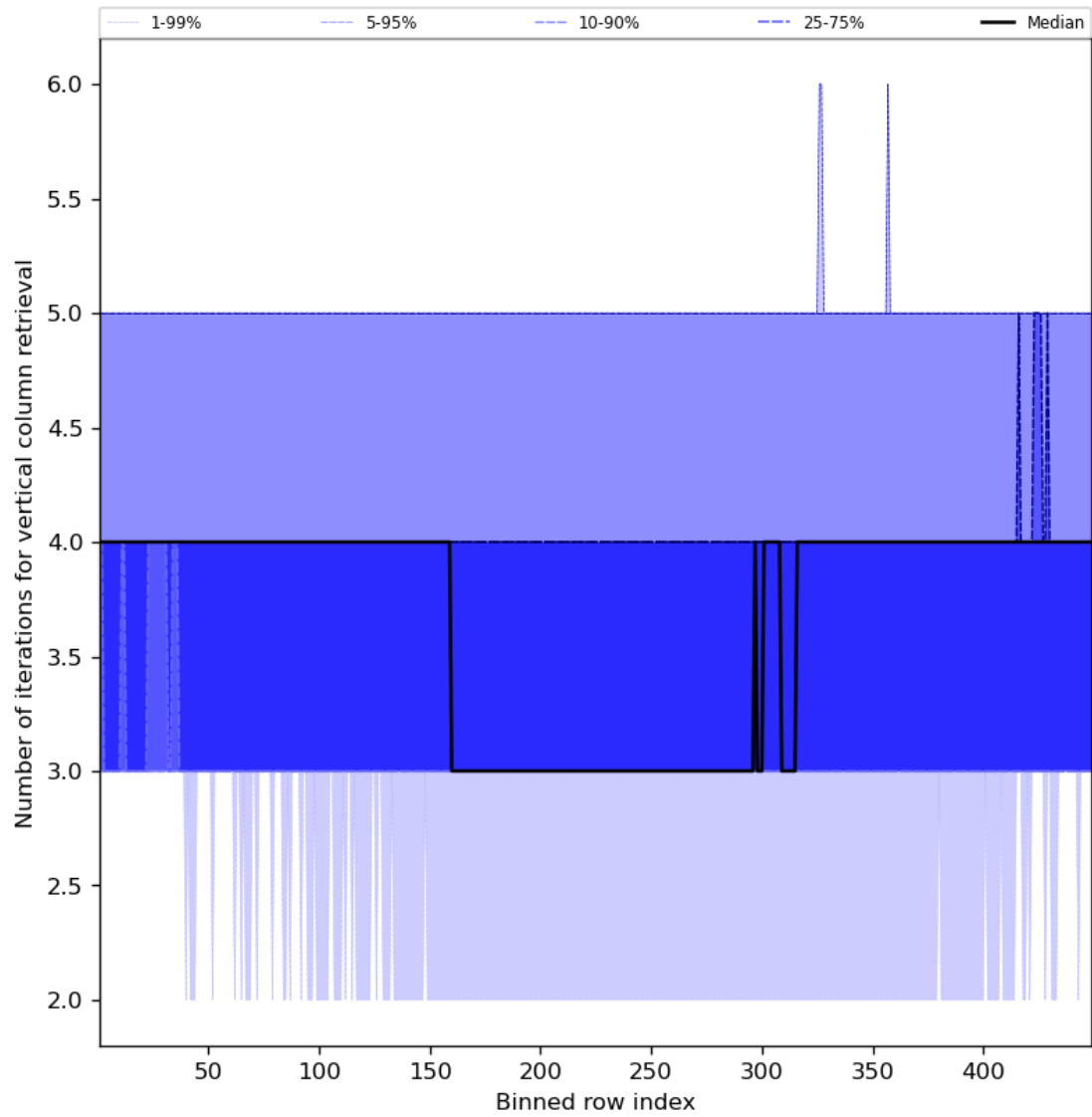
Figure 33: Along track statistics of “Number of iterations for vertical column retrieval” for 2023-10-30 to 2023-11-01
