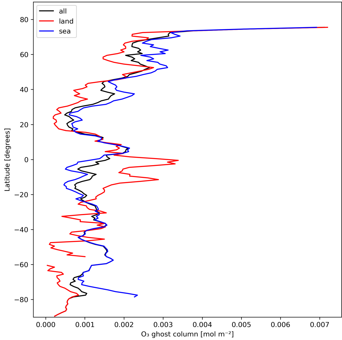
Figure 18: Zonal average of “O 3 ghost column” for 2023-10-30 to 2023-11-01.
