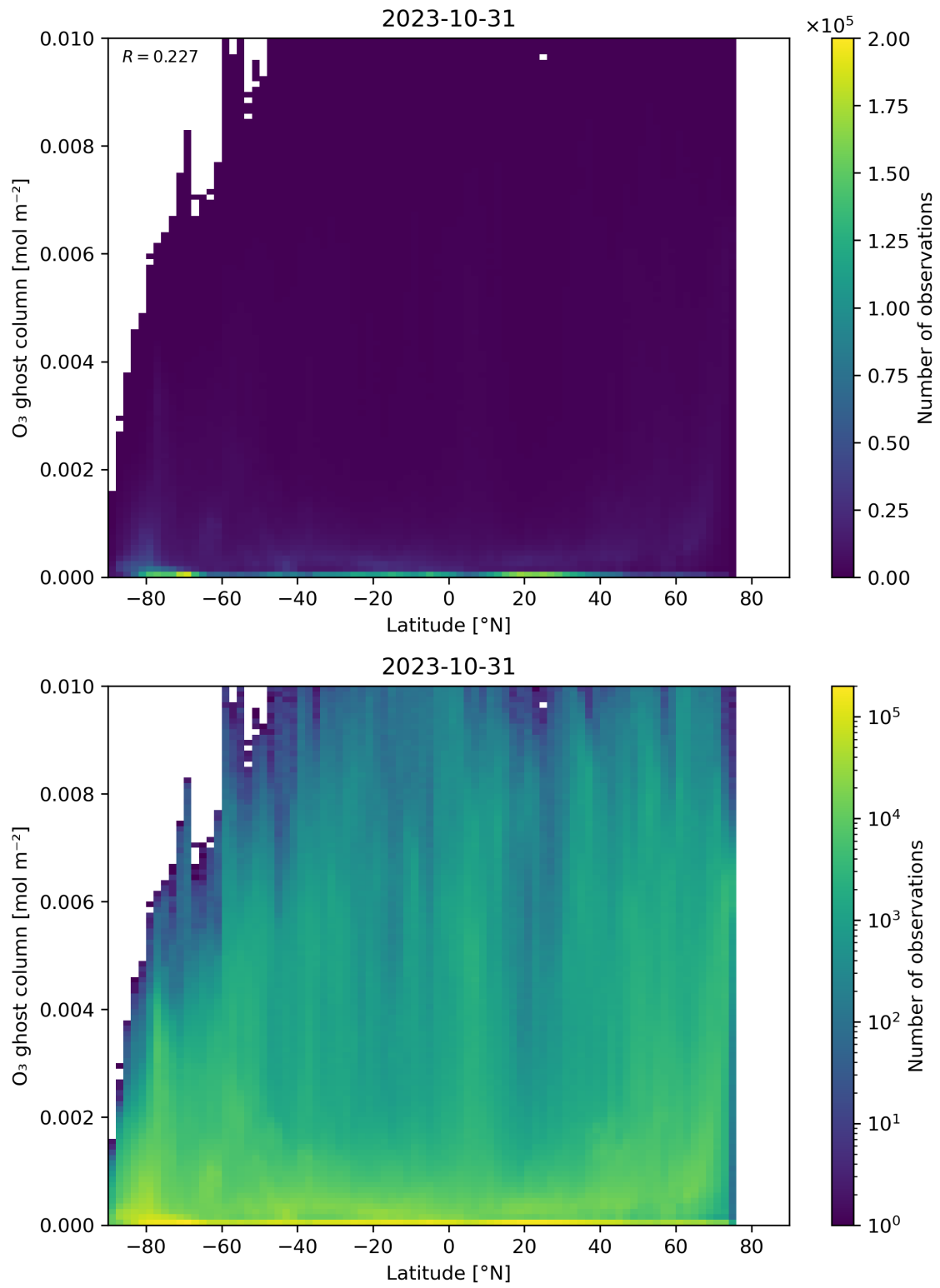
Figure 35: Scatter density plot of “Latitude” against “O 3 ghost column” for 2023-10-30 to 2023-11-01.
