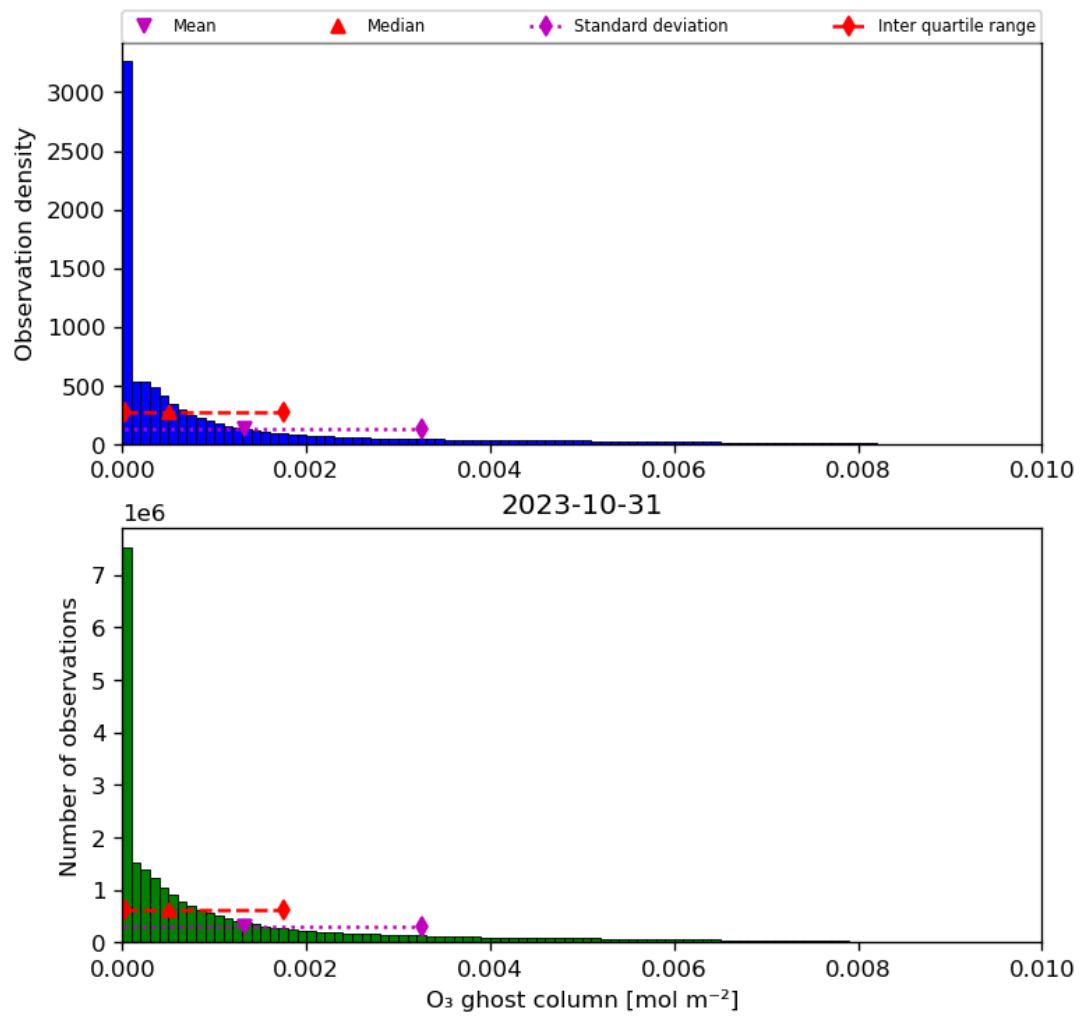
Figure 25: Histogram of “O 3 ghost column” for 2023-10-30 to 2023-11-01
