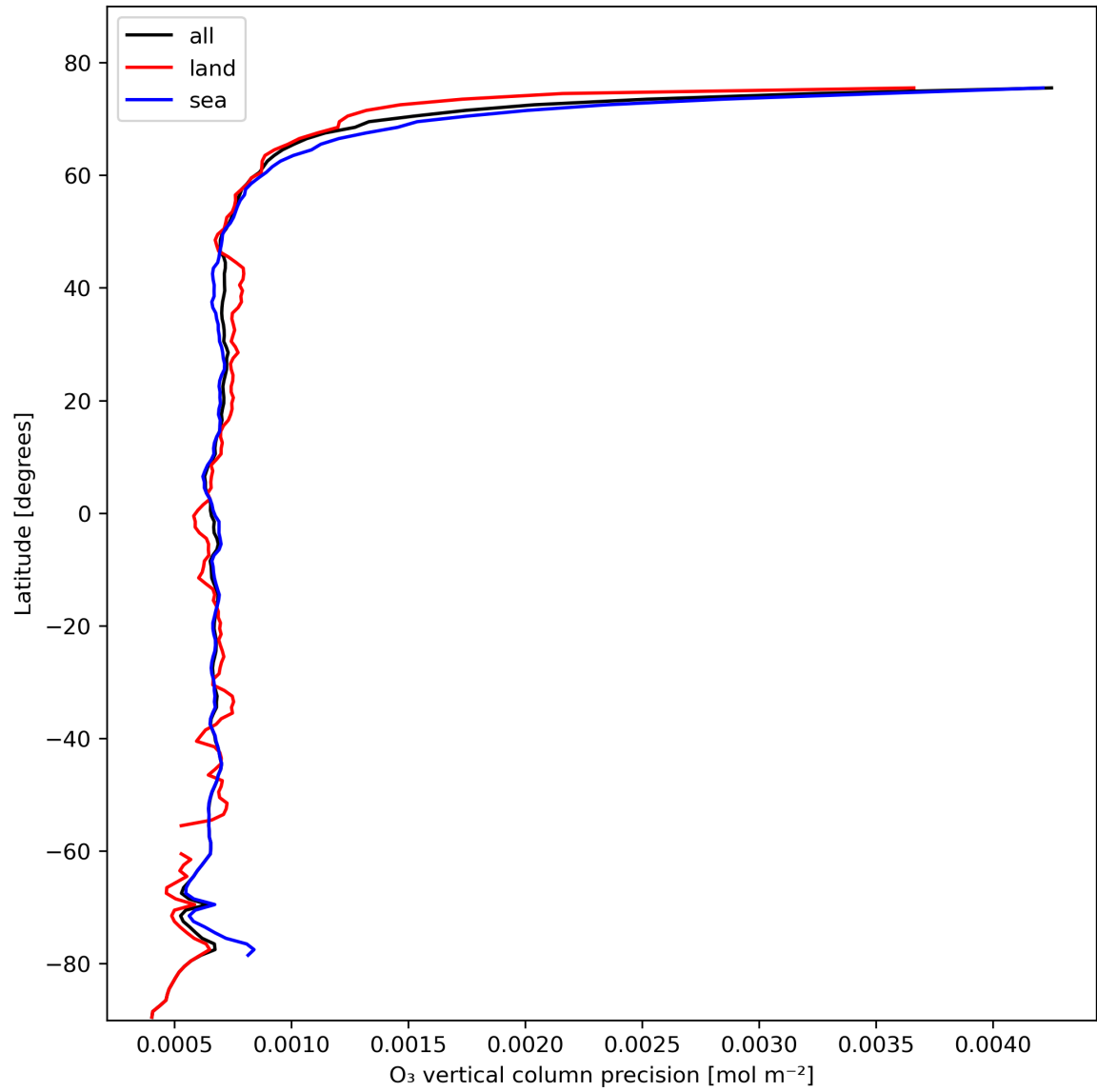
Figure 15: Zonal average of “O 3 vertical column precision” for 2023-10-30 to 2023-11-01.
