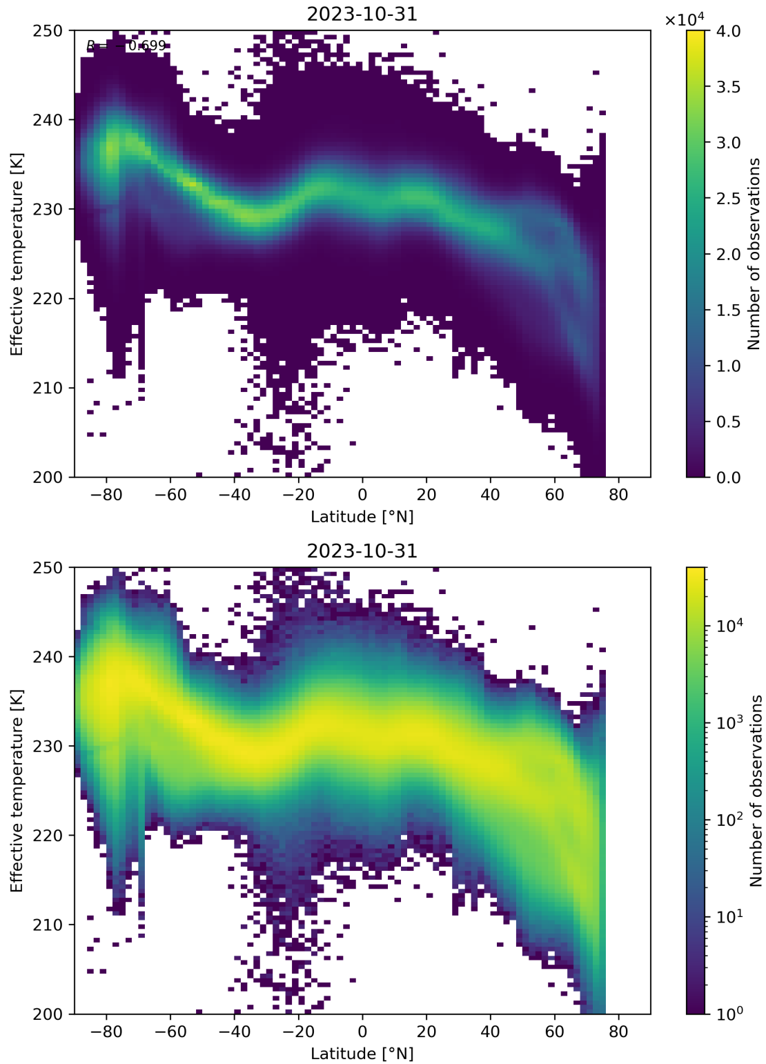
Figure 34: Scatter density plot of “Latitude” against “Effective temperature” for 2023-10-30 to 2023-11-01.
