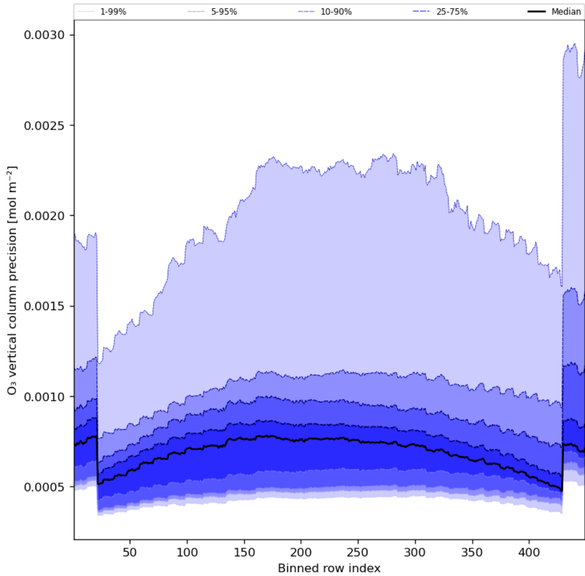
Figure 29: Along track statistics of “O 3 vertical column precision” for 2023-10-30 to 2023-11-01
