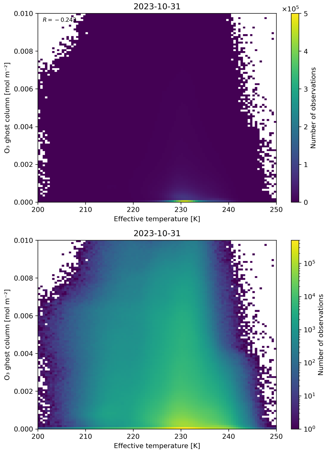
Figure 38: Scatter density plot of “Effective temperature” against “O 3 ghost column” for 2023-10-30 to 2023-11-01.
