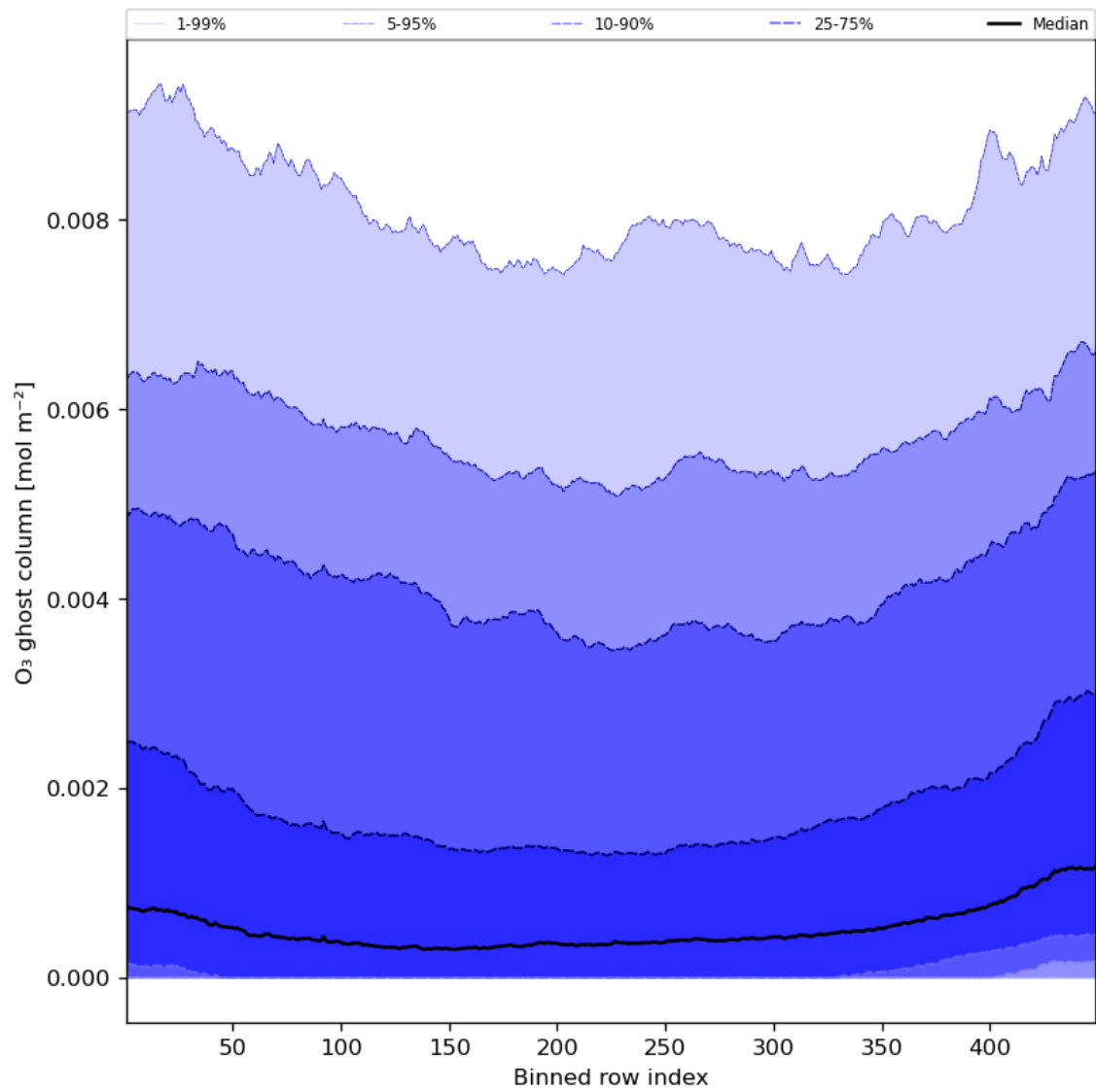
Figure 32: Along track statistics of “O 3 ghost column” for 2023-10-30 to 2023-11-01
