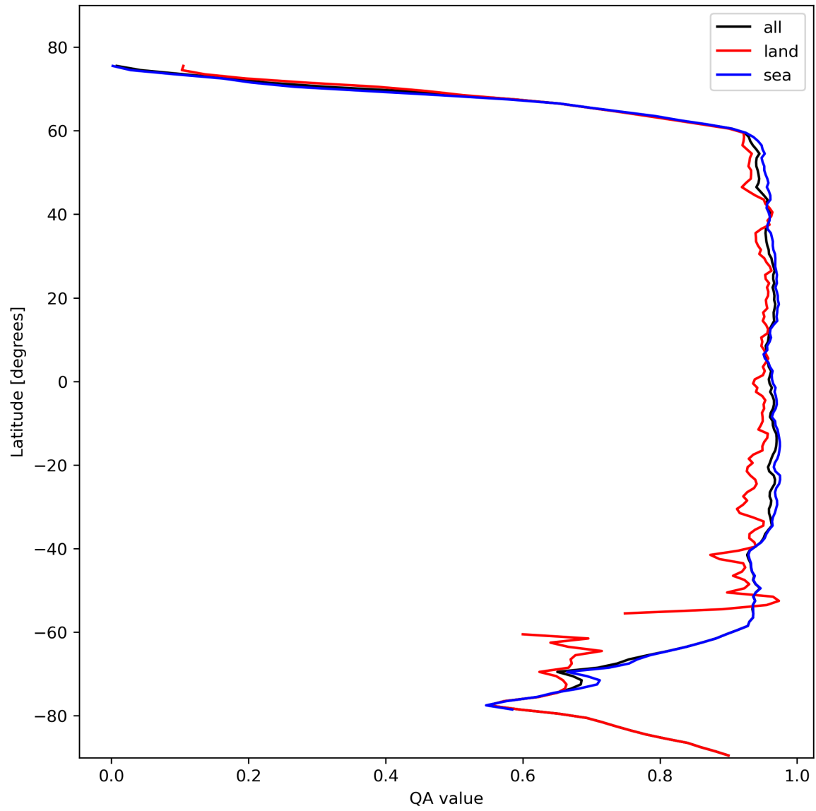
Figure 13: Zonal average of “QA value” for 2023-10-30 to 2023-11-01.
