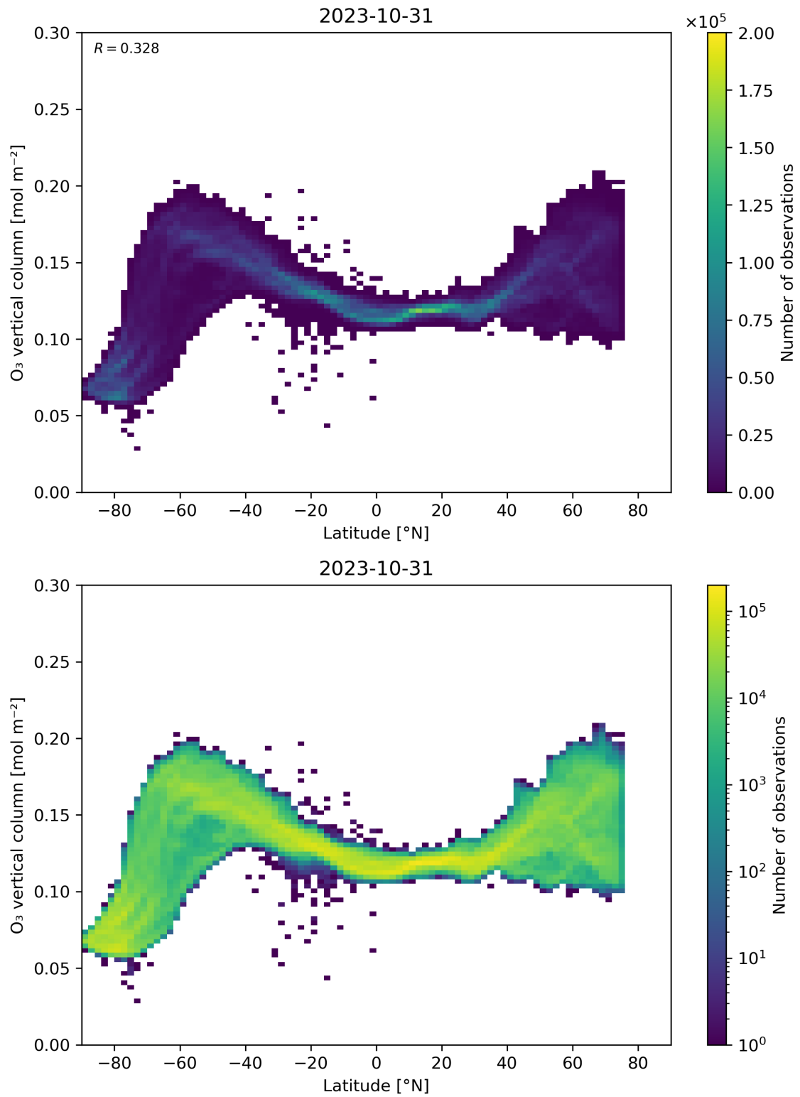
Figure 36: Scatter density plot of “Latitude” against “O 3 vertical column” for 2023-10-30 to 2023-11-01.
