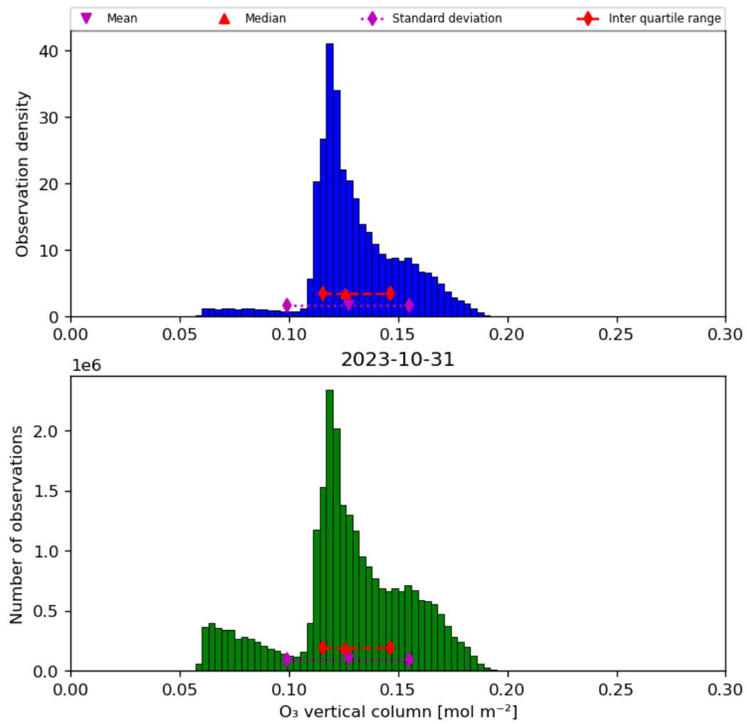
Figure 21: Histogram of “O 3 vertical column” for 2023-10-30 to 2023-11-01
