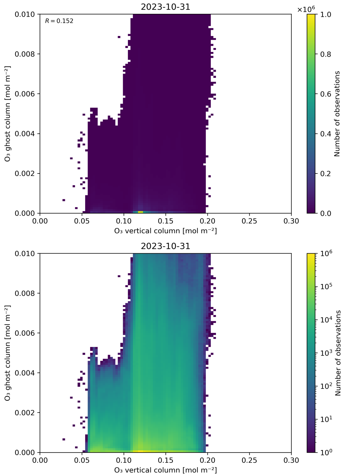
Figure 40: Scatter density plot of “O 3 vertical column” against “O 3 ghost column” for 2023-10-30 to 2023-11-01.
