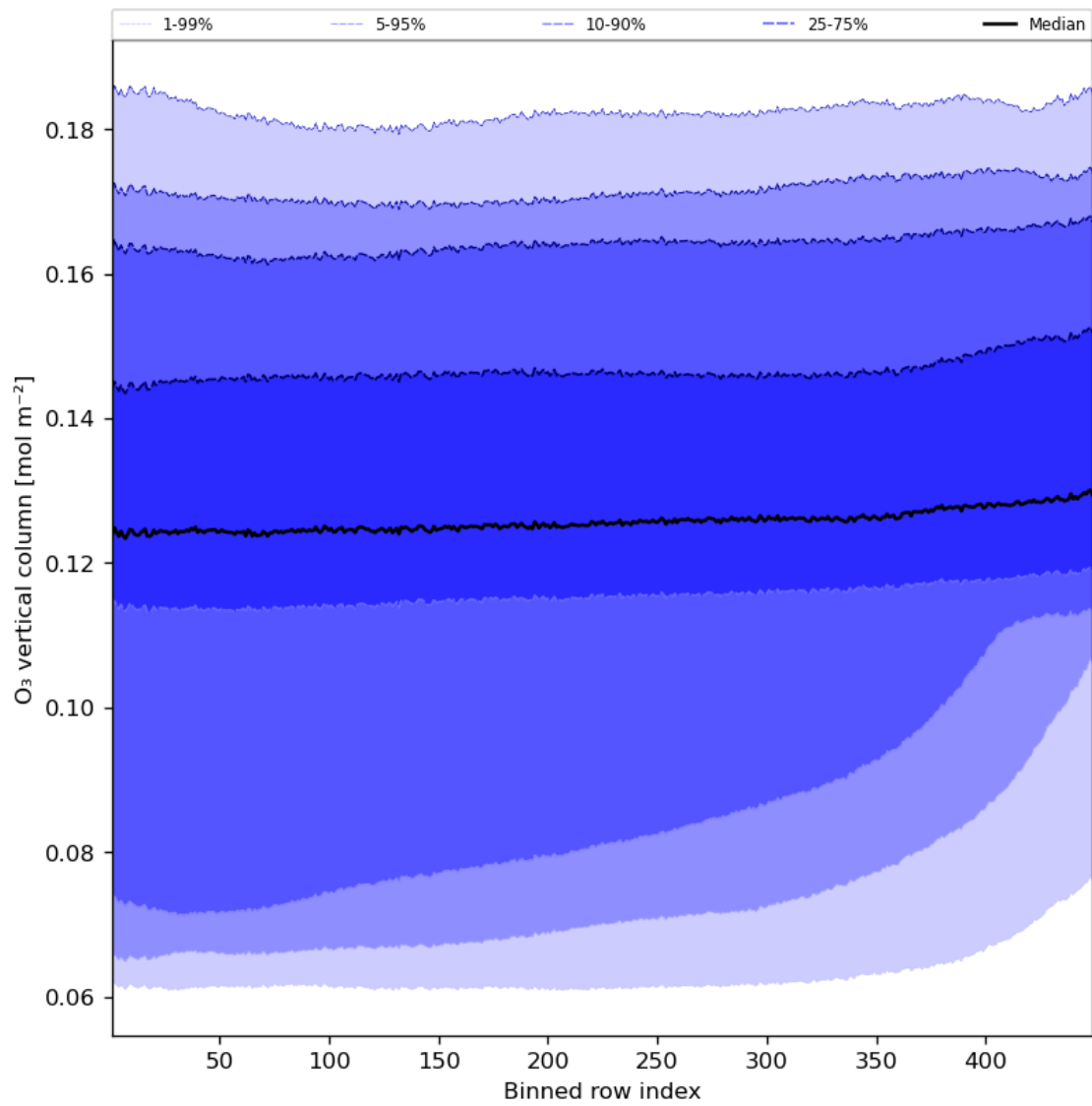
Figure 28: Along track statistics of “O 3 vertical column” for 2023-10-30 to 2023-11-01
