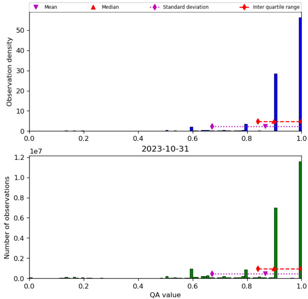
Figure 20: Histogram of “QA value” for 2023-10-30 to 2023-11-01
