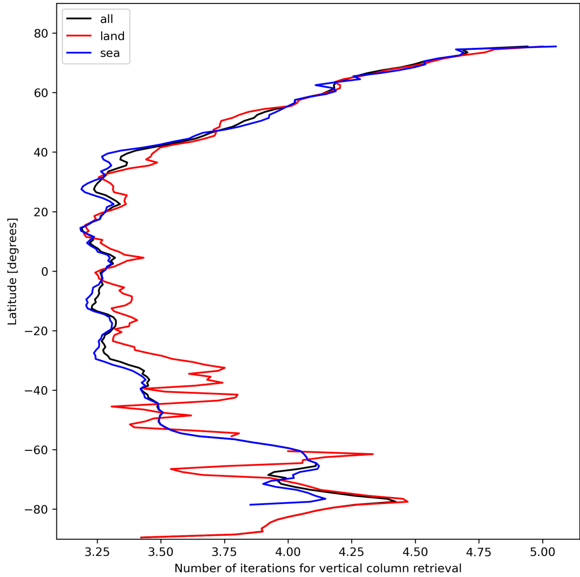
Figure 19: Zonal average of “Number of iterations for vertical column retrieval” for 2023-10-30 to 2023-11-01.
