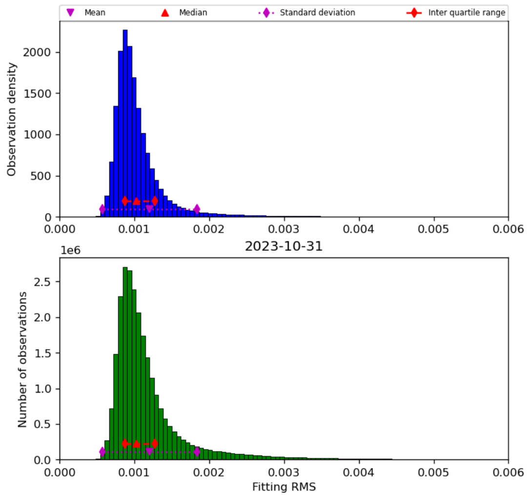
Figure 23: Histogram of “Fitting RMS” for 2023-10-30 to 2023-11-01
