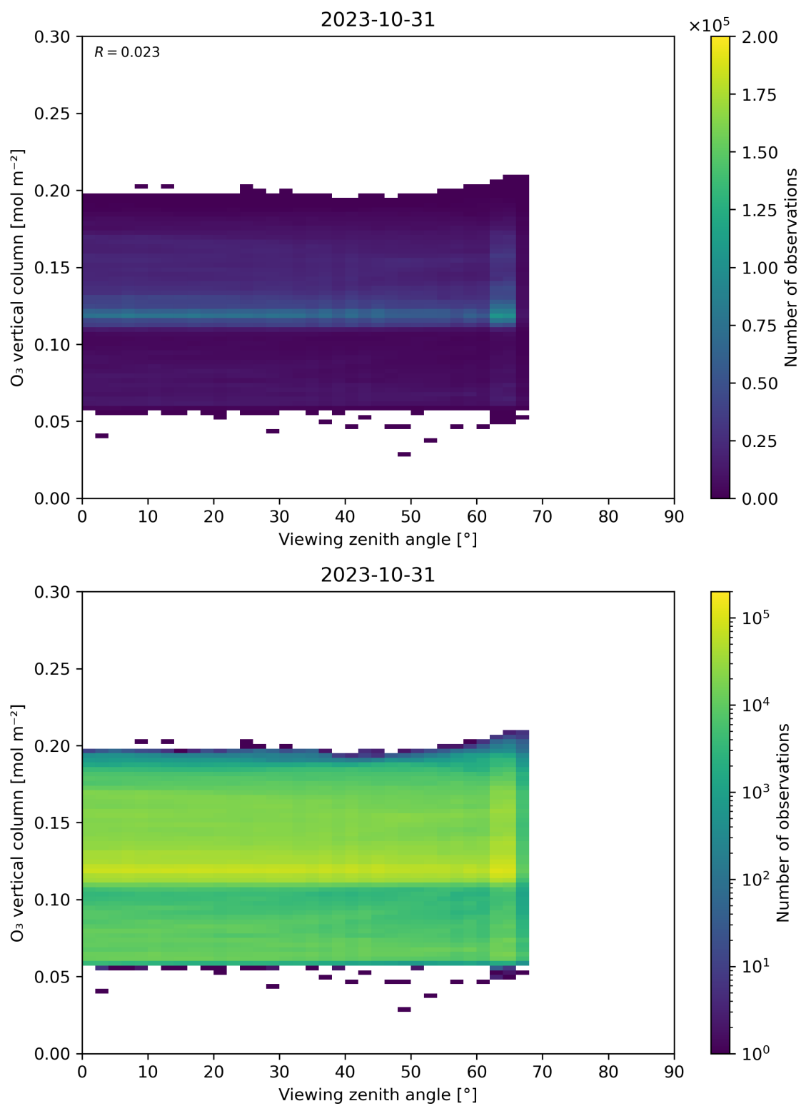
Figure 52: Scatter density plot of “Viewing zenith angle” against “O 3 vertical column” for 2023-10-30 to 2023-11-01.
