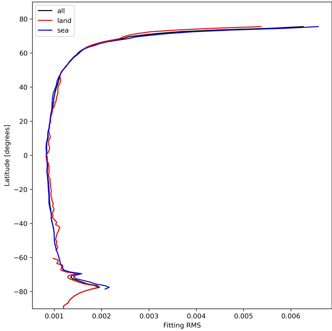
Figure 16: Zonal average of “Fitting RMS” for 2023-10-30 to 2023-11-01.
