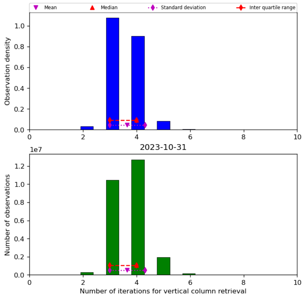
Figure 26: Histogram of “Number of iterations for vertical column retrieval” for 2023-10-30 to 2023-11-01
