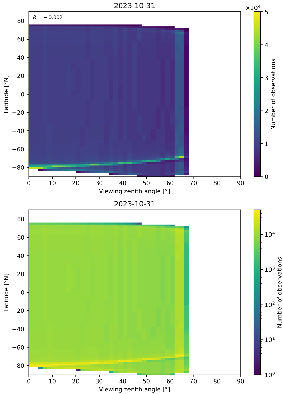
Figure 49: Scatter density plot of “Viewing zenith angle” against “Latitude” for 2023-10-30 to 2023-11-01.
