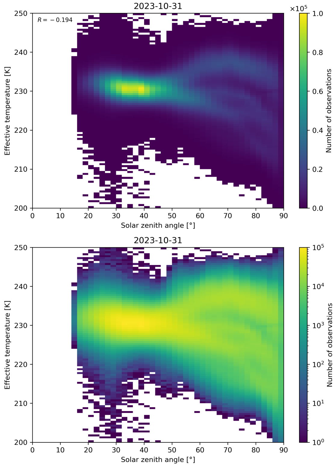
Figure 45: Scatter density plot of “Solar zenith angle” against “Effective temperature” for 2023-10-30 to 2023-11-01.
