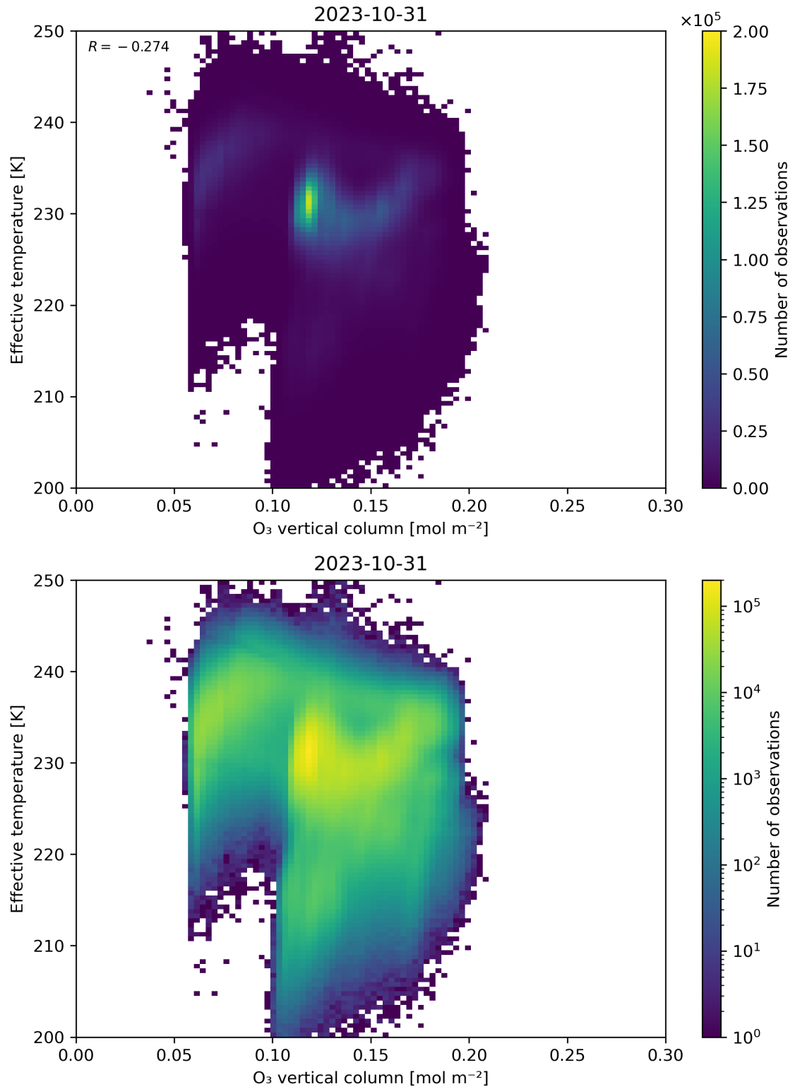
Figure 39: Scatter density plot of “O 3 vertical column” against “Effective temperature” for 2023-10-30 to 2023-11-01.
