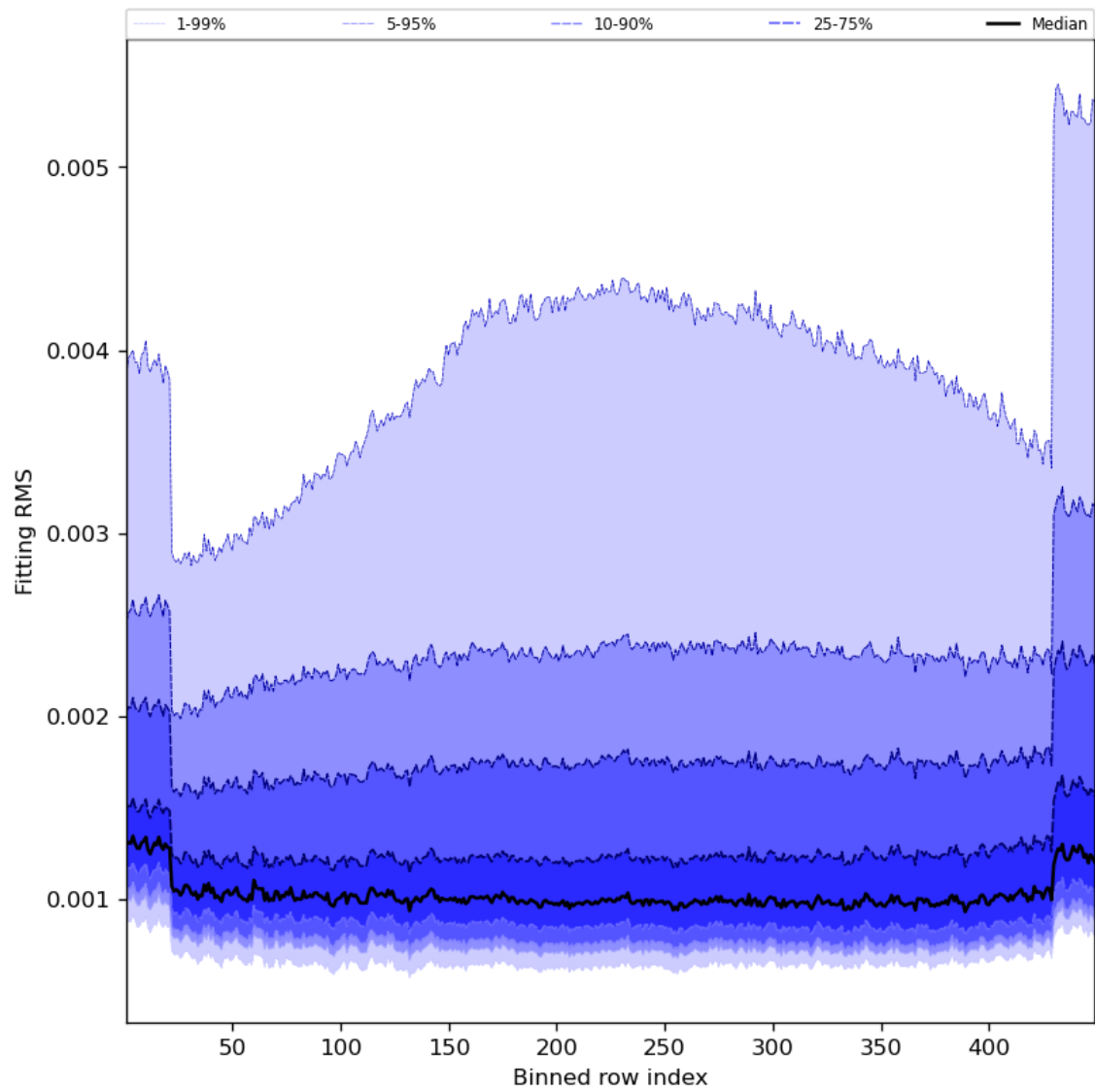
Figure 30: Along track statistics of “Fitting RMS” for 2023-10-30 to 2023-11-01
