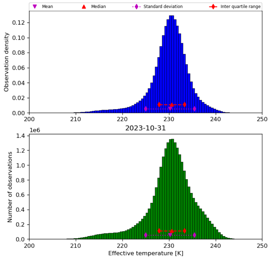
Figure 24: Histogram of “Effective temperature” for 2023-10-30 to 2023-11-01
