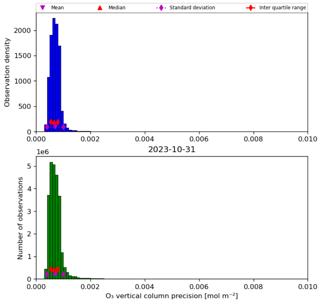
Figure 22: Histogram of “O 3 vertical column precision” for 2023-10-30 to 2023-11-01
