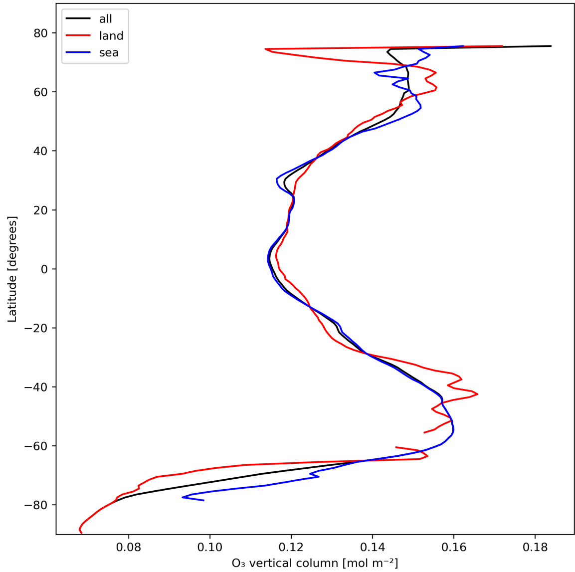
Figure 14: Zonal average of “O 3 vertical column” for 2023-10-30 to 2023-11-01.
