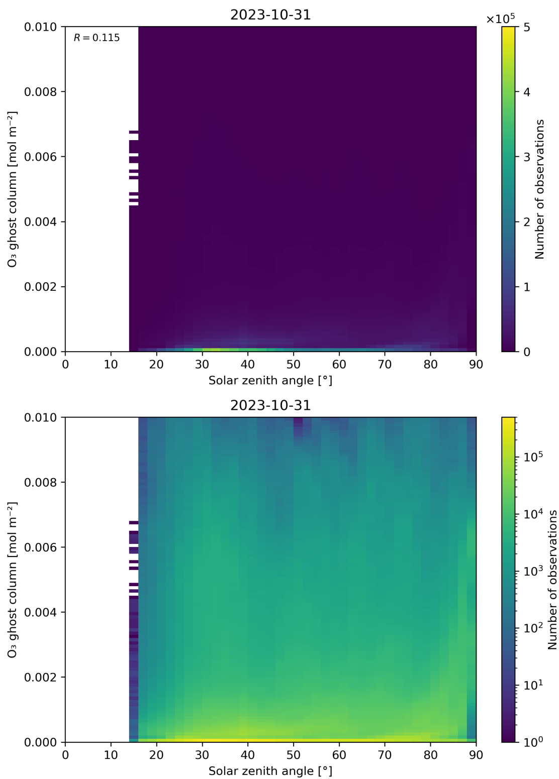
Figure 46: Scatter density plot of “Solar zenith angle” against “O 3 ghost column” for 2023-10-30 to 2023-11-01.
