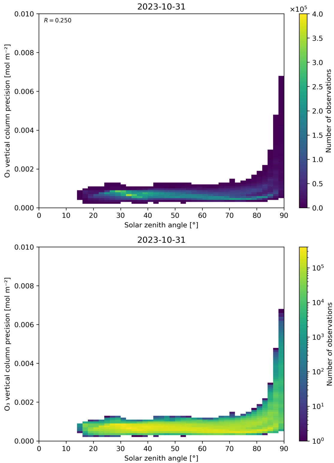
Figure 48: Scatter density plot of “Solar zenith angle” against “O 3 vertical column precision” for 2023-10-30 to 2023-11-01.
