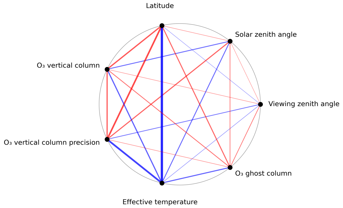
Figure 1: Map of correlation graph for 2023-10-30 to 2023-11-01.
