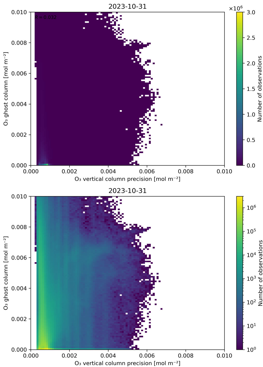
Figure 43: Scatter density plot of “O 3 vertical column precision” against “O 3 ghost column” for 2023-10-30 to 2023-11-01.
