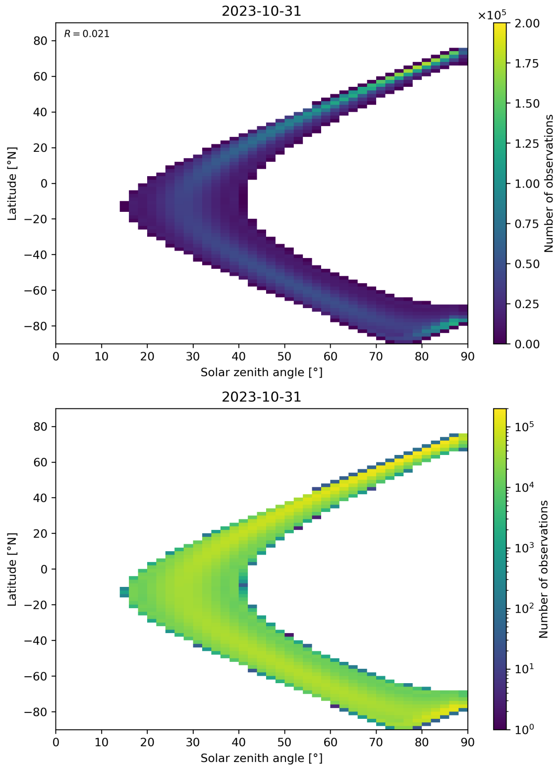
Figure 44: Scatter density plot of “Solar zenith angle” against “Latitude” for 2023-10-30 to 2023-11-01.
