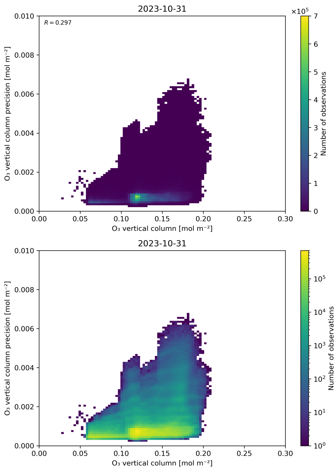
Figure 41: Scatter density plot of “O 3 vertical column” against “O 3 vertical column precision” for 2023-10-30 to 2023-11-01.
