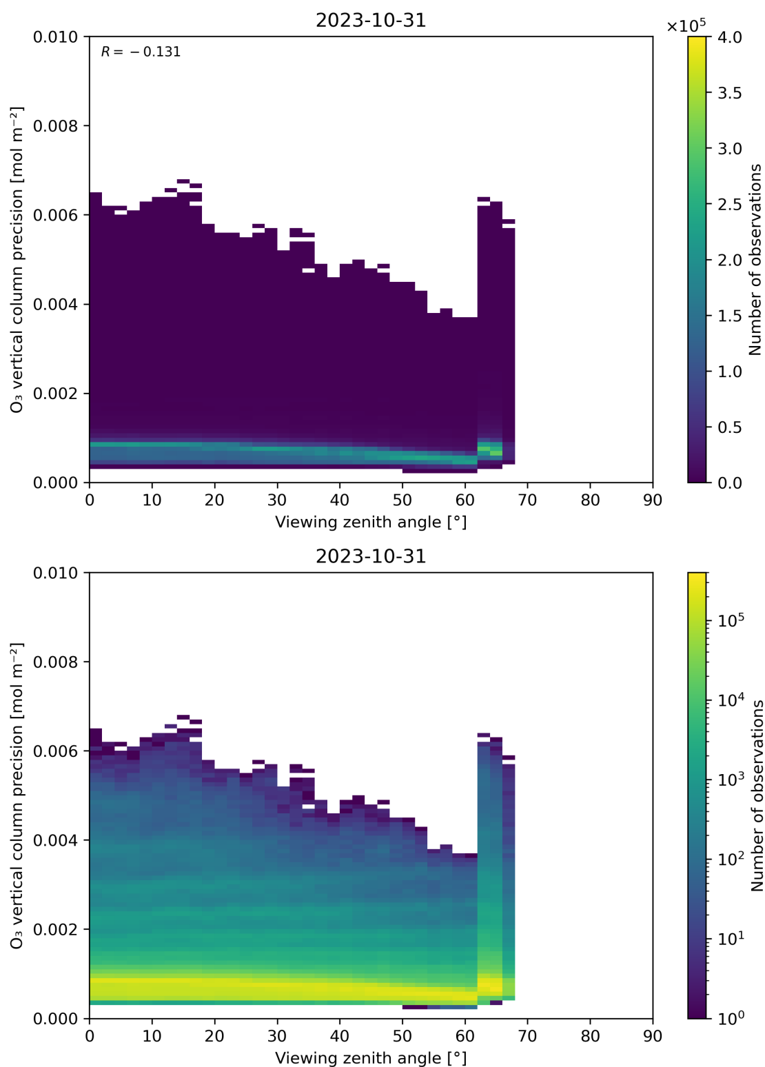
Figure 53: Scatter density plot of “Viewing zenith angle” against “O 3 vertical column precision” for 2023-10-30 to 2023-11-01.
