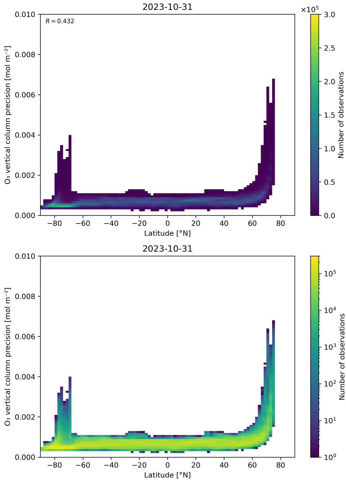
Figure 37: Scatter density plot of “Latitude” against “O 3 vertical column precision” for 2023-10-30 to 2023-11-01.
