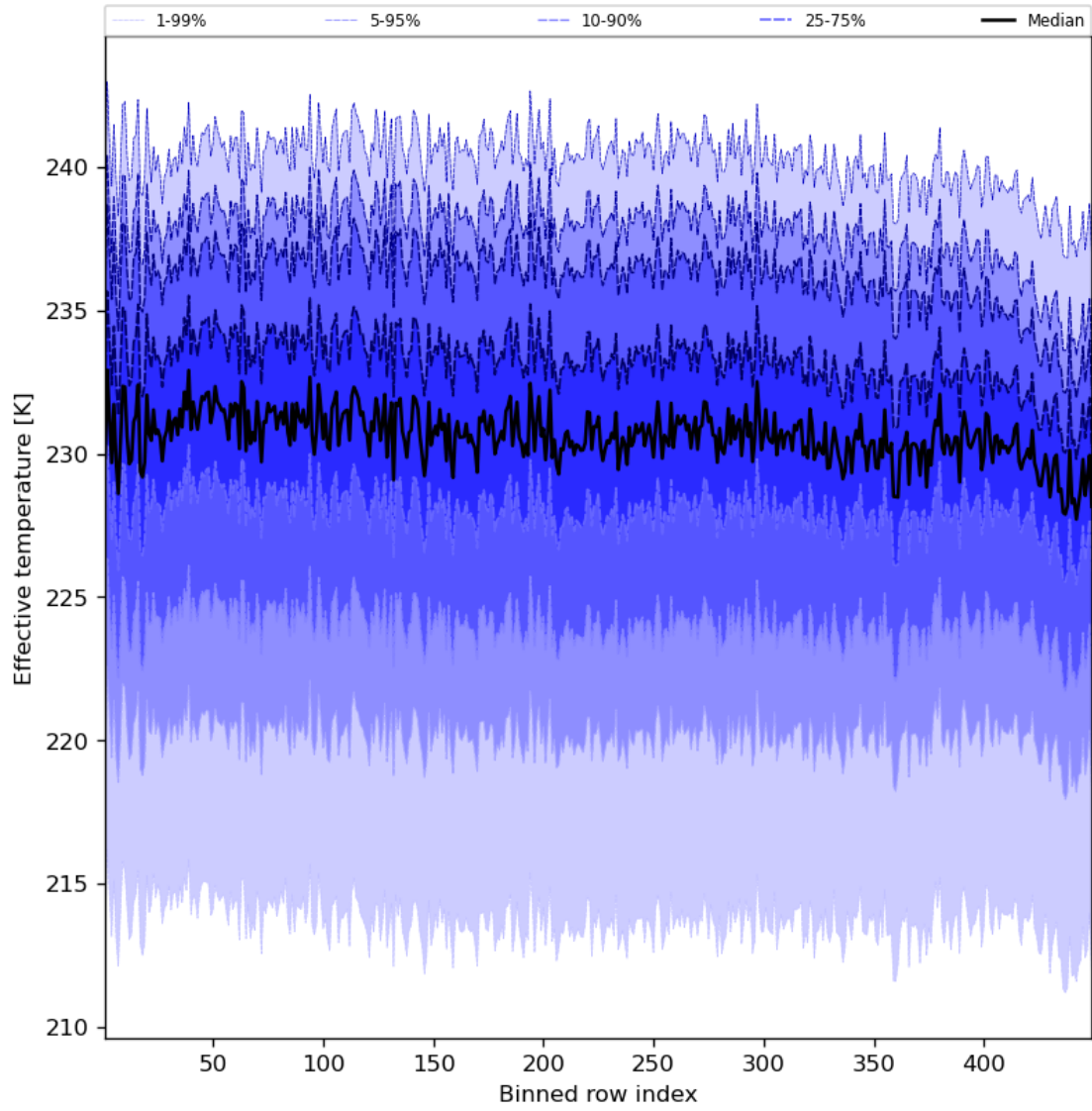
Figure 31: Along track statistics of “Effective temperature” for 2023-10-30 to 2023-11-01
