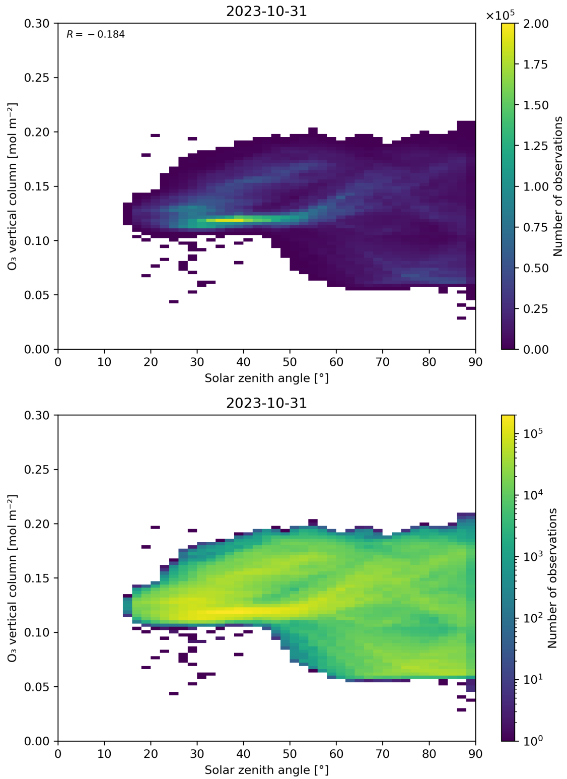
Figure 47: Scatter density plot of “Solar zenith angle” against “O 3 vertical column” for 2023-10-30 to 2023-11-01.
