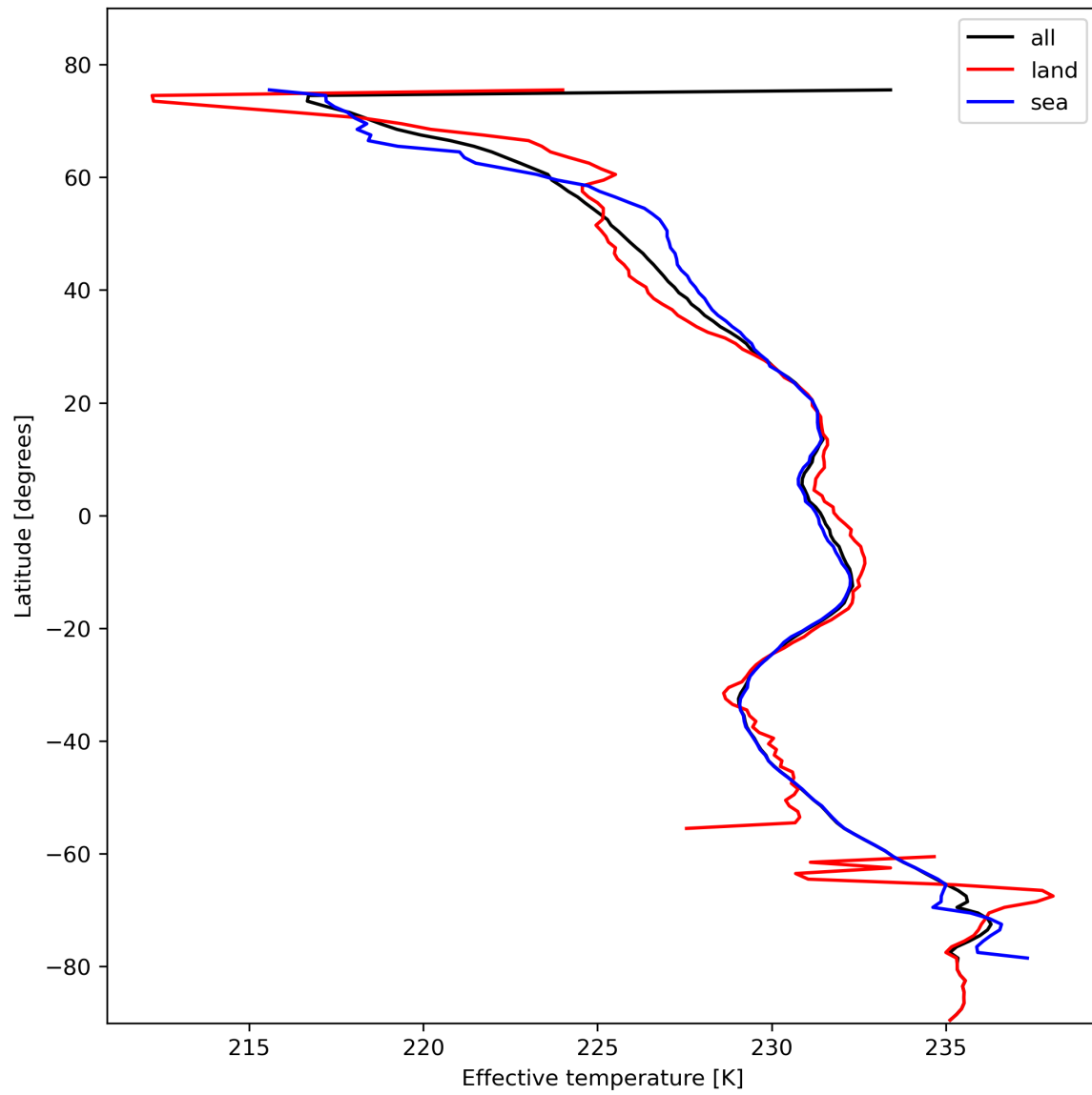
Figure 17: Zonal average of “Effective temperature” for 2023-10-30 to 2023-11-01.
