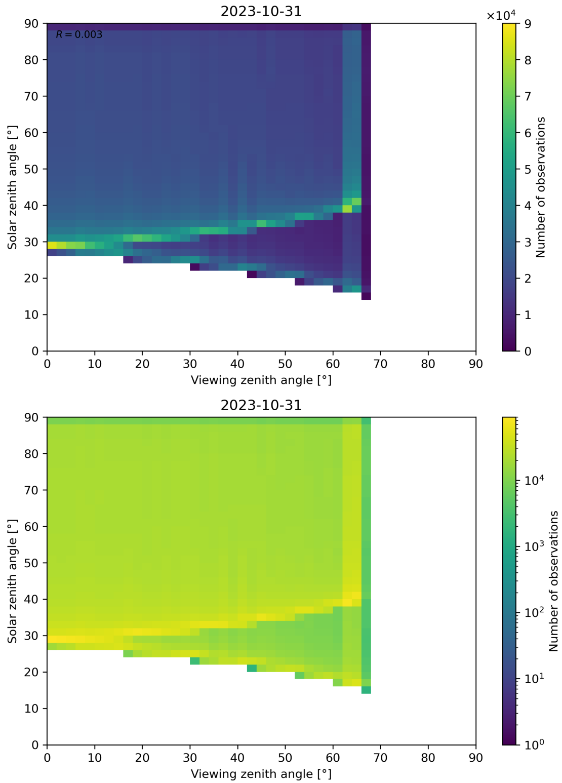
Figure 54: Scatter density plot of “Viewing zenith angle” against “Solar zenith angle” for 2023-10-30 to 2023-11-01.
