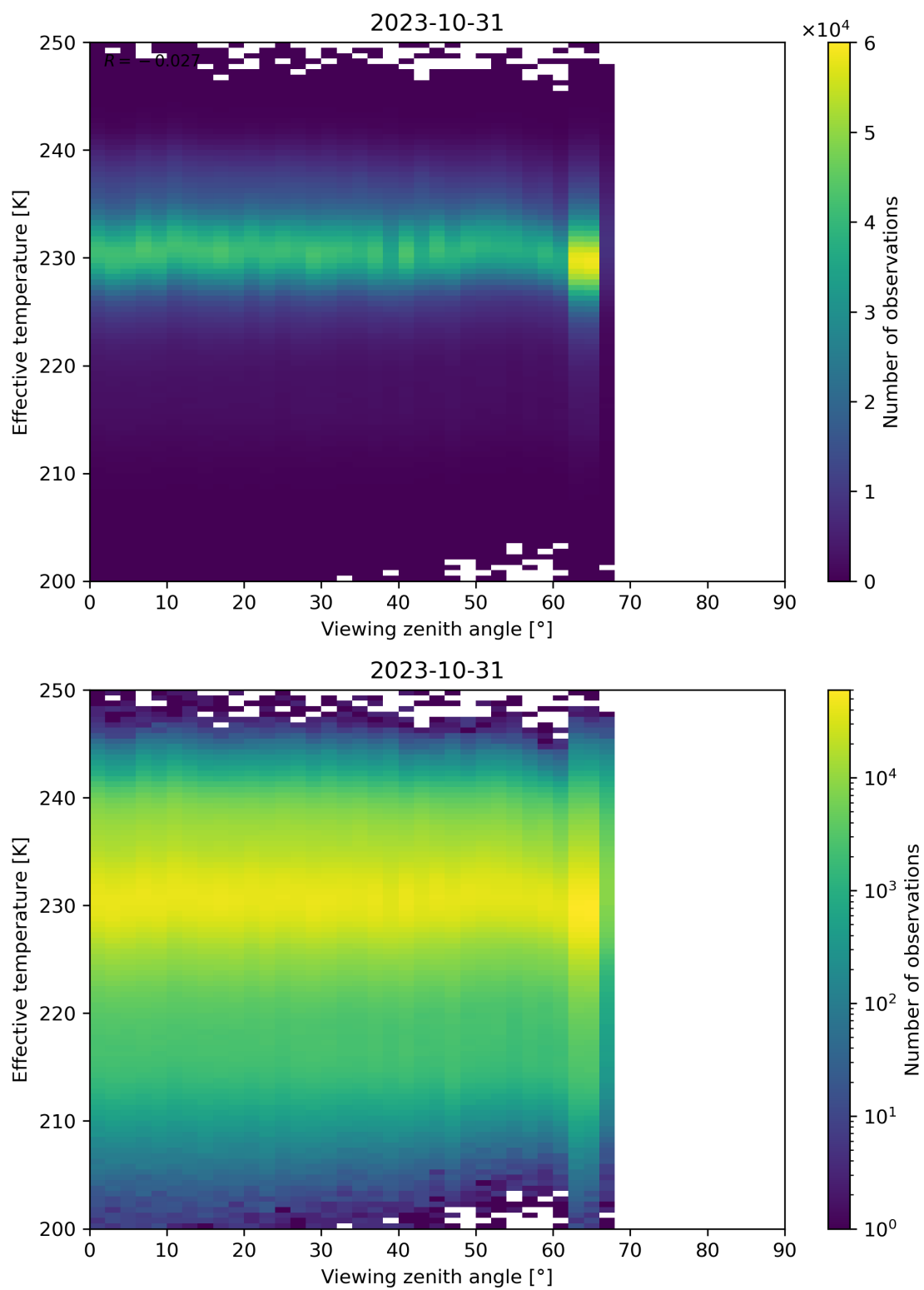
Figure 50: Scatter density plot of “Viewing zenith angle” against “Effective temperature” for 2023-10-30 to 2023-11-01.
