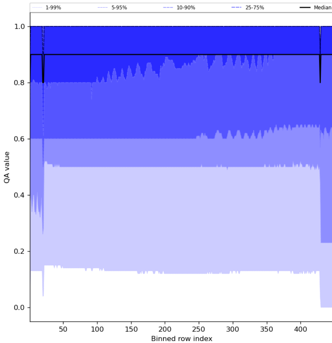
Figure 27: Along track statistics of “QA value” for 2023-10-30 to 2023-11-01
