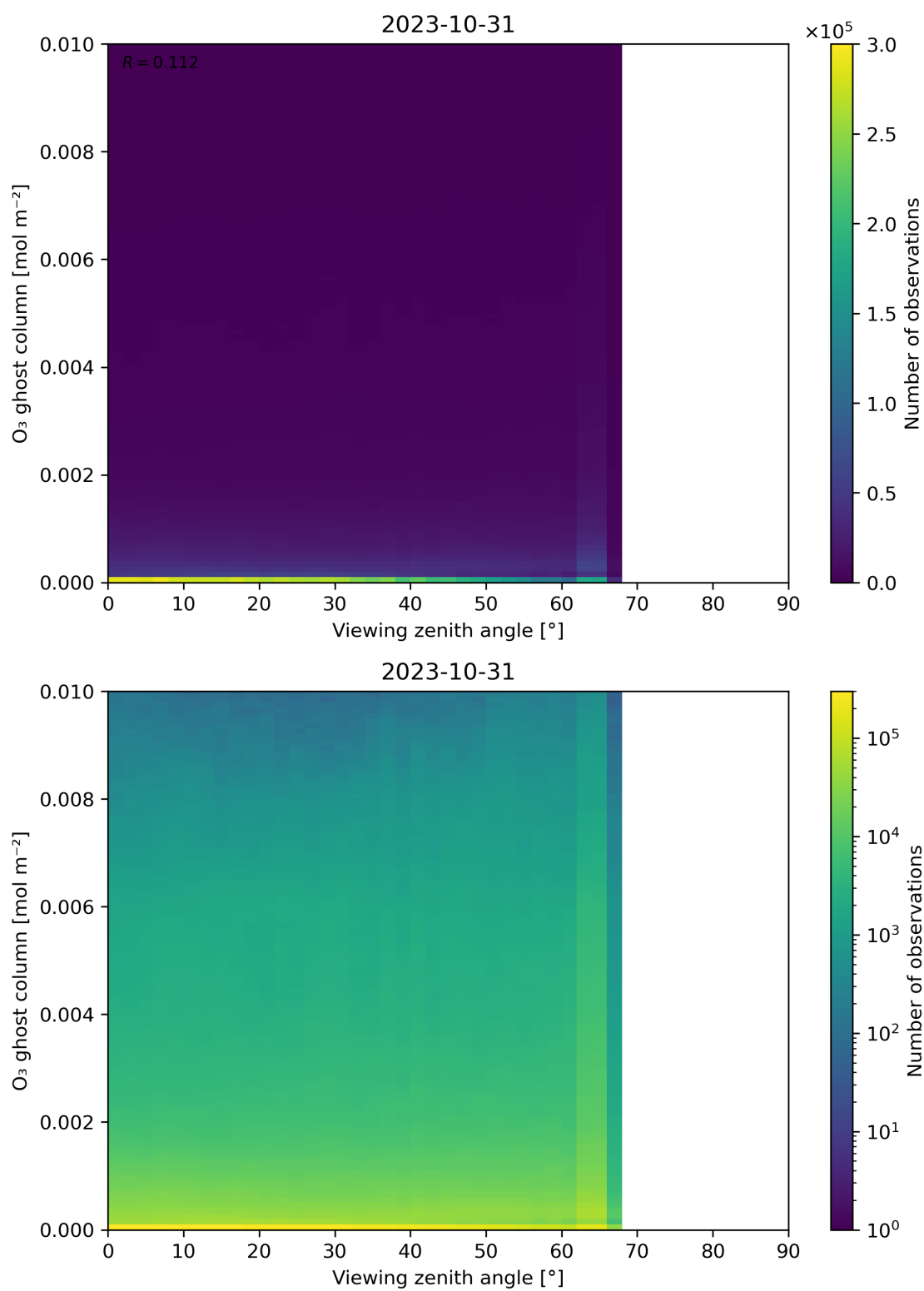
Figure 51: Scatter density plot of “Viewing zenith angle” against “O 3 ghost column” for 2023-10-30 to 2023-11-01.
