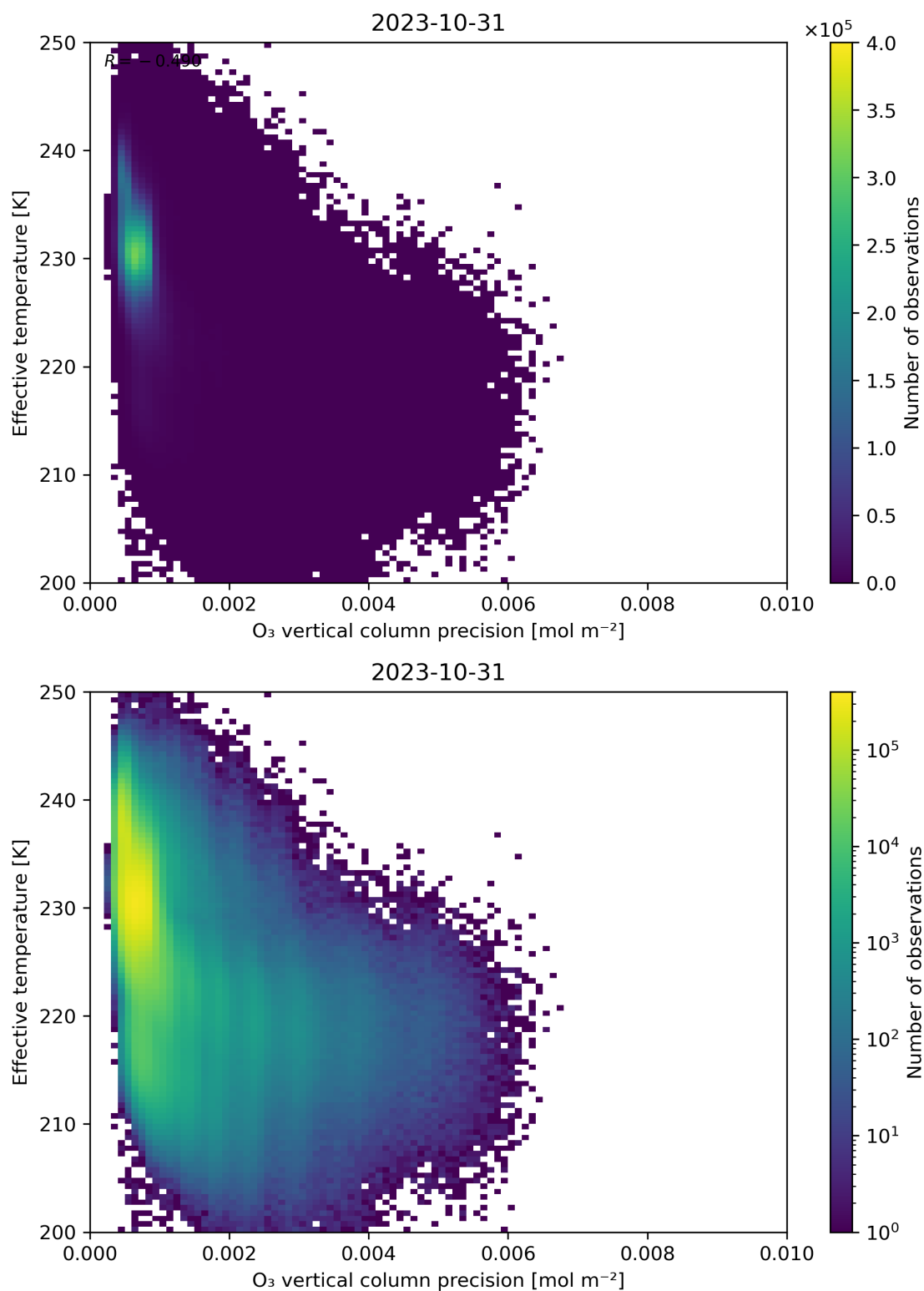
Figure 42: Scatter density plot of “O 3 vertical column precision” against “Effective temperature” for 2023-10-30 to 2023-11-01.
