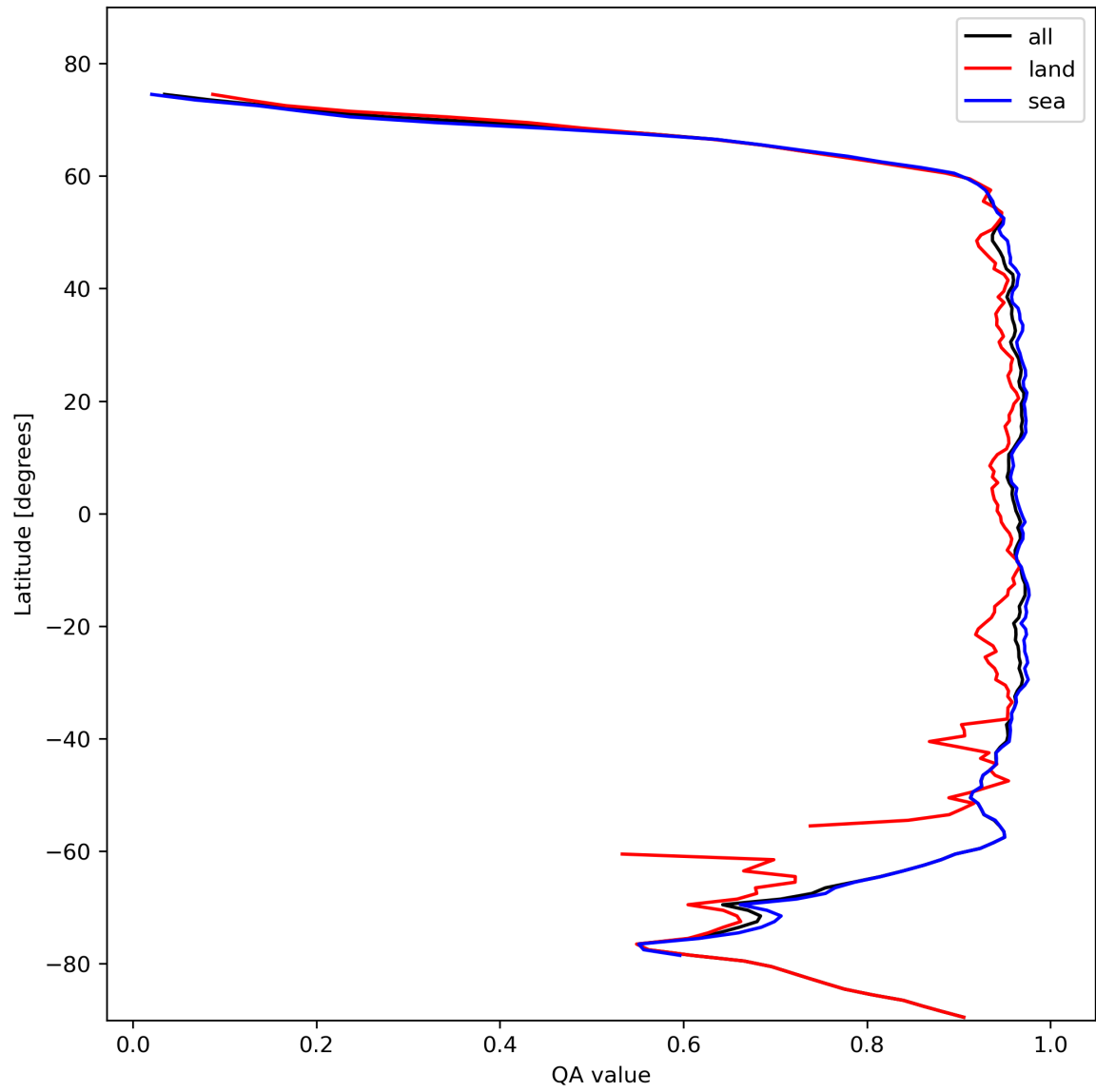
Figure 13: Zonal average of “QA value” for 2023-10-31 to 2023-11-02.
