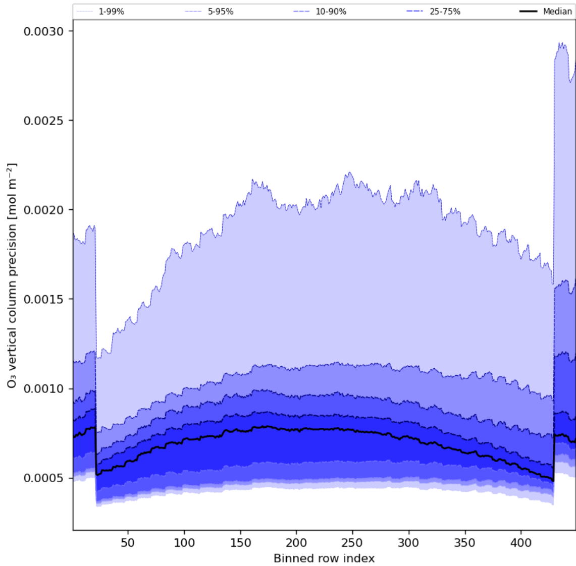
Figure 29: Along track statistics of “O 3 vertical column precision” for 2023-10-31 to 2023-11-02
