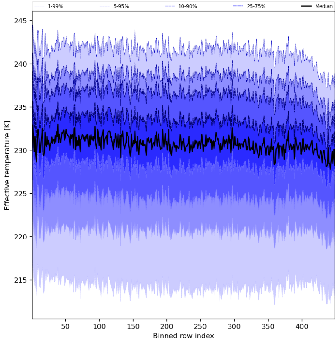
Figure 31: Along track statistics of “Effective temperature” for 2023-10-31 to 2023-11-02
