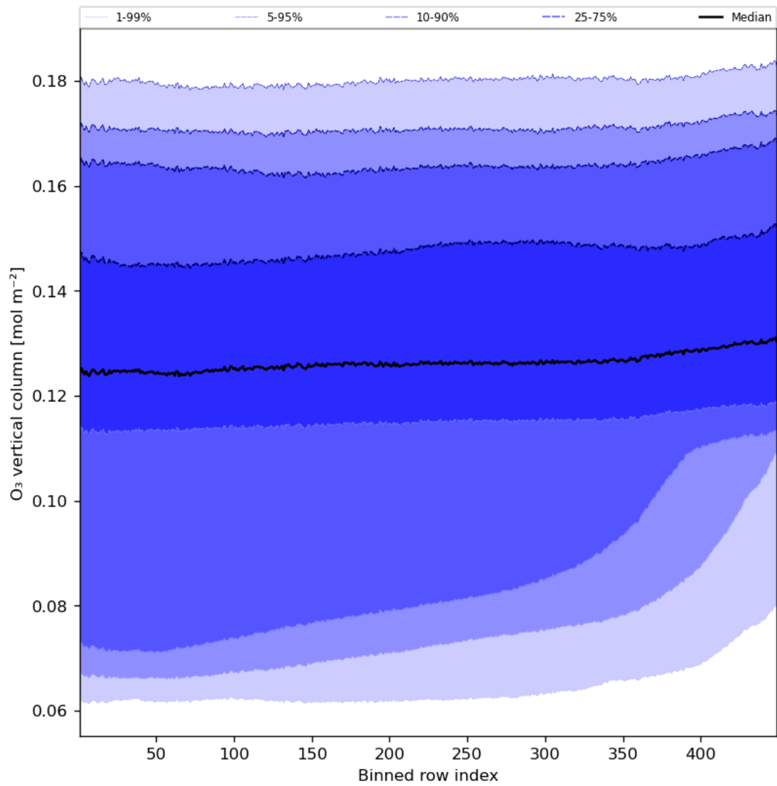
Figure 28: Along track statistics of “O 3 vertical column” for 2023-10-31 to 2023-11-02
