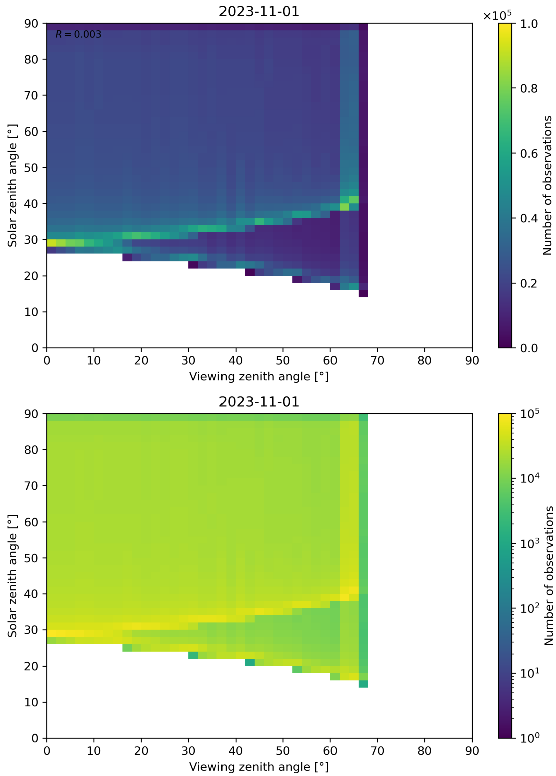
Figure 54: Scatter density plot of “Viewing zenith angle” against “Solar zenith angle” for 2023-10-31 to 2023-11-02.
