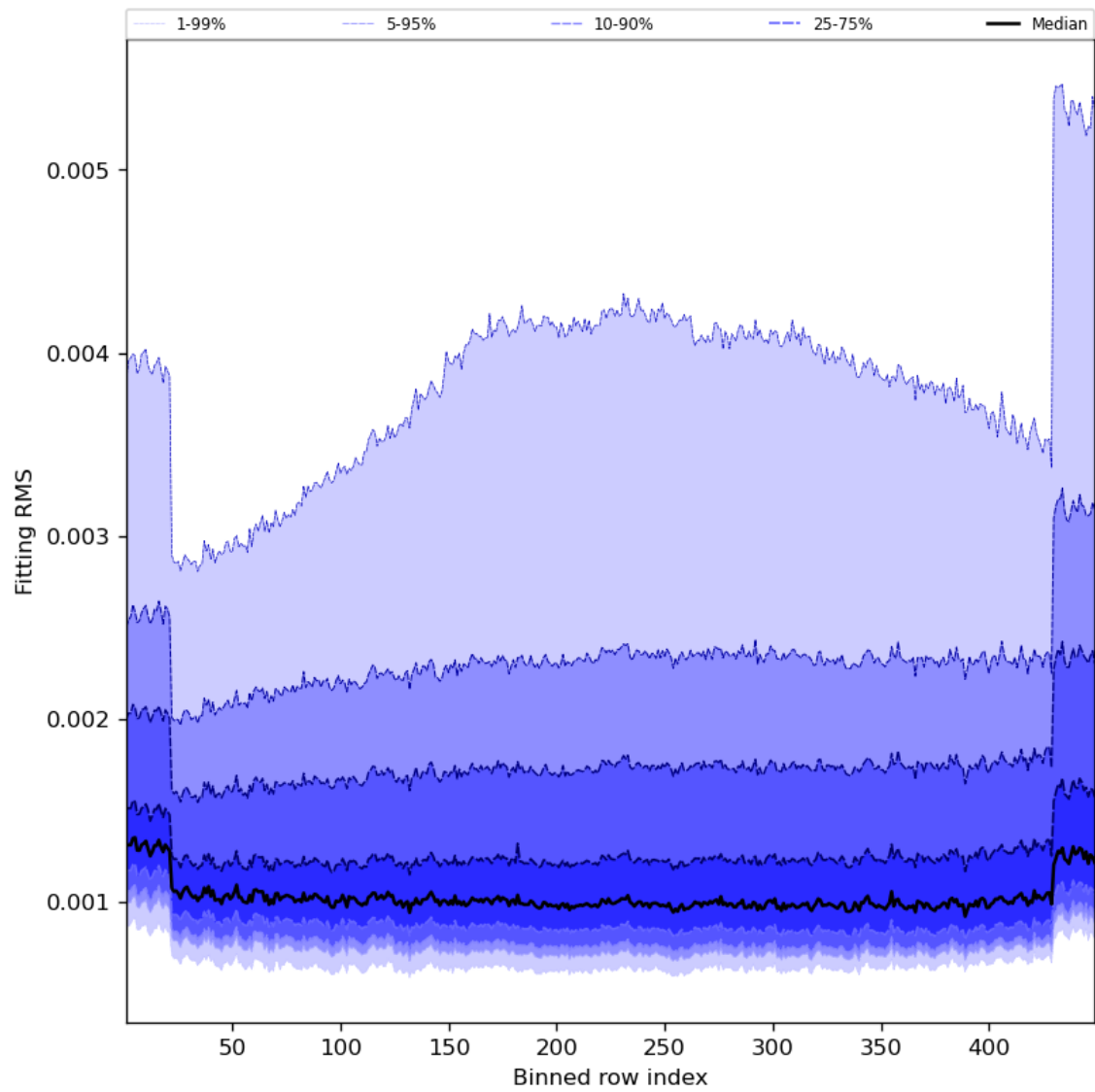
Figure 30: Along track statistics of “Fitting RMS” for 2023-10-31 to 2023-11-02
