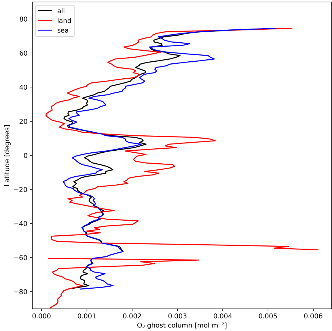
Figure 18: Zonal average of “O 3 ghost column” for 2023-10-31 to 2023-11-02.
