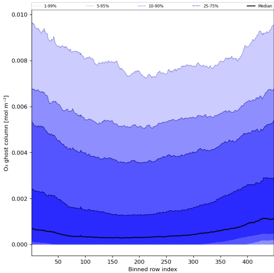
Figure 32: Along track statistics of “O 3 ghost column” for 2023-10-31 to 2023-11-02
