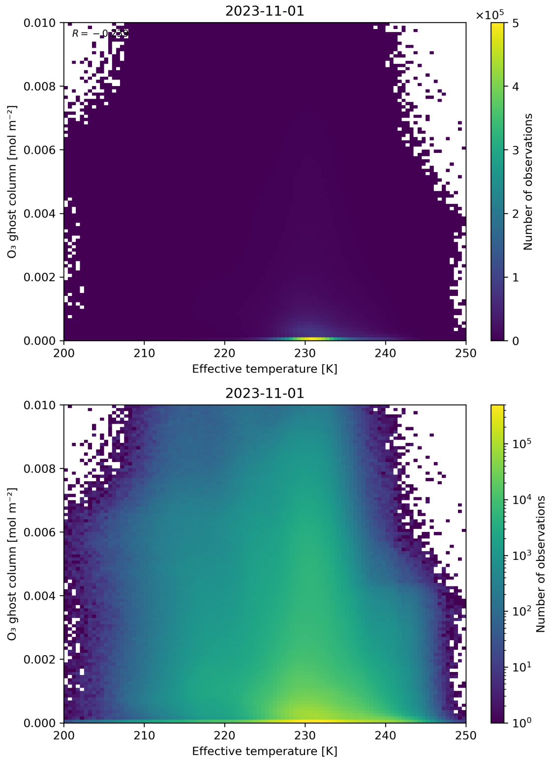
Figure 38: Scatter density plot of “Effective temperature” against “O 3 ghost column” for 2023-10-31 to 2023-11-02.
