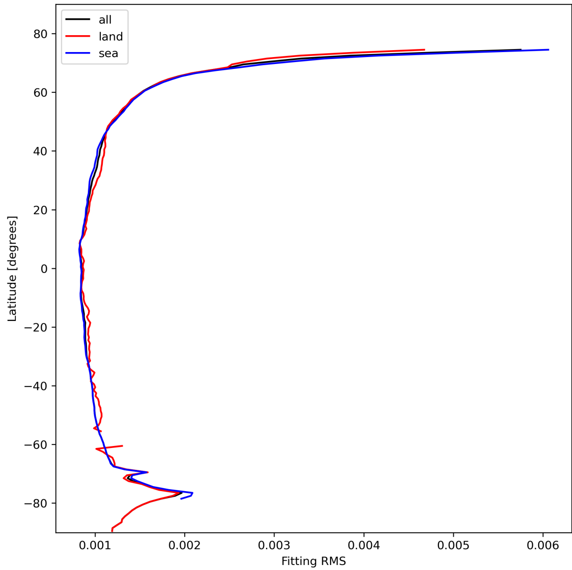
Figure 16: Zonal average of “Fitting RMS” for 2023-10-31 to 2023-11-02.
