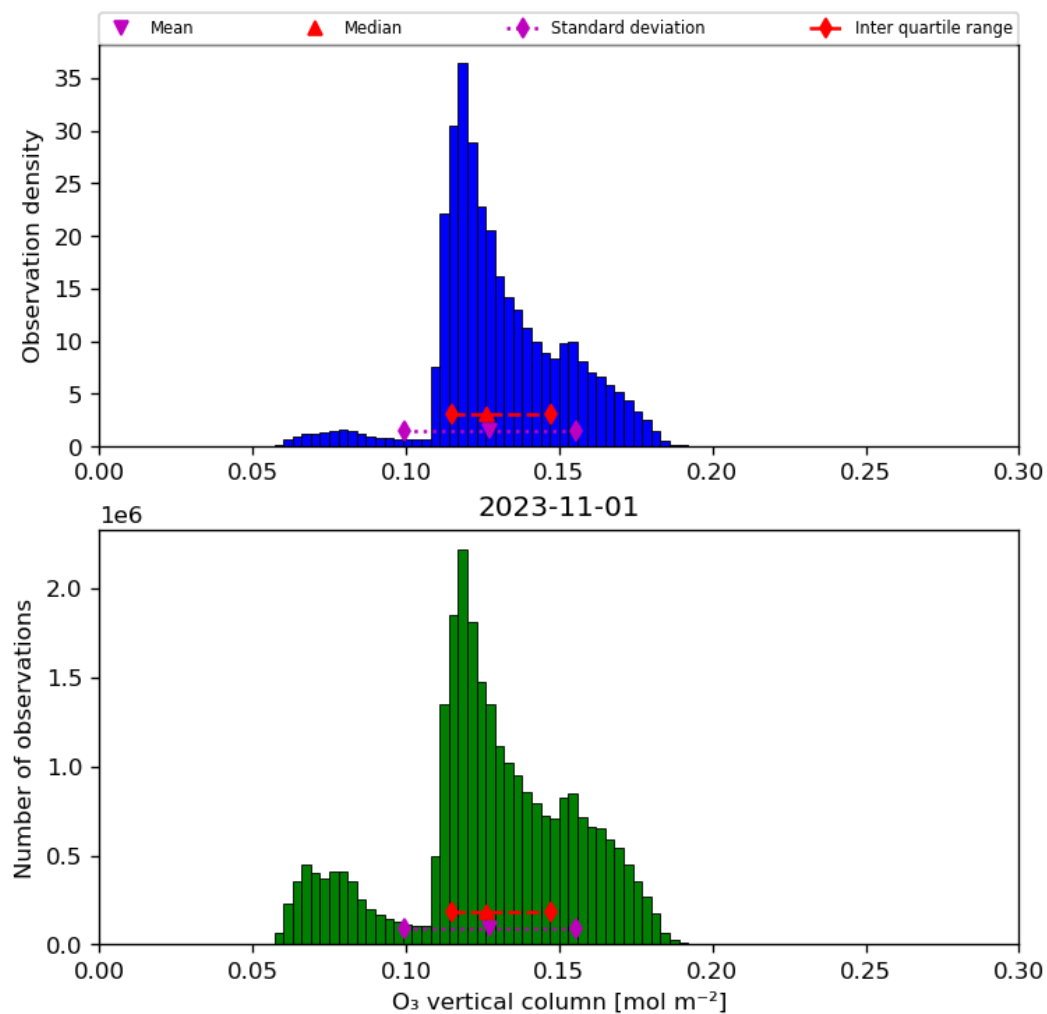
Figure 21: Histogram of “O 3 vertical column” for 2023-10-31 to 2023-11-02
