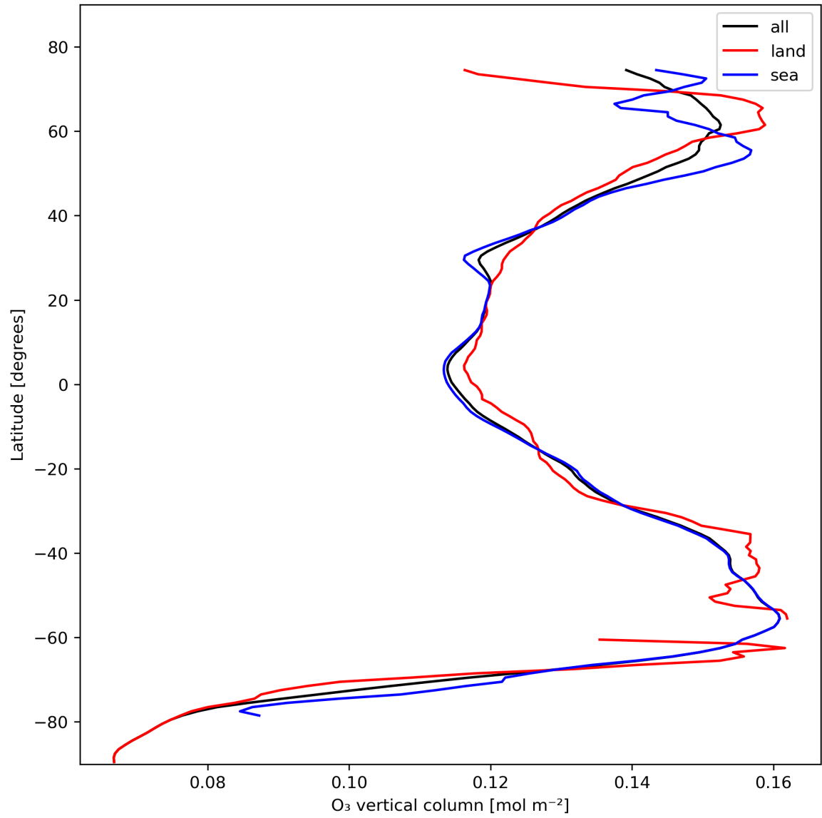
Figure 14: Zonal average of “O 3 vertical column” for 2023-10-31 to 2023-11-02.
