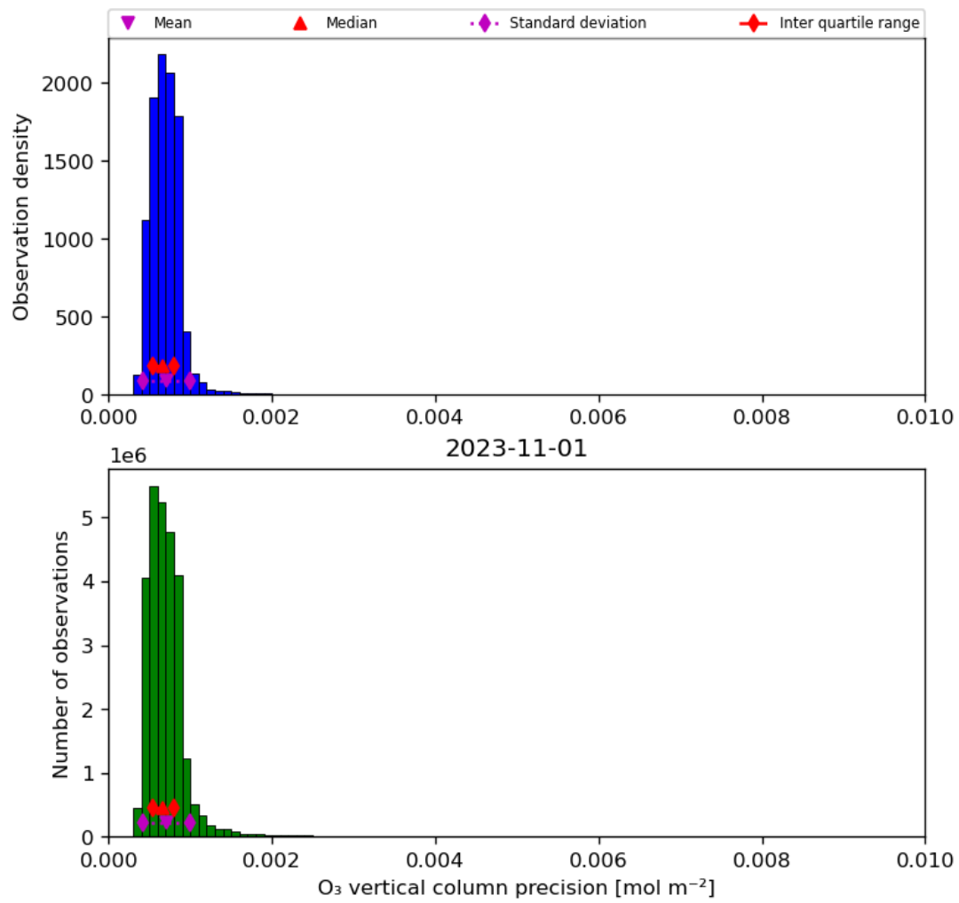
Figure 22: Histogram of “O 3 vertical column precision” for 2023-10-31 to 2023-11-02
