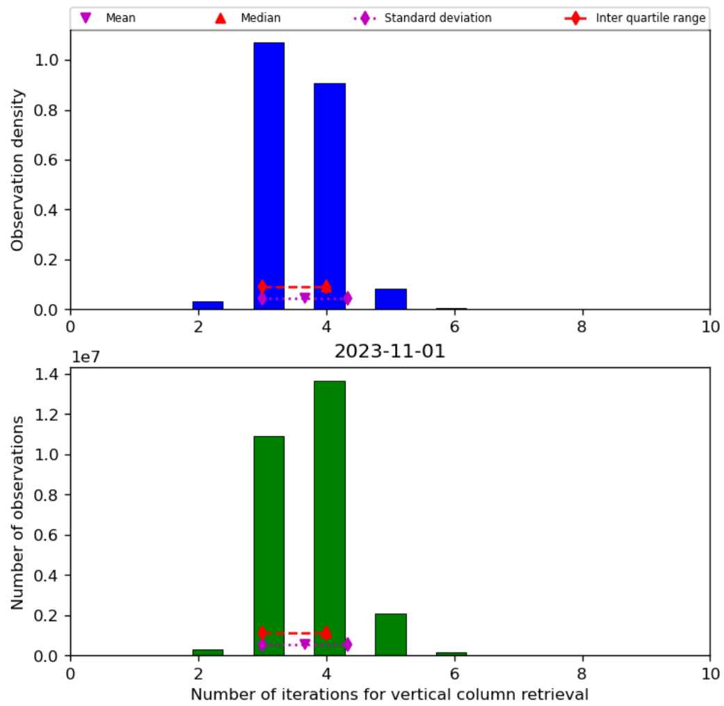
Figure 26: Histogram of “Number of iterations for vertical column retrieval” for 2023-10-31 to 2023-11-02
