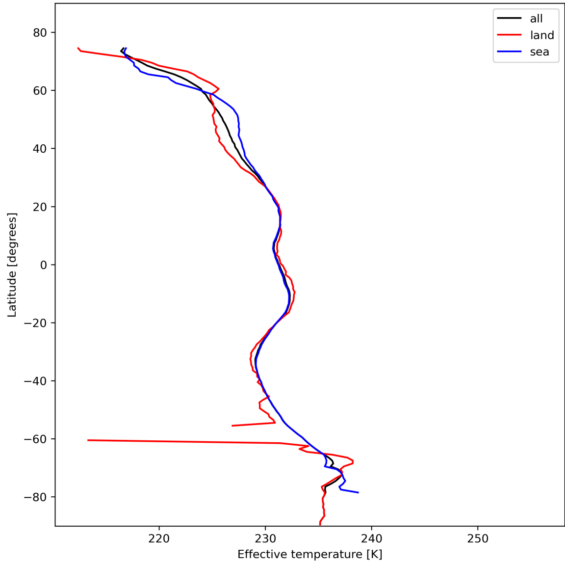
Figure 17: Zonal average of "Effective temperature" for 2023-10-31 to 2023-11-02.
