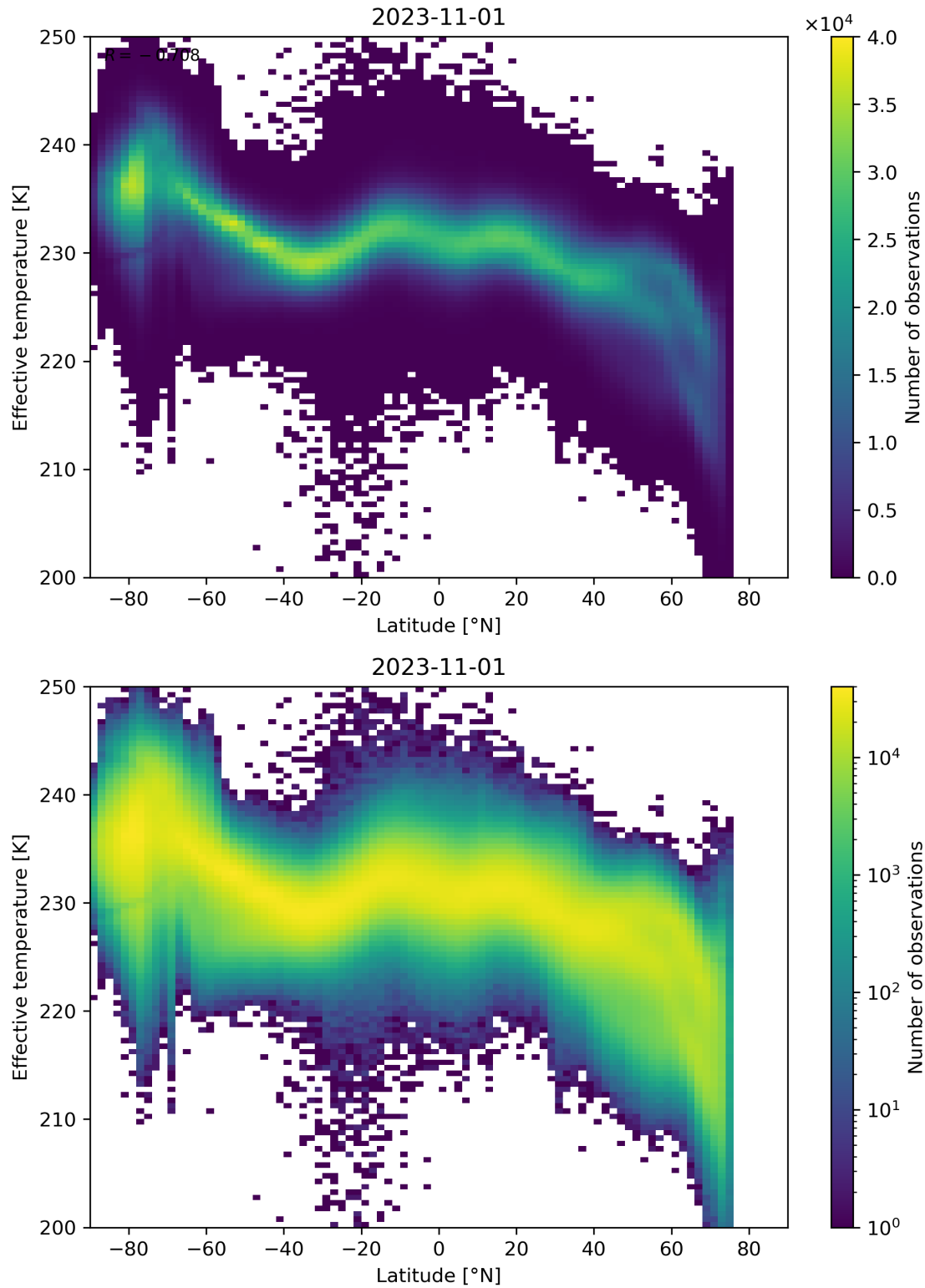
Figure 34: Scatter density plot of “Latitude” against “Effective temperature” for 2023-10-31 to 2023-11-02.
