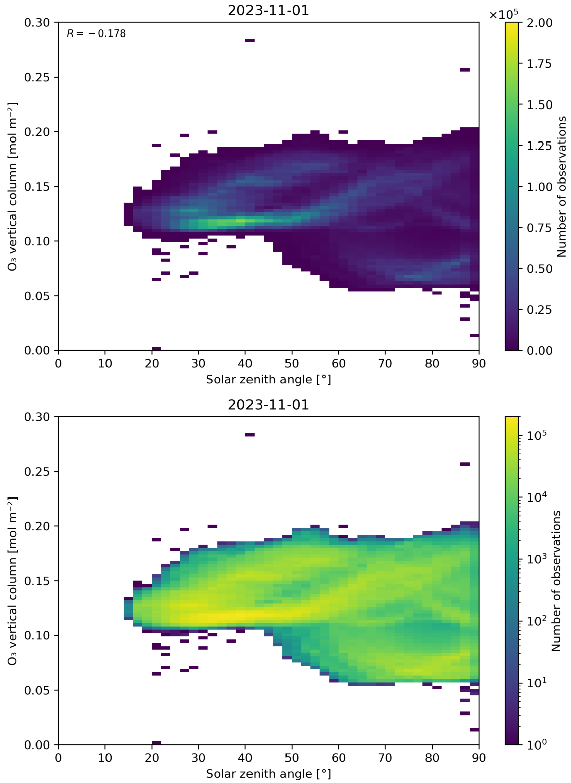
Figure 47: Scatter density plot of “Solar zenith angle” against “O 3 vertical column” for 2023-10-31 to 2023-11-02.
