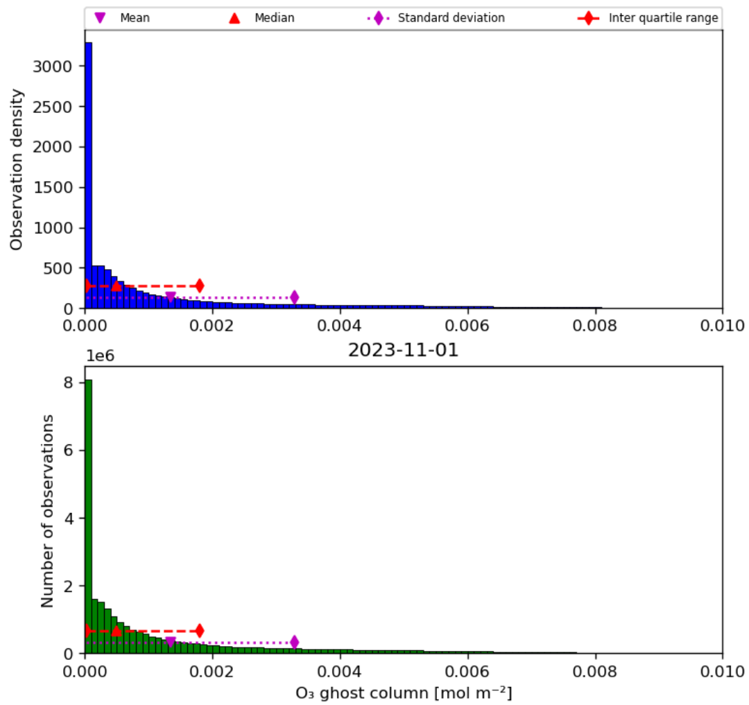
Figure 25: Histogram of “O 3 ghost column” for 2023-10-31 to 2023-11-02
