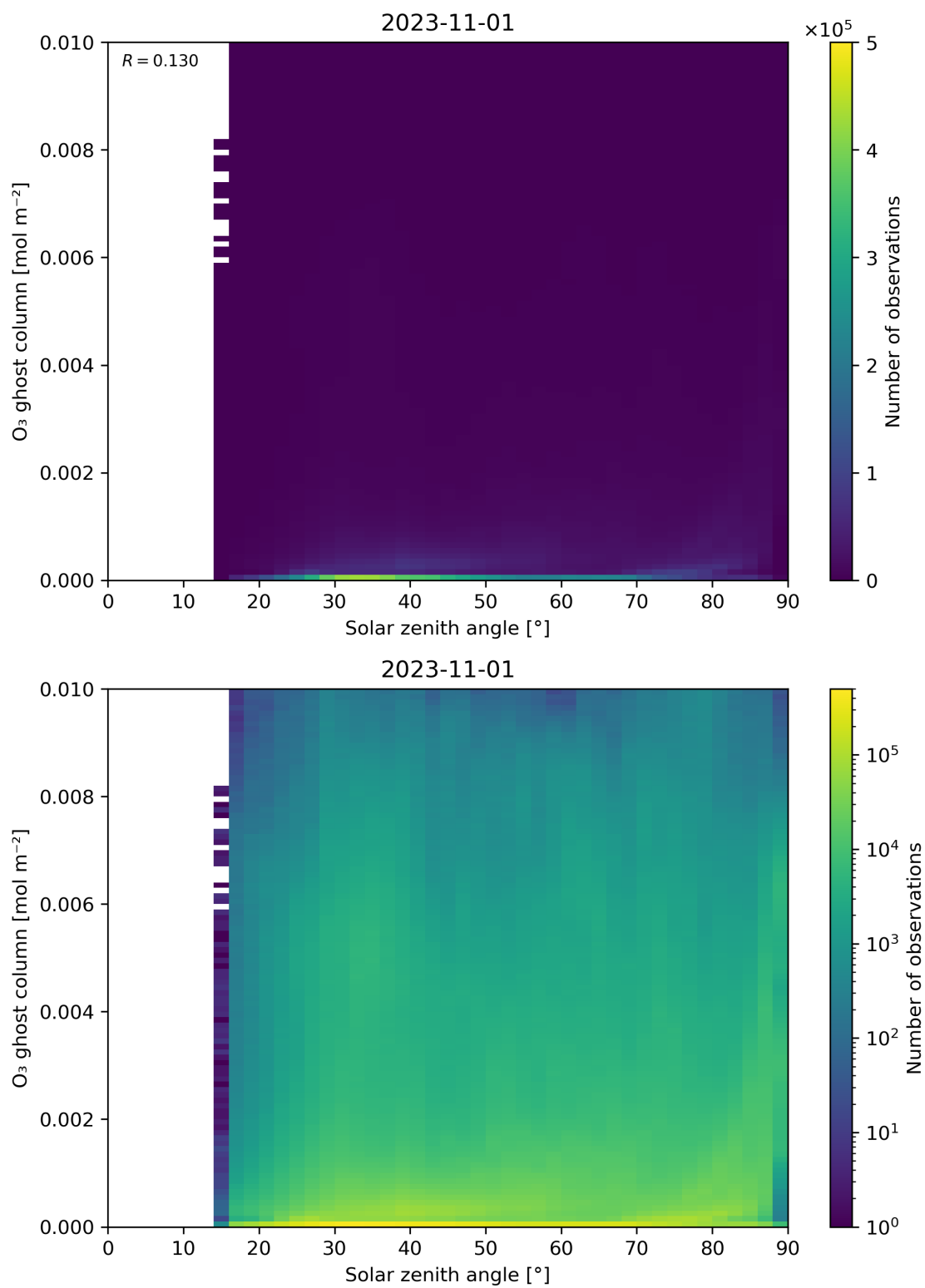
Figure 46: Scatter density plot of “Solar zenith angle” against “O 3 ghost column” for 2023-10-31 to 2023-11-02.
