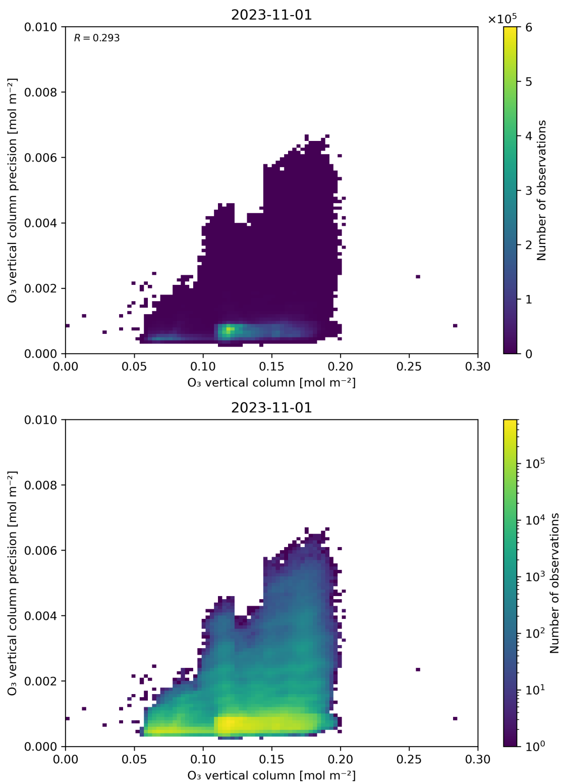
Figure 41: Scatter density plot of “O 3 vertical column” against “O 3 vertical column precision” for 2023-10-31 to 2023-11-02.
