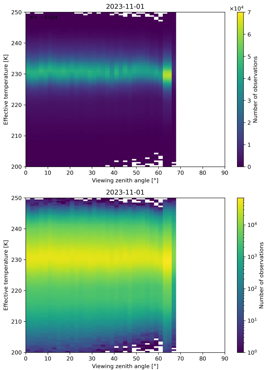
Figure 50: Scatter density plot of “Viewing zenith angle” against “Effective temperature” for 2023-10-31 to 2023-11-02.
