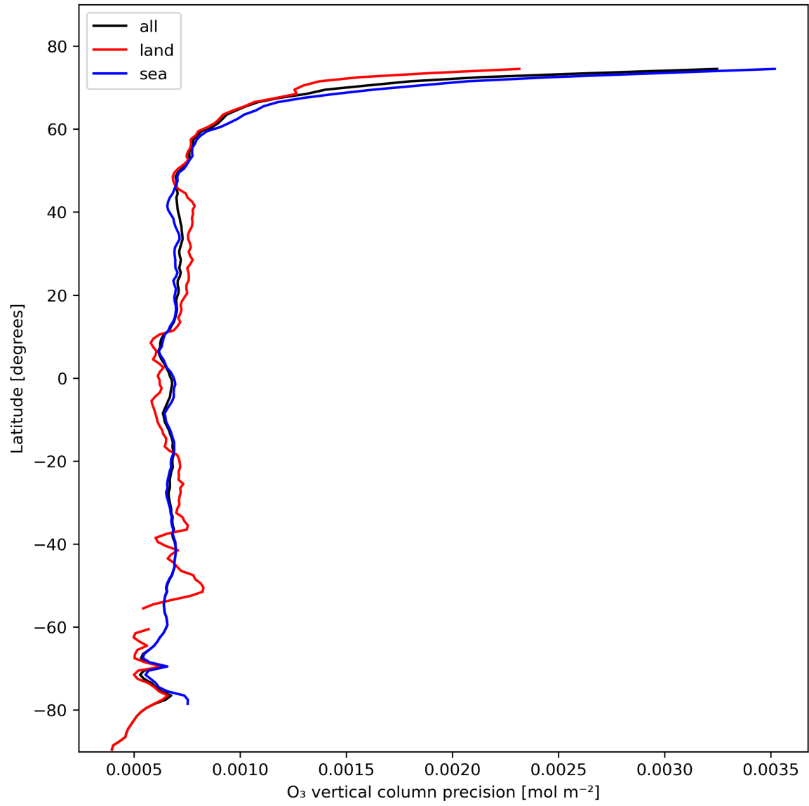
Figure 15: Zonal average of “O 3 vertical column precision” for 2023-10-31 to 2023-11-02.
