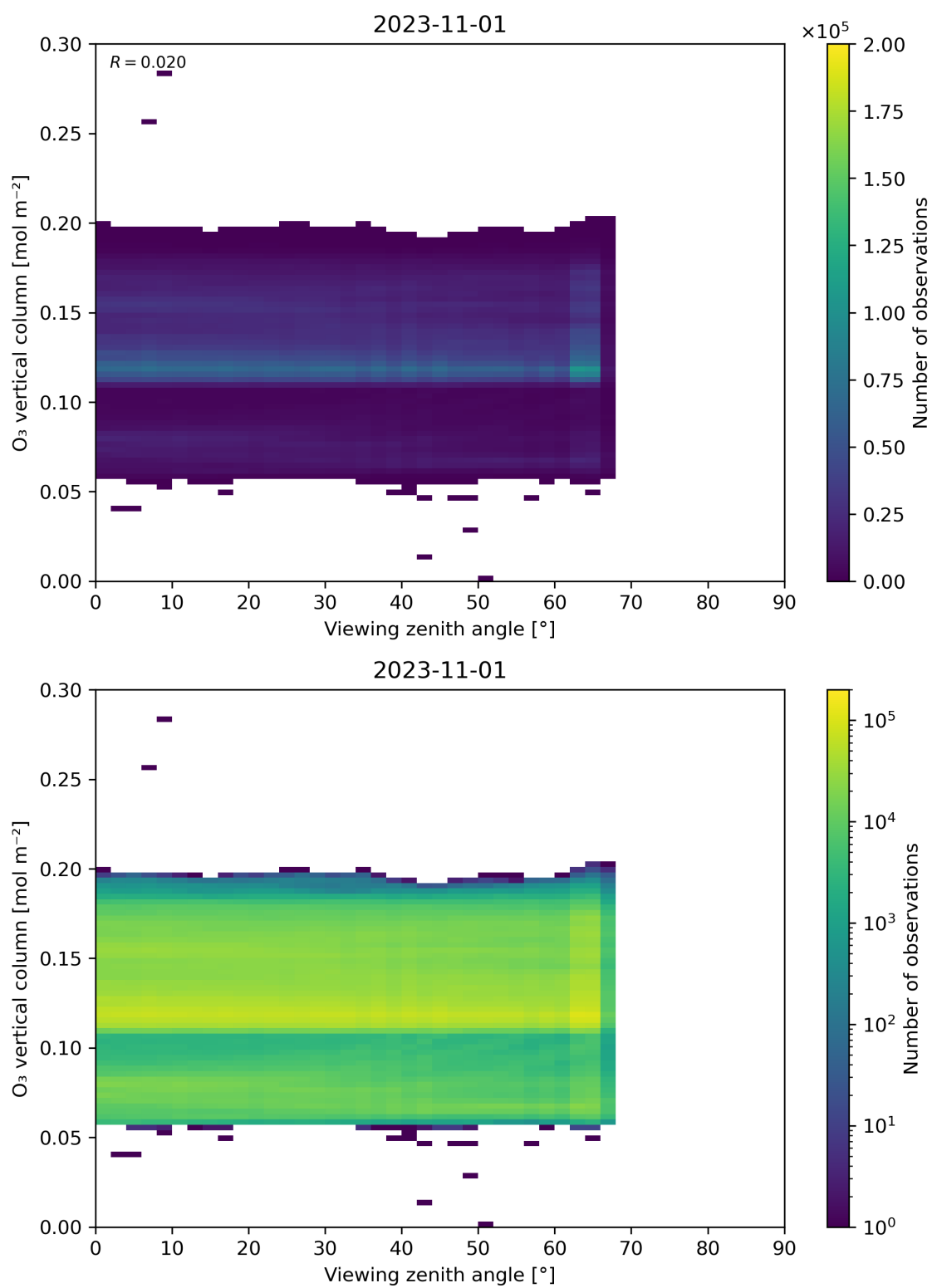
Figure 52: Scatter density plot of “Viewing zenith angle” against “O 3 vertical column” for 2023-10-31 to 2023-11-02.
