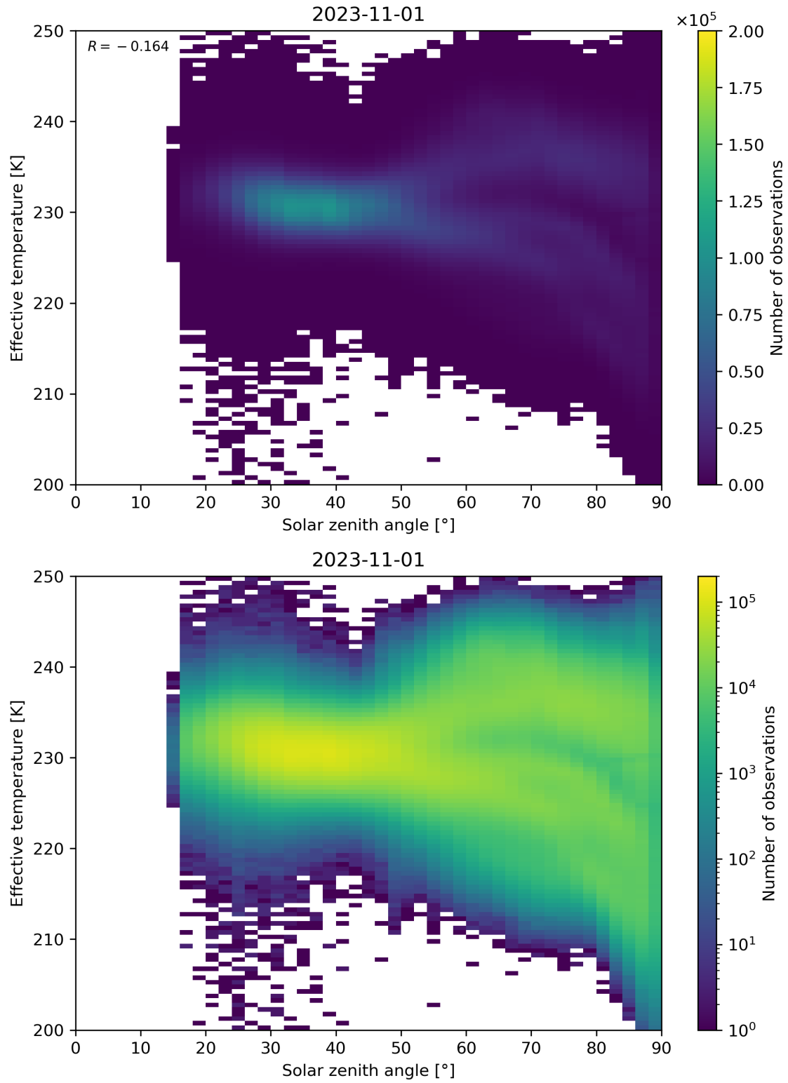
Figure 45: Scatter density plot of “Solar zenith angle” against “Effective temperature” for 2023-10-31 to 2023-11-02.
