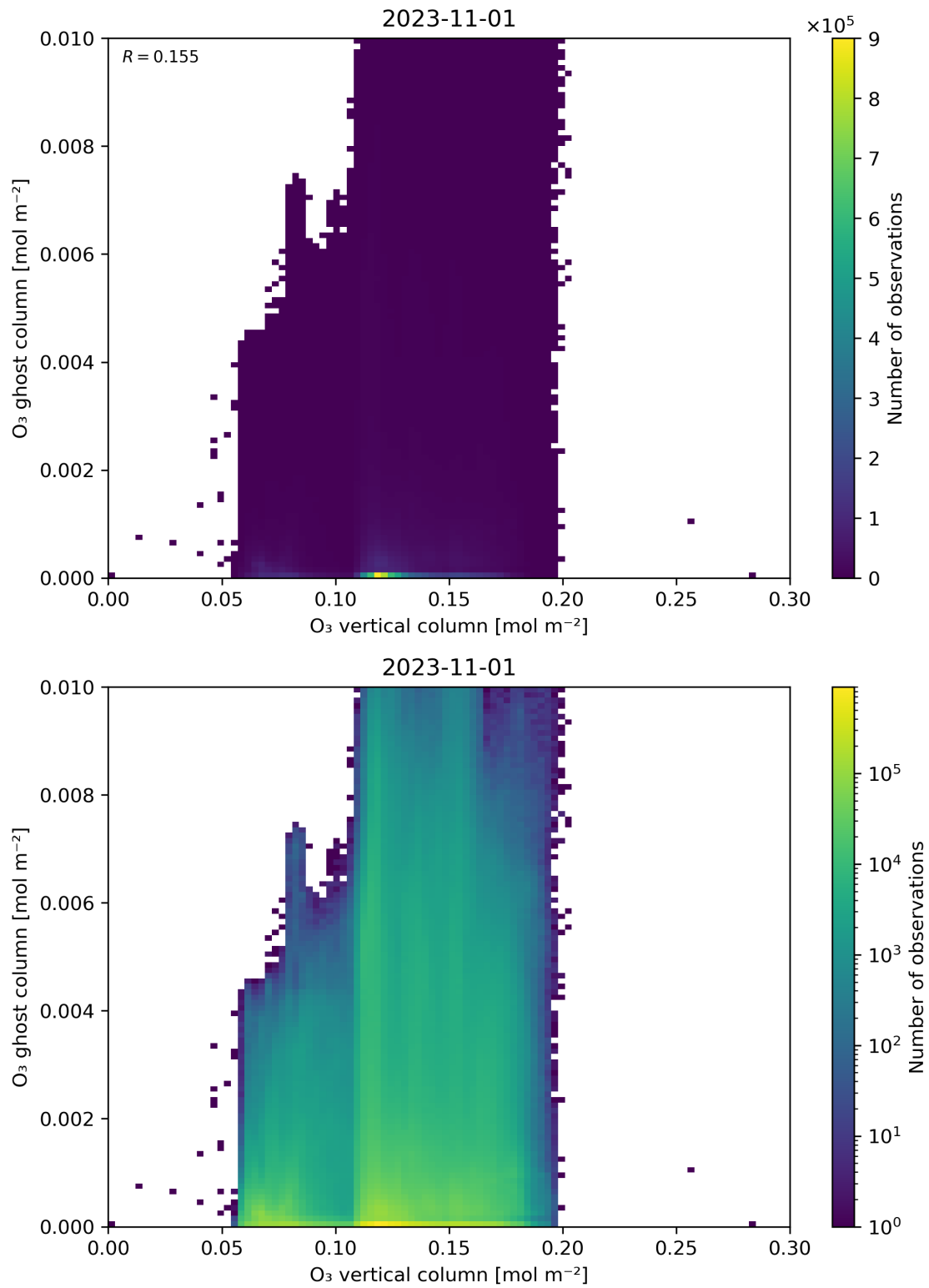
Figure 40: Scatter density plot of “O 3 vertical column” against “O 3 ghost column” for 2023-10-31 to 2023-11-02.
