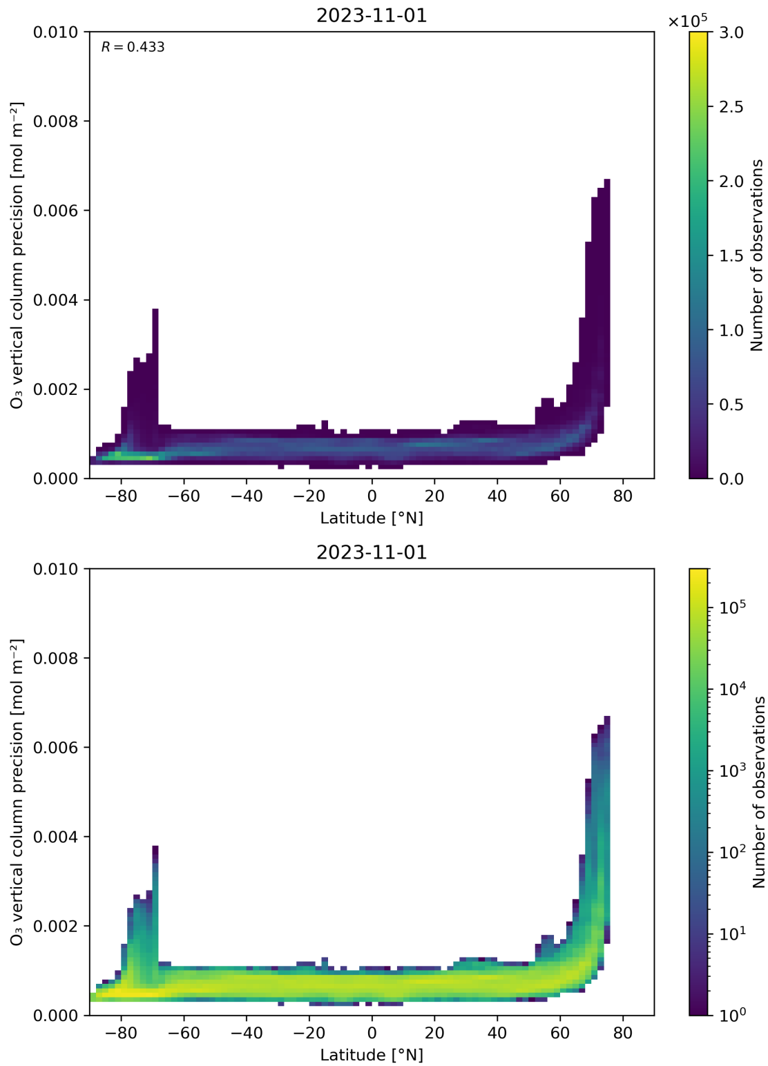
Figure 37: Scatter density plot of “Latitude” against “O 3 vertical column precision” for 2023-10-31 to 2023-11-02.
