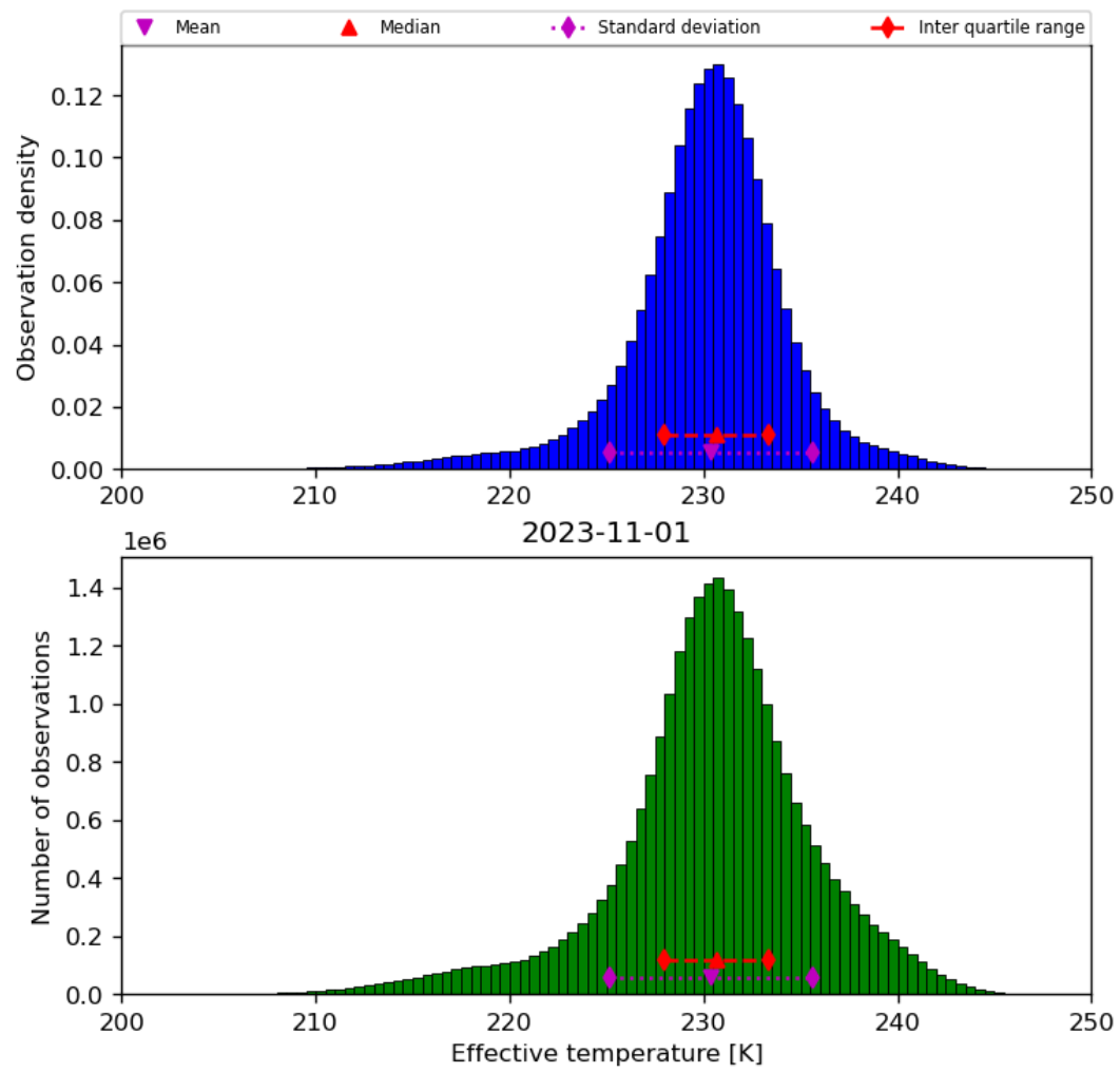
Figure 24: Histogram of “Effective temperature” for 2023-10-31 to 2023-11-02
