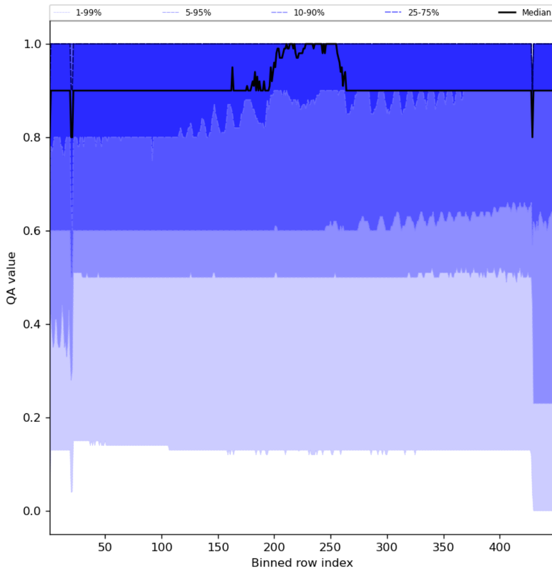
Figure 27: Along track statistics of “QA value” for 2023-10-31 to 2023-11-02
