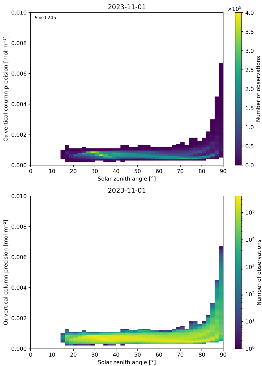
Figure 48: Scatter density plot of “Solar zenith angle” against “O 3 vertical column precision” for 2023-10-31 to 2023-11-02.
