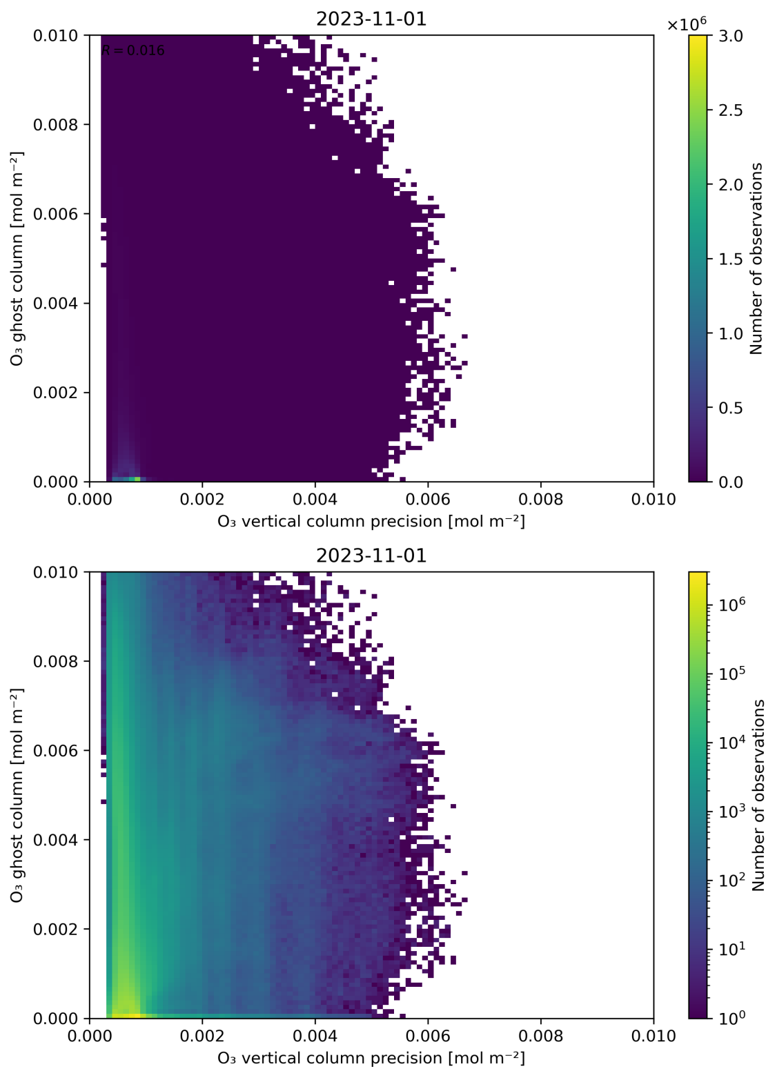
Figure 43: Scatter density plot of “O 3 vertical column precision” against “O 3 ghost column” for 2023-10-31 to 2023-11-02.
