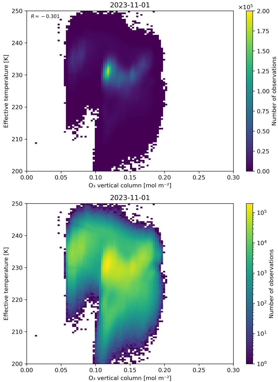
Figure 39: Scatter density plot of “O 3 vertical column” against “Effective temperature” for 2023-10-31 to 2023-11-02.
