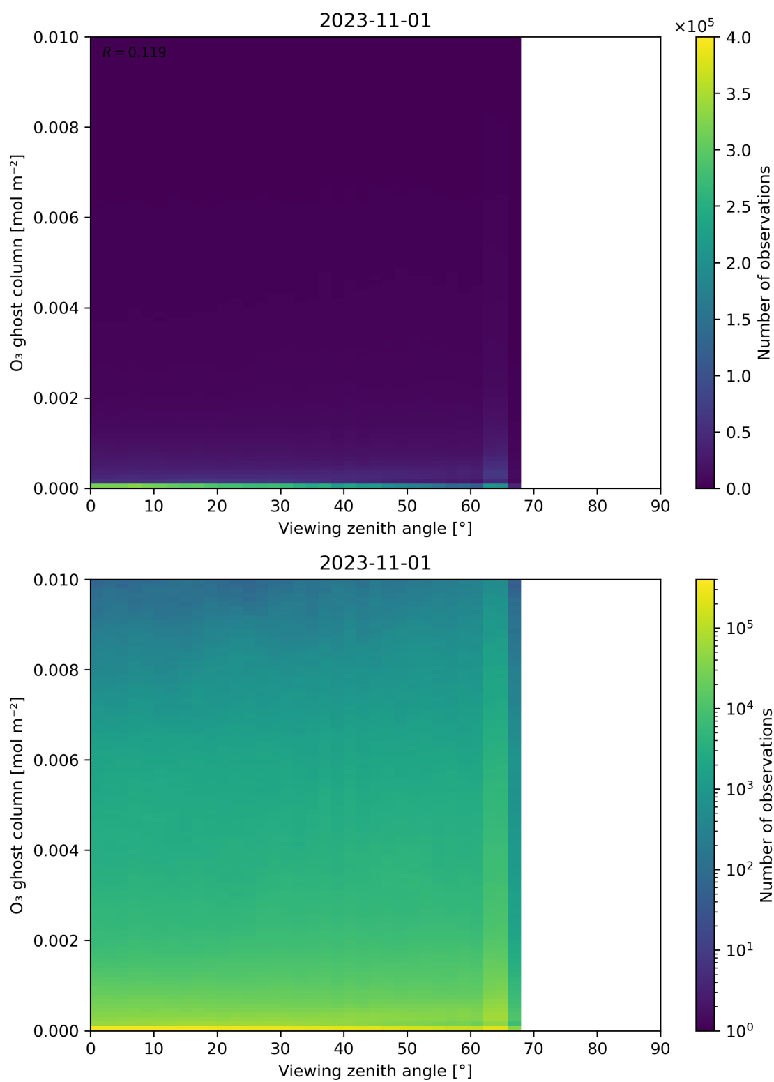
Figure 51: Scatter density plot of “Viewing zenith angle” against “O 3 ghost column” for 2023-10-31 to 2023-11-02.
