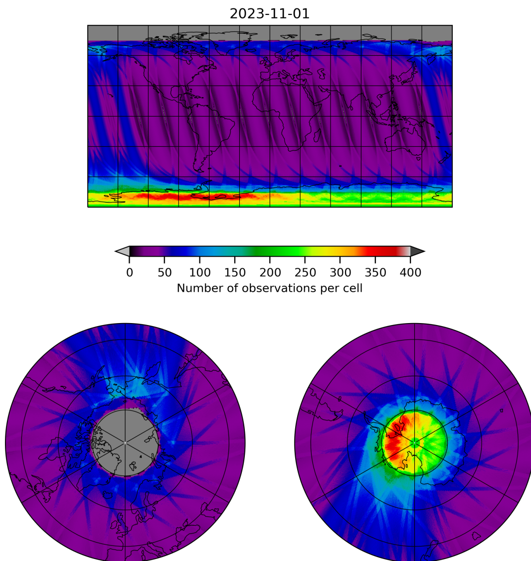
Figure 12: Map of the number of observations for 2023-10-31 to 2023-11-02
