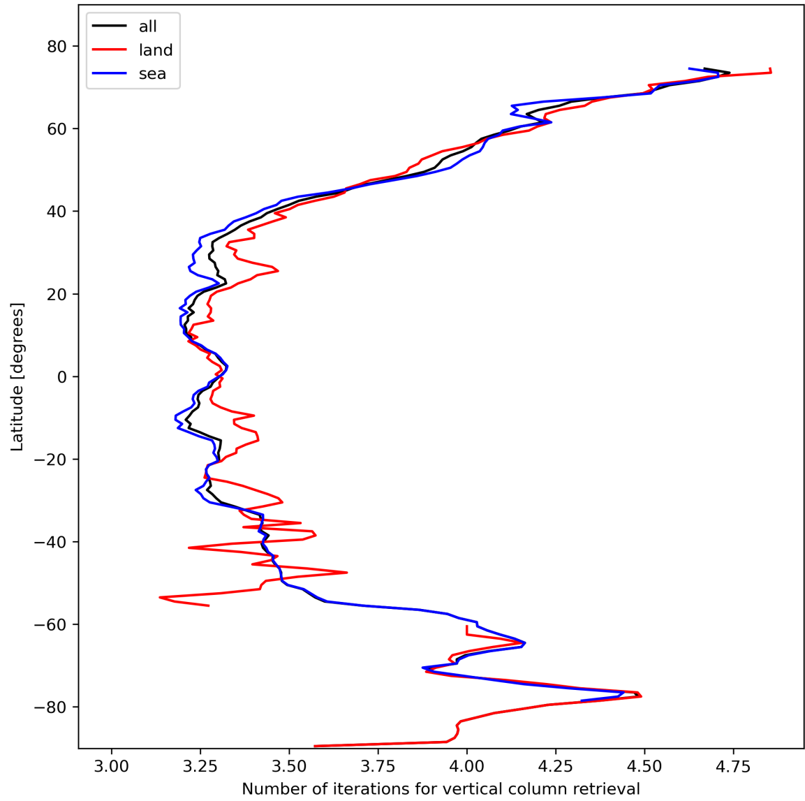
Figure 19: Zonal average of “Number of iterations for vertical column retrieval” for 2023-10-31 to 2023-11-02.
