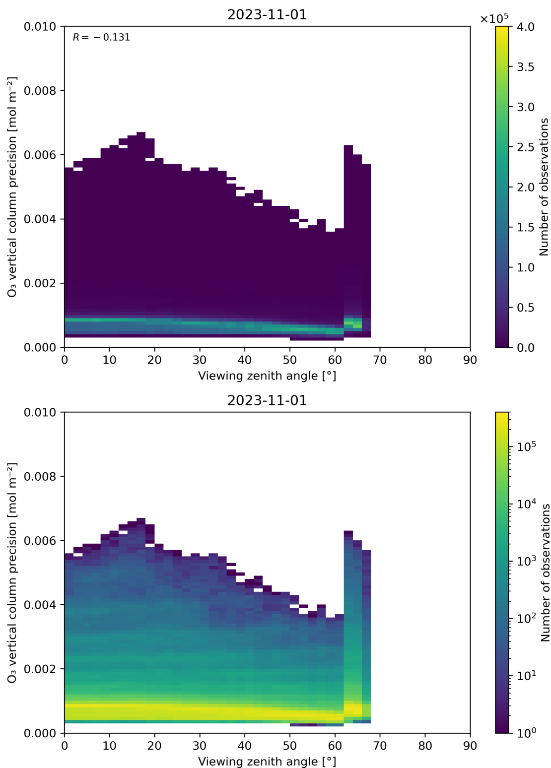
Figure 53: Scatter density plot of “Viewing zenith angle” against “O 3 vertical column precision” for 2023-10-31 to 2023-11-02.
