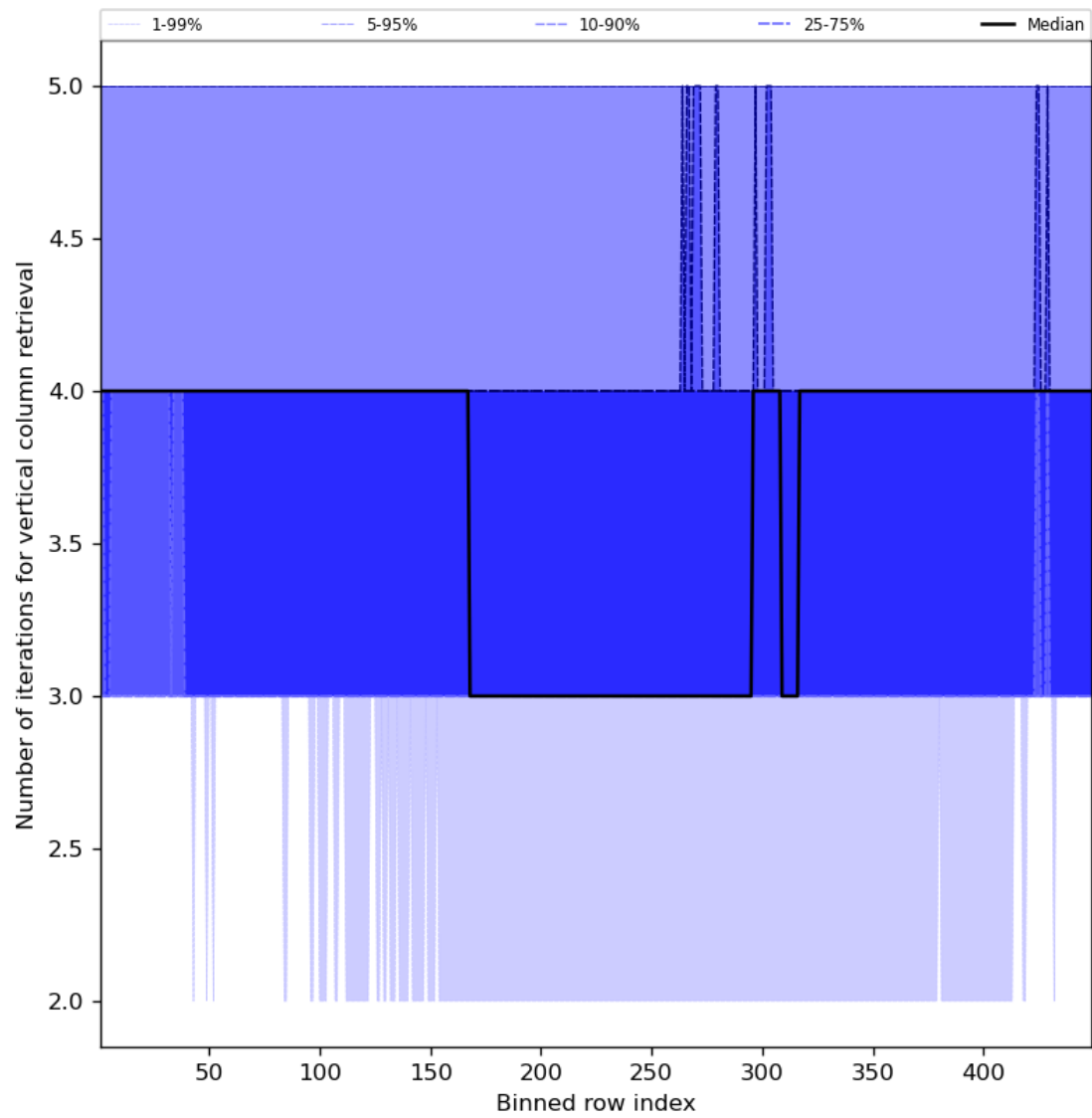
Figure 33: Along track statistics of “Number of iterations for vertical column retrieval” for 2023-10-31 to 2023-11-02
