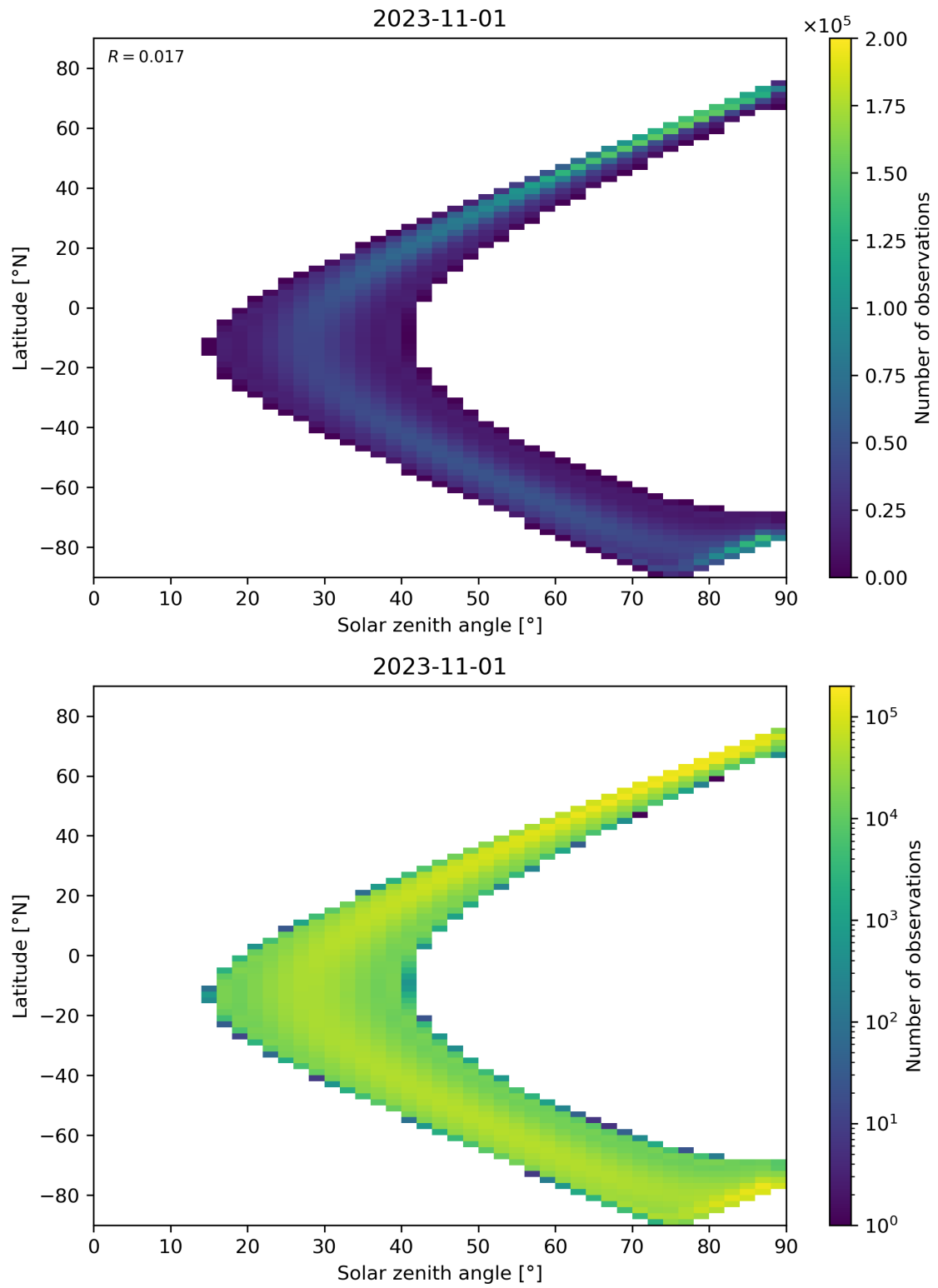
Figure 44: Scatter density plot of “Solar zenith angle” against “Latitude” for 2023-10-31 to 2023-11-02.
