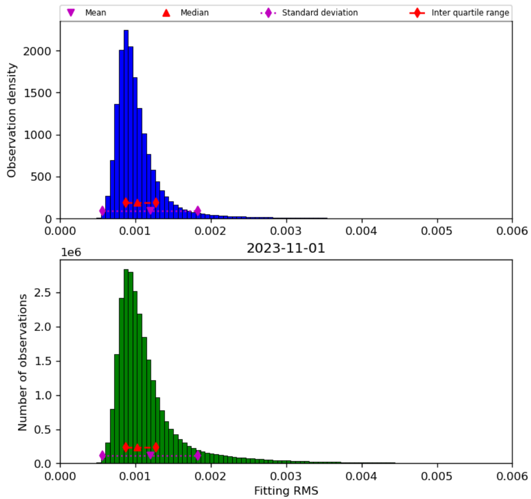
Figure 23: Histogram of “Fitting RMS” for 2023-10-31 to 2023-11-02
