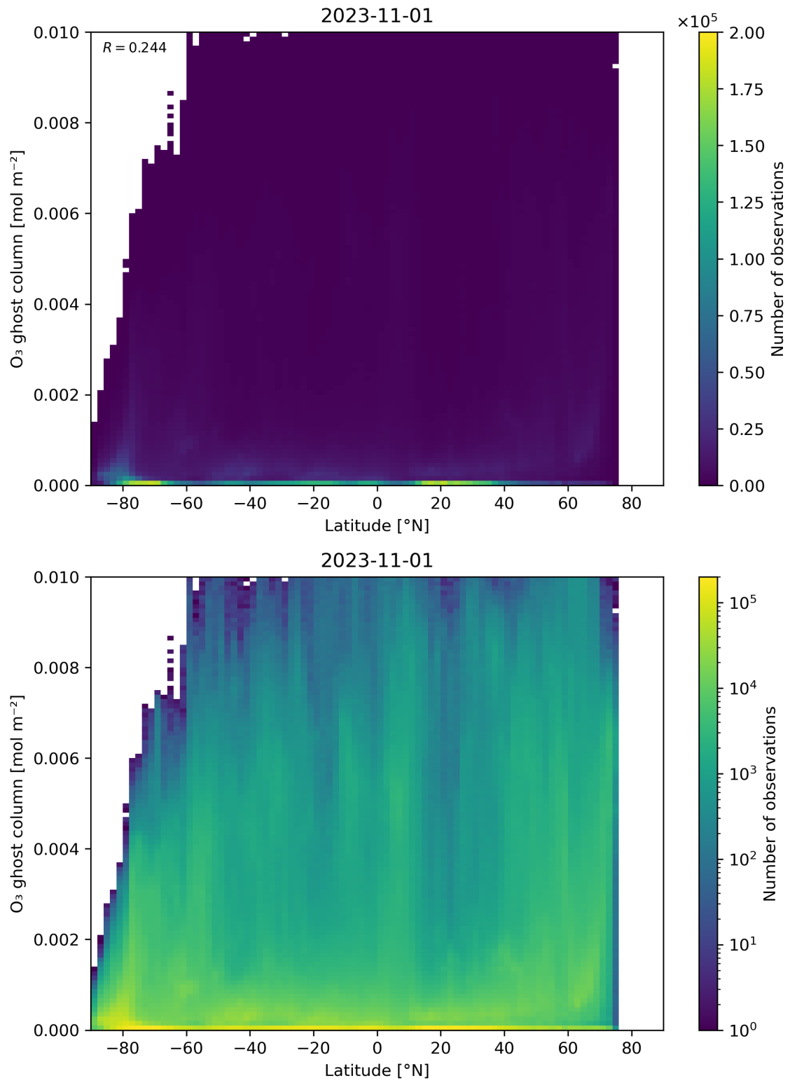
Figure 35: Scatter density plot of “Latitude” against “O 3 ghost column” for 2023-10-31 to 2023-11-02.
