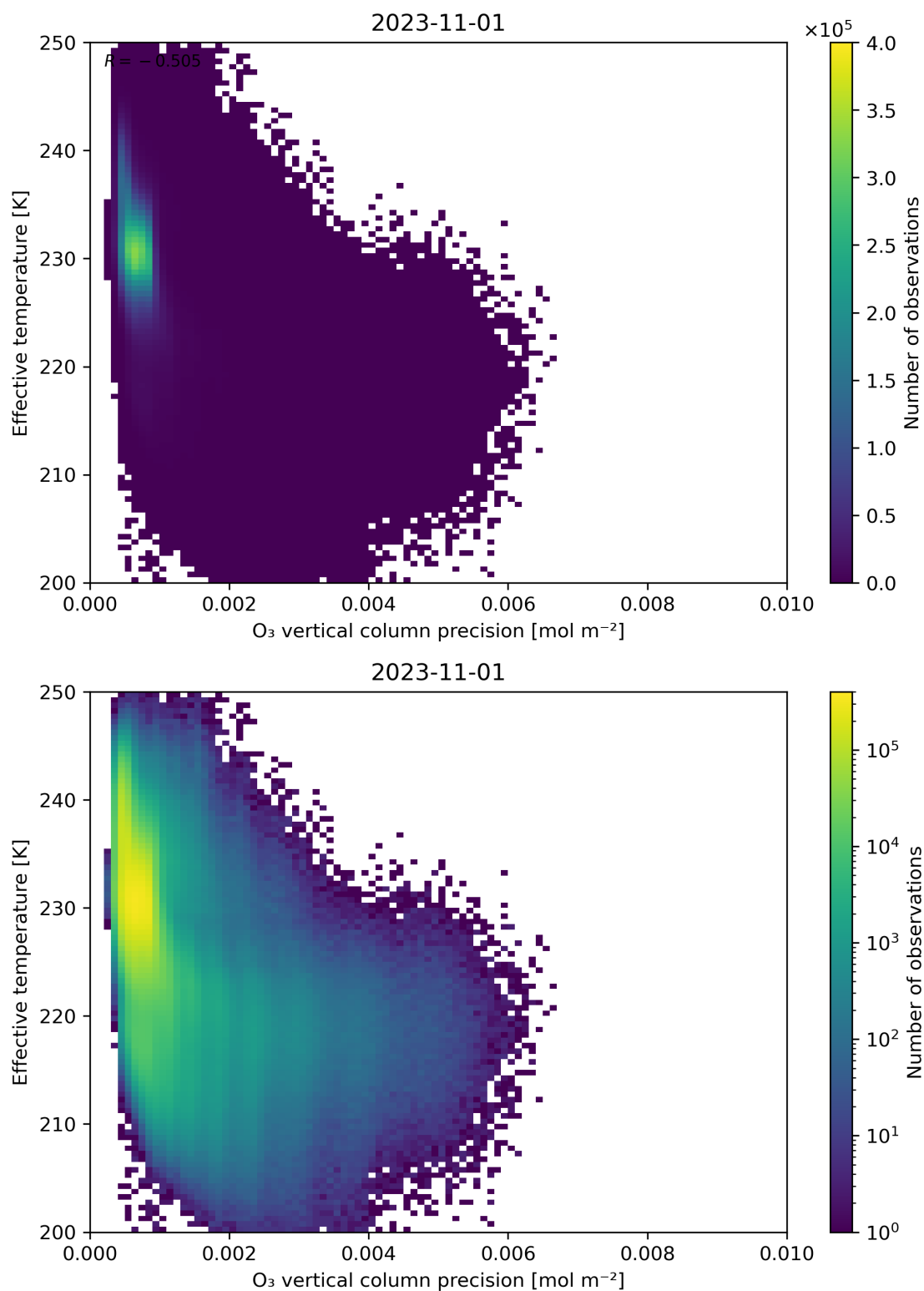
Figure 42: Scatter density plot of “O 3 vertical column precision” against “Effective temperature” for 2023-10-31 to 2023-11-02.
