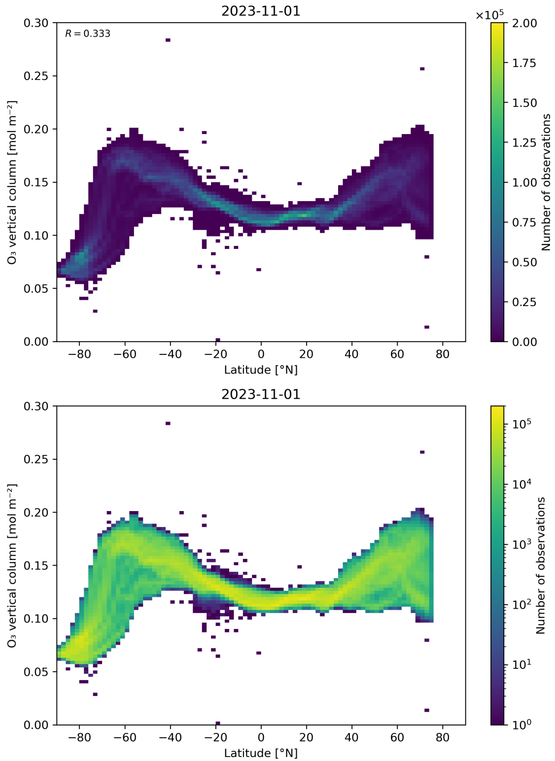
Figure 36: Scatter density plot of “Latitude” against “O 3 vertical column” for 2023-10-31 to 2023-11-02.
