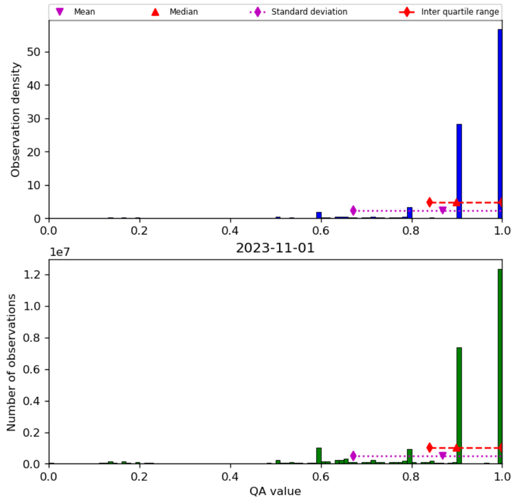
Figure 20: Histogram of “QA value” for 2023-10-31 to 2023-11-02
