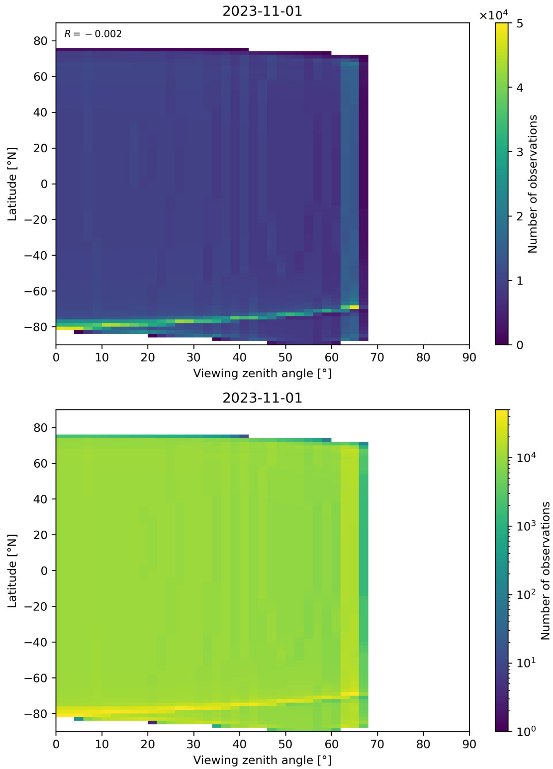
Figure 49: Scatter density plot of “Viewing zenith angle” against “Latitude” for 2023-10-31 to 2023-11-02.
