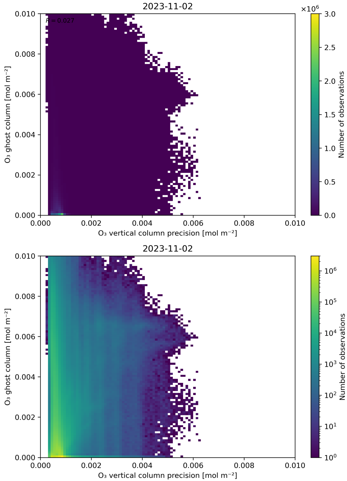
Figure 43: Scatter density plot of “O 3 vertical column precision” against “O 3 ghost column” for 2023-11-02 to 2023-11-03.
