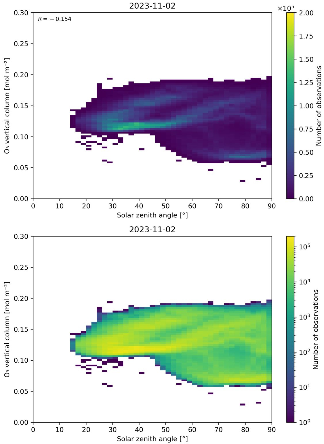
Figure 47: Scatter density plot of “Solar zenith angle” against “O 3 vertical column” for 2023-11-02 to 2023-11-03.
