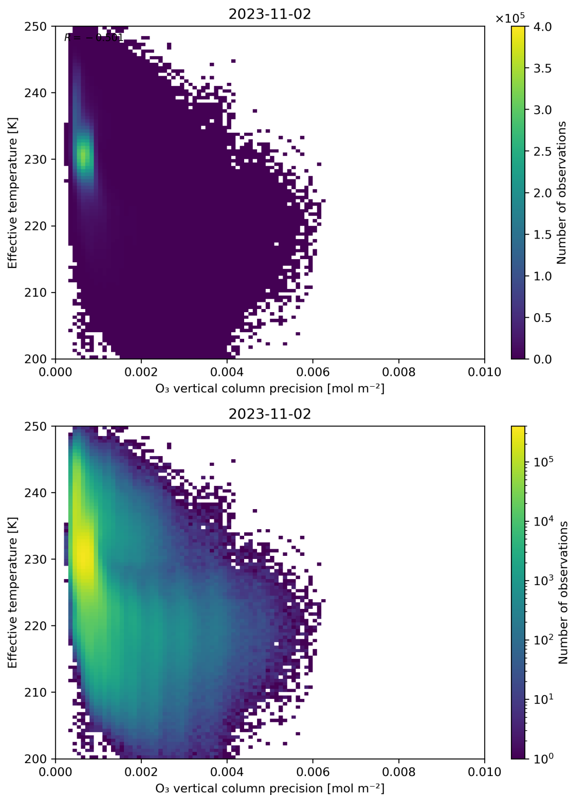
Figure 42: Scatter density plot of “O 3 vertical column precision” against “Effective temperature” for 2023-11-02 to 2023-11-03.
