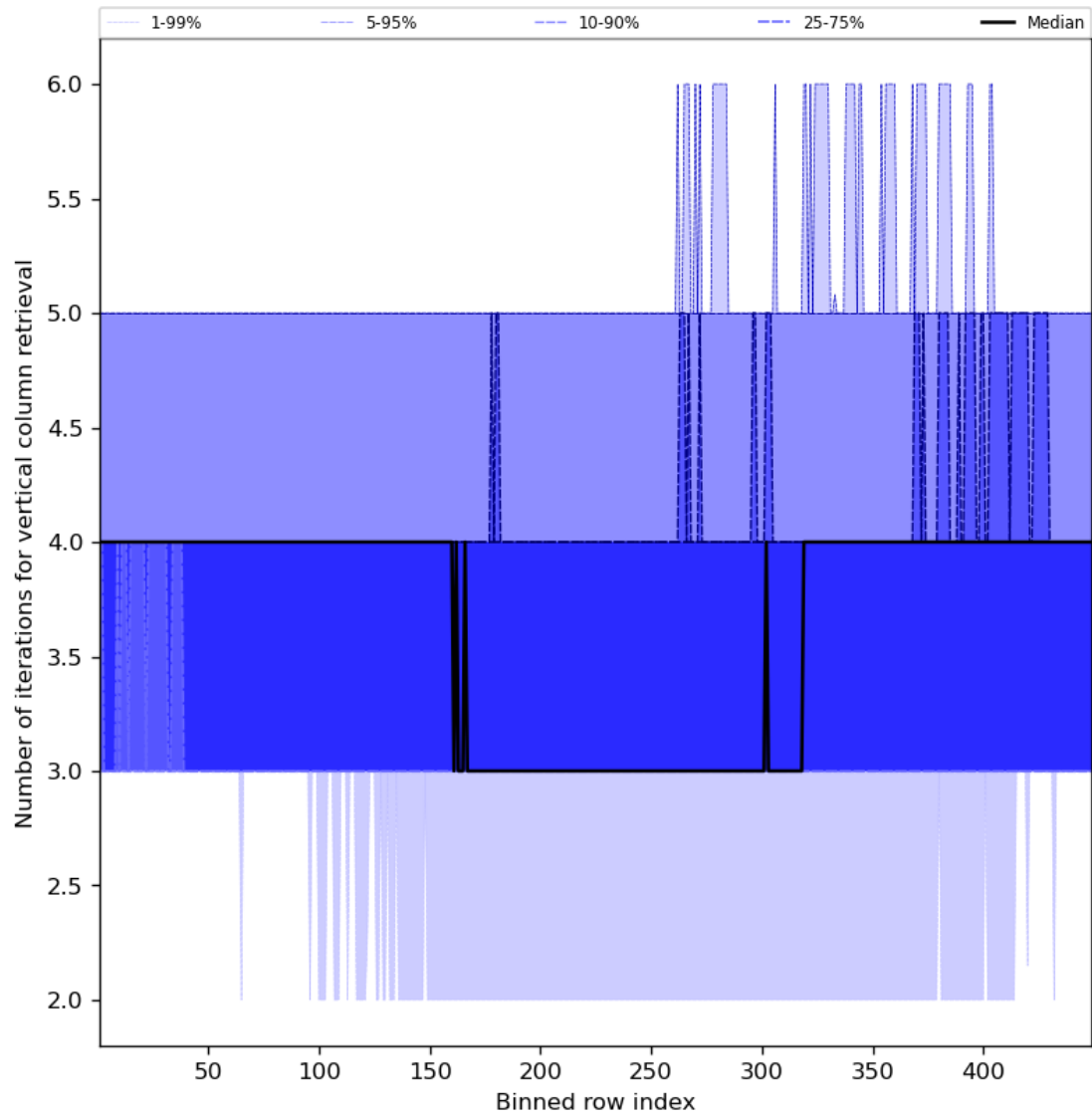
Figure 33: Along track statistics of “Number of iterations for vertical column retrieval” for 2023-11-02 to 2023-11-03
