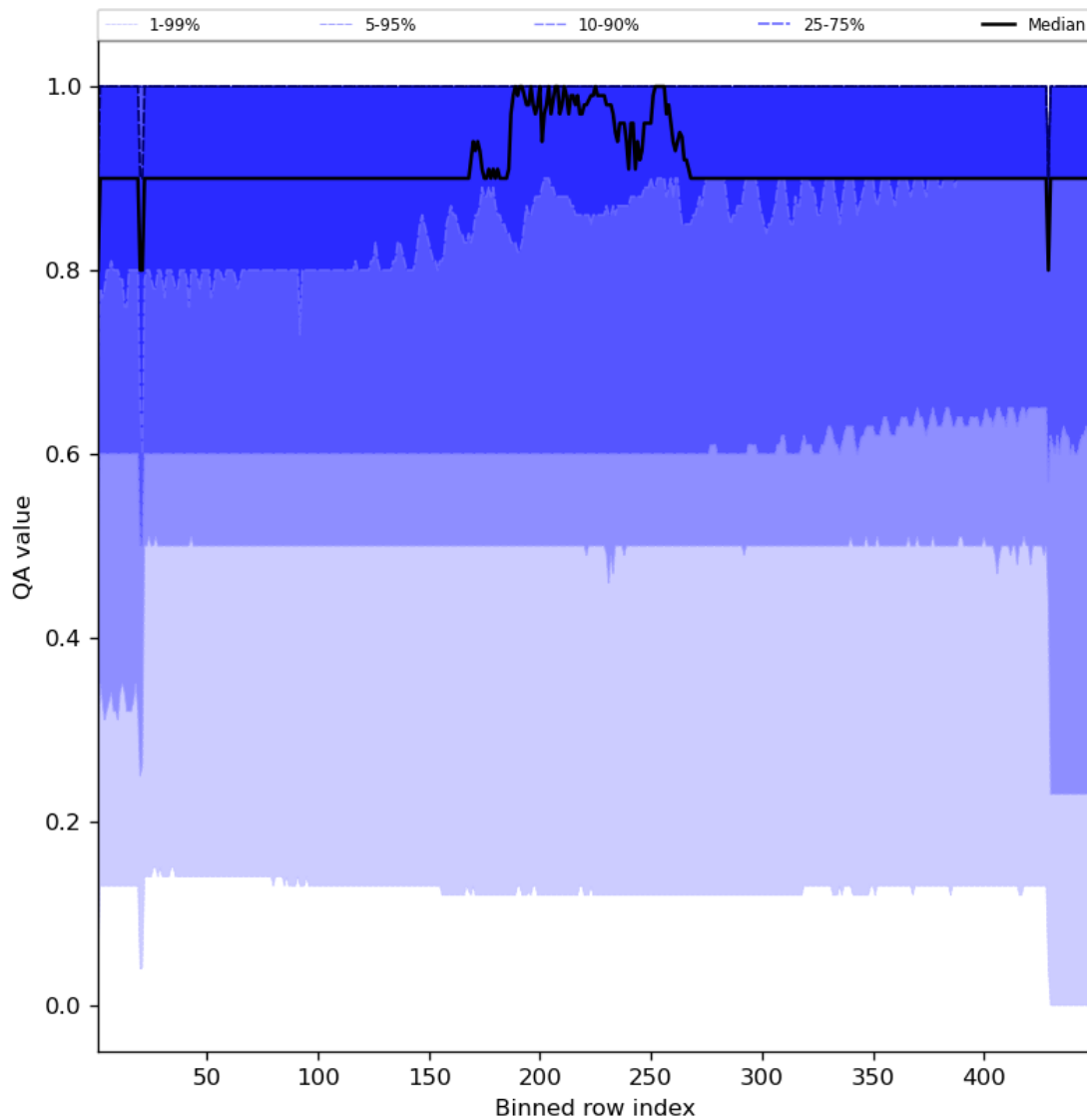
Figure 27: Along track statistics of “QA value” for 2023-11-02 to 2023-11-03
