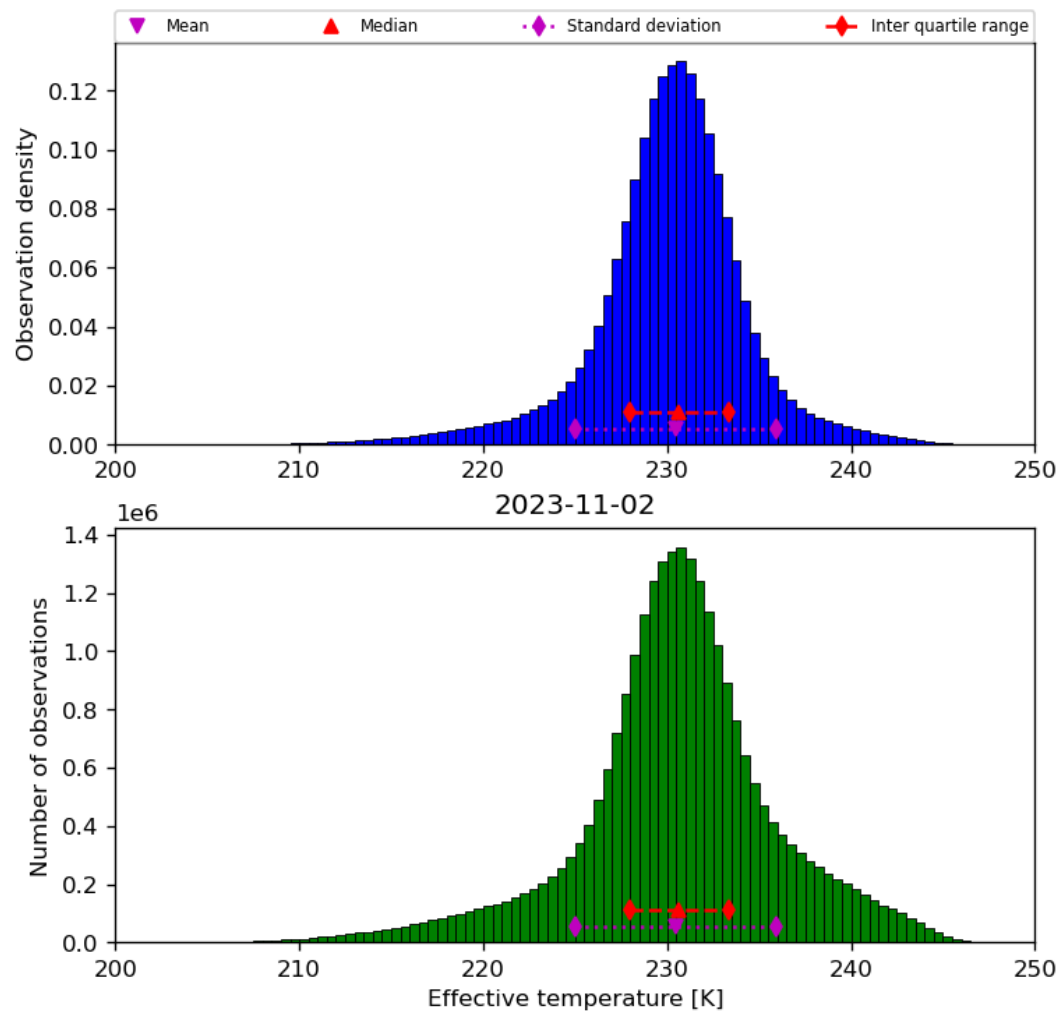
Figure 24: Histogram of “Effective temperature” for 2023-11-02 to 2023-11-03
