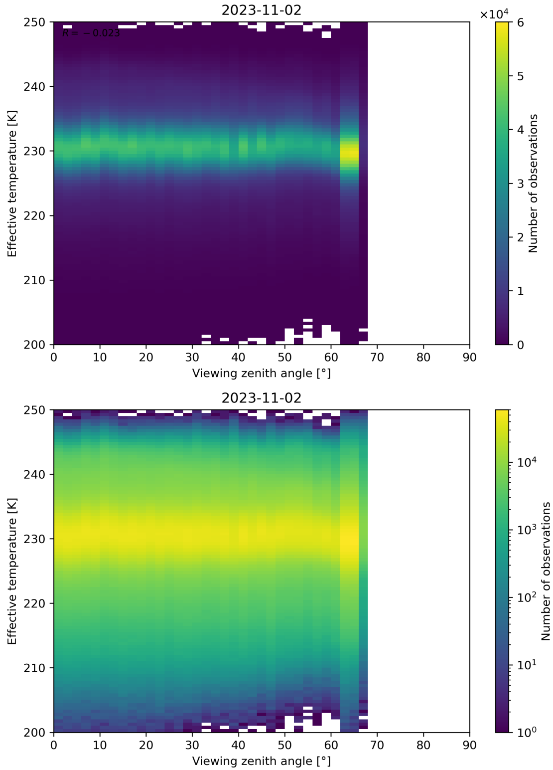
Figure 50: Scatter density plot of “Viewing zenith angle” against “Effective temperature” for 2023-11-02 to 2023-11-03.
