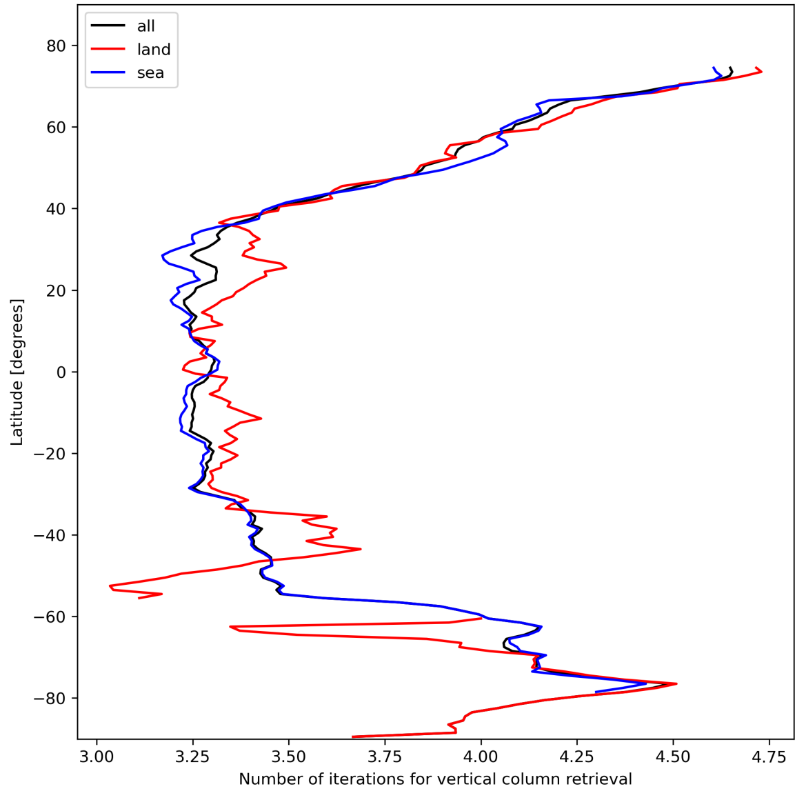
Figure 19: Zonal average of “Number of iterations for vertical column retrieval” for 2023-11-02 to 2023-11-03.
