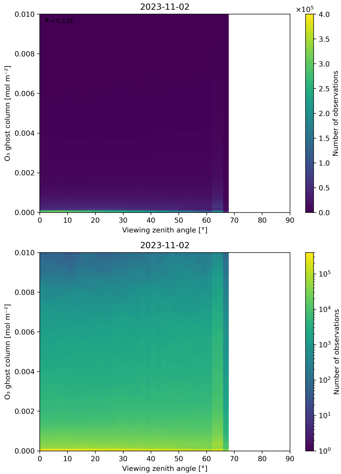
Figure 51: Scatter density plot of “Viewing zenith angle” against “O 3 ghost column” for 2023-11-02 to 2023-11-03.
