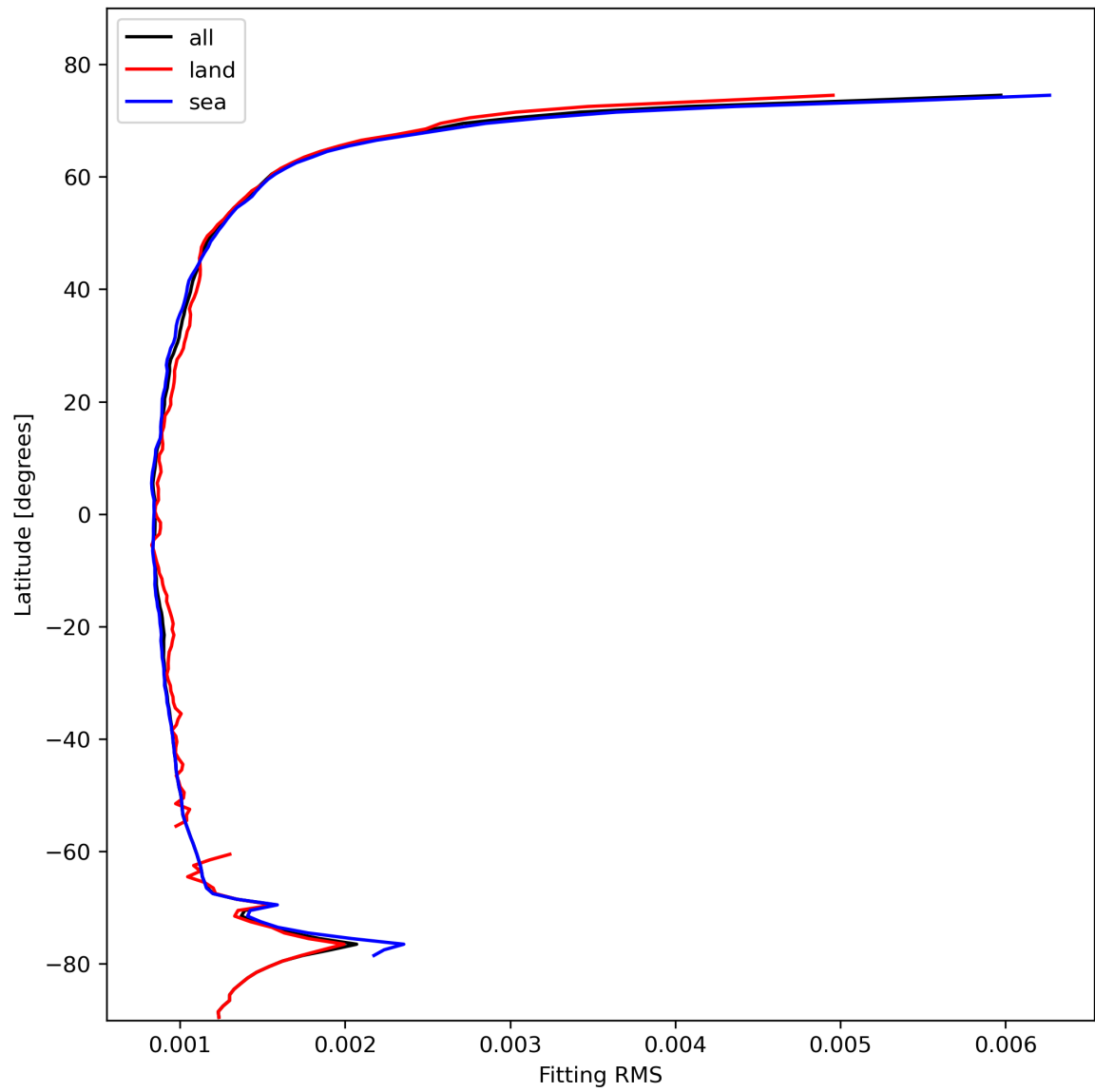
Figure 16: Zonal average of “Fitting RMS” for 2023-11-02 to 2023-11-03.
