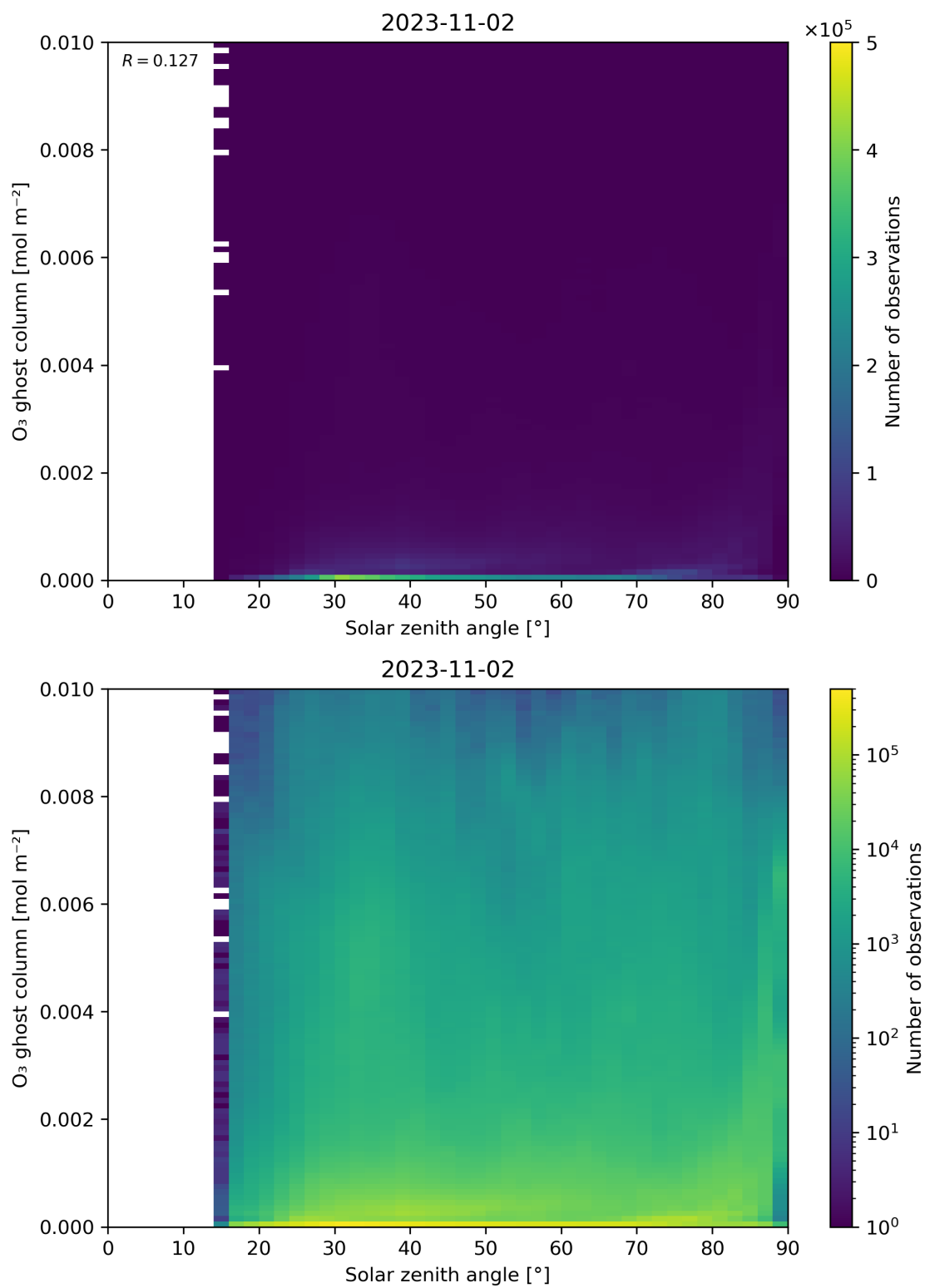
Figure 46: Scatter density plot of “Solar zenith angle” against “O 3 ghost column” for 2023-11-02 to 2023-11-03.
