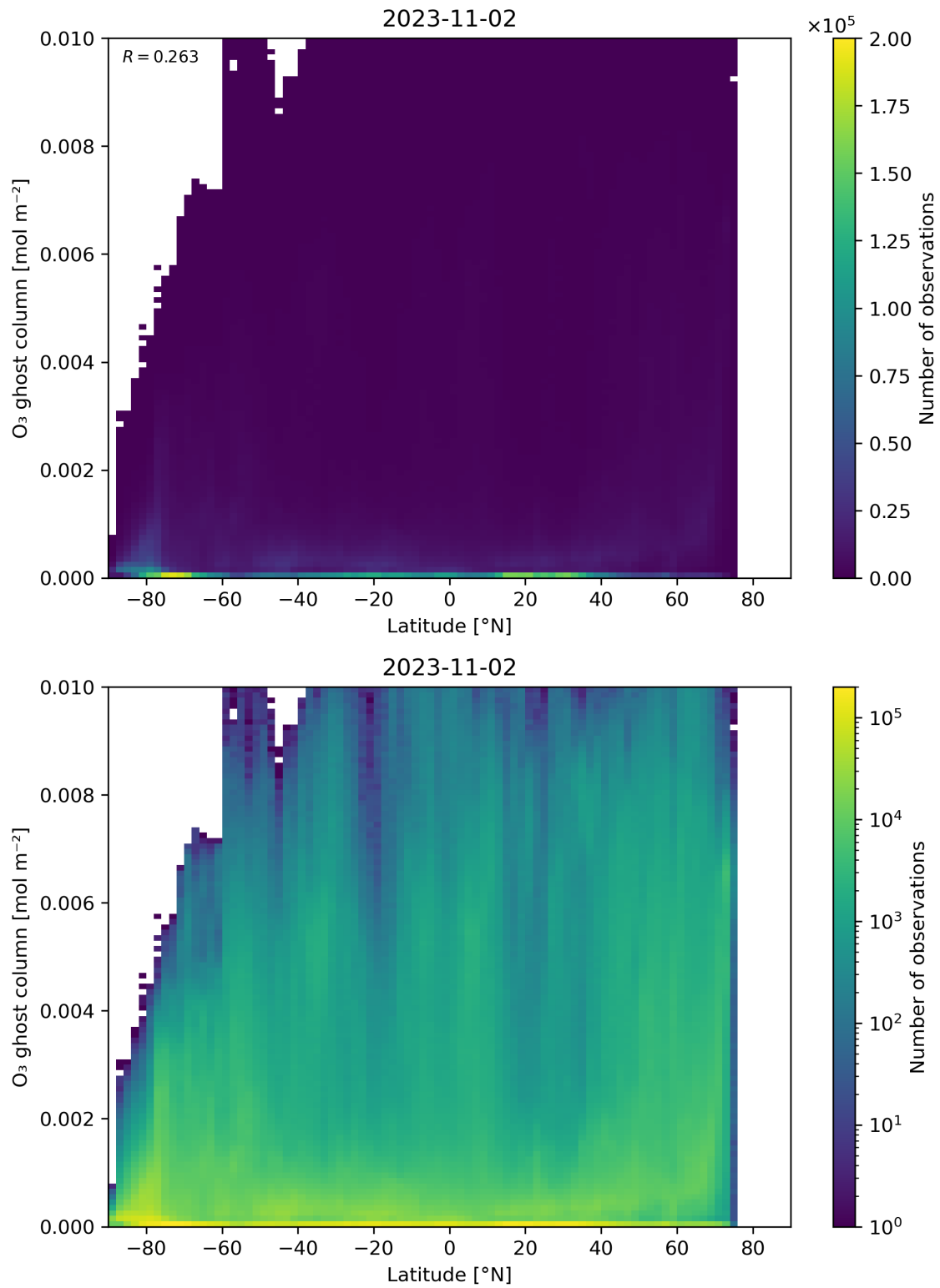
Figure 35: Scatter density plot of “Latitude” against “O 3 ghost column” for 2023-11-02 to 2023-11-03.
