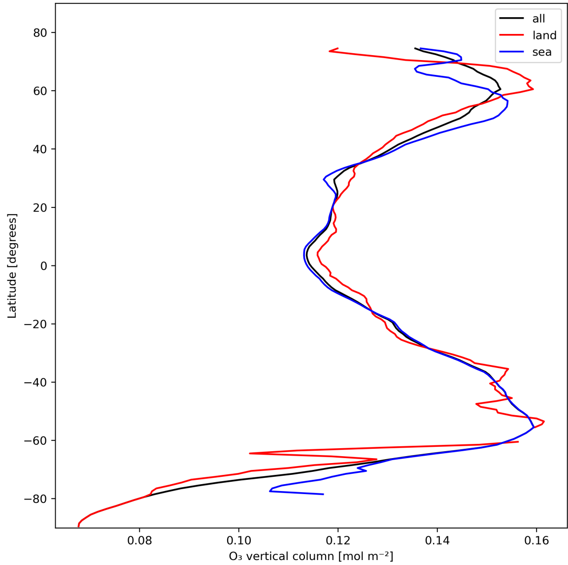
Figure 14: Zonal average of “O 3 vertical column” for 2023-11-02 to 2023-11-03.
