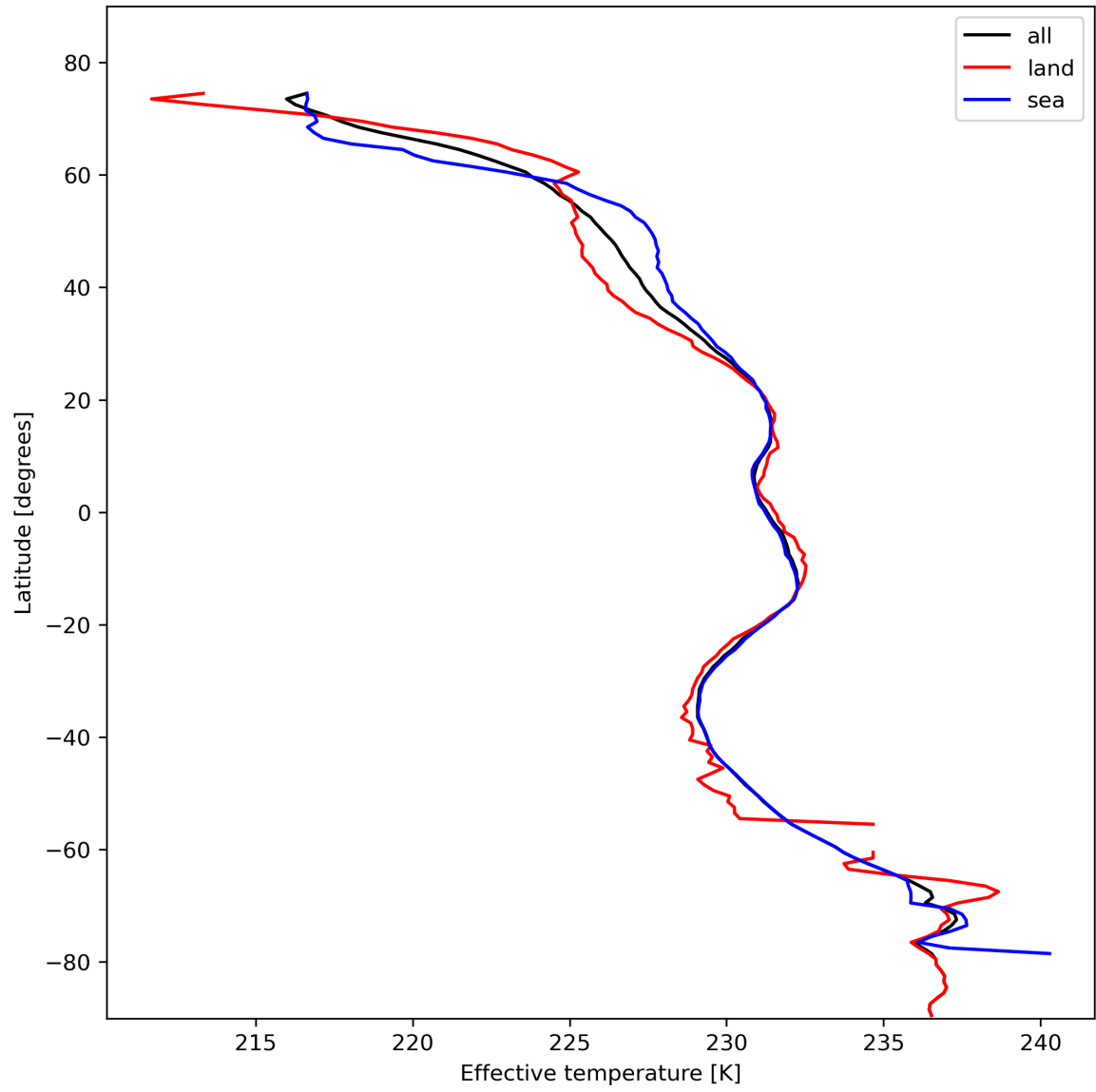
Figure 17: Zonal average of “Effective temperature” for 2023-11-02 to 2023-11-03.
