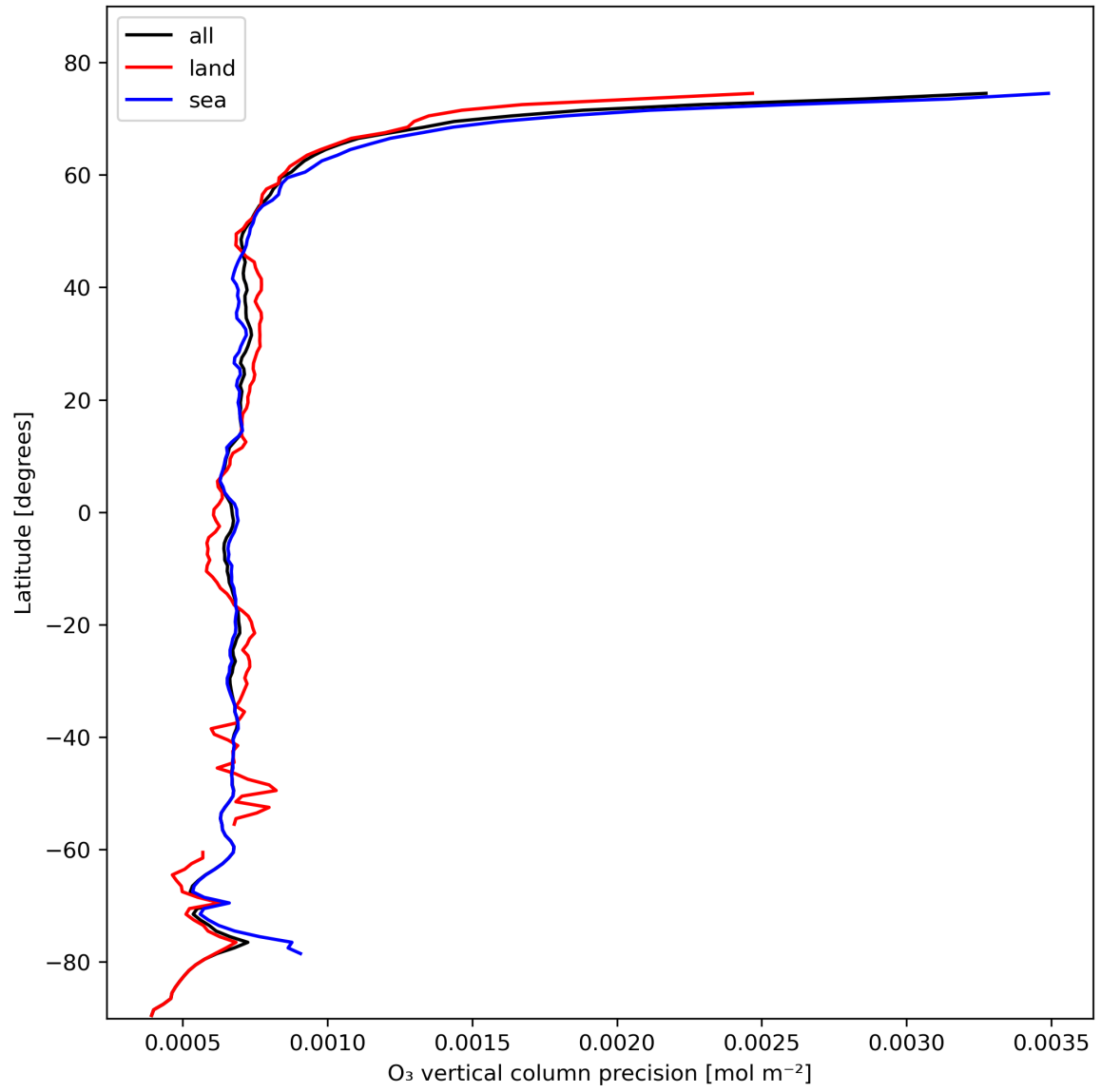
Figure 15: Zonal average of “O 3 vertical column precision” for 2023-11-02 to 2023-11-03.
