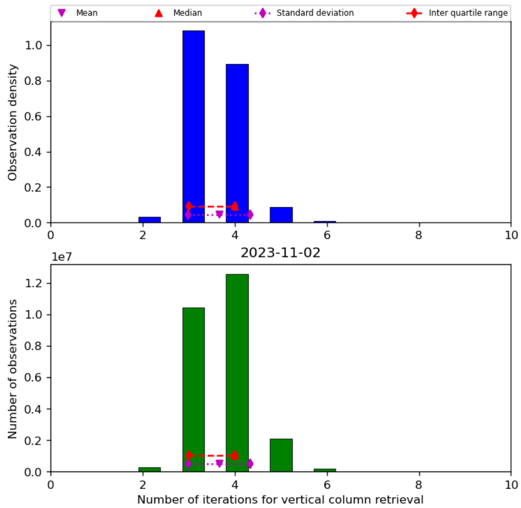
Figure 26: Histogram of “Number of iterations for vertical column retrieval” for 2023-11-02 to 2023-11-03
