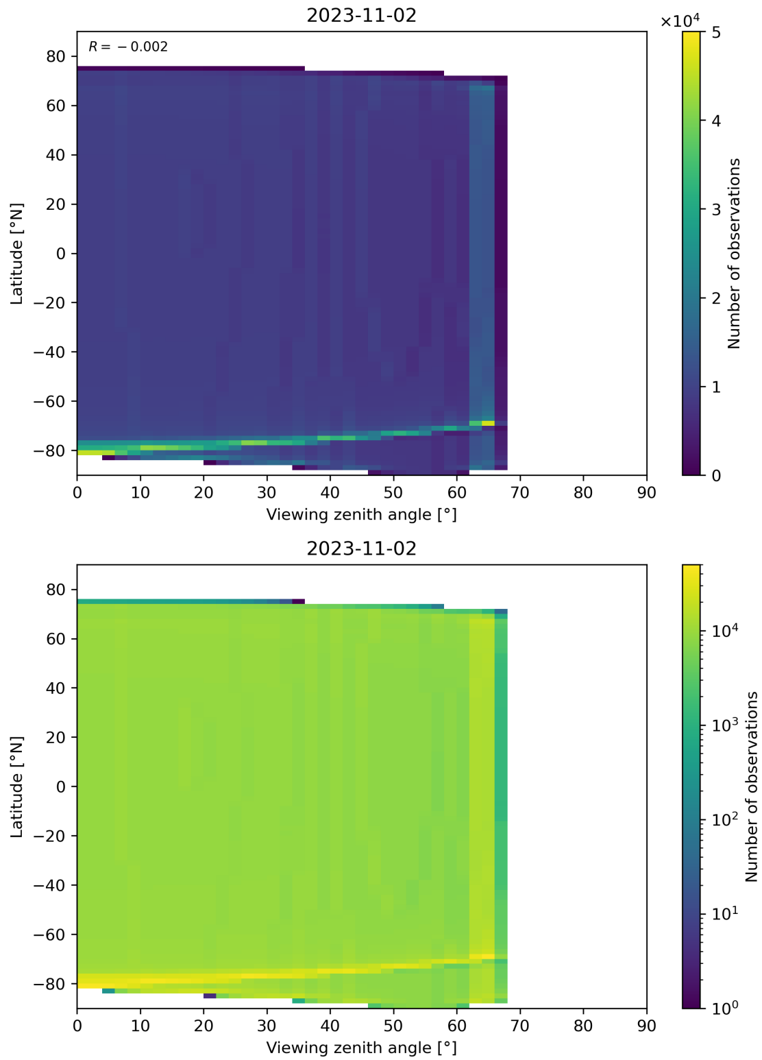
Figure 49: Scatter density plot of “Viewing zenith angle” against “Latitude” for 2023-11-02 to 2023-11-03.
