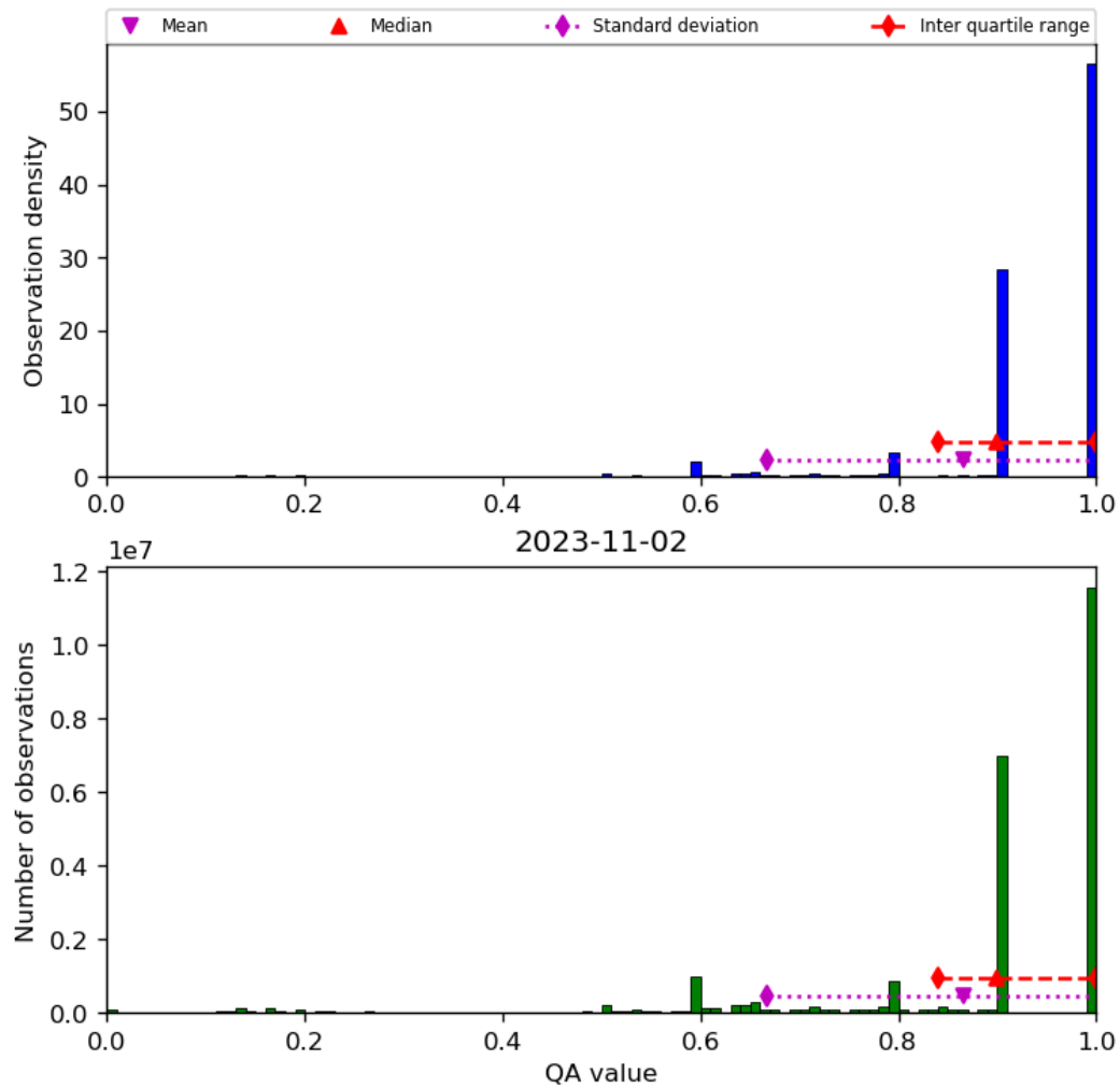
Figure 20: Histogram of “QA value” for 2023-11-02 to 2023-11-03
