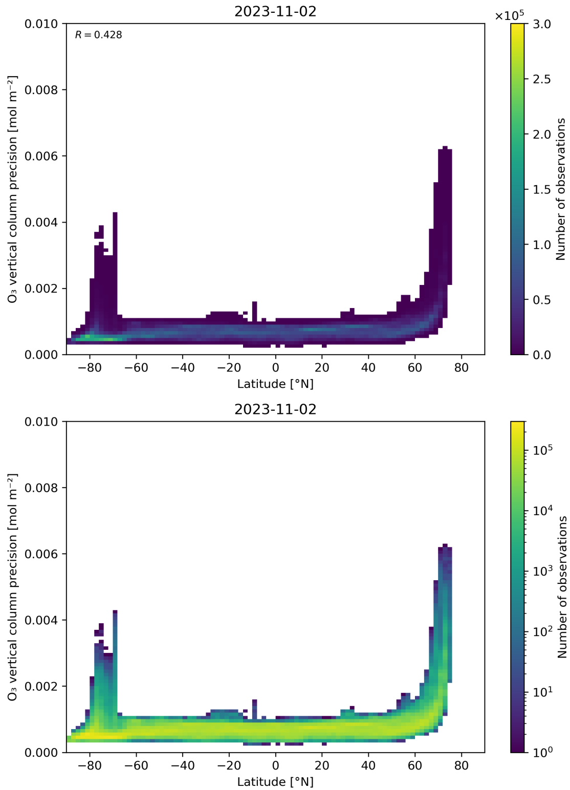
Figure 37: Scatter density plot of “Latitude” against “O 3 vertical column precision” for 2023-11-02 to 2023-11-03.
