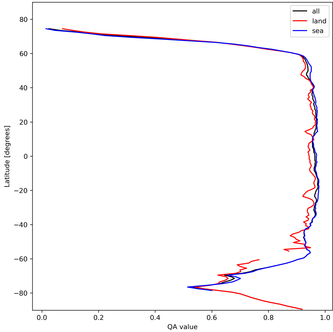
Figure 13: Zonal average of “QA value” for 2023-11-02 to 2023-11-03.
