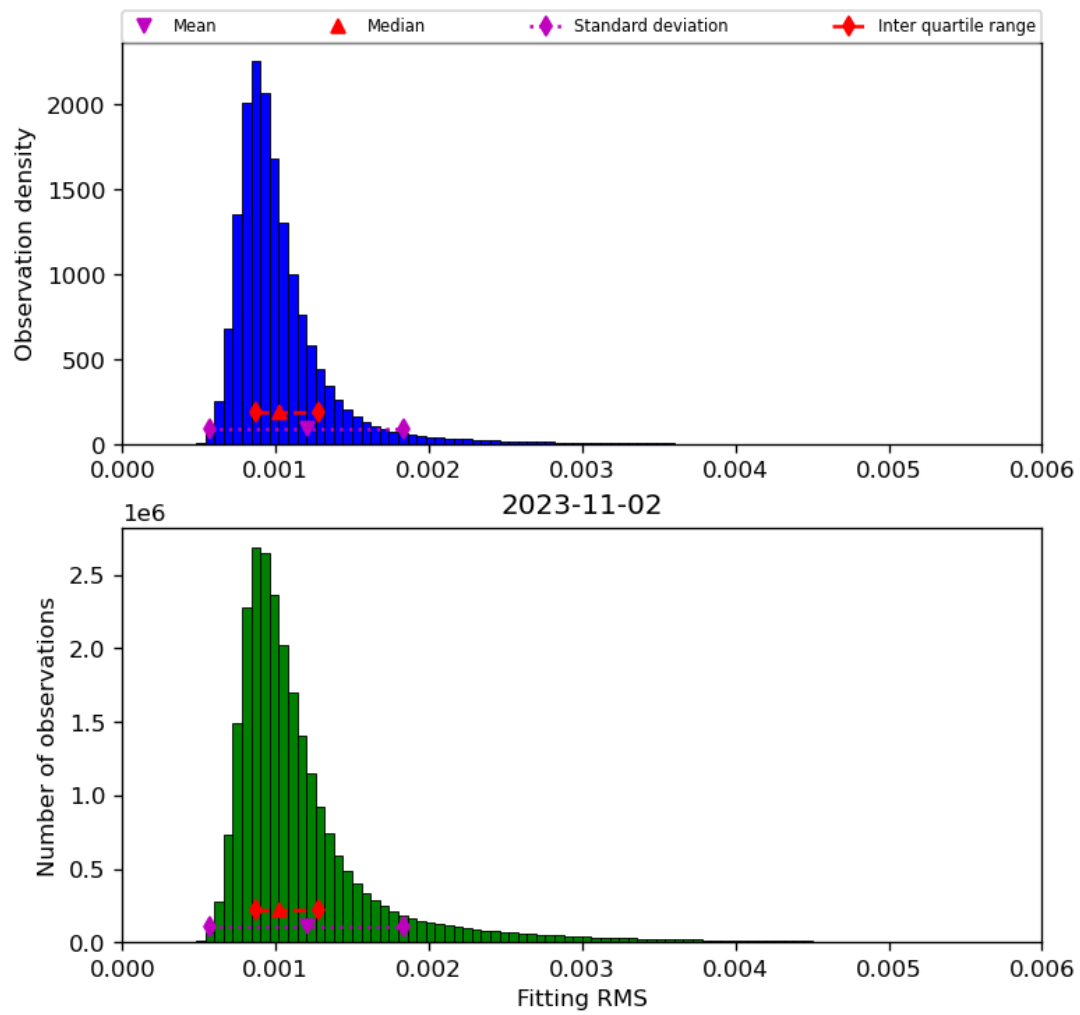
Figure 23: Histogram of “Fitting RMS” for 2023-11-02 to 2023-11-03
