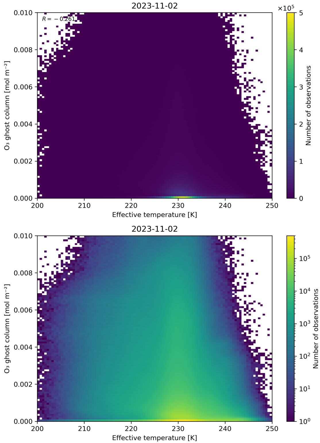
Figure 38: Scatter density plot of “Effective temperature” against “O 3 ghost column” for 2023-11-02 to 2023-11-03.
