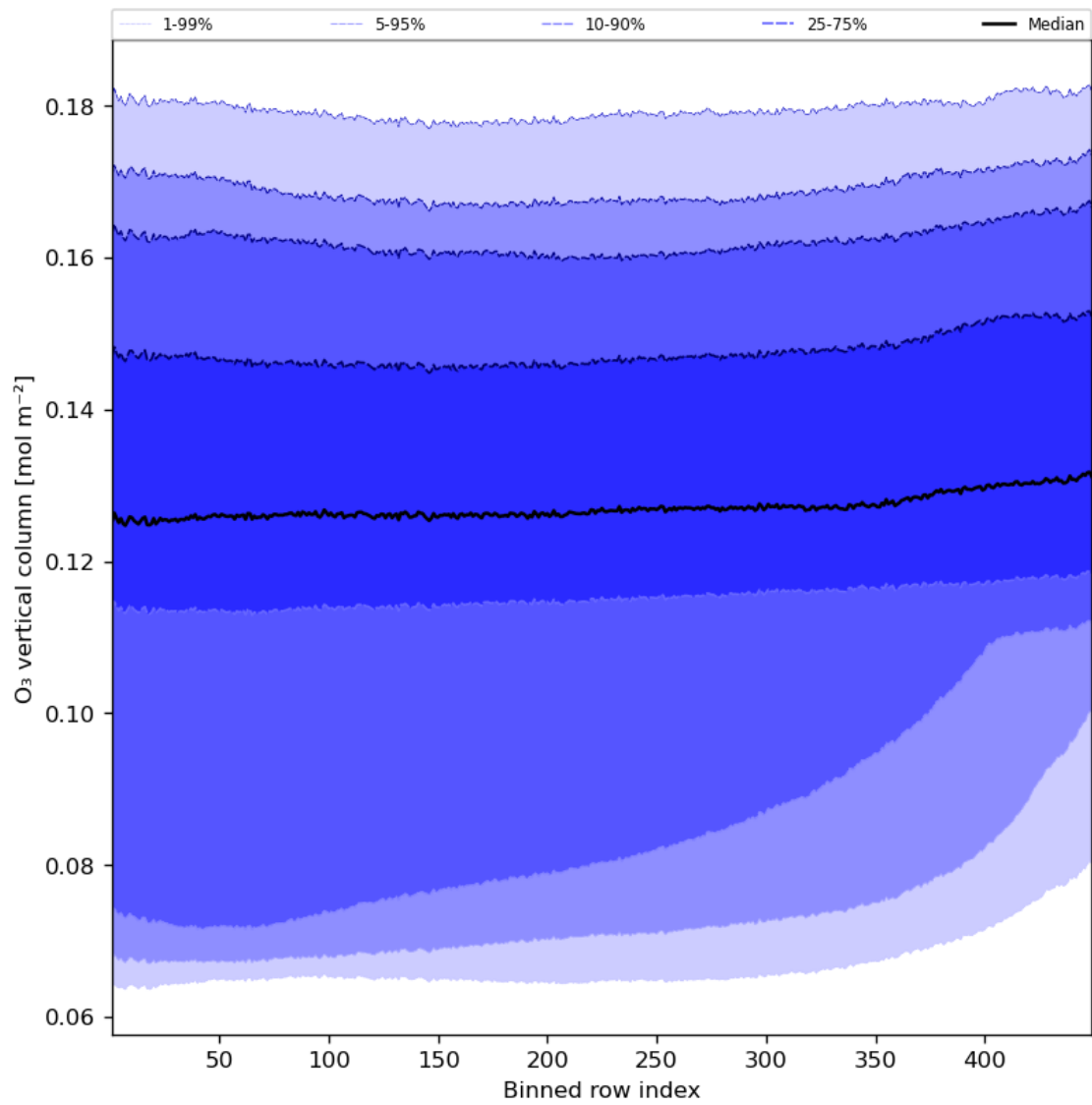
Figure 28: Along track statistics of “O 3 vertical column” for 2023-11-02 to 2023-11-03
