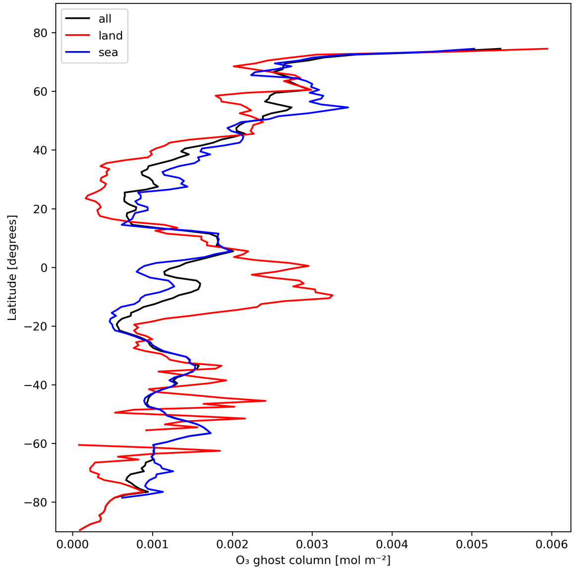
Figure 18: Zonal average of “O 3 ghost column” for 2023-11-02 to 2023-11-03.
