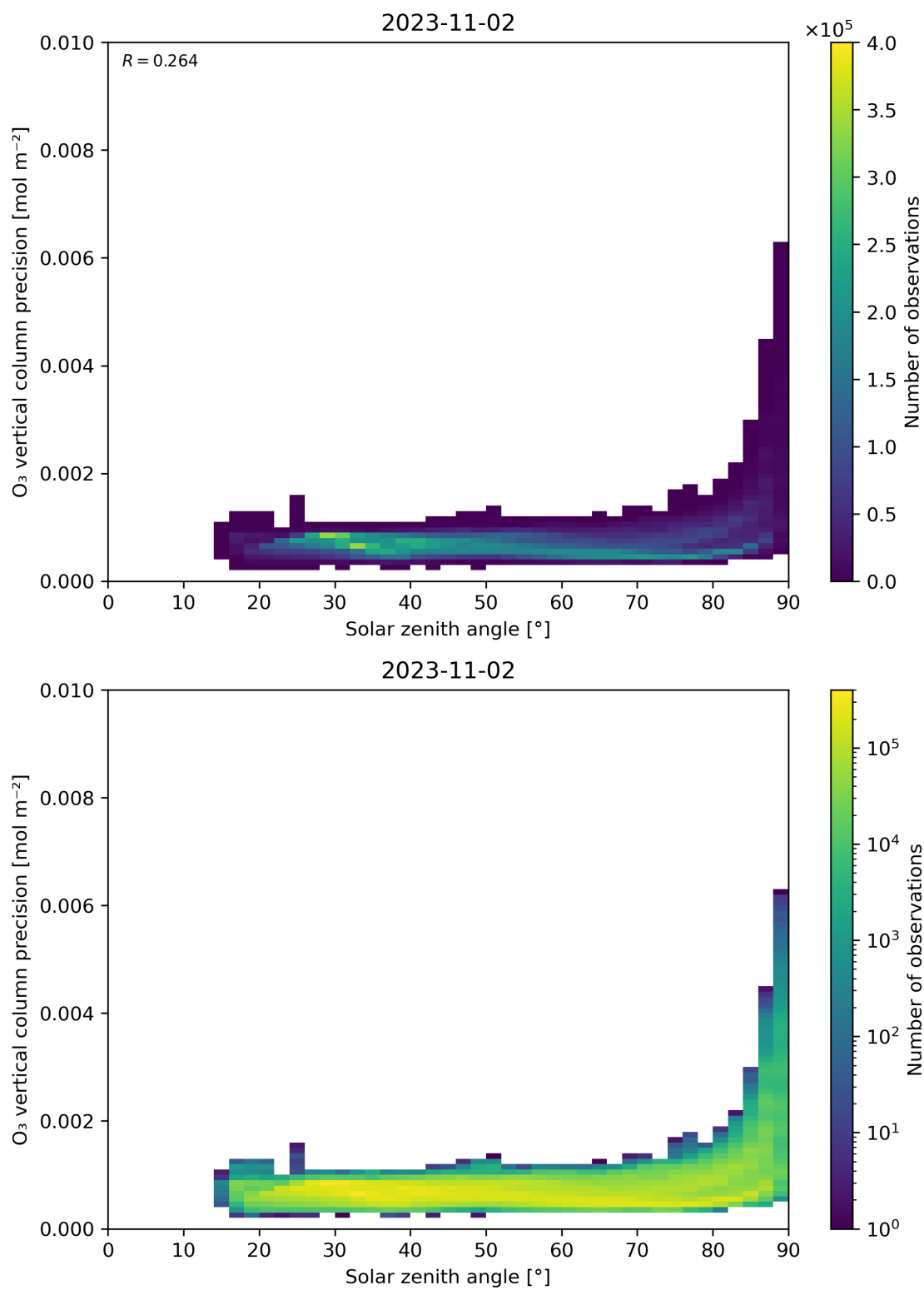
Figure 48: Scatter density plot of “Solar zenith angle” against “O 3 vertical column precision” for 2023-11-02 to 2023-11-03.
