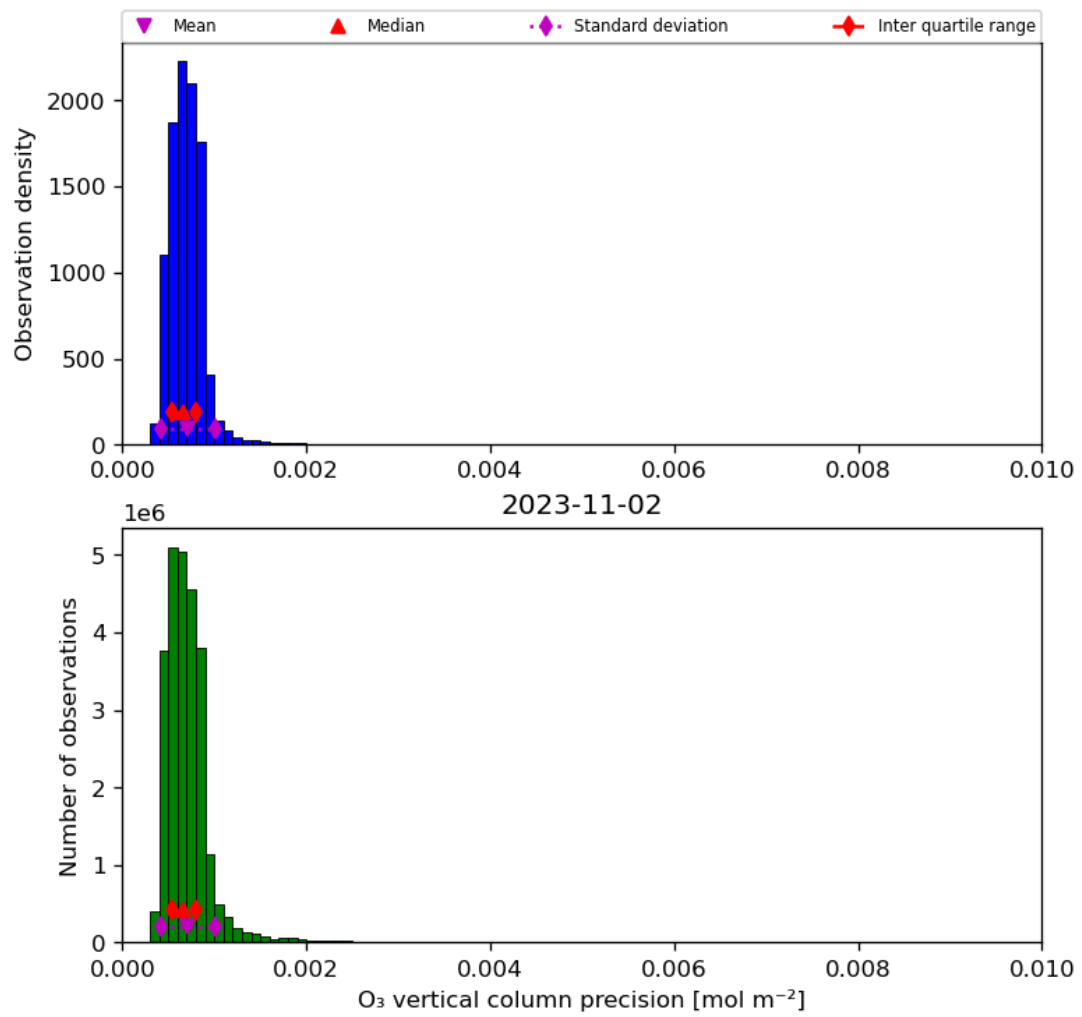
Figure 22: Histogram of “O 3 vertical column precision” for 2023-11-02 to 2023-11-03
