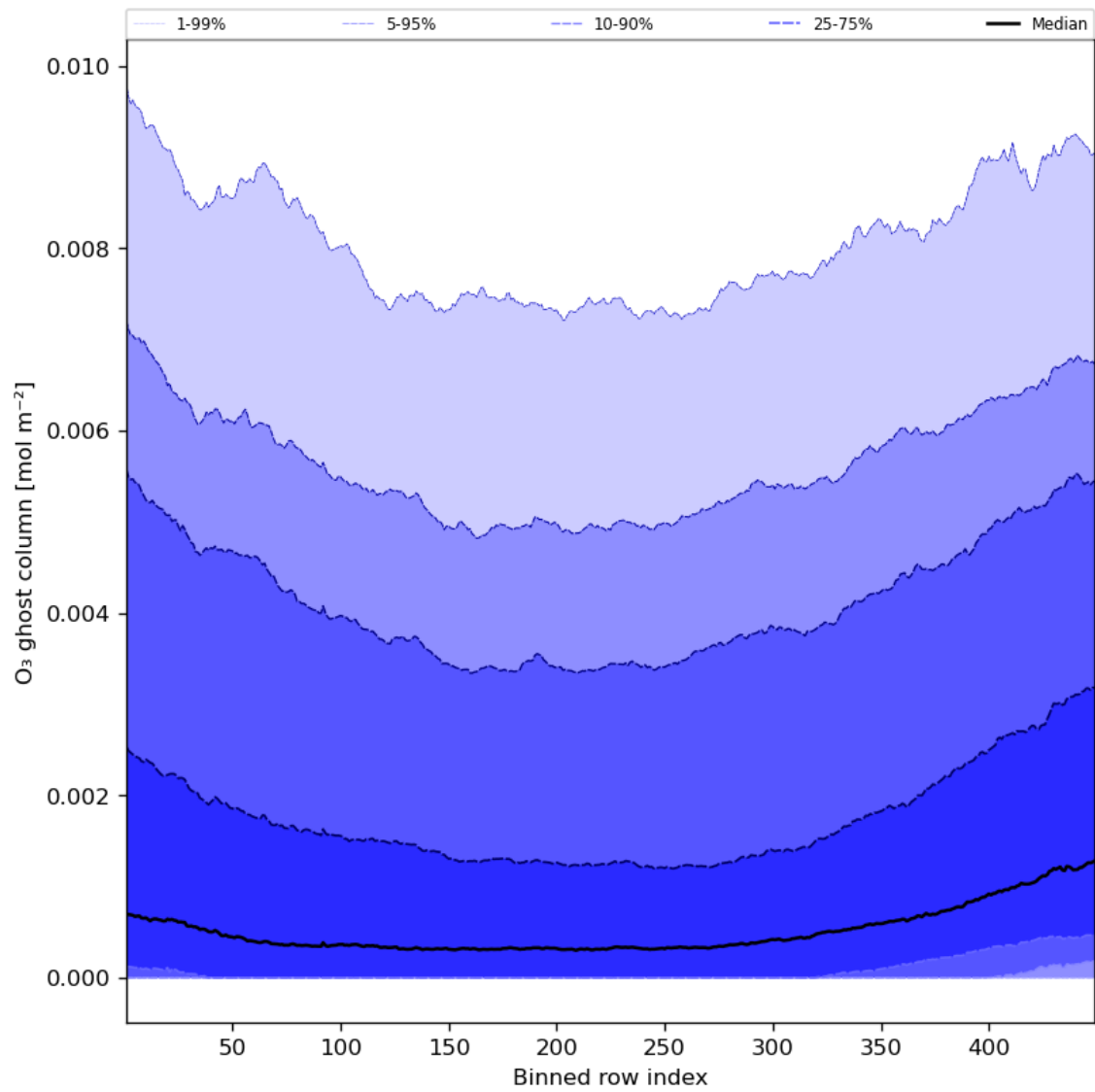
Figure 32: Along track statistics of “O 3 ghost column” for 2023-11-02 to 2023-11-03
