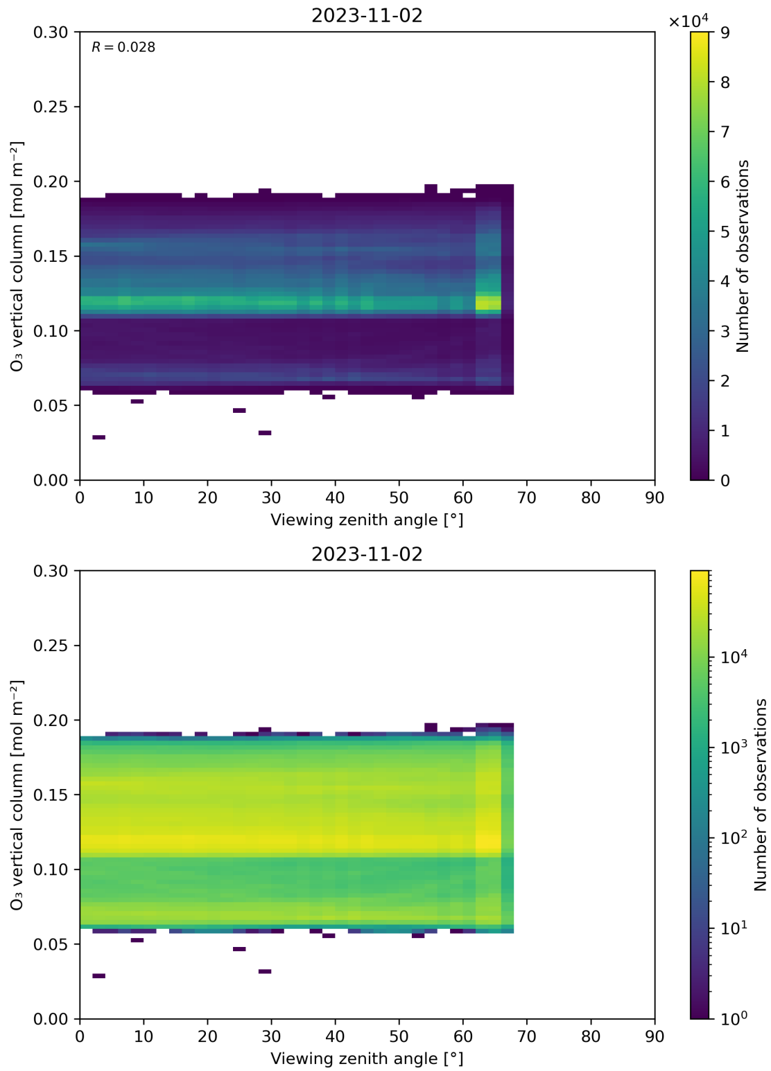
Figure 52: Scatter density plot of “Viewing zenith angle” against “O 3 vertical column” for 2023-11-02 to 2023-11-03.
