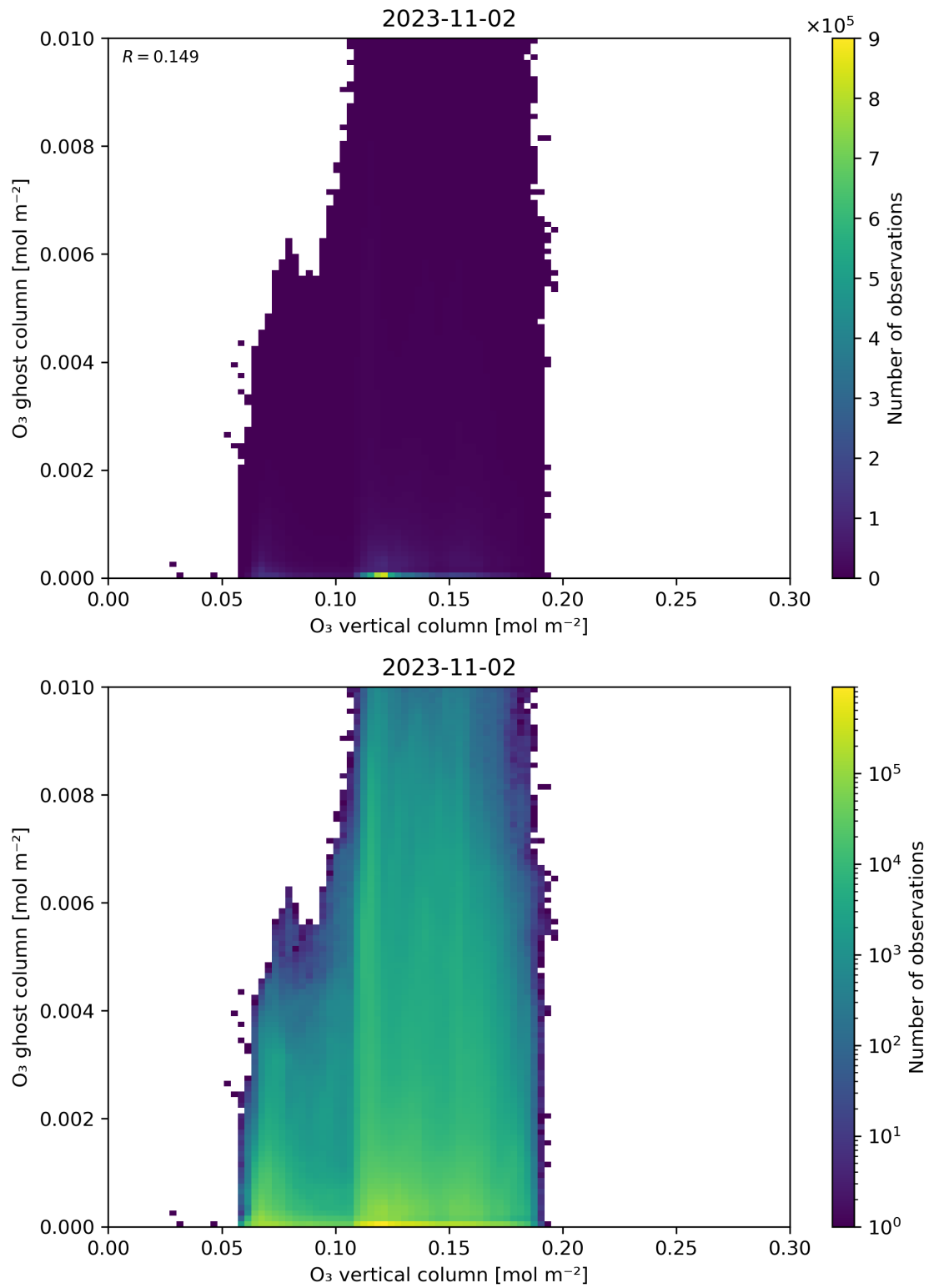
Figure 40: Scatter density plot of “O 3 vertical column” against “O 3 ghost column” for 2023-11-02 to 2023-11-03.
