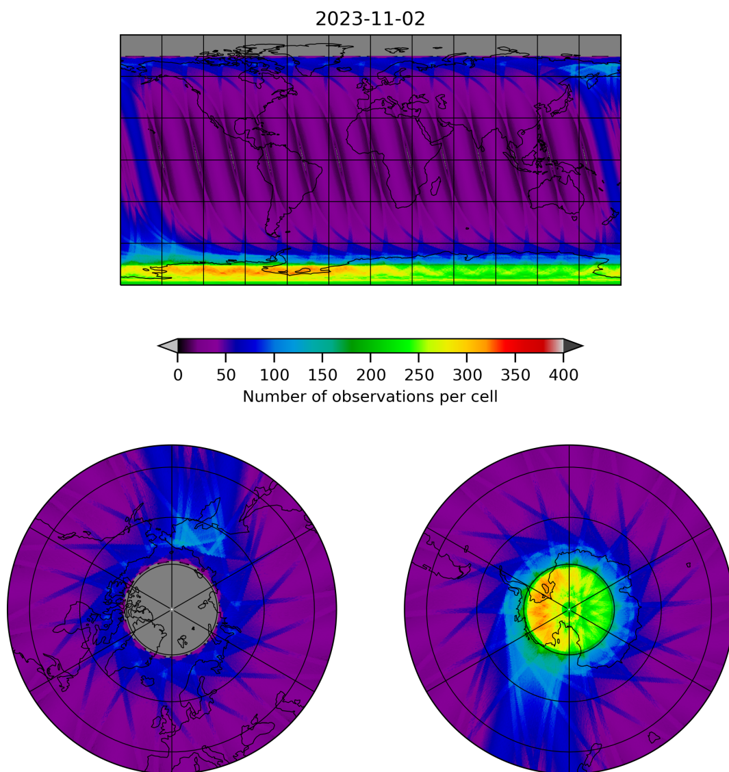
Figure 12: Map of the number of observations for 2023-11-02 to 2023-11-03
