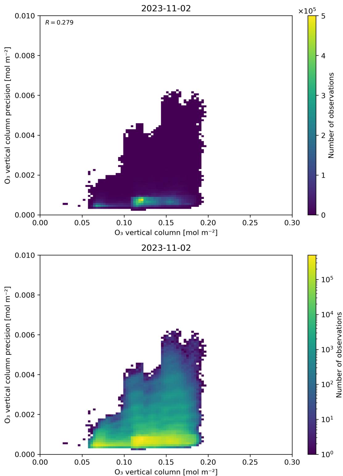
Figure 41: Scatter density plot of “O 3 vertical column” against “O 3 vertical column precision” for 2023-11-02 to 2023-11-03.
