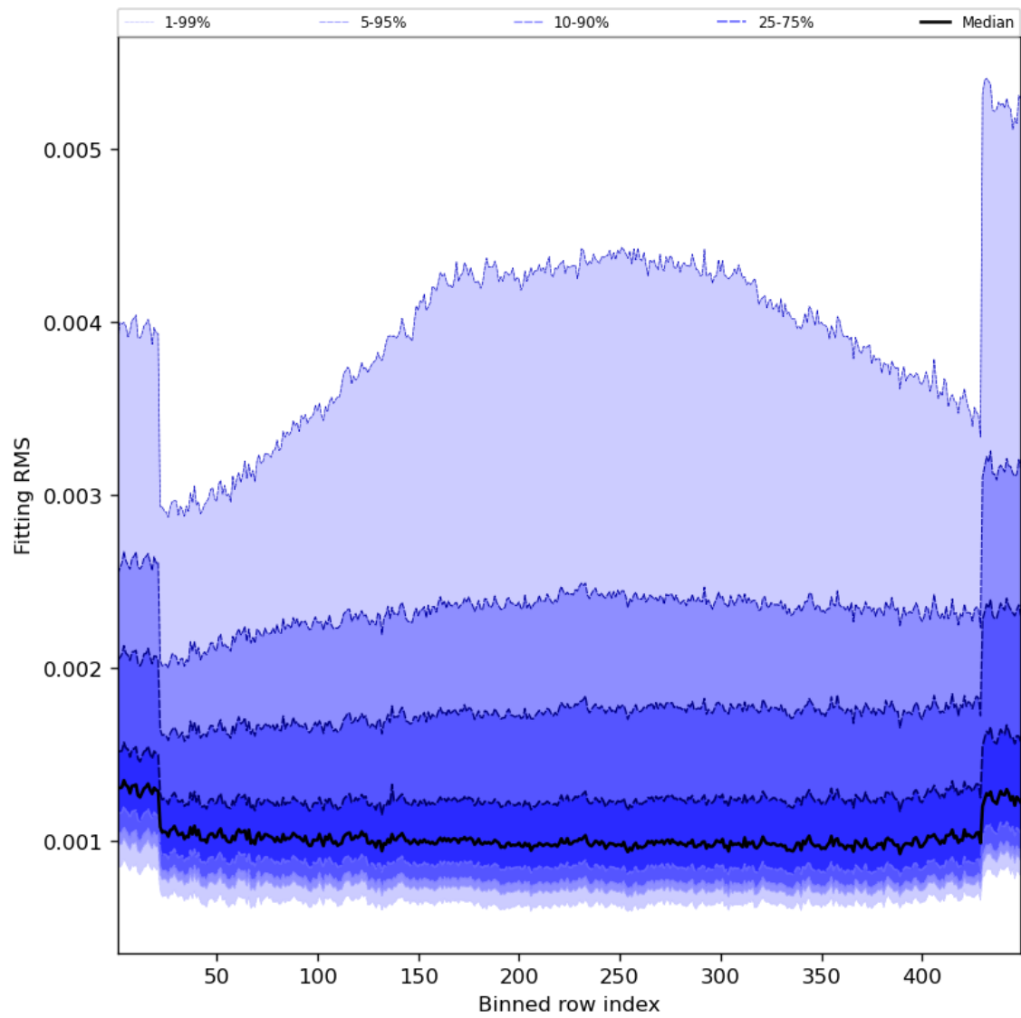
Figure 30: Along track statistics of “Fitting RMS” for 2023-11-02 to 2023-11-03
