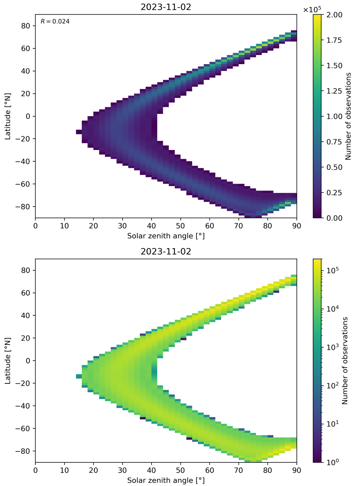
Figure 44: Scatter density plot of “Solar zenith angle” against “Latitude” for 2023-11-02 to 2023-11-03.
