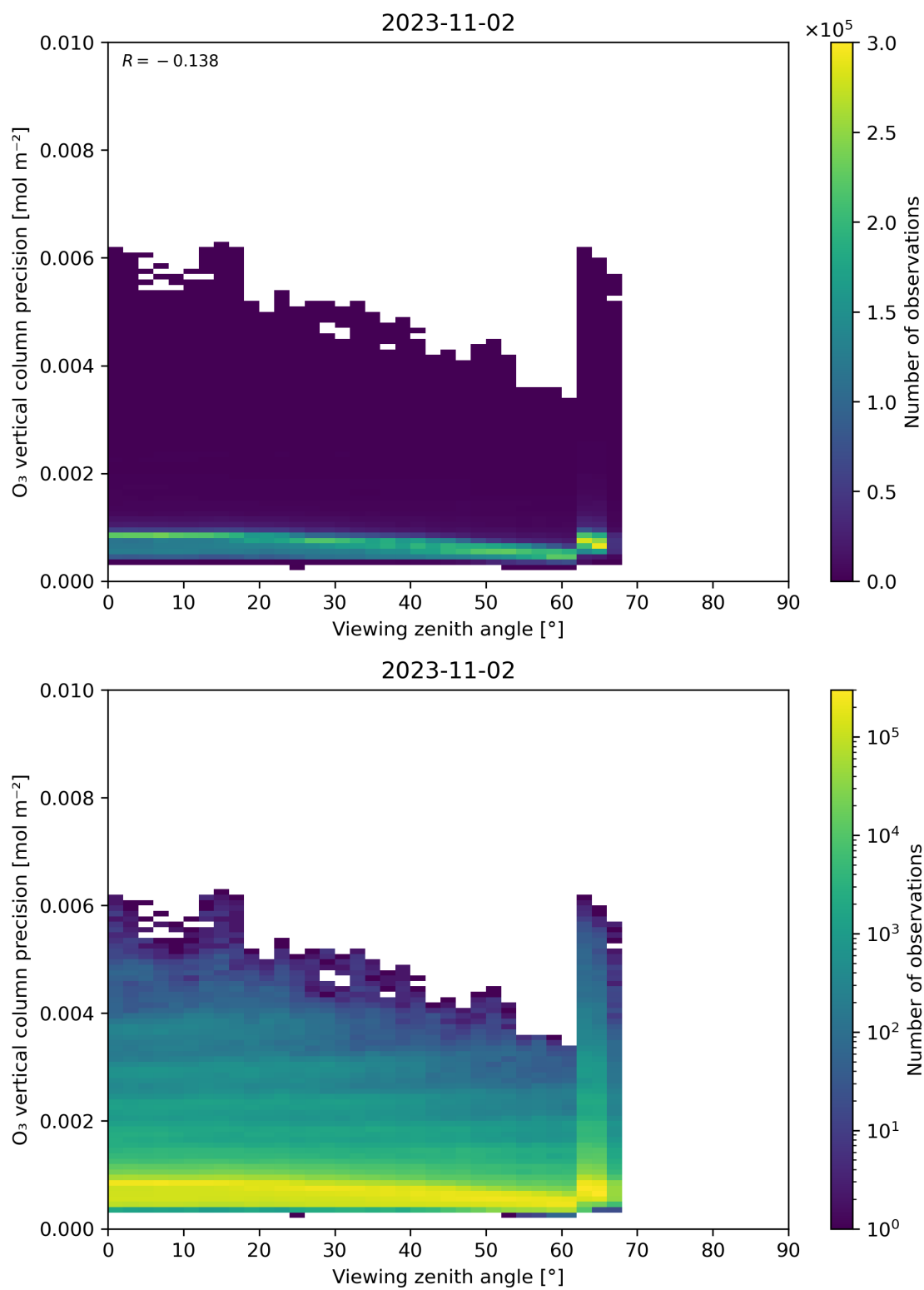
Figure 53: Scatter density plot of “Viewing zenith angle” against “O 3 vertical column precision” for 2023-11-02 to 2023-11-03.
