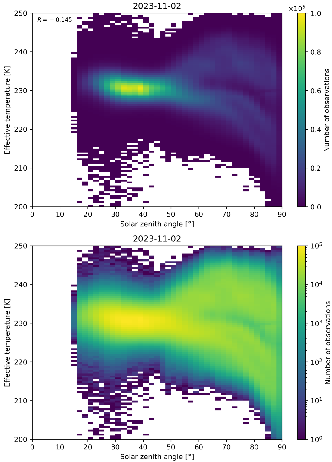
Figure 45: Scatter density plot of “Solar zenith angle” against “Effective temperature” for 2023-11-02 to 2023-11-03.
