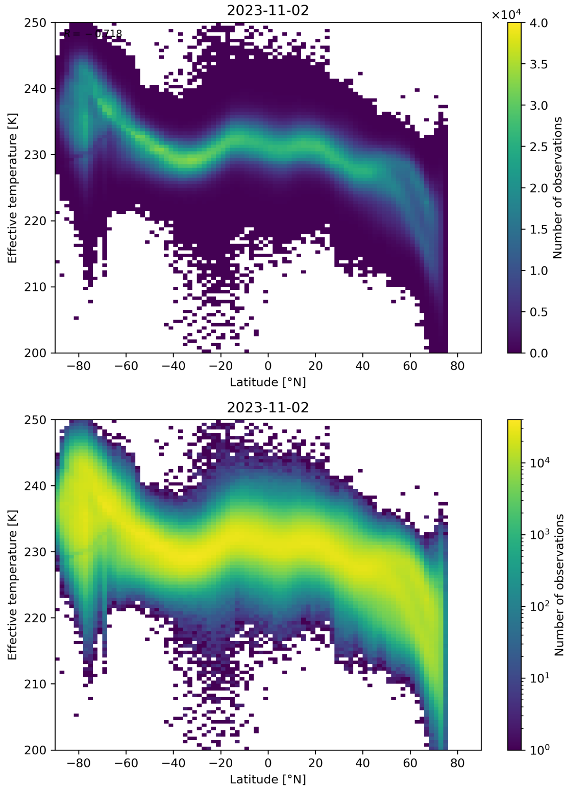
Figure 34: Scatter density plot of “Latitude” against “Effective temperature” for 2023-11-02 to 2023-11-03.
