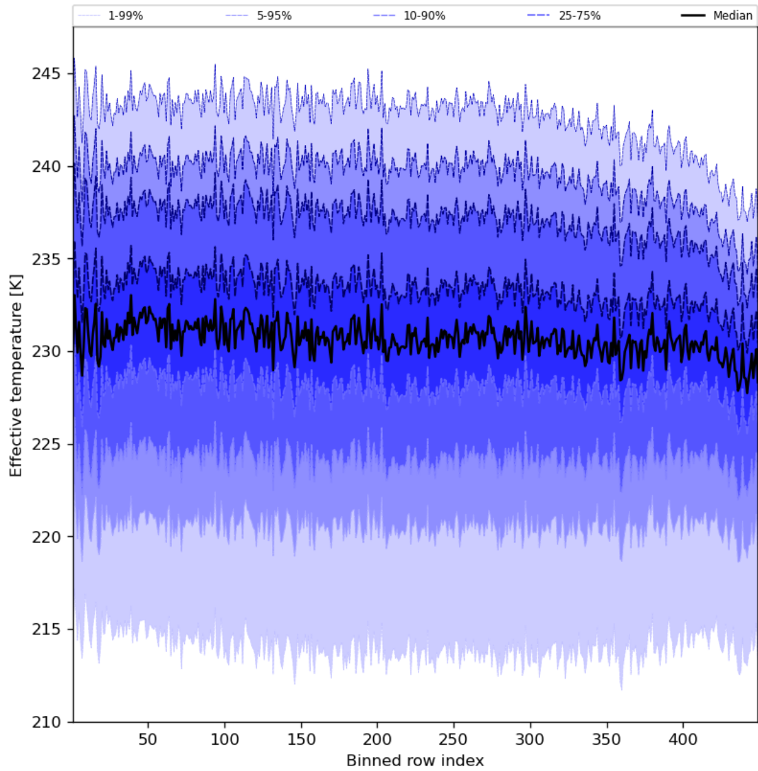
Figure 31: Along track statistics of “Effective temperature” for 2023-11-02 to 2023-11-03
