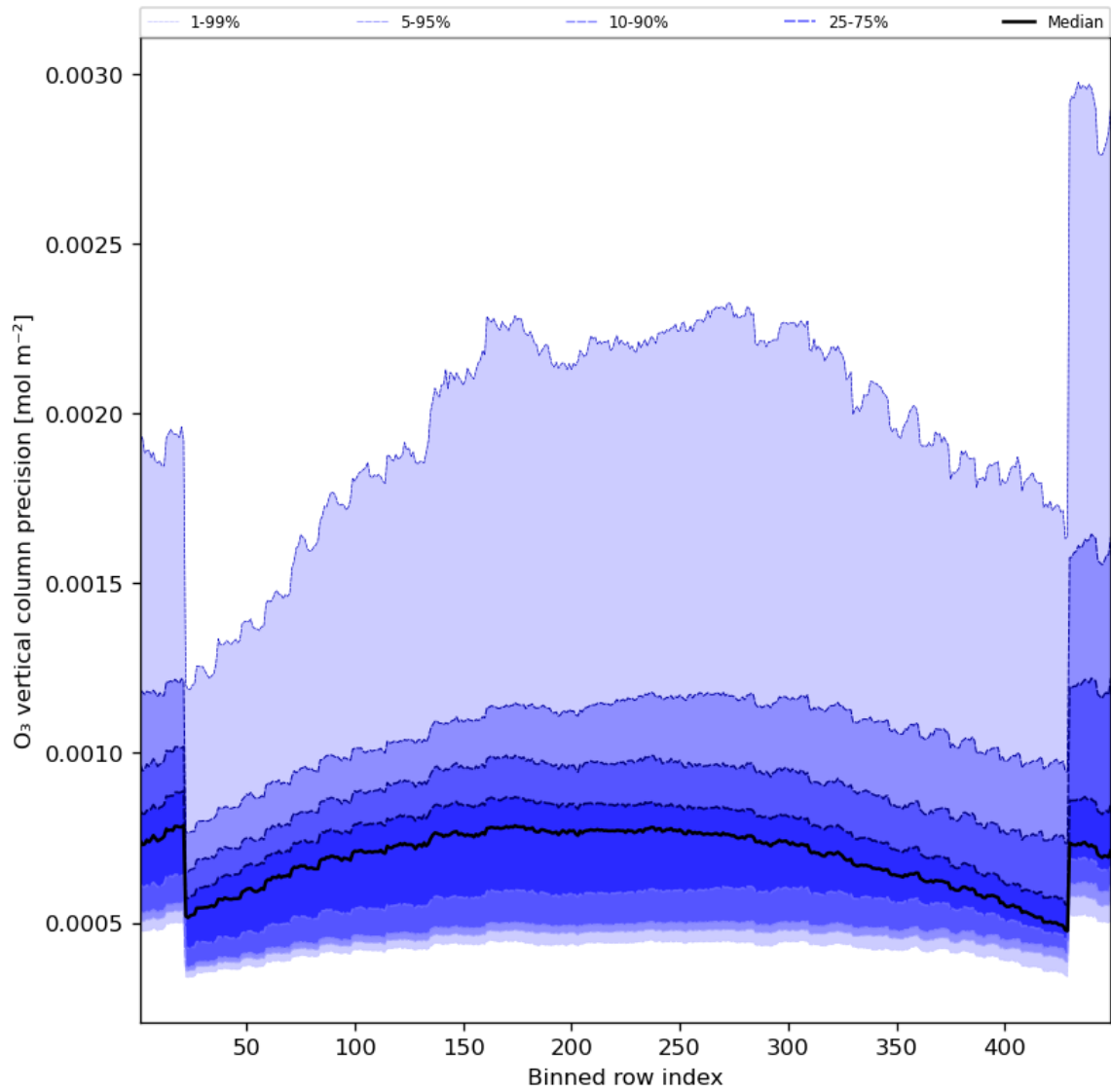
Figure 29: Along track statistics of “O 3 vertical column precision” for 2023-11-02 to 2023-11-03
