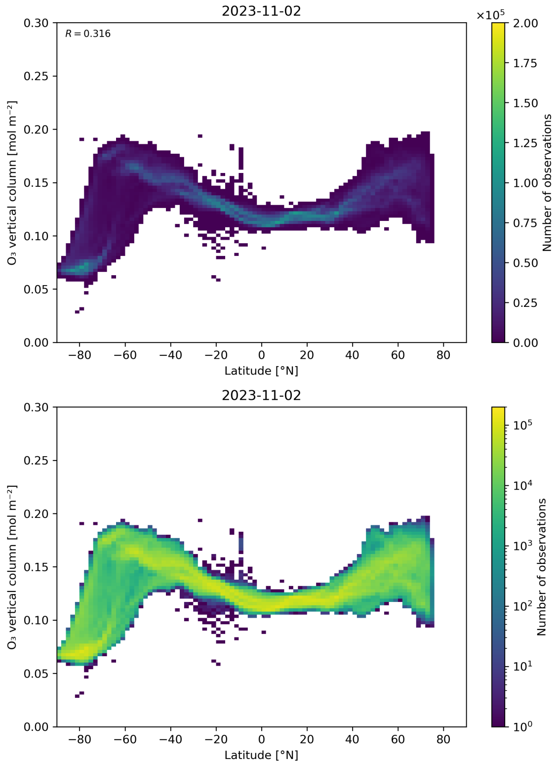
Figure 36: Scatter density plot of “Latitude” against “O 3 vertical column” for 2023-11-02 to 2023-11-03.
