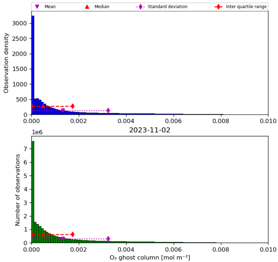
Figure 25: Histogram of “O 3 ghost column” for 2023-11-02 to 2023-11-03
