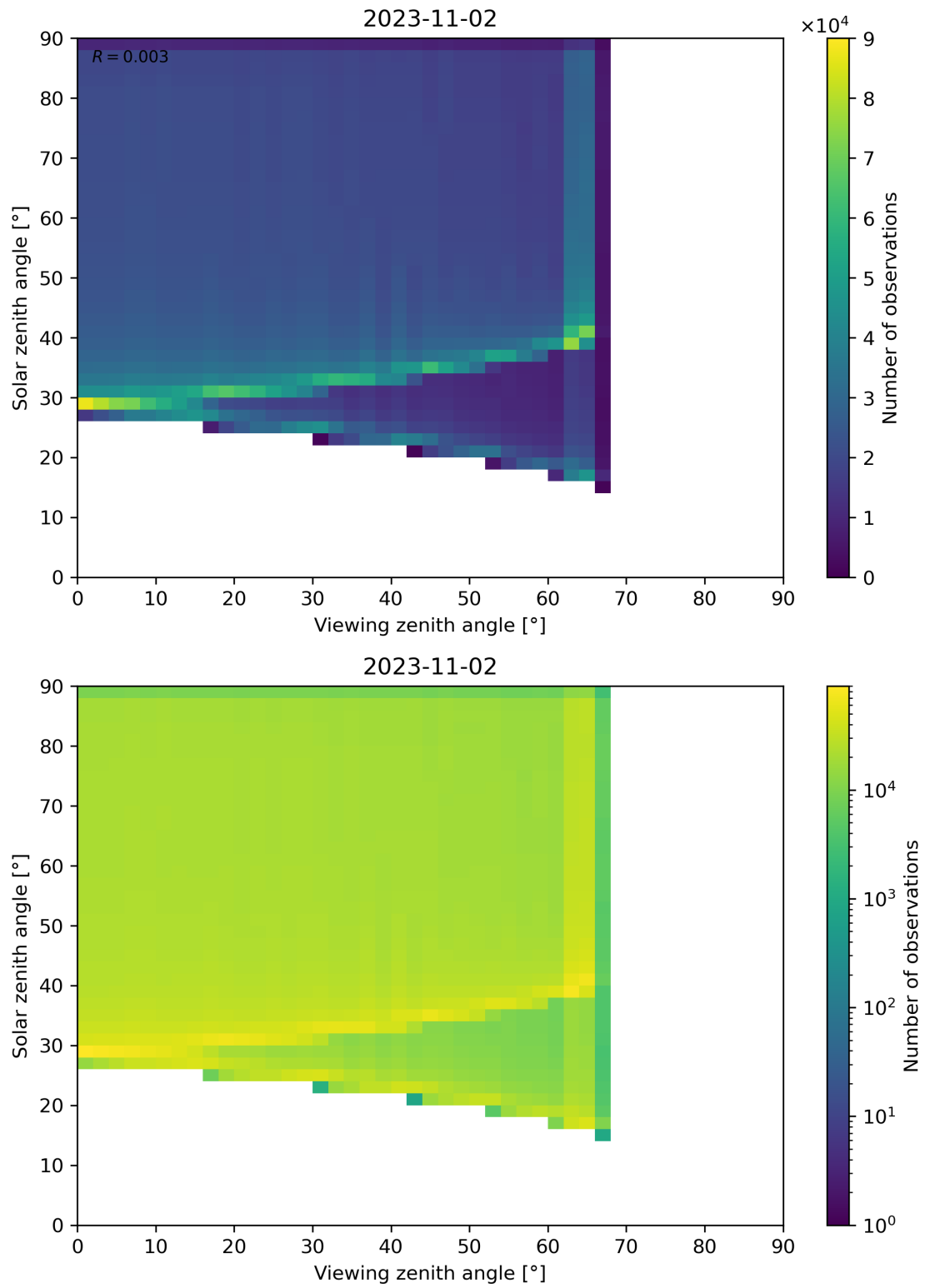
Figure 54: Scatter density plot of “Viewing zenith angle” against “Solar zenith angle” for 2023-11-02 to 2023-11-03.
