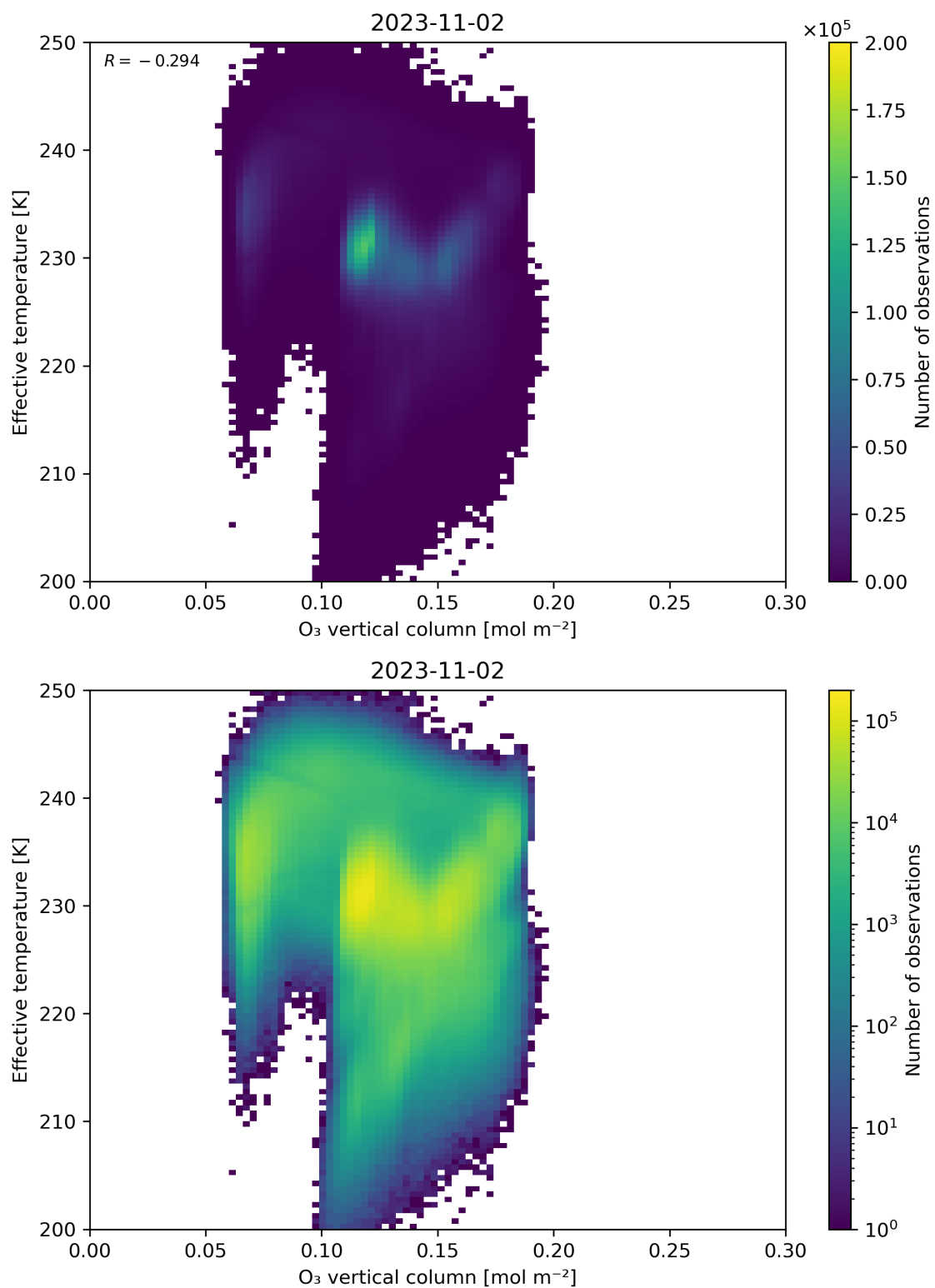
Figure 39: Scatter density plot of “O 3 vertical column” against “Effective temperature” for 2023-11-02 to 2023-11-03.
