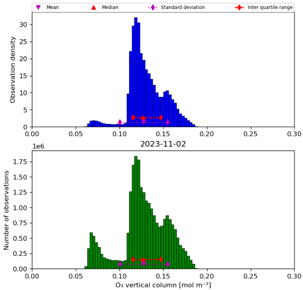
Figure 21: Histogram of “O 3 vertical column” for 2023-11-02 to 2023-11-03
