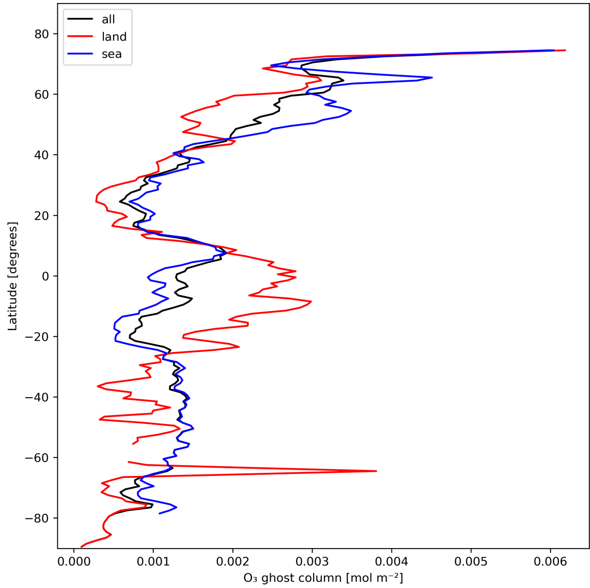
Figure 18: Zonal average of “O 3 ghost column” for 2023-11-02 to 2023-11-04.
