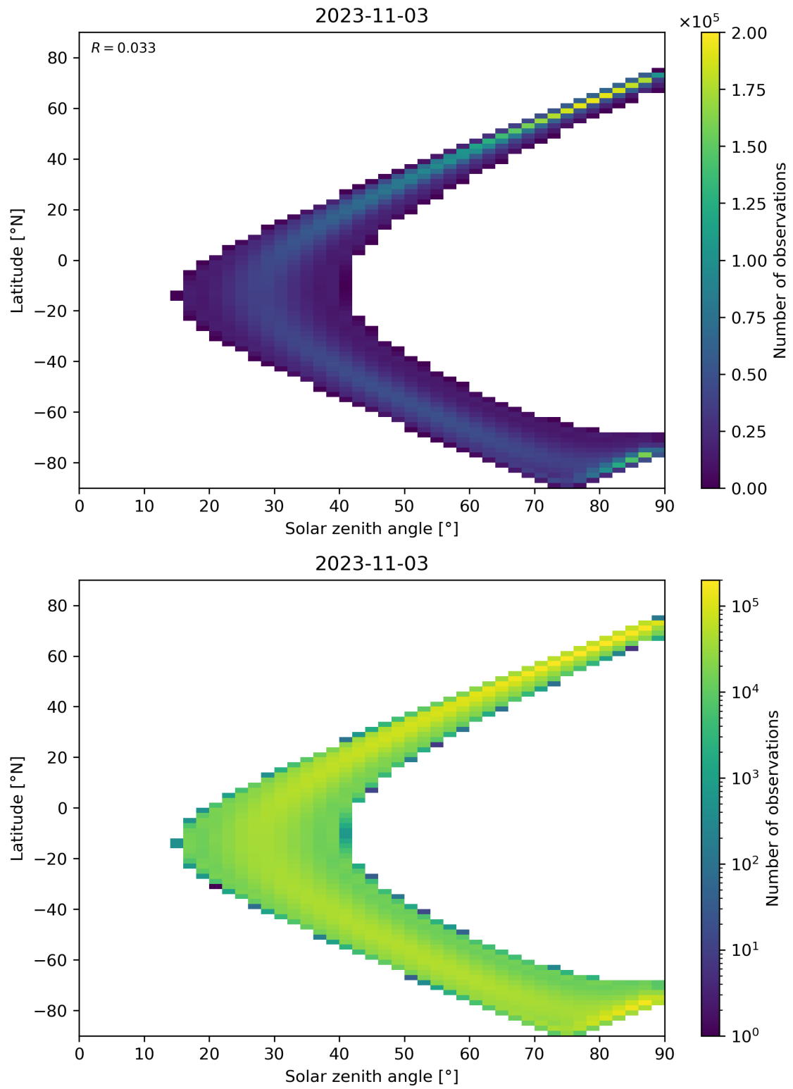
Figure 44: Scatter density plot of “Solar zenith angle” against “Latitude” for 2023-11-02 to 2023-11-04.
