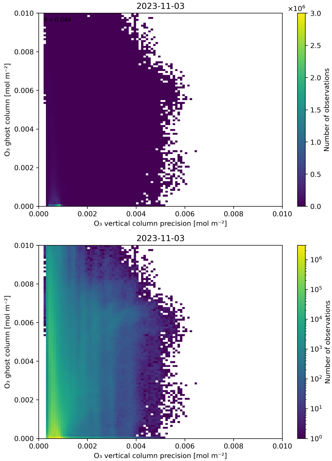
Figure 43: Scatter density plot of “ \text{O}_3 vertical column precision” against “ \text{O}_3 ghost column” for 2023-11-02 to 2023-11-04.
