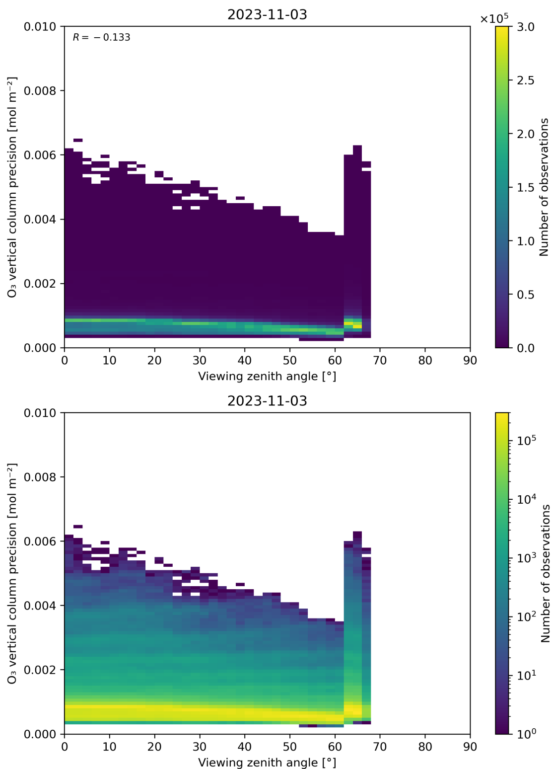
Figure 53: Scatter density plot of “Viewing zenith angle” against “O 3 vertical column precision” for 2023-11-02 to 2023-11-04.
