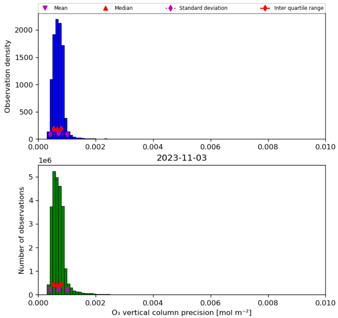
Figure 22: Histogram of “O 3 vertical column precision” for 2023-11-02 to 2023-11-04
