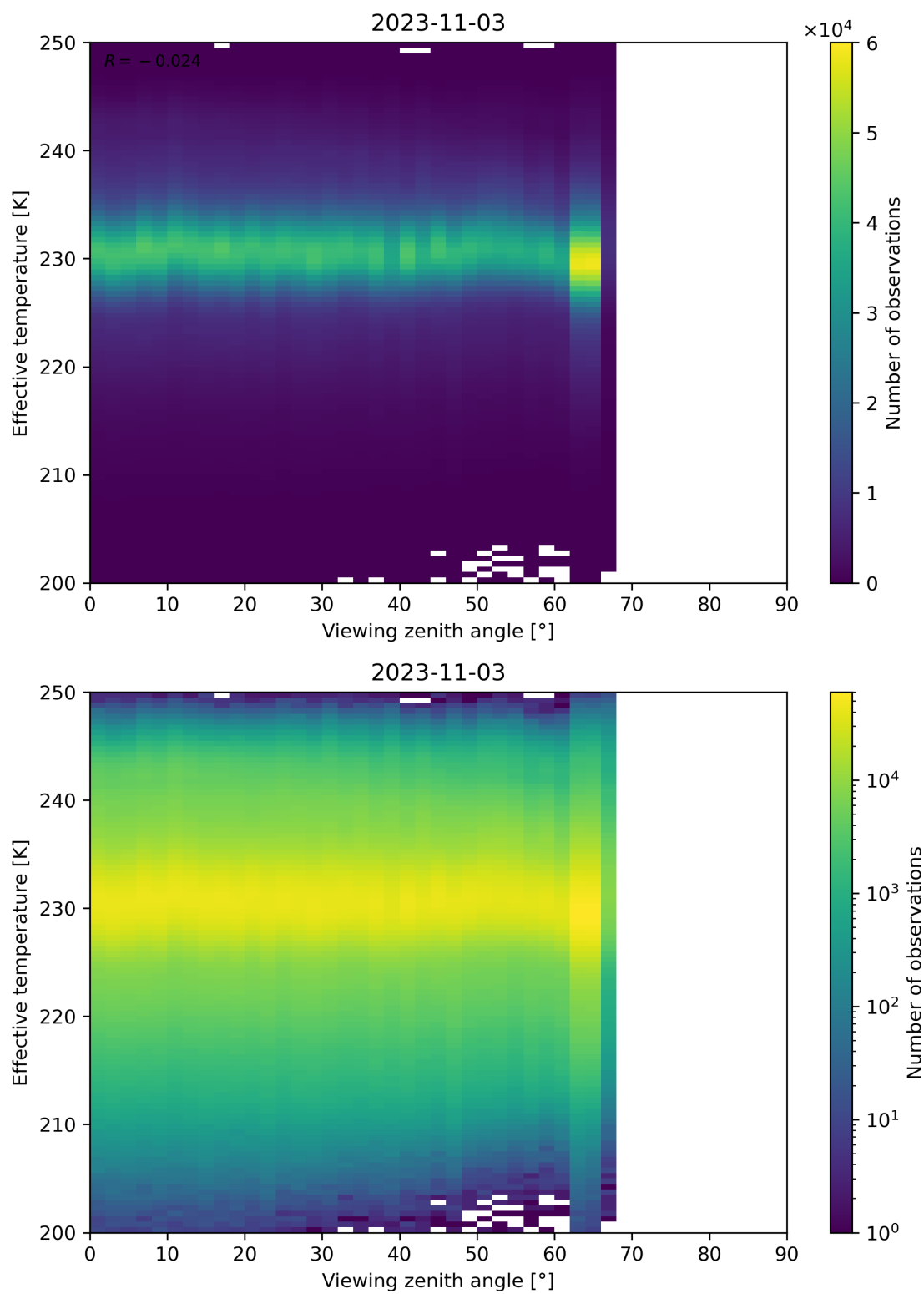
Figure 50: Scatter density plot of “Viewing zenith angle” against “Effective temperature” for 2023-11-02 to 2023-11-04.
