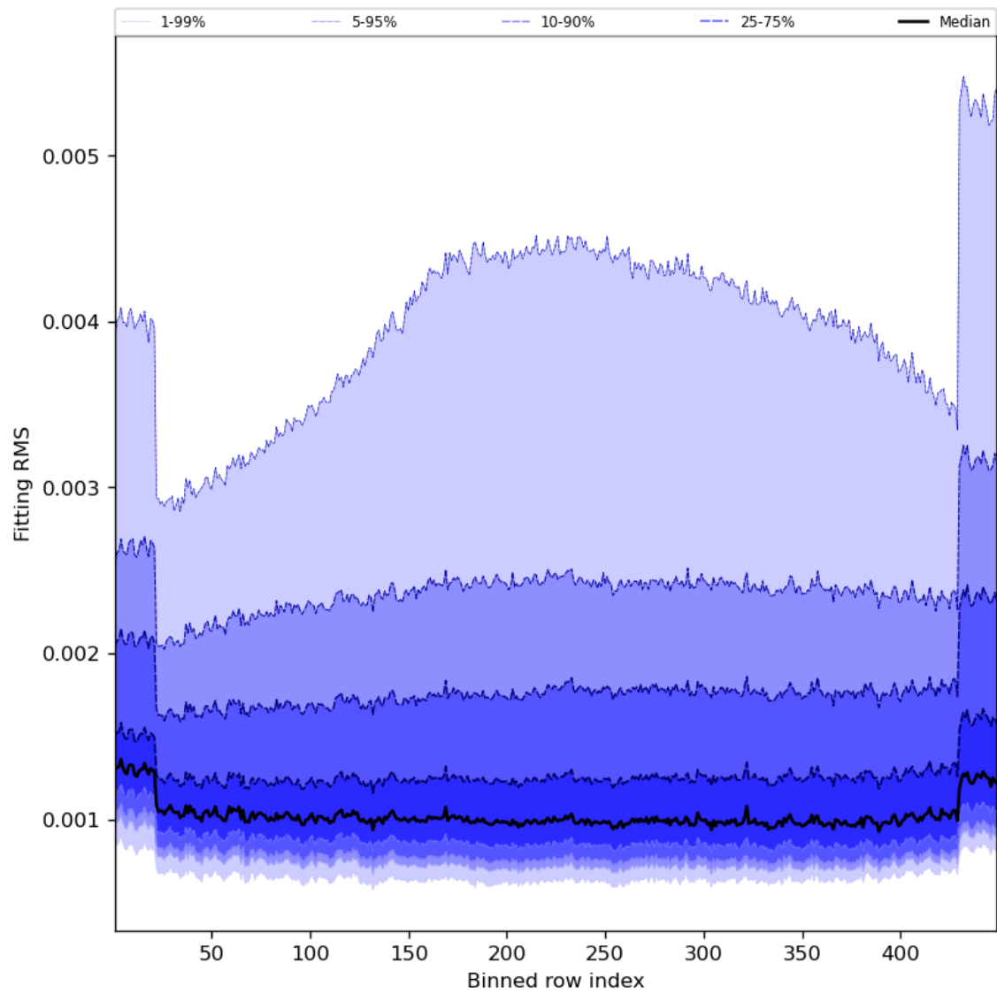
Figure 30: Along track statistics of “Fitting RMS” for 2023-11-02 to 2023-11-04
