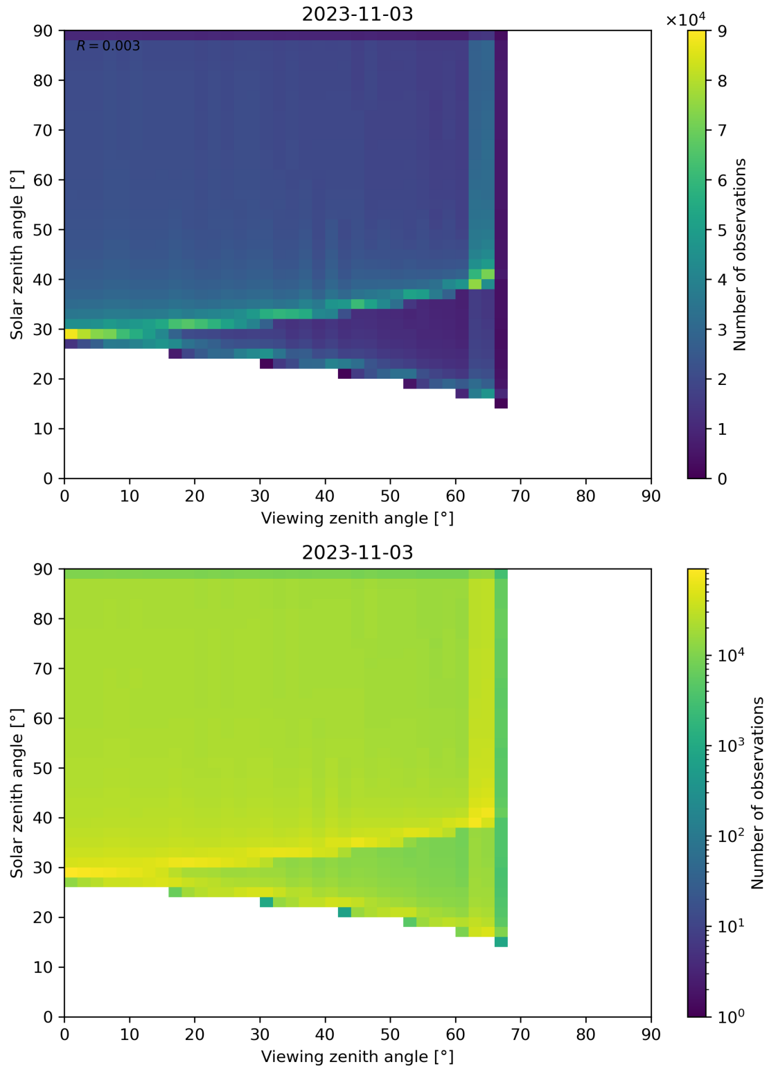
Figure 54: Scatter density plot of “Viewing zenith angle” against “Solar zenith angle” for 2023-11-02 to 2023-11-04.
