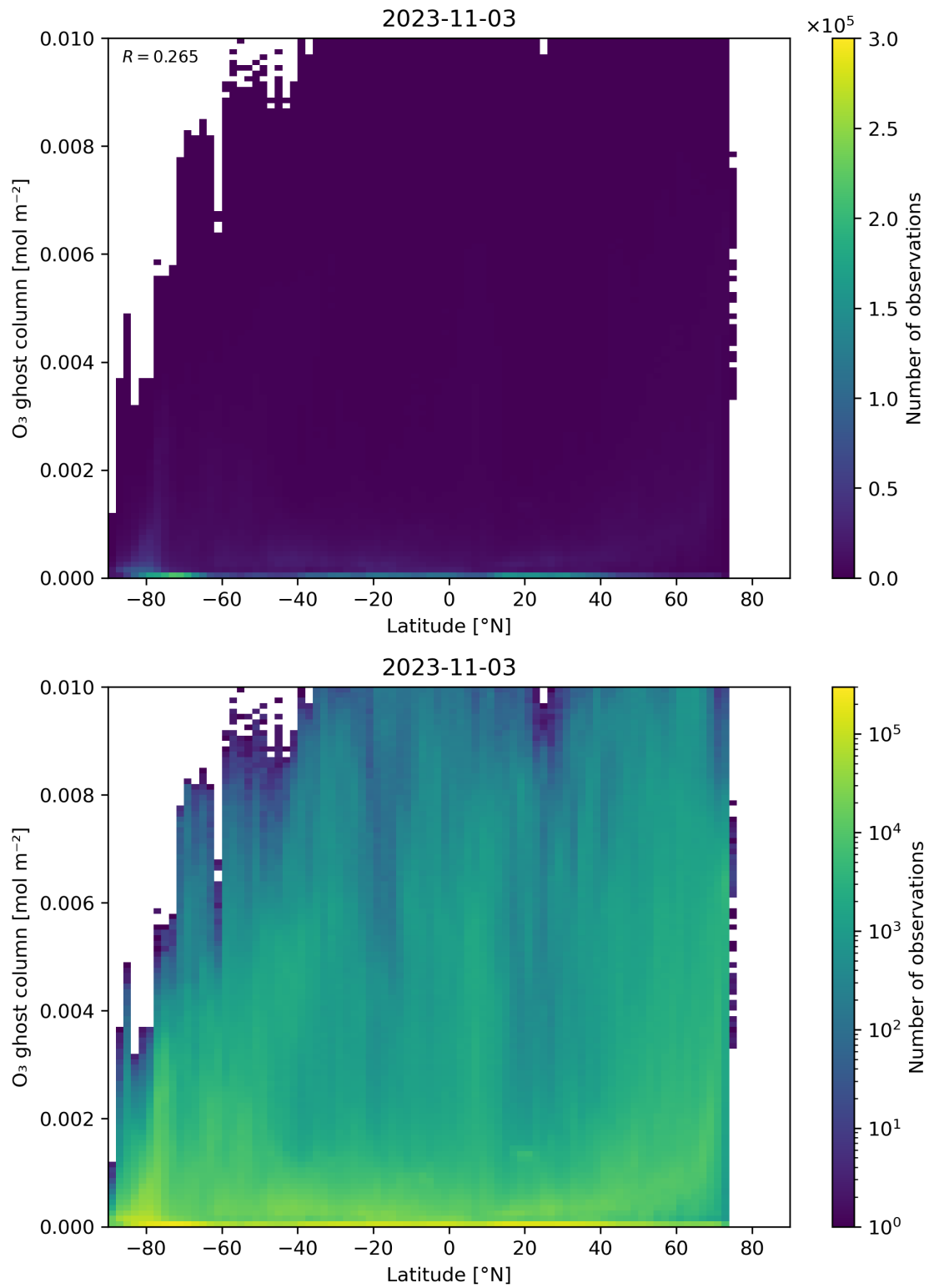
Figure 35: Scatter density plot of “Latitude” against “O 3 ghost column” for 2023-11-02 to 2023-11-04.
