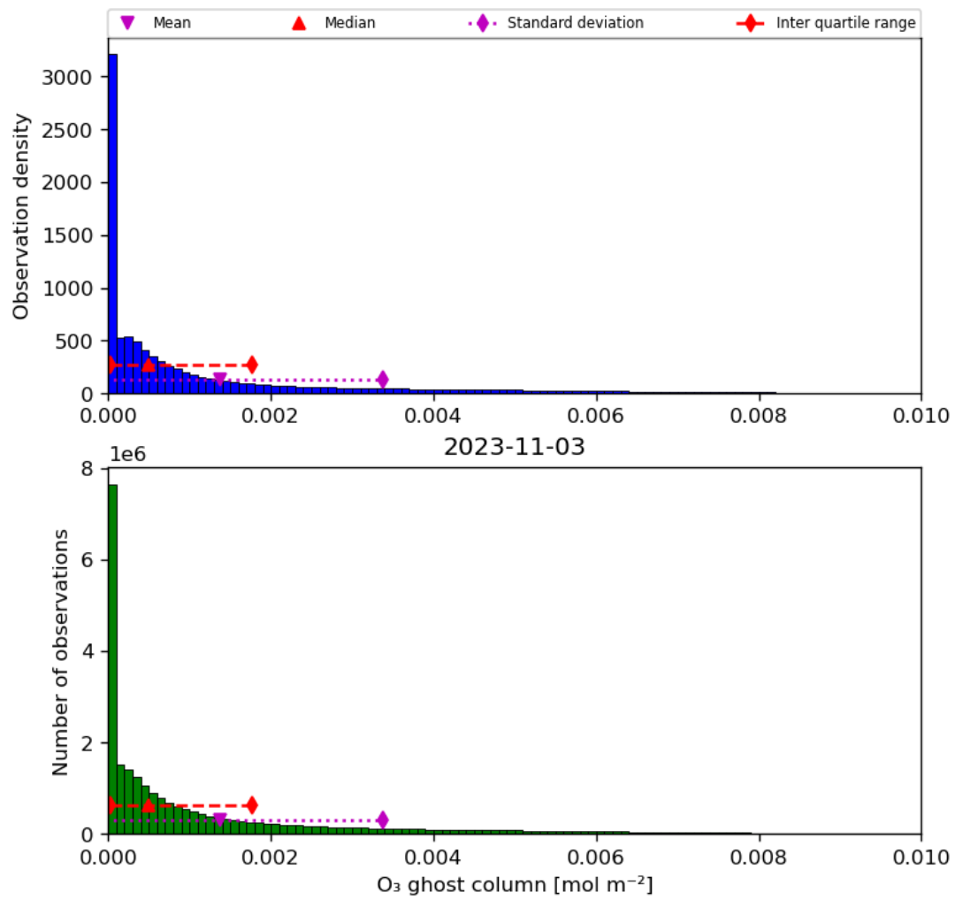
Figure 25: Histogram of “O 3 ghost column” for 2023-11-02 to 2023-11-04
