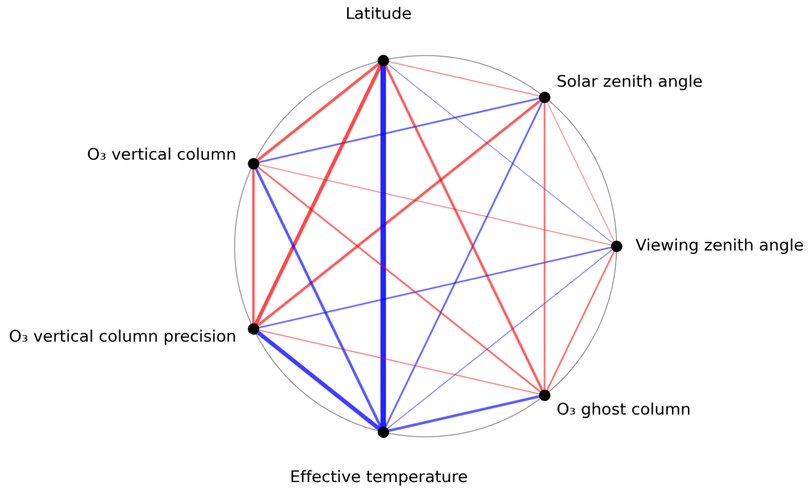
Figure 1: Map of correlation graph for 2023-11-02 to 2023-11-04.
