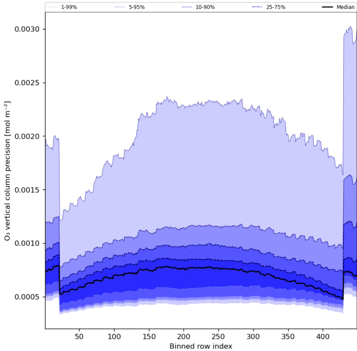
Figure 29: Along track statistics of “O 3 vertical column precision” for 2023-11-02 to 2023-11-04
