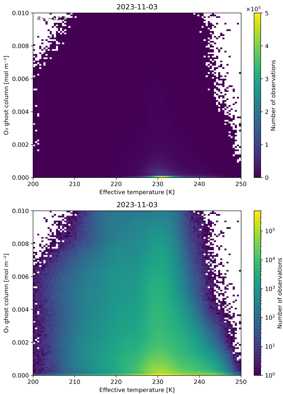
Figure 38: Scatter density plot of “Effective temperature” against “O 3 ghost column” for 2023-11-02 to 2023-11-04.
