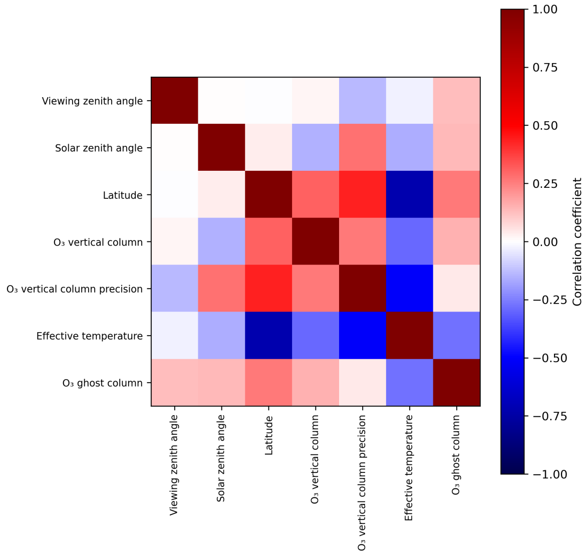
Figure 2: Map of correlation matrix for 2023-11-02 to 2023-11-04.
