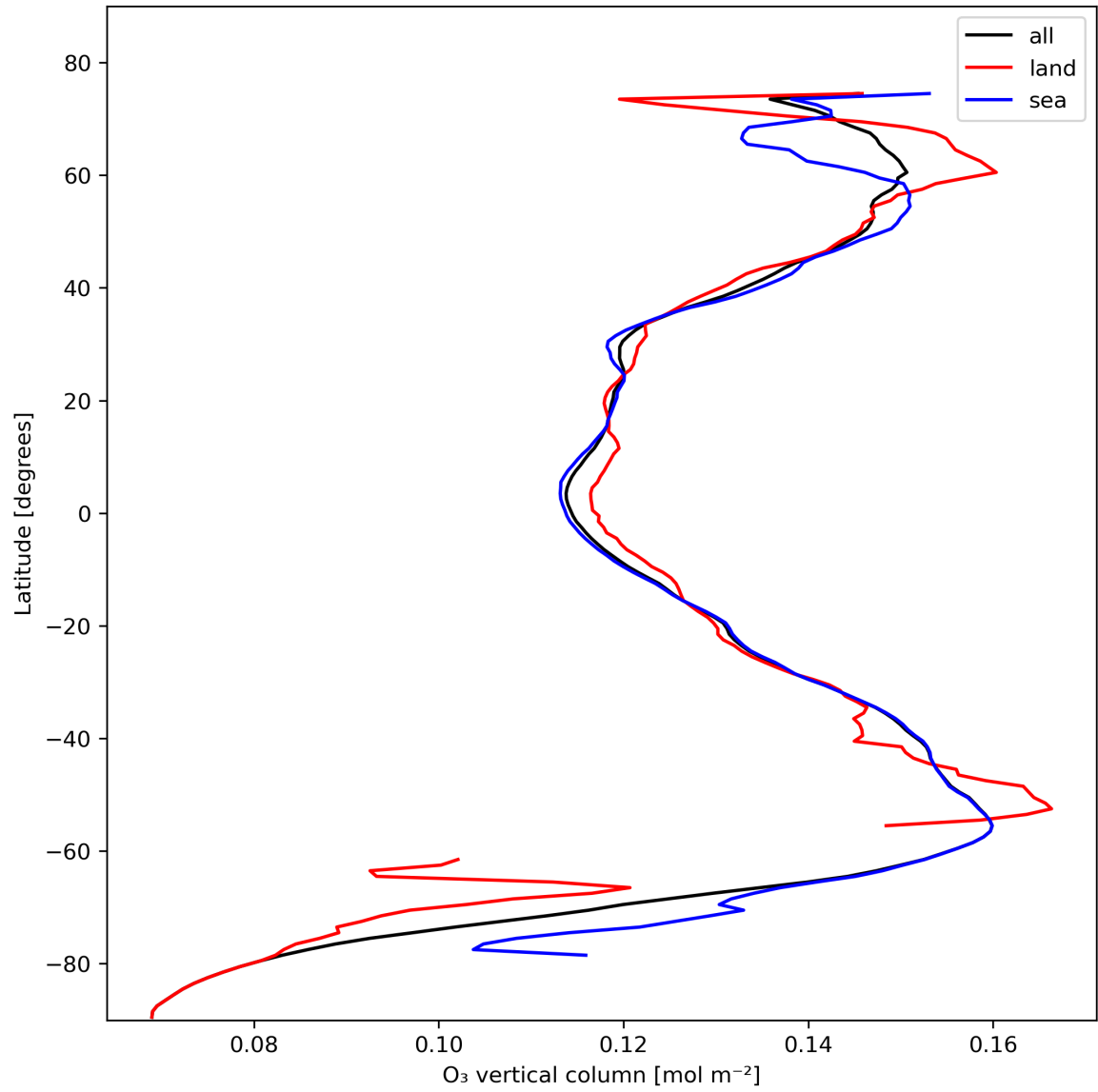
Figure 14: Zonal average of “O 3 vertical column” for 2023-11-02 to 2023-11-04.
