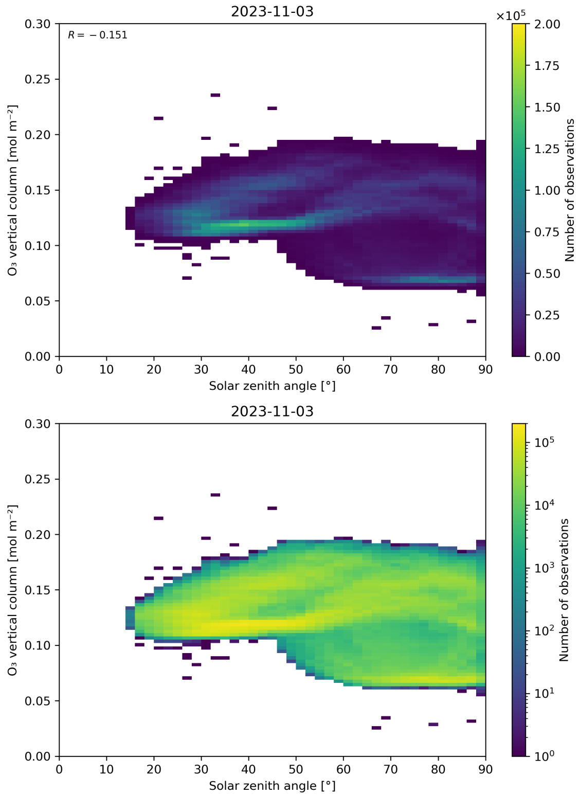
Figure 47: Scatter density plot of “Solar zenith angle” against “O 3 vertical column” for 2023-11-02 to 2023-11-04.
