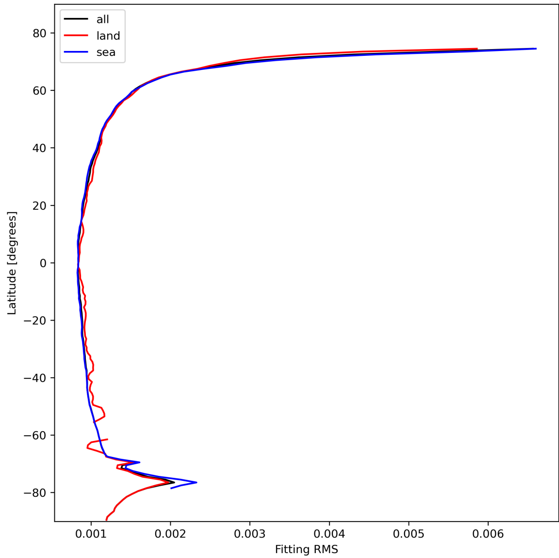
Figure 16: Zonal average of “Fitting RMS” for 2023-11-02 to 2023-11-04.
