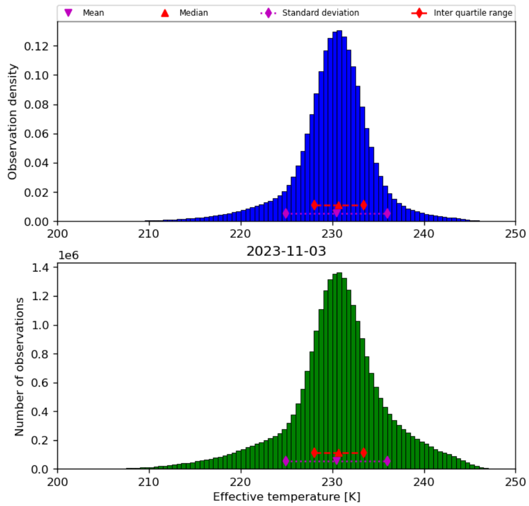
Figure 24: Histogram of “Effective temperature” for 2023-11-02 to 2023-11-04
