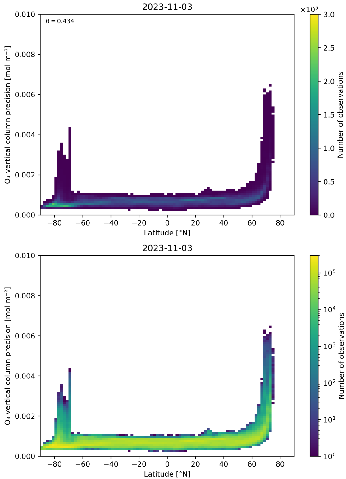
Figure 37: Scatter density plot of “Latitude” against “O 3 vertical column precision” for 2023-11-02 to 2023-11-04.
