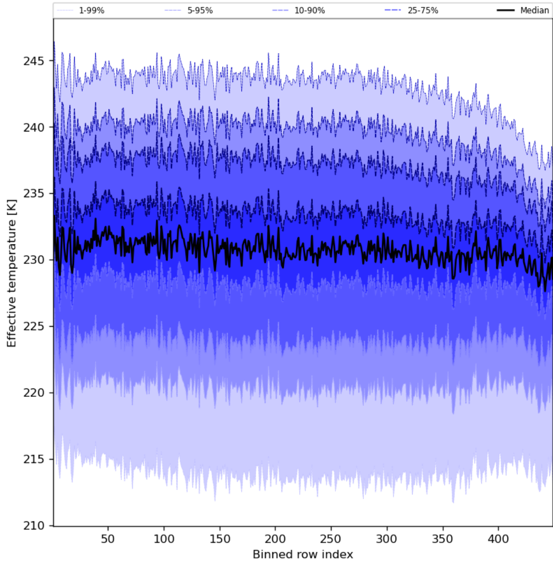
Figure 31: Along track statistics of “Effective temperature” for 2023-11-02 to 2023-11-04
