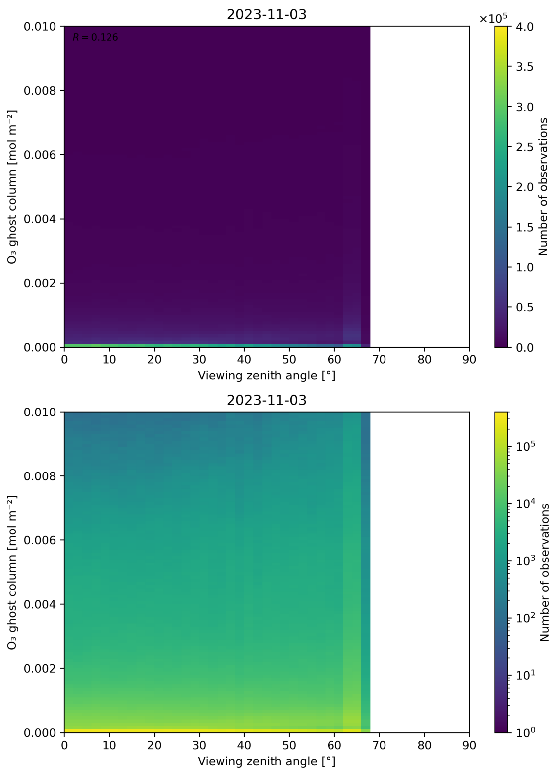
Figure 51: Scatter density plot of “Viewing zenith angle” against “O 3 ghost column” for 2023-11-02 to 2023-11-04.
