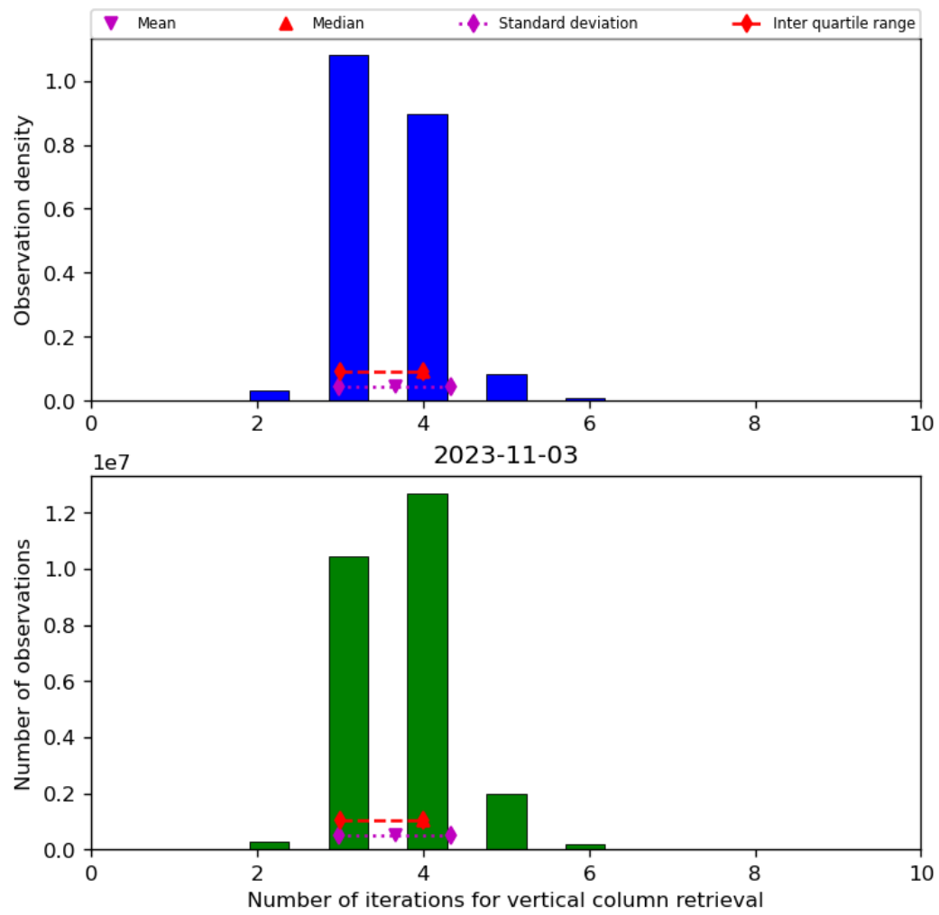
Figure 26: Histogram of “Number of iterations for vertical column retrieval” for 2023-11-02 to 2023-11-04
