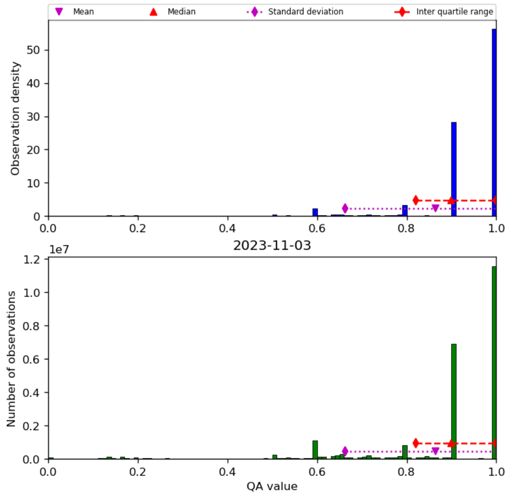
Figure 20: Histogram of “QA value” for 2023-11-02 to 2023-11-04
