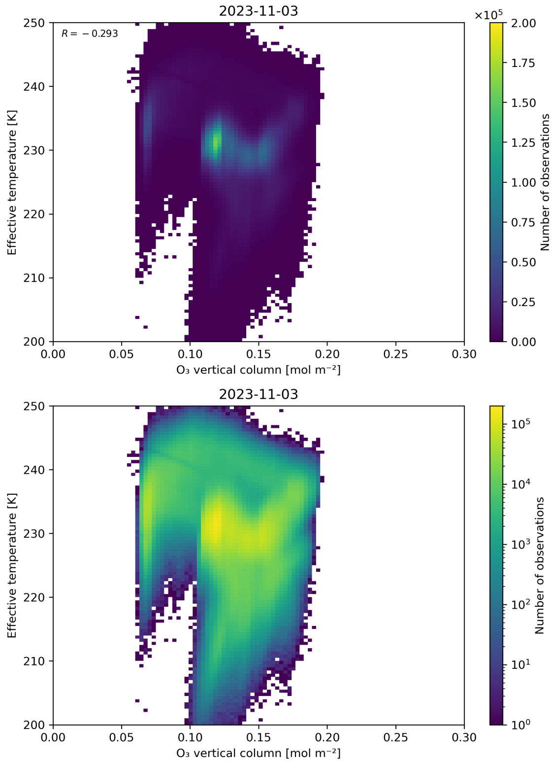
Figure 39: Scatter density plot of “O 3 vertical column” against “Effective temperature” for 2023-11-02 to 2023-11-04.
