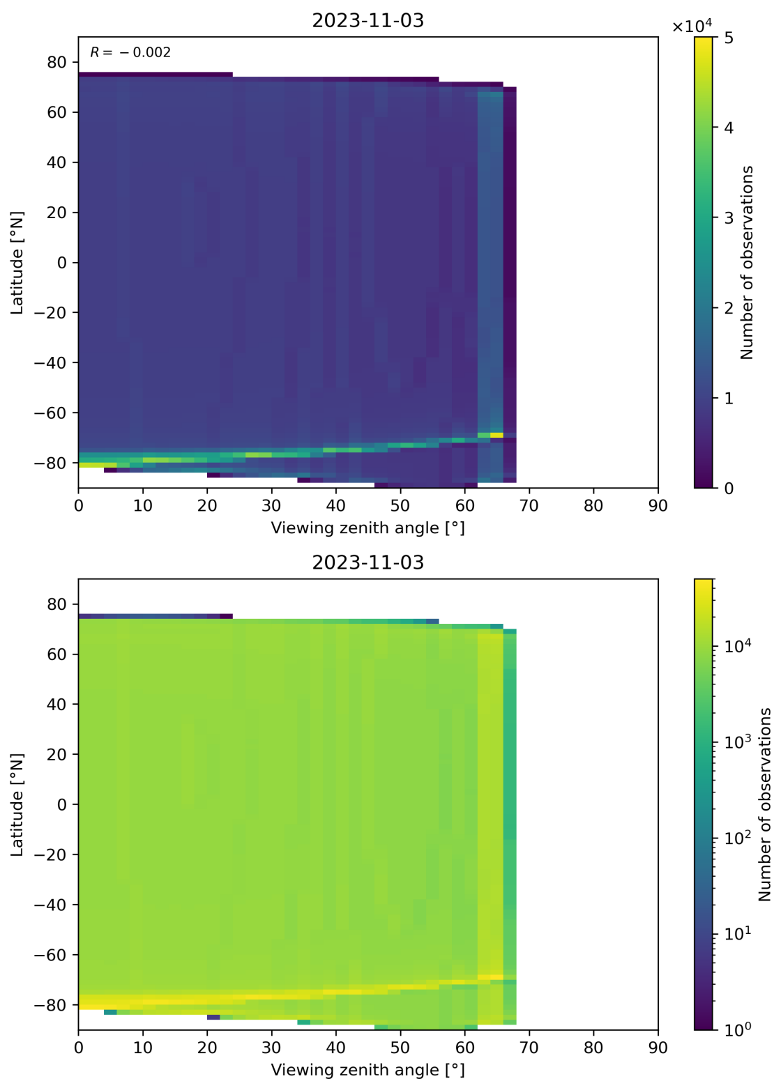
Figure 49: Scatter density plot of “Viewing zenith angle” against “Latitude” for 2023-11-02 to 2023-11-04.
