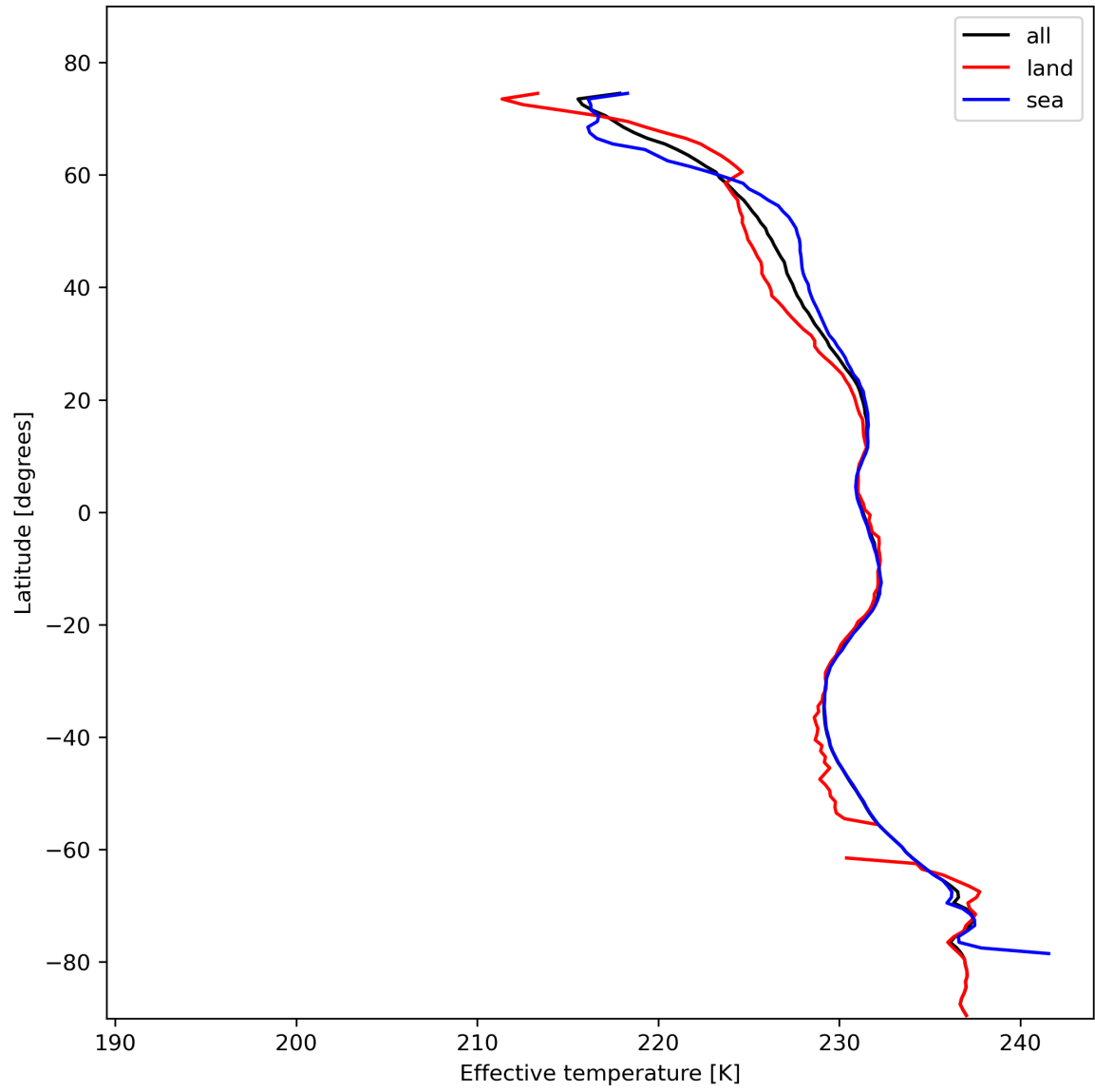
Figure 17: Zonal average of "Effective temperature" for 2023-11-02 to 2023-11-04.
