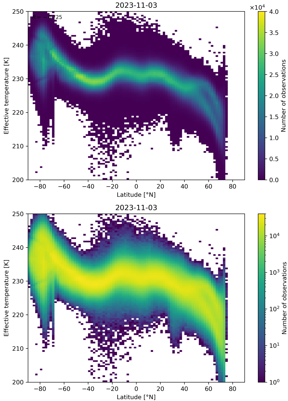
Figure 34: Scatter density plot of “Latitude” against “Effective temperature” for 2023-11-02 to 2023-11-04.
