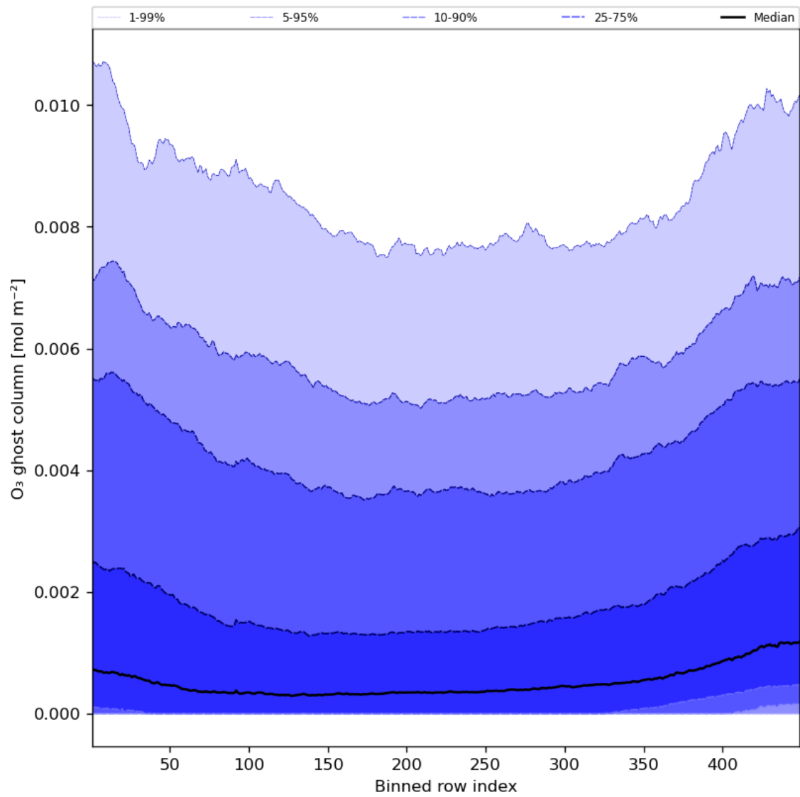
Figure 32: Along track statistics of “O 3 ghost column” for 2023-11-02 to 2023-11-04
