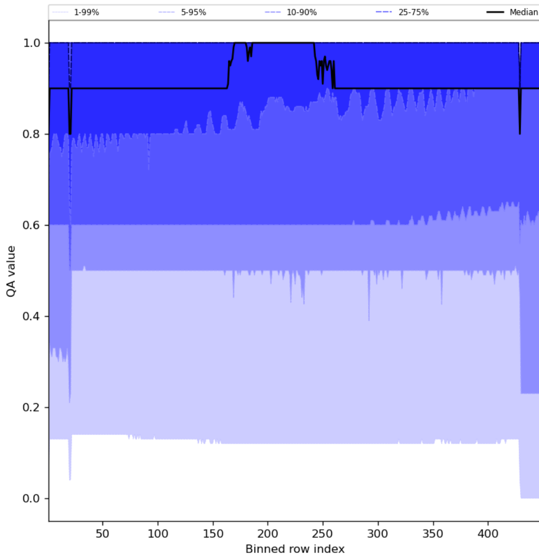
Figure 27: Along track statistics of “QA value” for 2023-11-02 to 2023-11-04
