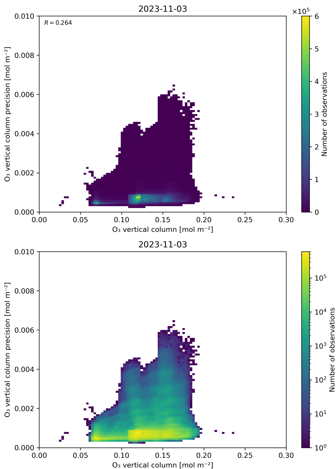
Figure 41: Scatter density plot of “O 3 vertical column” against “O 3 vertical column precision” for 2023-11-02 to 2023-11-04.
