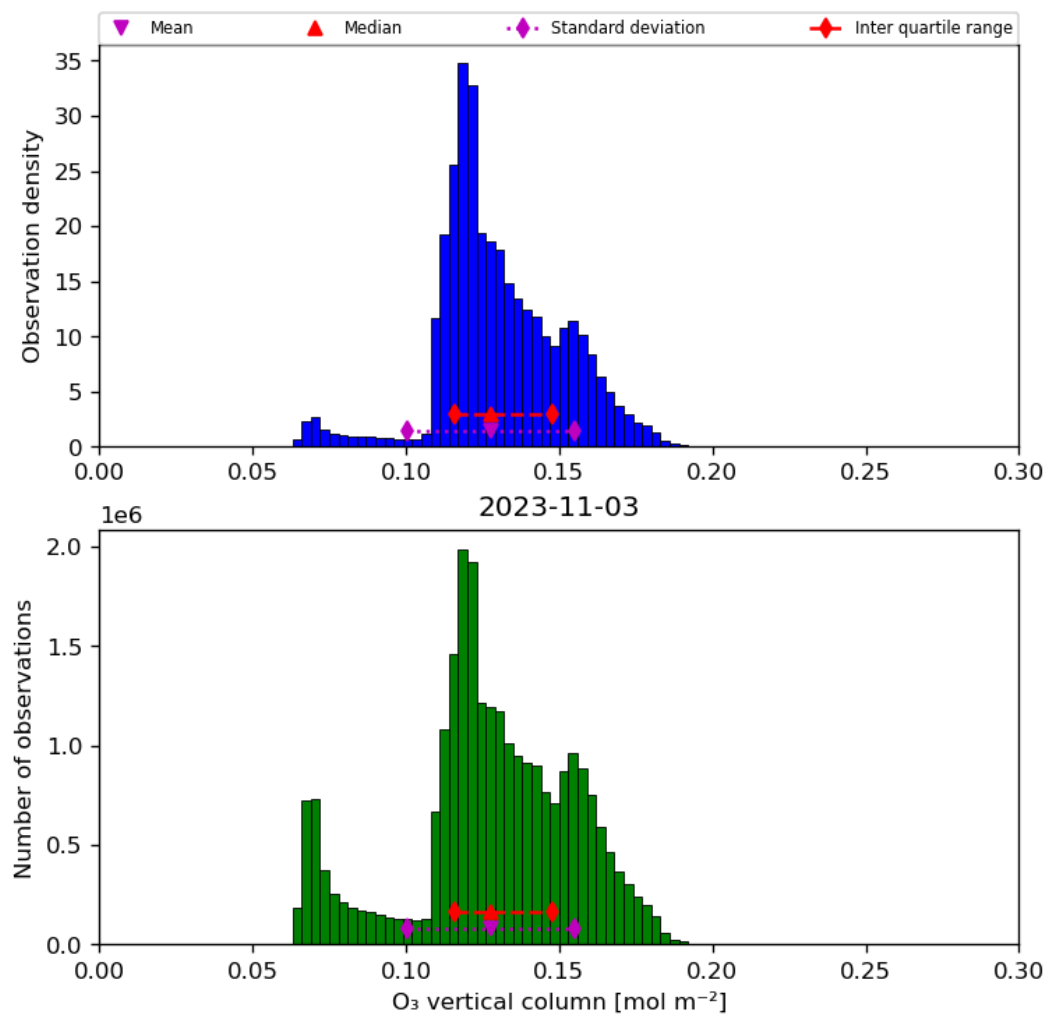
Figure 21: Histogram of “O 3 vertical column” for 2023-11-02 to 2023-11-04
