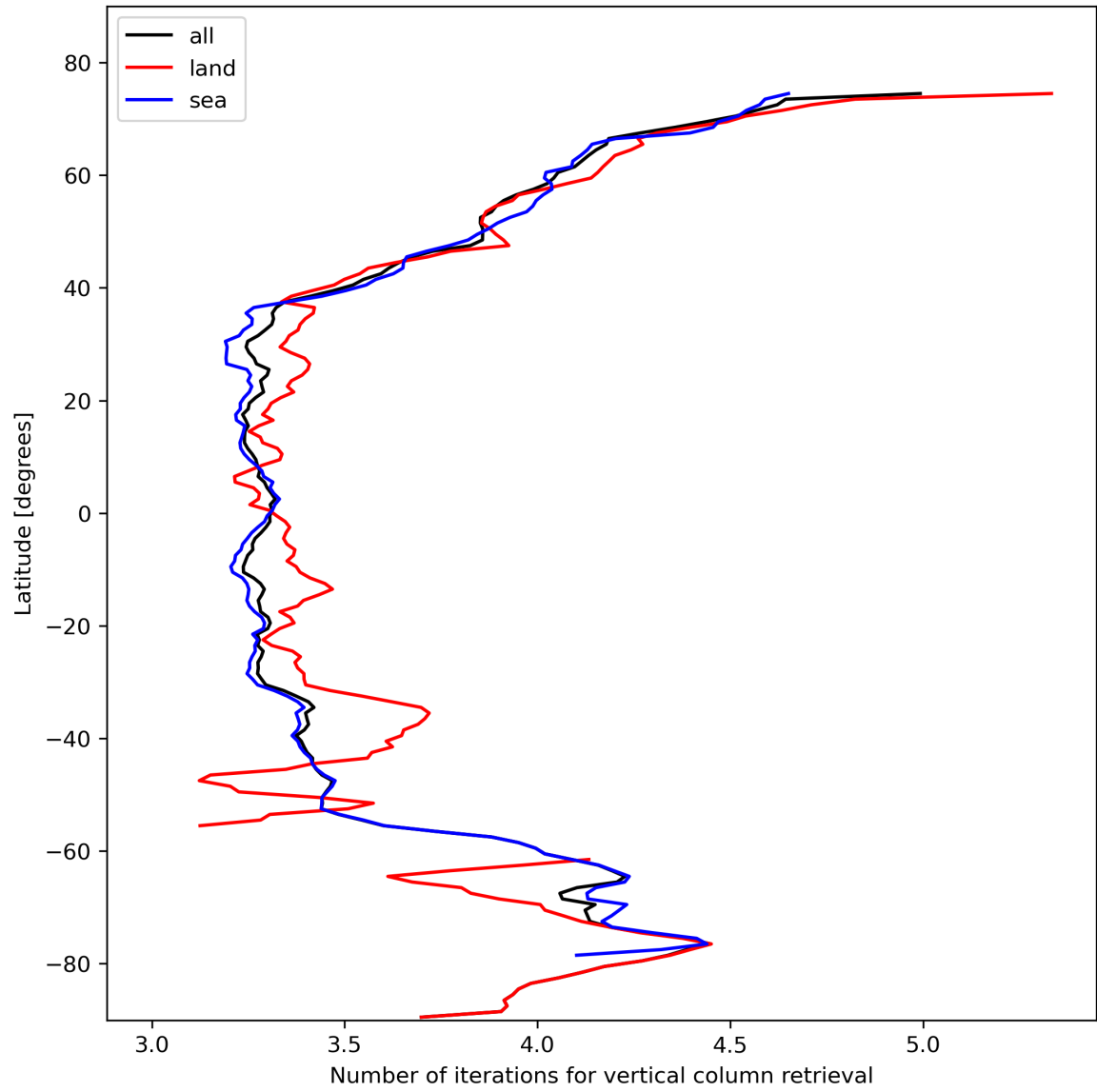
Figure 19: Zonal average of “Number of iterations for vertical column retrieval” for 2023-11-02 to 2023-11-04.
