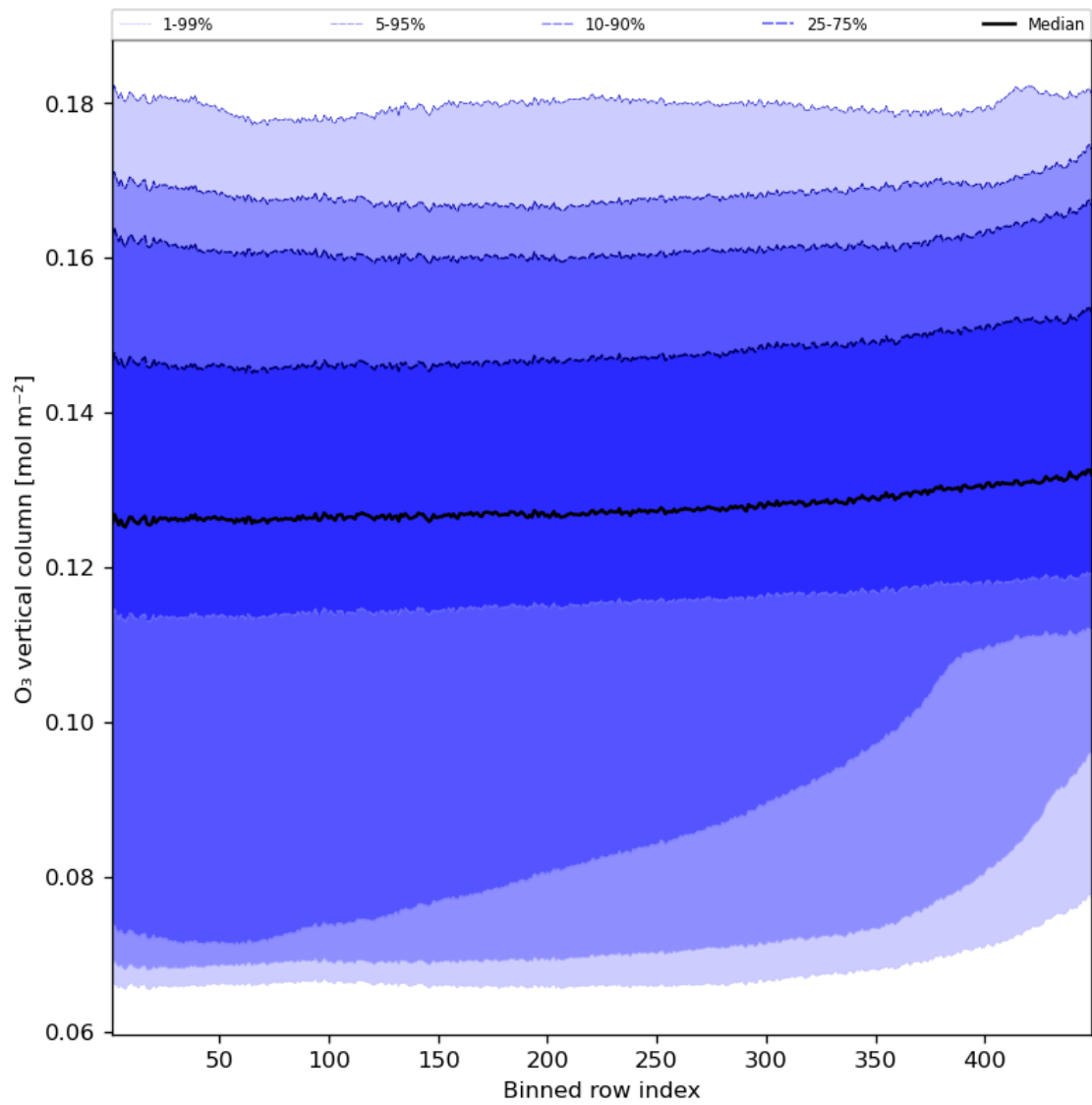
Figure 28: Along track statistics of “O 3 vertical column” for 2023-11-02 to 2023-11-04
