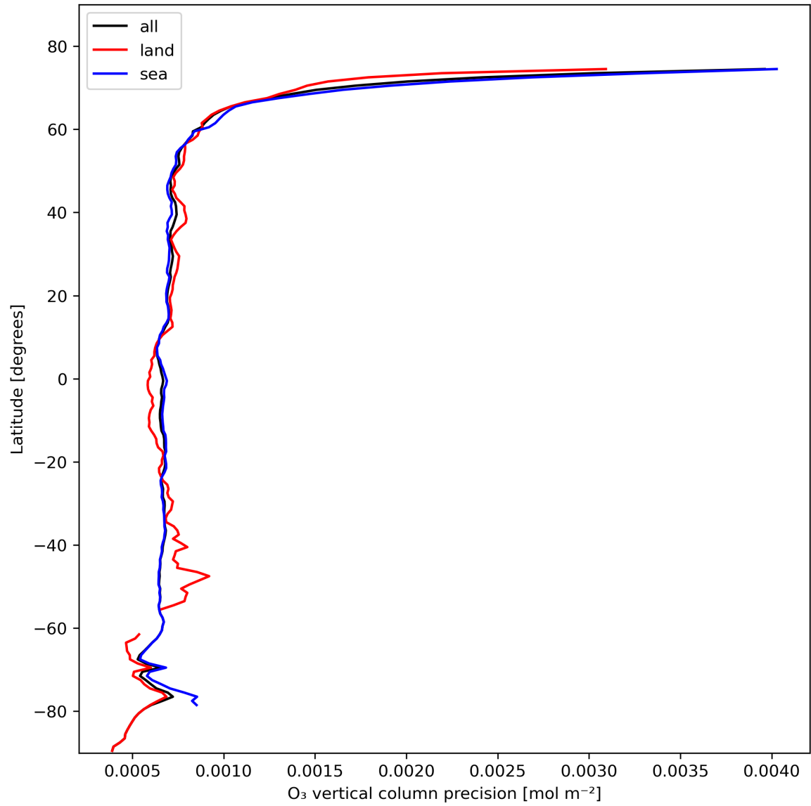
Figure 15: Zonal average of “O 3 vertical column precision” for 2023-11-02 to 2023-11-04.
