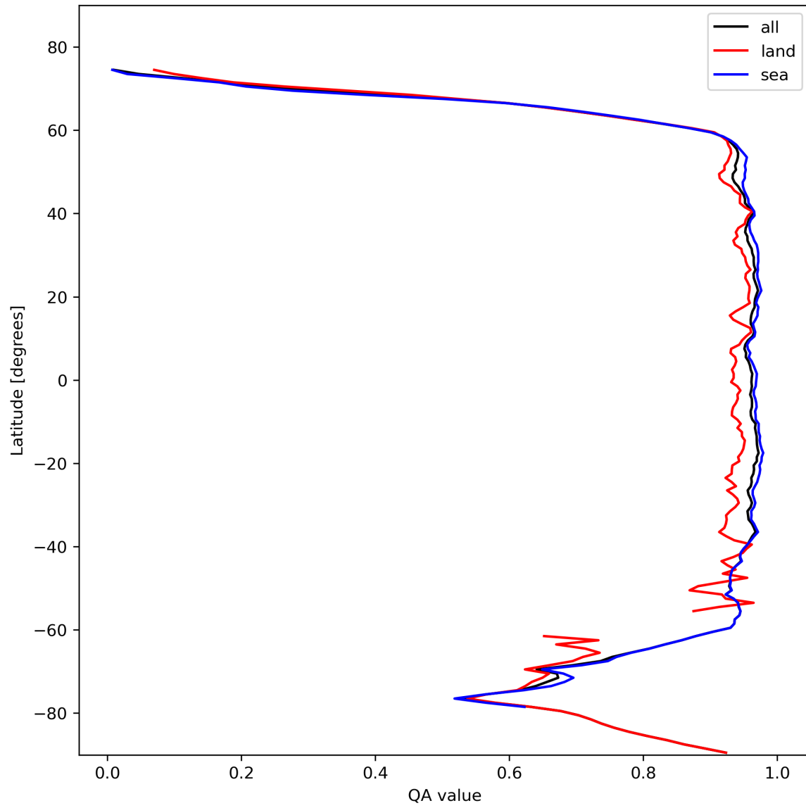
Figure 13: Zonal average of “QA value” for 2023-11-02 to 2023-11-04.
