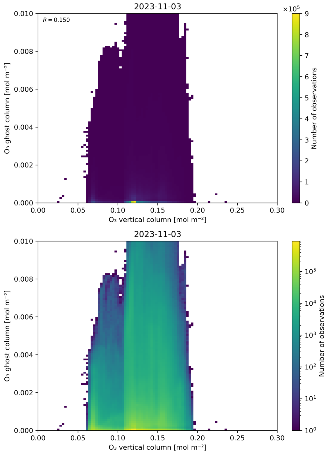
Figure 40: Scatter density plot of “O 3 vertical column” against “O 3 ghost column” for 2023-11-02 to 2023-11-04.
