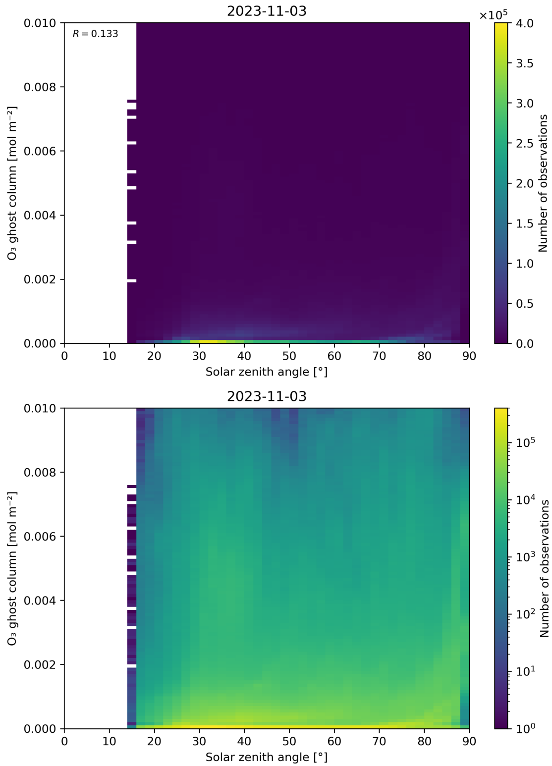
Figure 46: Scatter density plot of “Solar zenith angle” against “O 3 ghost column” for 2023-11-02 to 2023-11-04.
