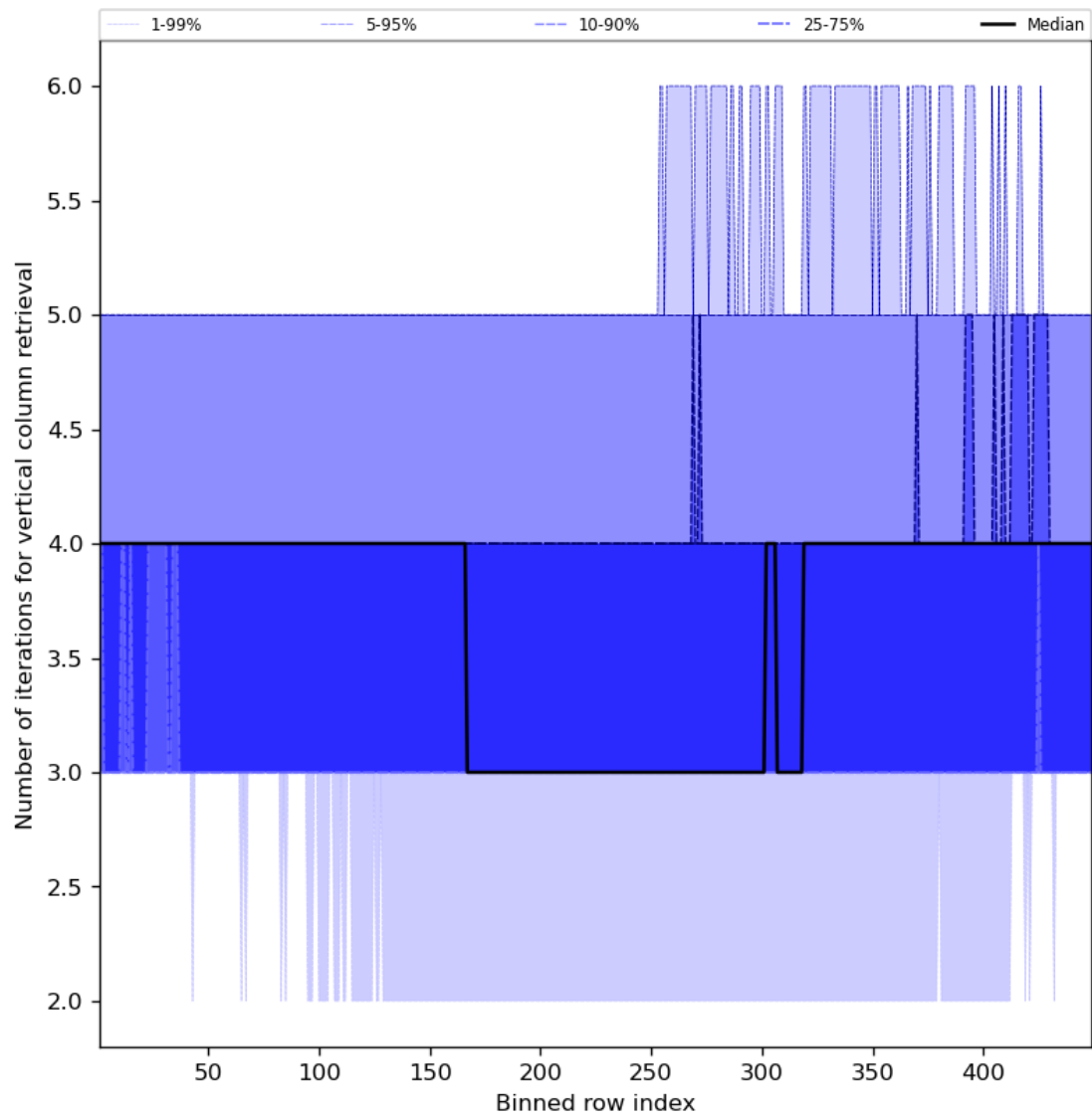
Figure 33: Along track statistics of “Number of iterations for vertical column retrieval” for 2023-11-02 to 2023-11-04
