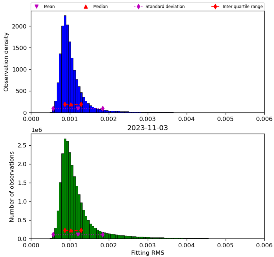
Figure 23: Histogram of “Fitting RMS” for 2023-11-02 to 2023-11-04
