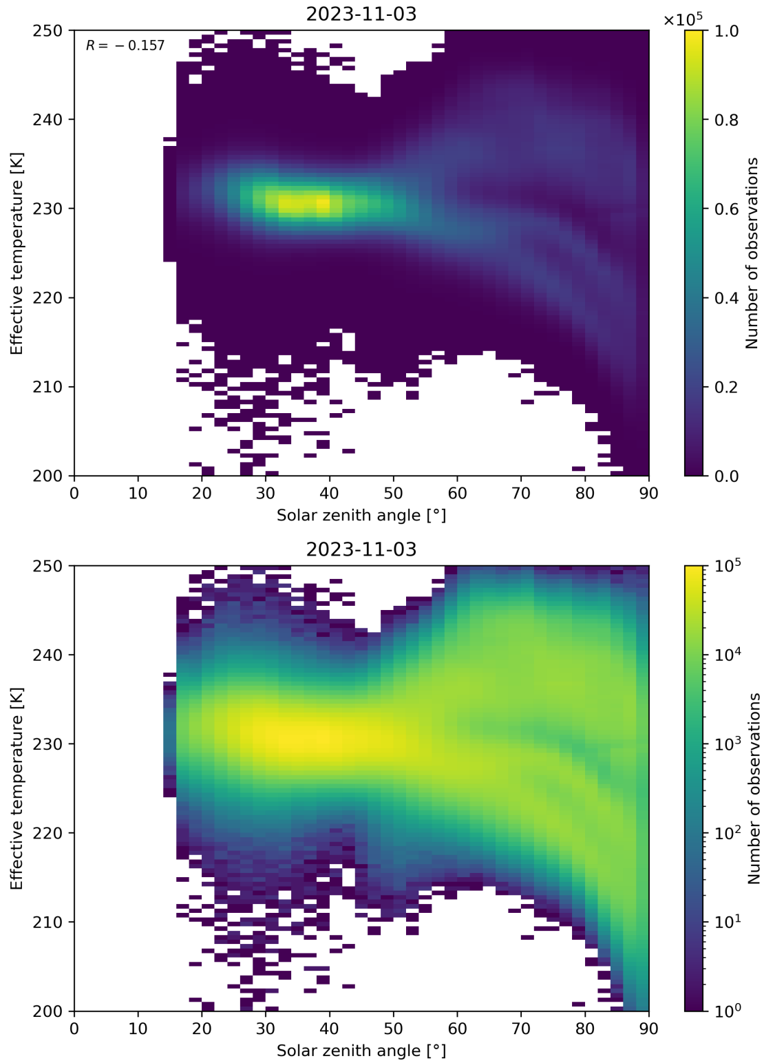
Figure 45: Scatter density plot of “Solar zenith angle” against “Effective temperature” for 2023-11-02 to 2023-11-04.
