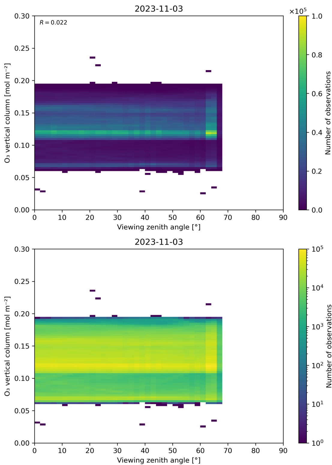
Figure 52: Scatter density plot of “Viewing zenith angle” against “O 3 vertical column” for 2023-11-02 to 2023-11-04.
