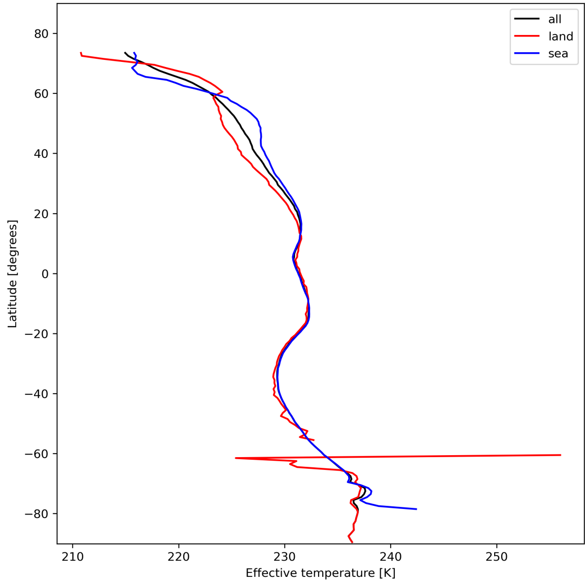
Figure 17: Zonal average of "Effective temperature" for 2023-11-03 to 2023-11-05.
