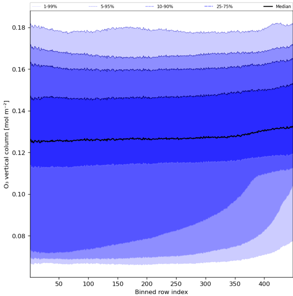
Figure 28: Along track statistics of “O 3 vertical column” for 2023-11-03 to 2023-11-05
