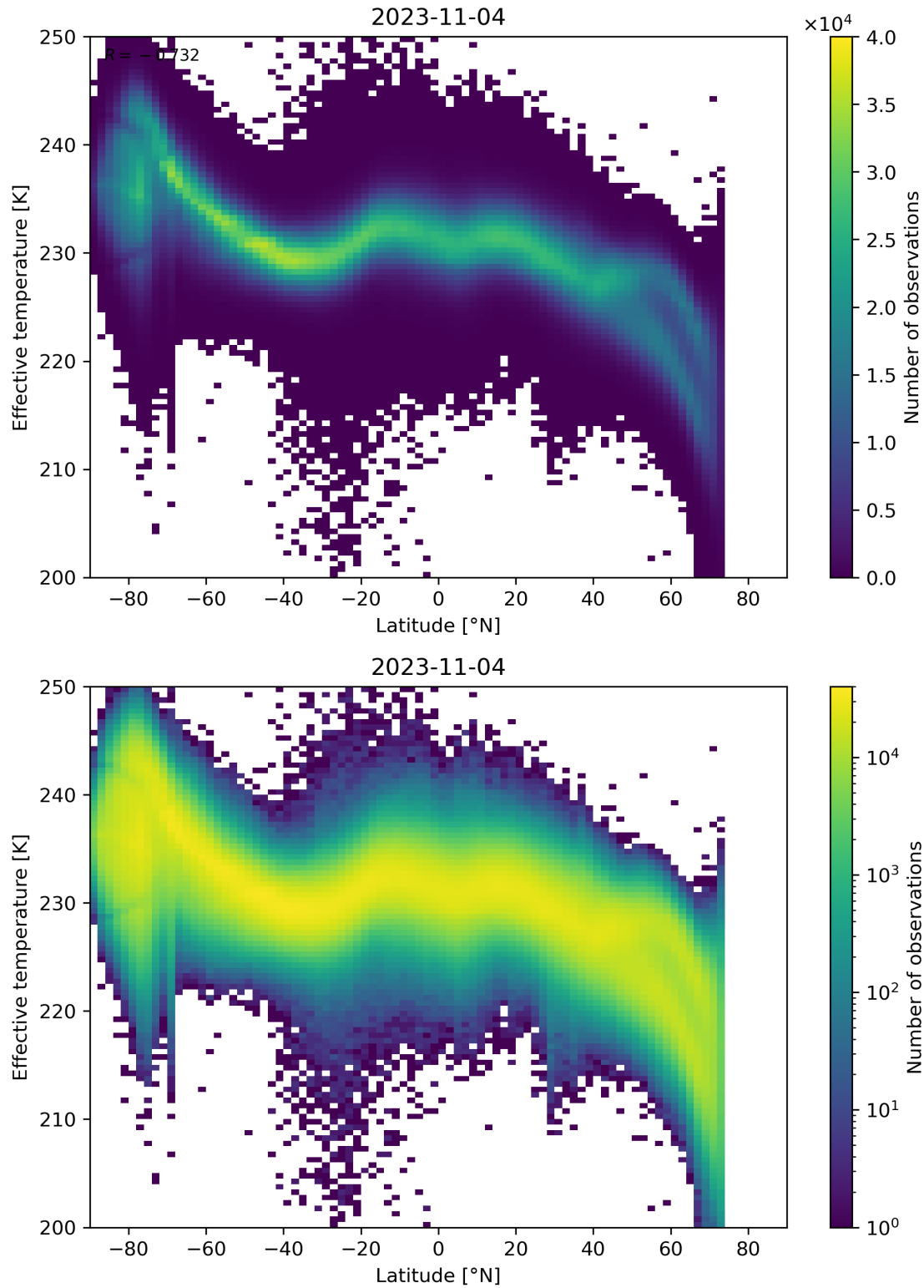
Figure 34: Scatter density plot of “Latitude” against “Effective temperature” for 2023-11-03 to 2023-11-05.
