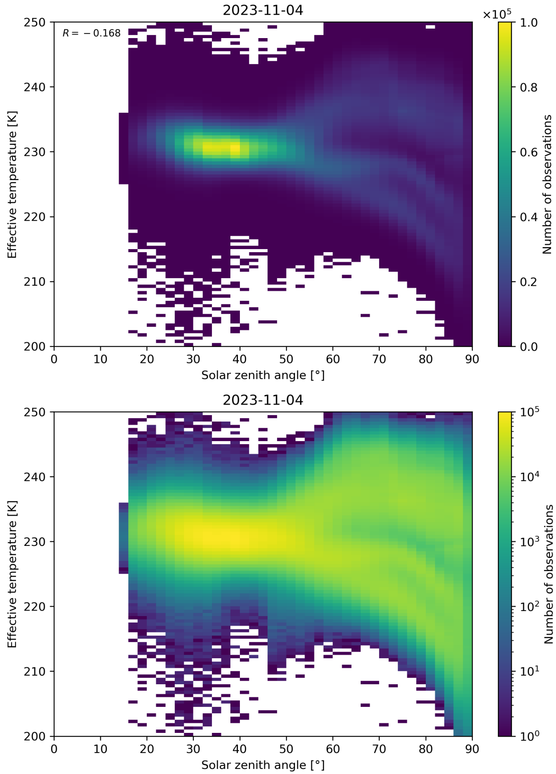
Figure 45: Scatter density plot of “Solar zenith angle” against “Effective temperature” for 2023-11-03 to 2023-11-05.
