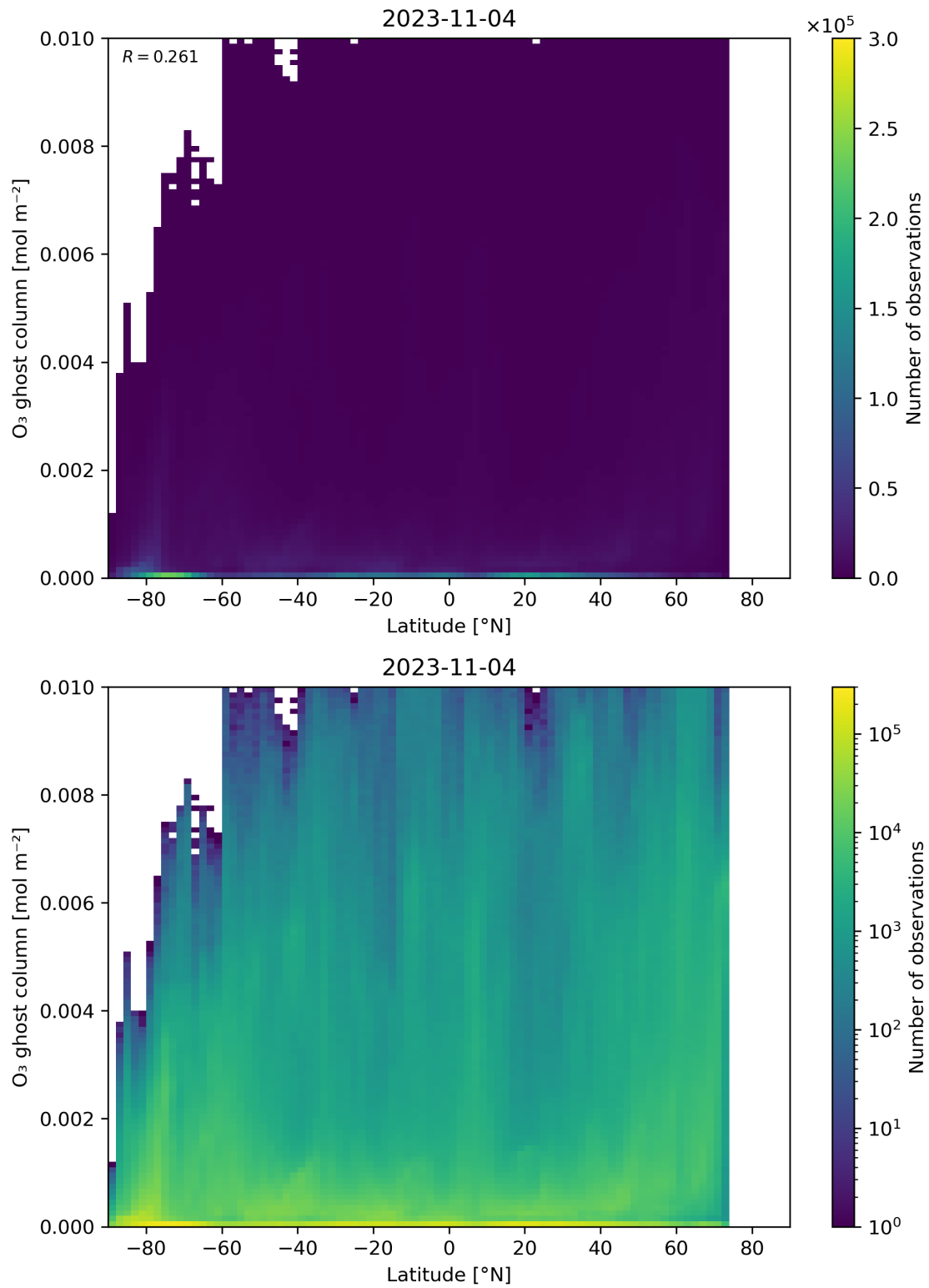
Figure 35: Scatter density plot of “Latitude” against “O 3 ghost column” for 2023-11-03 to 2023-11-05.
