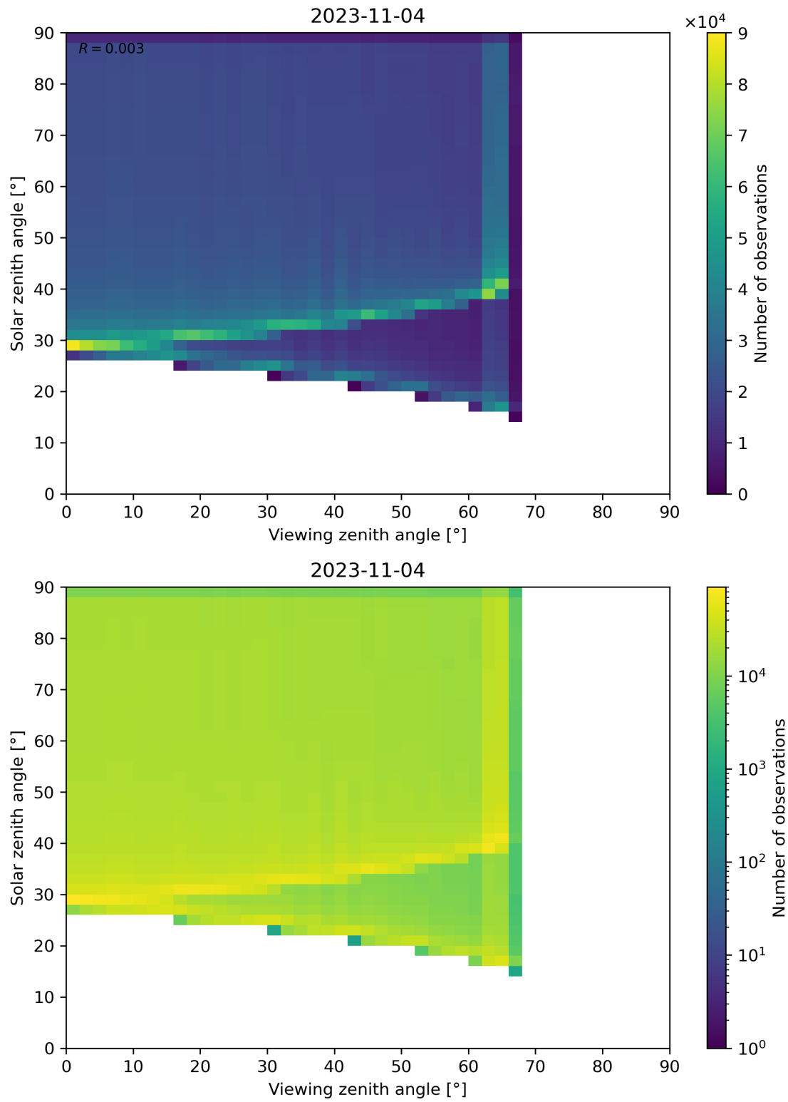
Figure 54: Scatter density plot of “Viewing zenith angle” against “Solar zenith angle” for 2023-11-03 to 2023-11-05.
