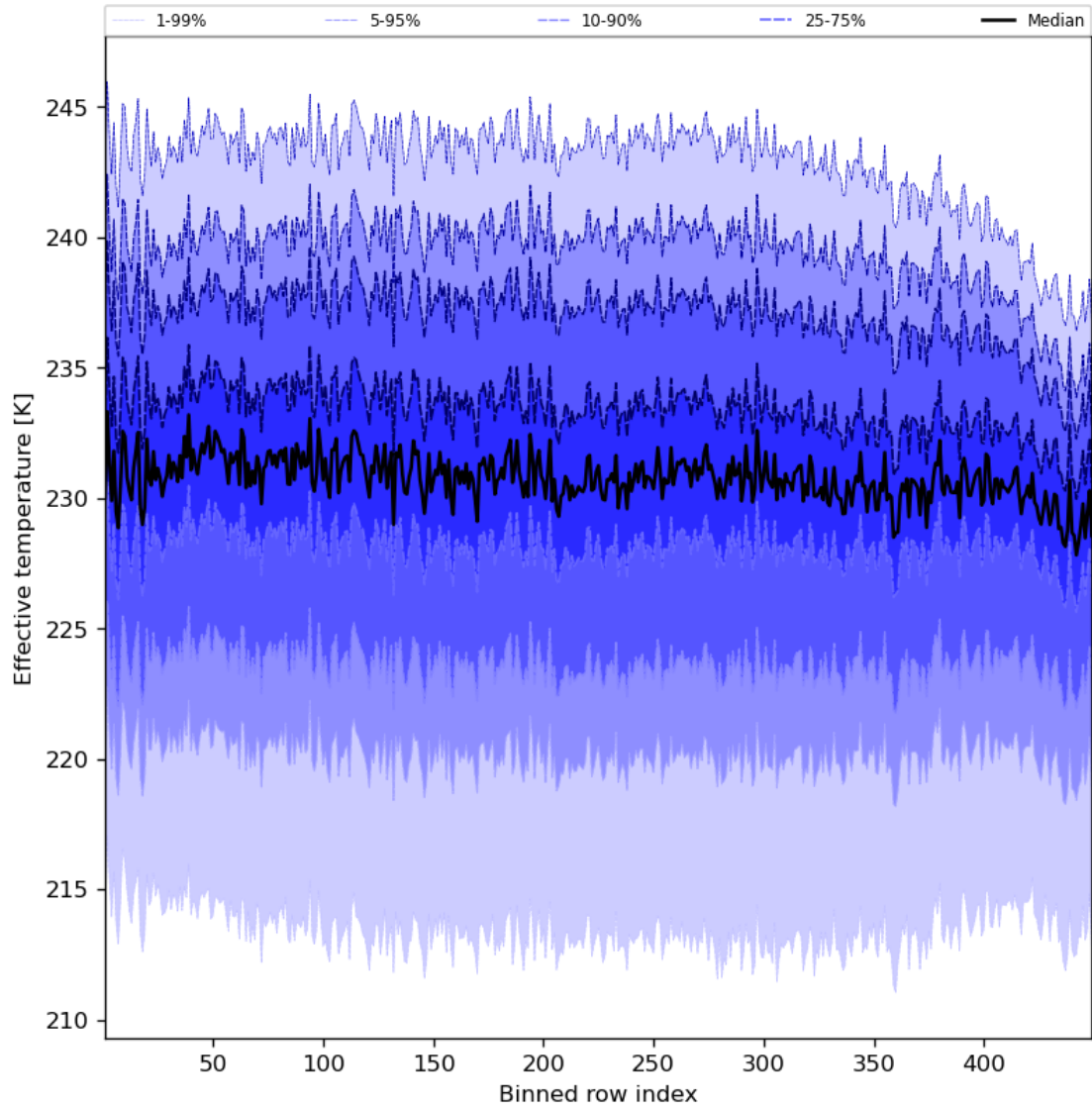
Figure 31: Along track statistics of “Effective temperature” for 2023-11-03 to 2023-11-05
