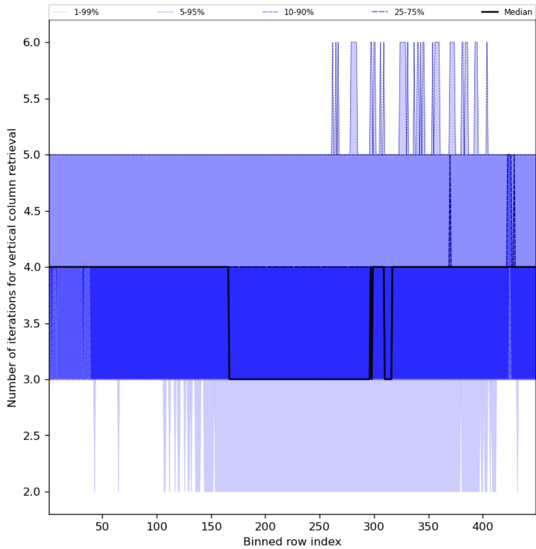
Figure 33: Along track statistics of “Number of iterations for vertical column retrieval” for 2023-11-03 to 2023-11-05
