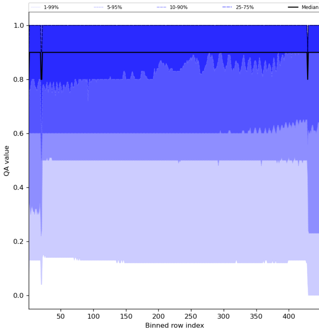
Figure 27: Along track statistics of “QA value” for 2023-11-03 to 2023-11-05
