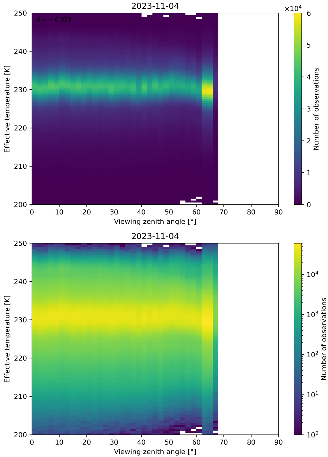
Figure 50: Scatter density plot of “Viewing zenith angle” against “Effective temperature” for 2023-11-03 to 2023-11-05.
