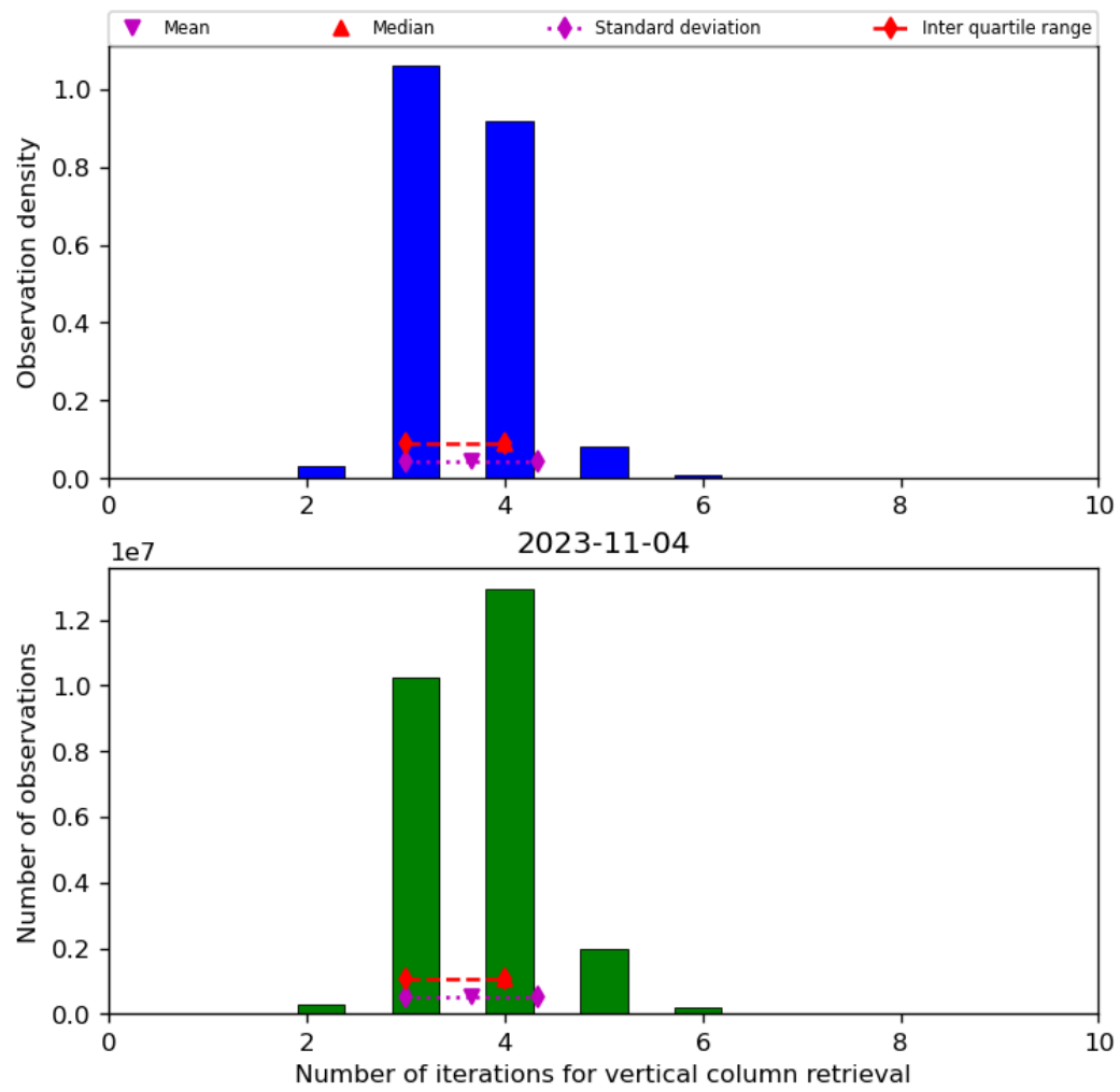
Figure 26: Histogram of “Number of iterations for vertical column retrieval” for 2023-11-03 to 2023-11-05
