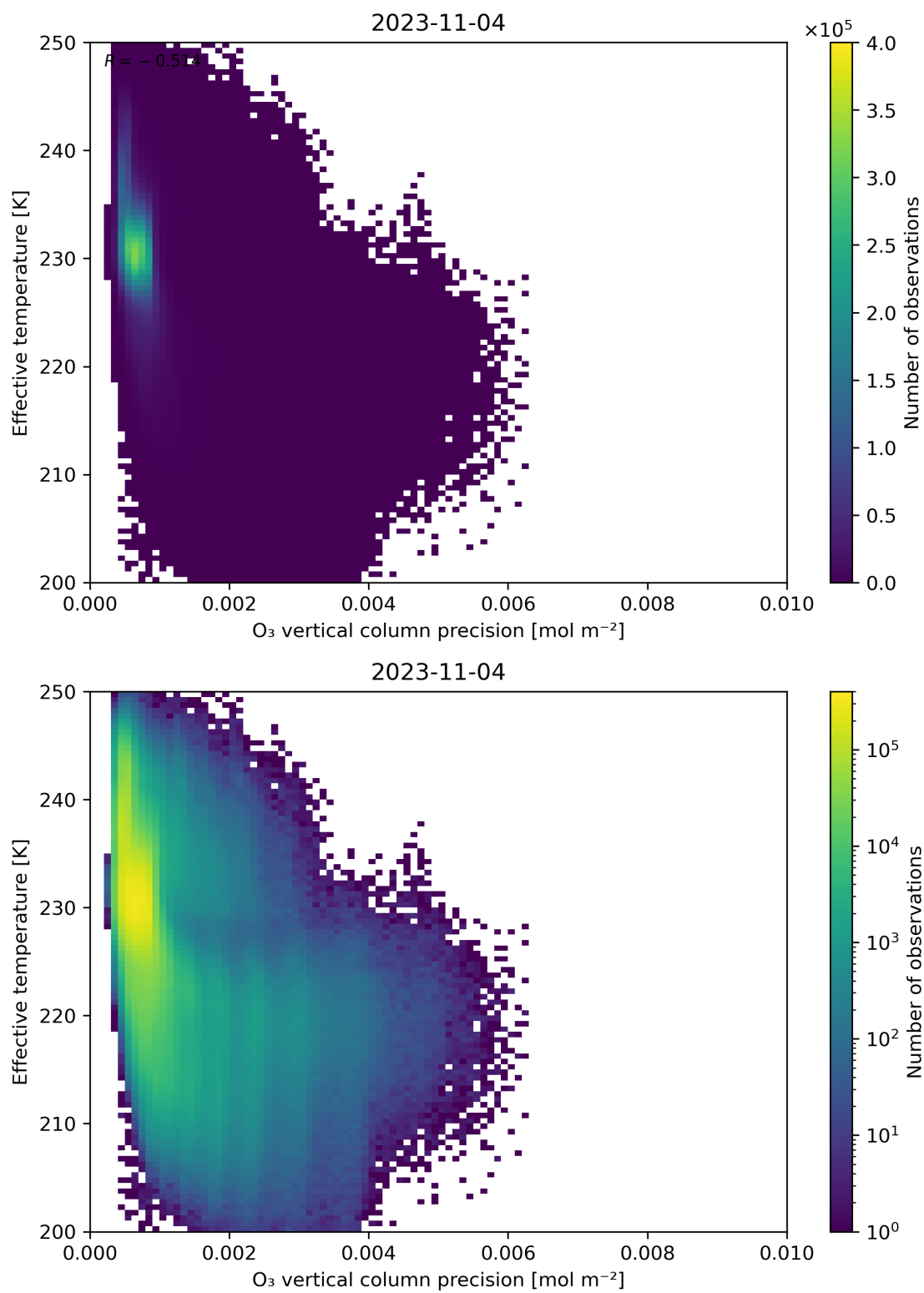
Figure 42: Scatter density plot of “O 3 vertical column precision” against “Effective temperature” for 2023-11-03 to 2023-11-05.
