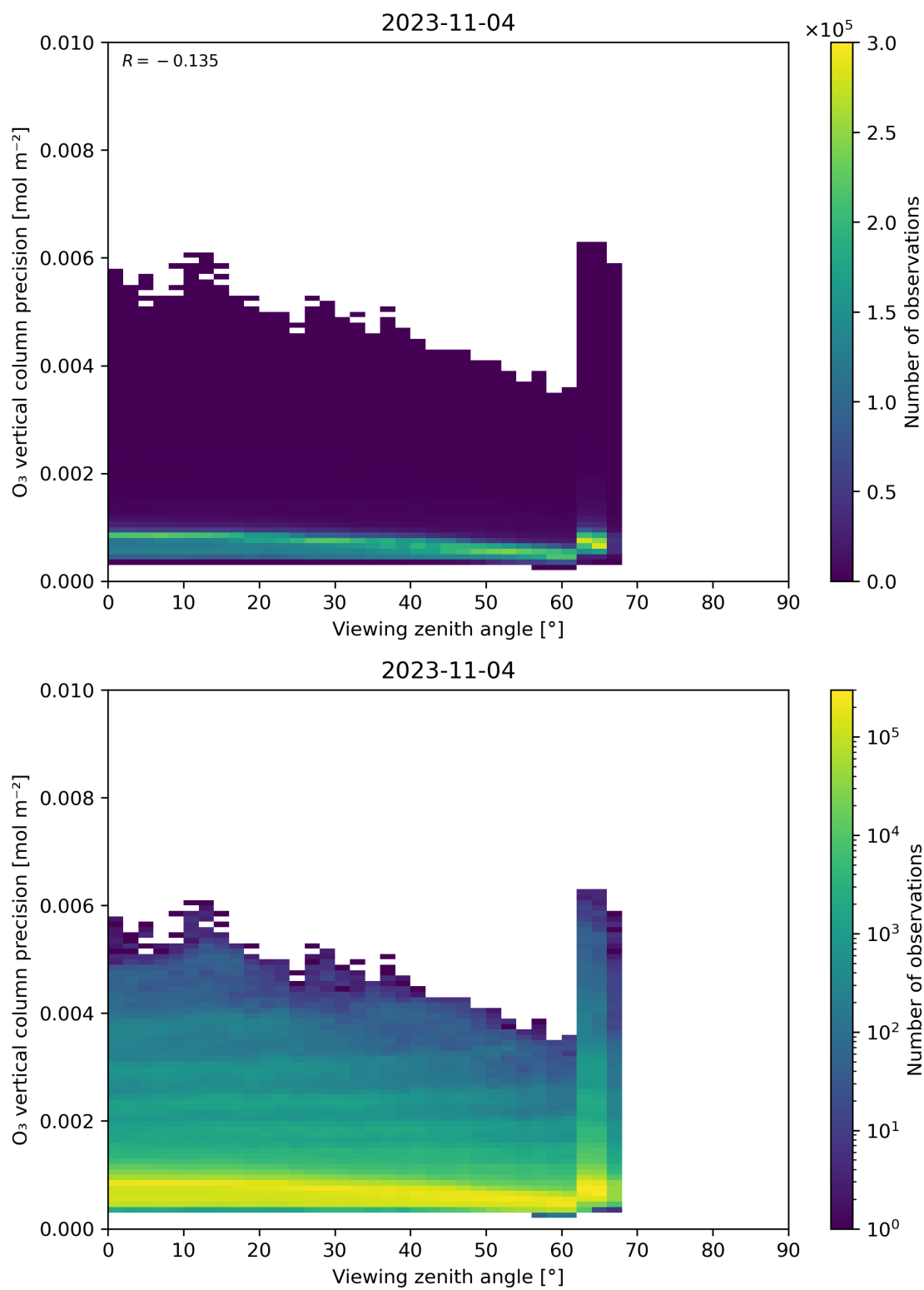
Figure 53: Scatter density plot of “Viewing zenith angle” against “O 3 vertical column precision” for 2023-11-03 to 2023-11-05.
