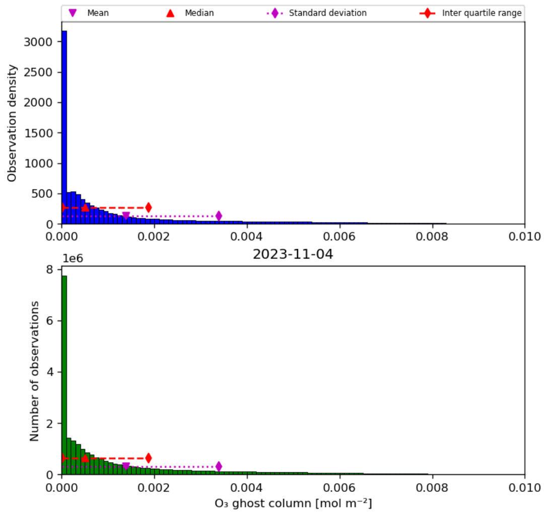
Figure 25: Histogram of “O 3 ghost column” for 2023-11-03 to 2023-11-05
