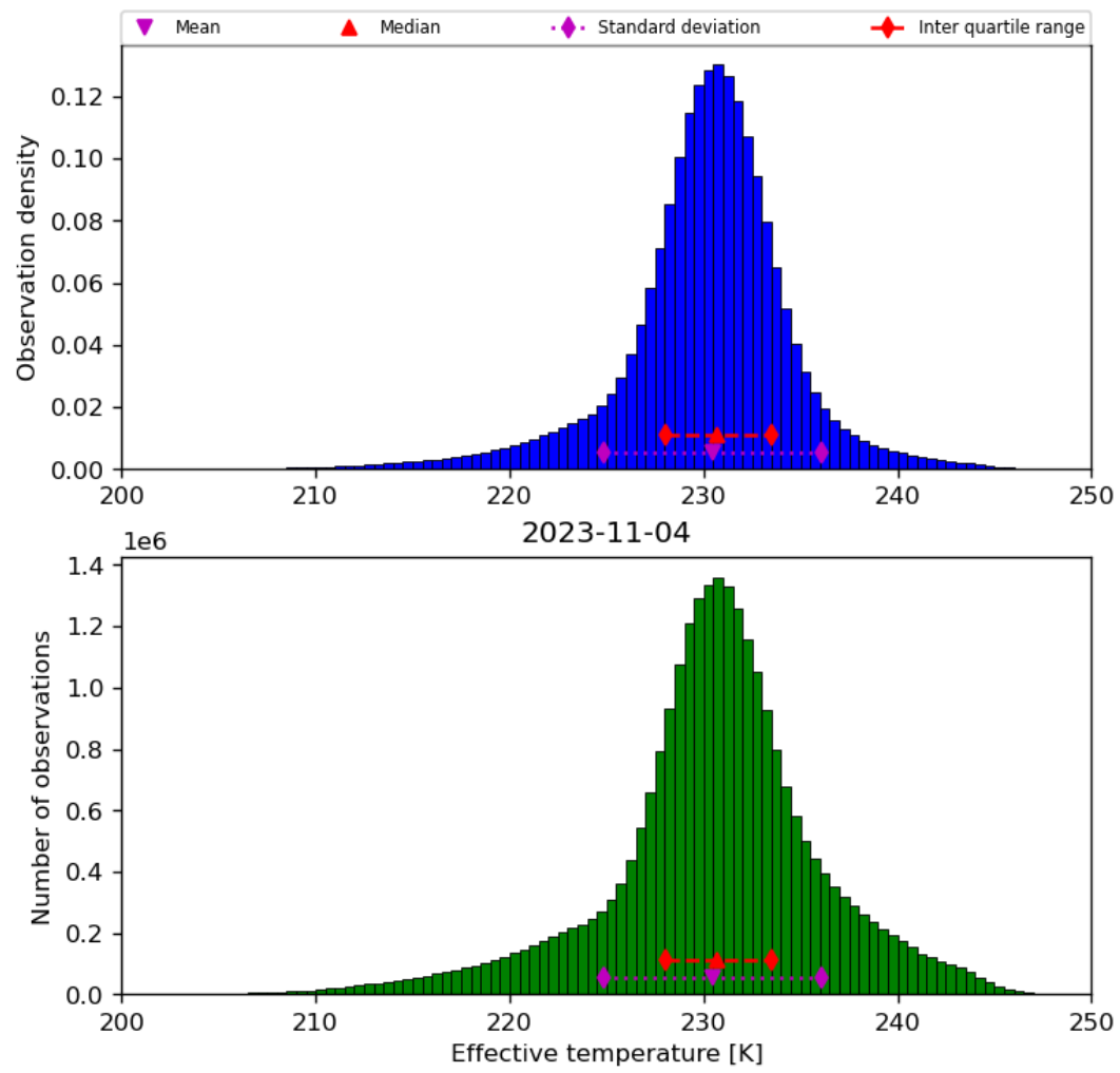
Figure 24: Histogram of “Effective temperature” for 2023-11-03 to 2023-11-05
