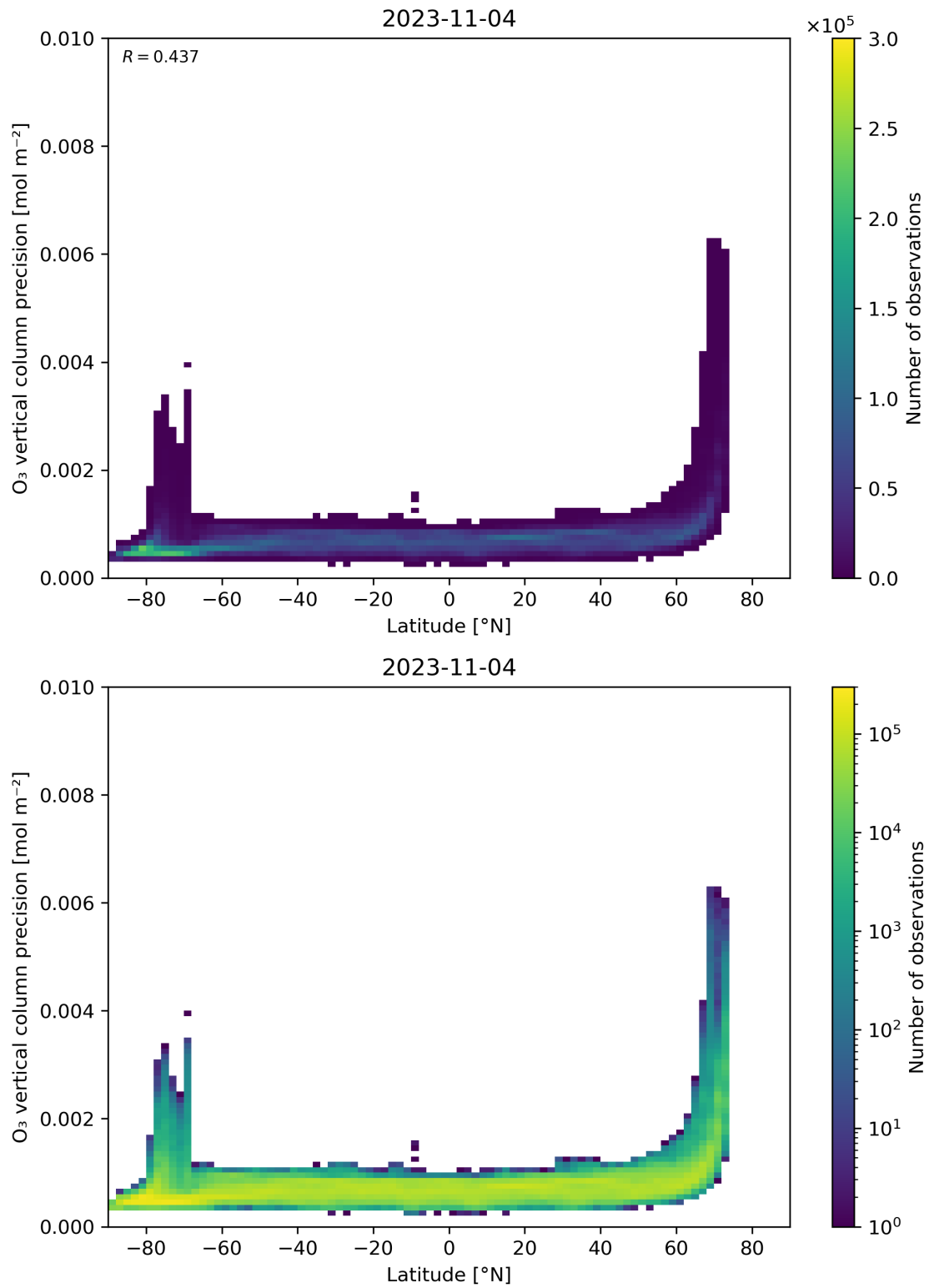
Figure 37: Scatter density plot of “Latitude” against “O 3 vertical column precision” for 2023-11-03 to 2023-11-05.
