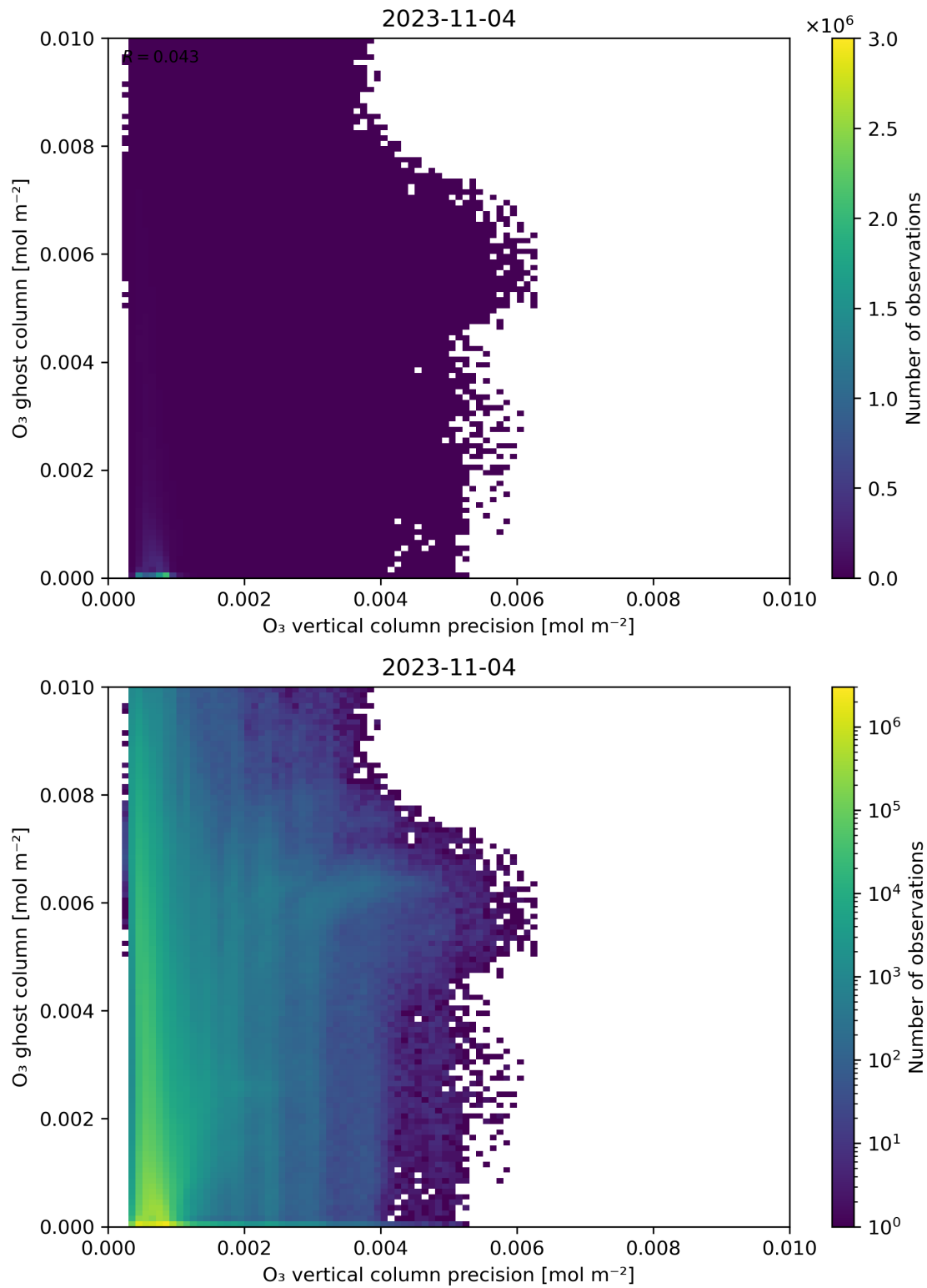
Figure 43: Scatter density plot of “ \text{O}_3 vertical column precision” against “ \text{O}_3 ghost column” for 2023-11-03 to 2023-11-05.
