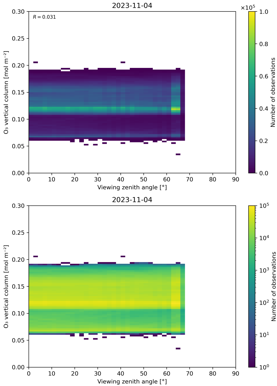
Figure 52: Scatter density plot of “Viewing zenith angle” against “O 3 vertical column” for 2023-11-03 to 2023-11-05.
