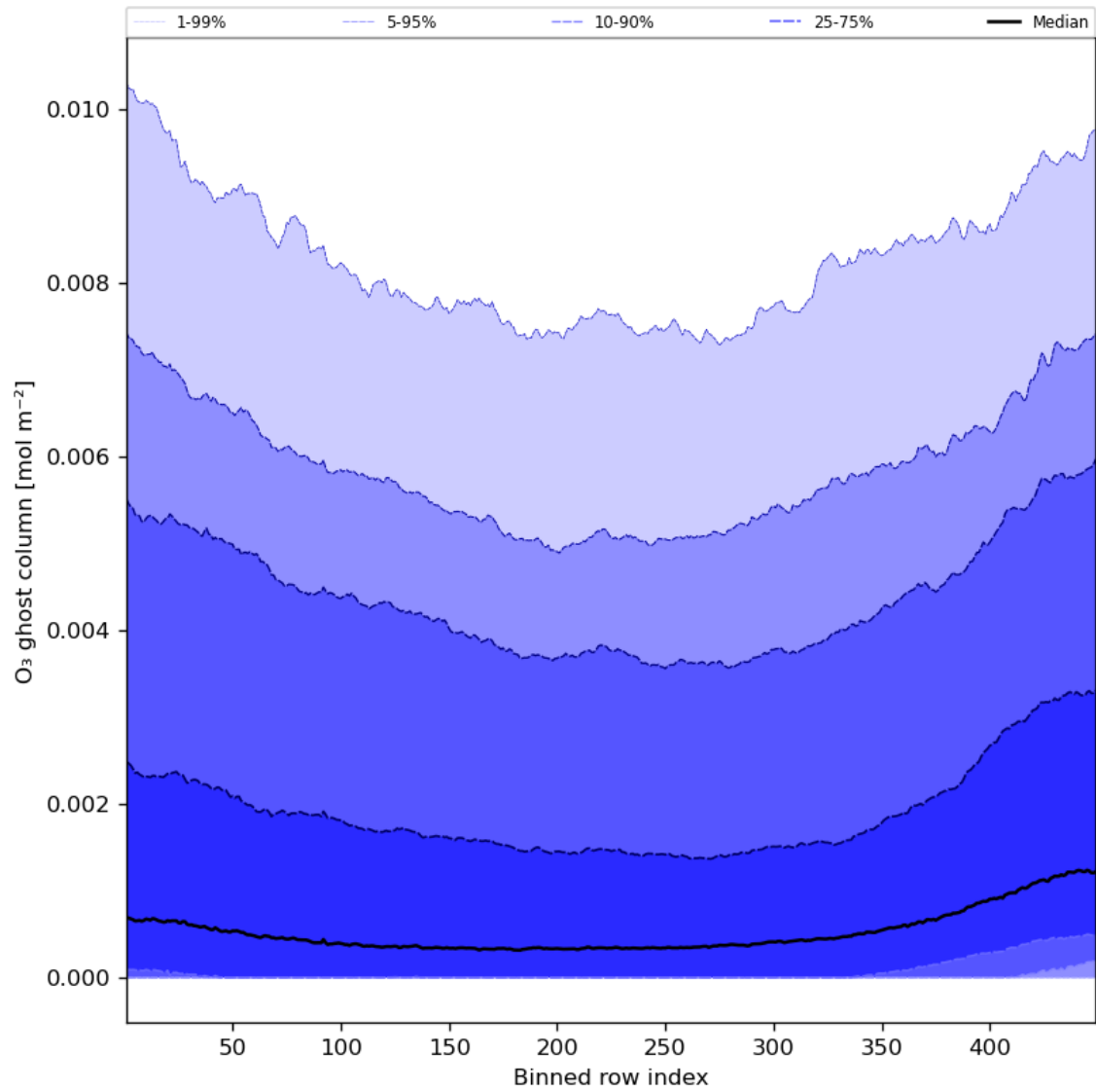
Figure 32: Along track statistics of “O 3 ghost column” for 2023-11-03 to 2023-11-05
