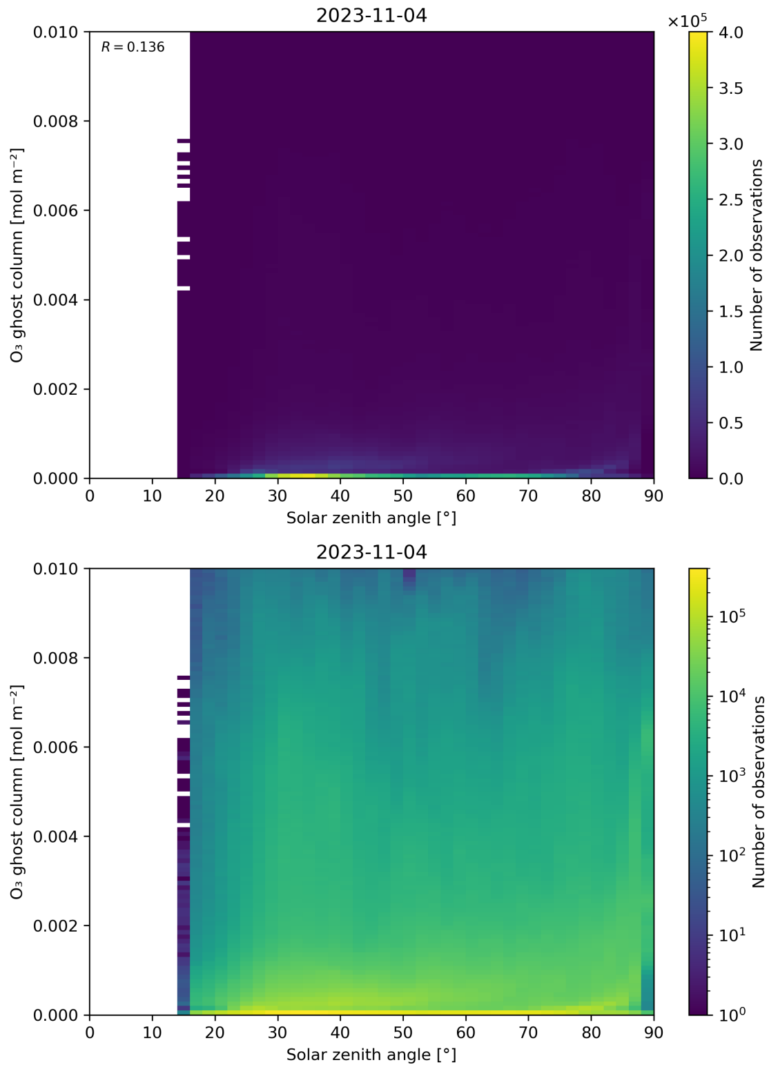
Figure 46: Scatter density plot of “Solar zenith angle” against “O 3 ghost column” for 2023-11-03 to 2023-11-05.
