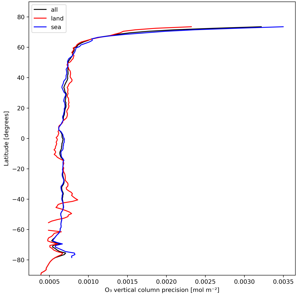
Figure 15: Zonal average of “O 3 vertical column precision” for 2023-11-03 to 2023-11-05.
