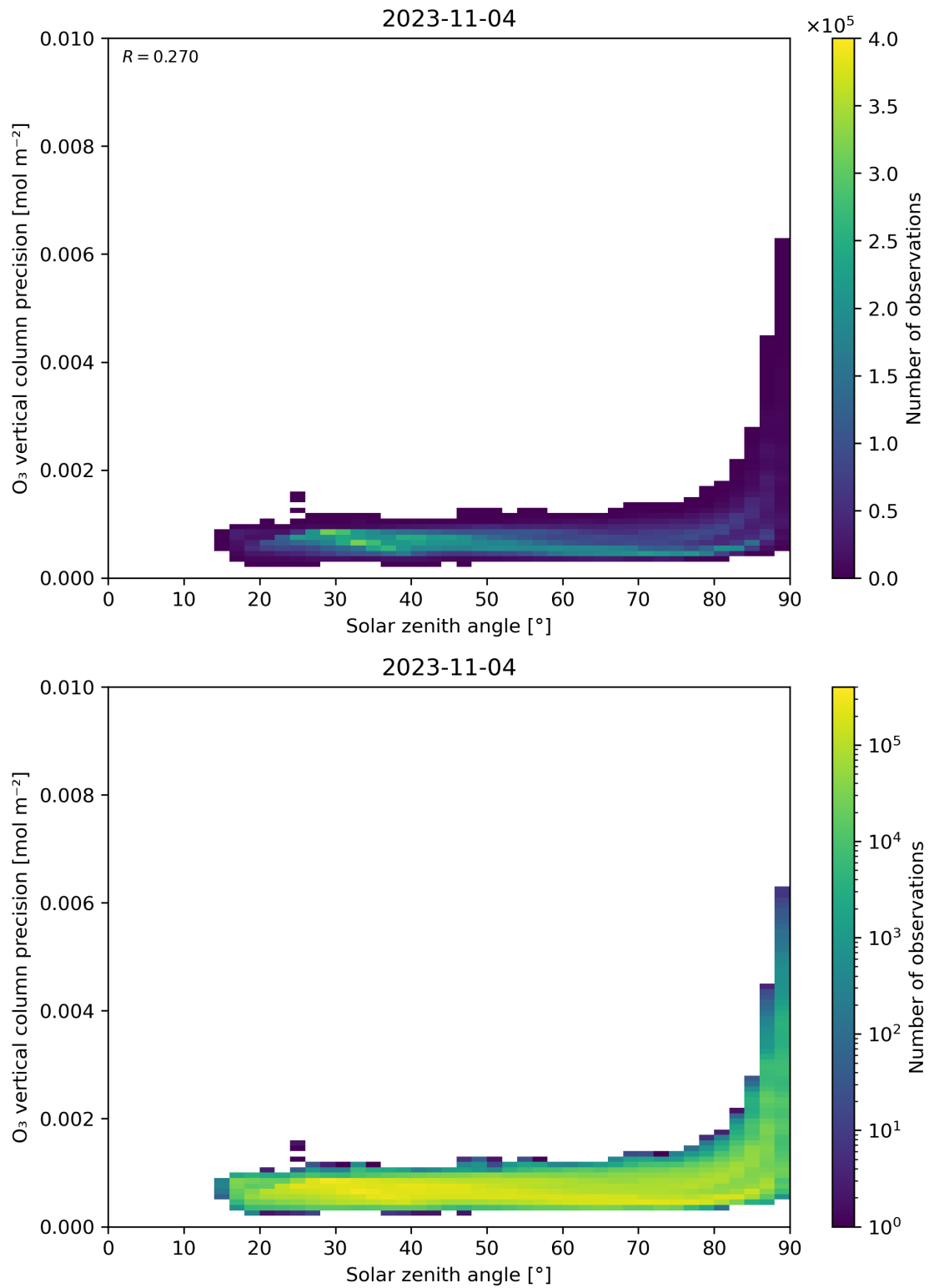
Figure 48: Scatter density plot of “Solar zenith angle” against “O 3 vertical column precision” for 2023-11-03 to 2023-11-05.
