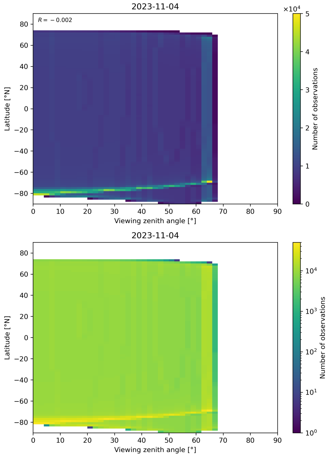
Figure 49: Scatter density plot of “Viewing zenith angle” against “Latitude” for 2023-11-03 to 2023-11-05.
