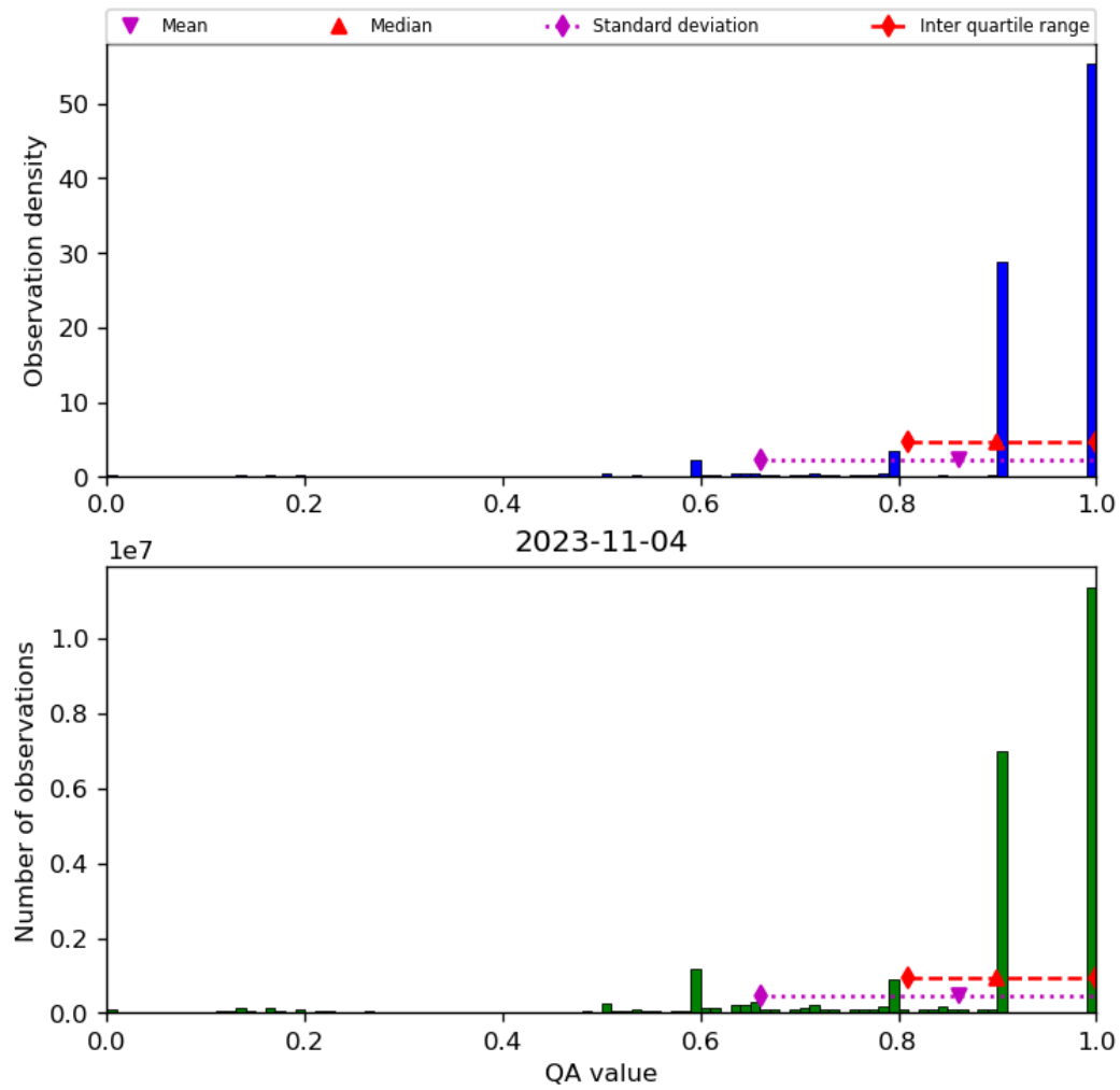
Figure 20: Histogram of “QA value” for 2023-11-03 to 2023-11-05
