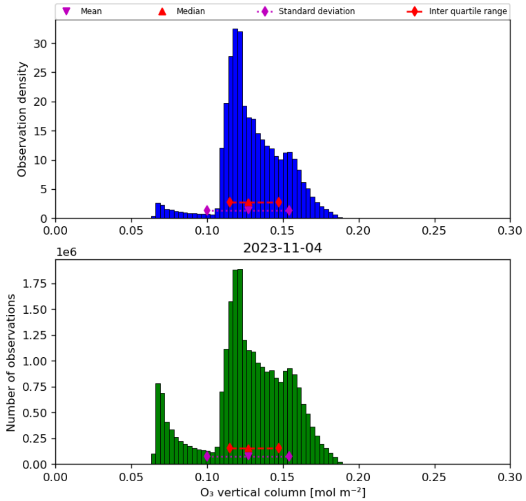
Figure 21: Histogram of “O 3 vertical column” for 2023-11-03 to 2023-11-05
