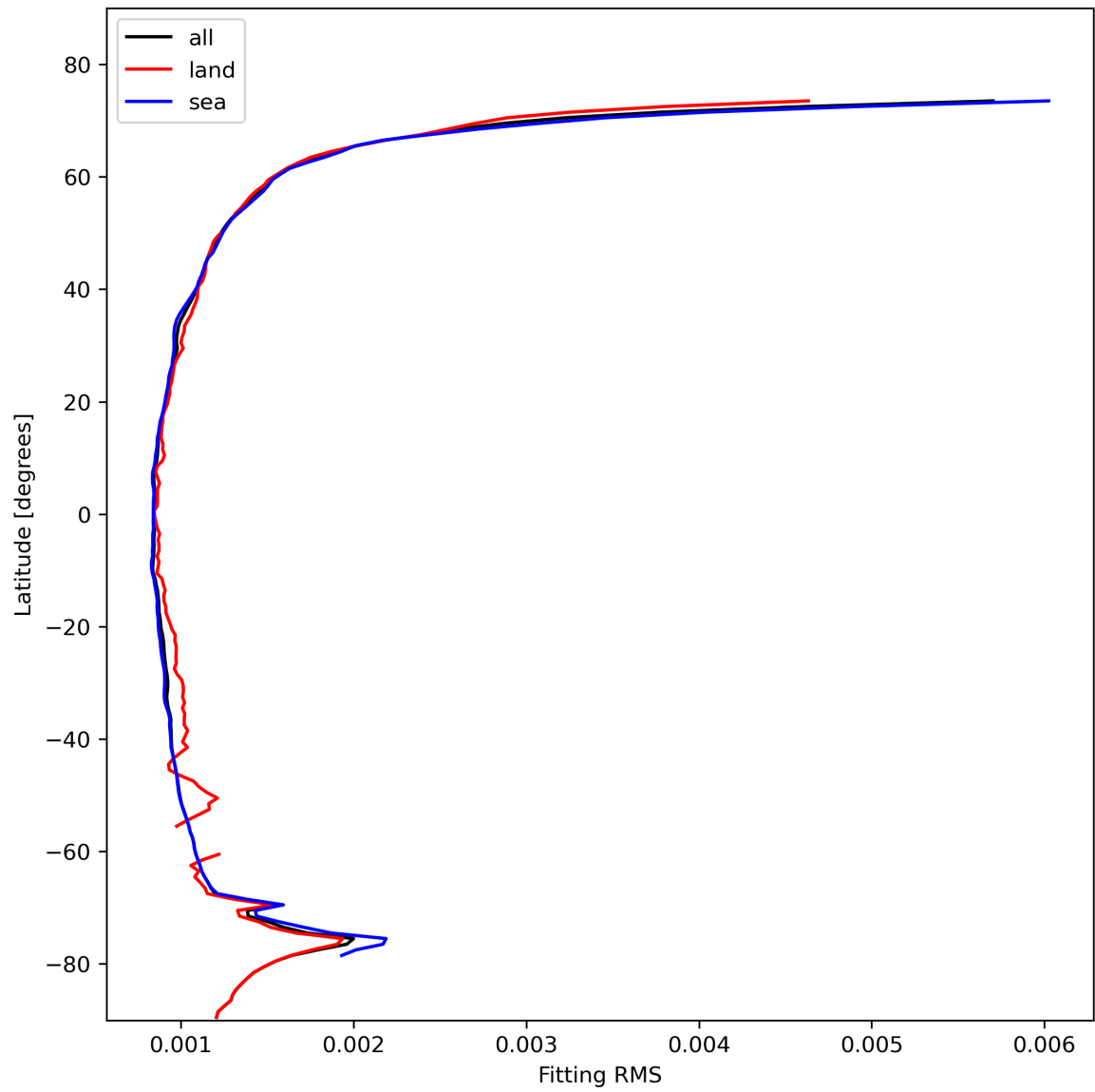
Figure 16: Zonal average of “Fitting RMS” for 2023-11-03 to 2023-11-05.
