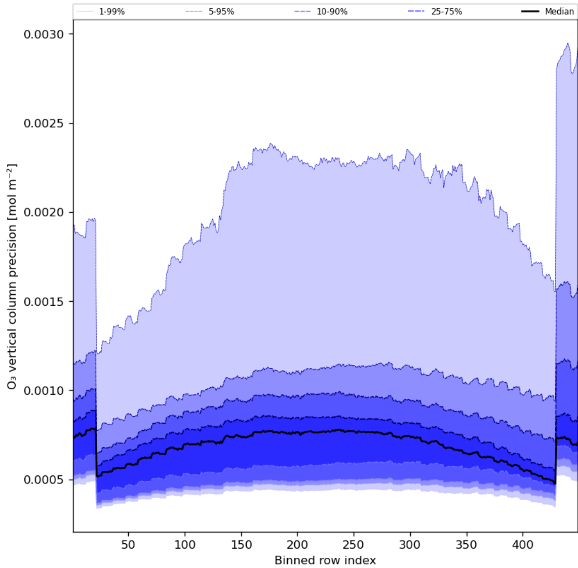
Figure 29: Along track statistics of “O 3 vertical column precision” for 2023-11-03 to 2023-11-05
