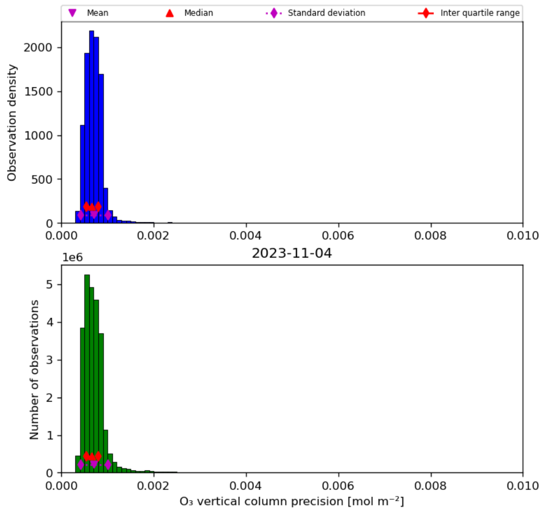
Figure 22: Histogram of “O 3 vertical column precision” for 2023-11-03 to 2023-11-05
