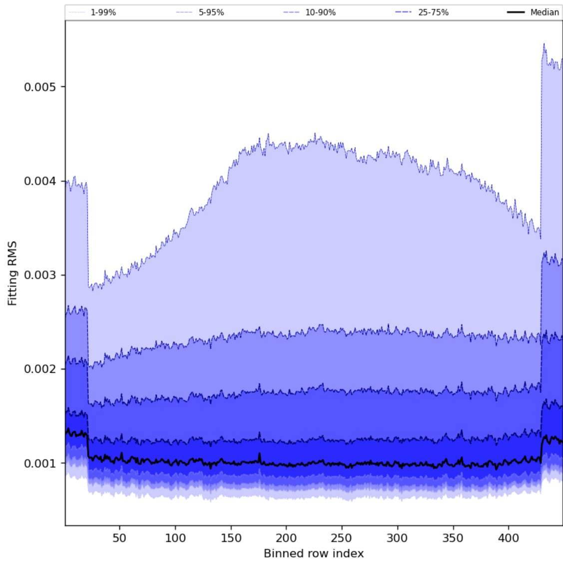
Figure 30: Along track statistics of “Fitting RMS” for 2023-11-03 to 2023-11-05
