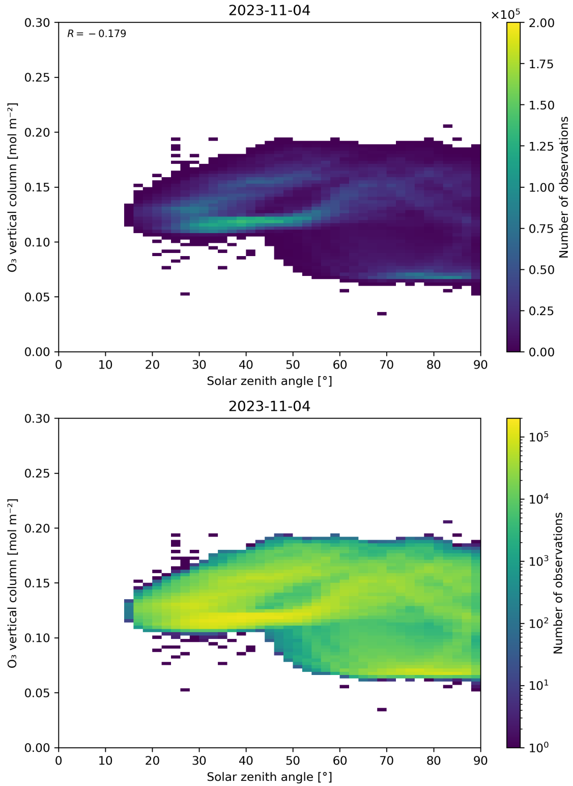
Figure 47: Scatter density plot of “Solar zenith angle” against “O 3 vertical column” for 2023-11-03 to 2023-11-05.
