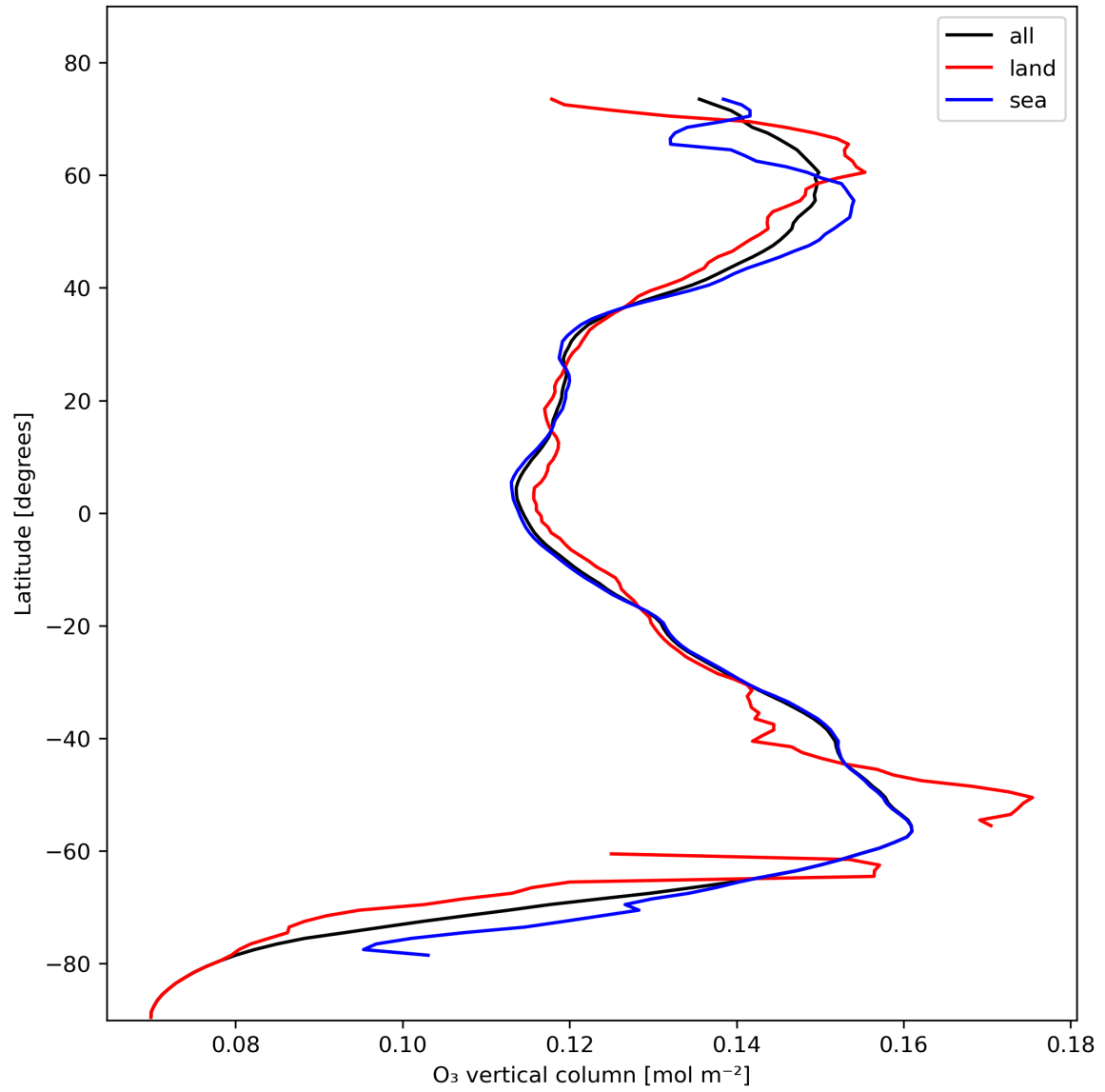
Figure 14: Zonal average of “O 3 vertical column” for 2023-11-03 to 2023-11-05.
