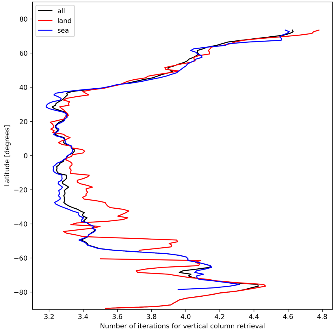
Figure 19: Zonal average of “Number of iterations for vertical column retrieval” for 2023-11-03 to 2023-11-05.
