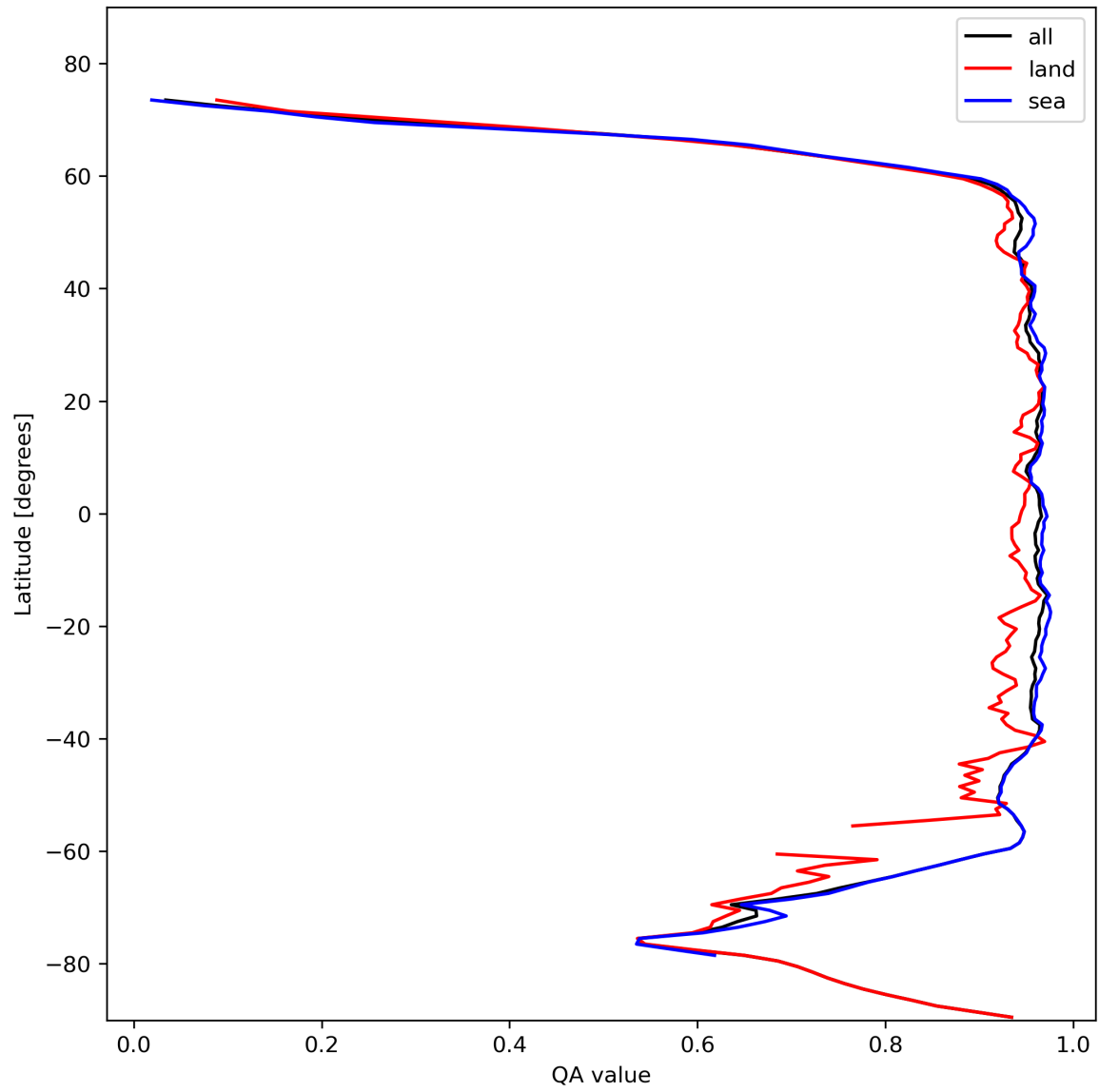
Figure 13: Zonal average of “QA value” for 2023-11-03 to 2023-11-05.
