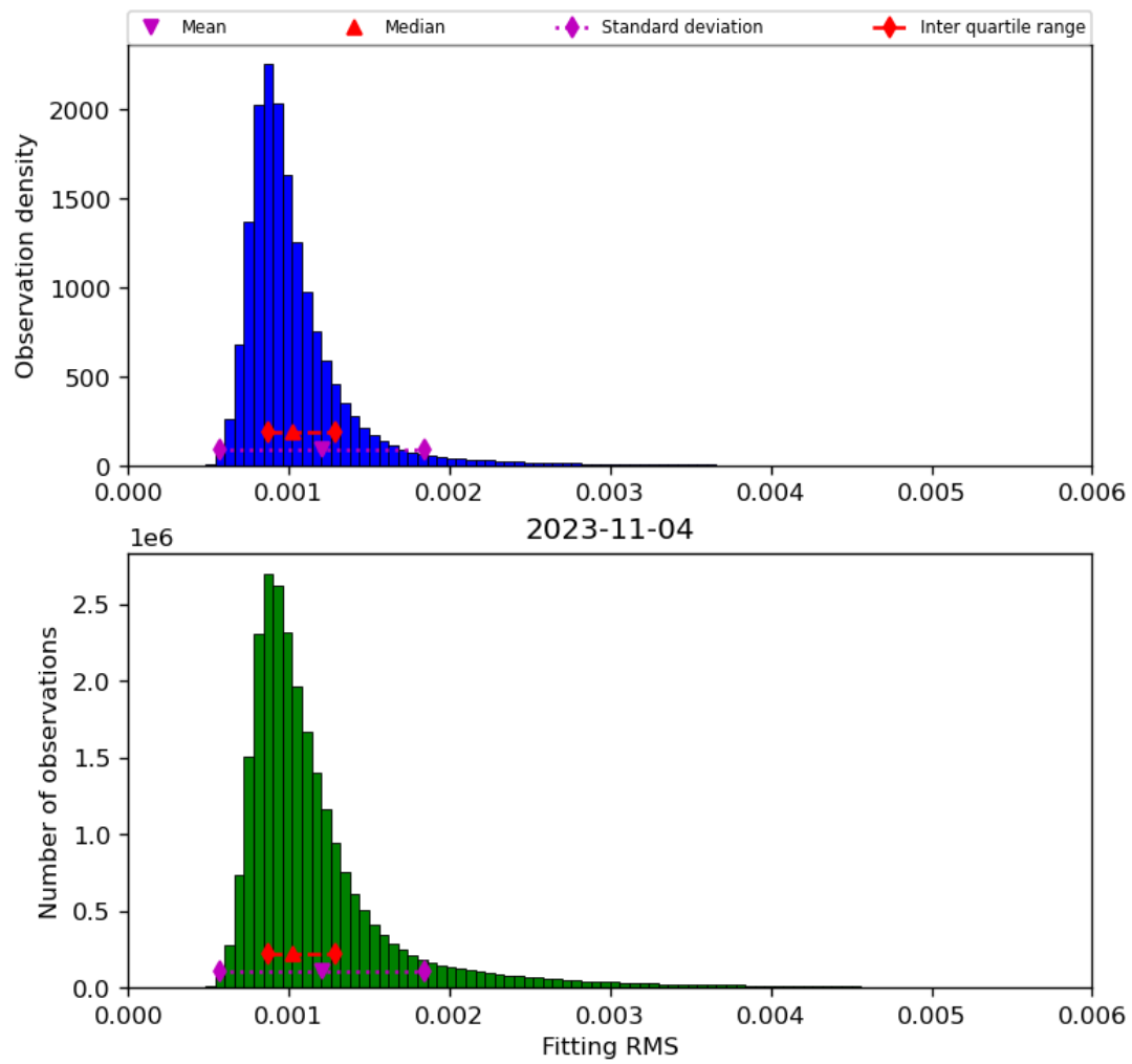
Figure 23: Histogram of “Fitting RMS” for 2023-11-03 to 2023-11-05
