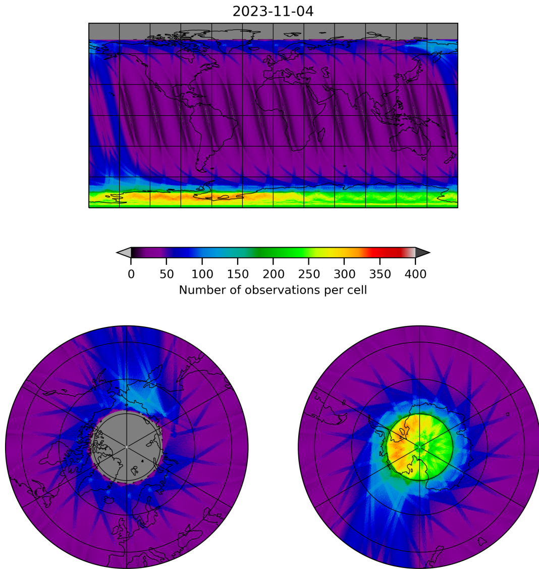
Figure 12: Map of the number of observations for 2023-11-03 to 2023-11-05
