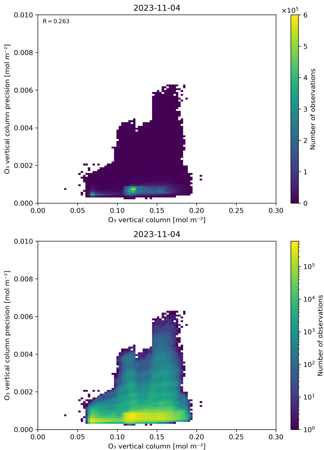
Figure 41: Scatter density plot of “O 3 vertical column” against “O 3 vertical column precision” for 2023-11-03 to 2023-11-05.
