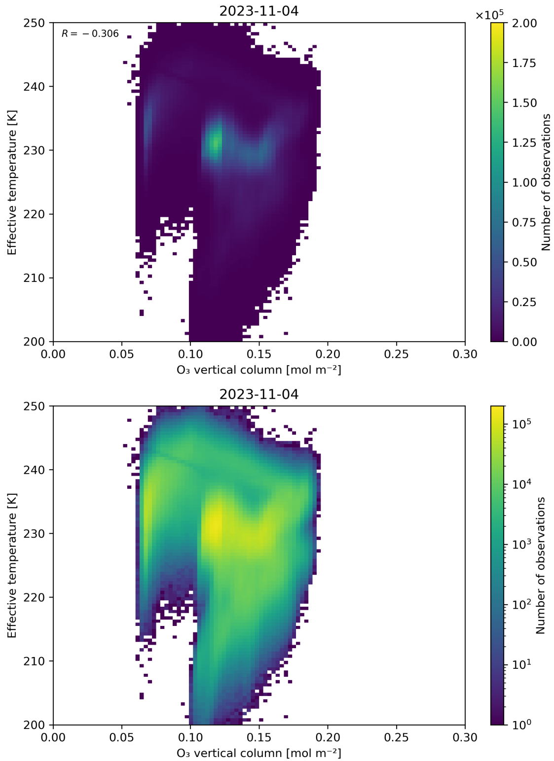
Figure 39: Scatter density plot of “O 3 vertical column” against “Effective temperature” for 2023-11-03 to 2023-11-05.
