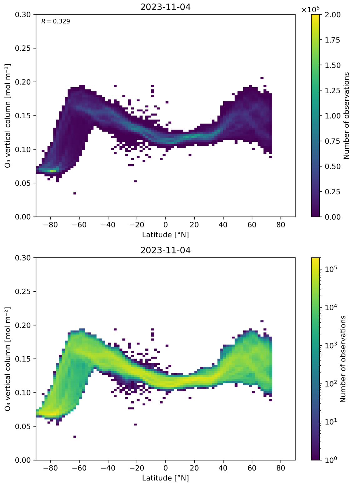
Figure 36: Scatter density plot of “Latitude” against “O 3 vertical column” for 2023-11-03 to 2023-11-05.
