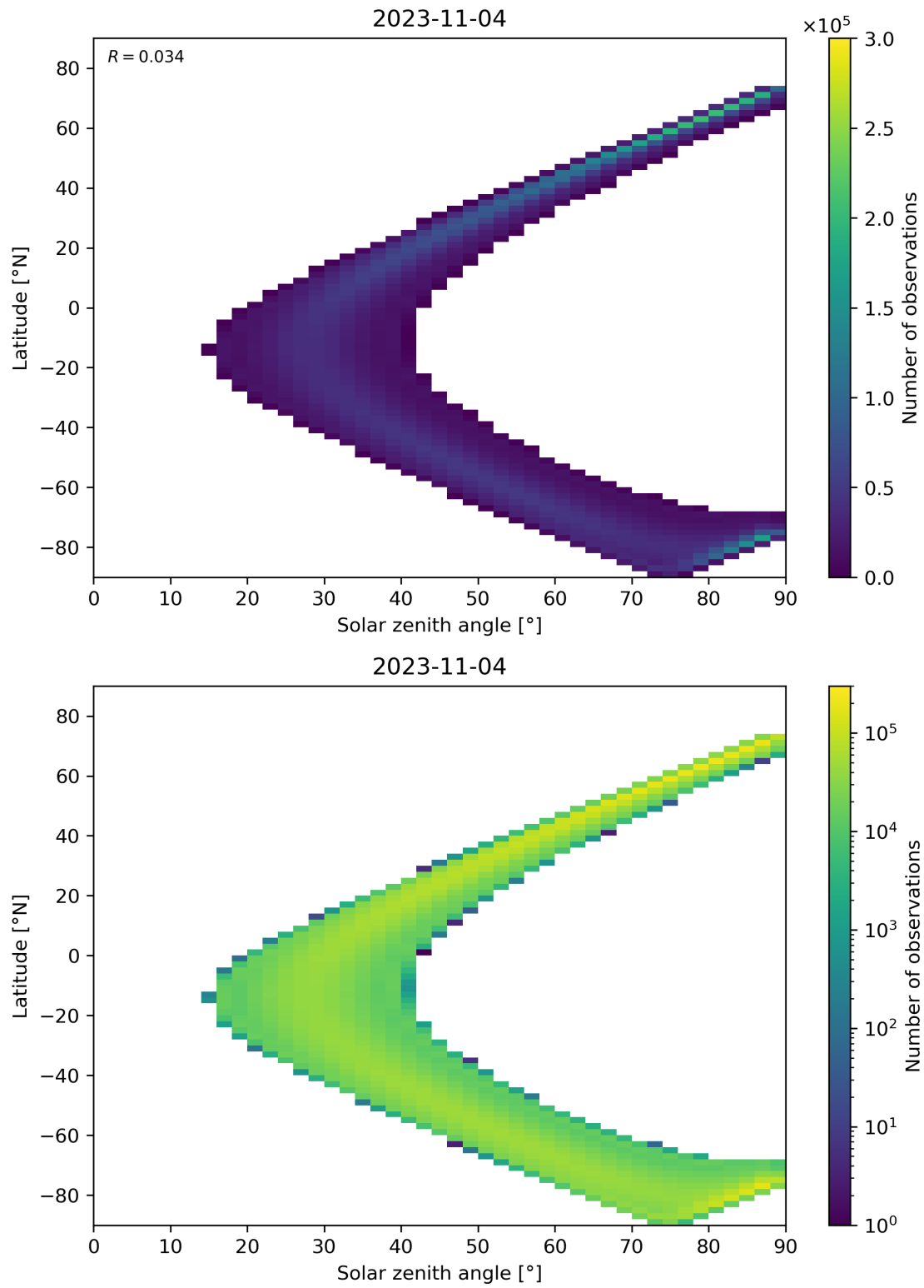
Figure 44: Scatter density plot of “Solar zenith angle” against “Latitude” for 2023-11-03 to 2023-11-05.
