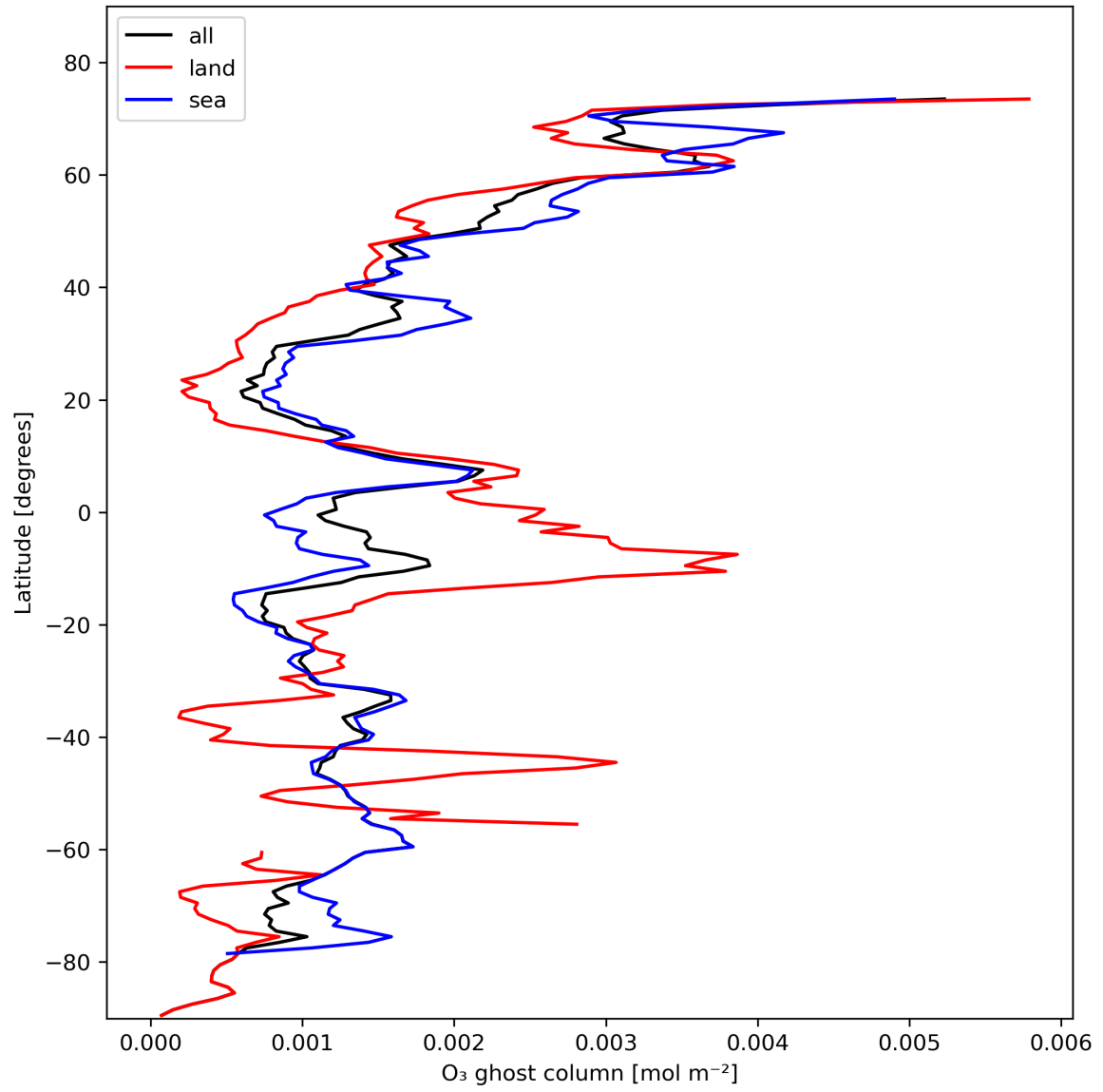
Figure 18: Zonal average of “O 3 ghost column” for 2023-11-03 to 2023-11-05.
