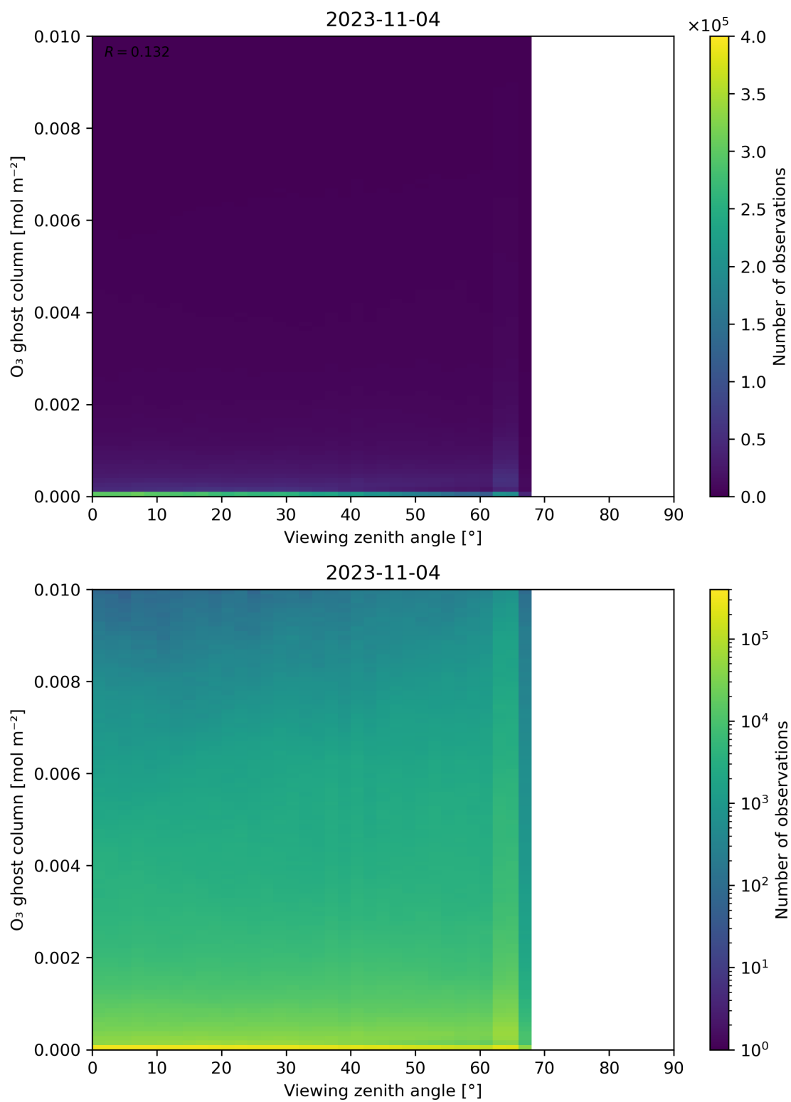
Figure 51: Scatter density plot of “Viewing zenith angle” against “O 3 ghost column” for 2023-11-03 to 2023-11-05.
