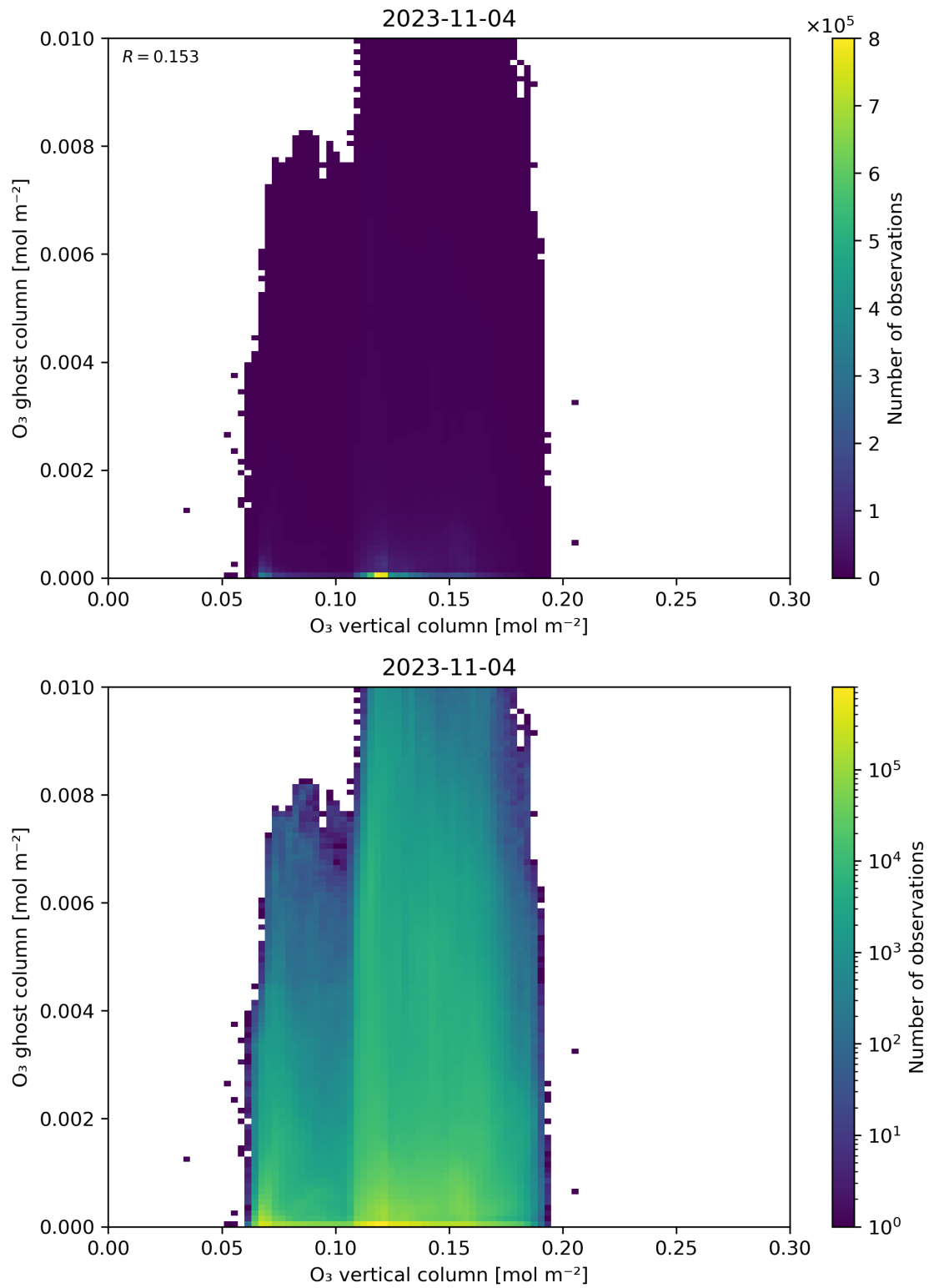
Figure 40: Scatter density plot of “O 3 vertical column” against “O 3 ghost column” for 2023-11-03 to 2023-11-05.
