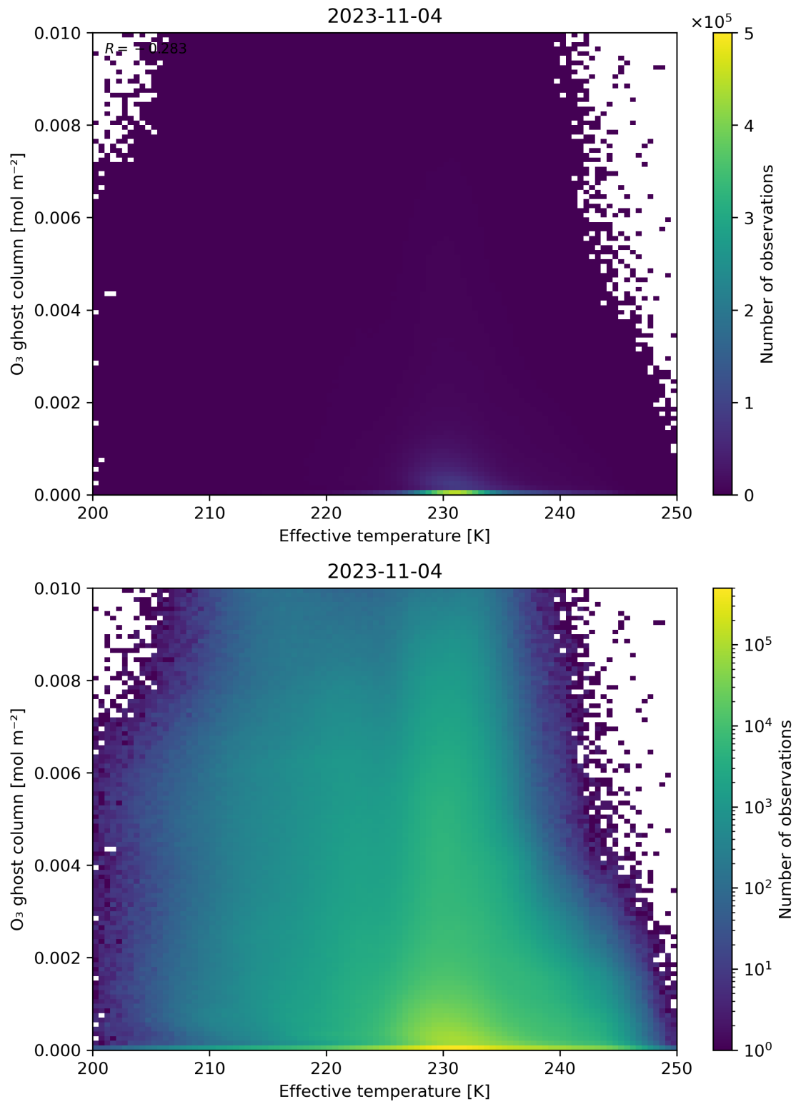
Figure 38: Scatter density plot of “Effective temperature” against “O 3 ghost column” for 2023-11-03 to 2023-11-05.
