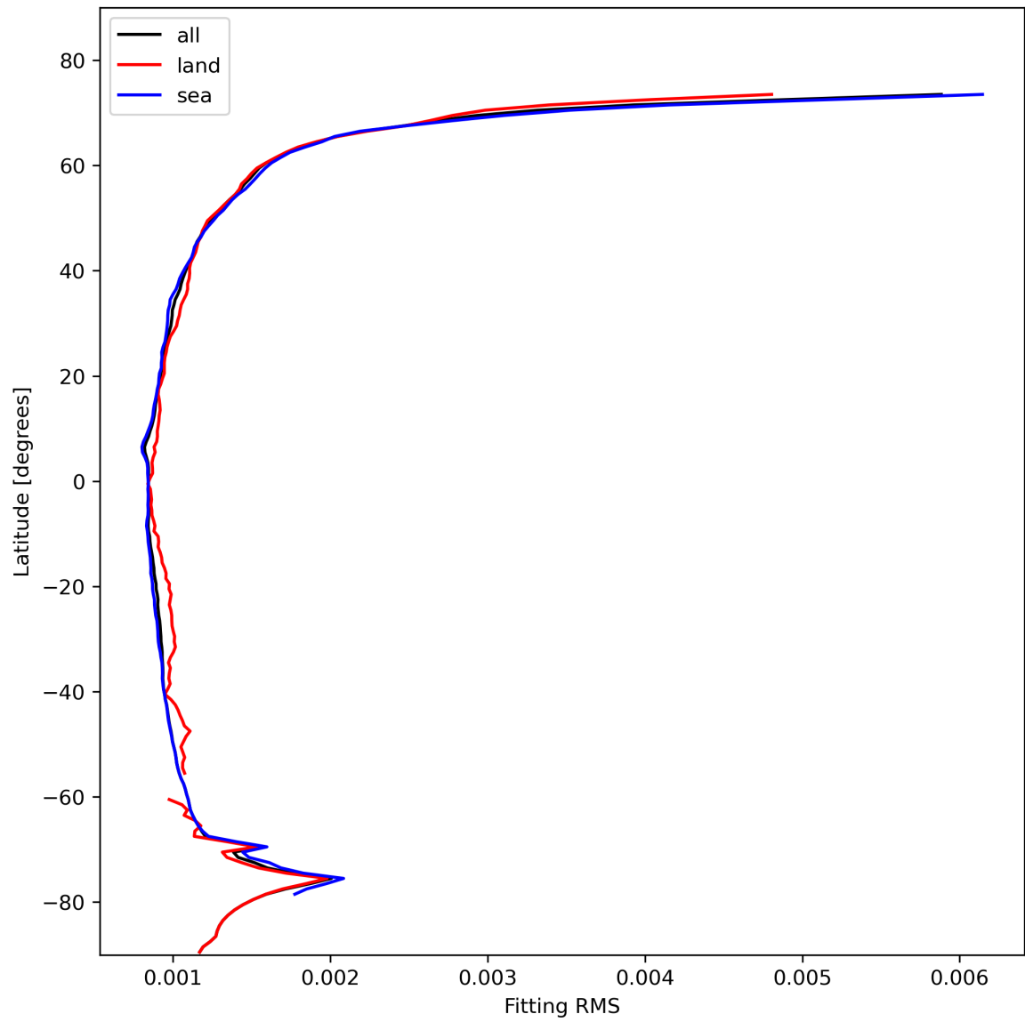
Figure 16: Zonal average of “Fitting RMS” for 2023-11-04 to 2023-11-06.
