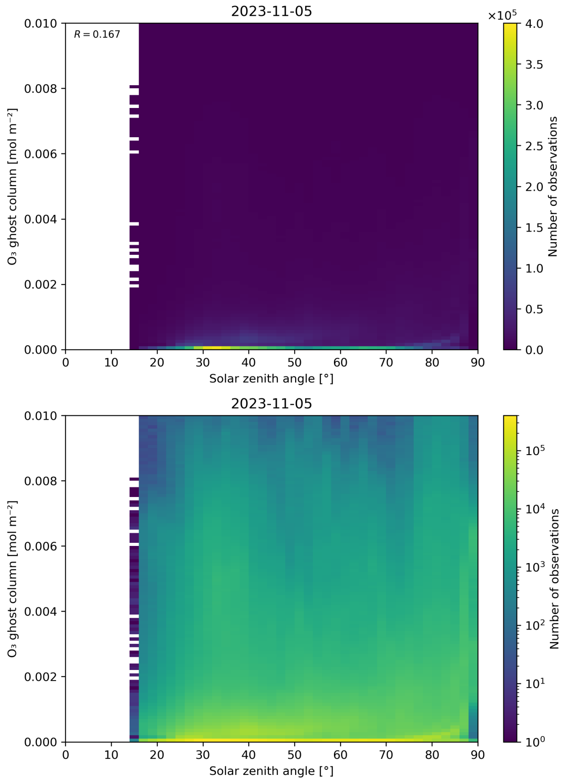
Figure 46: Scatter density plot of “Solar zenith angle” against “O 3 ghost column” for 2023-11-04 to 2023-11-06.
