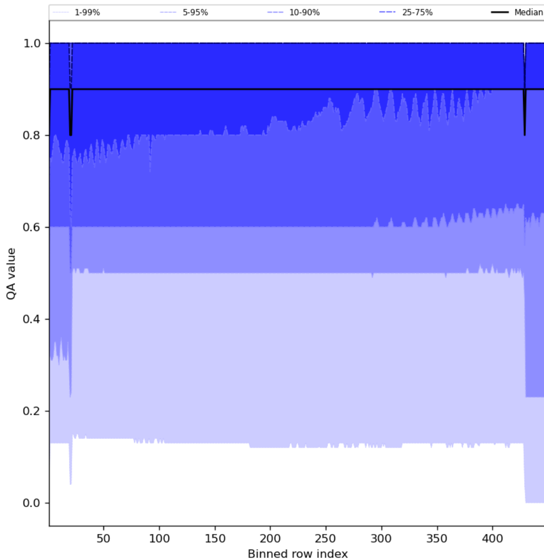
Figure 27: Along track statistics of “QA value” for 2023-11-04 to 2023-11-06
