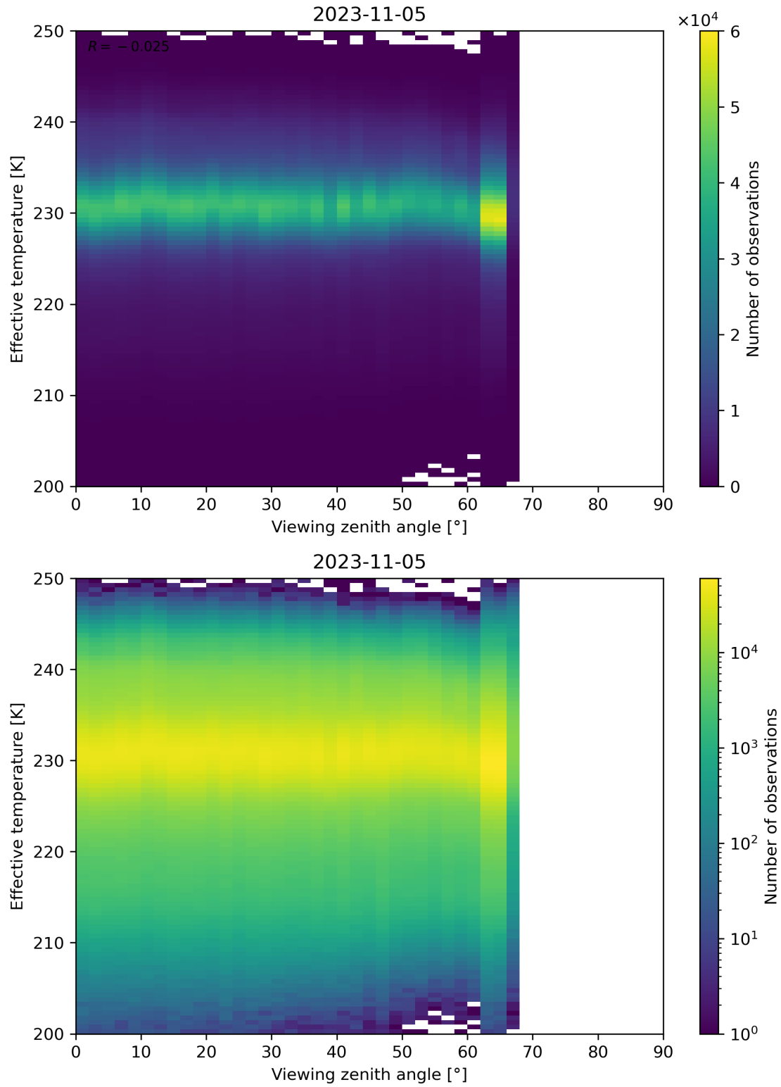
Figure 50: Scatter density plot of “Viewing zenith angle” against “Effective temperature” for 2023-11-04 to 2023-11-06.
