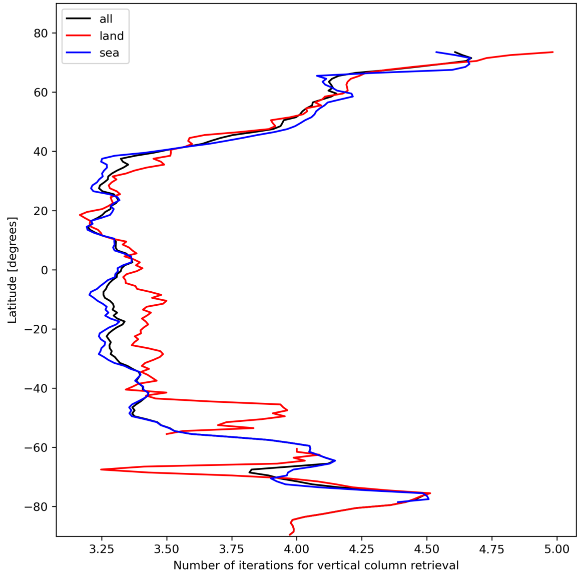
Figure 19: Zonal average of “Number of iterations for vertical column retrieval” for 2023-11-04 to 2023-11-06.
