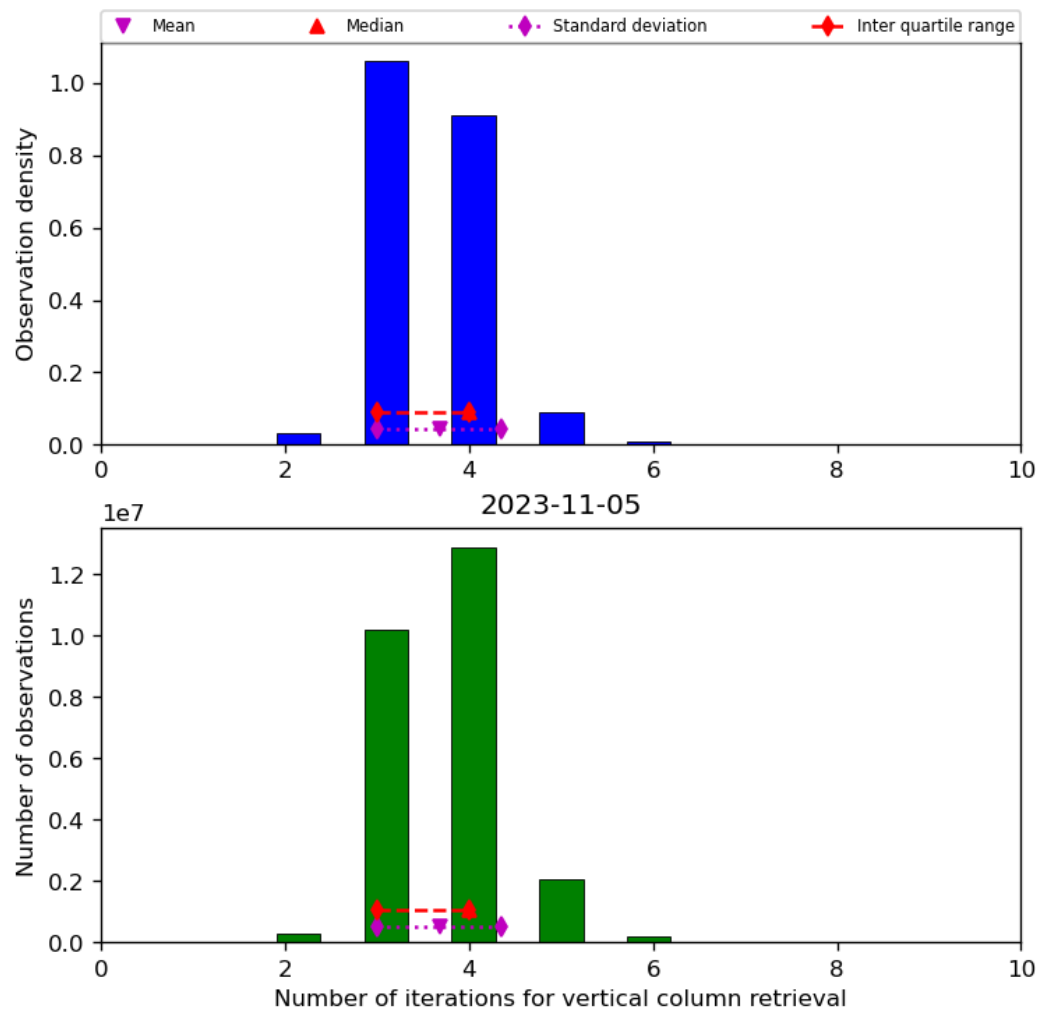
Figure 26: Histogram of “Number of iterations for vertical column retrieval” for 2023-11-04 to 2023-11-06
