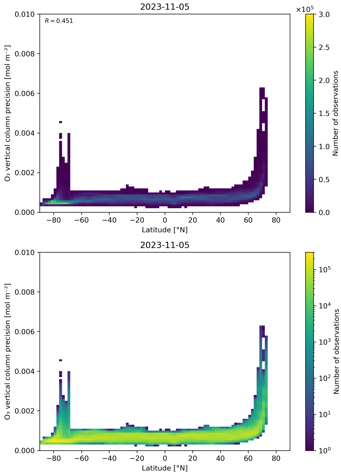
Figure 37: Scatter density plot of “Latitude” against “O 3 vertical column precision” for 2023-11-04 to 2023-11-06.
