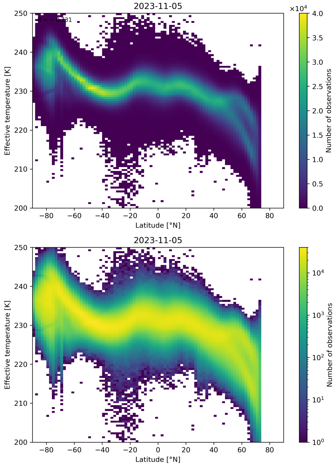
Figure 34: Scatter density plot of “Latitude” against “Effective temperature” for 2023-11-04 to 2023-11-06.
