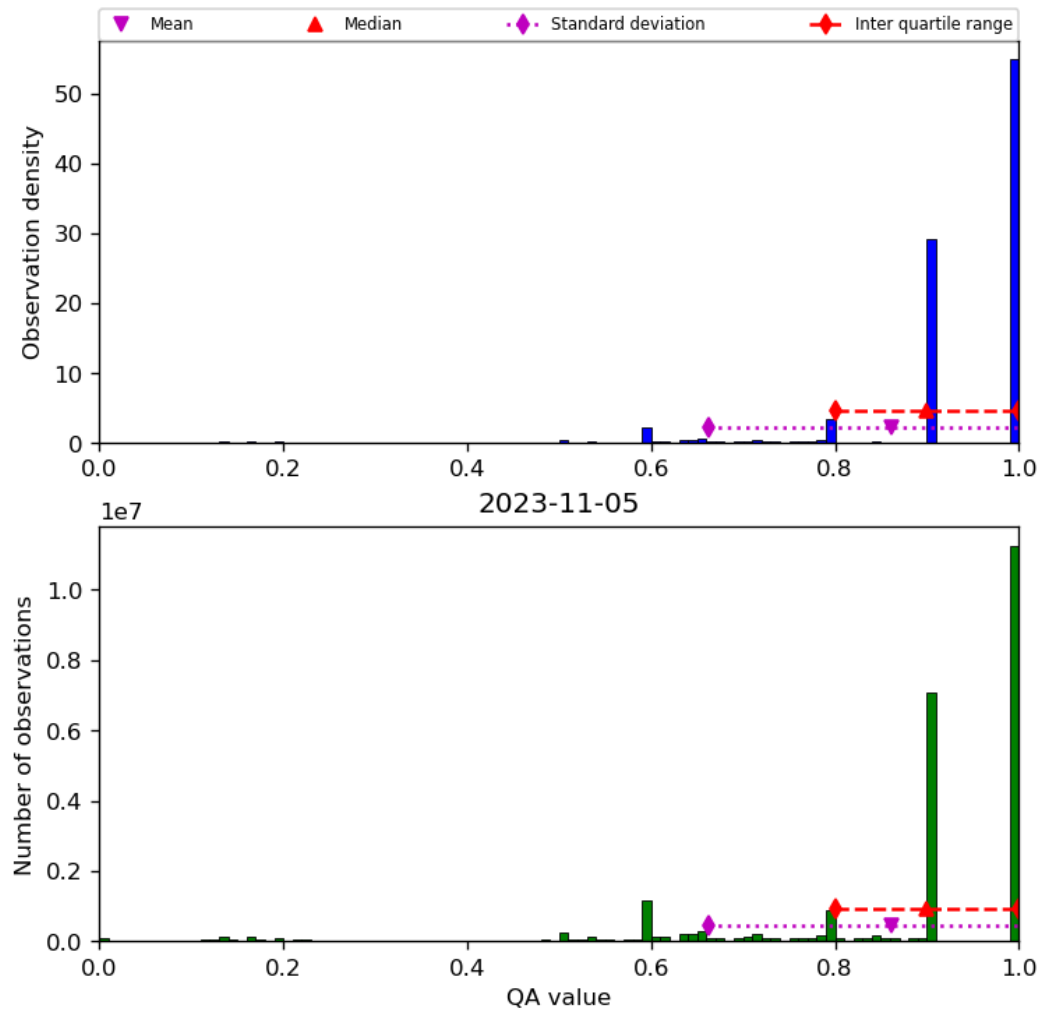
Figure 20: Histogram of “QA value” for 2023-11-04 to 2023-11-06
