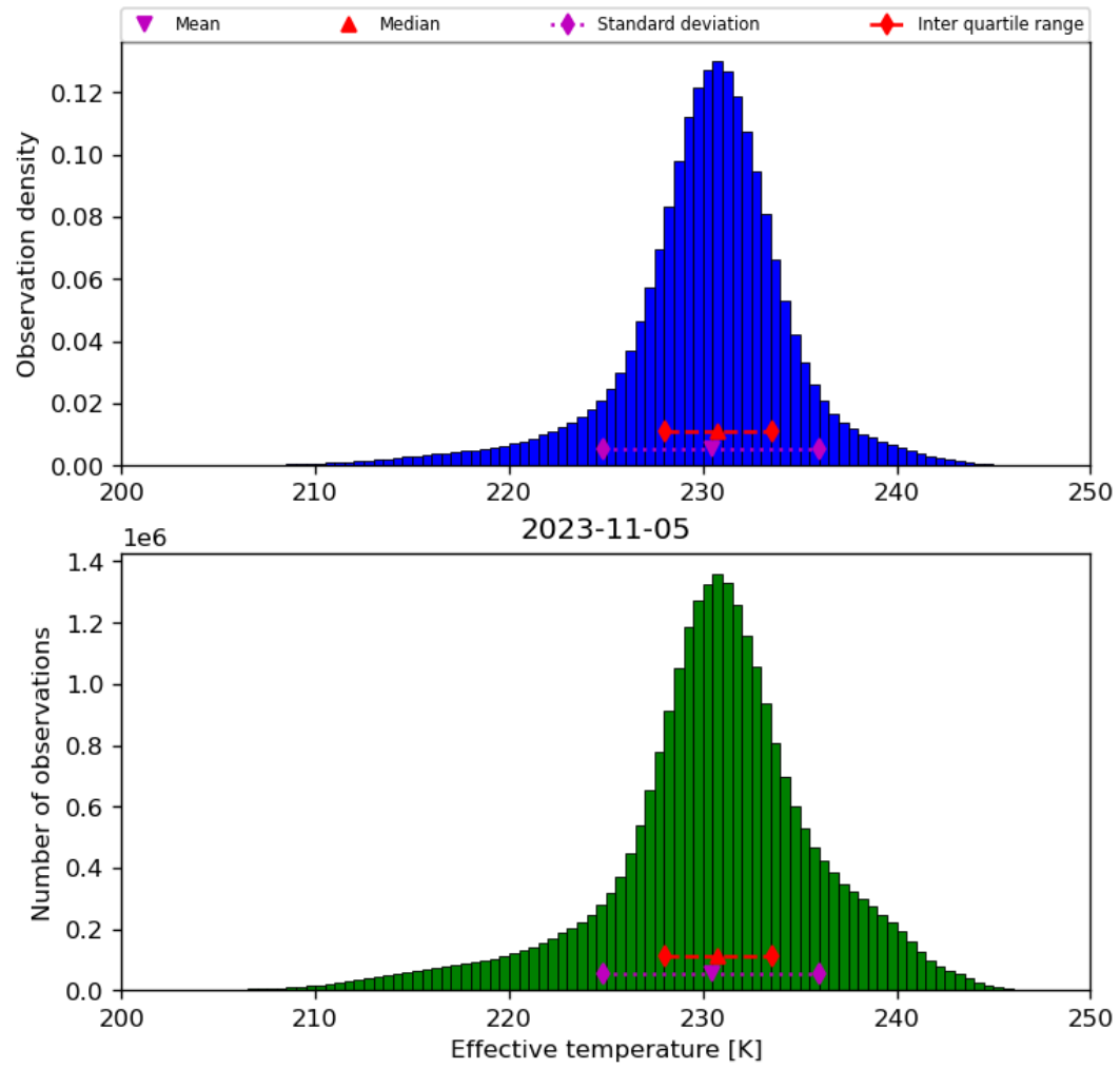
Figure 24: Histogram of “Effective temperature” for 2023-11-04 to 2023-11-06
