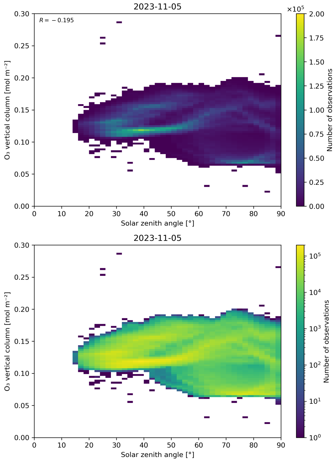
Figure 47: Scatter density plot of “Solar zenith angle” against “O 3 vertical column” for 2023-11-04 to 2023-11-06.
