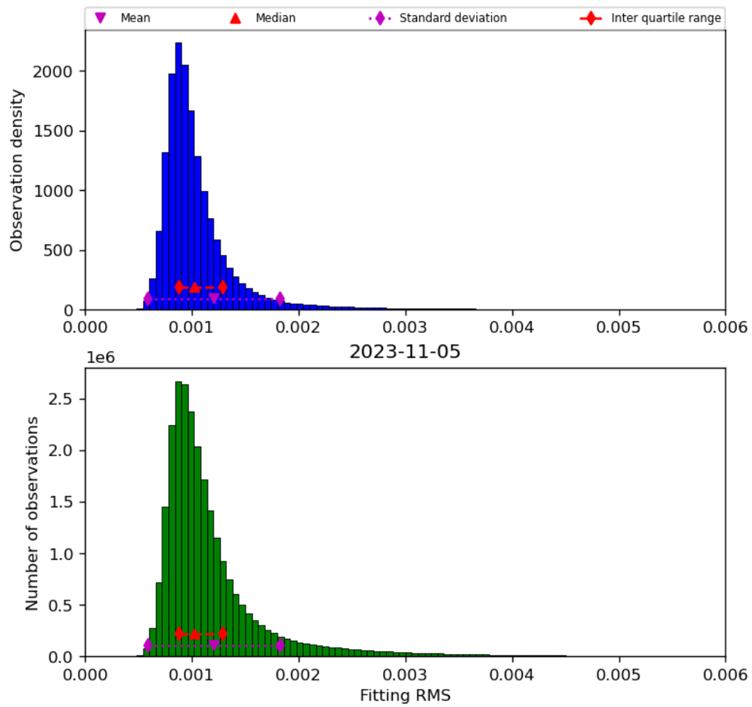
Figure 23: Histogram of “Fitting RMS” for 2023-11-04 to 2023-11-06
