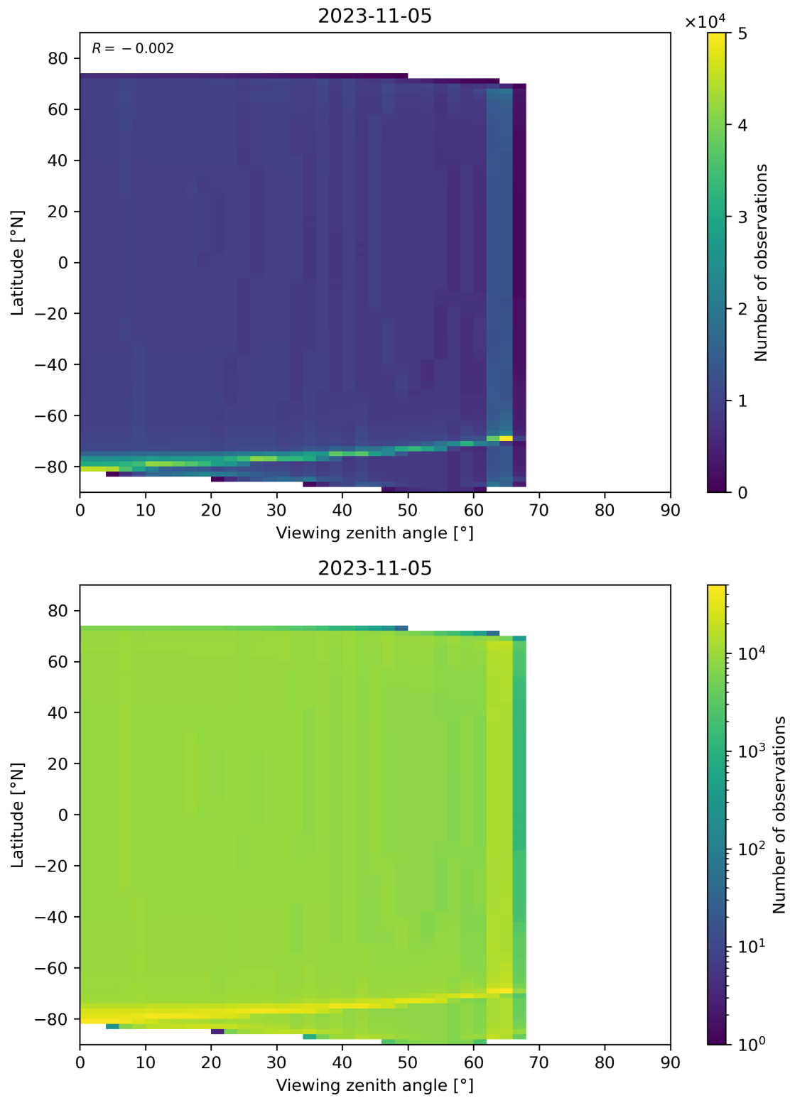
Figure 49: Scatter density plot of “Viewing zenith angle” against “Latitude” for 2023-11-04 to 2023-11-06.
