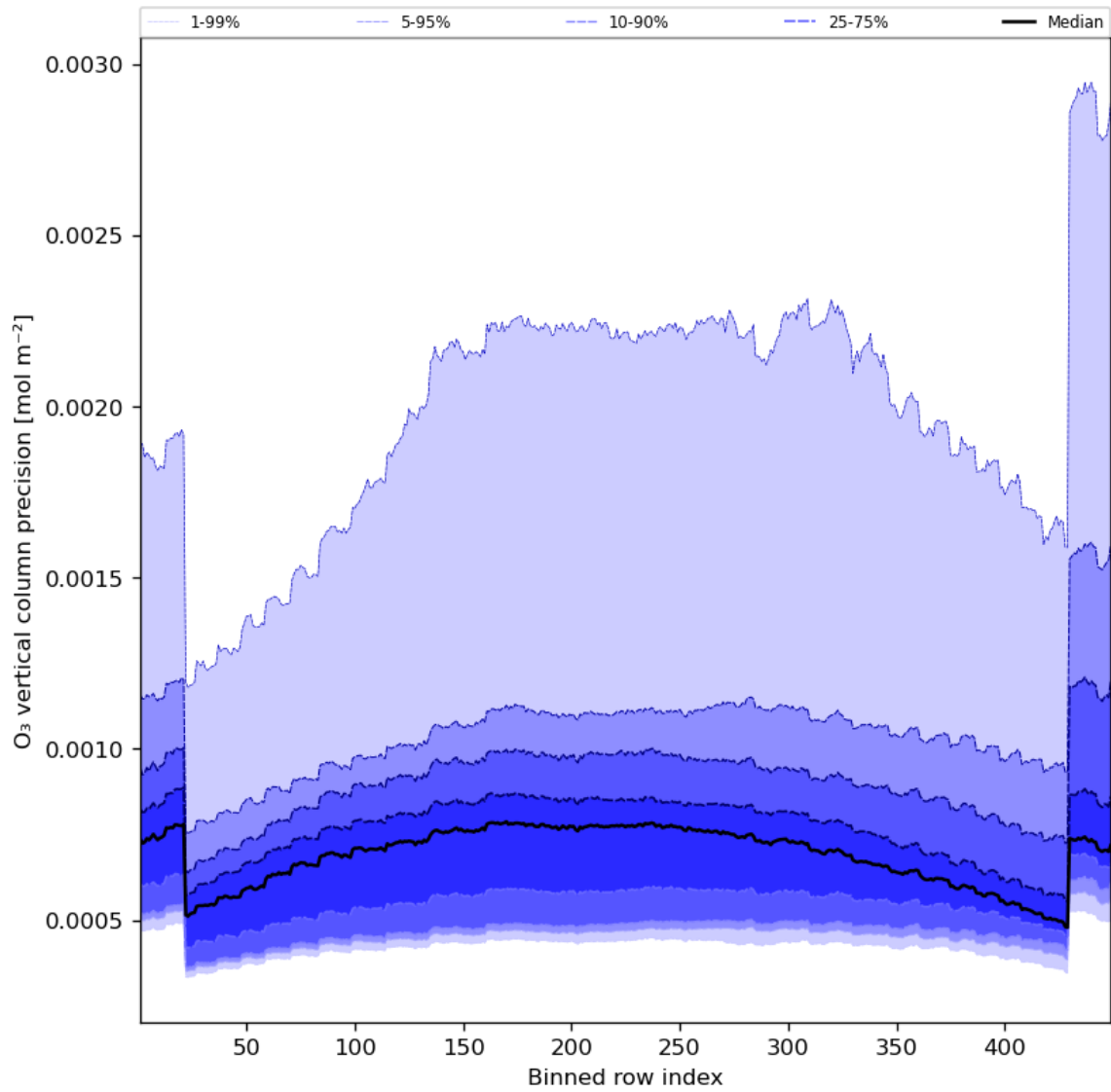
Figure 29: Along track statistics of “O 3 vertical column precision” for 2023-11-04 to 2023-11-06
