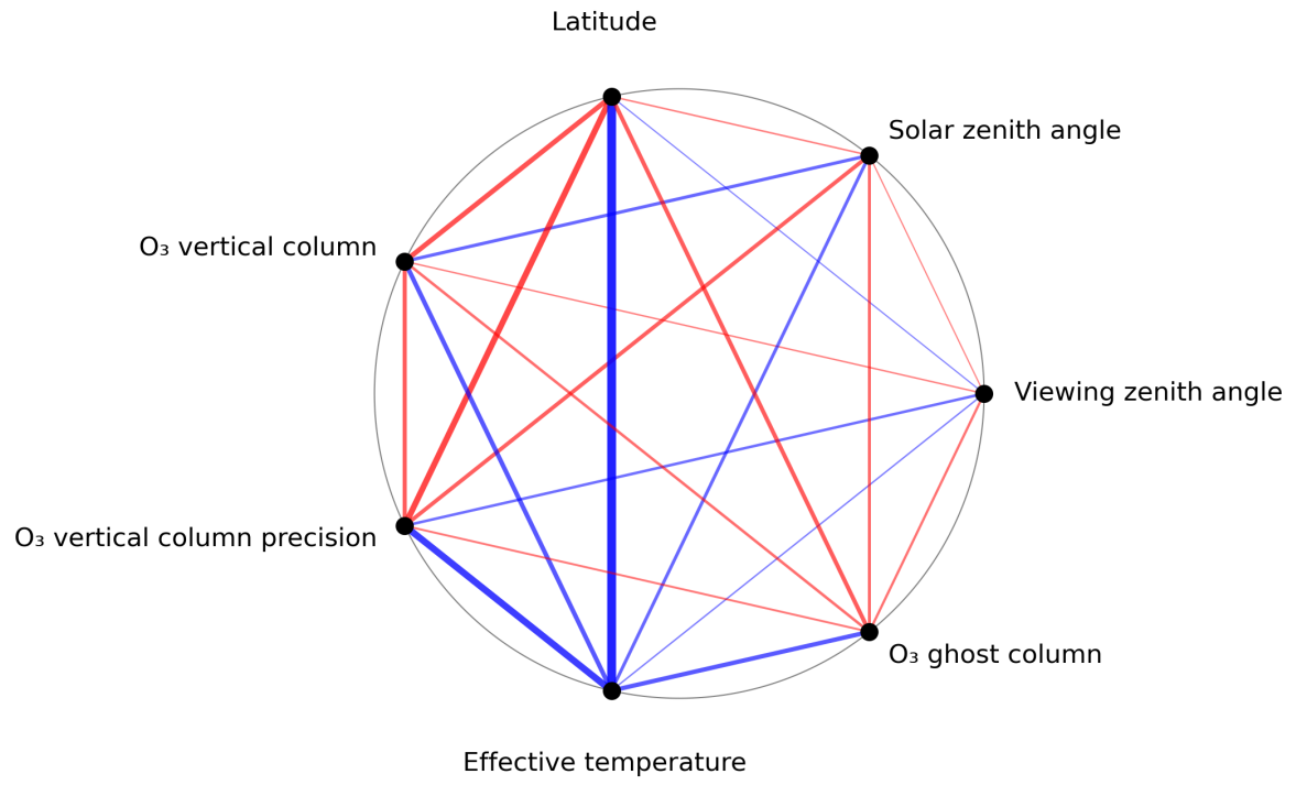
Figure 1: Map of correlation graph for 2023-11-04 to 2023-11-06.
