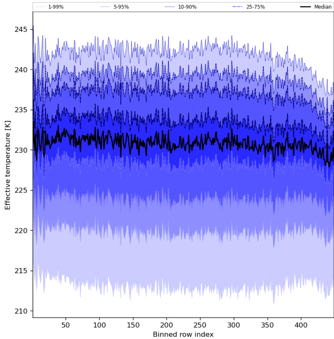
Figure 31: Along track statistics of “Effective temperature” for 2023-11-04 to 2023-11-06
