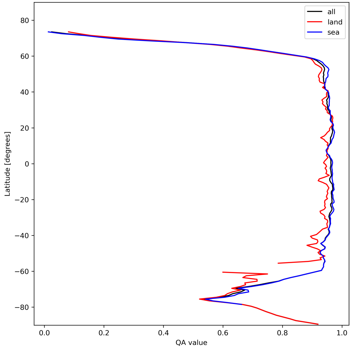
Figure 13: Zonal average of “QA value” for 2023-11-04 to 2023-11-06.
