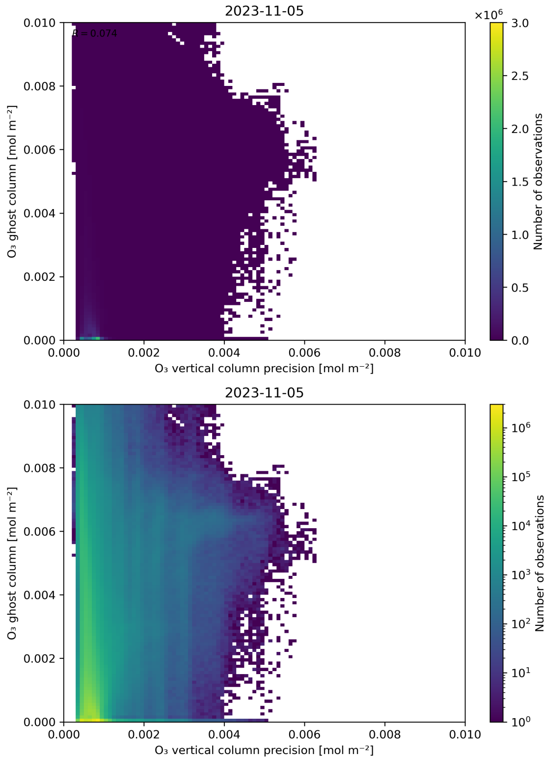
Figure 43: Scatter density plot of “ \text{O}_3 vertical column precision” against “ \text{O}_3 ghost column” for 2023-11-04 to 2023-11-06.
