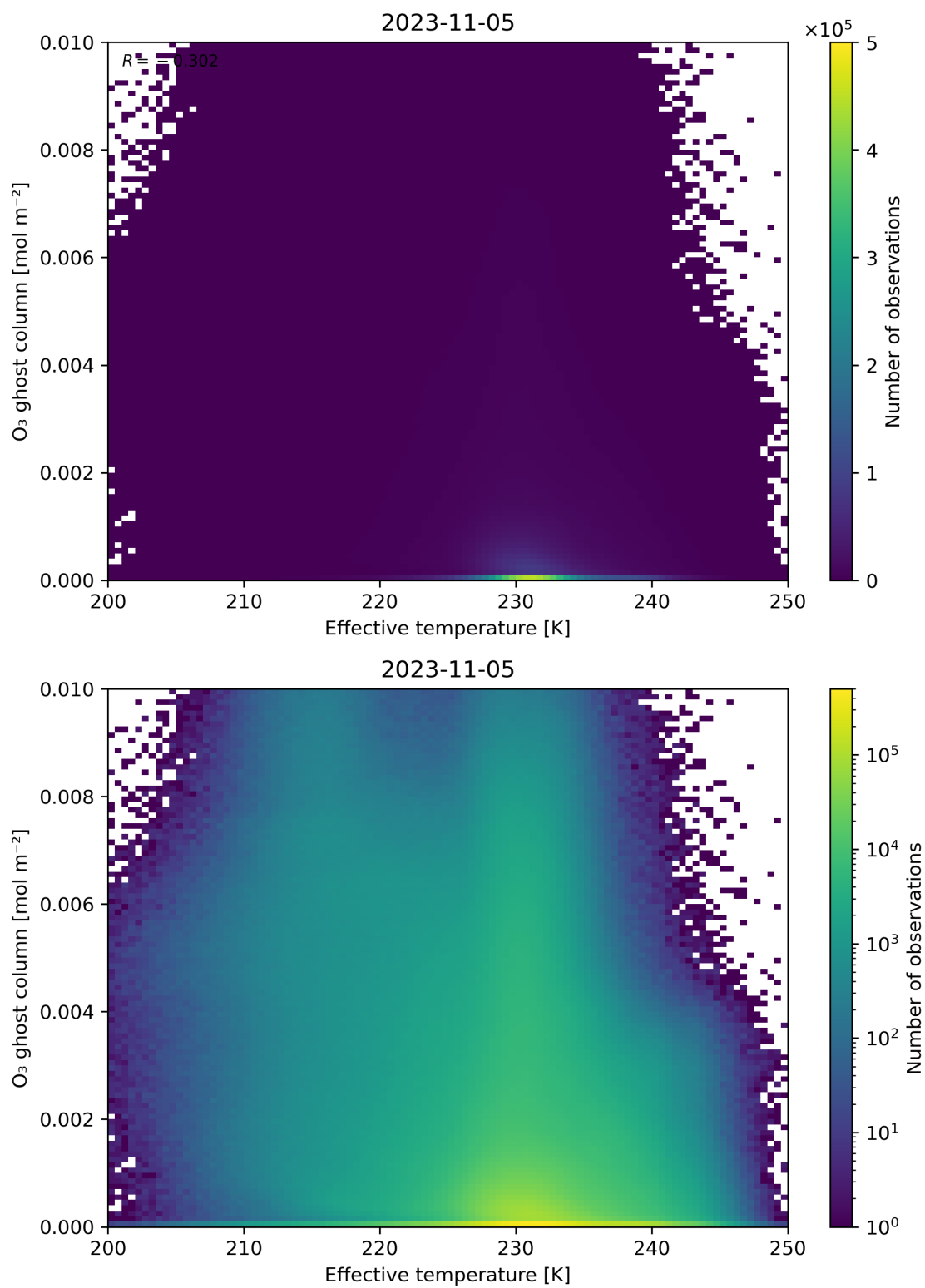
Figure 38: Scatter density plot of “Effective temperature” against “O 3 ghost column” for 2023-11-04 to 2023-11-06.
