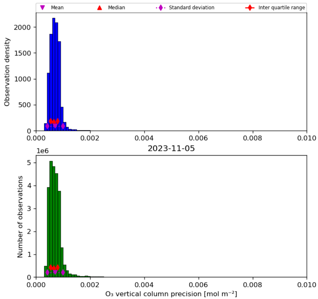
Figure 22: Histogram of “O 3 vertical column precision” for 2023-11-04 to 2023-11-06
