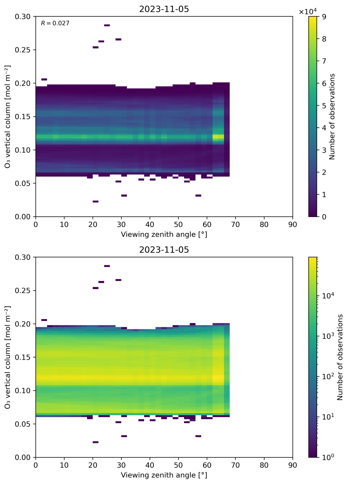
Figure 52: Scatter density plot of “Viewing zenith angle” against “O 3 vertical column” for 2023-11-04 to 2023-11-06.
