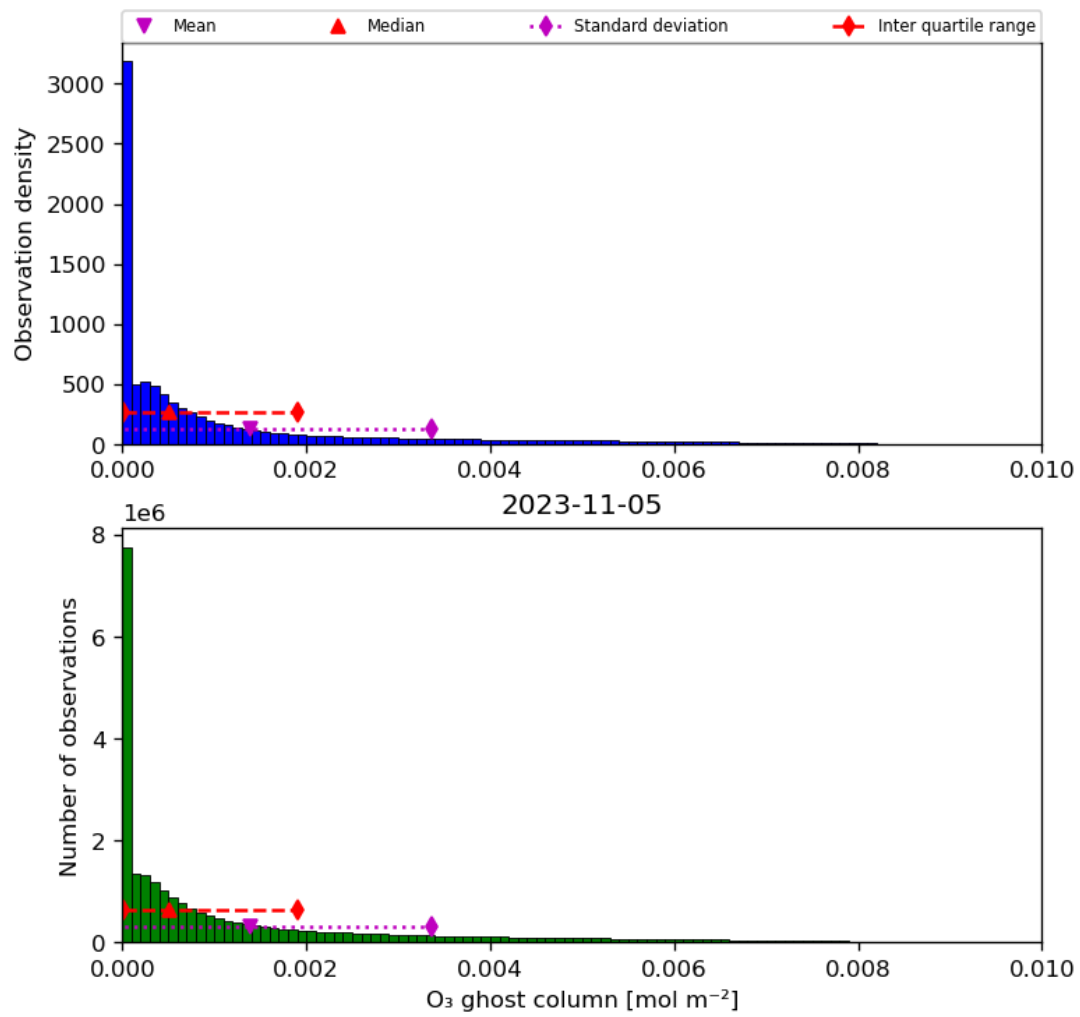
Figure 25: Histogram of “O 3 ghost column” for 2023-11-04 to 2023-11-06
