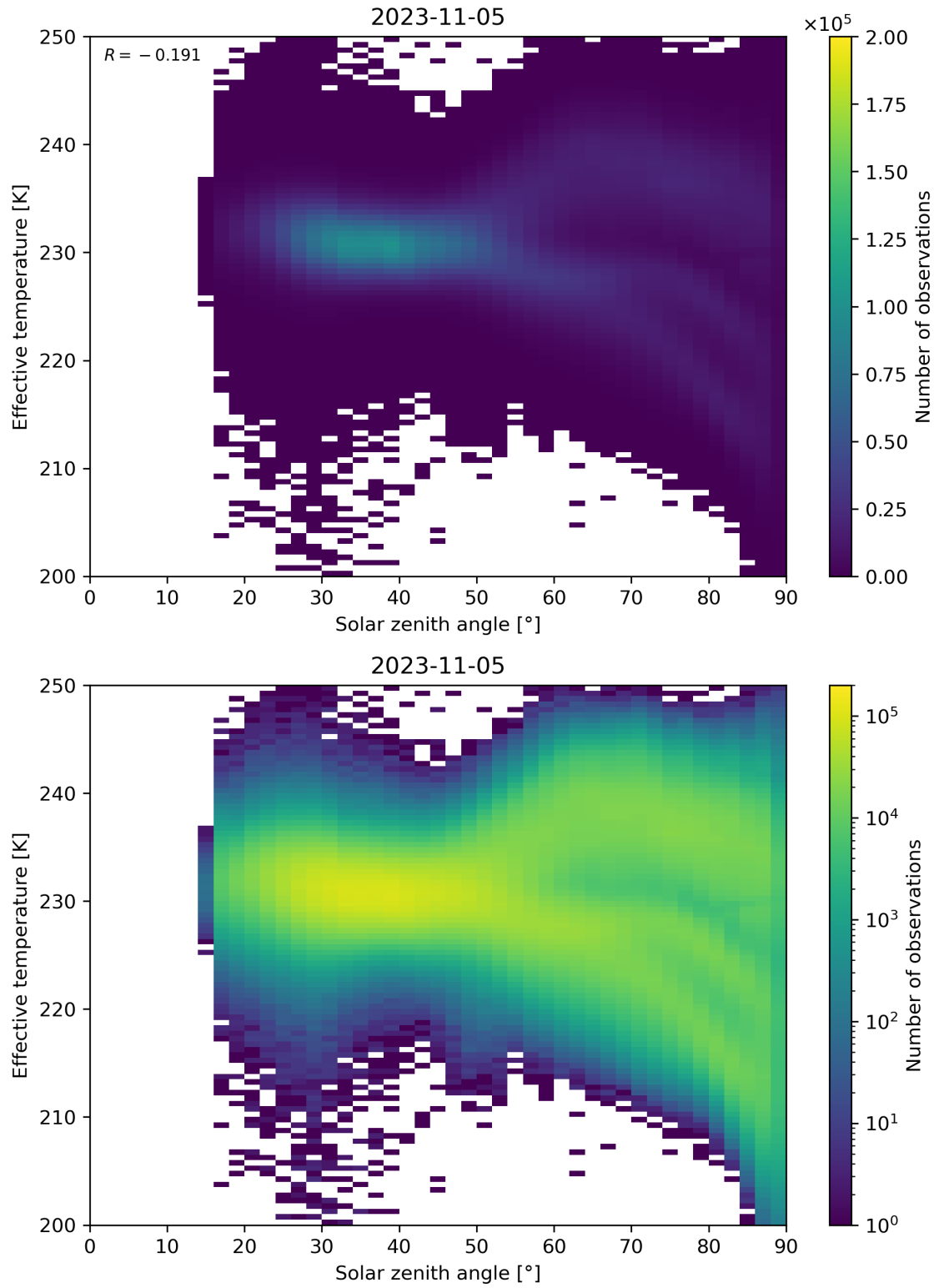
Figure 45: Scatter density plot of “Solar zenith angle” against “Effective temperature” for 2023-11-04 to 2023-11-06.
