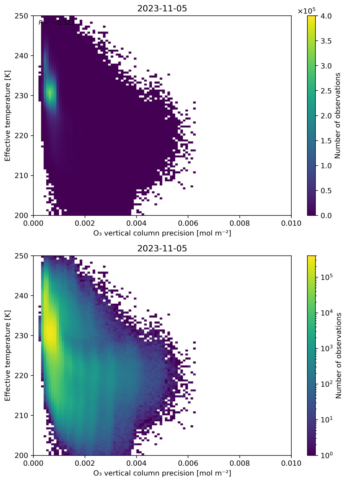
Figure 42: Scatter density plot of “O 3 vertical column precision” against “Effective temperature” for 2023-11-04 to 2023-11-06.
