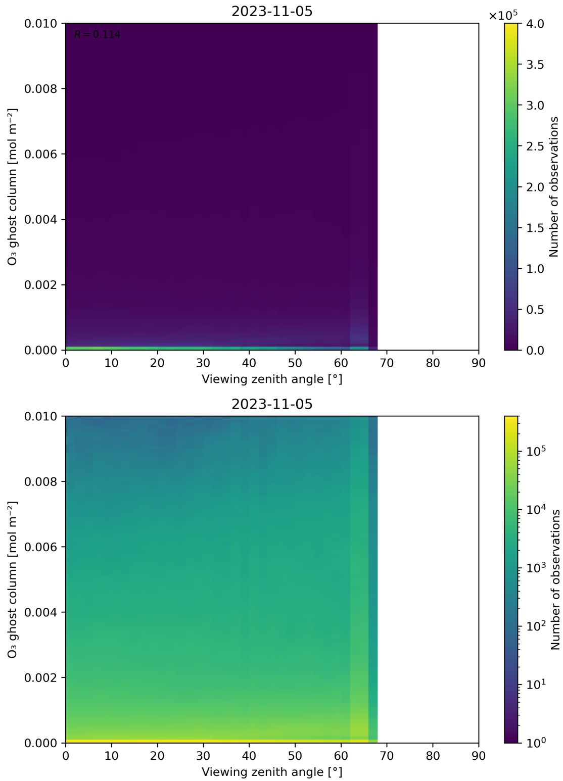
Figure 51: Scatter density plot of “Viewing zenith angle” against “O 3 ghost column” for 2023-11-04 to 2023-11-06.
