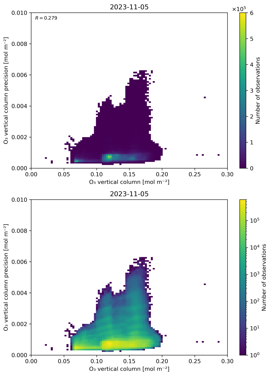
Figure 41: Scatter density plot of “O 3 vertical column” against “O 3 vertical column precision” for 2023-11-04 to 2023-11-06.
