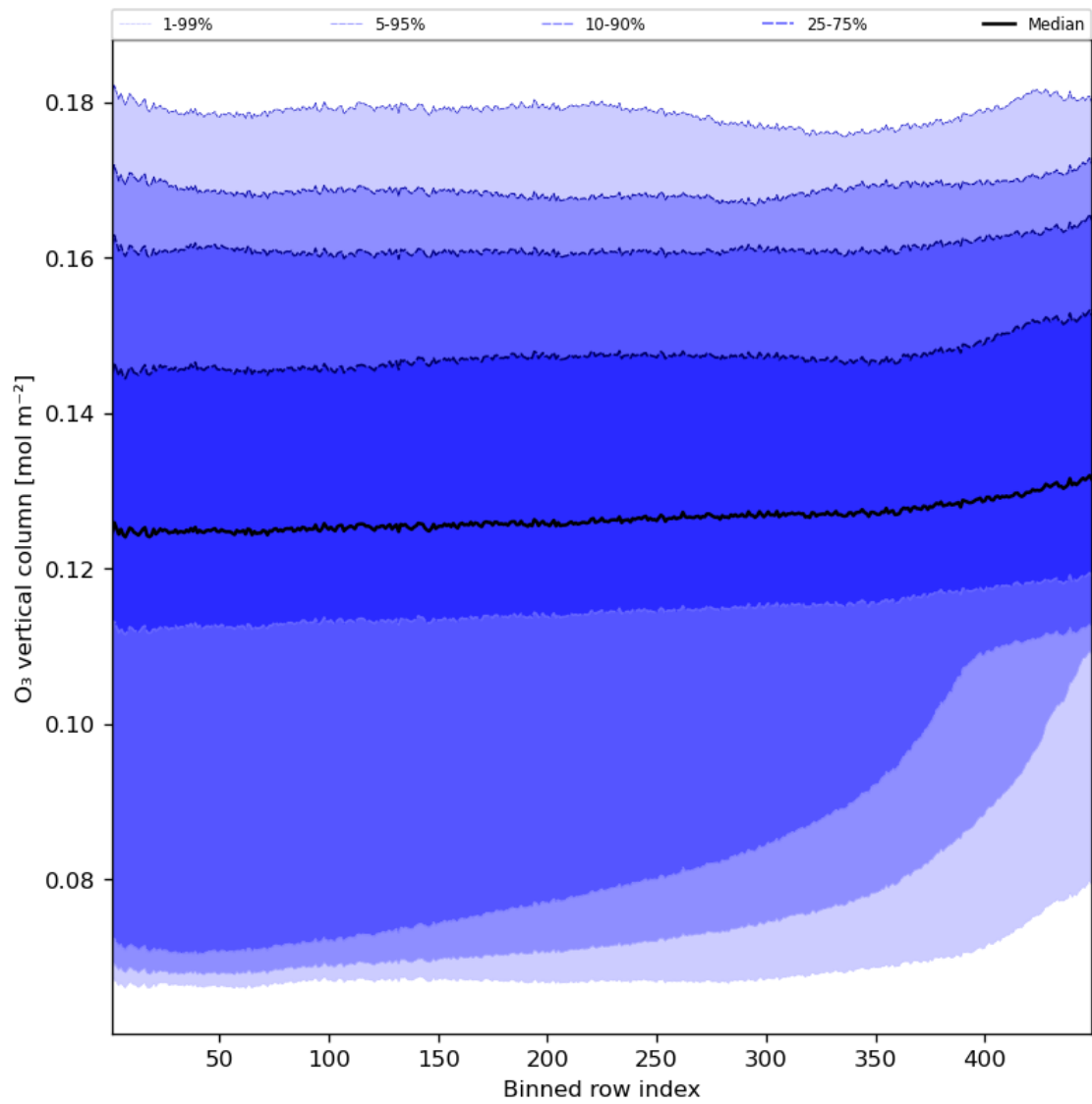
Figure 28: Along track statistics of “O 3 vertical column” for 2023-11-04 to 2023-11-06
