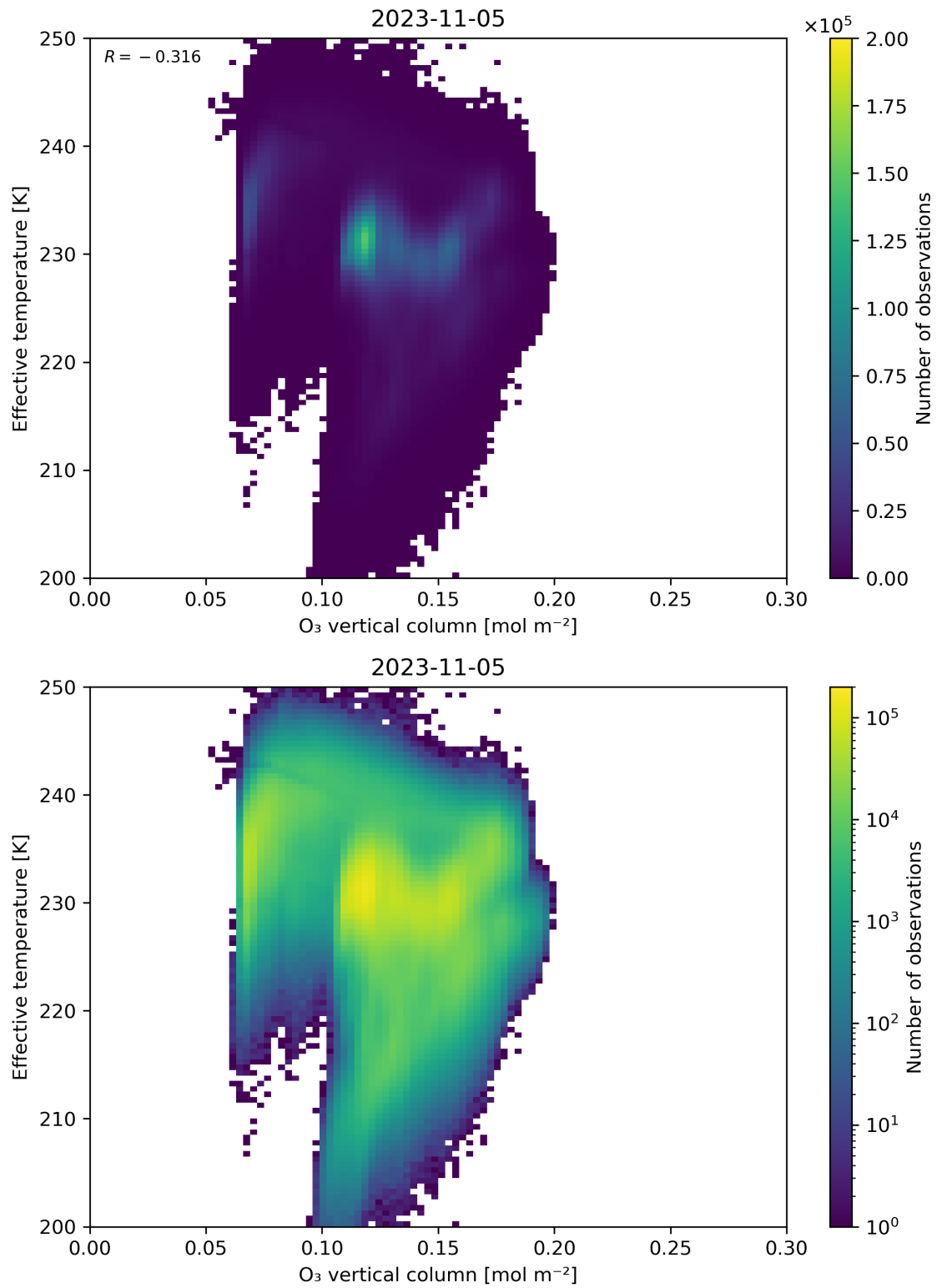
Figure 39: Scatter density plot of “O 3 vertical column” against “Effective temperature” for 2023-11-04 to 2023-11-06.
