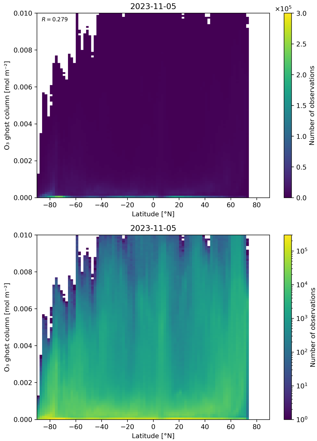
Figure 35: Scatter density plot of “Latitude” against “O 3 ghost column” for 2023-11-04 to 2023-11-06.
