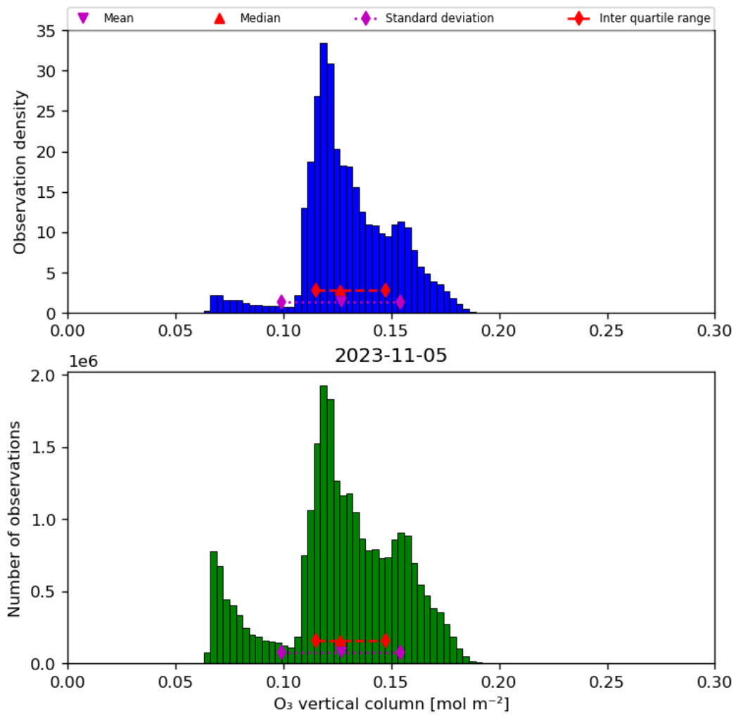
Figure 21: Histogram of “O 3 vertical column” for 2023-11-04 to 2023-11-06
