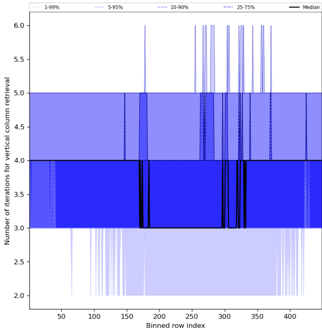
Figure 33: Along track statistics of “Number of iterations for vertical column retrieval” for 2023-11-04 to 2023-11-06
