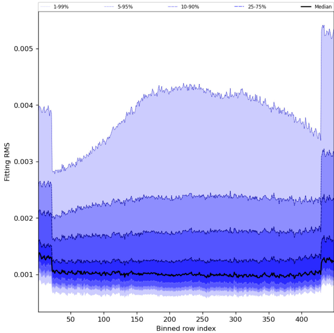
Figure 30: Along track statistics of “Fitting RMS” for 2023-11-04 to 2023-11-06
