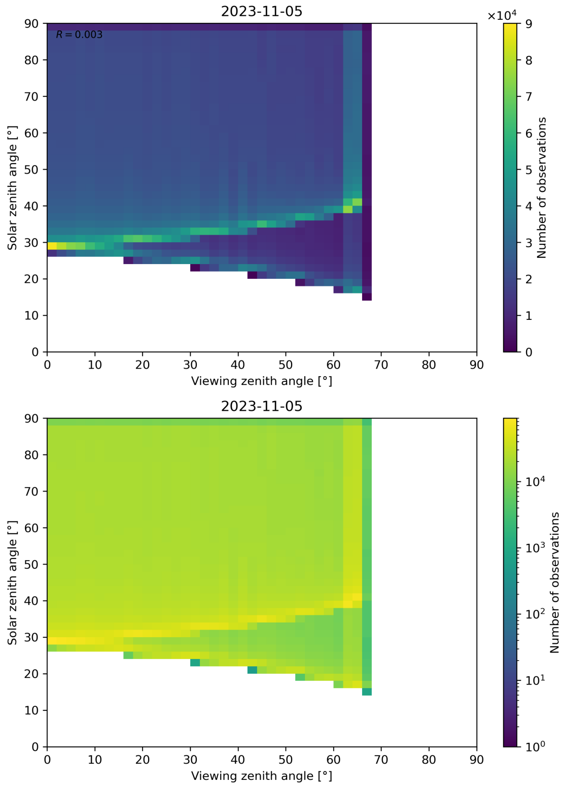
Figure 54: Scatter density plot of “Viewing zenith angle” against “Solar zenith angle” for 2023-11-04 to 2023-11-06.
