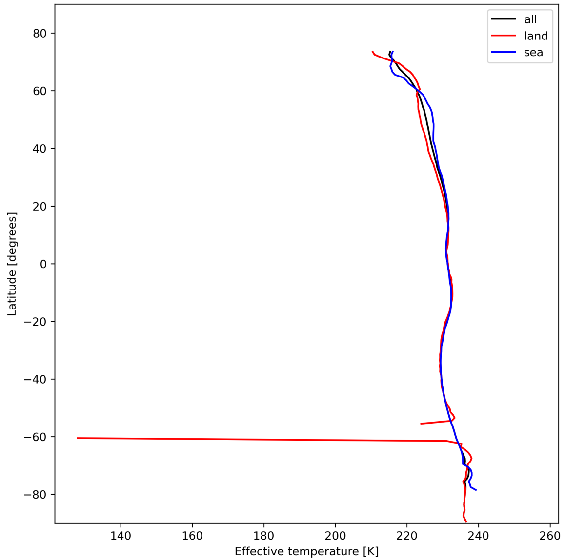
Figure 17: Zonal average of "Effective temperature" for 2023-11-04 to 2023-11-06.
