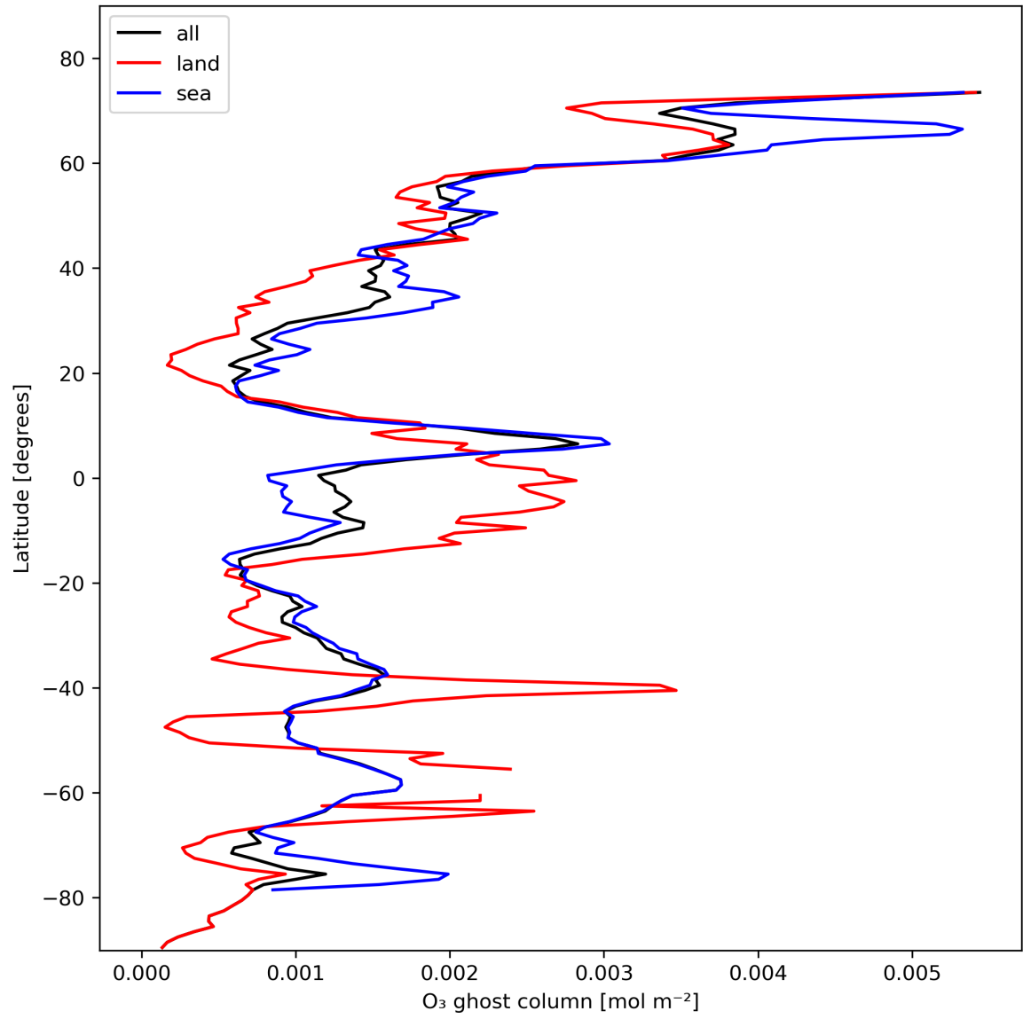
Figure 18: Zonal average of “O 3 ghost column” for 2023-11-04 to 2023-11-06.
