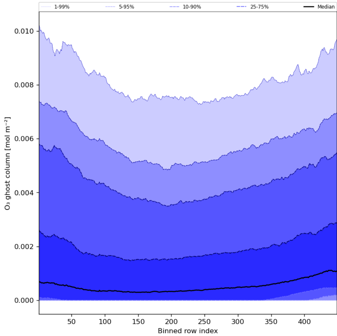
Figure 32: Along track statistics of “O 3 ghost column” for 2023-11-04 to 2023-11-06
