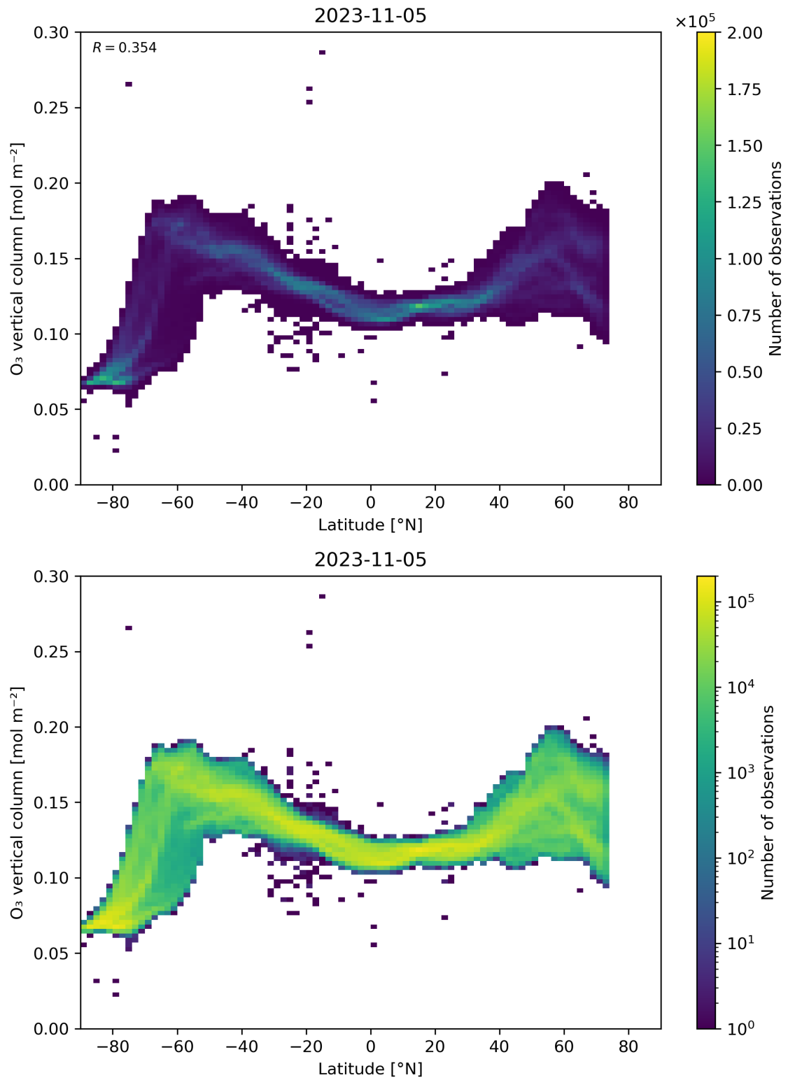
Figure 36: Scatter density plot of “Latitude” against “O 3 vertical column” for 2023-11-04 to 2023-11-06.
