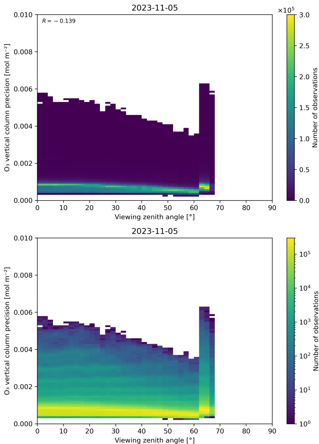
Figure 53: Scatter density plot of “Viewing zenith angle” against “O 3 vertical column precision” for 2023-11-04 to 2023-11-06.
