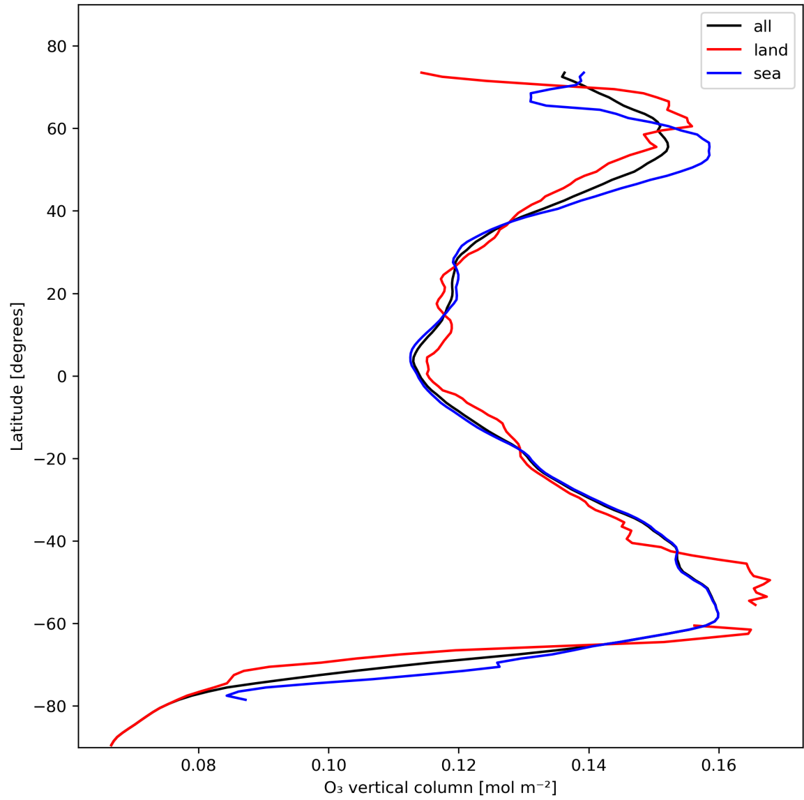
Figure 14: Zonal average of “O 3 vertical column” for 2023-11-04 to 2023-11-06.
