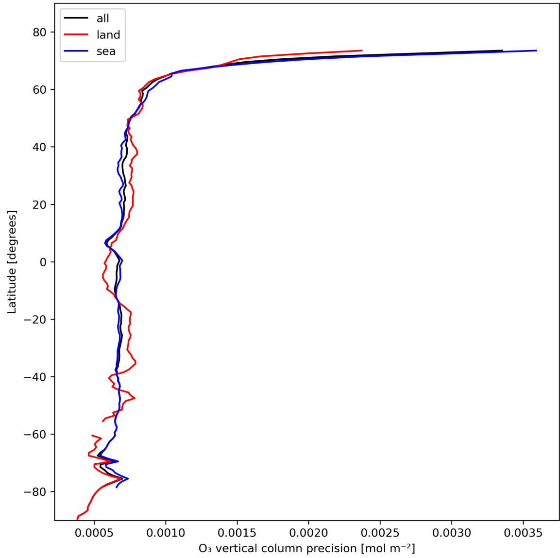
Figure 15: Zonal average of “O 3 vertical column precision” for 2023-11-04 to 2023-11-06.
