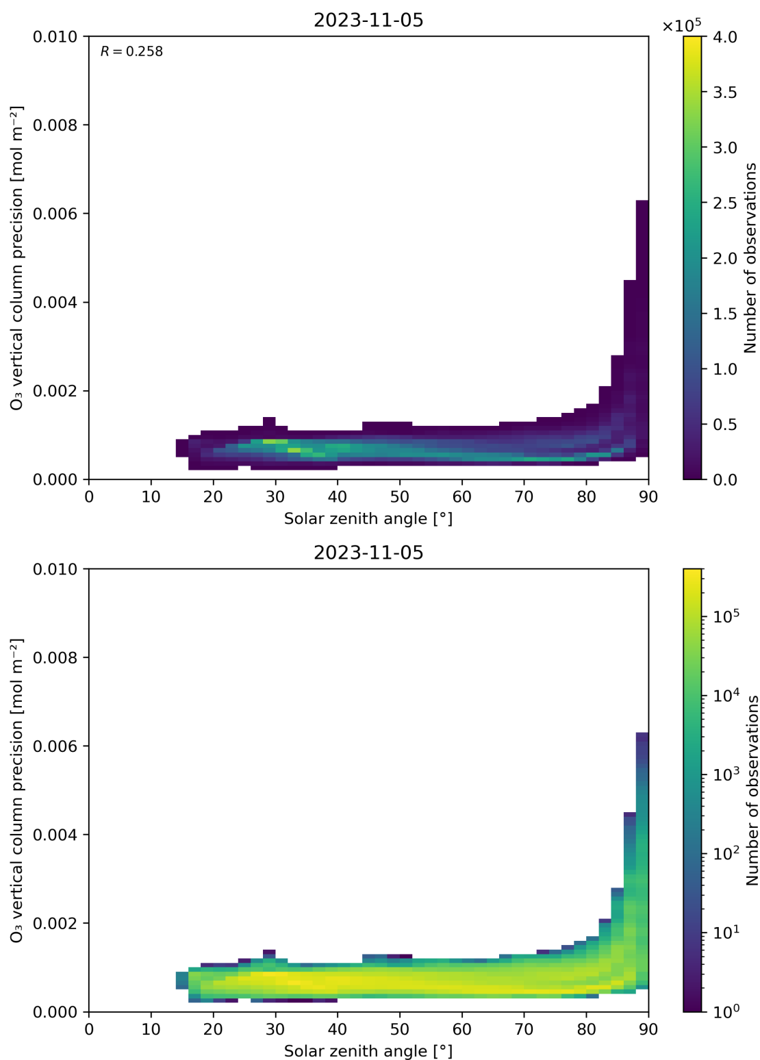
Figure 48: Scatter density plot of “Solar zenith angle” against “O 3 vertical column precision” for 2023-11-04 to 2023-11-06.
