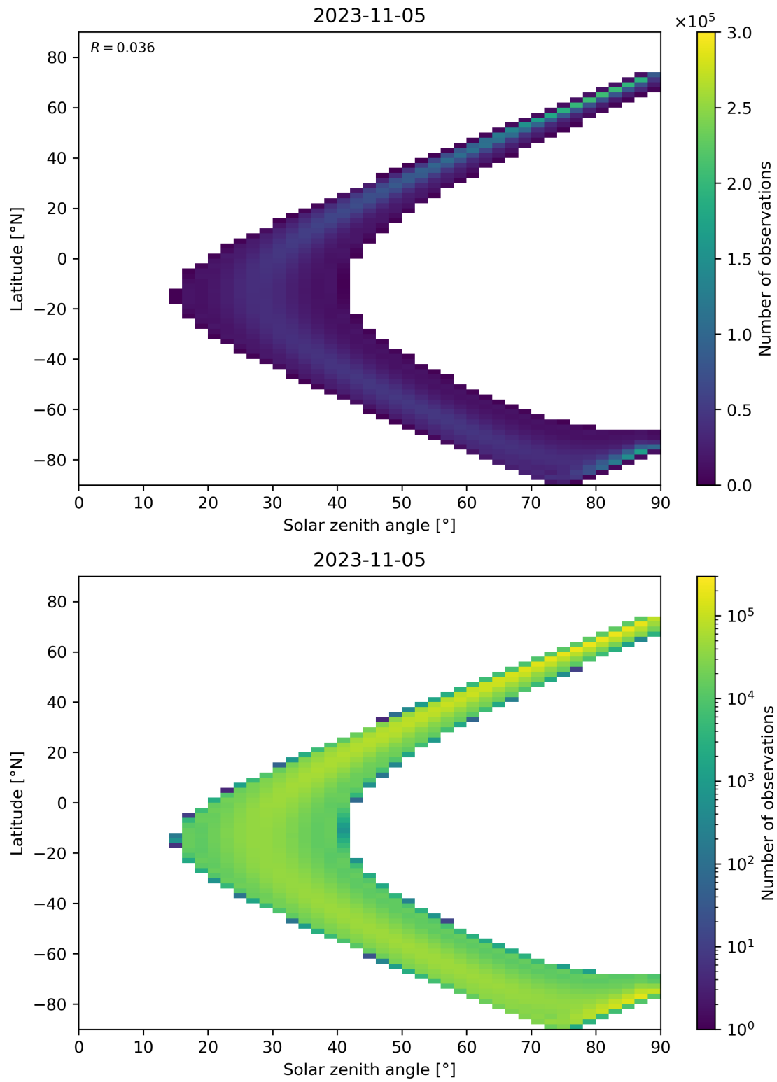
Figure 44: Scatter density plot of “Solar zenith angle” against “Latitude” for 2023-11-04 to 2023-11-06.
