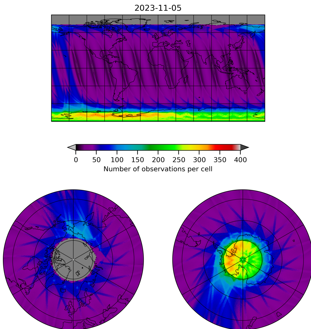
Figure 12: Map of the number of observations for 2023-11-04 to 2023-11-06
