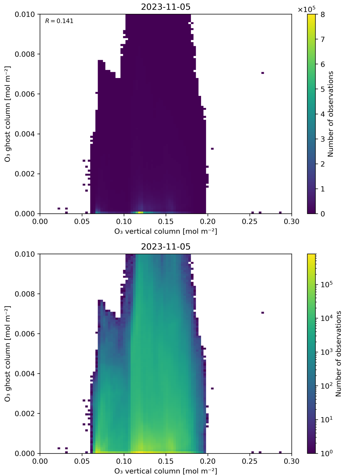
Figure 40: Scatter density plot of “O 3 vertical column” against “O 3 ghost column” for 2023-11-04 to 2023-11-06.
