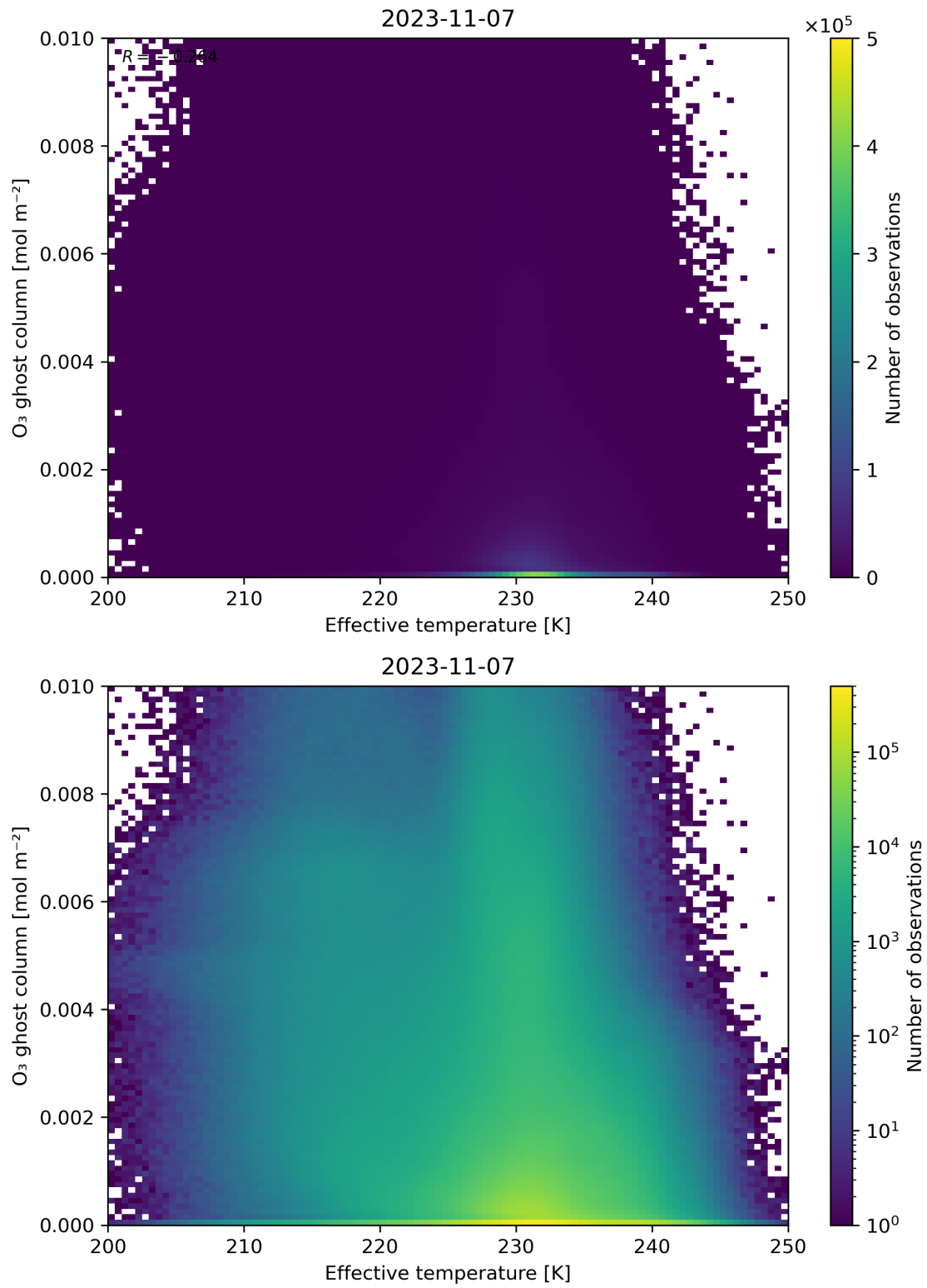
Figure 38: Scatter density plot of “Effective temperature” against “O 3 ghost column” for 2023-11-07 to 2023-11-08.
