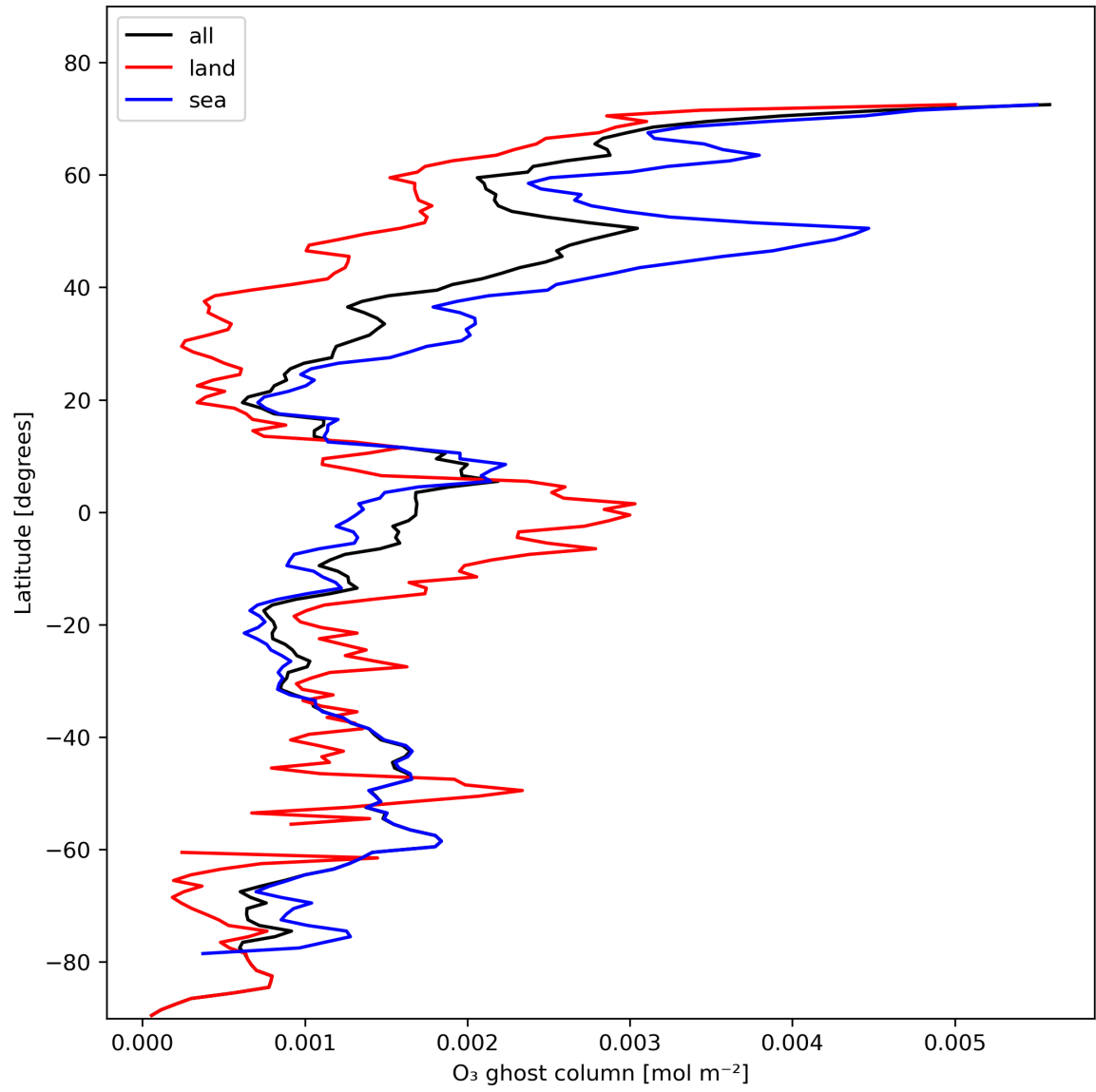
Figure 18: Zonal average of “O 3 ghost column” for 2023-11-07 to 2023-11-08.
