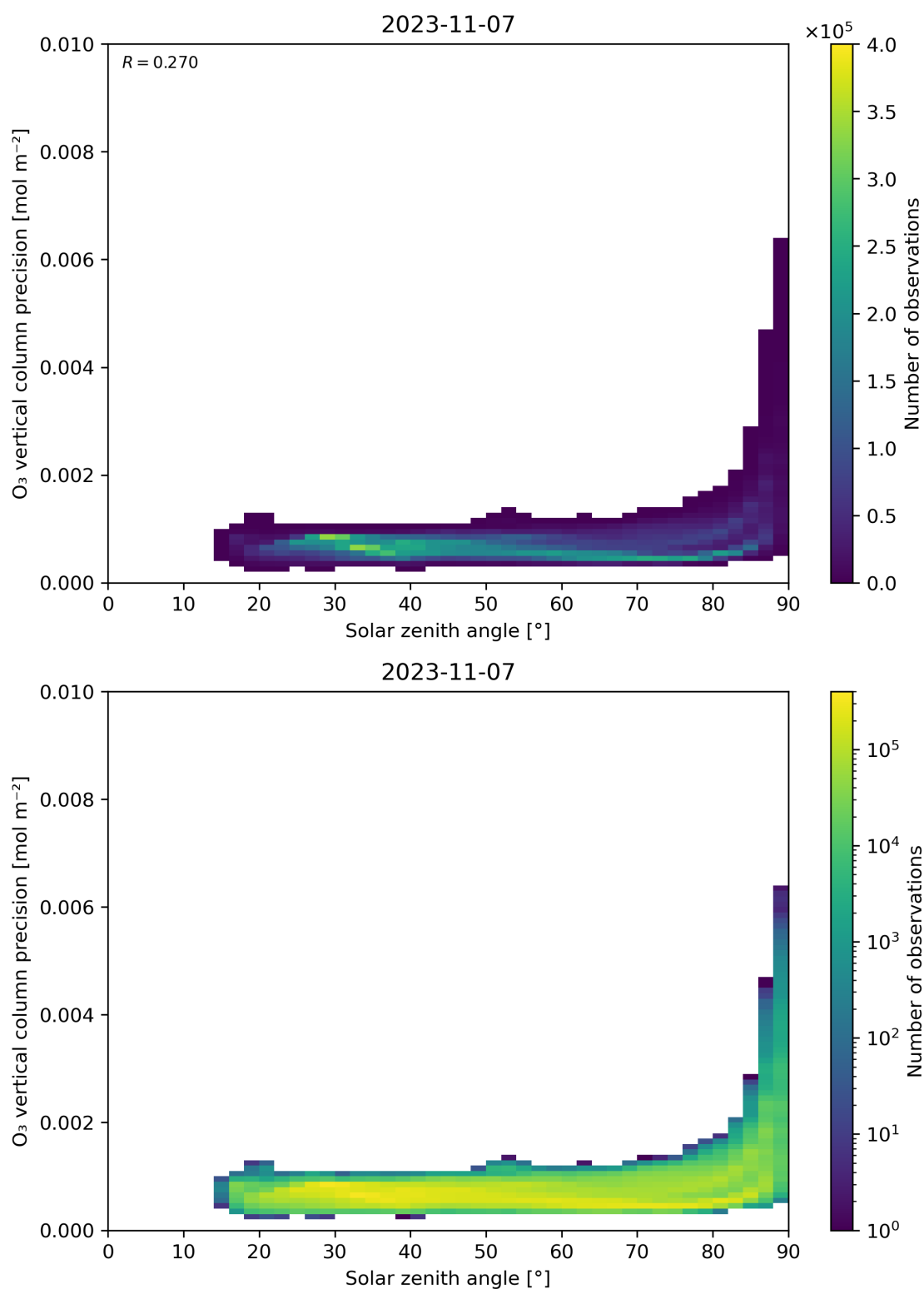
Figure 48: Scatter density plot of “Solar zenith angle” against “O 3 vertical column precision” for 2023-11-07 to 2023-11-08.
