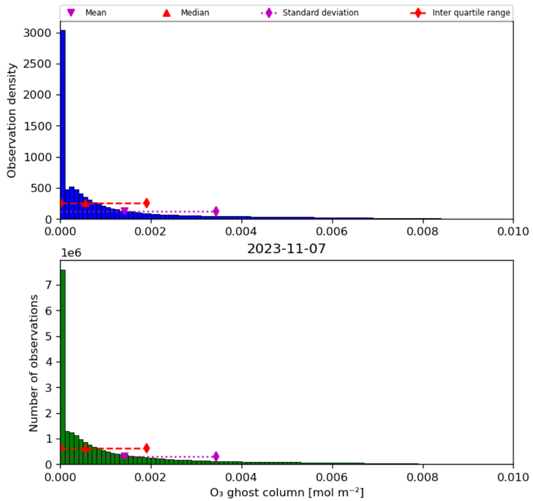
Figure 25: Histogram of “O 3 ghost column” for 2023-11-07 to 2023-11-08
