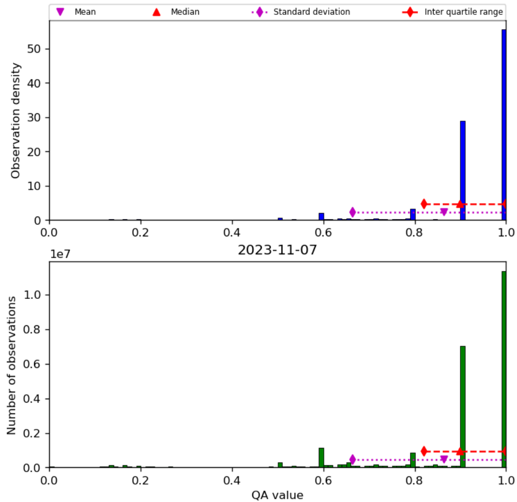
Figure 20: Histogram of “QA value” for 2023-11-07 to 2023-11-08
