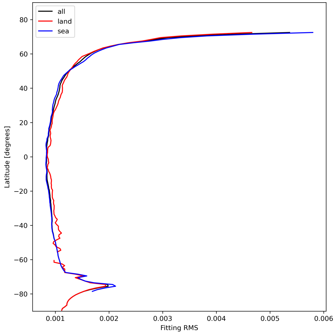
Figure 16: Zonal average of “Fitting RMS” for 2023-11-07 to 2023-11-08.
