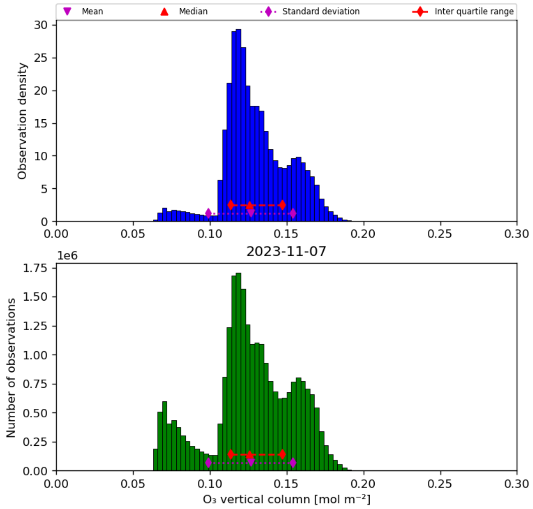
Figure 21: Histogram of “O 3 vertical column” for 2023-11-07 to 2023-11-08
