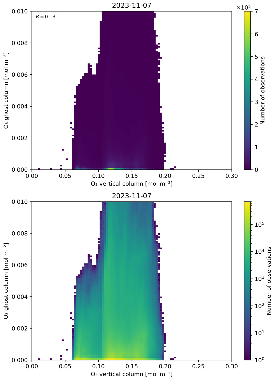
Figure 40: Scatter density plot of “O 3 vertical column” against “O 3 ghost column” for 2023-11-07 to 2023-11-08.
