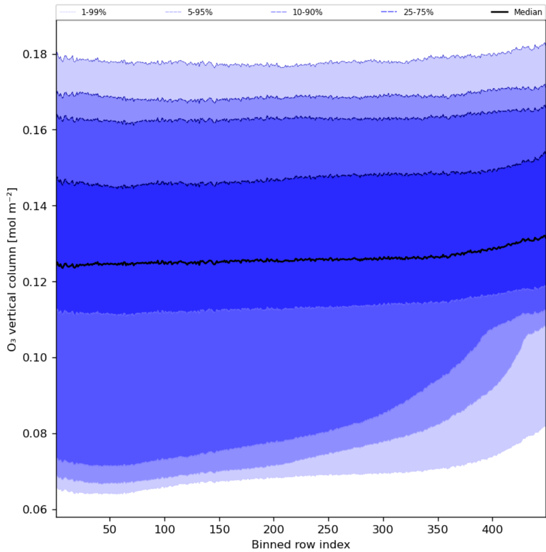
Figure 28: Along track statistics of “O 3 vertical column” for 2023-11-07 to 2023-11-08
