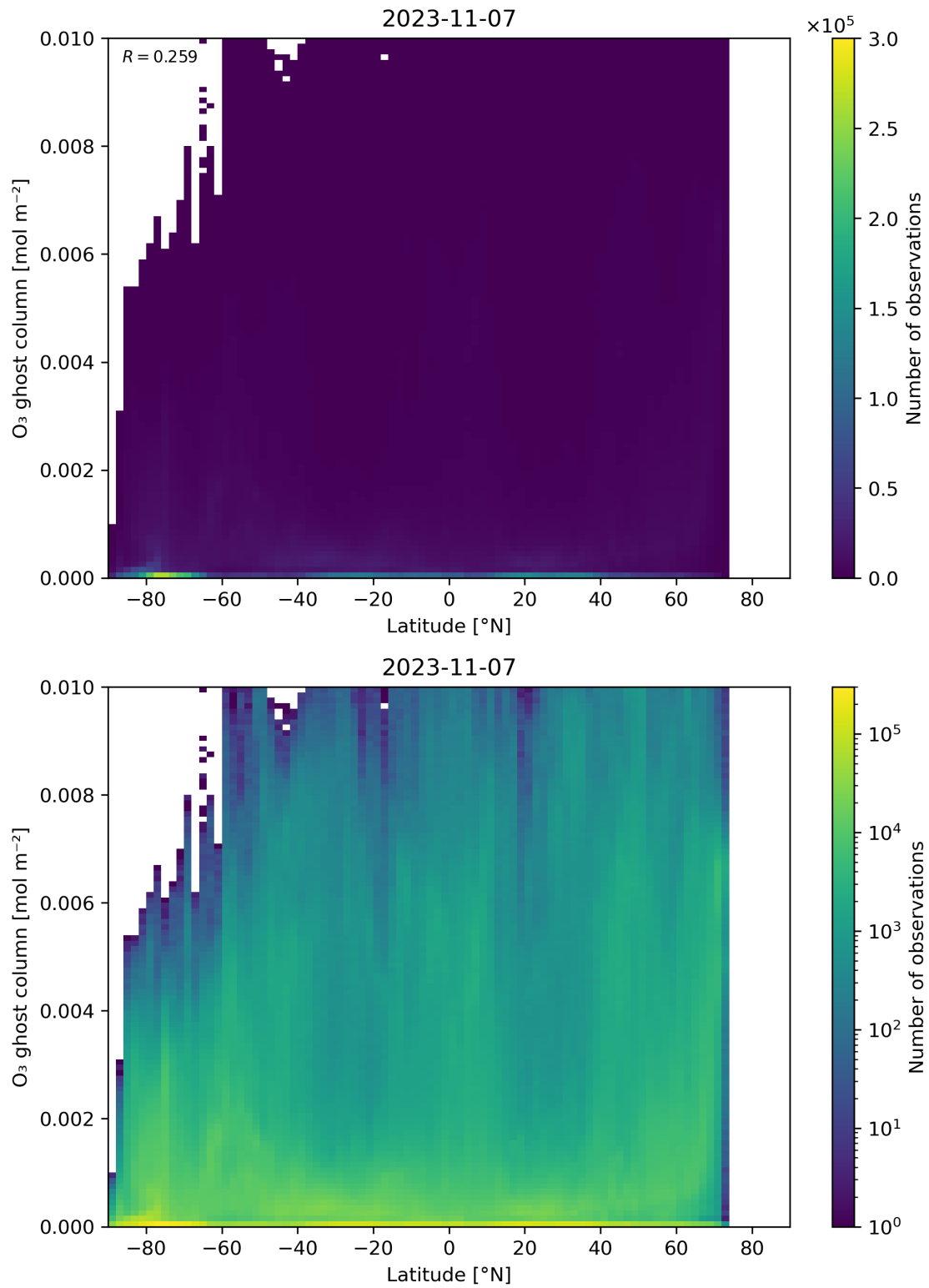
Figure 35: Scatter density plot of “Latitude” against “O 3 ghost column” for 2023-11-07 to 2023-11-08.
