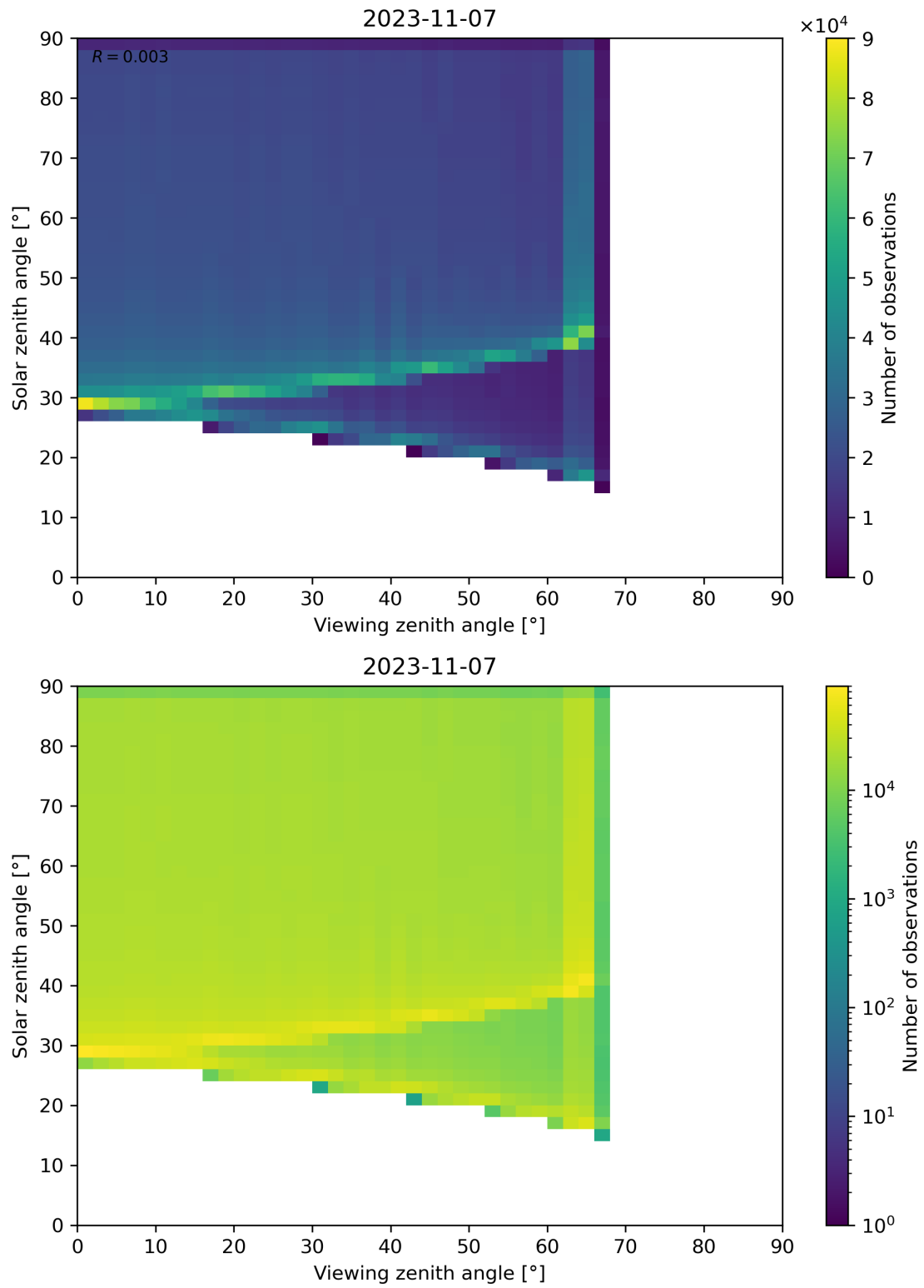
Figure 54: Scatter density plot of “Viewing zenith angle” against “Solar zenith angle” for 2023-11-07 to 2023-11-08.
