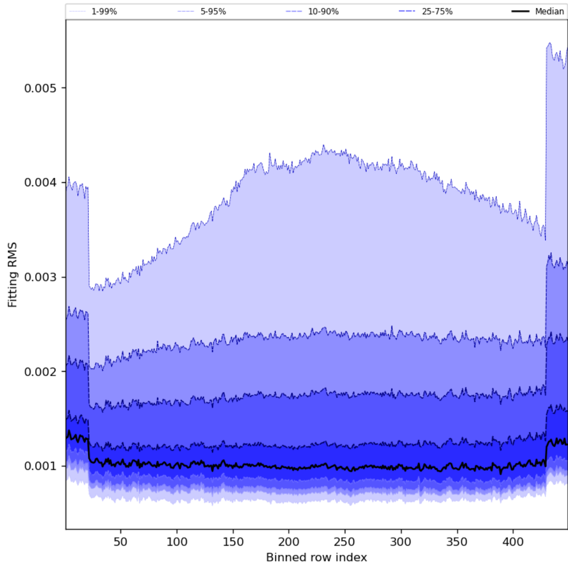
Figure 30: Along track statistics of “Fitting RMS” for 2023-11-07 to 2023-11-08
