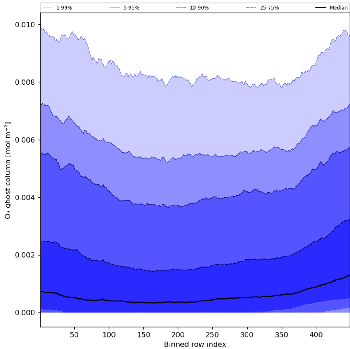
Figure 32: Along track statistics of “O 3 ghost column” for 2023-11-07 to 2023-11-08
