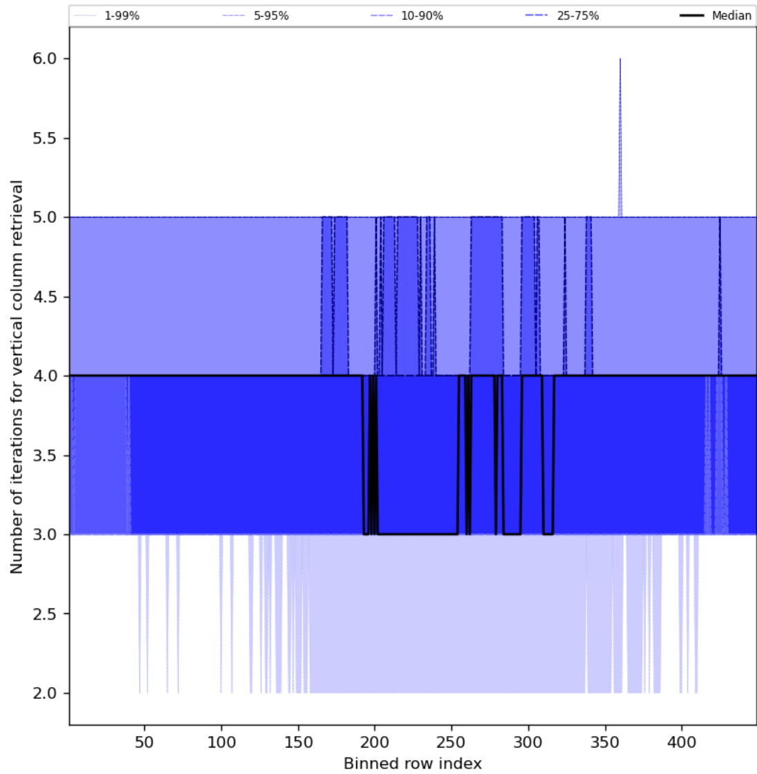
Figure 33: Along track statistics of “Number of iterations for vertical column retrieval” for 2023-11-07 to 2023-11-08
