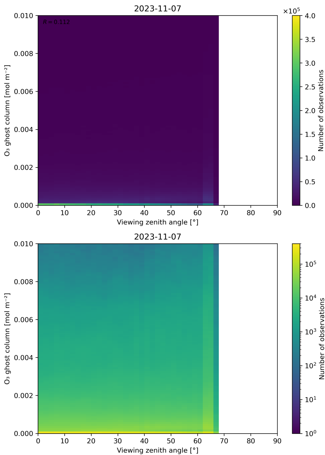
Figure 51: Scatter density plot of “Viewing zenith angle” against “O 3 ghost column” for 2023-11-07 to 2023-11-08.
