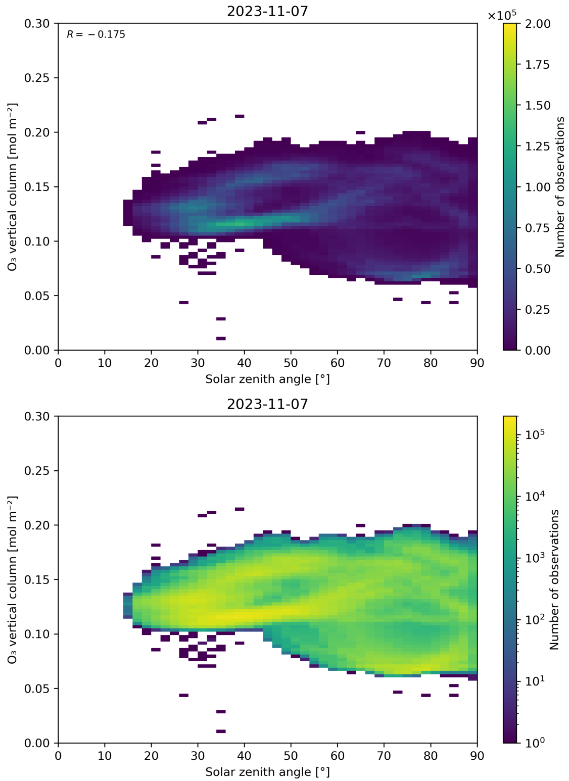
Figure 47: Scatter density plot of “Solar zenith angle” against “O 3 vertical column” for 2023-11-07 to 2023-11-08.
