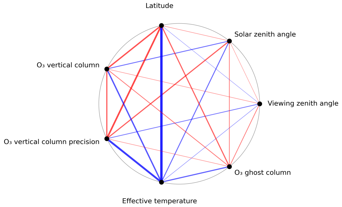
Figure 1: Map of correlation graph for 2023-11-07 to 2023-11-08.
