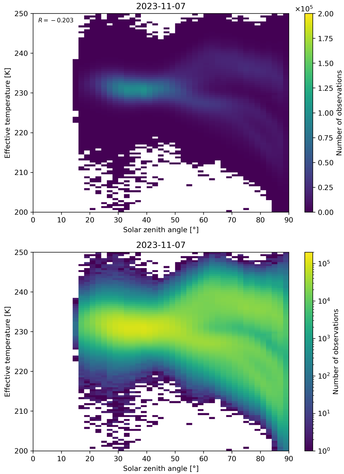
Figure 45: Scatter density plot of “Solar zenith angle” against “Effective temperature” for 2023-11-07 to 2023-11-08.
