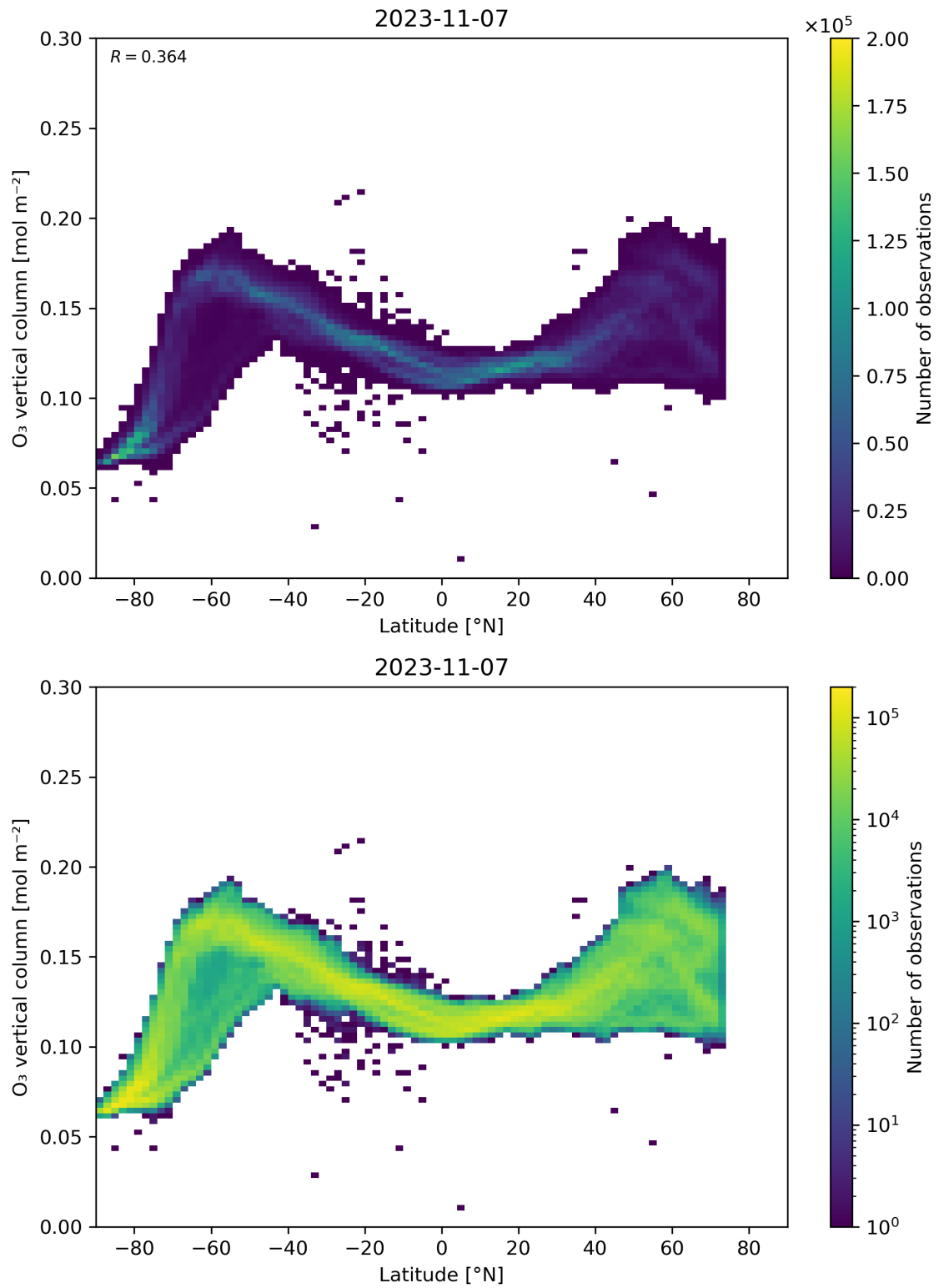
Figure 36: Scatter density plot of “Latitude” against “O 3 vertical column” for 2023-11-07 to 2023-11-08.
