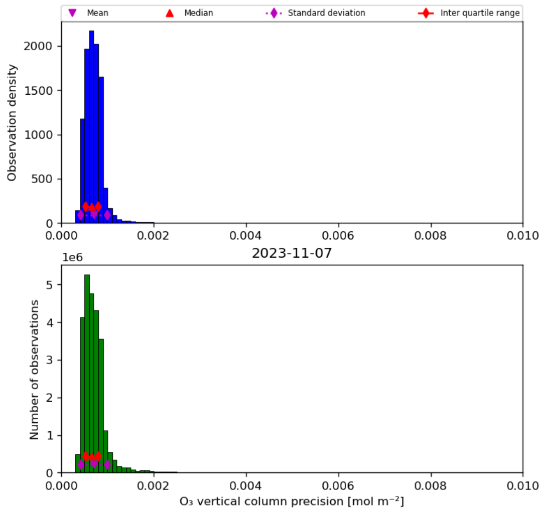
Figure 22: Histogram of “O 3 vertical column precision” for 2023-11-07 to 2023-11-08
