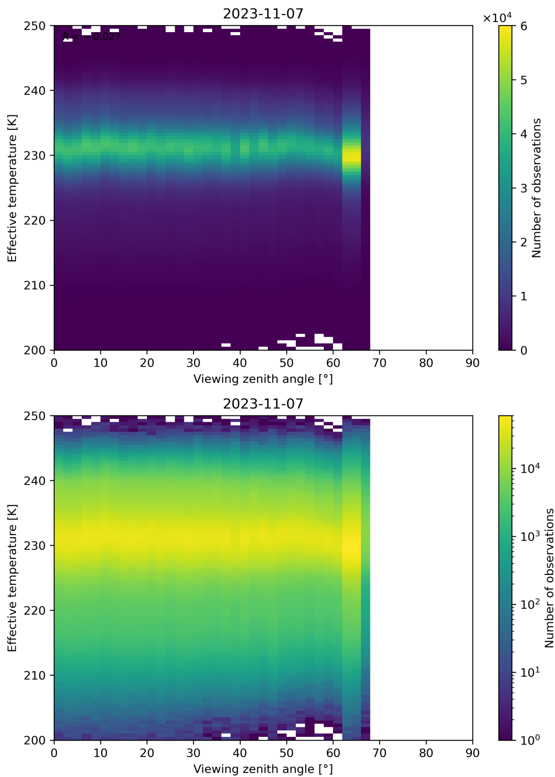
Figure 50: Scatter density plot of “Viewing zenith angle” against “Effective temperature” for 2023-11-07 to 2023-11-08.
