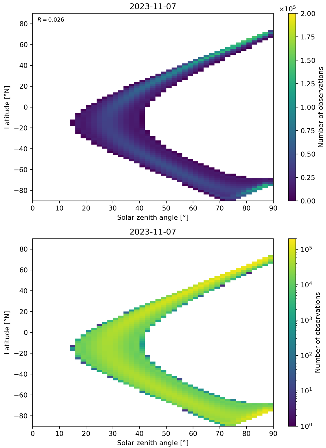
Figure 44: Scatter density plot of “Solar zenith angle” against “Latitude” for 2023-11-07 to 2023-11-08.
