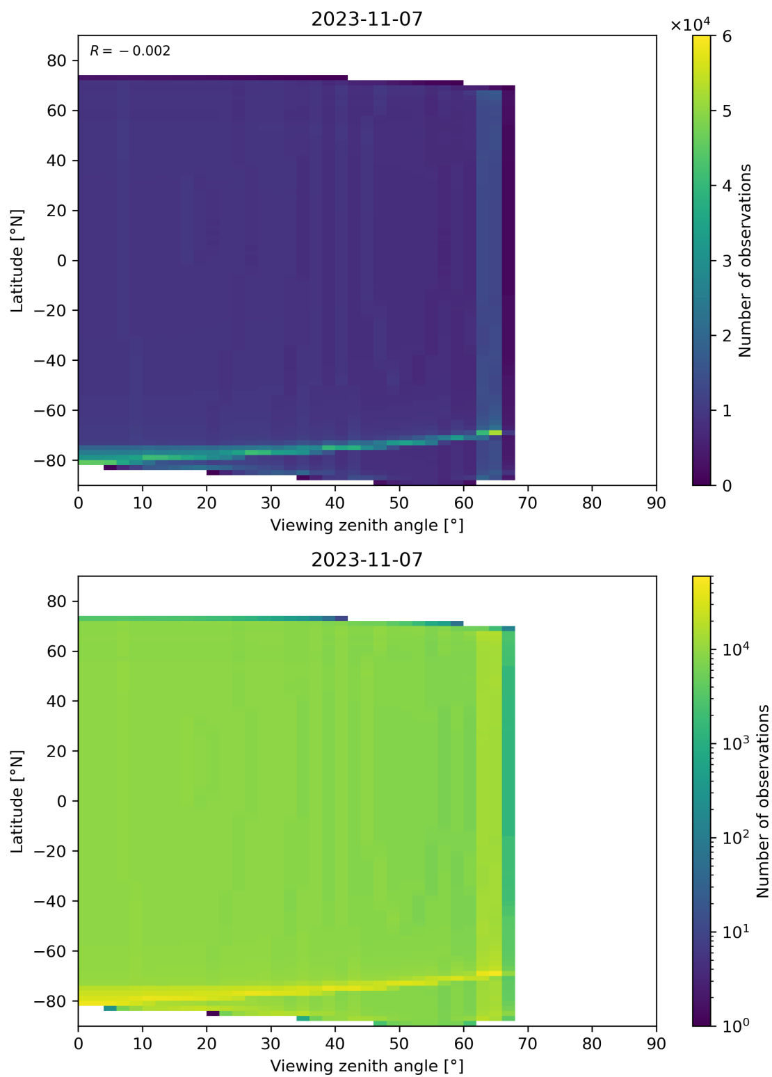
Figure 49: Scatter density plot of “Viewing zenith angle” against “Latitude” for 2023-11-07 to 2023-11-08.
