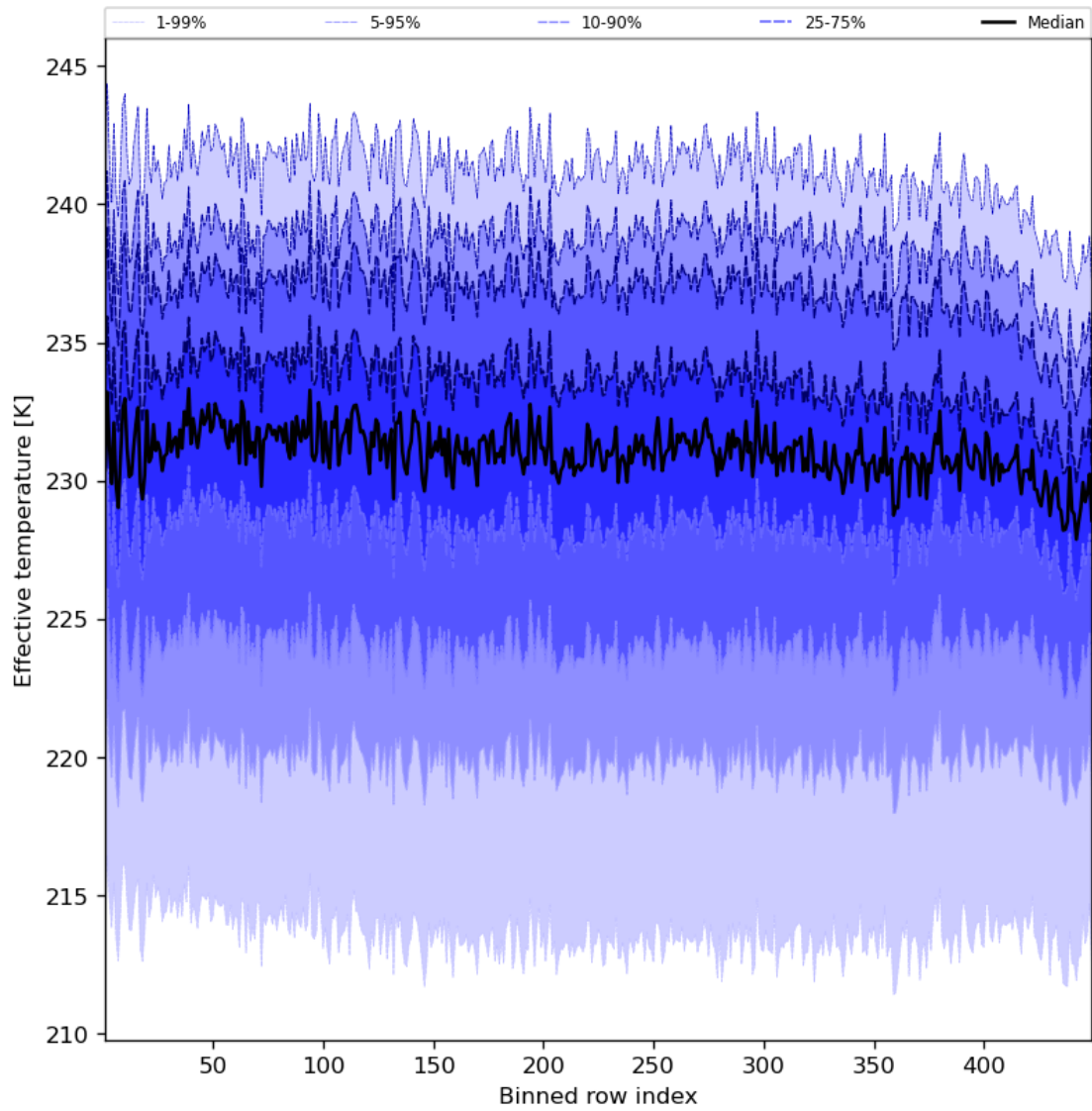
Figure 31: Along track statistics of “Effective temperature” for 2023-11-07 to 2023-11-08
