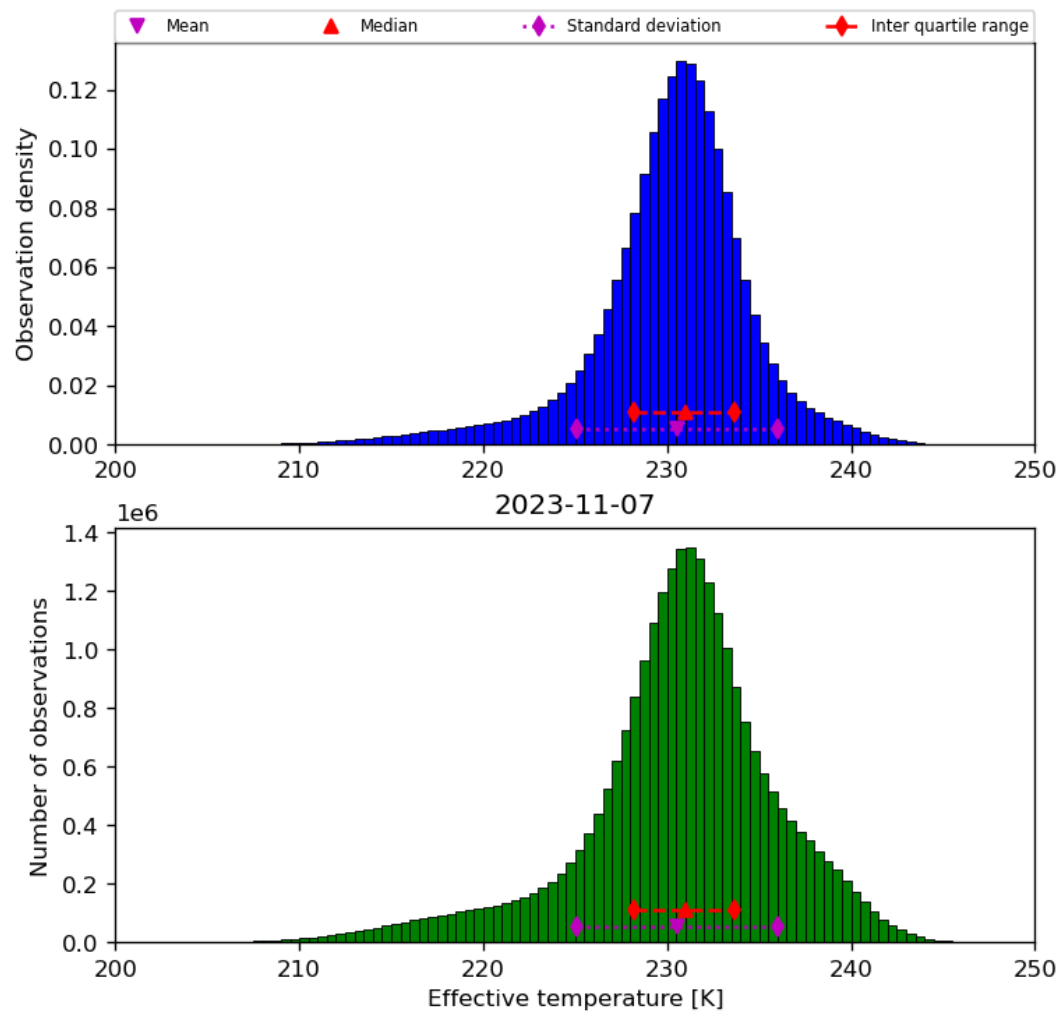
Figure 24: Histogram of “Effective temperature” for 2023-11-07 to 2023-11-08
