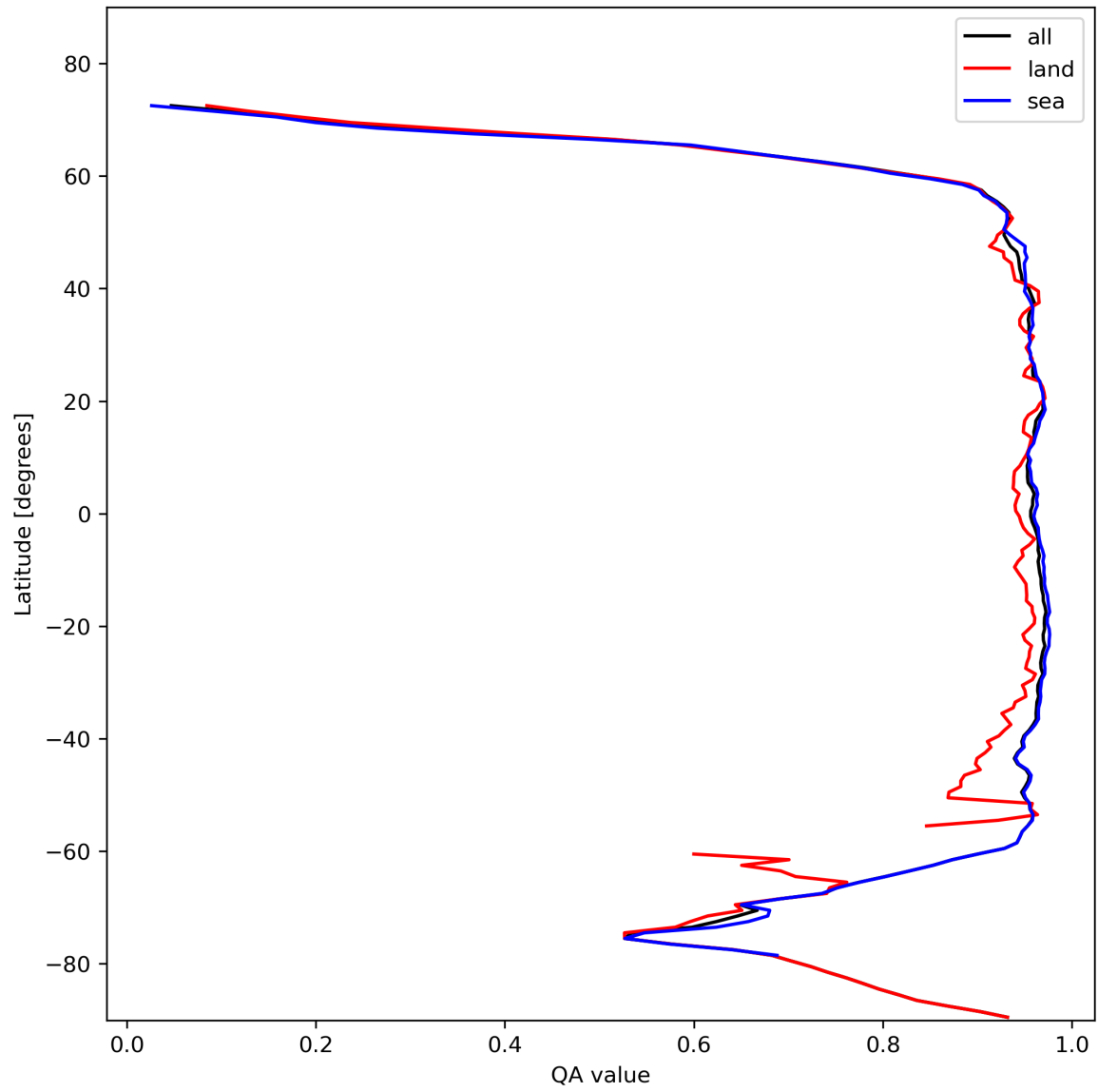
Figure 13: Zonal average of “QA value” for 2023-11-07 to 2023-11-08.
