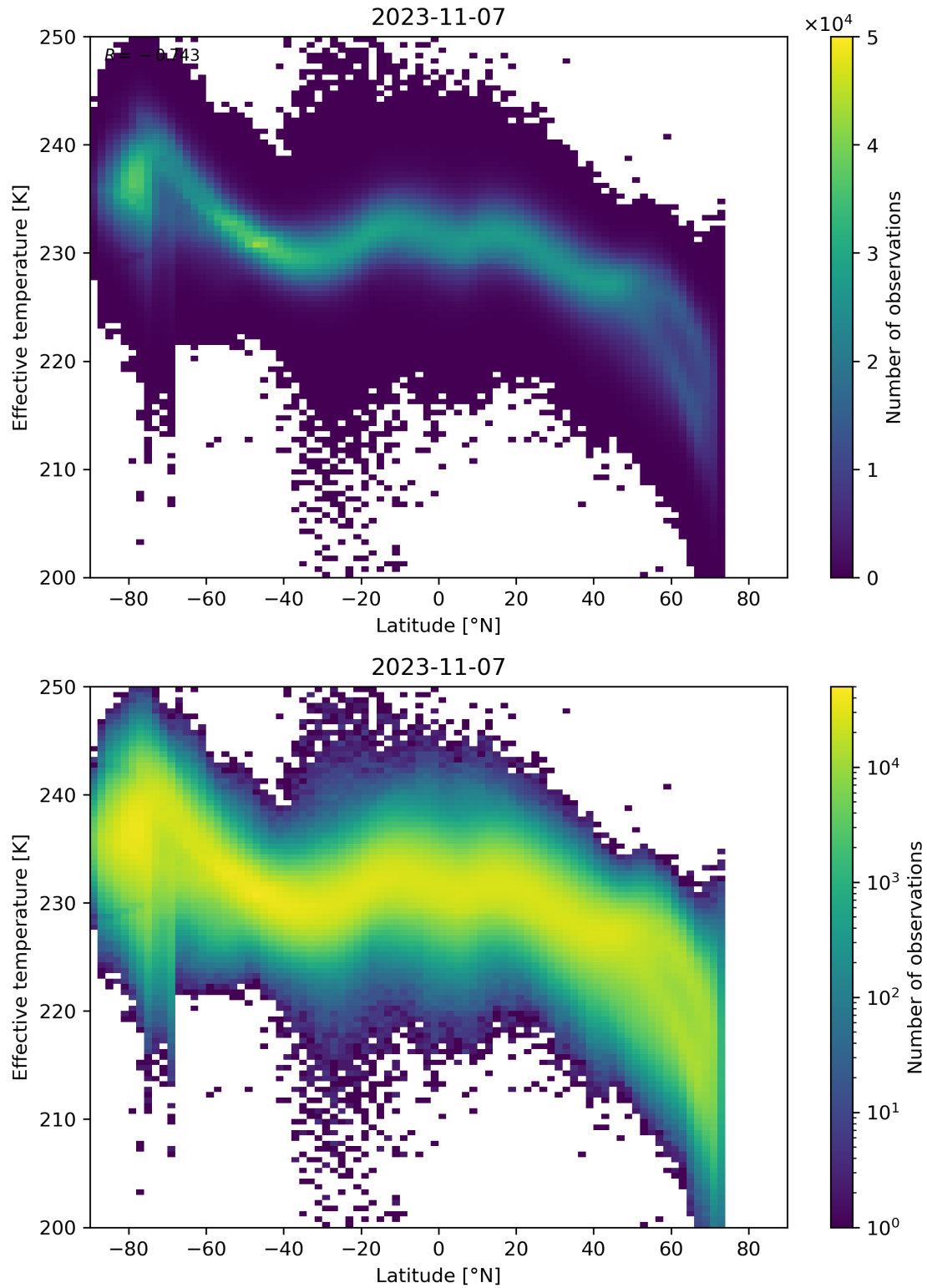
Figure 34: Scatter density plot of “Latitude” against “Effective temperature” for 2023-11-07 to 2023-11-08.
