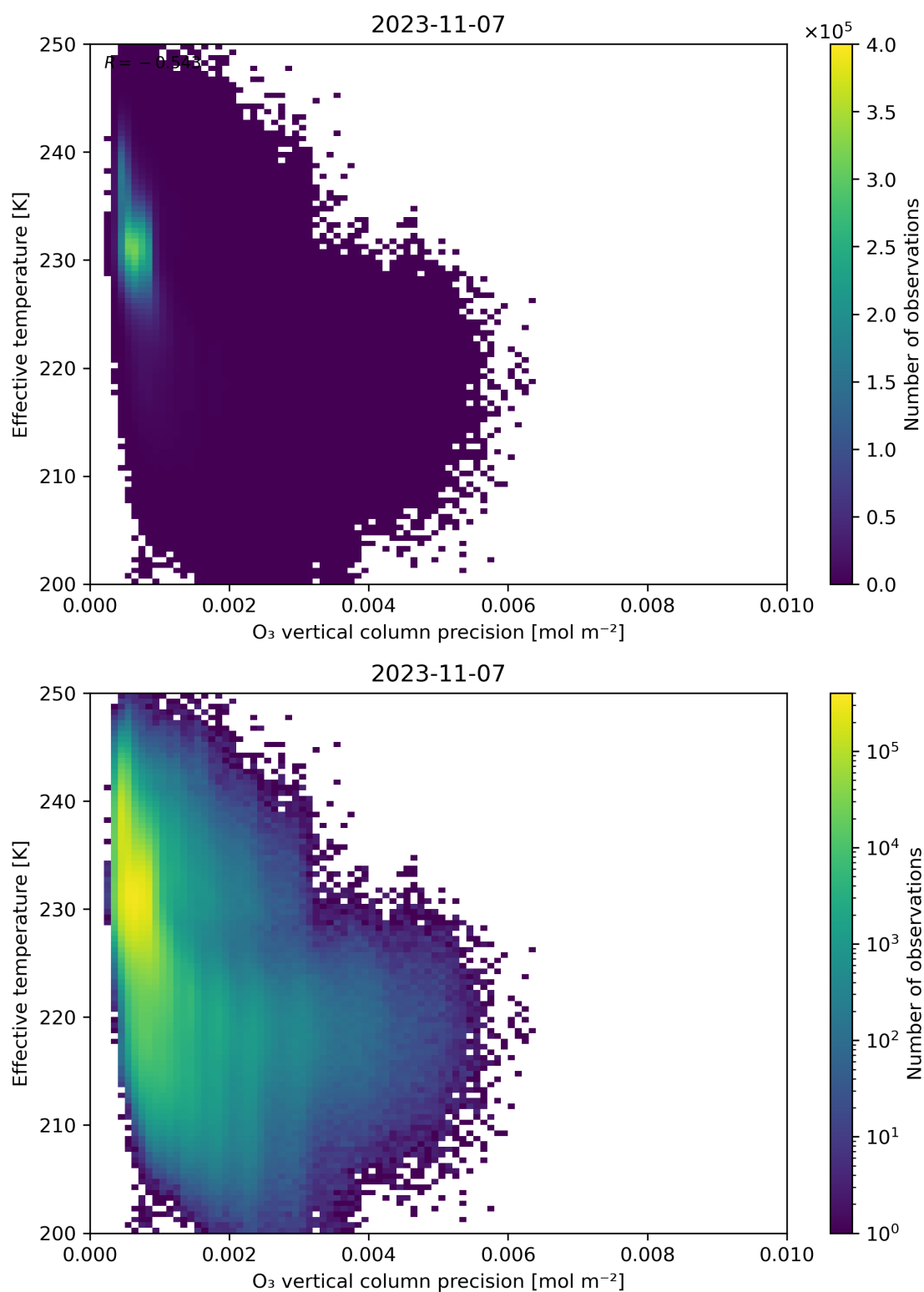
Figure 42: Scatter density plot of “O 3 vertical column precision” against “Effective temperature” for 2023-11-07 to 2023-11-08.
