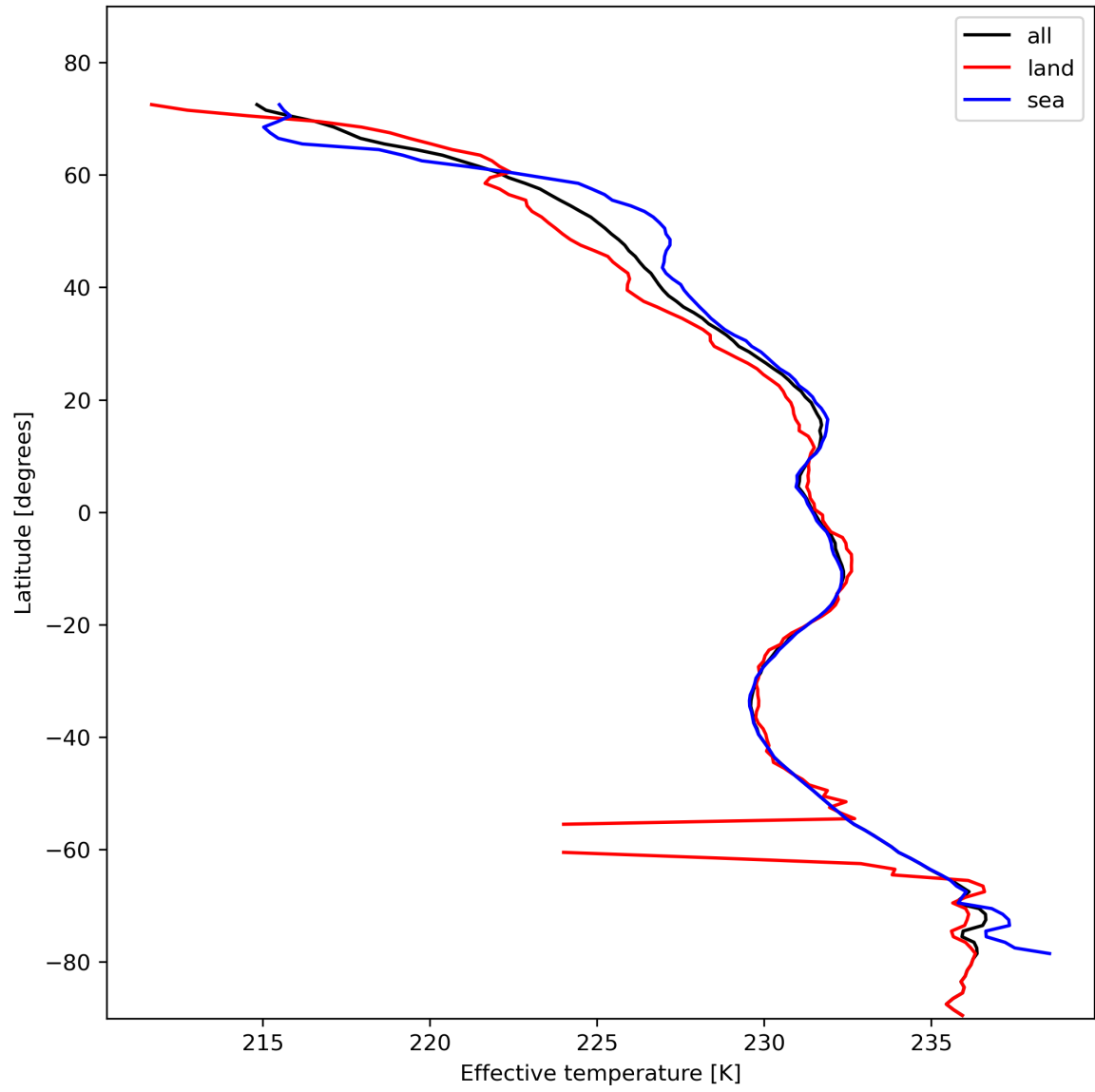
Figure 17: Zonal average of “Effective temperature” for 2023-11-07 to 2023-11-08.
