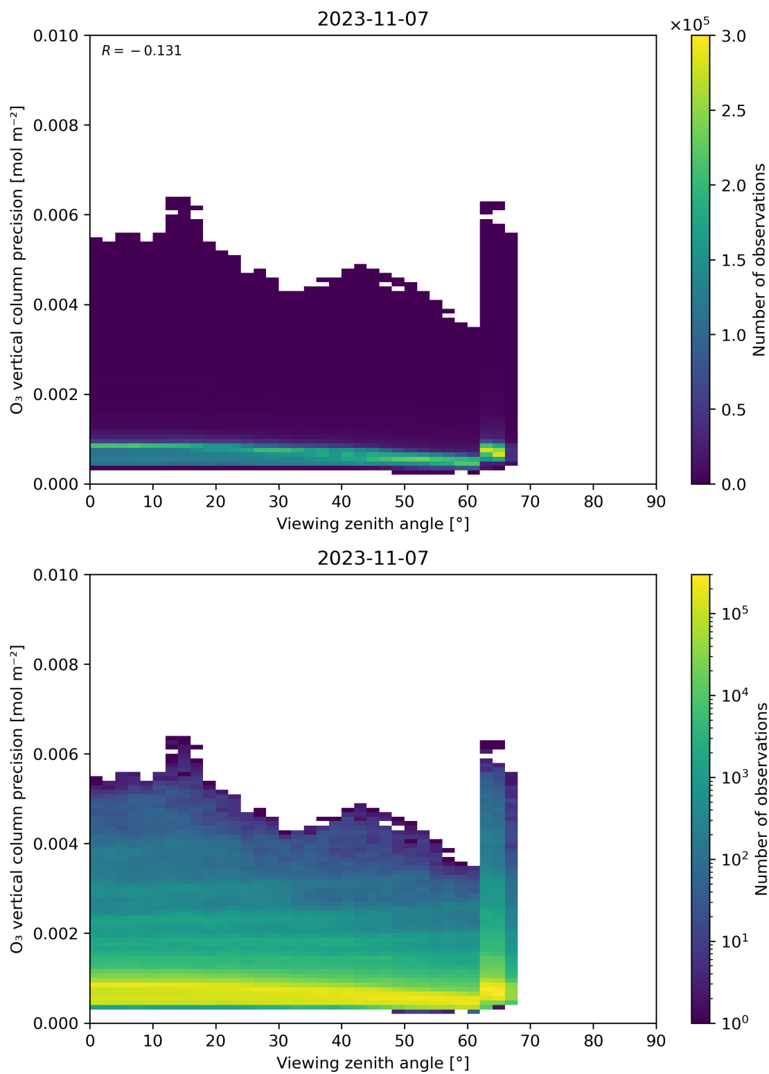
Figure 53: Scatter density plot of “Viewing zenith angle” against “O 3 vertical column precision” for 2023-11-07 to 2023-11-08.
