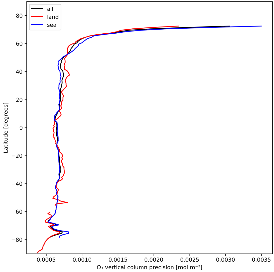
Figure 15: Zonal average of “O 3 vertical column precision” for 2023-11-07 to 2023-11-08.
