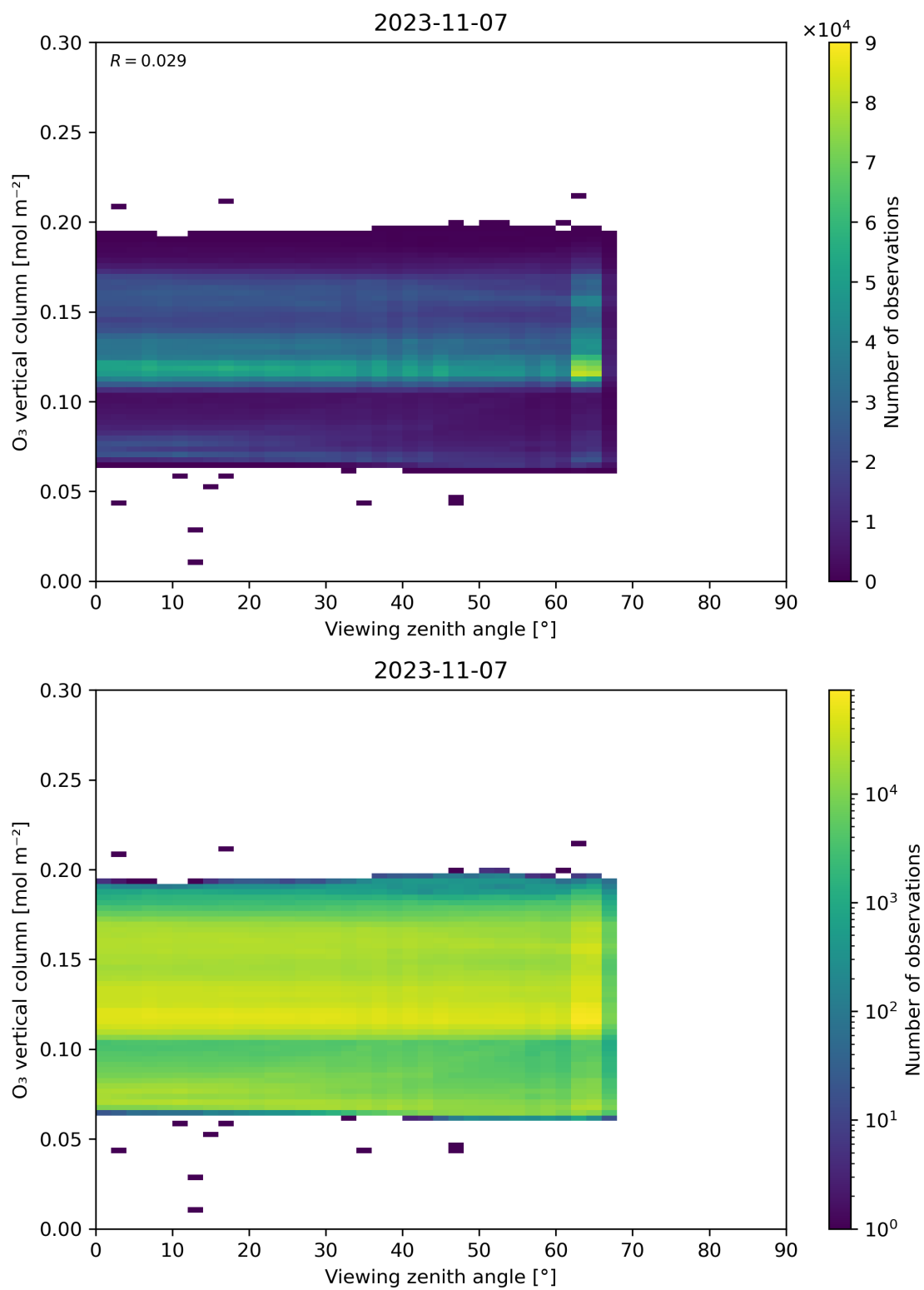
Figure 52: Scatter density plot of “Viewing zenith angle” against “O 3 vertical column” for 2023-11-07 to 2023-11-08.
