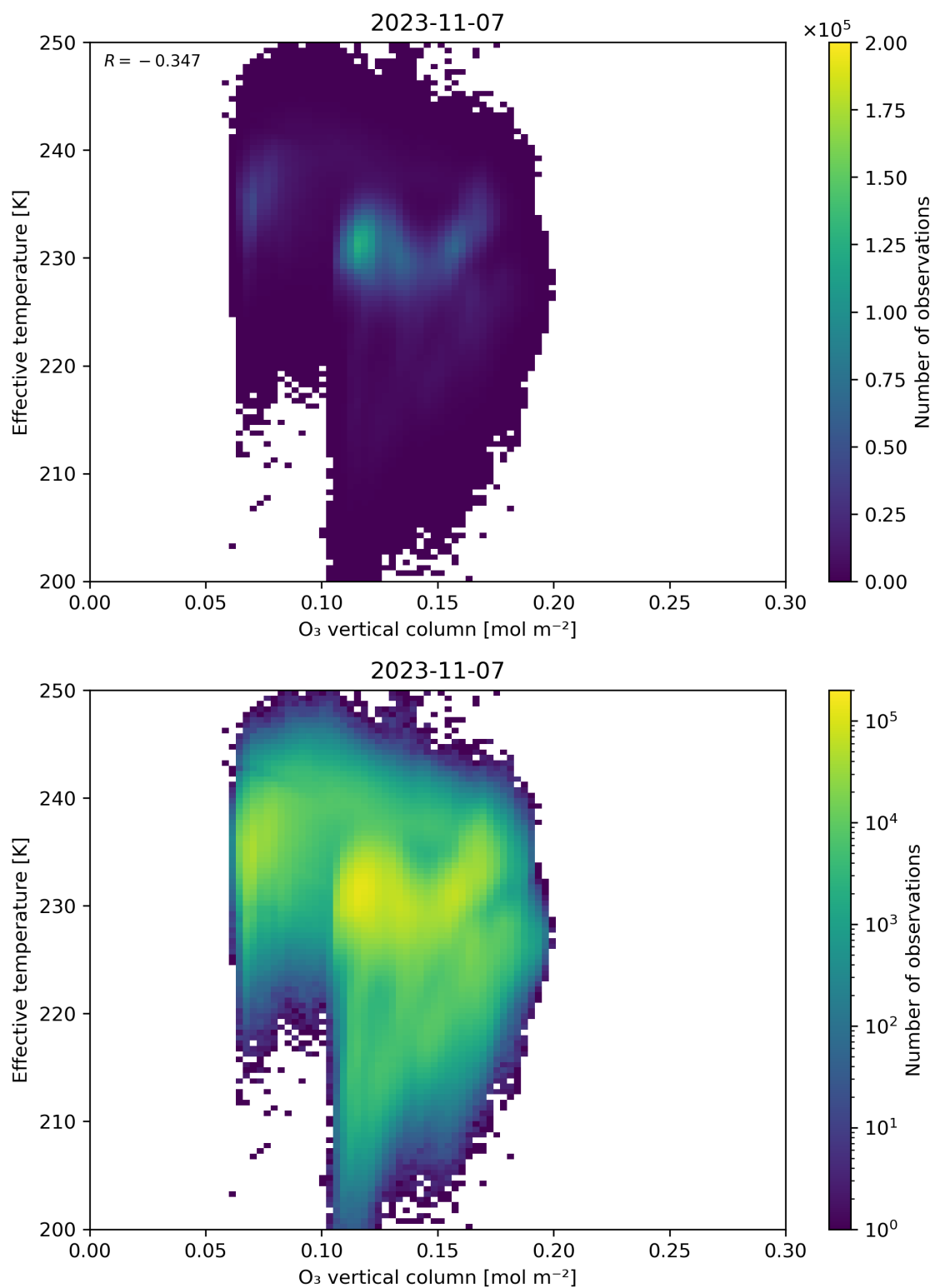
Figure 39: Scatter density plot of “O 3 vertical column” against “Effective temperature” for 2023-11-07 to 2023-11-08.
