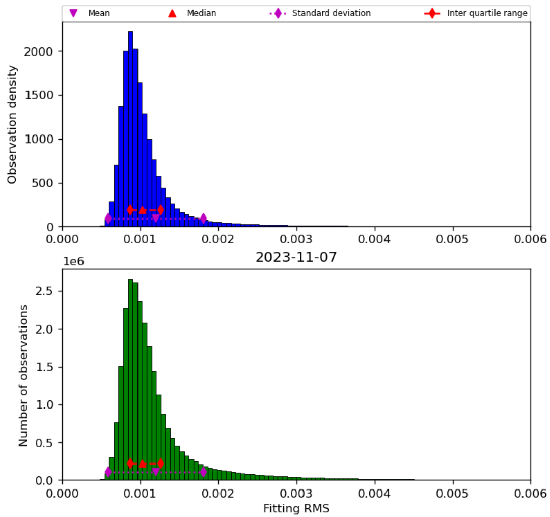
Figure 23: Histogram of “Fitting RMS” for 2023-11-07 to 2023-11-08
