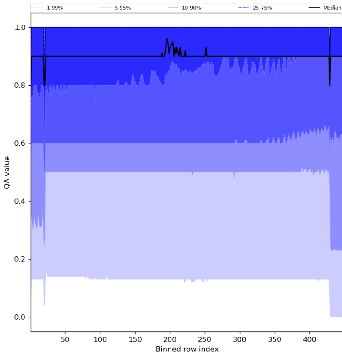
Figure 27: Along track statistics of “QA value” for 2023-11-07 to 2023-11-08
