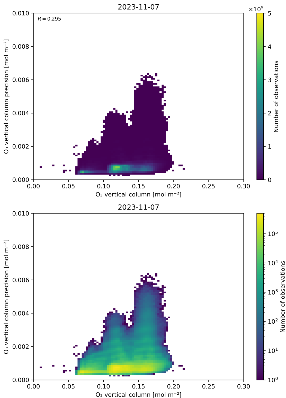
Figure 41: Scatter density plot of “O 3 vertical column” against “O 3 vertical column precision” for 2023-11-07 to 2023-11-08.
