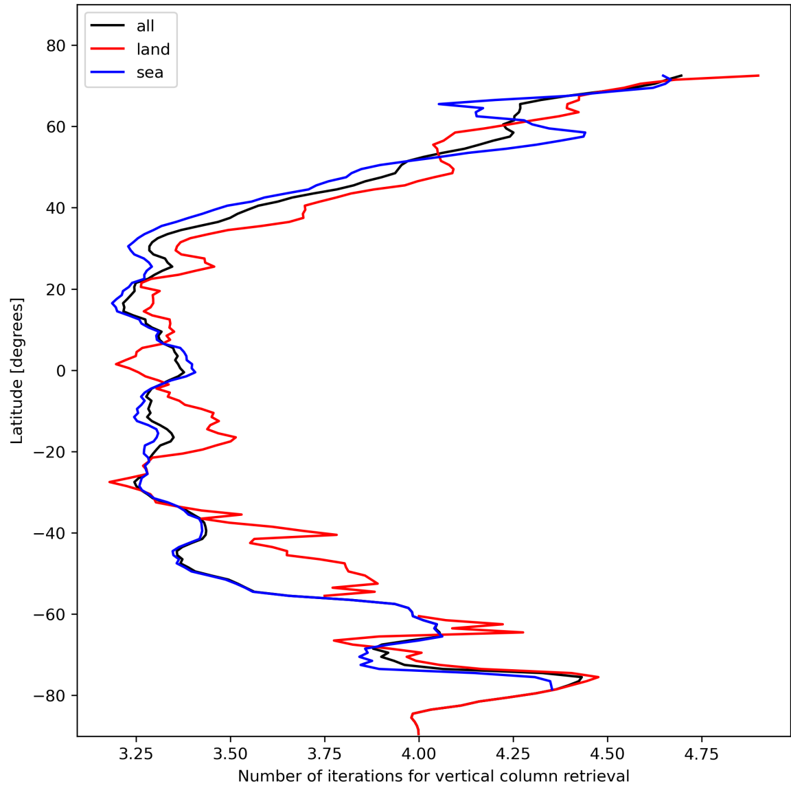
Figure 19: Zonal average of “Number of iterations for vertical column retrieval” for 2023-11-07 to 2023-11-08.
