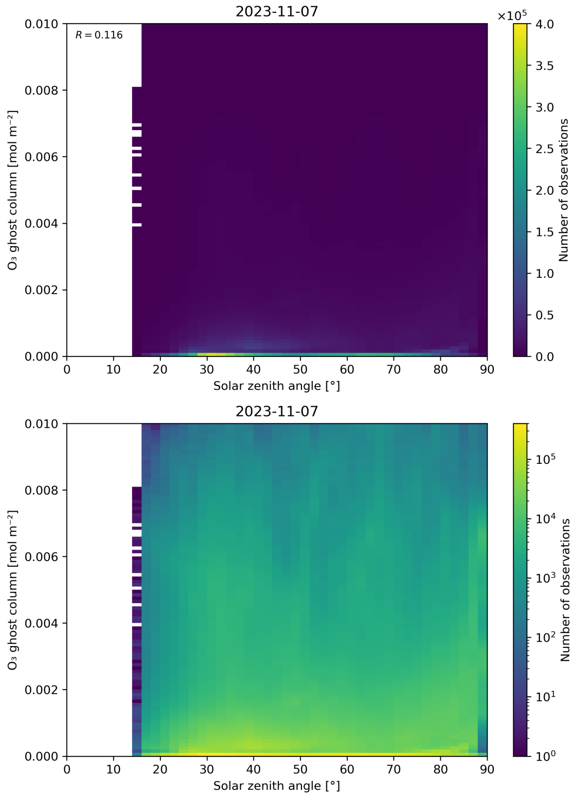
Figure 46: Scatter density plot of “Solar zenith angle” against “O 3 ghost column” for 2023-11-07 to 2023-11-08.
