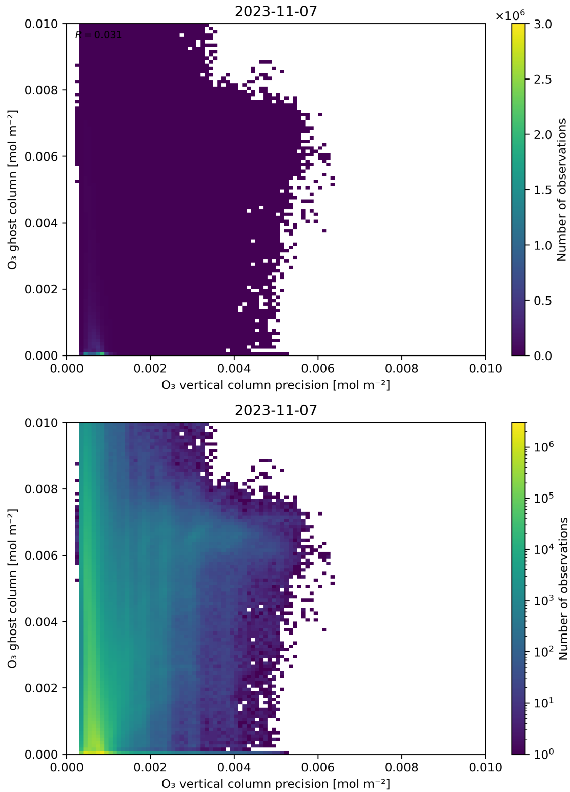
Figure 43: Scatter density plot of “O 3 vertical column precision” against “O 3 ghost column” for 2023-11-07 to 2023-11-08.
