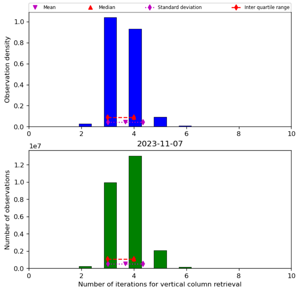
Figure 26: Histogram of “Number of iterations for vertical column retrieval” for 2023-11-07 to 2023-11-08
