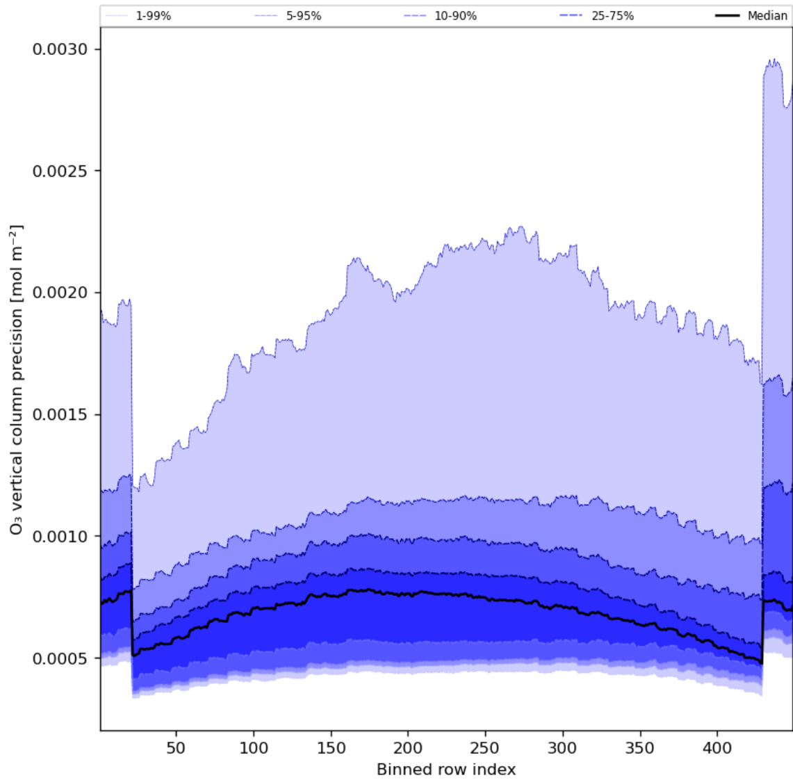
Figure 29: Along track statistics of “O 3 vertical column precision” for 2023-11-07 to 2023-11-08
