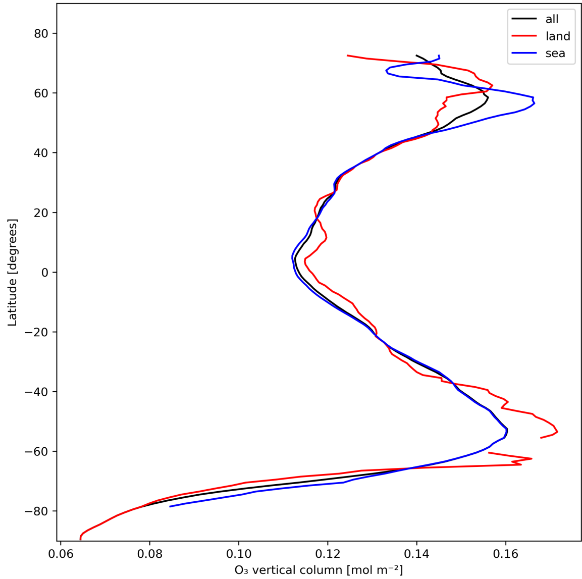
Figure 14: Zonal average of “O 3 vertical column” for 2023-11-07 to 2023-11-08.
