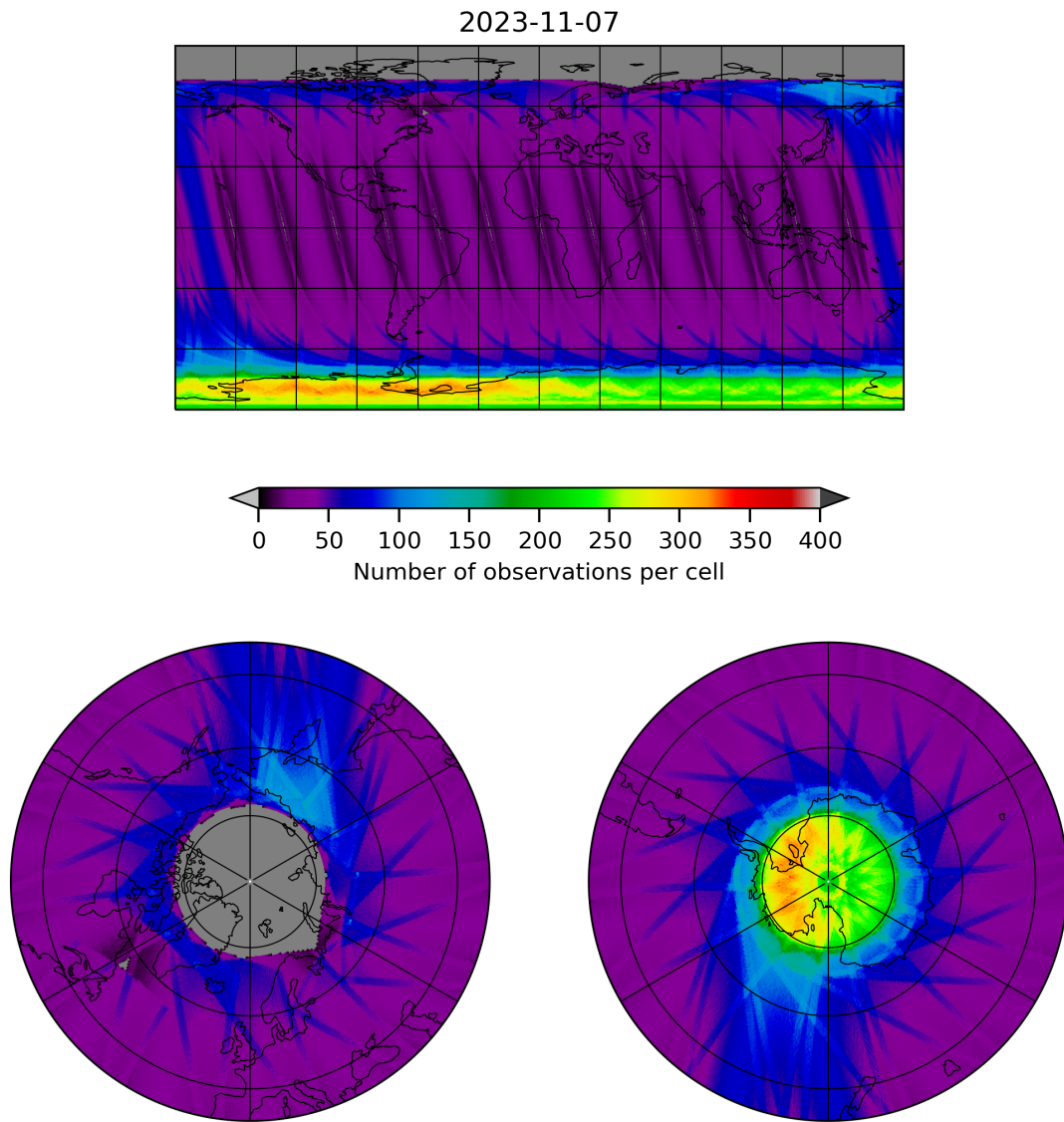
Figure 12: Map of the number of observations for 2023-11-07 to 2023-11-08
