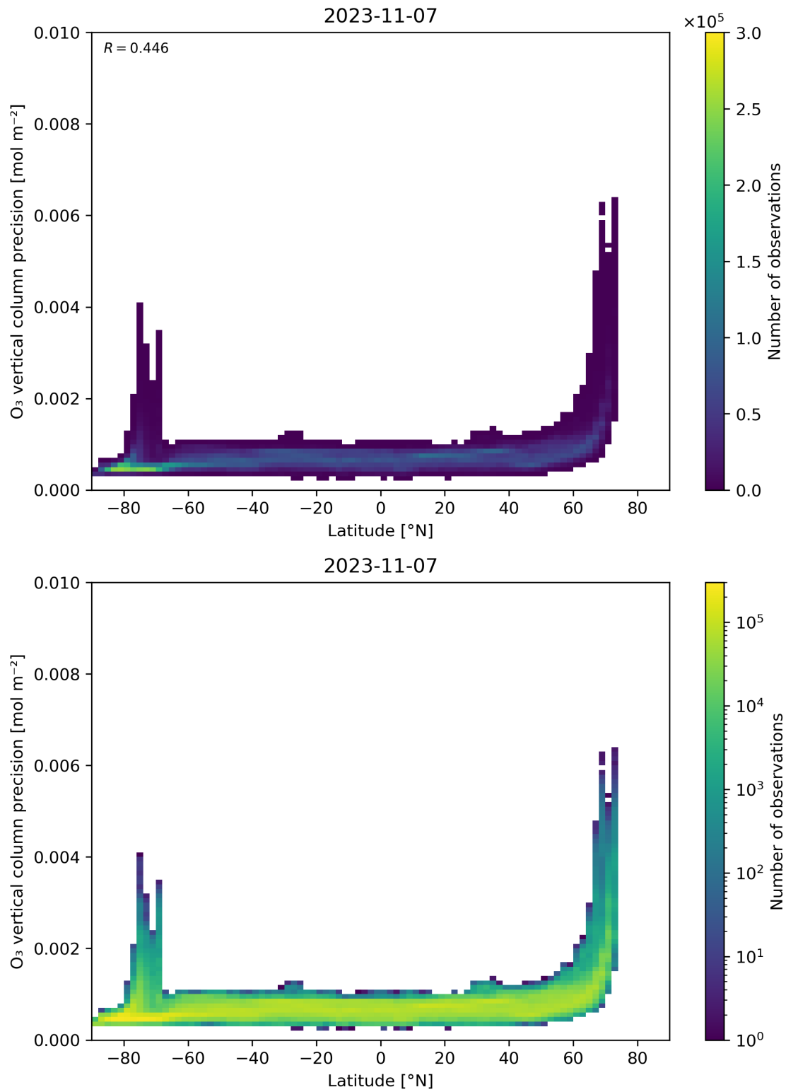
Figure 37: Scatter density plot of “Latitude” against “O 3 vertical column precision” for 2023-11-07 to 2023-11-08.
