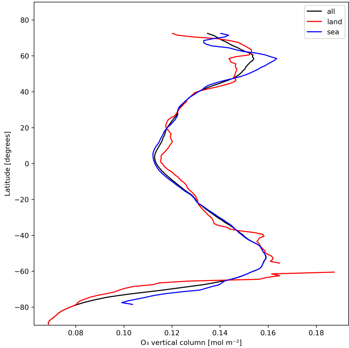
Figure 14: Zonal average of “O 3 vertical column” for 2023-11-07 to 2023-11-09.
