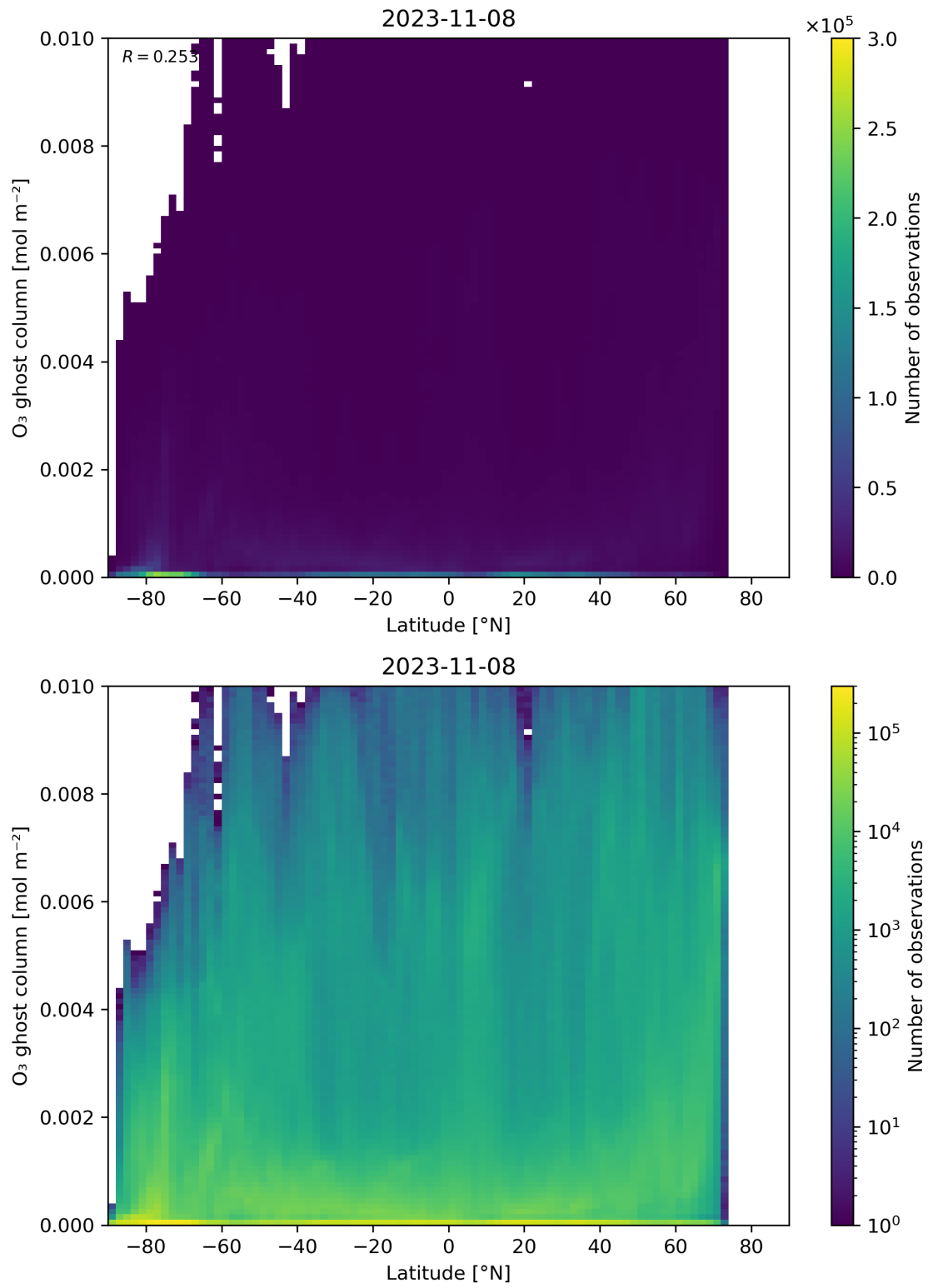
Figure 35: Scatter density plot of “Latitude” against “O 3 ghost column” for 2023-11-07 to 2023-11-09.
