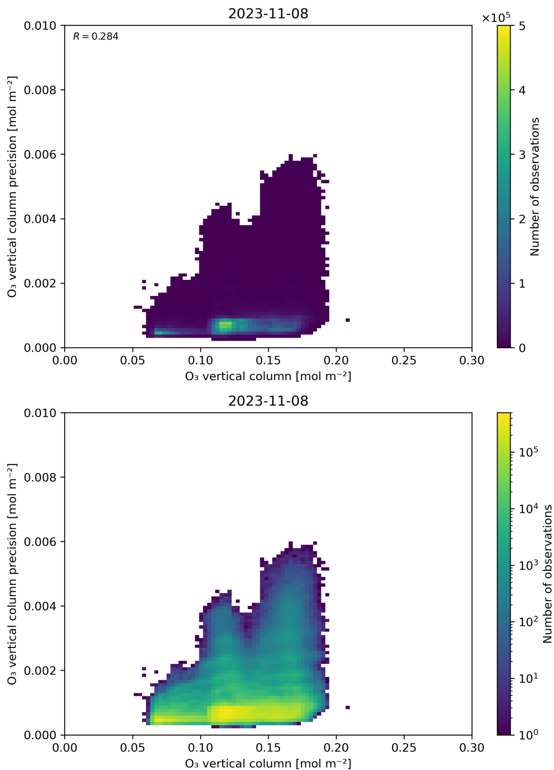
Figure 41: Scatter density plot of “O 3 vertical column” against “O 3 vertical column precision” for 2023-11-07 to 2023-11-09.
