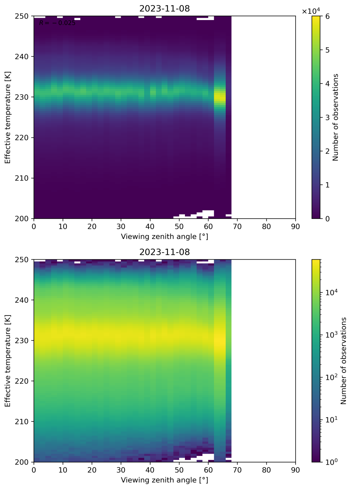
Figure 50: Scatter density plot of “Viewing zenith angle” against “Effective temperature” for 2023-11-07 to 2023-11-09.
