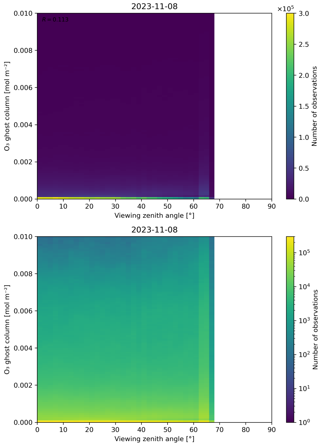
Figure 51: Scatter density plot of “Viewing zenith angle” against “O 3 ghost column” for 2023-11-07 to 2023-11-09.
