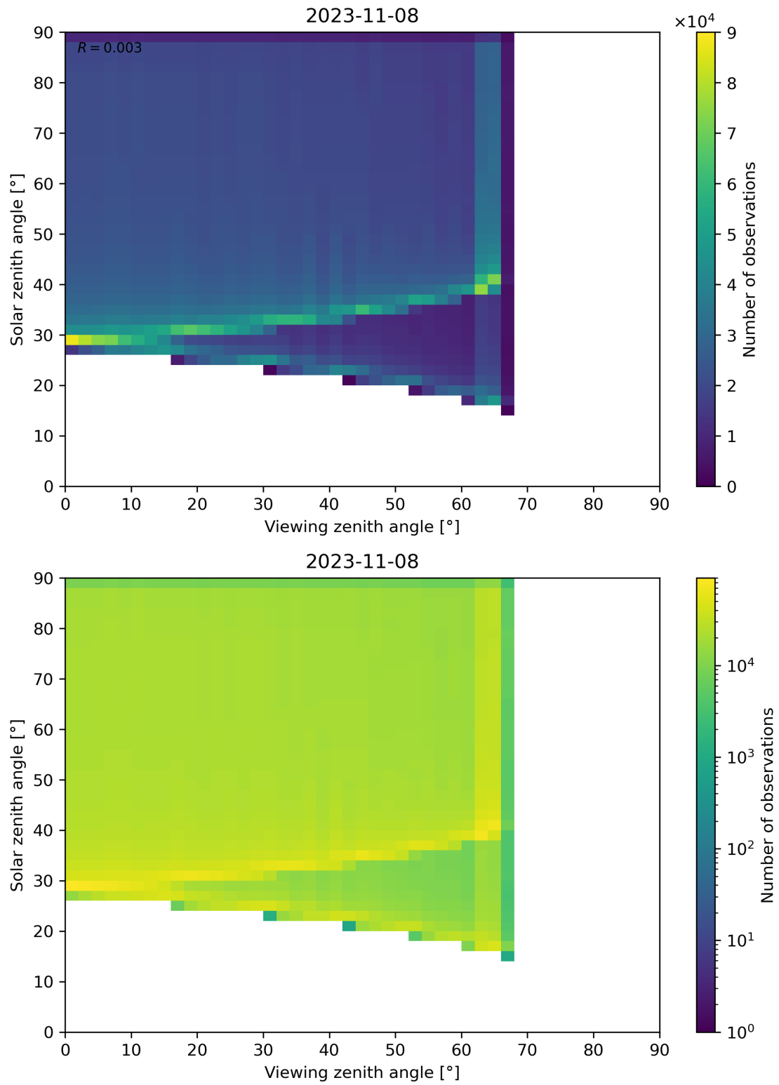
Figure 54: Scatter density plot of “Viewing zenith angle” against “Solar zenith angle” for 2023-11-07 to 2023-11-09.
