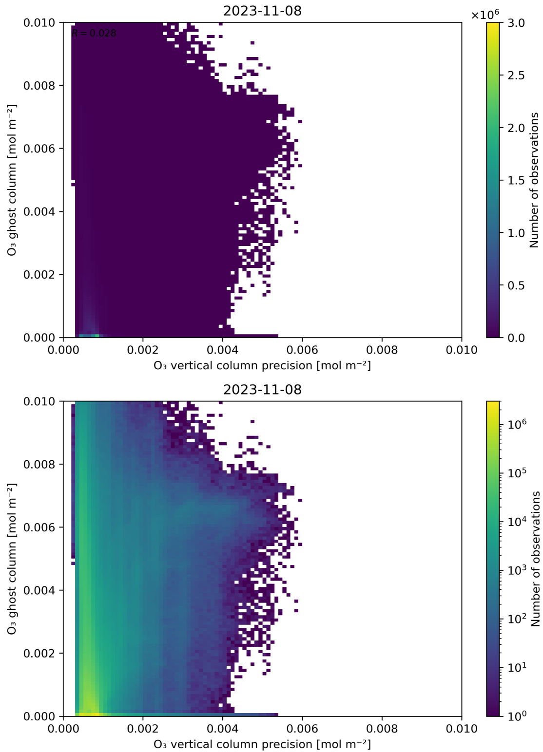
Figure 43: Scatter density plot of “ \text{O}_3 vertical column precision” against “ \text{O}_3 ghost column” for 2023-11-07 to 2023-11-09.
