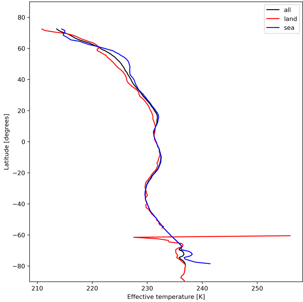
Figure 17: Zonal average of "Effective temperature" for 2023-11-07 to 2023-11-09.
