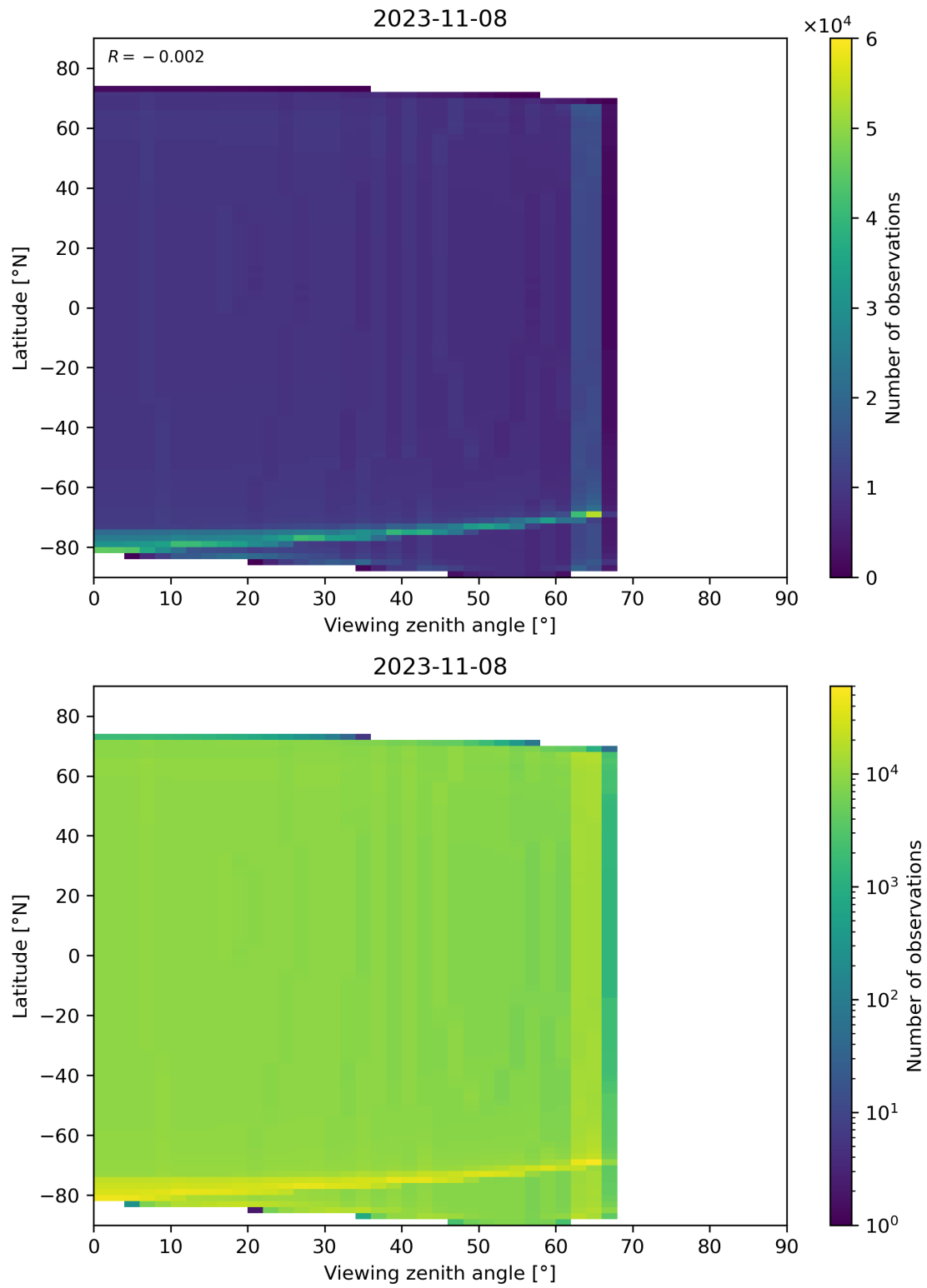
Figure 49: Scatter density plot of “Viewing zenith angle” against “Latitude” for 2023-11-07 to 2023-11-09.
