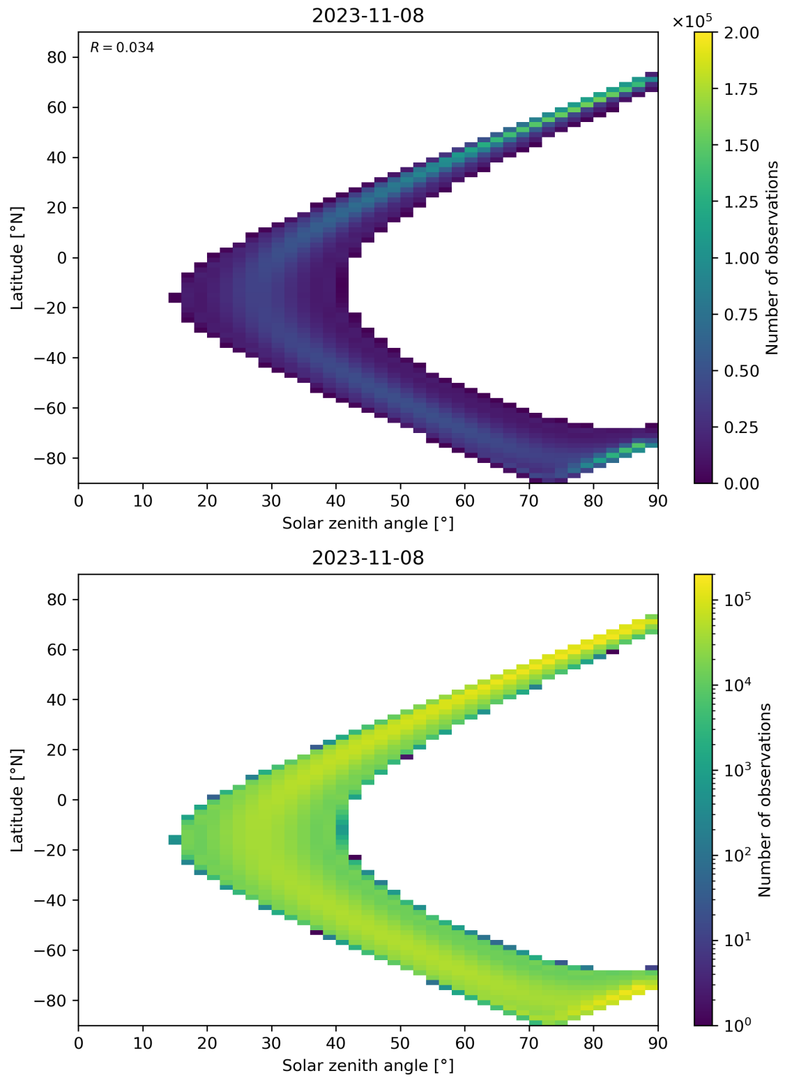
Figure 44: Scatter density plot of “Solar zenith angle” against “Latitude” for 2023-11-07 to 2023-11-09.
