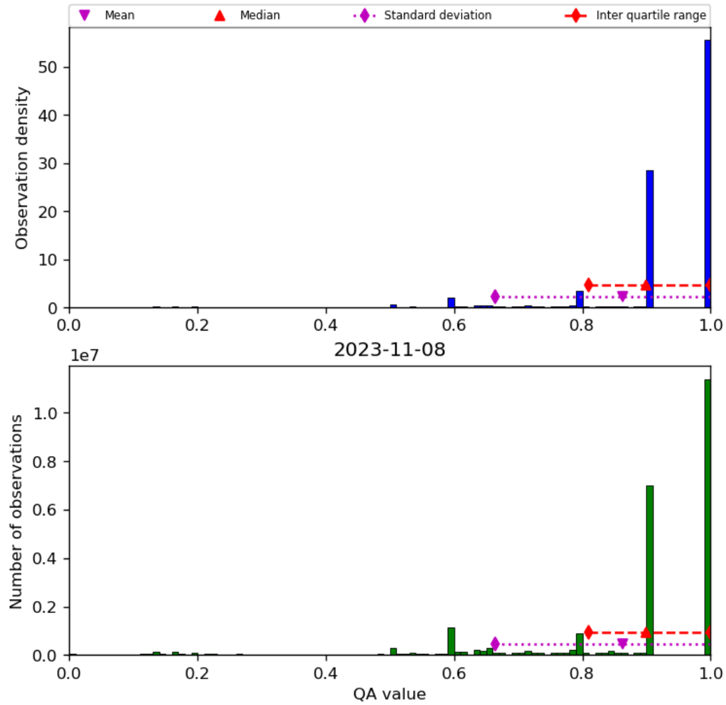
Figure 20: Histogram of “QA value” for 2023-11-07 to 2023-11-09
