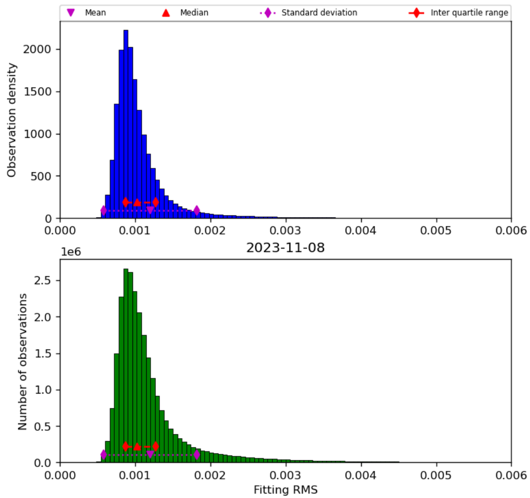
Figure 23: Histogram of “Fitting RMS” for 2023-11-07 to 2023-11-09
