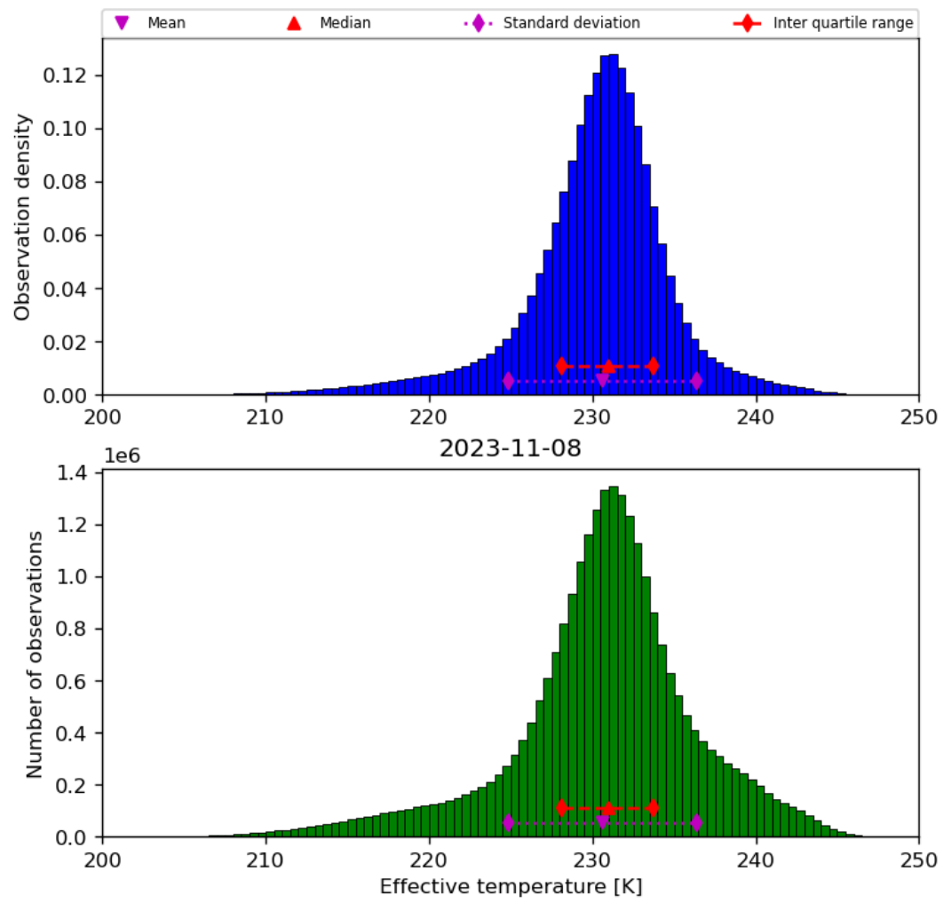
Figure 24: Histogram of “Effective temperature” for 2023-11-07 to 2023-11-09
