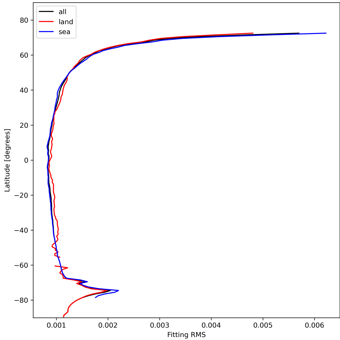
Figure 16: Zonal average of “Fitting RMS” for 2023-11-07 to 2023-11-09.
