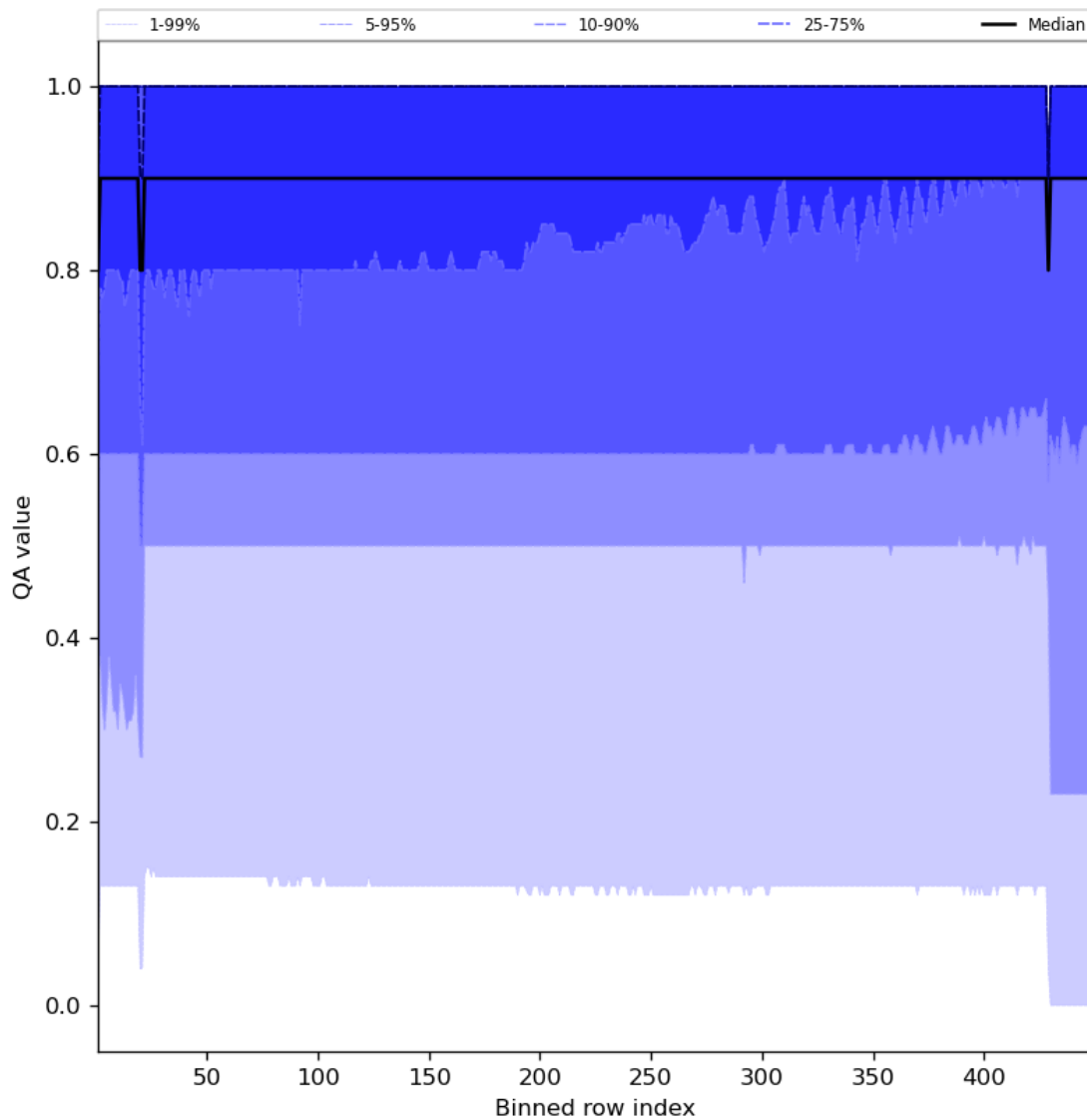
Figure 27: Along track statistics of “QA value” for 2023-11-07 to 2023-11-09
