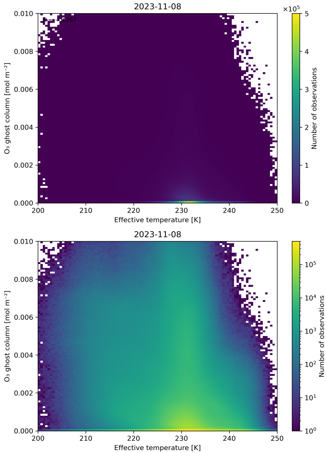
Figure 38: Scatter density plot of “Effective temperature” against “O 3 ghost column” for 2023-11-07 to 2023-11-09.
