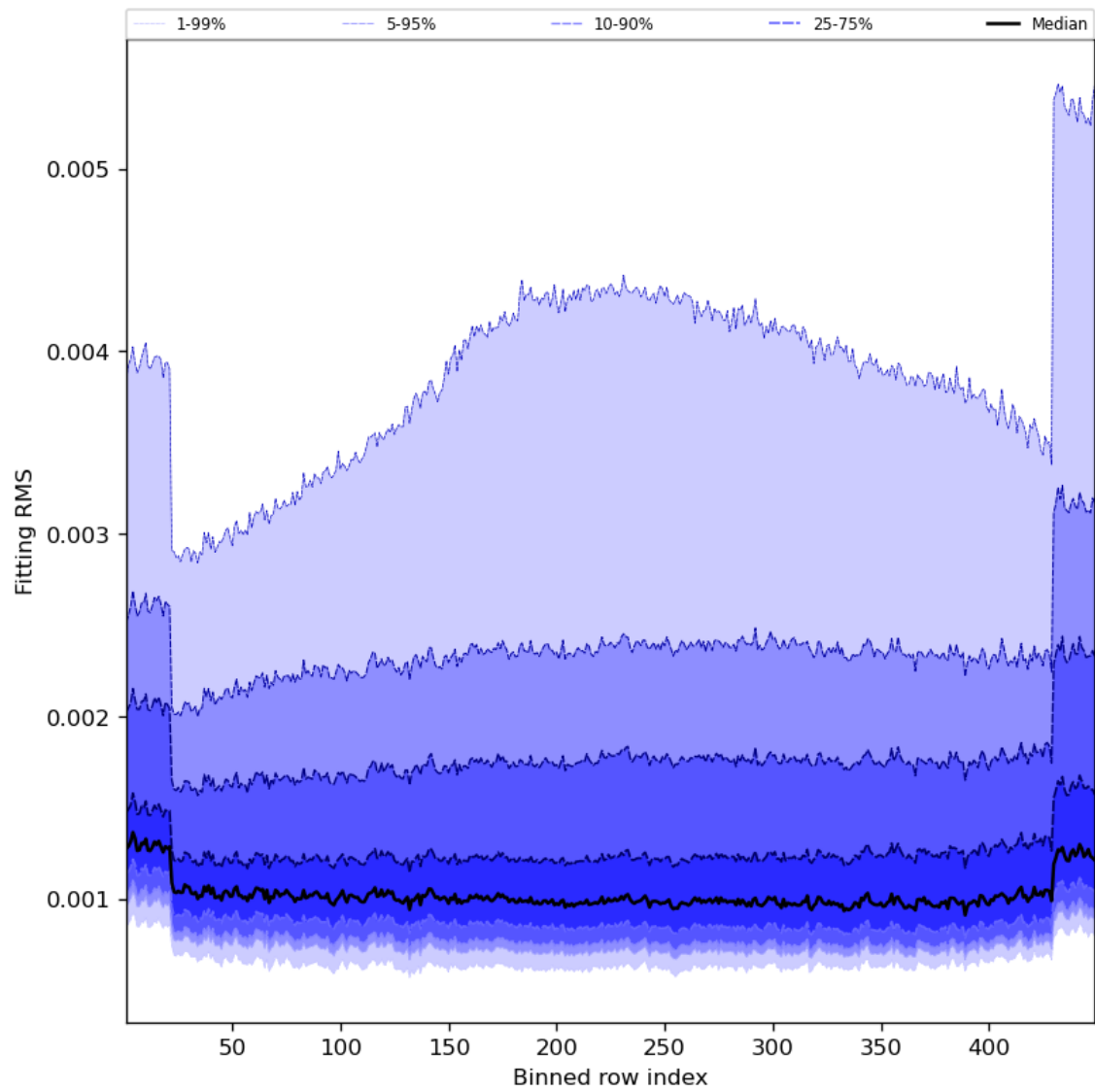
Figure 30: Along track statistics of “Fitting RMS” for 2023-11-07 to 2023-11-09
