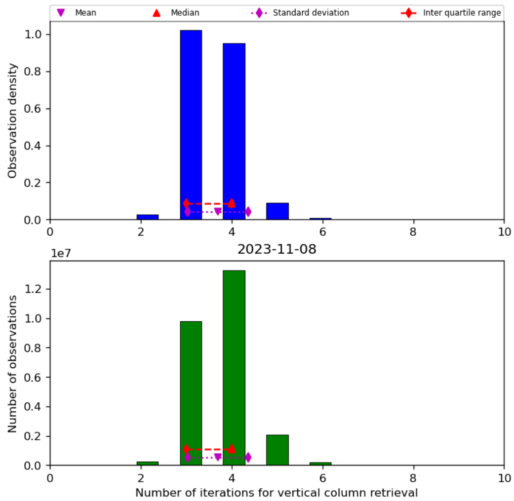
Figure 26: Histogram of “Number of iterations for vertical column retrieval” for 2023-11-07 to 2023-11-09
