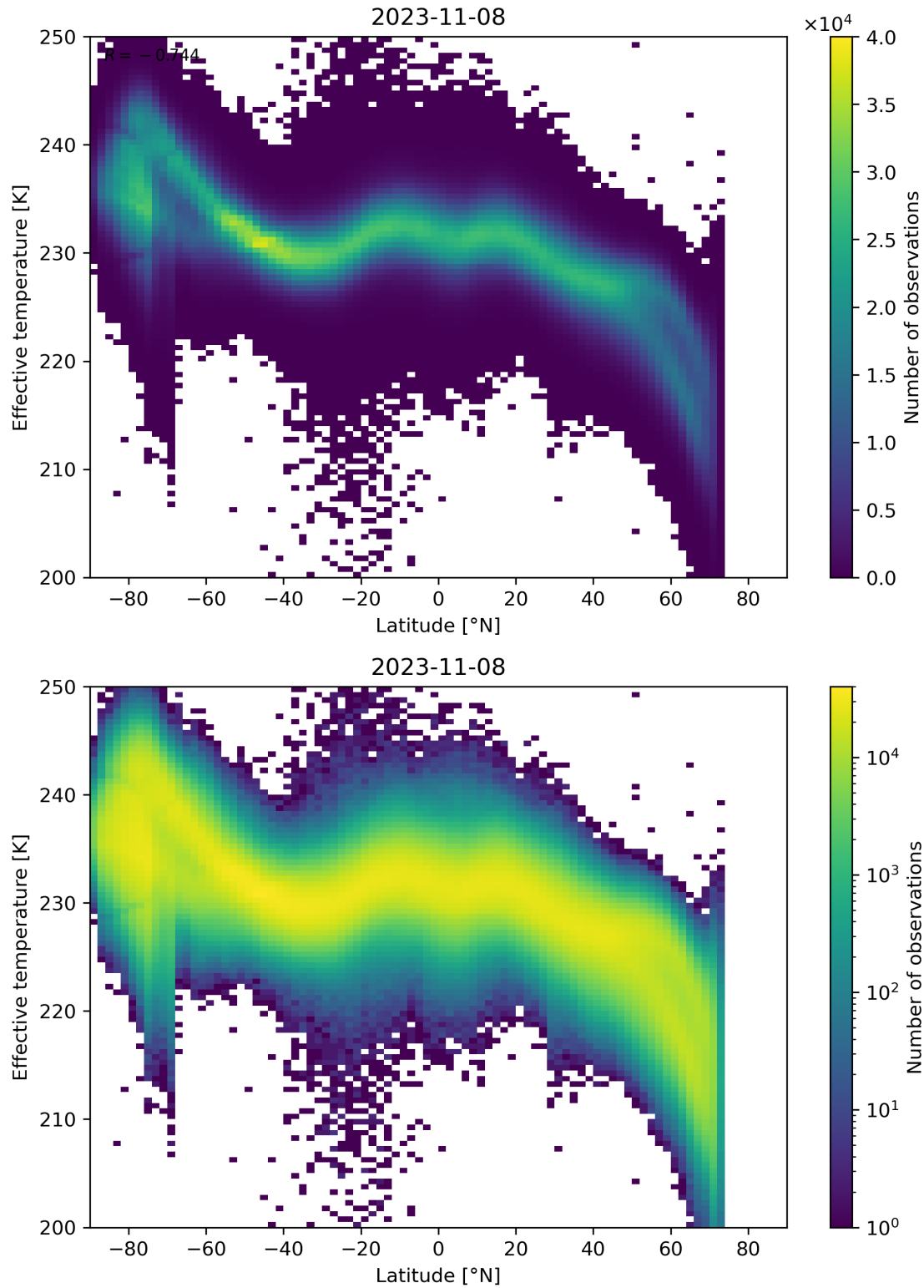
Figure 34: Scatter density plot of “Latitude” against “Effective temperature” for 2023-11-07 to 2023-11-09.
