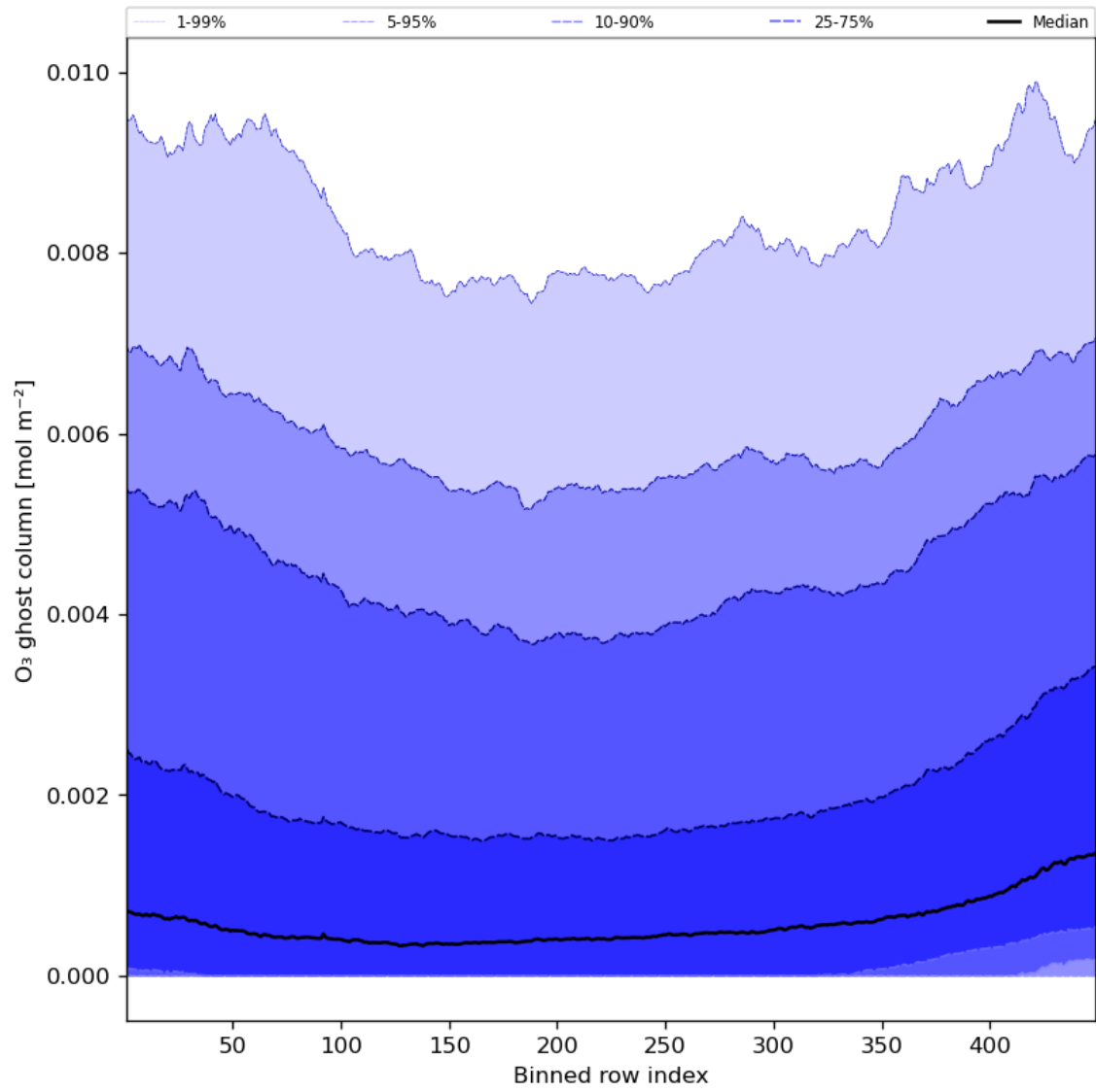
Figure 32: Along track statistics of “O 3 ghost column” for 2023-11-07 to 2023-11-09
