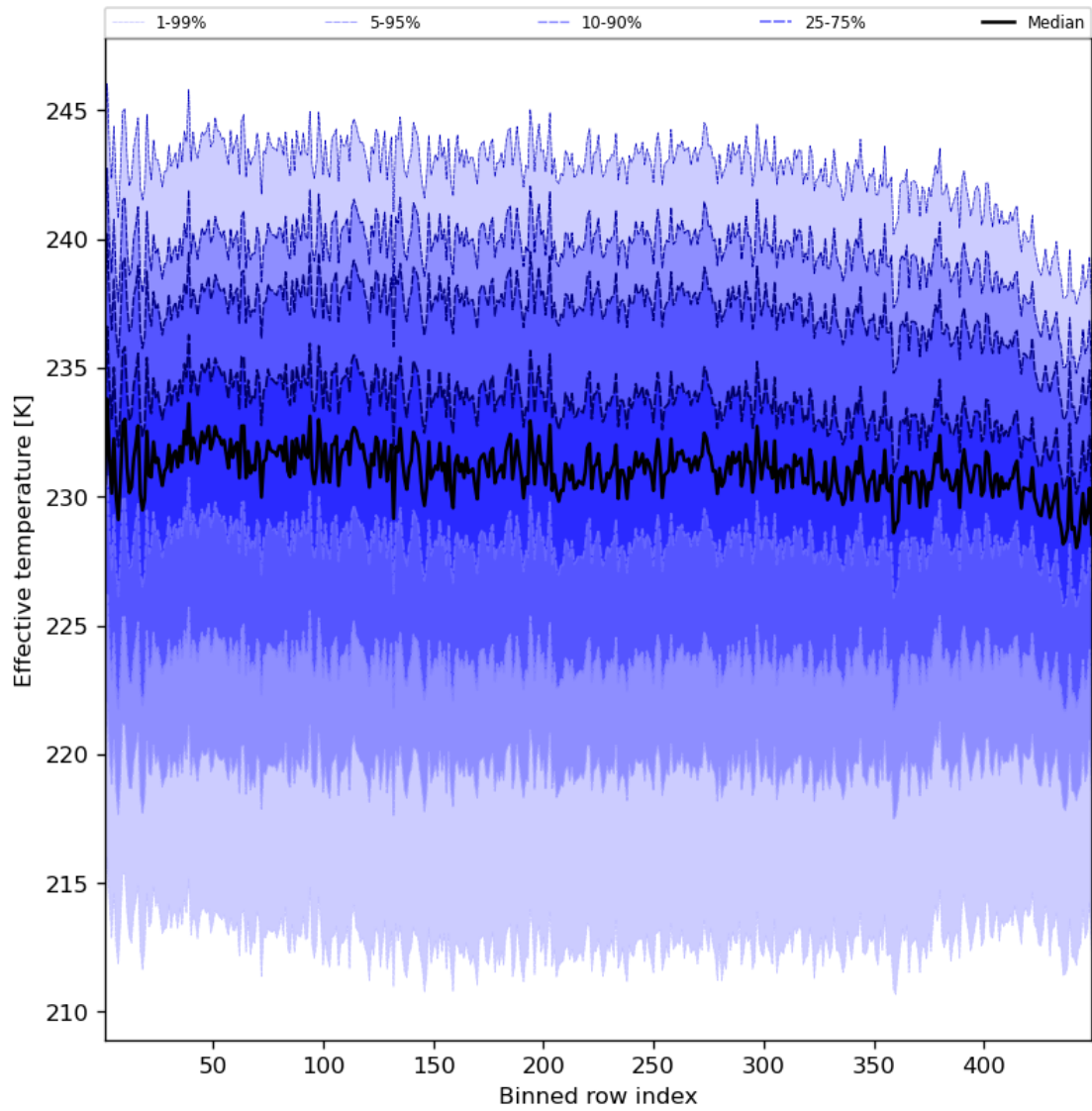
Figure 31: Along track statistics of “Effective temperature” for 2023-11-07 to 2023-11-09
