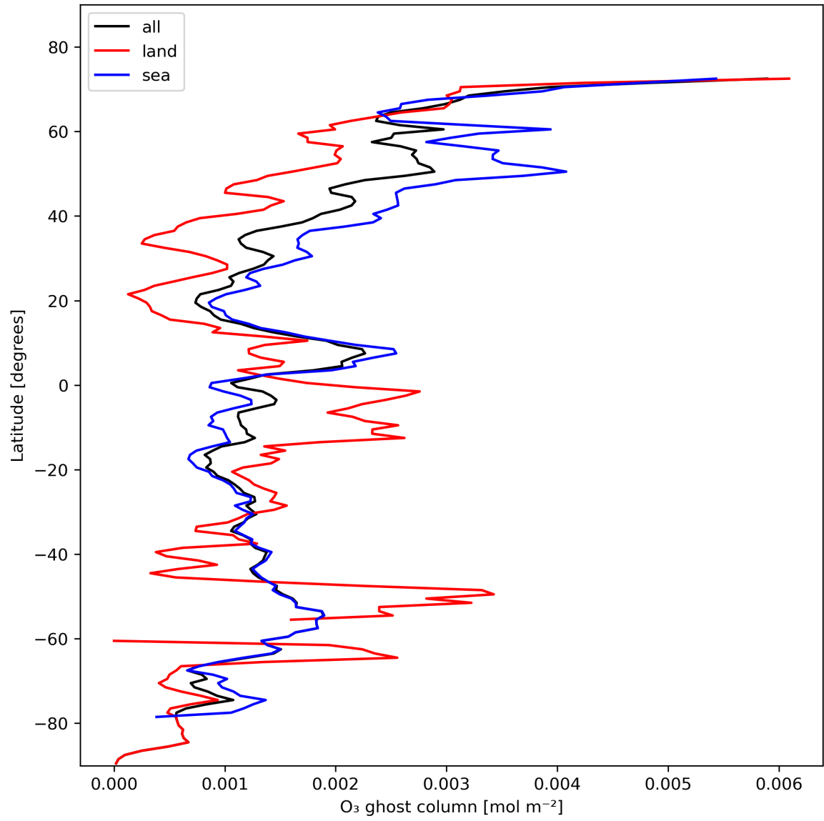
Figure 18: Zonal average of “O 3 ghost column” for 2023-11-07 to 2023-11-09.
