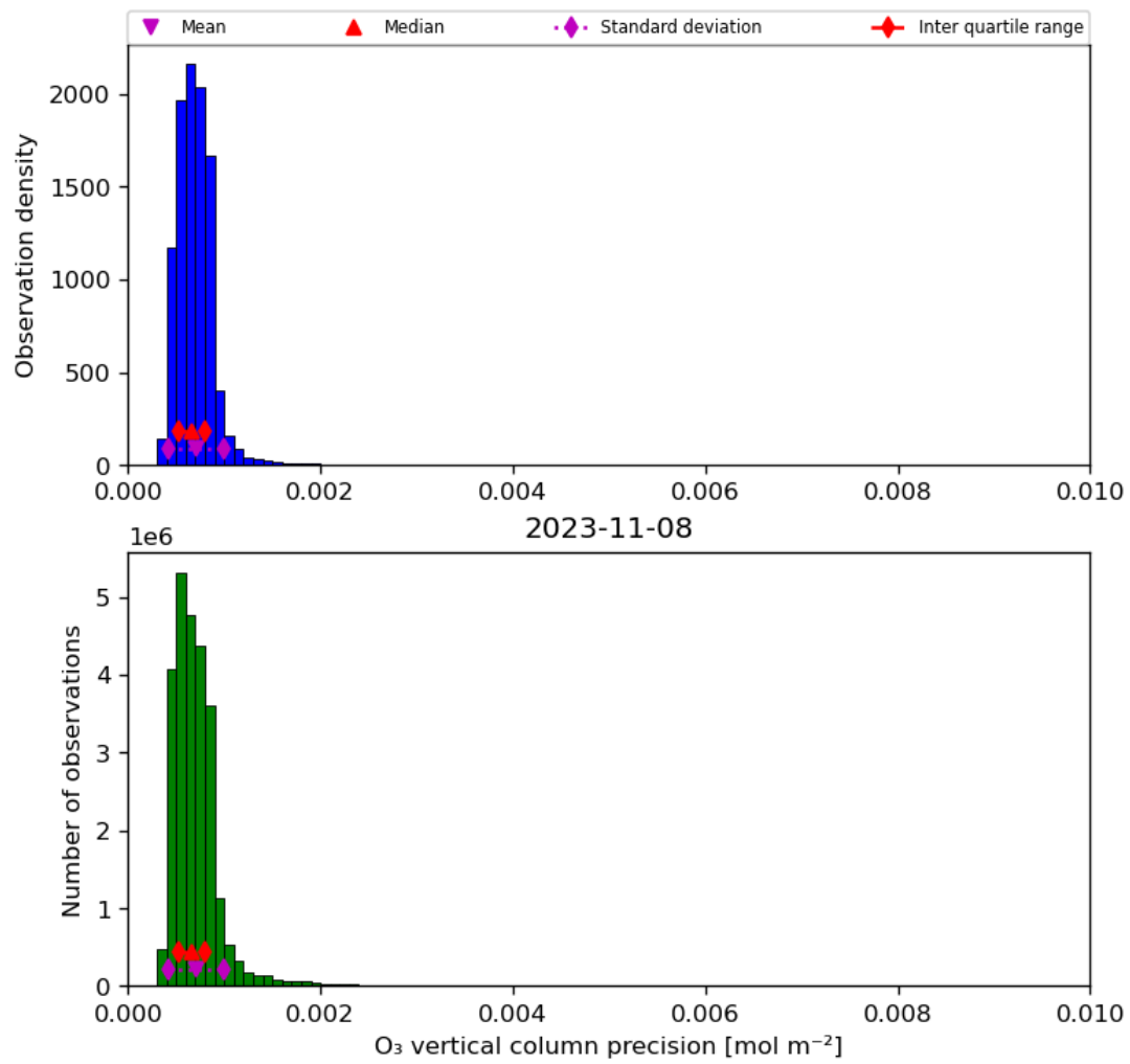
Figure 22: Histogram of “O 3 vertical column precision” for 2023-11-07 to 2023-11-09
