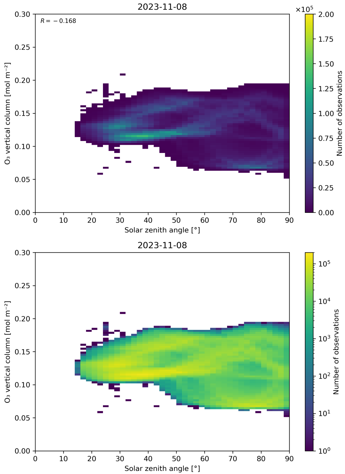
Figure 47: Scatter density plot of “Solar zenith angle” against “O 3 vertical column” for 2023-11-07 to 2023-11-09.
