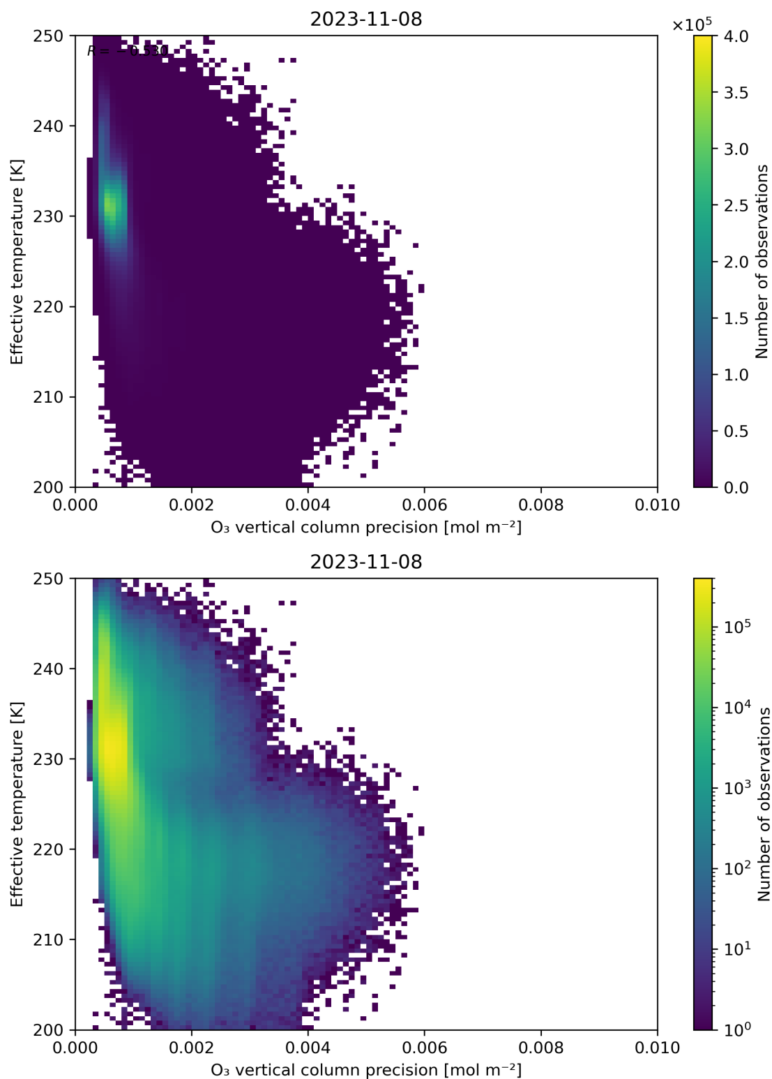
Figure 42: Scatter density plot of “O 3 vertical column precision” against “Effective temperature” for 2023-11-07 to 2023-11-09.
