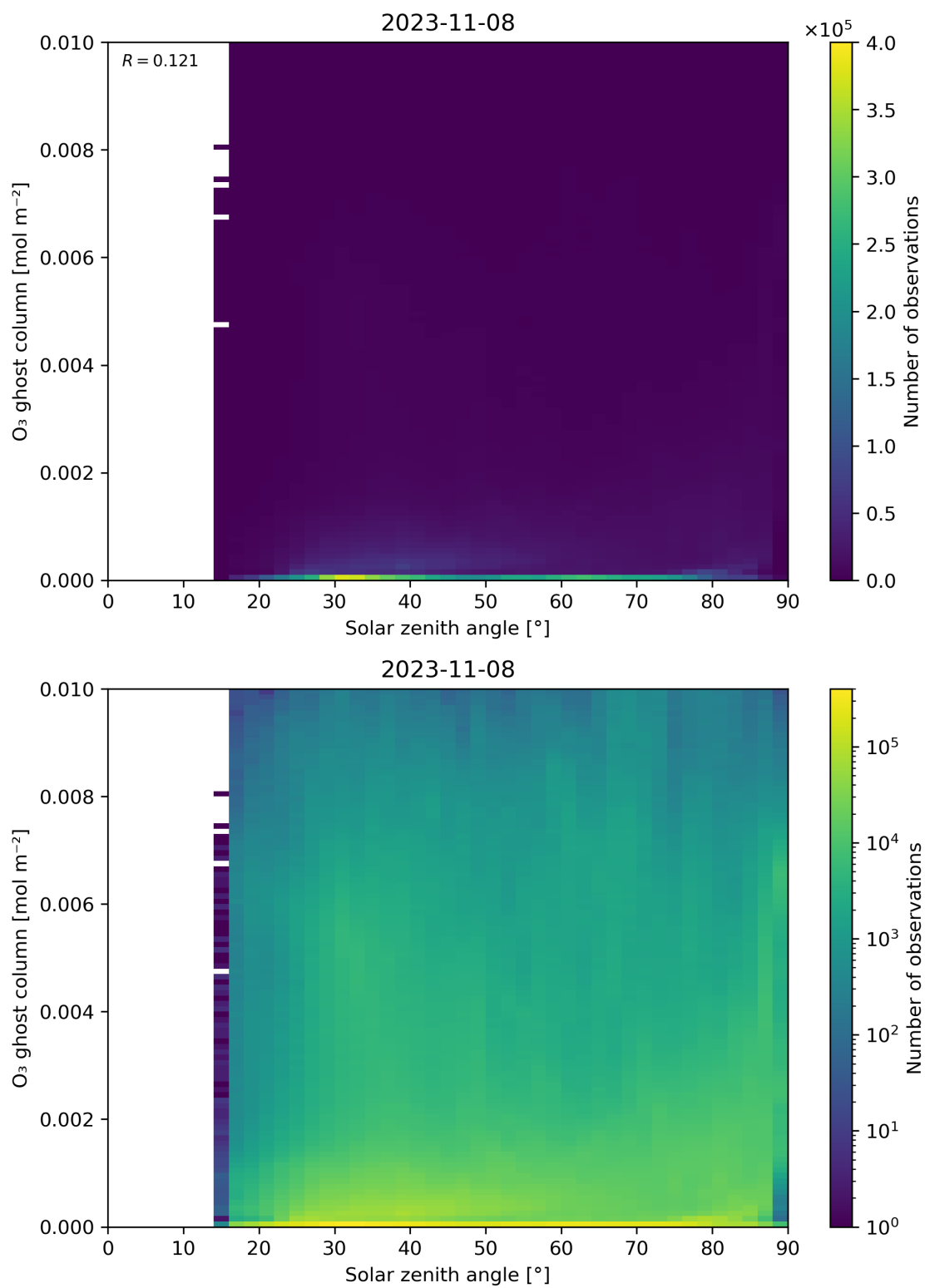
Figure 46: Scatter density plot of “Solar zenith angle” against “O 3 ghost column” for 2023-11-07 to 2023-11-09.
