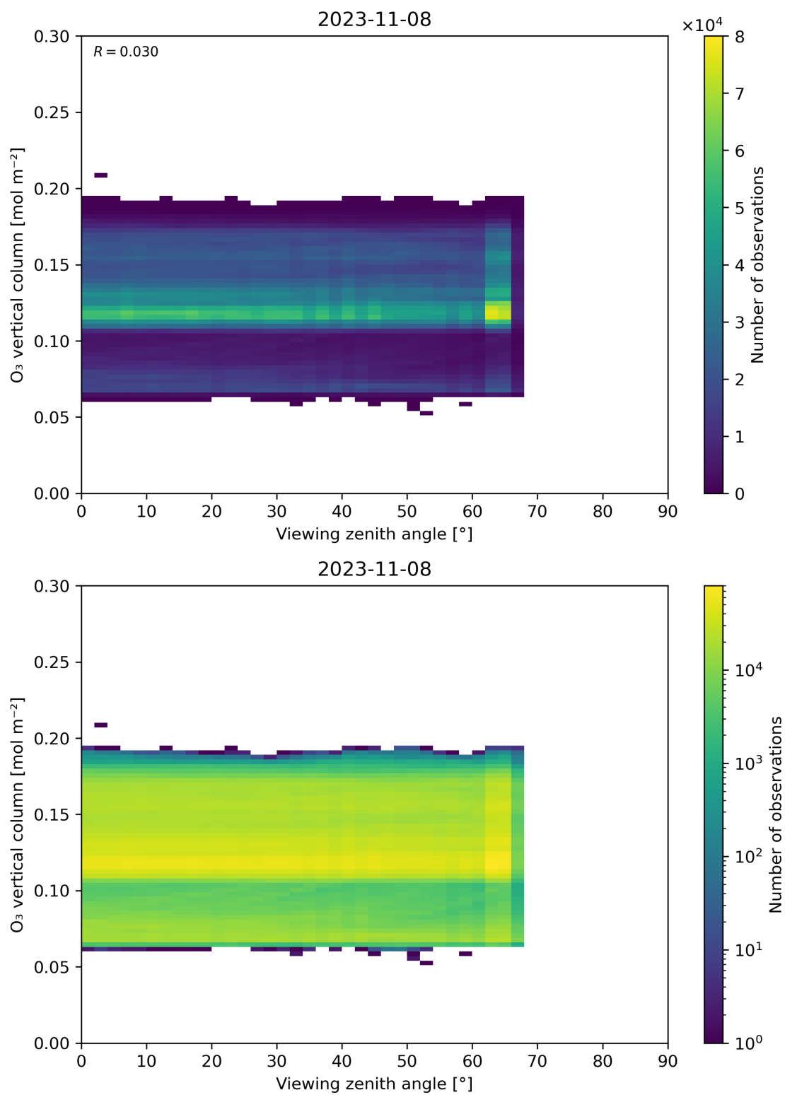
Figure 52: Scatter density plot of “Viewing zenith angle” against “O 3 vertical column” for 2023-11-07 to 2023-11-09.
