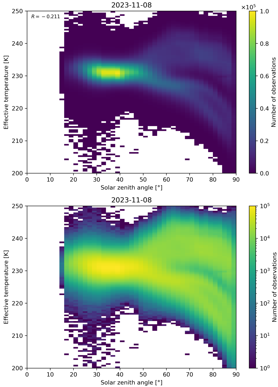
Figure 45: Scatter density plot of “Solar zenith angle” against “Effective temperature” for 2023-11-07 to 2023-11-09.
