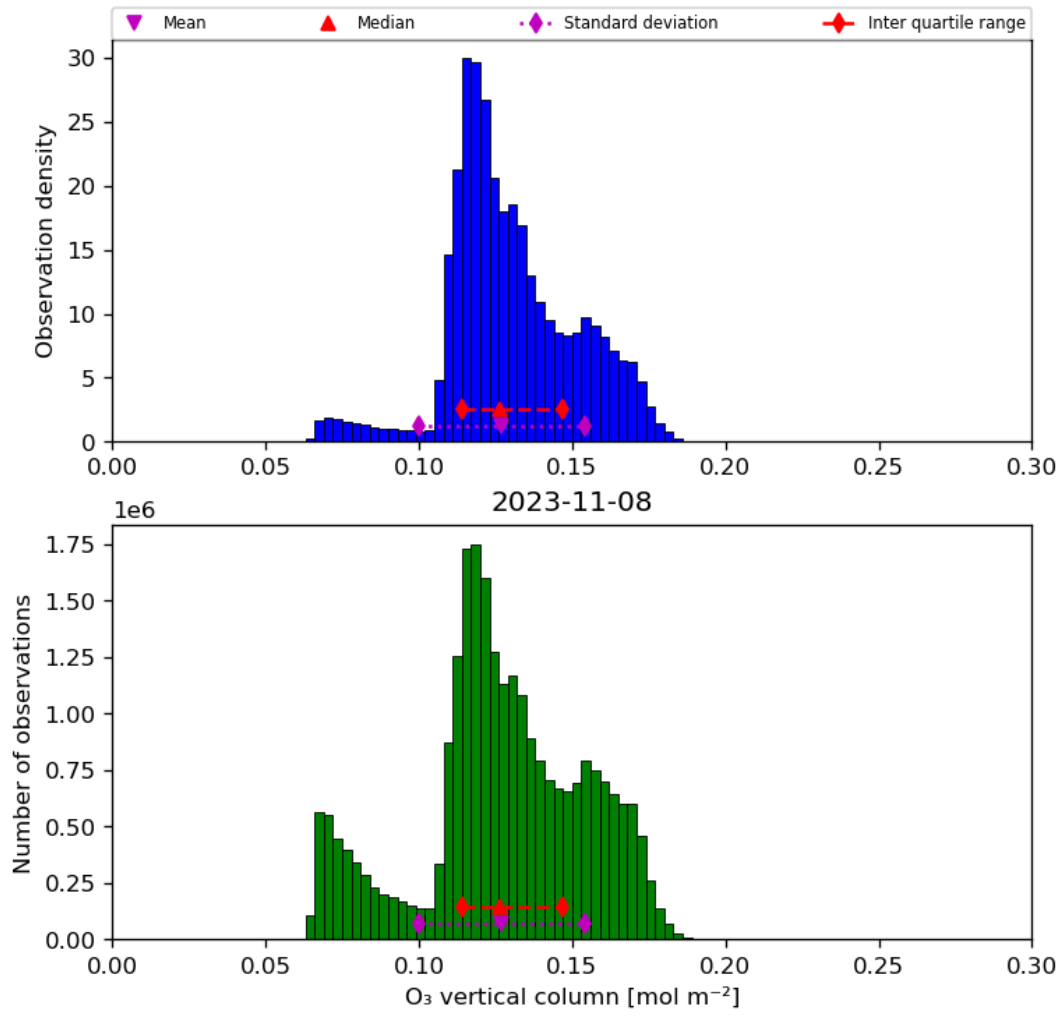
Figure 21: Histogram of “O 3 vertical column” for 2023-11-07 to 2023-11-09
