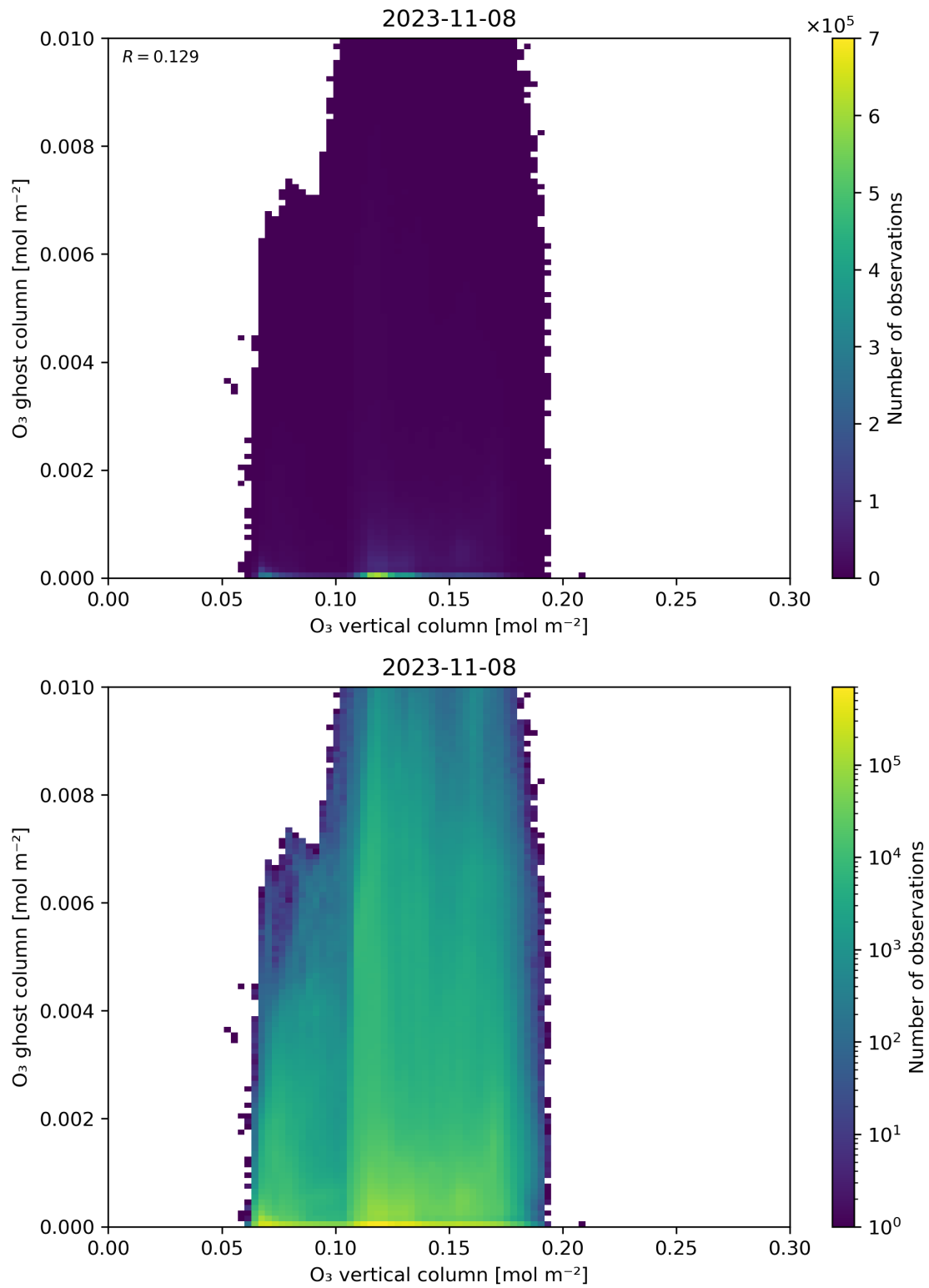
Figure 40: Scatter density plot of “O 3 vertical column” against “O 3 ghost column” for 2023-11-07 to 2023-11-09.
