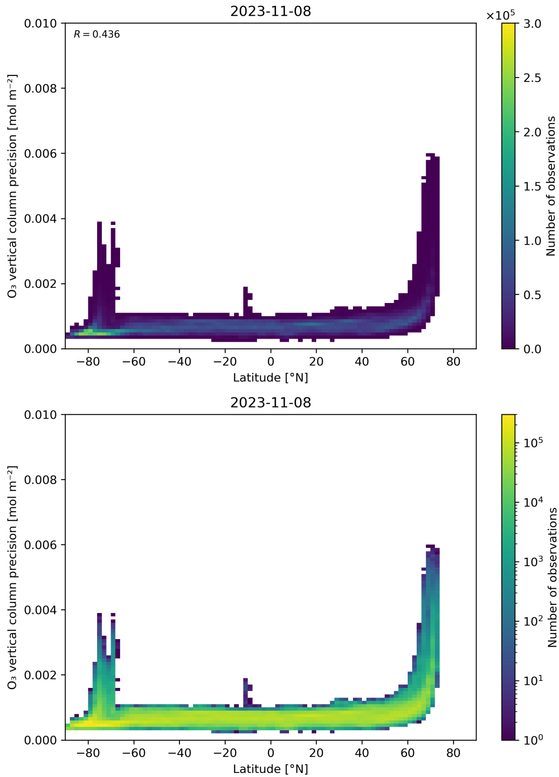
Figure 37: Scatter density plot of “Latitude” against “O 3 vertical column precision” for 2023-11-07 to 2023-11-09.
