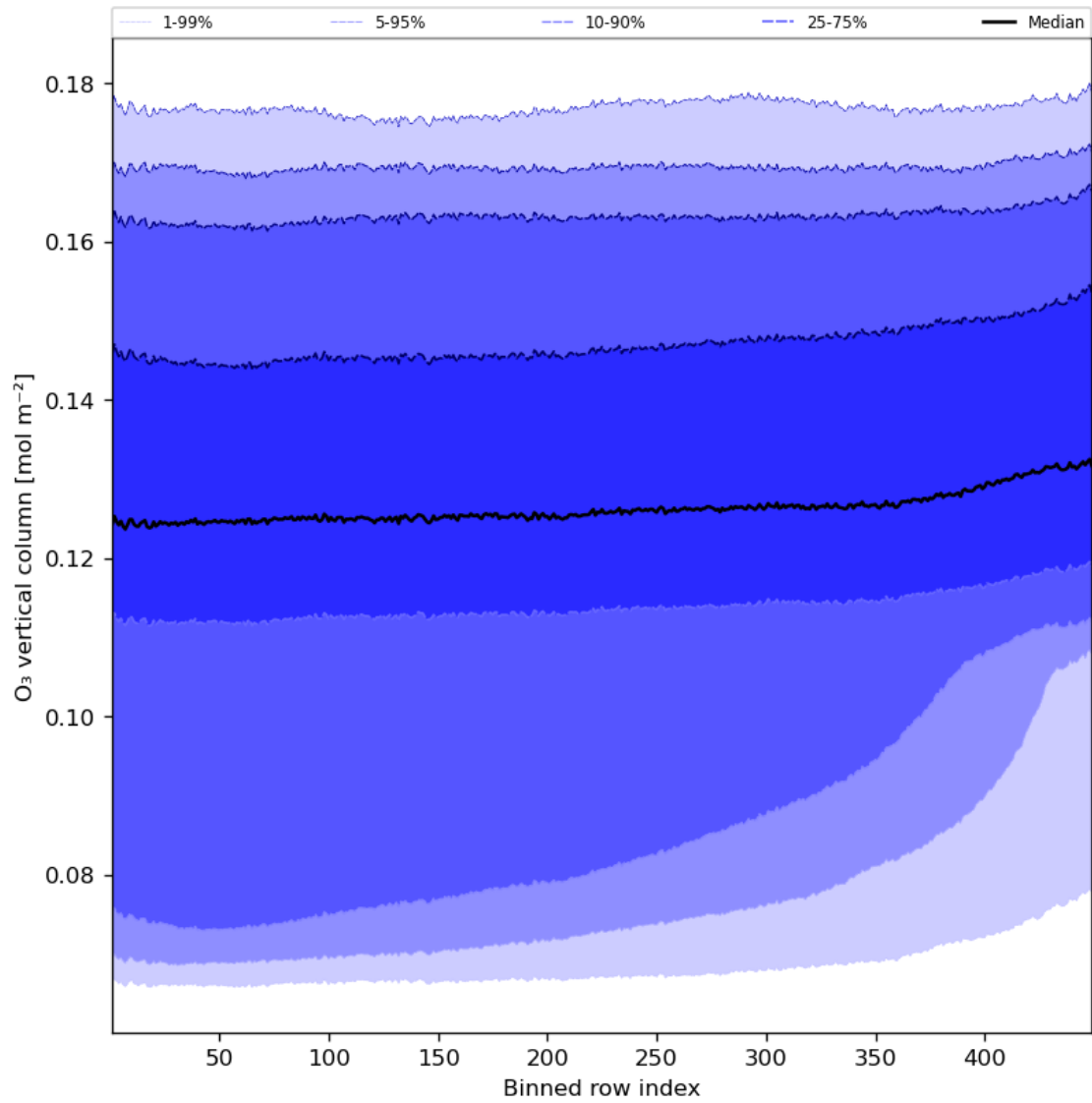
Figure 28: Along track statistics of “O 3 vertical column” for 2023-11-07 to 2023-11-09
