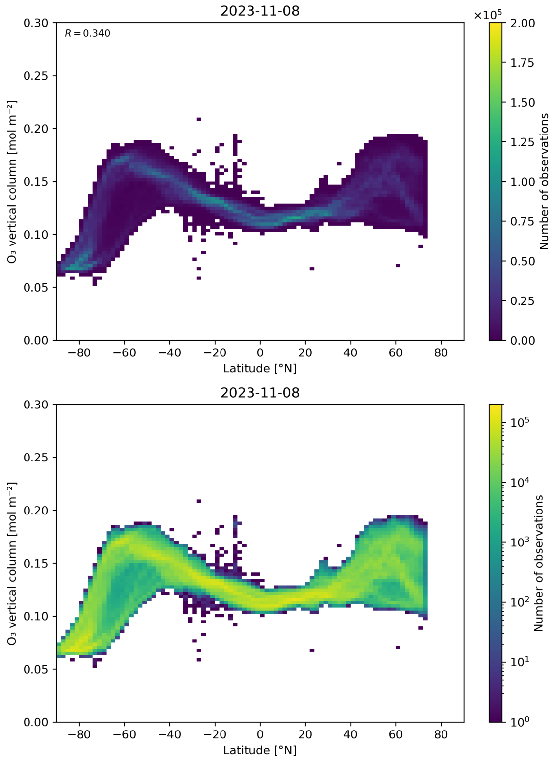
Figure 36: Scatter density plot of “Latitude” against “O 3 vertical column” for 2023-11-07 to 2023-11-09.
