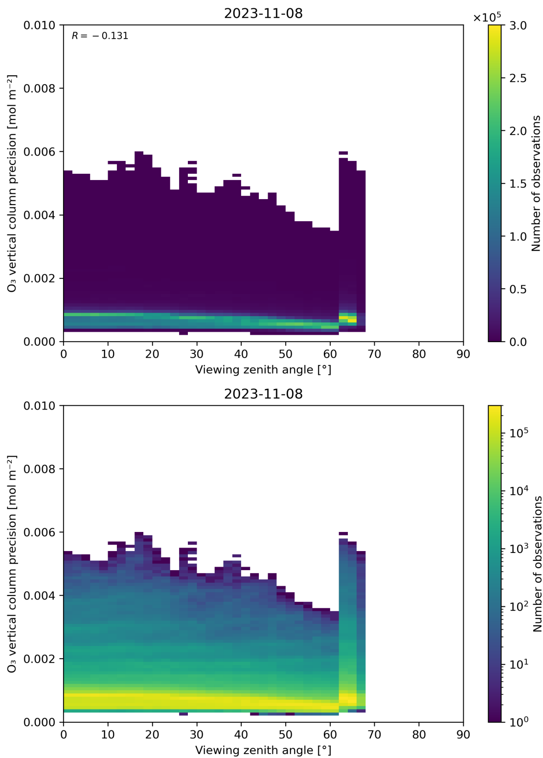
Figure 53: Scatter density plot of “Viewing zenith angle” against “O 3 vertical column precision” for 2023-11-07 to 2023-11-09.
