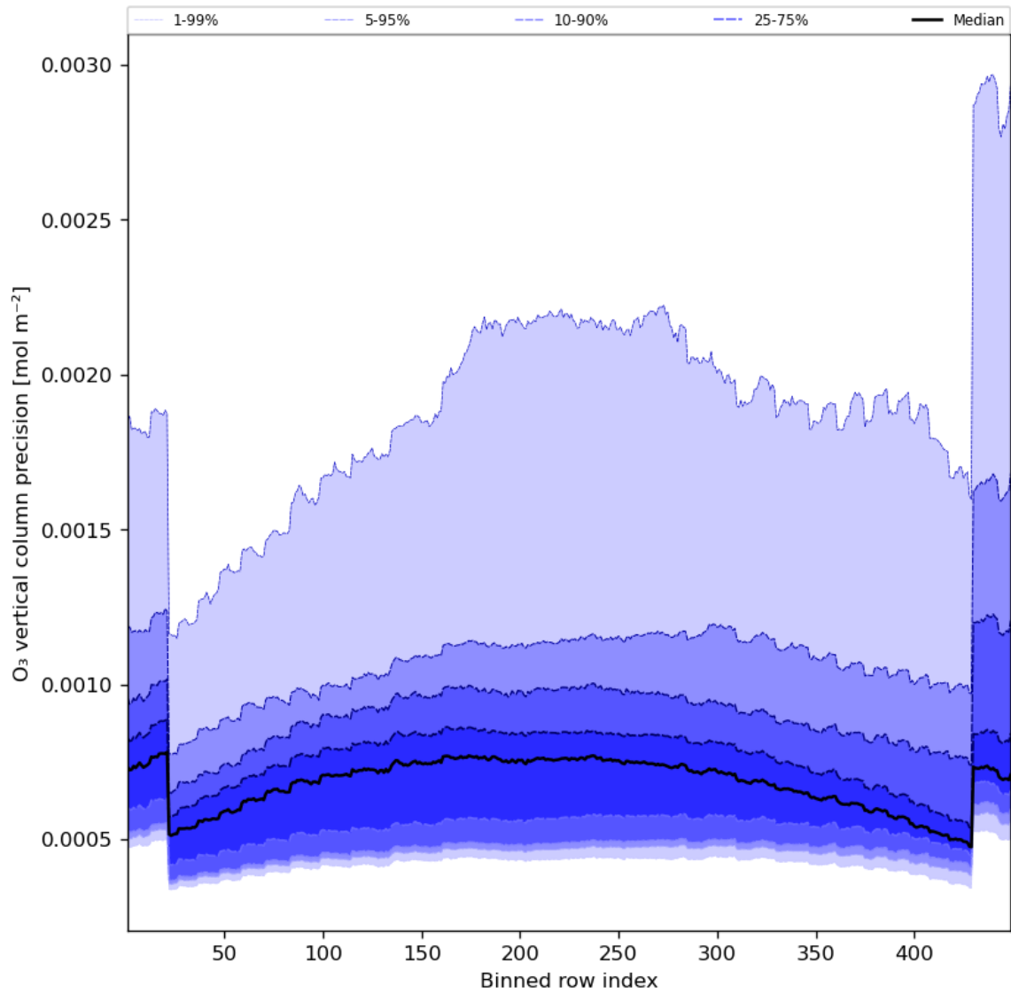
Figure 29: Along track statistics of “O 3 vertical column precision” for 2023-11-07 to 2023-11-09
