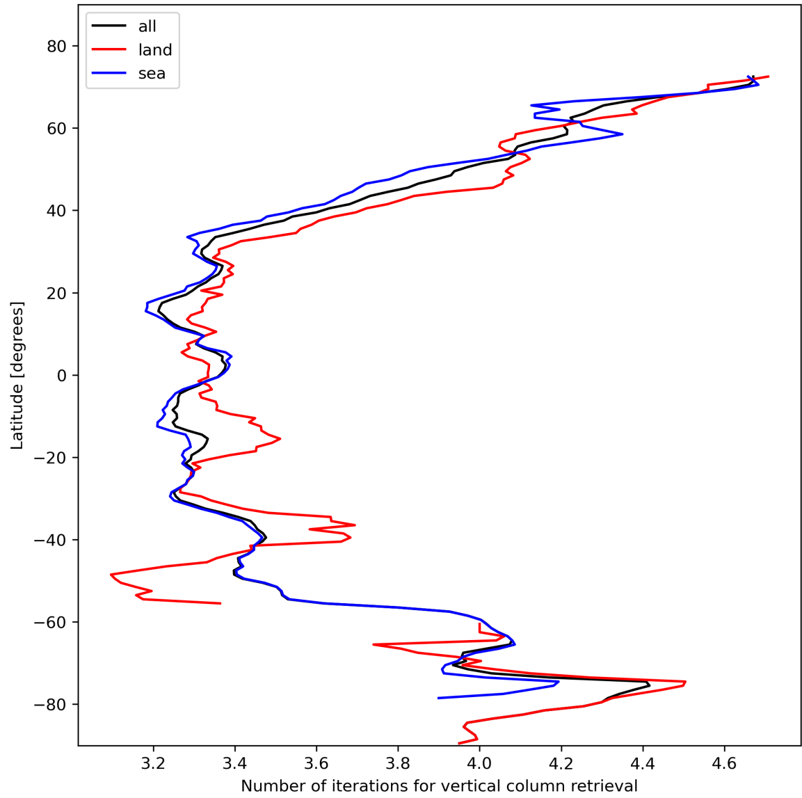
Figure 19: Zonal average of “Number of iterations for vertical column retrieval” for 2023-11-07 to 2023-11-09.
