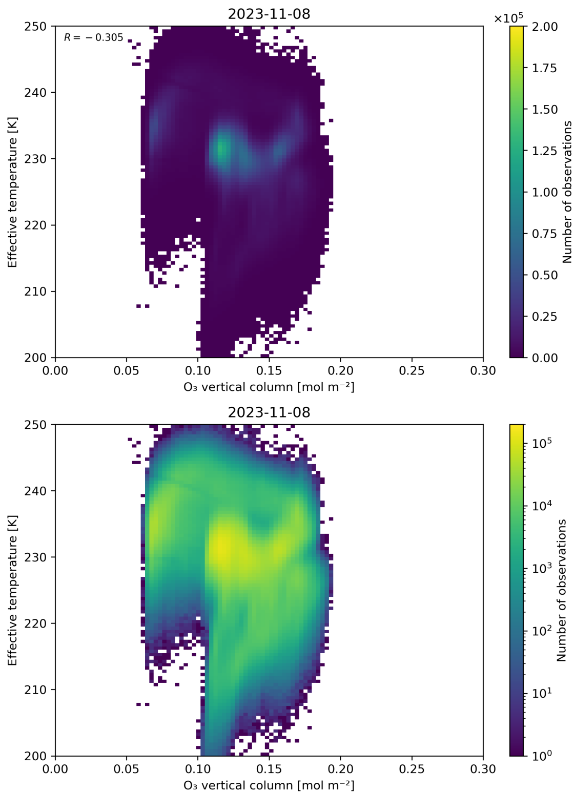
Figure 39: Scatter density plot of “O 3 vertical column” against “Effective temperature” for 2023-11-07 to 2023-11-09.
