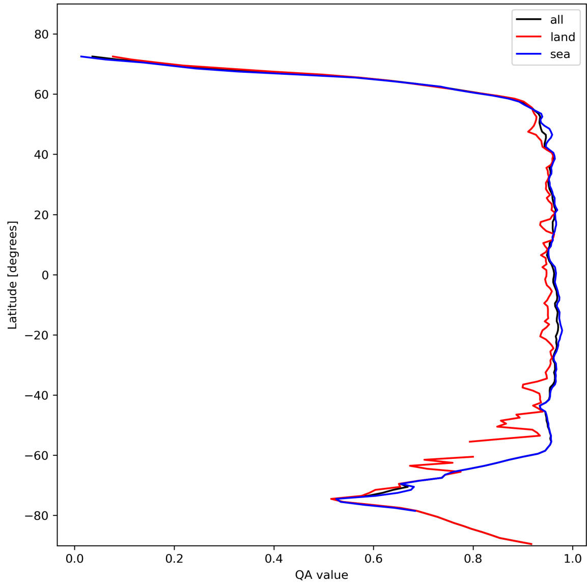
Figure 13: Zonal average of “QA value” for 2023-11-07 to 2023-11-09.
