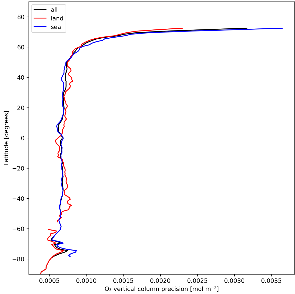
Figure 15: Zonal average of “O 3 vertical column precision” for 2023-11-07 to 2023-11-09.
