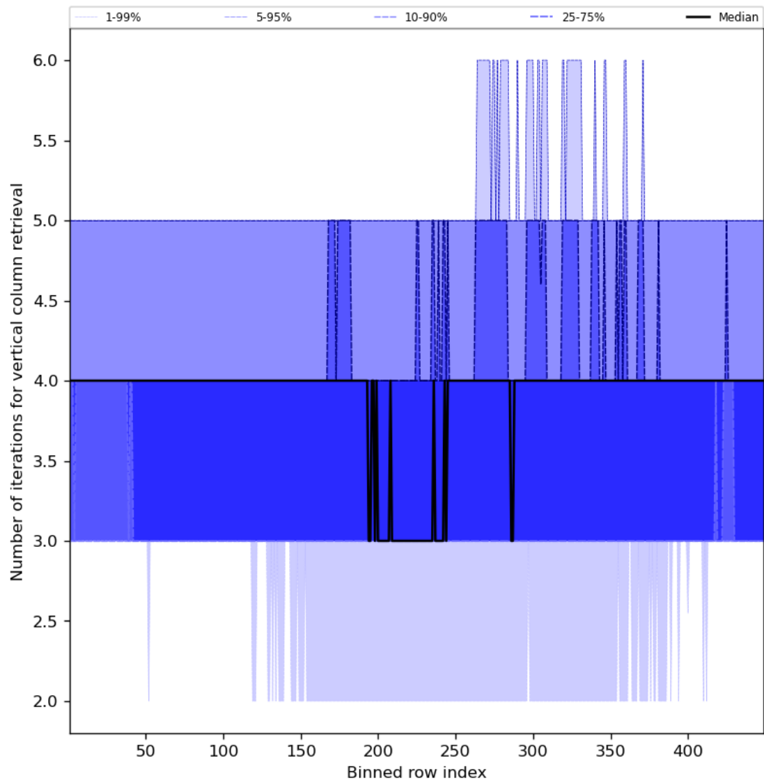
Figure 33: Along track statistics of “Number of iterations for vertical column retrieval” for 2023-11-07 to 2023-11-09
