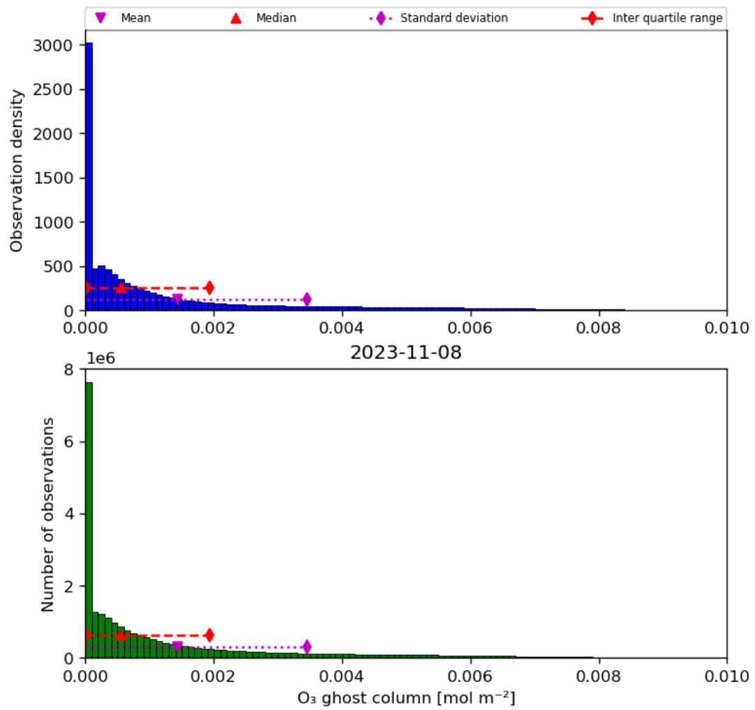
Figure 25: Histogram of “O 3 ghost column” for 2023-11-07 to 2023-11-09
