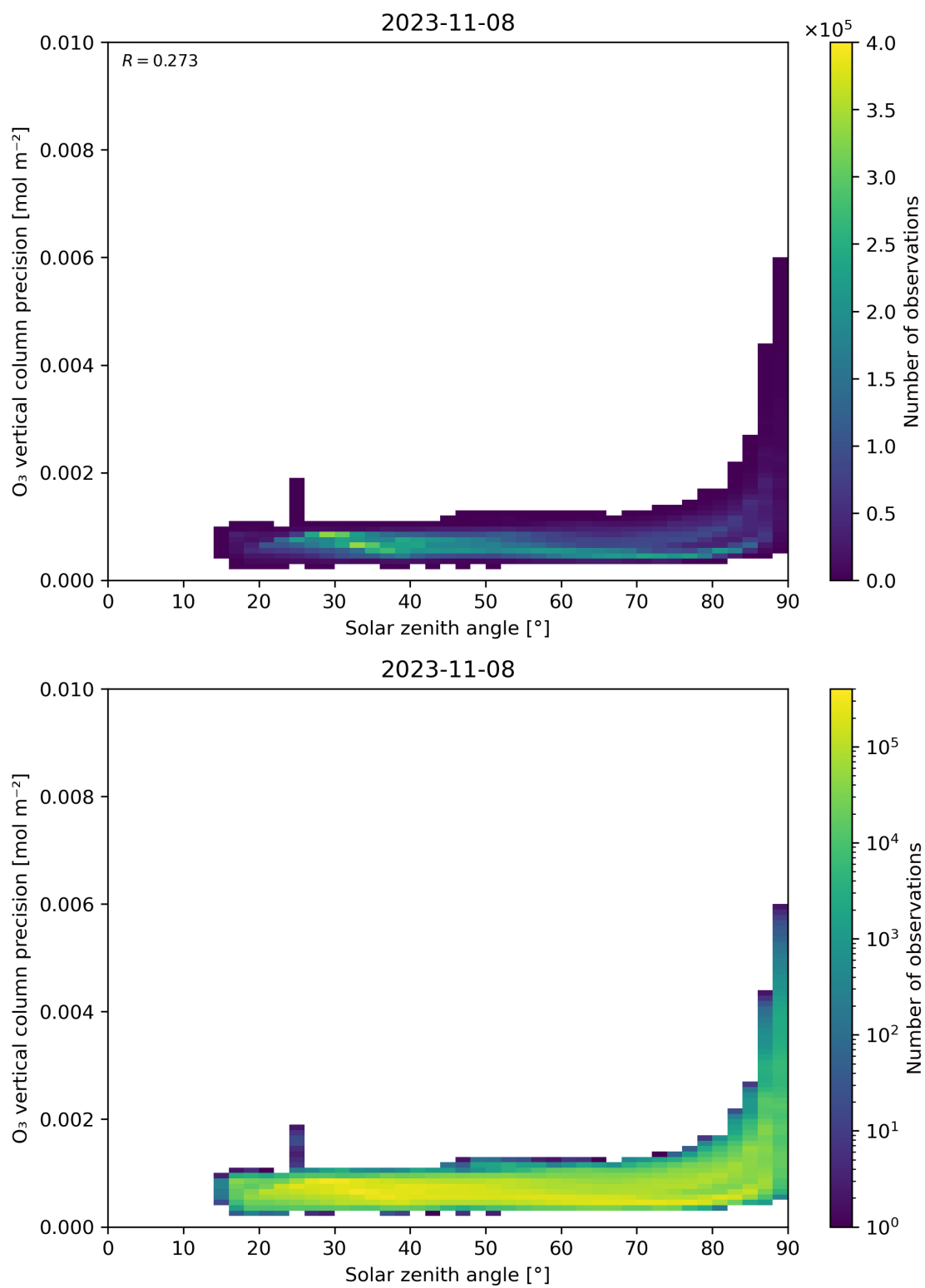
Figure 48: Scatter density plot of “Solar zenith angle” against “O 3 vertical column precision” for 2023-11-07 to 2023-11-09.
