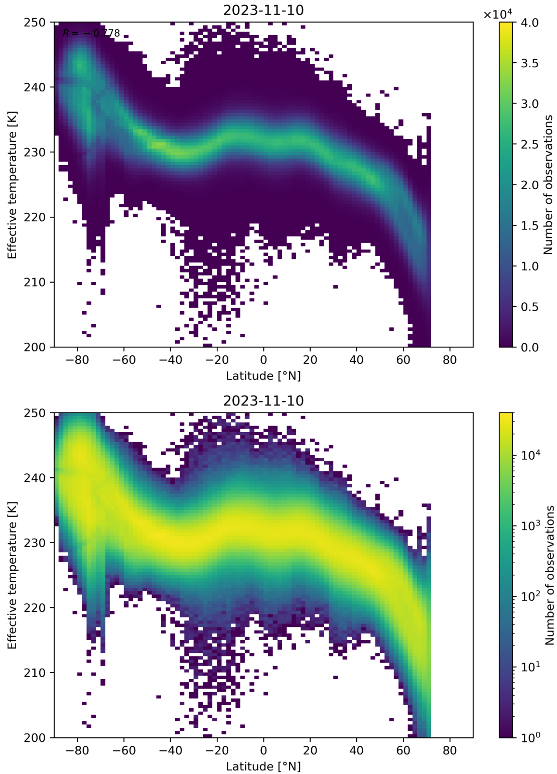
Figure 34: Scatter density plot of “Latitude” against “Effective temperature” for 2023-11-09 to 2023-11-11.
