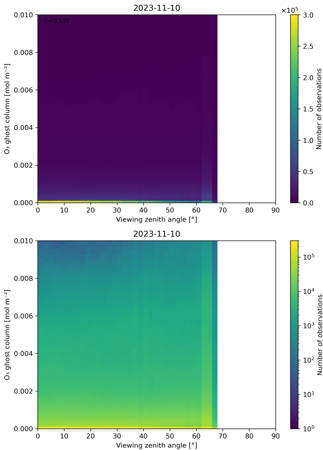
Figure 51: Scatter density plot of “Viewing zenith angle” against “O 3 ghost column” for 2023-11-09 to 2023-11-11.
