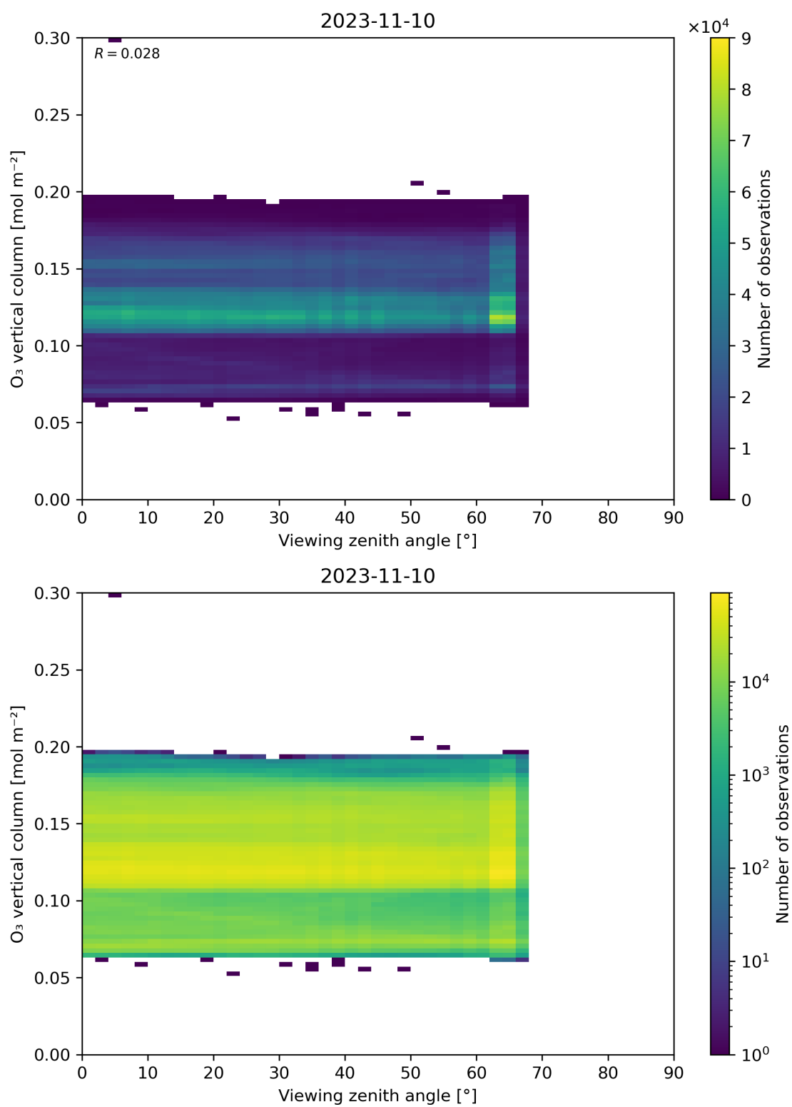
Figure 52: Scatter density plot of “Viewing zenith angle” against “O 3 vertical column” for 2023-11-09 to 2023-11-11.
