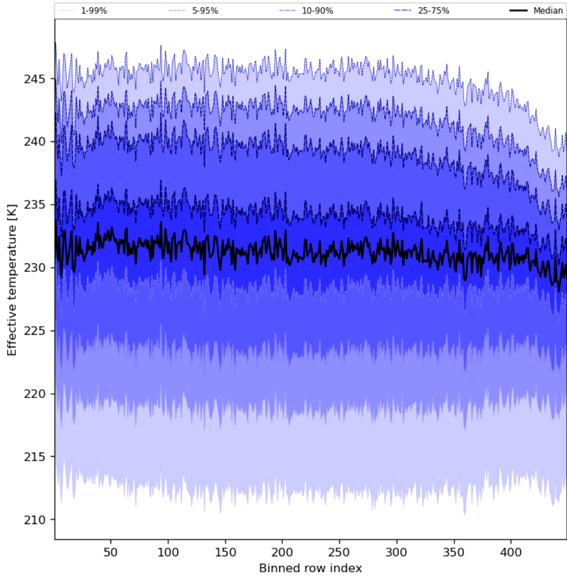
Figure 31: Along track statistics of “Effective temperature” for 2023-11-09 to 2023-11-11
