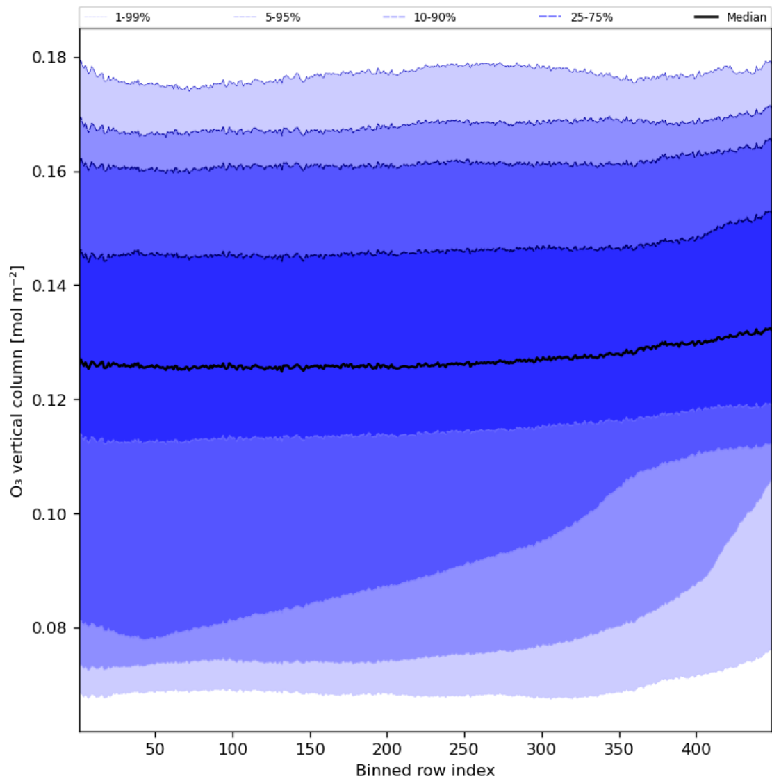
Figure 28: Along track statistics of “O 3 vertical column” for 2023-11-09 to 2023-11-11
