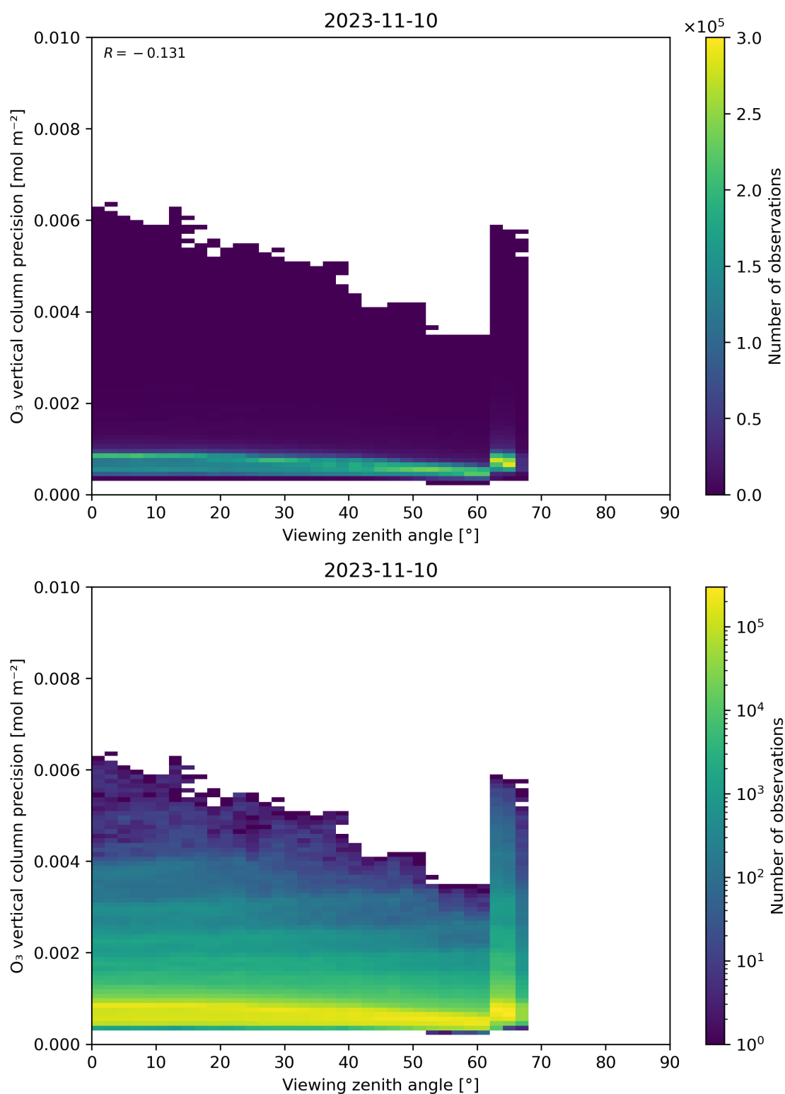
Figure 53: Scatter density plot of “Viewing zenith angle” against “O 3 vertical column precision” for 2023-11-09 to 2023-11-11.
