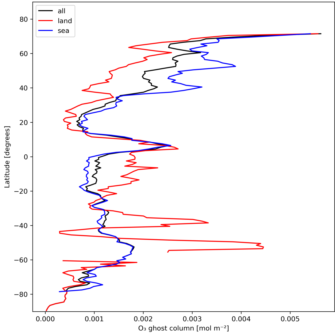
Figure 18: Zonal average of “O 3 ghost column” for 2023-11-09 to 2023-11-11.
