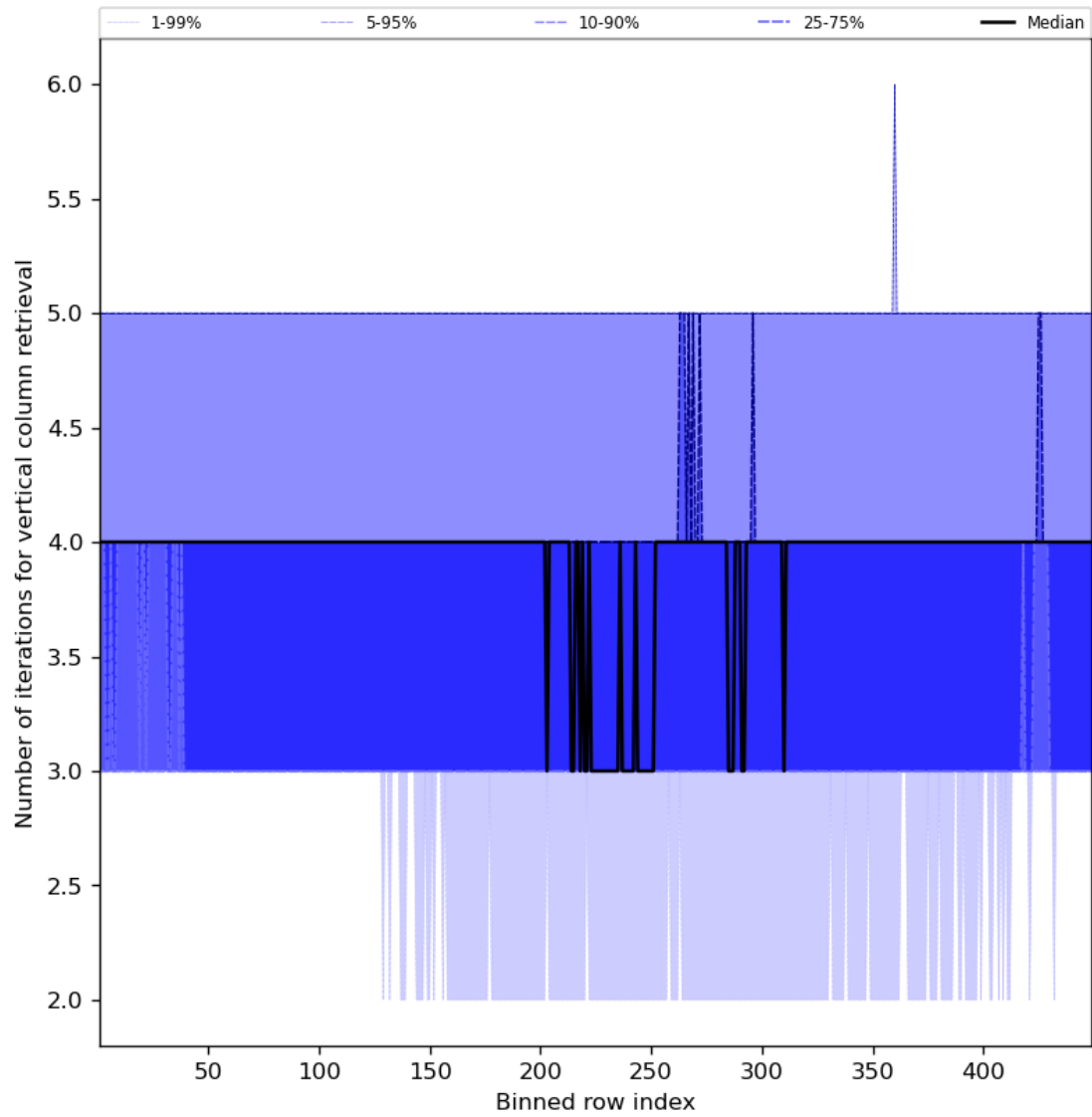
Figure 33: Along track statistics of “Number of iterations for vertical column retrieval” for 2023-11-09 to 2023-11-11
