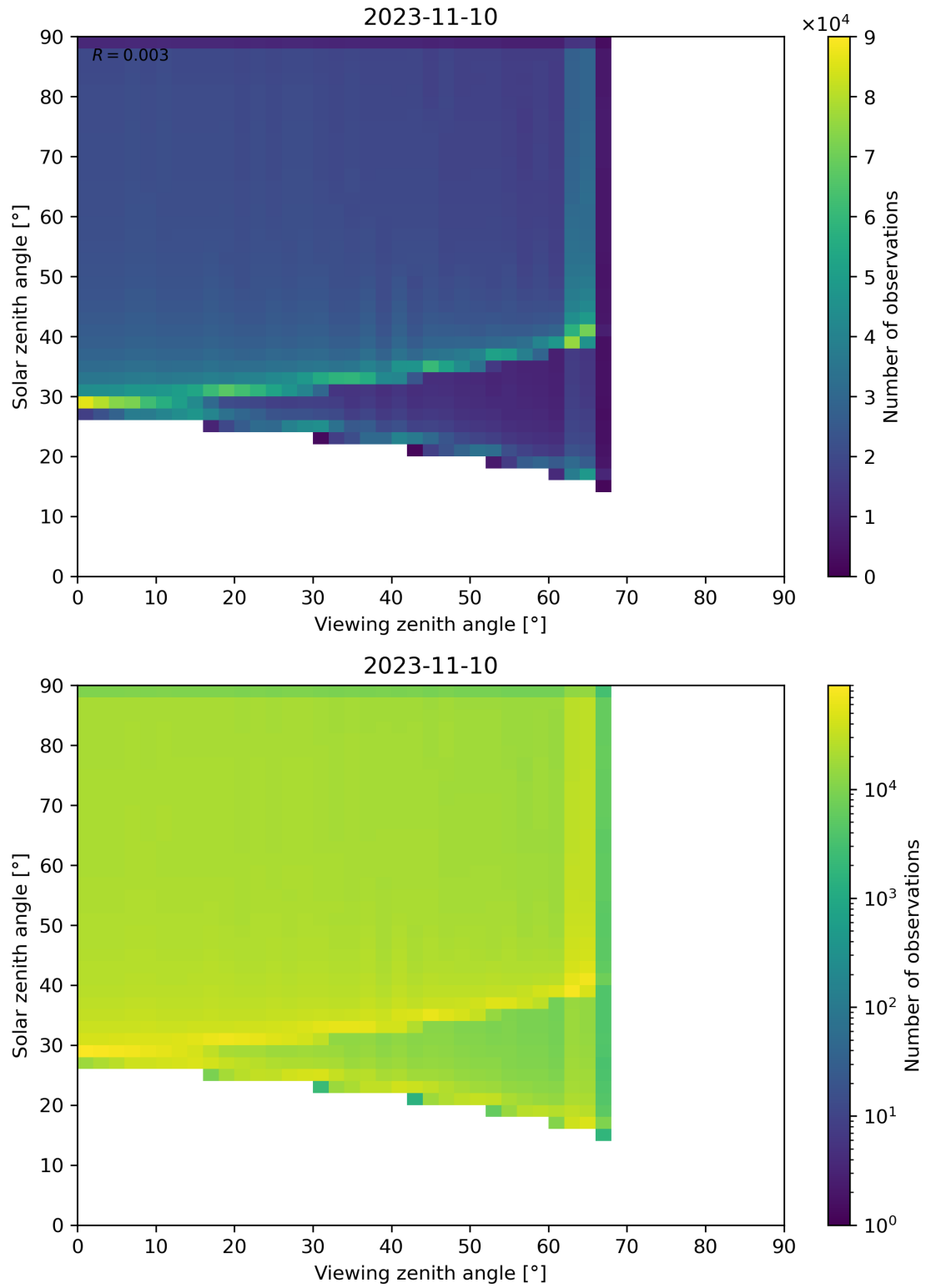
Figure 54: Scatter density plot of “Viewing zenith angle” against “Solar zenith angle” for 2023-11-09 to 2023-11-11.
