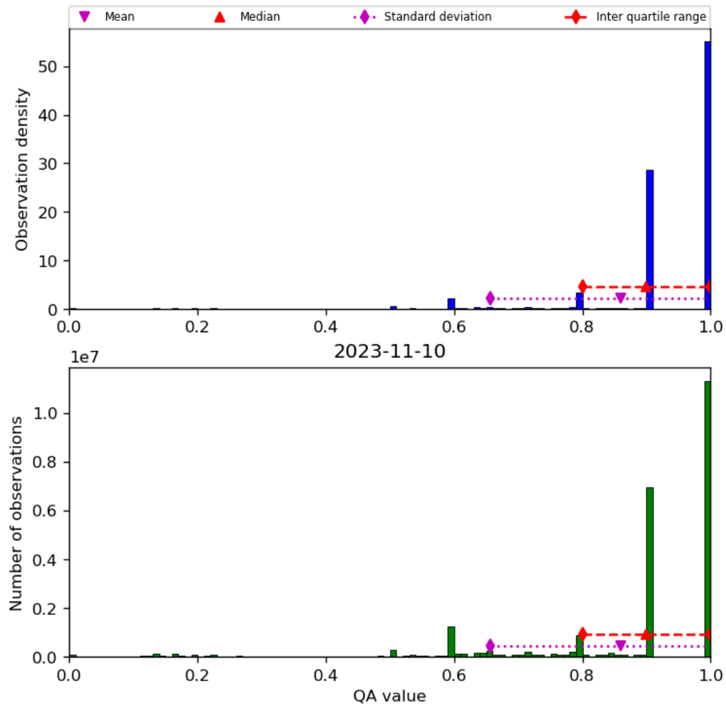
Figure 20: Histogram of “QA value” for 2023-11-09 to 2023-11-11
