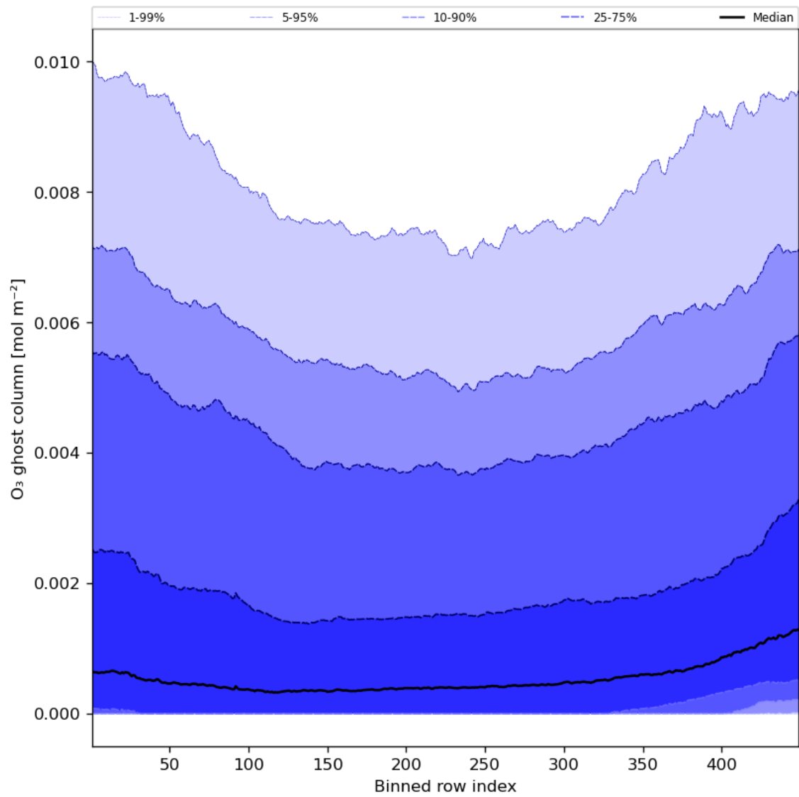
Figure 32: Along track statistics of “O 3 ghost column” for 2023-11-09 to 2023-11-11
