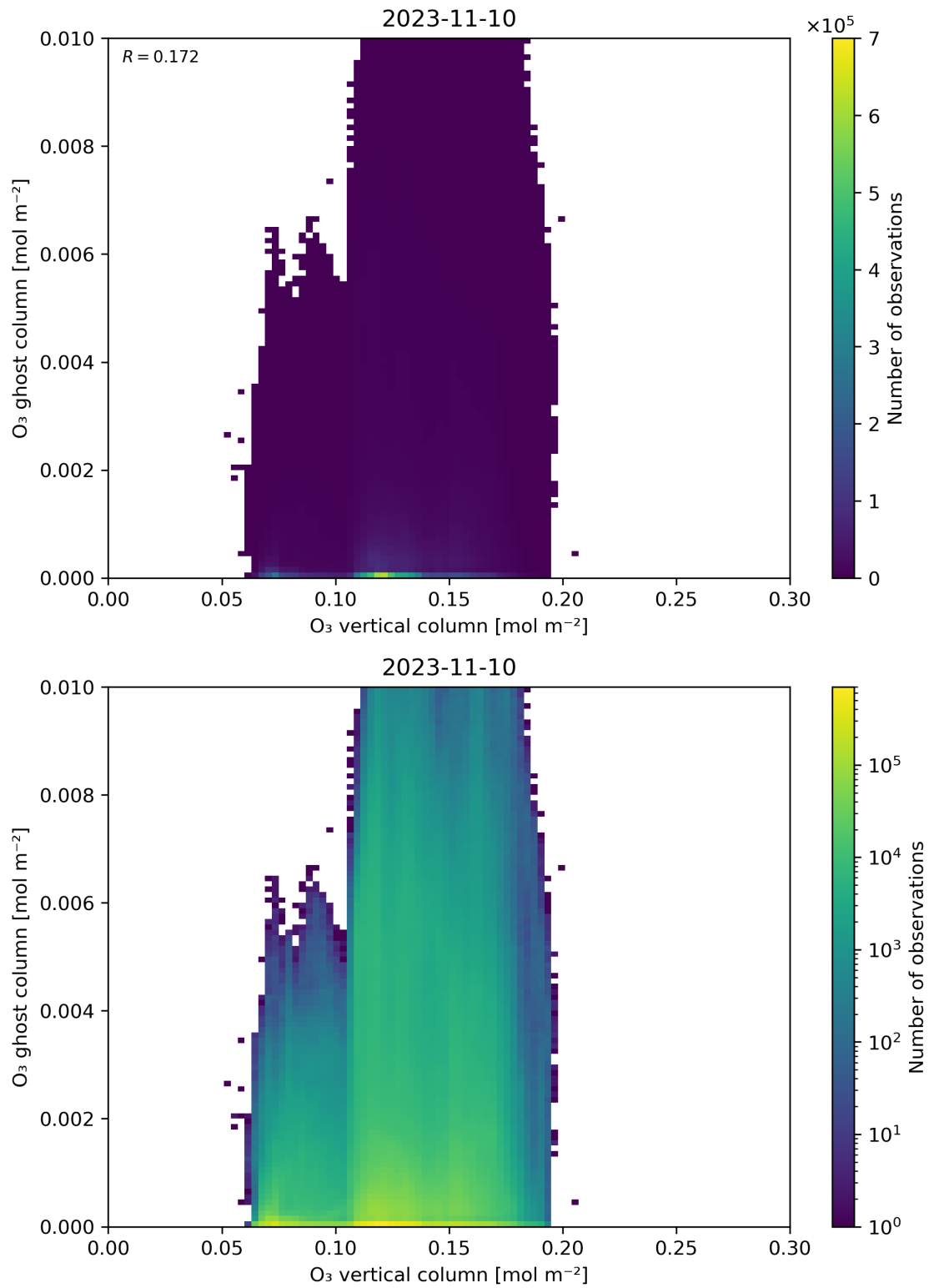
Figure 40: Scatter density plot of “O 3 vertical column” against “O 3 ghost column” for 2023-11-09 to 2023-11-11.
