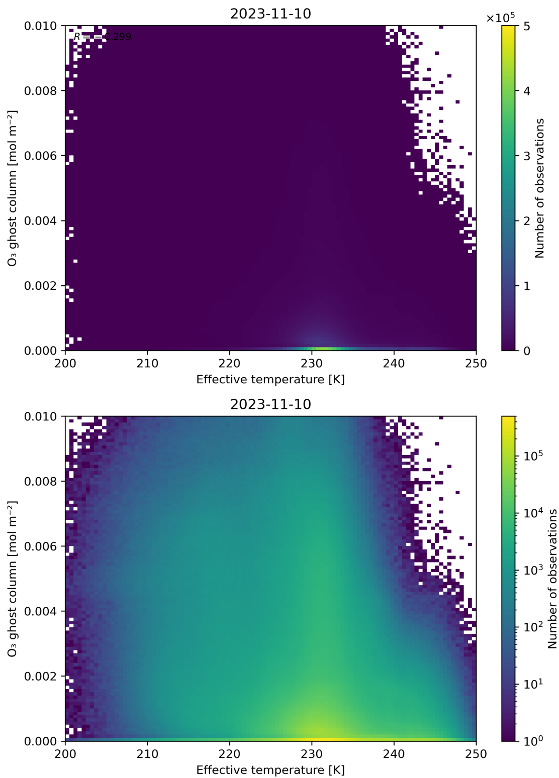
Figure 38: Scatter density plot of “Effective temperature” against “O 3 ghost column” for 2023-11-09 to 2023-11-11.
