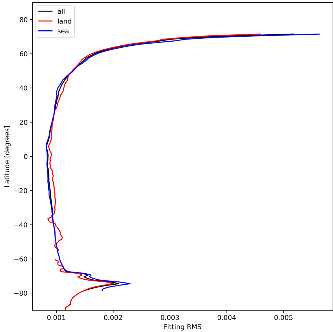
Figure 16: Zonal average of “Fitting RMS” for 2023-11-09 to 2023-11-11.
