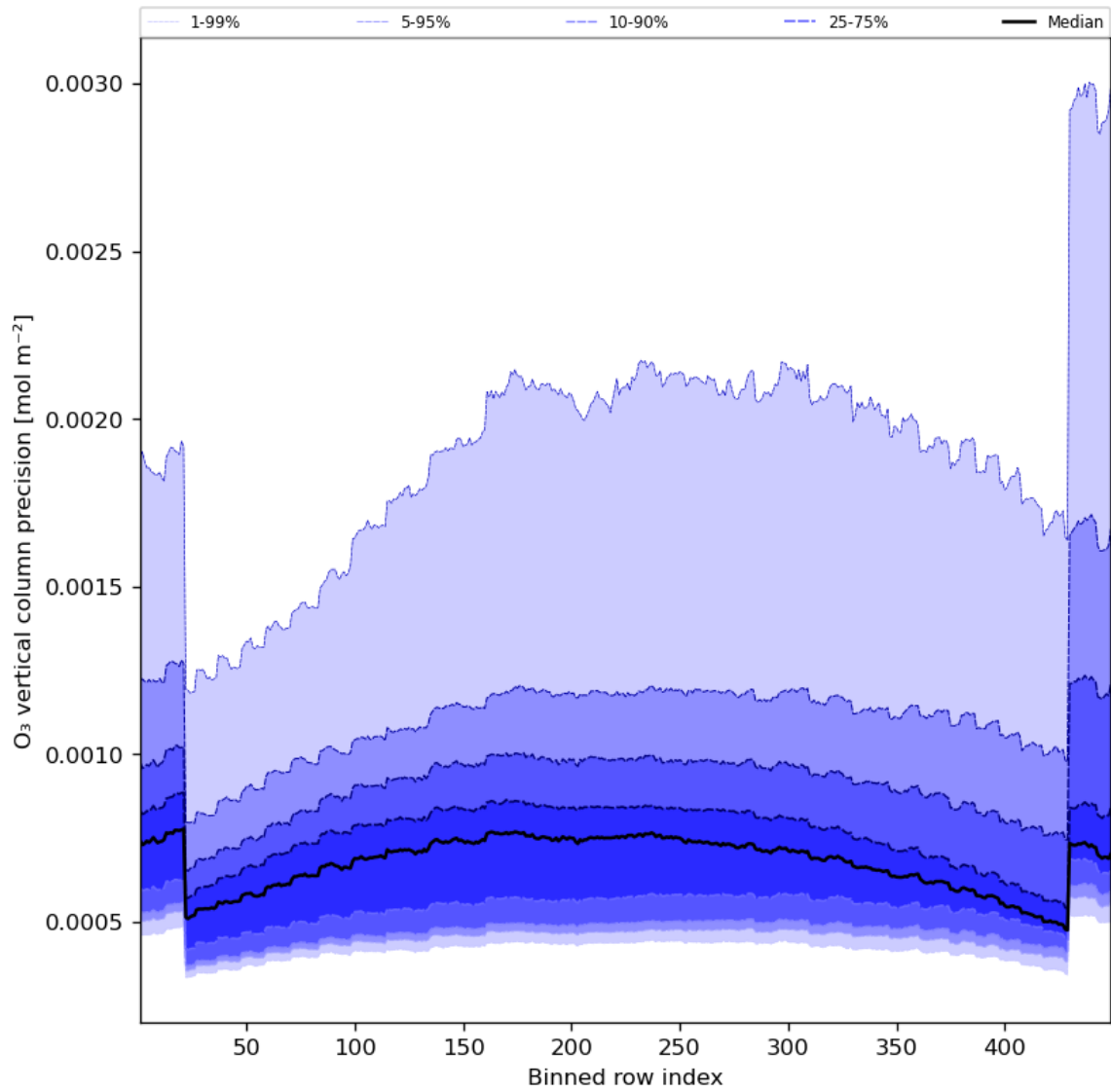
Figure 29: Along track statistics of “O 3 vertical column precision” for 2023-11-09 to 2023-11-11
