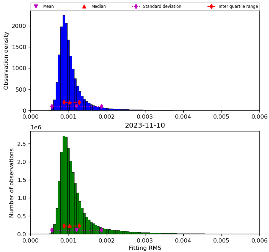
Figure 23: Histogram of “Fitting RMS” for 2023-11-09 to 2023-11-11
