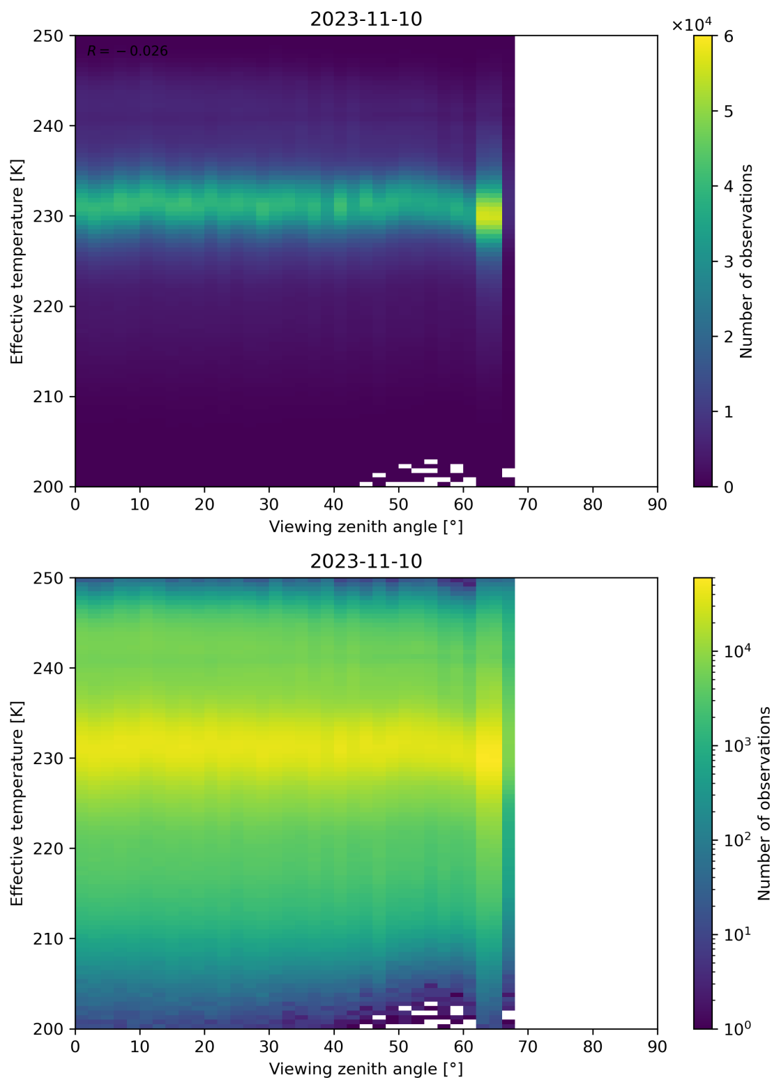
Figure 50: Scatter density plot of “Viewing zenith angle” against “Effective temperature” for 2023-11-09 to 2023-11-11.
