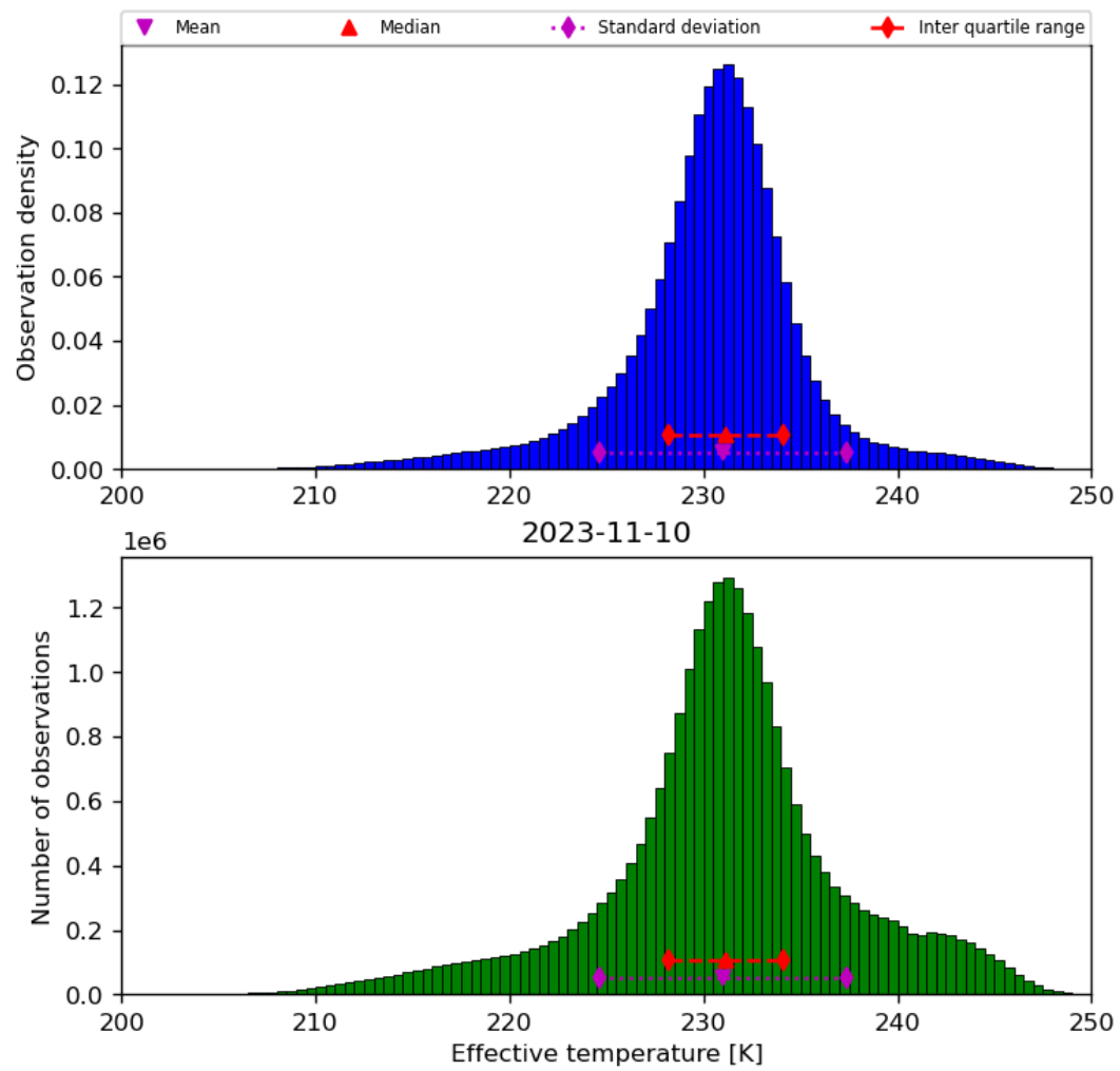
Figure 24: Histogram of “Effective temperature” for 2023-11-09 to 2023-11-11
