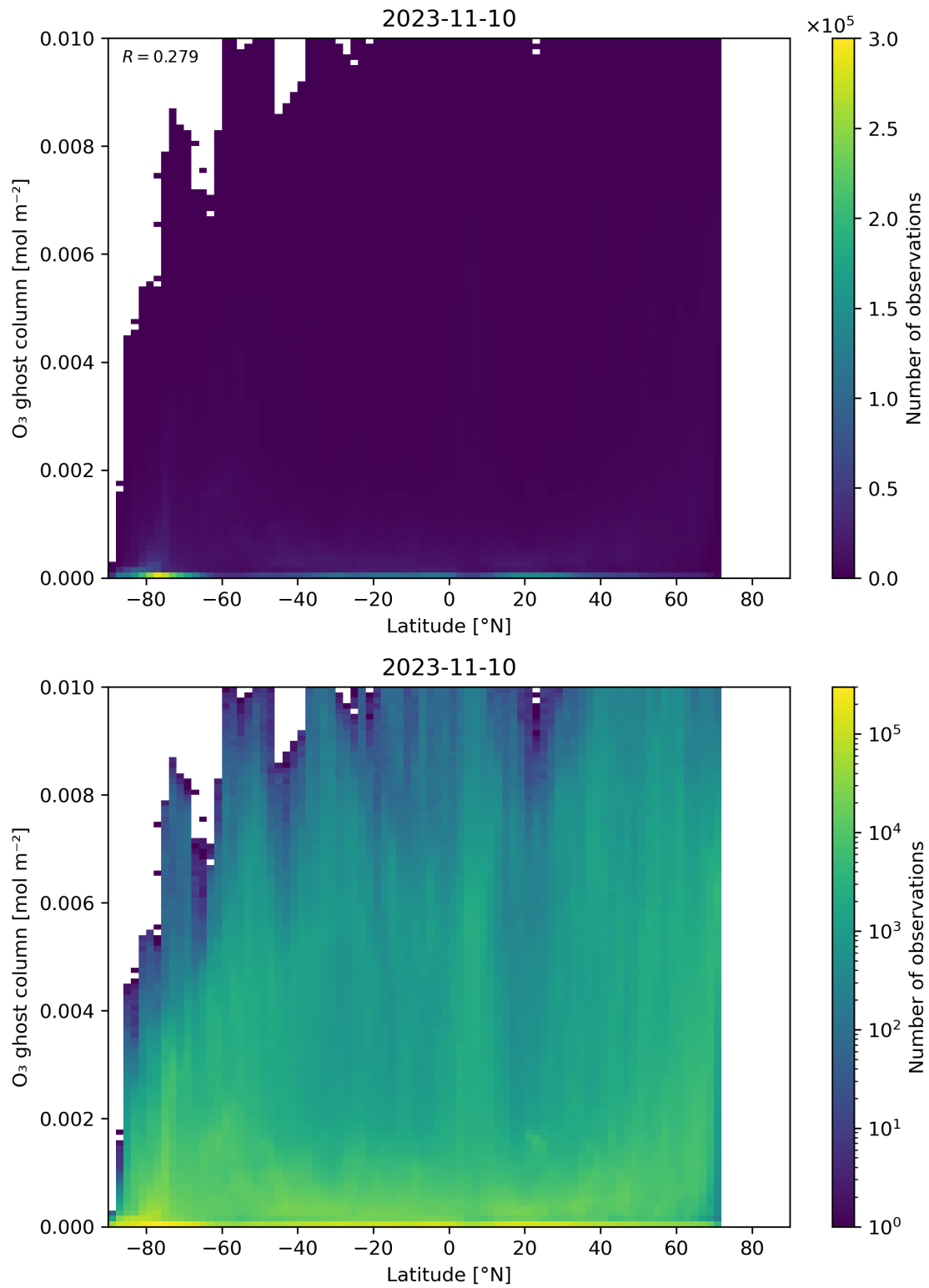
Figure 35: Scatter density plot of “Latitude” against “O 3 ghost column” for 2023-11-09 to 2023-11-11.
