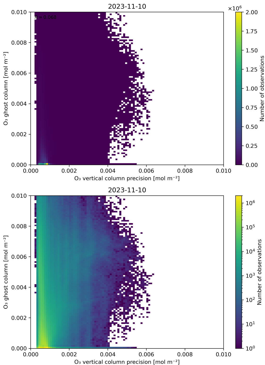
Figure 43: Scatter density plot of “O 3 vertical column precision” against “O 3 ghost column” for 2023-11-09 to 2023-11-11.
