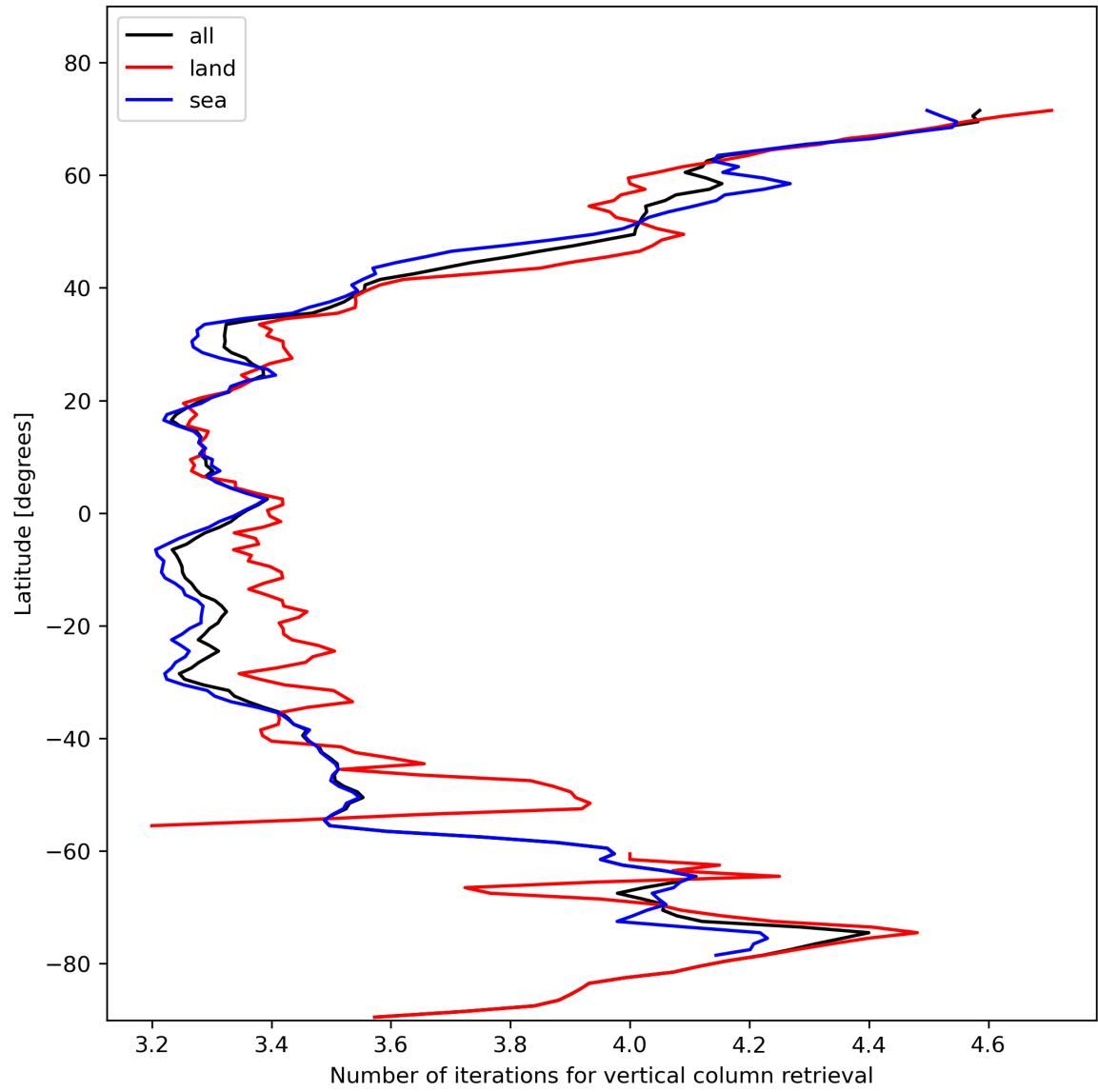
Figure 19: Zonal average of “Number of iterations for vertical column retrieval” for 2023-11-09 to 2023-11-11.
