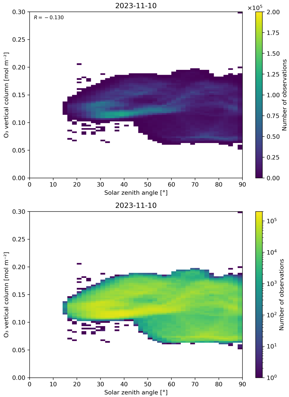
Figure 47: Scatter density plot of “Solar zenith angle” against “O 3 vertical column” for 2023-11-09 to 2023-11-11.
