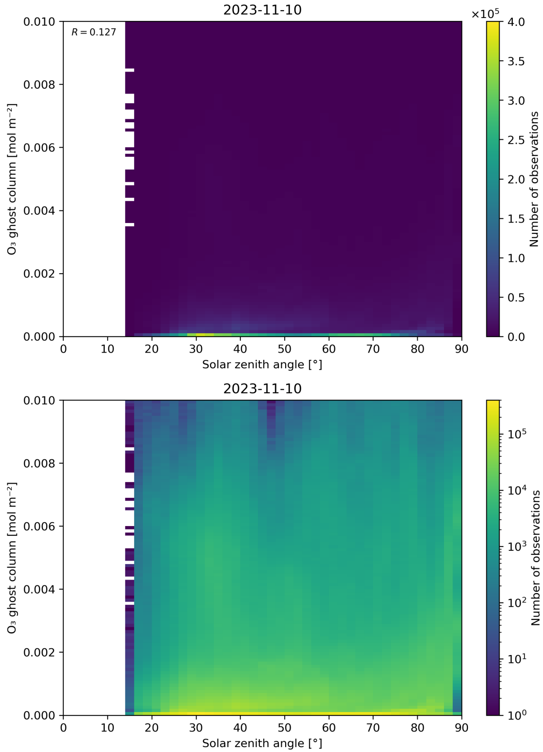
Figure 46: Scatter density plot of “Solar zenith angle” against “O 3 ghost column” for 2023-11-09 to 2023-11-11.
