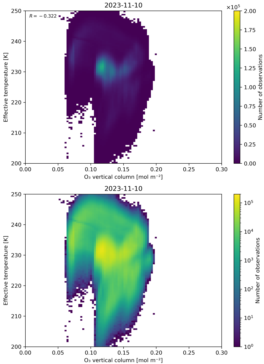
Figure 39: Scatter density plot of “O 3 vertical column” against “Effective temperature” for 2023-11-09 to 2023-11-11.
