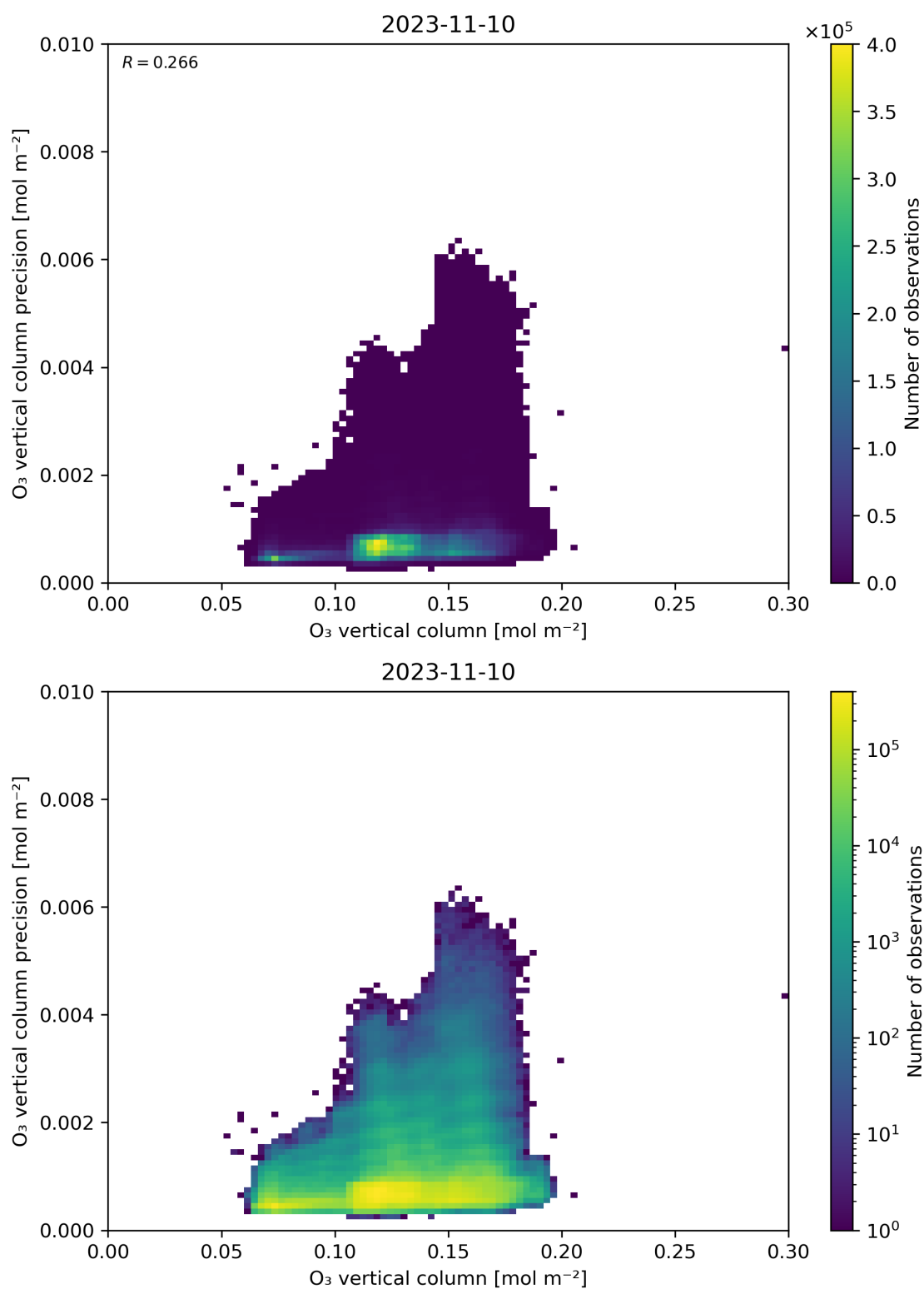
Figure 41: Scatter density plot of “O 3 vertical column” against “O 3 vertical column precision” for 2023-11-09 to 2023-11-11.
