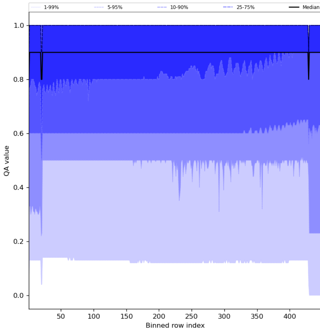
Figure 27: Along track statistics of “QA value” for 2023-11-09 to 2023-11-11
