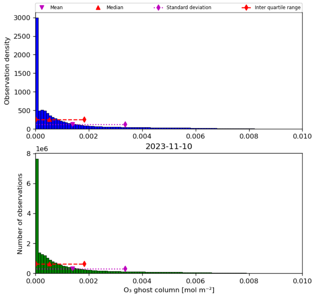
Figure 25: Histogram of “O 3 ghost column” for 2023-11-09 to 2023-11-11
