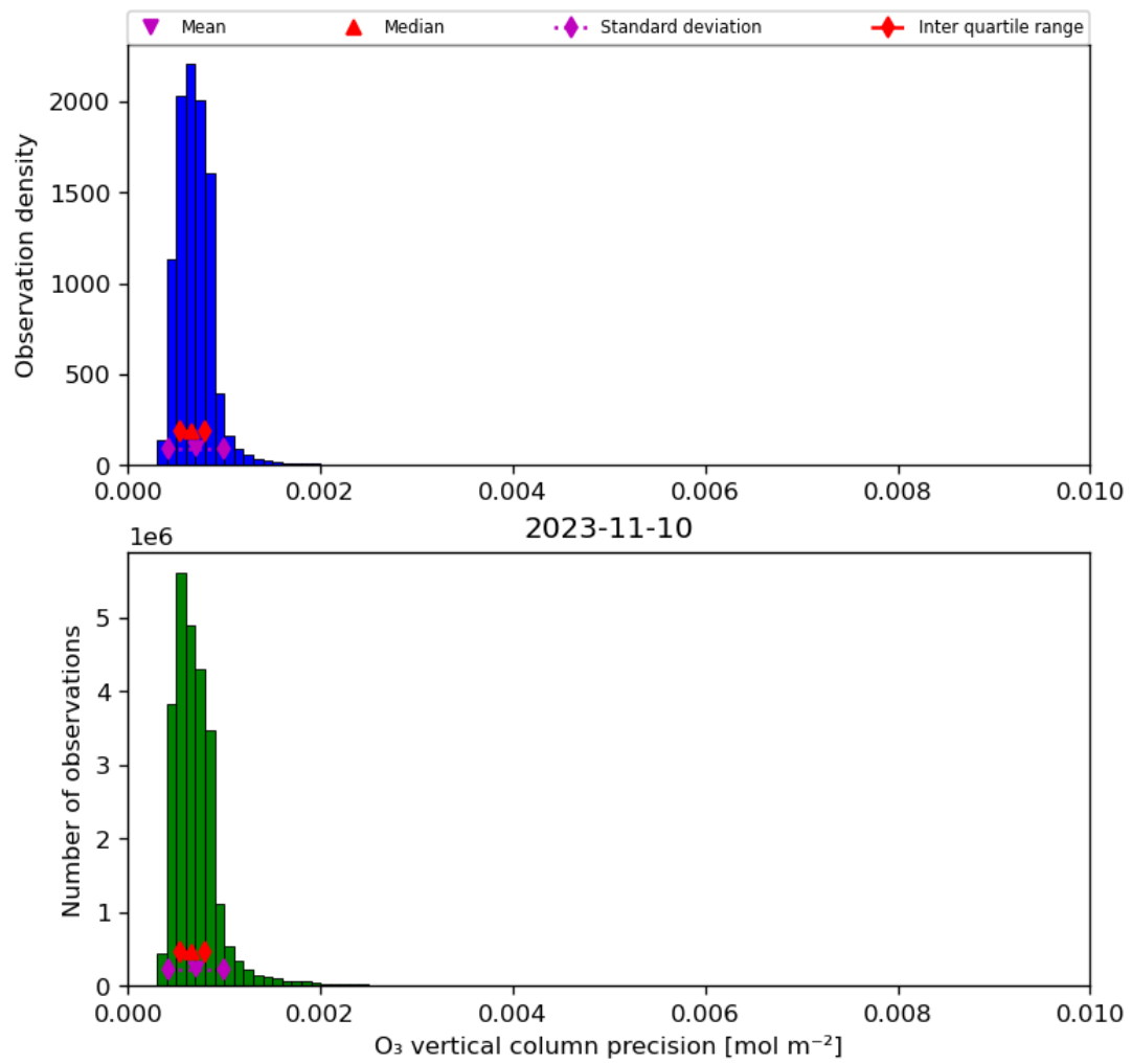
Figure 22: Histogram of “O 3 vertical column precision” for 2023-11-09 to 2023-11-11
