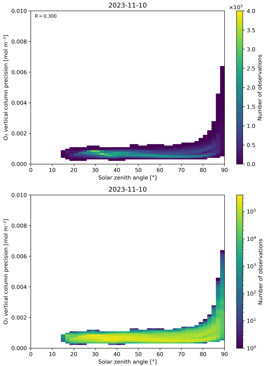
Figure 48: Scatter density plot of “Solar zenith angle” against “O 3 vertical column precision” for 2023-11-09 to 2023-11-11.
