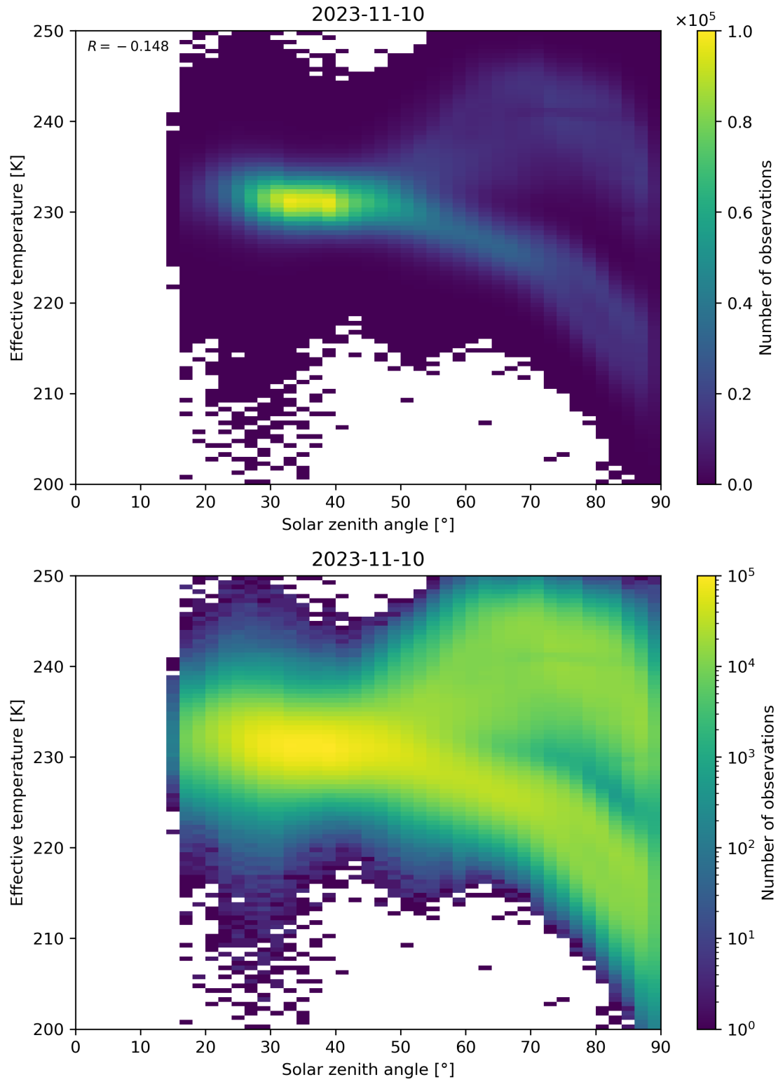
Figure 45: Scatter density plot of “Solar zenith angle” against “Effective temperature” for 2023-11-09 to 2023-11-11.
