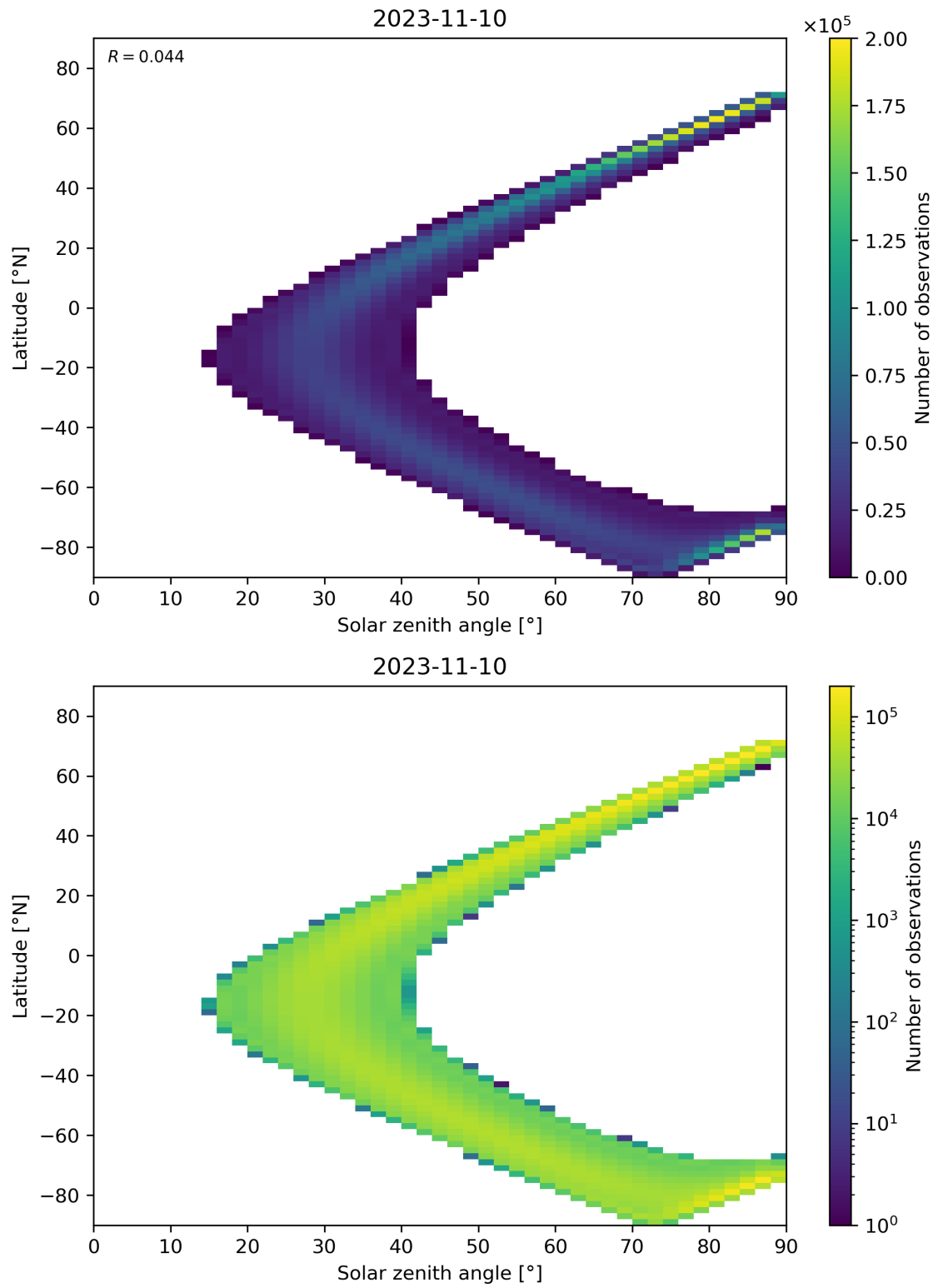
Figure 44: Scatter density plot of “Solar zenith angle” against “Latitude” for 2023-11-09 to 2023-11-11.
