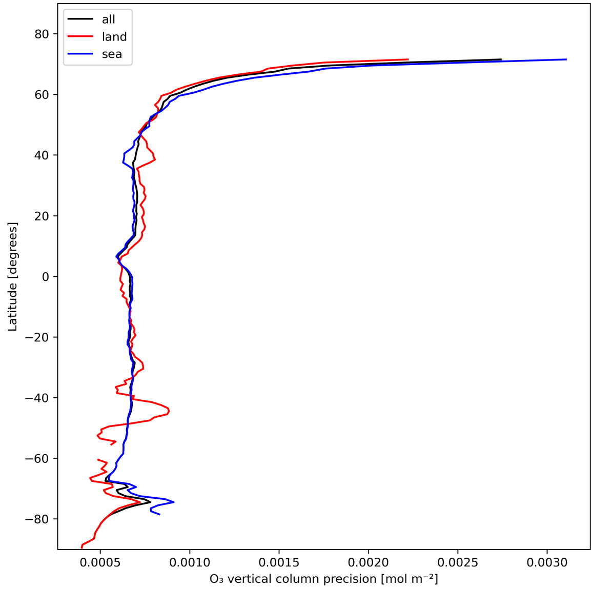
Figure 15: Zonal average of “O 3 vertical column precision” for 2023-11-09 to 2023-11-11.
