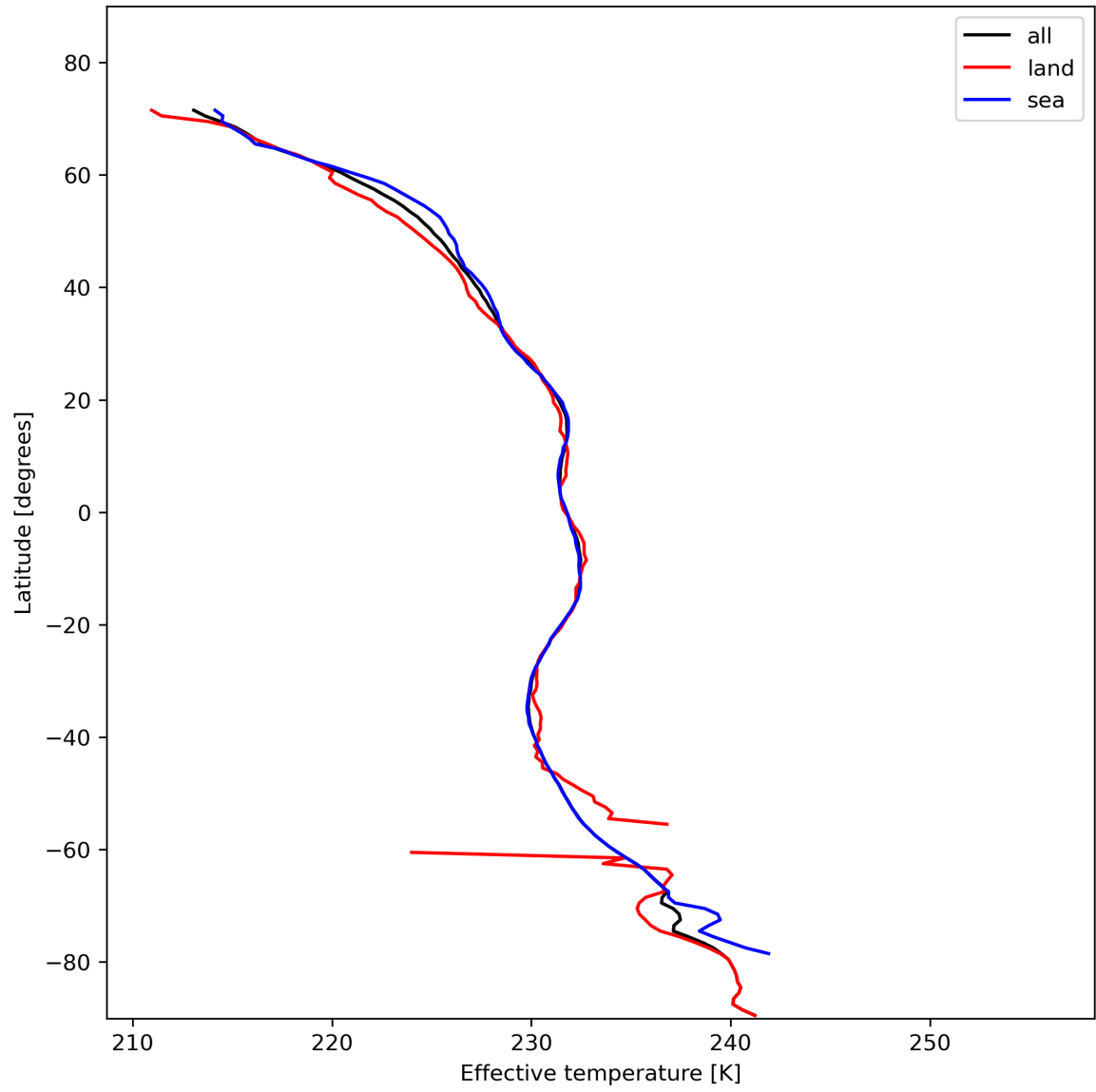
Figure 17: Zonal average of "Effective temperature" for 2023-11-09 to 2023-11-11.
