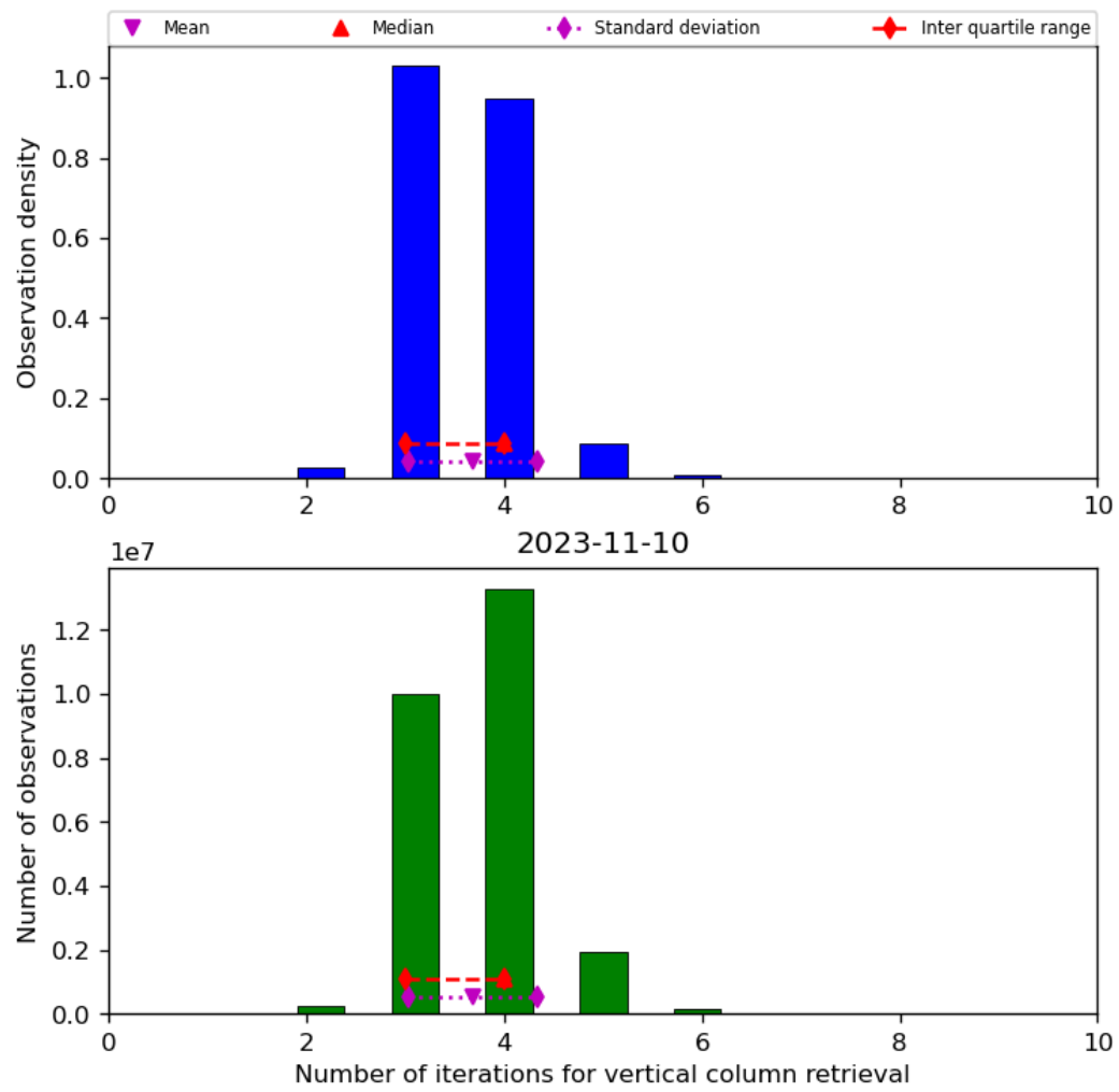
Figure 26: Histogram of “Number of iterations for vertical column retrieval” for 2023-11-09 to 2023-11-11
