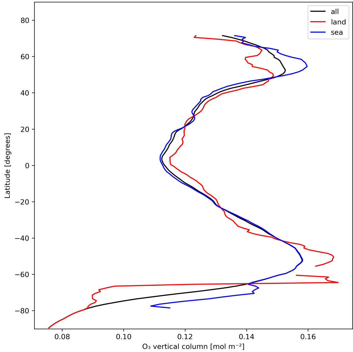
Figure 14: Zonal average of “O 3 vertical column” for 2023-11-09 to 2023-11-11.
