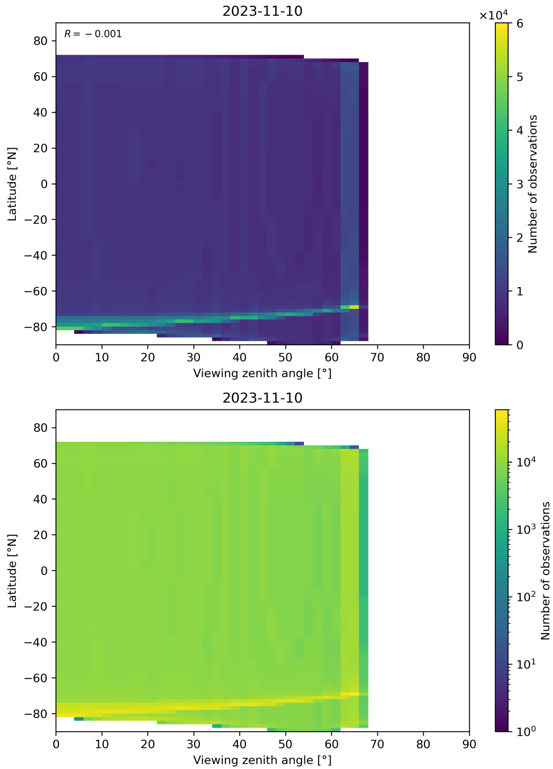
Figure 49: Scatter density plot of “Viewing zenith angle” against “Latitude” for 2023-11-09 to 2023-11-11.
