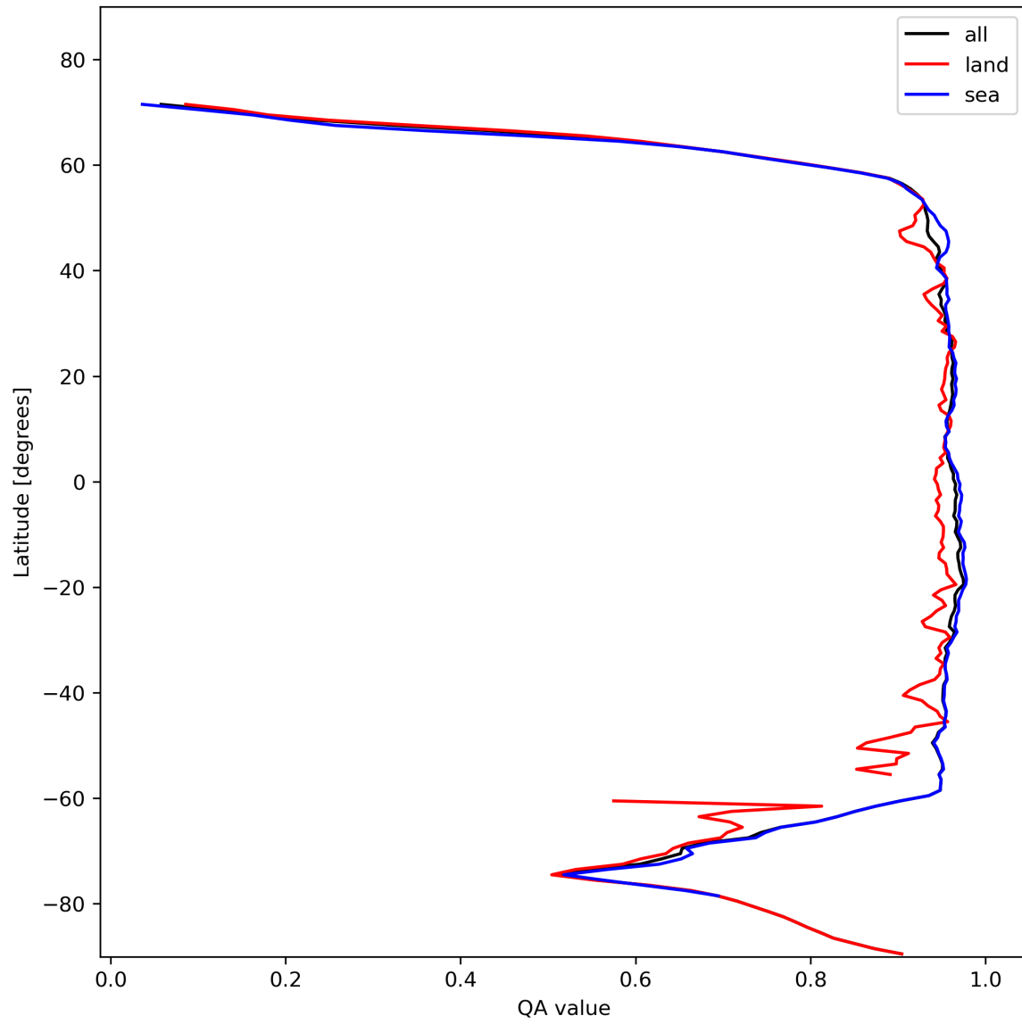
Figure 13: Zonal average of “QA value” for 2023-11-09 to 2023-11-11.
