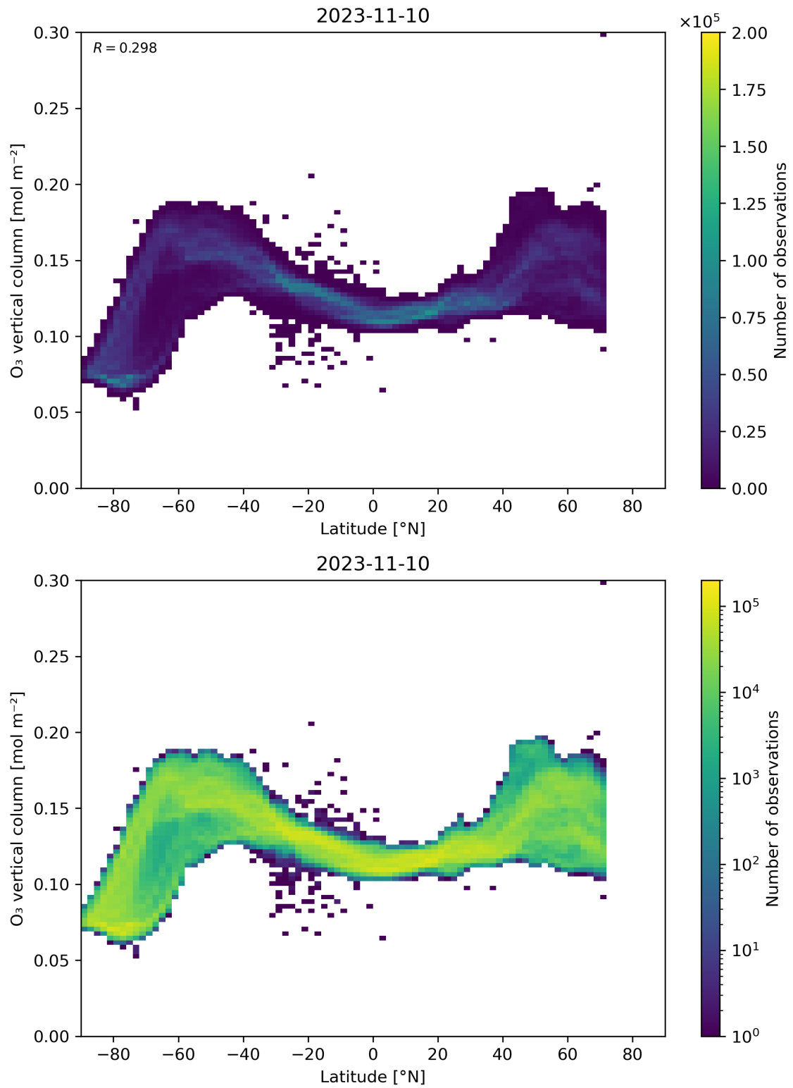
Figure 36: Scatter density plot of “Latitude” against “O 3 vertical column” for 2023-11-09 to 2023-11-11.
