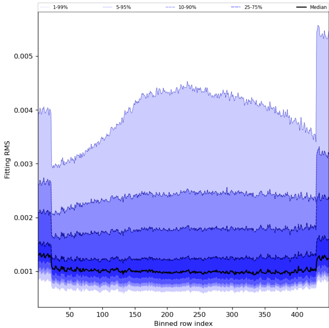
Figure 30: Along track statistics of “Fitting RMS” for 2023-11-09 to 2023-11-11
