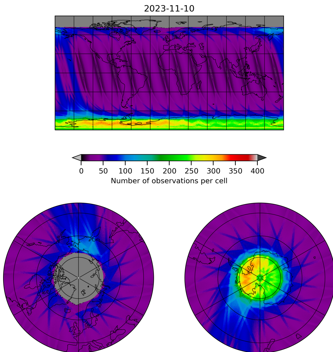
Figure 12: Map of the number of observations for 2023-11-09 to 2023-11-11
