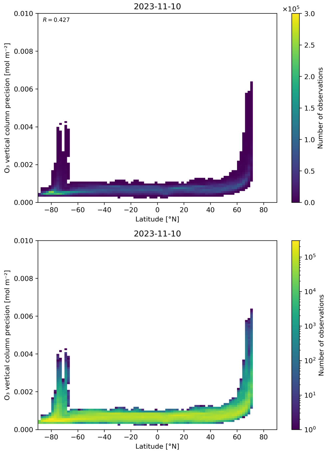
Figure 37: Scatter density plot of “Latitude” against “O 3 vertical column precision” for 2023-11-09 to 2023-11-11.
