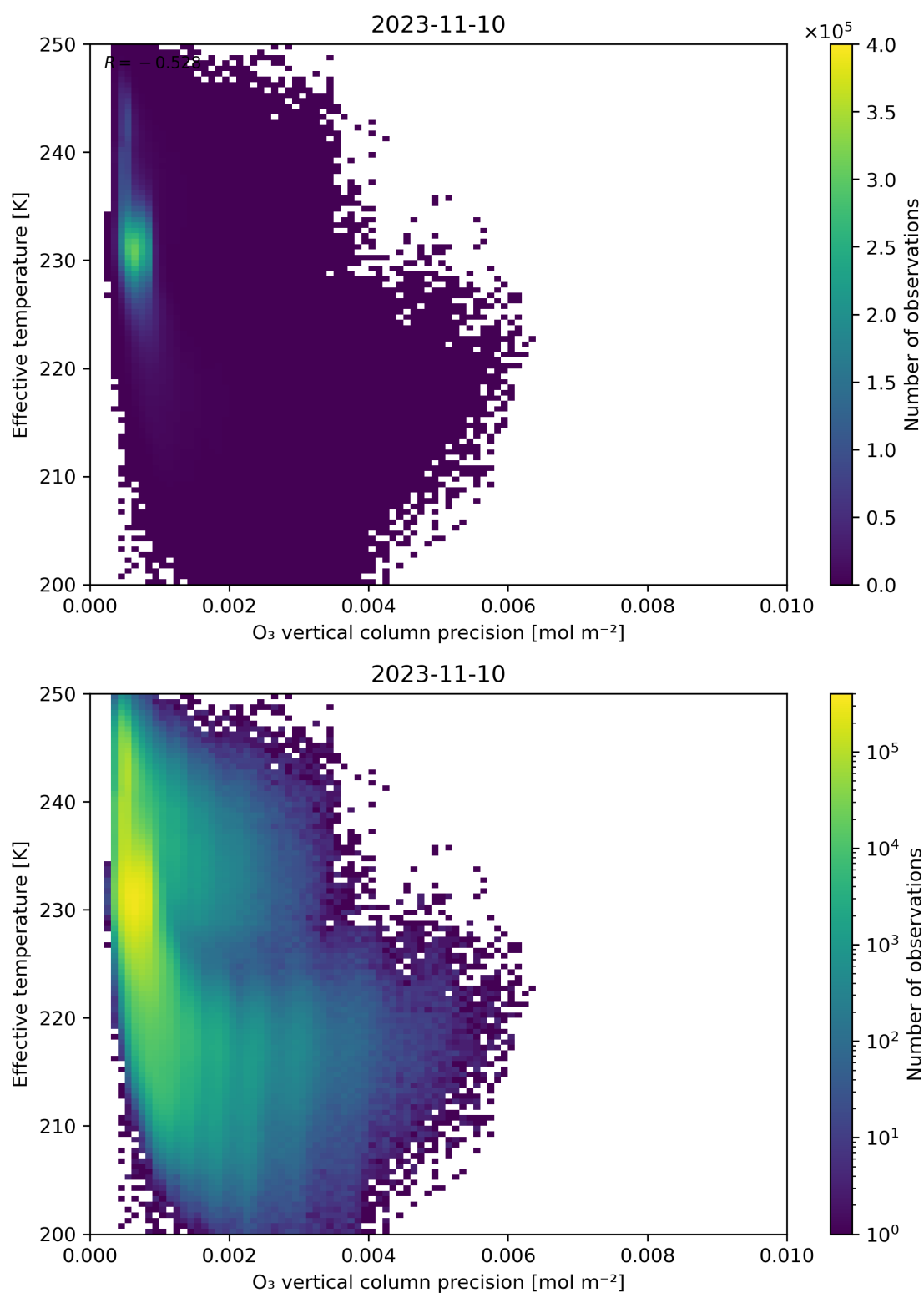
Figure 42: Scatter density plot of “O 3 vertical column precision” against “Effective temperature” for 2023-11-09 to 2023-11-11.
