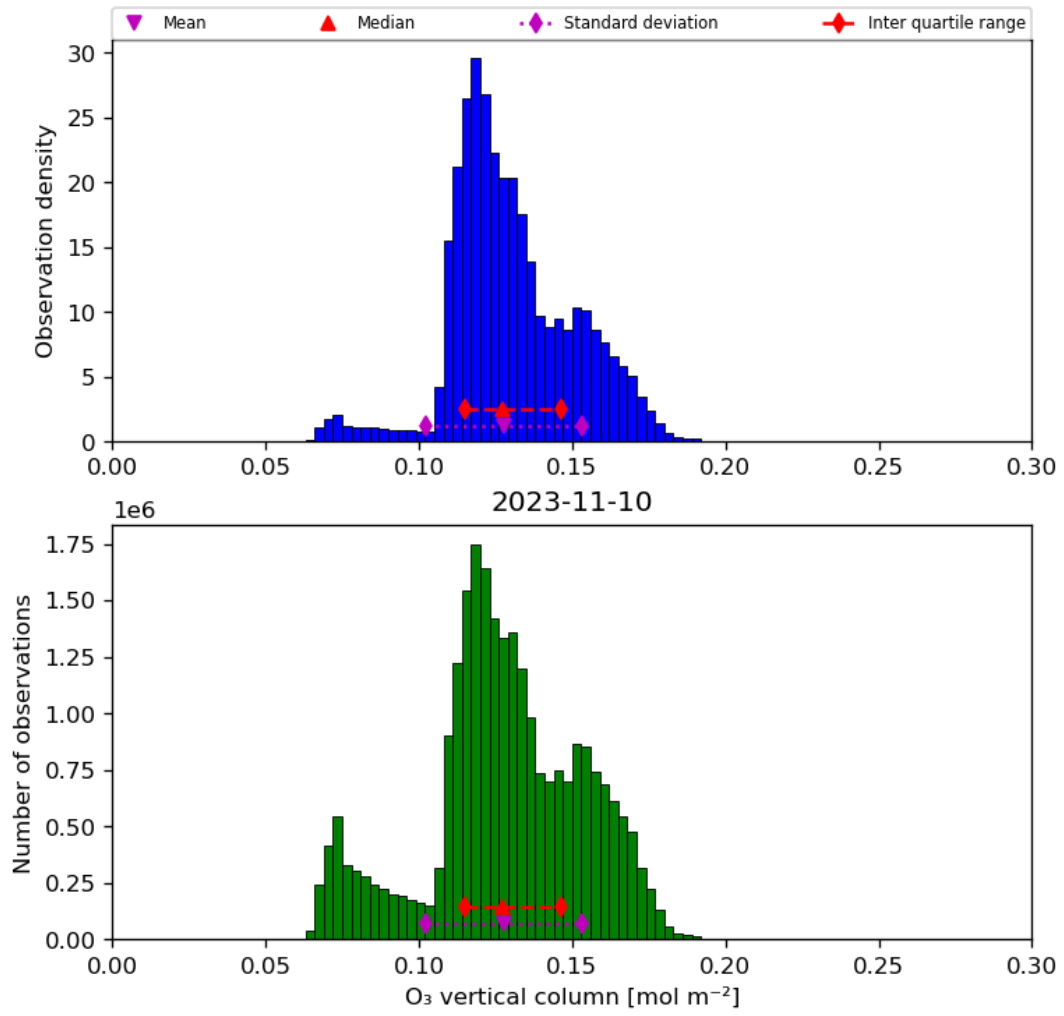
Figure 21: Histogram of “O 3 vertical column” for 2023-11-09 to 2023-11-11
