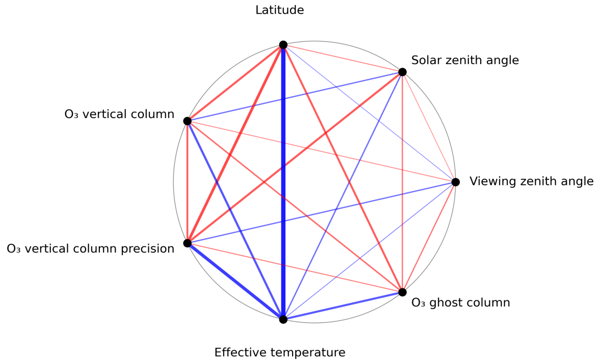
Figure 1: Map of correlation graph for 2023-11-09 to 2023-11-11.
