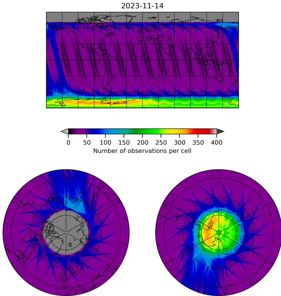
Figure 12: Map of the number of observations for 2023-11-13 to 2023-11-15
