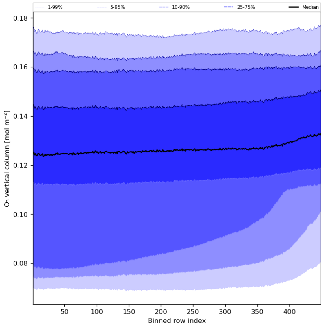
Figure 28: Along track statistics of “O 3 vertical column” for 2023-11-13 to 2023-11-15
