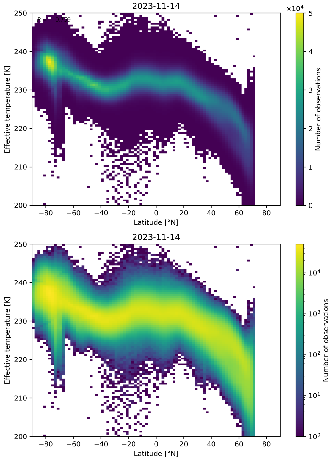
Figure 34: Scatter density plot of “Latitude” against “Effective temperature” for 2023-11-13 to 2023-11-15.
