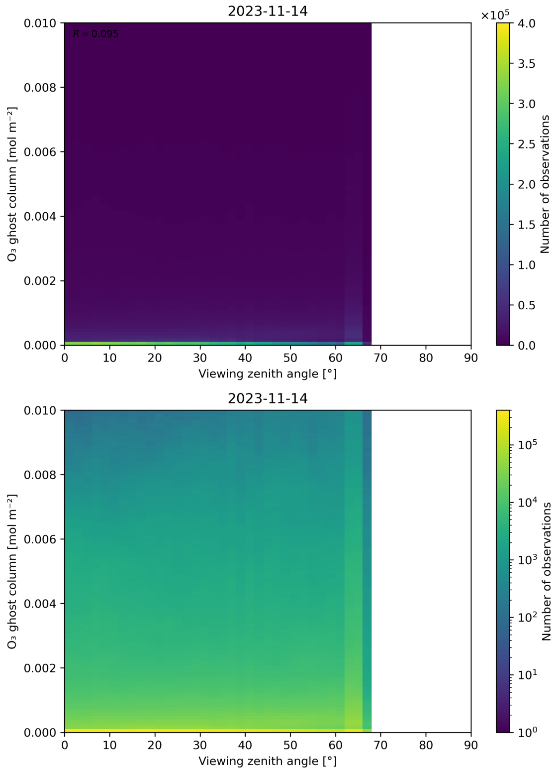
Figure 51: Scatter density plot of “Viewing zenith angle” against “O 3 ghost column” for 2023-11-13 to 2023-11-15.
