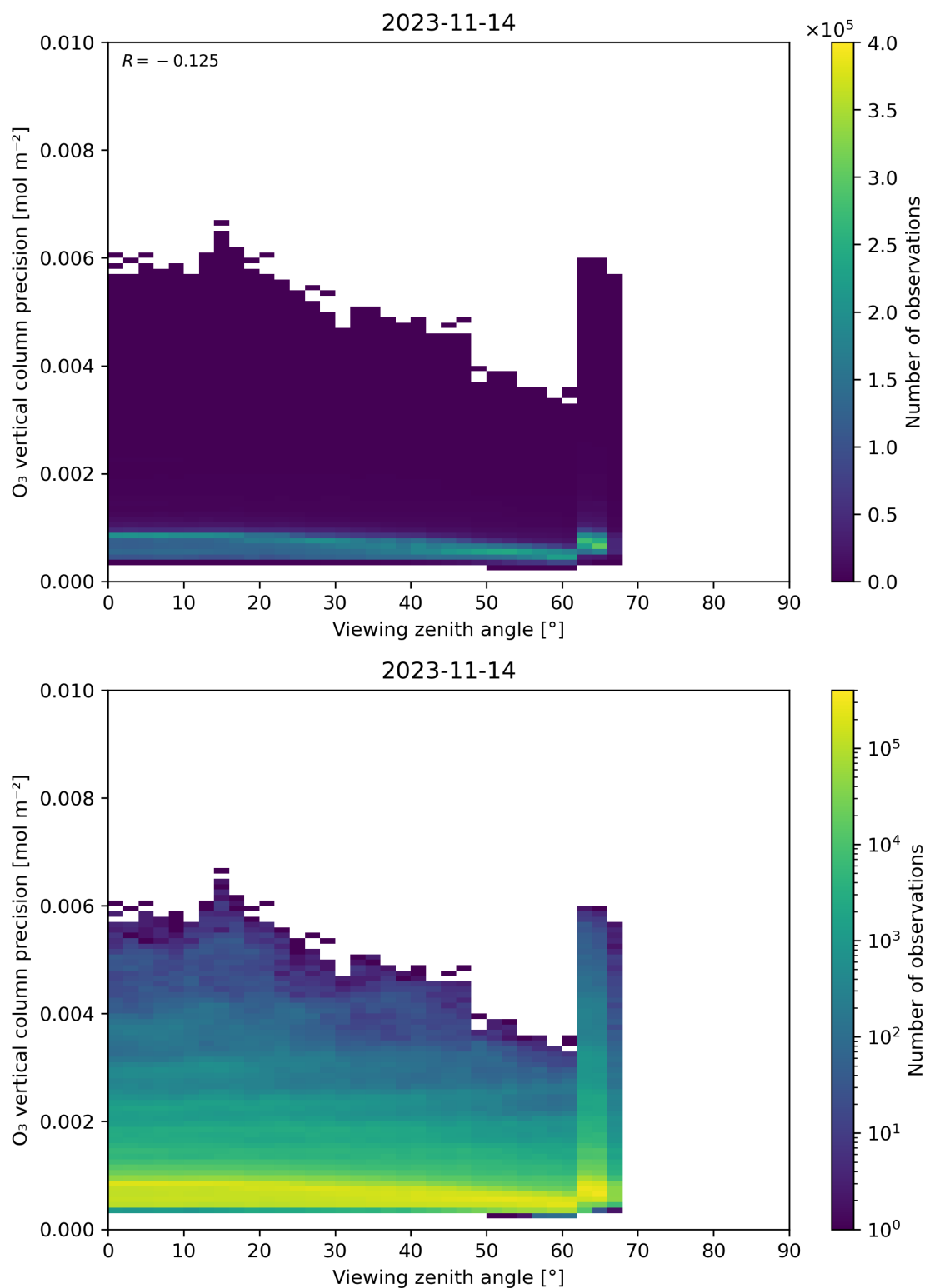
Figure 53: Scatter density plot of “Viewing zenith angle” against “O 3 vertical column precision” for 2023-11-13 to 2023-11-15.
