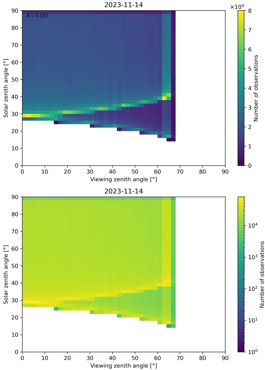
Figure 54: Scatter density plot of “Viewing zenith angle” against “Solar zenith angle” for 2023-11-13 to 2023-11-15.
