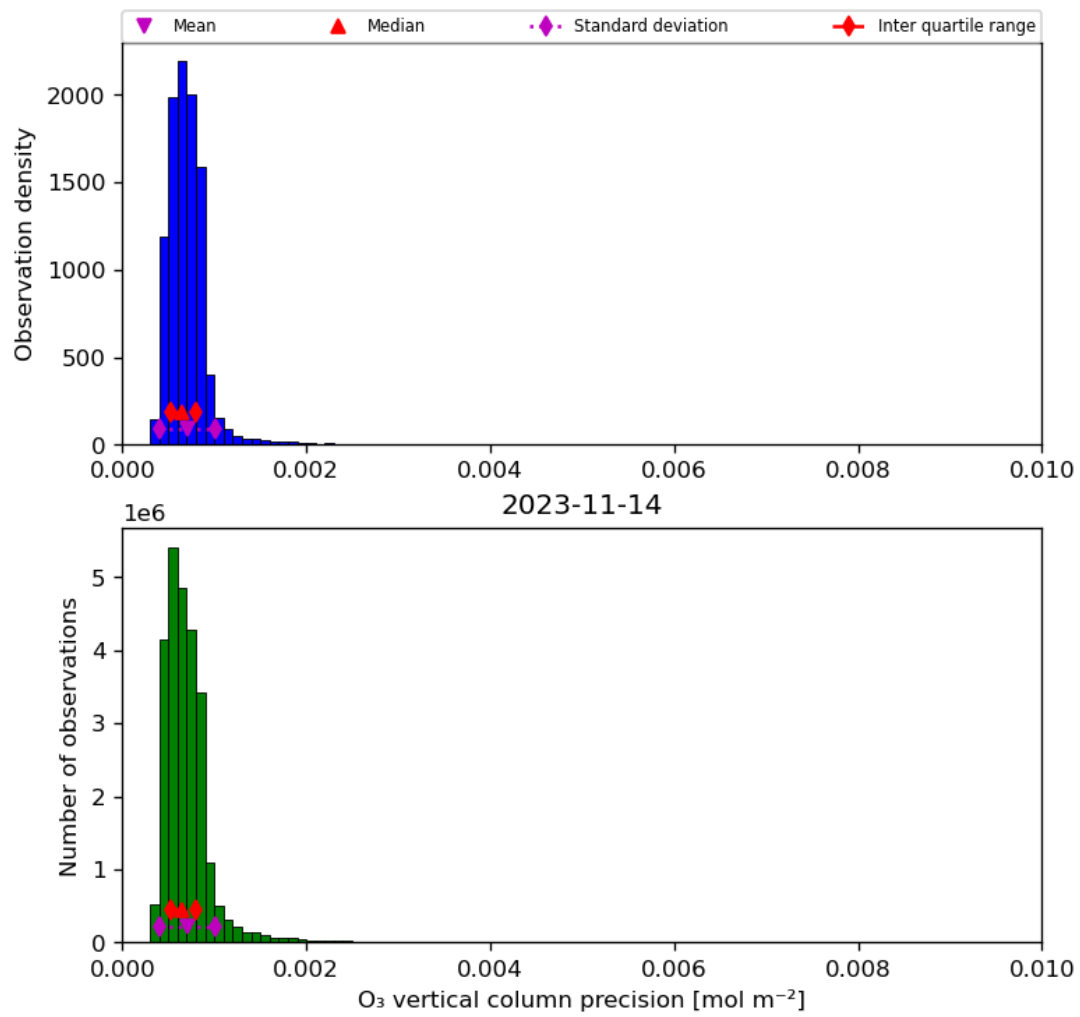
Figure 22: Histogram of “O 3 vertical column precision” for 2023-11-13 to 2023-11-15
