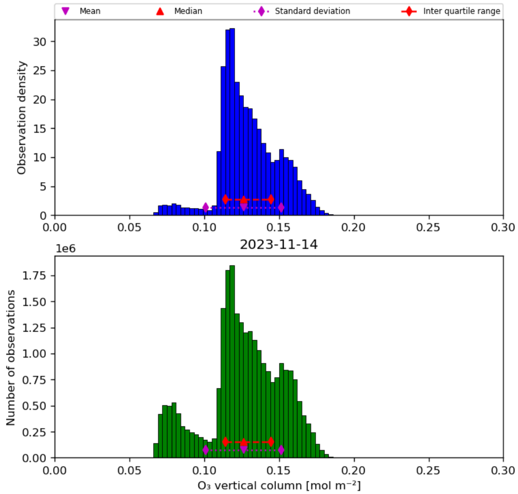
Figure 21: Histogram of “O 3 vertical column” for 2023-11-13 to 2023-11-15
