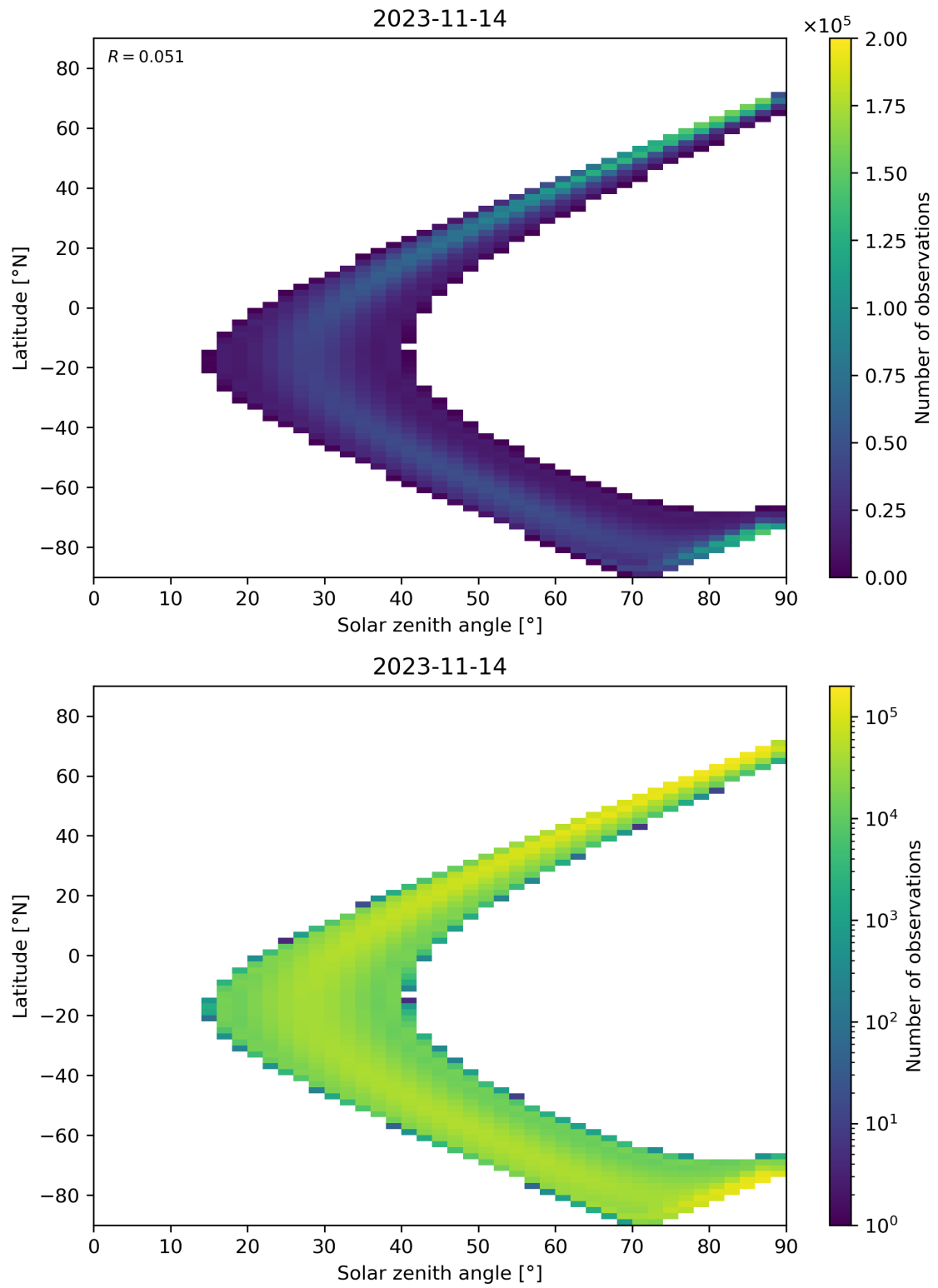
Figure 44: Scatter density plot of “Solar zenith angle” against “Latitude” for 2023-11-13 to 2023-11-15.
