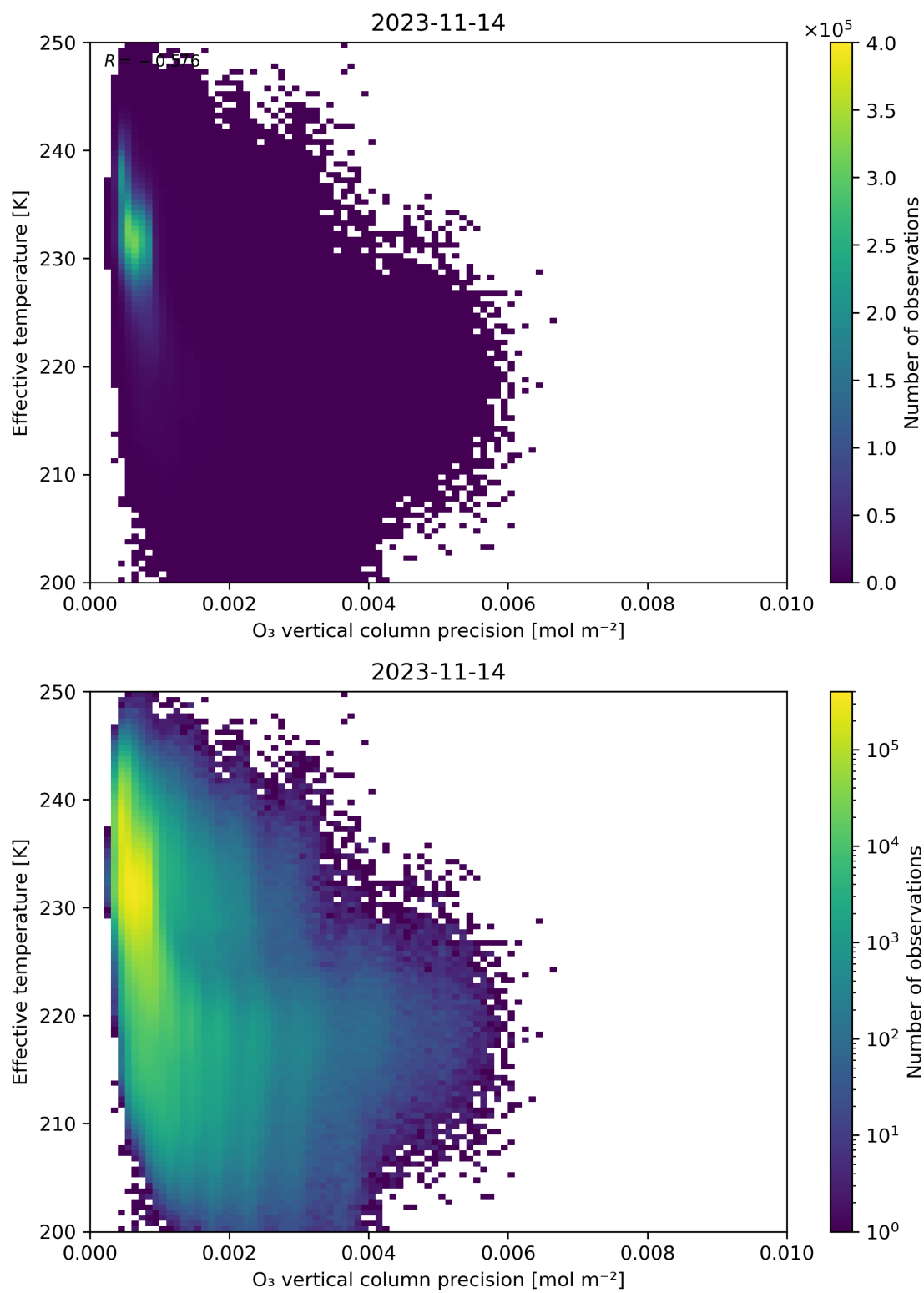
Figure 42: Scatter density plot of “O 3 vertical column precision” against “Effective temperature” for 2023-11-13 to 2023-11-15.
