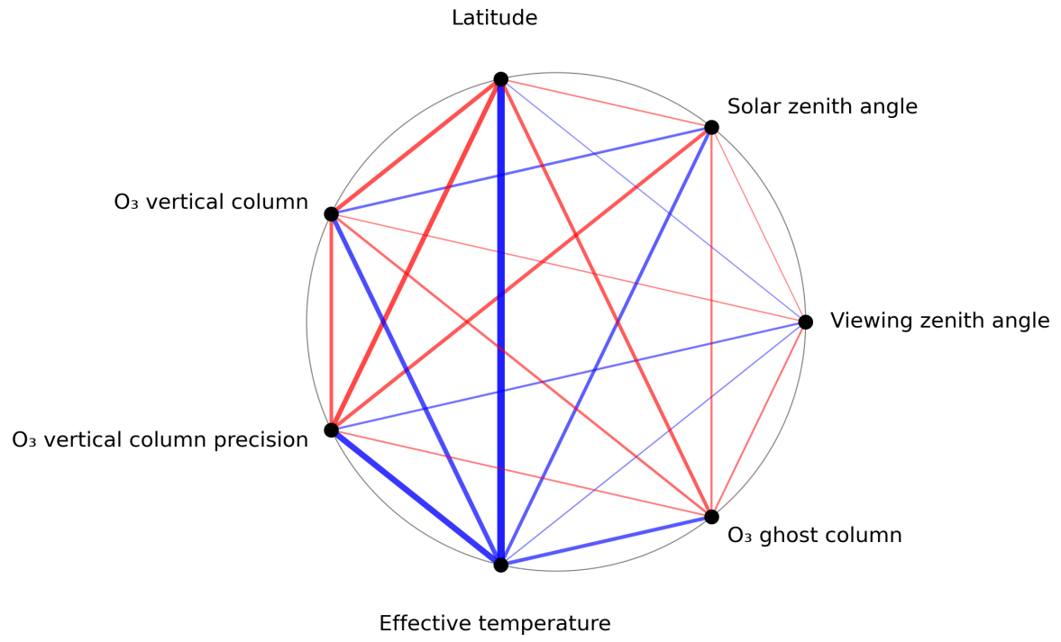
Figure 1: Map of correlation graph for 2023-11-13 to 2023-11-15.
