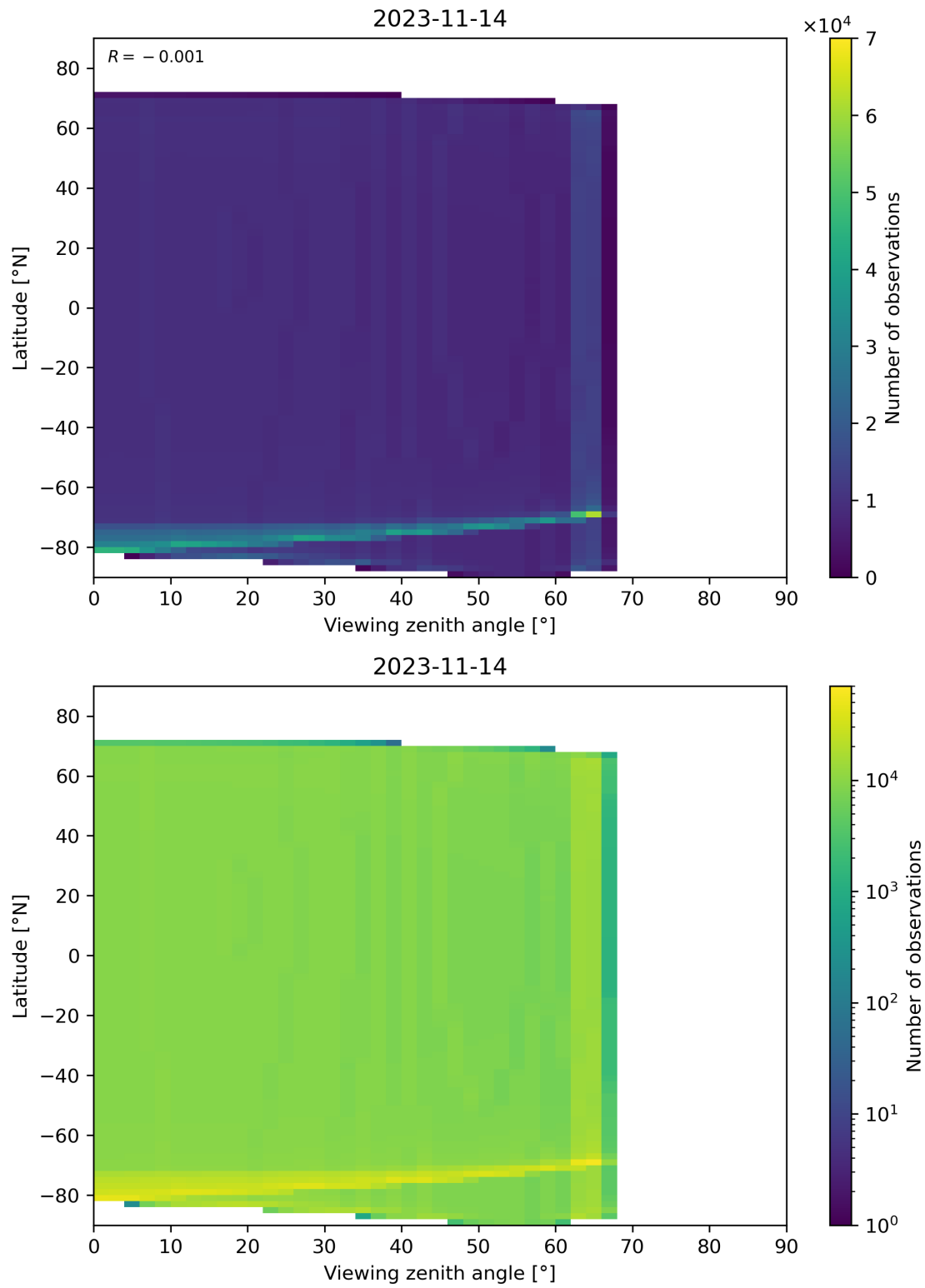
Figure 49: Scatter density plot of “Viewing zenith angle” against “Latitude” for 2023-11-13 to 2023-11-15.
