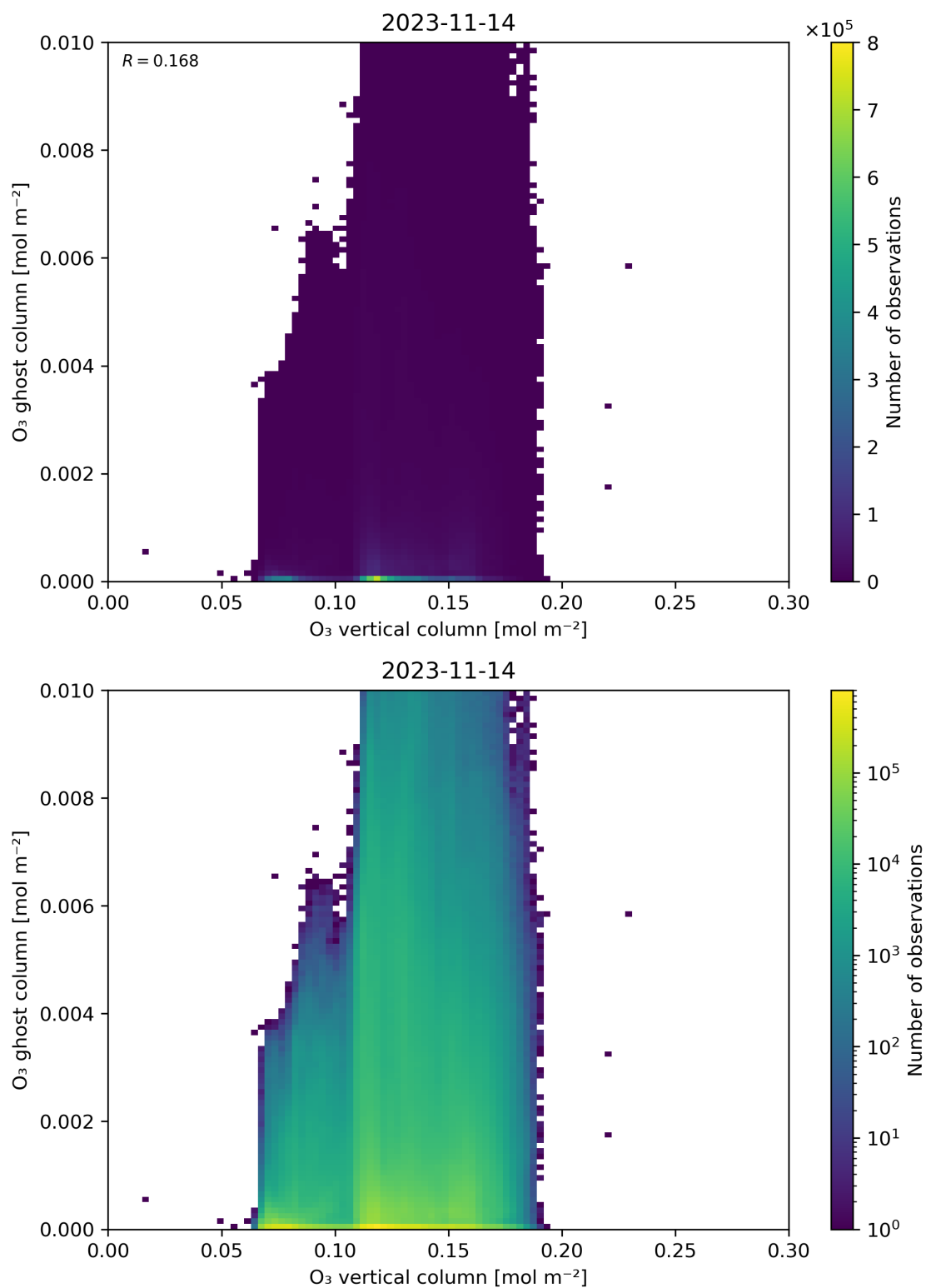
Figure 40: Scatter density plot of “O 3 vertical column” against “O 3 ghost column” for 2023-11-13 to 2023-11-15.
