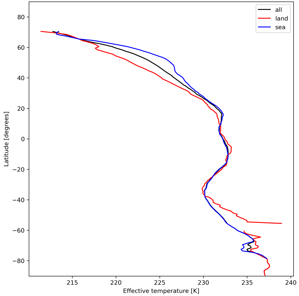
Figure 17: Zonal average of "Effective temperature" for 2023-11-13 to 2023-11-15.
