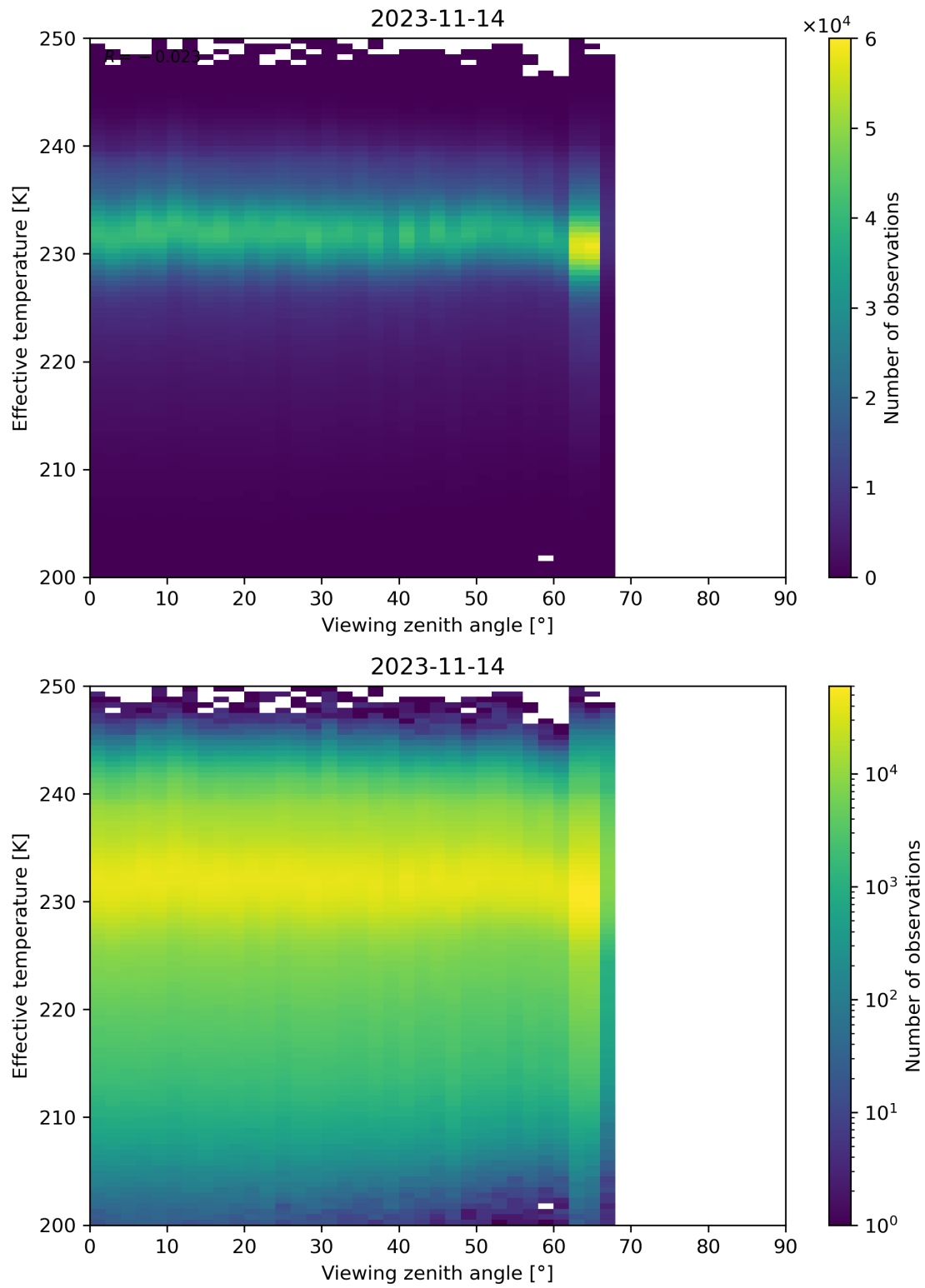
Figure 50: Scatter density plot of “Viewing zenith angle” against “Effective temperature” for 2023-11-13 to 2023-11-15.
