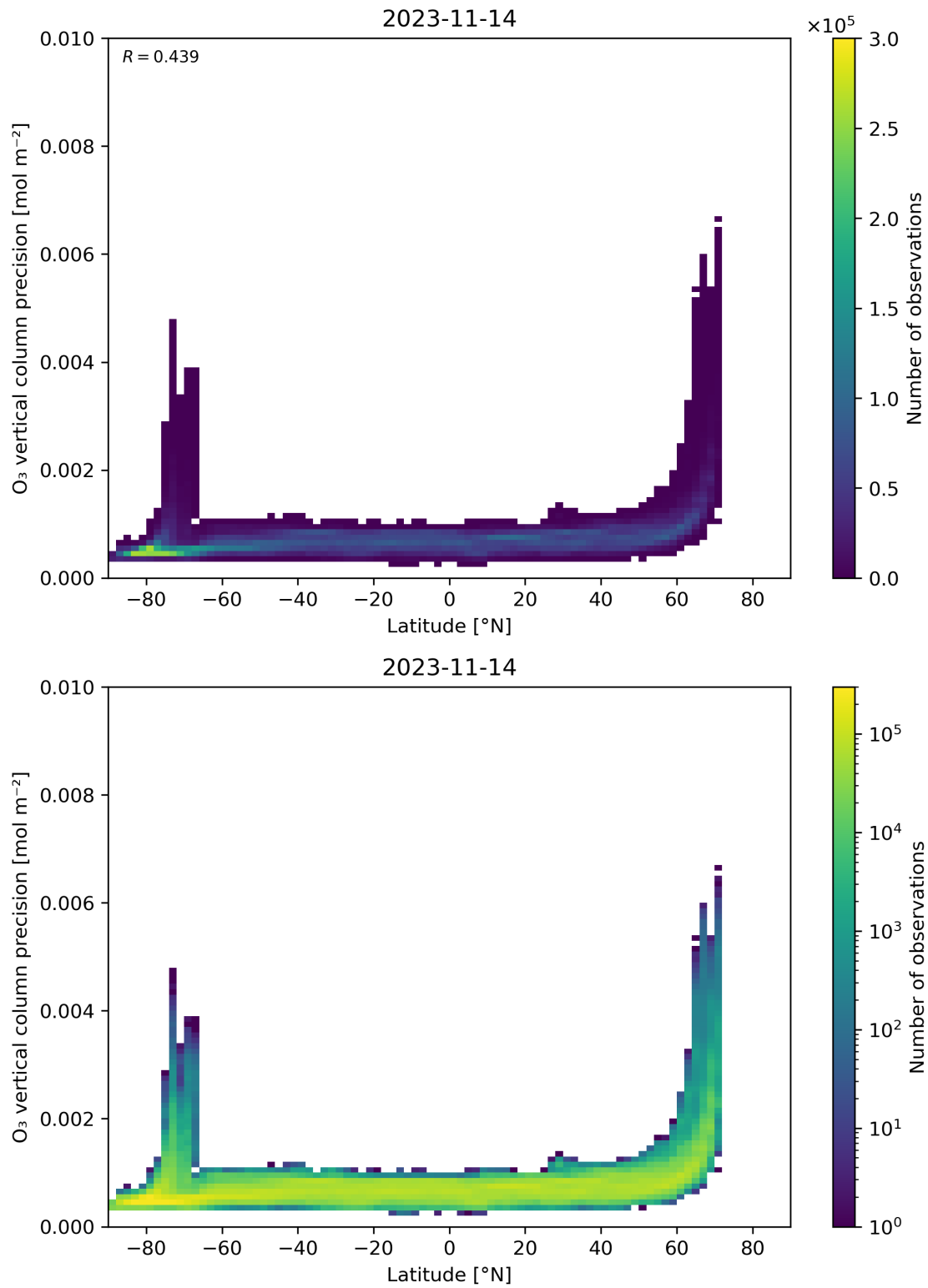
Figure 37: Scatter density plot of “Latitude” against “O 3 vertical column precision” for 2023-11-13 to 2023-11-15.
