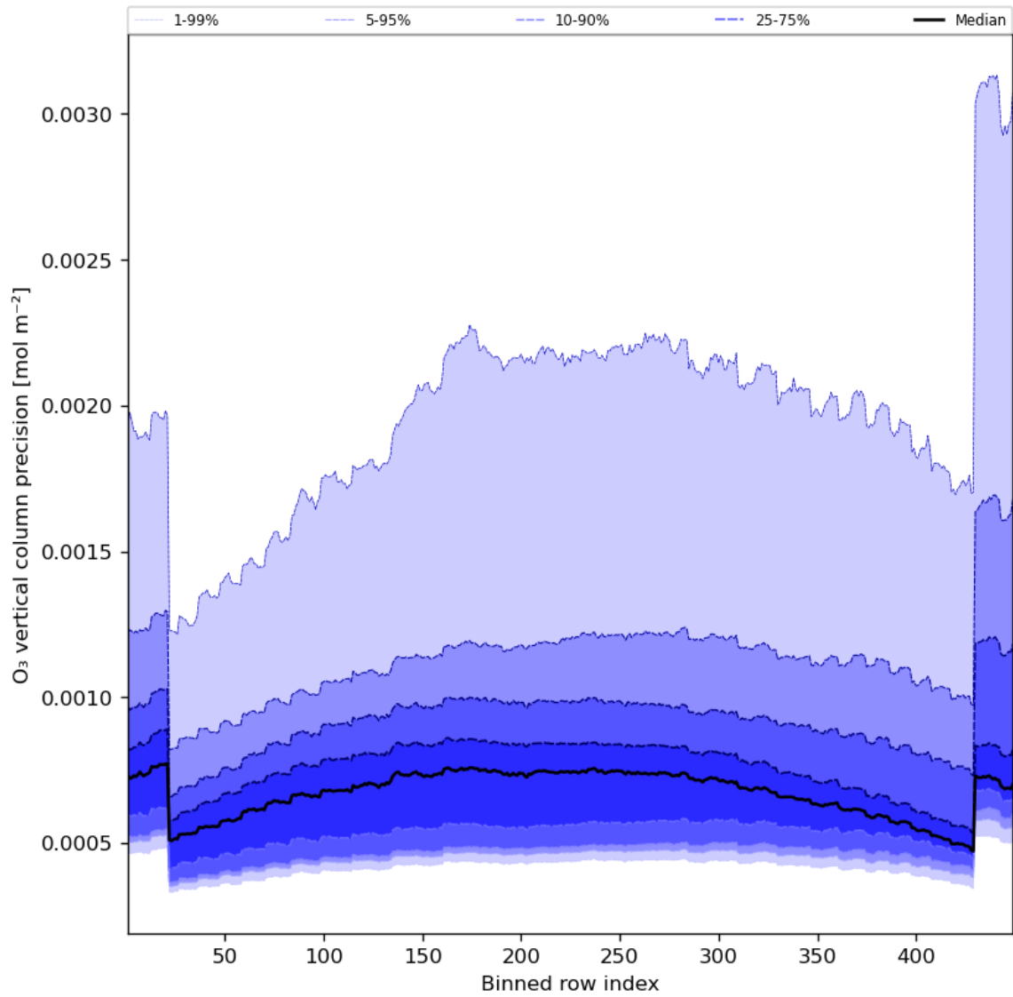
Figure 29: Along track statistics of “O 3 vertical column precision” for 2023-11-13 to 2023-11-15
