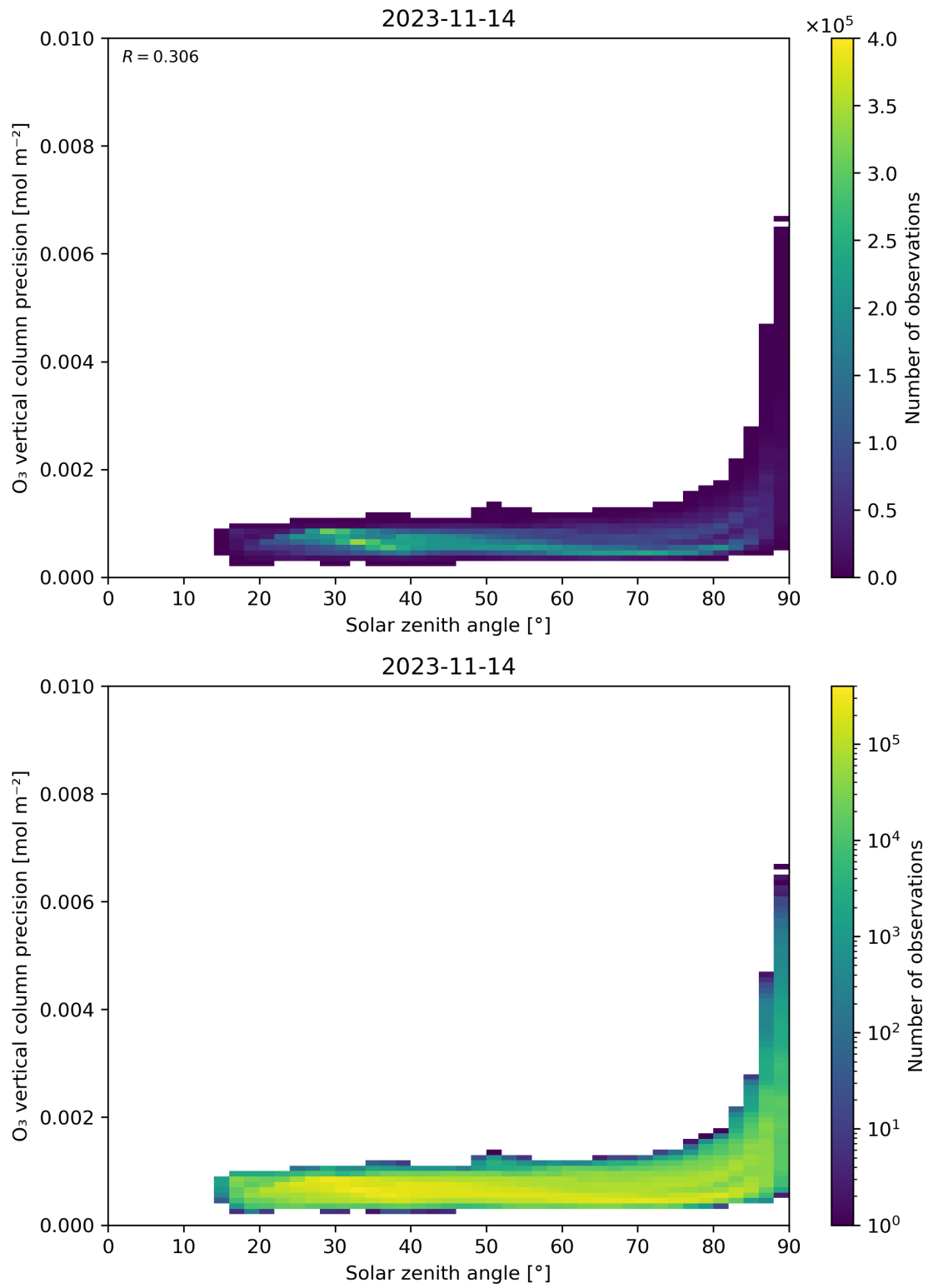
Figure 48: Scatter density plot of “Solar zenith angle” against “O 3 vertical column precision” for 2023-11-13 to 2023-11-15.
