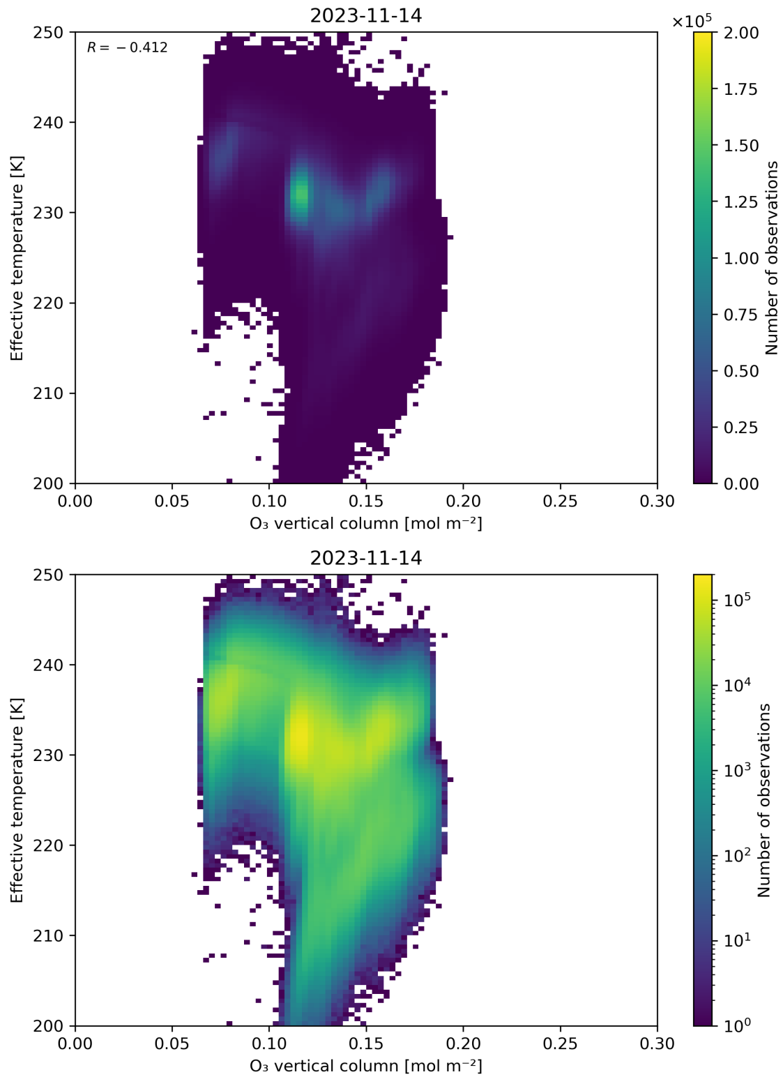
Figure 39: Scatter density plot of “O 3 vertical column” against “Effective temperature” for 2023-11-13 to 2023-11-15.
