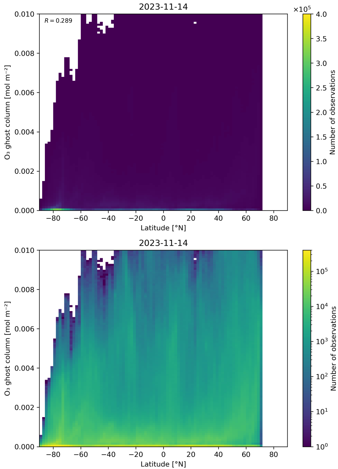
Figure 35: Scatter density plot of “Latitude” against “O 3 ghost column” for 2023-11-13 to 2023-11-15.
