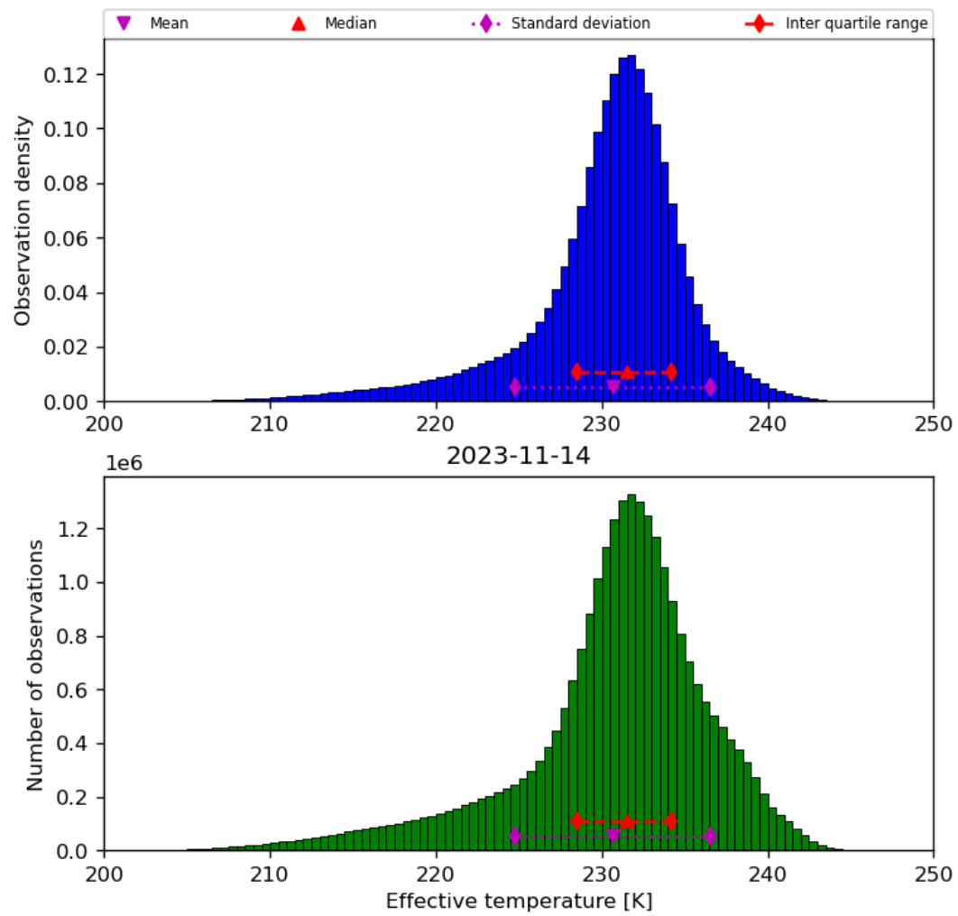
Figure 24: Histogram of “Effective temperature” for 2023-11-13 to 2023-11-15
