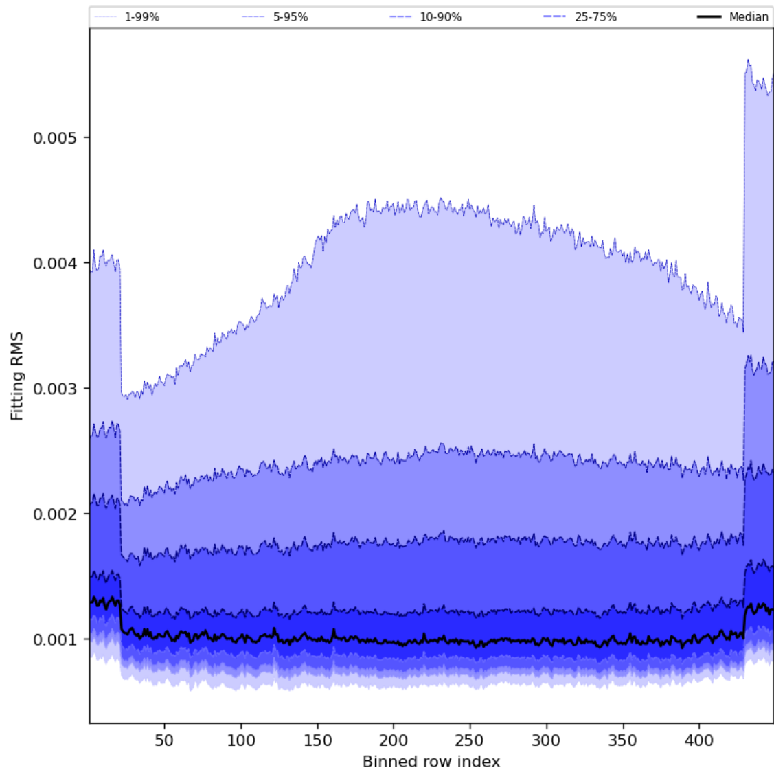
Figure 30: Along track statistics of “Fitting RMS” for 2023-11-13 to 2023-11-15
