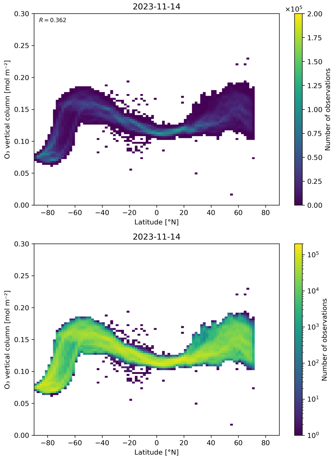
Figure 36: Scatter density plot of “Latitude” against “O 3 vertical column” for 2023-11-13 to 2023-11-15.
