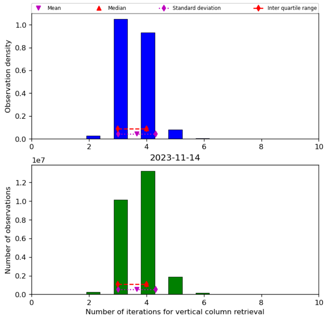
Figure 26: Histogram of “Number of iterations for vertical column retrieval” for 2023-11-13 to 2023-11-15
