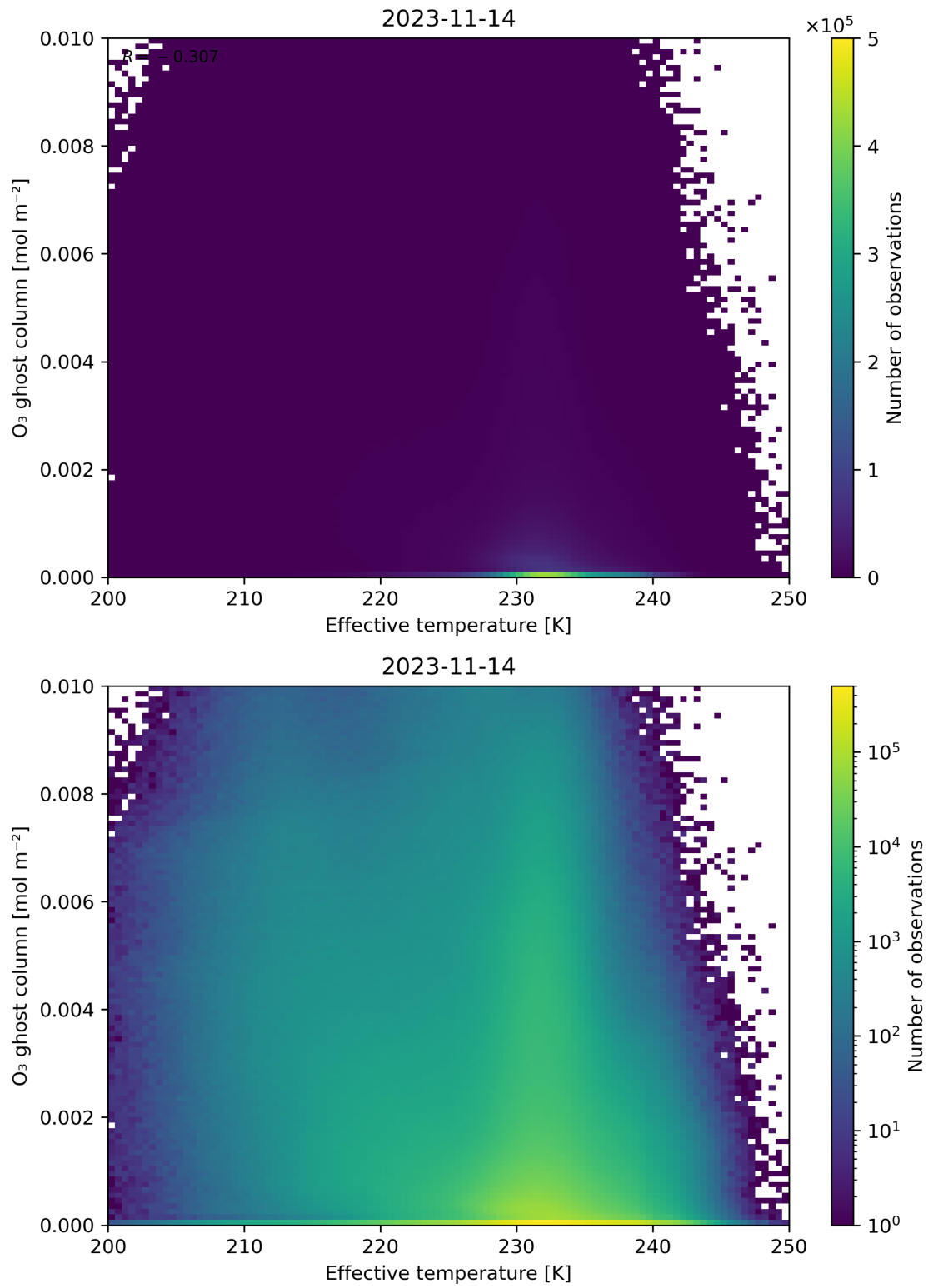
Figure 38: Scatter density plot of “Effective temperature” against “O 3 ghost column” for 2023-11-13 to 2023-11-15.
