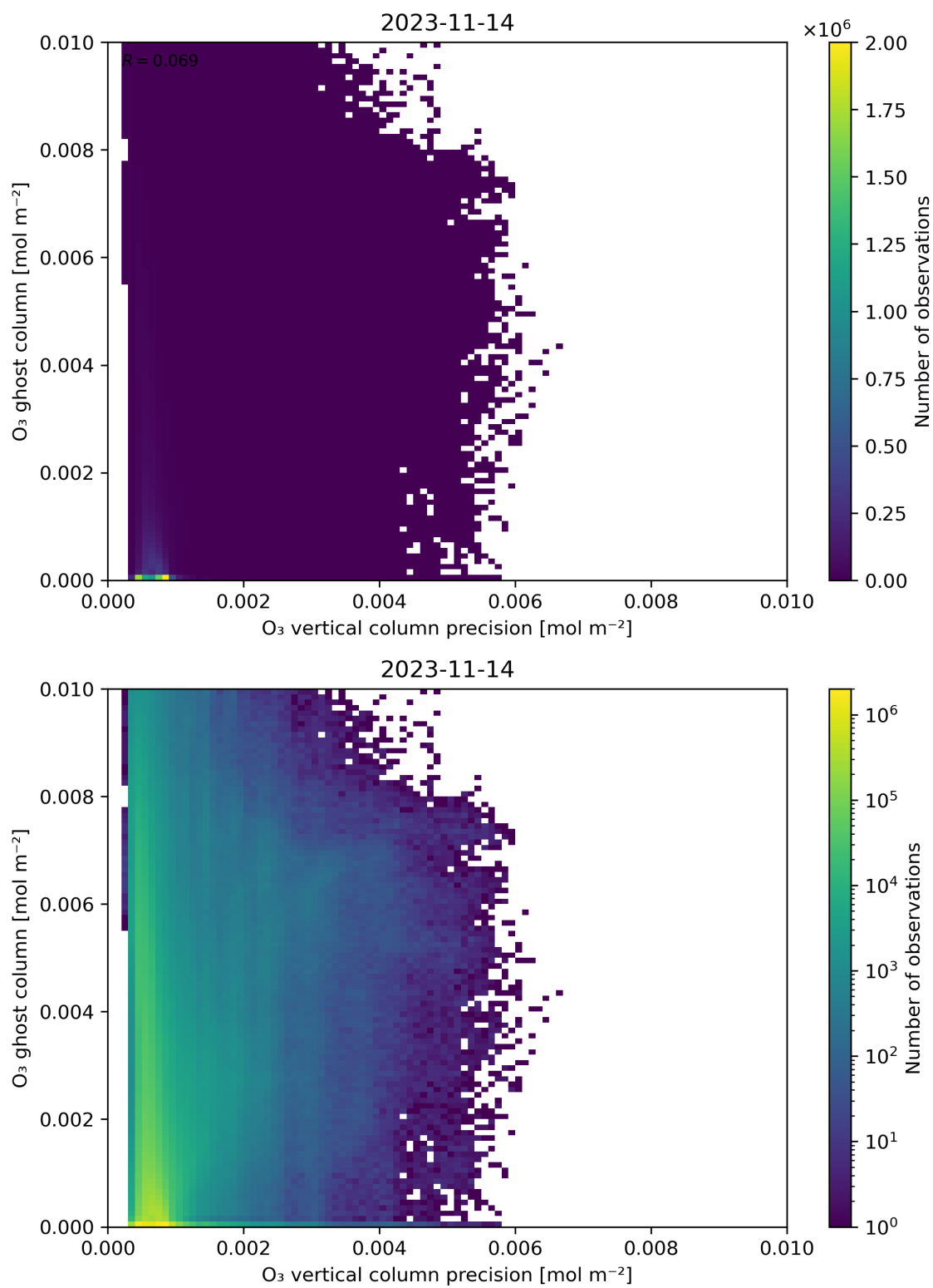
Figure 43: Scatter density plot of “ \text{O}_3 vertical column precision” against “ \text{O}_3 ghost column” for 2023-11-13 to 2023-11-15.
