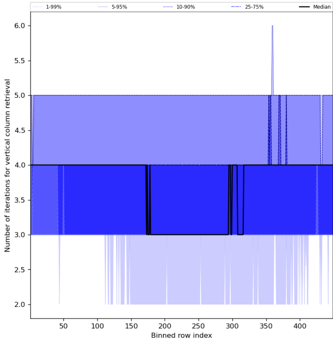
Figure 33: Along track statistics of “Number of iterations for vertical column retrieval” for 2023-11-13 to 2023-11-15
