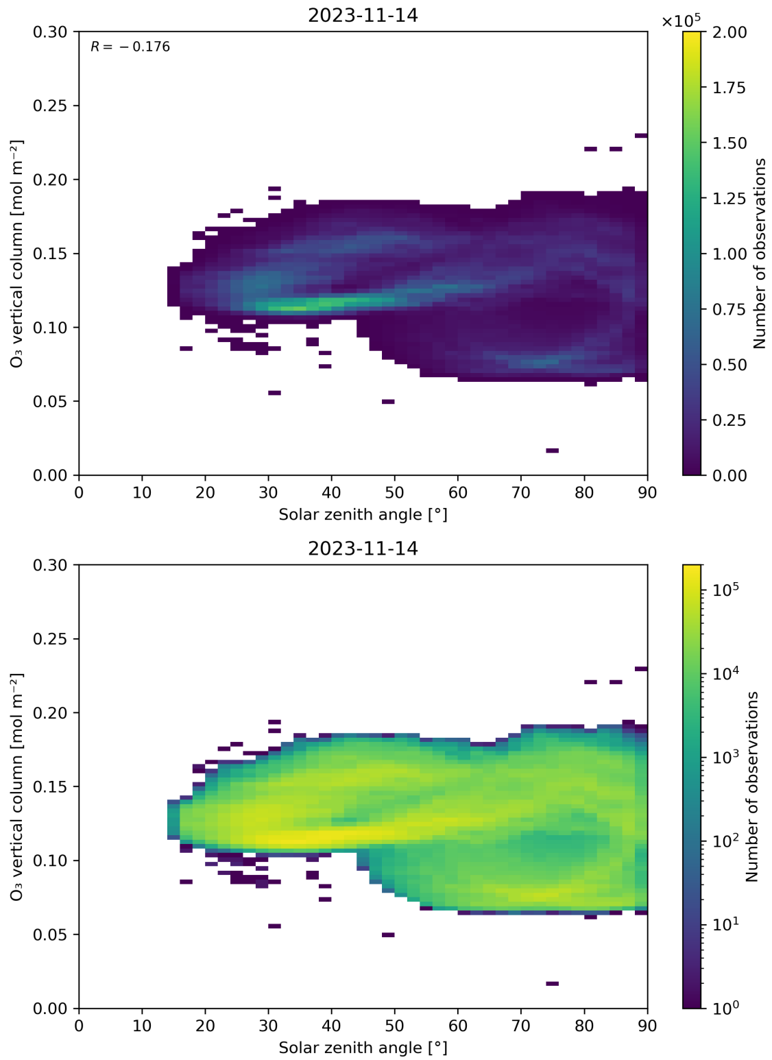
Figure 47: Scatter density plot of “Solar zenith angle” against “O 3 vertical column” for 2023-11-13 to 2023-11-15.
