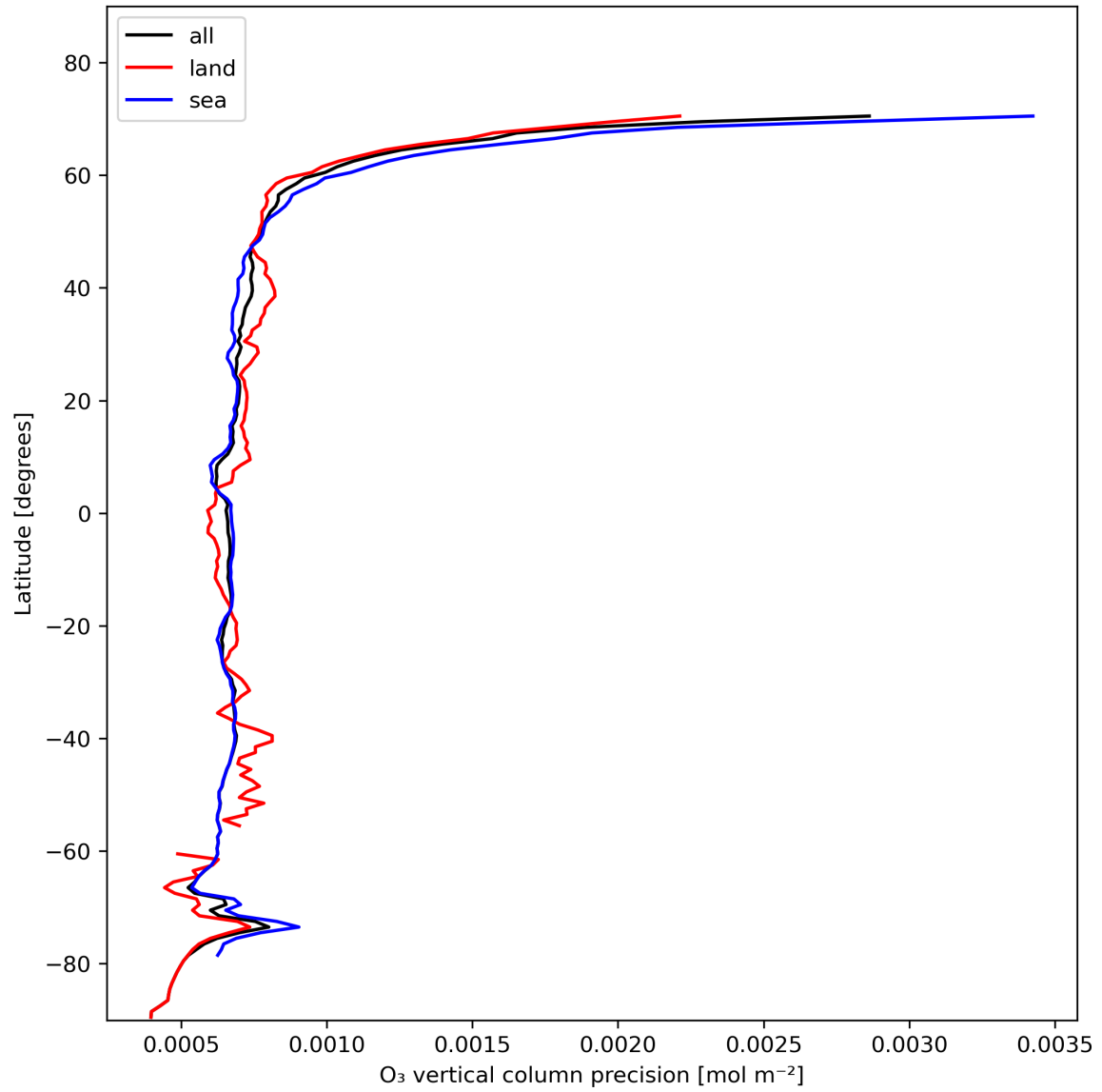
Figure 15: Zonal average of “O 3 vertical column precision” for 2023-11-13 to 2023-11-15.
