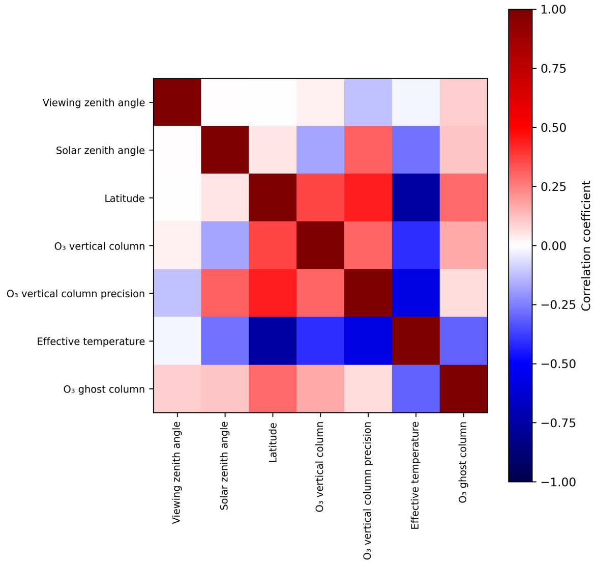
Figure 2: Map of correlation matrix for 2023-11-13 to 2023-11-15.
