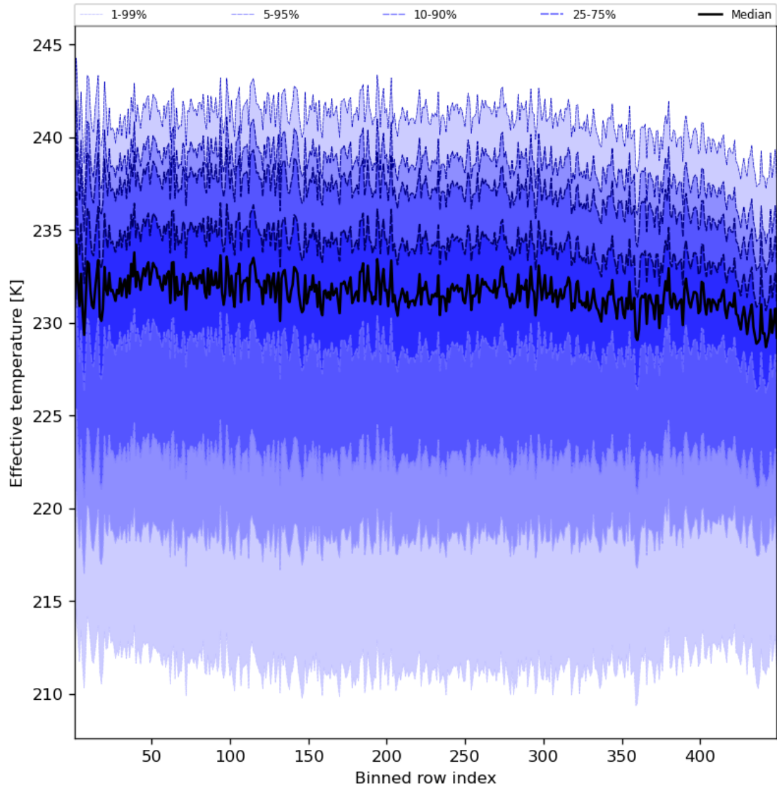
Figure 31: Along track statistics of “Effective temperature” for 2023-11-13 to 2023-11-15
