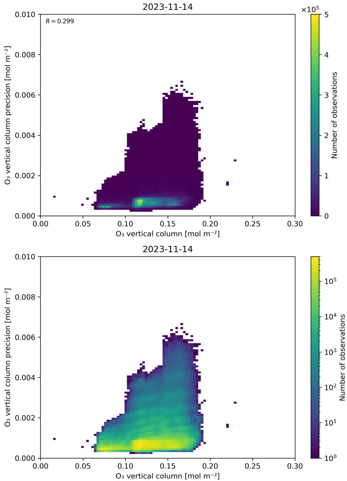
Figure 41: Scatter density plot of “O 3 vertical column” against “O 3 vertical column precision” for 2023-11-13 to 2023-11-15.
