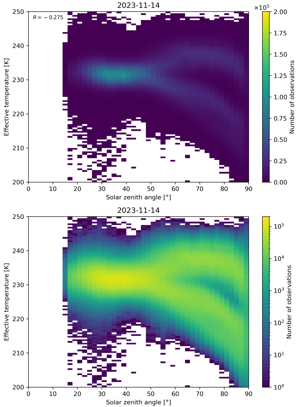
Figure 45: Scatter density plot of “Solar zenith angle” against “Effective temperature” for 2023-11-13 to 2023-11-15.
