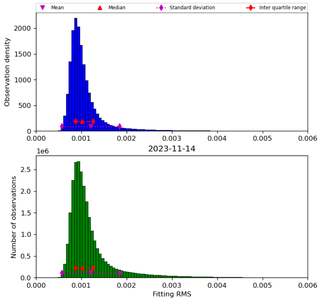
Figure 23: Histogram of “Fitting RMS” for 2023-11-13 to 2023-11-15
