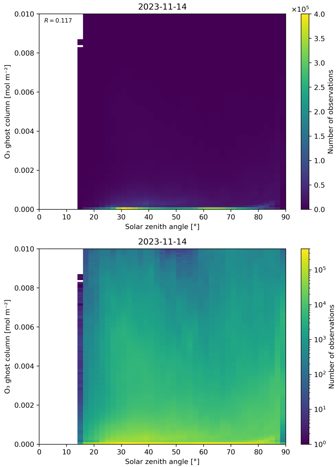
Figure 46: Scatter density plot of “Solar zenith angle” against “O 3 ghost column” for 2023-11-13 to 2023-11-15.
