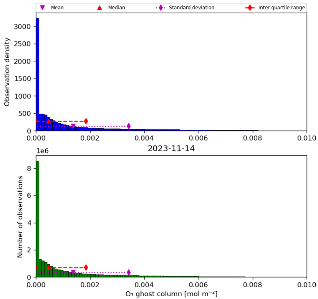
Figure 25: Histogram of “O 3 ghost column” for 2023-11-13 to 2023-11-15
