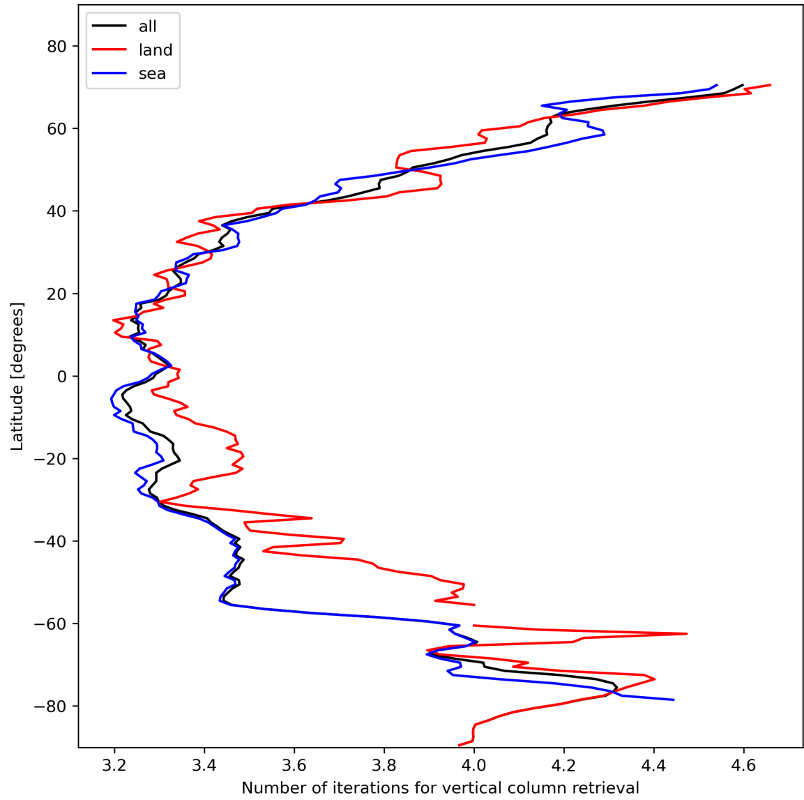
Figure 19: Zonal average of “Number of iterations for vertical column retrieval” for 2023-11-13 to 2023-11-15.
