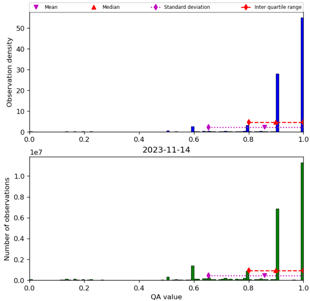
Figure 20: Histogram of “QA value” for 2023-11-13 to 2023-11-15
