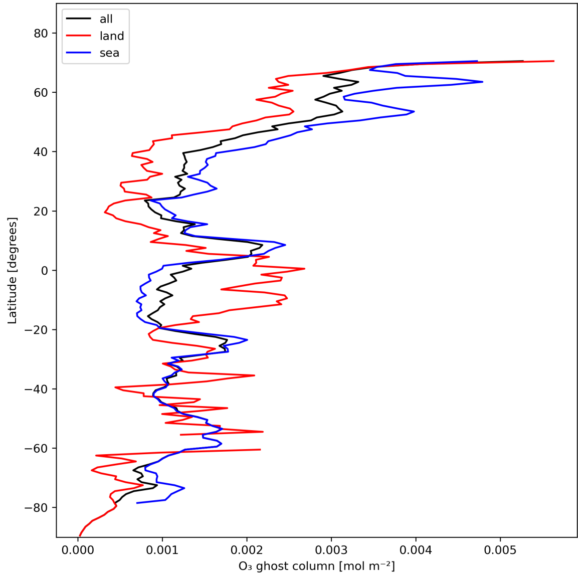
Figure 18: Zonal average of “O 3 ghost column” for 2023-11-13 to 2023-11-15.
