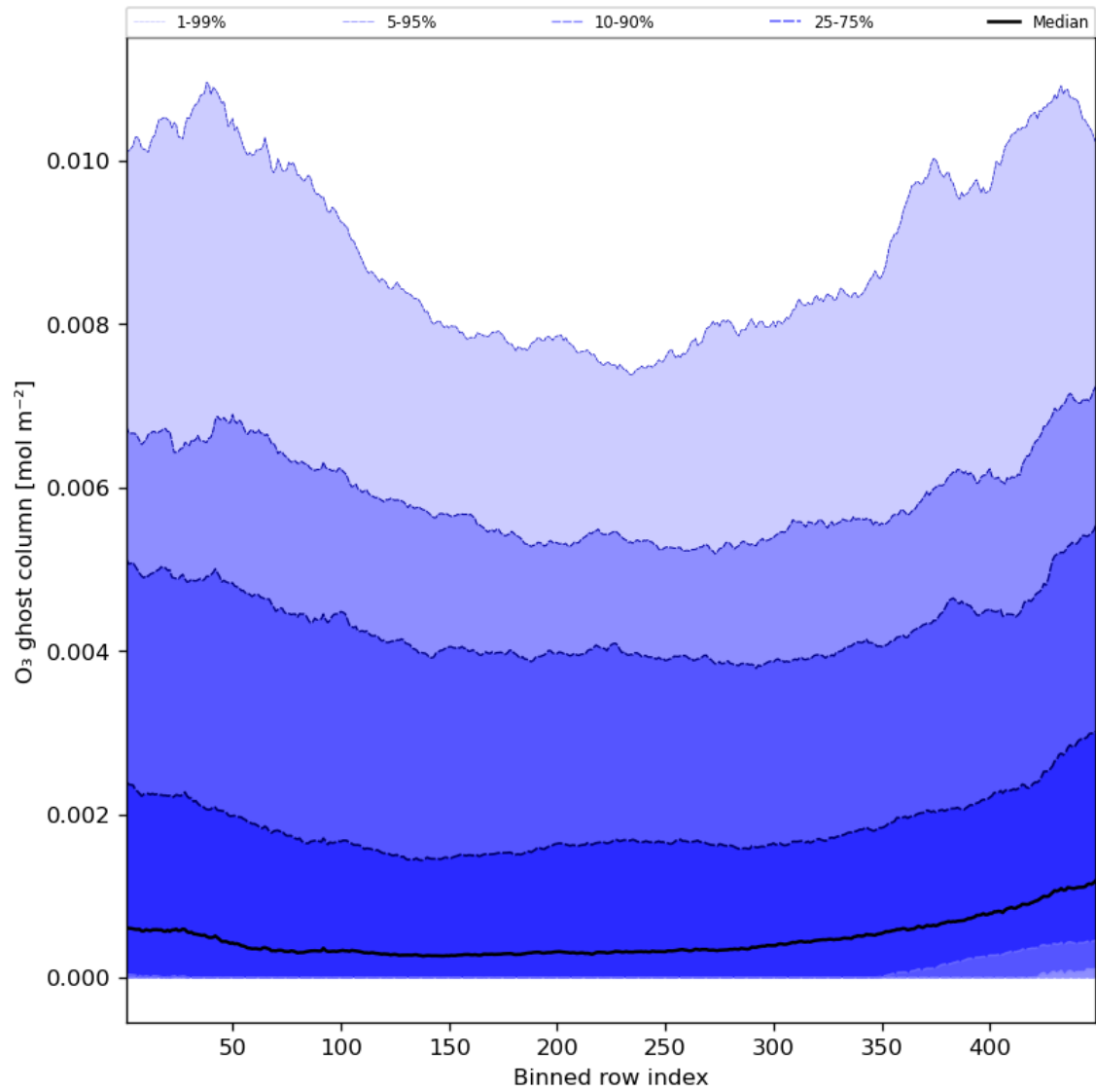
Figure 32: Along track statistics of “O 3 ghost column” for 2023-11-13 to 2023-11-15
