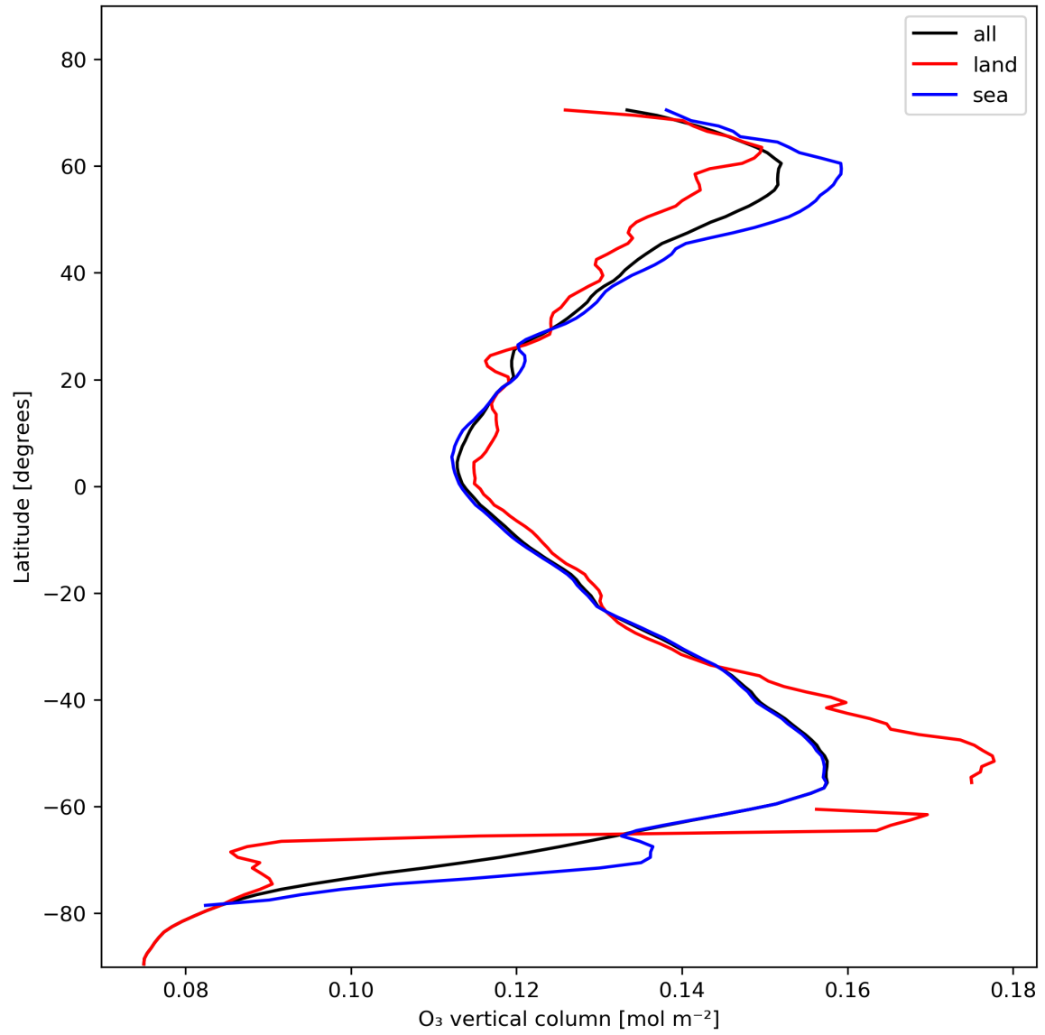
Figure 14: Zonal average of “O 3 vertical column” for 2023-11-13 to 2023-11-15.
