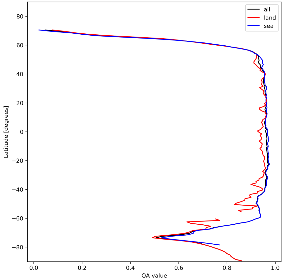
Figure 13: Zonal average of “QA value” for 2023-11-13 to 2023-11-15.
