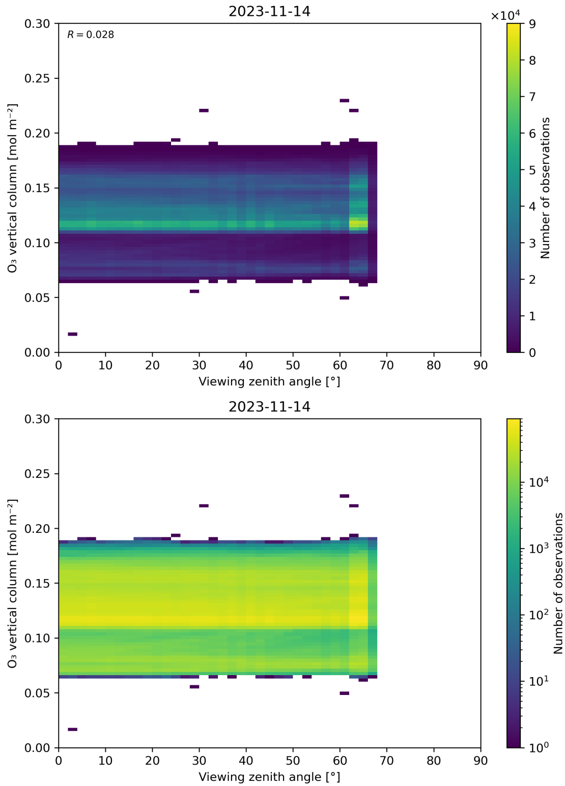
Figure 52: Scatter density plot of “Viewing zenith angle” against “O 3 vertical column” for 2023-11-13 to 2023-11-15.
