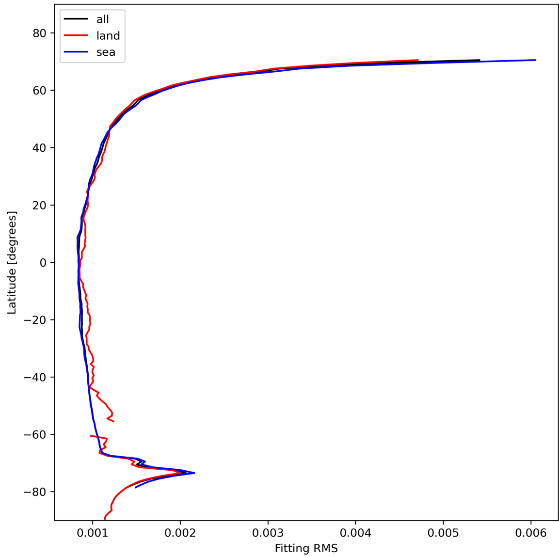
Figure 16: Zonal average of “Fitting RMS” for 2023-11-13 to 2023-11-15.
