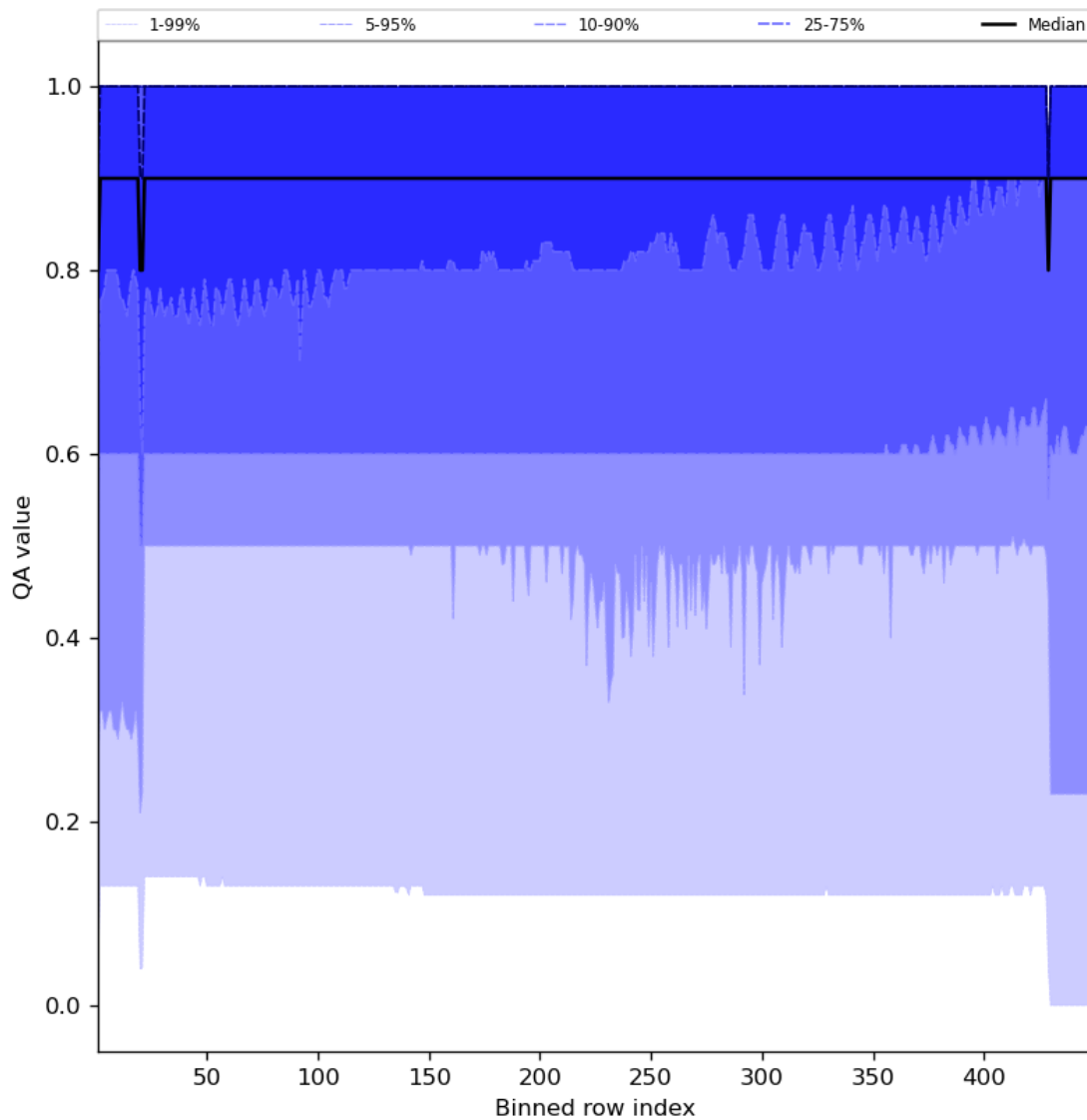
Figure 27: Along track statistics of “QA value” for 2023-11-13 to 2023-11-15
