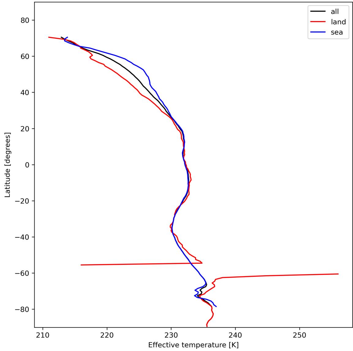
Figure 17: Zonal average of "Effective temperature" for 2023-11-14 to 2023-11-16.
