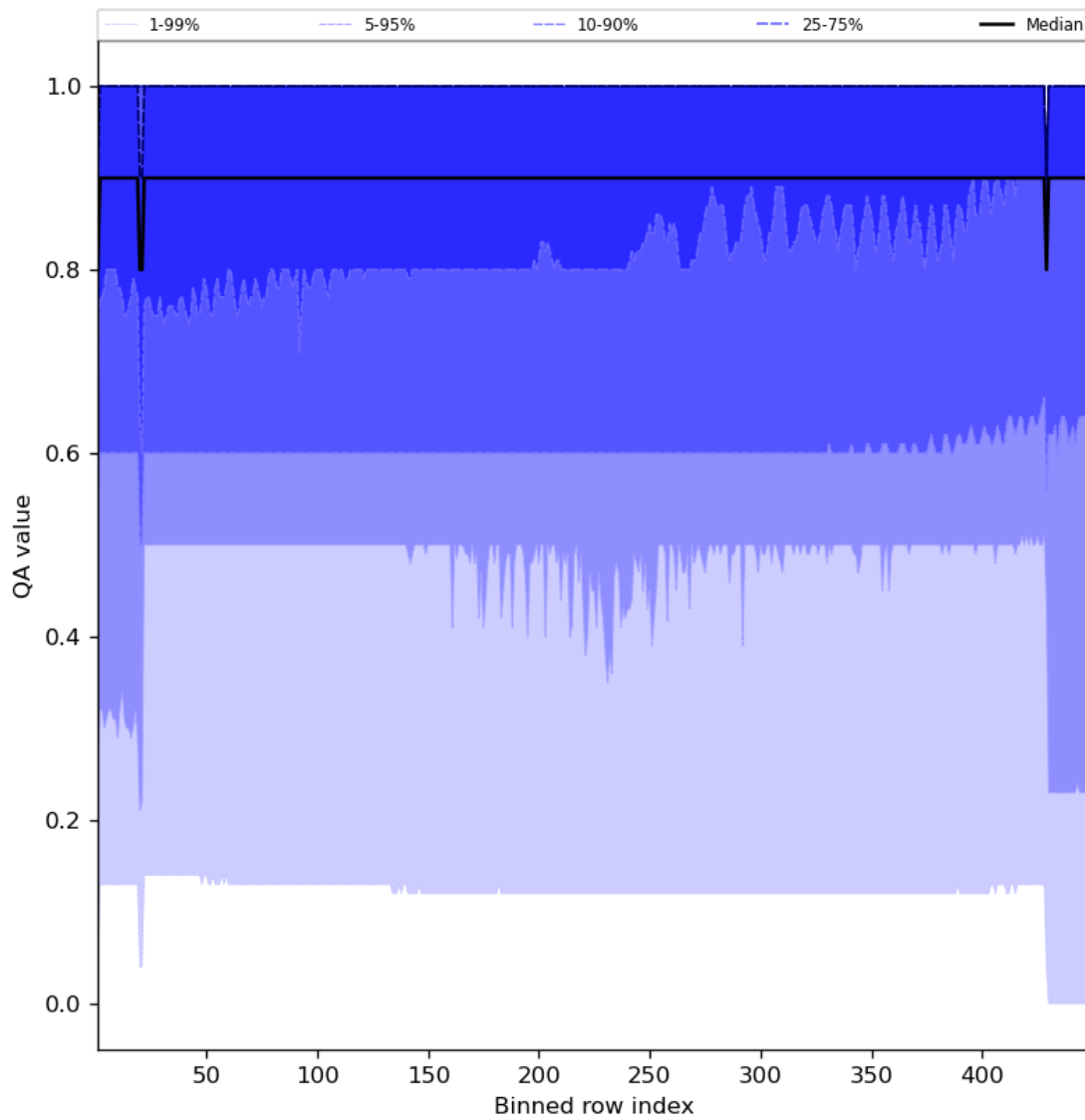
Figure 27: Along track statistics of “QA value” for 2023-11-14 to 2023-11-16
