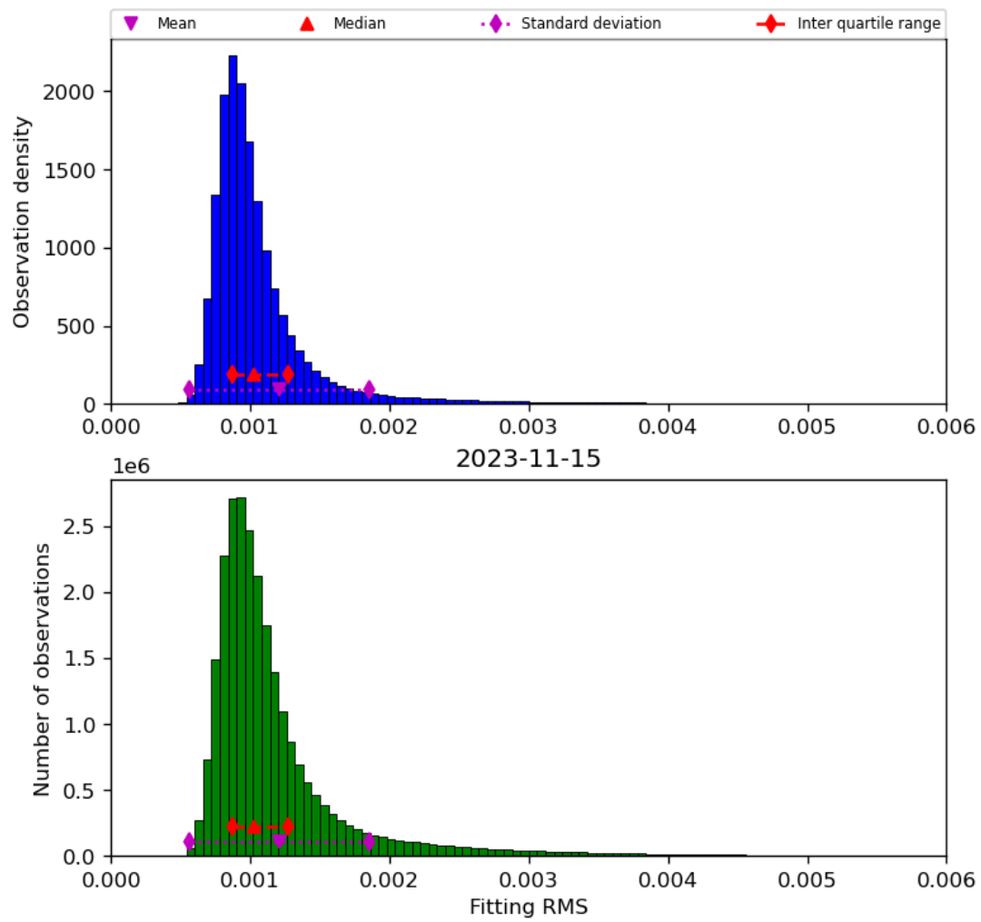
Figure 23: Histogram of “Fitting RMS” for 2023-11-14 to 2023-11-16
