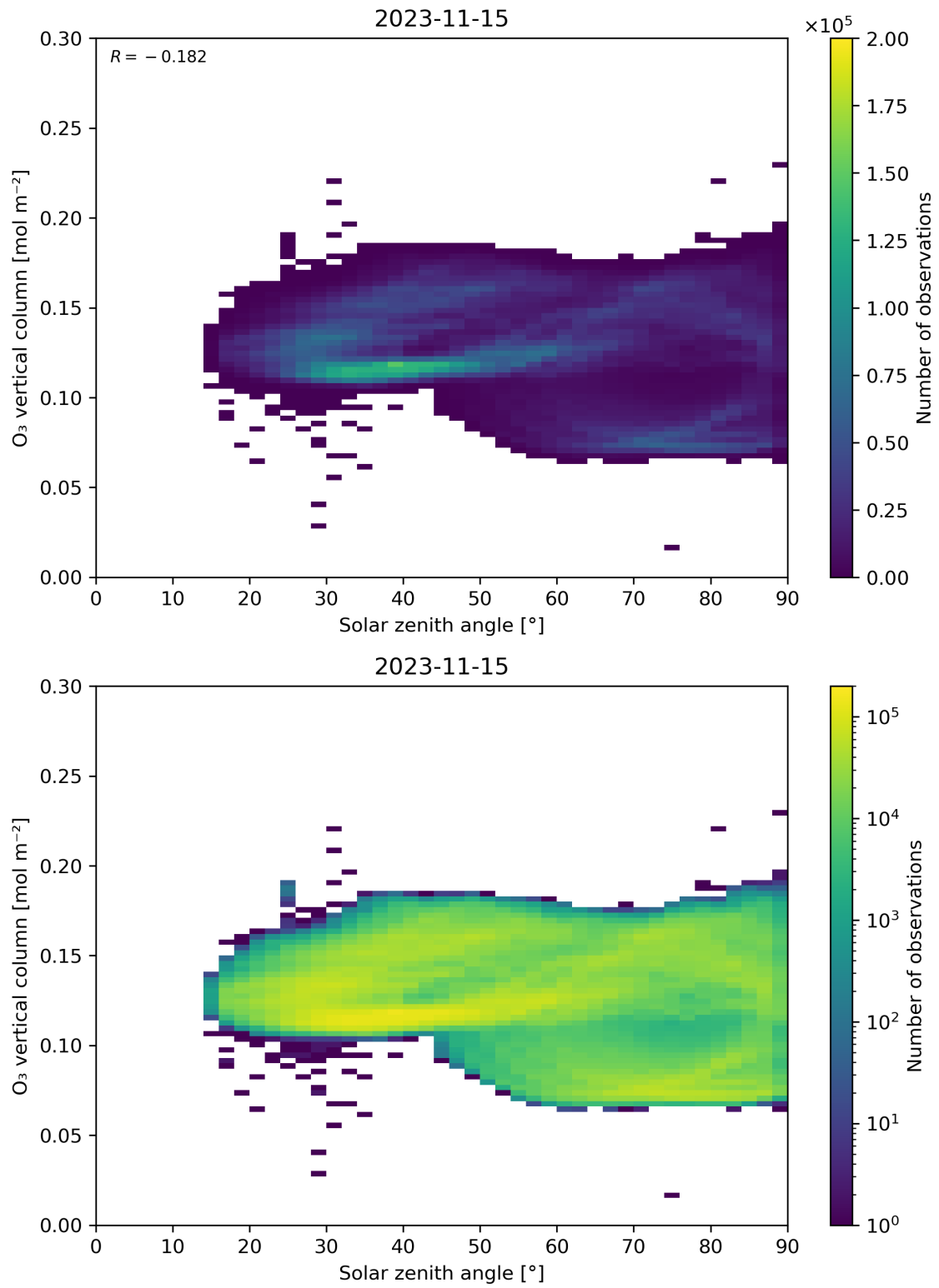
Figure 47: Scatter density plot of “Solar zenith angle” against “O 3 vertical column” for 2023-11-14 to 2023-11-16.
