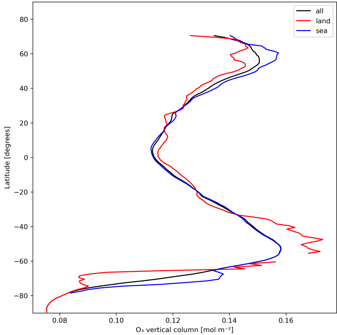
Figure 14: Zonal average of “O 3 vertical column” for 2023-11-14 to 2023-11-16.
