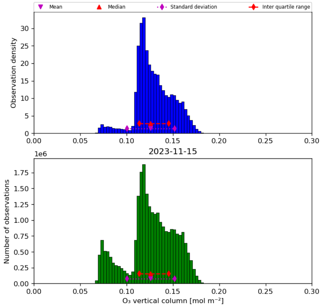
Figure 21: Histogram of “O 3 vertical column” for 2023-11-14 to 2023-11-16
