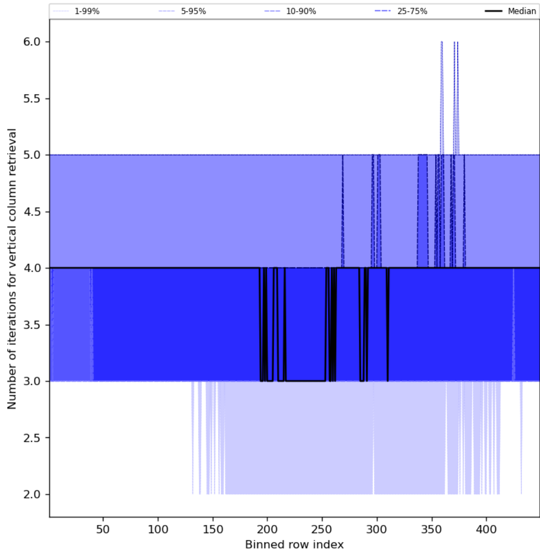
Figure 33: Along track statistics of “Number of iterations for vertical column retrieval” for 2023-11-14 to 2023-11-16
