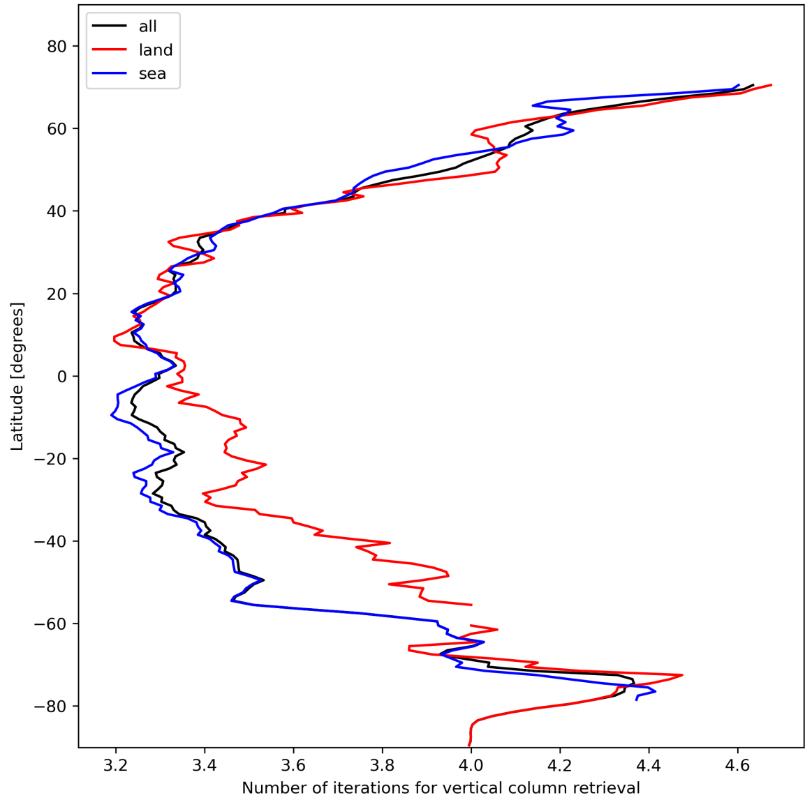
Figure 19: Zonal average of “Number of iterations for vertical column retrieval” for 2023-11-14 to 2023-11-16.
