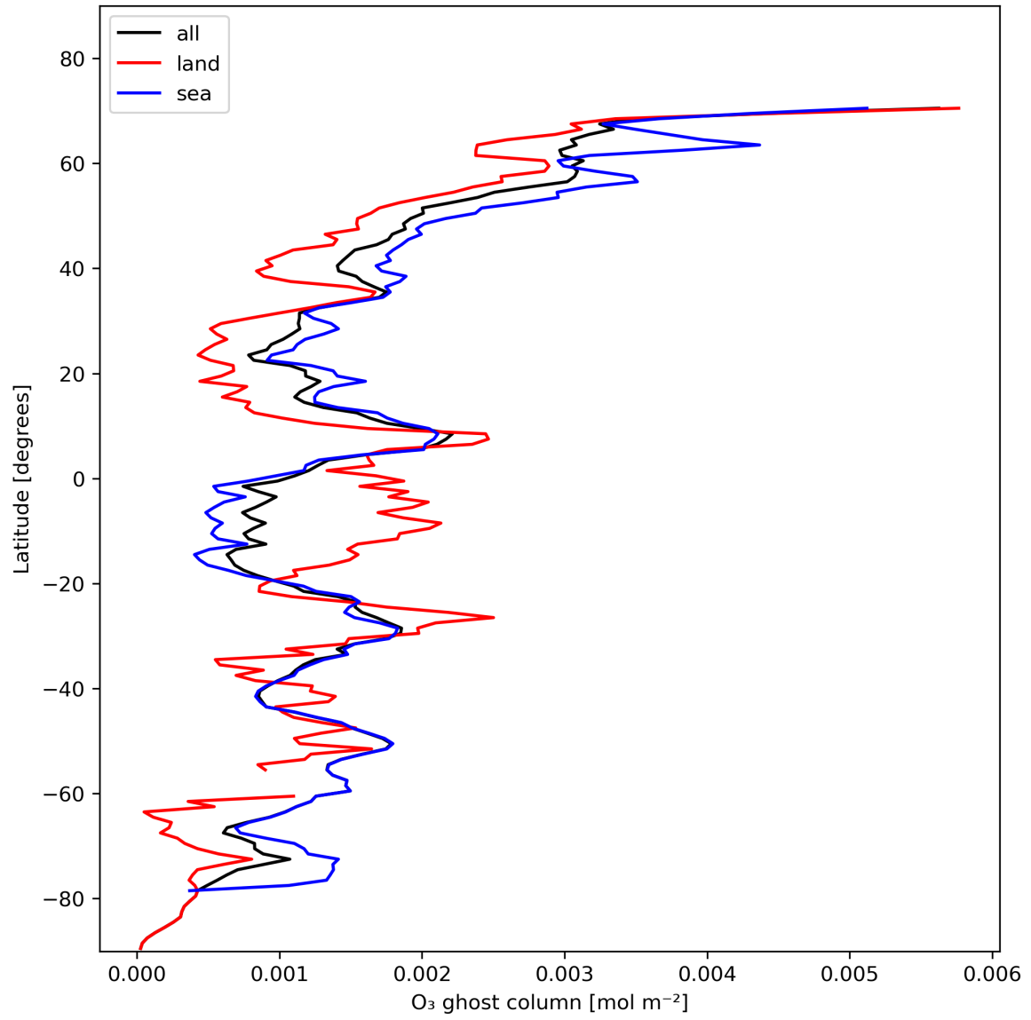
Figure 18: Zonal average of "O 3 ghost column" for 2023-11-14 to 2023-11-16.
