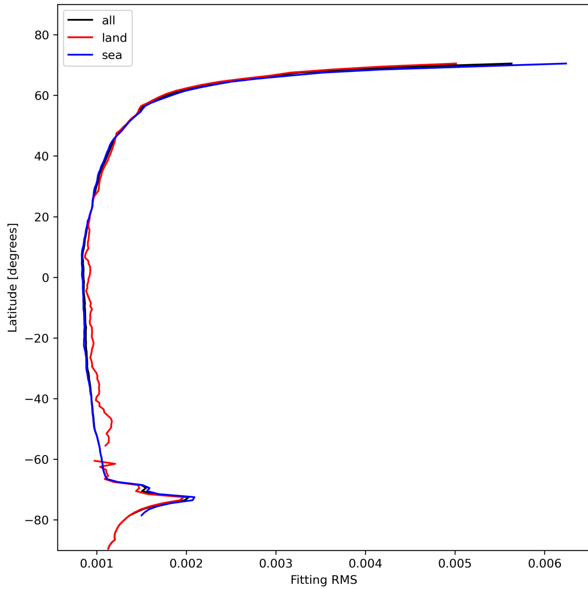
Figure 16: Zonal average of “Fitting RMS” for 2023-11-14 to 2023-11-16.
