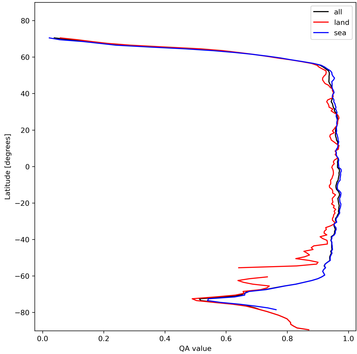
Figure 13: Zonal average of “QA value” for 2023-11-14 to 2023-11-16.
