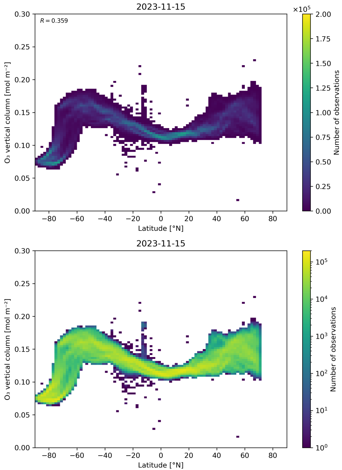
Figure 36: Scatter density plot of “Latitude” against “O 3 vertical column” for 2023-11-14 to 2023-11-16.
