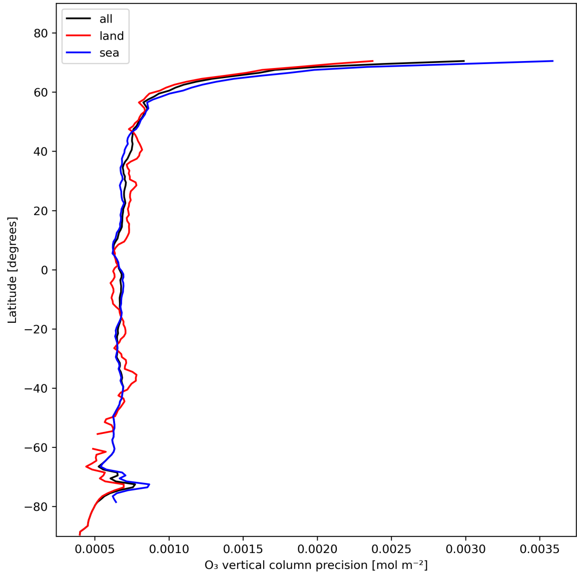
Figure 15: Zonal average of “O 3 vertical column precision” for 2023-11-14 to 2023-11-16.
