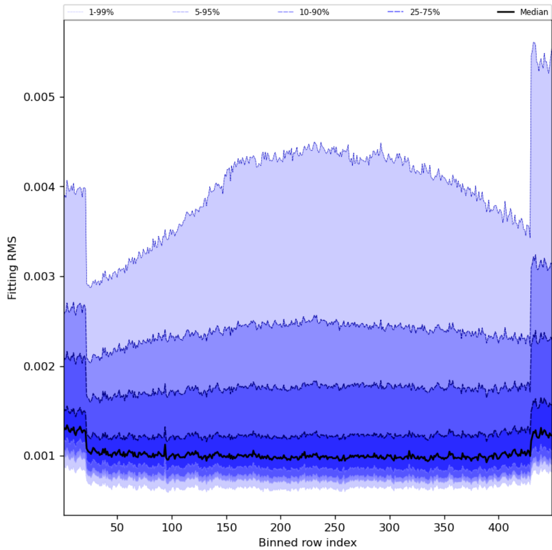
Figure 30: Along track statistics of “Fitting RMS” for 2023-11-14 to 2023-11-16
