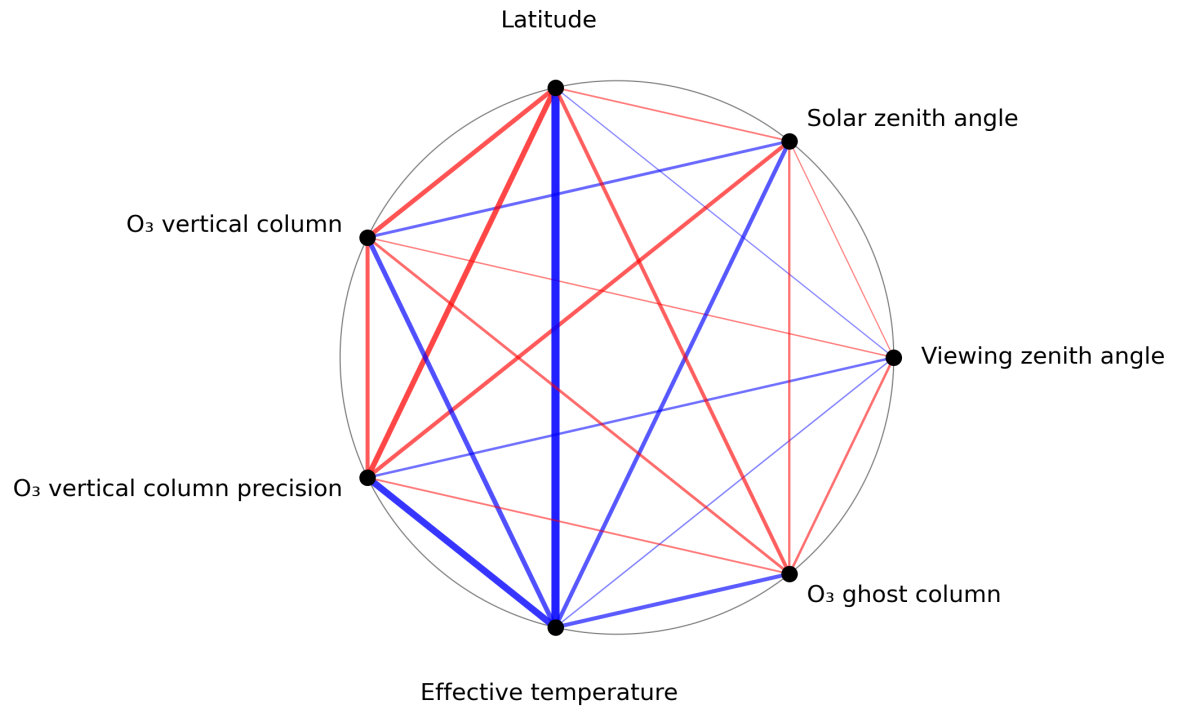
Figure 1: Map of correlation graph for 2023-11-14 to 2023-11-16.
