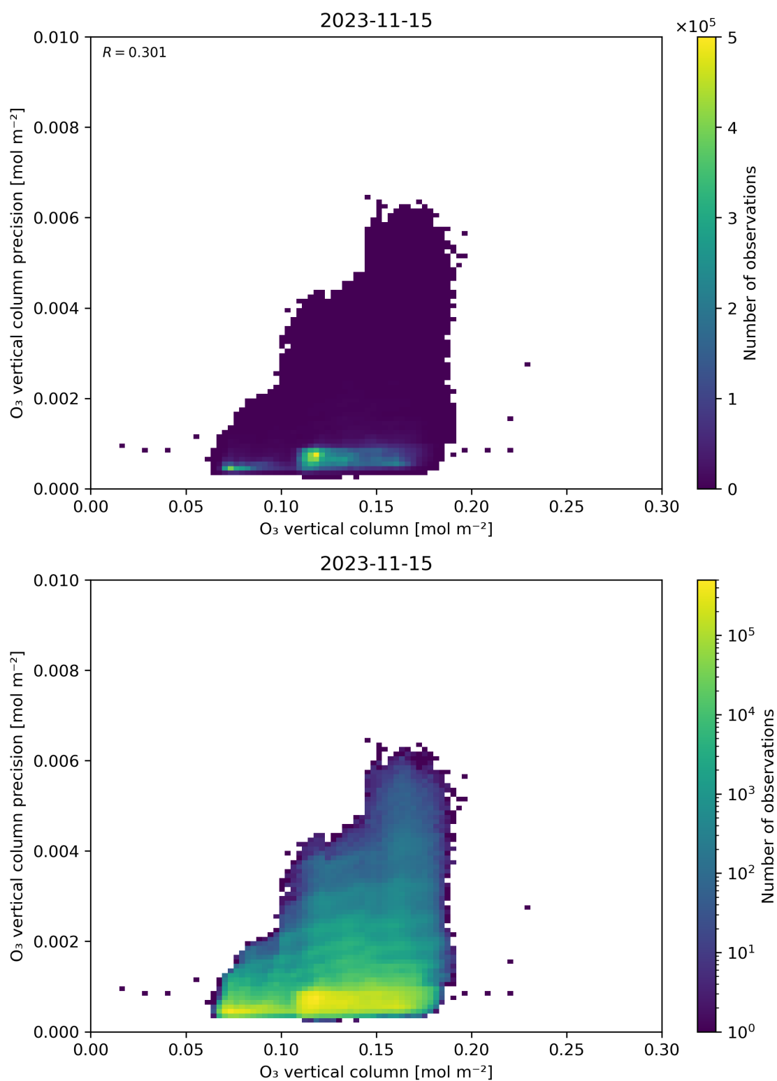
Figure 41: Scatter density plot of “O 3 vertical column” against “O 3 vertical column precision” for 2023-11-14 to 2023-11-16.
