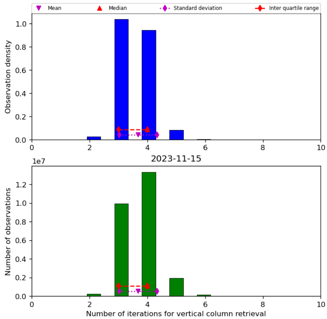
Figure 26: Histogram of “Number of iterations for vertical column retrieval” for 2023-11-14 to 2023-11-16
