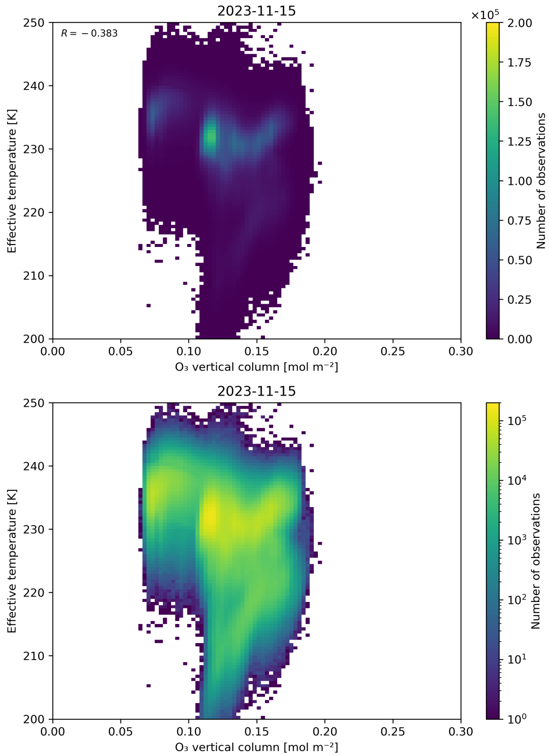
Figure 39: Scatter density plot of “O 3 vertical column” against “Effective temperature” for 2023-11-14 to 2023-11-16.
