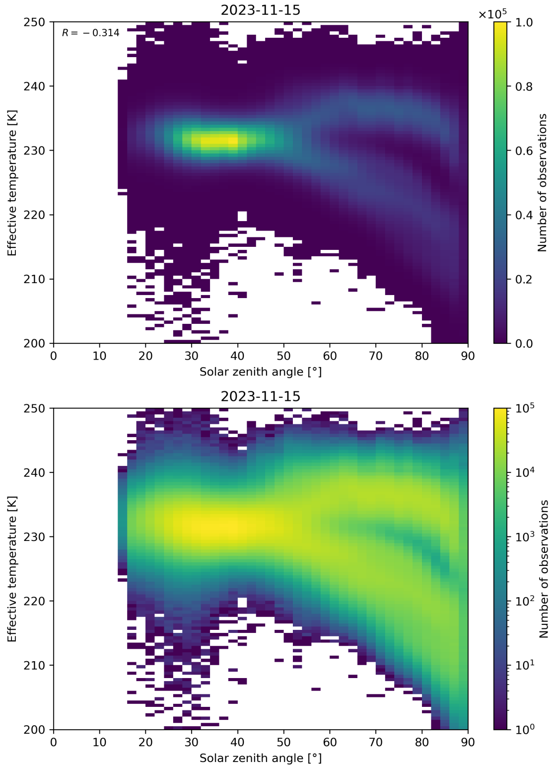
Figure 45: Scatter density plot of “Solar zenith angle” against “Effective temperature” for 2023-11-14 to 2023-11-16.
