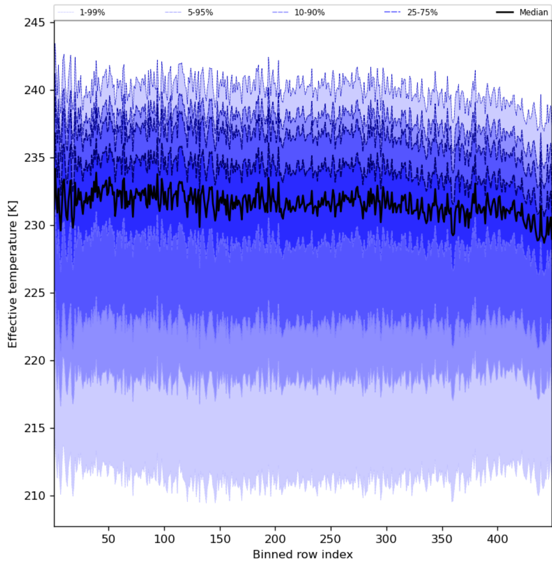
Figure 31: Along track statistics of “Effective temperature” for 2023-11-14 to 2023-11-16
