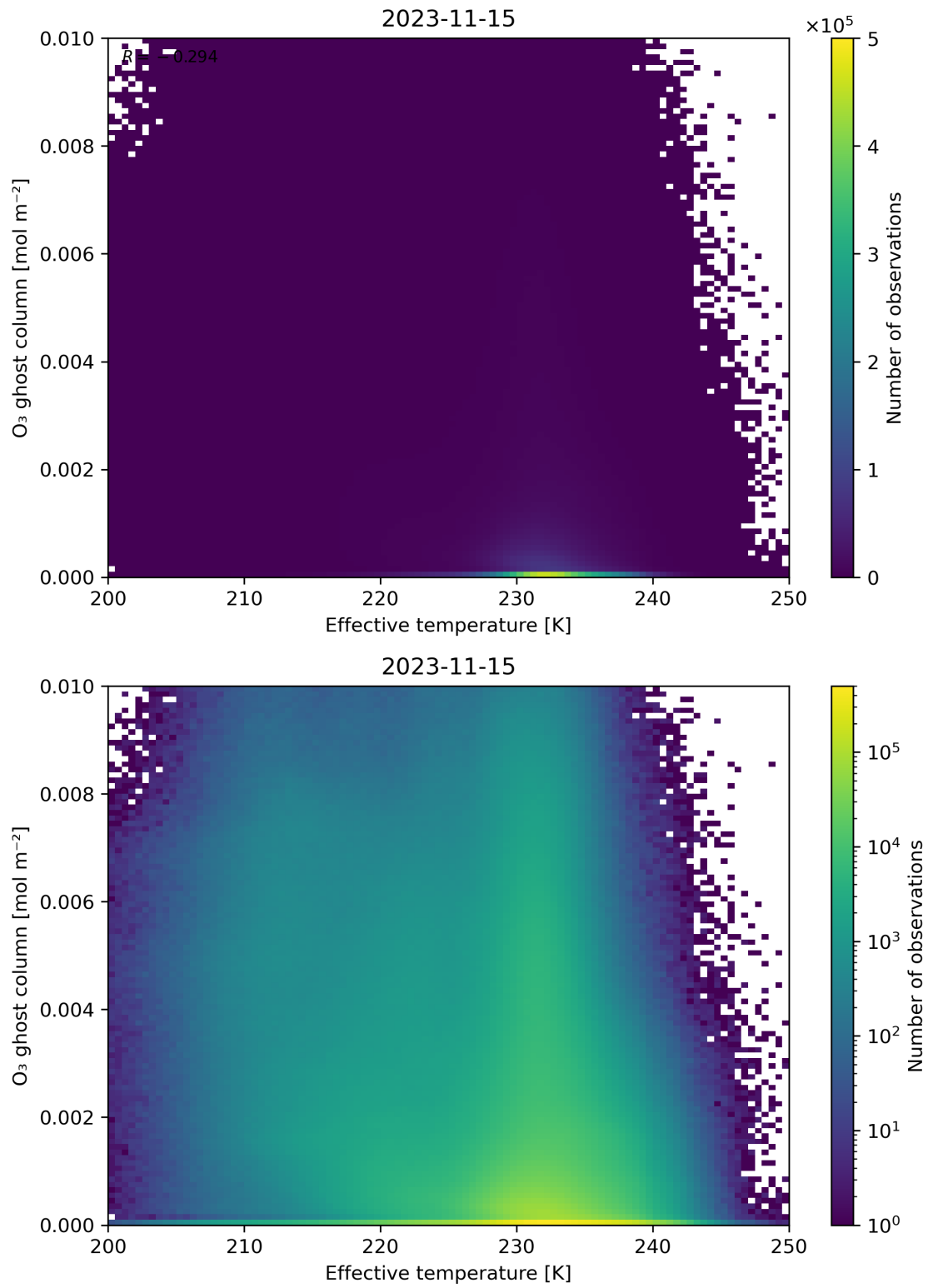
Figure 38: Scatter density plot of “Effective temperature” against “O 3 ghost column” for 2023-11-14 to 2023-11-16.
