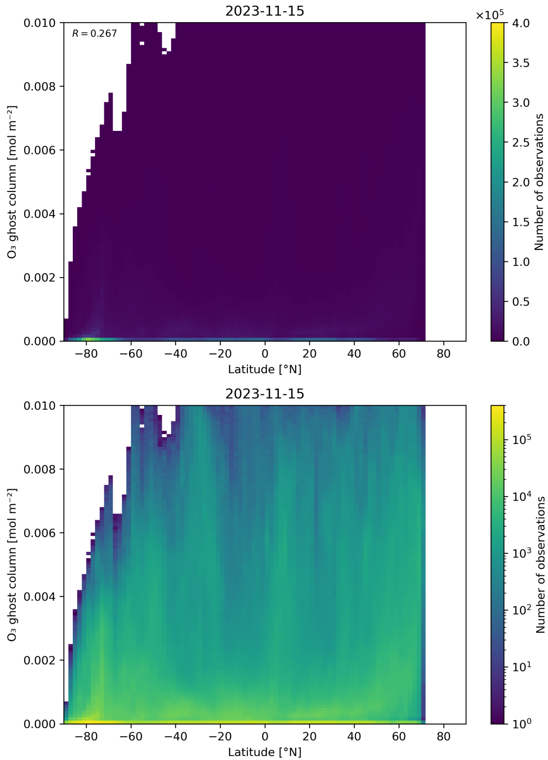
Figure 35: Scatter density plot of “Latitude” against “O 3 ghost column” for 2023-11-14 to 2023-11-16.
