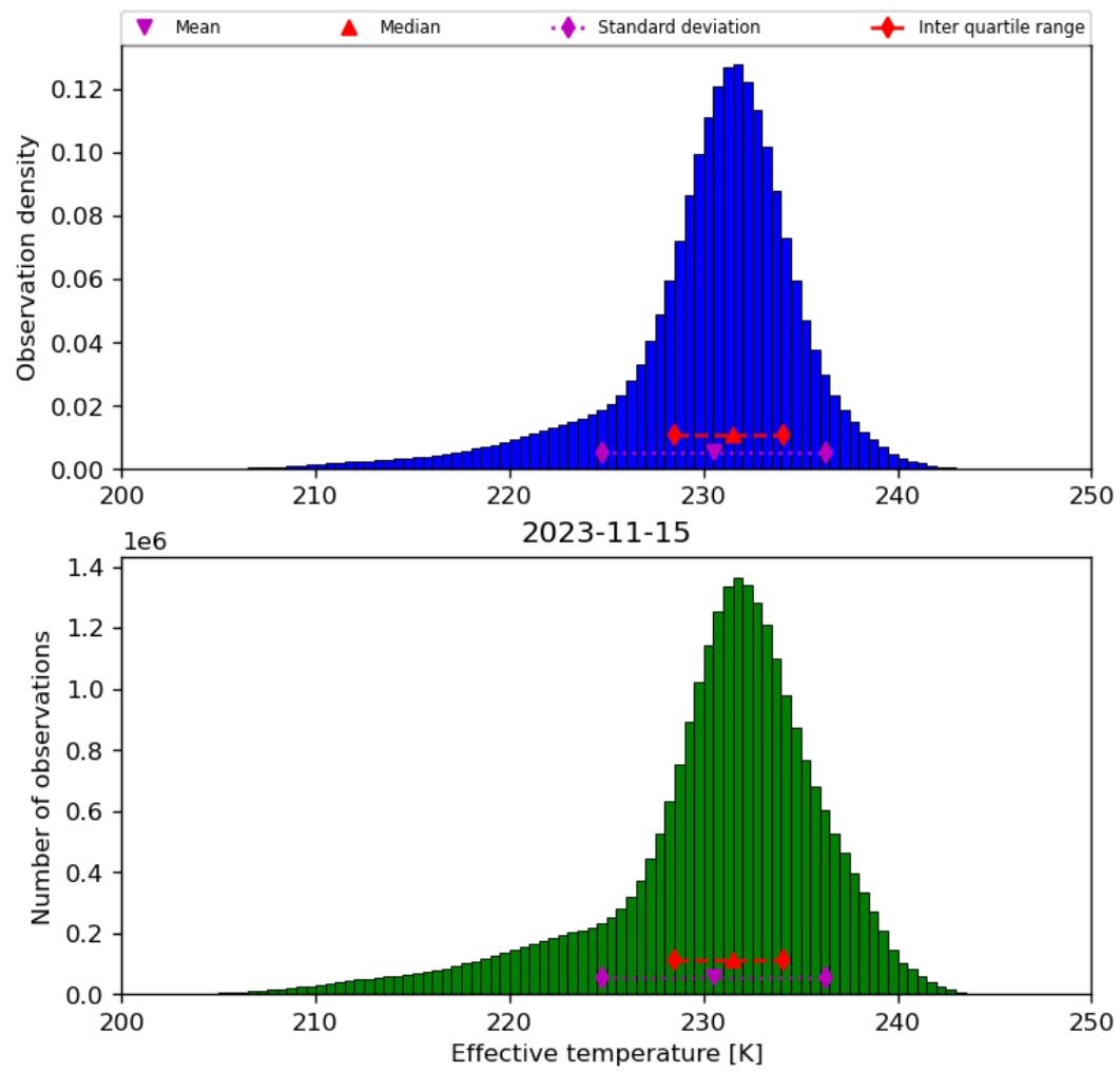
Figure 24: Histogram of “Effective temperature” for 2023-11-14 to 2023-11-16
