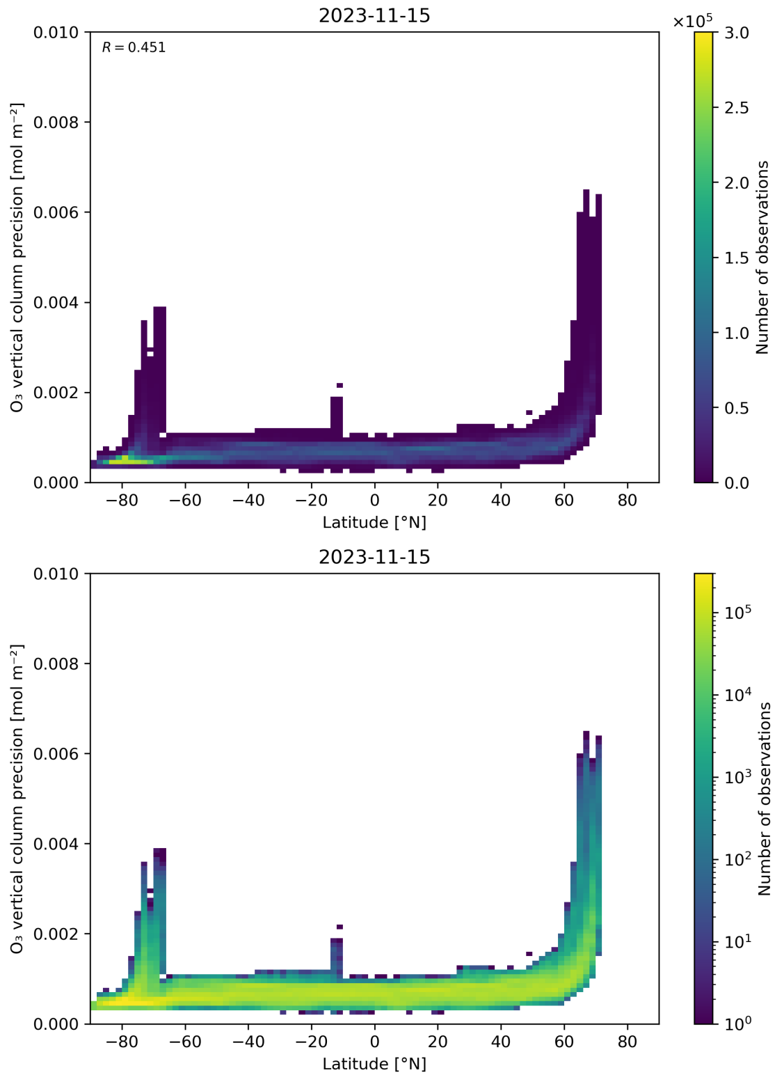
Figure 37: Scatter density plot of “Latitude” against “O 3 vertical column precision” for 2023-11-14 to 2023-11-16.
