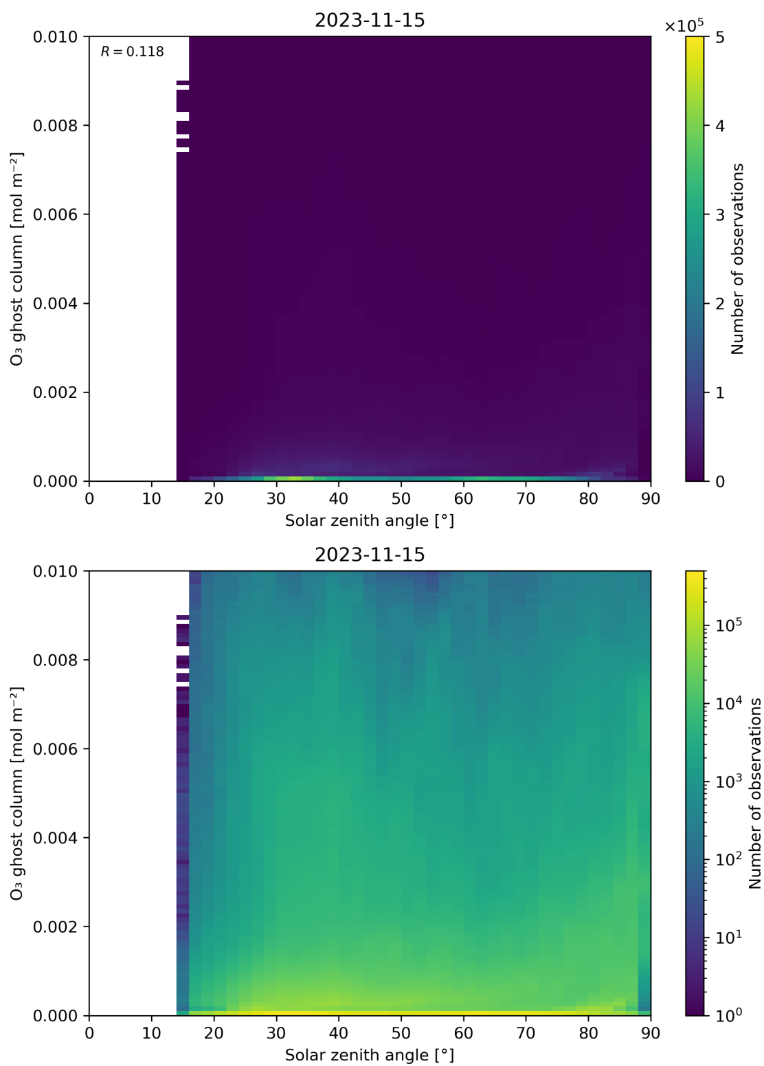
Figure 46: Scatter density plot of “Solar zenith angle” against “O 3 ghost column” for 2023-11-14 to 2023-11-16.
