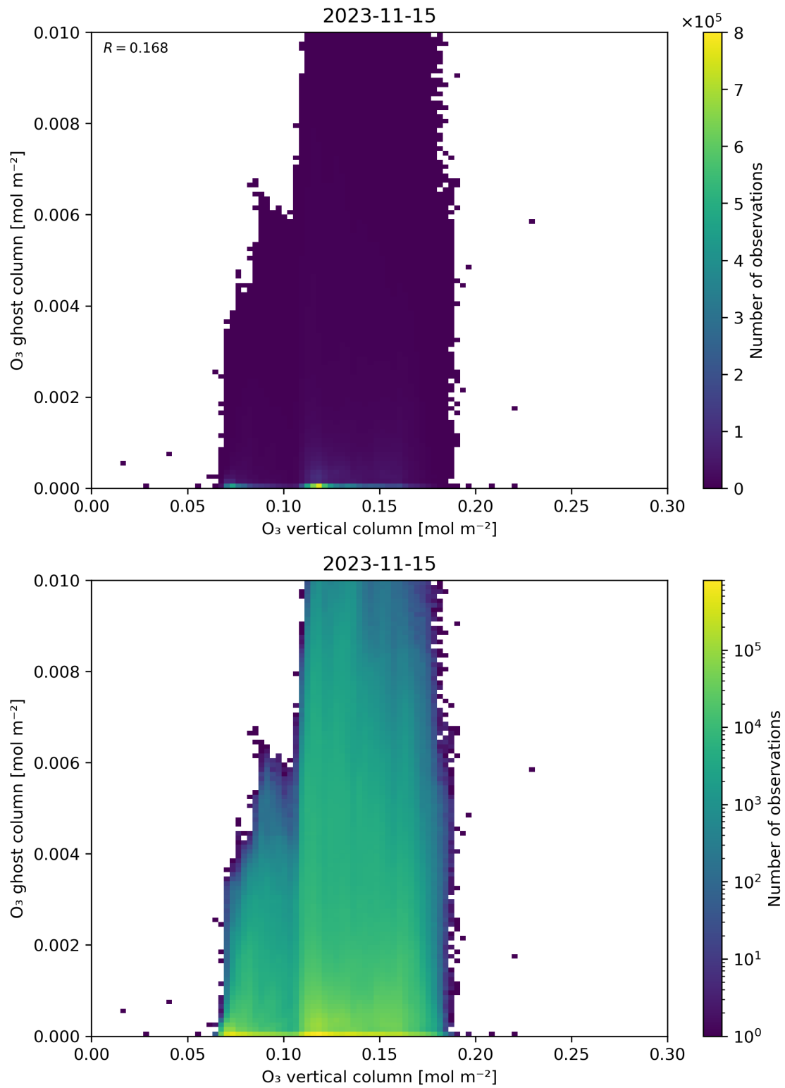
Figure 40: Scatter density plot of “O 3 vertical column” against “O 3 ghost column” for 2023-11-14 to 2023-11-16.
