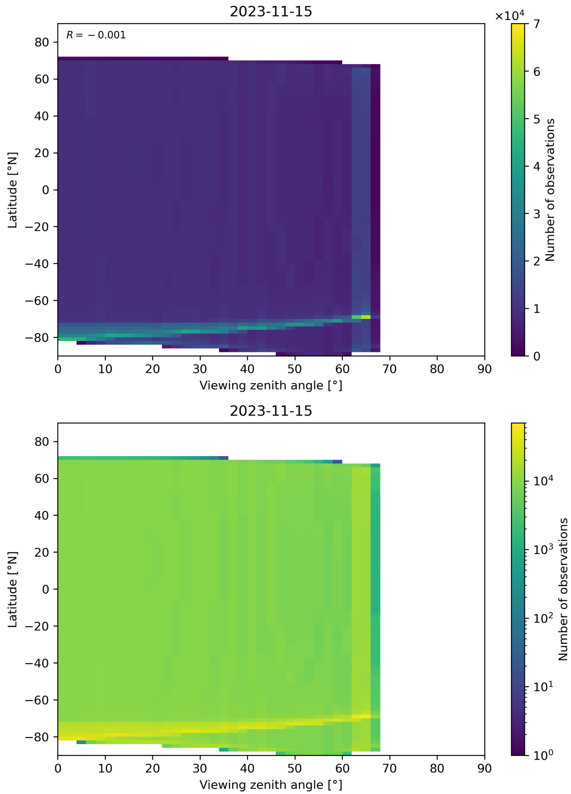
Figure 49: Scatter density plot of “Viewing zenith angle” against “Latitude” for 2023-11-14 to 2023-11-16.
