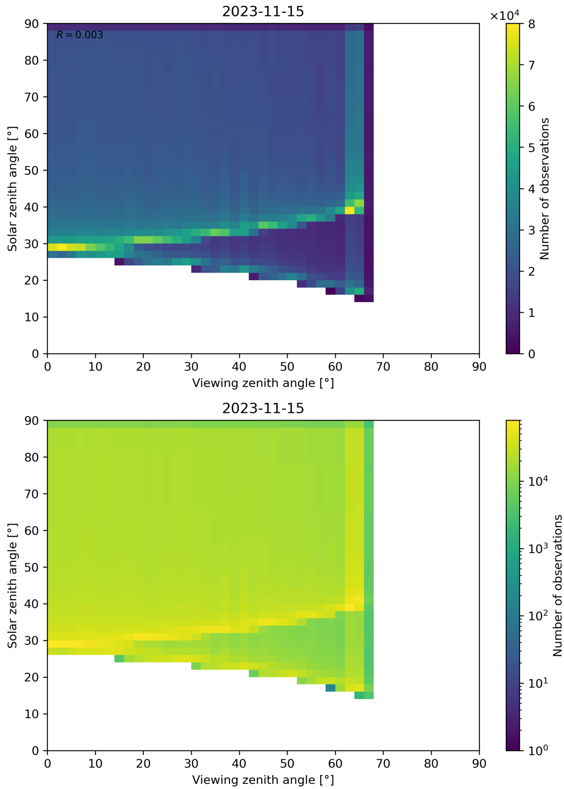
Figure 54: Scatter density plot of “Viewing zenith angle” against “Solar zenith angle” for 2023-11-14 to 2023-11-16.
