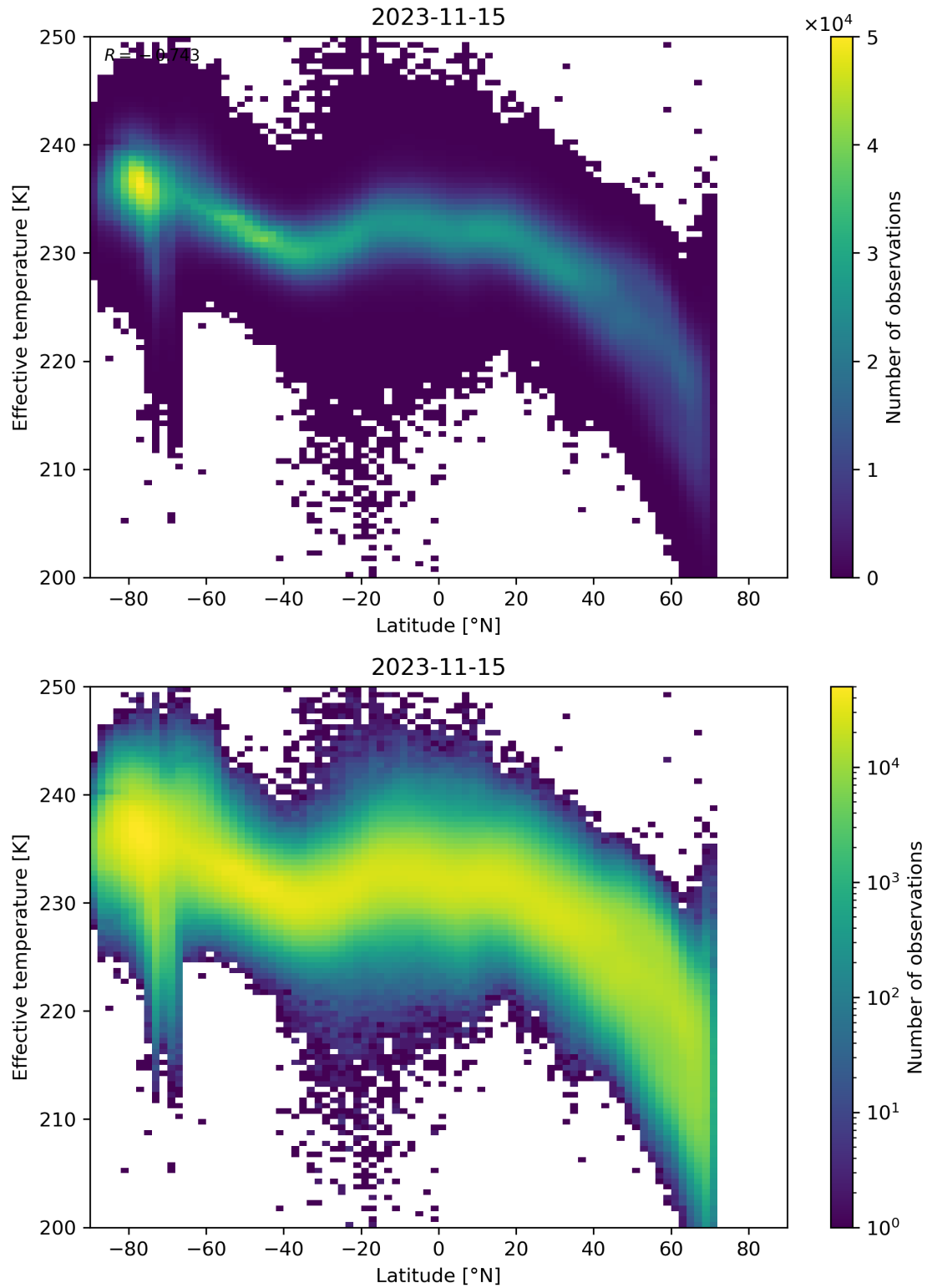
Figure 34: Scatter density plot of “Latitude” against “Effective temperature” for 2023-11-14 to 2023-11-16.
