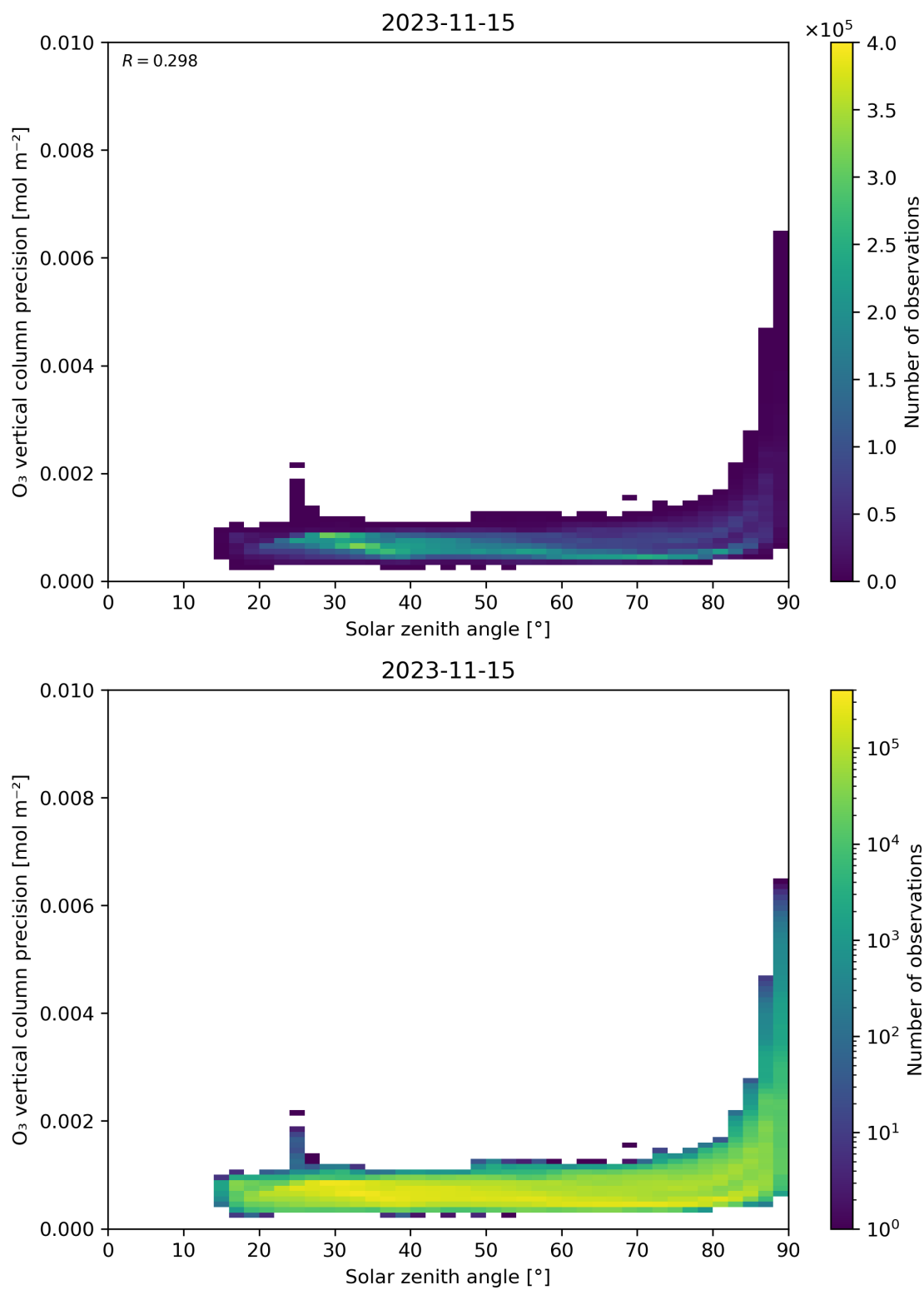
Figure 48: Scatter density plot of “Solar zenith angle” against “O 3 vertical column precision” for 2023-11-14 to 2023-11-16.
