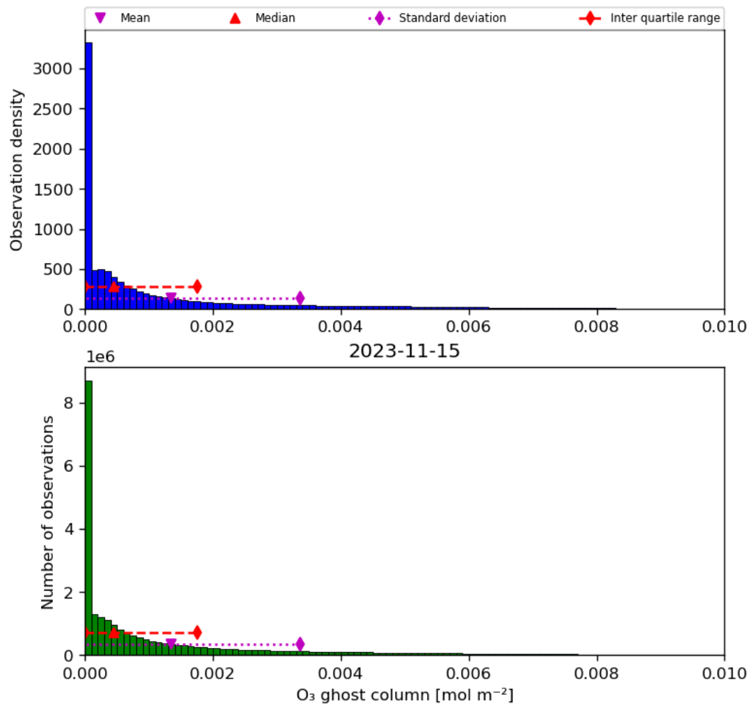
Figure 25: Histogram of “O 3 ghost column” for 2023-11-14 to 2023-11-16
