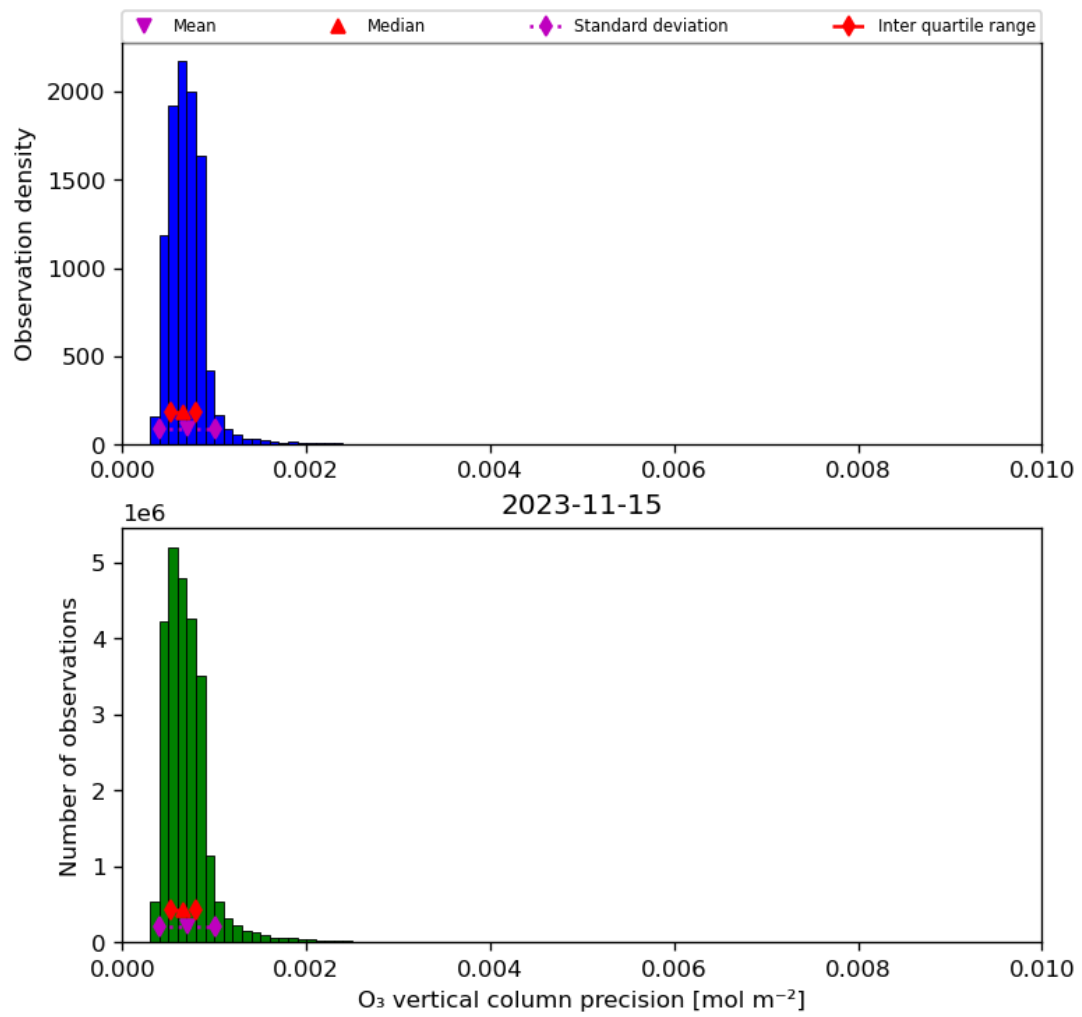
Figure 22: Histogram of “O 3 vertical column precision” for 2023-11-14 to 2023-11-16
