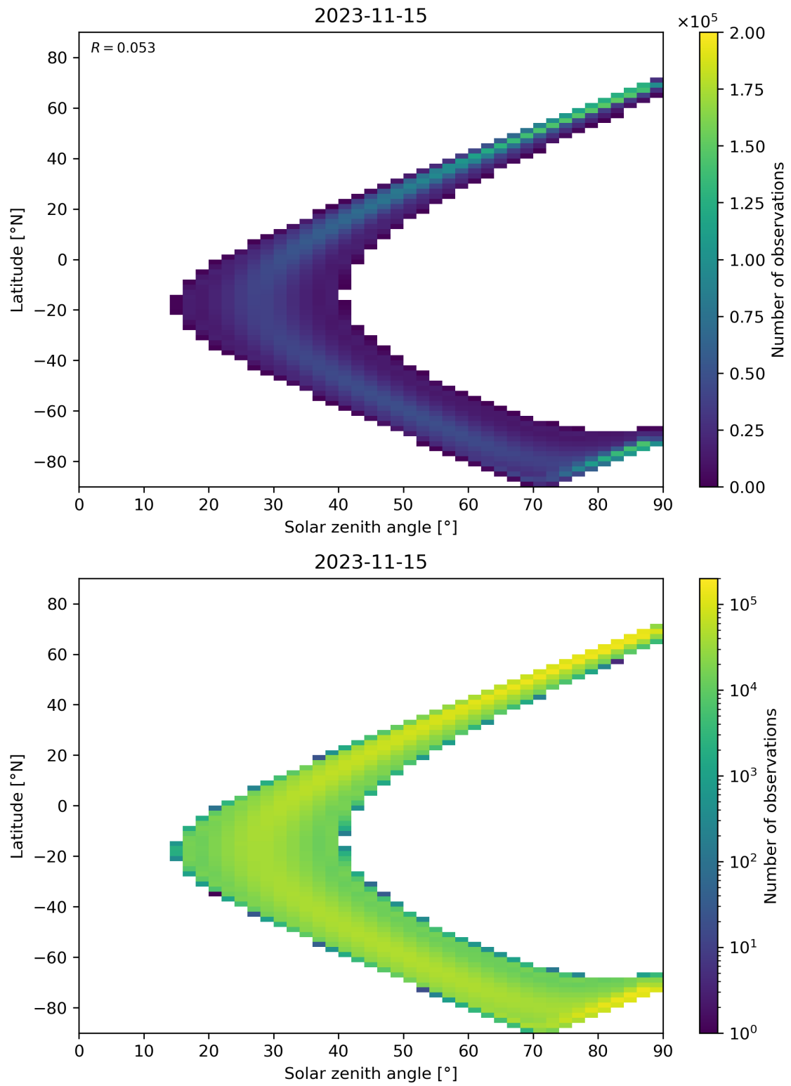
Figure 44: Scatter density plot of “Solar zenith angle” against “Latitude” for 2023-11-14 to 2023-11-16.
