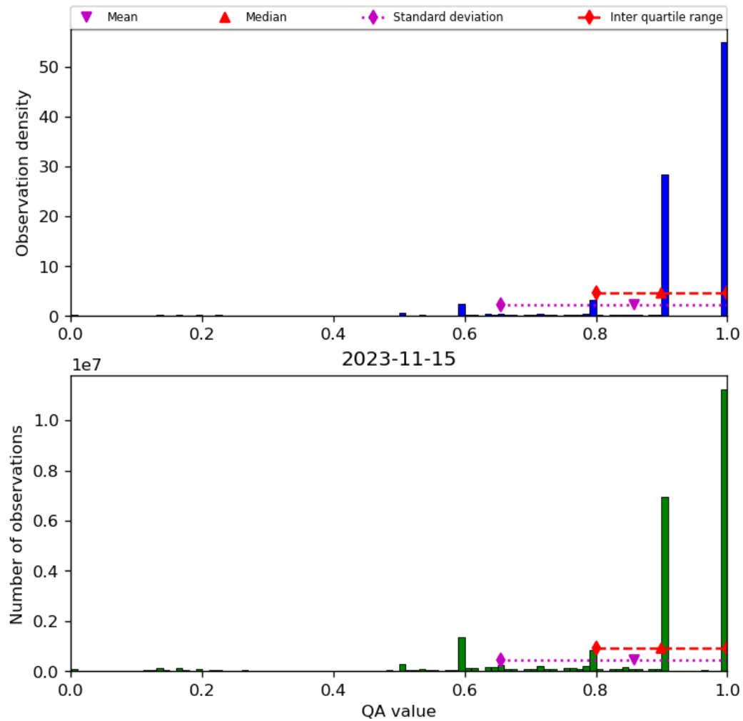
Figure 20: Histogram of “QA value” for 2023-11-14 to 2023-11-16
