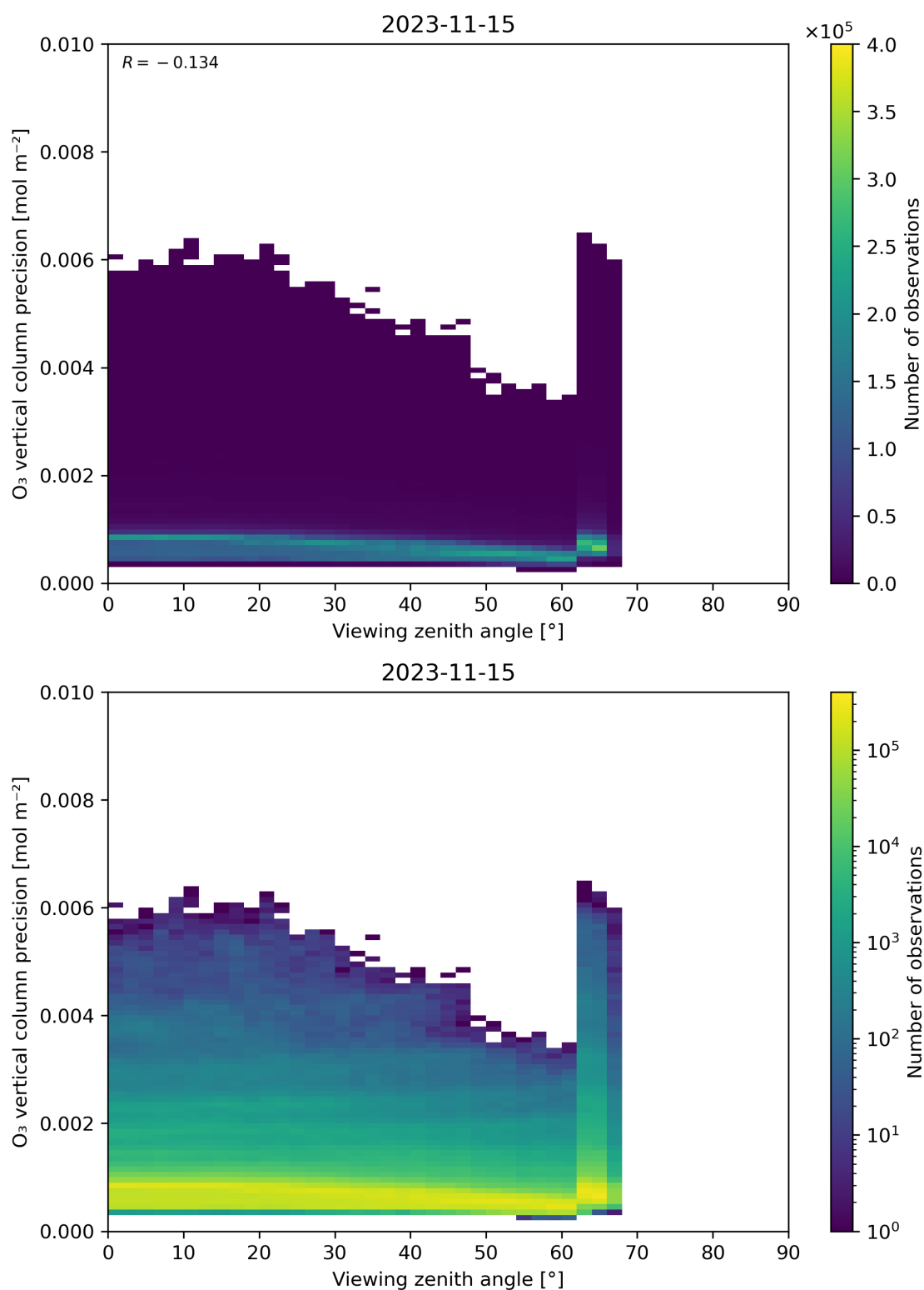
Figure 53: Scatter density plot of “Viewing zenith angle” against “O 3 vertical column precision” for 2023-11-14 to 2023-11-16.
