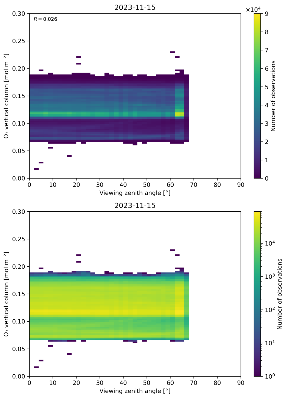
Figure 52: Scatter density plot of “Viewing zenith angle” against “O 3 vertical column” for 2023-11-14 to 2023-11-16.
