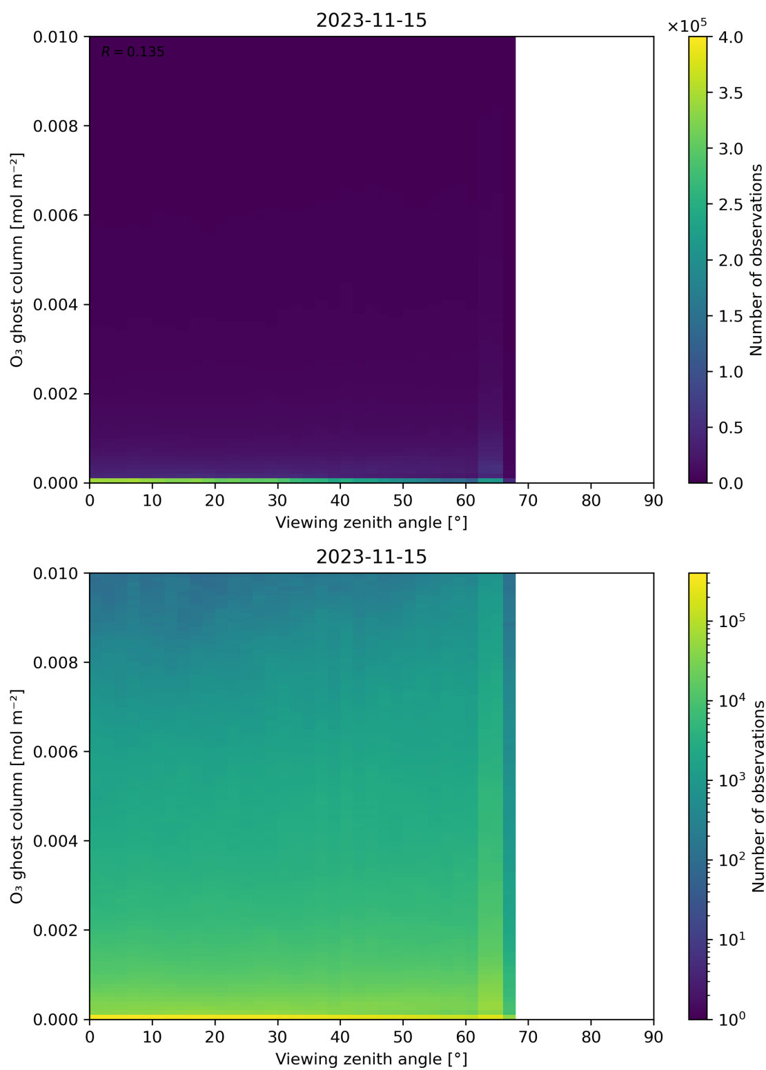
Figure 51: Scatter density plot of “Viewing zenith angle” against “O 3 ghost column” for 2023-11-14 to 2023-11-16.
