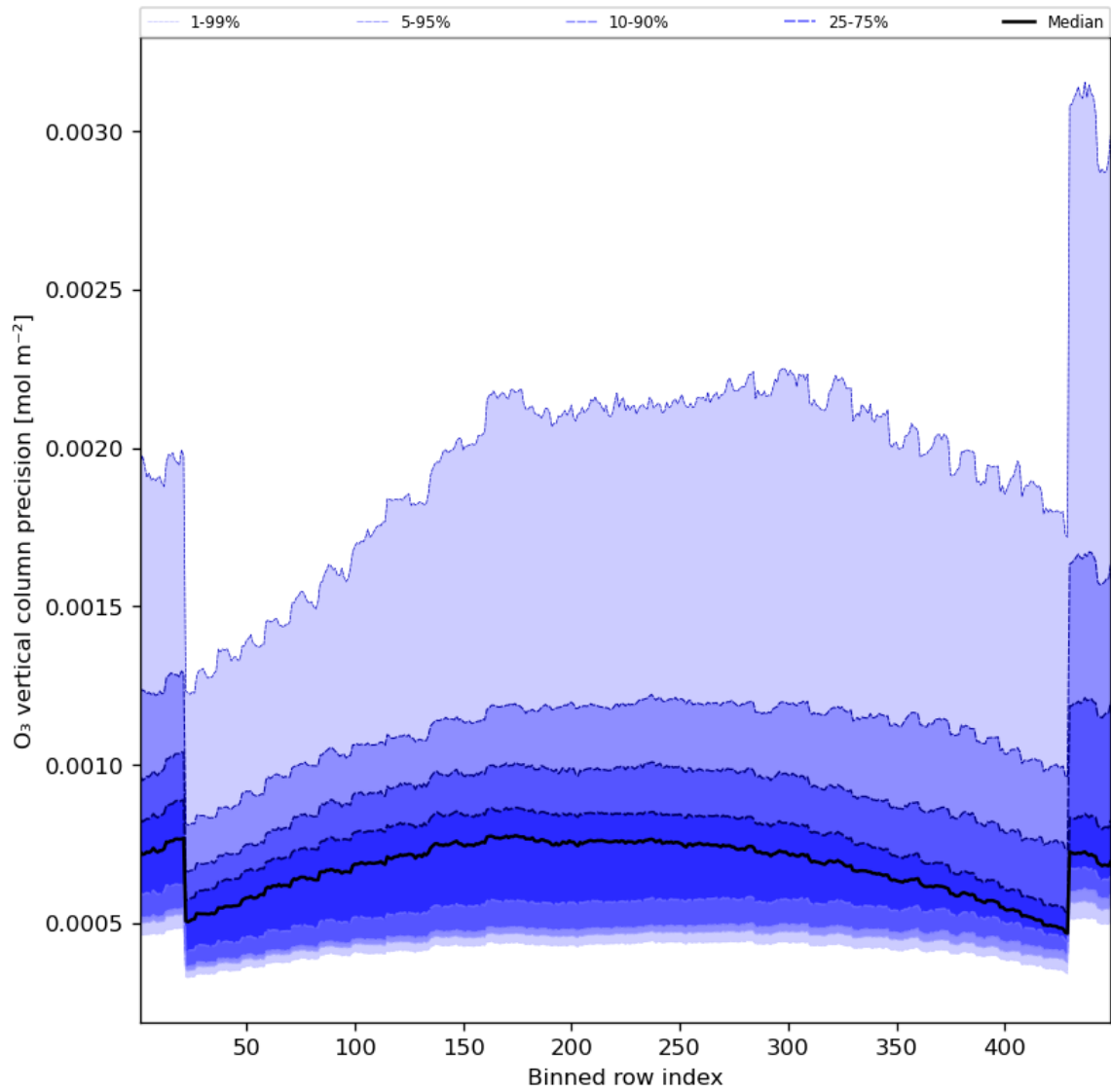
Figure 29: Along track statistics of “O 3 vertical column precision” for 2023-11-14 to 2023-11-16
