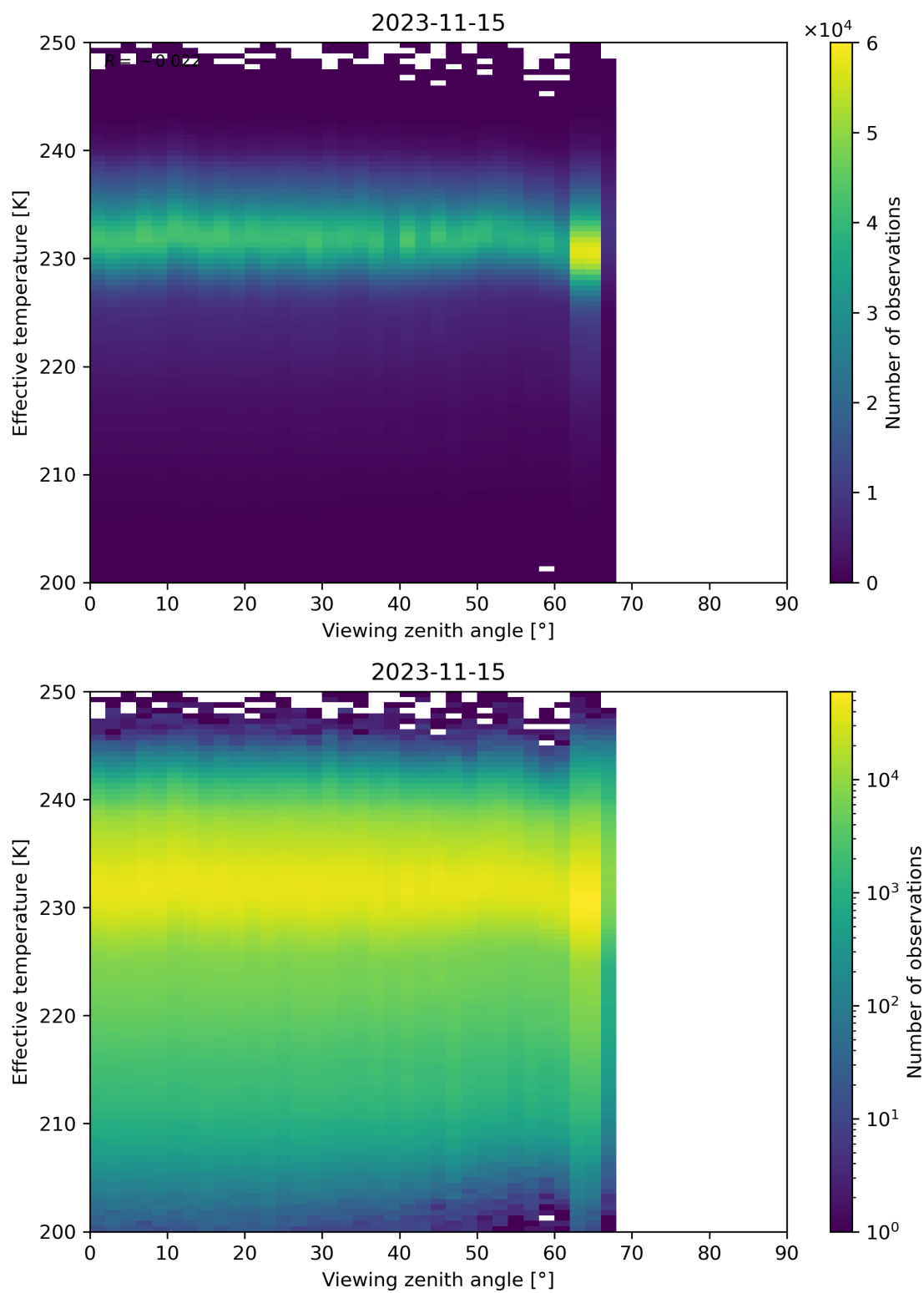
Figure 50: Scatter density plot of “Viewing zenith angle” against “Effective temperature” for 2023-11-14 to 2023-11-16.
