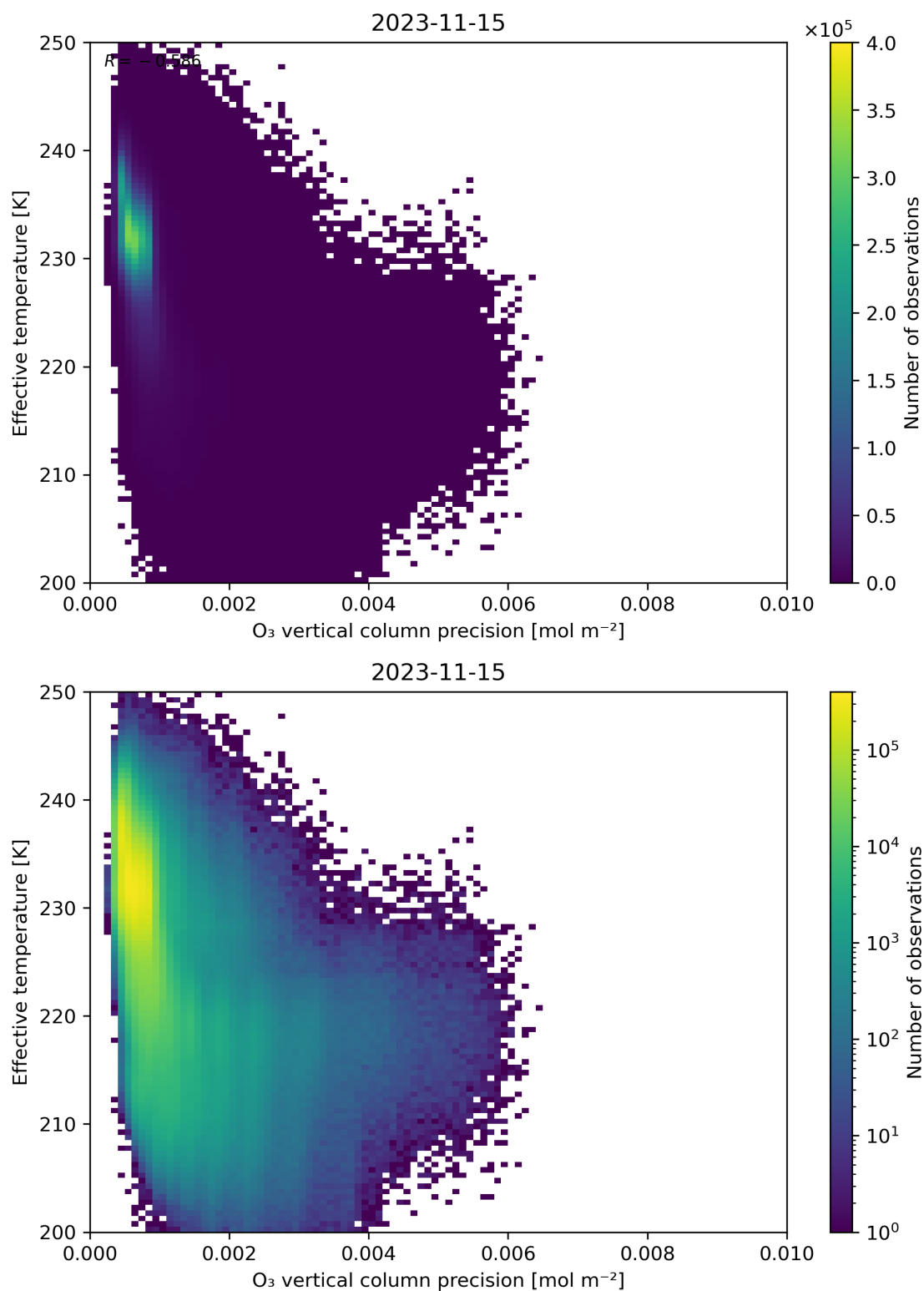
Figure 42: Scatter density plot of “O 3 vertical column precision” against “Effective temperature” for 2023-11-14 to 2023-11-16.
