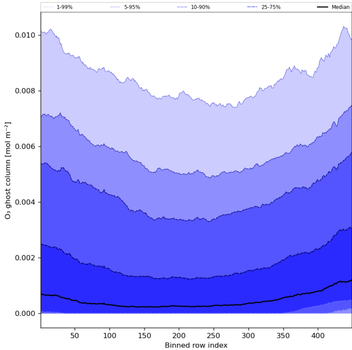
Figure 32: Along track statistics of “O 3 ghost column” for 2023-11-14 to 2023-11-16
