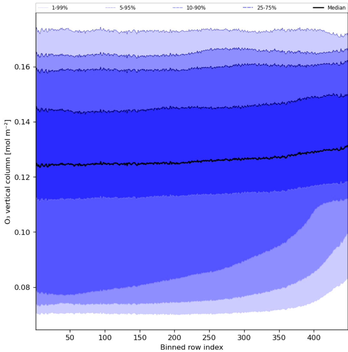
Figure 28: Along track statistics of “O 3 vertical column” for 2023-11-14 to 2023-11-16
