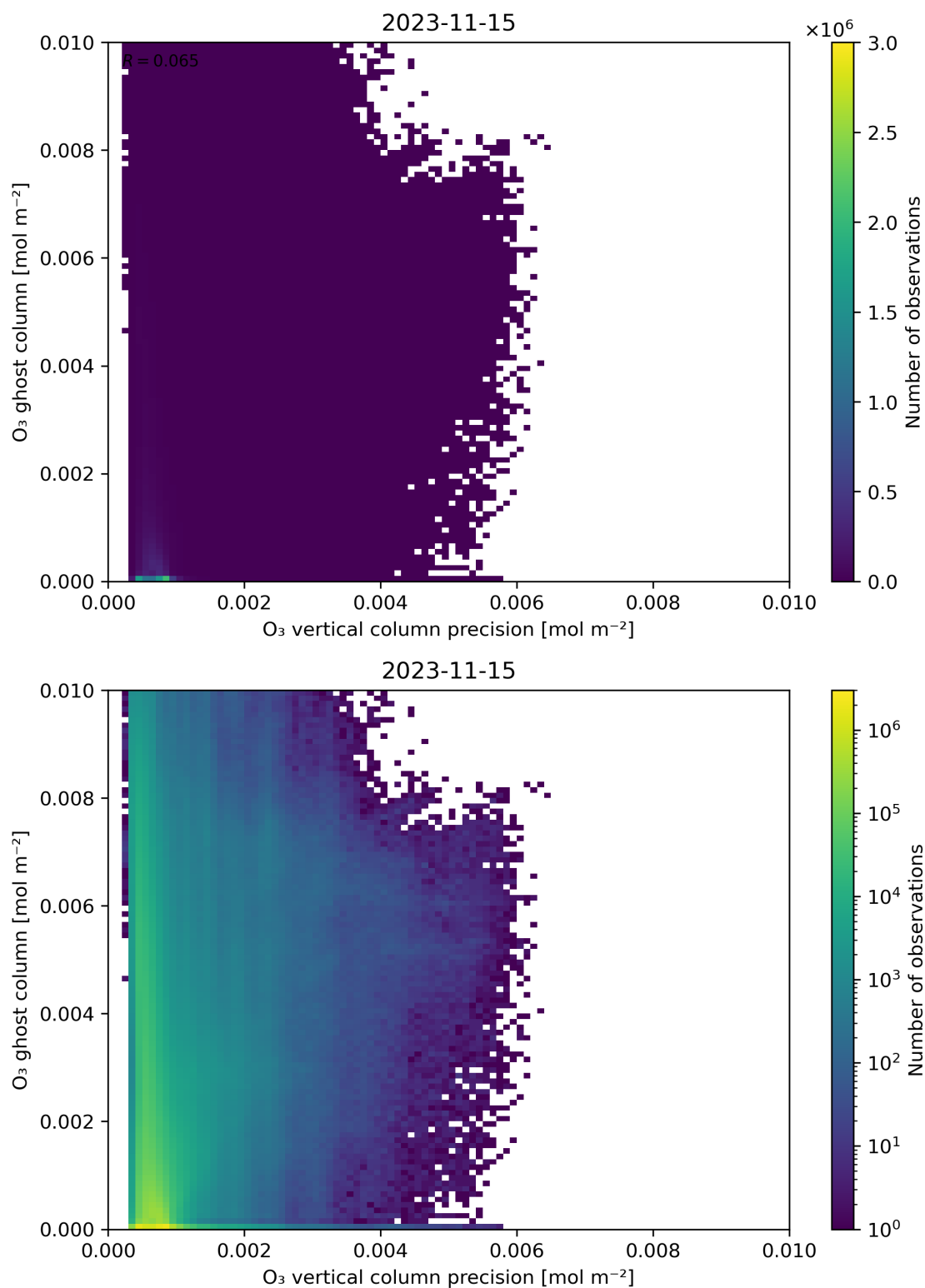
Figure 43: Scatter density plot of “O 3 vertical column precision” against “O 3 ghost column” for 2023-11-14 to 2023-11-16.
