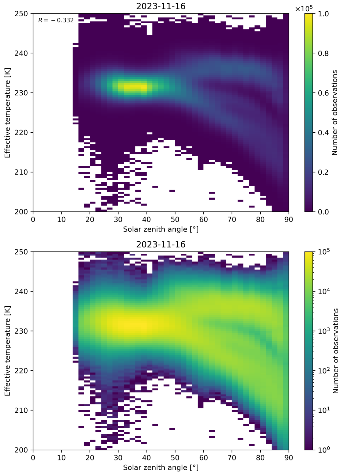
Figure 45: Scatter density plot of “Solar zenith angle” against “Effective temperature” for 2023-11-15 to 2023-11-17.
