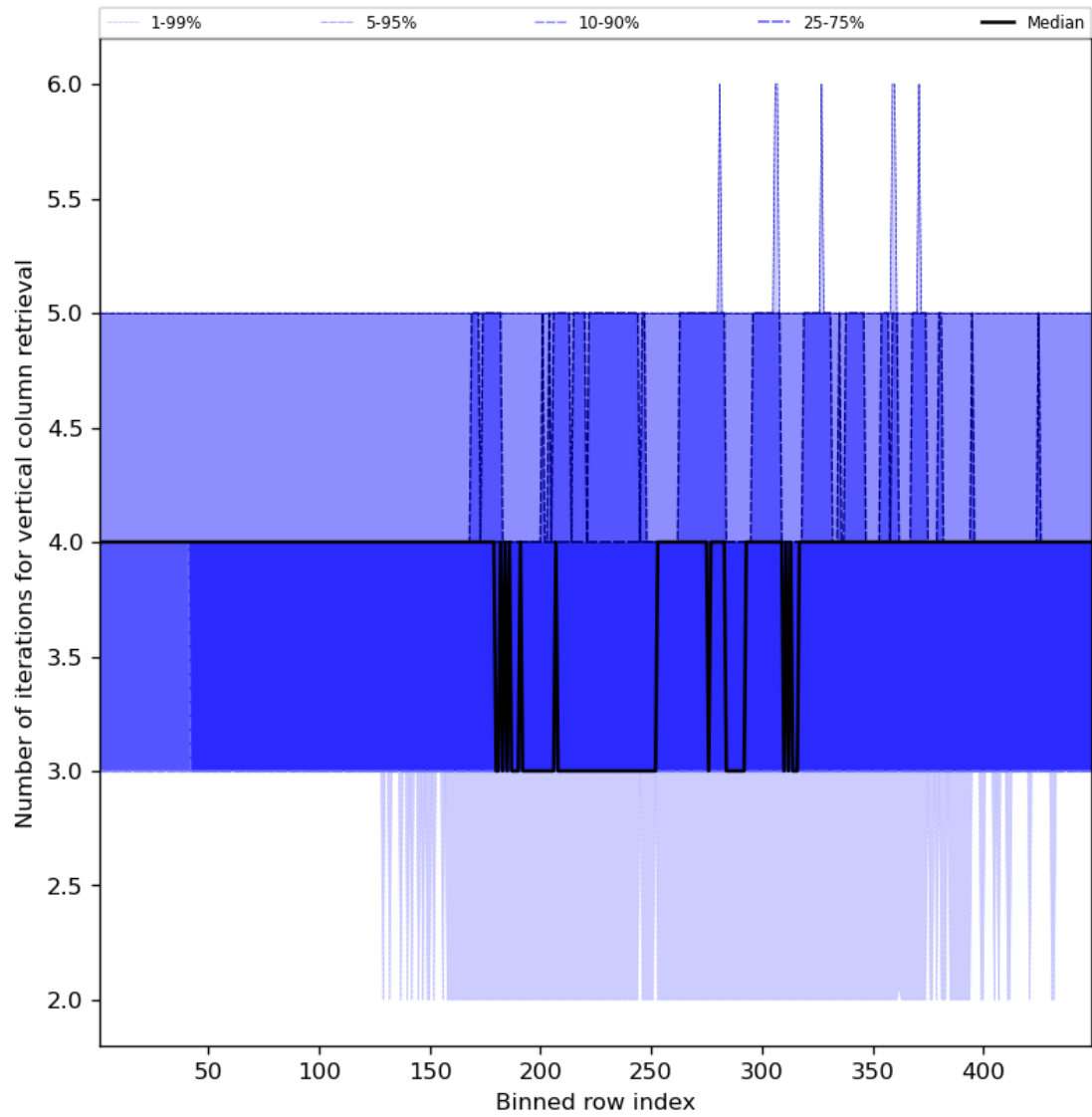
Figure 33: Along track statistics of “Number of iterations for vertical column retrieval” for 2023-11-15 to 2023-11-17
