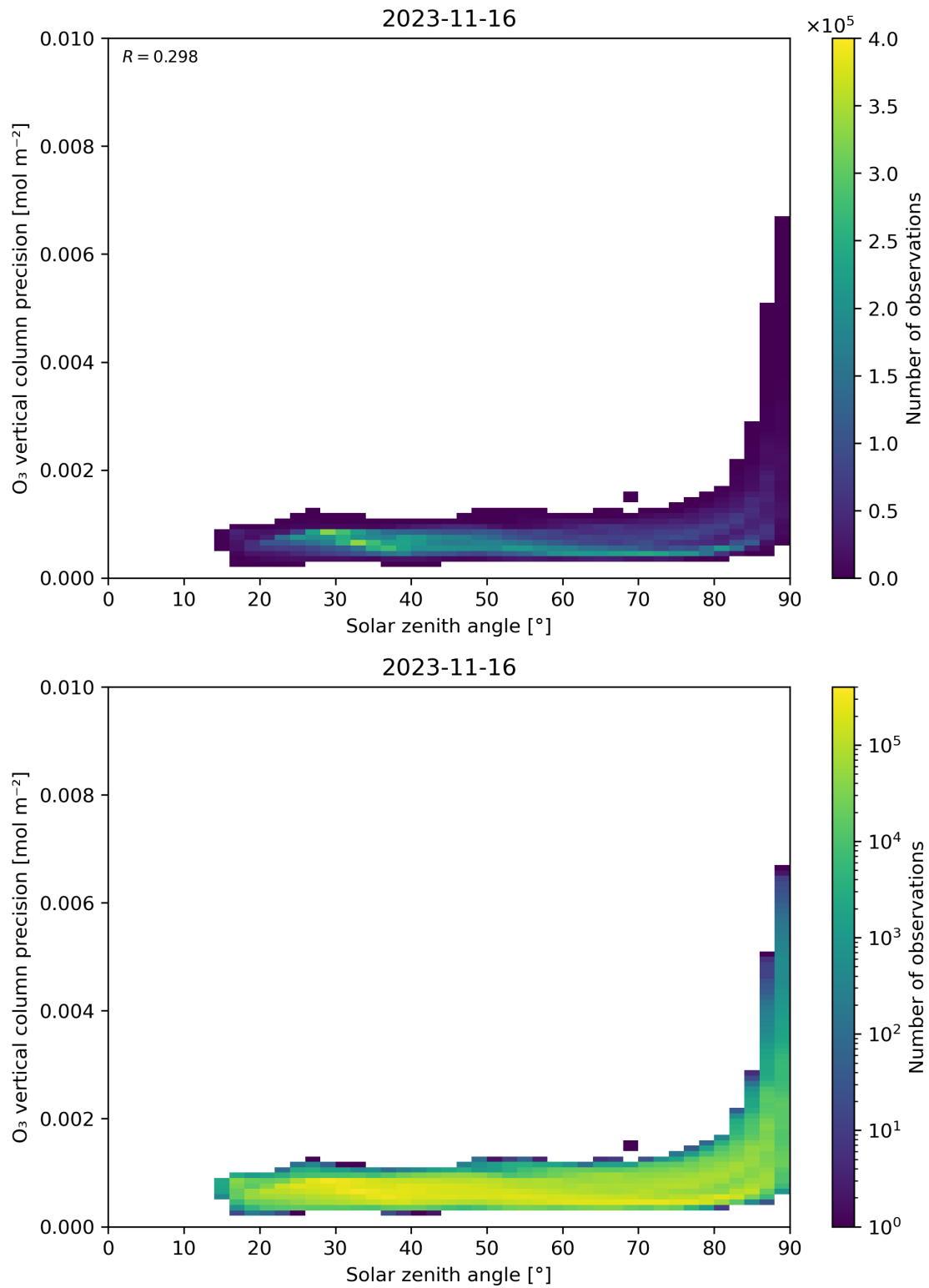
Figure 48: Scatter density plot of “Solar zenith angle” against “O 3 vertical column precision” for 2023-11-15 to 2023-11-17.
