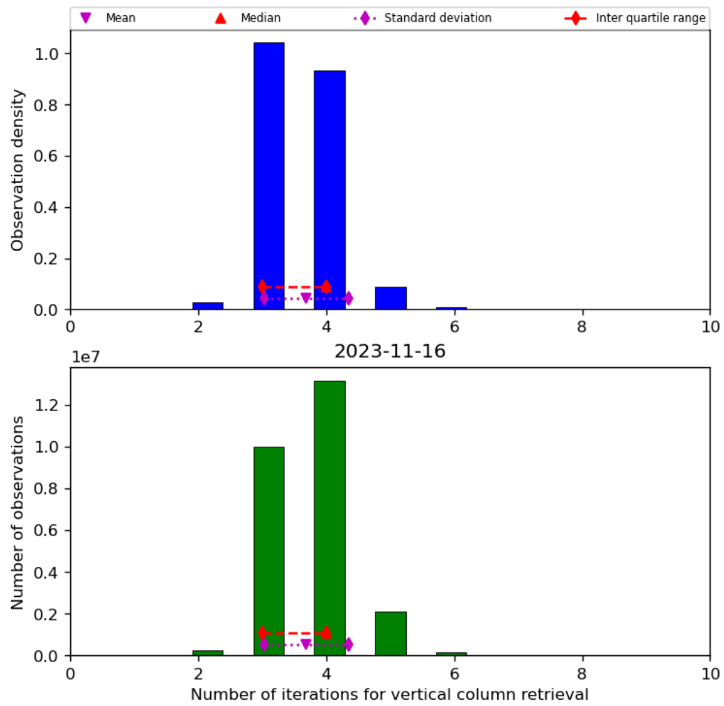
Figure 26: Histogram of “Number of iterations for vertical column retrieval” for 2023-11-15 to 2023-11-17
