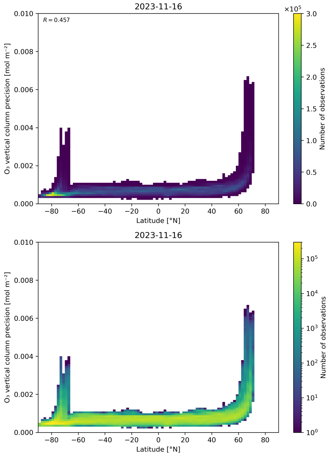
Figure 37: Scatter density plot of “Latitude” against “O 3 vertical column precision” for 2023-11-15 to 2023-11-17.
