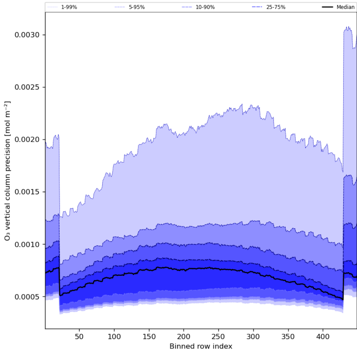
Figure 29: Along track statistics of “O 3 vertical column precision” for 2023-11-15 to 2023-11-17
