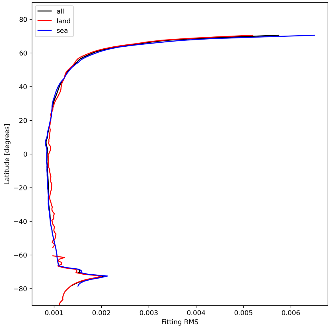
Figure 16: Zonal average of “Fitting RMS” for 2023-11-15 to 2023-11-17.
