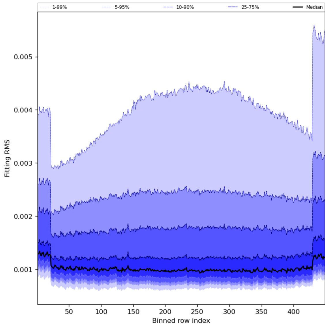
Figure 30: Along track statistics of “Fitting RMS” for 2023-11-15 to 2023-11-17
