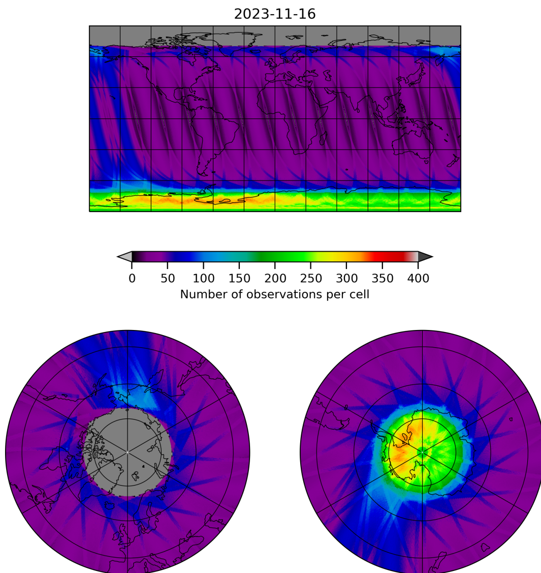
Figure 12: Map of the number of observations for 2023-11-15 to 2023-11-17
