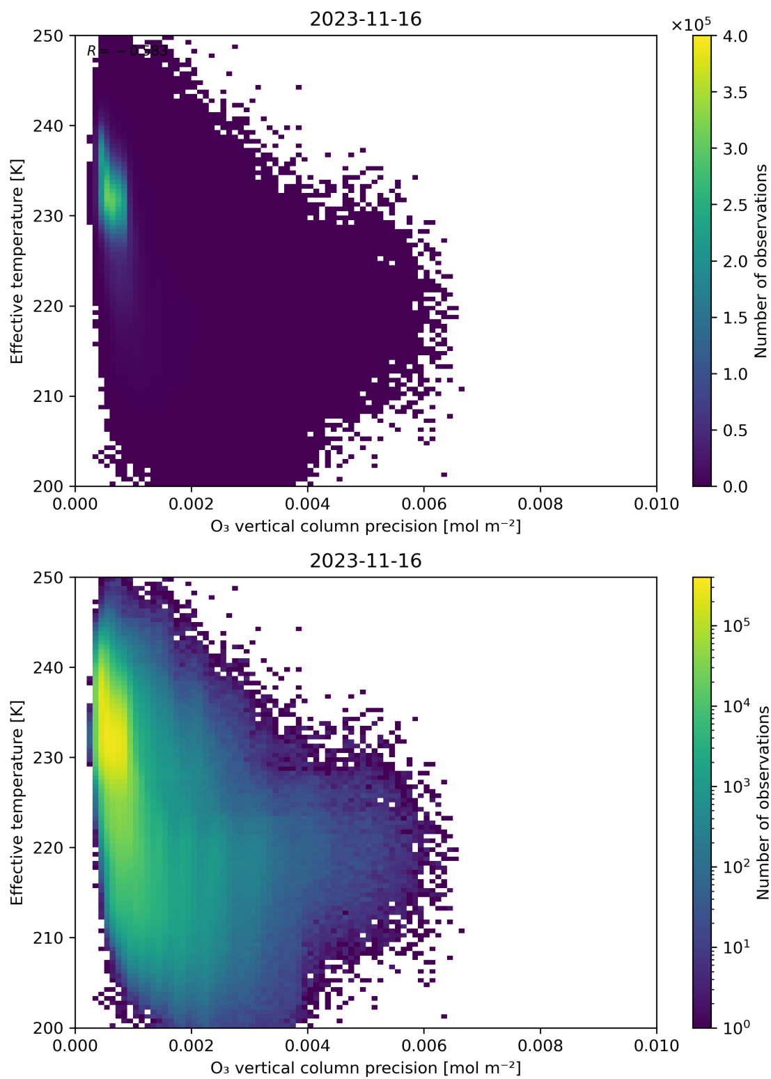
Figure 42: Scatter density plot of “O 3 vertical column precision” against “Effective temperature” for 2023-11-15 to 2023-11-17.
