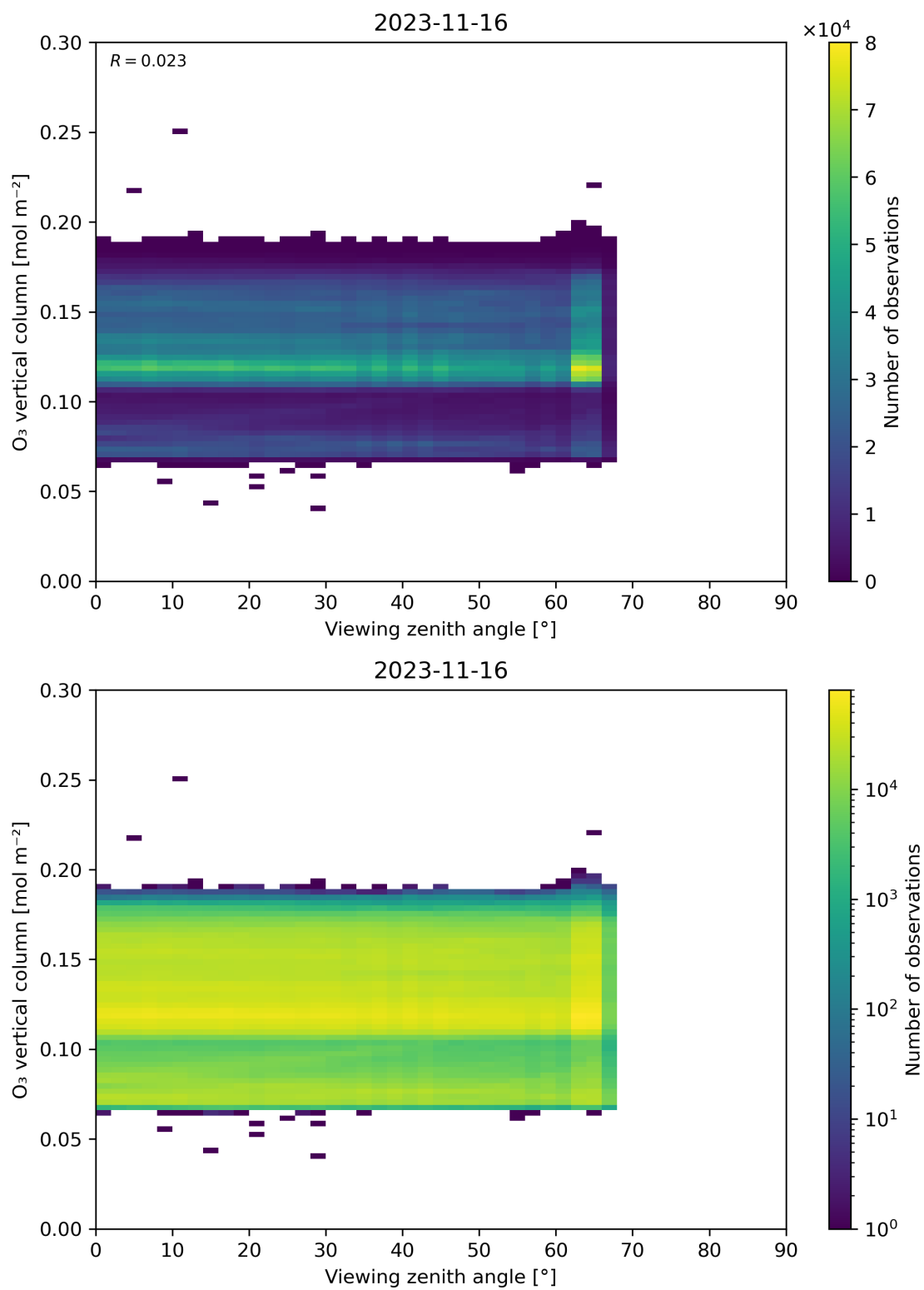
Figure 52: Scatter density plot of “Viewing zenith angle” against “O 3 vertical column” for 2023-11-15 to 2023-11-17.
