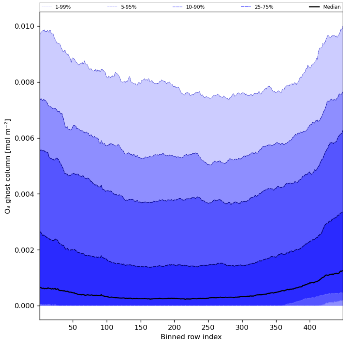
Figure 32: Along track statistics of "O 3 ghost column" for 2023-11-15 to 2023-11-17
