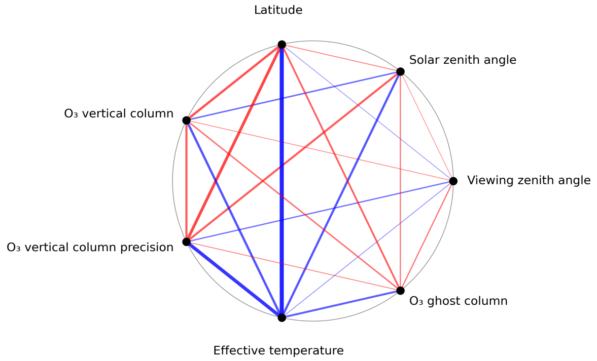
Figure 1: Map of correlation graph for 2023-11-15 to 2023-11-17.
