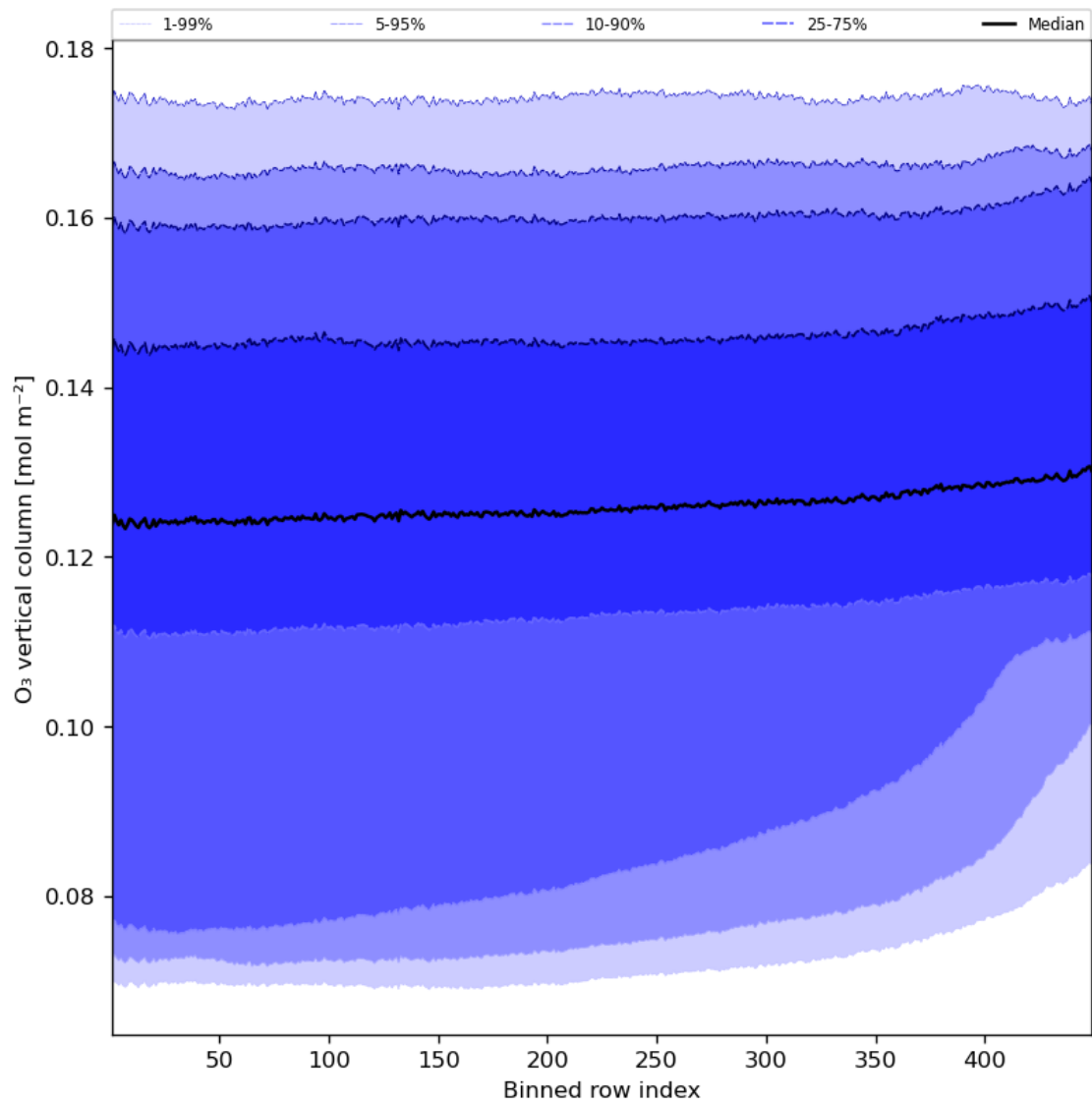
Figure 28: Along track statistics of “O 3 vertical column” for 2023-11-15 to 2023-11-17
