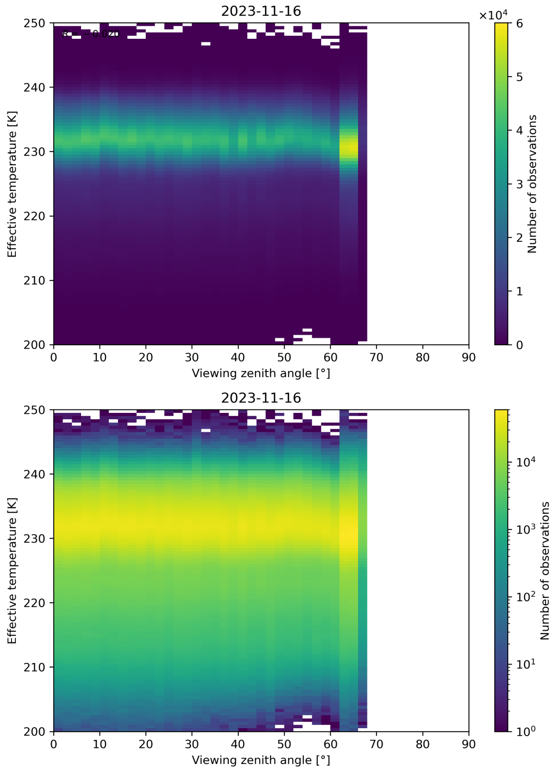
Figure 50: Scatter density plot of “Viewing zenith angle” against “Effective temperature” for 2023-11-15 to 2023-11-17.
