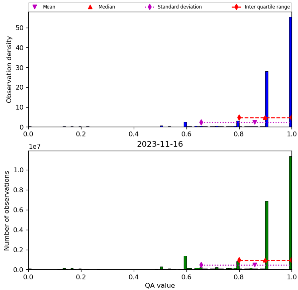
Figure 20: Histogram of “QA value” for 2023-11-15 to 2023-11-17
