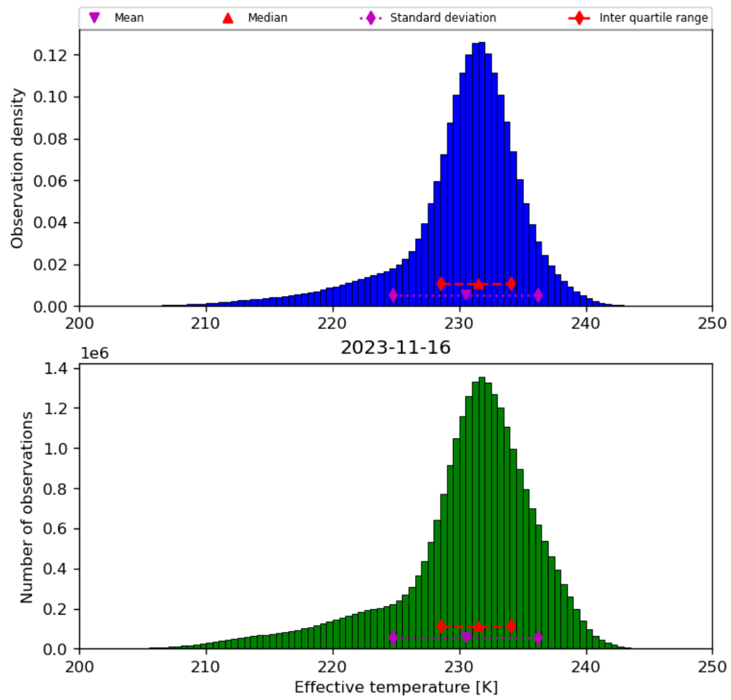
Figure 24: Histogram of “Effective temperature” for 2023-11-15 to 2023-11-17
