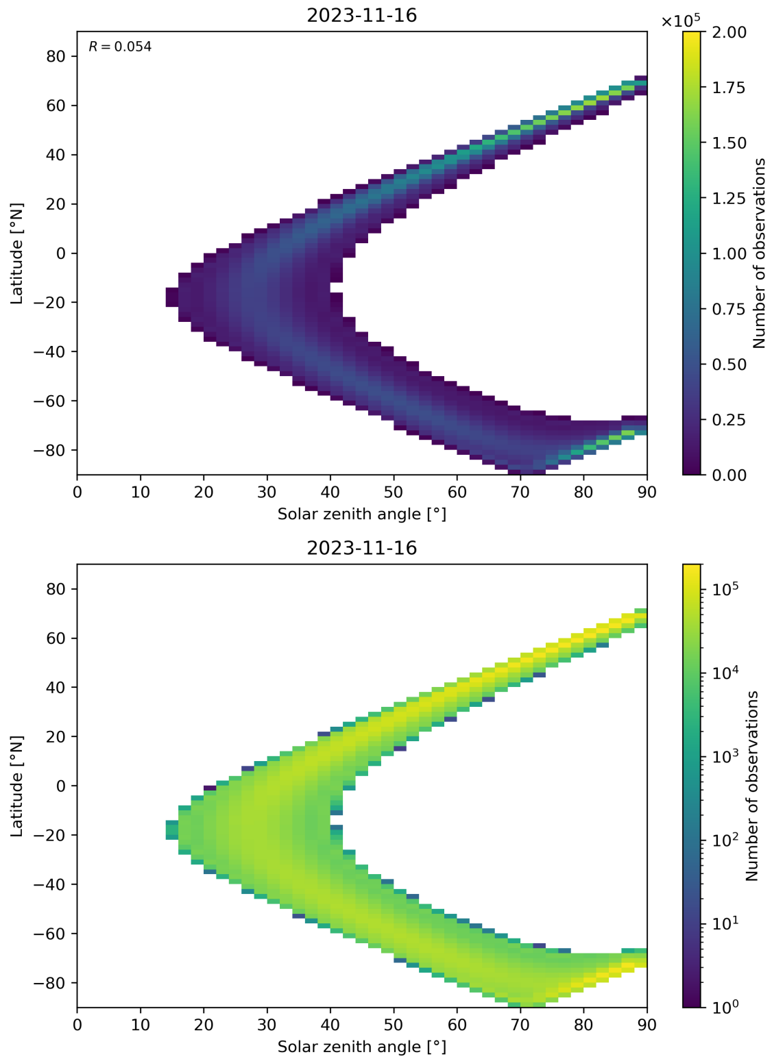
Figure 44: Scatter density plot of “Solar zenith angle” against “Latitude” for 2023-11-15 to 2023-11-17.
