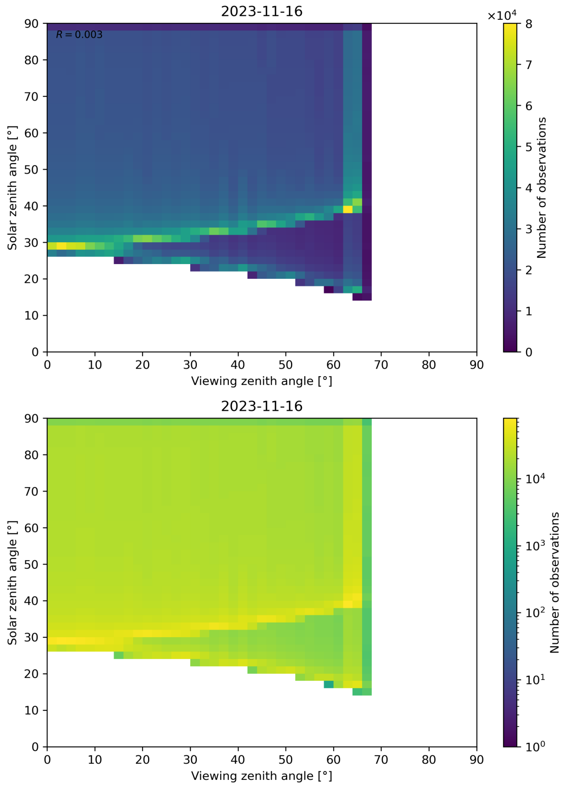
Figure 54: Scatter density plot of “Viewing zenith angle” against “Solar zenith angle” for 2023-11-15 to 2023-11-17.
