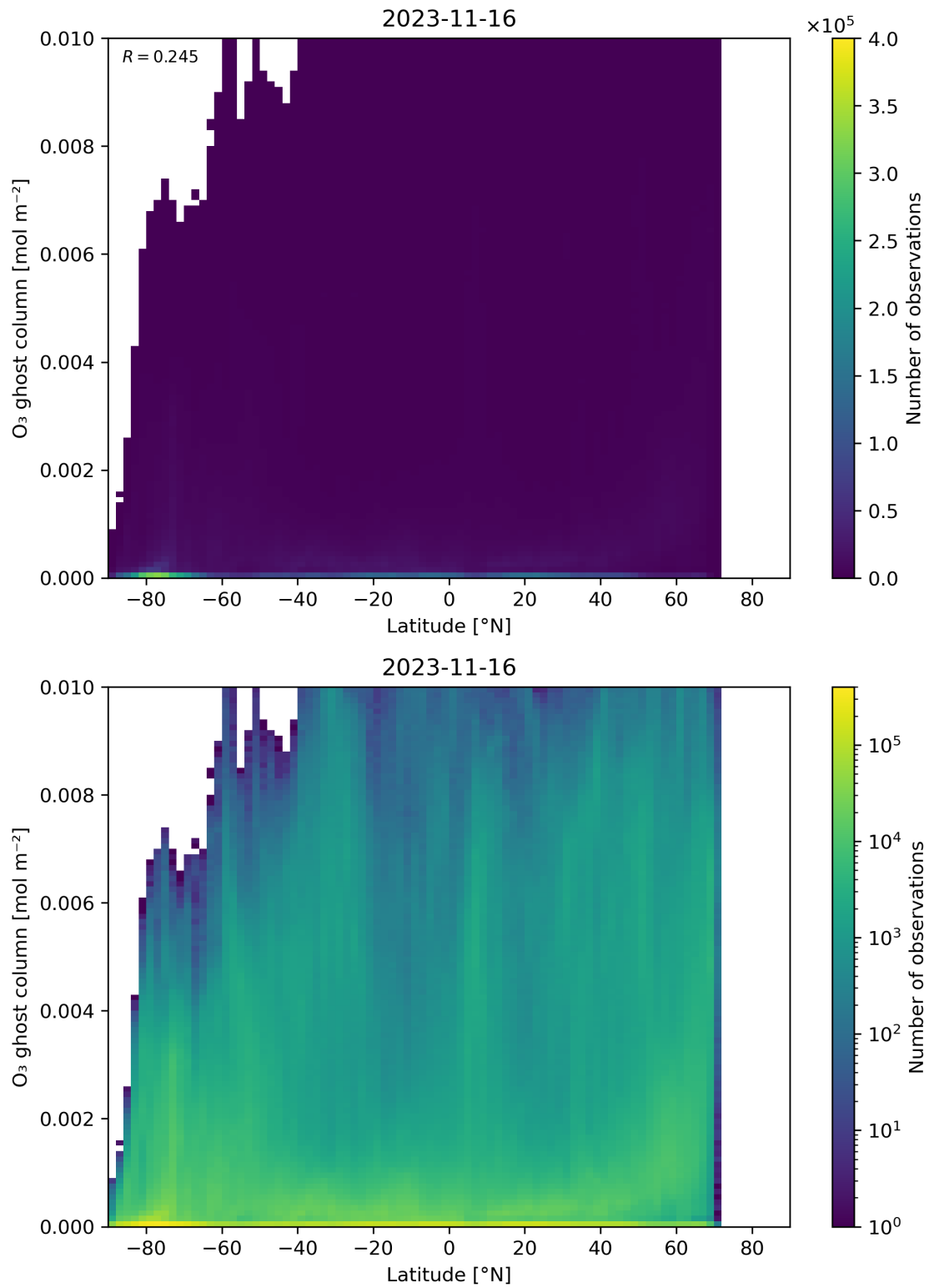
Figure 35: Scatter density plot of “Latitude” against “O 3 ghost column” for 2023-11-15 to 2023-11-17.
