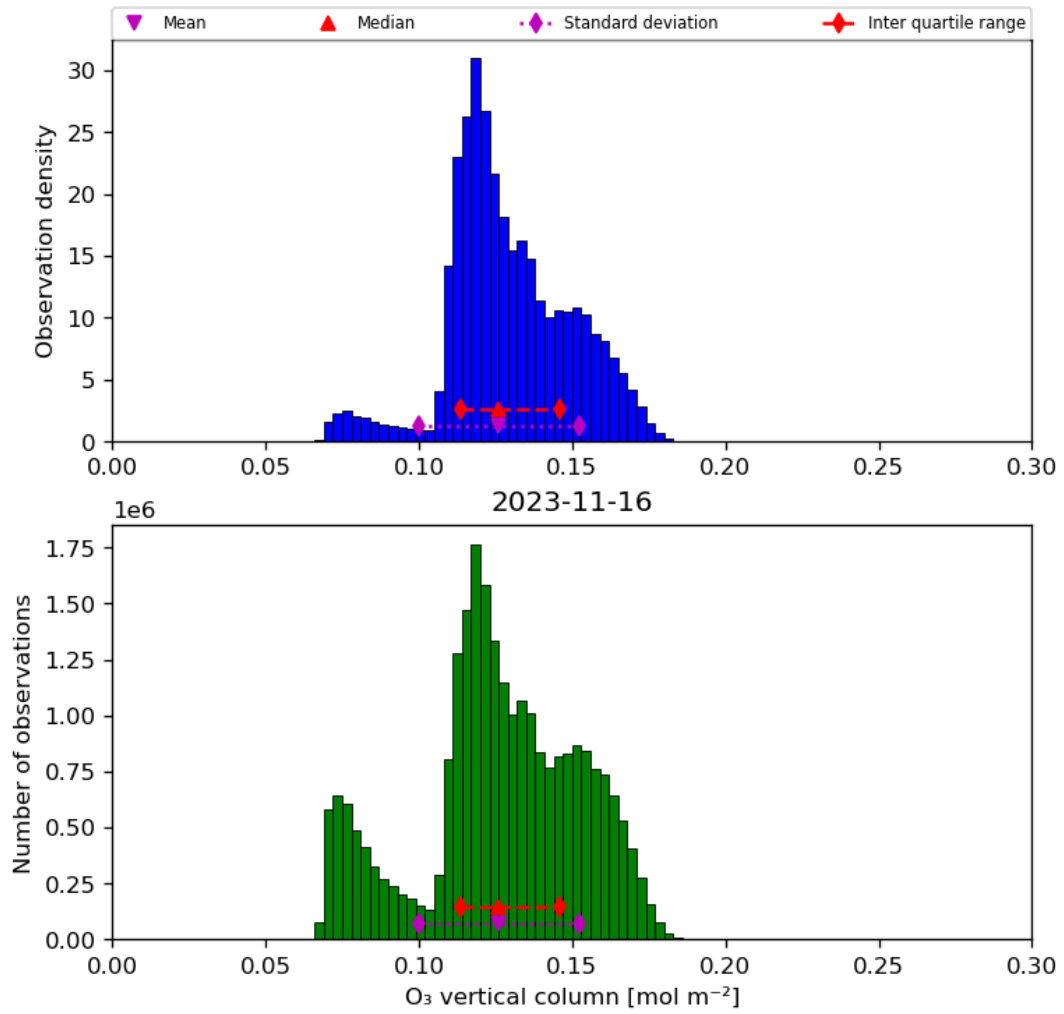
Figure 21: Histogram of “O 3 vertical column” for 2023-11-15 to 2023-11-17
