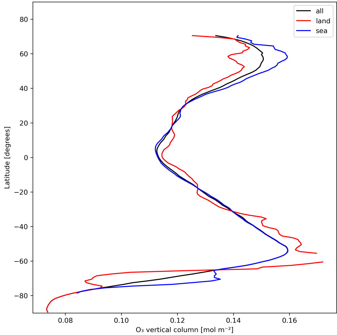
Figure 14: Zonal average of “O 3 vertical column” for 2023-11-15 to 2023-11-17.
