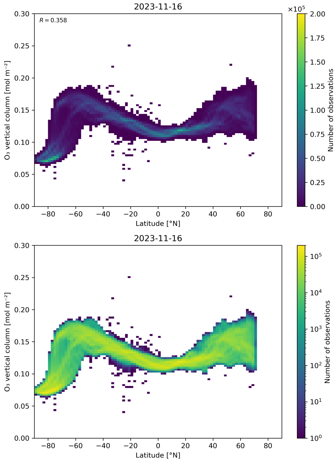
Figure 36: Scatter density plot of “Latitude” against “O 3 vertical column” for 2023-11-15 to 2023-11-17.
