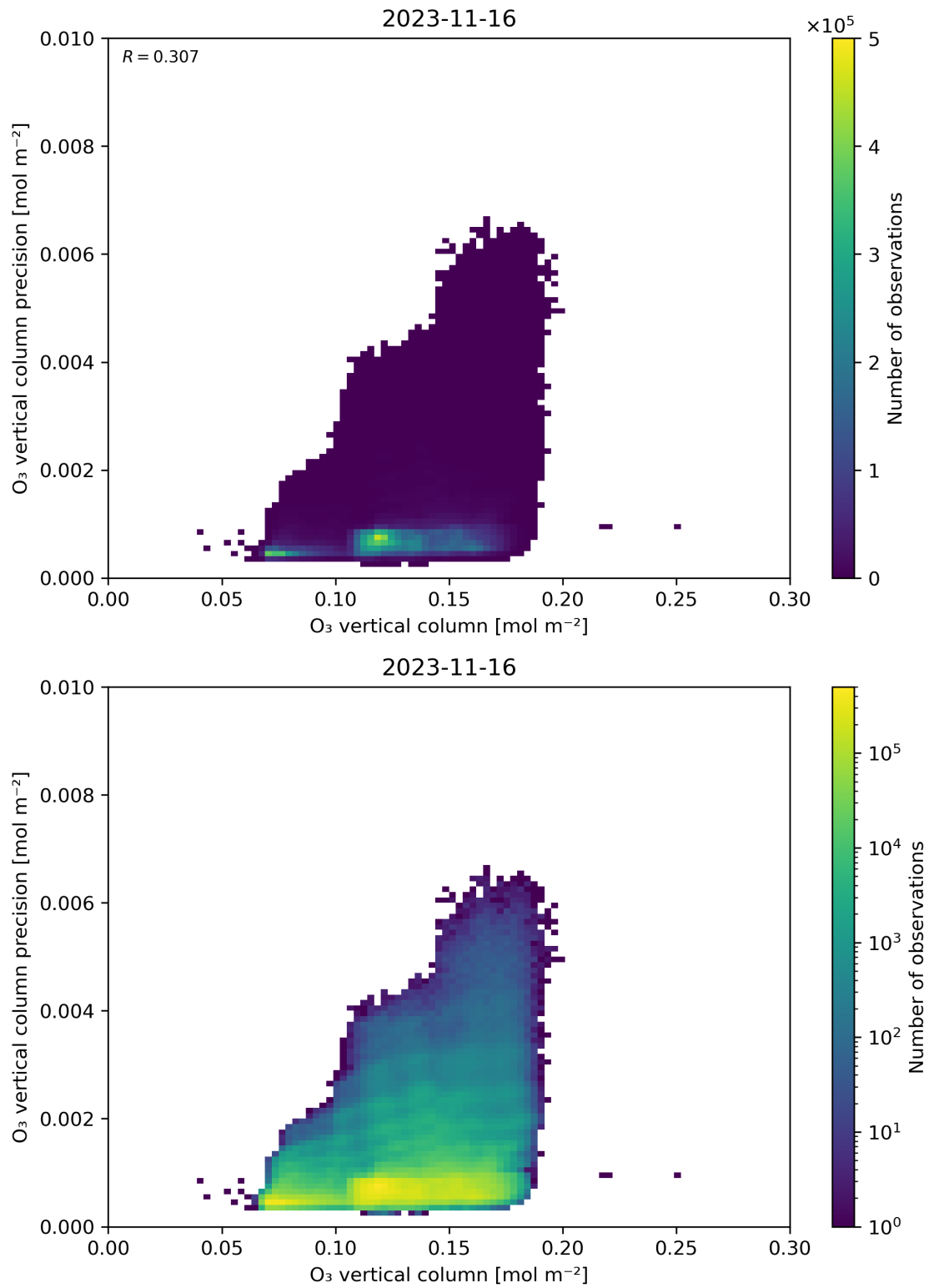
Figure 41: Scatter density plot of “O 3 vertical column” against “O 3 vertical column precision” for 2023-11-15 to 2023-11-17.
