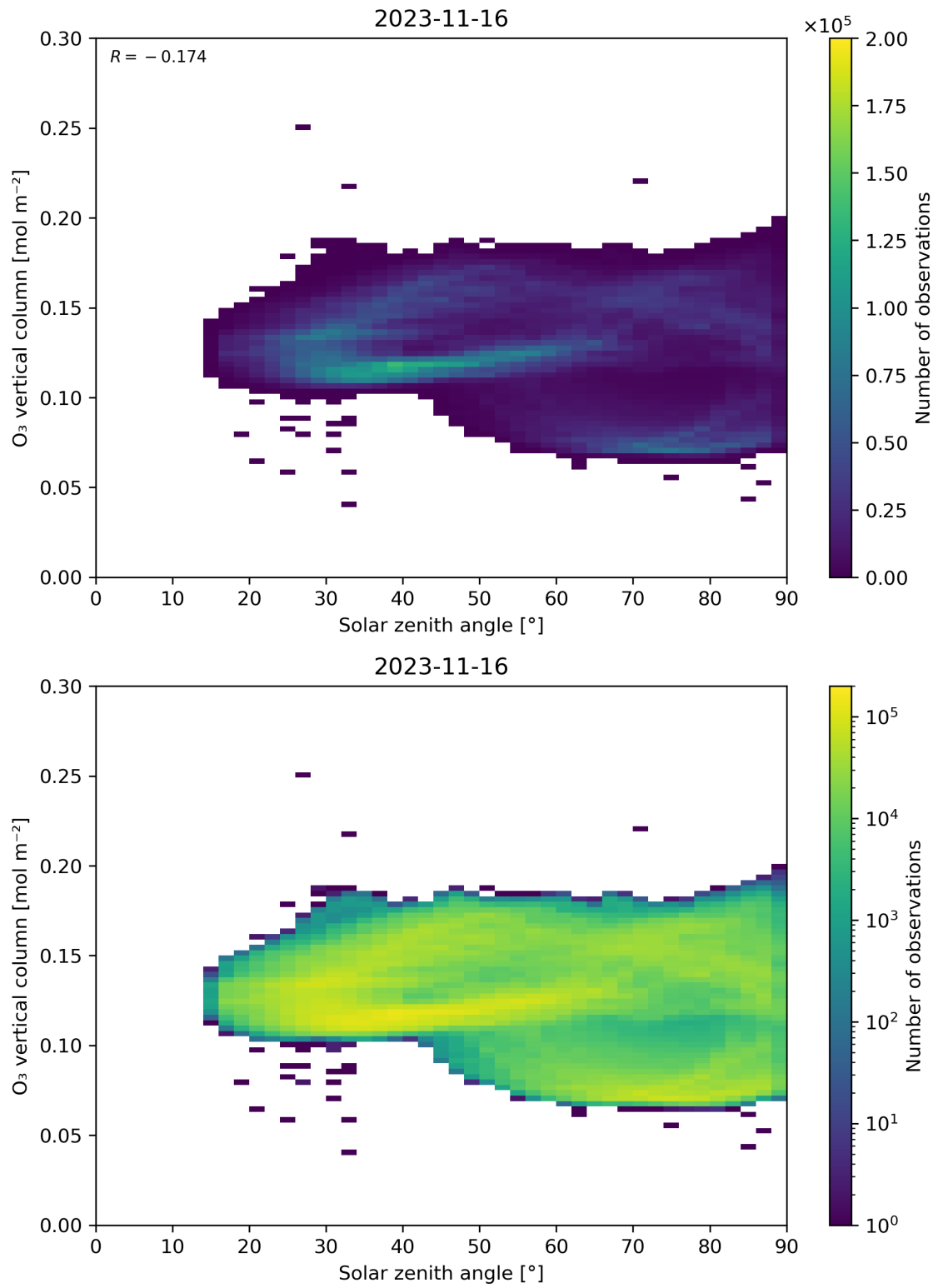
Figure 47: Scatter density plot of “Solar zenith angle” against “O 3 vertical column” for 2023-11-15 to 2023-11-17.
