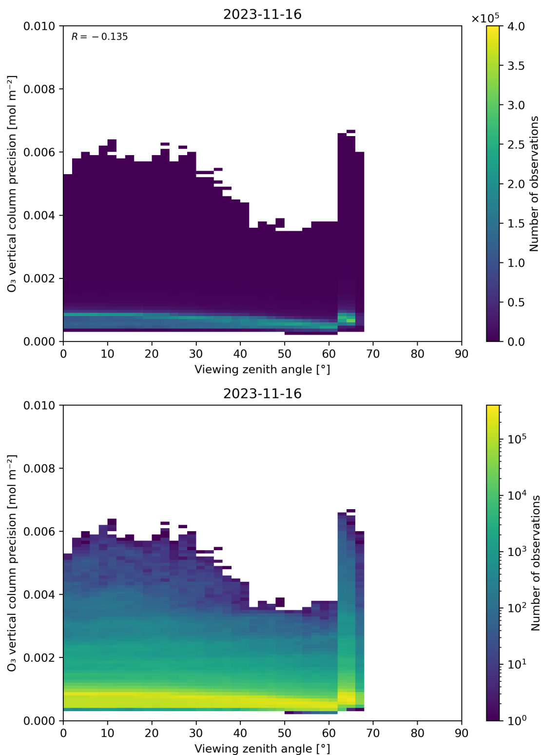
Figure 53: Scatter density plot of “Viewing zenith angle” against “O 3 vertical column precision” for 2023-11-15 to 2023-11-17.
