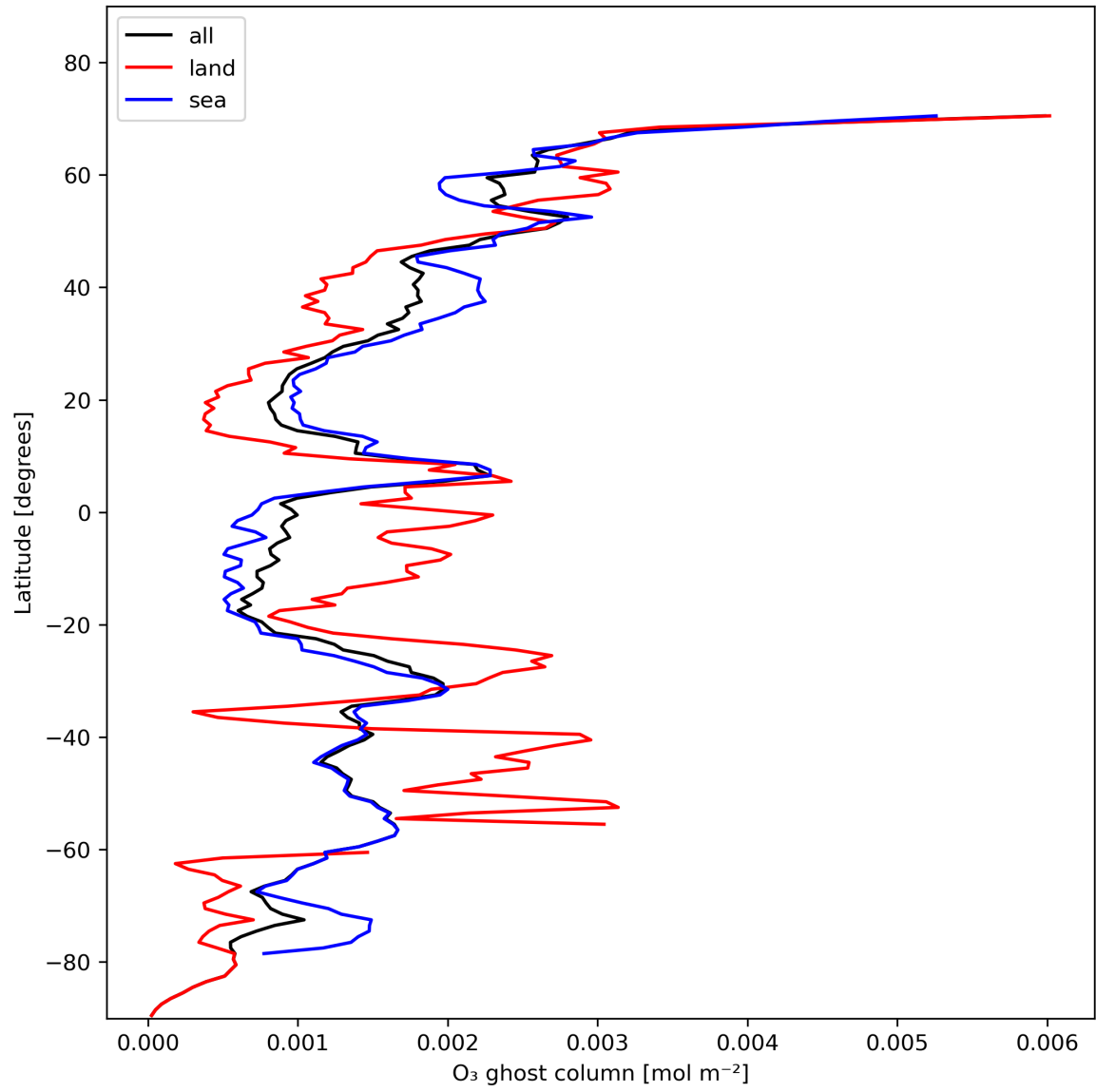
Figure 18: Zonal average of “O 3 ghost column” for 2023-11-15 to 2023-11-17.
