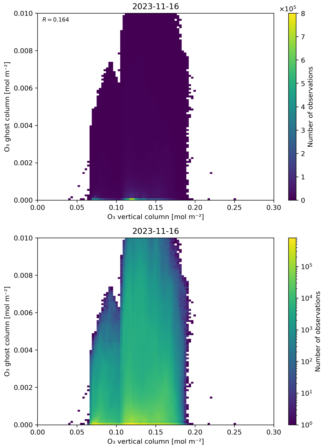
Figure 40: Scatter density plot of “O 3 vertical column” against “O 3 ghost column” for 2023-11-15 to 2023-11-17.
