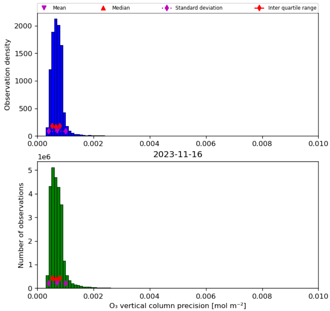
Figure 22: Histogram of “O 3 vertical column precision” for 2023-11-15 to 2023-11-17
