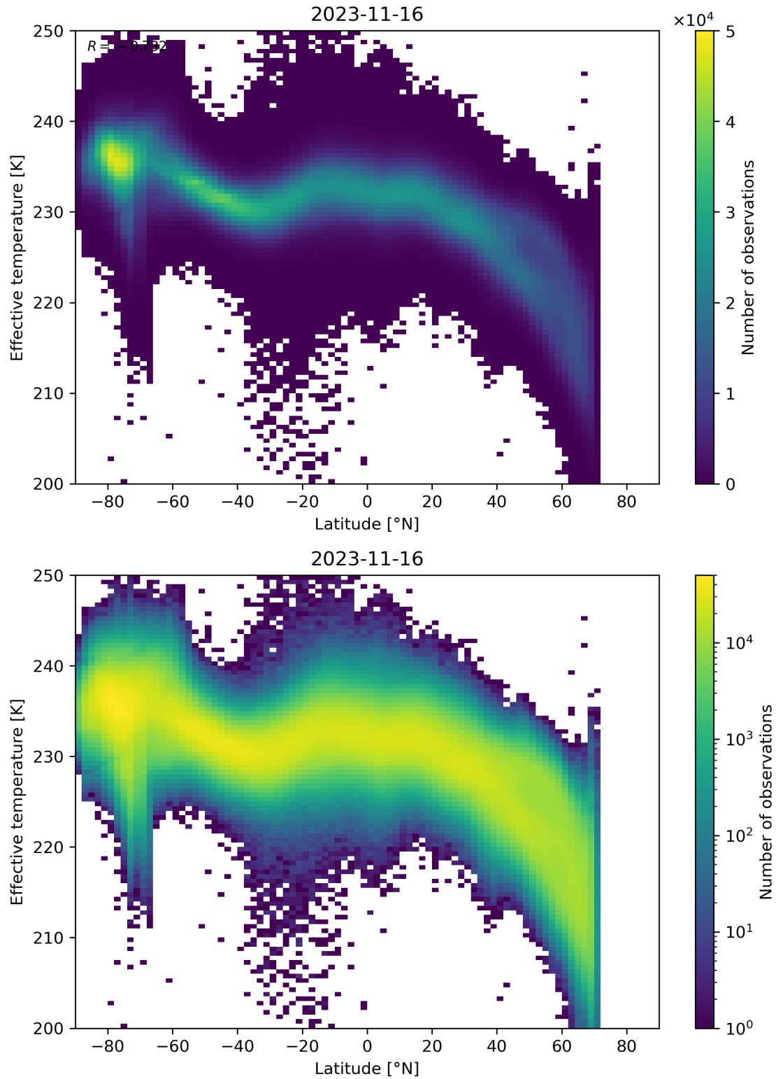
Figure 34: Scatter density plot of “Latitude” against “Effective temperature” for 2023-11-15 to 2023-11-17.
