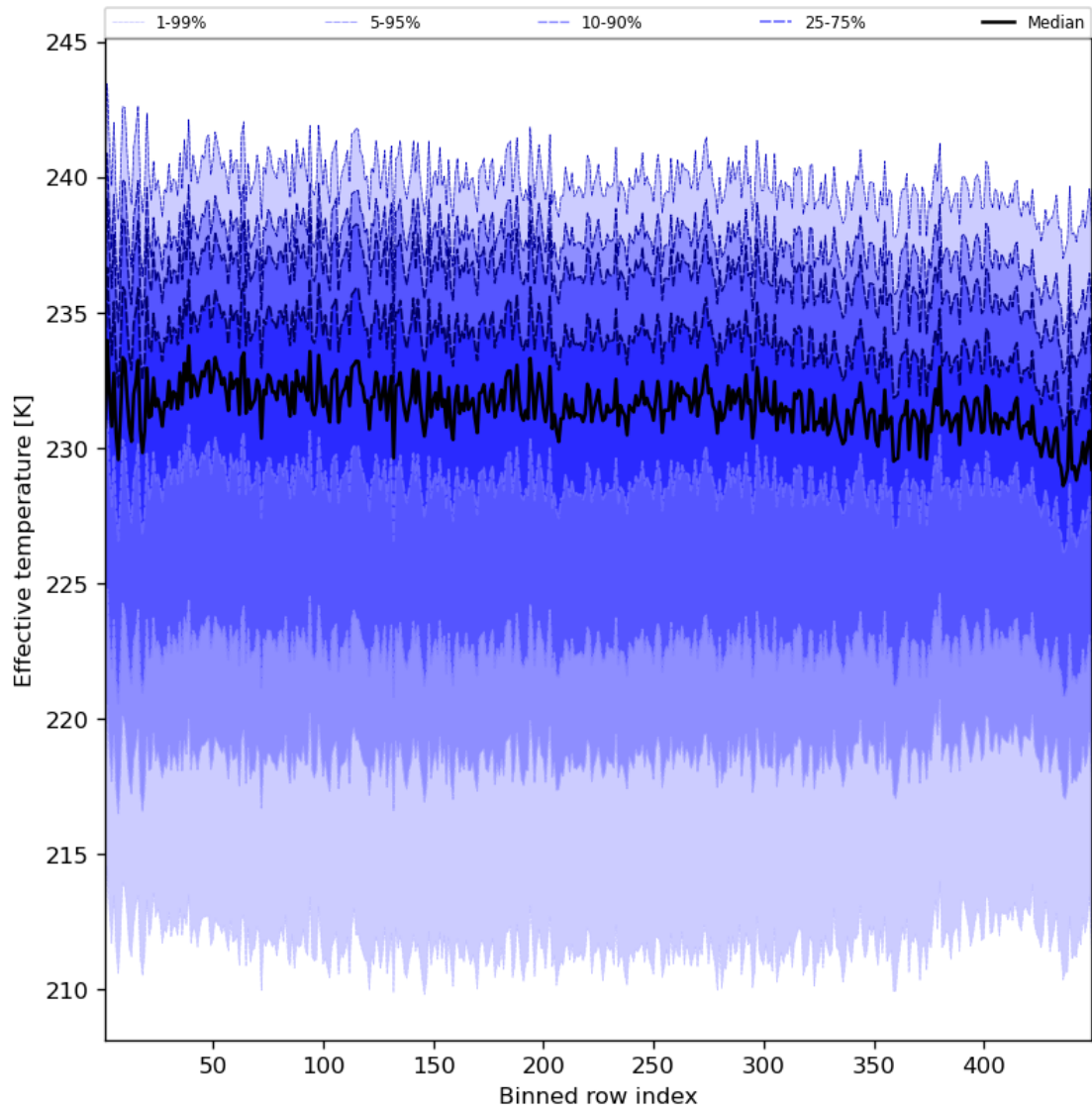
Figure 31: Along track statistics of “Effective temperature” for 2023-11-15 to 2023-11-17
