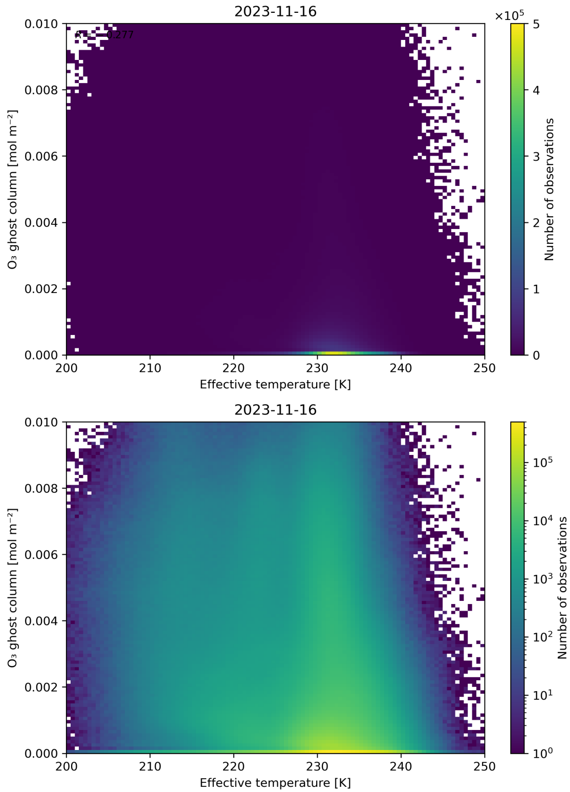
Figure 38: Scatter density plot of “Effective temperature” against “O 3 ghost column” for 2023-11-15 to 2023-11-17.
