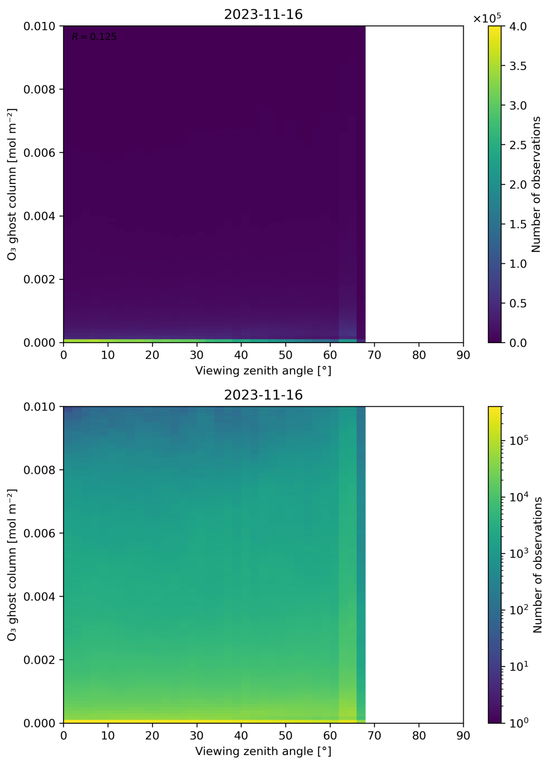
Figure 51: Scatter density plot of “Viewing zenith angle” against “O 3 ghost column” for 2023-11-15 to 2023-11-17.
