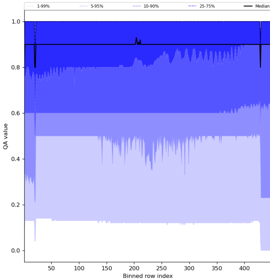
Figure 27: Along track statistics of “QA value” for 2023-11-15 to 2023-11-17
