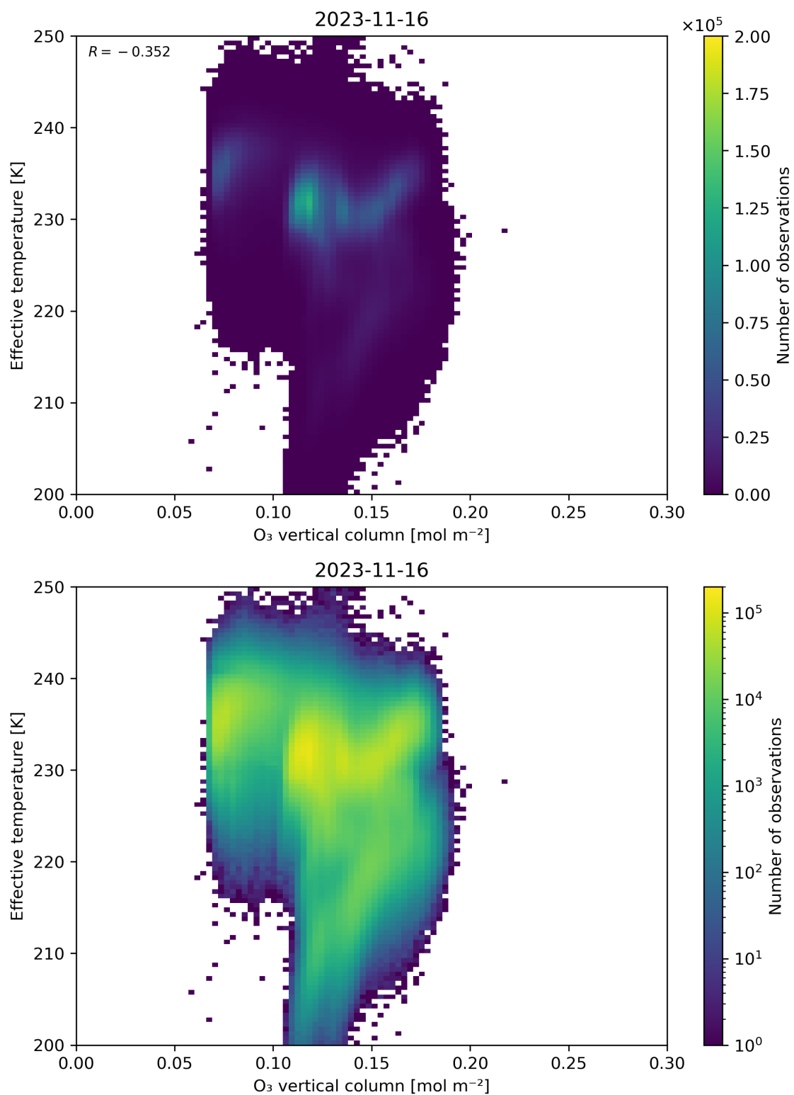
Figure 39: Scatter density plot of “O 3 vertical column” against “Effective temperature” for 2023-11-15 to 2023-11-17.
