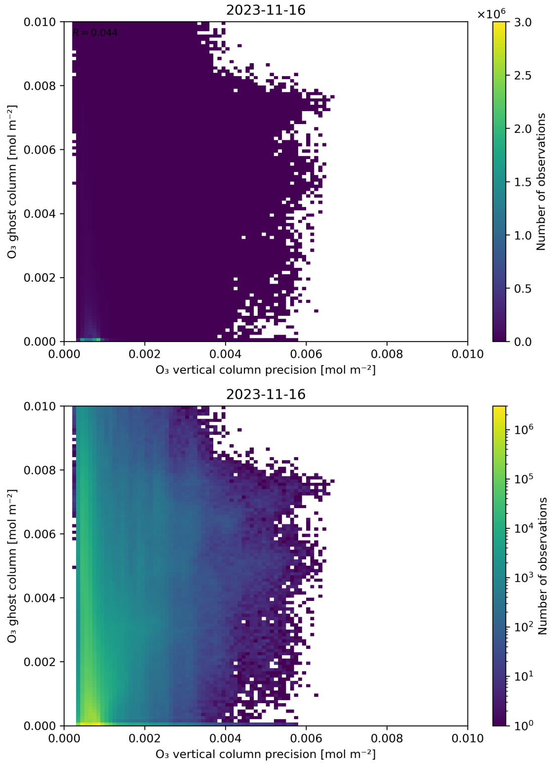
Figure 43: Scatter density plot of “ O_3 vertical column precision” against “ O_3 ghost column” for 2023-11-15 to 2023-11-17.
