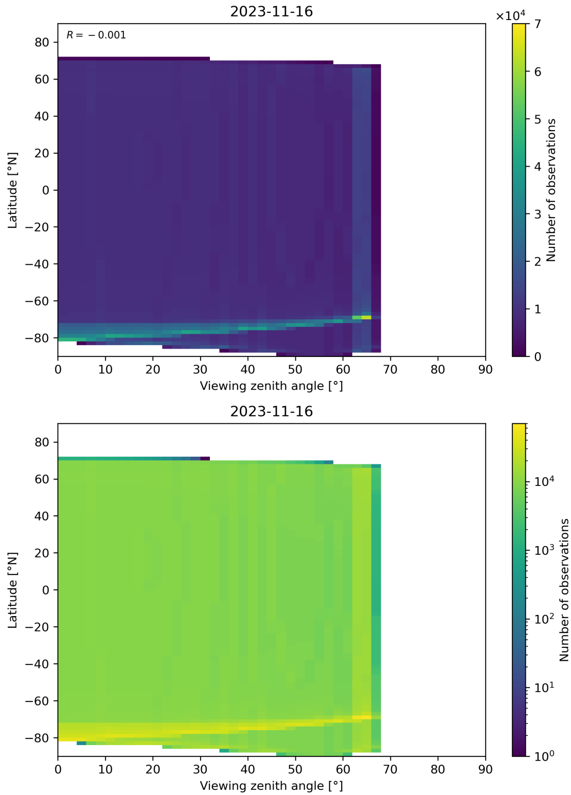
Figure 49: Scatter density plot of “Viewing zenith angle” against “Latitude” for 2023-11-15 to 2023-11-17.
