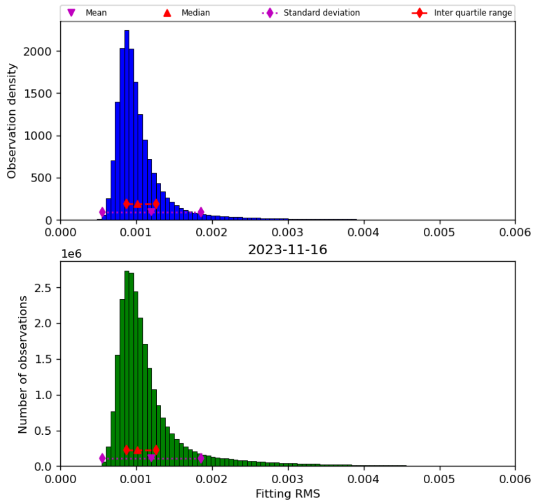
Figure 23: Histogram of “Fitting RMS” for 2023-11-15 to 2023-11-17
