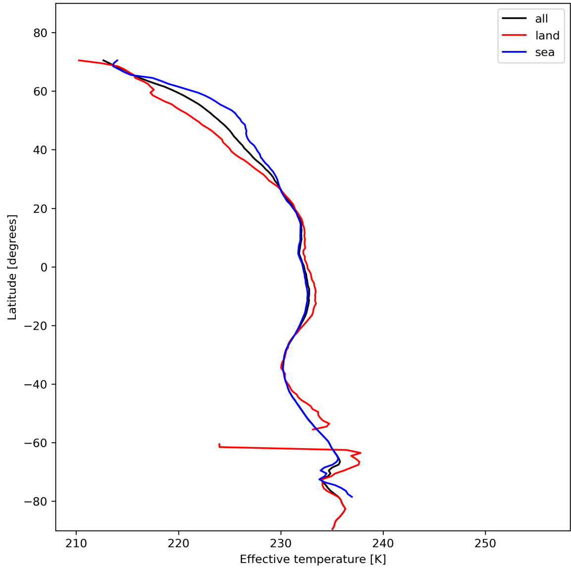
Figure 17: Zonal average of “Effective temperature” for 2023-11-15 to 2023-11-17.
