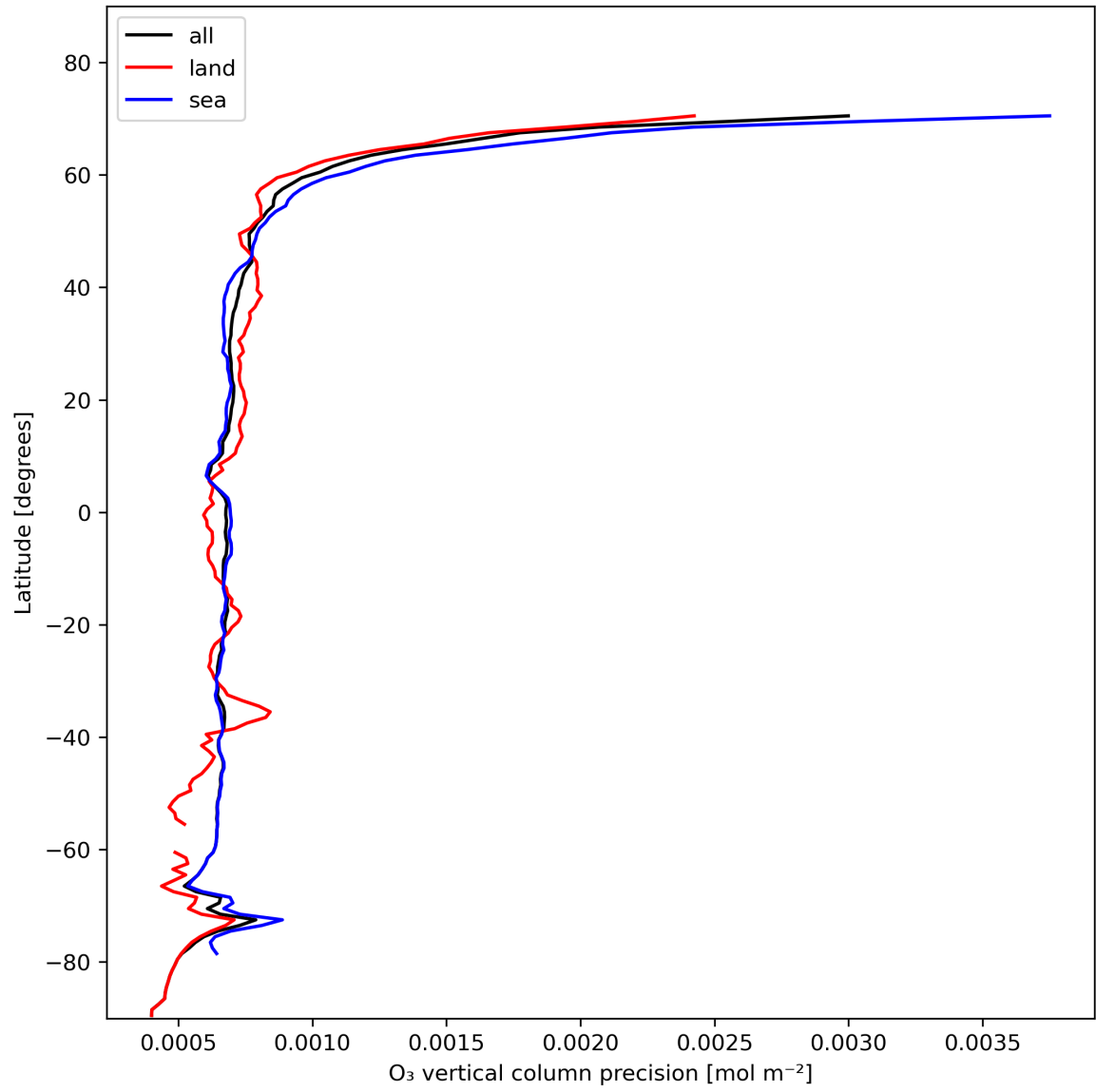
Figure 15: Zonal average of “O 3 vertical column precision” for 2023-11-15 to 2023-11-17.
