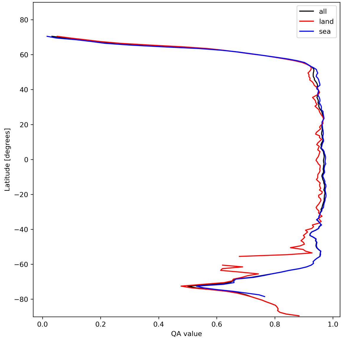
Figure 13: Zonal average of “QA value” for 2023-11-15 to 2023-11-17.
