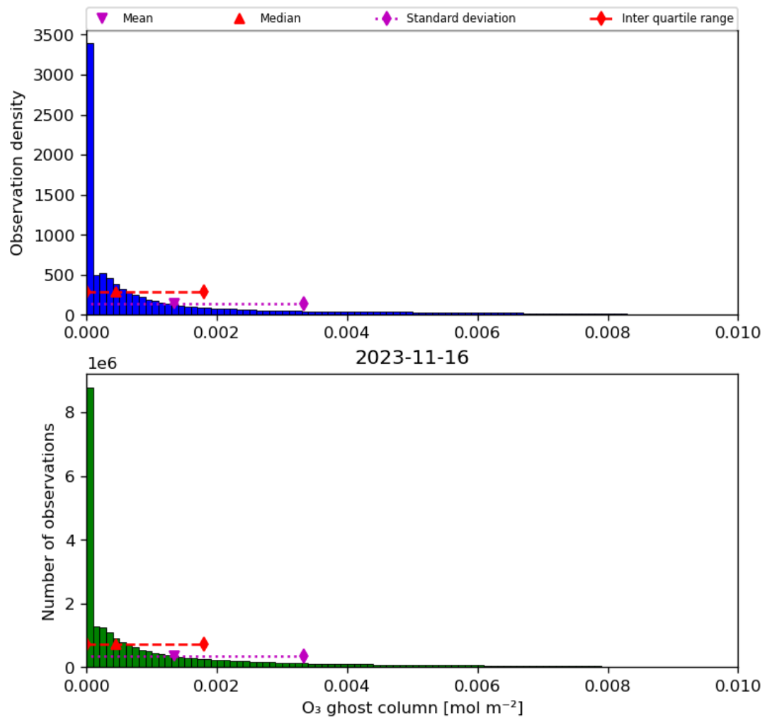
Figure 25: Histogram of "O 3 ghost column" for 2023-11-15 to 2023-11-17
