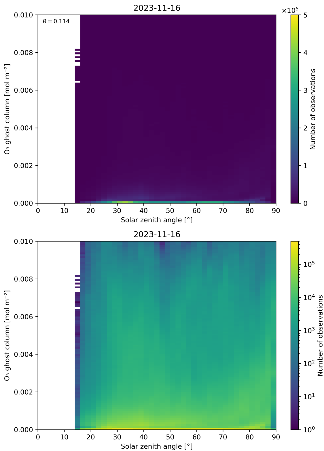
Figure 46: Scatter density plot of “Solar zenith angle” against “O 3 ghost column” for 2023-11-15 to 2023-11-17.
