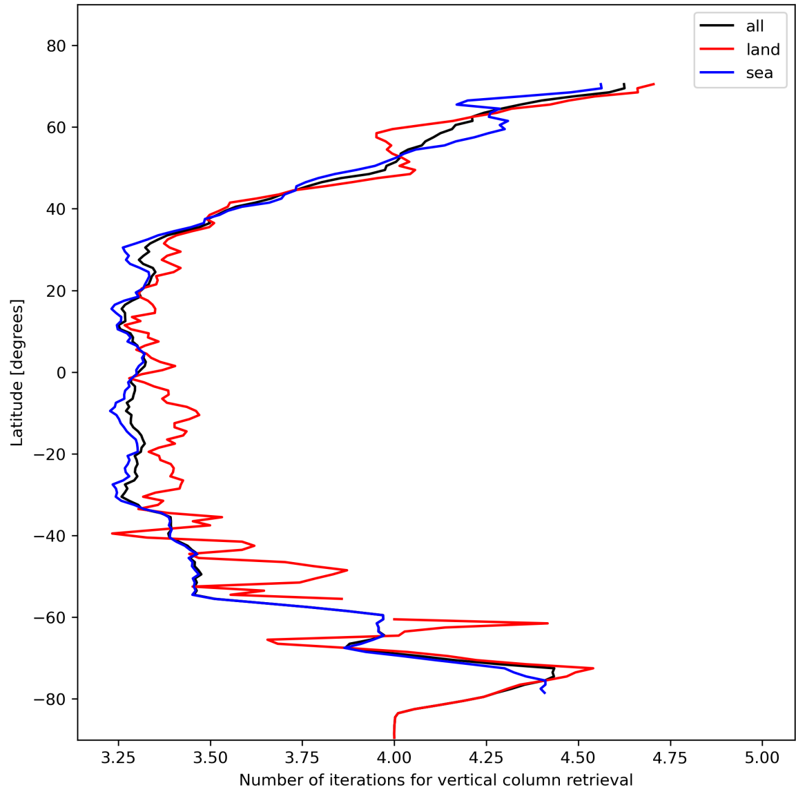
Figure 19: Zonal average of “Number of iterations for vertical column retrieval” for 2023-11-15 to 2023-11-17.
