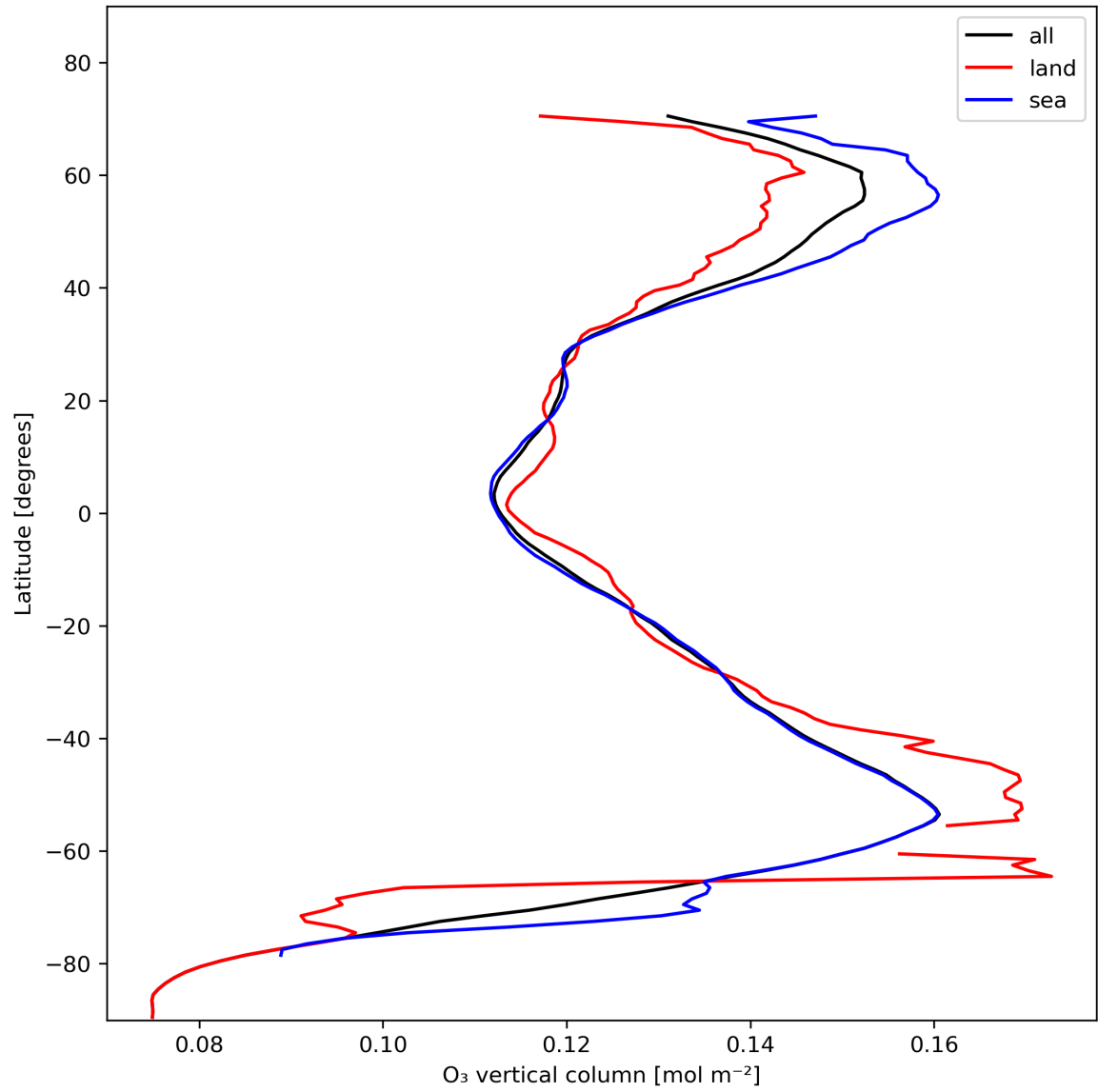
Figure 14: Zonal average of “O 3 vertical column” for 2023-11-16 to 2023-11-18.
