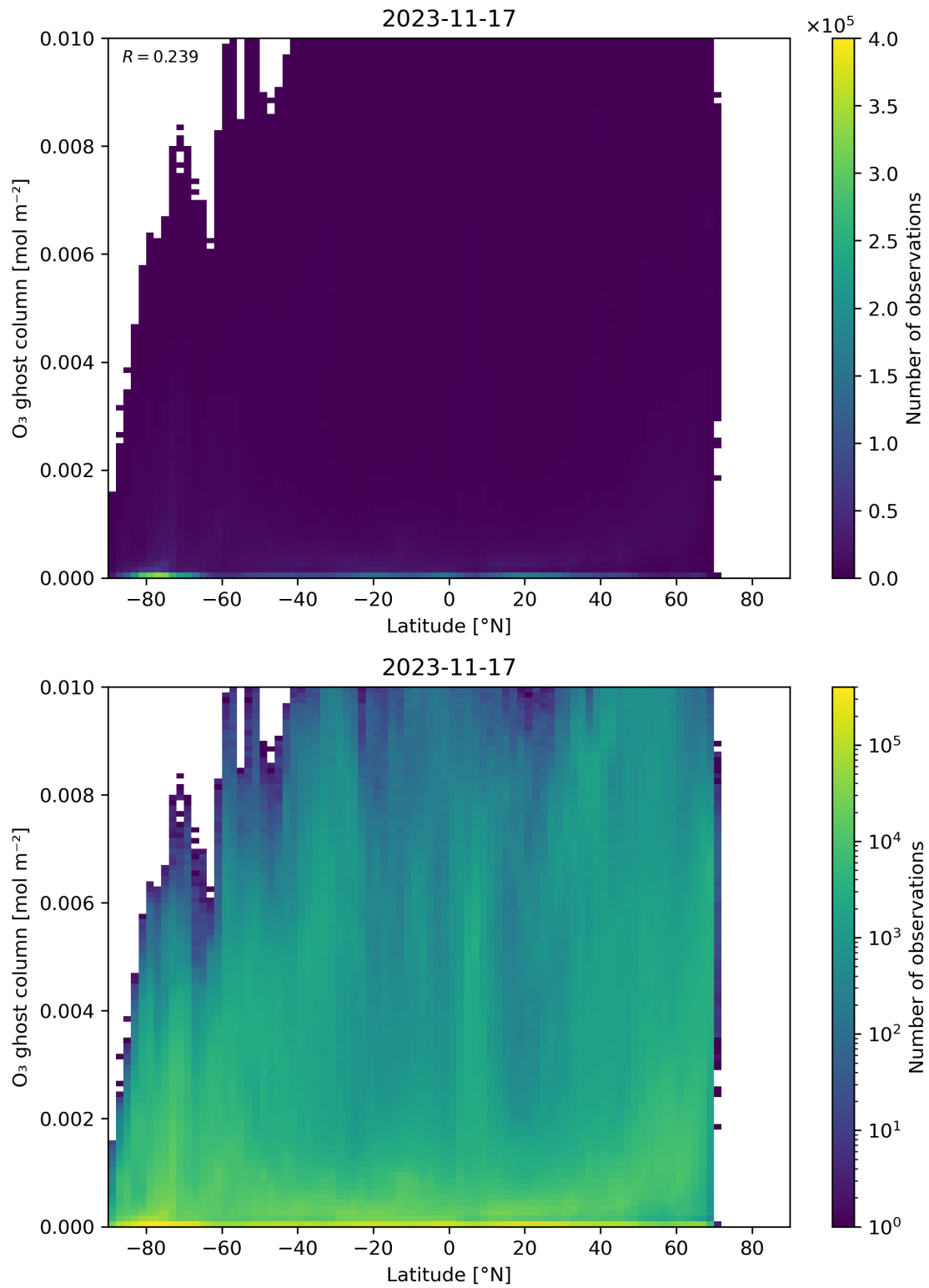
Figure 35: Scatter density plot of “Latitude” against “O 3 ghost column” for 2023-11-16 to 2023-11-18.
