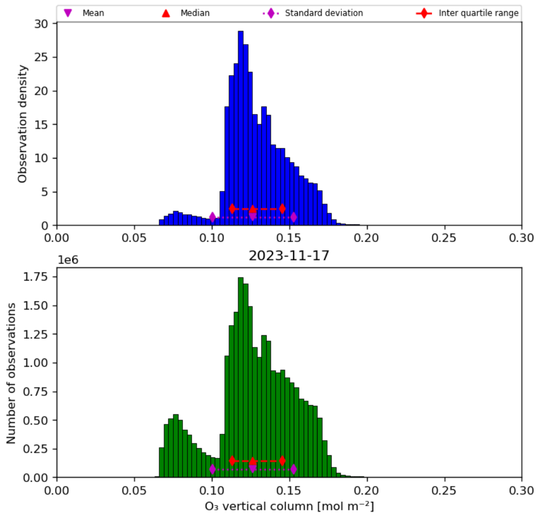
Figure 21: Histogram of “O 3 vertical column” for 2023-11-16 to 2023-11-18
