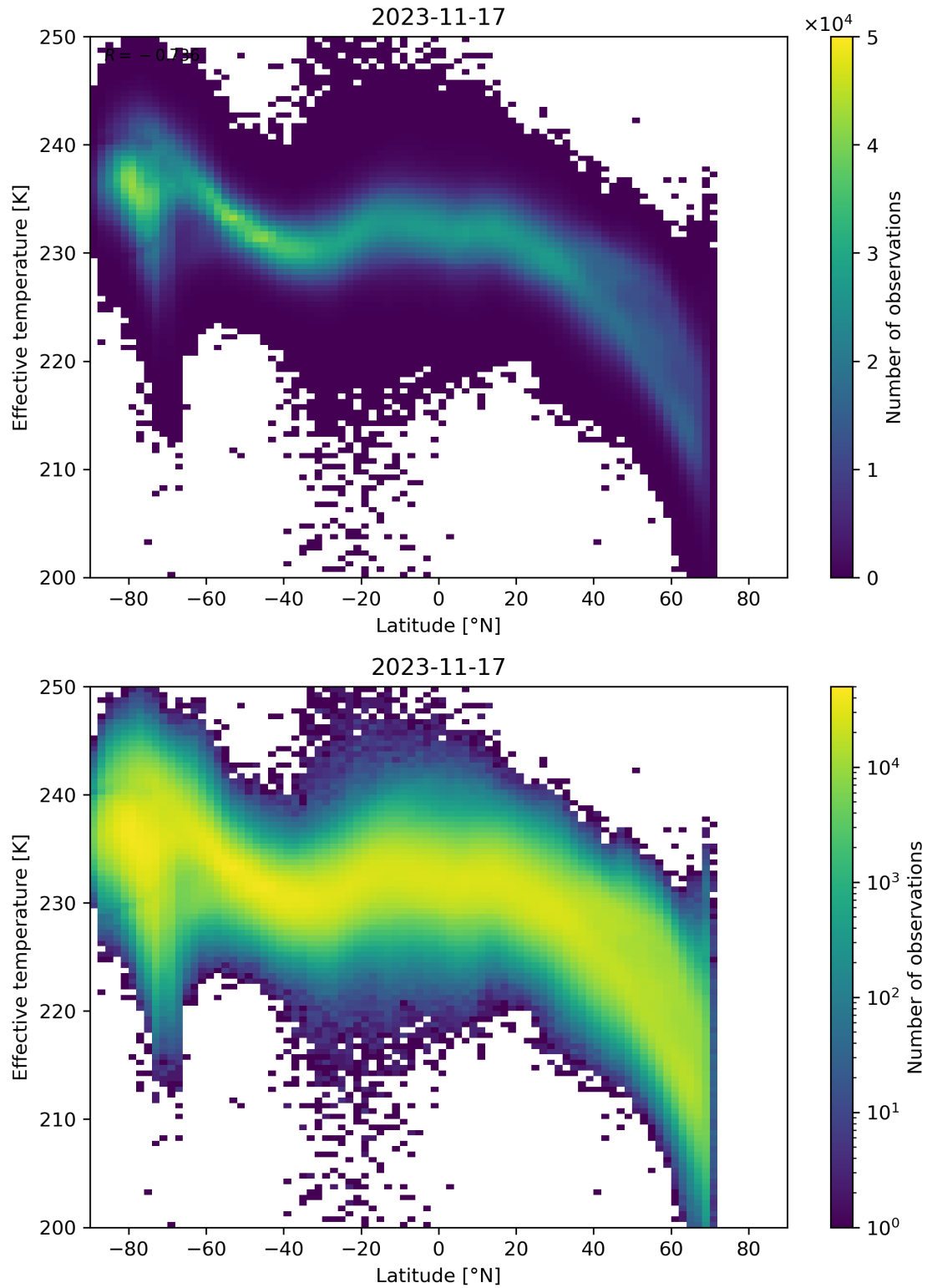
Figure 34: Scatter density plot of “Latitude” against “Effective temperature” for 2023-11-16 to 2023-11-18.
