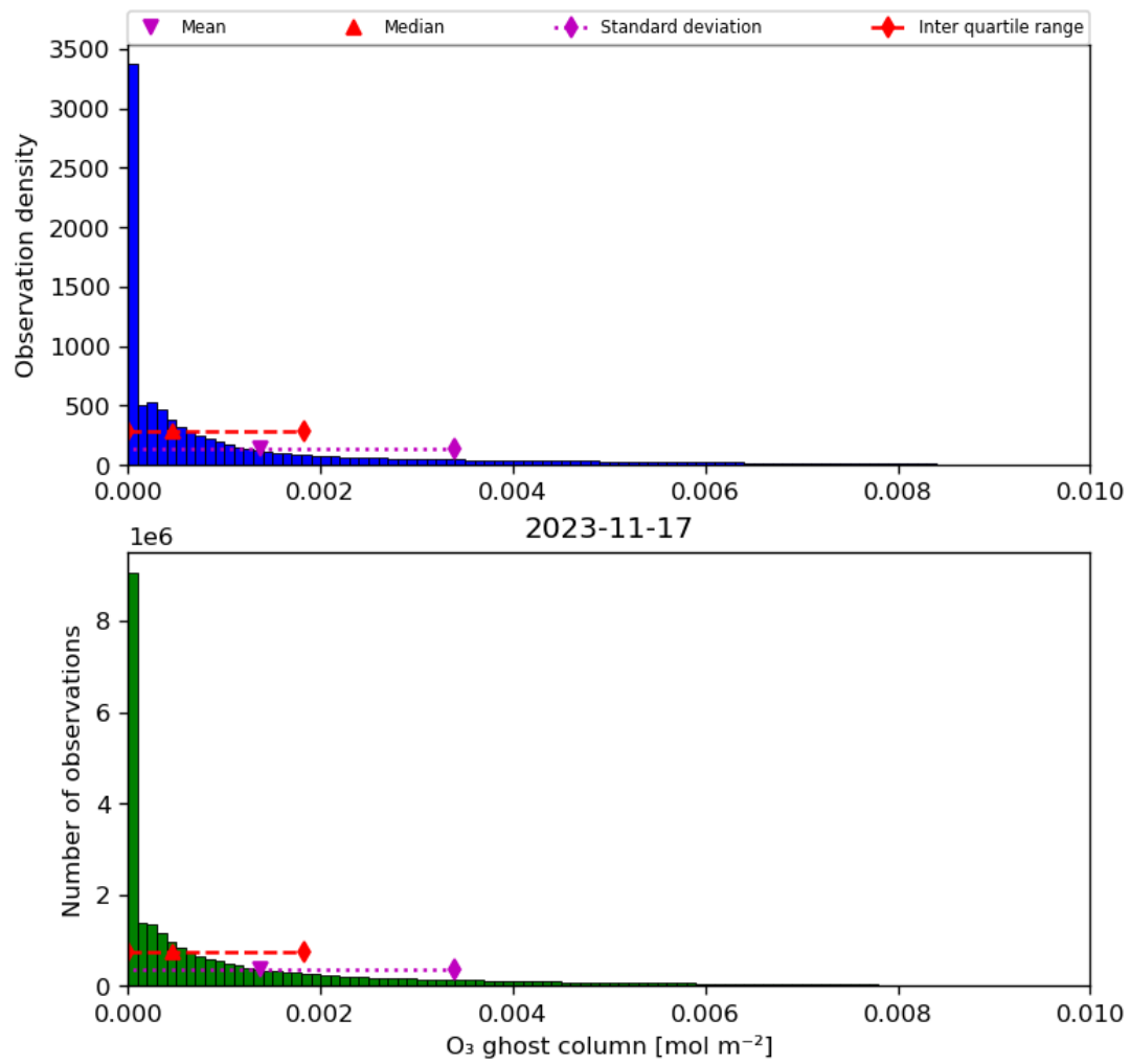
Figure 25: Histogram of “O 3 ghost column” for 2023-11-16 to 2023-11-18
