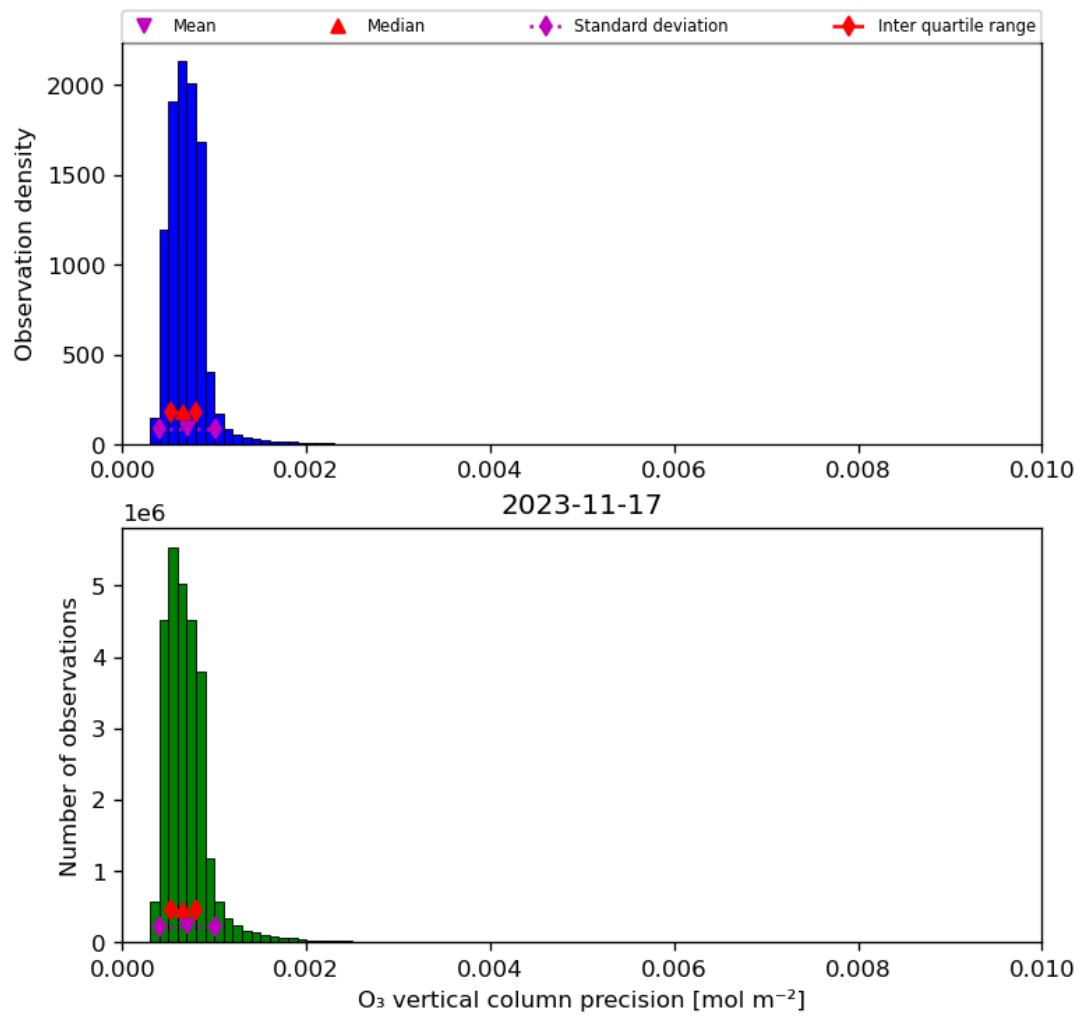
Figure 22: Histogram of “O 3 vertical column precision” for 2023-11-16 to 2023-11-18
