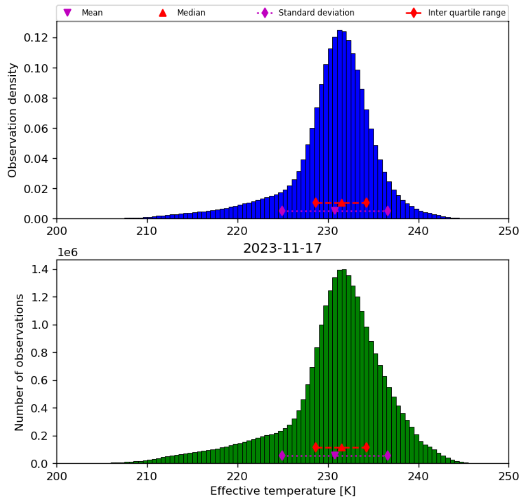
Figure 24: Histogram of “Effective temperature” for 2023-11-16 to 2023-11-18
