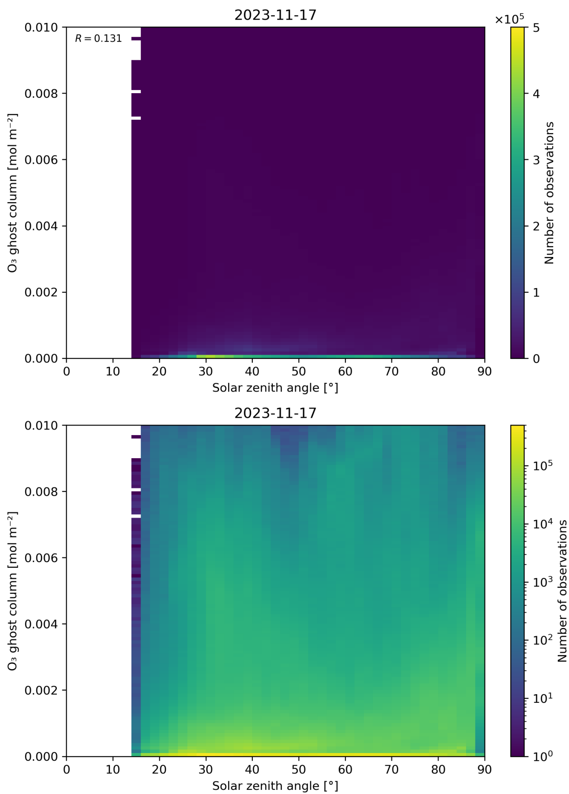
Figure 46: Scatter density plot of “Solar zenith angle” against “O 3 ghost column” for 2023-11-16 to 2023-11-18.
