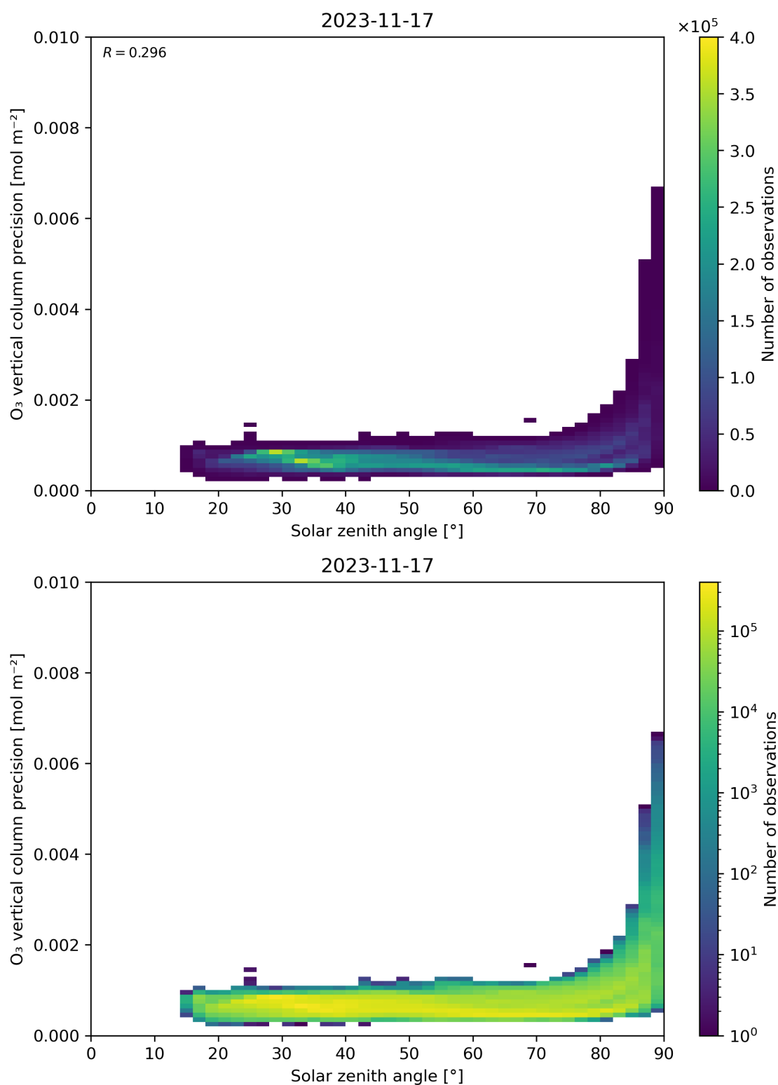
Figure 48: Scatter density plot of “Solar zenith angle” against “O 3 vertical column precision” for 2023-11-16 to 2023-11-18.
