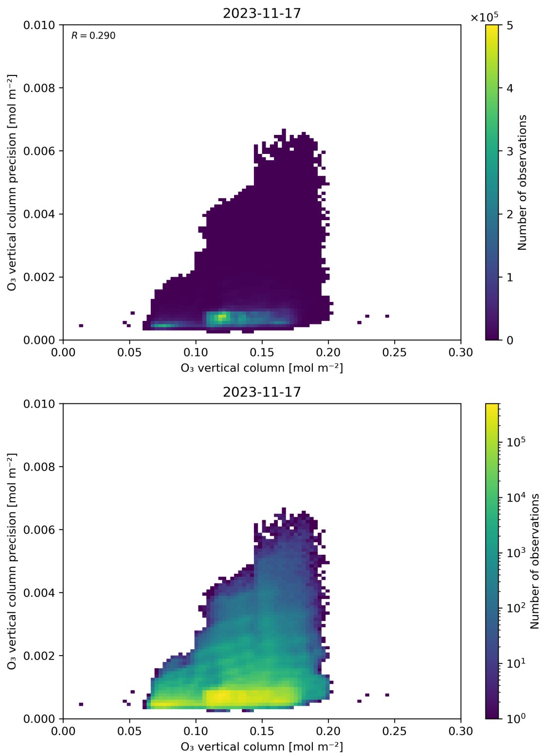
Figure 41: Scatter density plot of “O 3 vertical column” against “O 3 vertical column precision” for 2023-11-16 to 2023-11-18.
