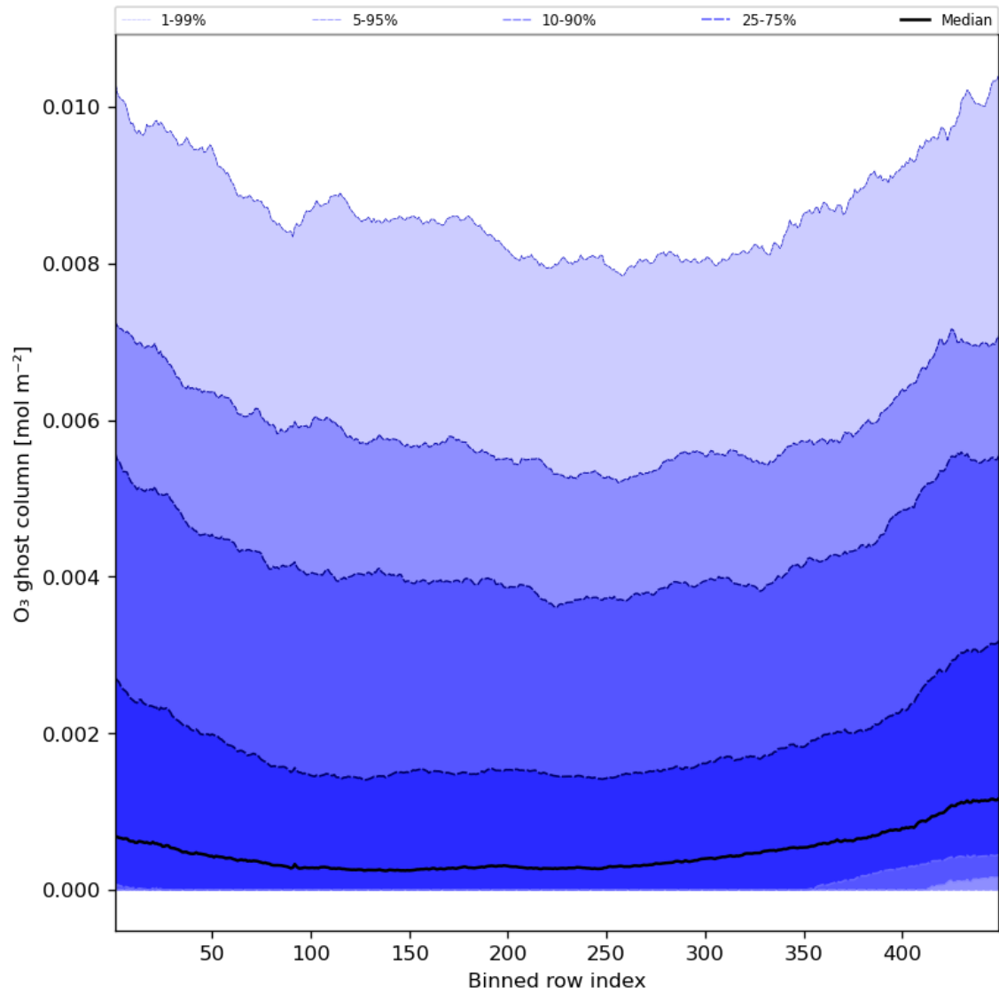
Figure 32: Along track statistics of “O 3 ghost column” for 2023-11-16 to 2023-11-18
