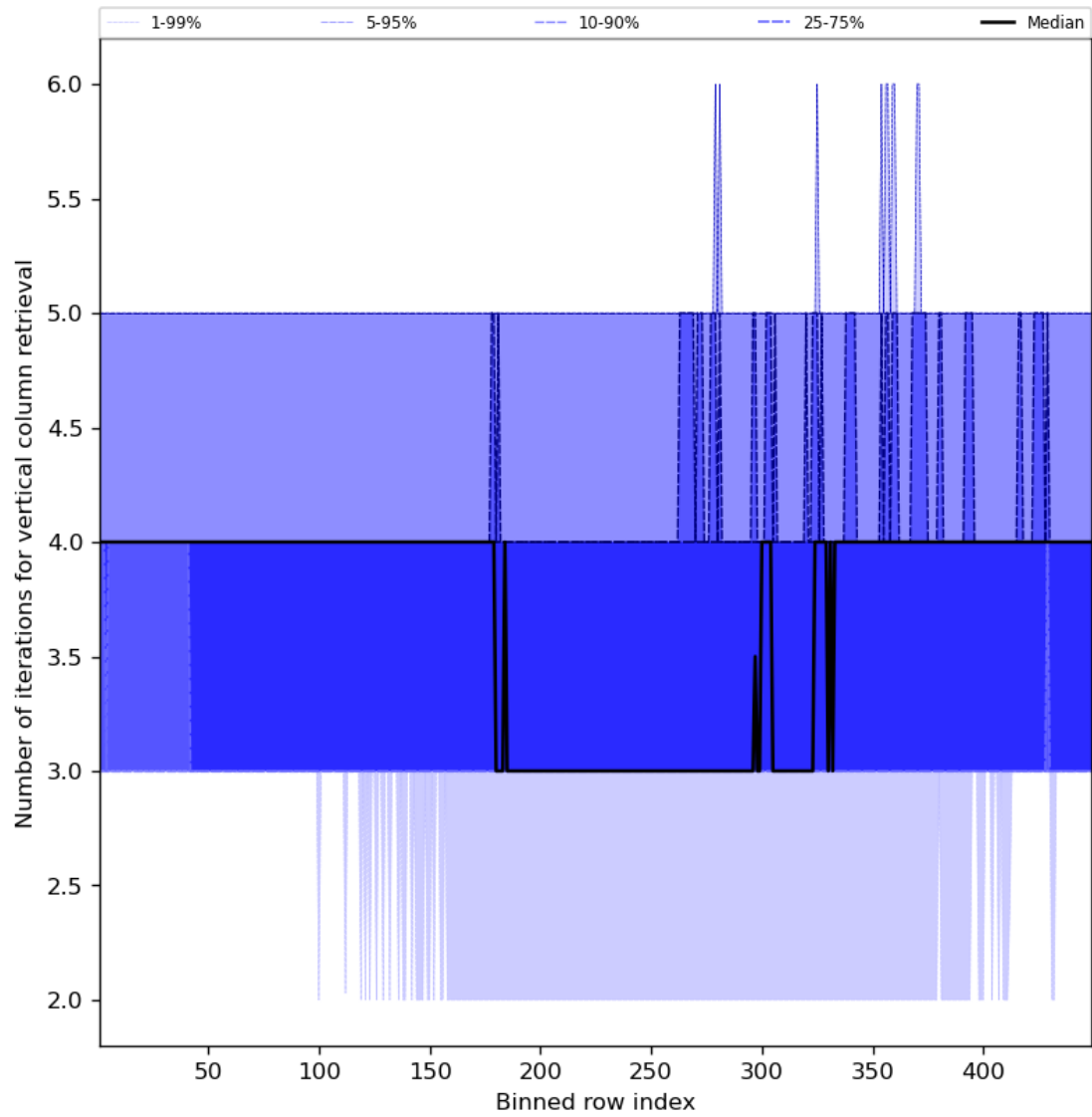
Figure 33: Along track statistics of “Number of iterations for vertical column retrieval” for 2023-11-16 to 2023-11-18
