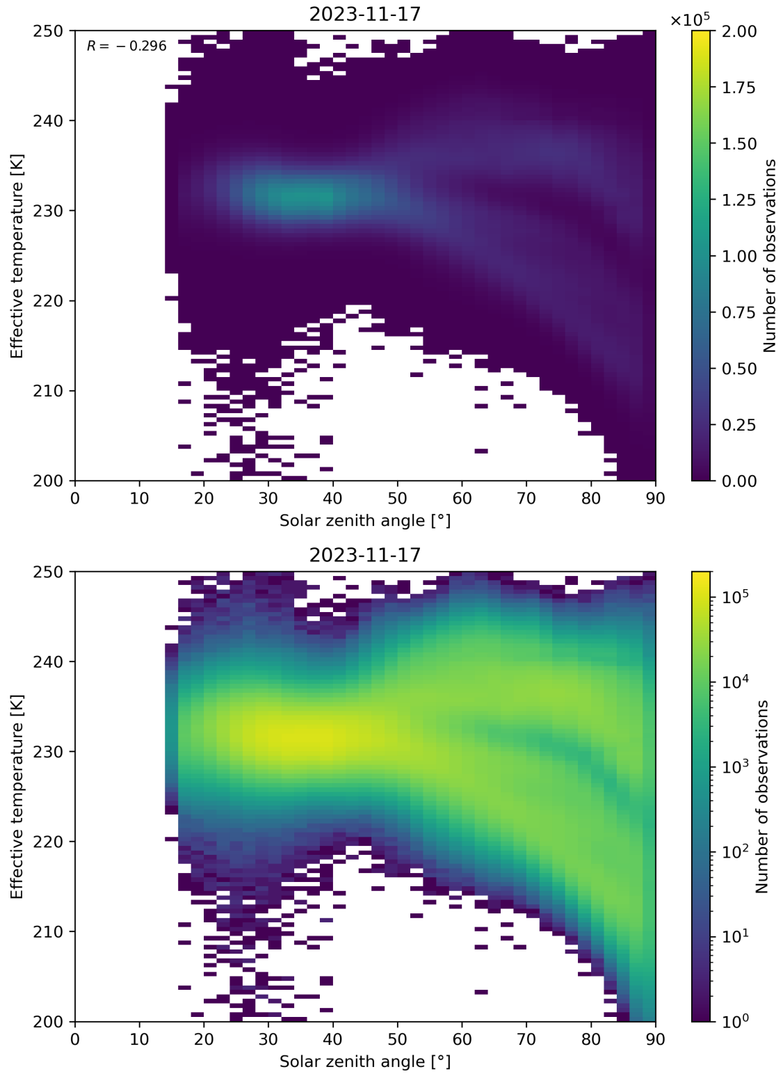
Figure 45: Scatter density plot of “Solar zenith angle” against “Effective temperature” for 2023-11-16 to 2023-11-18.
