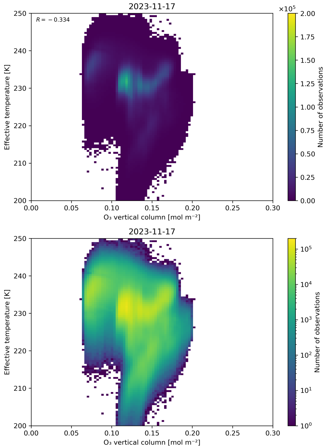
Figure 39: Scatter density plot of “O 3 vertical column” against “Effective temperature” for 2023-11-16 to 2023-11-18.
