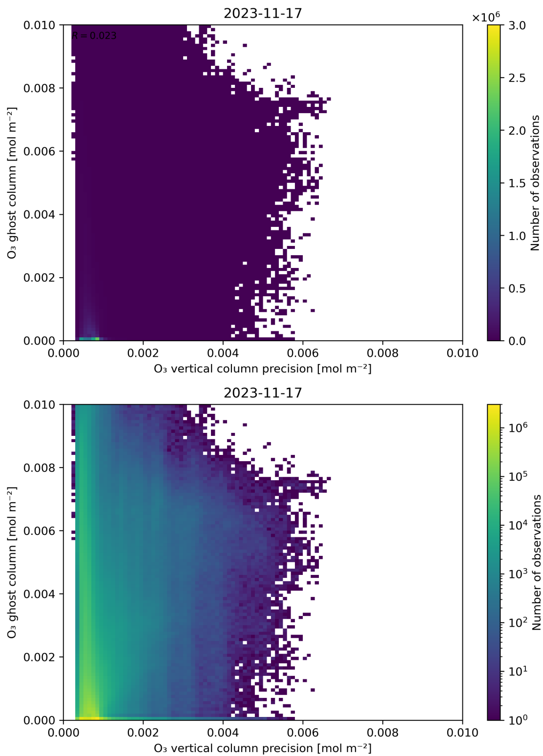
Figure 43: Scatter density plot of “ O_3 vertical column precision” against “ O_3 ghost column” for 2023-11-16 to 2023-11-18.
