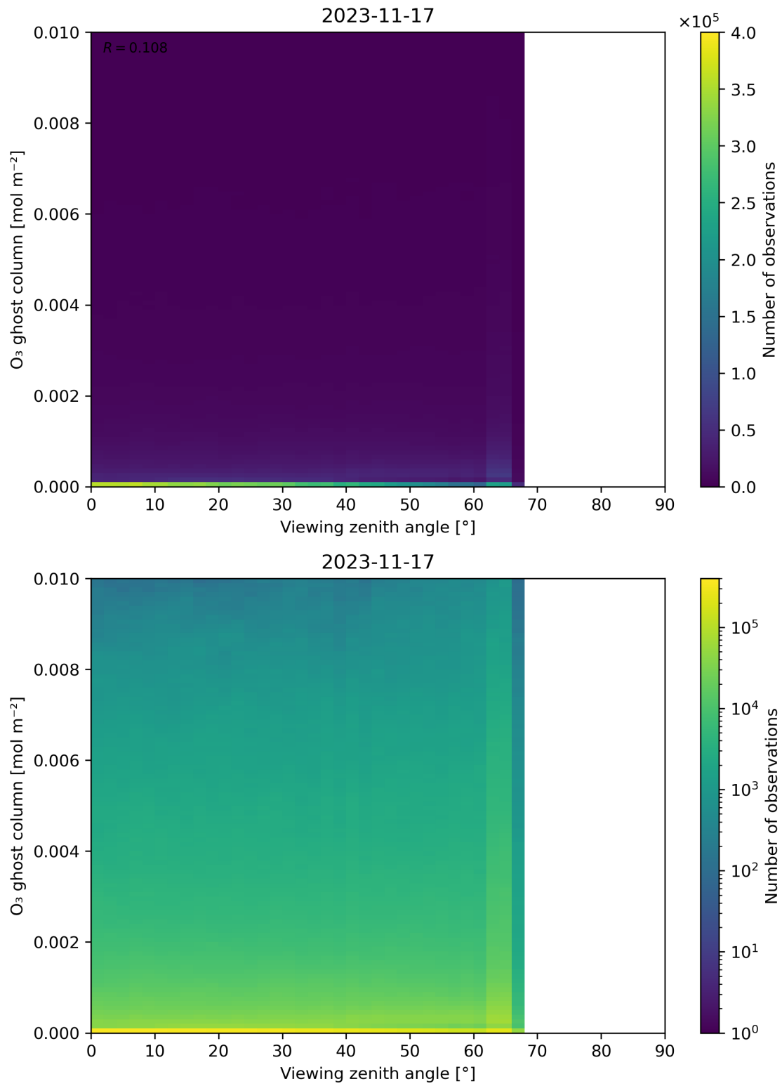
Figure 51: Scatter density plot of “Viewing zenith angle” against “O 3 ghost column” for 2023-11-16 to 2023-11-18.
