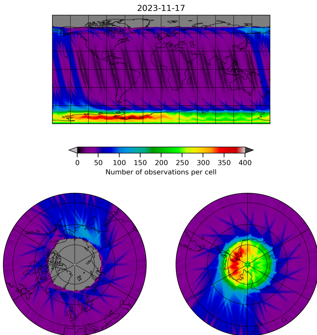
Figure 12: Map of the number of observations for 2023-11-16 to 2023-11-18
