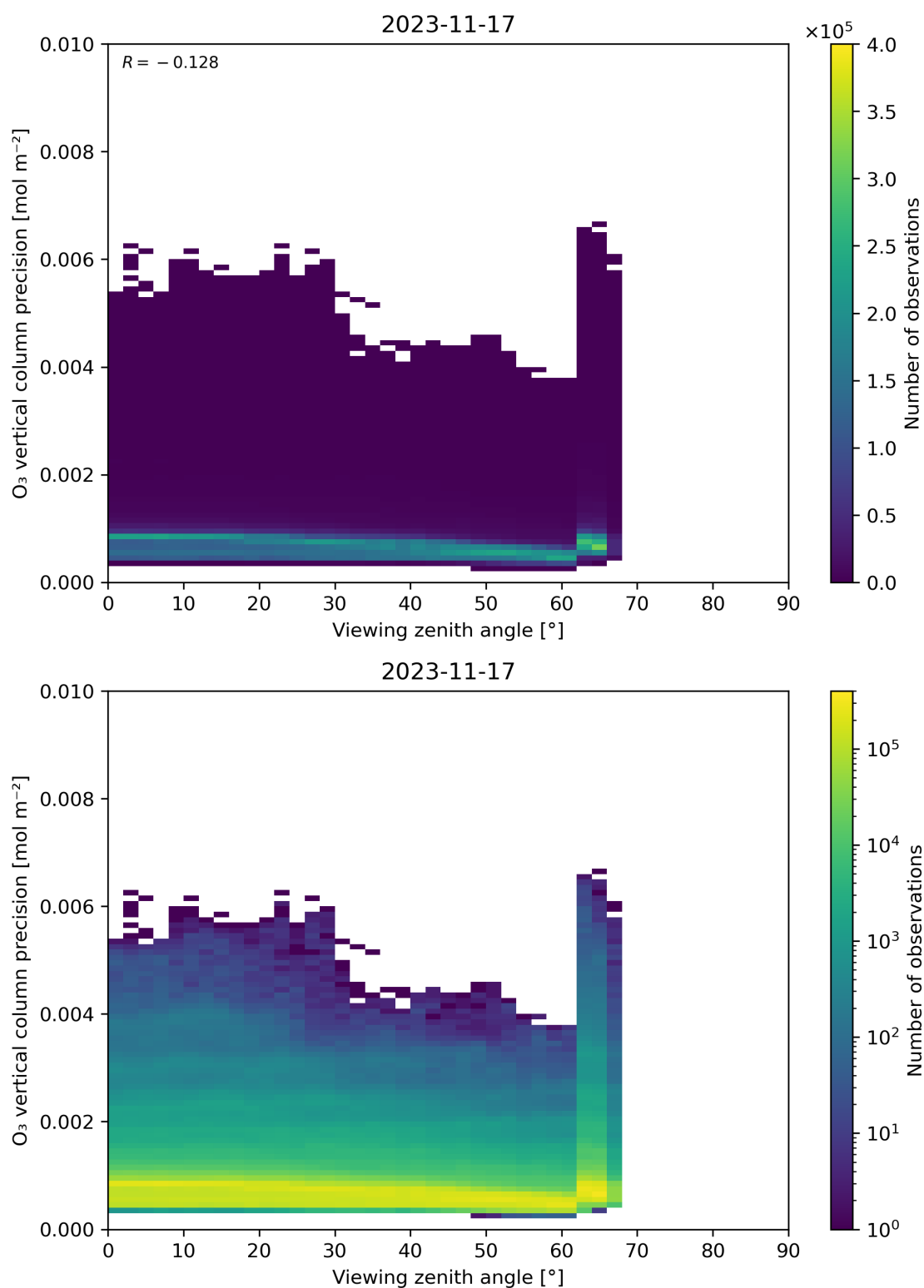
Figure 53: Scatter density plot of “Viewing zenith angle” against “O 3 vertical column precision” for 2023-11-16 to 2023-11-18.
