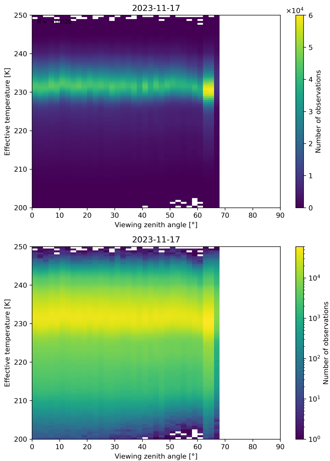
Figure 50: Scatter density plot of “Viewing zenith angle” against “Effective temperature” for 2023-11-16 to 2023-11-18.
