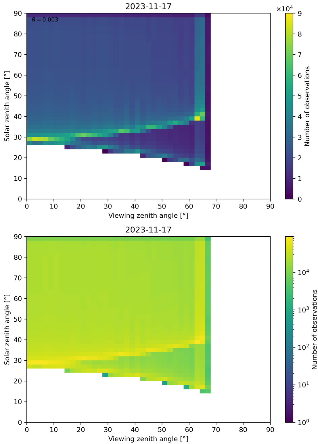
Figure 54: Scatter density plot of “Viewing zenith angle” against “Solar zenith angle” for 2023-11-16 to 2023-11-18.
