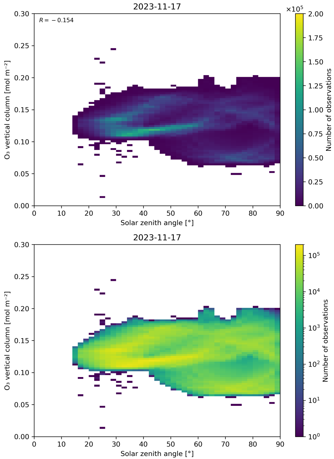
Figure 47: Scatter density plot of “Solar zenith angle” against “O 3 vertical column” for 2023-11-16 to 2023-11-18.
