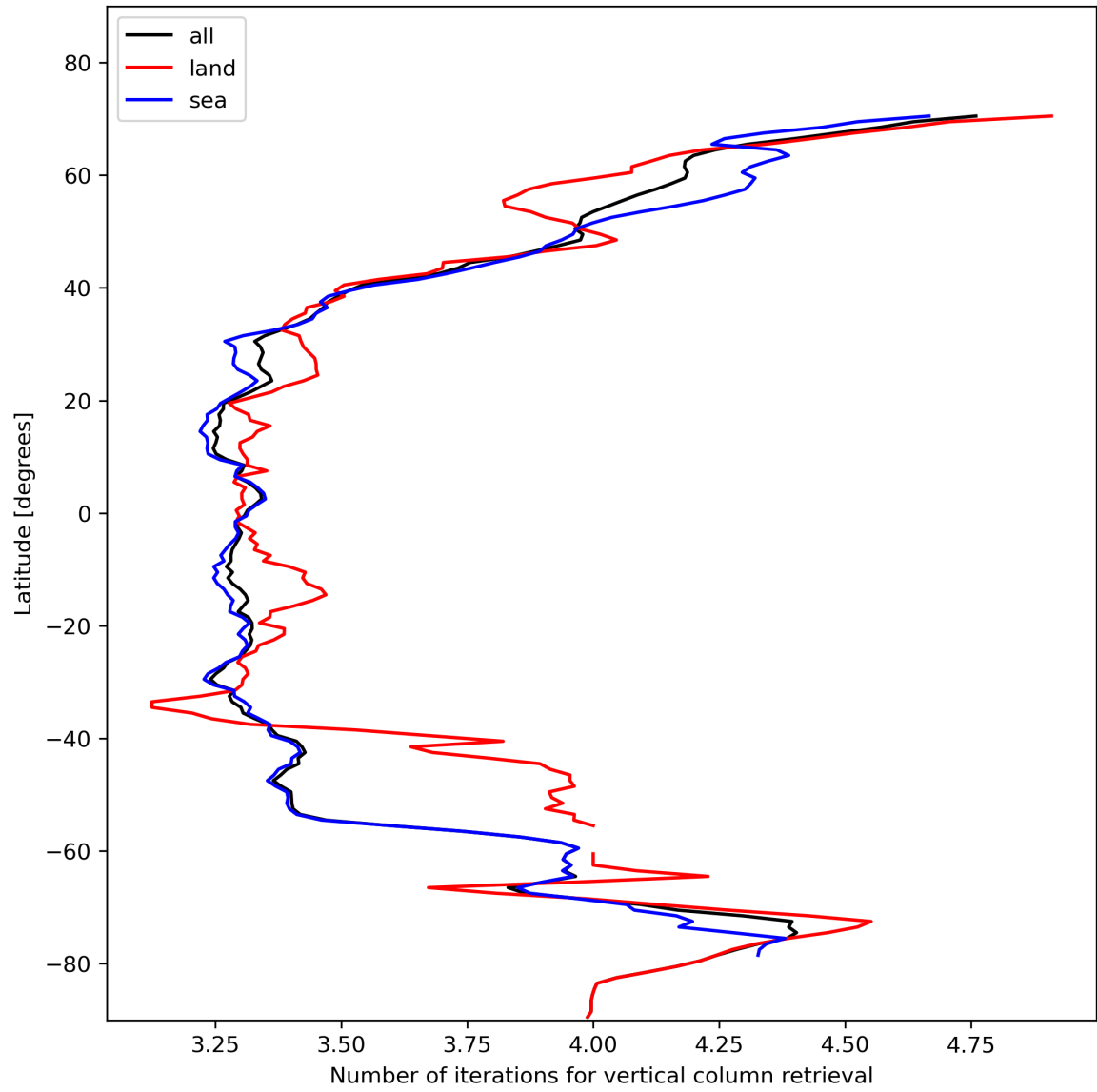
Figure 19: Zonal average of “Number of iterations for vertical column retrieval” for 2023-11-16 to 2023-11-18.
