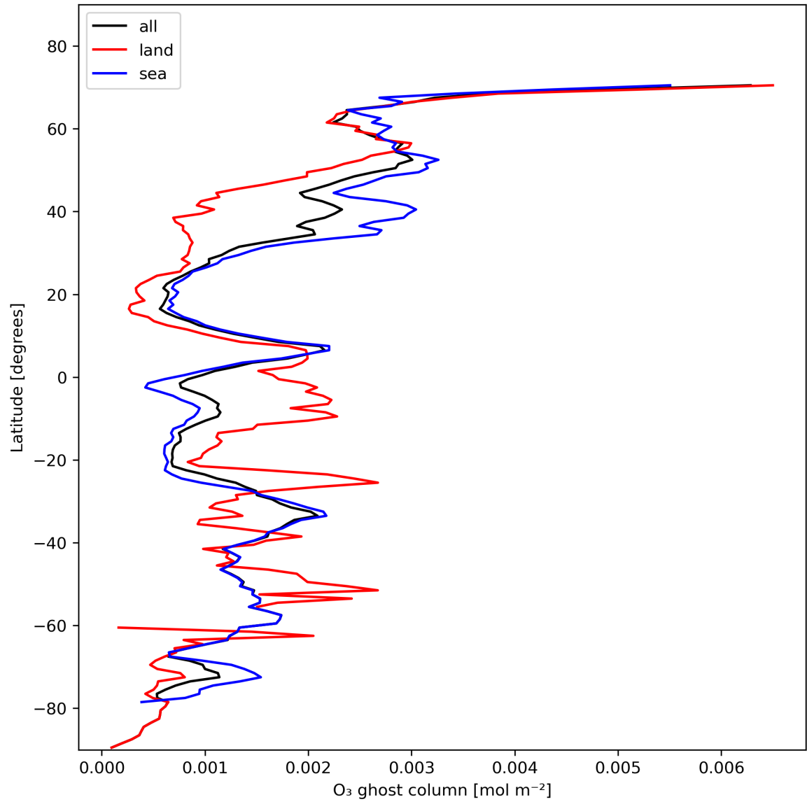
Figure 18: Zonal average of “O 3 ghost column” for 2023-11-16 to 2023-11-18.
