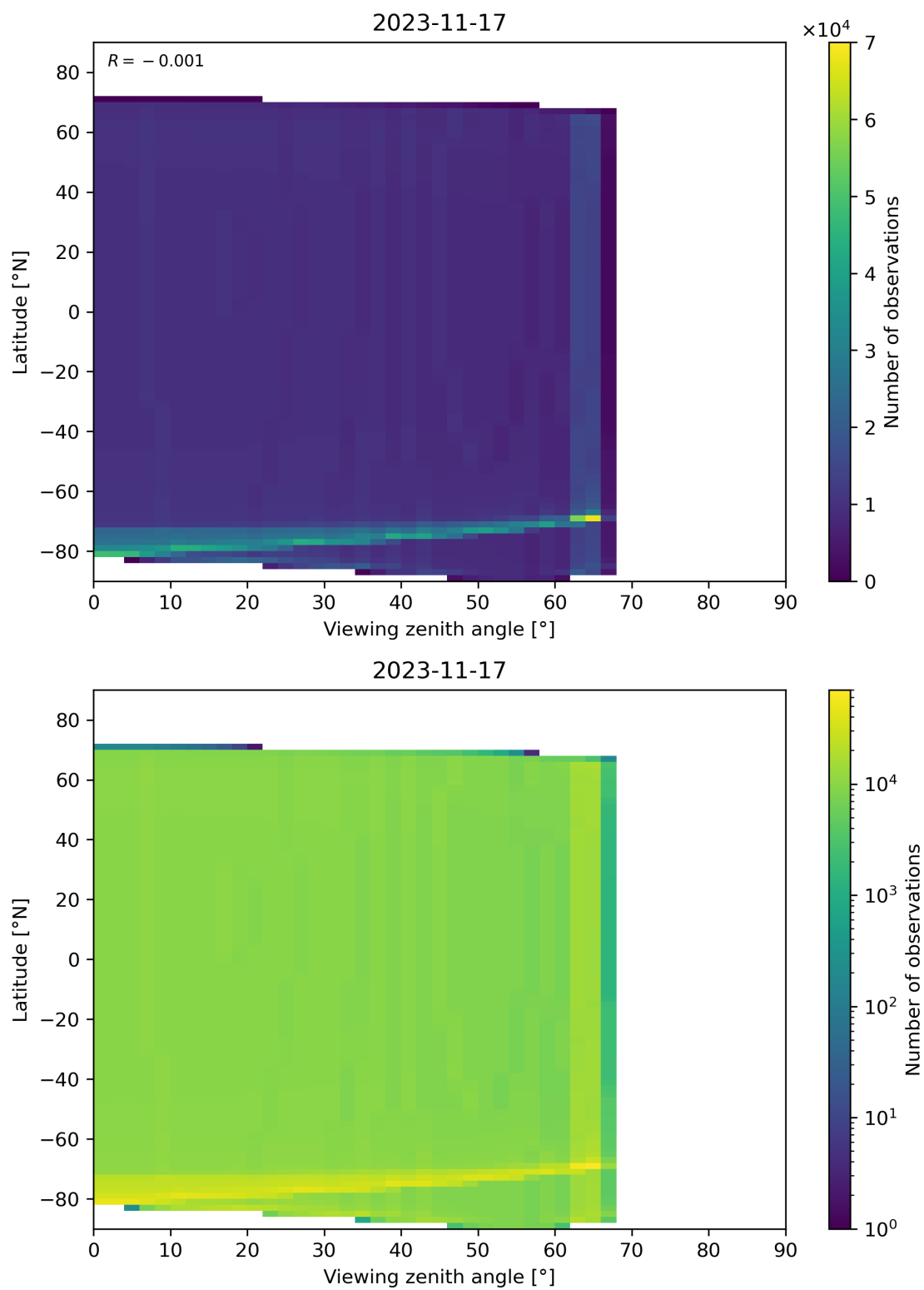
Figure 49: Scatter density plot of “Viewing zenith angle” against “Latitude” for 2023-11-16 to 2023-11-18.
