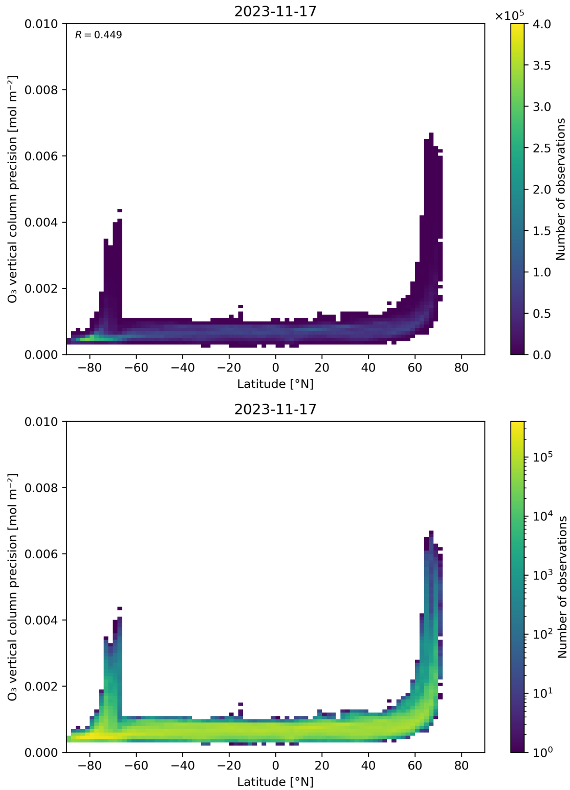
Figure 37: Scatter density plot of “Latitude” against “O 3 vertical column precision” for 2023-11-16 to 2023-11-18.
