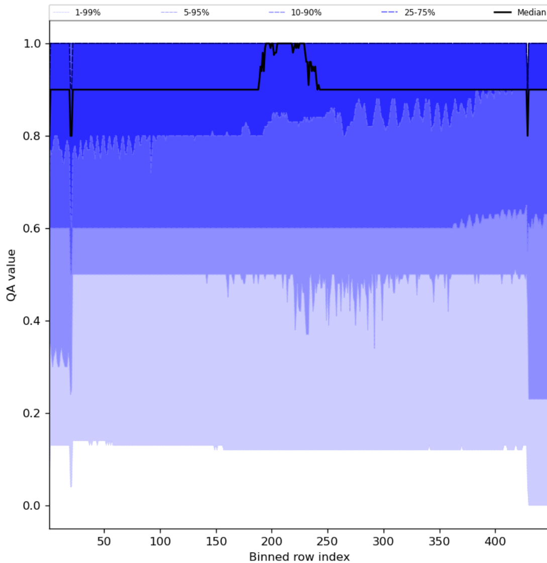
Figure 27: Along track statistics of “QA value” for 2023-11-16 to 2023-11-18
