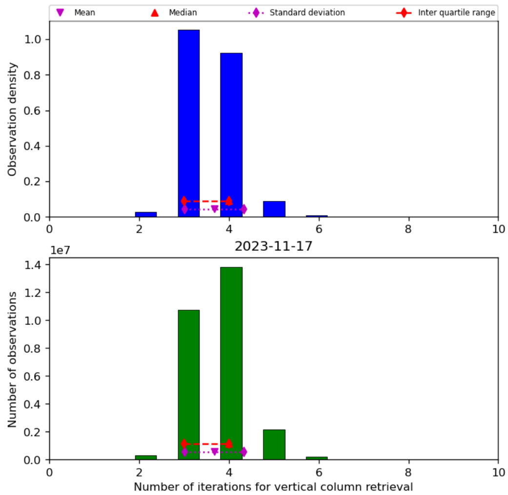
Figure 26: Histogram of “Number of iterations for vertical column retrieval” for 2023-11-16 to 2023-11-18
