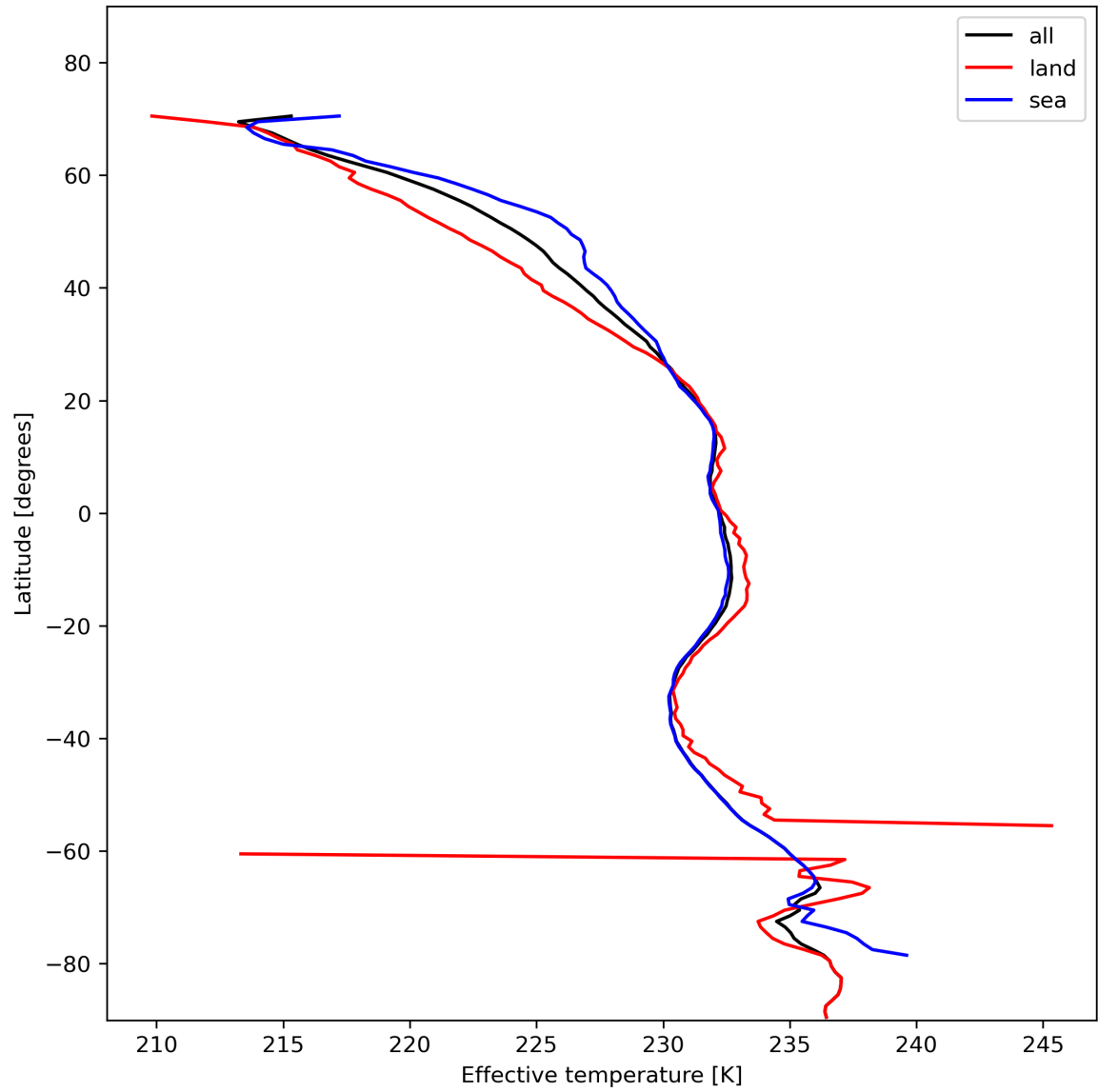
Figure 17: Zonal average of “Effective temperature” for 2023-11-16 to 2023-11-18.
