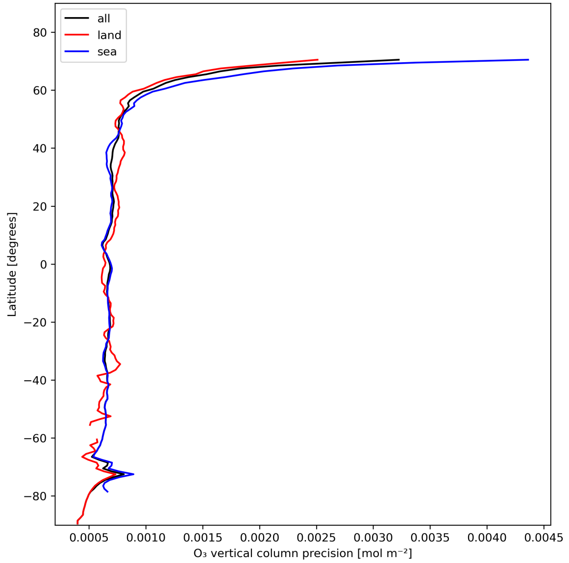
Figure 15: Zonal average of “O 3 vertical column precision” for 2023-11-16 to 2023-11-18.
