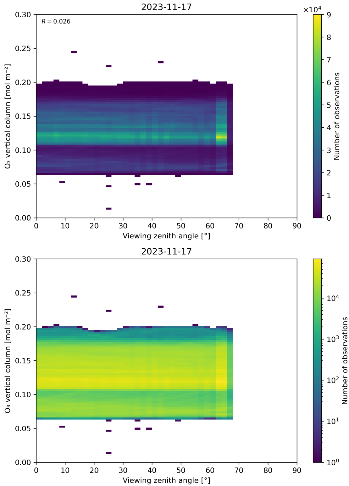
Figure 52: Scatter density plot of “Viewing zenith angle” against “O 3 vertical column” for 2023-11-16 to 2023-11-18.
