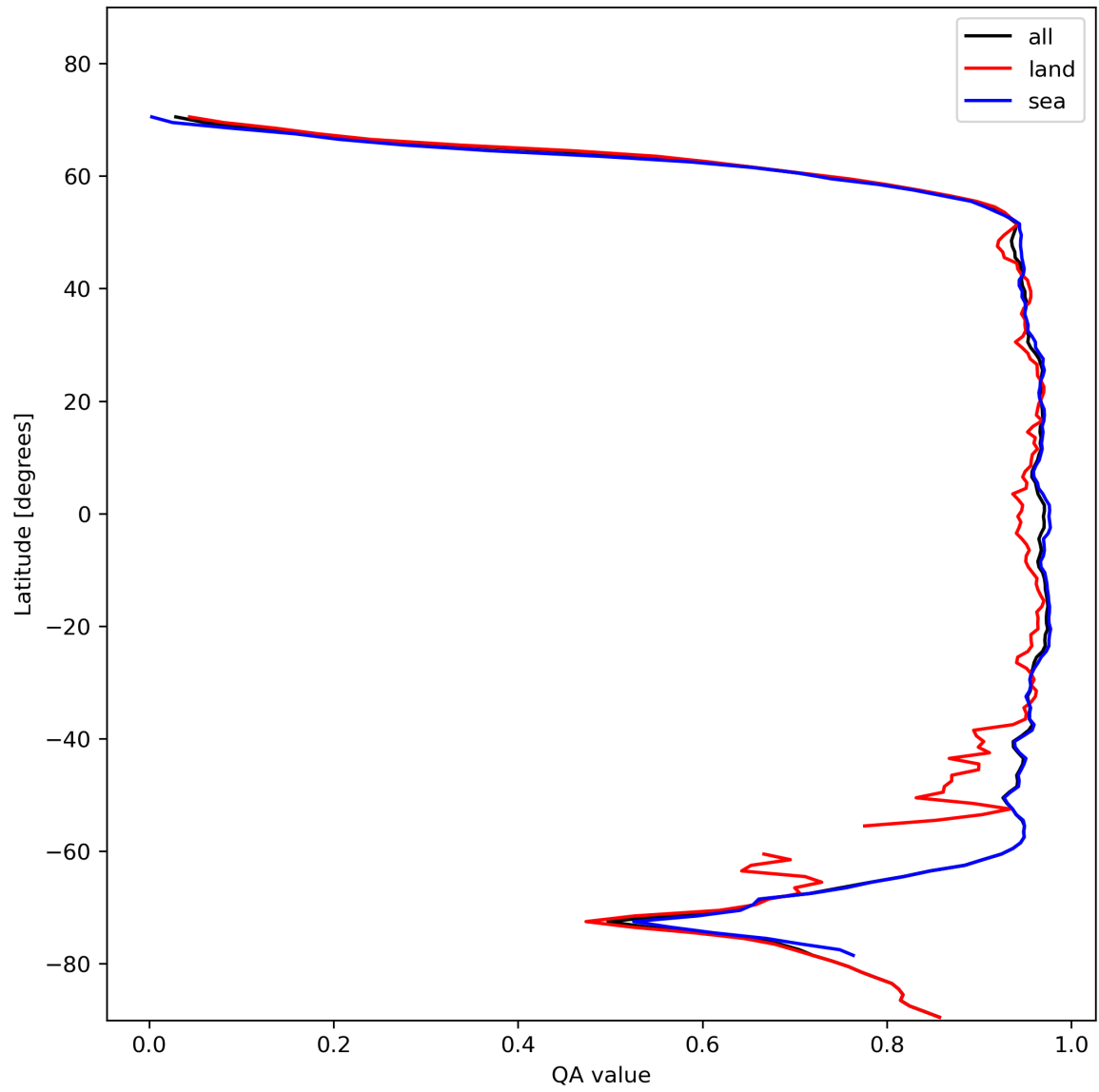
Figure 13: Zonal average of “QA value” for 2023-11-16 to 2023-11-18.
