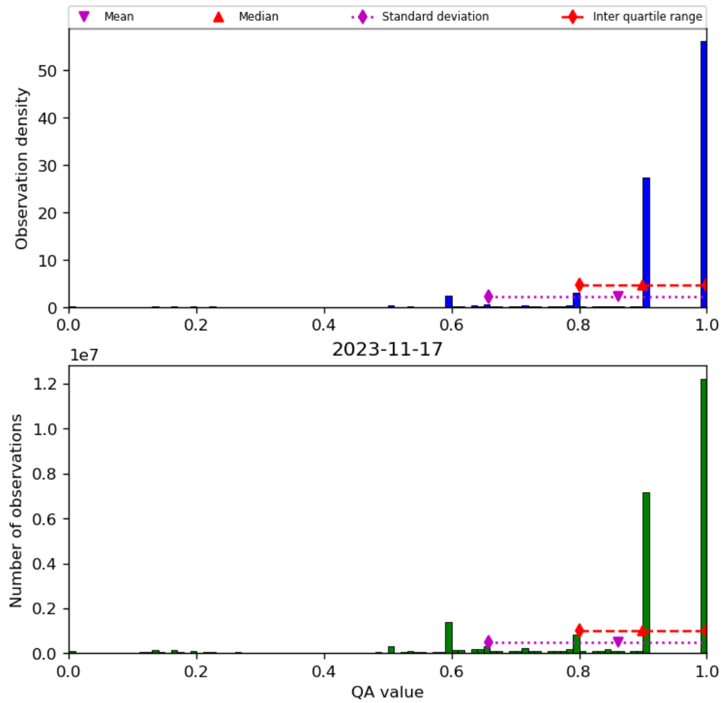
Figure 20: Histogram of “QA value” for 2023-11-16 to 2023-11-18
