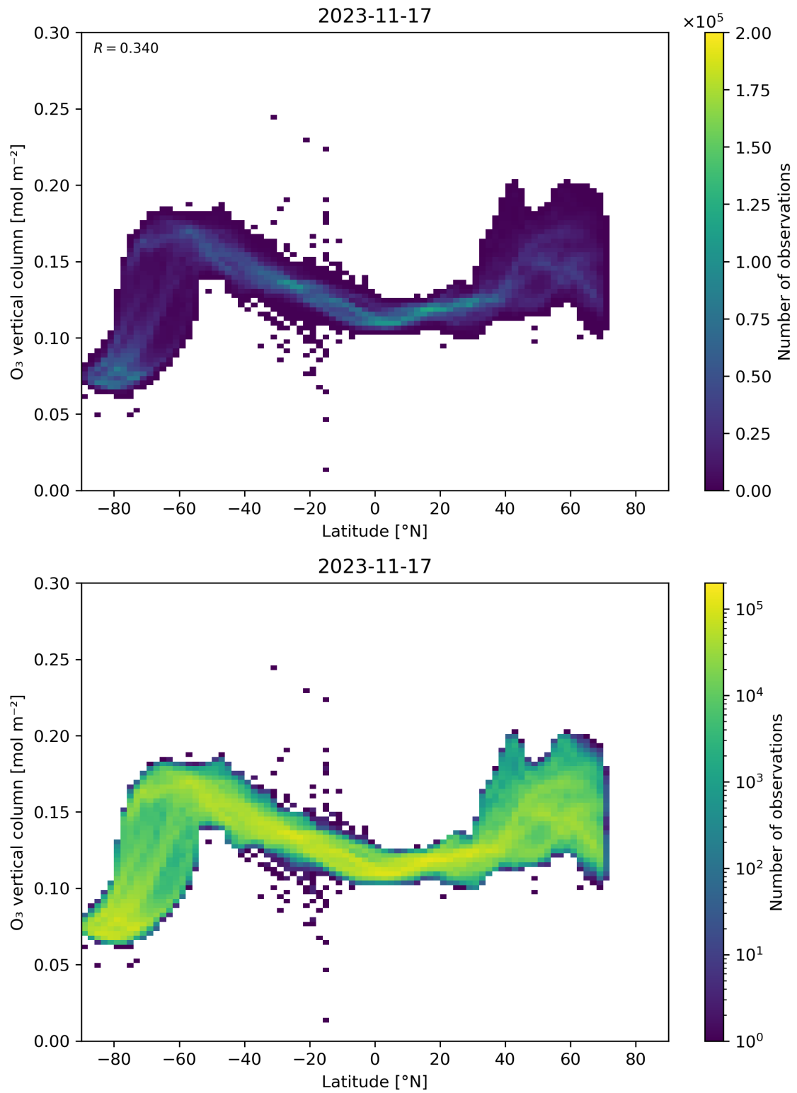
Figure 36: Scatter density plot of “Latitude” against “O 3 vertical column” for 2023-11-16 to 2023-11-18.
