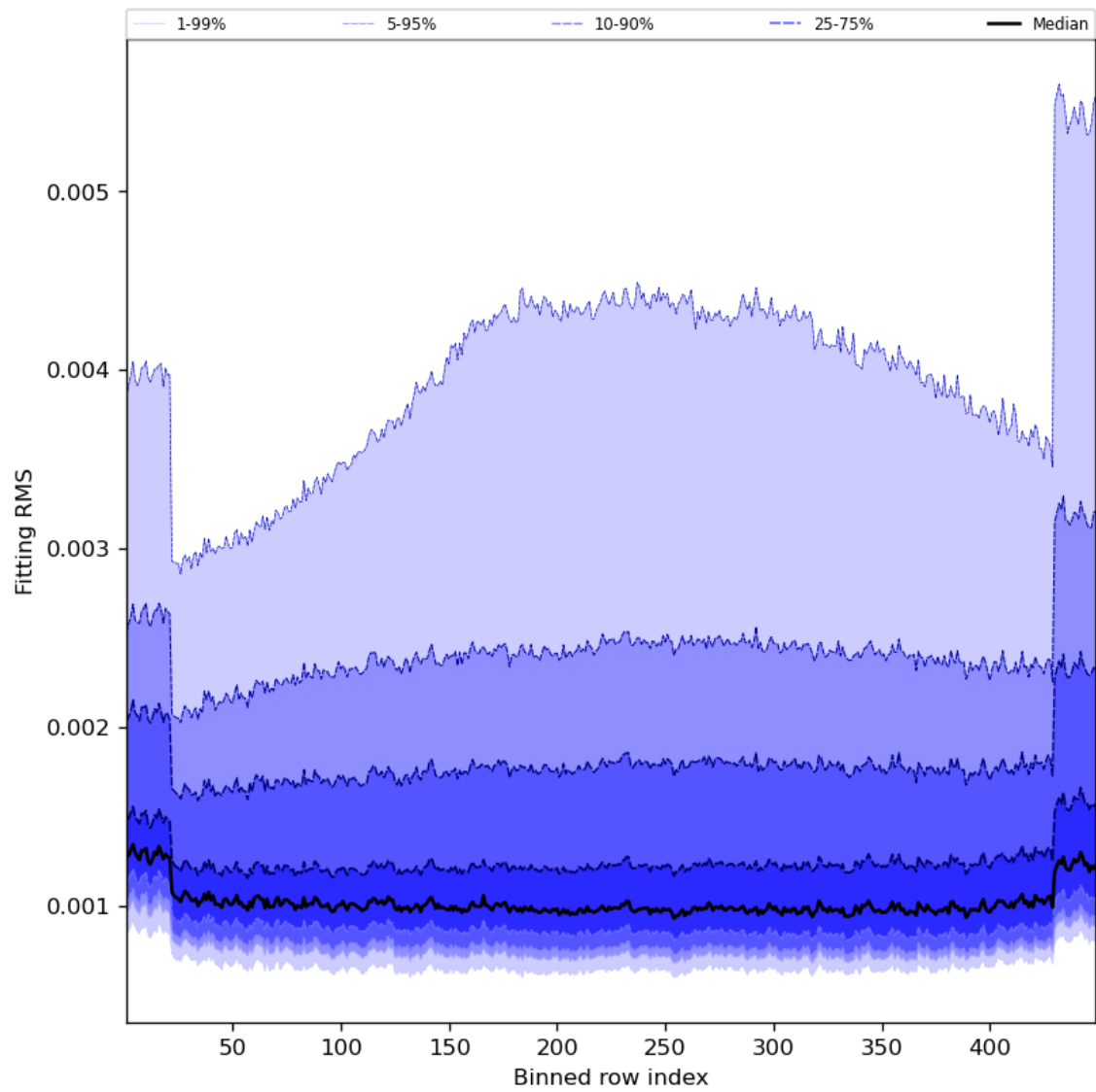
Figure 30: Along track statistics of “Fitting RMS” for 2023-11-16 to 2023-11-18
