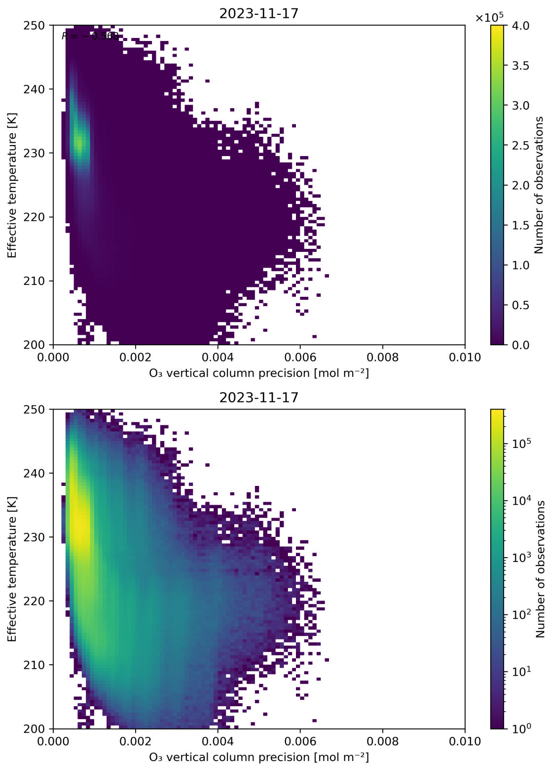
Figure 42: Scatter density plot of “O 3 vertical column precision” against “Effective temperature” for 2023-11-16 to 2023-11-18.
