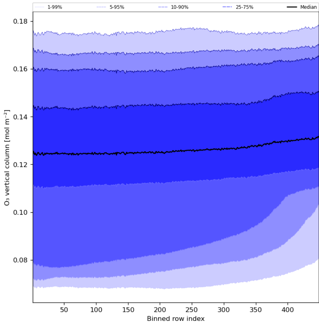
Figure 28: Along track statistics of “O 3 vertical column” for 2023-11-16 to 2023-11-18
