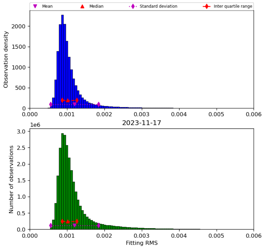
Figure 23: Histogram of “Fitting RMS” for 2023-11-16 to 2023-11-18
