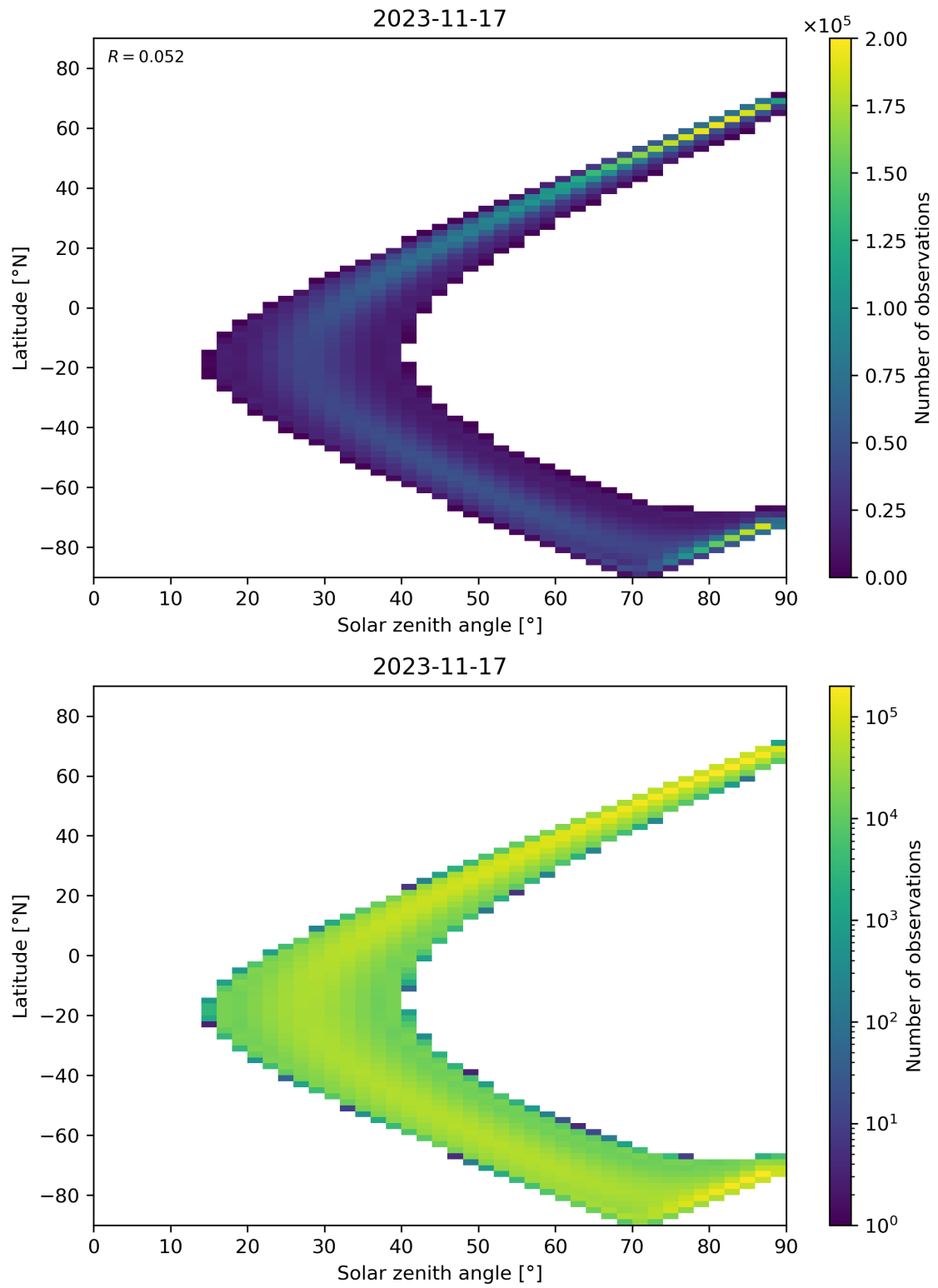
Figure 44: Scatter density plot of “Solar zenith angle” against “Latitude” for 2023-11-16 to 2023-11-18.
