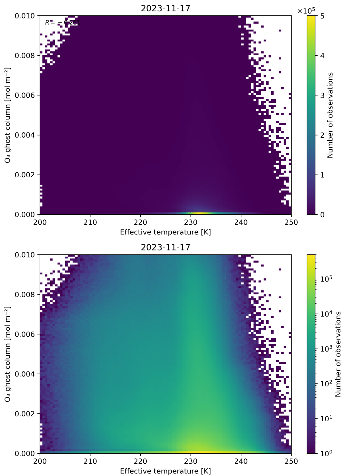
Figure 38: Scatter density plot of “Effective temperature” against “O 3 ghost column” for 2023-11-16 to 2023-11-18.
