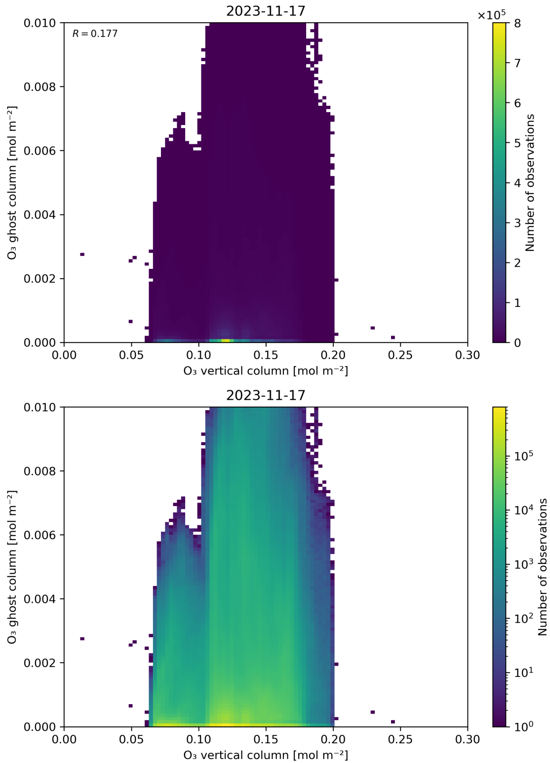
Figure 40: Scatter density plot of “O 3 vertical column” against “O 3 ghost column” for 2023-11-16 to 2023-11-18.
