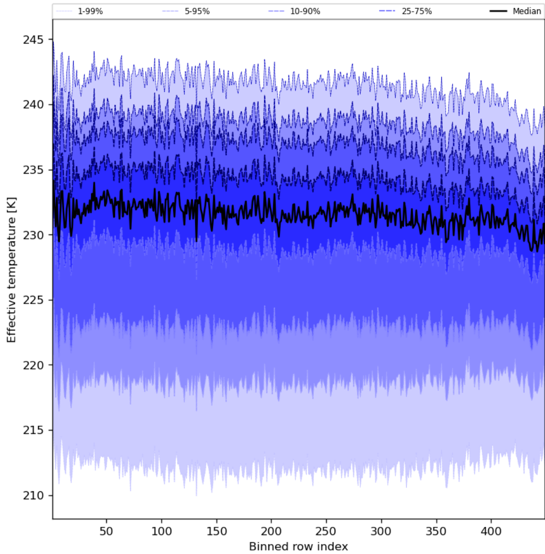
Figure 31: Along track statistics of “Effective temperature” for 2023-11-16 to 2023-11-18
