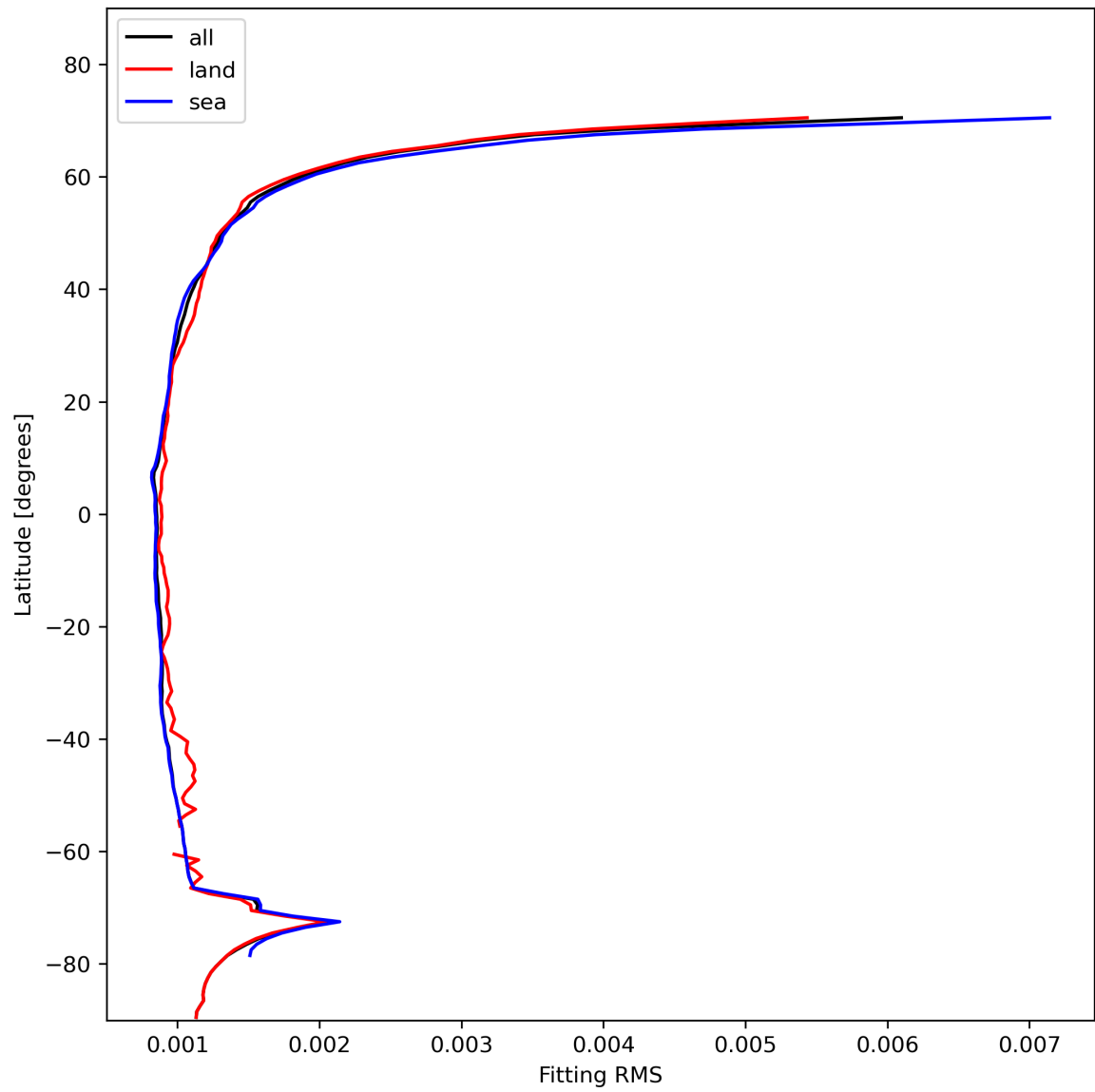
Figure 16: Zonal average of “Fitting RMS” for 2023-11-16 to 2023-11-18.
