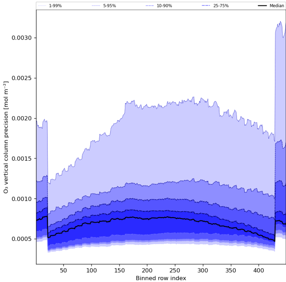
Figure 29: Along track statistics of “O 3 vertical column precision” for 2023-11-16 to 2023-11-18
