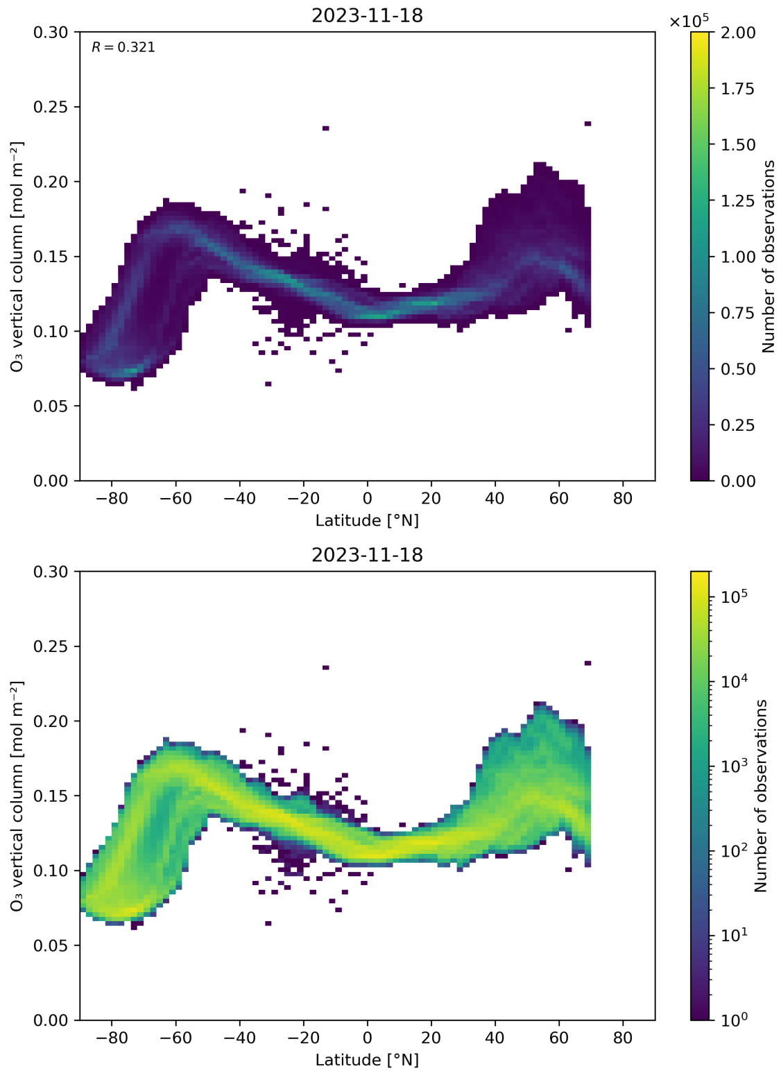
Figure 36: Scatter density plot of “Latitude” against “O 3 vertical column” for 2023-11-18 to 2023-11-19.
