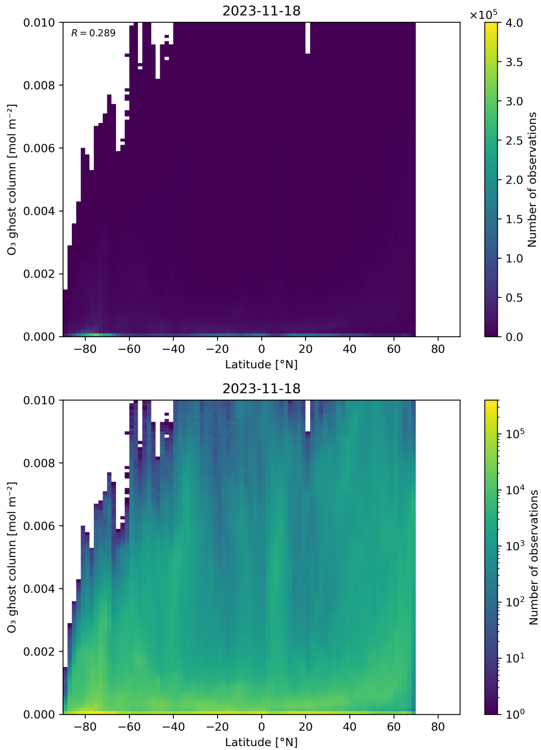
Figure 35: Scatter density plot of “Latitude” against “O 3 ghost column” for 2023-11-18 to 2023-11-19.
