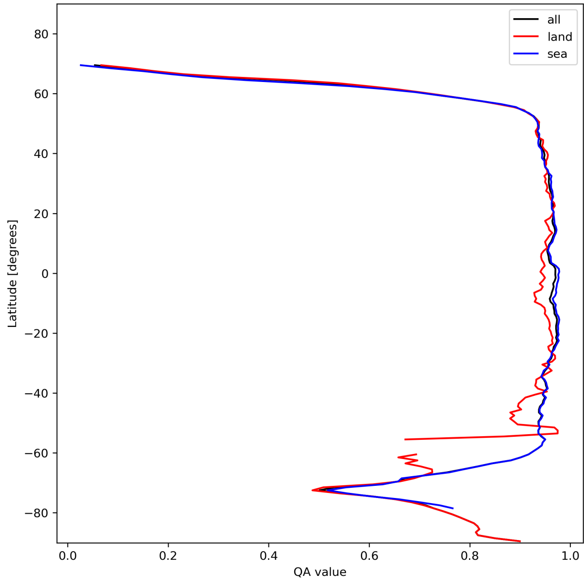
Figure 13: Zonal average of “QA value” for 2023-11-18 to 2023-11-19.
