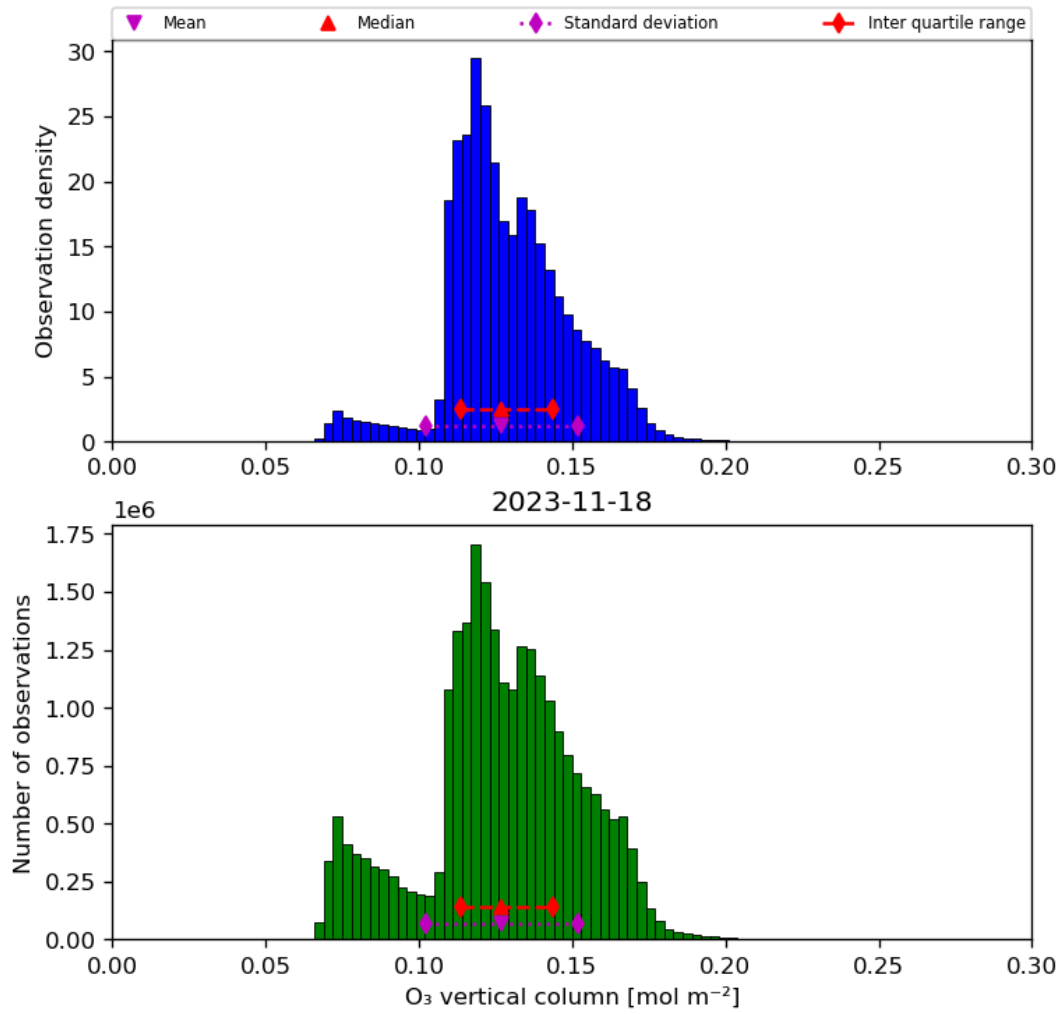
Figure 21: Histogram of “O 3 vertical column” for 2023-11-18 to 2023-11-19
