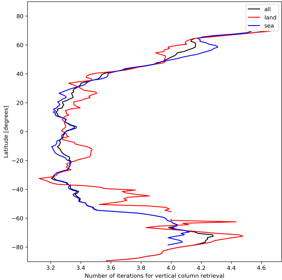
Figure 19: Zonal average of “Number of iterations for vertical column retrieval” for 2023-11-18 to 2023-11-19.
