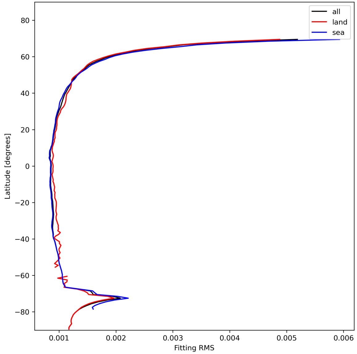
Figure 16: Zonal average of “Fitting RMS” for 2023-11-18 to 2023-11-19.
