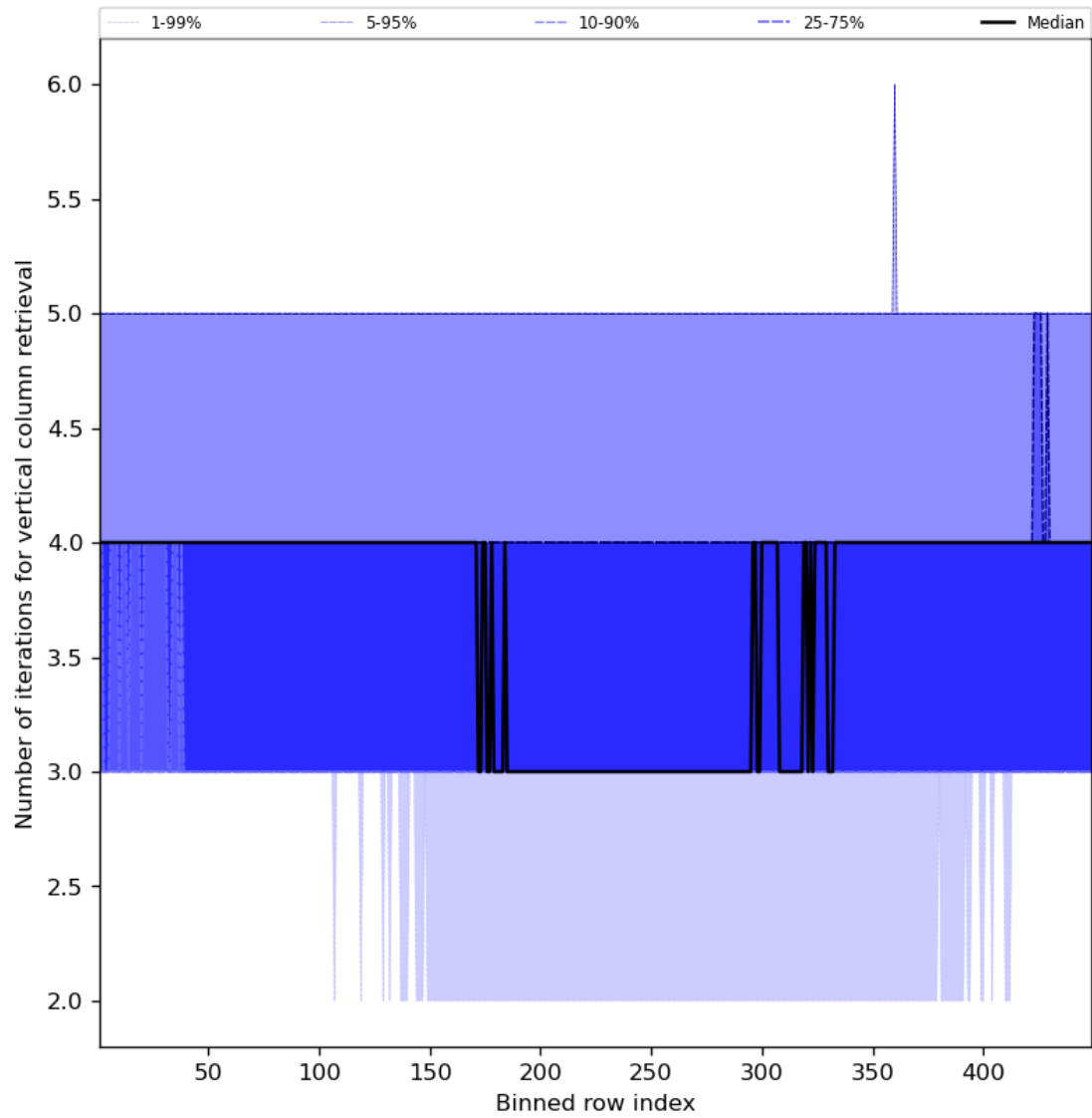
Figure 33: Along track statistics of “Number of iterations for vertical column retrieval” for 2023-11-18 to 2023-11-19
