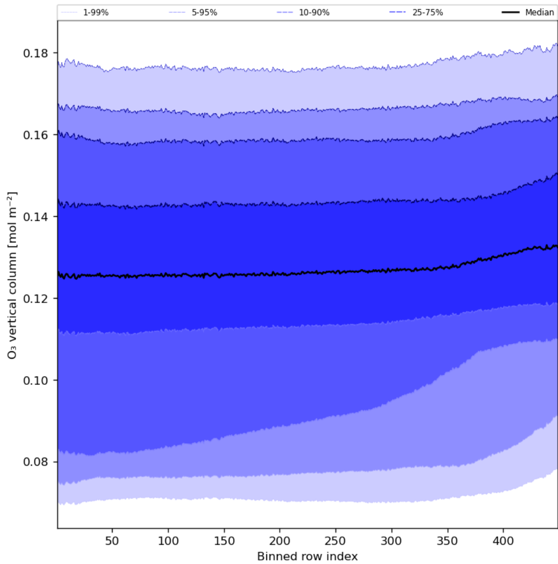
Figure 28: Along track statistics of “O 3 vertical column” for 2023-11-18 to 2023-11-19
