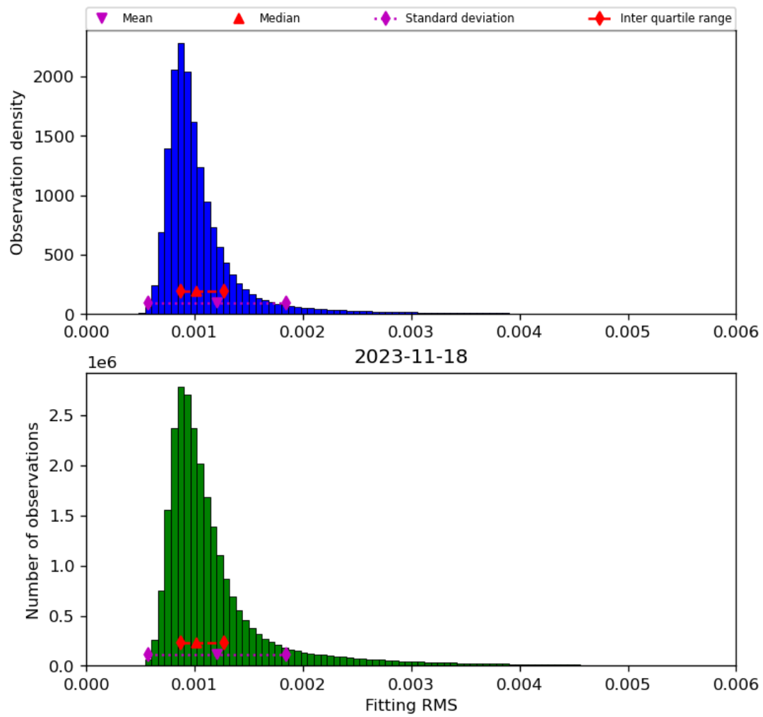
Figure 23: Histogram of “Fitting RMS” for 2023-11-18 to 2023-11-19
