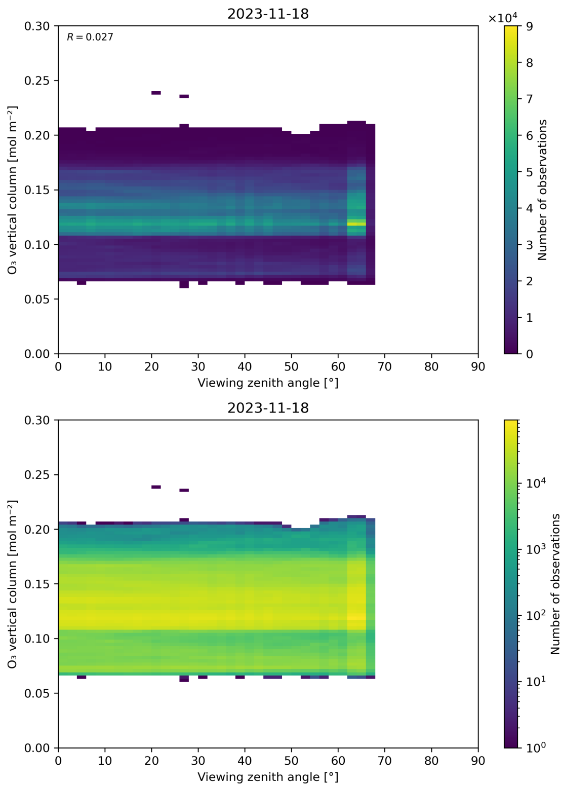
Figure 52: Scatter density plot of “Viewing zenith angle” against “O 3 vertical column” for 2023-11-18 to 2023-11-19.
