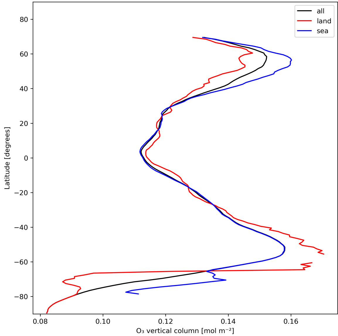
Figure 14: Zonal average of “O 3 vertical column” for 2023-11-18 to 2023-11-19.
