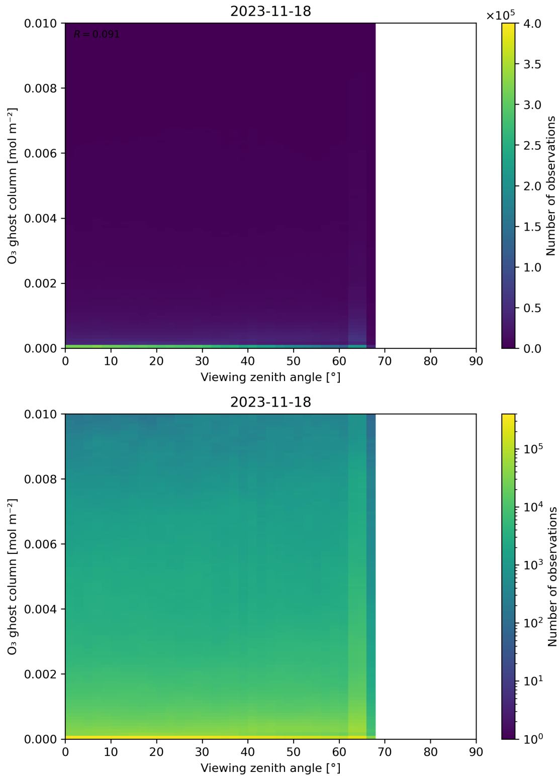
Figure 51: Scatter density plot of “Viewing zenith angle” against “O 3 ghost column” for 2023-11-18 to 2023-11-19.
