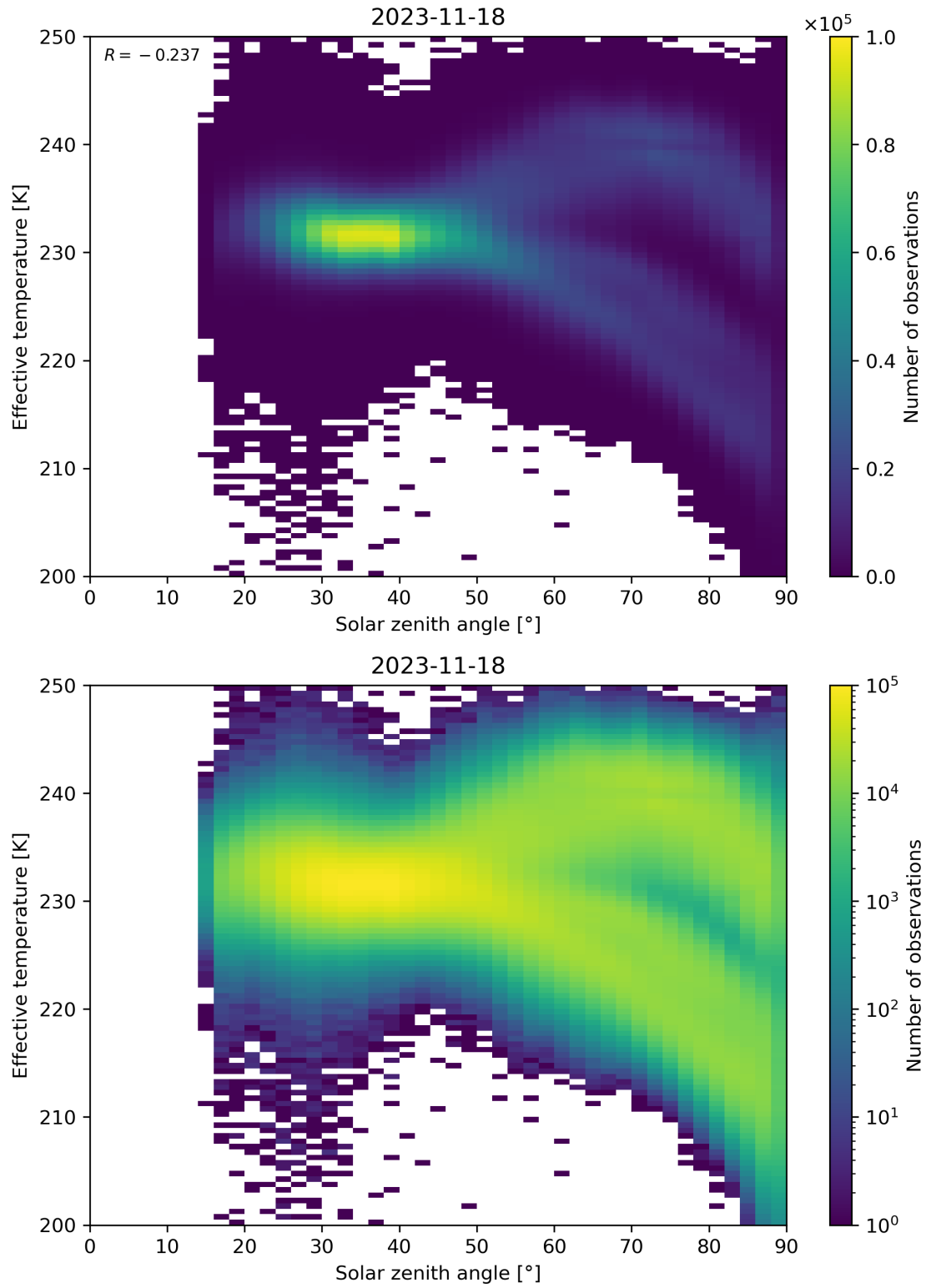
Figure 45: Scatter density plot of “Solar zenith angle” against “Effective temperature” for 2023-11-18 to 2023-11-19.
