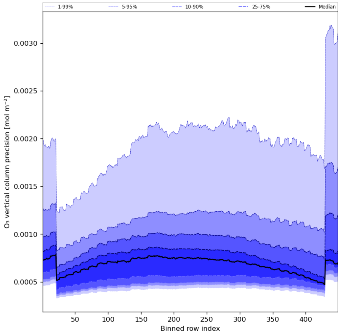
Figure 29: Along track statistics of “O 3 vertical column precision” for 2023-11-18 to 2023-11-19
