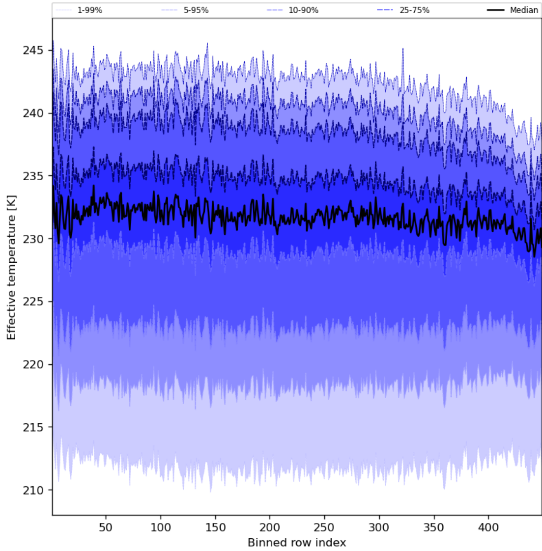
Figure 31: Along track statistics of “Effective temperature” for 2023-11-18 to 2023-11-19
