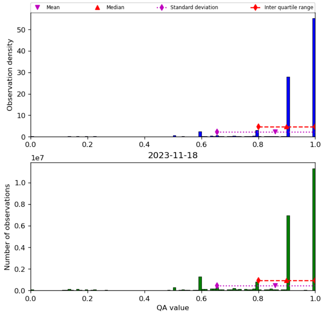
Figure 20: Histogram of “QA value” for 2023-11-18 to 2023-11-19
