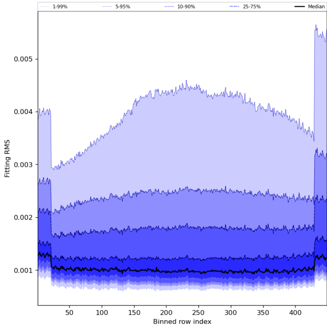
Figure 30: Along track statistics of “Fitting RMS” for 2023-11-18 to 2023-11-19
