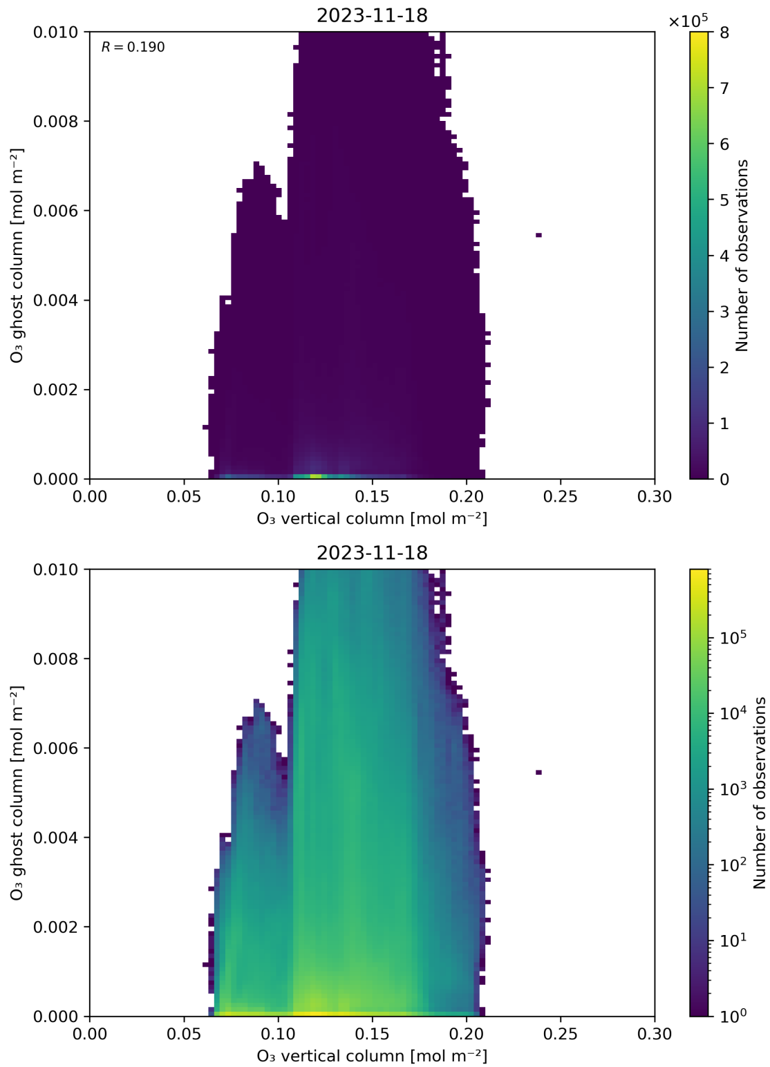
Figure 40: Scatter density plot of “O 3 vertical column” against “O 3 ghost column” for 2023-11-18 to 2023-11-19.
