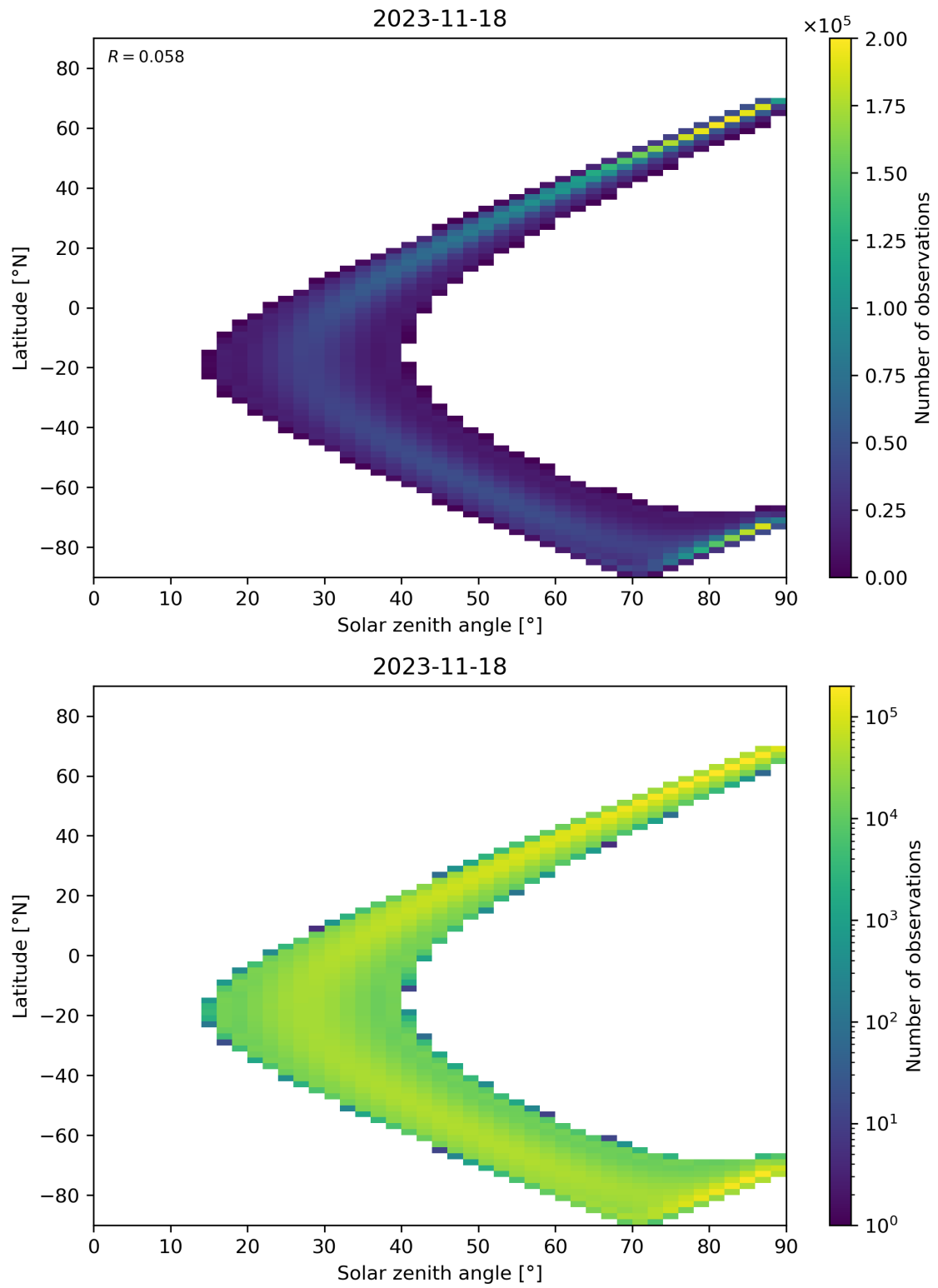
Figure 44: Scatter density plot of “Solar zenith angle” against “Latitude” for 2023-11-18 to 2023-11-19.
