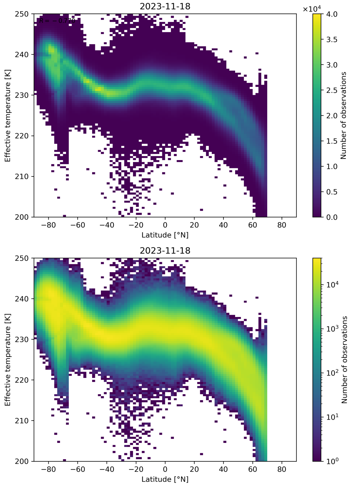
Figure 34: Scatter density plot of “Latitude” against “Effective temperature” for 2023-11-18 to 2023-11-19.
