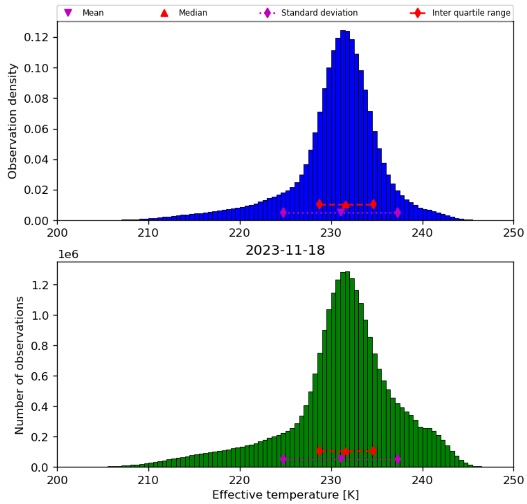
Figure 24: Histogram of “Effective temperature” for 2023-11-18 to 2023-11-19
