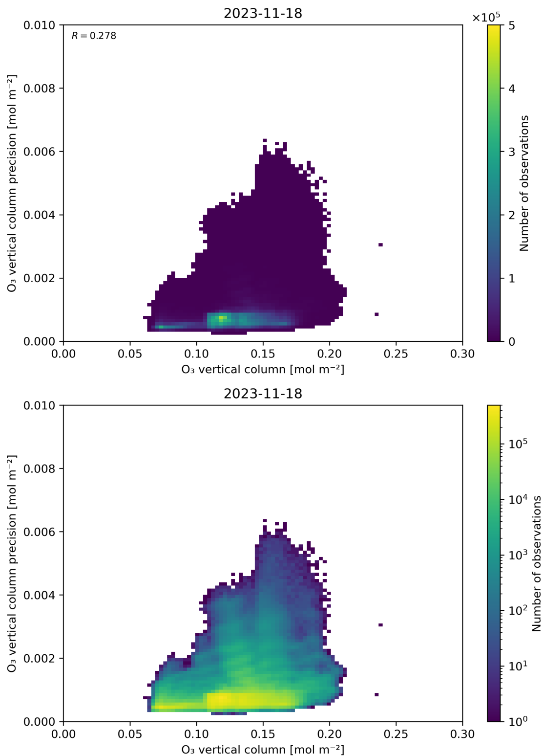
Figure 41: Scatter density plot of “O 3 vertical column” against “O 3 vertical column precision” for 2023-11-18 to 2023-11-19.
