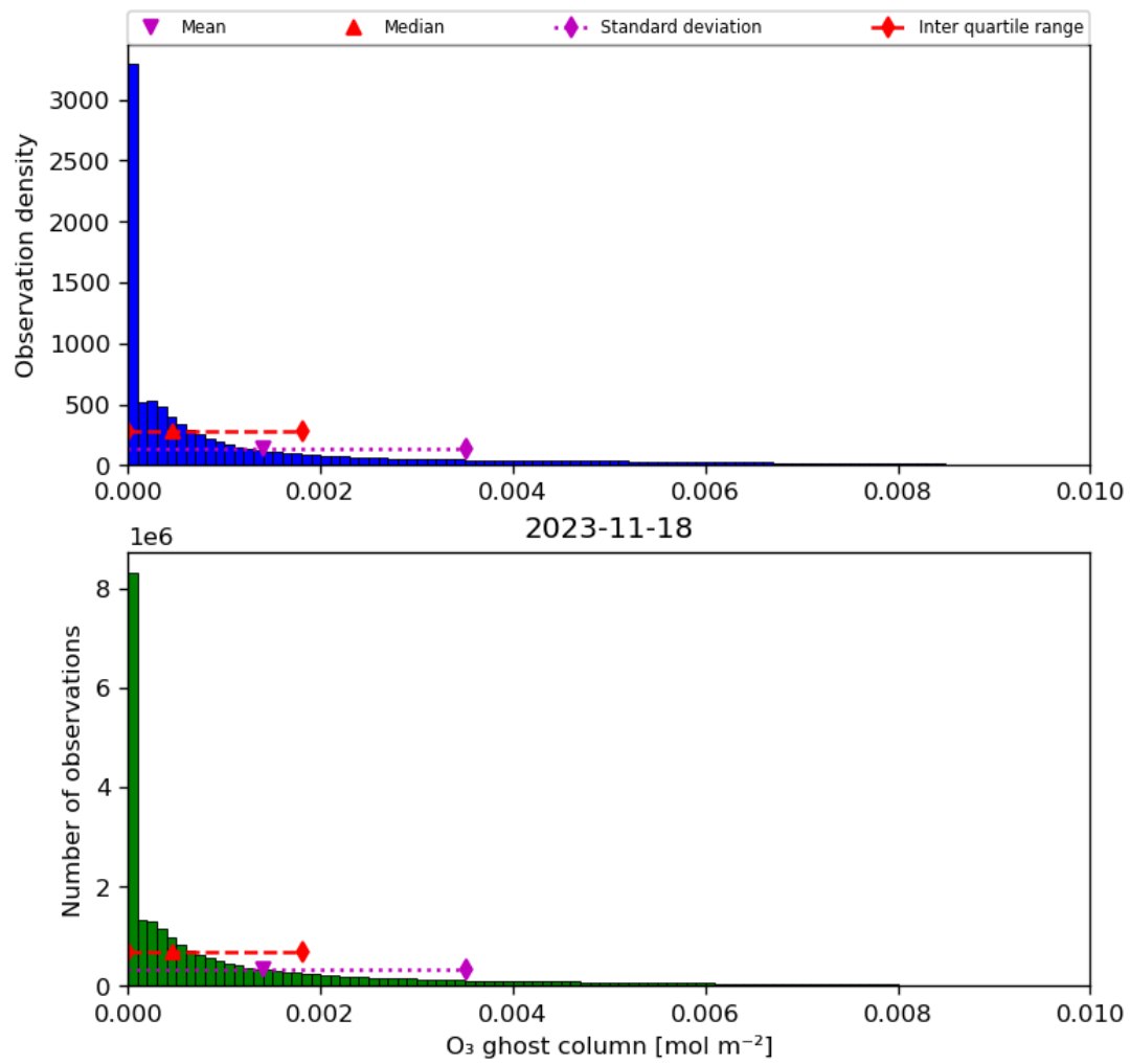
Figure 25: Histogram of “O 3 ghost column” for 2023-11-18 to 2023-11-19
