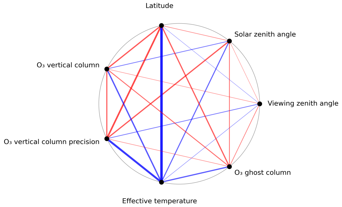
Figure 1: Map of correlation graph for 2023-11-18 to 2023-11-19.
