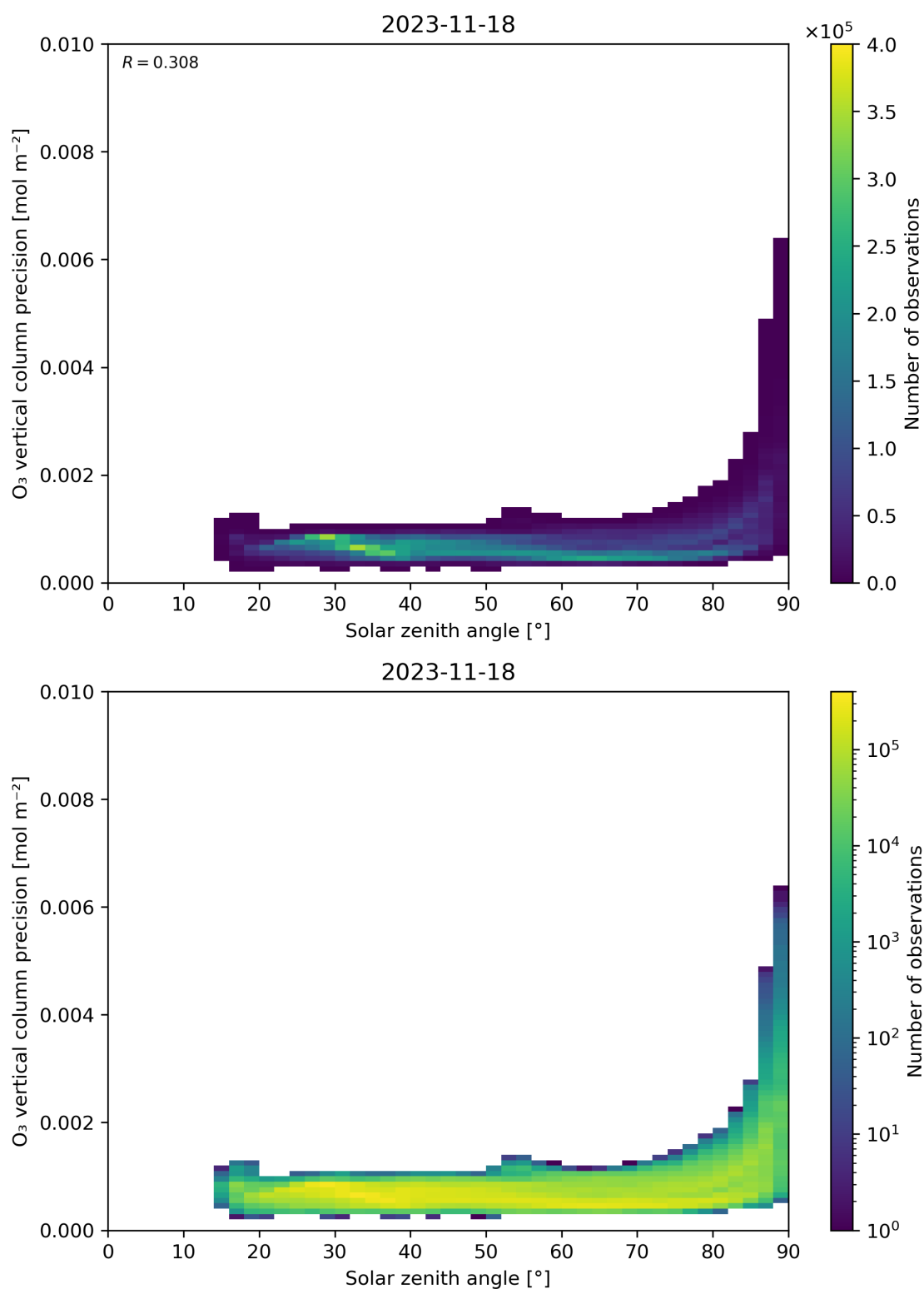
Figure 48: Scatter density plot of “Solar zenith angle” against “O 3 vertical column precision” for 2023-11-18 to 2023-11-19.
