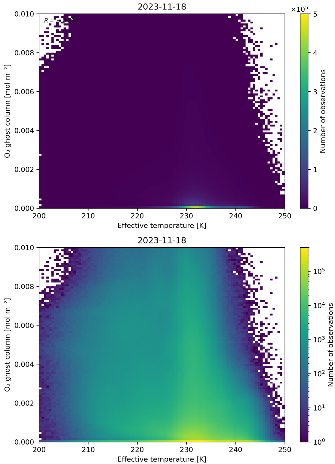
Figure 38: Scatter density plot of “Effective temperature” against “O 3 ghost column” for 2023-11-18 to 2023-11-19.
