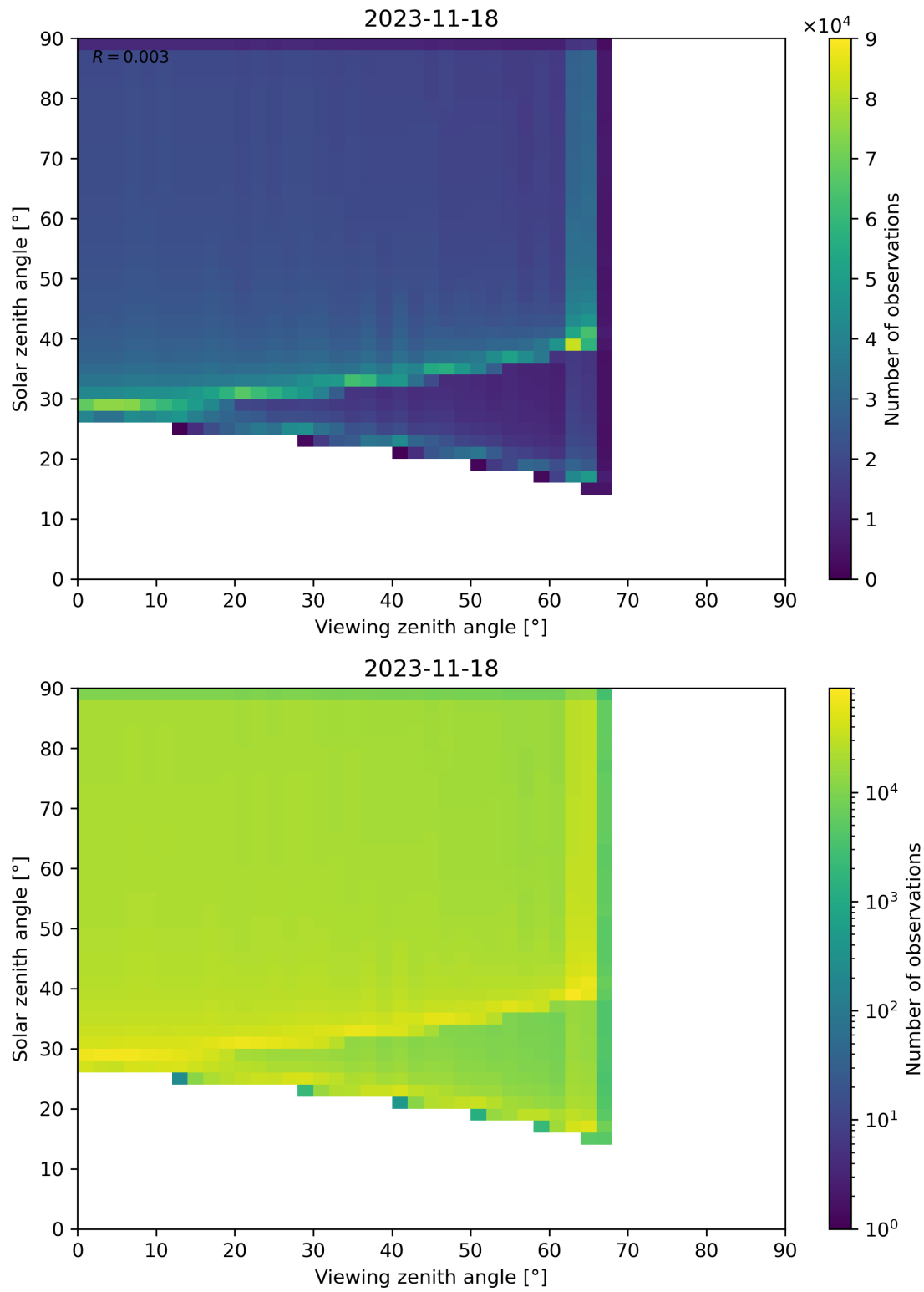
Figure 54: Scatter density plot of “Viewing zenith angle” against “Solar zenith angle” for 2023-11-18 to 2023-11-19.
