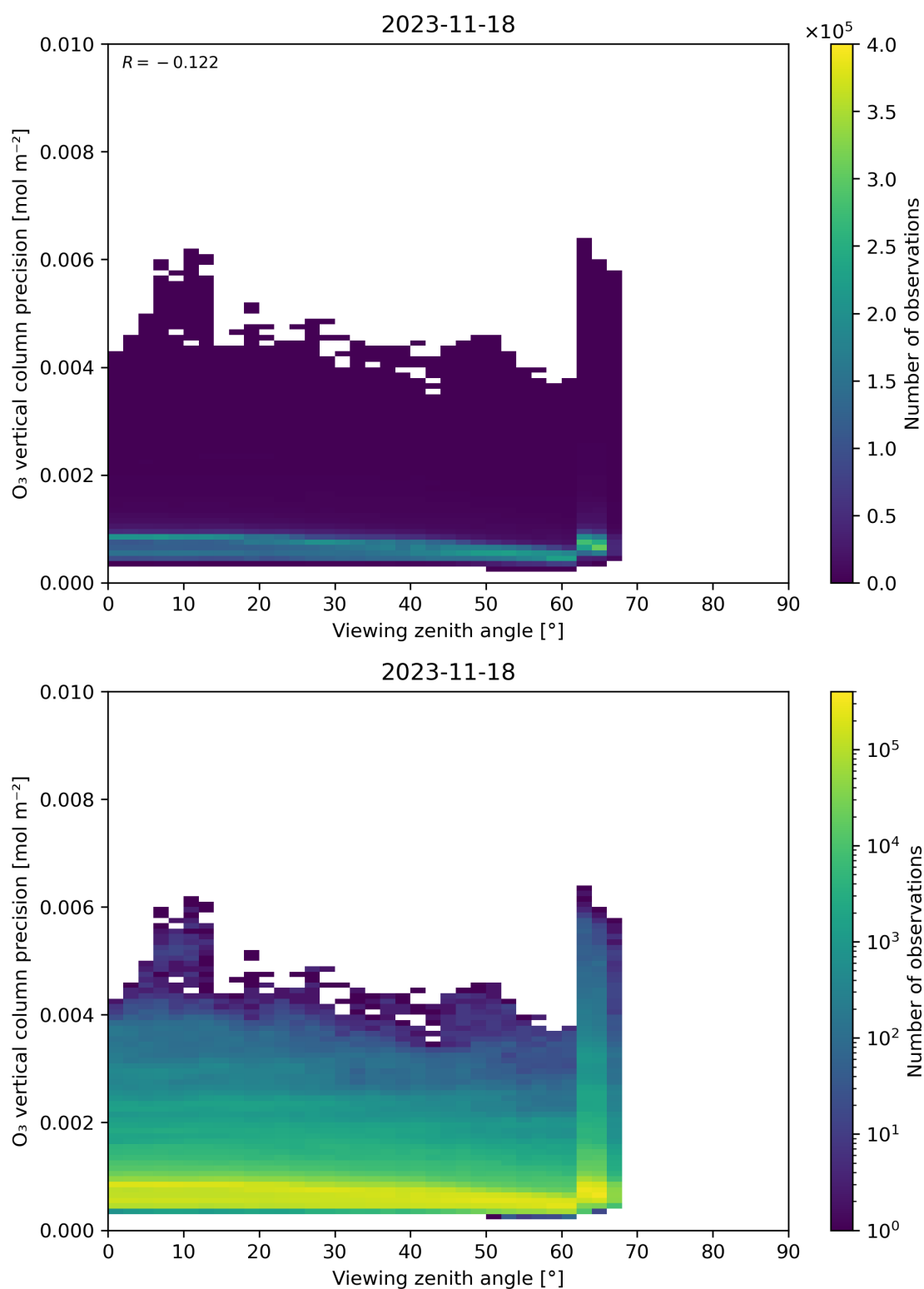
Figure 53: Scatter density plot of “Viewing zenith angle” against “O 3 vertical column precision” for 2023-11-18 to 2023-11-19.
