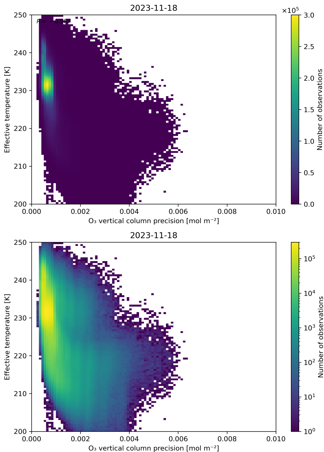
Figure 42: Scatter density plot of “O 3 vertical column precision” against “Effective temperature” for 2023-11-18 to 2023-11-19.
