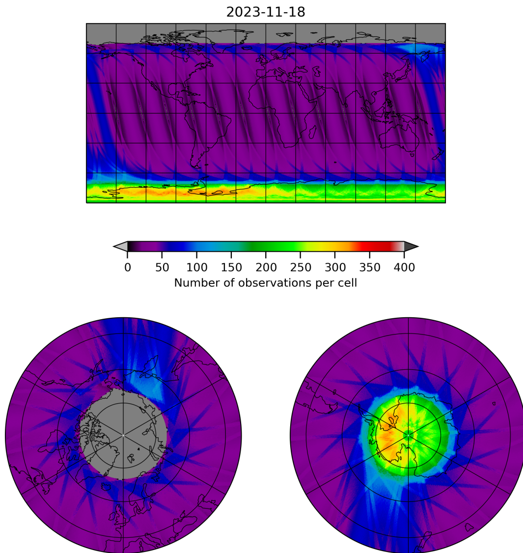
Figure 12: Map of the number of observations for 2023-11-18 to 2023-11-19
