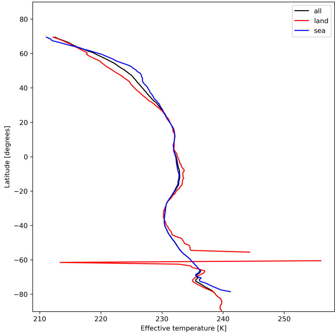
Figure 17: Zonal average of “Effective temperature” for 2023-11-18 to 2023-11-19.
