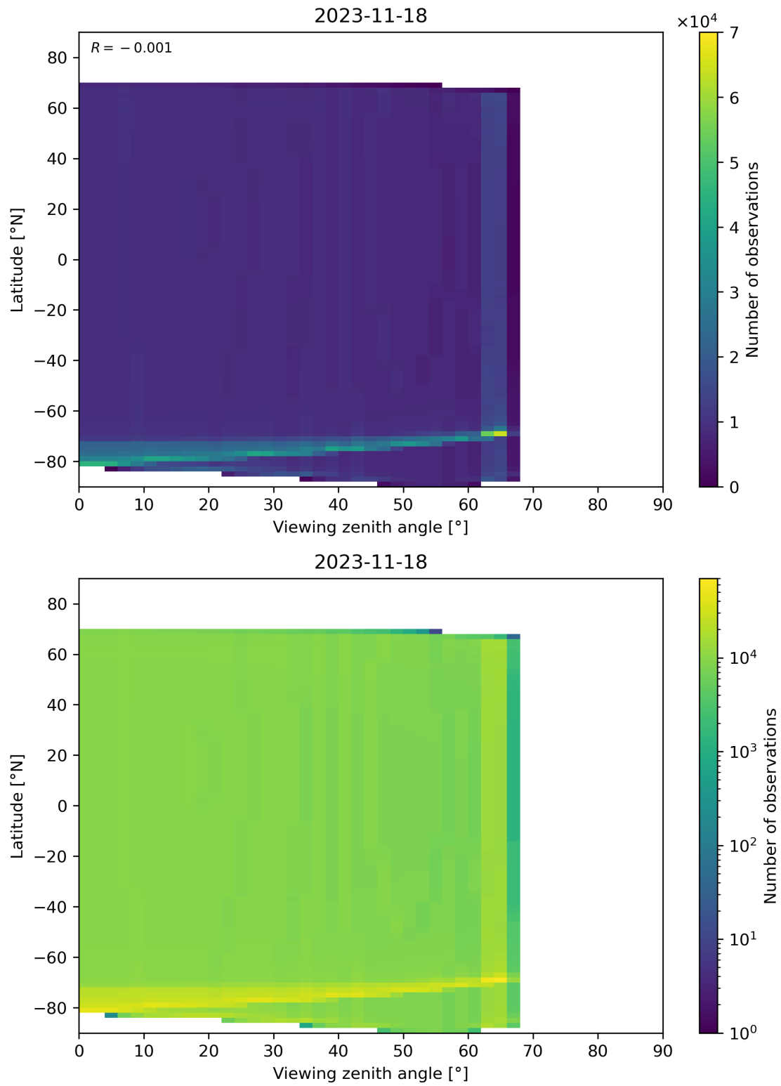
Figure 49: Scatter density plot of “Viewing zenith angle” against “Latitude” for 2023-11-18 to 2023-11-19.
