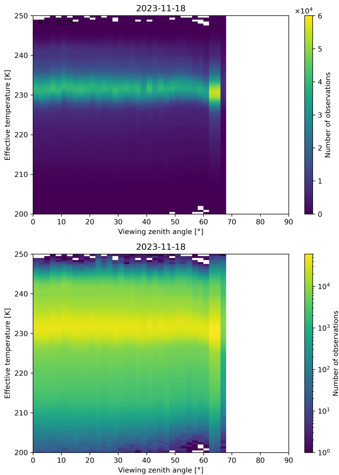
Figure 50: Scatter density plot of “Viewing zenith angle” against “Effective temperature” for 2023-11-18 to 2023-11-19.
