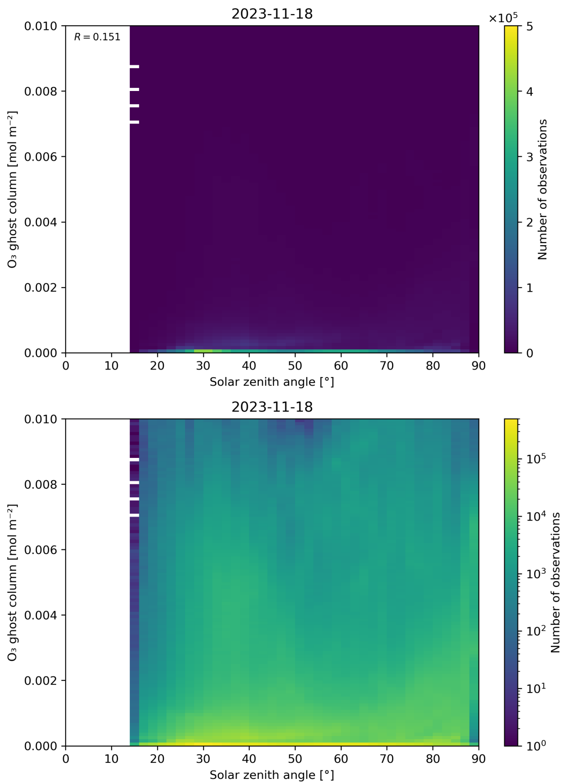
Figure 46: Scatter density plot of “Solar zenith angle” against “O 3 ghost column” for 2023-11-18 to 2023-11-19.
