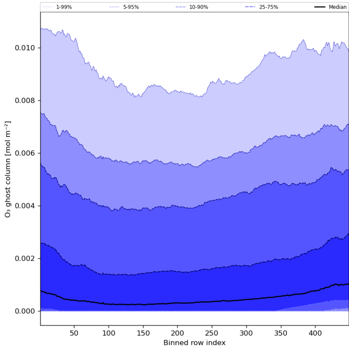
Figure 32: Along track statistics of “O 3 ghost column” for 2023-11-18 to 2023-11-19
