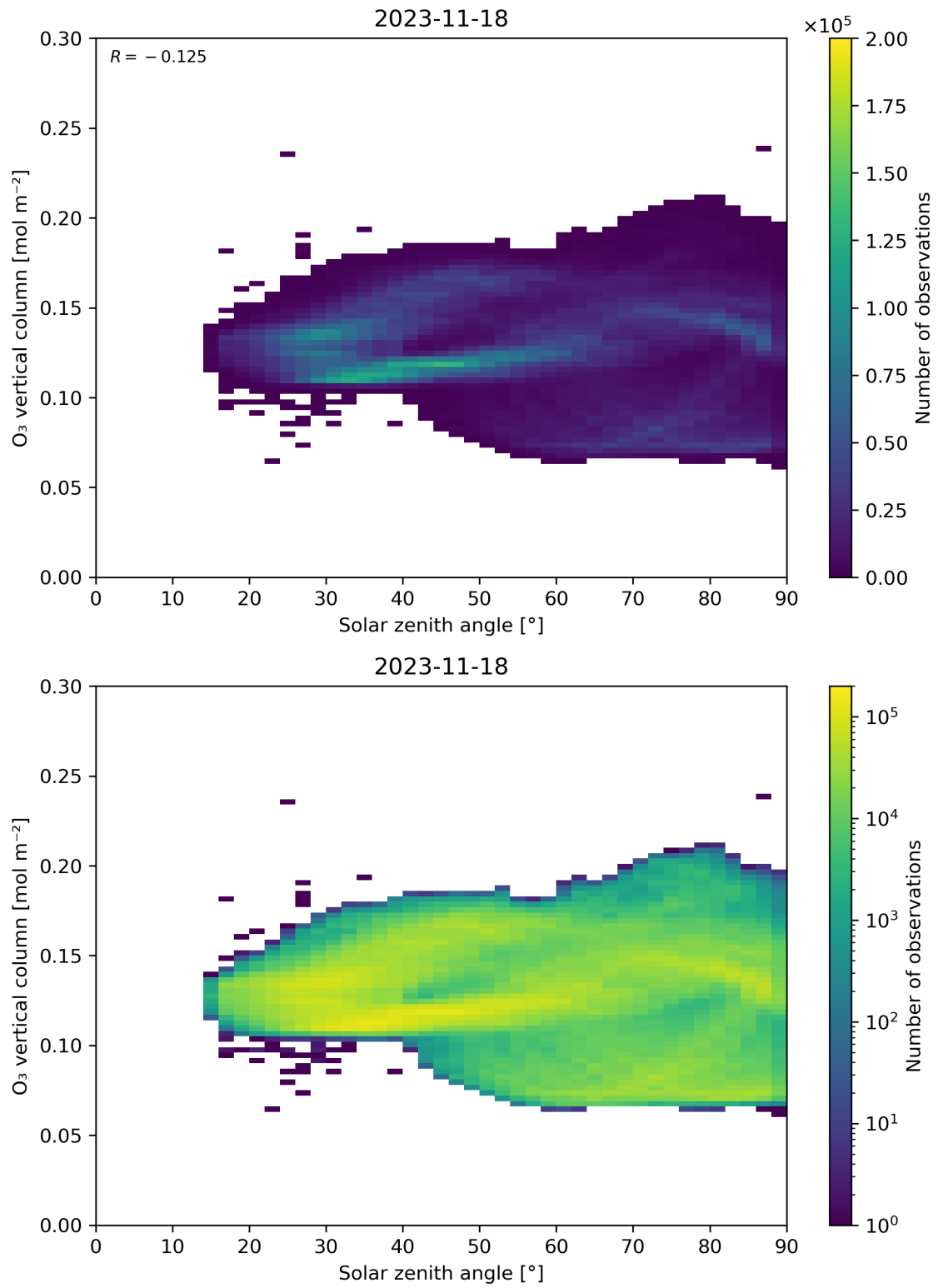
Figure 47: Scatter density plot of “Solar zenith angle” against “O 3 vertical column” for 2023-11-18 to 2023-11-19.
