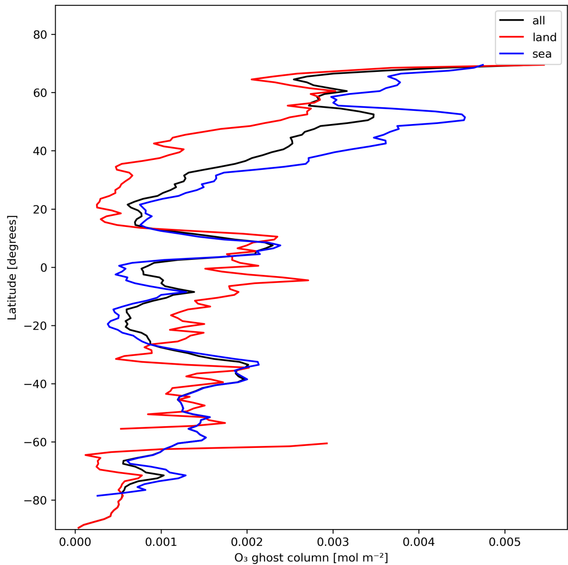
Figure 18: Zonal average of “O 3 ghost column” for 2023-11-18 to 2023-11-19.
