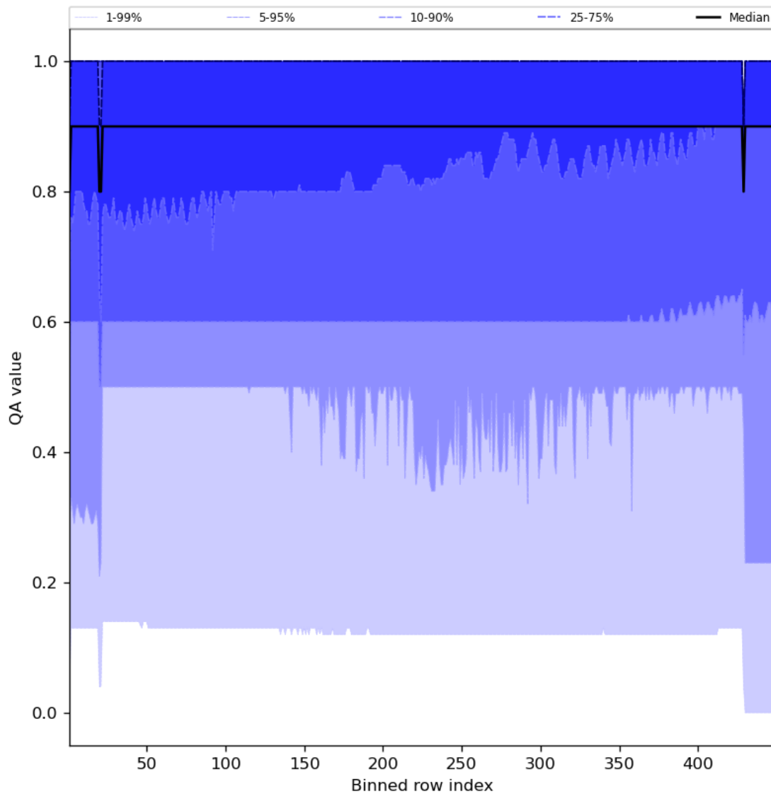
Figure 27: Along track statistics of “QA value” for 2023-11-18 to 2023-11-19
