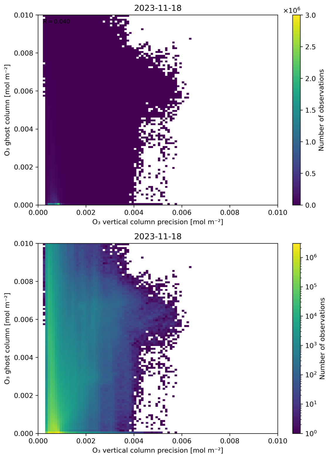
Figure 43: Scatter density plot of “O 3 vertical column precision” against “O 3 ghost column” for 2023-11-18 to 2023-11-19.
