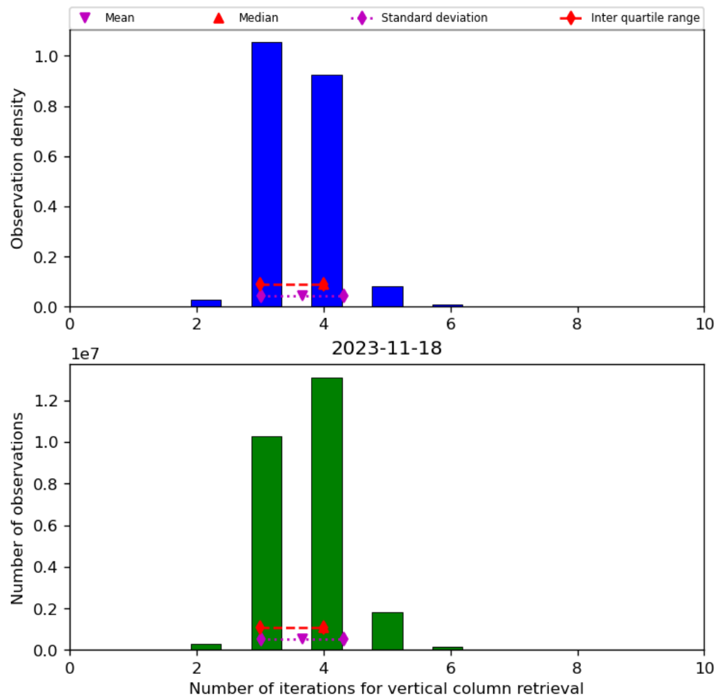
Figure 26: Histogram of “Number of iterations for vertical column retrieval” for 2023-11-18 to 2023-11-19
