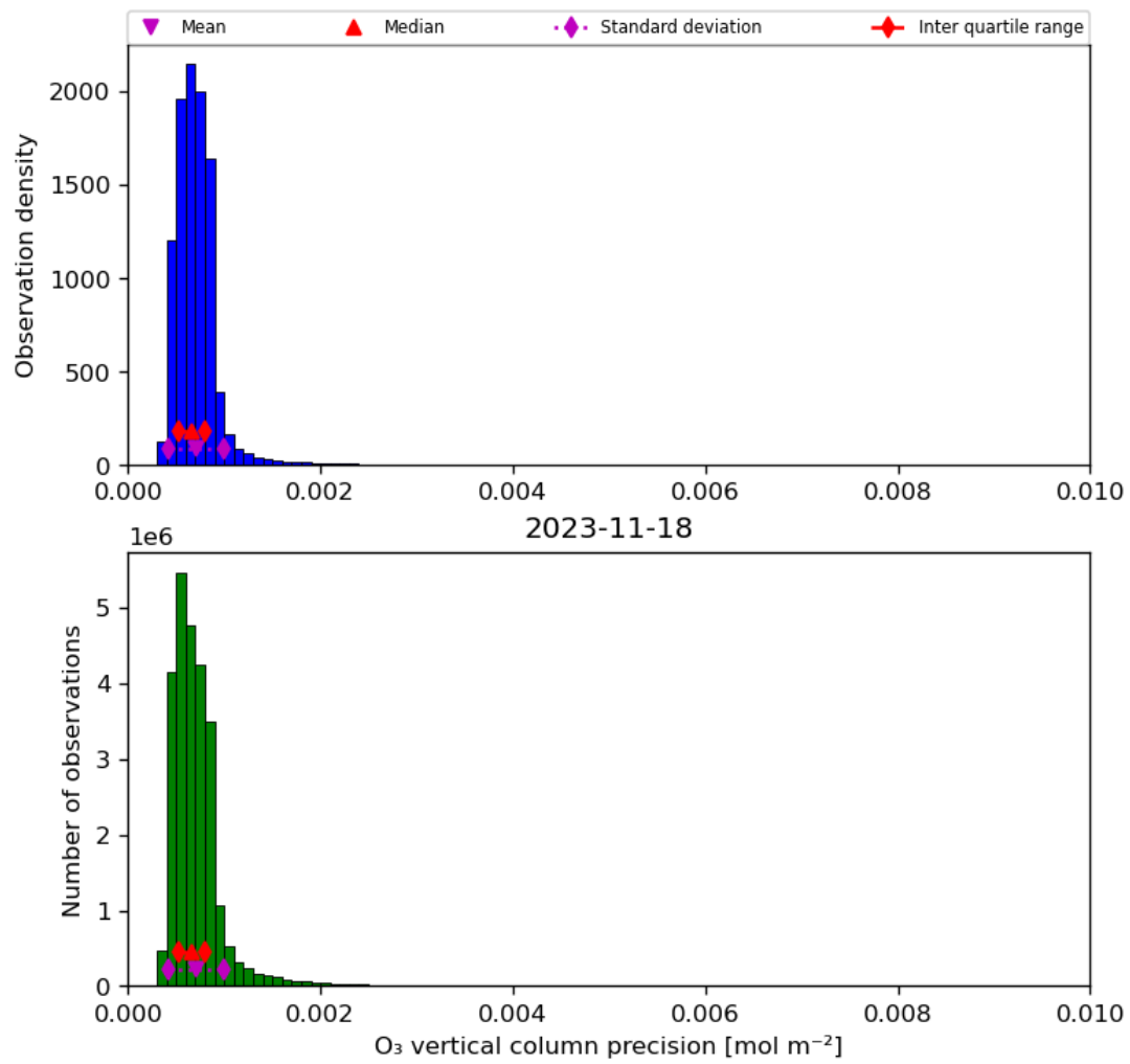
Figure 22: Histogram of “O 3 vertical column precision” for 2023-11-18 to 2023-11-19
