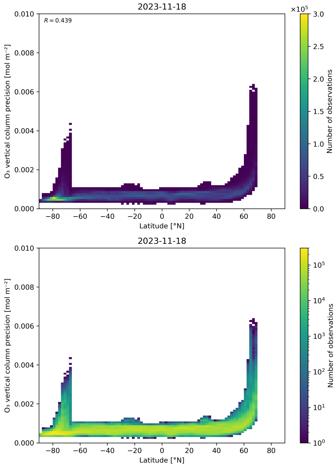
Figure 37: Scatter density plot of “Latitude” against “O 3 vertical column precision” for 2023-11-18 to 2023-11-19.
