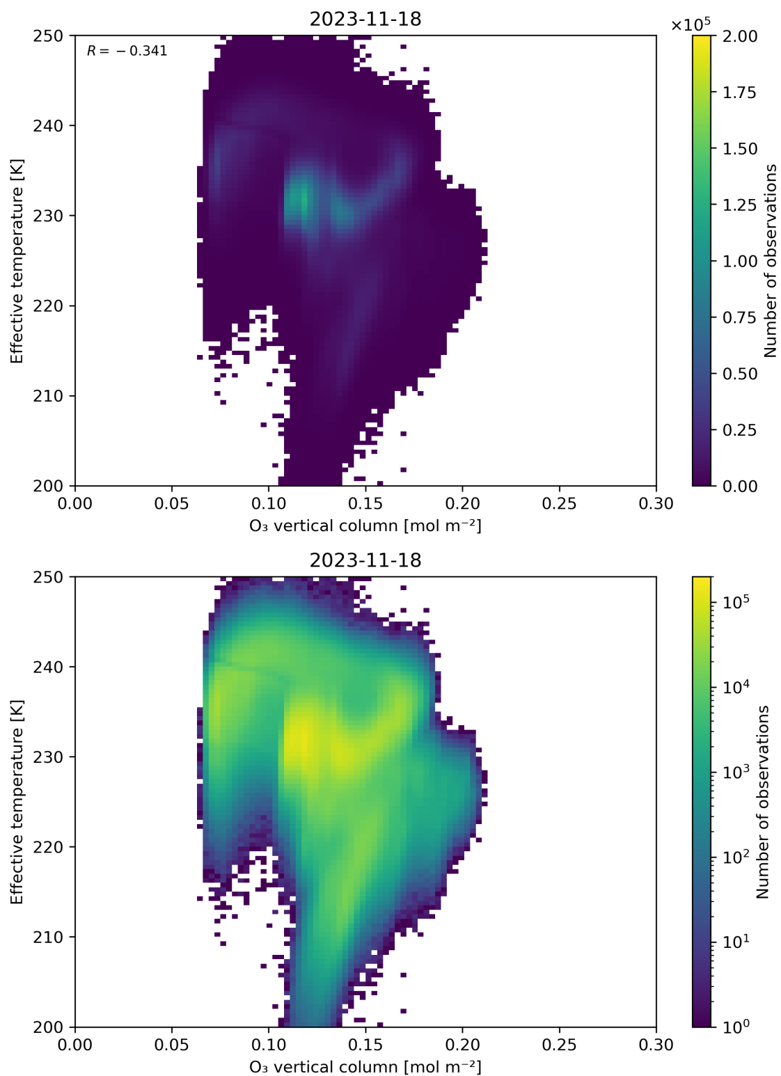
Figure 39: Scatter density plot of “O 3 vertical column” against “Effective temperature” for 2023-11-18 to 2023-11-19.
