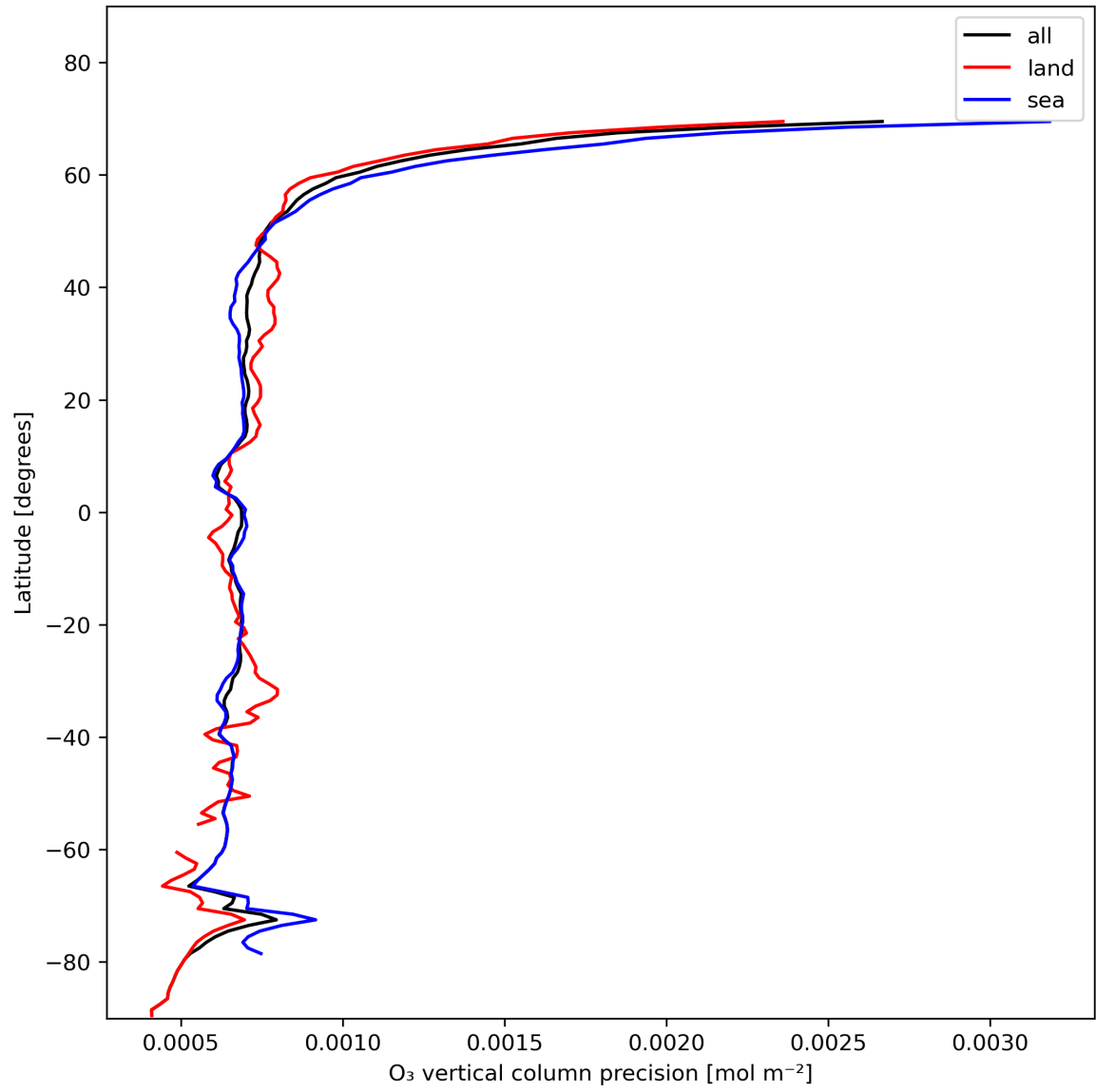
Figure 15: Zonal average of “O 3 vertical column precision” for 2023-11-18 to 2023-11-19.
