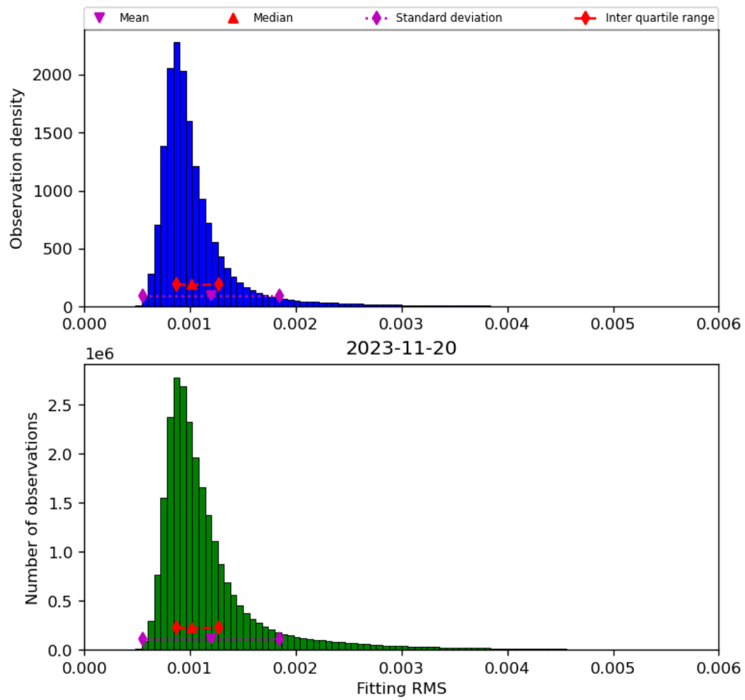
Figure 23: Histogram of “Fitting RMS” for 2023-11-19 to 2023-11-21
