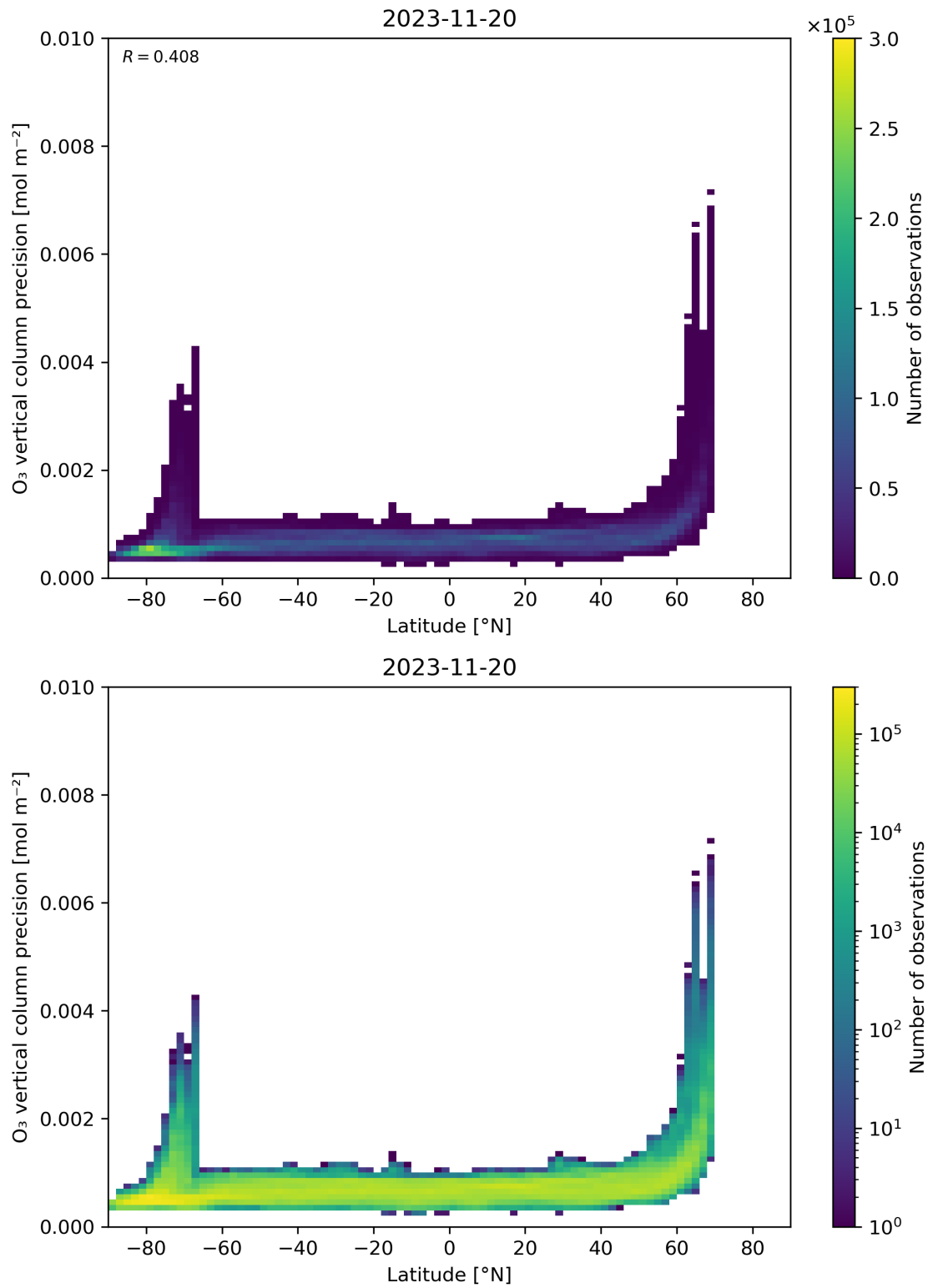
Figure 37: Scatter density plot of “Latitude” against “O 3 vertical column precision” for 2023-11-19 to 2023-11-21.
