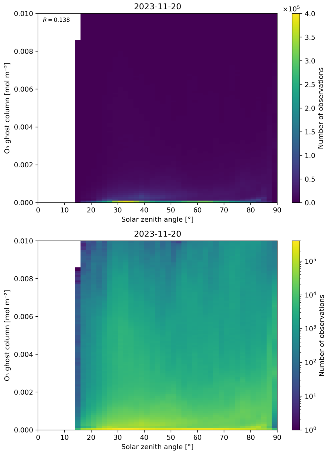
Figure 46: Scatter density plot of “Solar zenith angle” against “O 3 ghost column” for 2023-11-19 to 2023-11-21.
