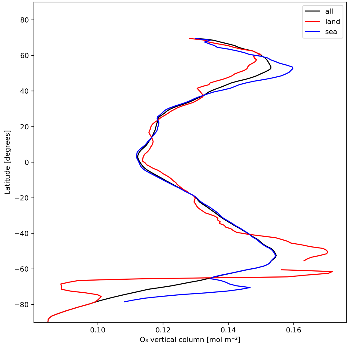
Figure 14: Zonal average of “O 3 vertical column” for 2023-11-19 to 2023-11-21.
