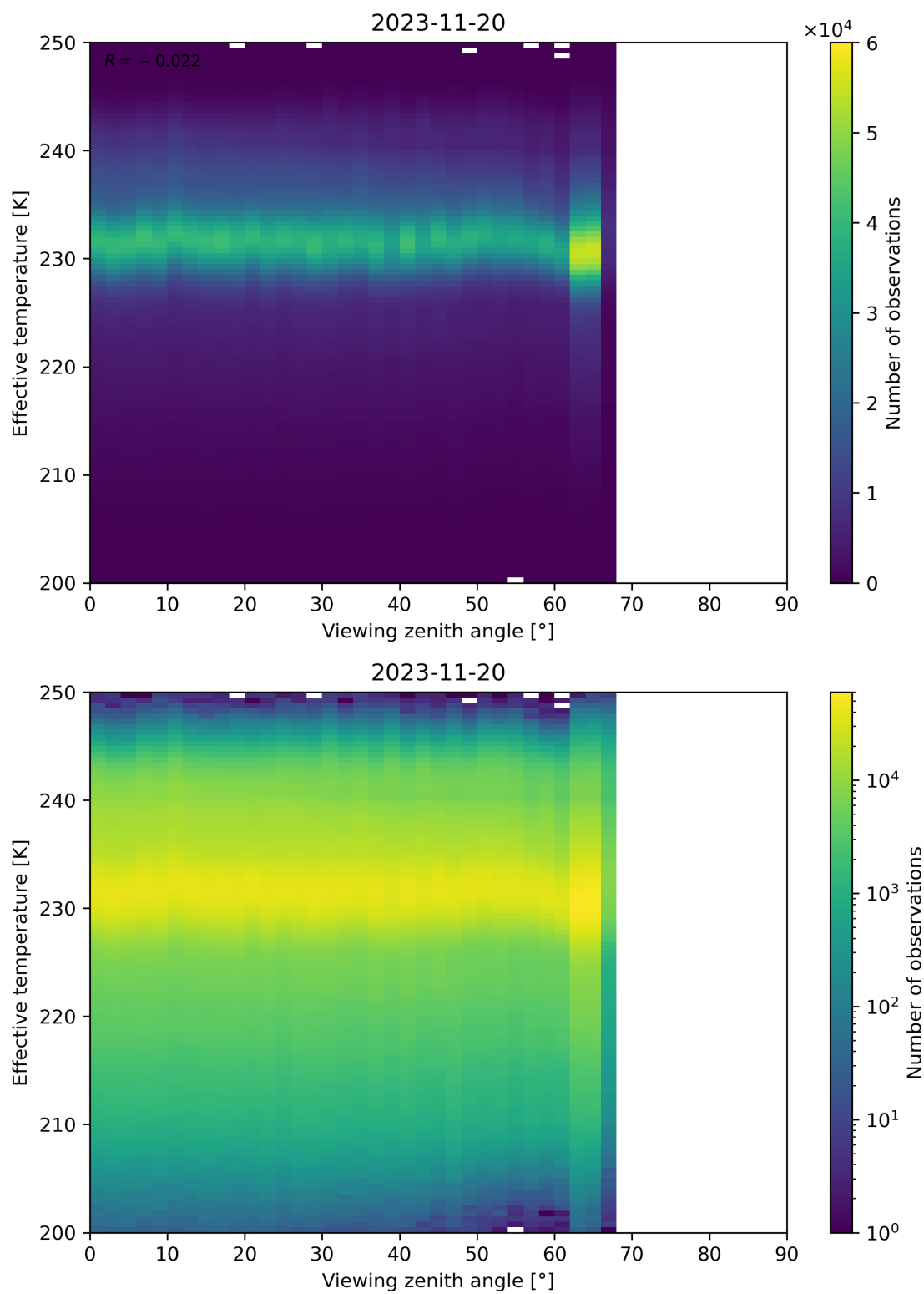
Figure 50: Scatter density plot of “Viewing zenith angle” against “Effective temperature” for 2023-11-19 to 2023-11-21.
