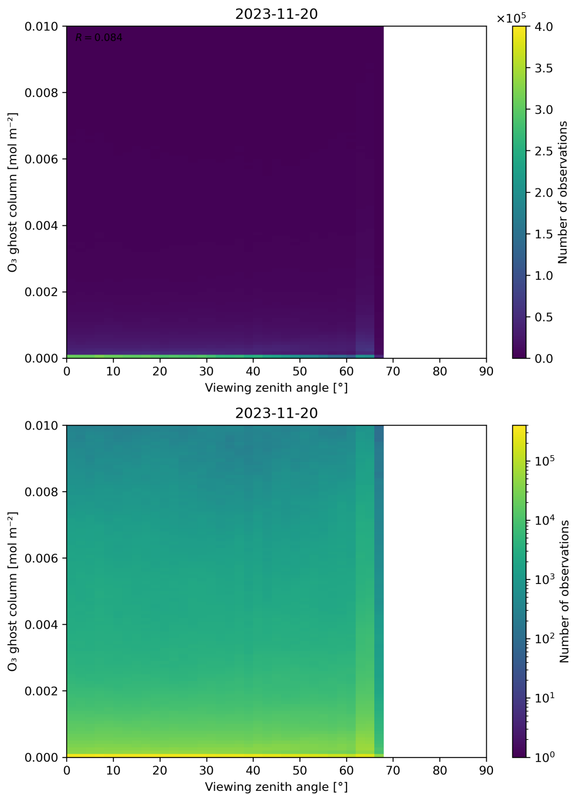
Figure 51: Scatter density plot of “Viewing zenith angle” against “O 3 ghost column” for 2023-11-19 to 2023-11-21.
