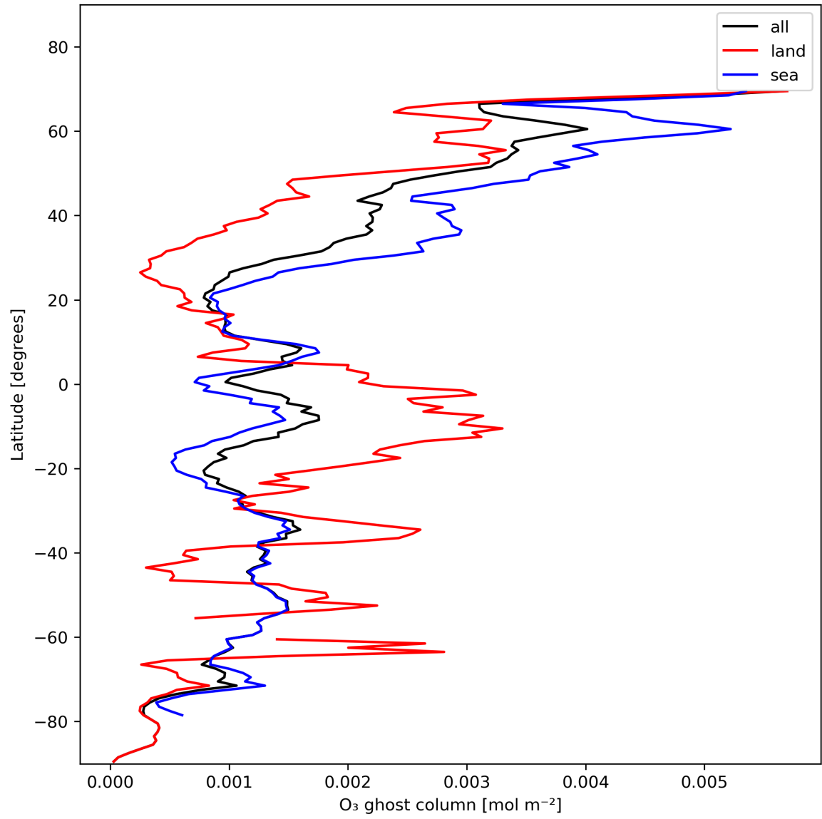
Figure 18: Zonal average of “O 3 ghost column” for 2023-11-19 to 2023-11-21.
