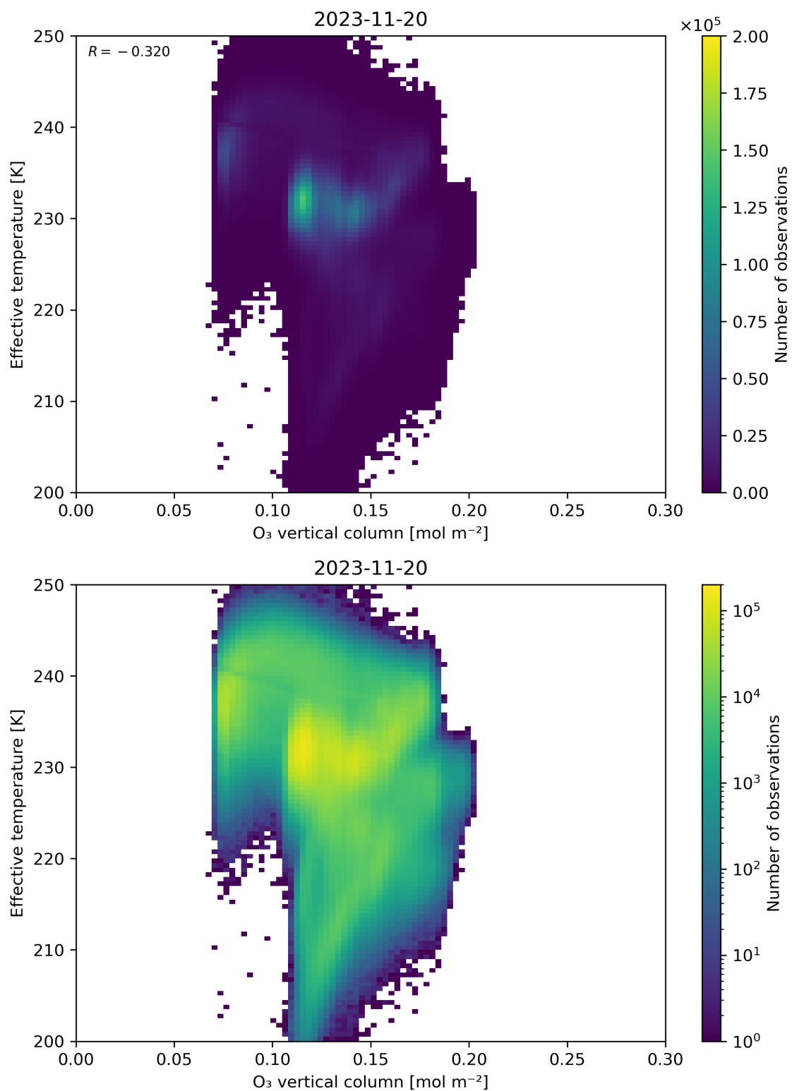
Figure 39: Scatter density plot of “O 3 vertical column” against “Effective temperature” for 2023-11-19 to 2023-11-21.
