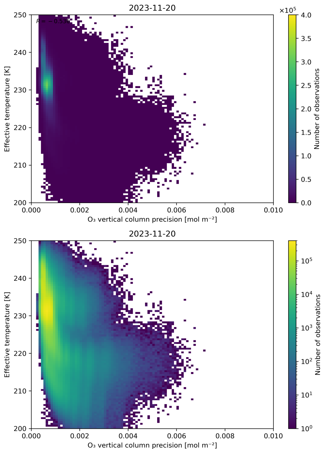
Figure 42: Scatter density plot of “O 3 vertical column precision” against “Effective temperature” for 2023-11-19 to 2023-11-21.
