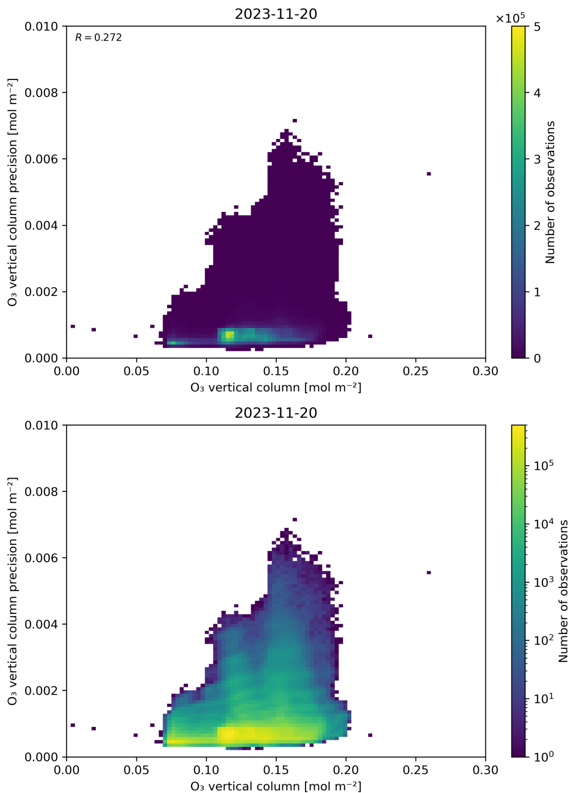
Figure 41: Scatter density plot of “O 3 vertical column” against “O 3 vertical column precision” for 2023-11-19 to 2023-11-21.
