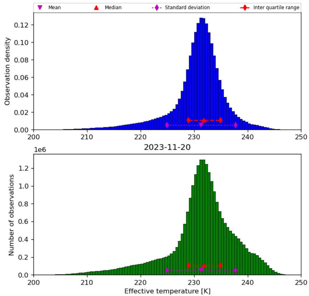
Figure 24: Histogram of “Effective temperature” for 2023-11-19 to 2023-11-21
