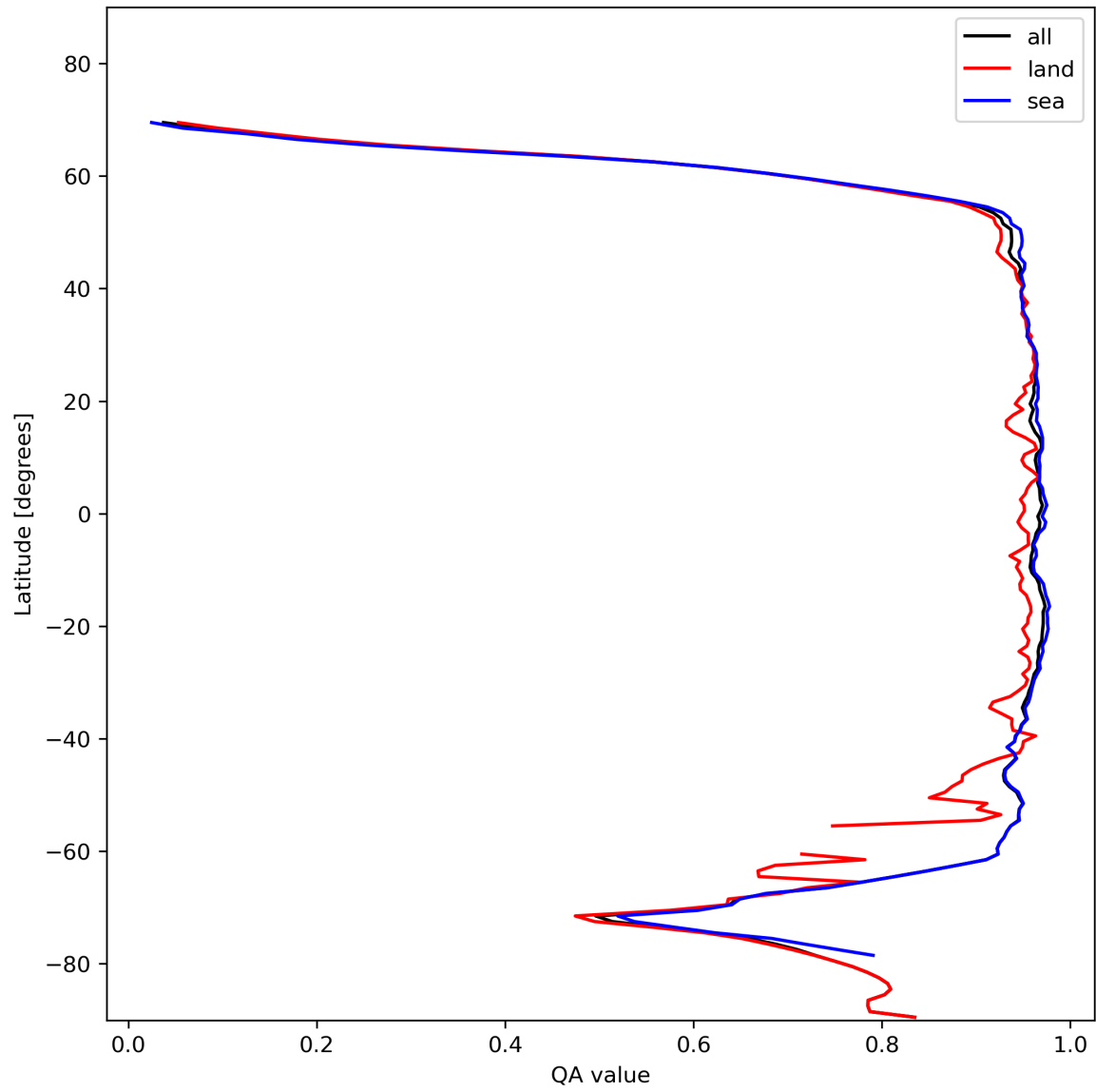
Figure 13: Zonal average of “QA value” for 2023-11-19 to 2023-11-21.
