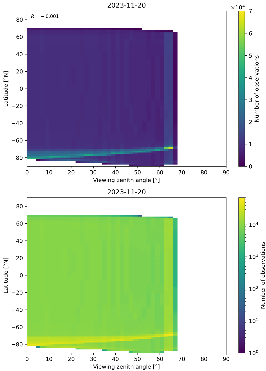
Figure 49: Scatter density plot of “Viewing zenith angle” against “Latitude” for 2023-11-19 to 2023-11-21.
