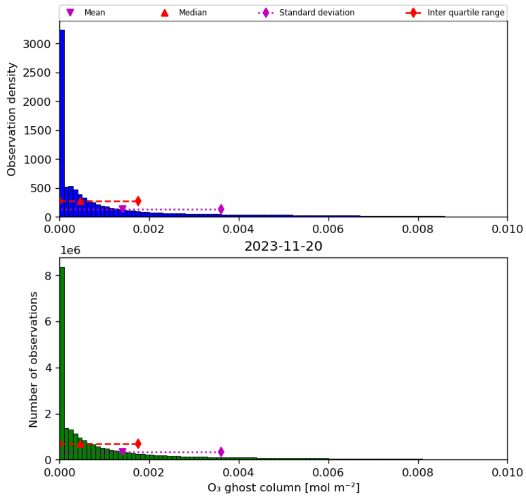
Figure 25: Histogram of "O 3 ghost column" for 2023-11-19 to 2023-11-21
