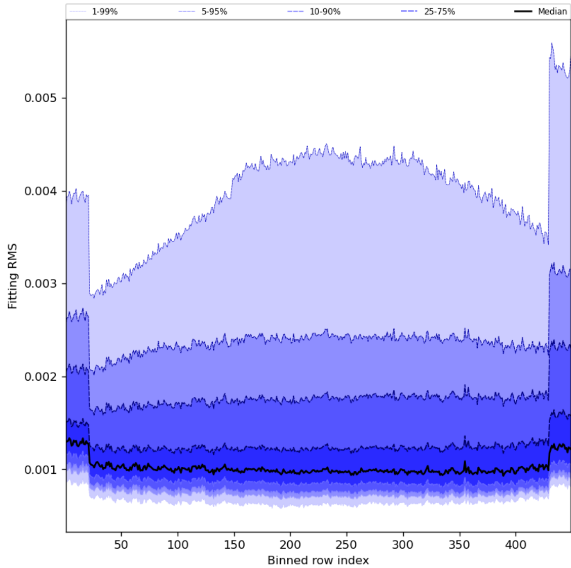
Figure 30: Along track statistics of “Fitting RMS” for 2023-11-19 to 2023-11-21
