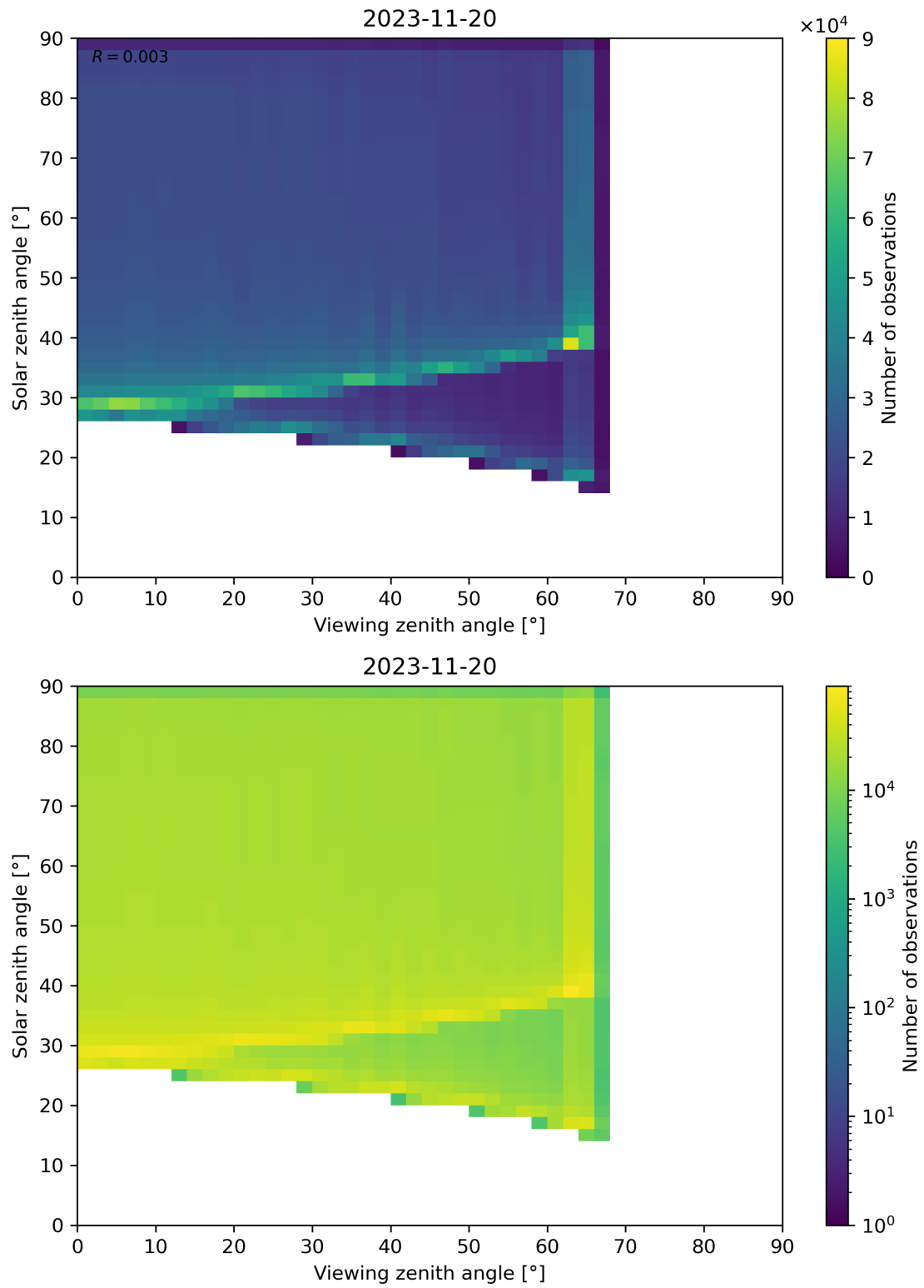
Figure 54: Scatter density plot of “Viewing zenith angle” against “Solar zenith angle” for 2023-11-19 to 2023-11-21.
