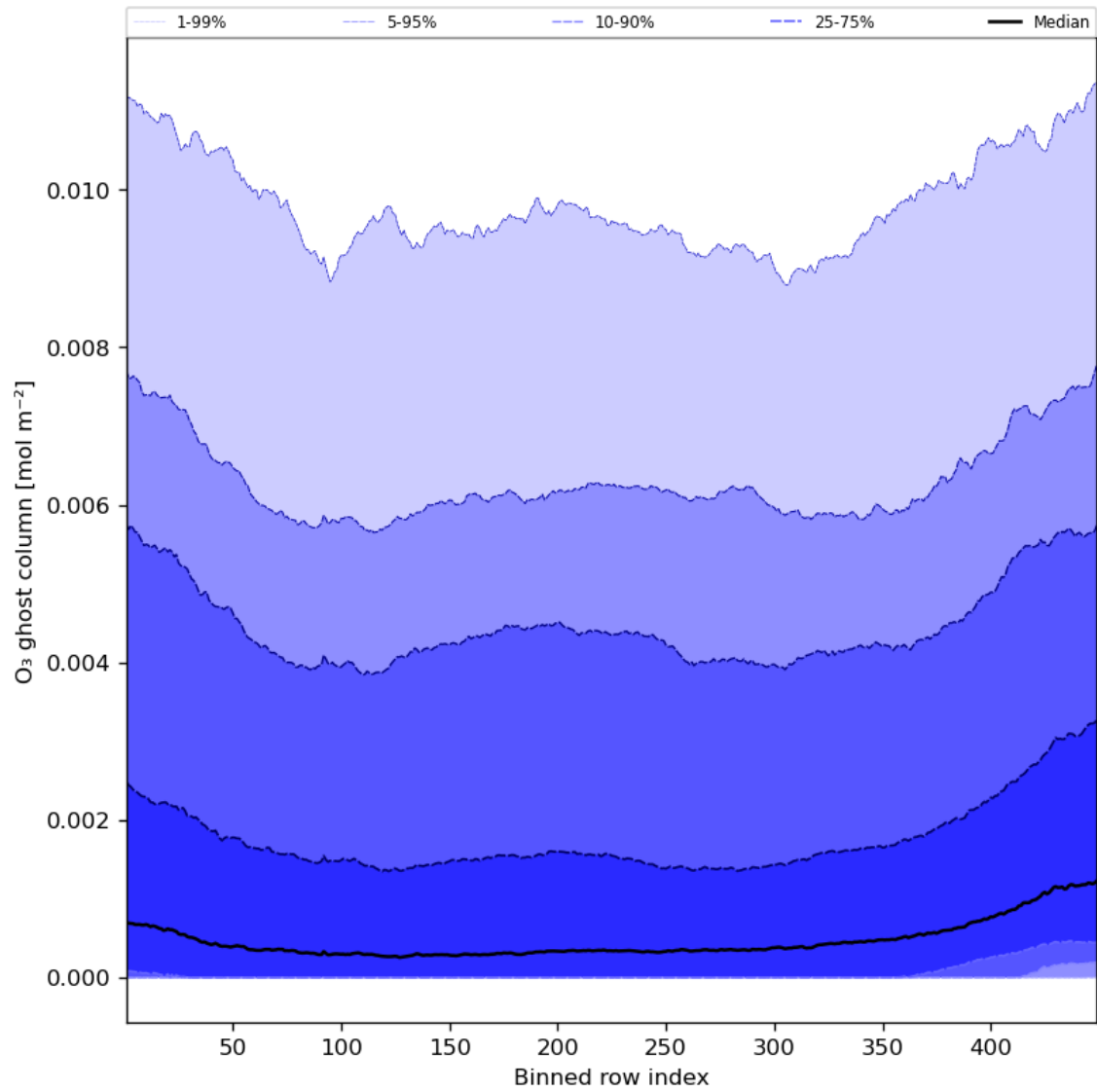
Figure 32: Along track statistics of “O 3 ghost column” for 2023-11-19 to 2023-11-21
