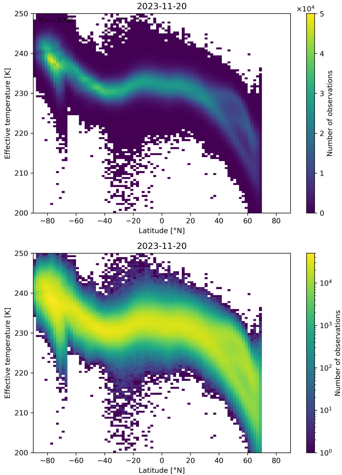
Figure 34: Scatter density plot of “Latitude” against “Effective temperature” for 2023-11-19 to 2023-11-21.
