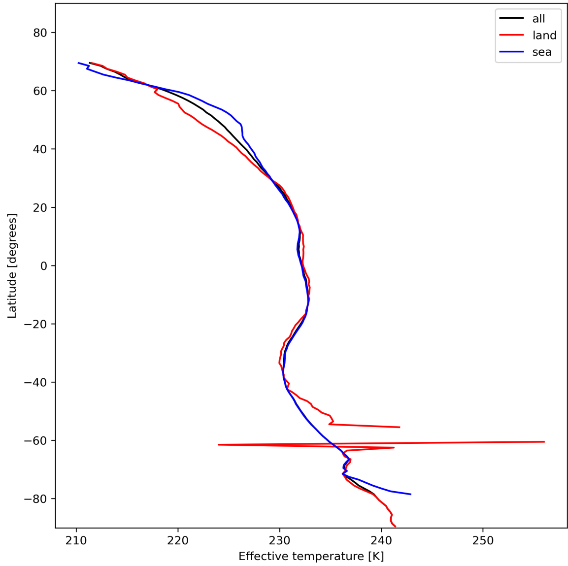
Figure 17: Zonal average of “Effective temperature” for 2023-11-19 to 2023-11-21.
