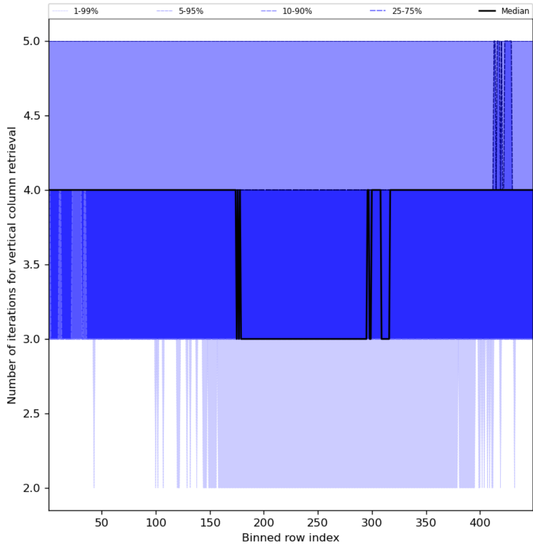
Figure 33: Along track statistics of “Number of iterations for vertical column retrieval” for 2023-11-19 to 2023-11-21
