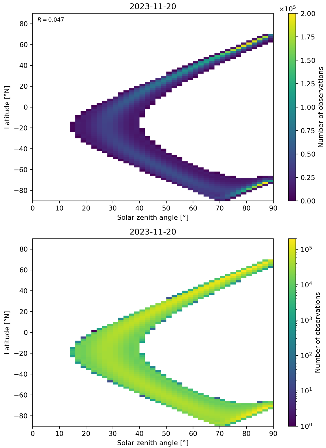
Figure 44: Scatter density plot of “Solar zenith angle” against “Latitude” for 2023-11-19 to 2023-11-21.
