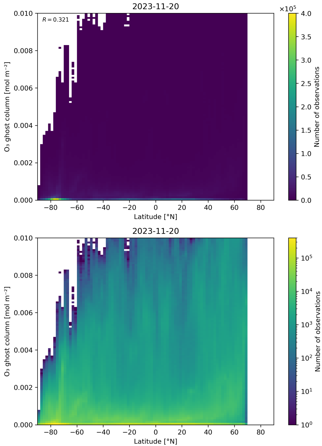
Figure 35: Scatter density plot of “Latitude” against “O 3 ghost column” for 2023-11-19 to 2023-11-21.
