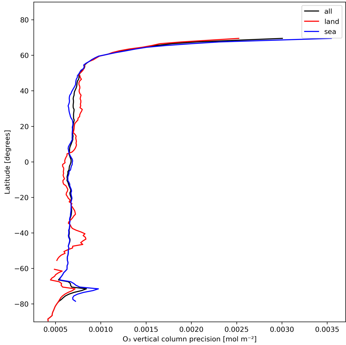
Figure 15: Zonal average of “O 3 vertical column precision” for 2023-11-19 to 2023-11-21.
