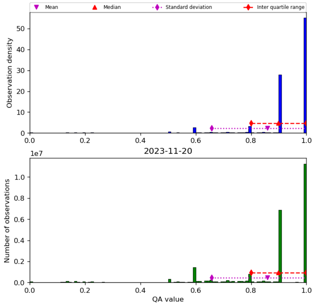
Figure 20: Histogram of “QA value” for 2023-11-19 to 2023-11-21
