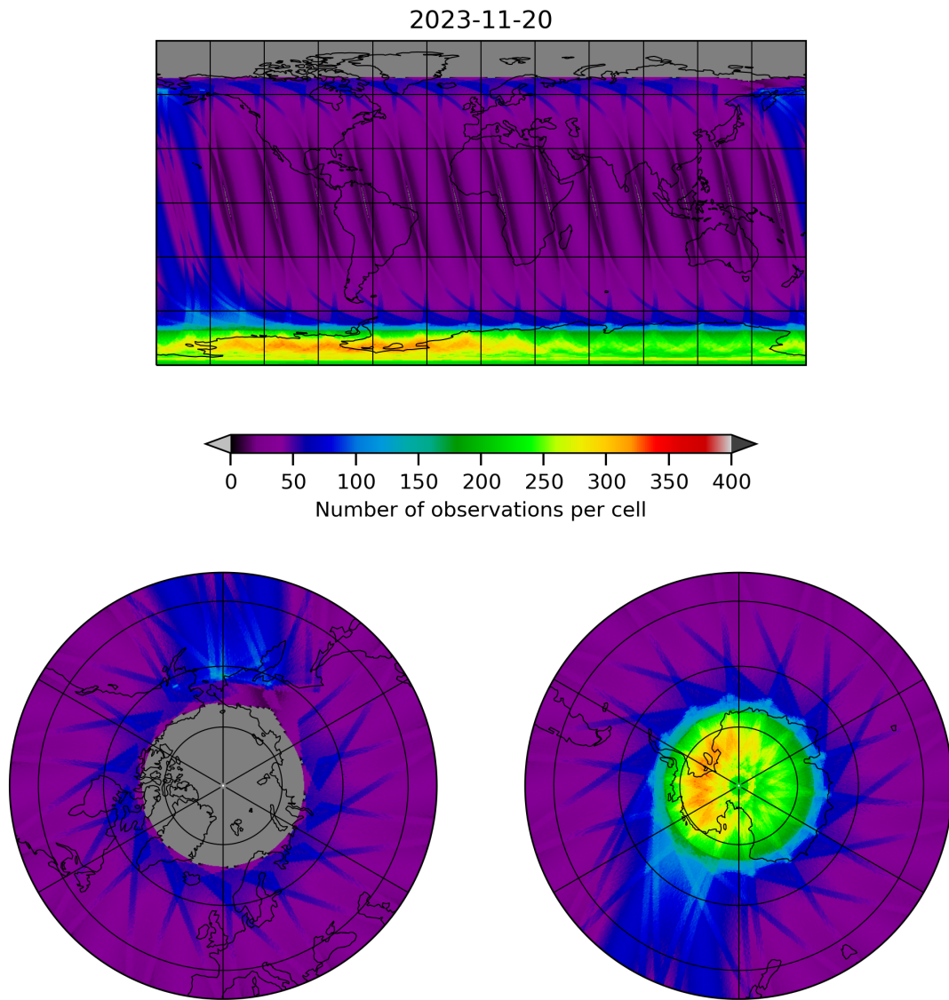
Figure 12: Map of the number of observations for 2023-11-19 to 2023-11-21
