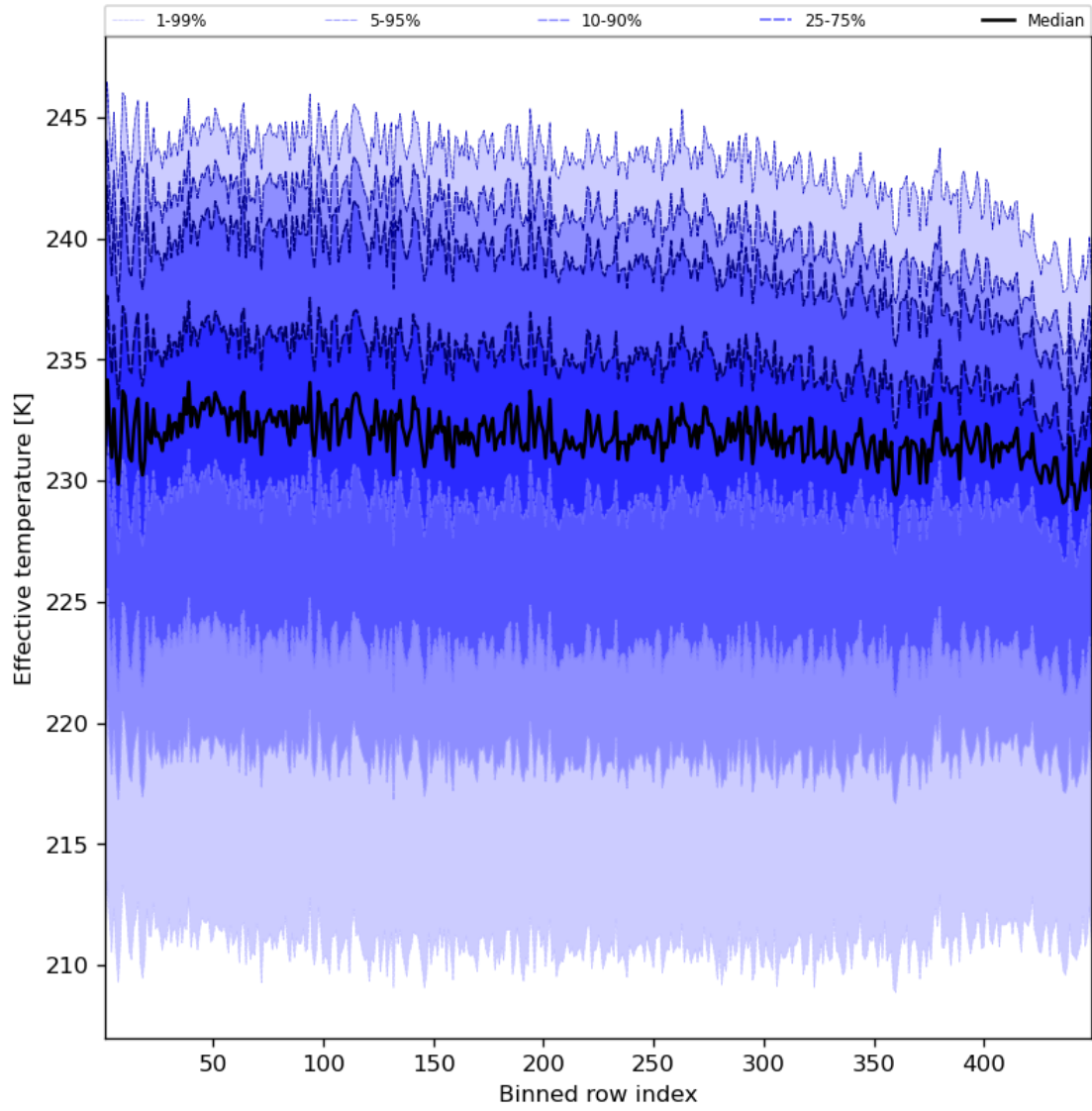
Figure 31: Along track statistics of “Effective temperature” for 2023-11-19 to 2023-11-21
