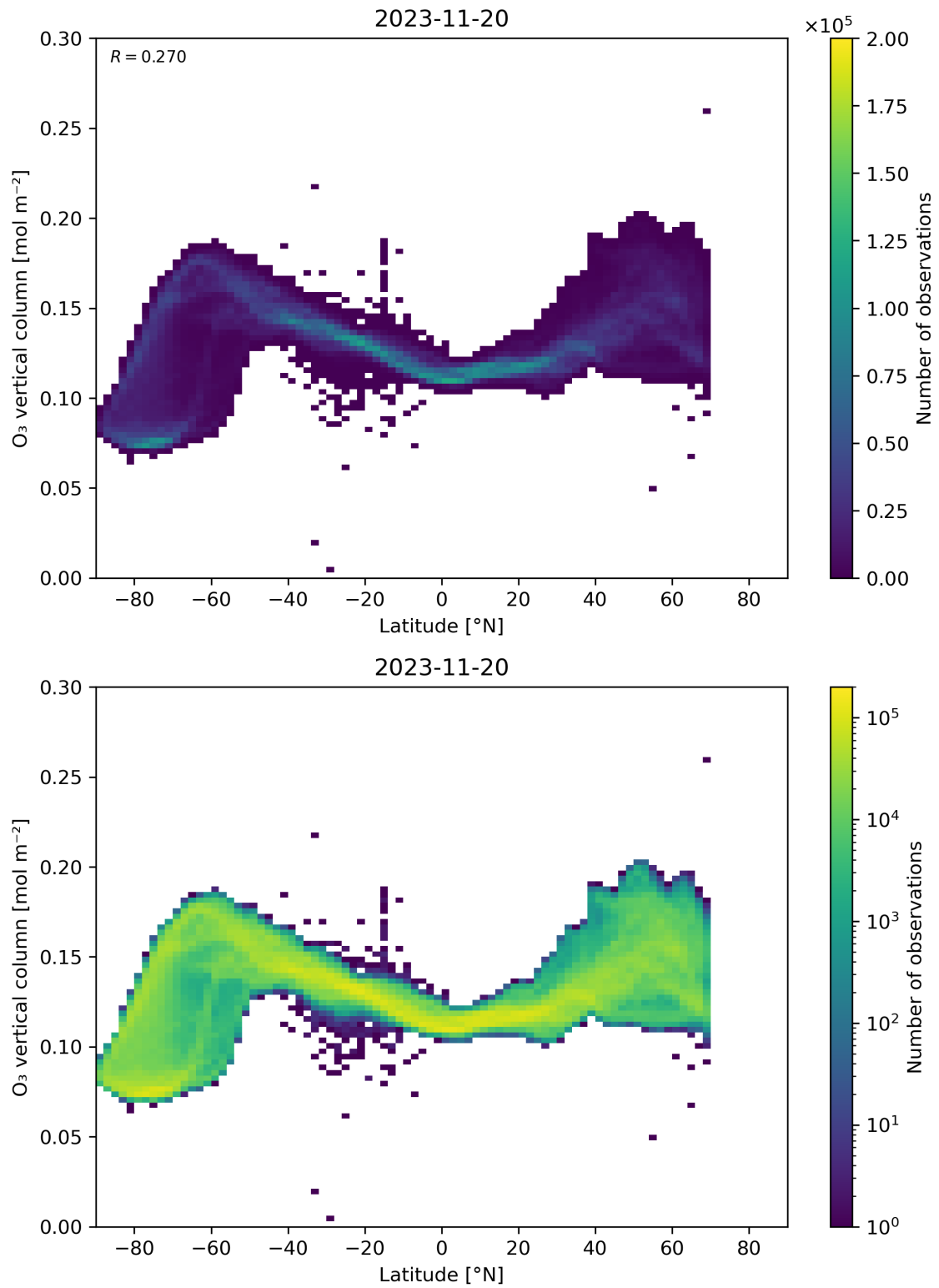
Figure 36: Scatter density plot of “Latitude” against “O 3 vertical column” for 2023-11-19 to 2023-11-21.
