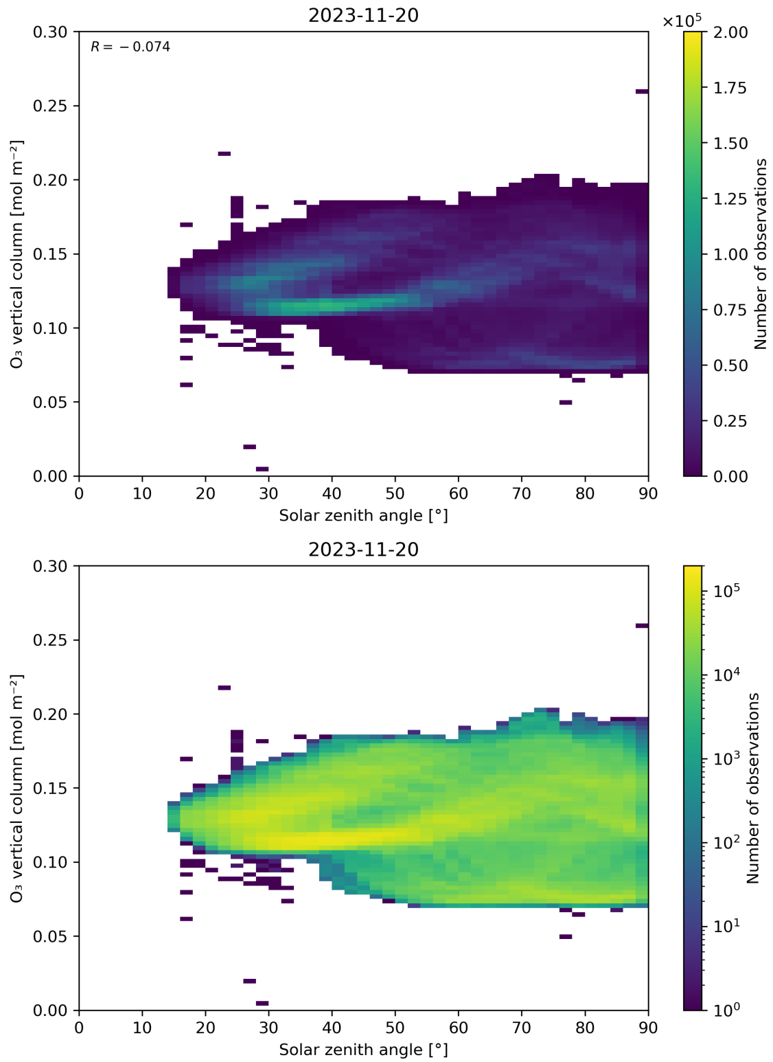
Figure 47: Scatter density plot of “Solar zenith angle” against “O 3 vertical column” for 2023-11-19 to 2023-11-21.
