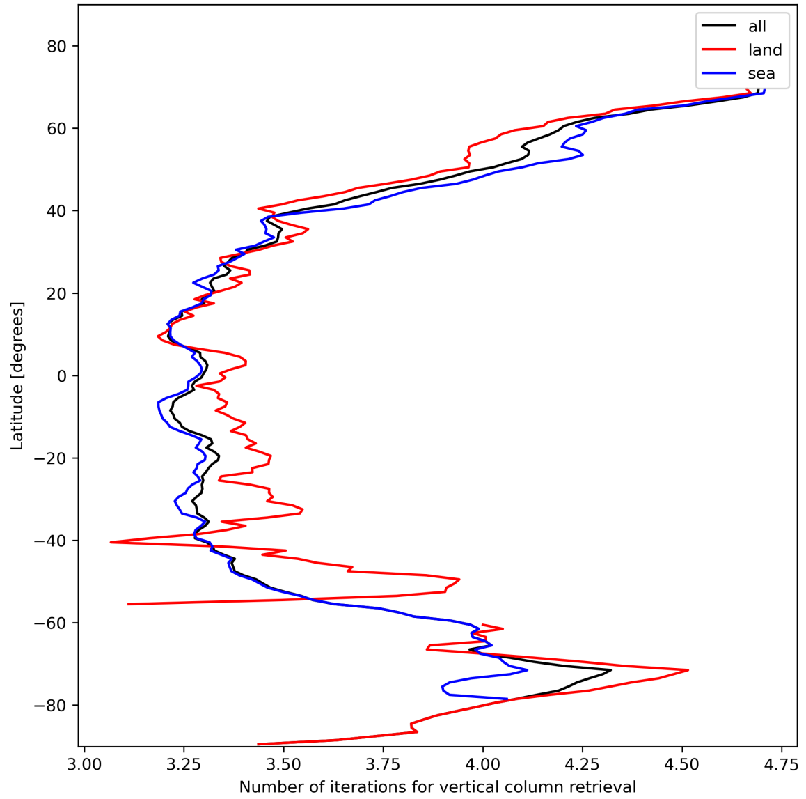
Figure 19: Zonal average of “Number of iterations for vertical column retrieval” for 2023-11-19 to 2023-11-21.
