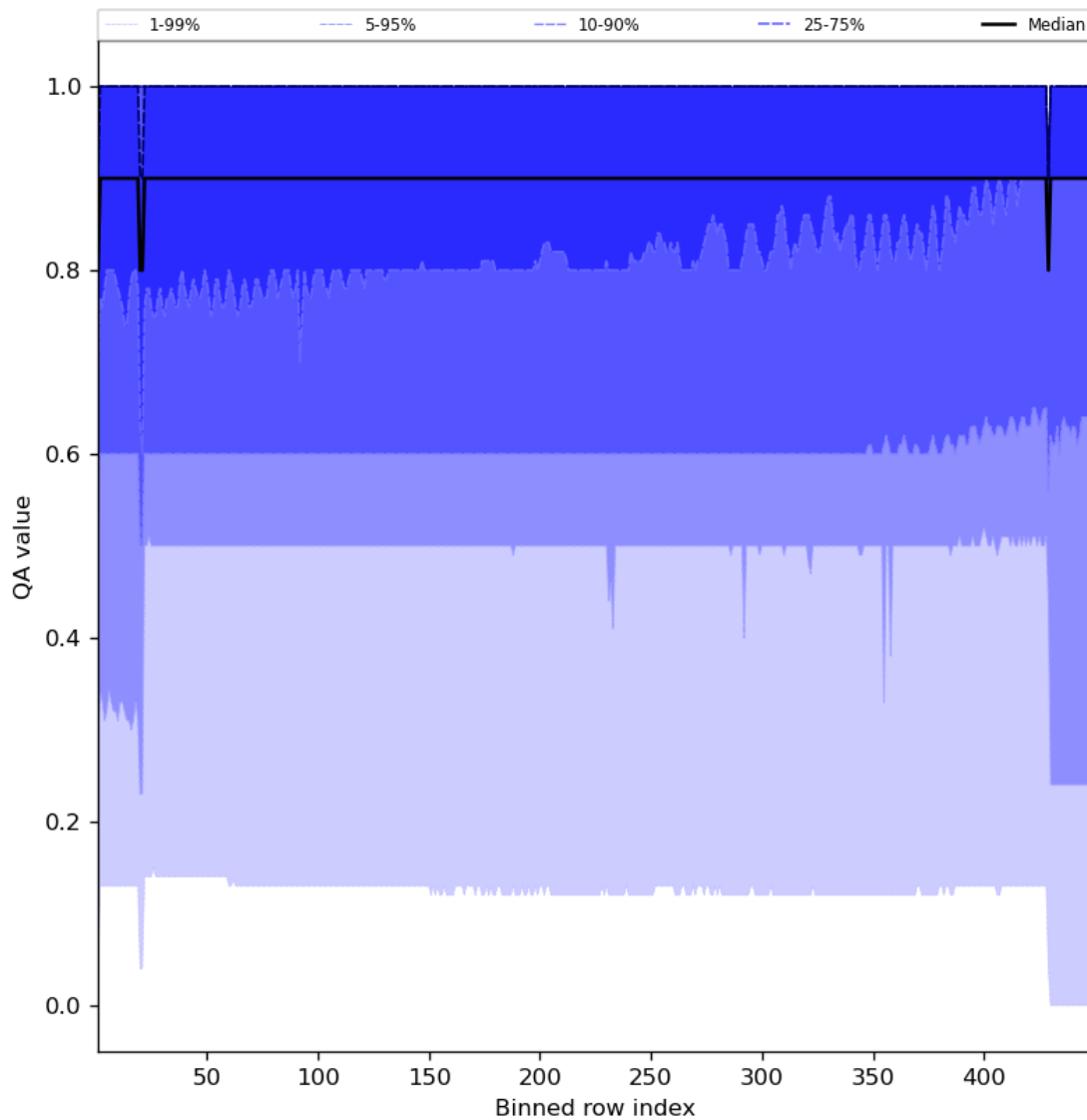
Figure 27: Along track statistics of “QA value” for 2023-11-19 to 2023-11-21
