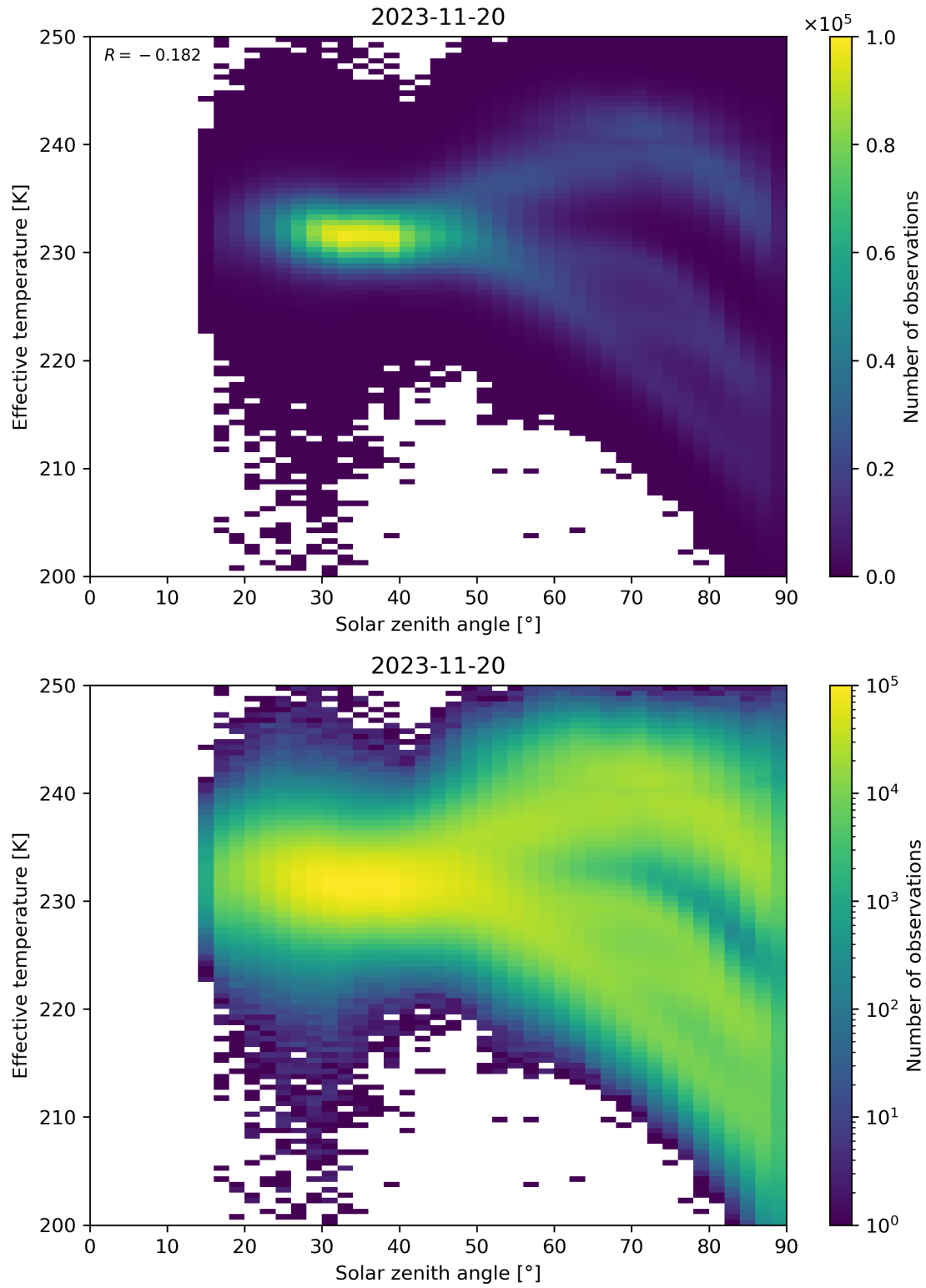
Figure 45: Scatter density plot of “Solar zenith angle” against “Effective temperature” for 2023-11-19 to 2023-11-21.
