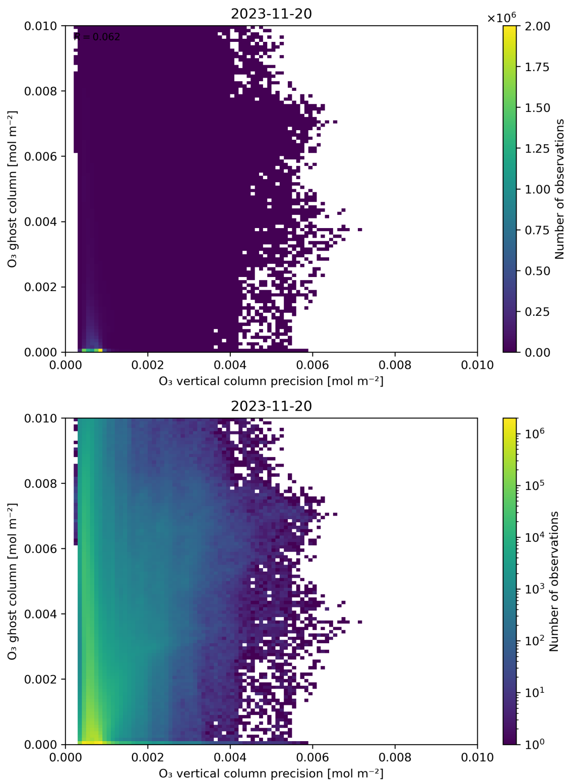
Figure 43: Scatter density plot of “ O_3 vertical column precision” against “ O_3 ghost column” for 2023-11-19 to 2023-11-21.
