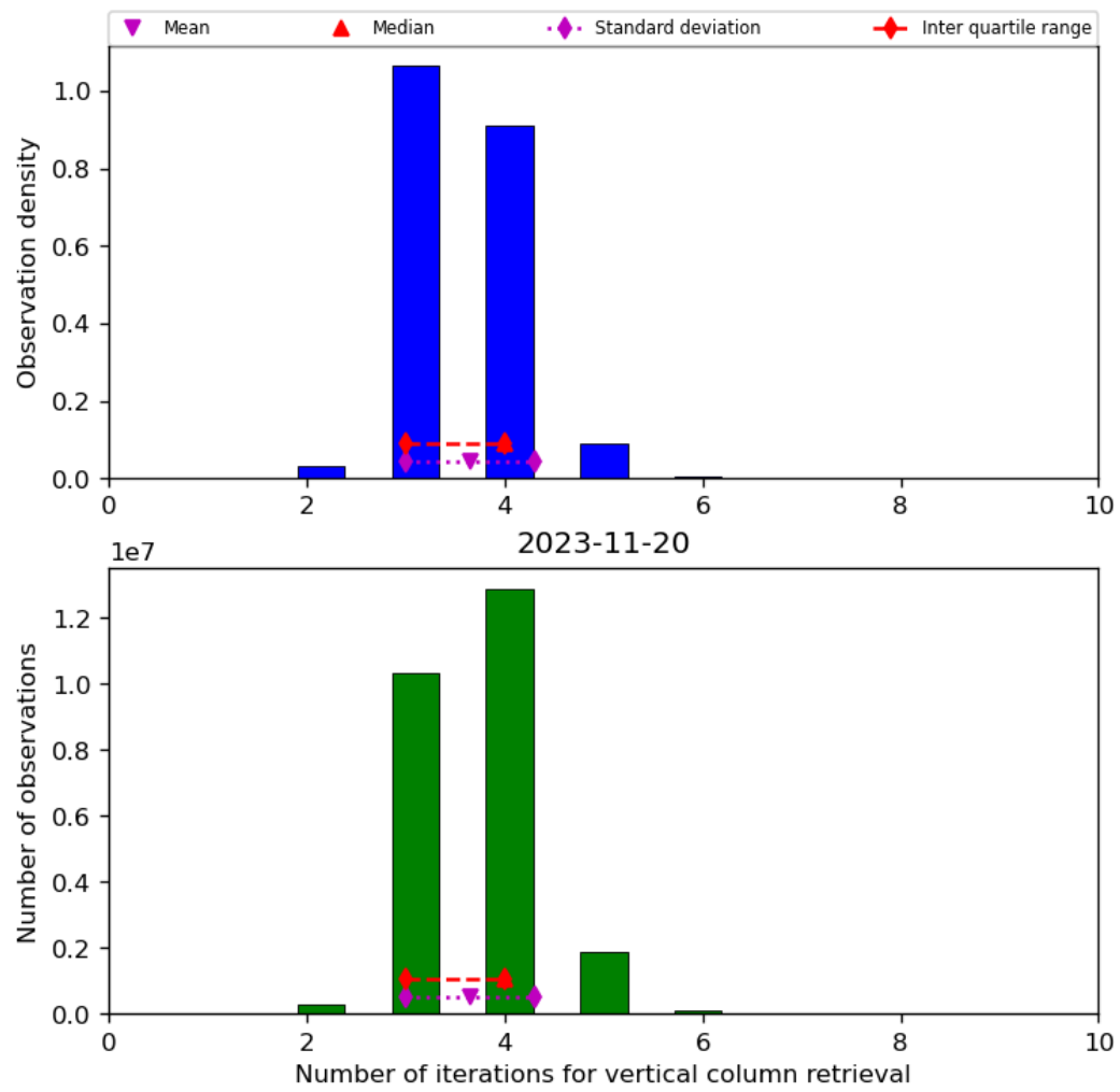
Figure 26: Histogram of “Number of iterations for vertical column retrieval” for 2023-11-19 to 2023-11-21
