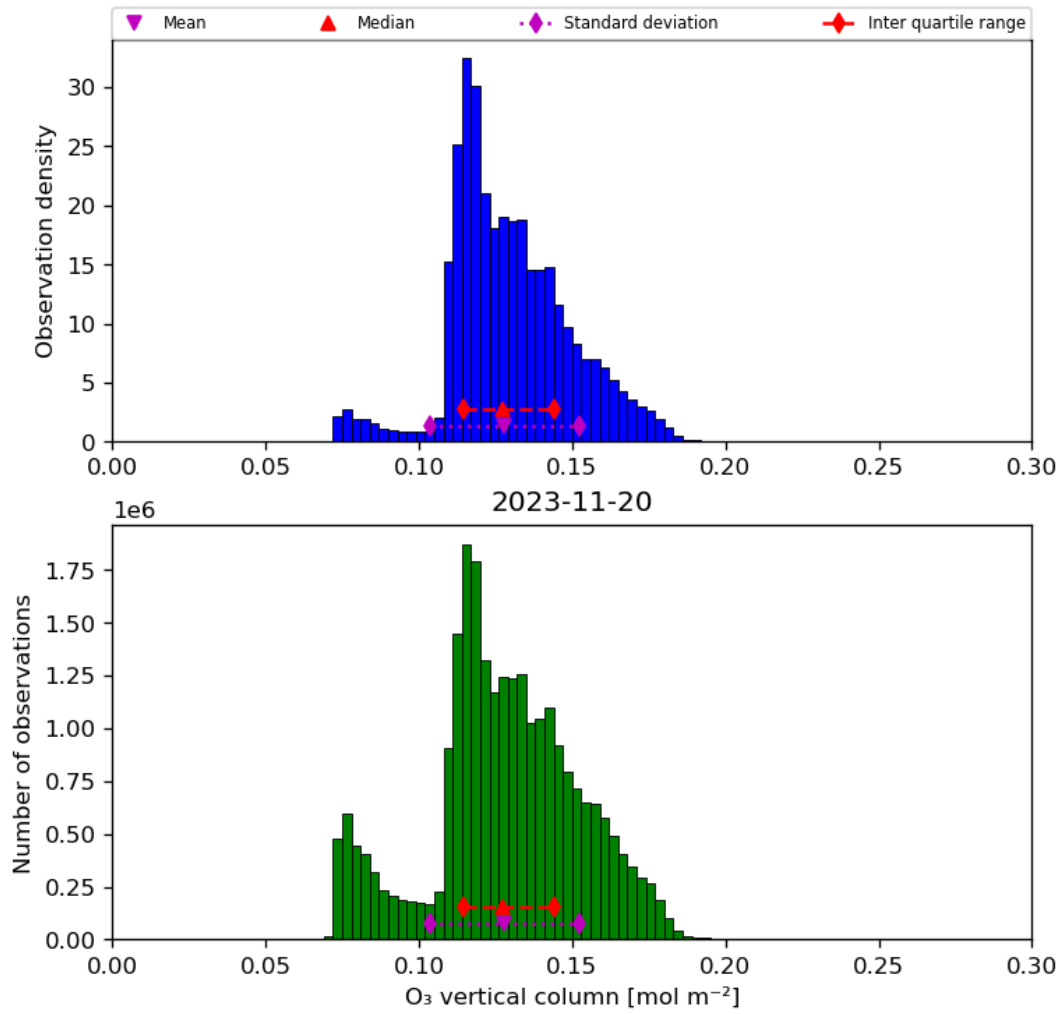
Figure 21: Histogram of “O 3 vertical column” for 2023-11-19 to 2023-11-21
