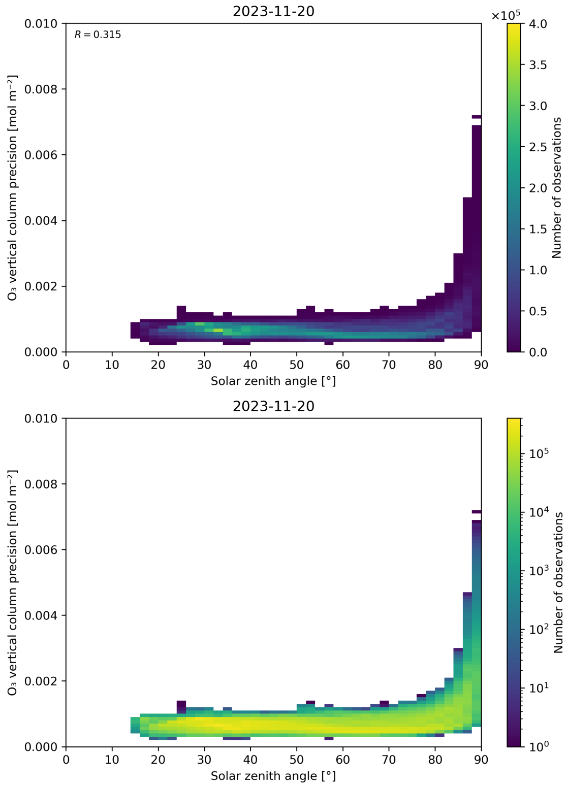
Figure 48: Scatter density plot of “Solar zenith angle” against “O 3 vertical column precision” for 2023-11-19 to 2023-11-21.
