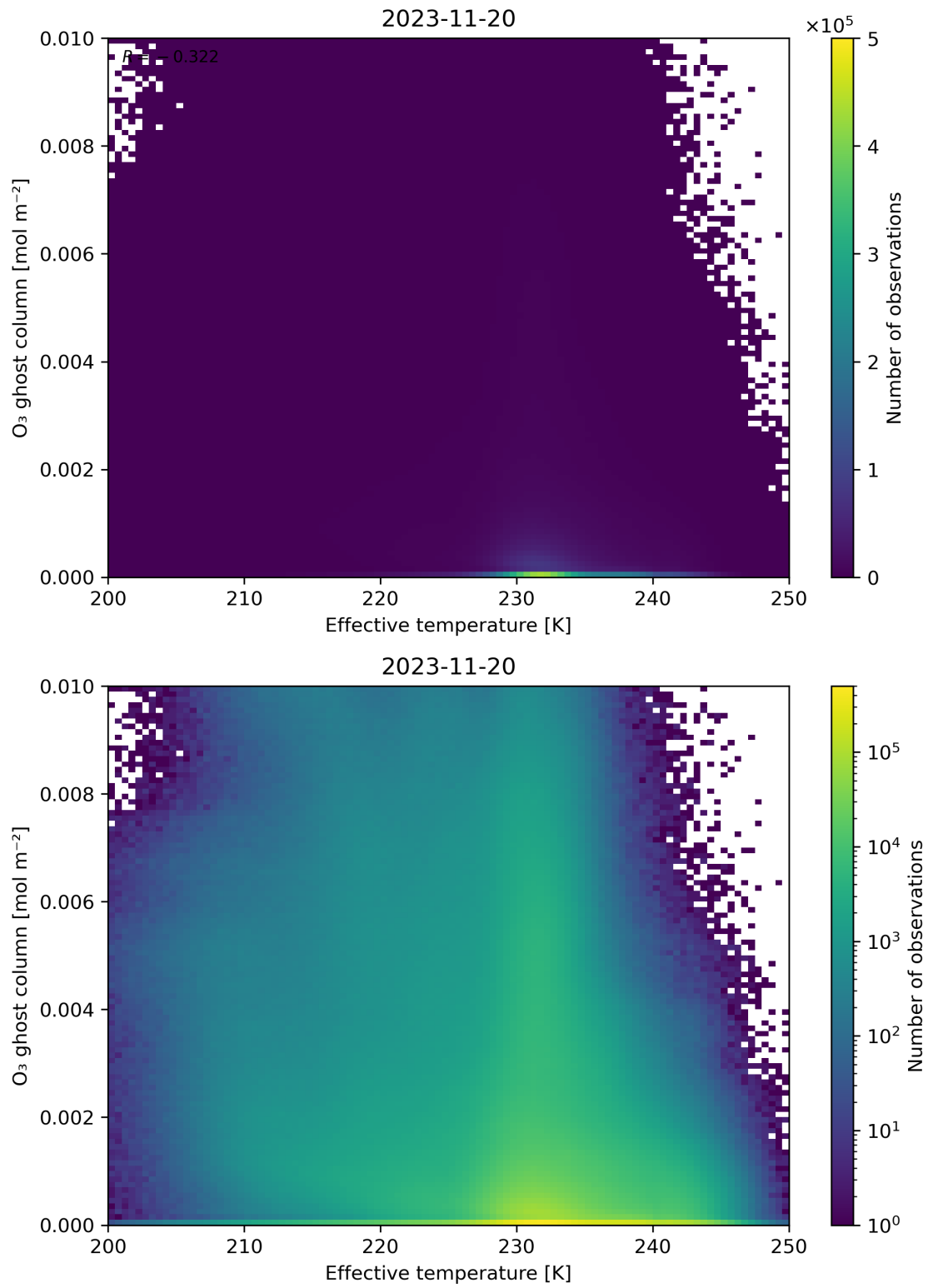
Figure 38: Scatter density plot of “Effective temperature” against “O 3 ghost column” for 2023-11-19 to 2023-11-21.
