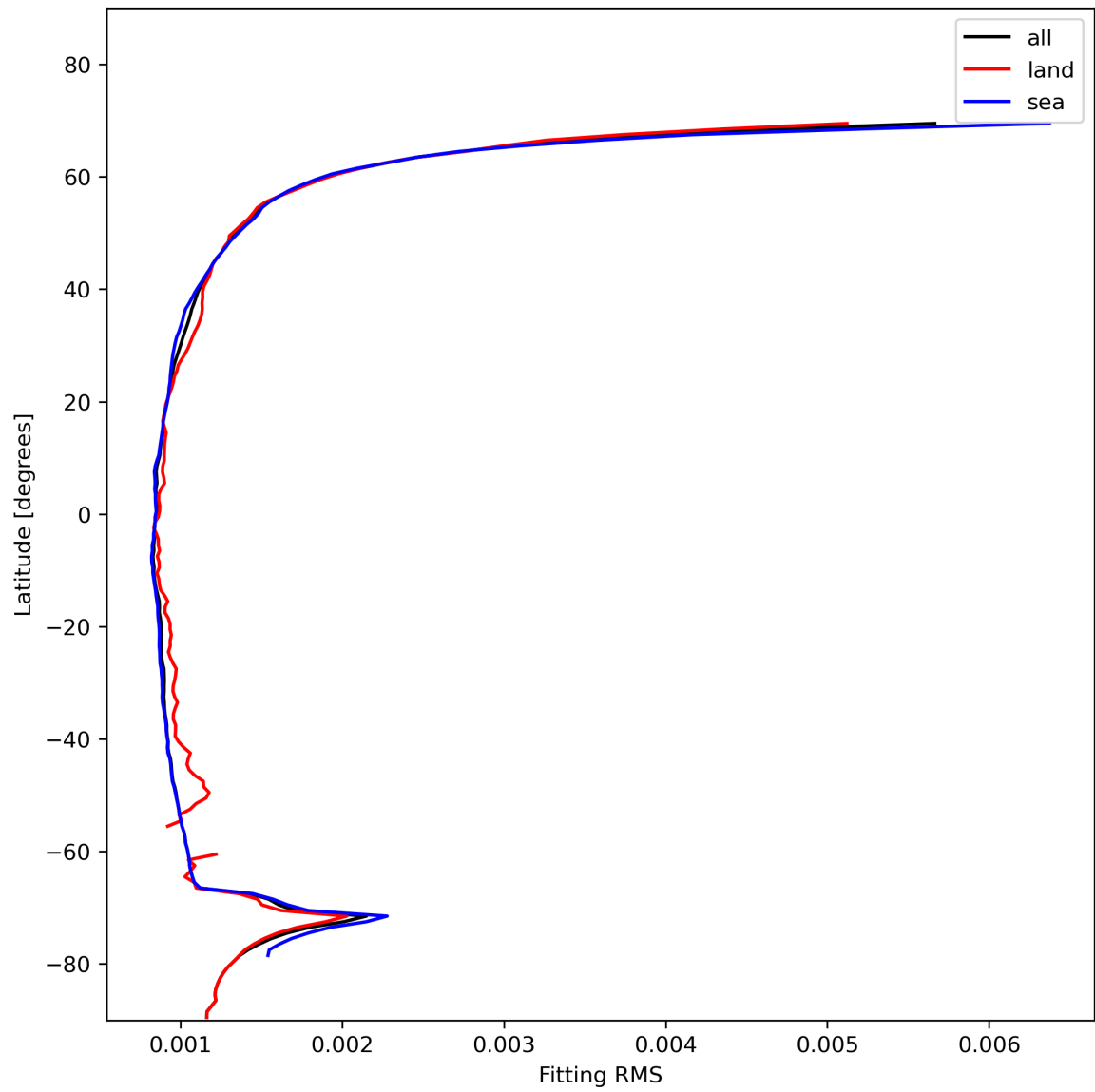
Figure 16: Zonal average of “Fitting RMS” for 2023-11-19 to 2023-11-21.
