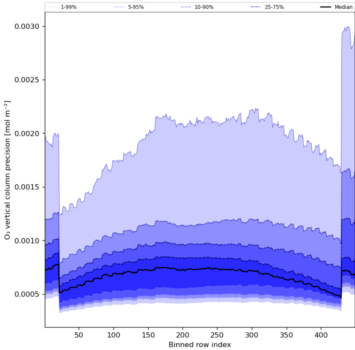
Figure 29: Along track statistics of “O 3 vertical column precision” for 2023-11-19 to 2023-11-21
