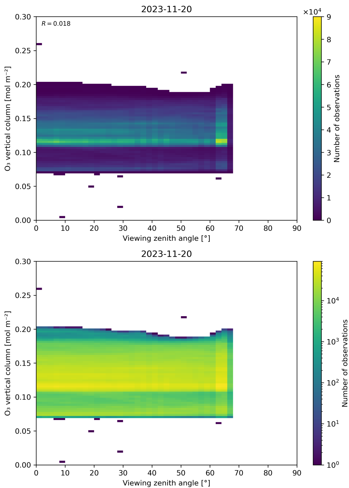
Figure 52: Scatter density plot of “Viewing zenith angle” against “O 3 vertical column” for 2023-11-19 to 2023-11-21.
