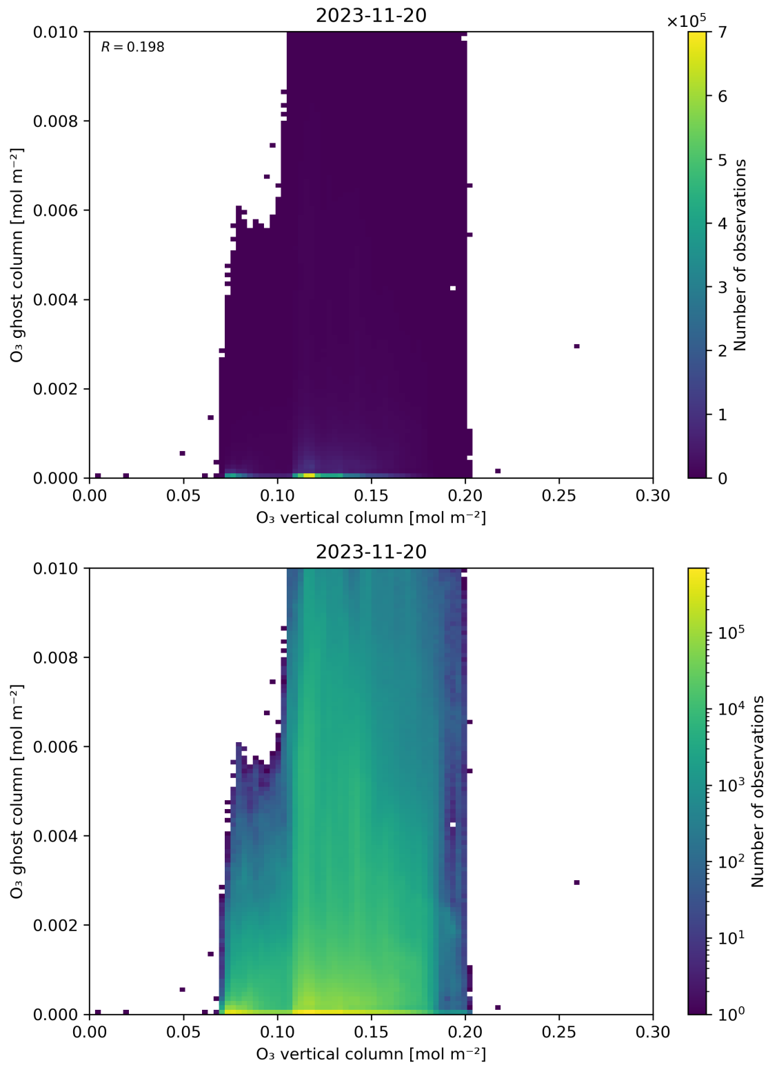
Figure 40: Scatter density plot of “O 3 vertical column” against “O 3 ghost column” for 2023-11-19 to 2023-11-21.
