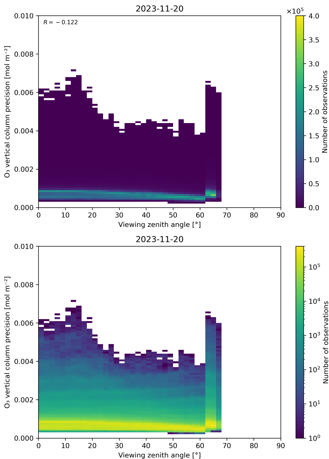
Figure 53: Scatter density plot of “Viewing zenith angle” against “O 3 vertical column precision” for 2023-11-19 to 2023-11-21.
