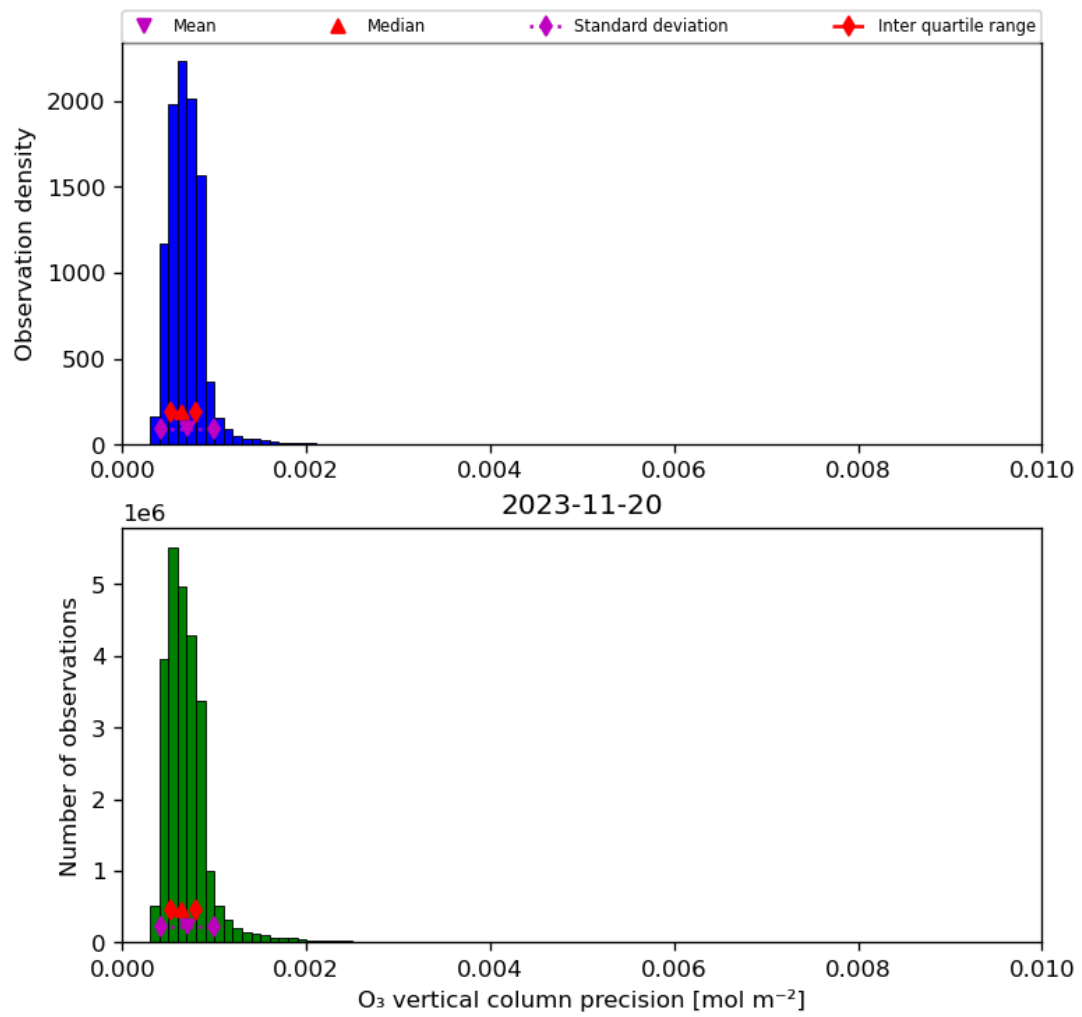
Figure 22: Histogram of “O 3 vertical column precision” for 2023-11-19 to 2023-11-21
