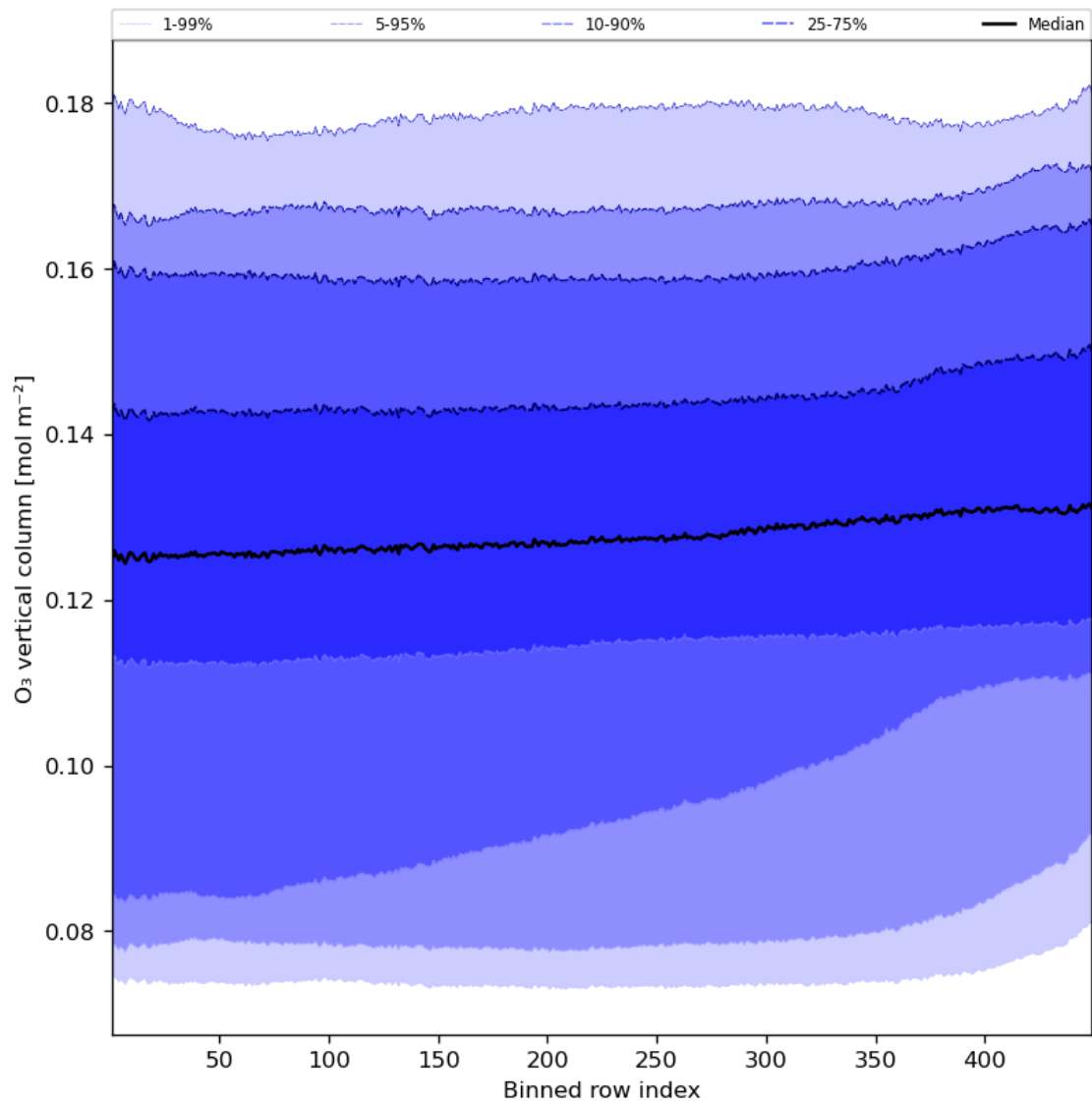
Figure 28: Along track statistics of “O 3 vertical column” for 2023-11-19 to 2023-11-21
