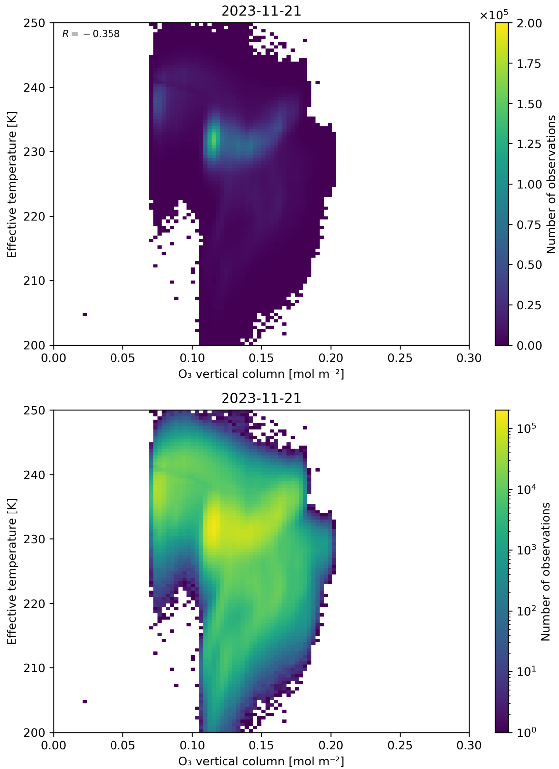
Figure 39: Scatter density plot of “O 3 vertical column” against “Effective temperature” for 2023-11-20 to 2023-11-22.
