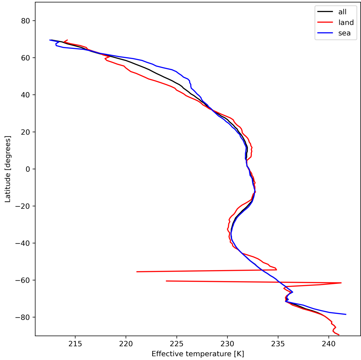
Figure 17: Zonal average of “Effective temperature” for 2023-11-20 to 2023-11-22.
