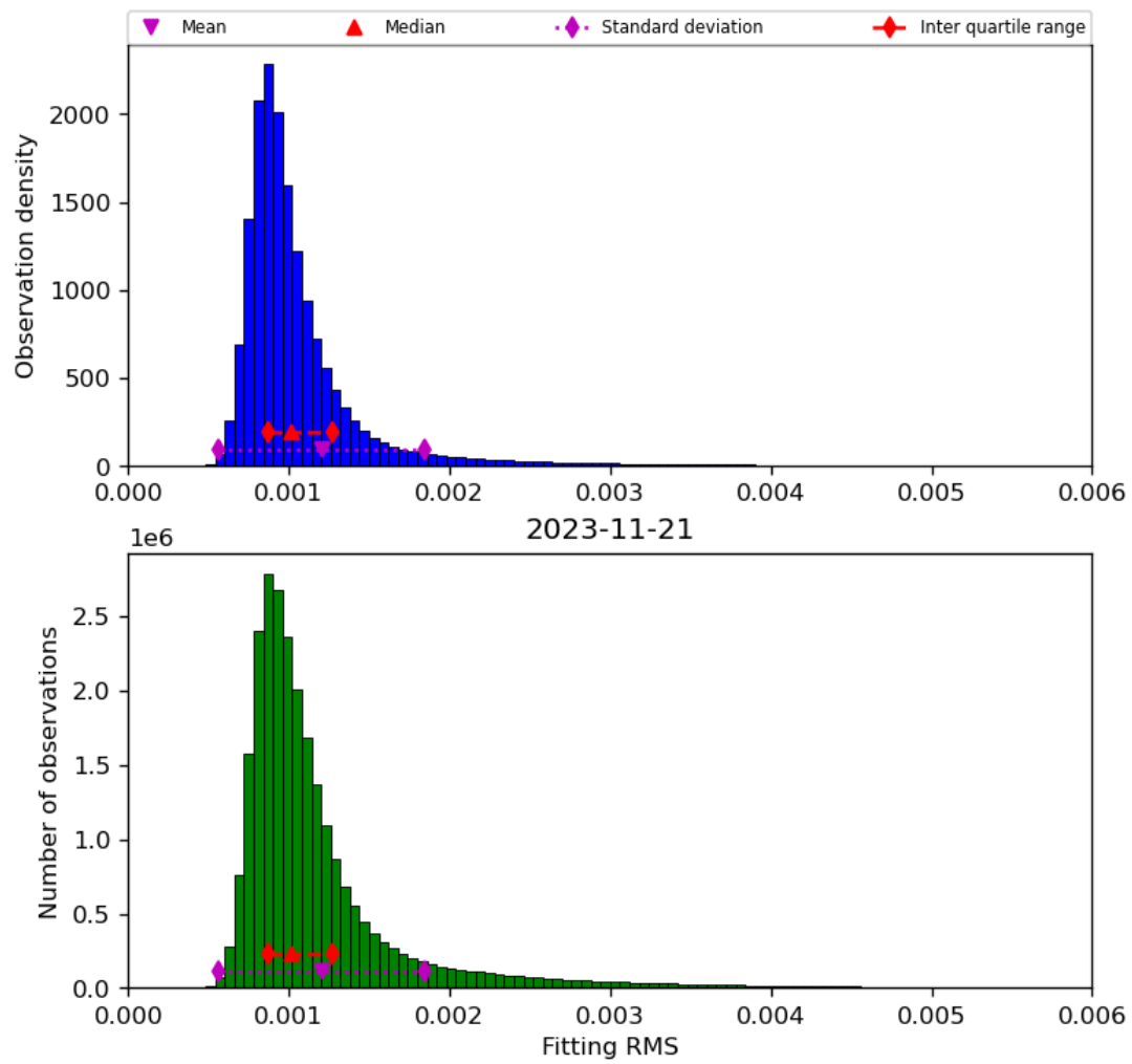
Figure 23: Histogram of “Fitting RMS” for 2023-11-20 to 2023-11-22
