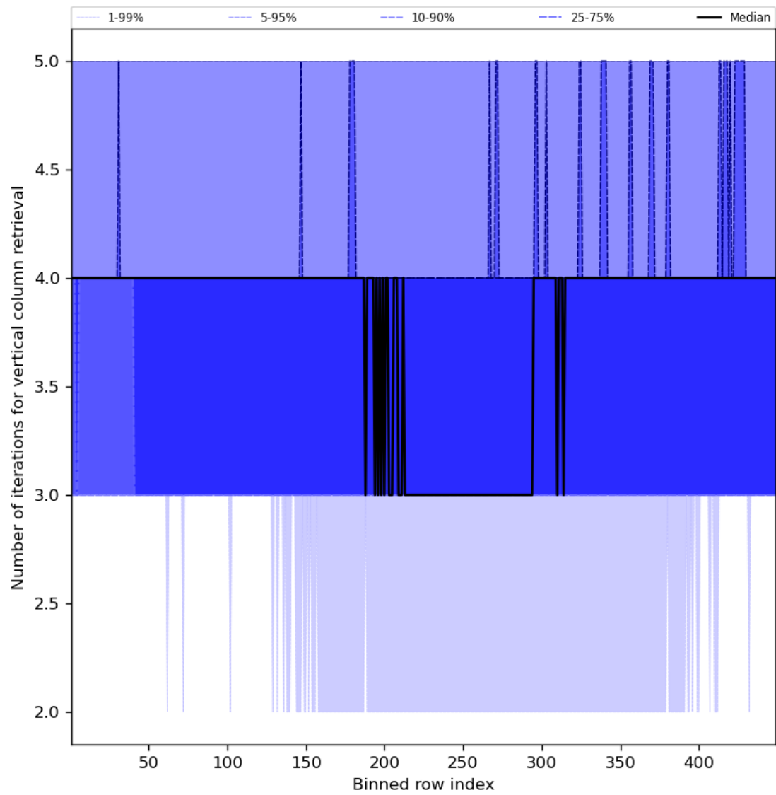
Figure 33: Along track statistics of “Number of iterations for vertical column retrieval” for 2023-11-20 to 2023-11-22
