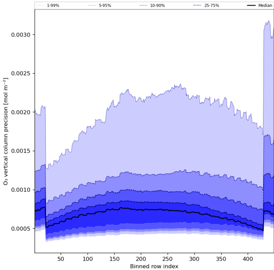
Figure 29: Along track statistics of “O 3 vertical column precision” for 2023-11-20 to 2023-11-22
