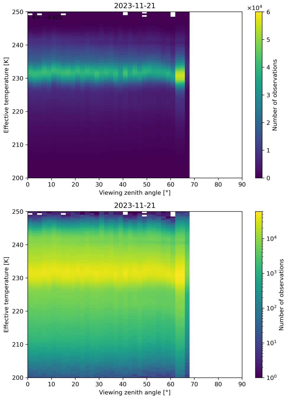
Figure 50: Scatter density plot of “Viewing zenith angle” against “Effective temperature” for 2023-11-20 to 2023-11-22.
