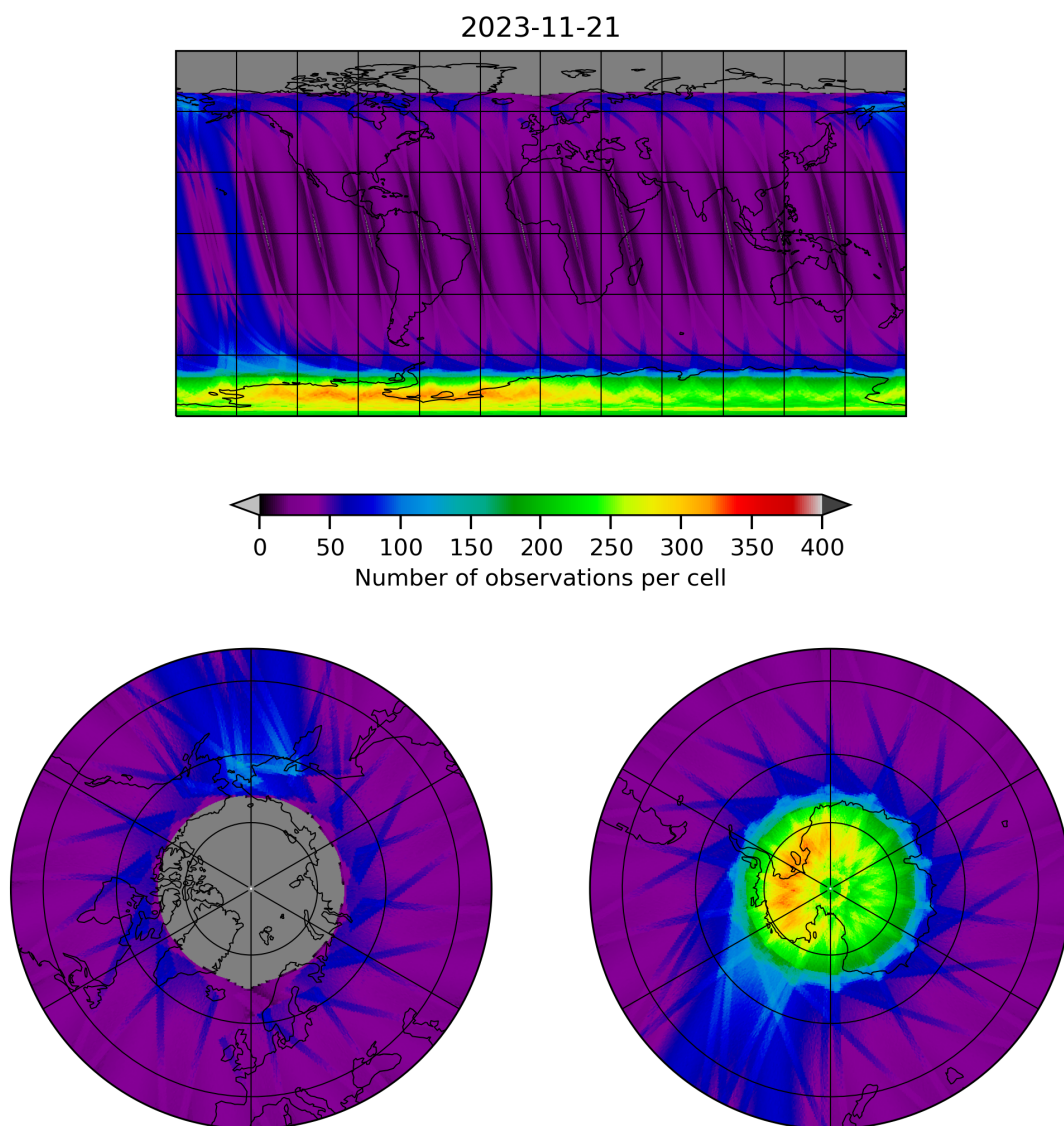
Figure 12: Map of the number of observations for 2023-11-20 to 2023-11-22
