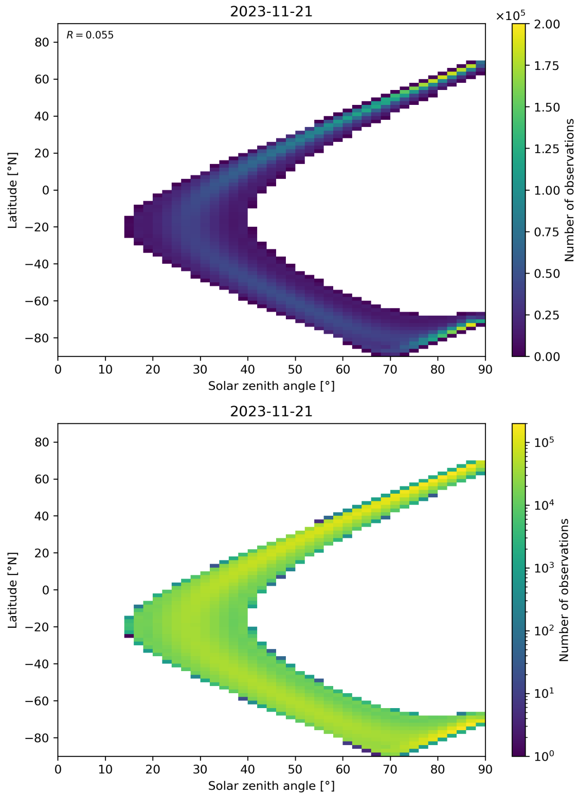
Figure 44: Scatter density plot of “Solar zenith angle” against “Latitude” for 2023-11-20 to 2023-11-22.
