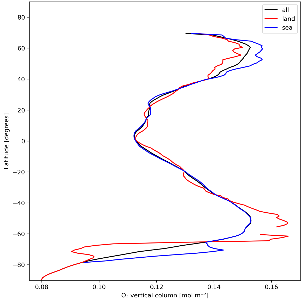
Figure 14: Zonal average of “O 3 vertical column” for 2023-11-20 to 2023-11-22.
