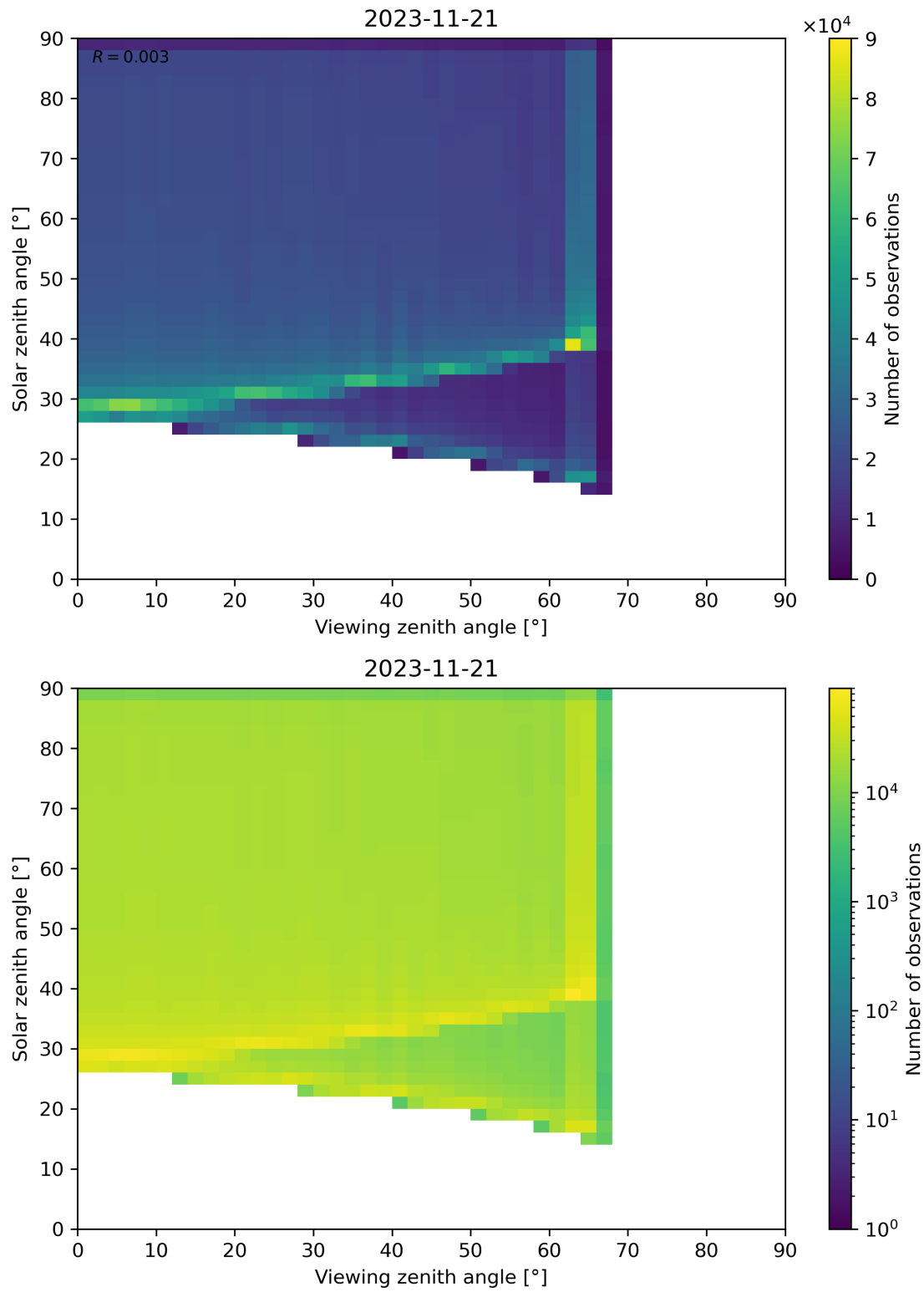
Figure 54: Scatter density plot of “Viewing zenith angle” against “Solar zenith angle” for 2023-11-20 to 2023-11-22.
