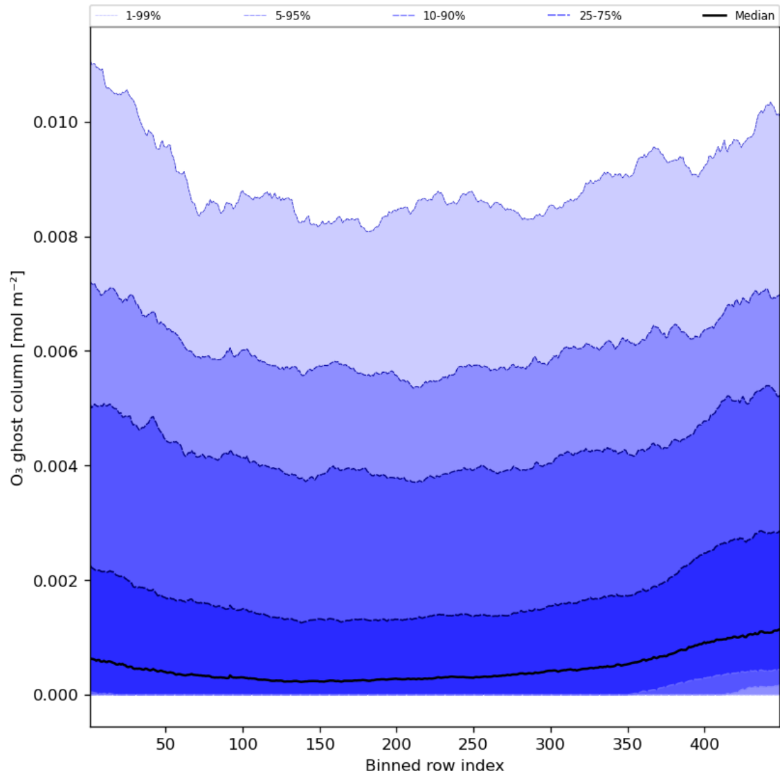
Figure 32: Along track statistics of “O 3 ghost column” for 2023-11-20 to 2023-11-22
