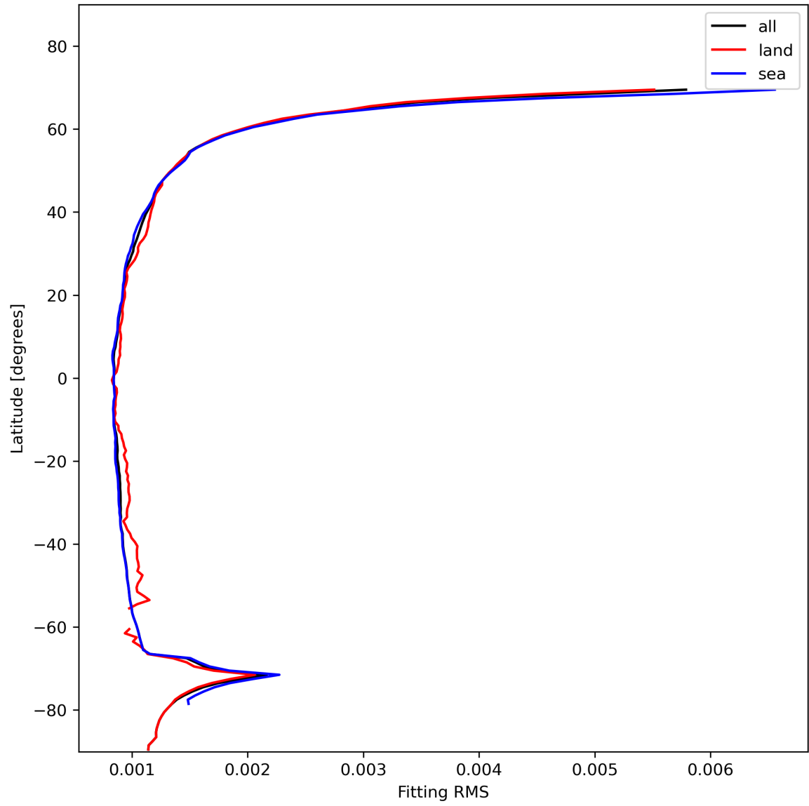
Figure 16: Zonal average of “Fitting RMS” for 2023-11-20 to 2023-11-22.
