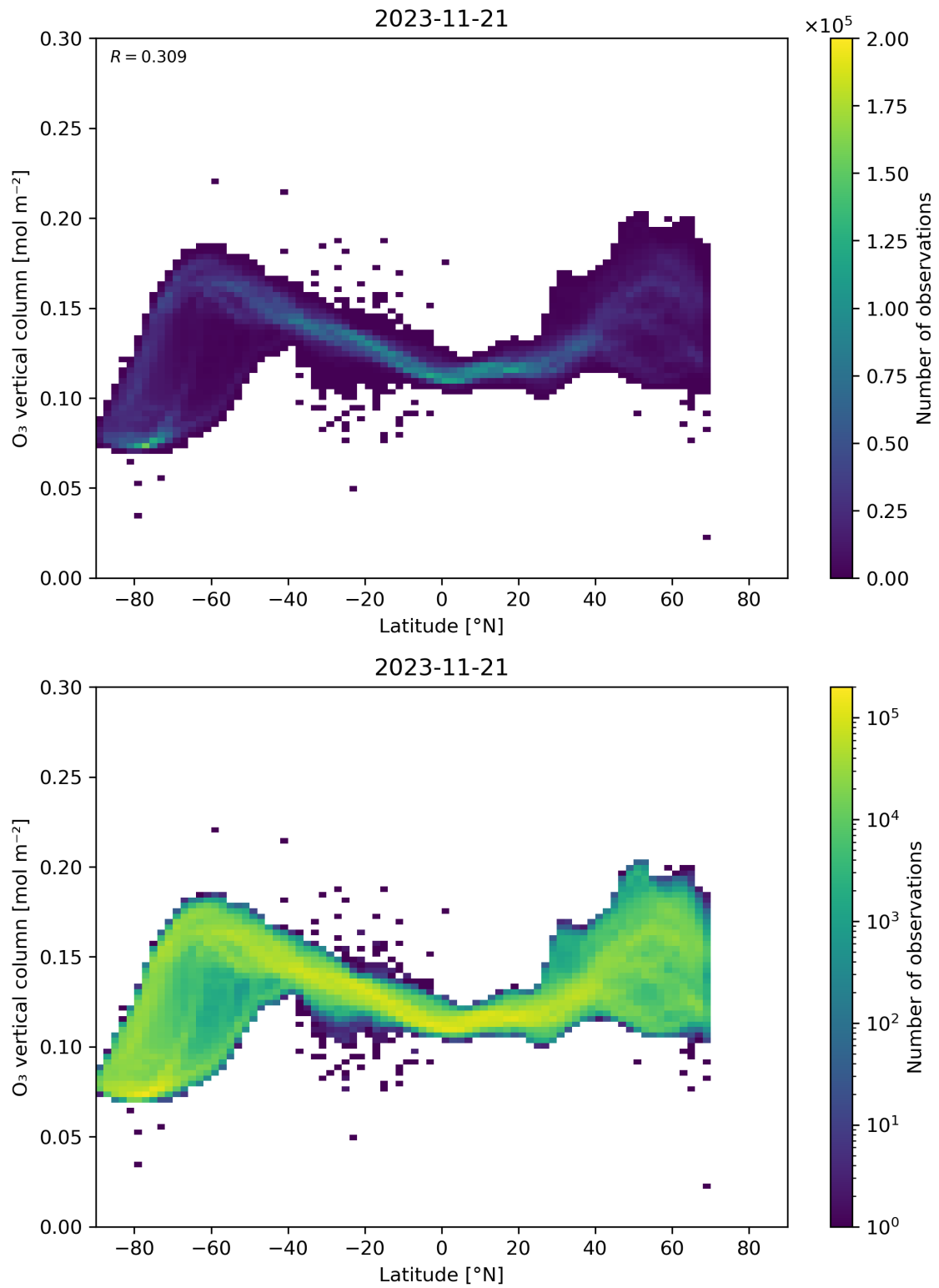
Figure 36: Scatter density plot of “Latitude” against “O 3 vertical column” for 2023-11-20 to 2023-11-22.
