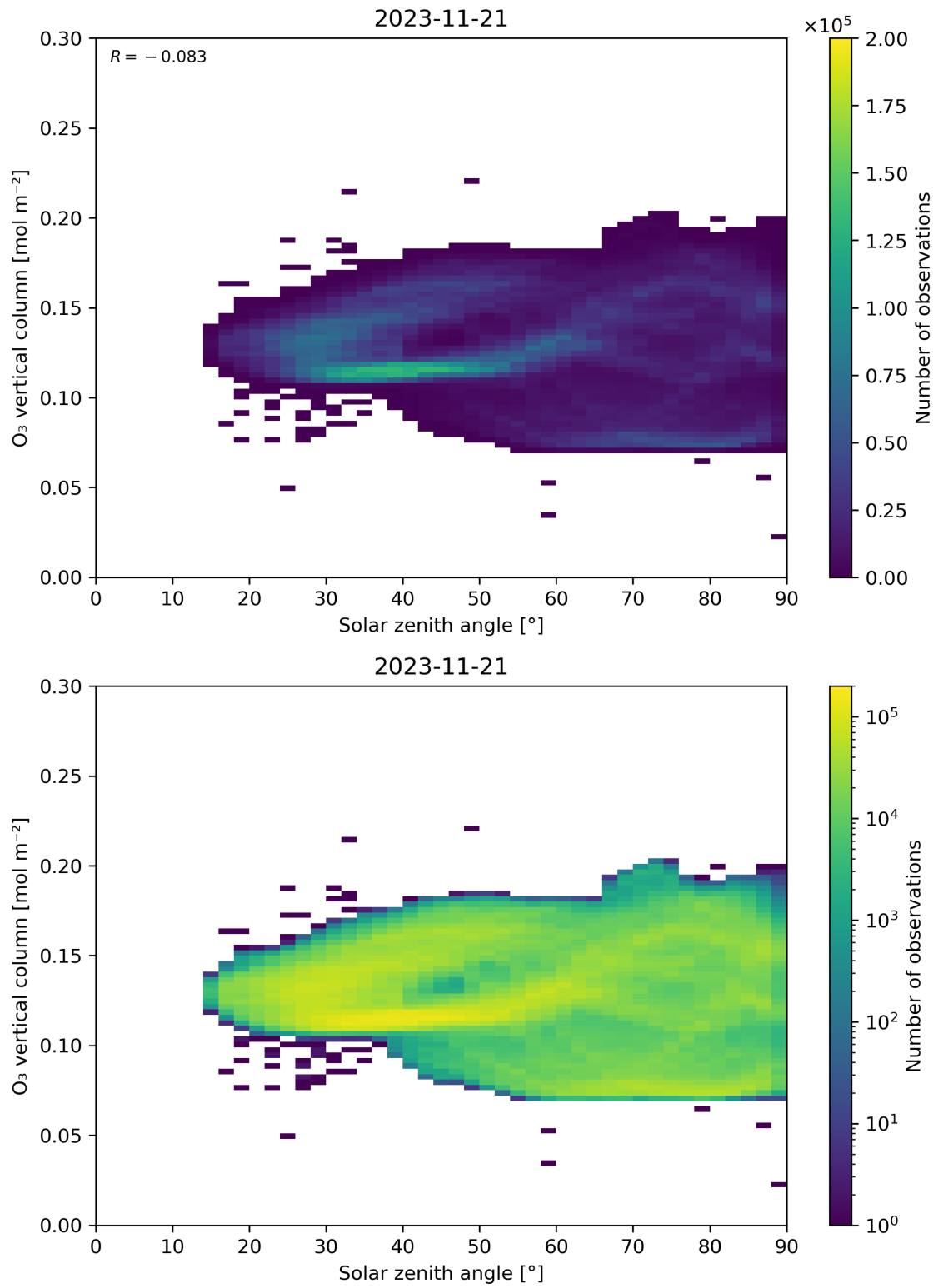
Figure 47: Scatter density plot of “Solar zenith angle” against “O 3 vertical column” for 2023-11-20 to 2023-11-22.
