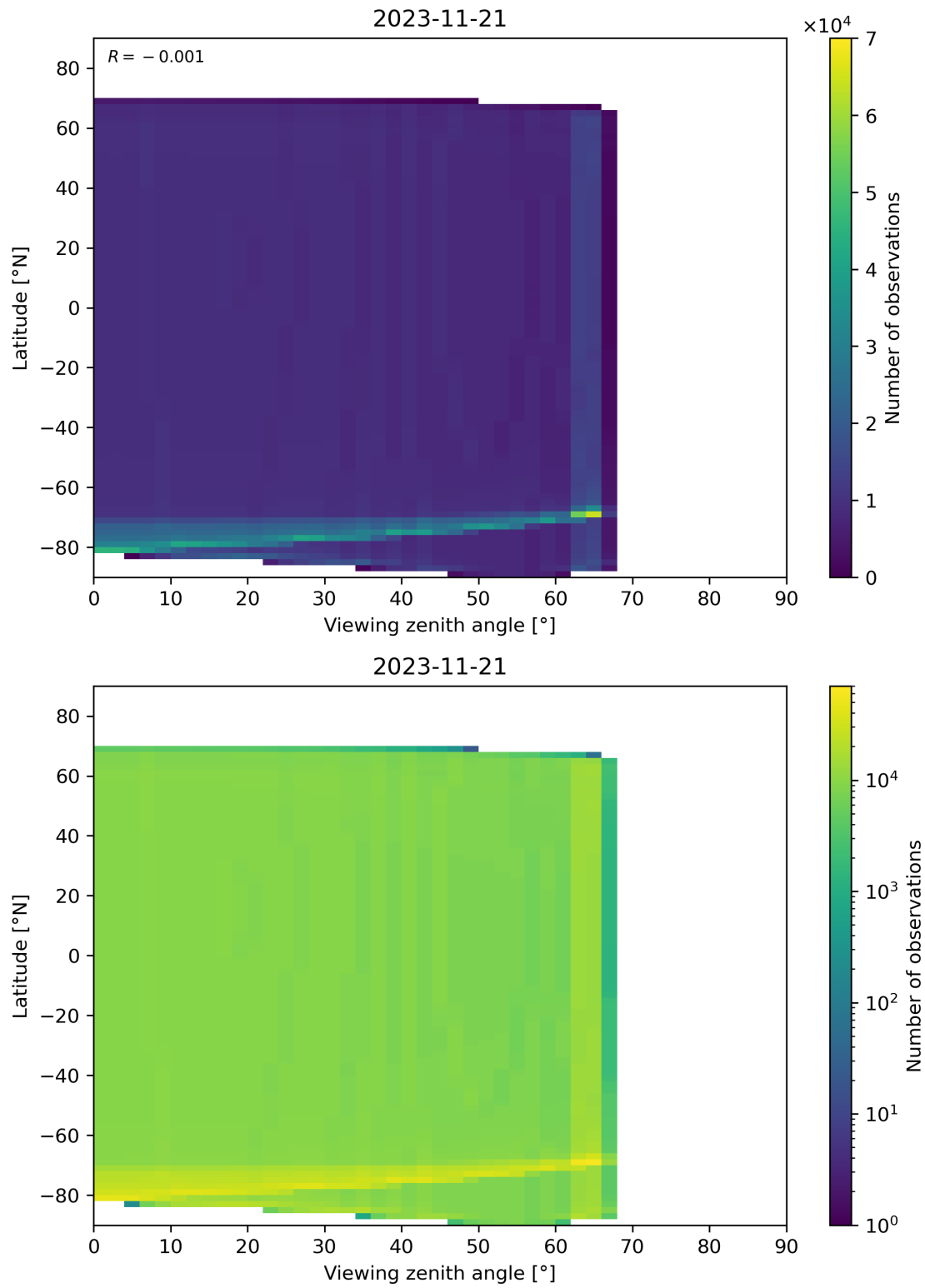
Figure 49: Scatter density plot of “Viewing zenith angle” against “Latitude” for 2023-11-20 to 2023-11-22.
