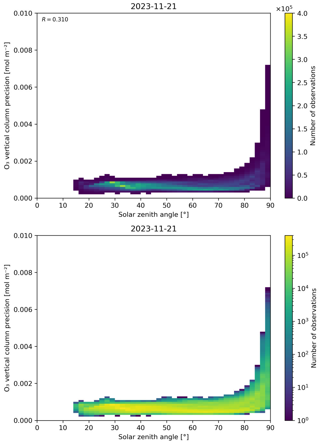
Figure 48: Scatter density plot of “Solar zenith angle” against “O 3 vertical column precision” for 2023-11-20 to 2023-11-22.
