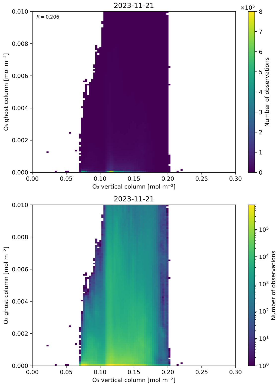
Figure 40: Scatter density plot of “O 3 vertical column” against “O 3 ghost column” for 2023-11-20 to 2023-11-22.
