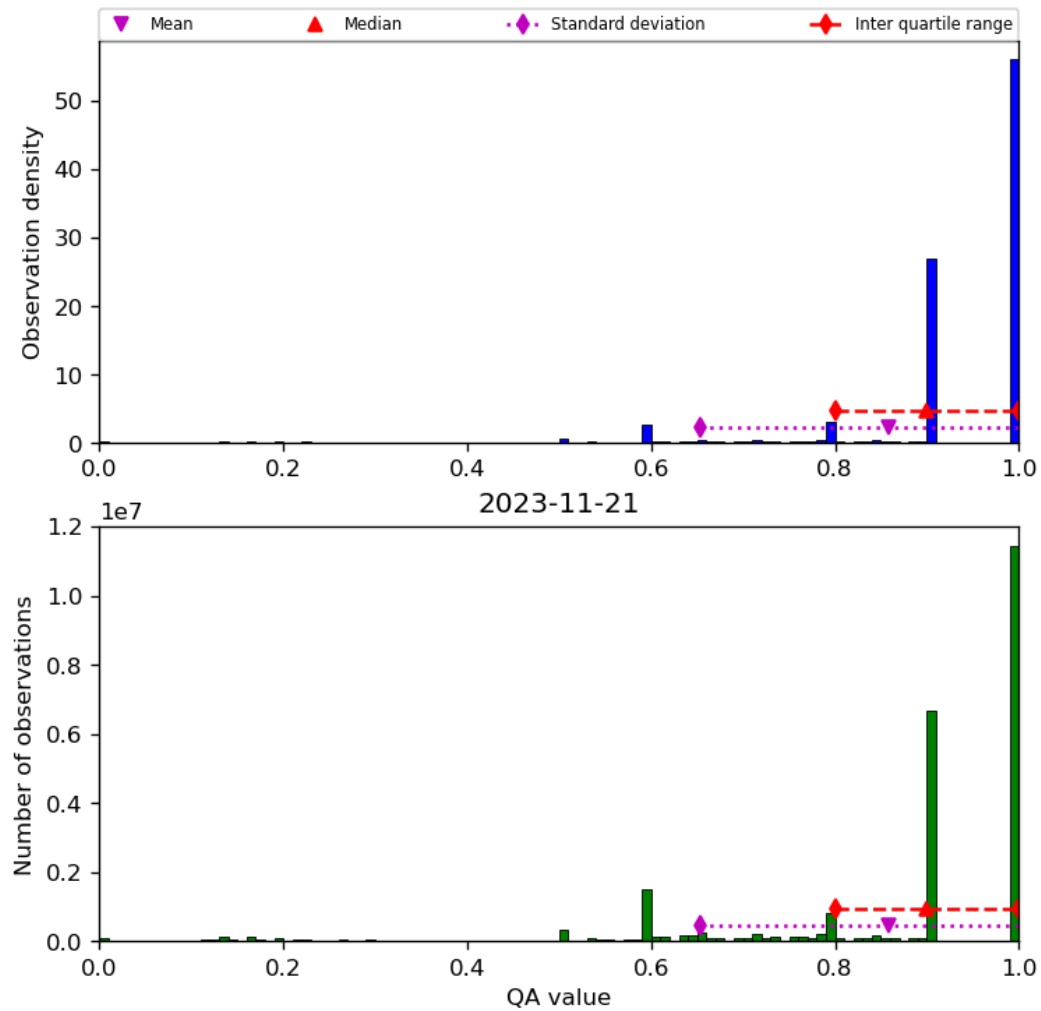
Figure 20: Histogram of “QA value” for 2023-11-20 to 2023-11-22
