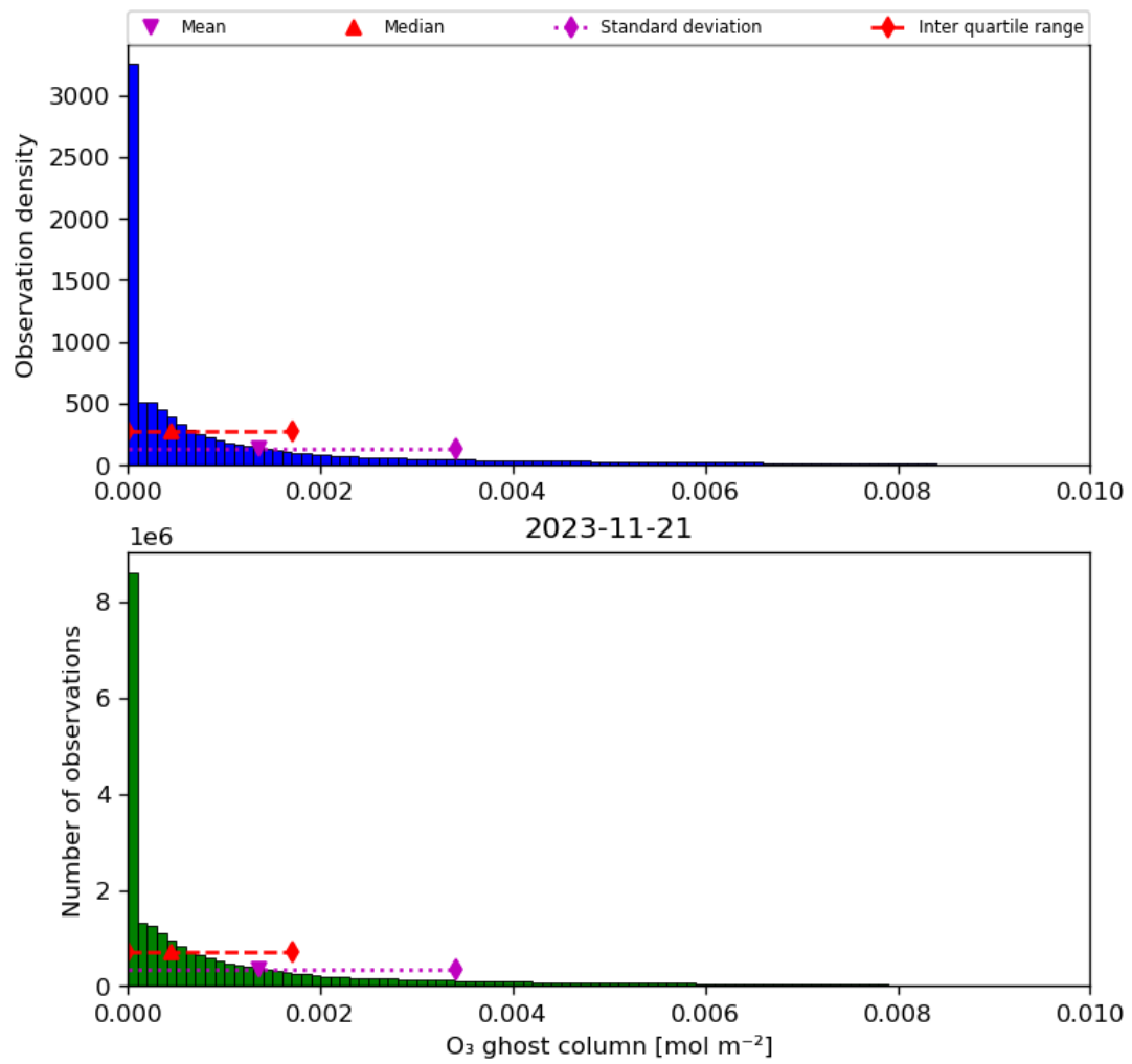
Figure 25: Histogram of "O 3 ghost column" for 2023-11-20 to 2023-11-22
