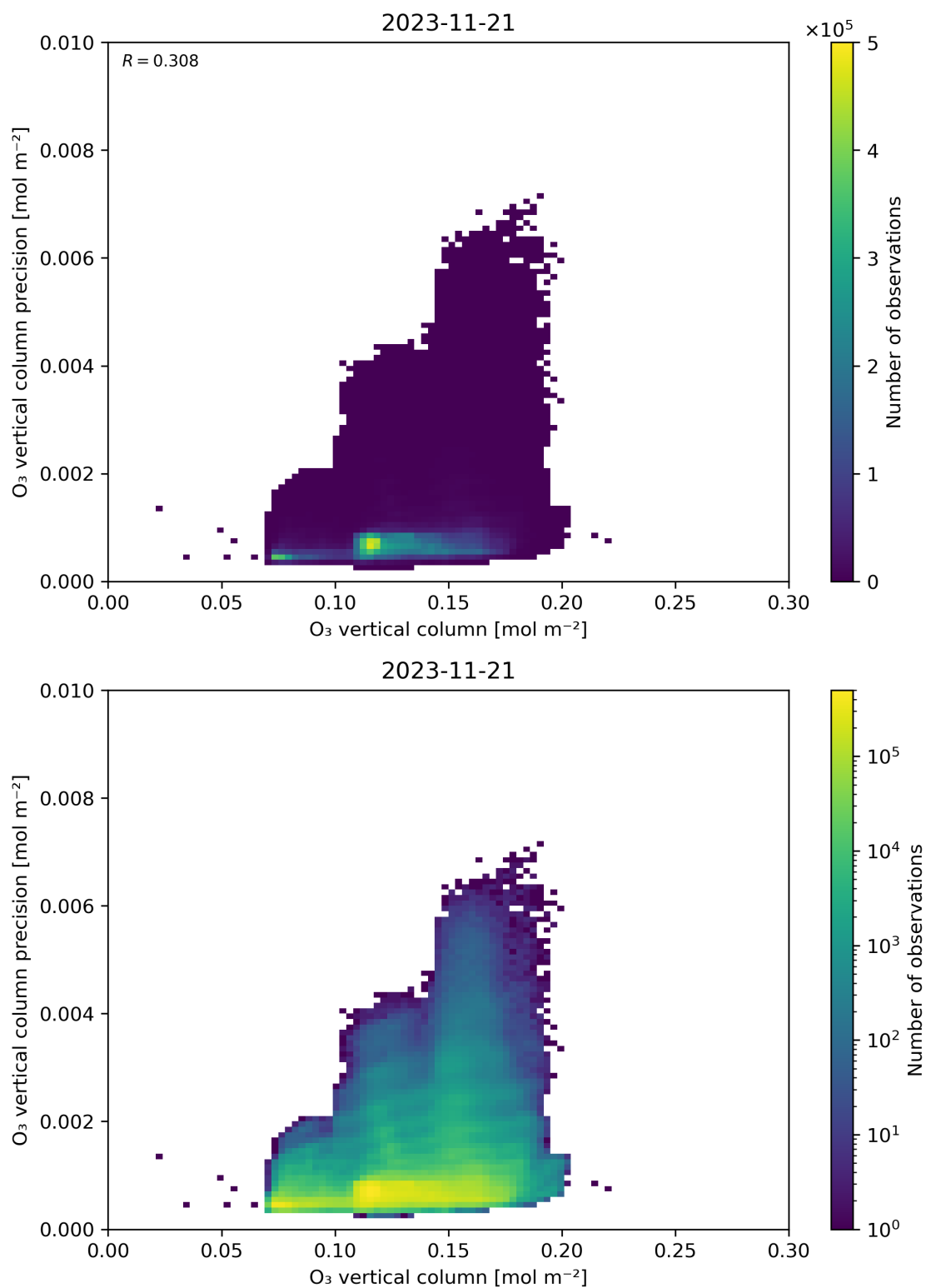
Figure 41: Scatter density plot of “O 3 vertical column” against “O 3 vertical column precision” for 2023-11-20 to 2023-11-22.
