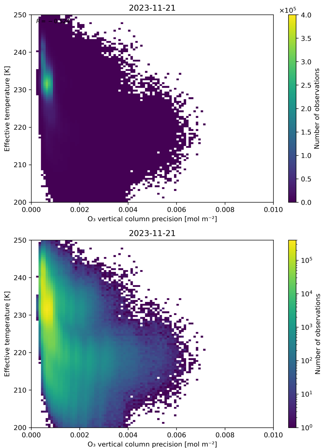
Figure 42: Scatter density plot of “O 3 vertical column precision” against “Effective temperature” for 2023-11-20 to 2023-11-22.
