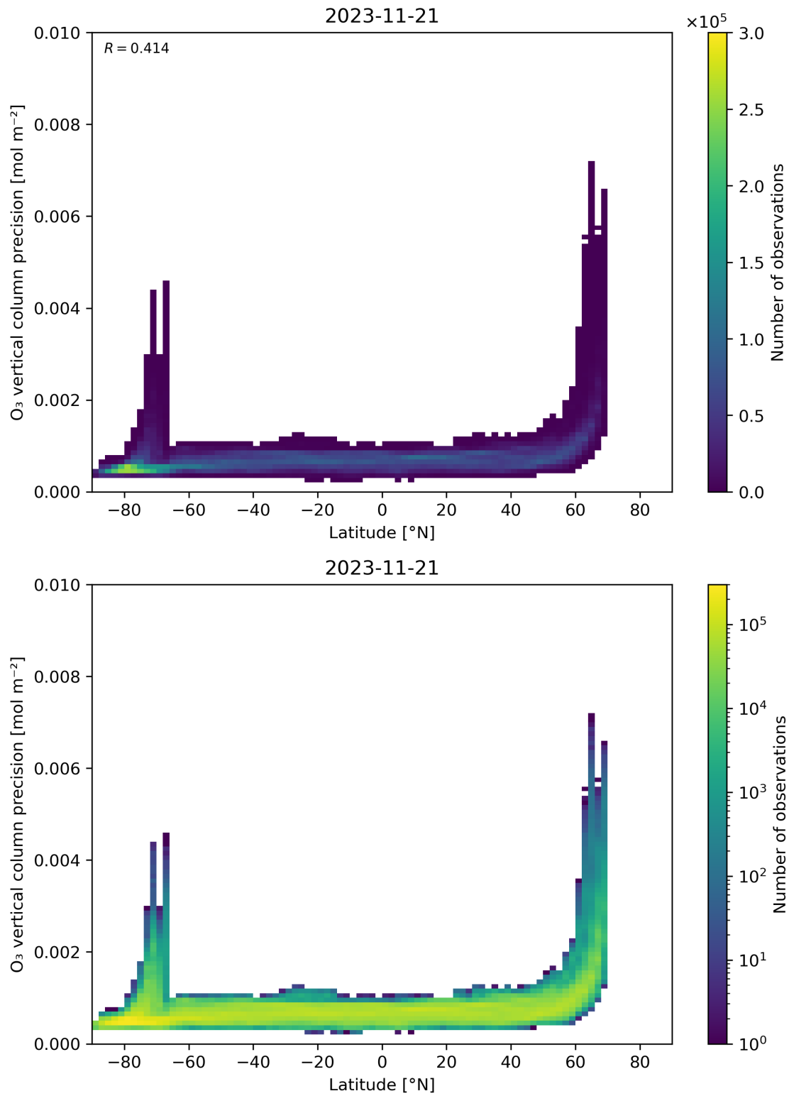
Figure 37: Scatter density plot of “Latitude” against “O 3 vertical column precision” for 2023-11-20 to 2023-11-22.
