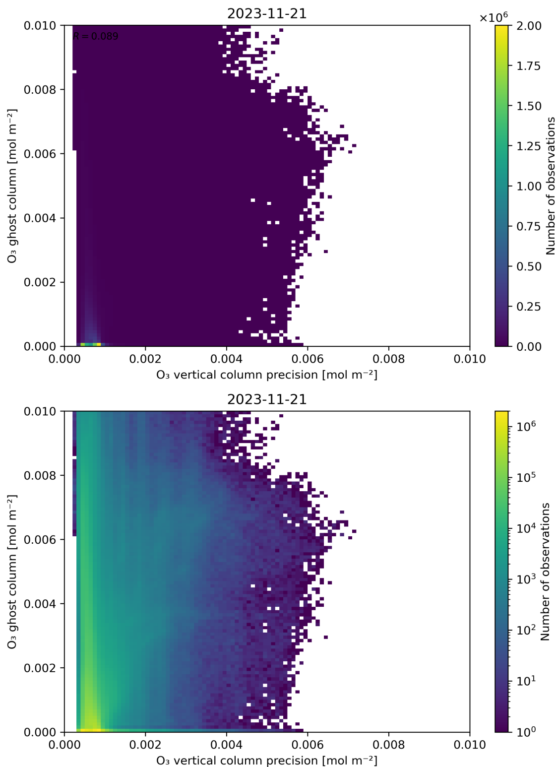
Figure 43: Scatter density plot of “ \text{O}_3 vertical column precision” against “ \text{O}_3 ghost column” for 2023-11-20 to 2023-11-22.
