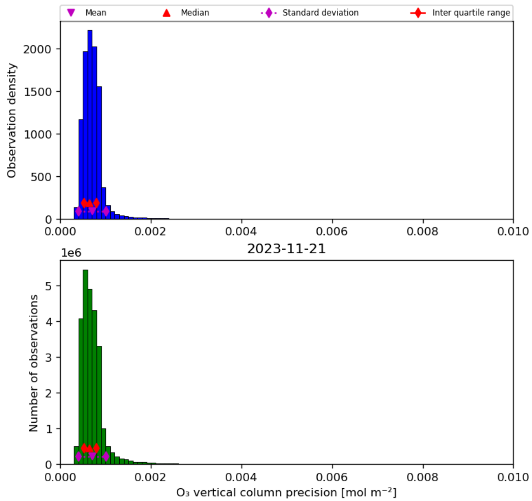
Figure 22: Histogram of “O 3 vertical column precision” for 2023-11-20 to 2023-11-22
