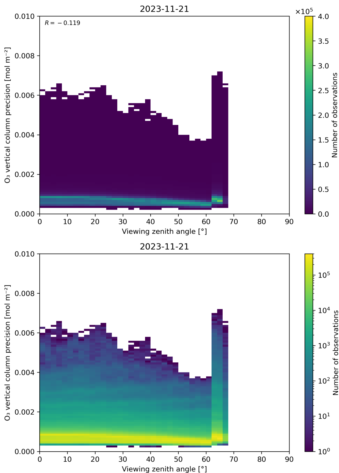
Figure 53: Scatter density plot of “Viewing zenith angle” against “O 3 vertical column precision” for 2023-11-20 to 2023-11-22.
