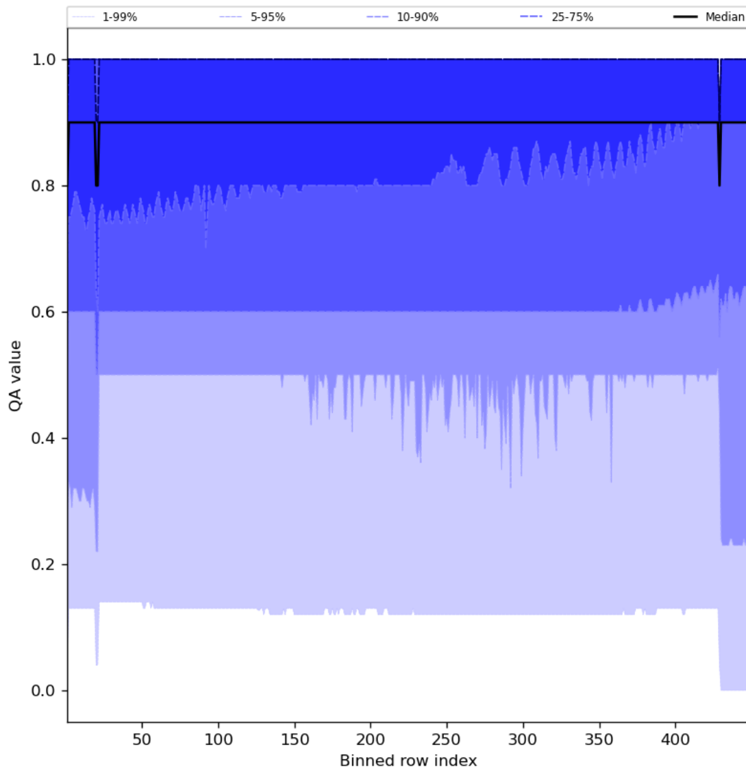
Figure 27: Along track statistics of “QA value” for 2023-11-20 to 2023-11-22
