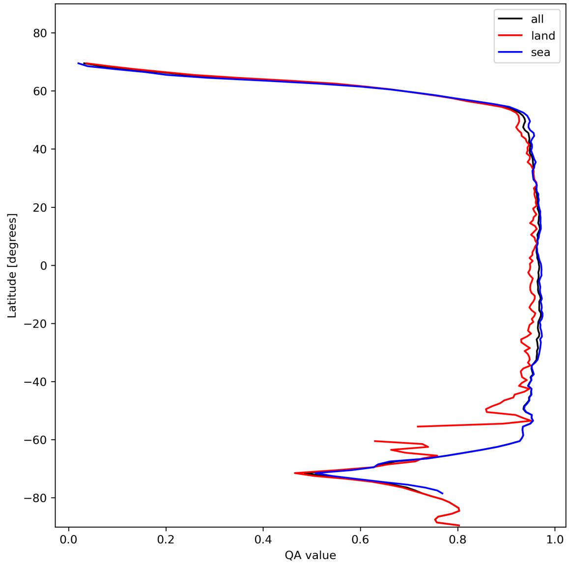
Figure 13: Zonal average of “QA value” for 2023-11-20 to 2023-11-22.
