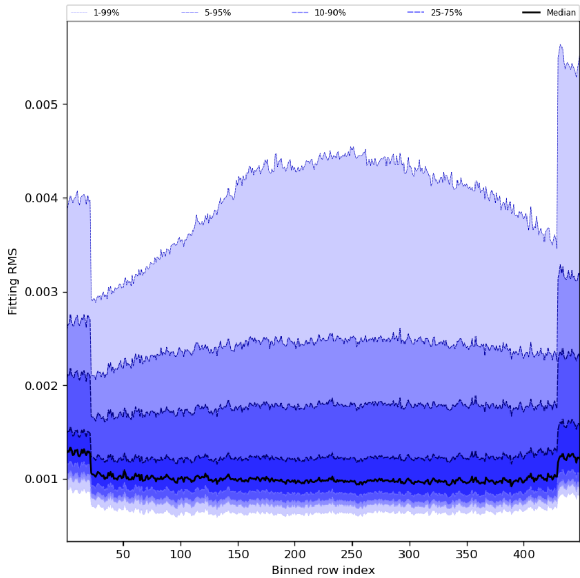
Figure 30: Along track statistics of “Fitting RMS” for 2023-11-20 to 2023-11-22
