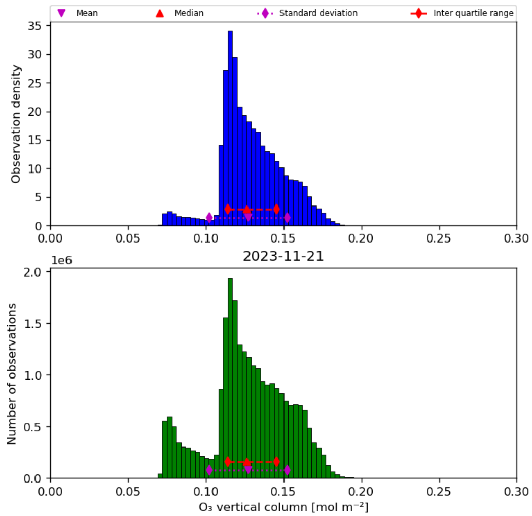
Figure 21: Histogram of “O 3 vertical column” for 2023-11-20 to 2023-11-22
