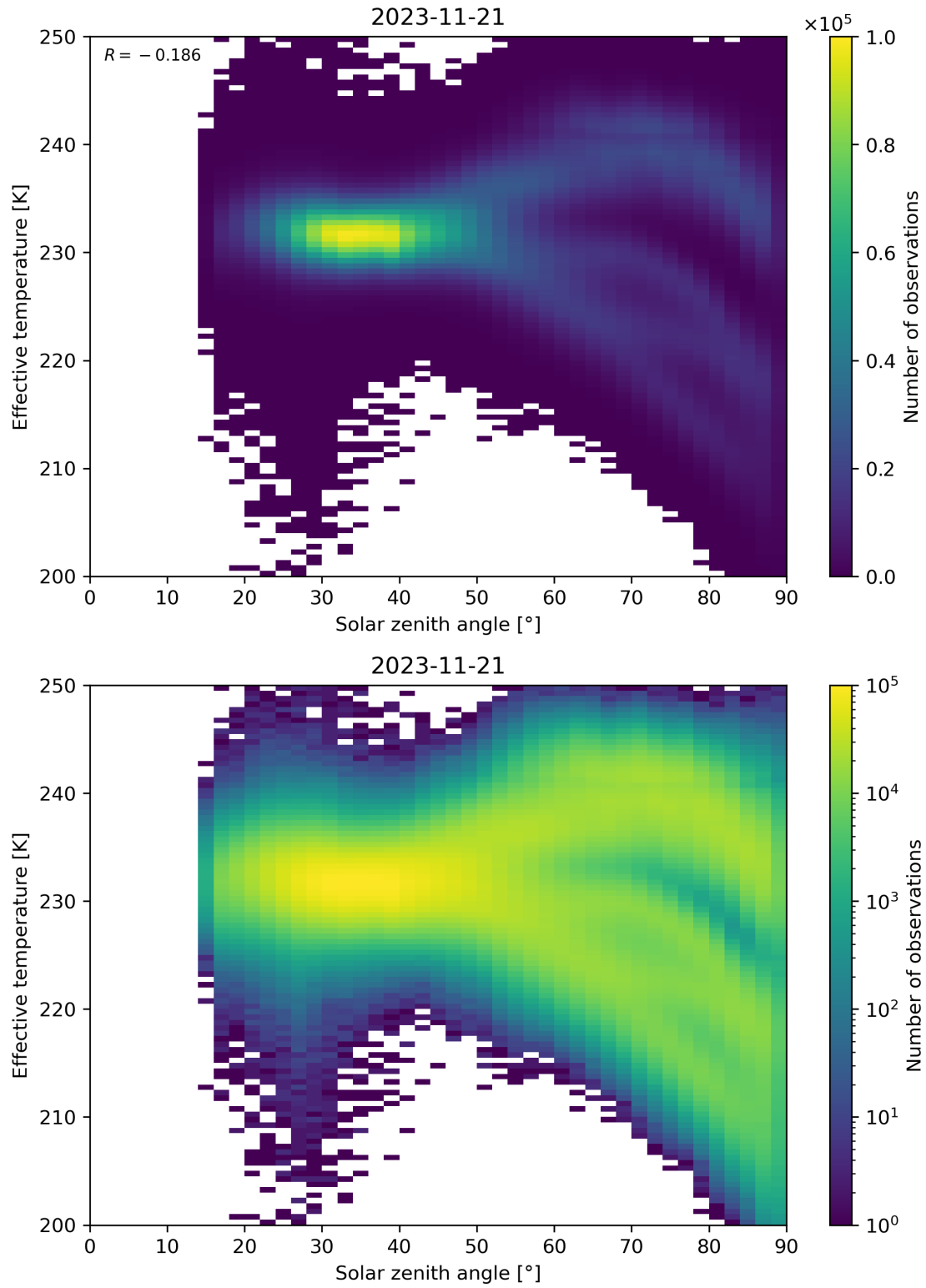
Figure 45: Scatter density plot of “Solar zenith angle” against “Effective temperature” for 2023-11-20 to 2023-11-22.
