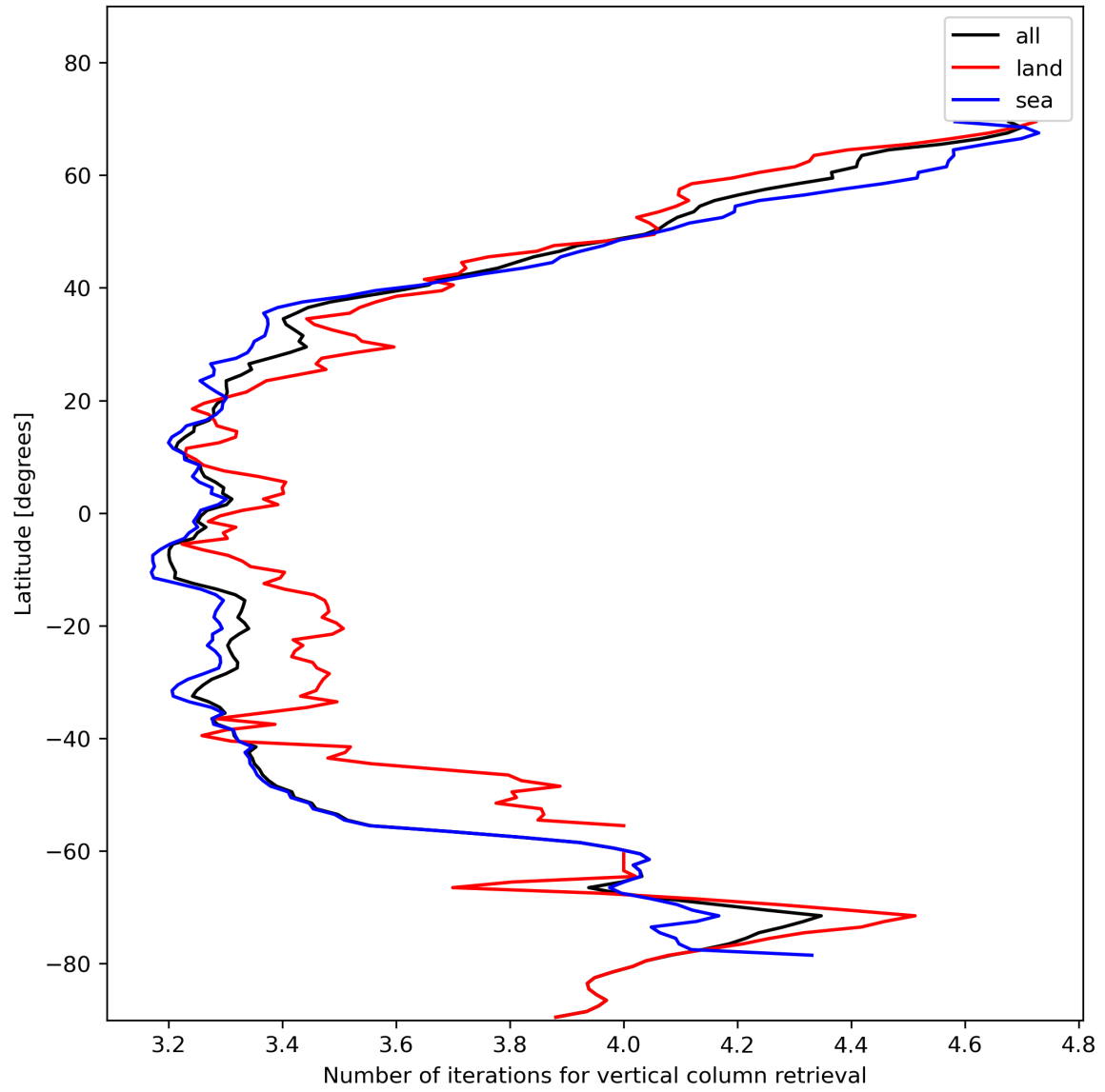
Figure 19: Zonal average of “Number of iterations for vertical column retrieval” for 2023-11-20 to 2023-11-22.
