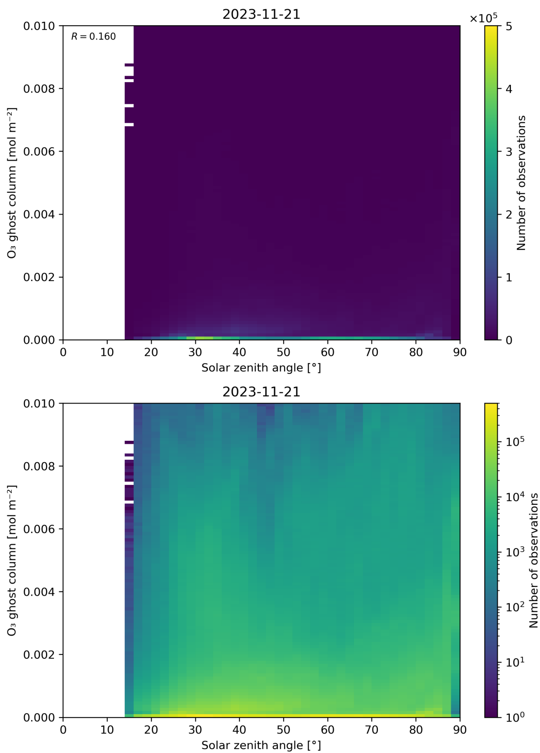
Figure 46: Scatter density plot of “Solar zenith angle” against “O 3 ghost column” for 2023-11-20 to 2023-11-22.
