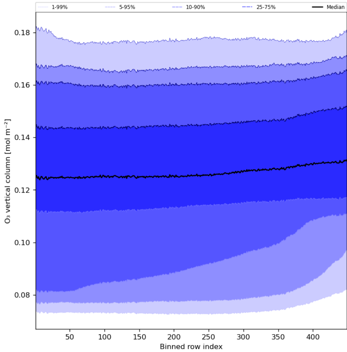
Figure 28: Along track statistics of “O 3 vertical column” for 2023-11-20 to 2023-11-22
