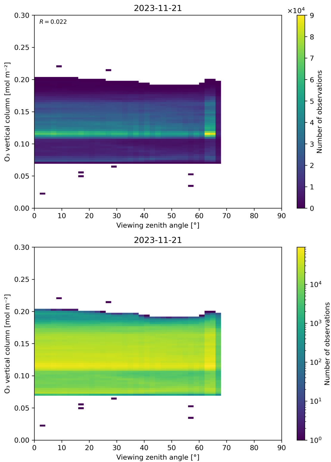
Figure 52: Scatter density plot of “Viewing zenith angle” against “O 3 vertical column” for 2023-11-20 to 2023-11-22.
