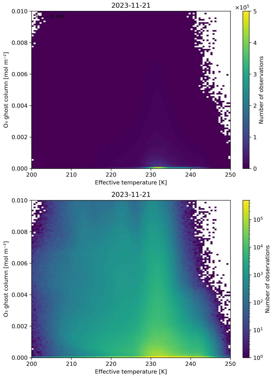
Figure 38: Scatter density plot of “Effective temperature” against “O 3 ghost column” for 2023-11-20 to 2023-11-22.
