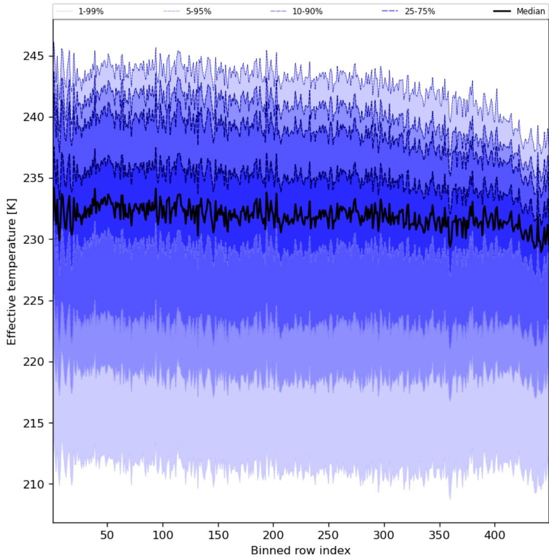
Figure 31: Along track statistics of “Effective temperature” for 2023-11-20 to 2023-11-22
