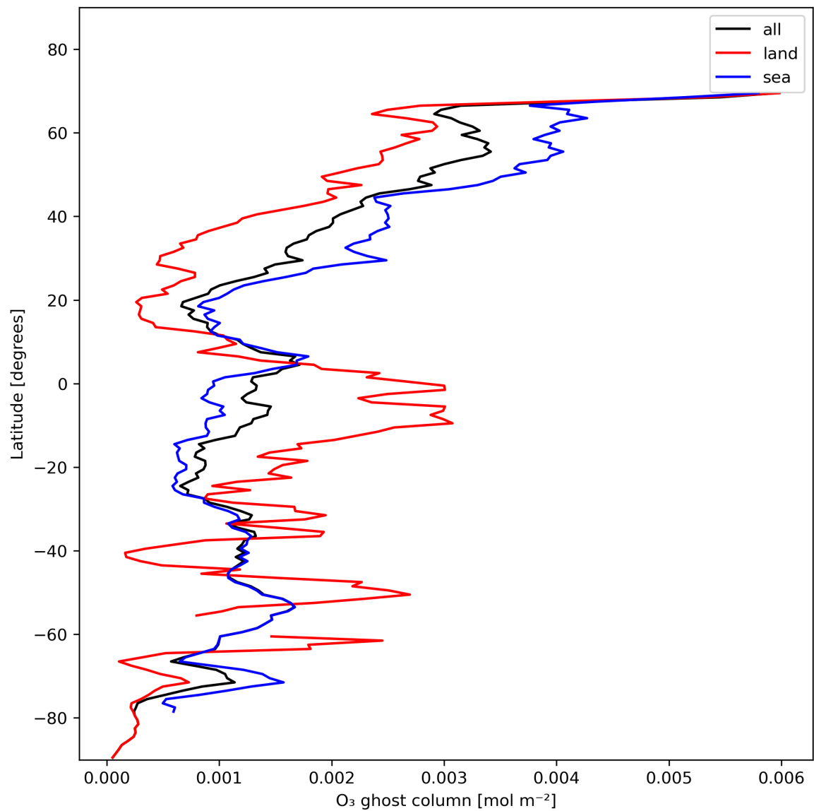
Figure 18: Zonal average of “O 3 ghost column” for 2023-11-20 to 2023-11-22.
