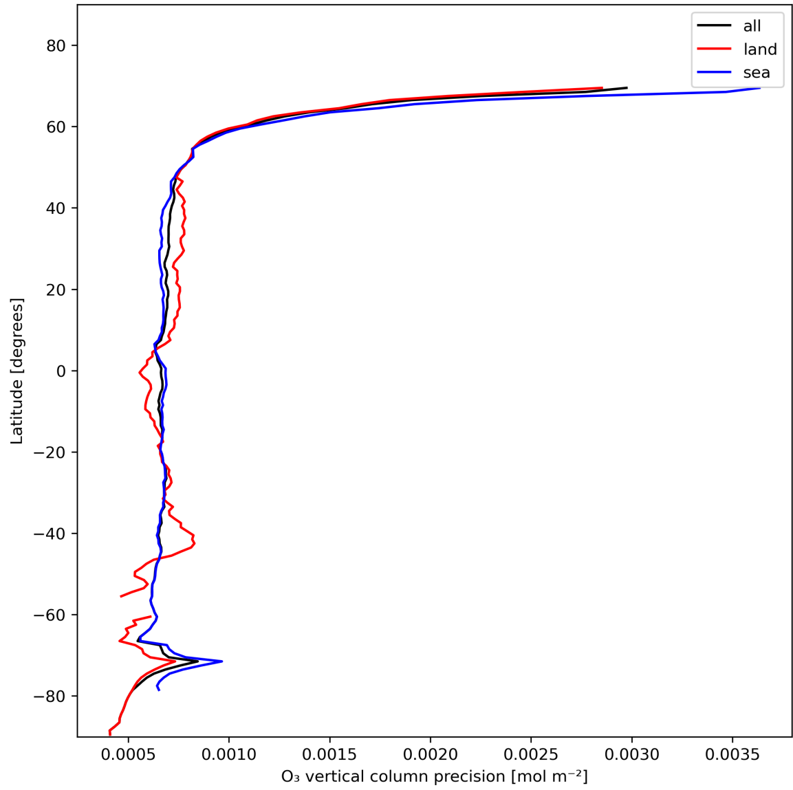
Figure 15: Zonal average of “O 3 vertical column precision” for 2023-11-20 to 2023-11-22.
