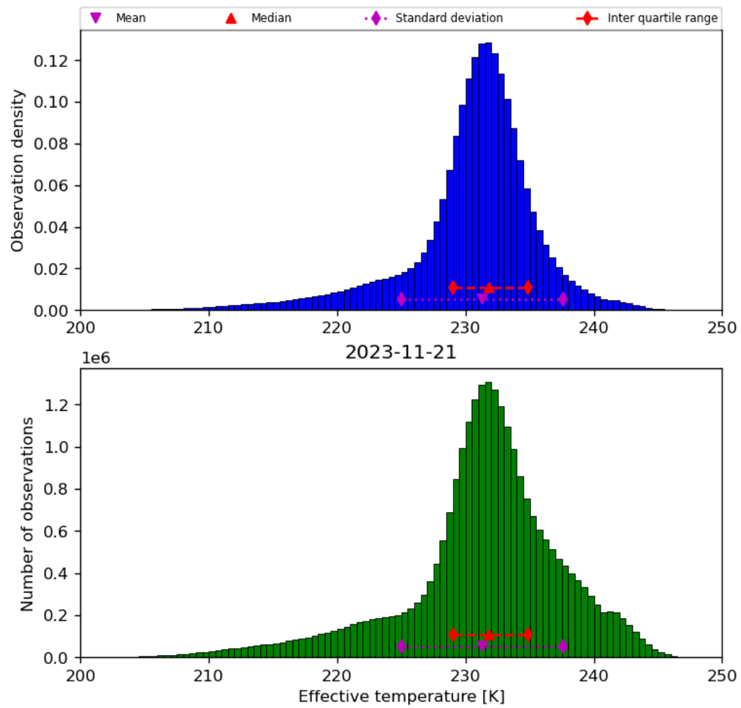
Figure 24: Histogram of “Effective temperature” for 2023-11-20 to 2023-11-22
