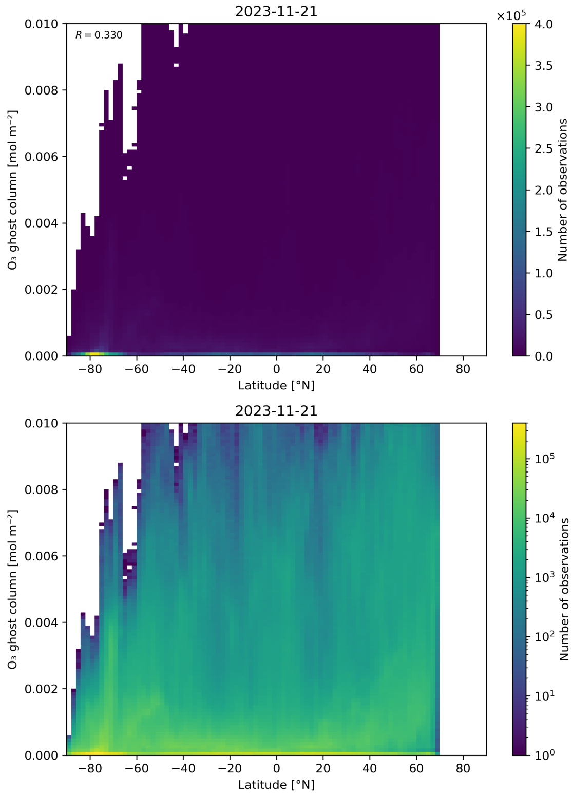
Figure 35: Scatter density plot of “Latitude” against “O 3 ghost column” for 2023-11-20 to 2023-11-22.
