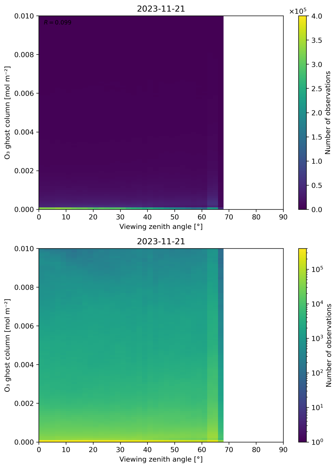
Figure 51: Scatter density plot of “Viewing zenith angle” against “O 3 ghost column” for 2023-11-20 to 2023-11-22.
