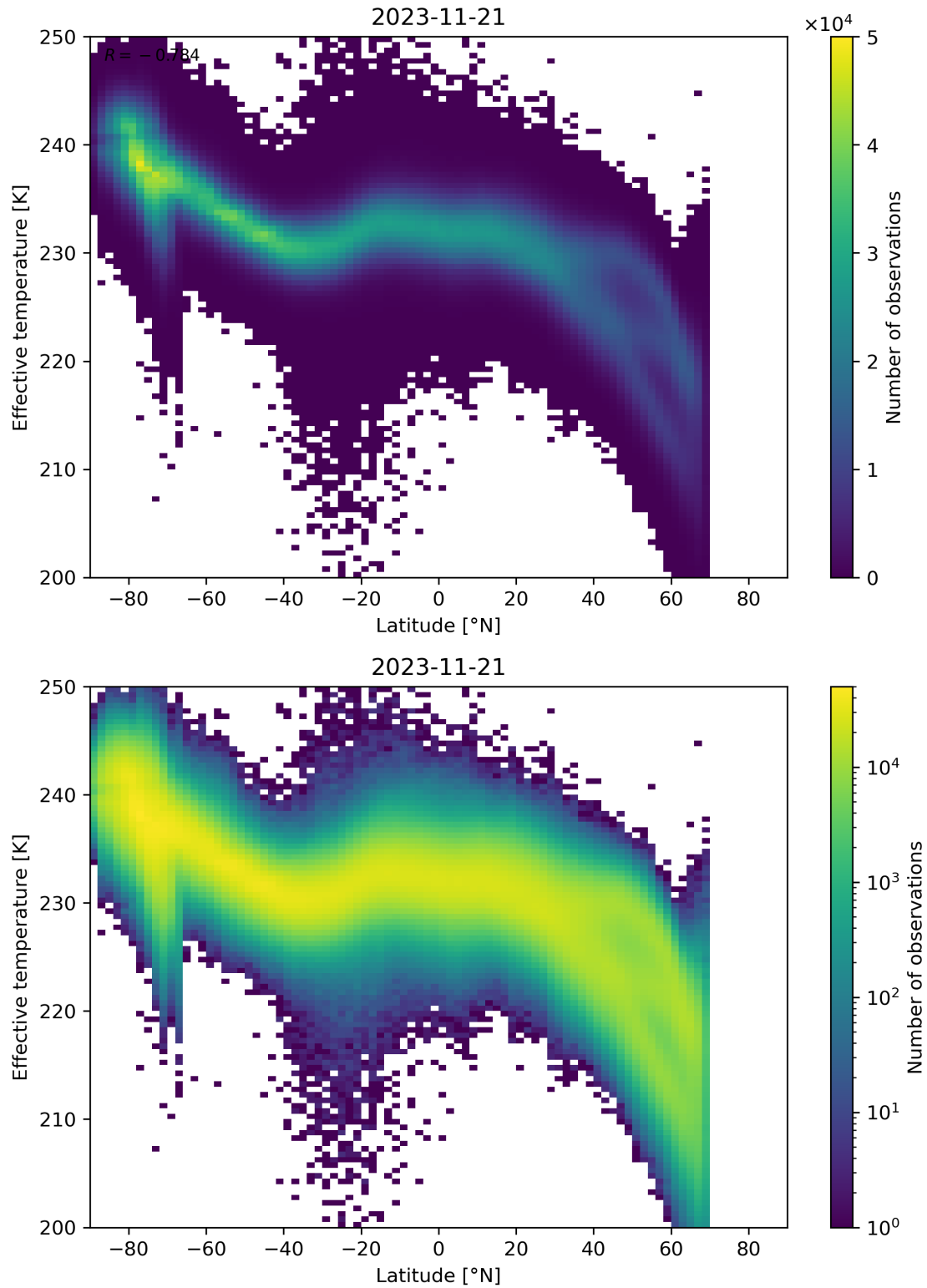
Figure 34: Scatter density plot of “Latitude” against “Effective temperature” for 2023-11-20 to 2023-11-22.
