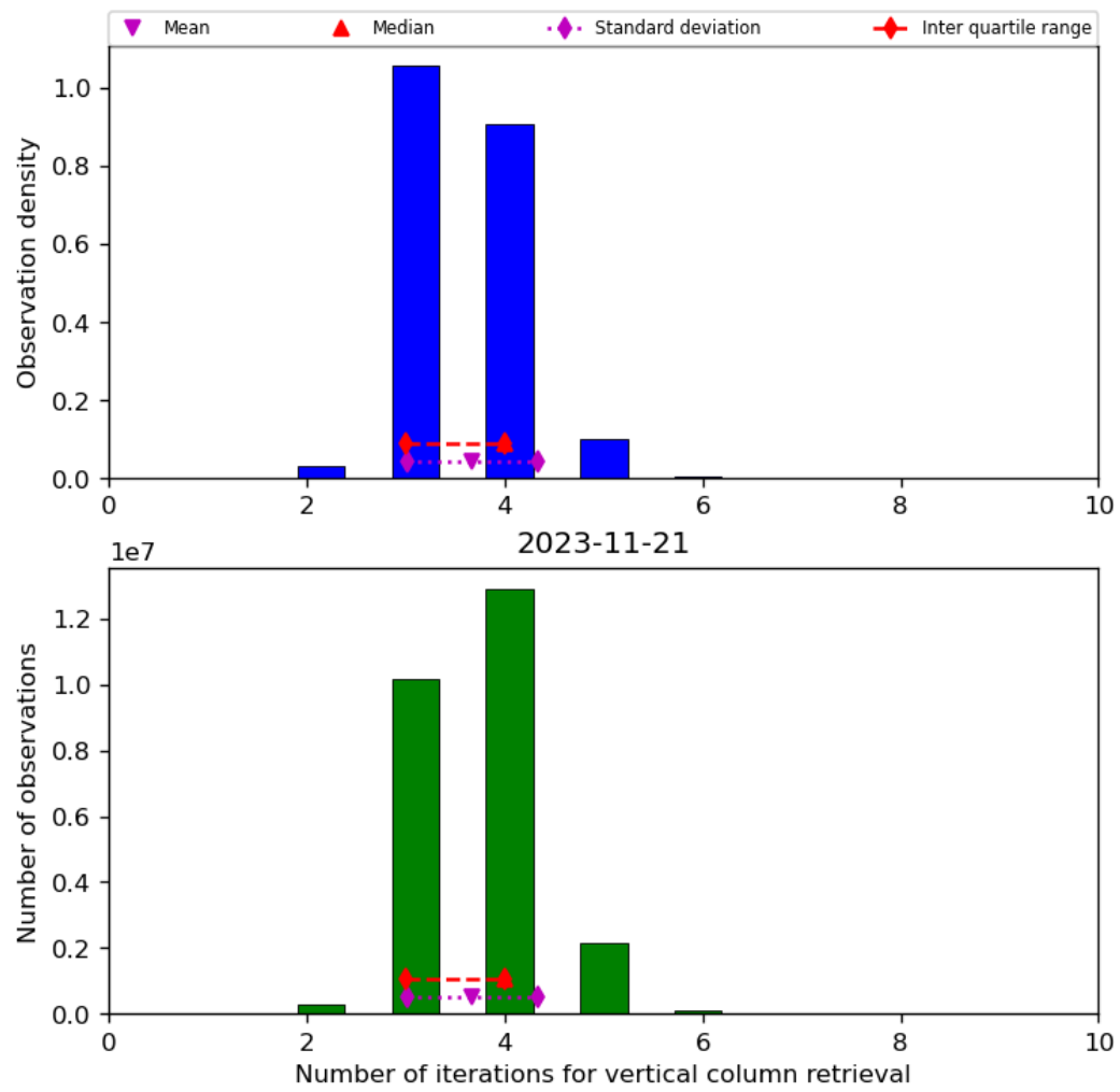
Figure 26: Histogram of “Number of iterations for vertical column retrieval” for 2023-11-20 to 2023-11-22
