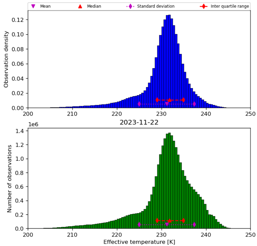
Figure 24: Histogram of “Effective temperature” for 2023-11-21 to 2023-11-23
