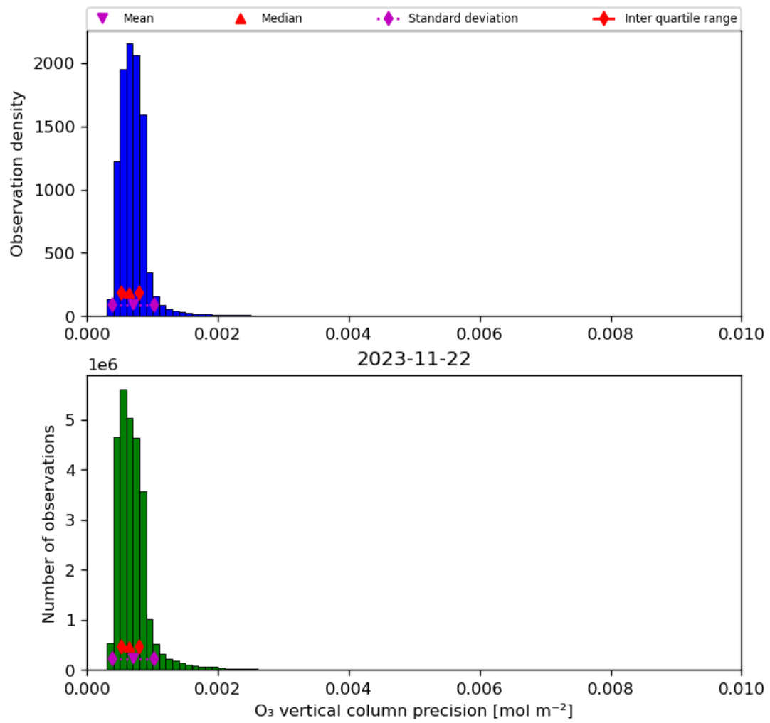
Figure 22: Histogram of “O 3 vertical column precision” for 2023-11-21 to 2023-11-23
