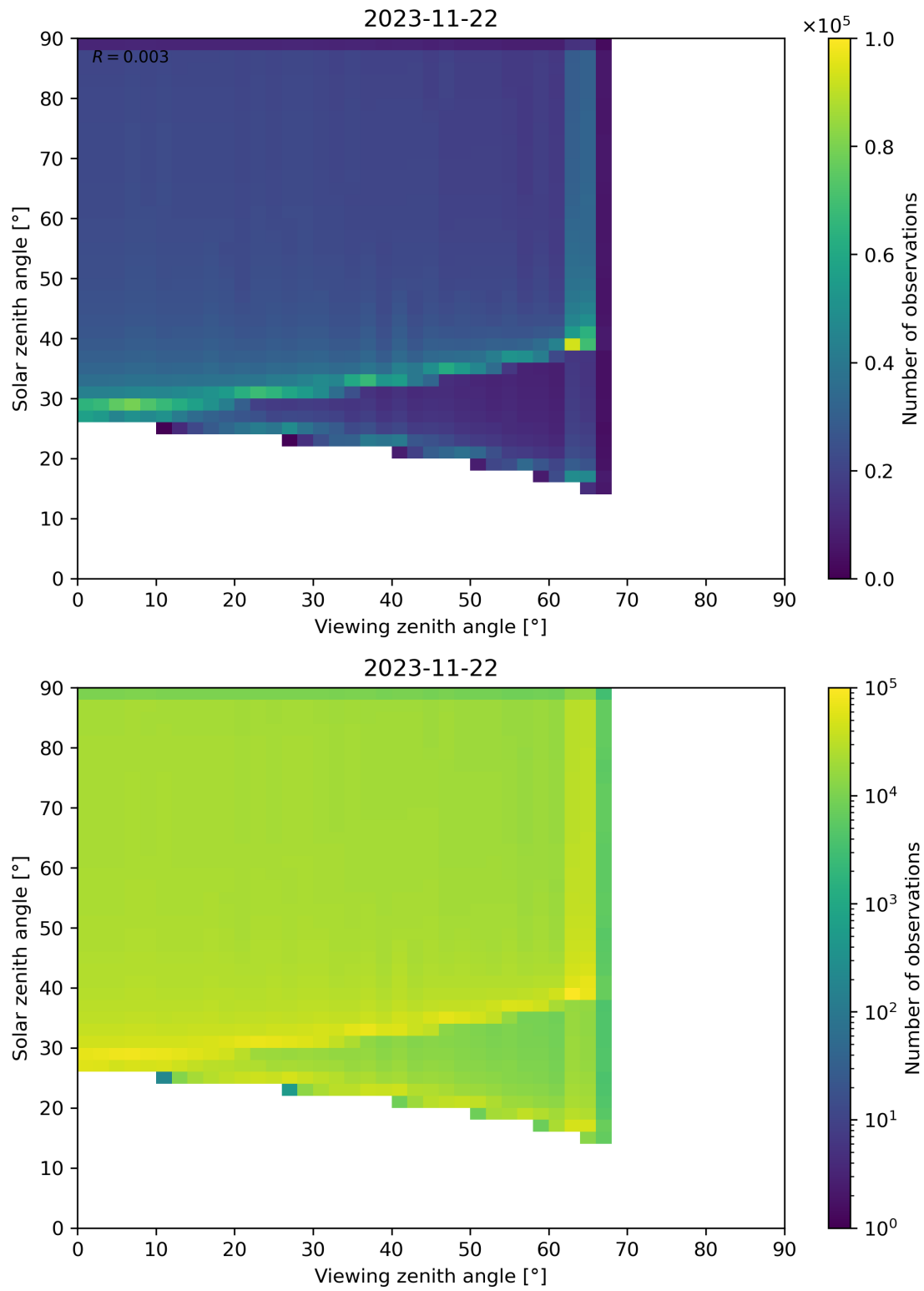
Figure 54: Scatter density plot of “Viewing zenith angle” against “Solar zenith angle” for 2023-11-21 to 2023-11-23.
