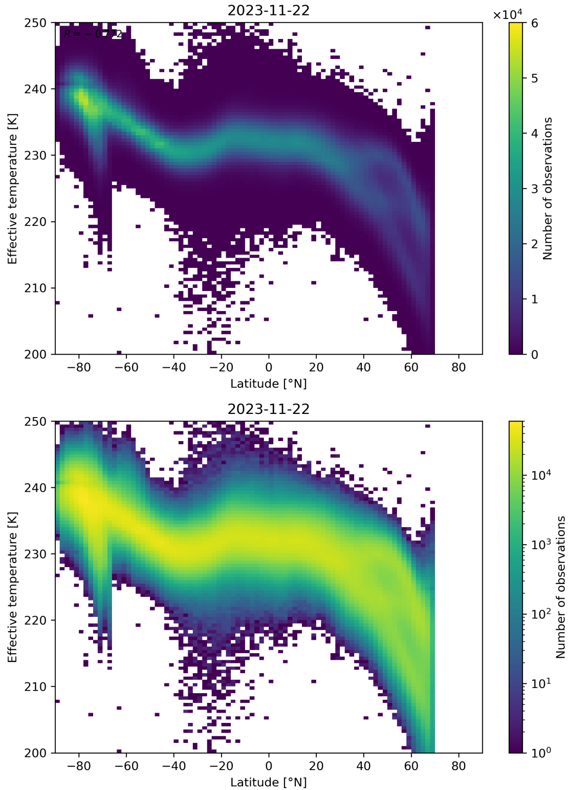
Figure 34: Scatter density plot of “Latitude” against “Effective temperature” for 2023-11-21 to 2023-11-23.
