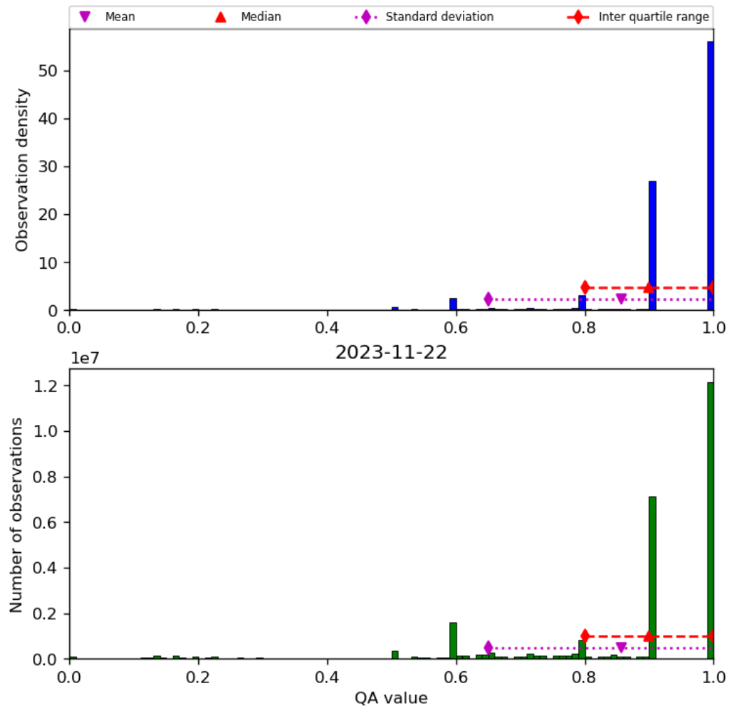
Figure 20: Histogram of “QA value” for 2023-11-21 to 2023-11-23
