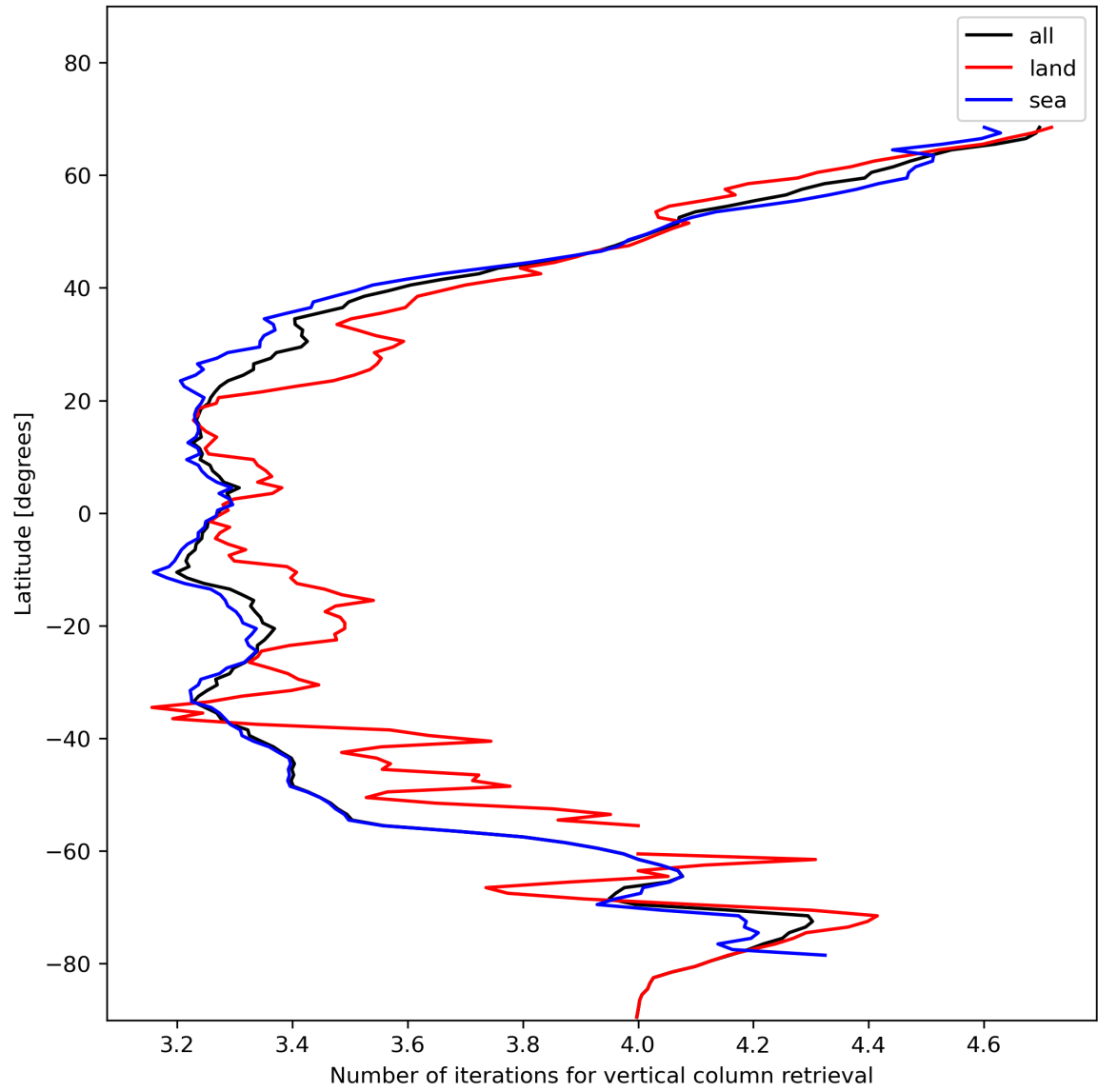
Figure 19: Zonal average of “Number of iterations for vertical column retrieval” for 2023-11-21 to 2023-11-23.
