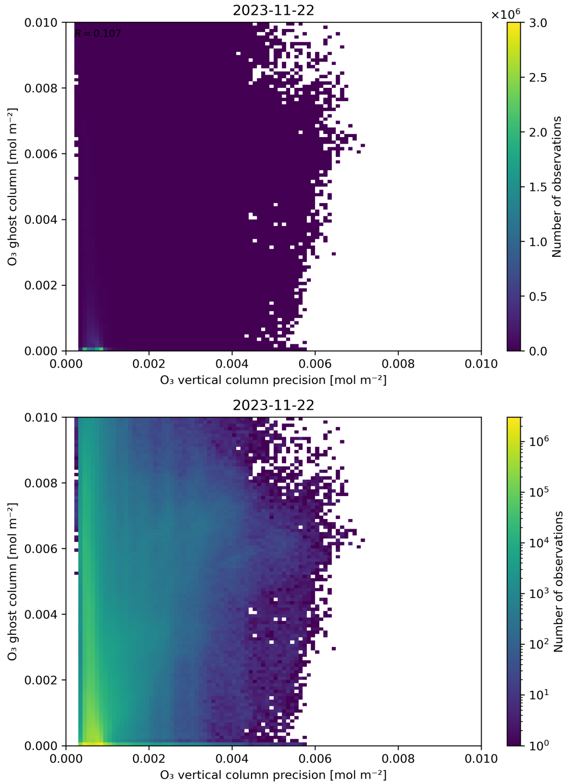
Figure 43: Scatter density plot of “O 3 vertical column precision” against “O 3 ghost column” for 2023-11-21 to 2023-11-23.
