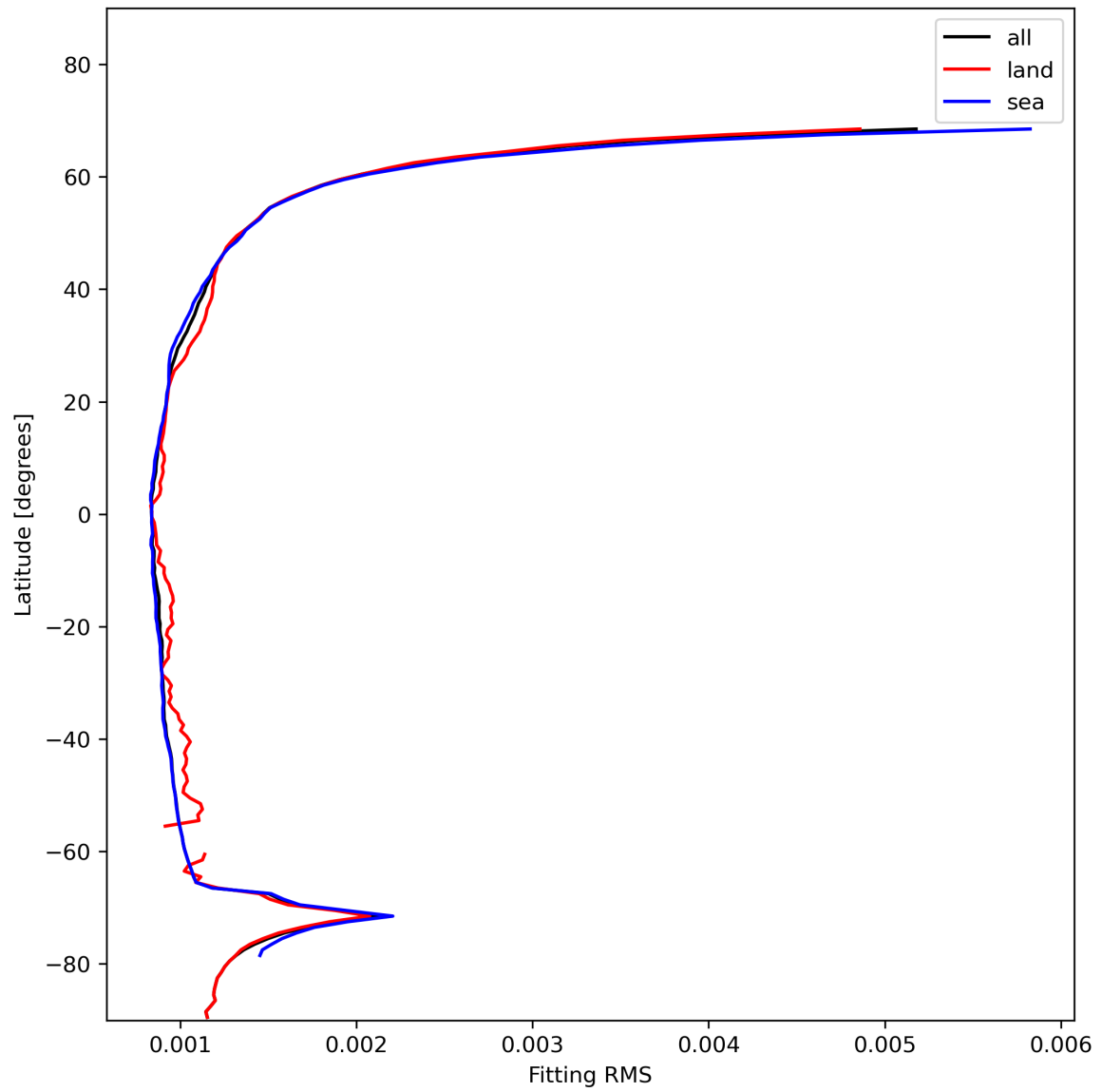
Figure 16: Zonal average of “Fitting RMS” for 2023-11-21 to 2023-11-23.
