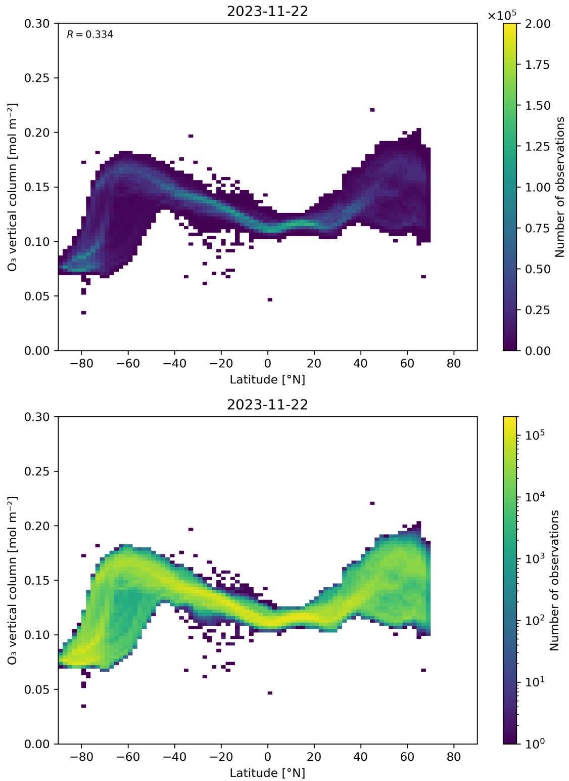
Figure 36: Scatter density plot of “Latitude” against “O 3 vertical column” for 2023-11-21 to 2023-11-23.
