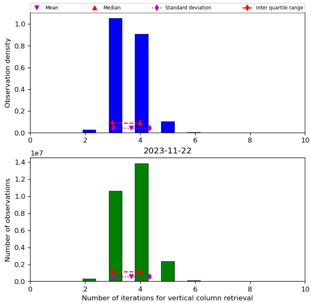
Figure 26: Histogram of “Number of iterations for vertical column retrieval” for 2023-11-21 to 2023-11-23
