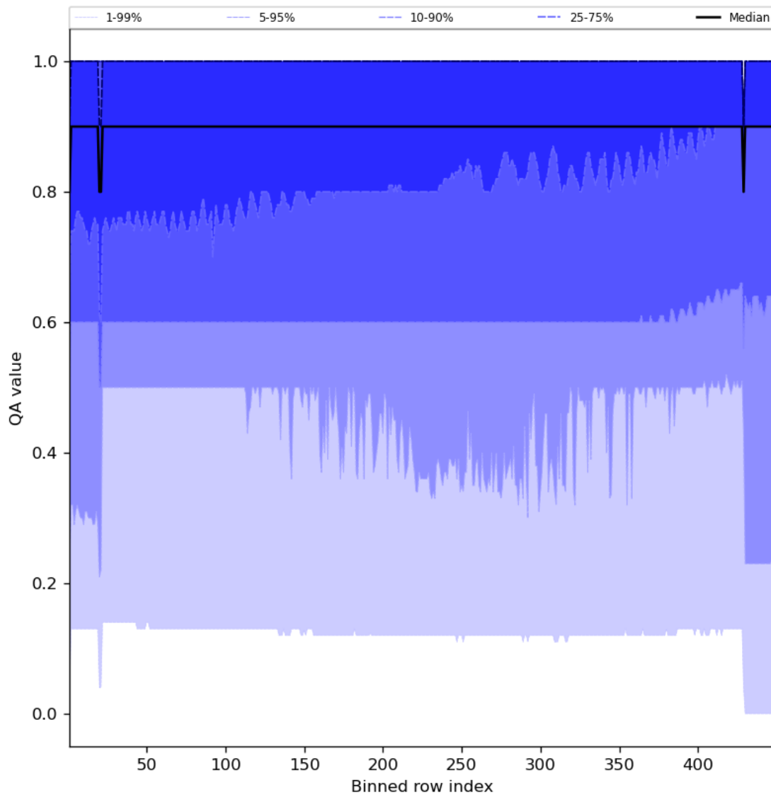
Figure 27: Along track statistics of “QA value” for 2023-11-21 to 2023-11-23
