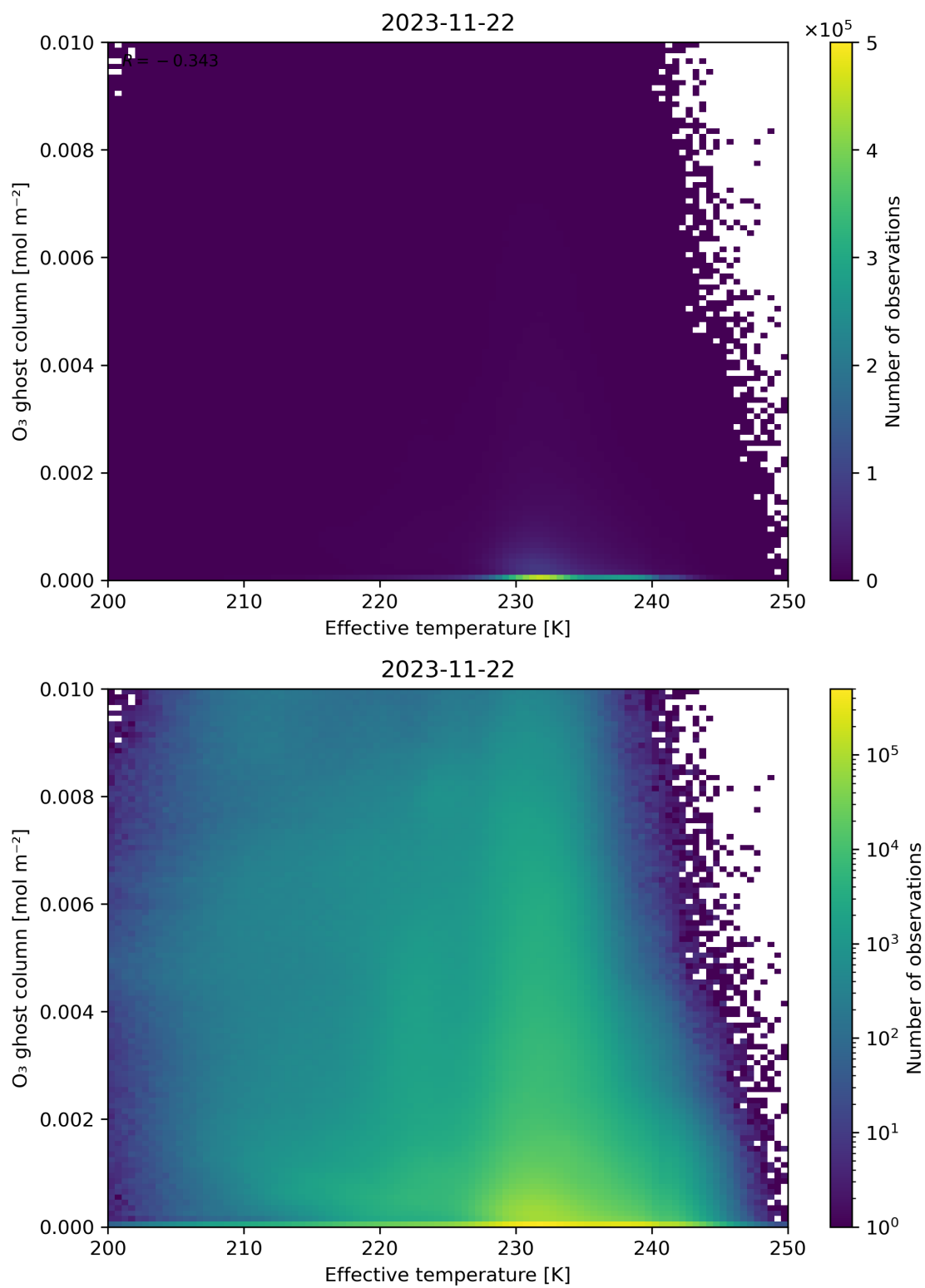
Figure 38: Scatter density plot of “Effective temperature” against “O 3 ghost column” for 2023-11-21 to 2023-11-23.
