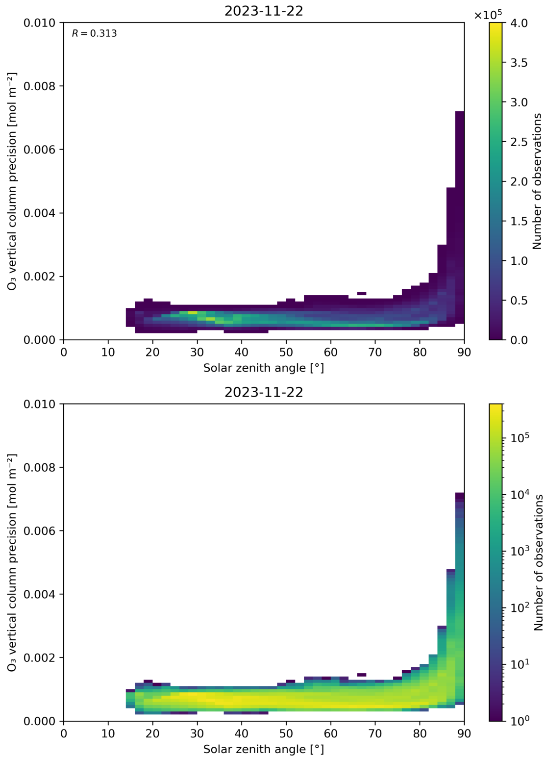
Figure 48: Scatter density plot of “Solar zenith angle” against “O 3 vertical column precision” for 2023-11-21 to 2023-11-23.
