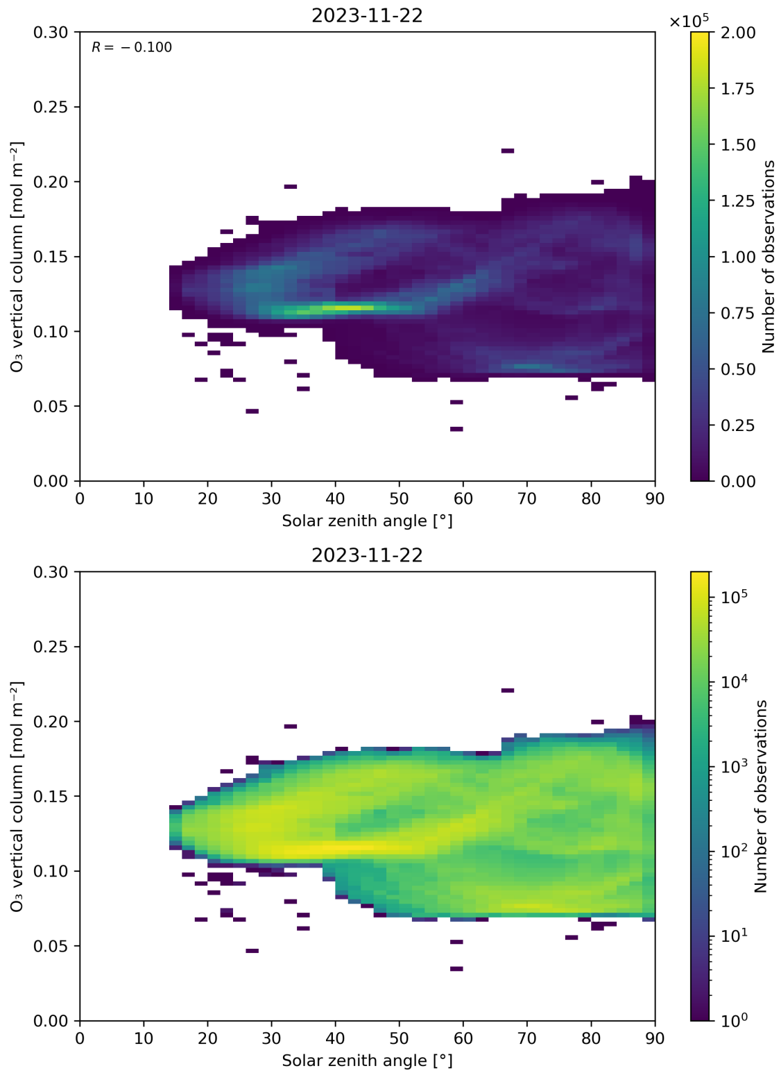
Figure 47: Scatter density plot of “Solar zenith angle” against “O 3 vertical column” for 2023-11-21 to 2023-11-23.
