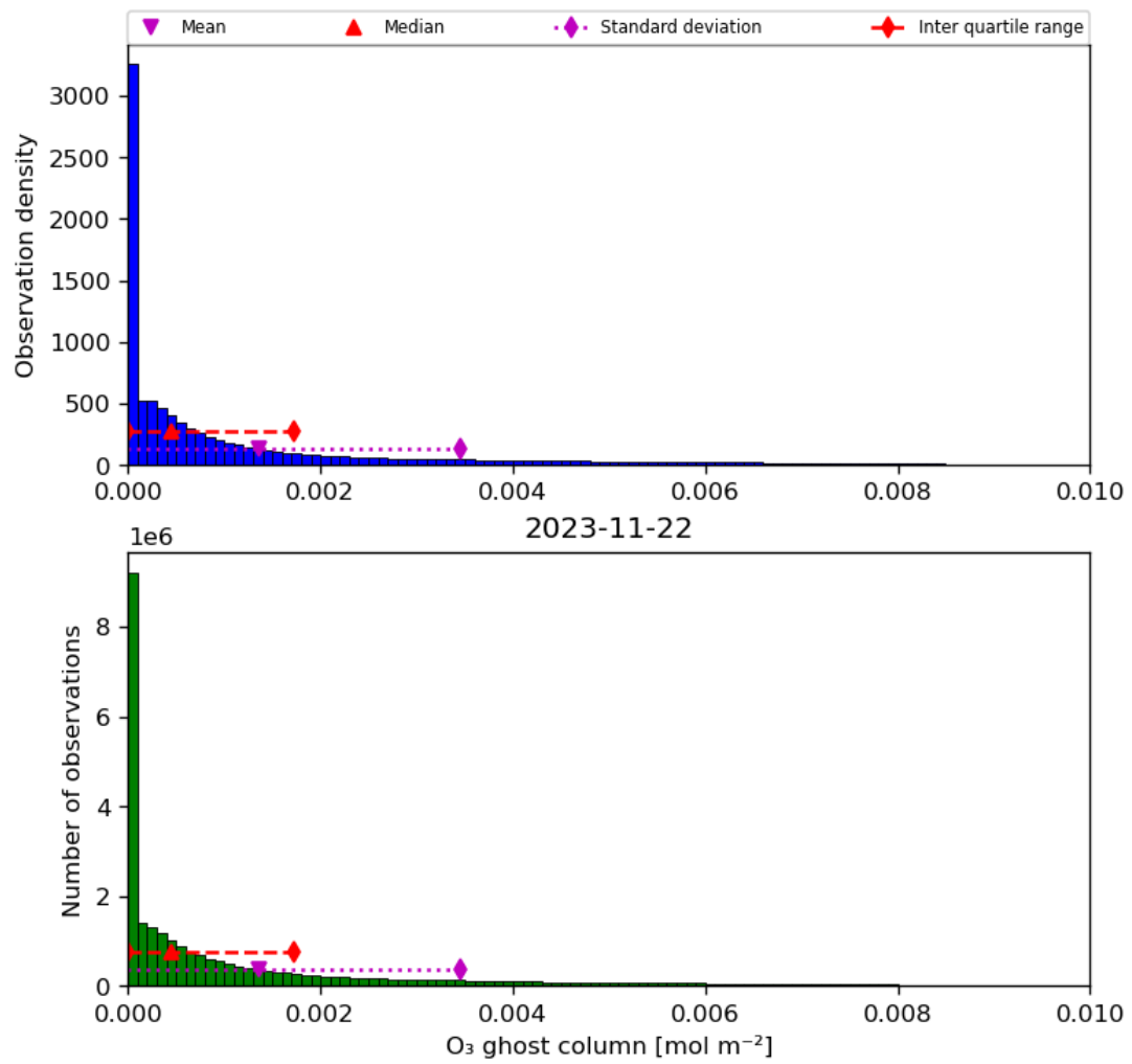
Figure 25: Histogram of “O 3 ghost column” for 2023-11-21 to 2023-11-23
