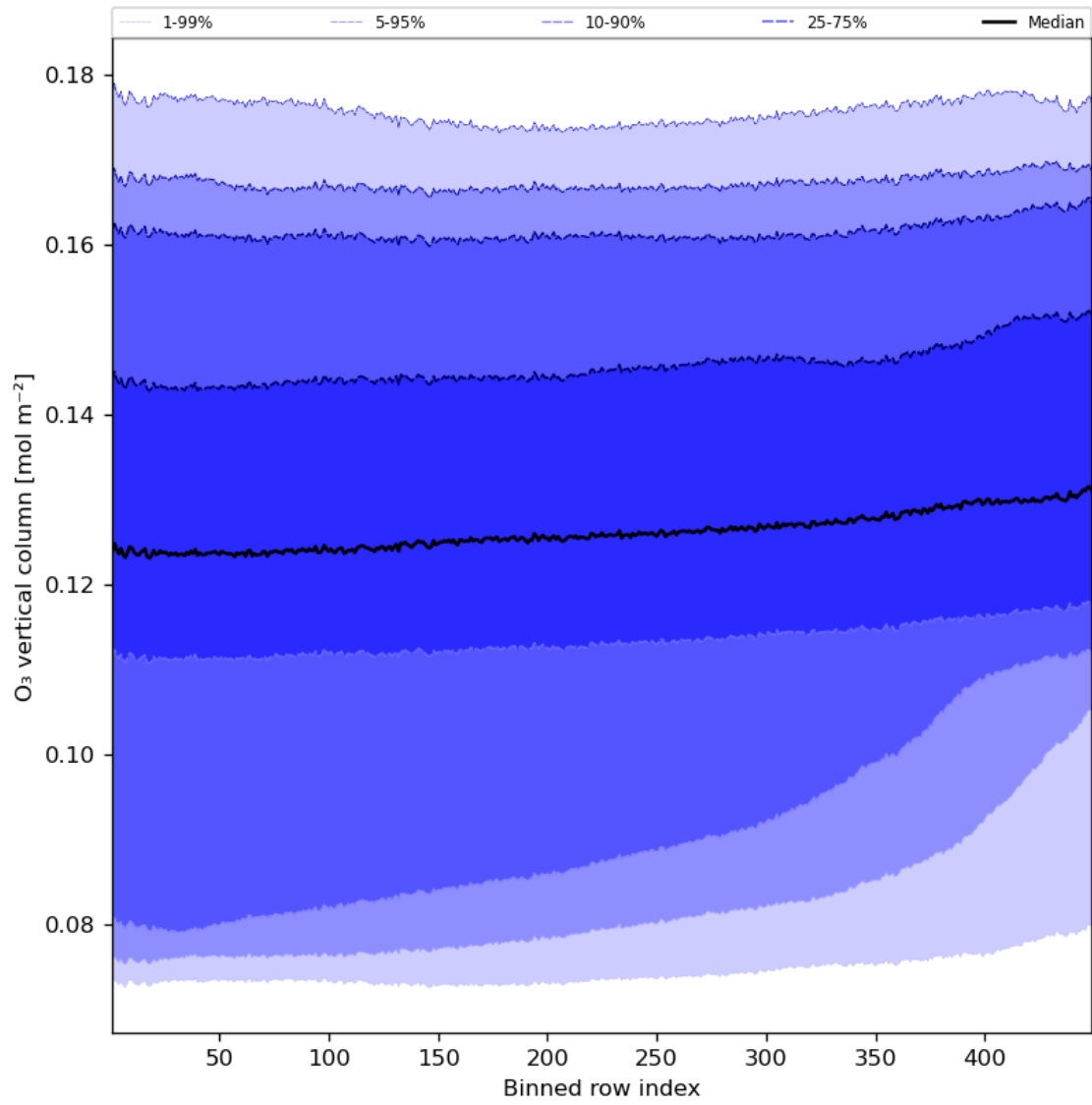
Figure 28: Along track statistics of “O 3 vertical column” for 2023-11-21 to 2023-11-23
