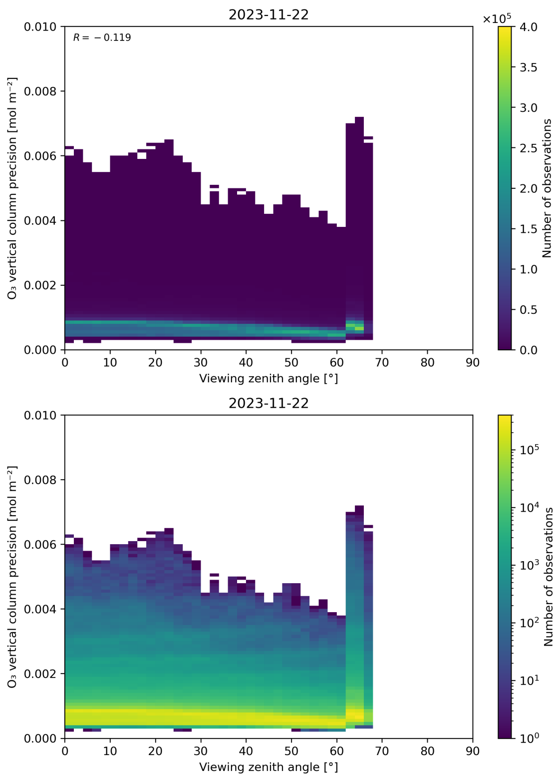
Figure 53: Scatter density plot of “Viewing zenith angle” against “O 3 vertical column precision” for 2023-11-21 to 2023-11-23.
