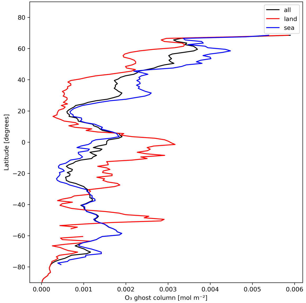
Figure 18: Zonal average of “O 3 ghost column” for 2023-11-21 to 2023-11-23.
