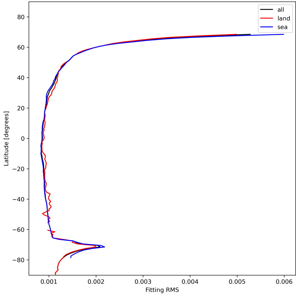
Figure 16: Zonal average of “Fitting RMS” for 2023-11-23 to 2023-11-24.
