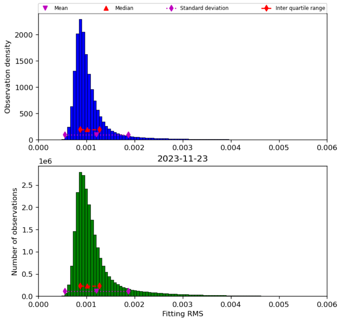
Figure 23: Histogram of “Fitting RMS” for 2023-11-23 to 2023-11-24
