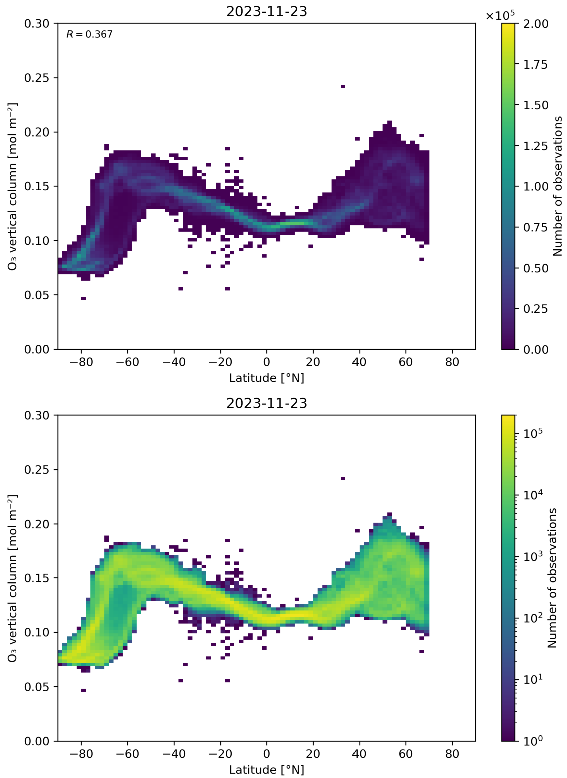
Figure 36: Scatter density plot of “Latitude” against “O 3 vertical column” for 2023-11-23 to 2023-11-24.
