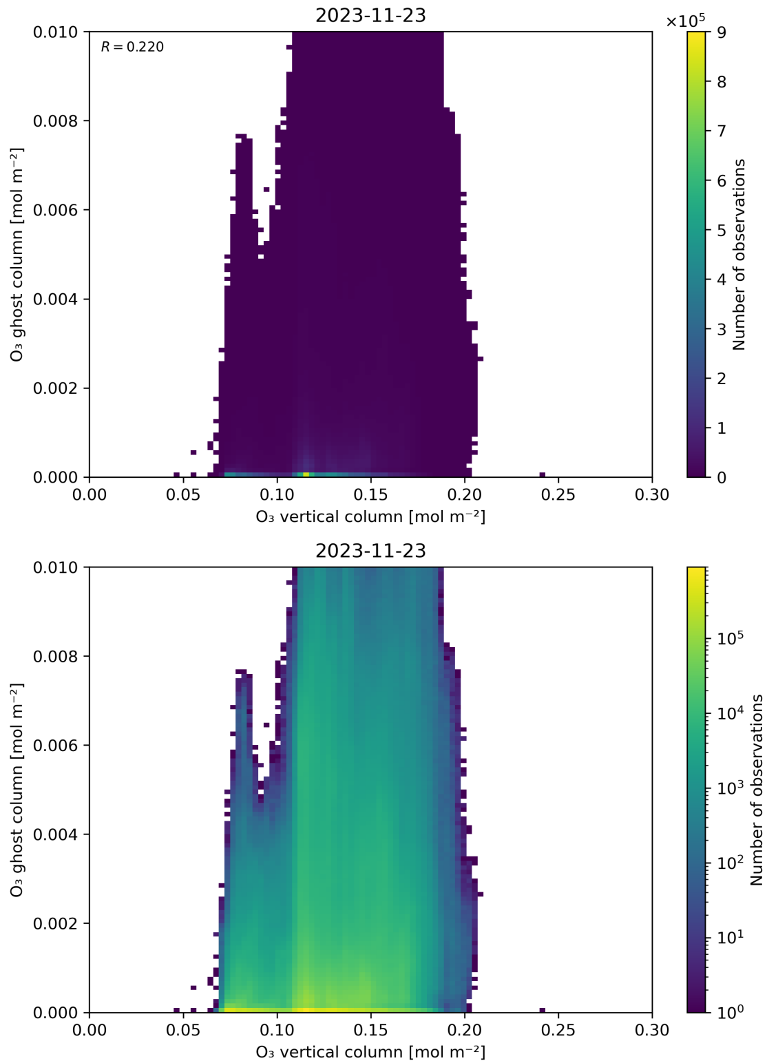
Figure 40: Scatter density plot of “O 3 vertical column” against “O 3 ghost column” for 2023-11-23 to 2023-11-24.
