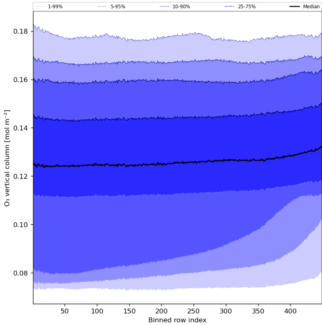
Figure 28: Along track statistics of “O 3 vertical column” for 2023-11-23 to 2023-11-24
