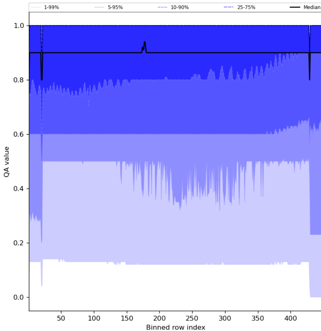
Figure 27: Along track statistics of “QA value” for 2023-11-23 to 2023-11-24
