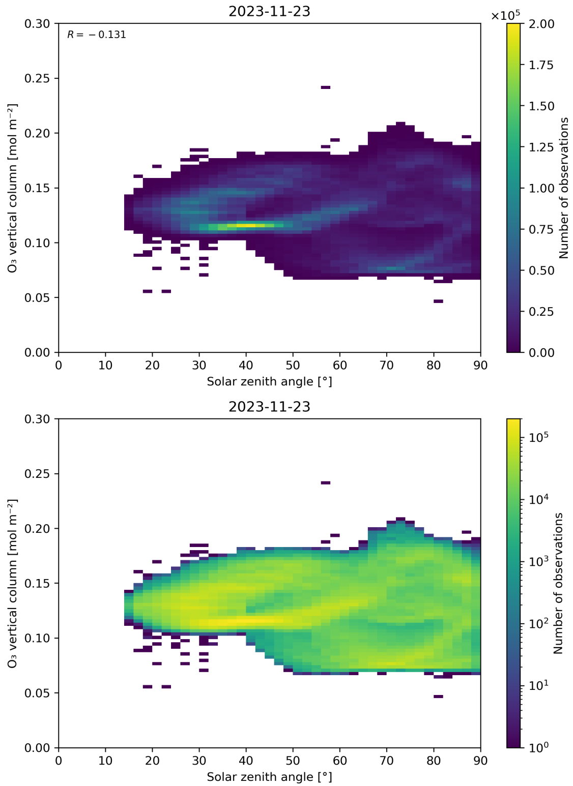
Figure 47: Scatter density plot of “Solar zenith angle” against “O 3 vertical column” for 2023-11-23 to 2023-11-24.
