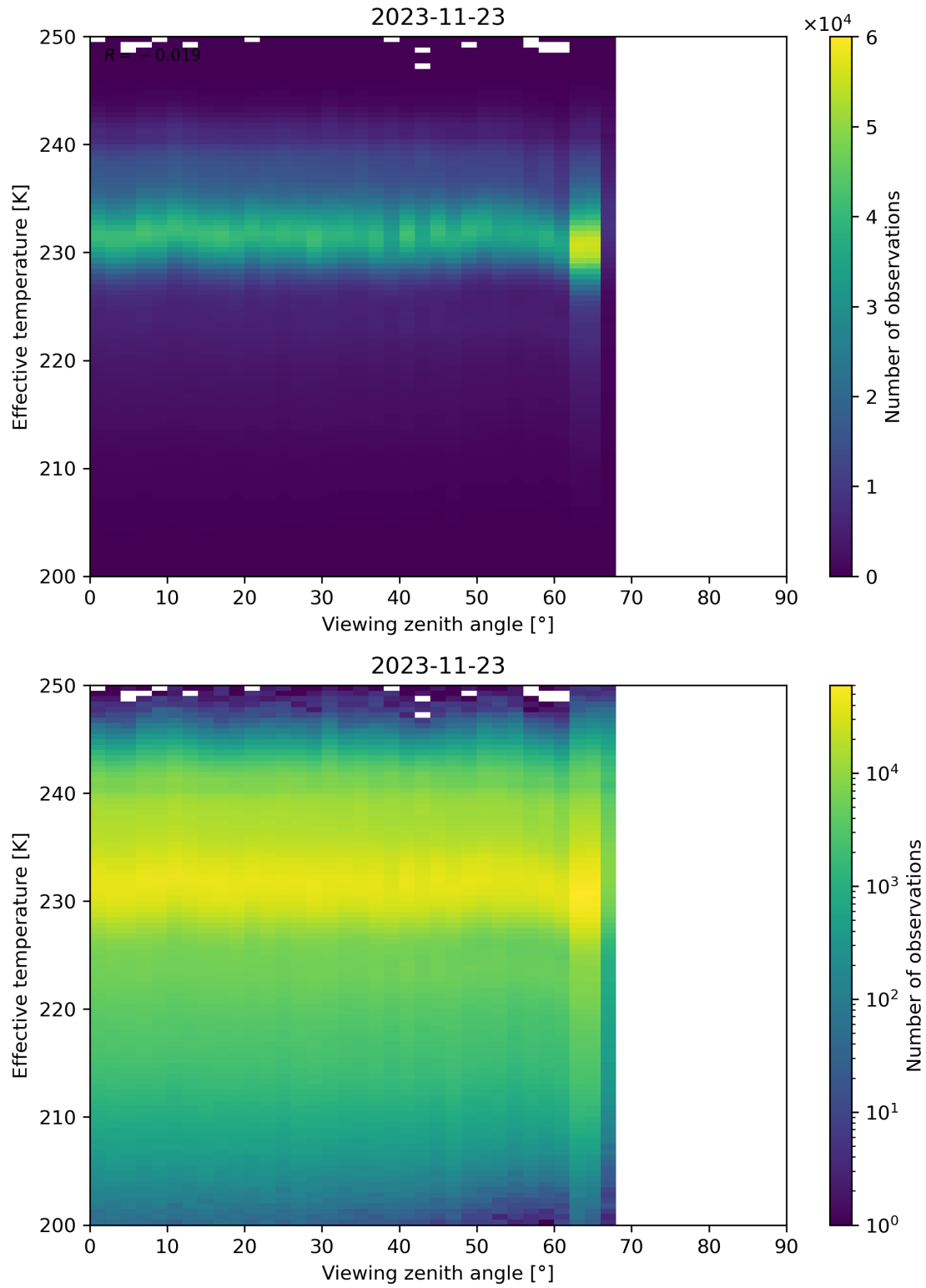
Figure 50: Scatter density plot of “Viewing zenith angle” against “Effective temperature” for 2023-11-23 to 2023-11-24.
