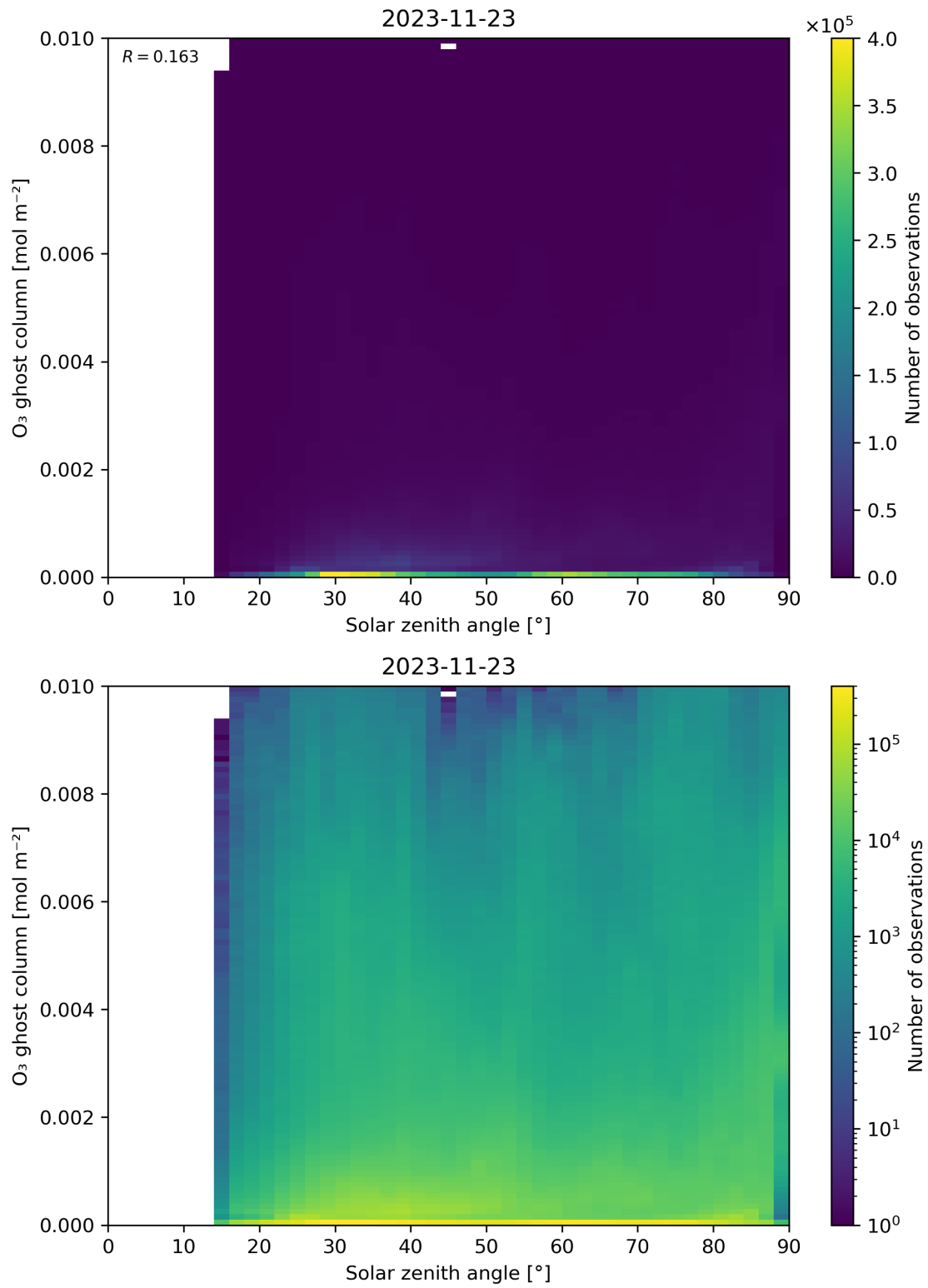
Figure 46: Scatter density plot of “Solar zenith angle” against “O 3 ghost column” for 2023-11-23 to 2023-11-24.
