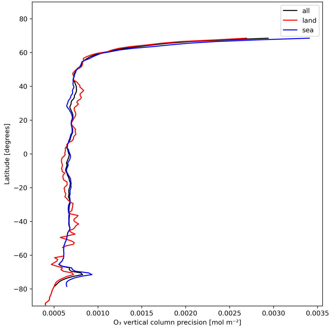
Figure 15: Zonal average of “O 3 vertical column precision” for 2023-11-23 to 2023-11-24.
