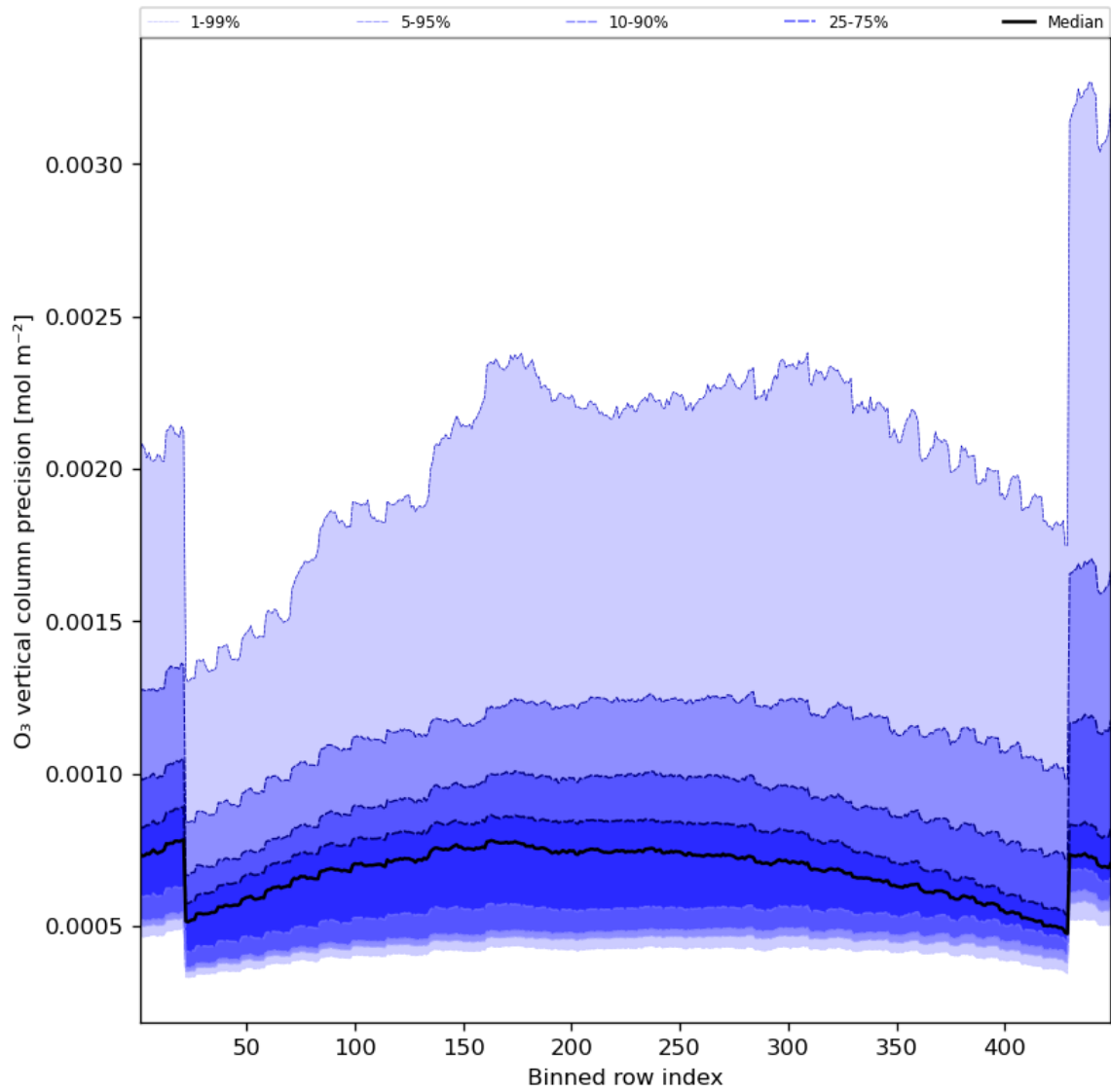
Figure 29: Along track statistics of “O 3 vertical column precision” for 2023-11-23 to 2023-11-24
