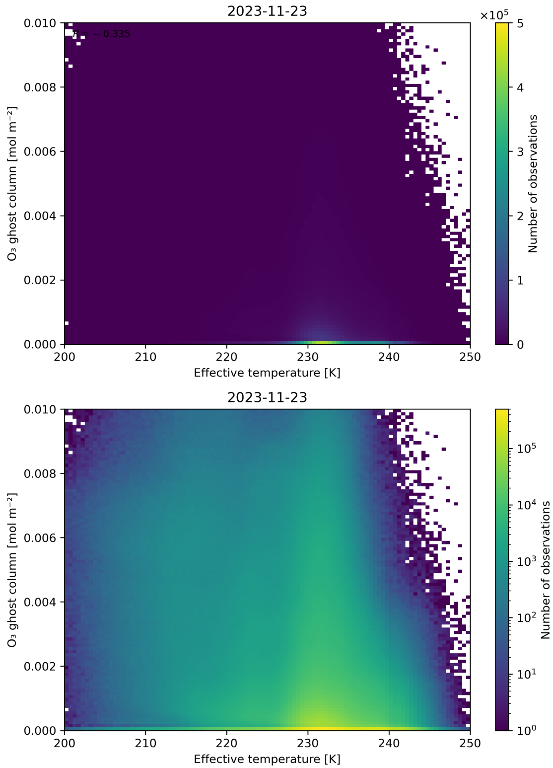
Figure 38: Scatter density plot of “Effective temperature” against “O 3 ghost column” for 2023-11-23 to 2023-11-24.
