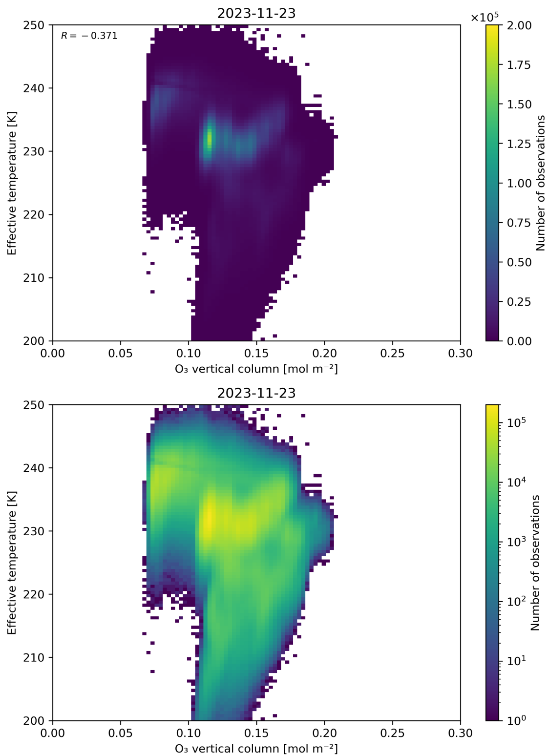
Figure 39: Scatter density plot of “O 3 vertical column” against “Effective temperature” for 2023-11-23 to 2023-11-24.
