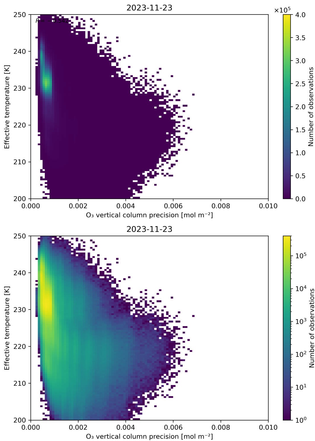
Figure 42: Scatter density plot of “O 3 vertical column precision” against “Effective temperature” for 2023-11-23 to 2023-11-24.
