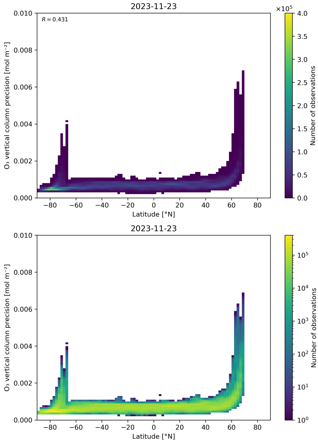
Figure 37: Scatter density plot of “Latitude” against “O 3 vertical column precision” for 2023-11-23 to 2023-11-24.
