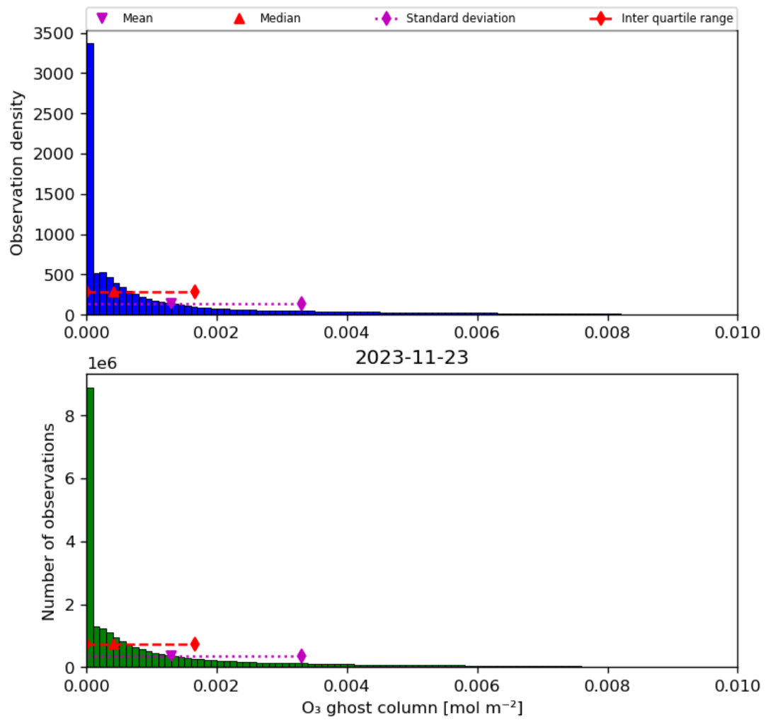
Figure 25: Histogram of “O 3 ghost column” for 2023-11-23 to 2023-11-24
