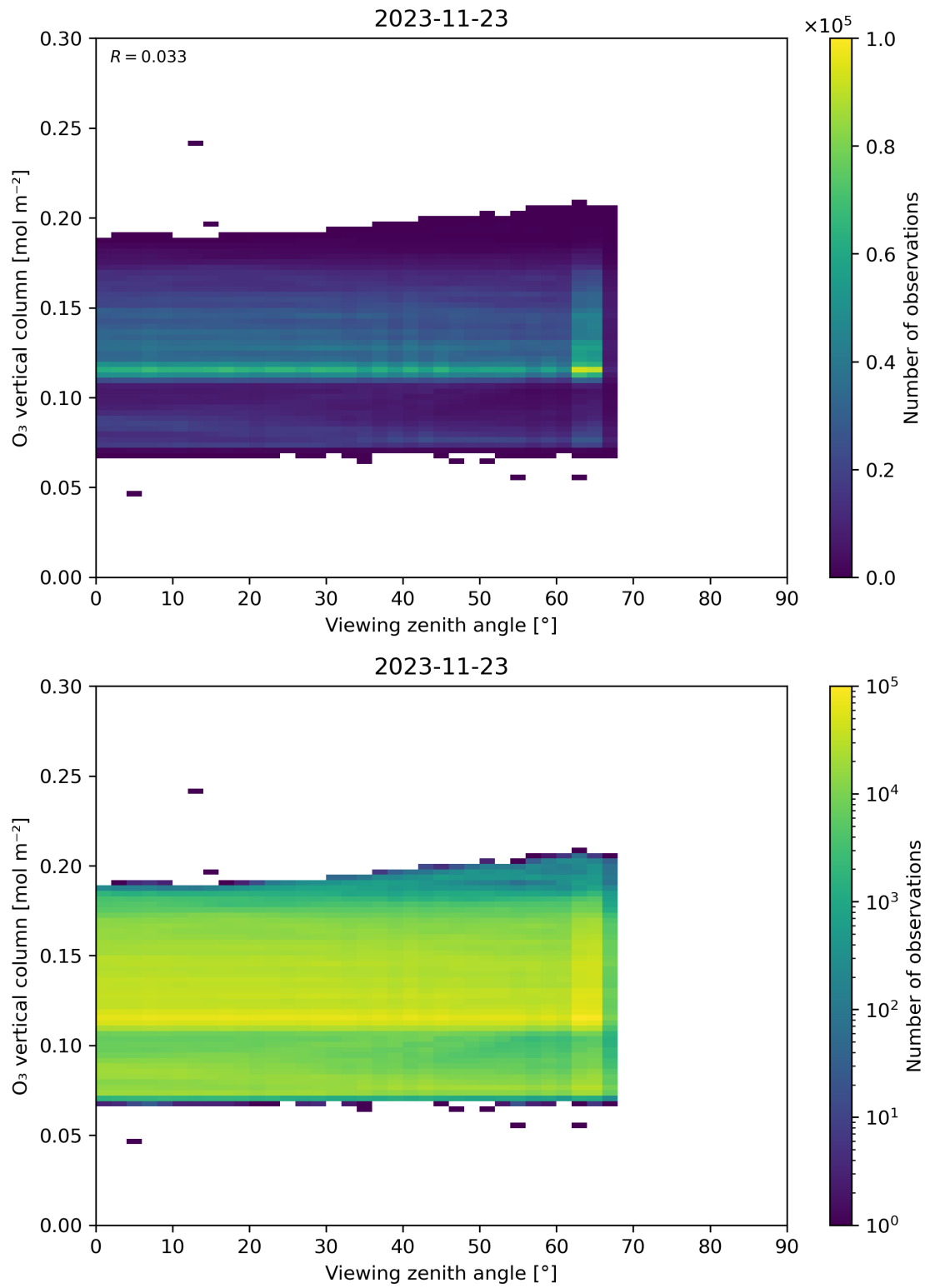
Figure 52: Scatter density plot of “Viewing zenith angle” against “O 3 vertical column” for 2023-11-23 to 2023-11-24.
