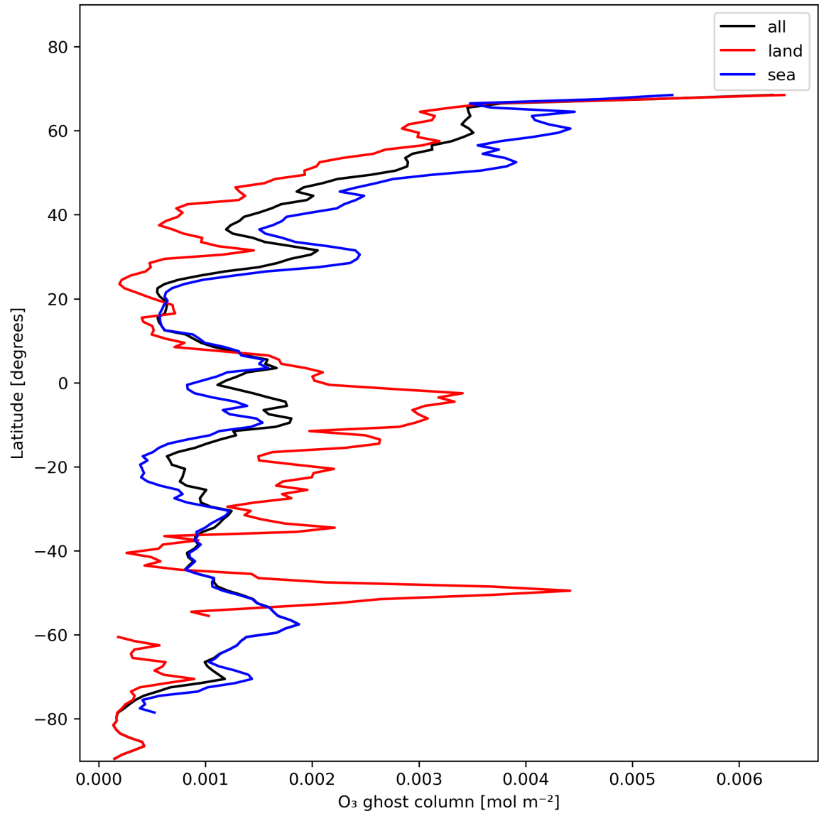
Figure 18: Zonal average of "O 3 ghost column" for 2023-11-23 to 2023-11-24.
