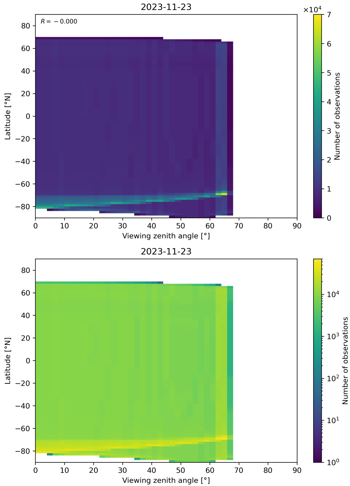
Figure 49: Scatter density plot of “Viewing zenith angle” against “Latitude” for 2023-11-23 to 2023-11-24.
