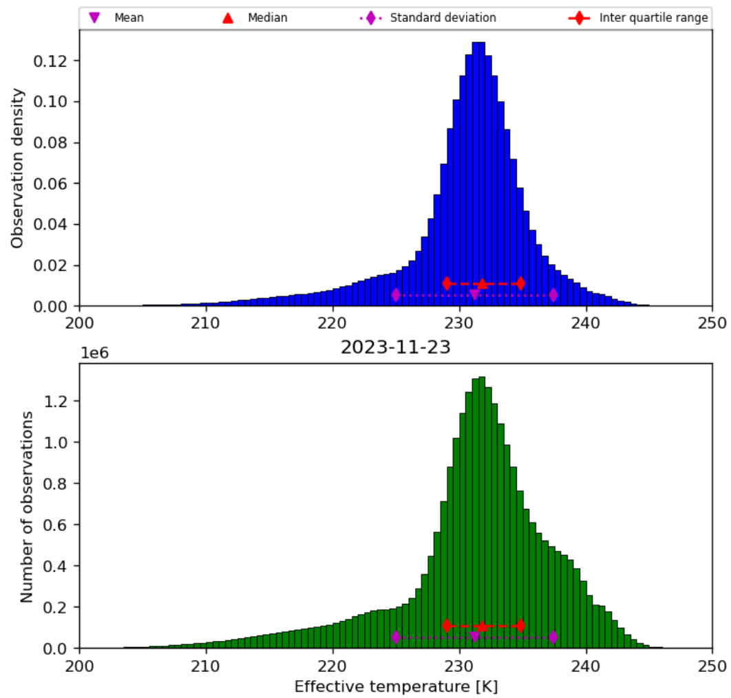
Figure 24: Histogram of “Effective temperature” for 2023-11-23 to 2023-11-24
