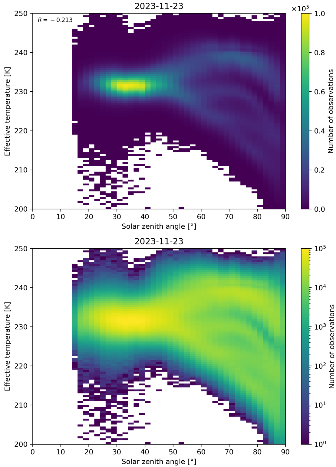
Figure 45: Scatter density plot of “Solar zenith angle” against “Effective temperature” for 2023-11-23 to 2023-11-24.
