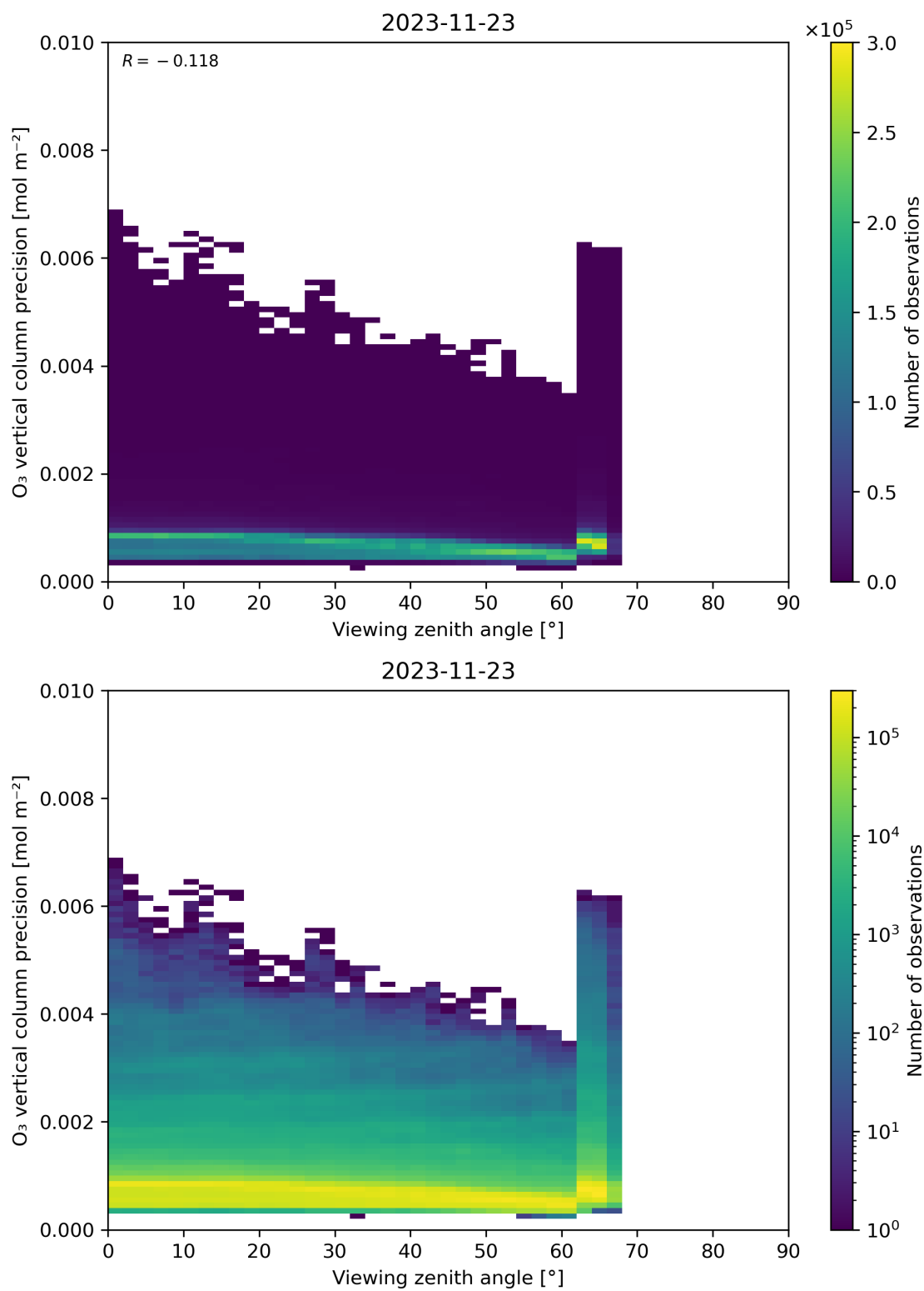
Figure 53: Scatter density plot of “Viewing zenith angle” against “O 3 vertical column precision” for 2023-11-23 to 2023-11-24.
