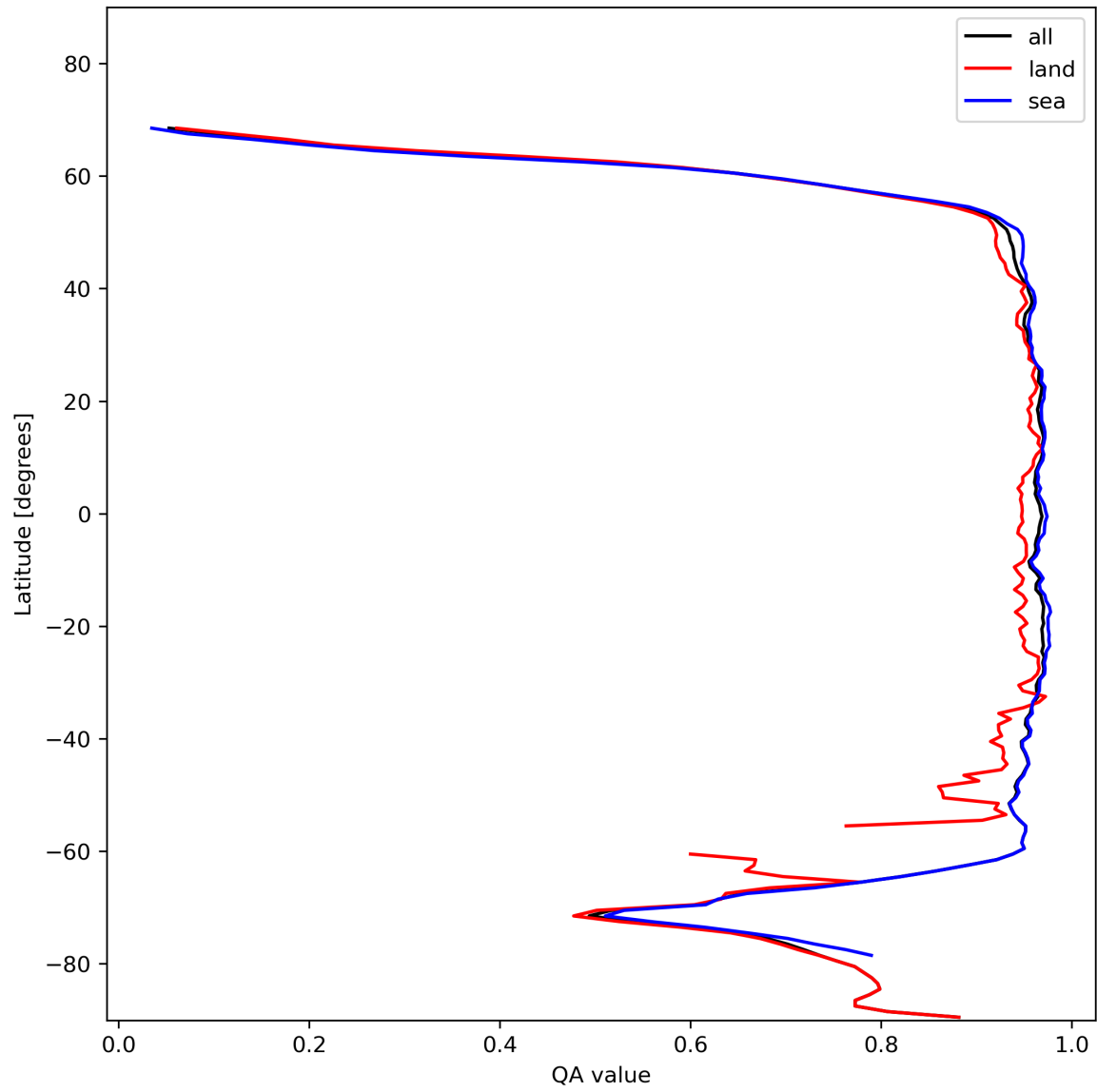
Figure 13: Zonal average of “QA value” for 2023-11-23 to 2023-11-24.
