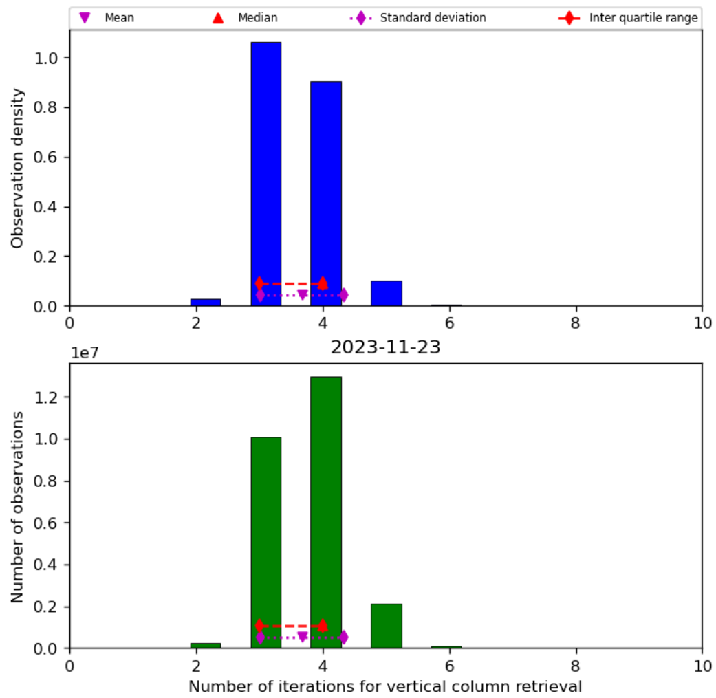
Figure 26: Histogram of “Number of iterations for vertical column retrieval” for 2023-11-23 to 2023-11-24
