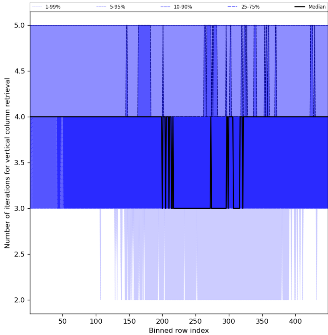
Figure 33: Along track statistics of “Number of iterations for vertical column retrieval” for 2023-11-23 to 2023-11-24
