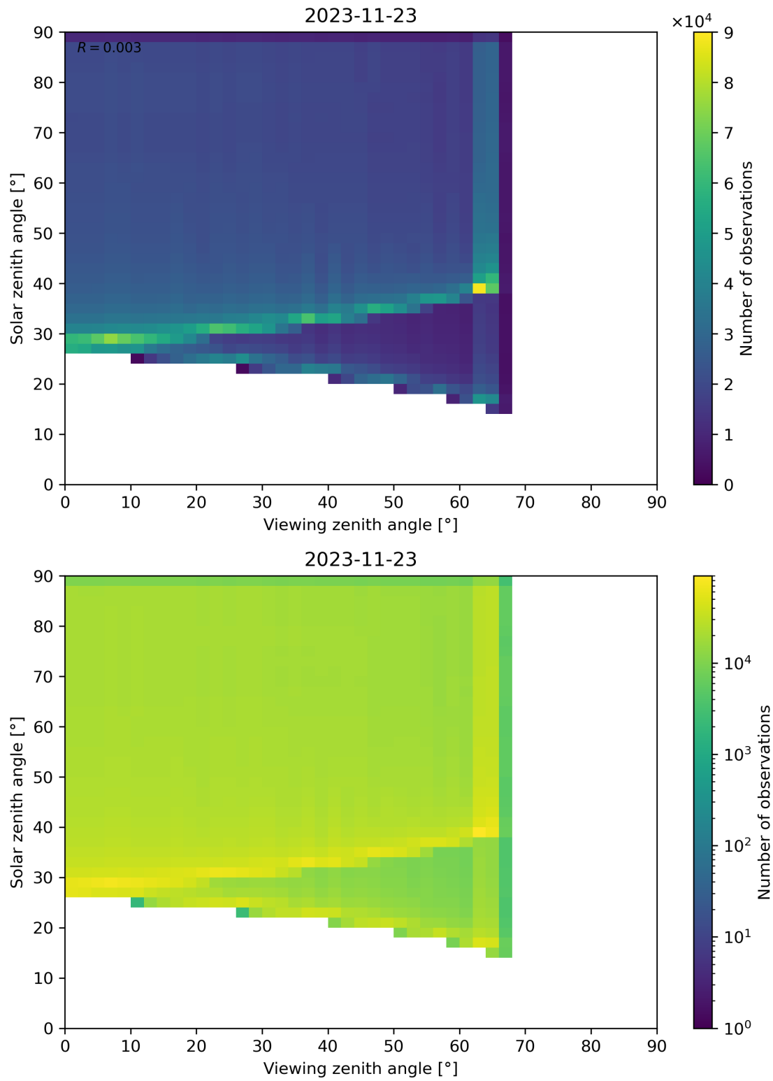
Figure 54: Scatter density plot of “Viewing zenith angle” against “Solar zenith angle” for 2023-11-23 to 2023-11-24.
