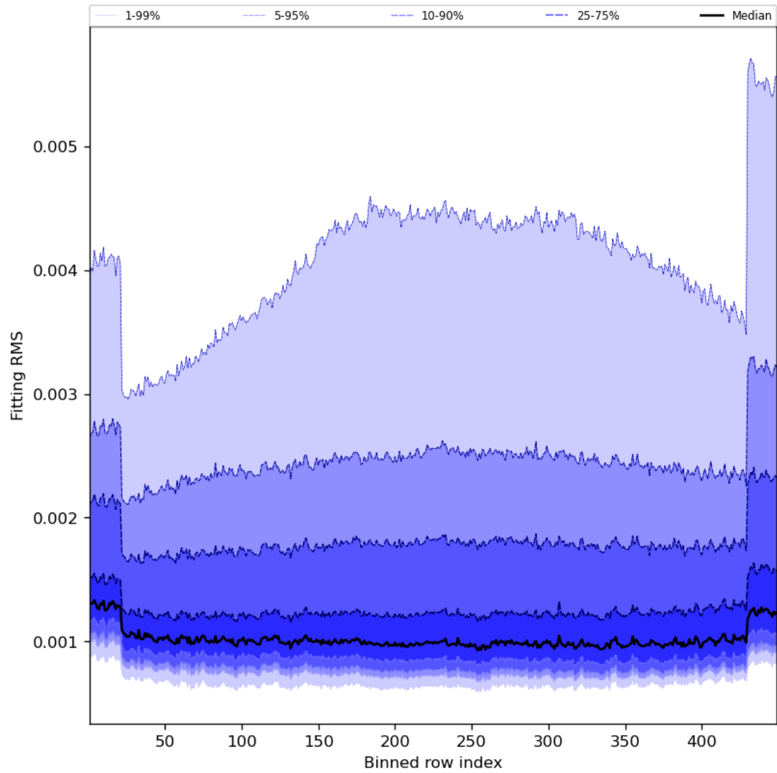
Figure 30: Along track statistics of “Fitting RMS” for 2023-11-23 to 2023-11-24
