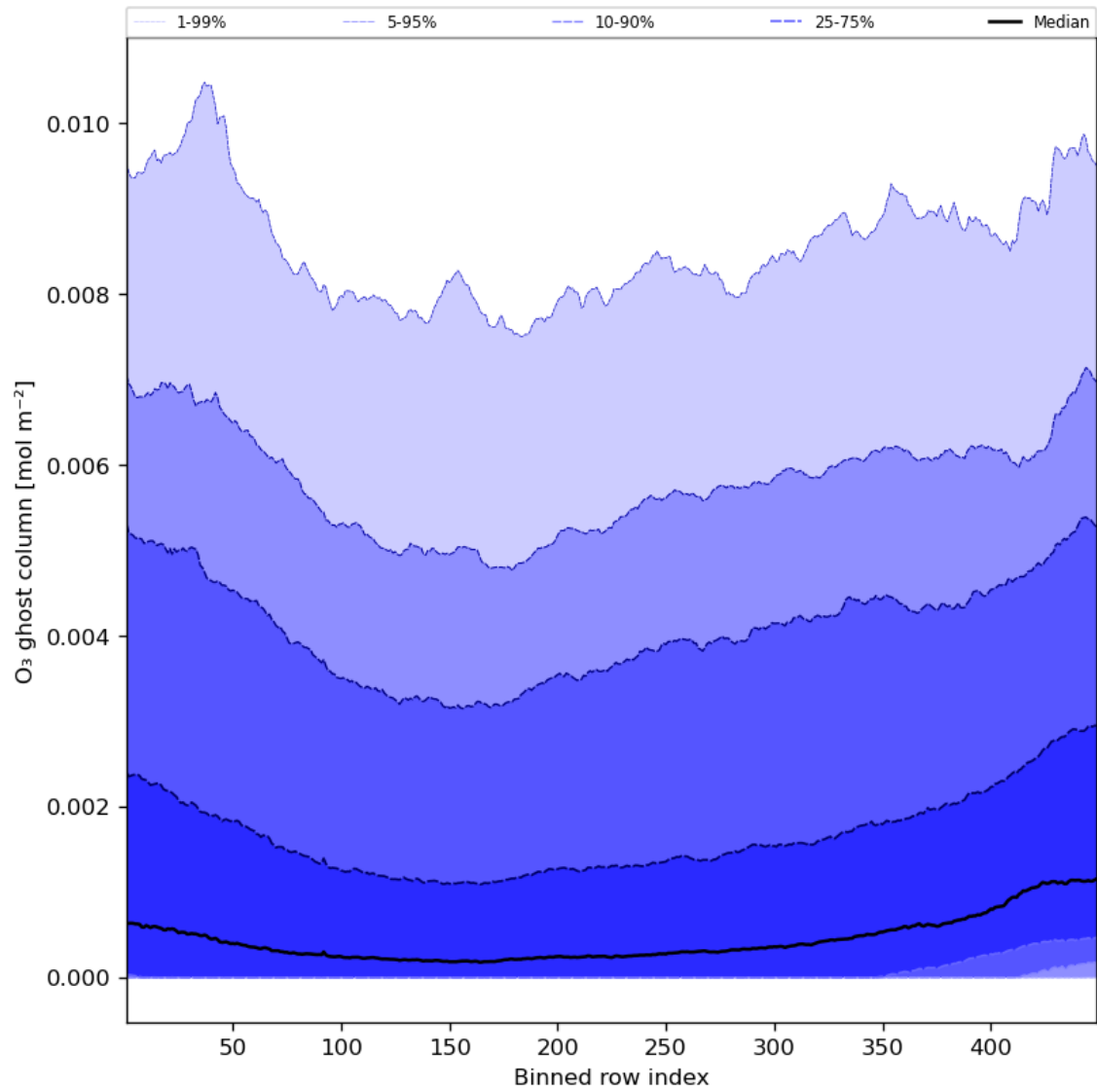
Figure 32: Along track statistics of "O 3 ghost column" for 2023-11-23 to 2023-11-24
