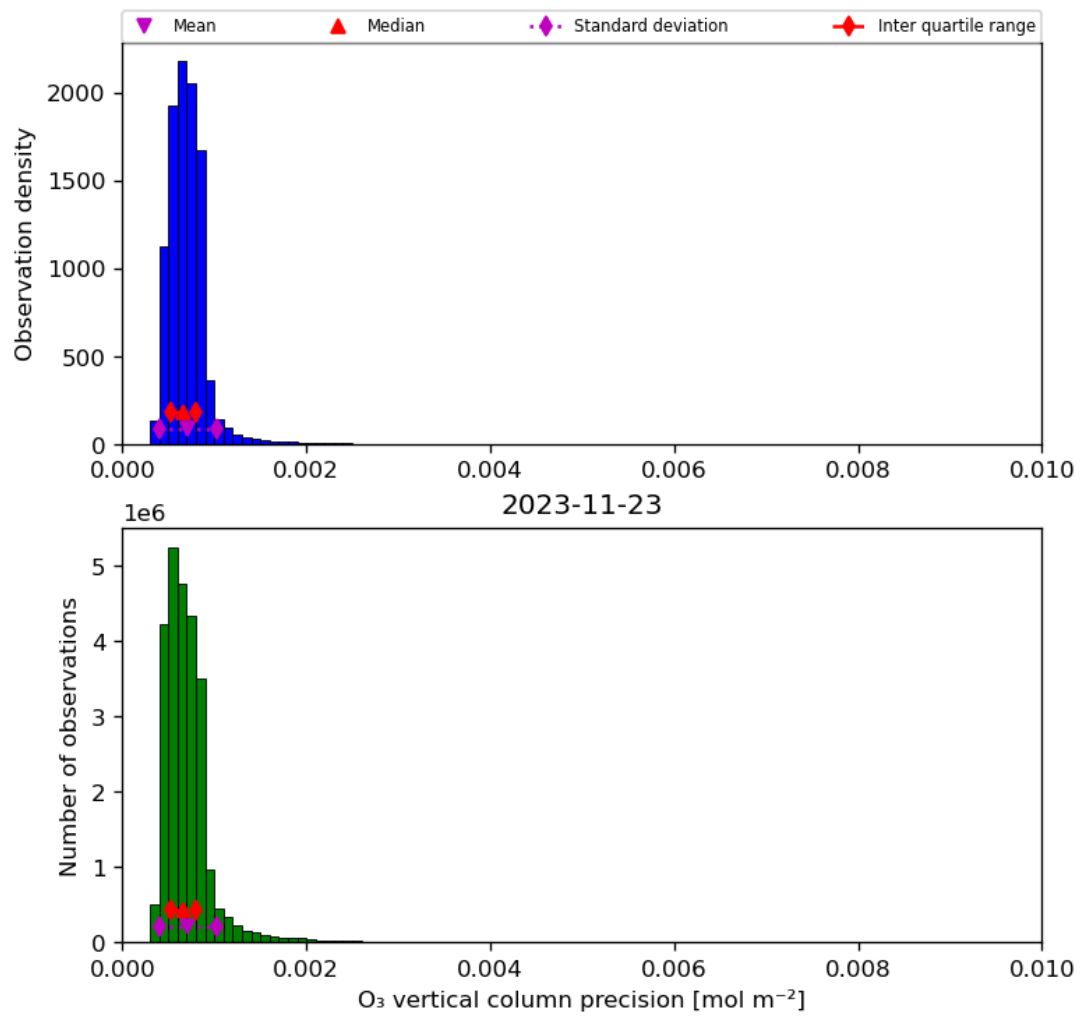
Figure 22: Histogram of “O 3 vertical column precision” for 2023-11-23 to 2023-11-24
