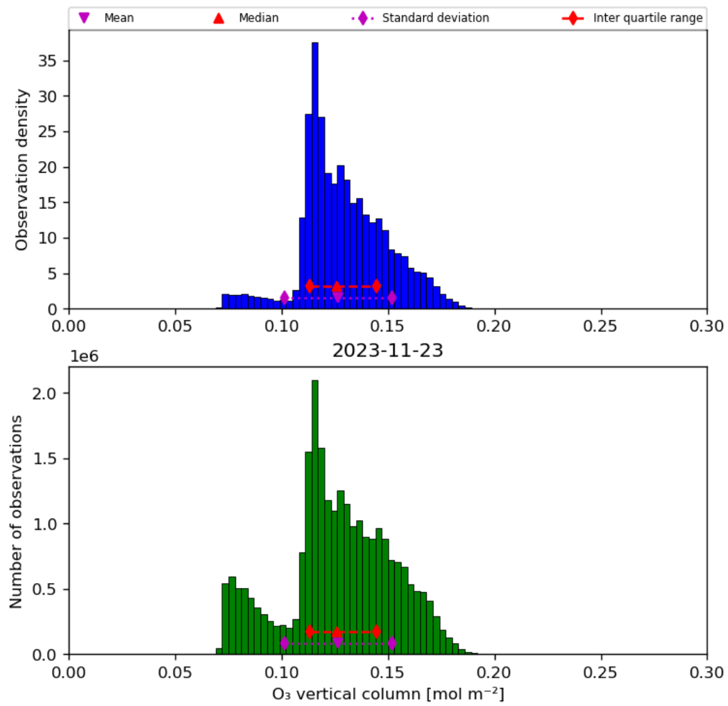
Figure 21: Histogram of “O 3 vertical column” for 2023-11-23 to 2023-11-24
