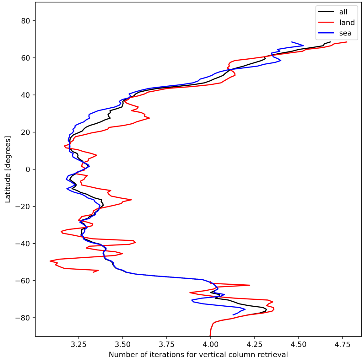
Figure 19: Zonal average of “Number of iterations for vertical column retrieval” for 2023-11-23 to 2023-11-24.
