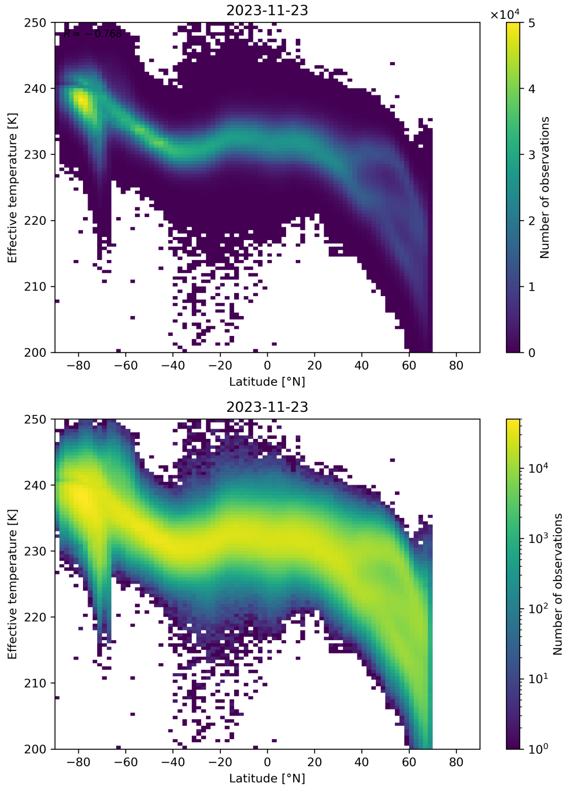
Figure 34: Scatter density plot of “Latitude” against “Effective temperature” for 2023-11-23 to 2023-11-24.
