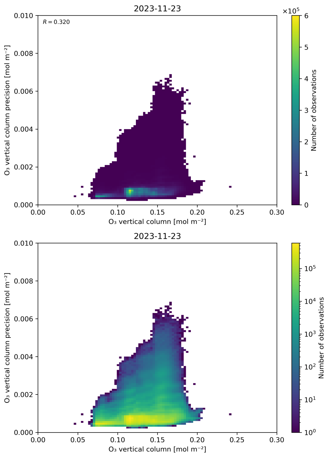
Figure 41: Scatter density plot of “O 3 vertical column” against “O 3 vertical column precision” for 2023-11-23 to 2023-11-24.
