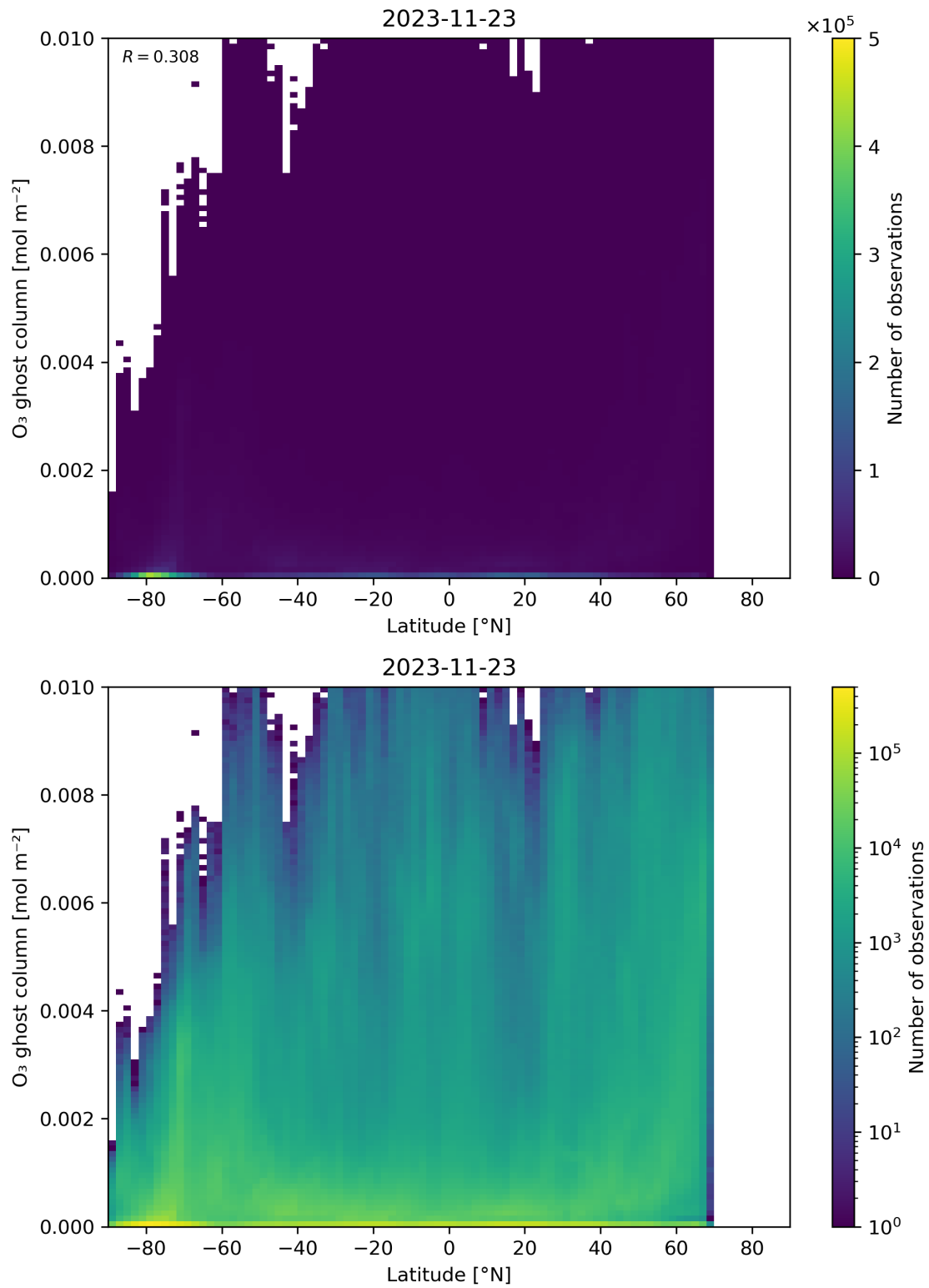
Figure 35: Scatter density plot of “Latitude” against “O 3 ghost column” for 2023-11-23 to 2023-11-24.
