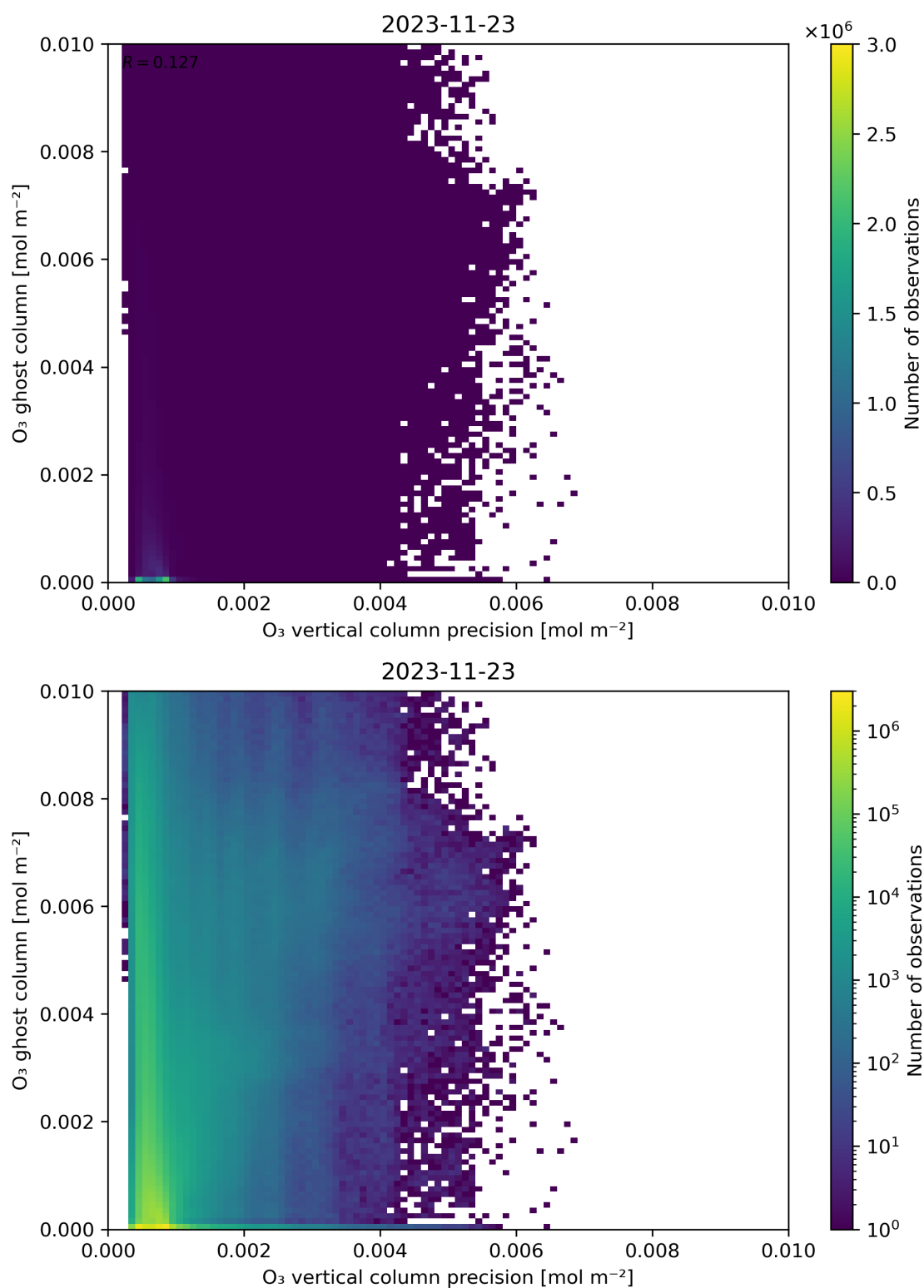
Figure 43: Scatter density plot of “ \text{O}_3 vertical column precision” against “ \text{O}_3 ghost column” for 2023-11-23 to 2023-11-24.
