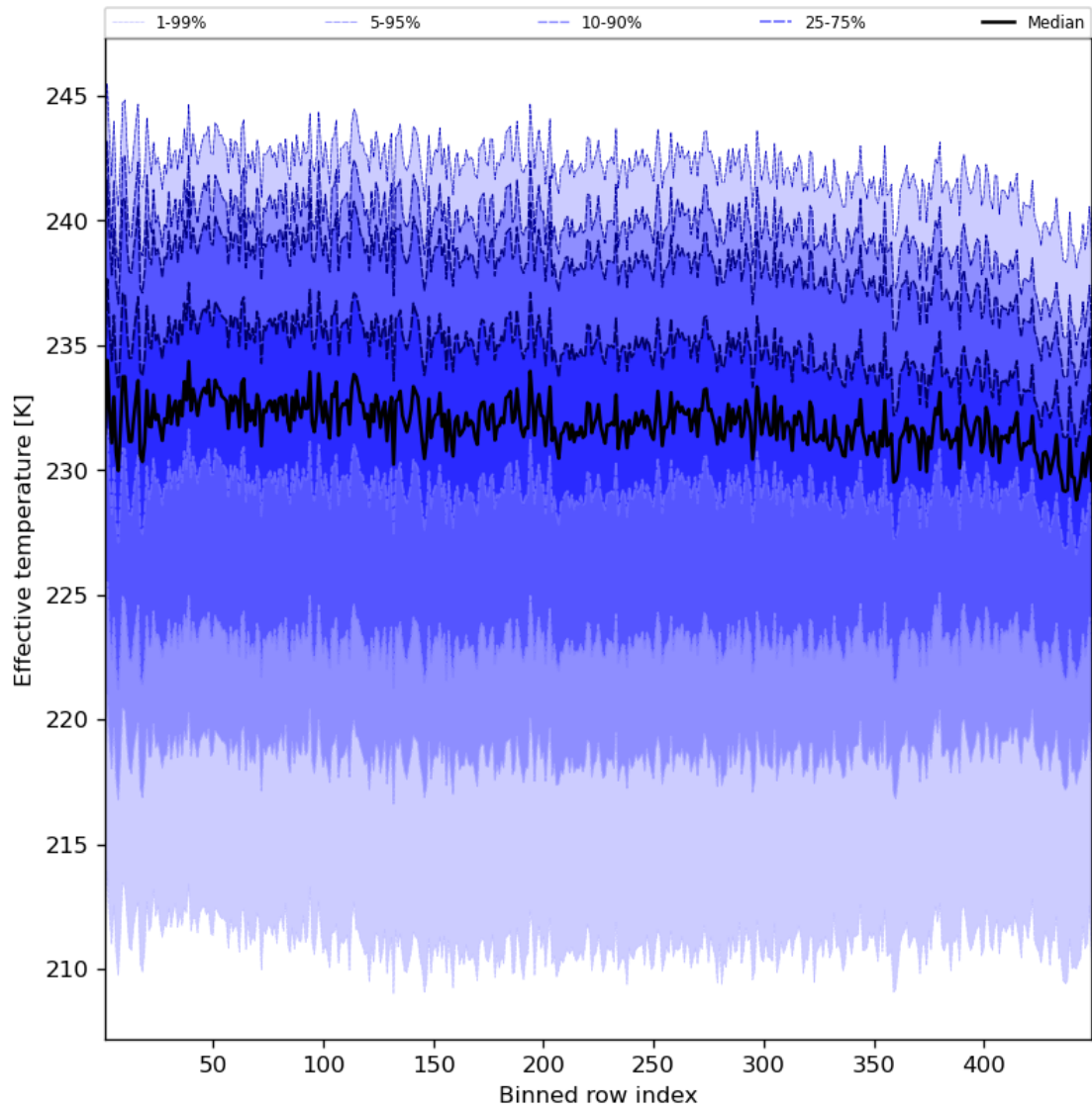
Figure 31: Along track statistics of "Effective temperature" for 2023-11-23 to 2023-11-24
