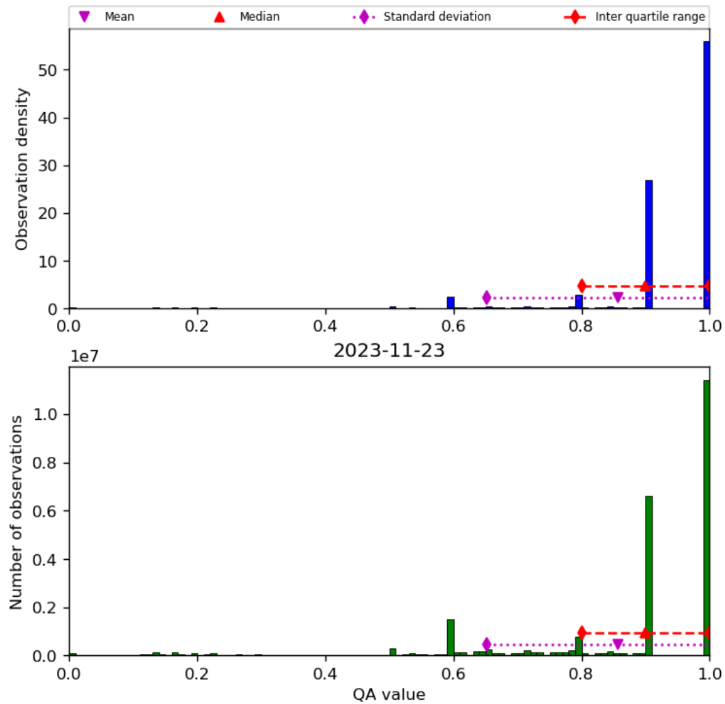
Figure 20: Histogram of “QA value” for 2023-11-23 to 2023-11-24
