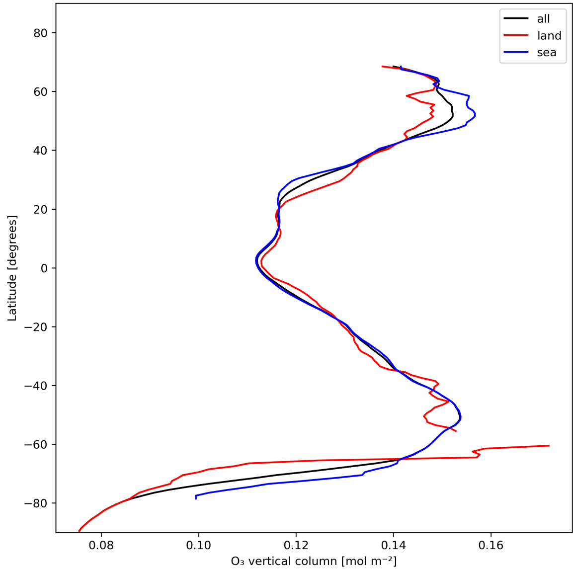
Figure 14: Zonal average of “O 3 vertical column” for 2023-11-23 to 2023-11-24.
