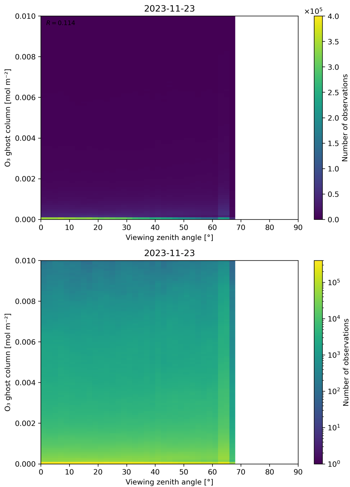
Figure 51: Scatter density plot of “Viewing zenith angle” against “O 3 ghost column” for 2023-11-23 to 2023-11-24.
