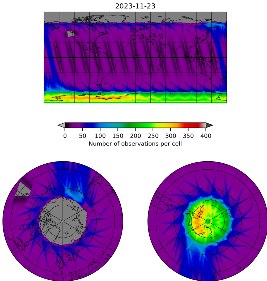
Figure 12: Map of the number of observations for 2023-11-23 to 2023-11-24
