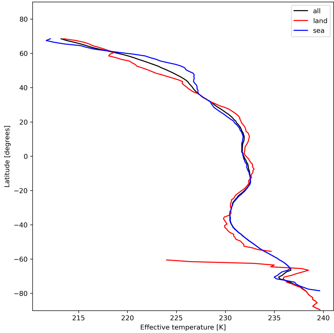
Figure 17: Zonal average of “Effective temperature” for 2023-11-23 to 2023-11-24.
