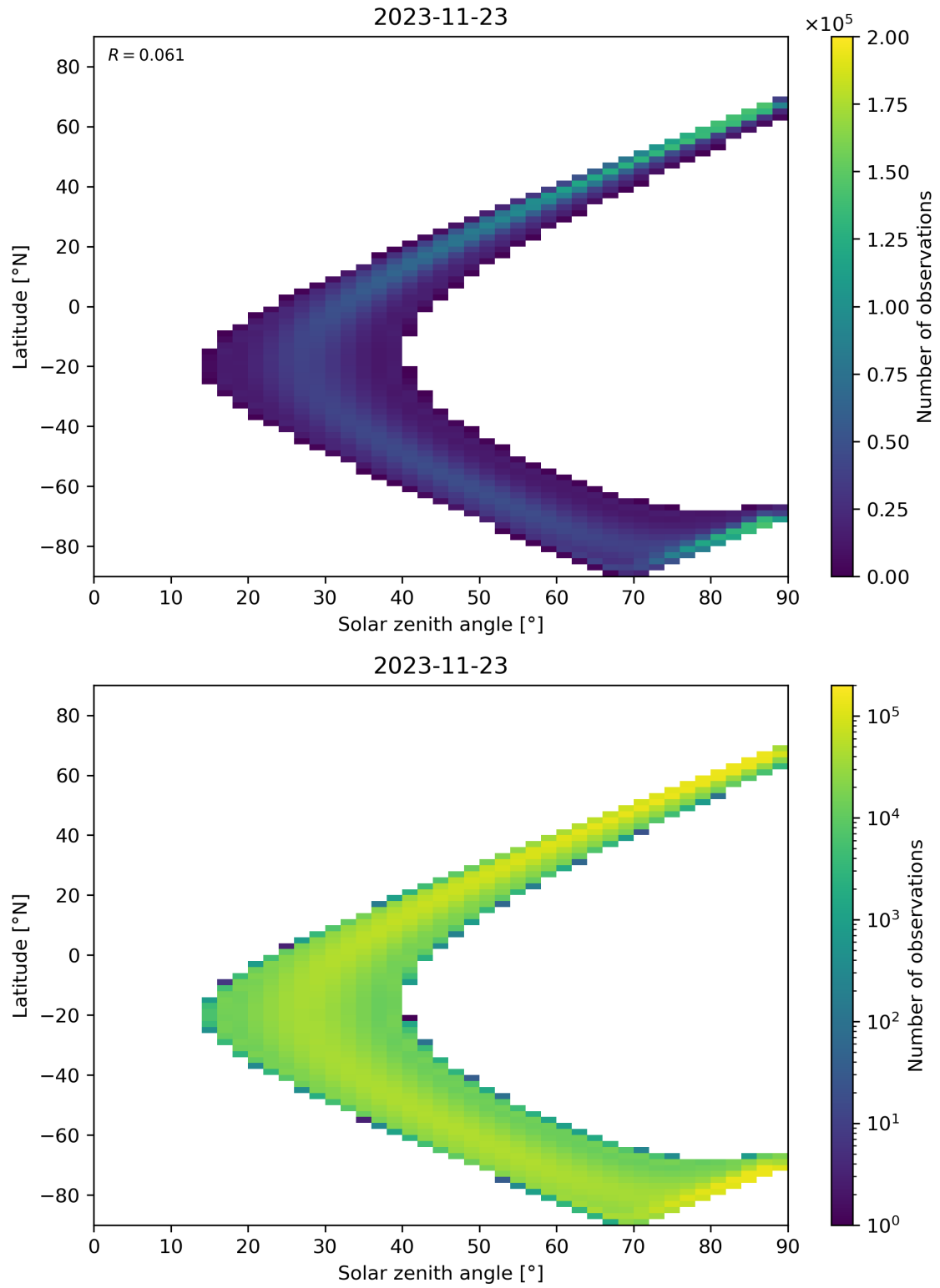
Figure 44: Scatter density plot of “Solar zenith angle” against “Latitude” for 2023-11-23 to 2023-11-24.
