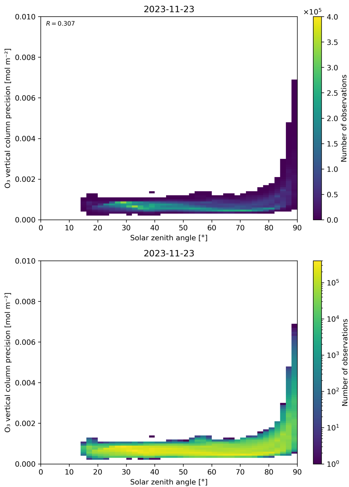
Figure 48: Scatter density plot of “Solar zenith angle” against “O 3 vertical column precision” for 2023-11-23 to 2023-11-24.
