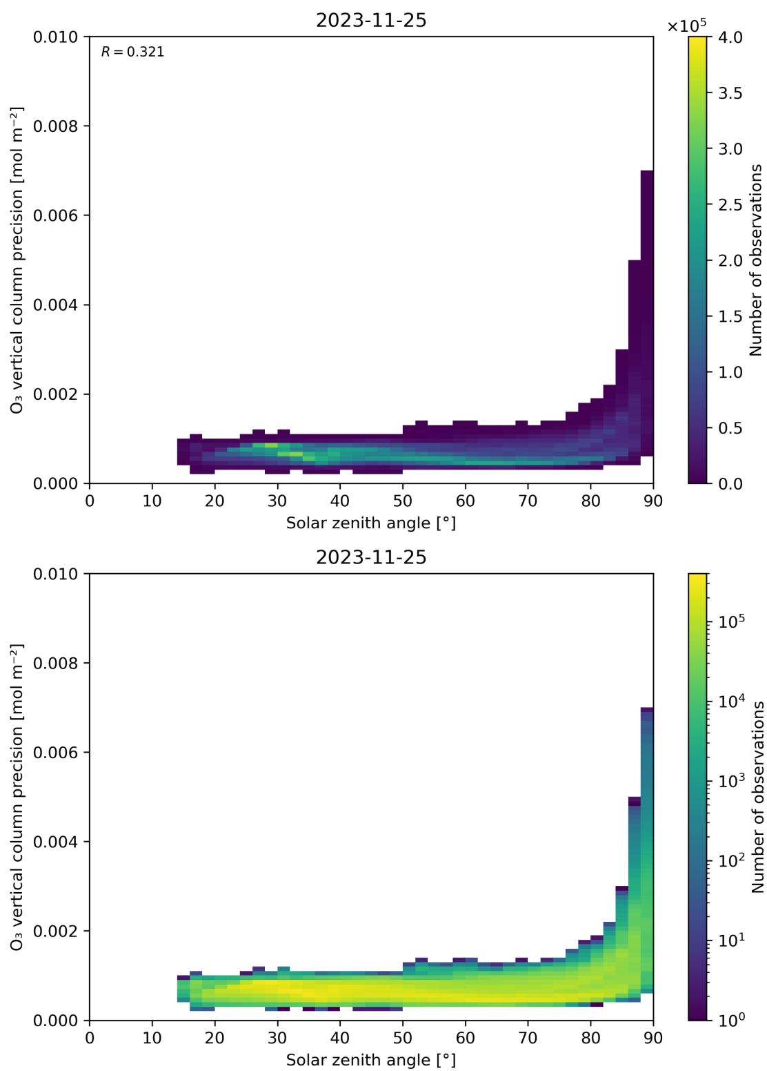
Figure 48: Scatter density plot of “Solar zenith angle” against “O 3 vertical column precision” for 2023-11-24 to 2023-11-26.
