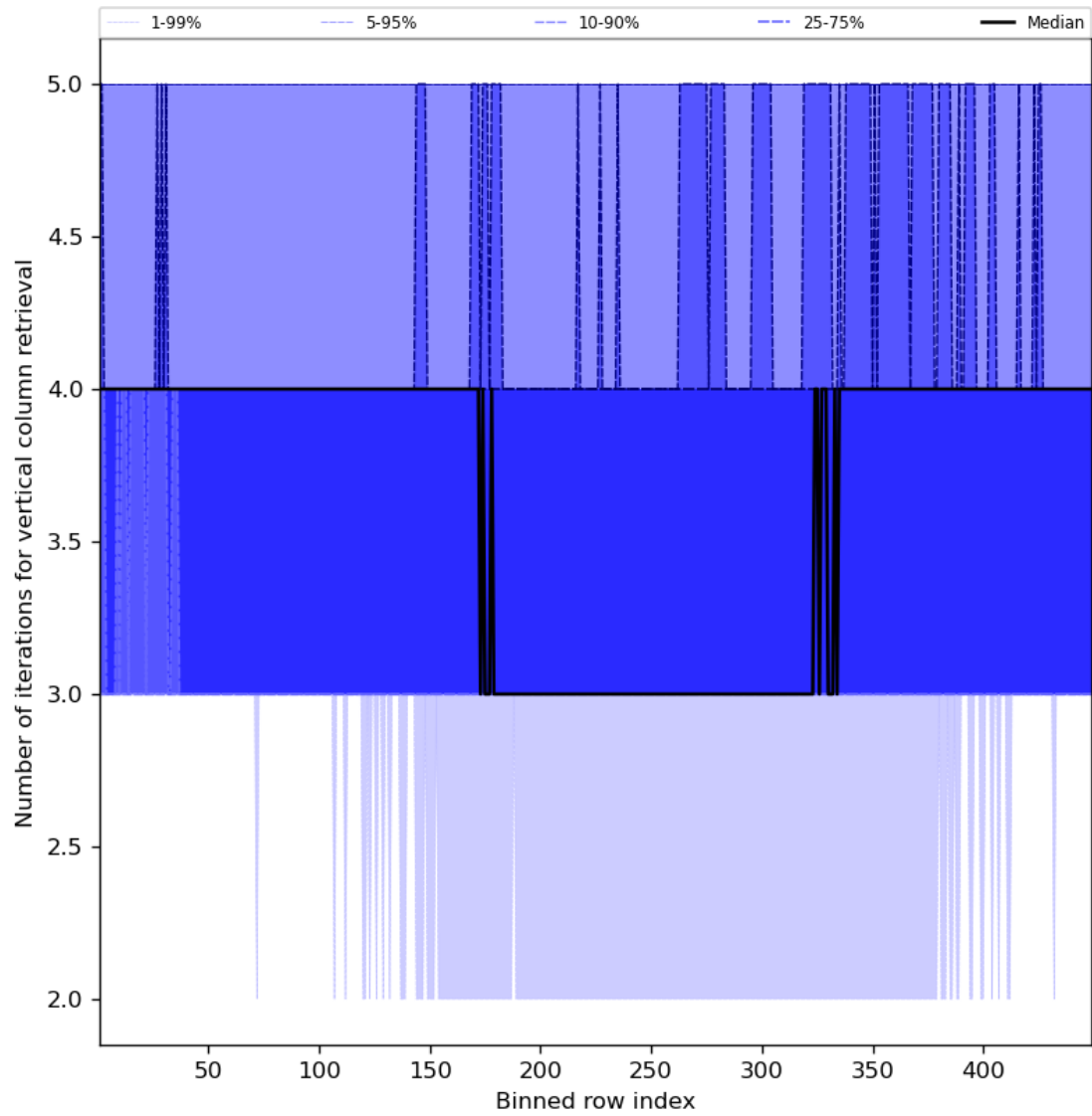
Figure 33: Along track statistics of “Number of iterations for vertical column retrieval” for 2023-11-24 to 2023-11-26
