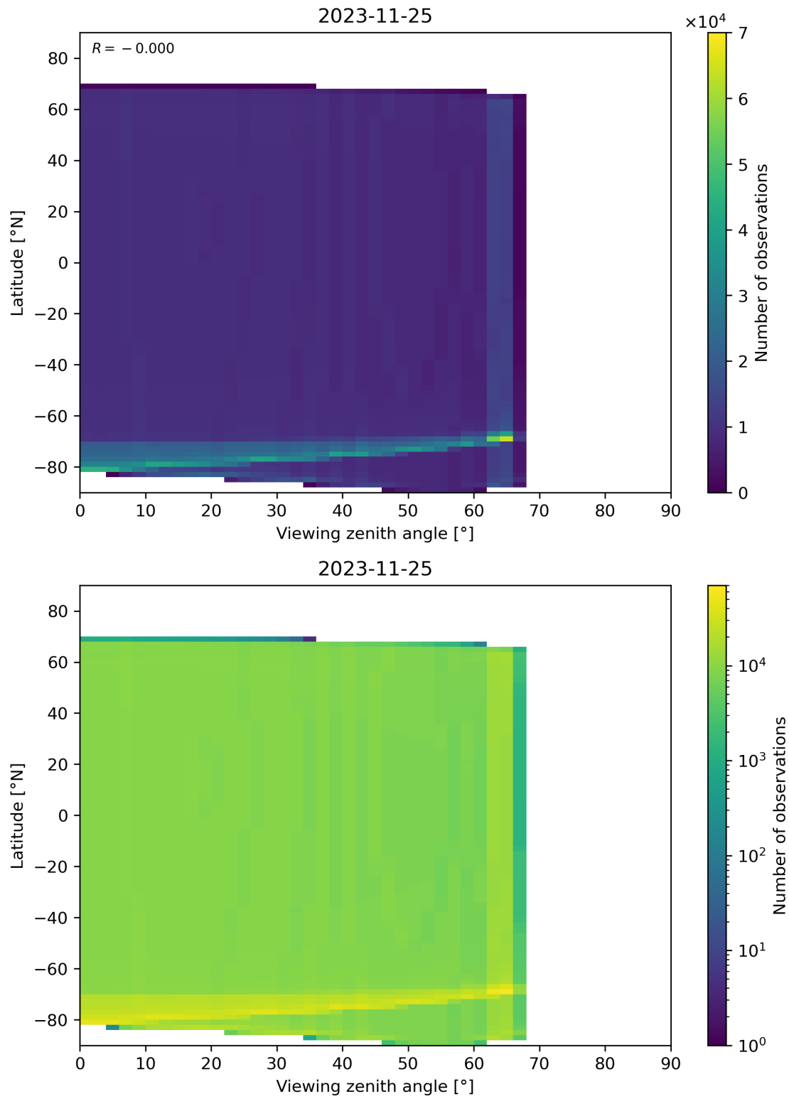
Figure 49: Scatter density plot of “Viewing zenith angle” against “Latitude” for 2023-11-24 to 2023-11-26.
