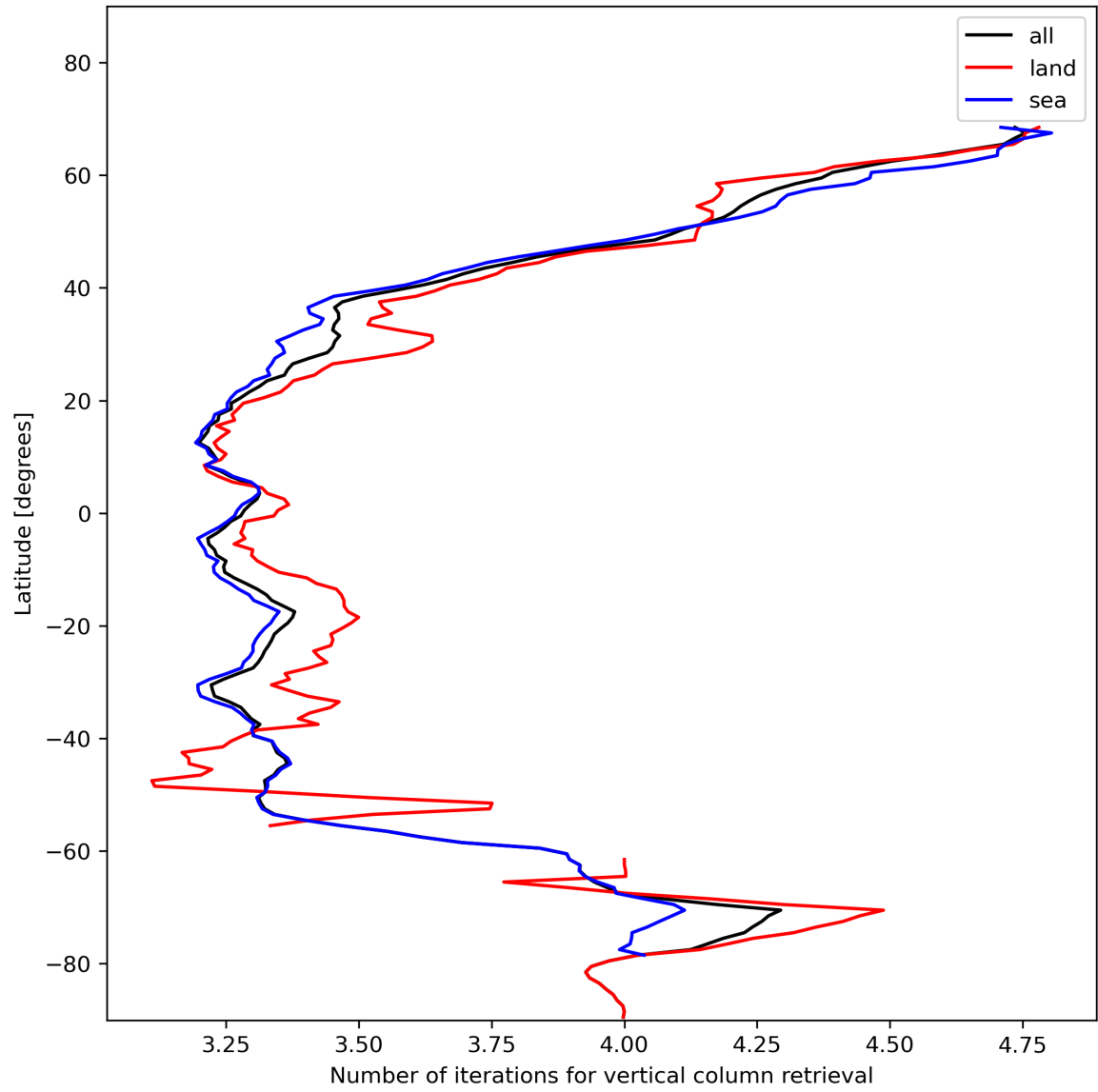
Figure 19: Zonal average of “Number of iterations for vertical column retrieval” for 2023-11-24 to 2023-11-26.
