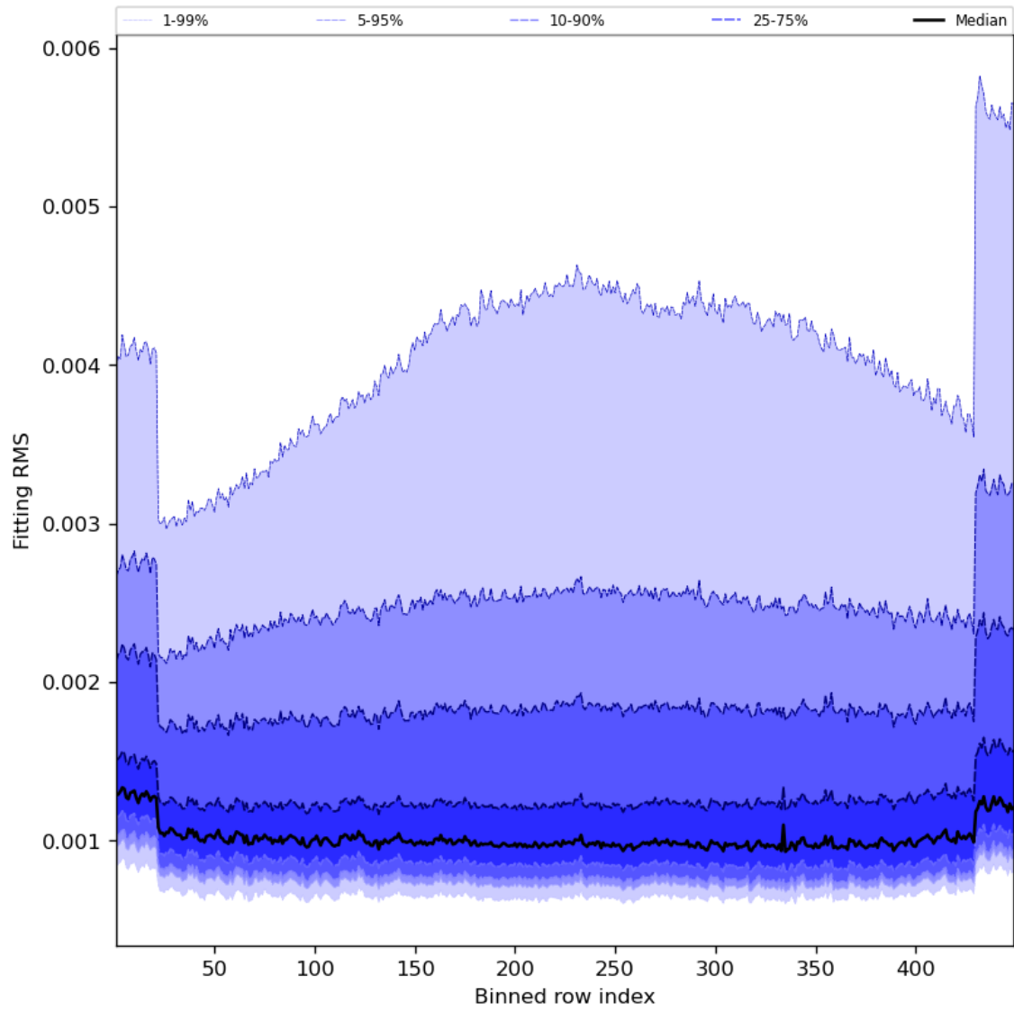
Figure 30: Along track statistics of “Fitting RMS” for 2023-11-24 to 2023-11-26
