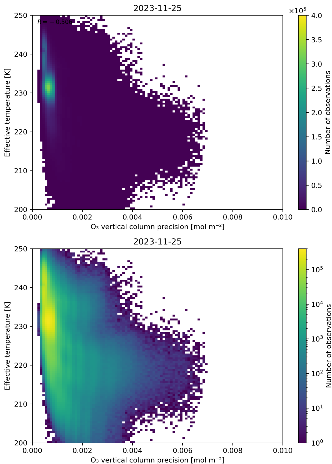
Figure 42: Scatter density plot of “O 3 vertical column precision” against “Effective temperature” for 2023-11-24 to 2023-11-26.
