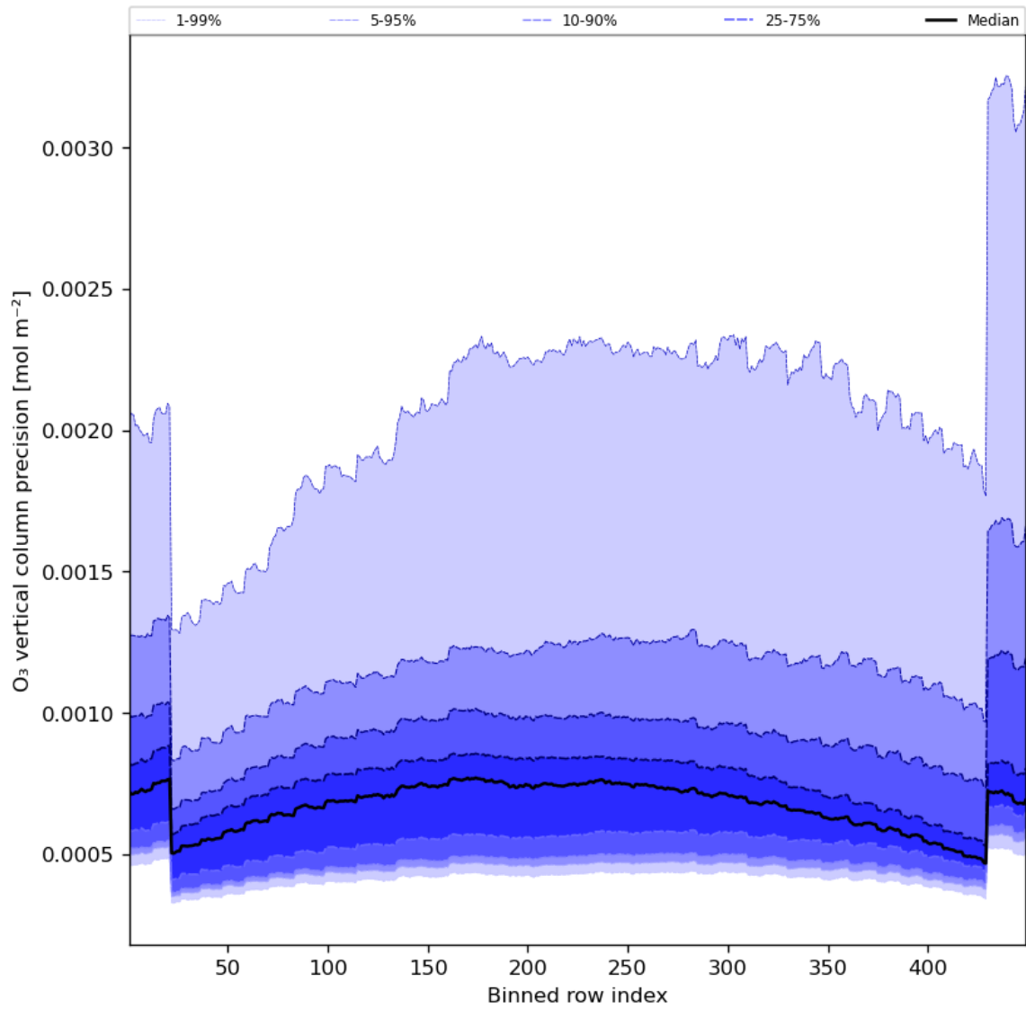
Figure 29: Along track statistics of “O 3 vertical column precision” for 2023-11-24 to 2023-11-26
