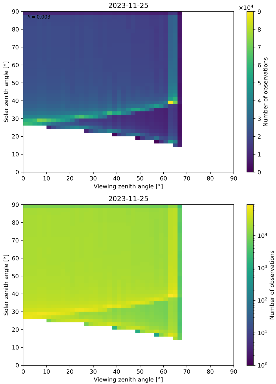
Figure 54: Scatter density plot of “Viewing zenith angle” against “Solar zenith angle” for 2023-11-24 to 2023-11-26.
