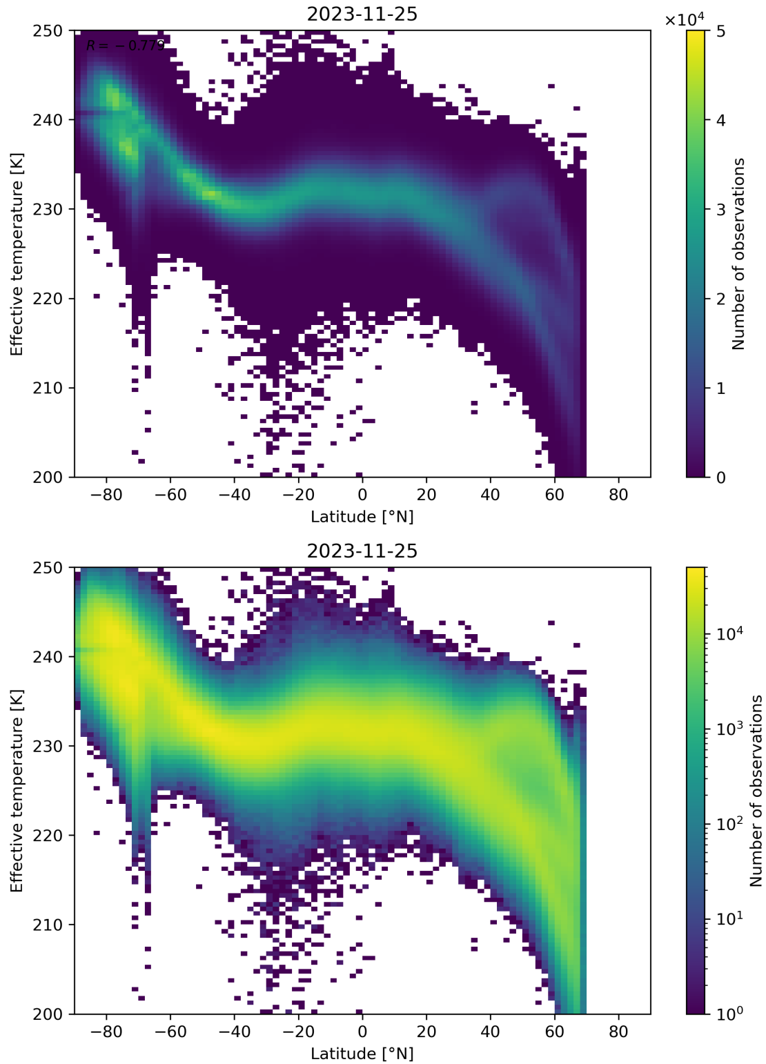
Figure 34: Scatter density plot of “Latitude” against “Effective temperature” for 2023-11-24 to 2023-11-26.
