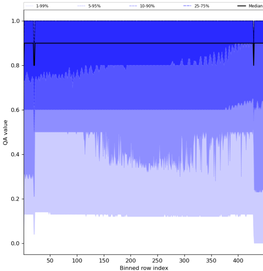
Figure 27: Along track statistics of “QA value” for 2023-11-24 to 2023-11-26
