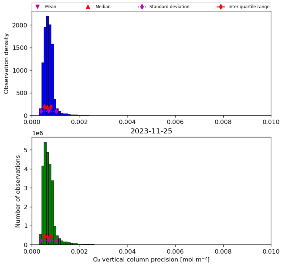
Figure 22: Histogram of “O 3 vertical column precision” for 2023-11-24 to 2023-11-26
