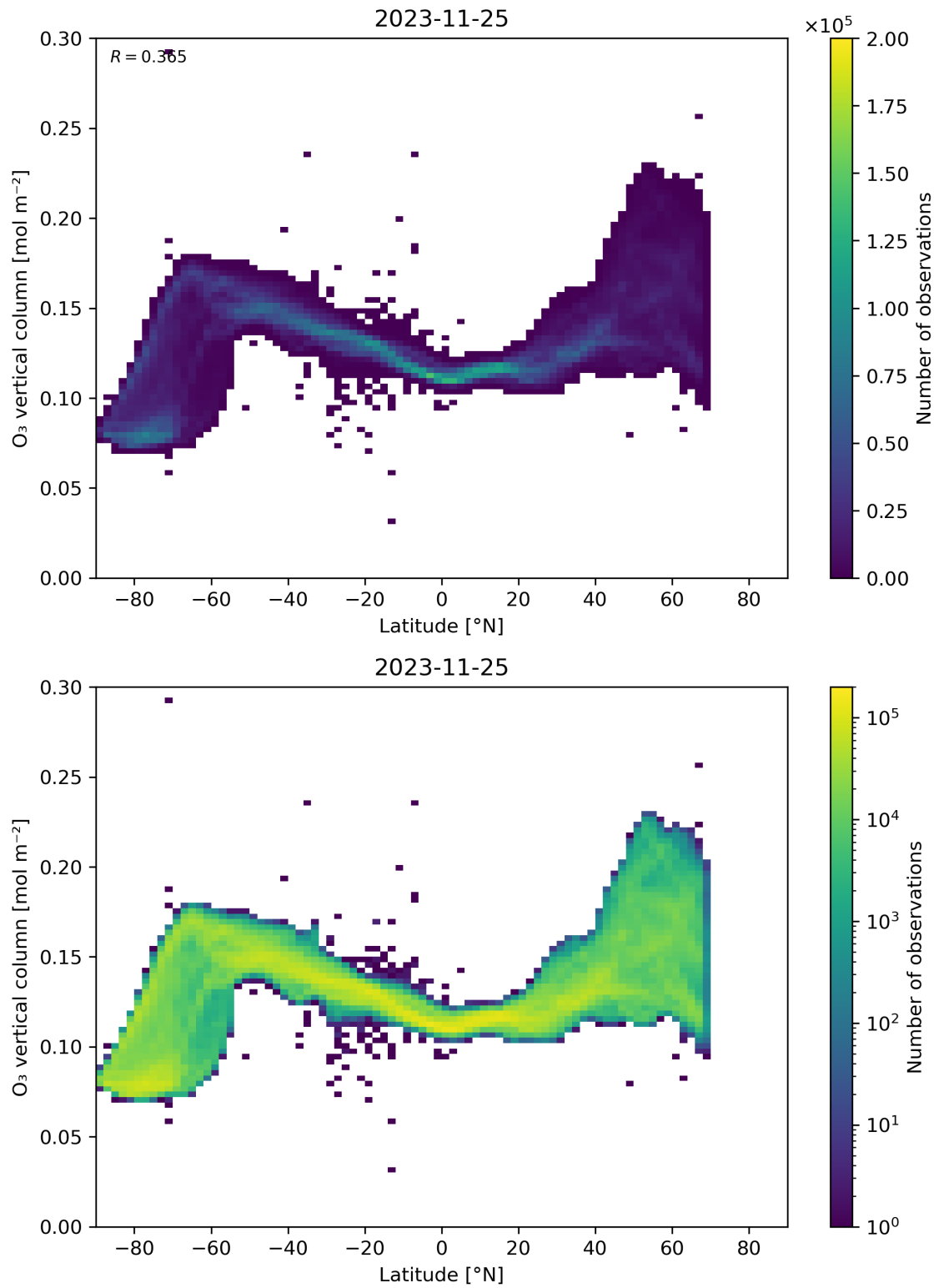
Figure 36: Scatter density plot of “Latitude” against “O 3 vertical column” for 2023-11-24 to 2023-11-26.
