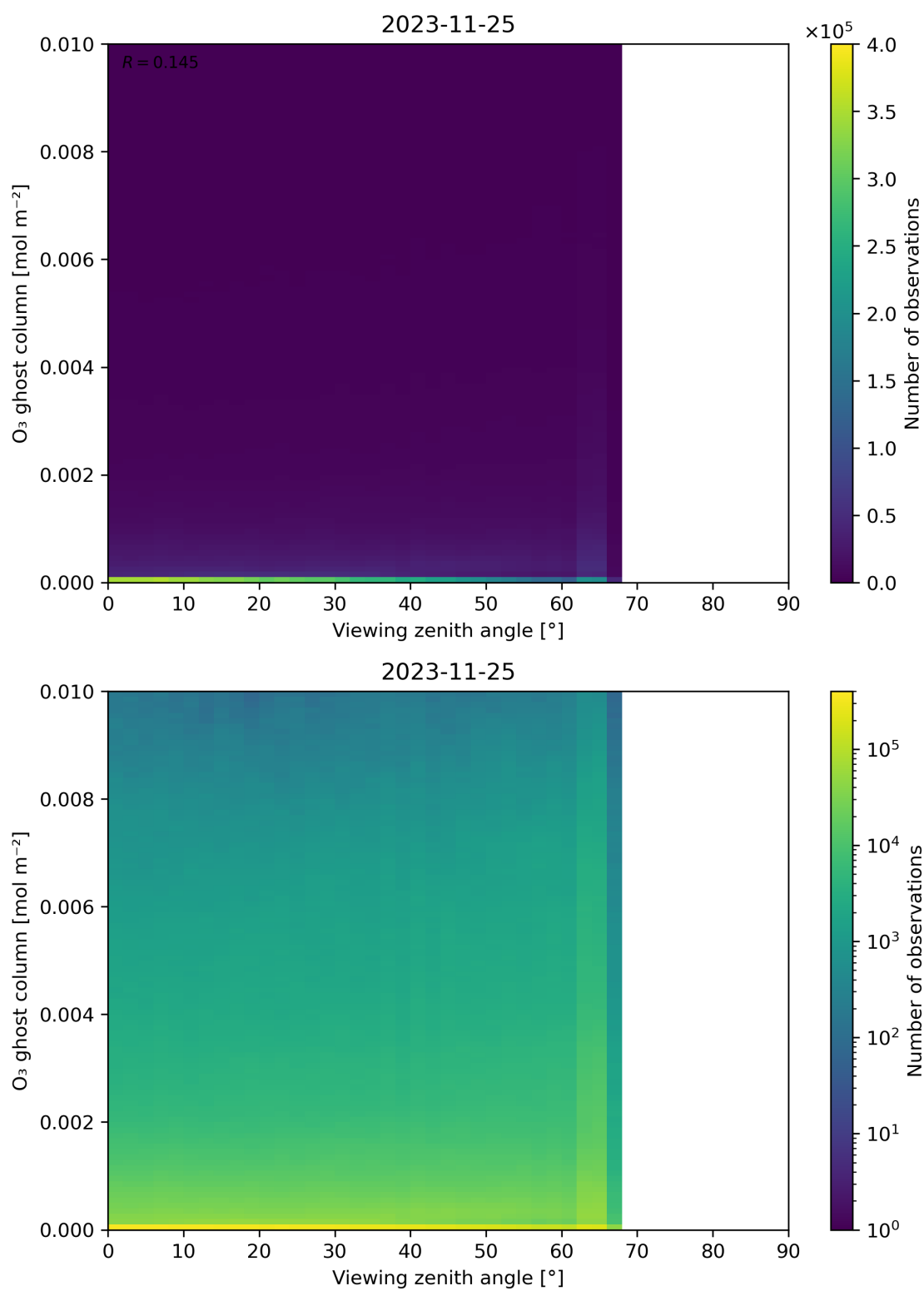
Figure 51: Scatter density plot of “Viewing zenith angle” against “O 3 ghost column” for 2023-11-24 to 2023-11-26.
