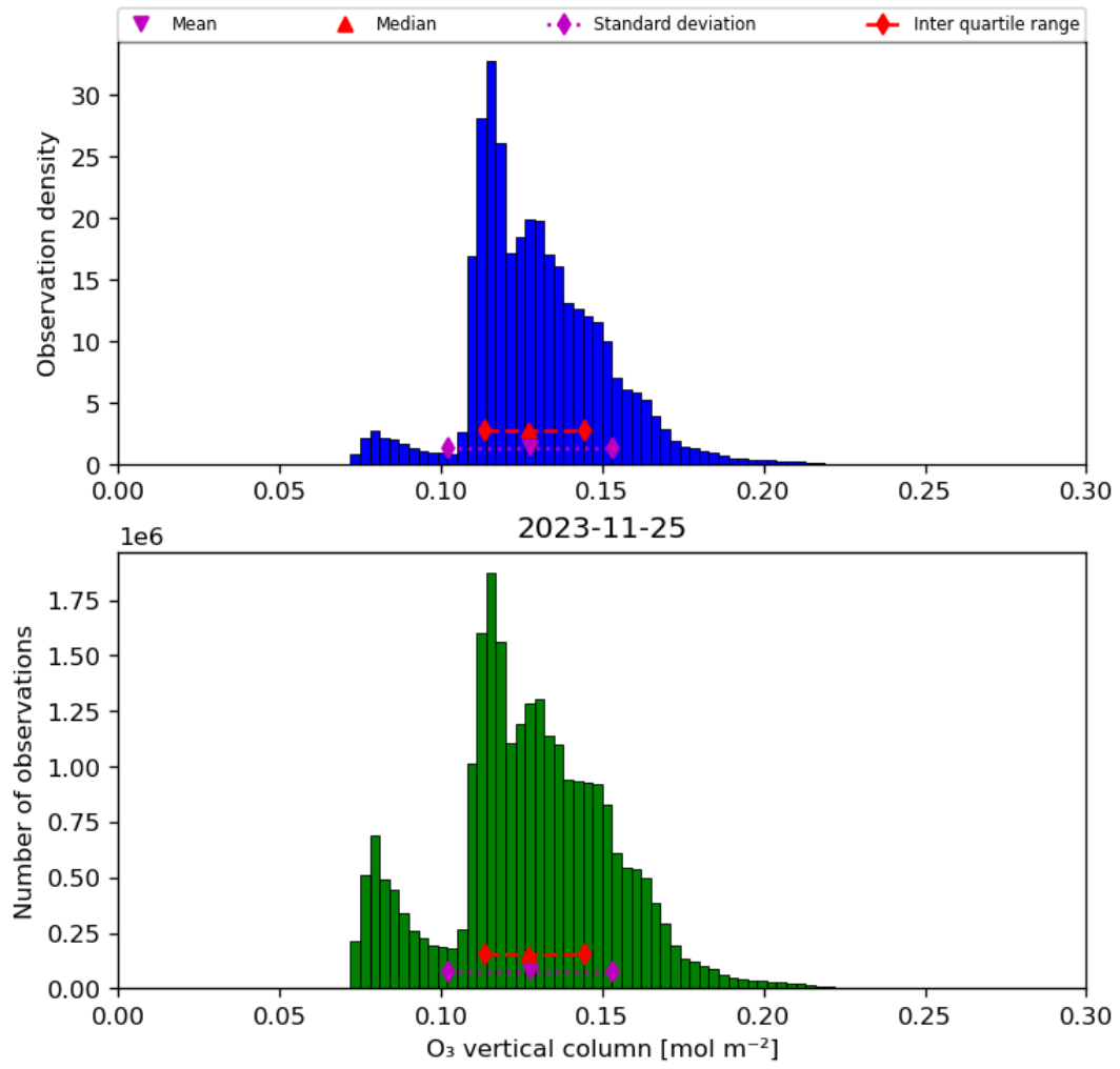
Figure 21: Histogram of “O 3 vertical column” for 2023-11-24 to 2023-11-26
