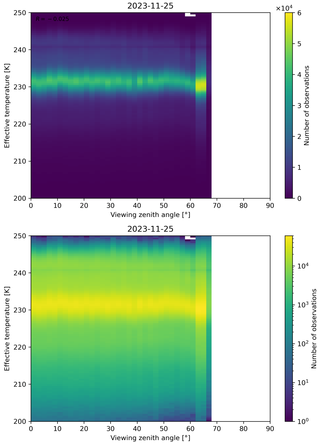
Figure 50: Scatter density plot of “Viewing zenith angle” against “Effective temperature” for 2023-11-24 to 2023-11-26.
