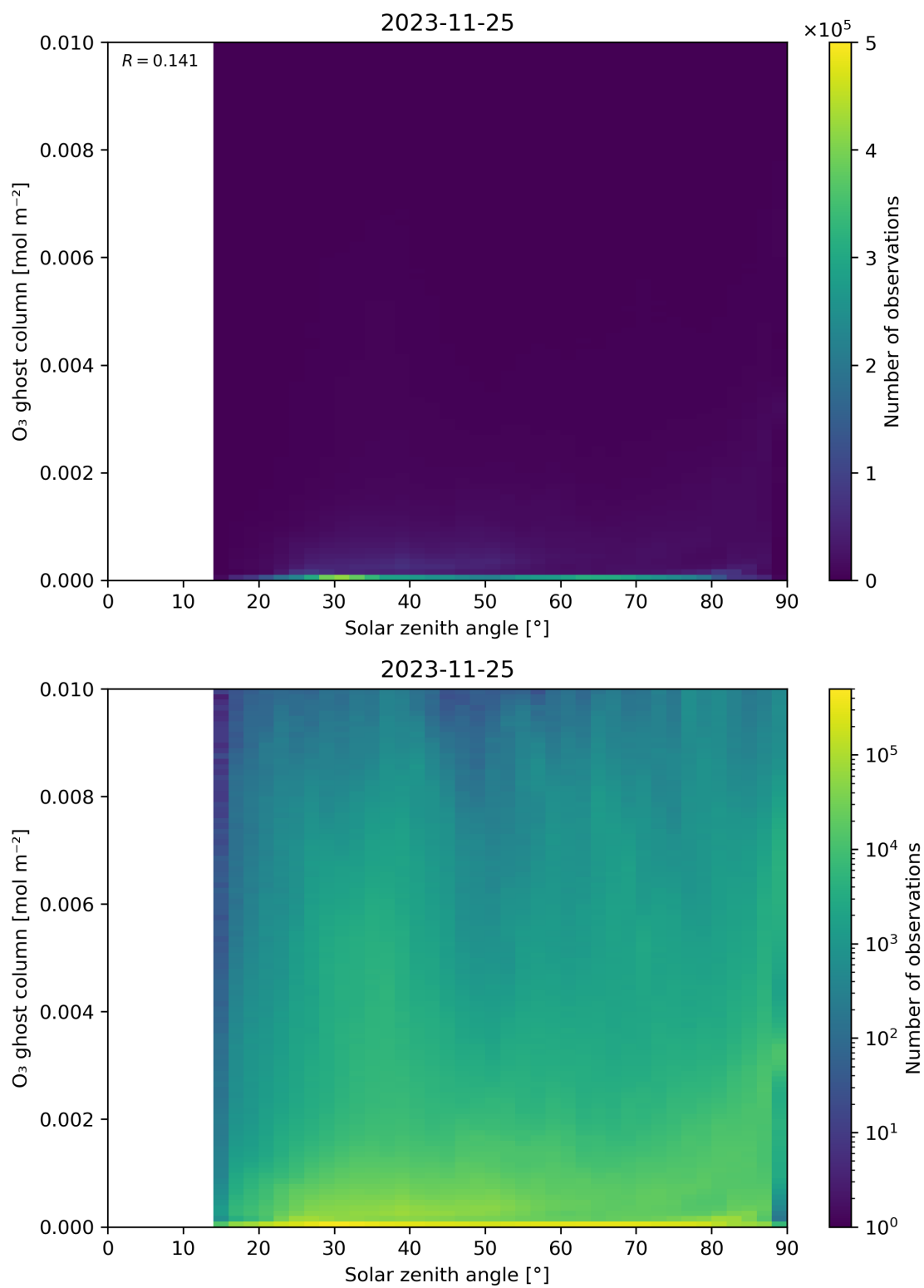
Figure 46: Scatter density plot of “Solar zenith angle” against “O 3 ghost column” for 2023-11-24 to 2023-11-26.
