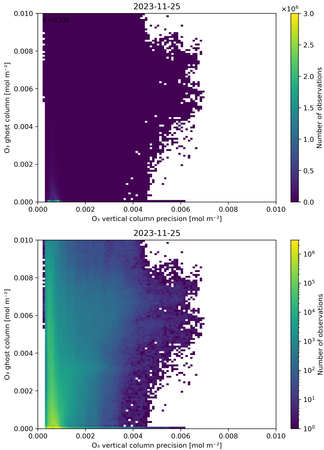
Figure 43: Scatter density plot of “O 3 vertical column precision” against “O 3 ghost column” for 2023-11-24 to 2023-11-26.
