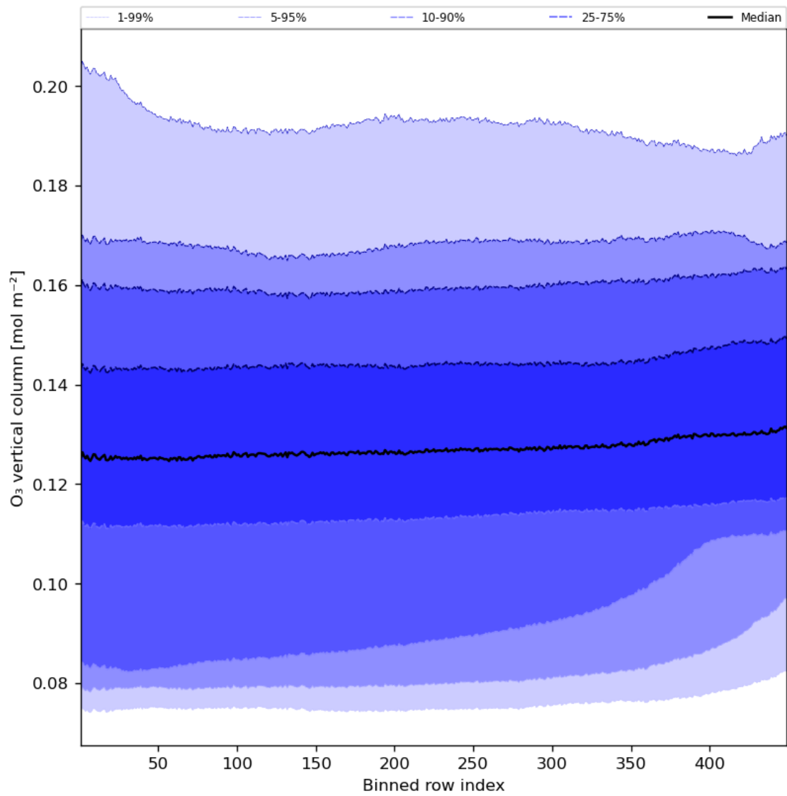
Figure 28: Along track statistics of “O 3 vertical column” for 2023-11-24 to 2023-11-26
