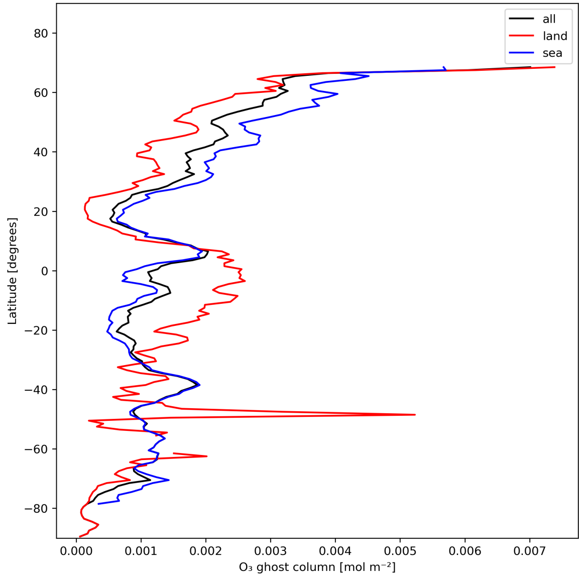
Figure 18: Zonal average of "O 3 ghost column" for 2023-11-24 to 2023-11-26.
