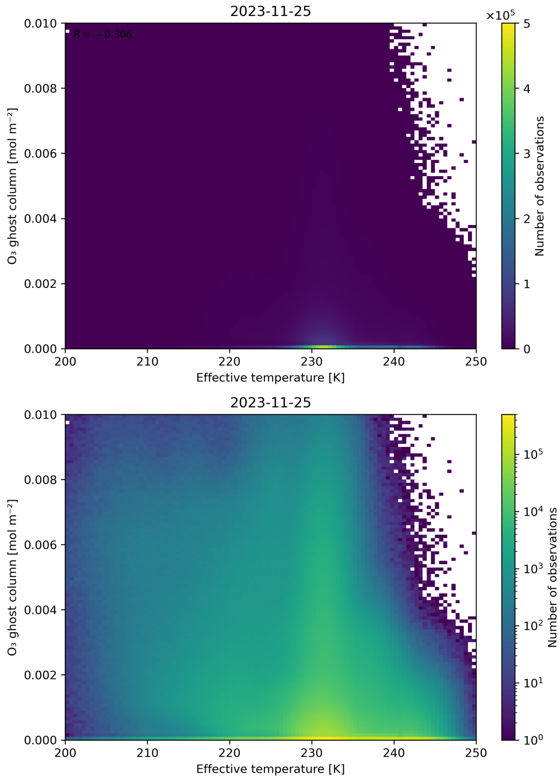
Figure 38: Scatter density plot of “Effective temperature” against “O 3 ghost column” for 2023-11-24 to 2023-11-26.
