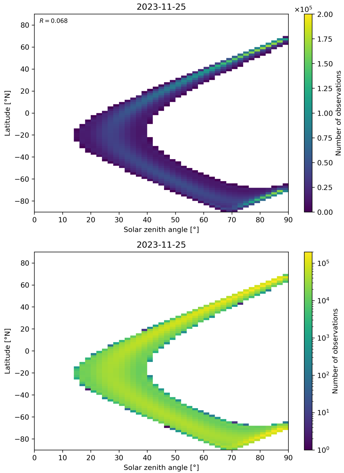
Figure 44: Scatter density plot of “Solar zenith angle” against “Latitude” for 2023-11-24 to 2023-11-26.
