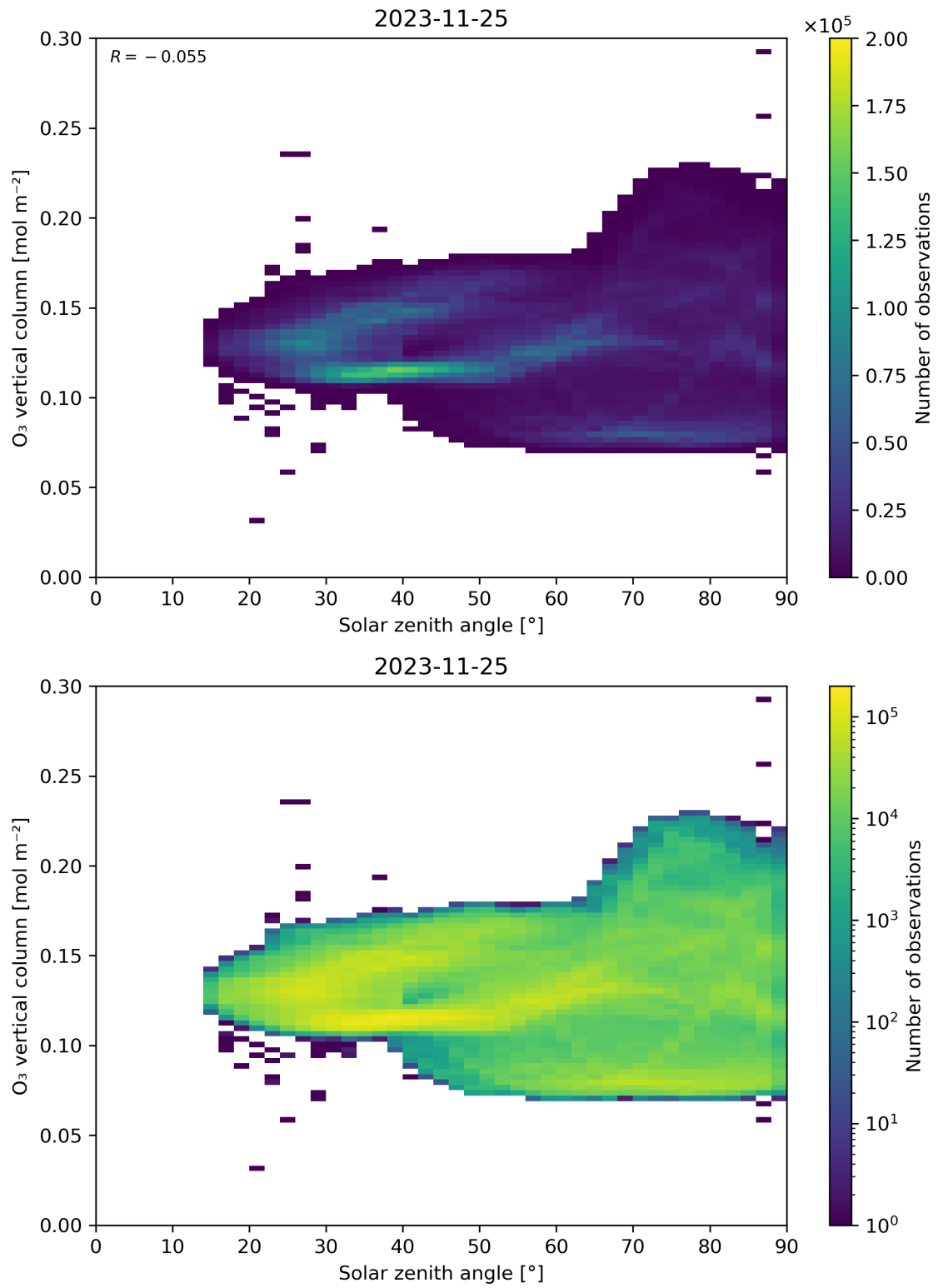
Figure 47: Scatter density plot of “Solar zenith angle” against “O 3 vertical column” for 2023-11-24 to 2023-11-26.
