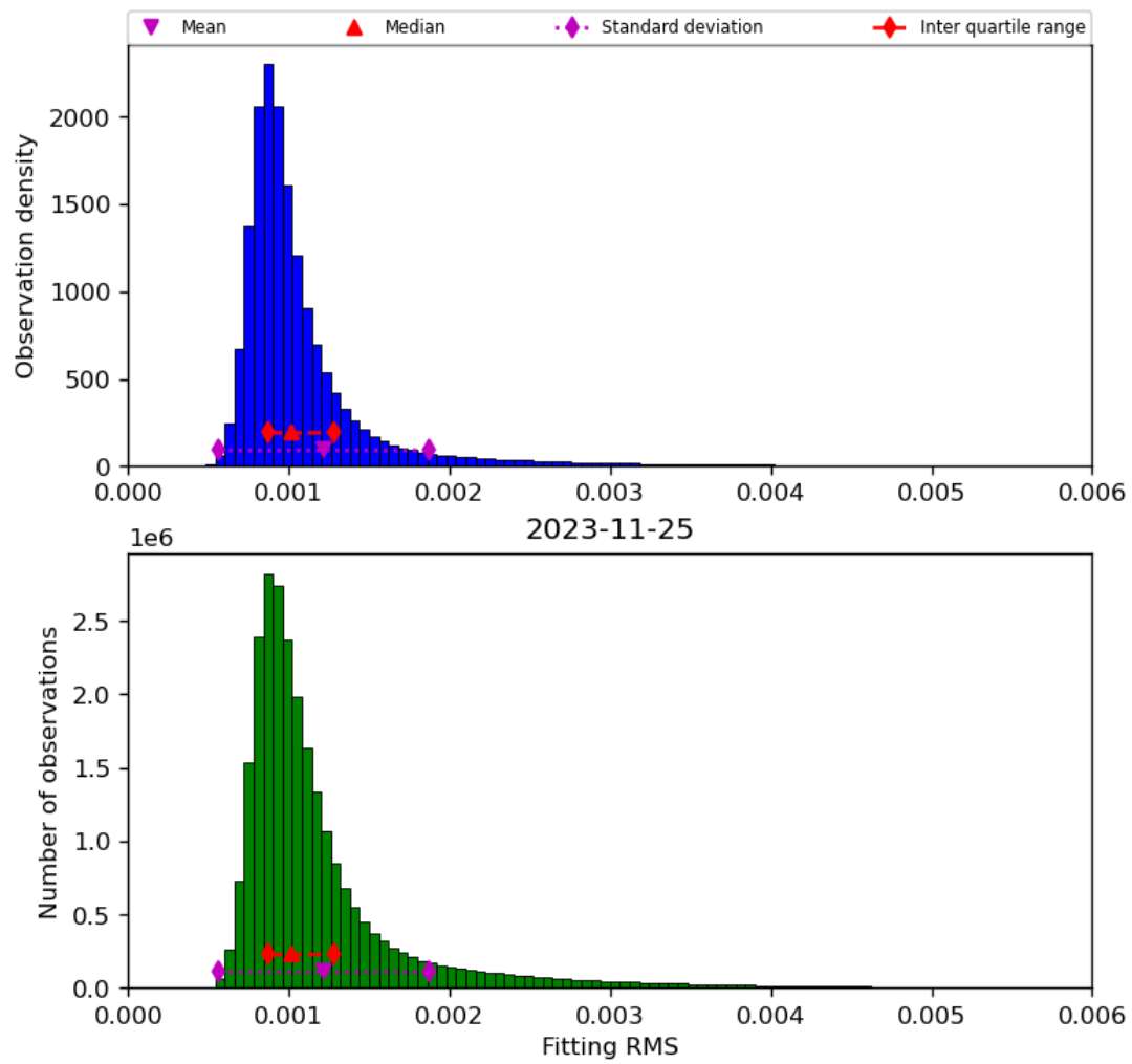
Figure 23: Histogram of “Fitting RMS” for 2023-11-24 to 2023-11-26
