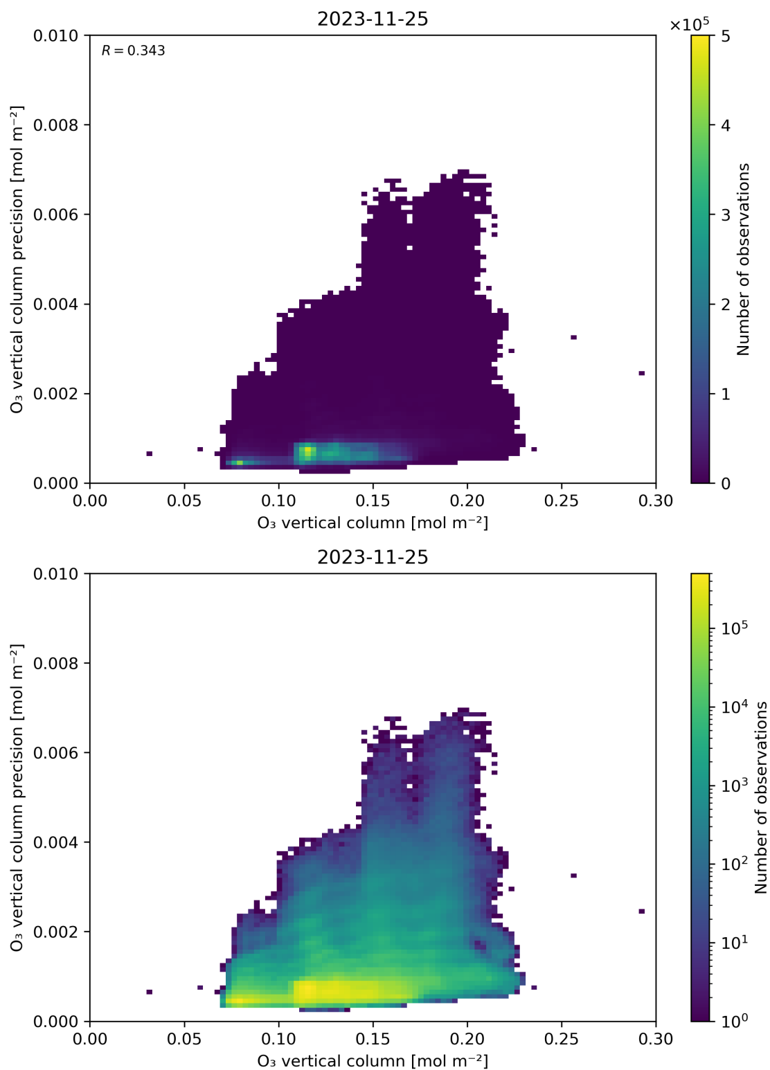
Figure 41: Scatter density plot of “O 3 vertical column” against “O 3 vertical column precision” for 2023-11-24 to 2023-11-26.
