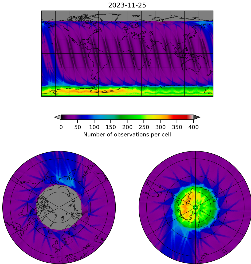
Figure 12: Map of the number of observations for 2023-11-24 to 2023-11-26
