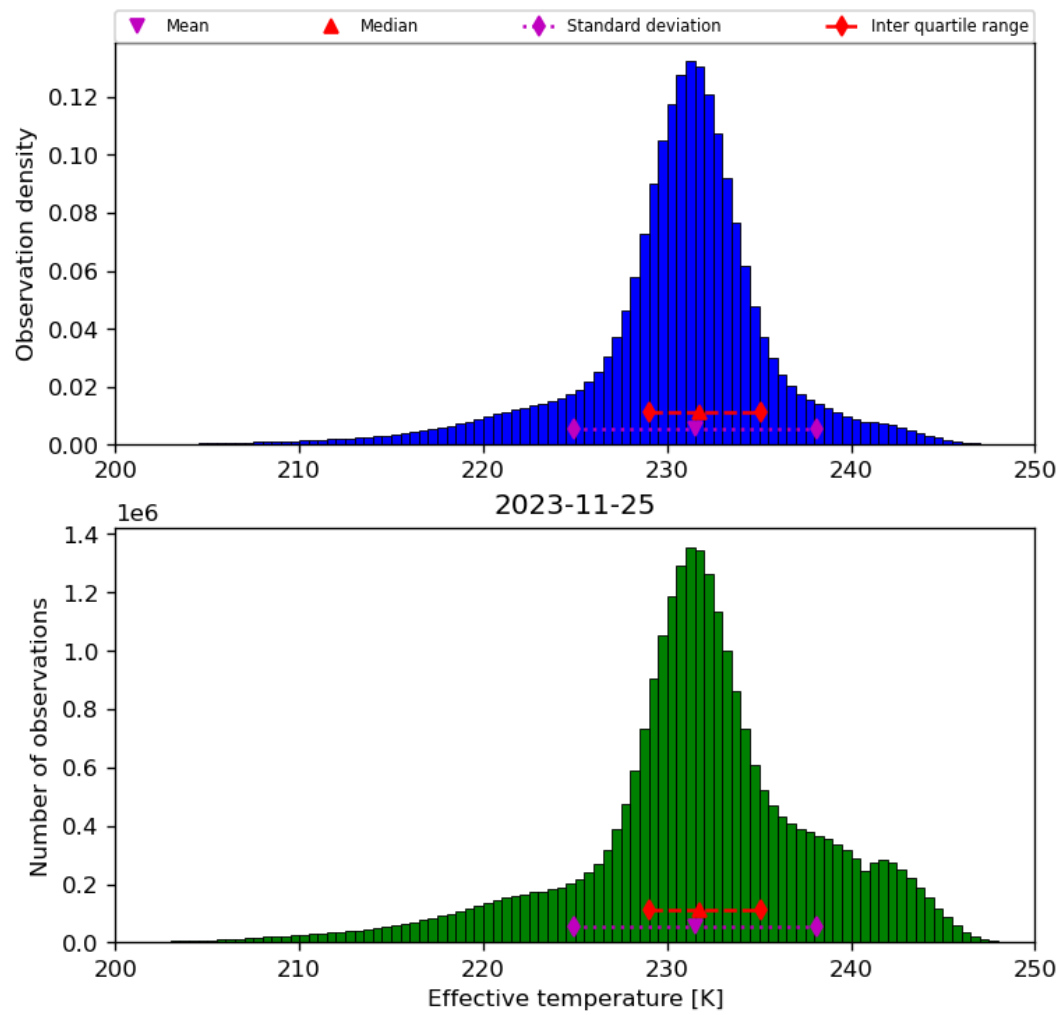
Figure 24: Histogram of “Effective temperature” for 2023-11-24 to 2023-11-26
