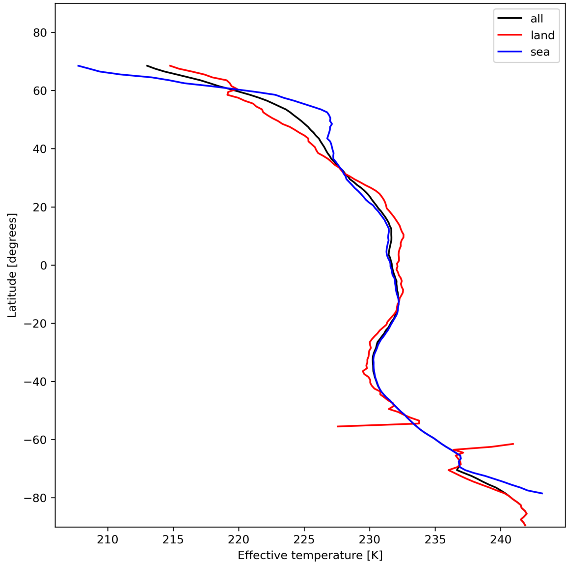
Figure 17: Zonal average of “Effective temperature” for 2023-11-24 to 2023-11-26.
