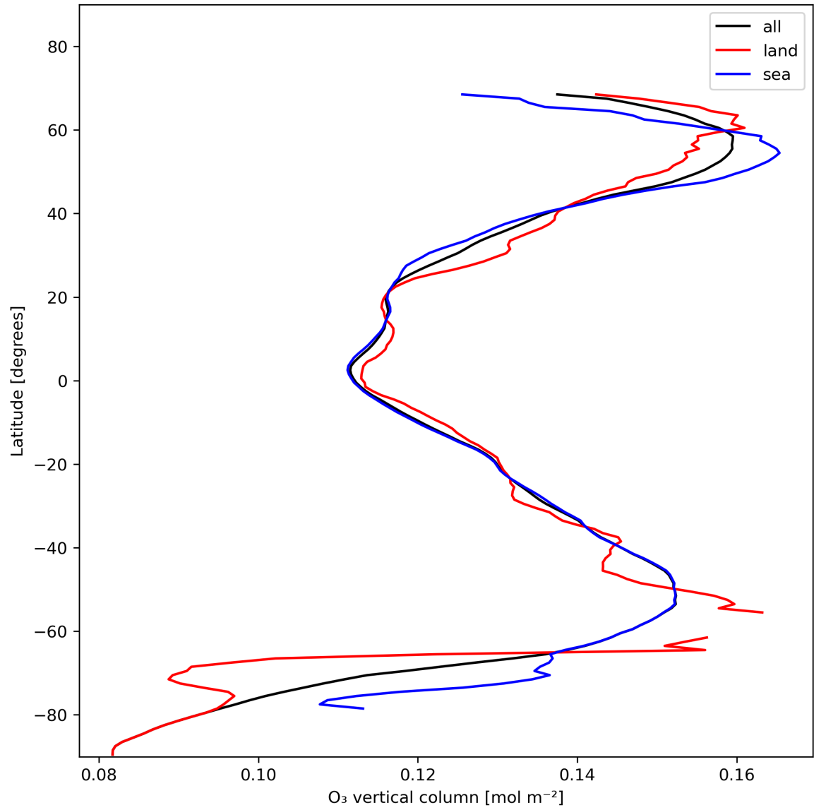
Figure 14: Zonal average of “O 3 vertical column” for 2023-11-24 to 2023-11-26.
