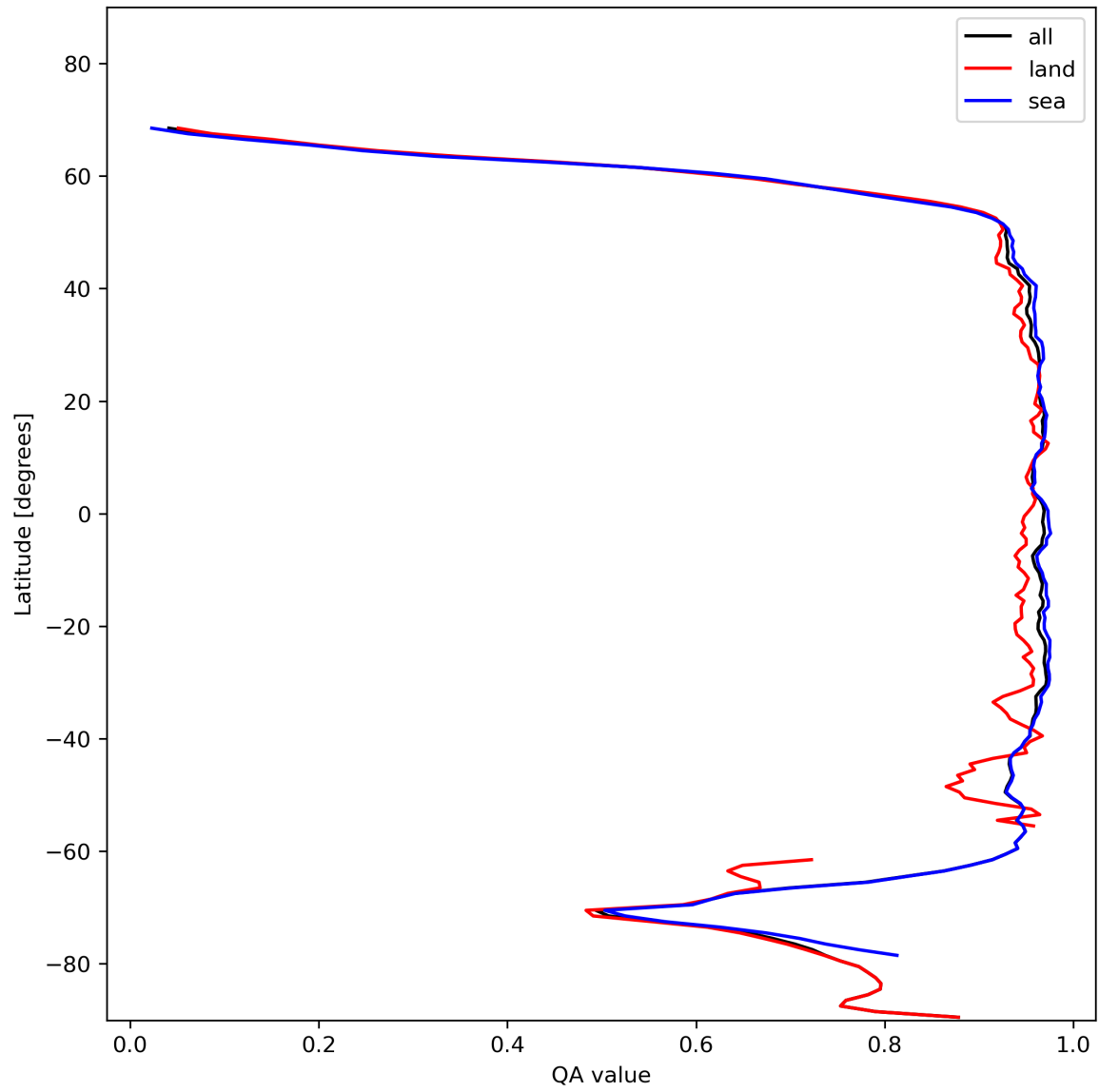
Figure 13: Zonal average of “QA value” for 2023-11-24 to 2023-11-26.
