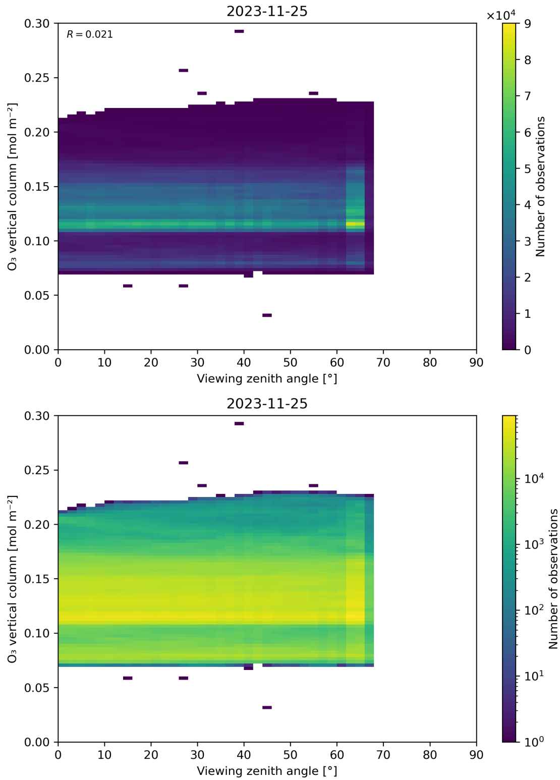
Figure 52: Scatter density plot of “Viewing zenith angle” against “O 3 vertical column” for 2023-11-24 to 2023-11-26.
