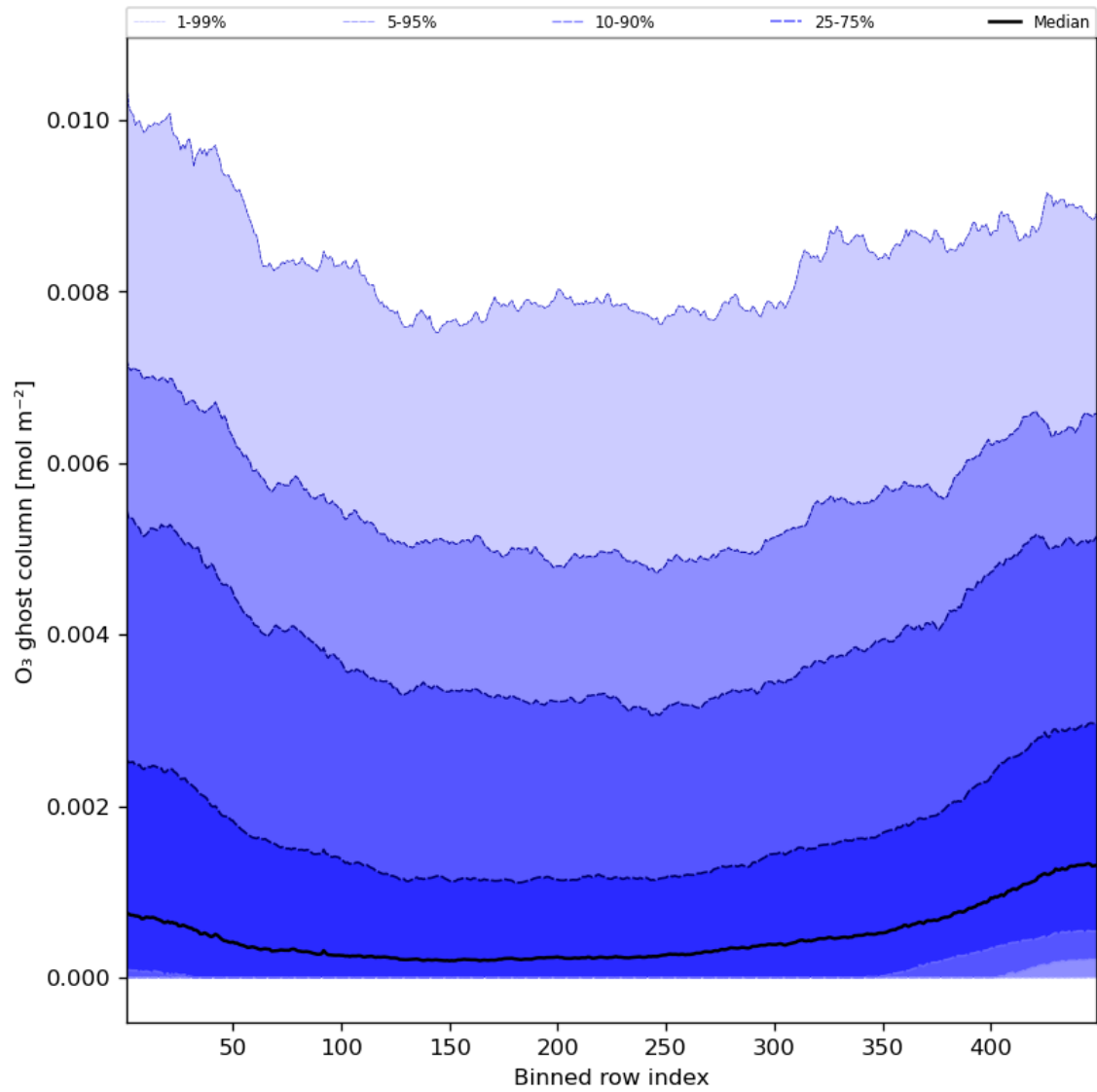
Figure 32: Along track statistics of “O 3 ghost column” for 2023-11-24 to 2023-11-26
