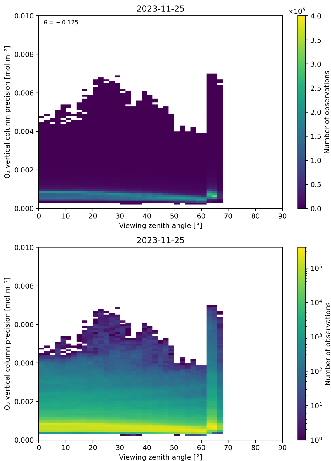
Figure 53: Scatter density plot of “Viewing zenith angle” against “O 3 vertical column precision” for 2023-11-24 to 2023-11-26.
