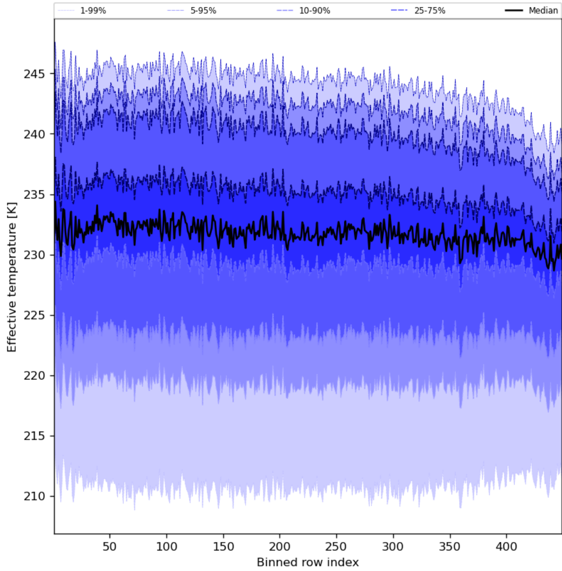
Figure 31: Along track statistics of “Effective temperature” for 2023-11-24 to 2023-11-26
