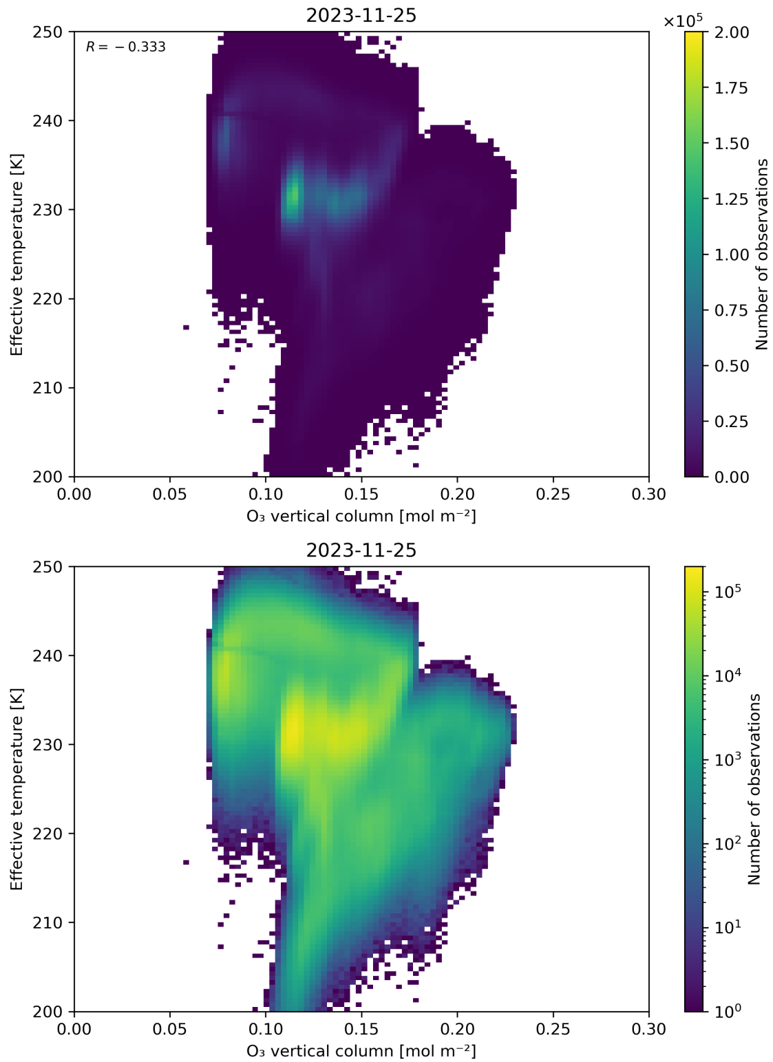
Figure 39: Scatter density plot of “O 3 vertical column” against “Effective temperature” for 2023-11-24 to 2023-11-26.
