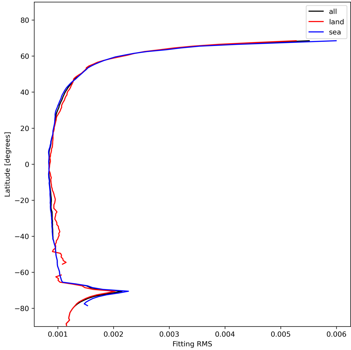
Figure 16: Zonal average of “Fitting RMS” for 2023-11-24 to 2023-11-26.
