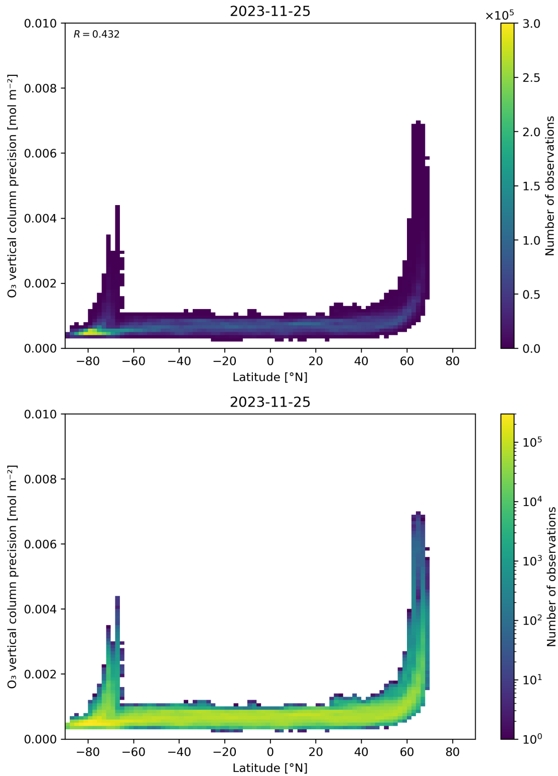
Figure 37: Scatter density plot of “Latitude” against “O 3 vertical column precision” for 2023-11-24 to 2023-11-26.
