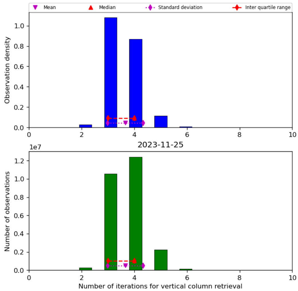
Figure 26: Histogram of “Number of iterations for vertical column retrieval” for 2023-11-24 to 2023-11-26
