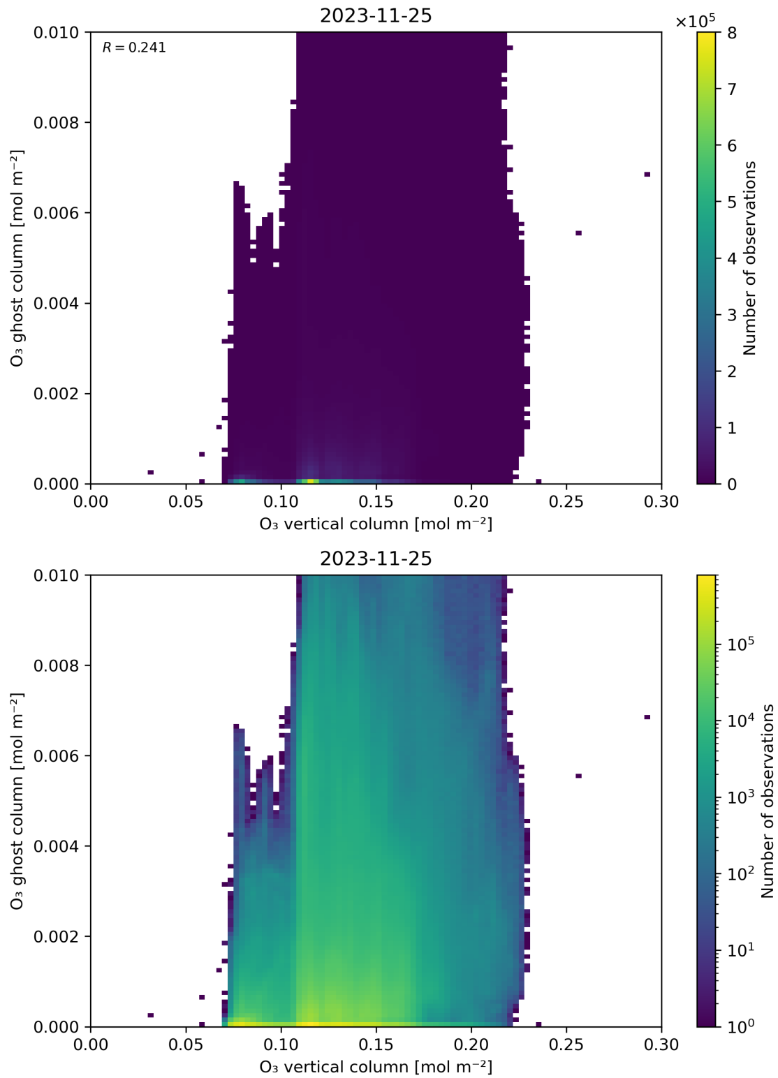
Figure 40: Scatter density plot of “O 3 vertical column” against “O 3 ghost column” for 2023-11-24 to 2023-11-26.
