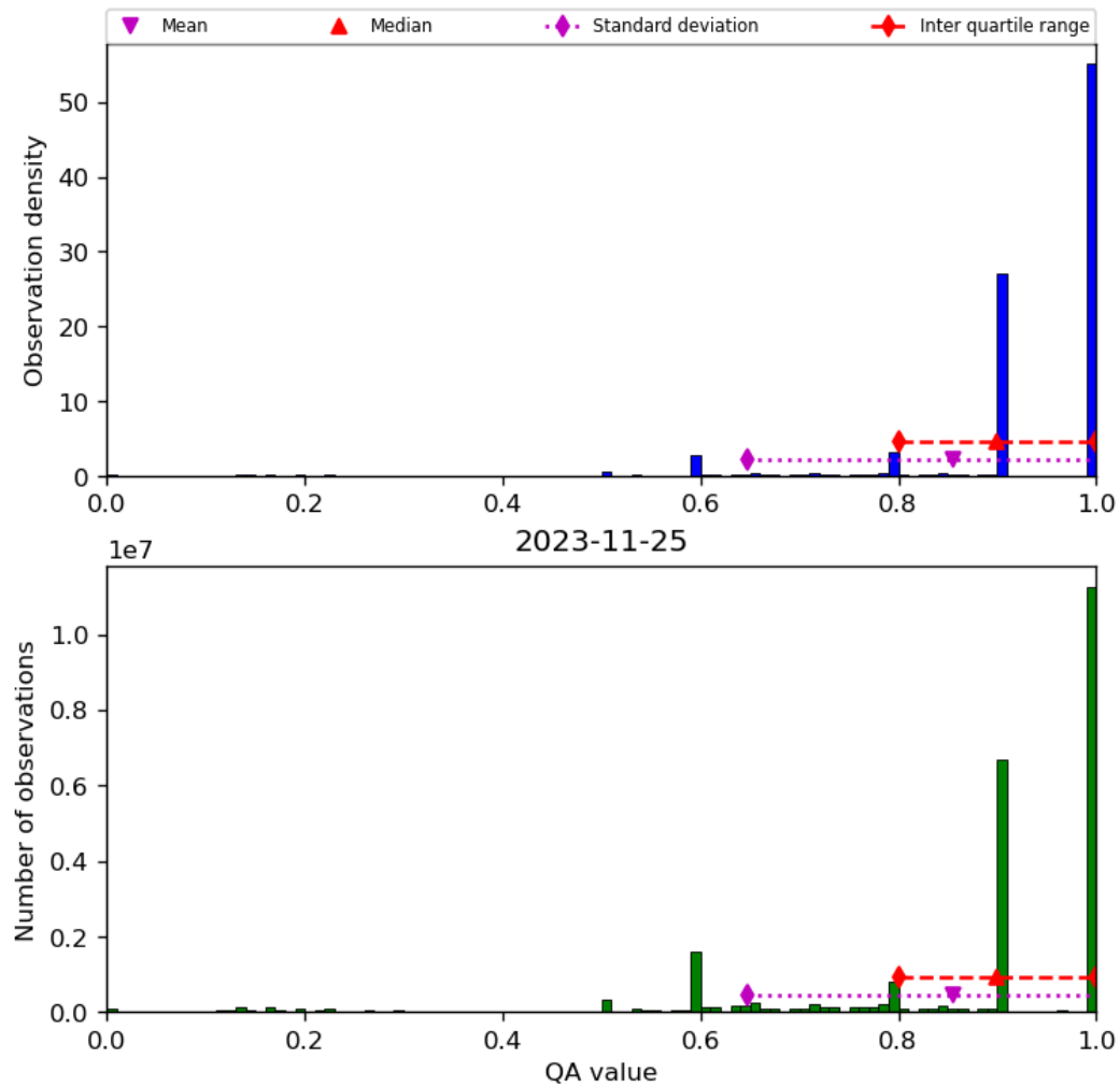
Figure 20: Histogram of “QA value” for 2023-11-24 to 2023-11-26
