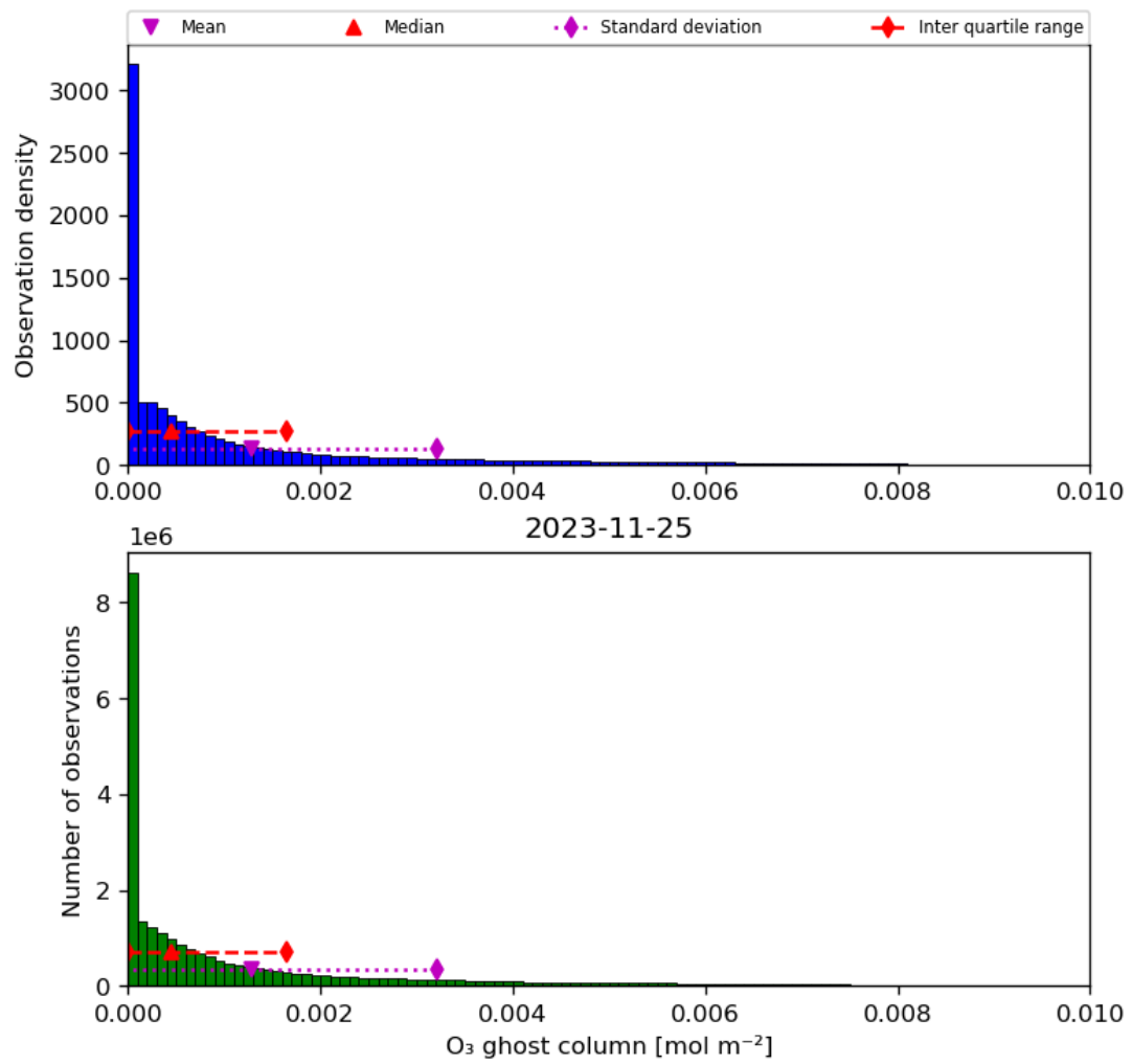
Figure 25: Histogram of “O 3 ghost column” for 2023-11-24 to 2023-11-26
