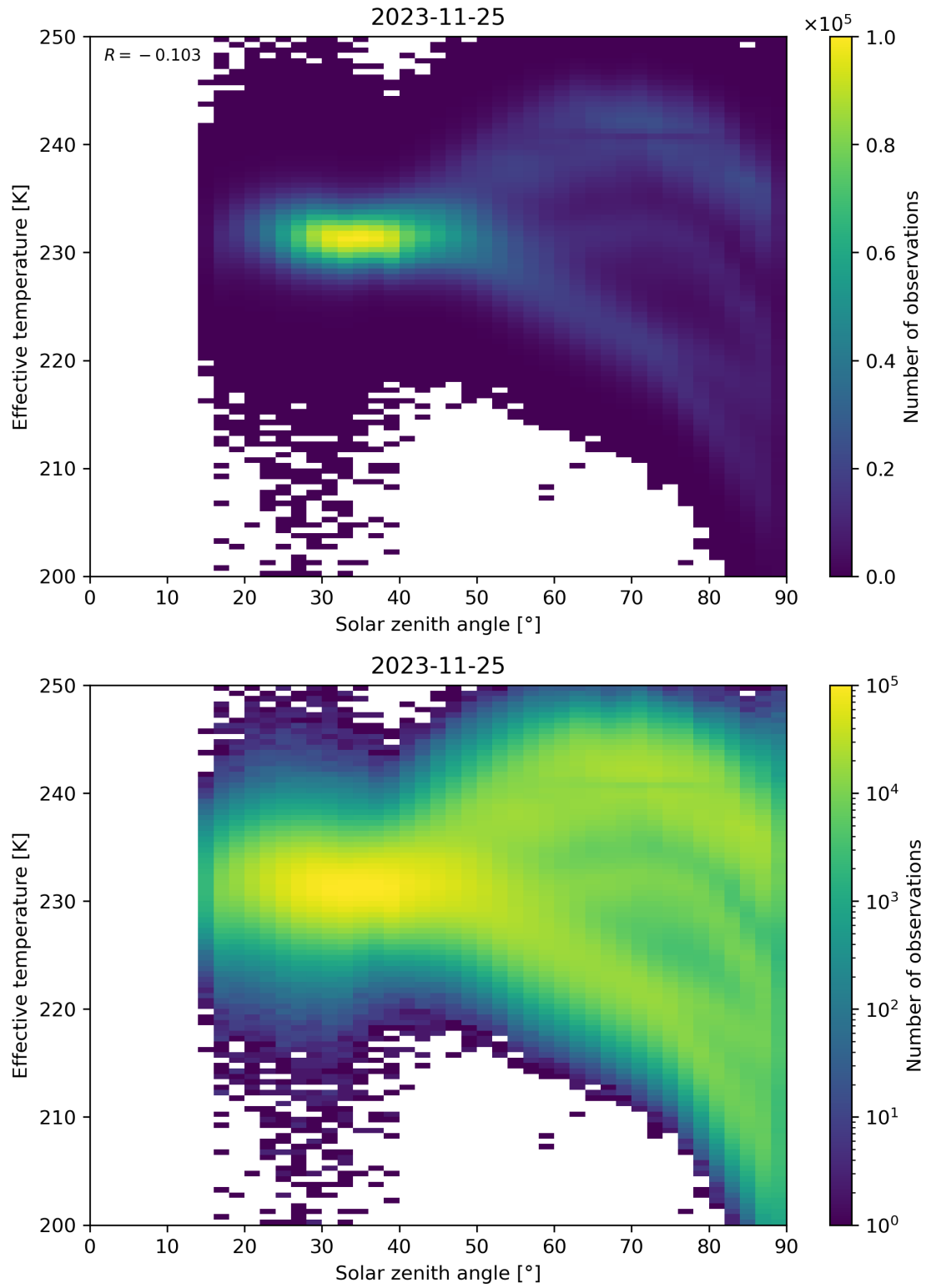
Figure 45: Scatter density plot of “Solar zenith angle” against “Effective temperature” for 2023-11-24 to 2023-11-26.
