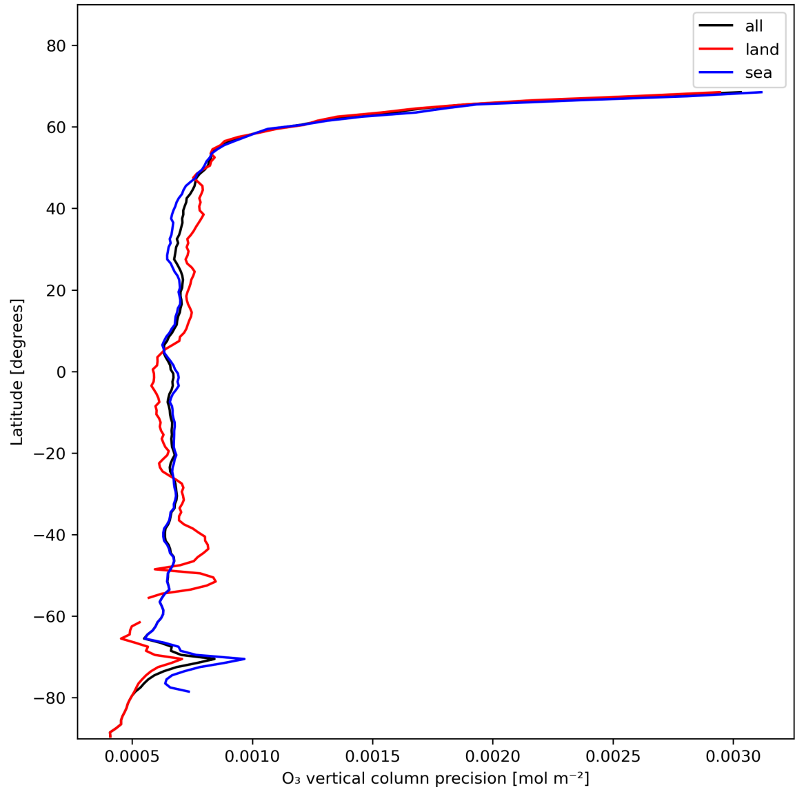
Figure 15: Zonal average of “O 3 vertical column precision” for 2023-11-24 to 2023-11-26.
