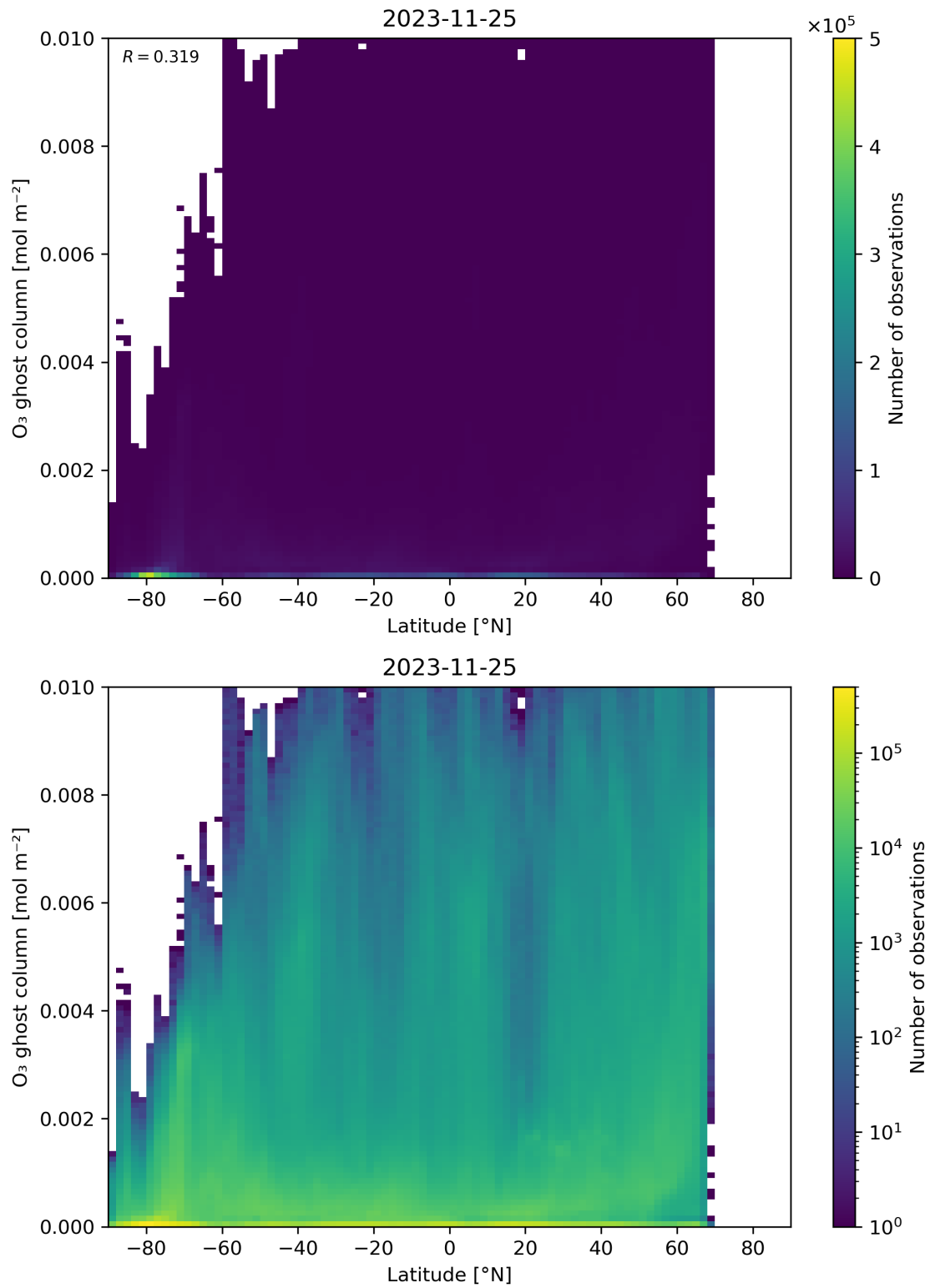
Figure 35: Scatter density plot of “Latitude” against “O 3 ghost column” for 2023-11-24 to 2023-11-26.
