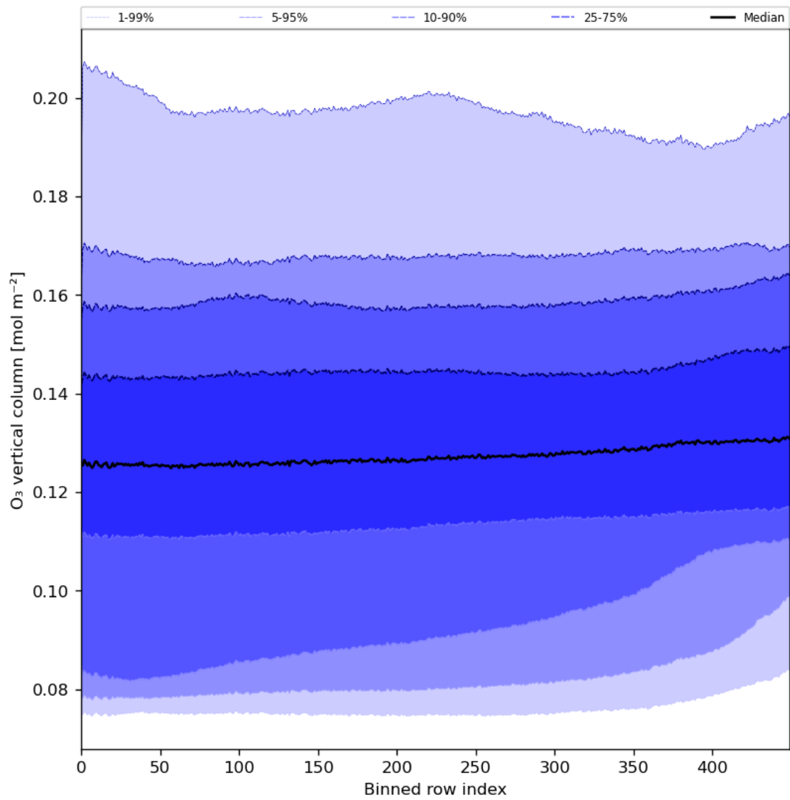
Figure 28: Along track statistics of “O 3 vertical column” for 2023-11-25 to 2023-11-27
