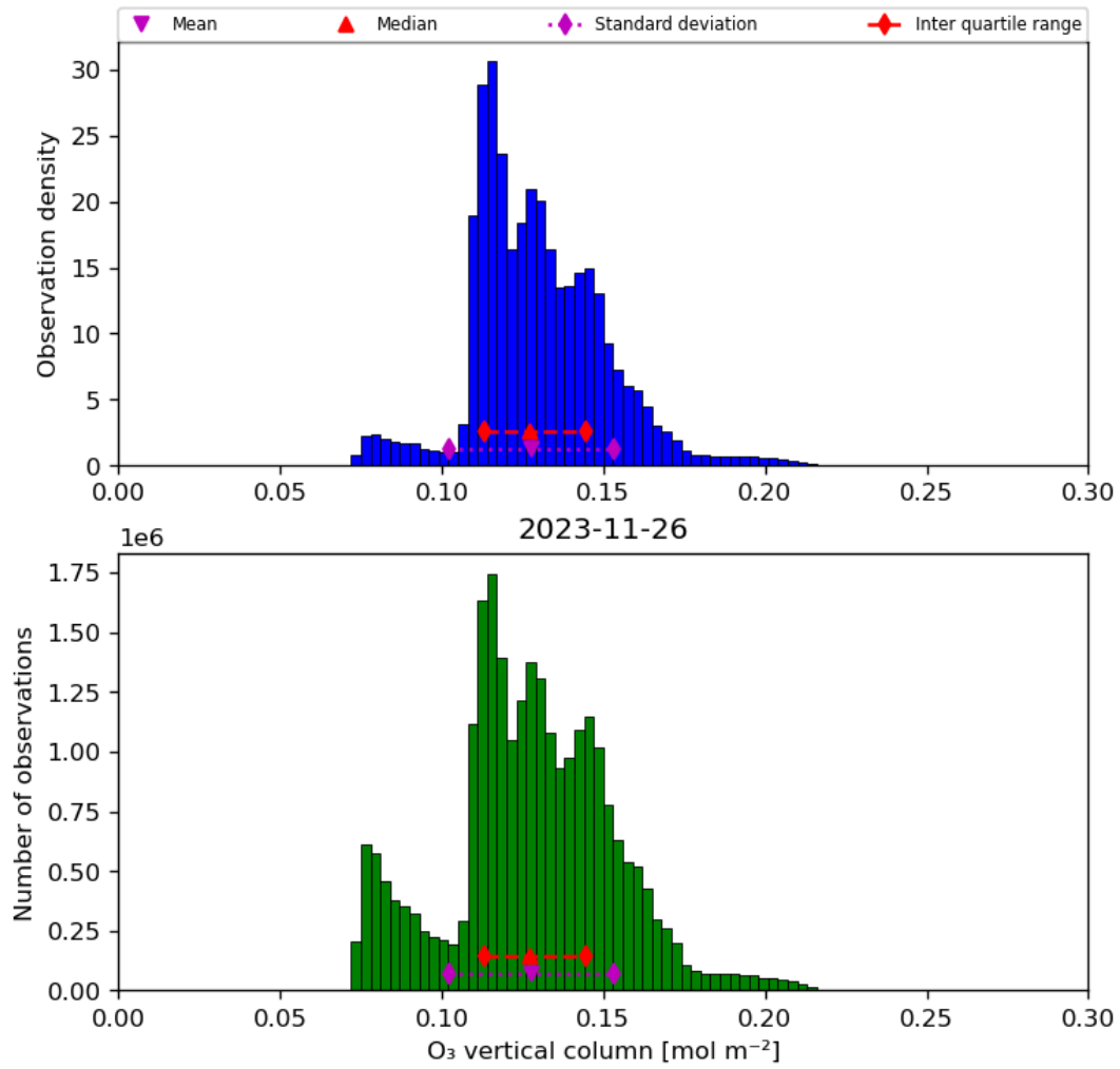
Figure 21: Histogram of “O 3 vertical column” for 2023-11-25 to 2023-11-27
