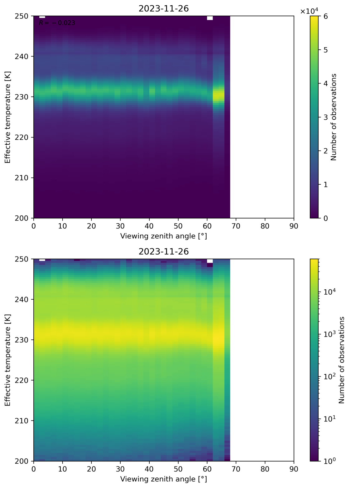
Figure 50: Scatter density plot of “Viewing zenith angle” against “Effective temperature” for 2023-11-25 to 2023-11-27.
