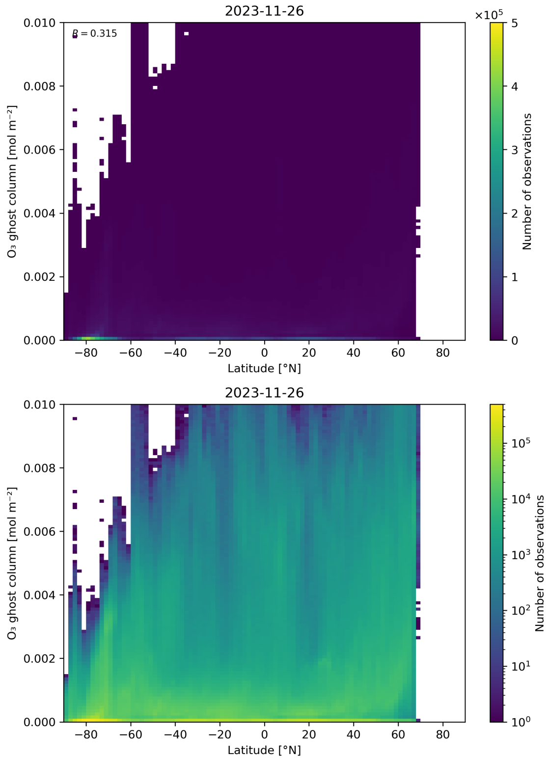
Figure 35: Scatter density plot of “Latitude” against “O 3 ghost column” for 2023-11-25 to 2023-11-27.
