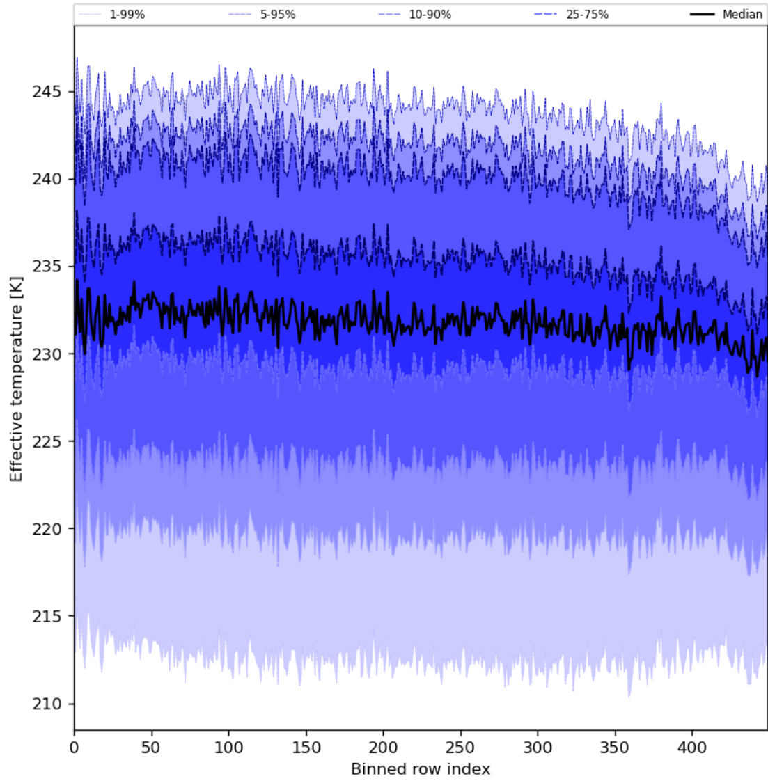
Figure 31: Along track statistics of “Effective temperature” for 2023-11-25 to 2023-11-27
