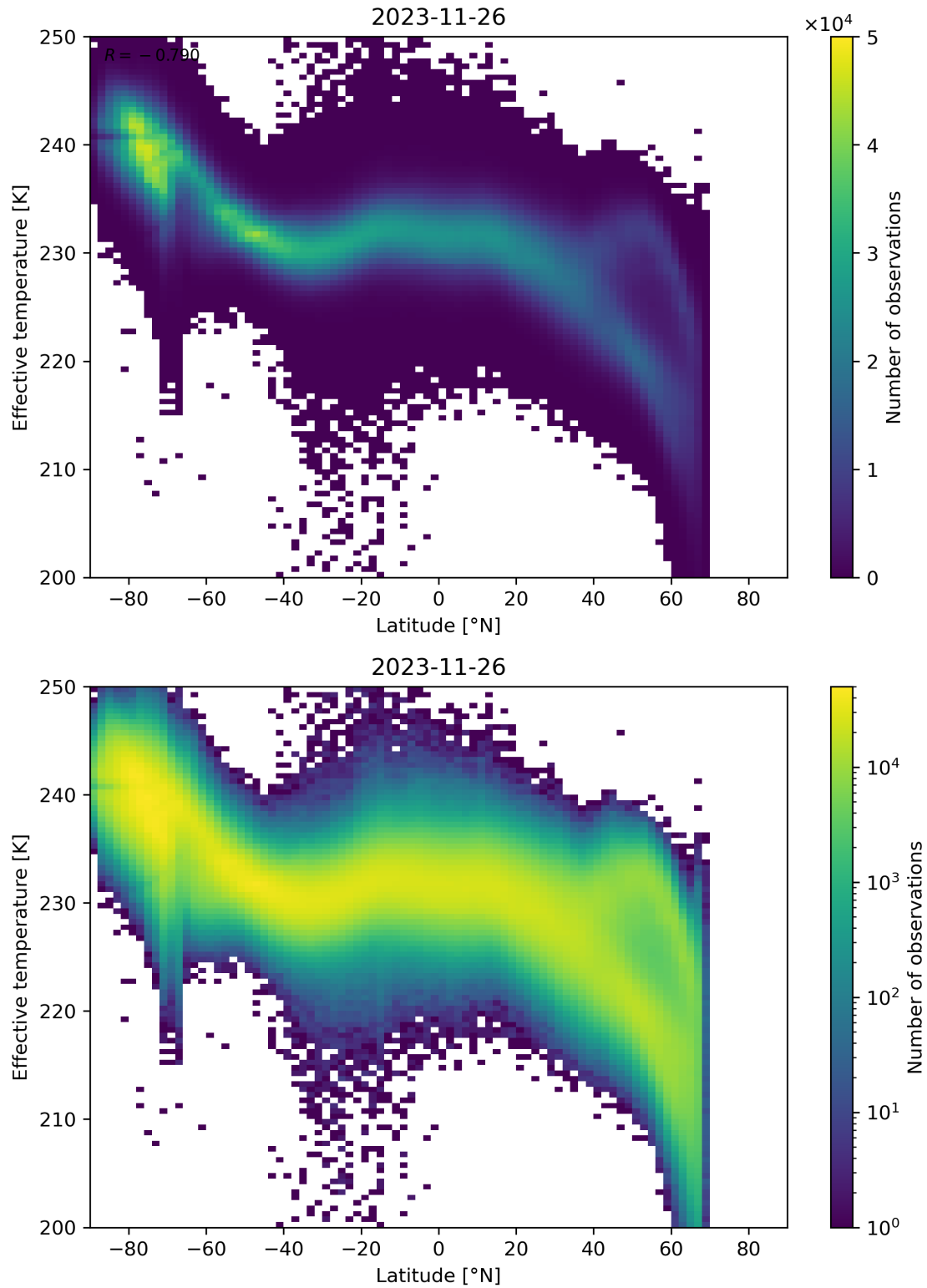
Figure 34: Scatter density plot of “Latitude” against “Effective temperature” for 2023-11-25 to 2023-11-27.
