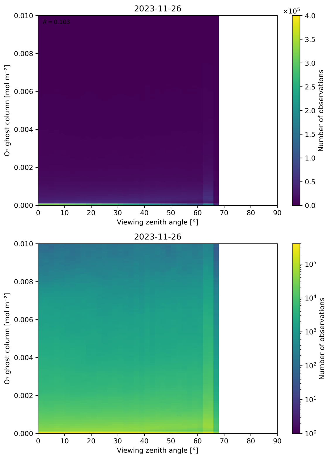
Figure 51: Scatter density plot of “Viewing zenith angle” against “O 3 ghost column” for 2023-11-25 to 2023-11-27.
