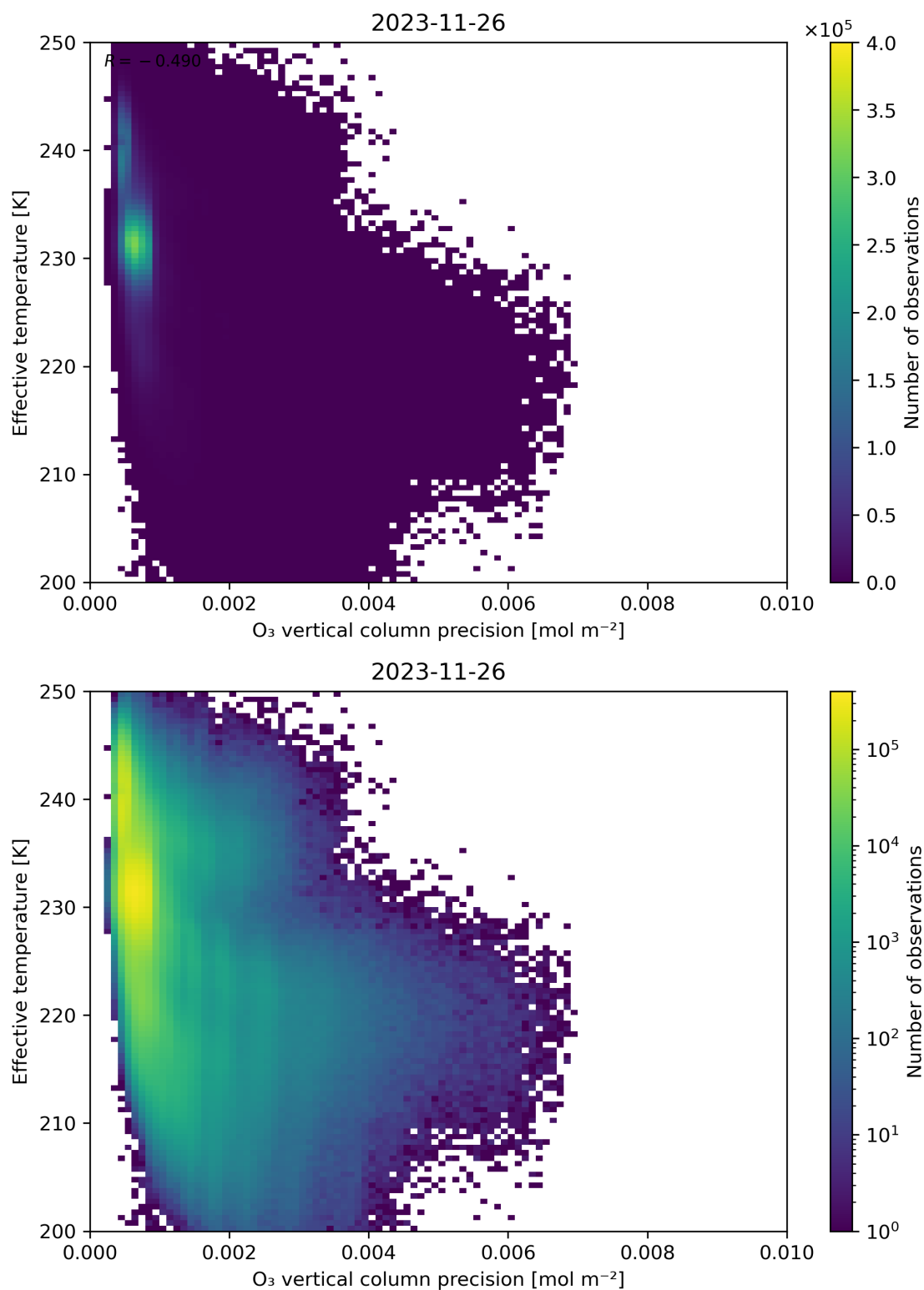
Figure 42: Scatter density plot of “O 3 vertical column precision” against “Effective temperature” for 2023-11-25 to 2023-11-27.
