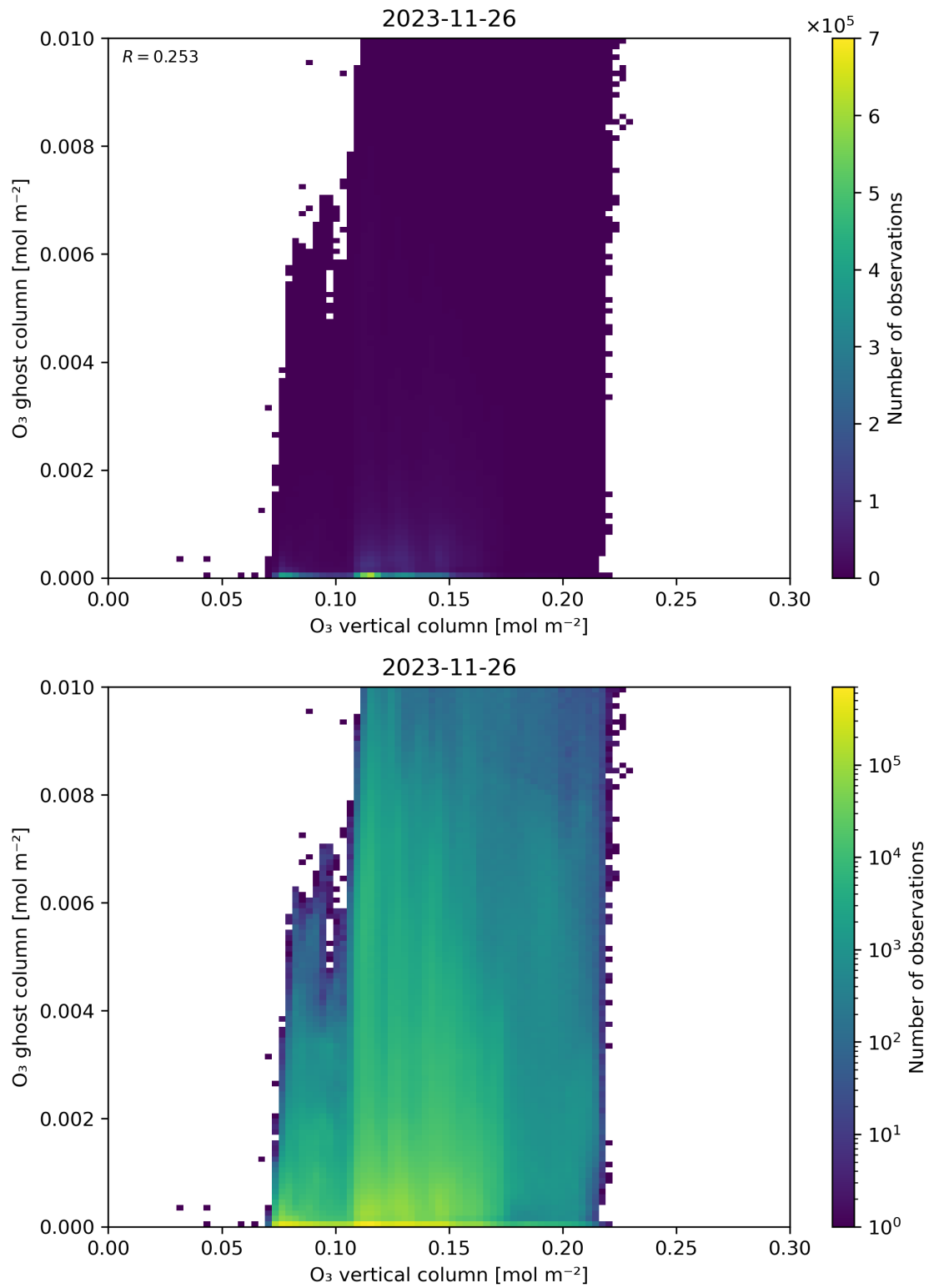
Figure 40: Scatter density plot of “O 3 vertical column” against “O 3 ghost column” for 2023-11-25 to 2023-11-27.
