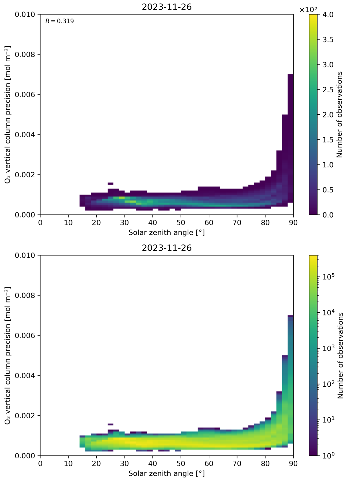
Figure 48: Scatter density plot of “Solar zenith angle” against “O 3 vertical column precision” for 2023-11-25 to 2023-11-27.
