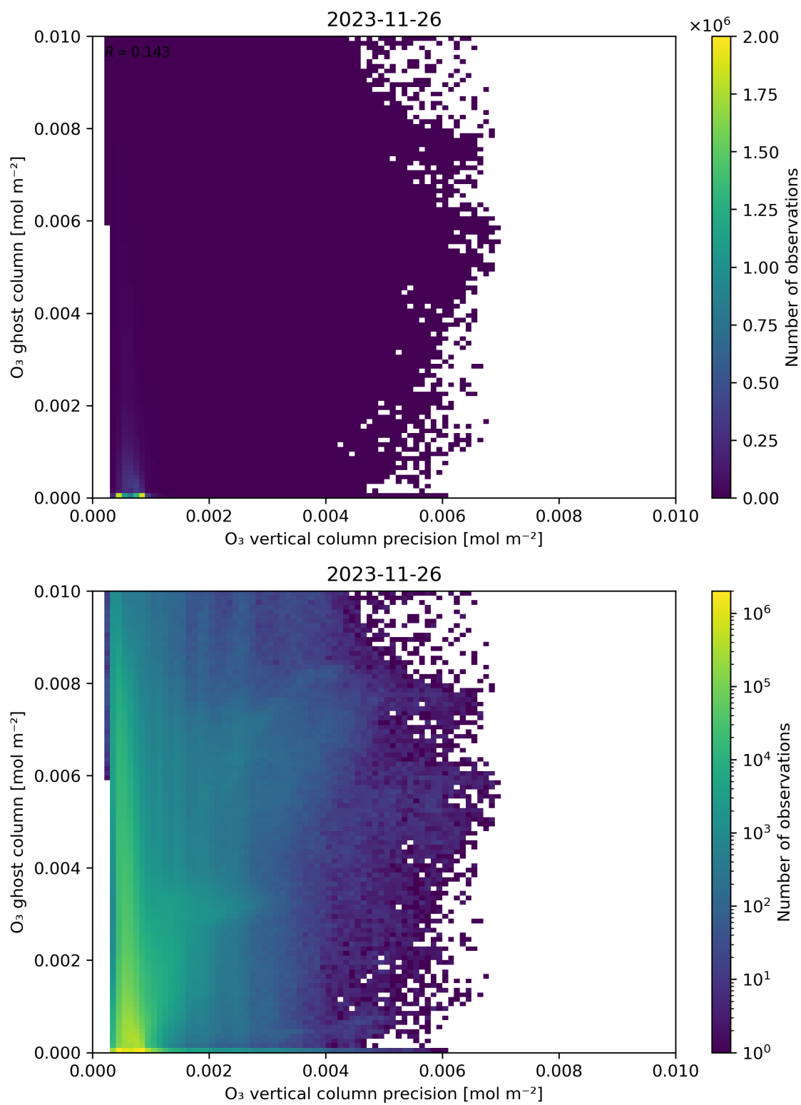
Figure 43: Scatter density plot of “ \text{O}_3 vertical column precision” against “ \text{O}_3 ghost column” for 2023-11-25 to 2023-11-27.
