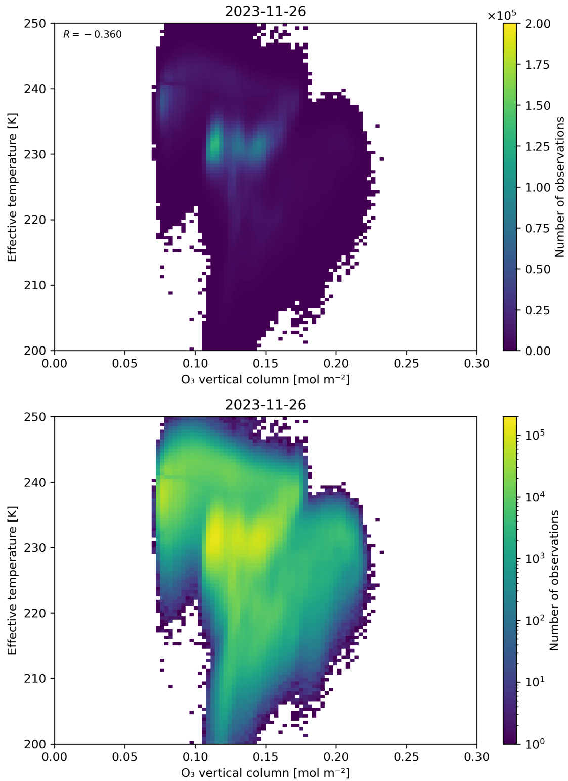
Figure 39: Scatter density plot of “O 3 vertical column” against “Effective temperature” for 2023-11-25 to 2023-11-27.
