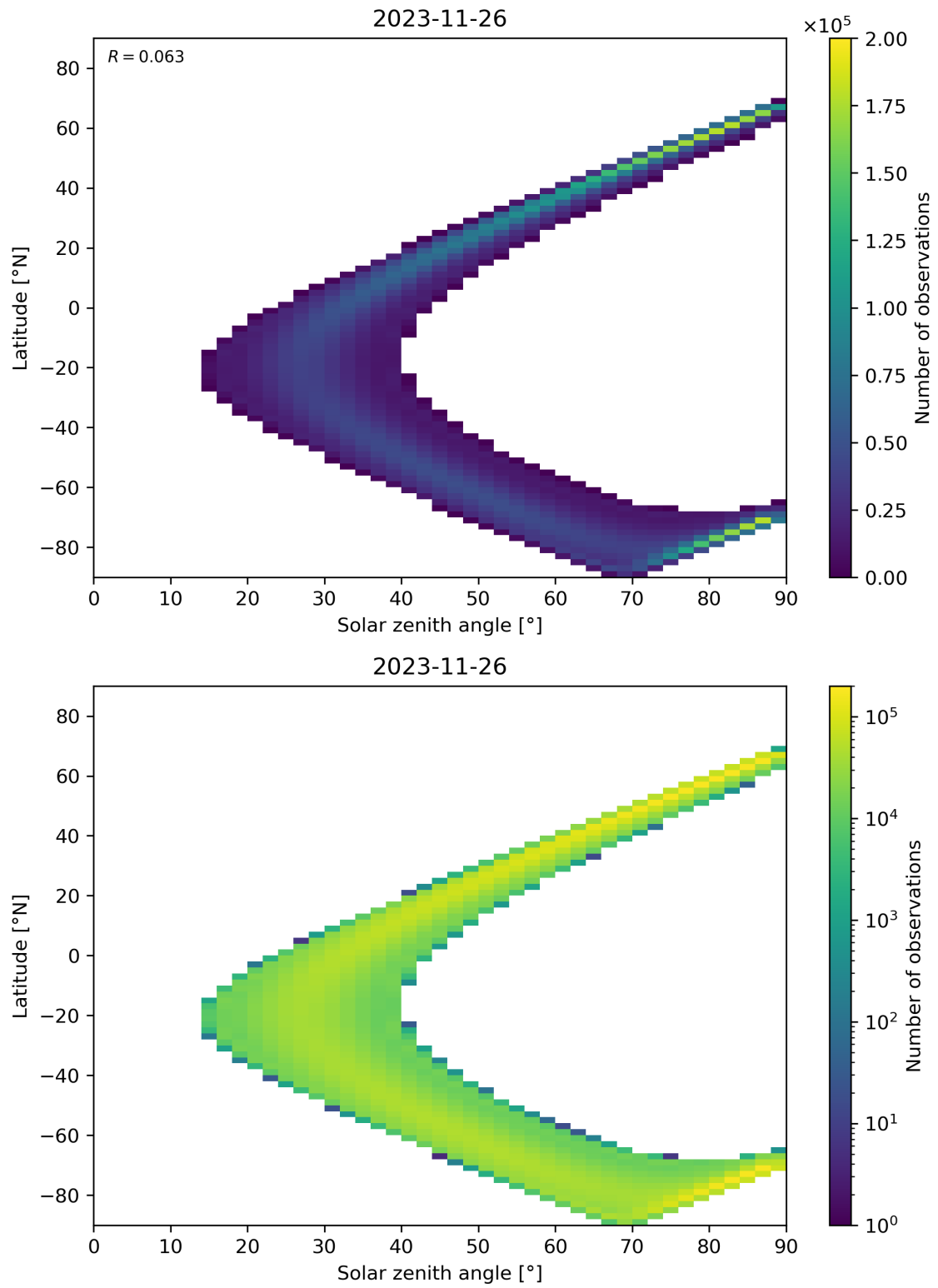
Figure 44: Scatter density plot of “Solar zenith angle” against “Latitude” for 2023-11-25 to 2023-11-27.
