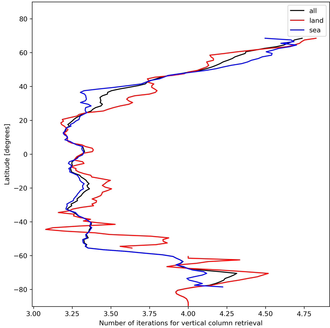
Figure 19: Zonal average of “Number of iterations for vertical column retrieval” for 2023-11-25 to 2023-11-27.
