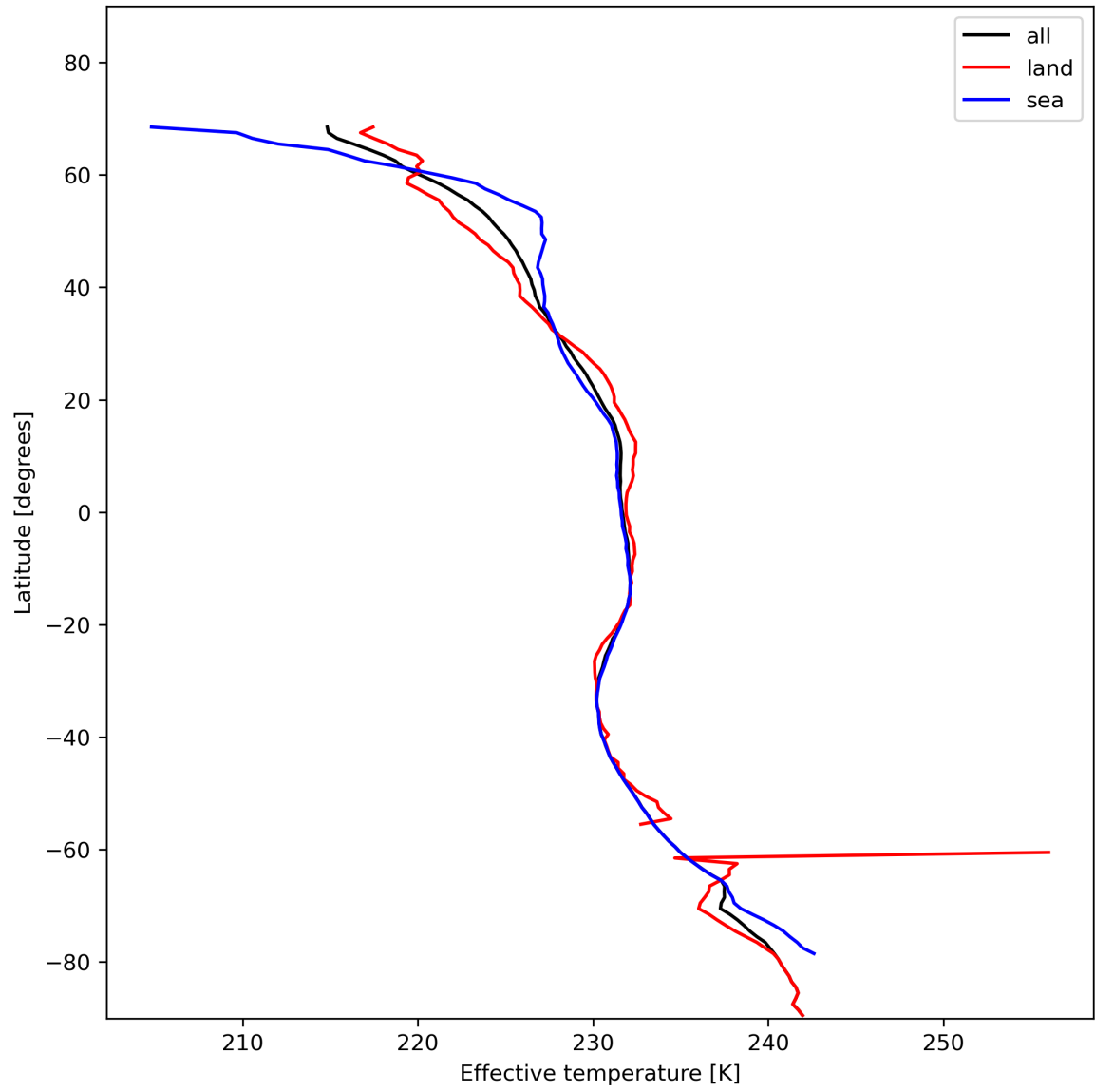
Figure 17: Zonal average of “Effective temperature” for 2023-11-25 to 2023-11-27.
