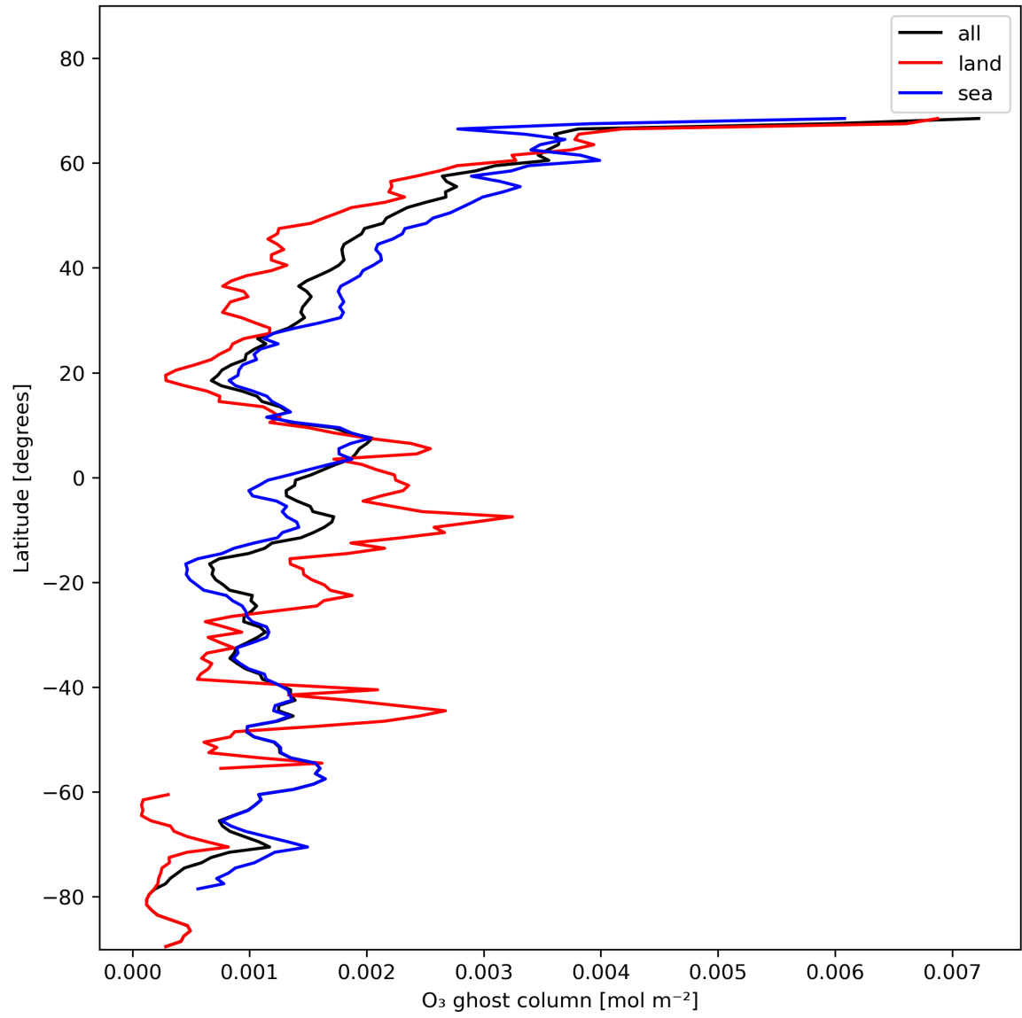
Figure 18: Zonal average of “O 3 ghost column” for 2023-11-25 to 2023-11-27.
