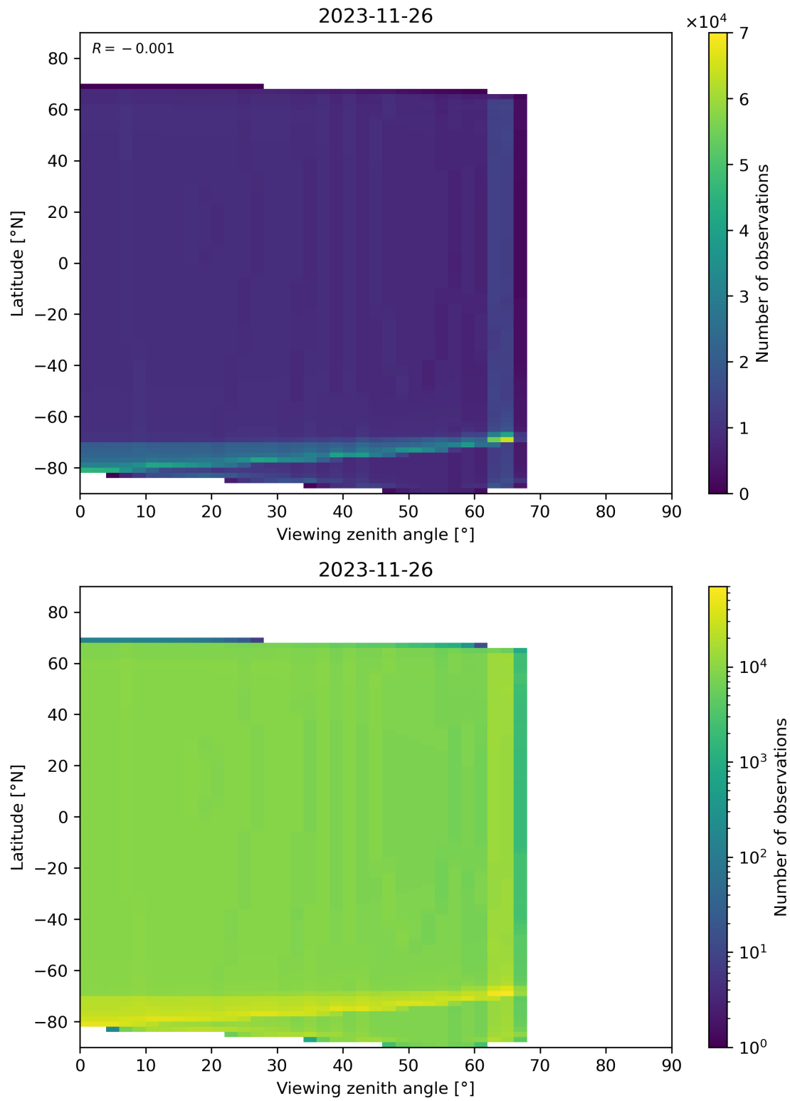
Figure 49: Scatter density plot of “Viewing zenith angle” against “Latitude” for 2023-11-25 to 2023-11-27.
