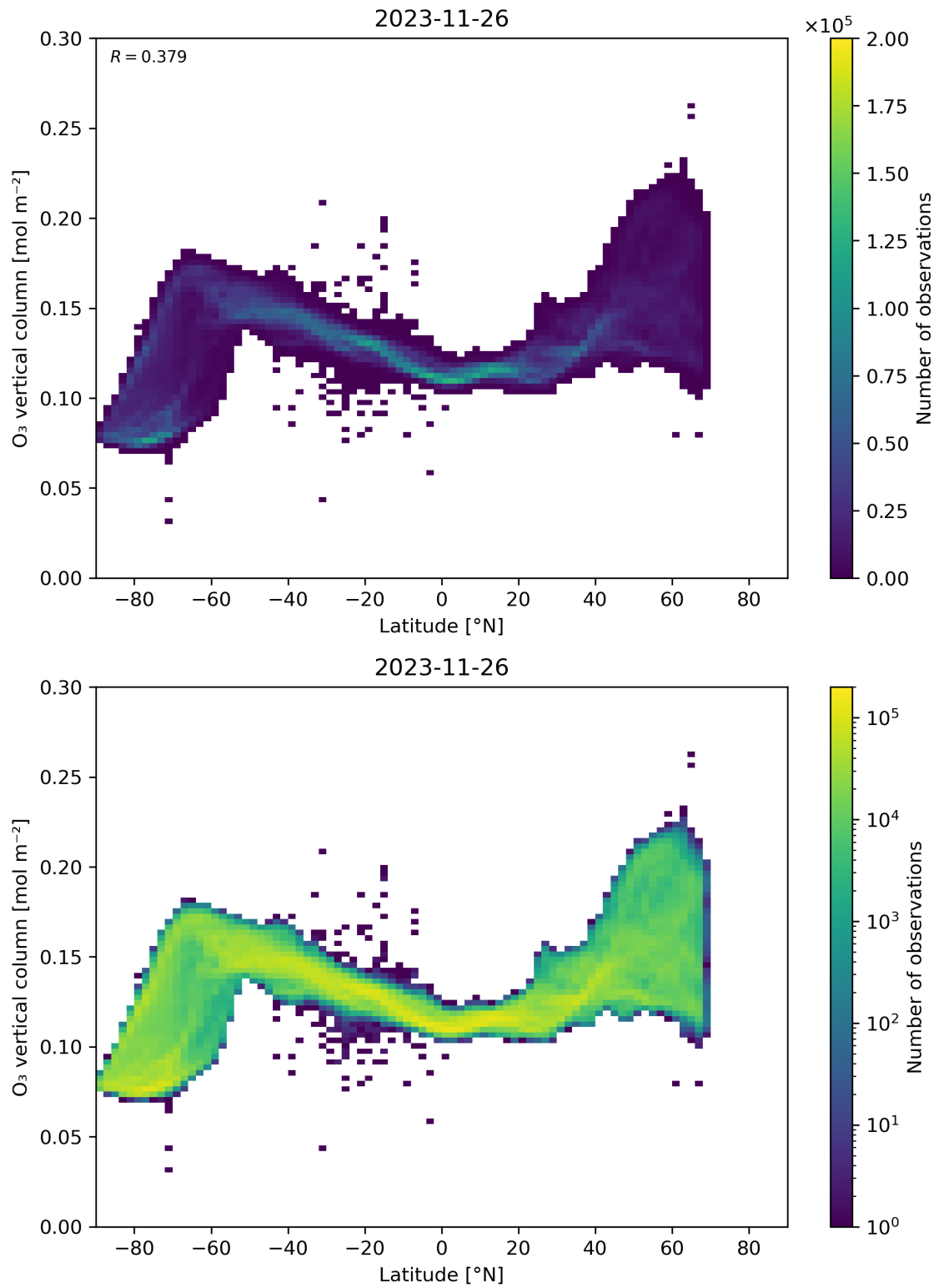
Figure 36: Scatter density plot of “Latitude” against “O 3 vertical column” for 2023-11-25 to 2023-11-27.
