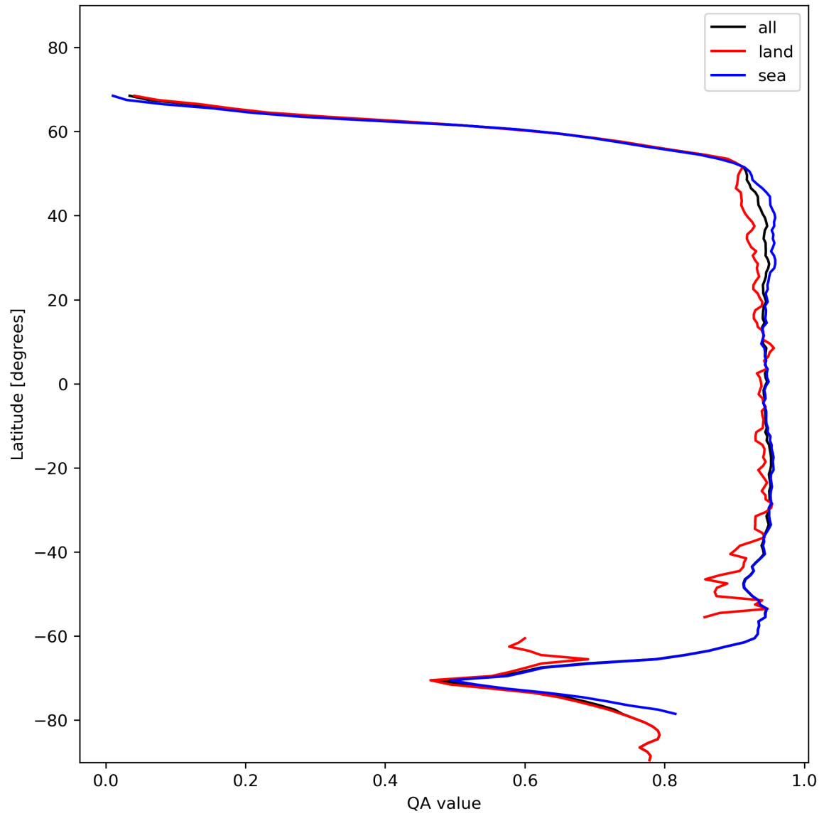
Figure 13: Zonal average of “QA value” for 2023-11-25 to 2023-11-27.
