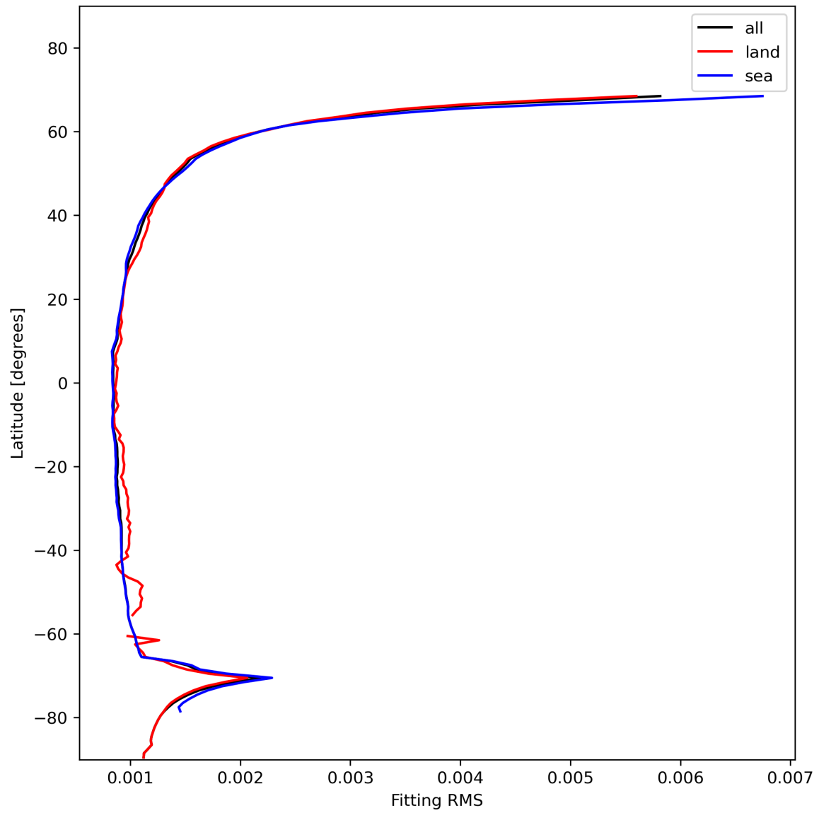
Figure 16: Zonal average of “Fitting RMS” for 2023-11-25 to 2023-11-27.
