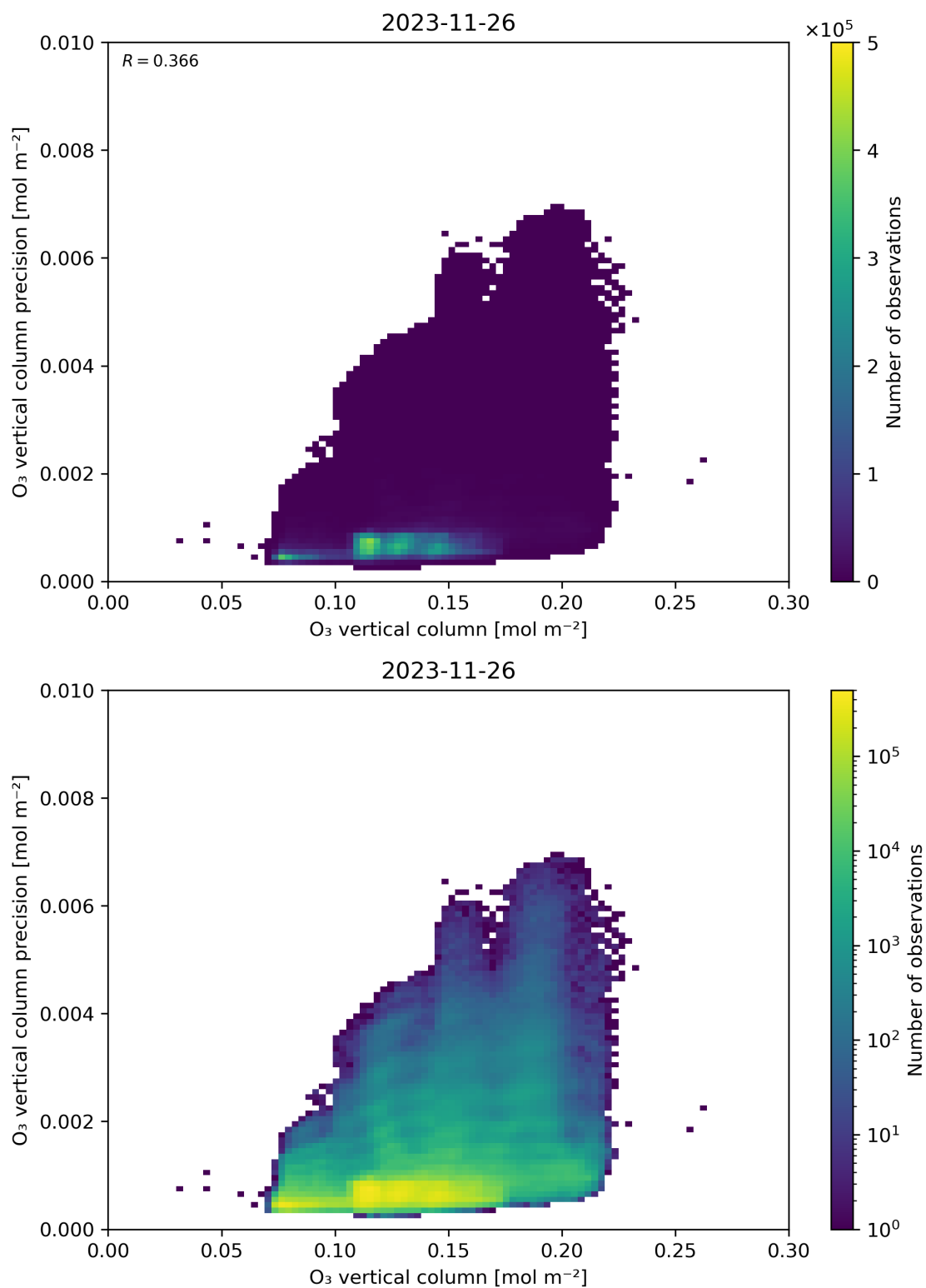
Figure 41: Scatter density plot of “O 3 vertical column” against “O 3 vertical column precision” for 2023-11-25 to 2023-11-27.
