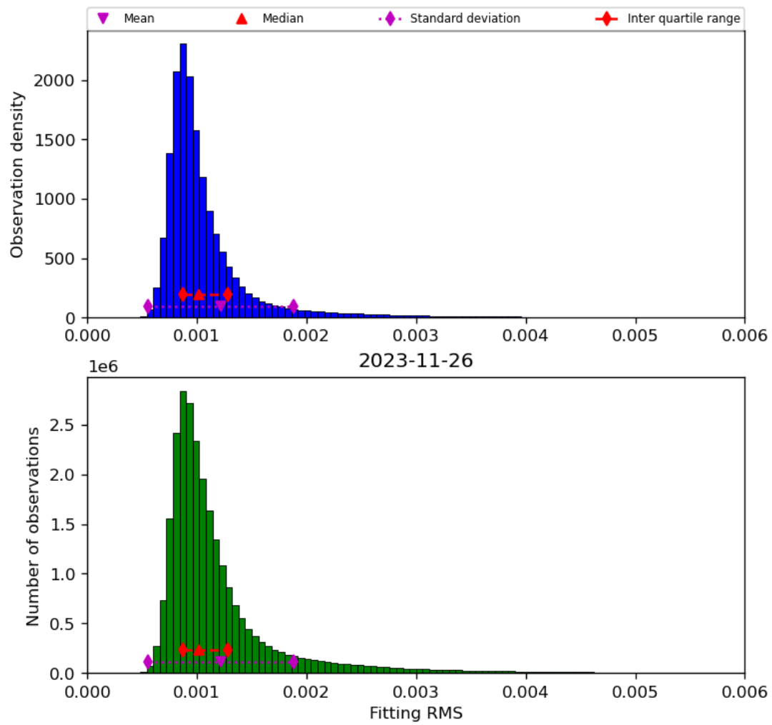
Figure 23: Histogram of “Fitting RMS” for 2023-11-25 to 2023-11-27
