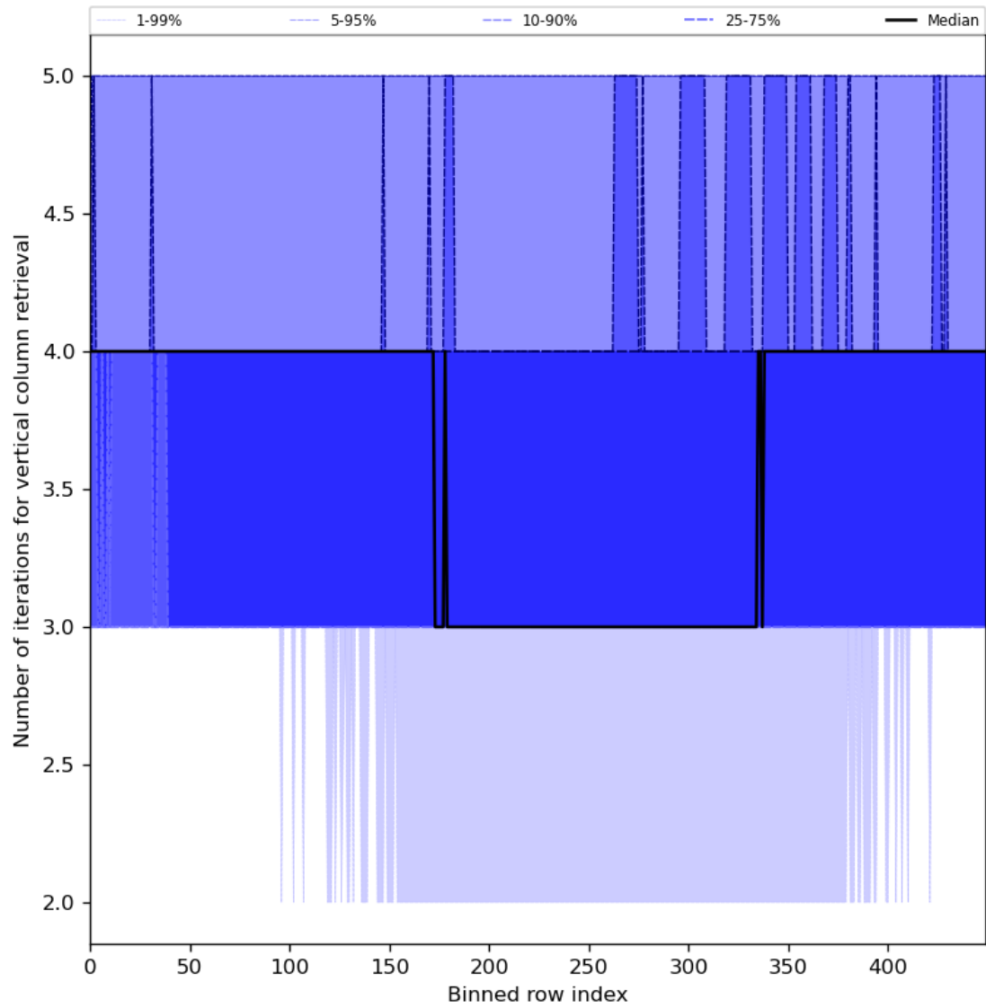
Figure 33: Along track statistics of “Number of iterations for vertical column retrieval” for 2023-11-25 to 2023-11-27
