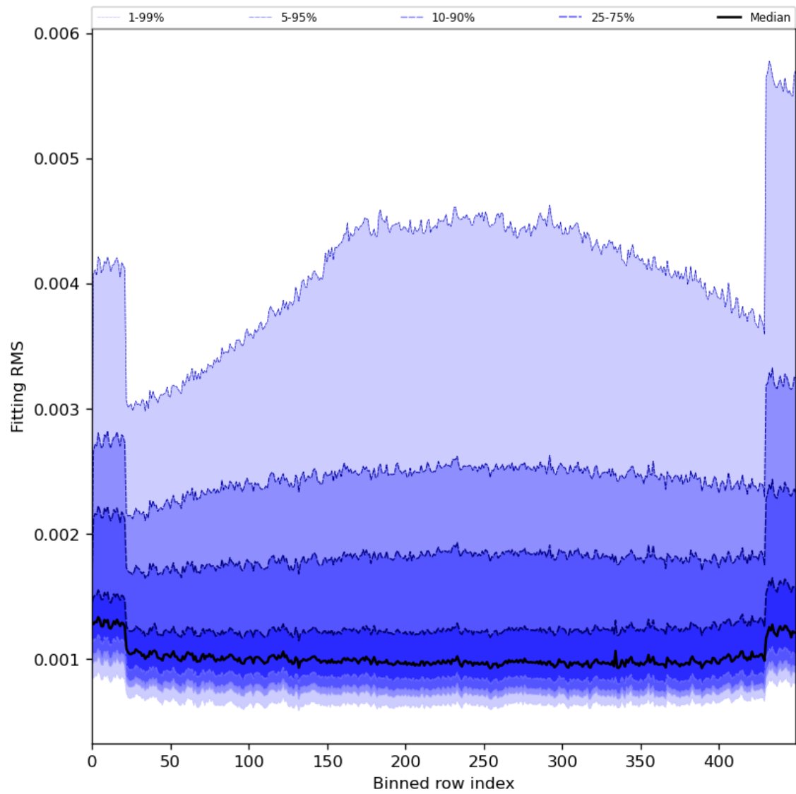
Figure 30: Along track statistics of “Fitting RMS” for 2023-11-25 to 2023-11-27
