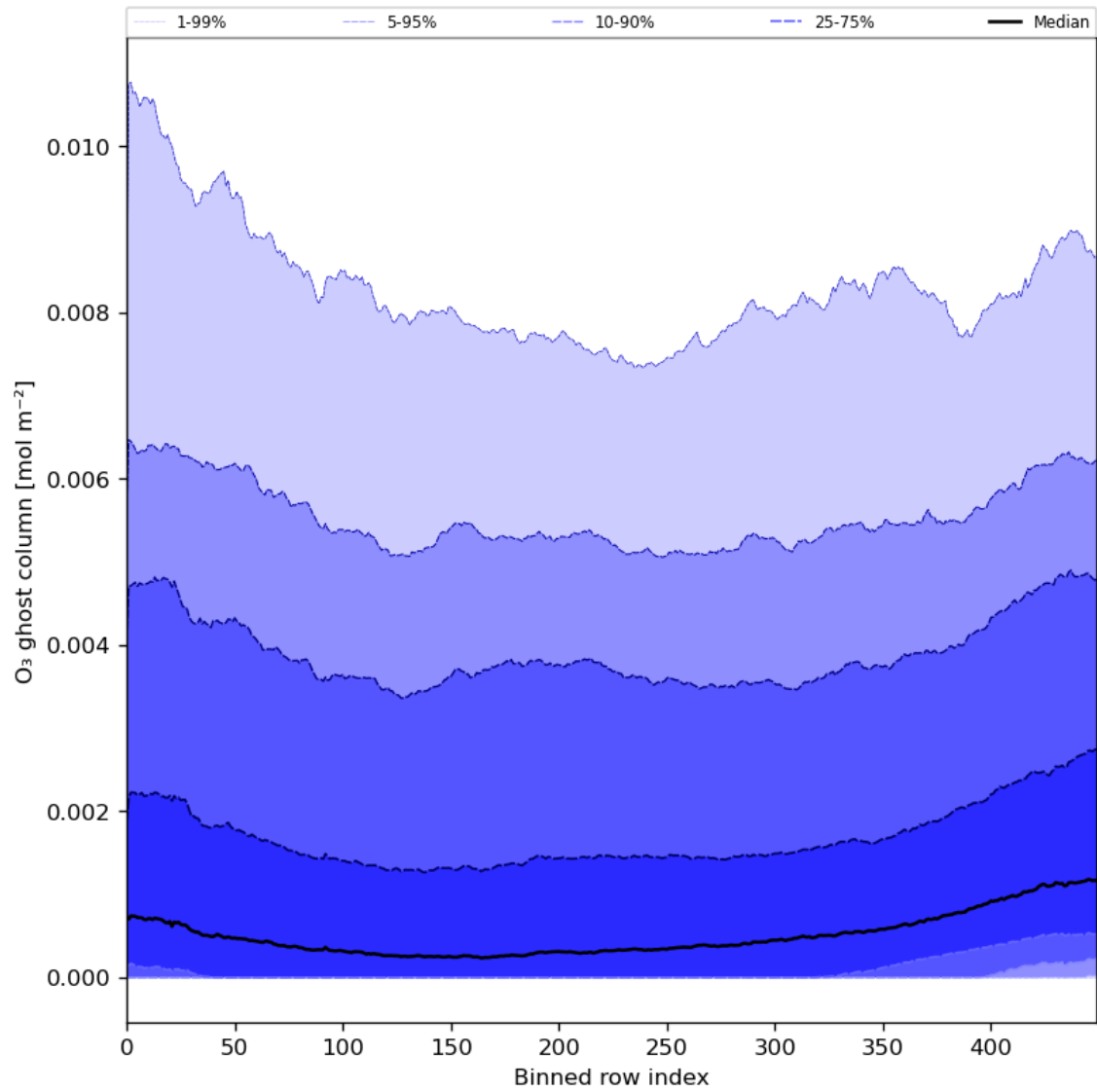
Figure 32: Along track statistics of “O 3 ghost column” for 2023-11-25 to 2023-11-27
