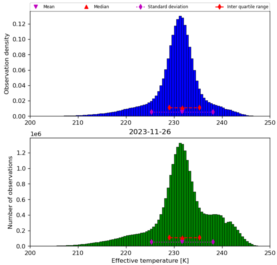
Figure 24: Histogram of “Effective temperature” for 2023-11-25 to 2023-11-27
