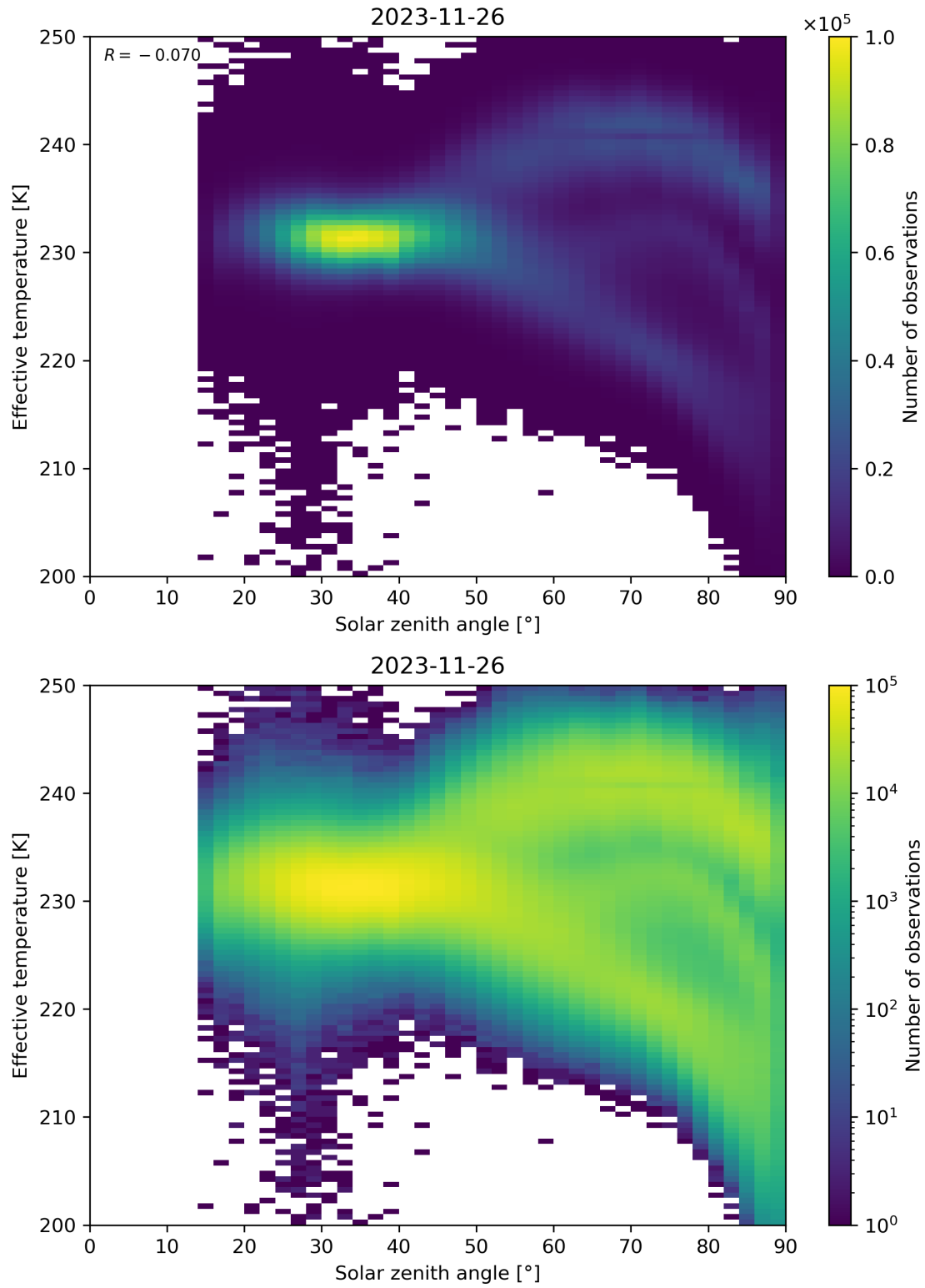
Figure 45: Scatter density plot of “Solar zenith angle” against “Effective temperature” for 2023-11-25 to 2023-11-27.
