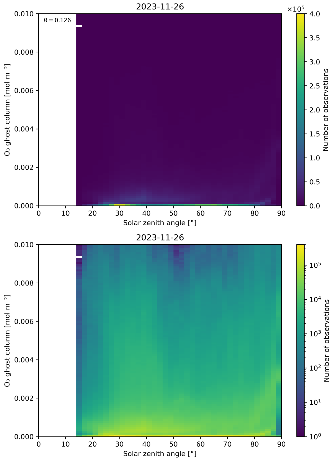
Figure 46: Scatter density plot of “Solar zenith angle” against “O 3 ghost column” for 2023-11-25 to 2023-11-27.
