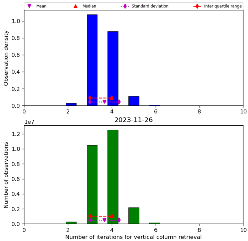
Figure 26: Histogram of “Number of iterations for vertical column retrieval” for 2023-11-25 to 2023-11-27
