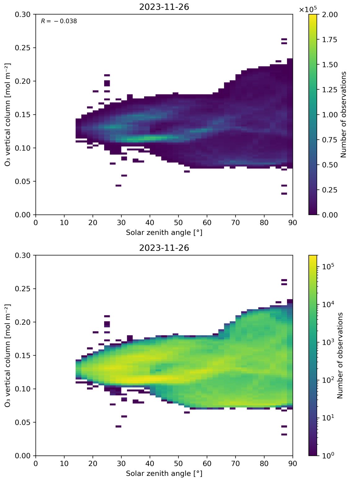
Figure 47: Scatter density plot of “Solar zenith angle” against “O 3 vertical column” for 2023-11-25 to 2023-11-27.
