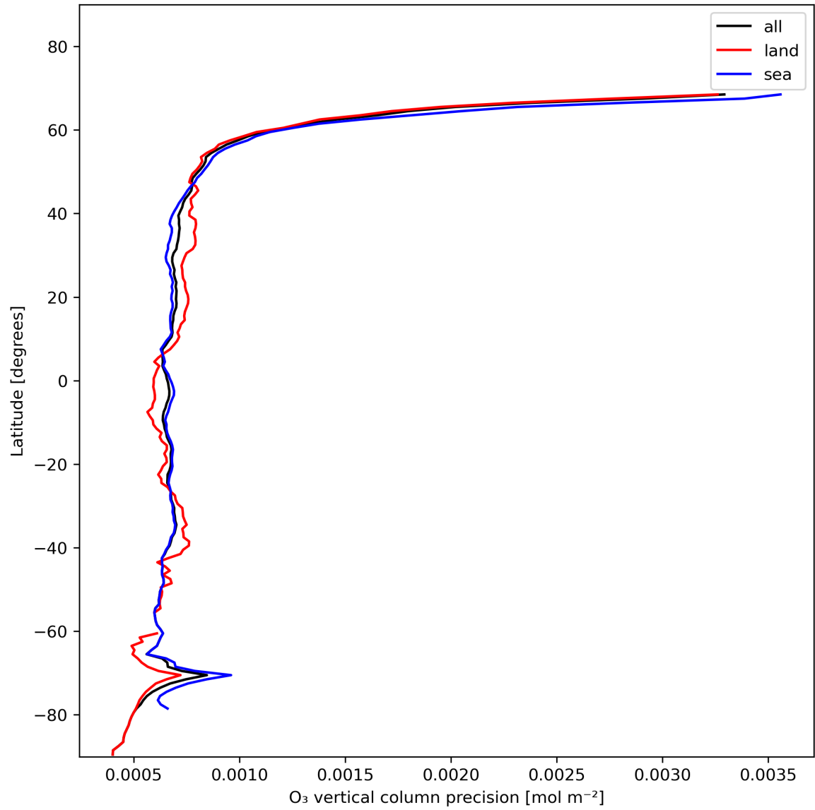
Figure 15: Zonal average of “O 3 vertical column precision” for 2023-11-25 to 2023-11-27.
