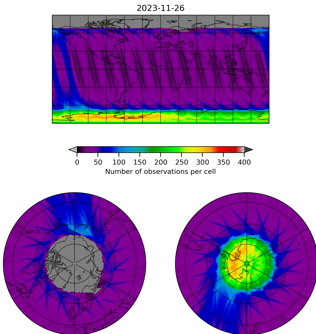
Figure 12: Map of the number of observations for 2023-11-25 to 2023-11-27
