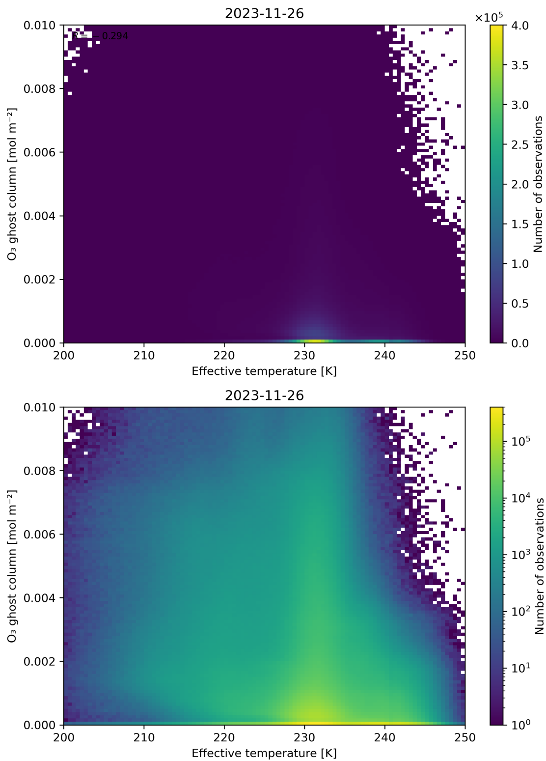
Figure 38: Scatter density plot of “Effective temperature” against “O 3 ghost column” for 2023-11-25 to 2023-11-27.
