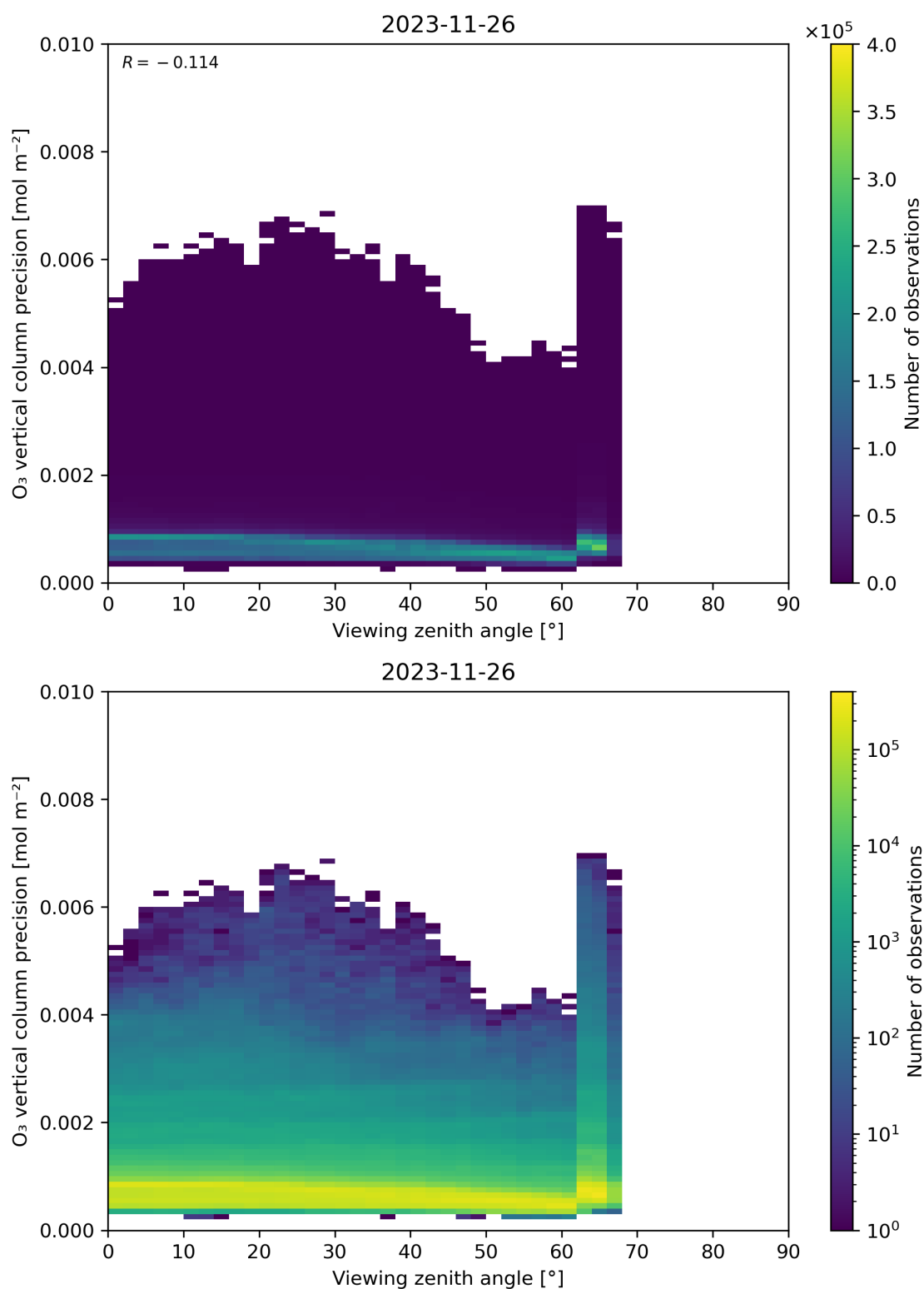
Figure 53: Scatter density plot of “Viewing zenith angle” against “O 3 vertical column precision” for 2023-11-25 to 2023-11-27.
