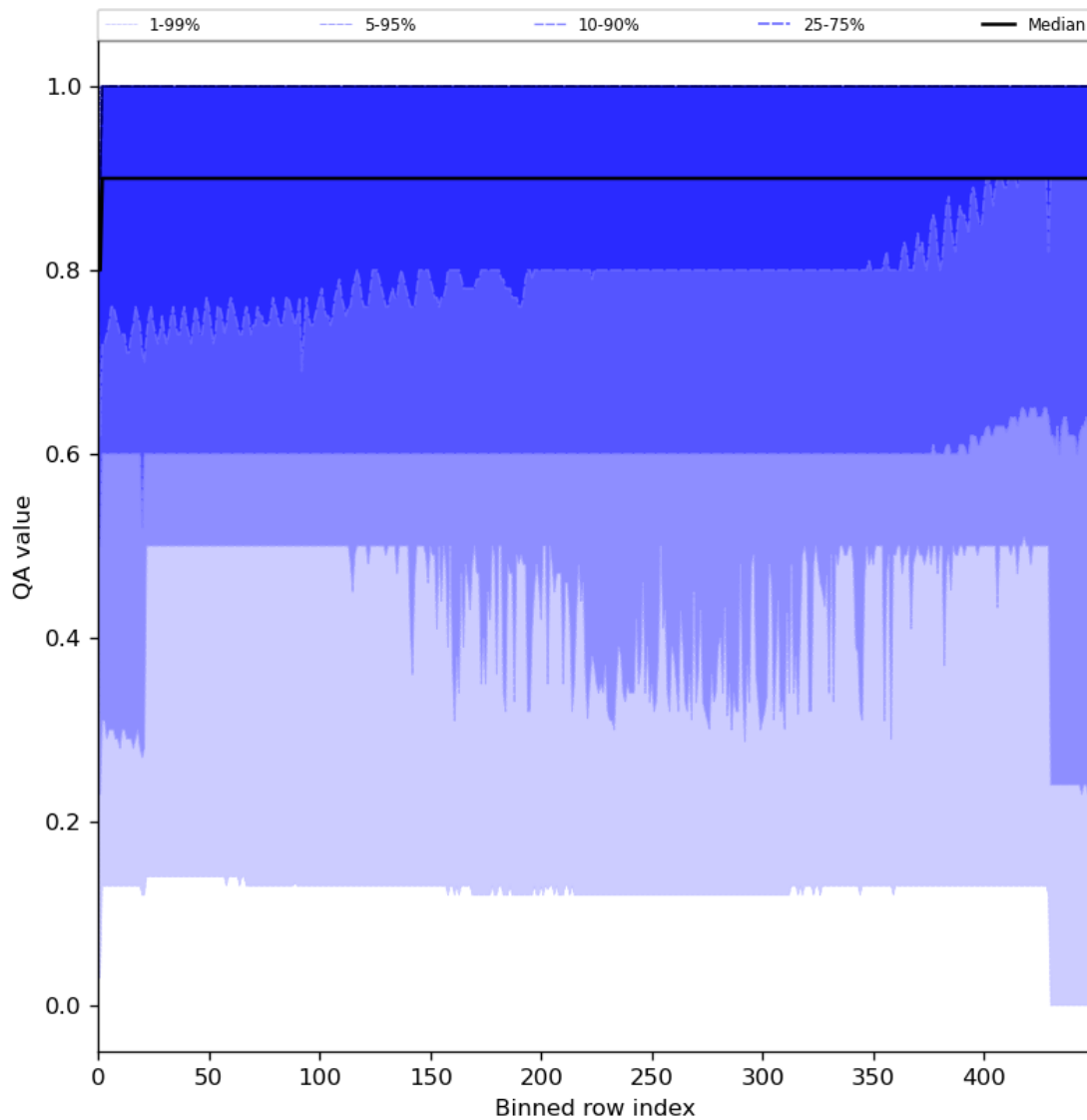
Figure 27: Along track statistics of “QA value” for 2023-11-25 to 2023-11-27
