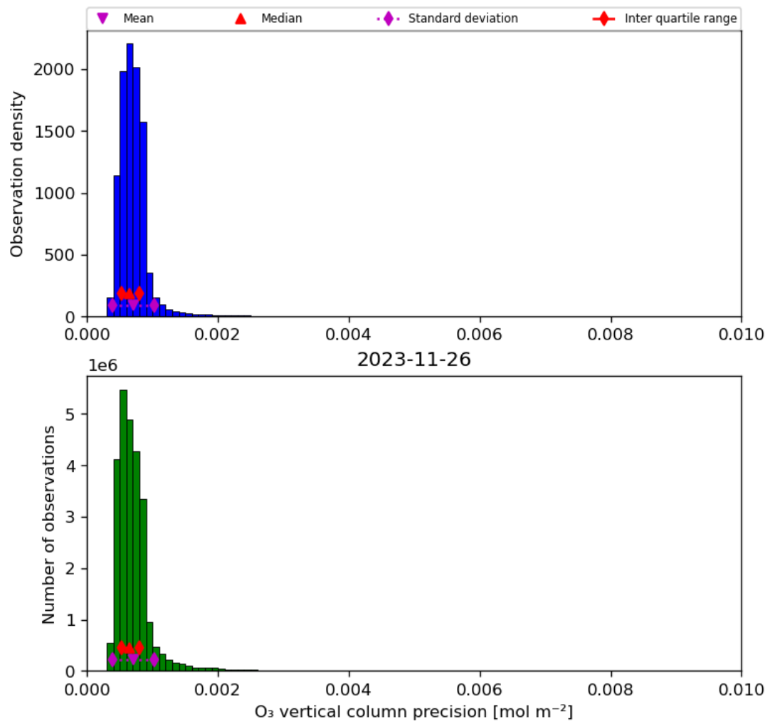
Figure 22: Histogram of “O 3 vertical column precision” for 2023-11-25 to 2023-11-27
