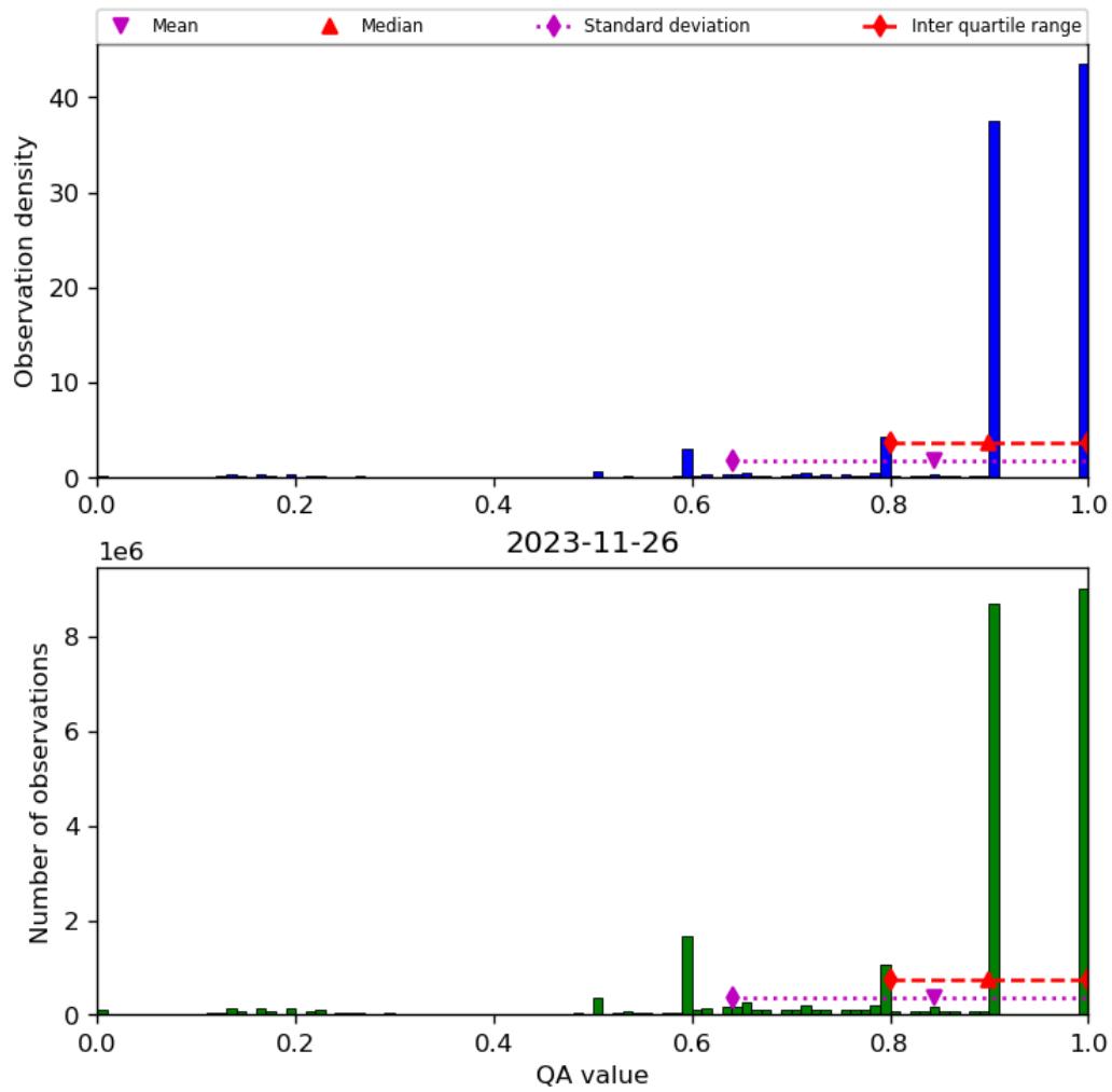
Figure 20: Histogram of “QA value” for 2023-11-25 to 2023-11-27
