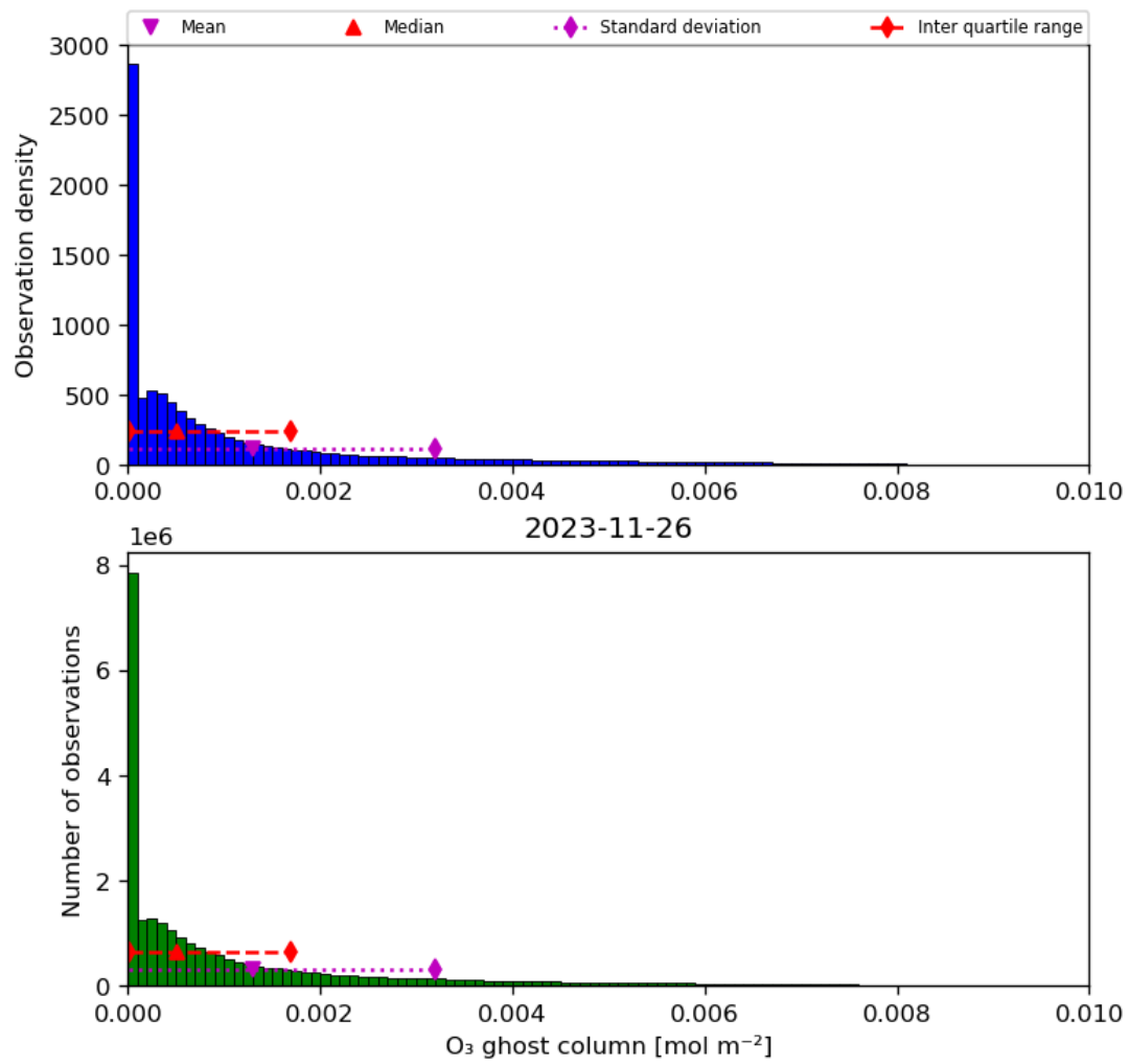
Figure 25: Histogram of “O 3 ghost column” for 2023-11-25 to 2023-11-27
