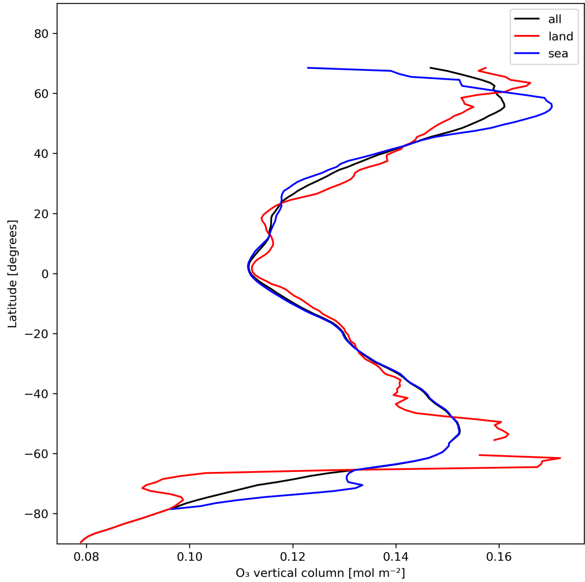
Figure 14: Zonal average of “O 3 vertical column” for 2023-11-25 to 2023-11-27.
