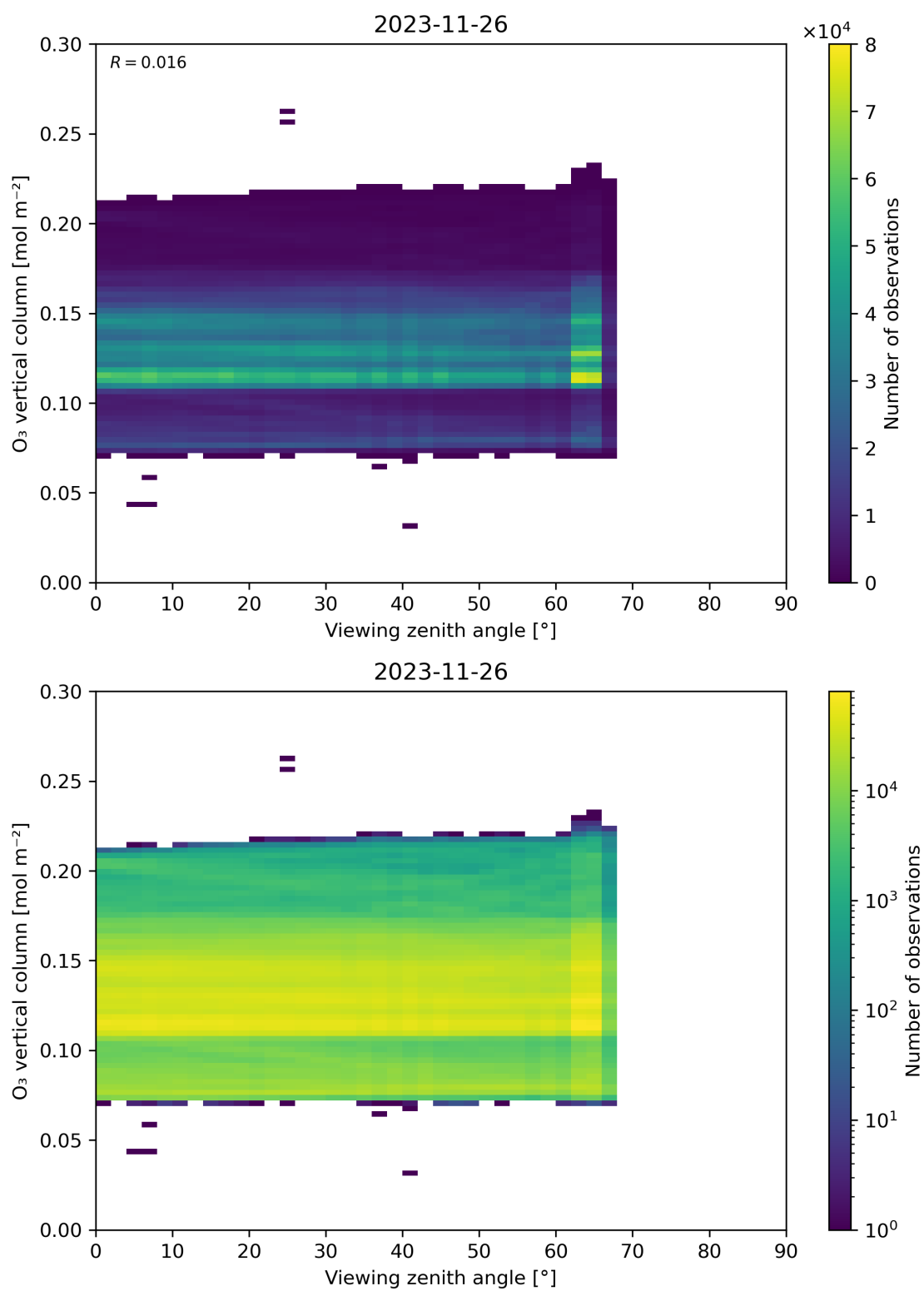
Figure 52: Scatter density plot of “Viewing zenith angle” against “O 3 vertical column” for 2023-11-25 to 2023-11-27.
