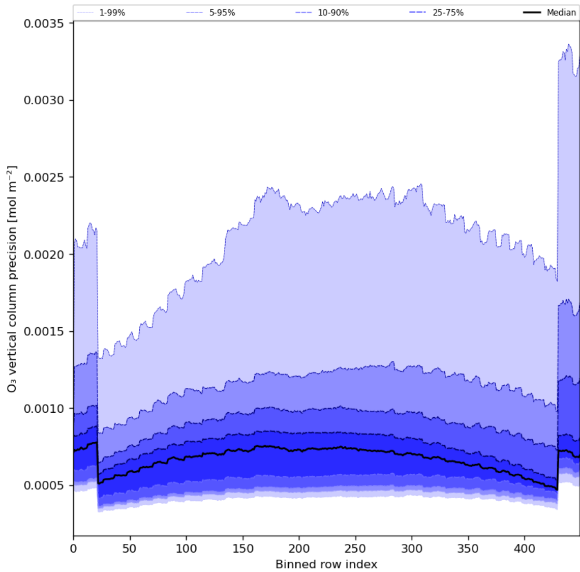
Figure 29: Along track statistics of “O 3 vertical column precision” for 2023-11-25 to 2023-11-27
