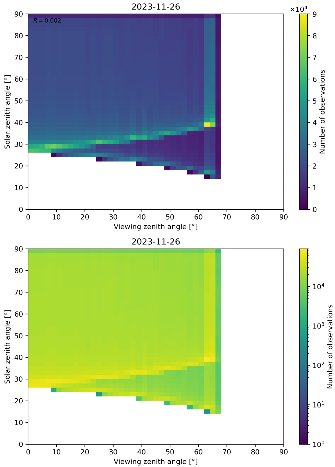
Figure 54: Scatter density plot of “Viewing zenith angle” against “Solar zenith angle” for 2023-11-25 to 2023-11-27.
