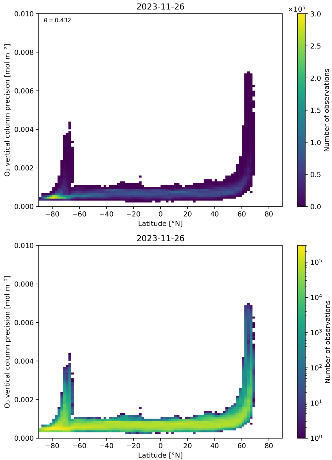
Figure 37: Scatter density plot of “Latitude” against “O 3 vertical column precision” for 2023-11-25 to 2023-11-27.
