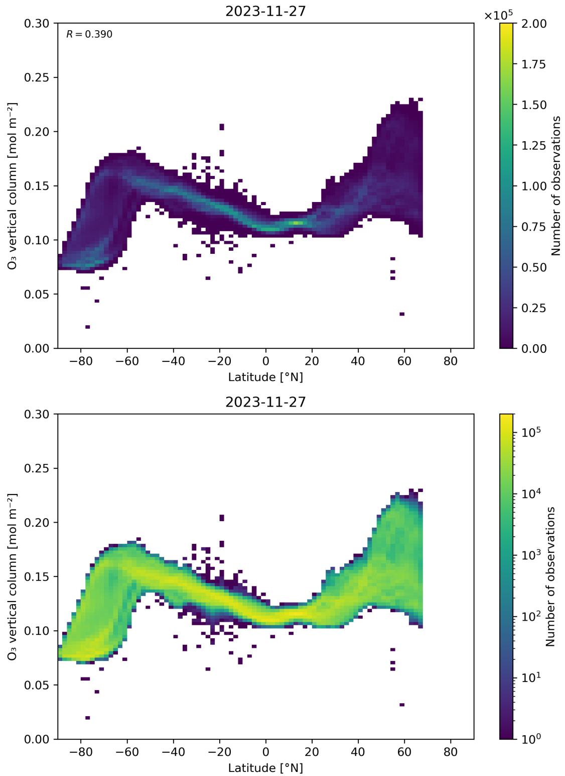
Figure 36: Scatter density plot of “Latitude” against “O 3 vertical column” for 2023-11-26 to 2023-11-28.
