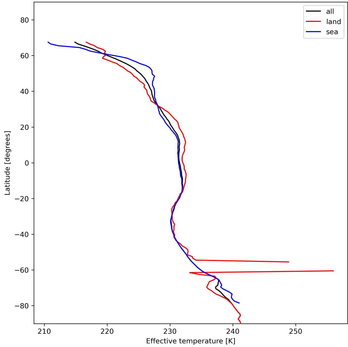
Figure 17: Zonal average of “Effective temperature” for 2023-11-26 to 2023-11-28.
