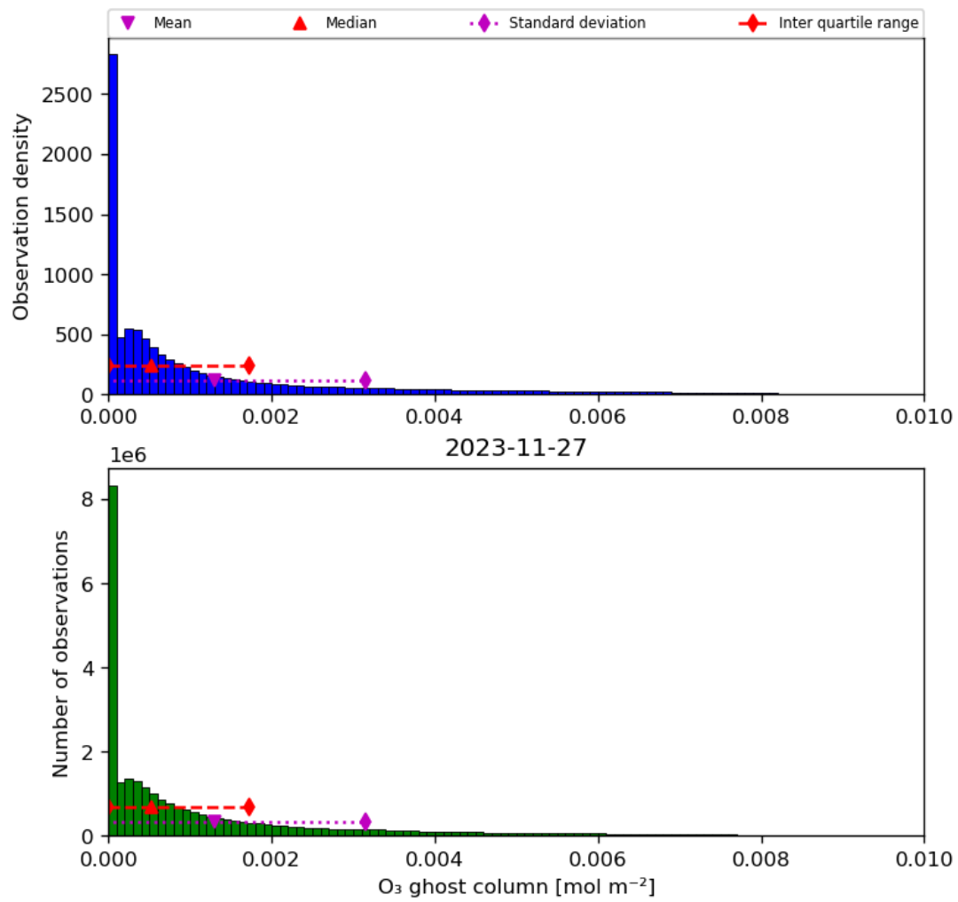
Figure 25: Histogram of “O 3 ghost column” for 2023-11-26 to 2023-11-28
