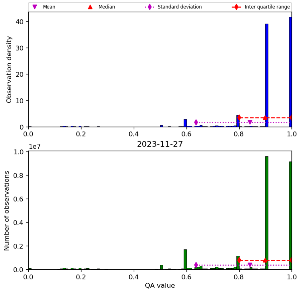
Figure 20: Histogram of “QA value” for 2023-11-26 to 2023-11-28
