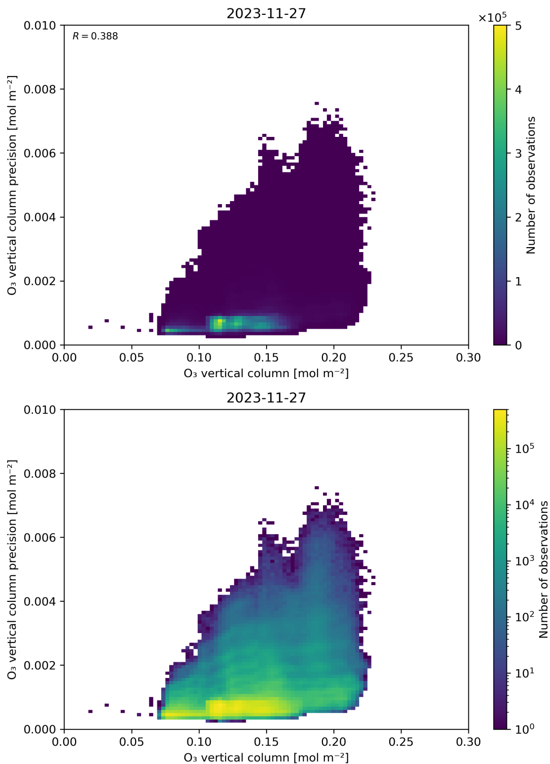
Figure 41: Scatter density plot of “O 3 vertical column” against “O 3 vertical column precision” for 2023-11-26 to 2023-11-28.
