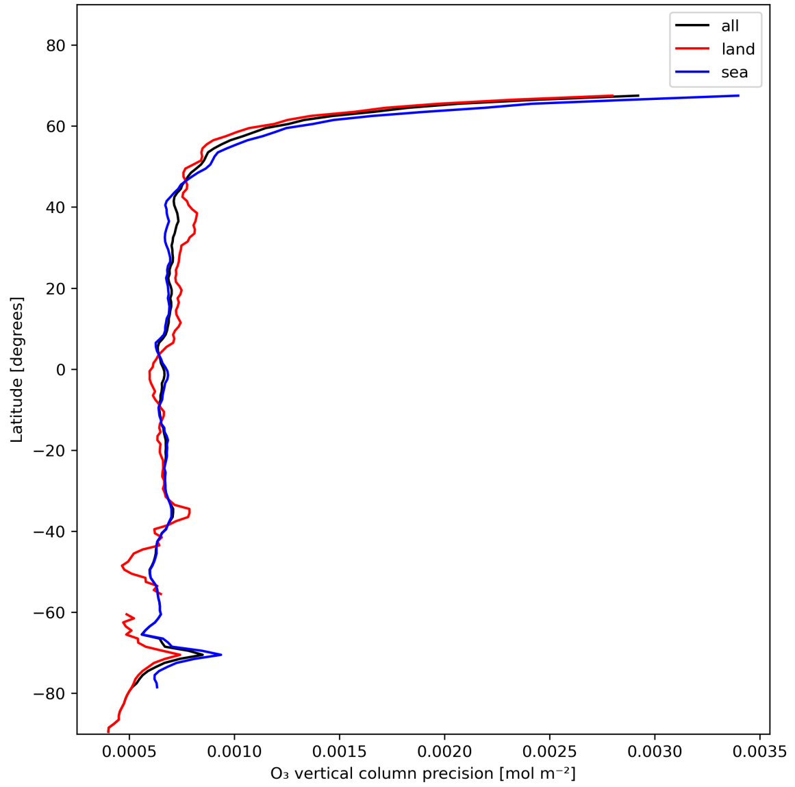
Figure 15: Zonal average of “O 3 vertical column precision” for 2023-11-26 to 2023-11-28.
