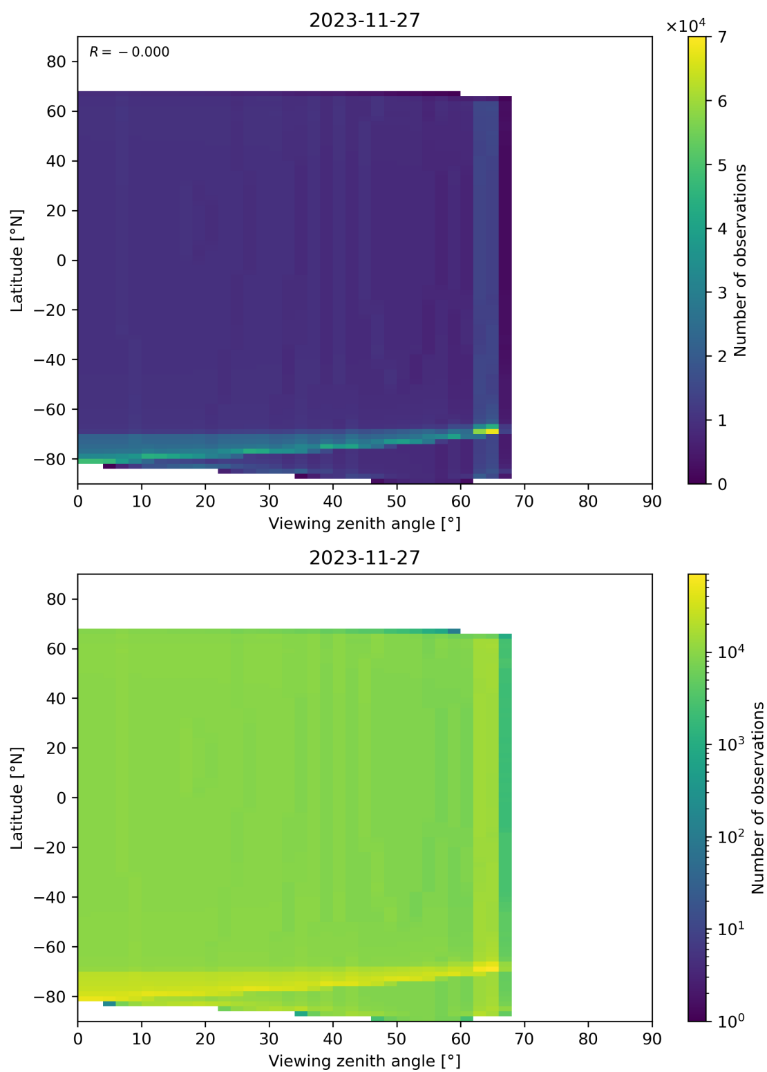
Figure 49: Scatter density plot of “Viewing zenith angle” against “Latitude” for 2023-11-26 to 2023-11-28.
