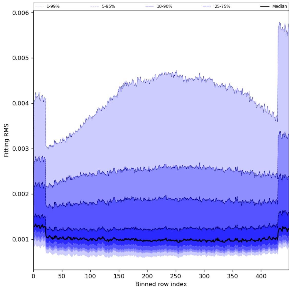
Figure 30: Along track statistics of “Fitting RMS” for 2023-11-26 to 2023-11-28
