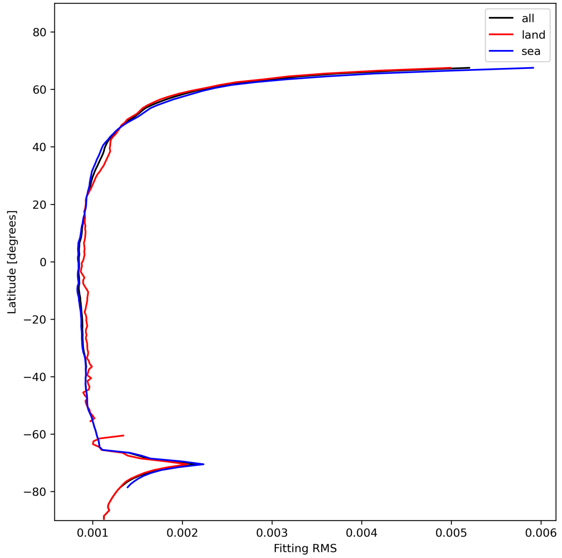
Figure 16: Zonal average of “Fitting RMS” for 2023-11-26 to 2023-11-28.
