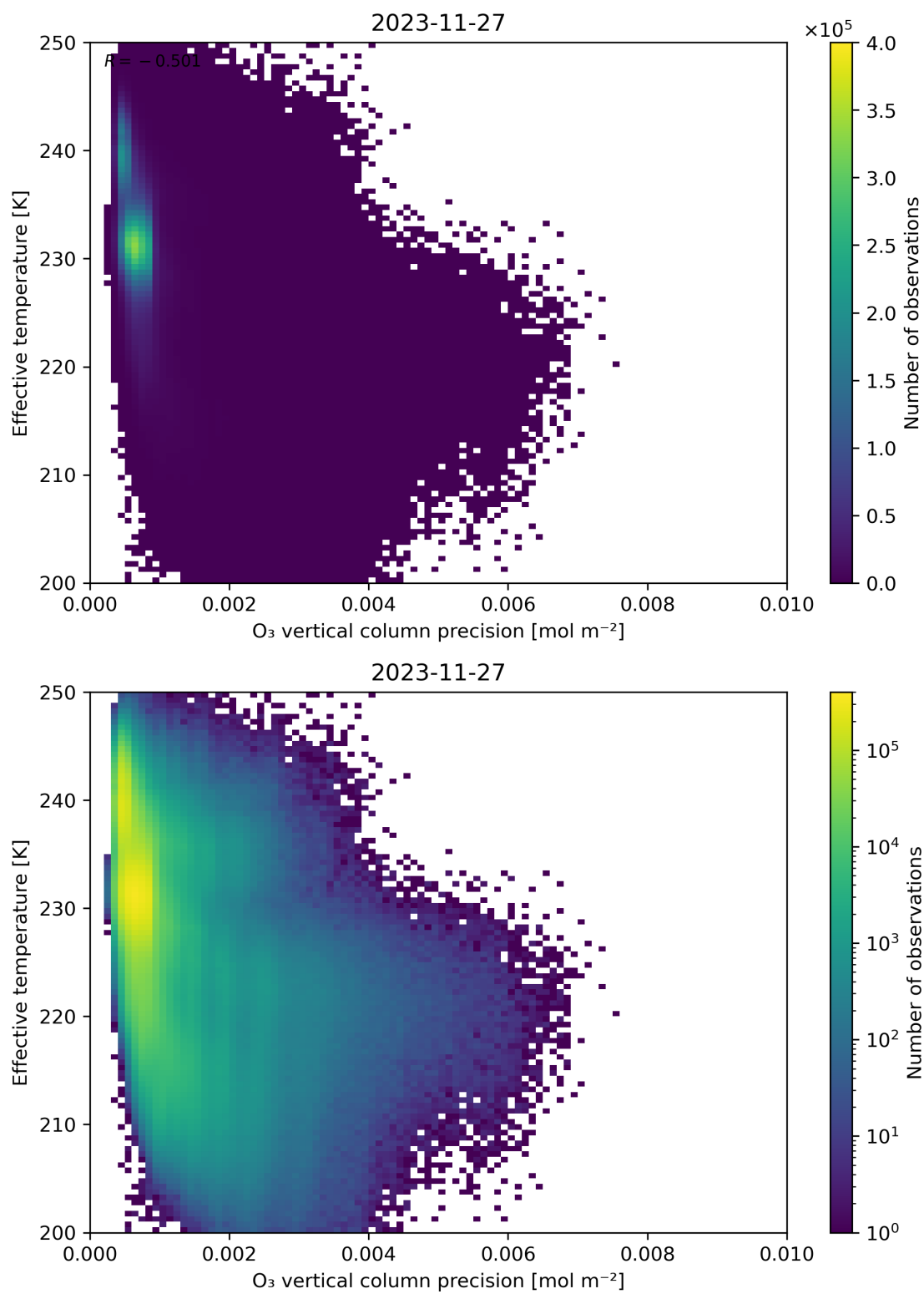
Figure 42: Scatter density plot of “O 3 vertical column precision” against “Effective temperature” for 2023-11-26 to 2023-11-28.
