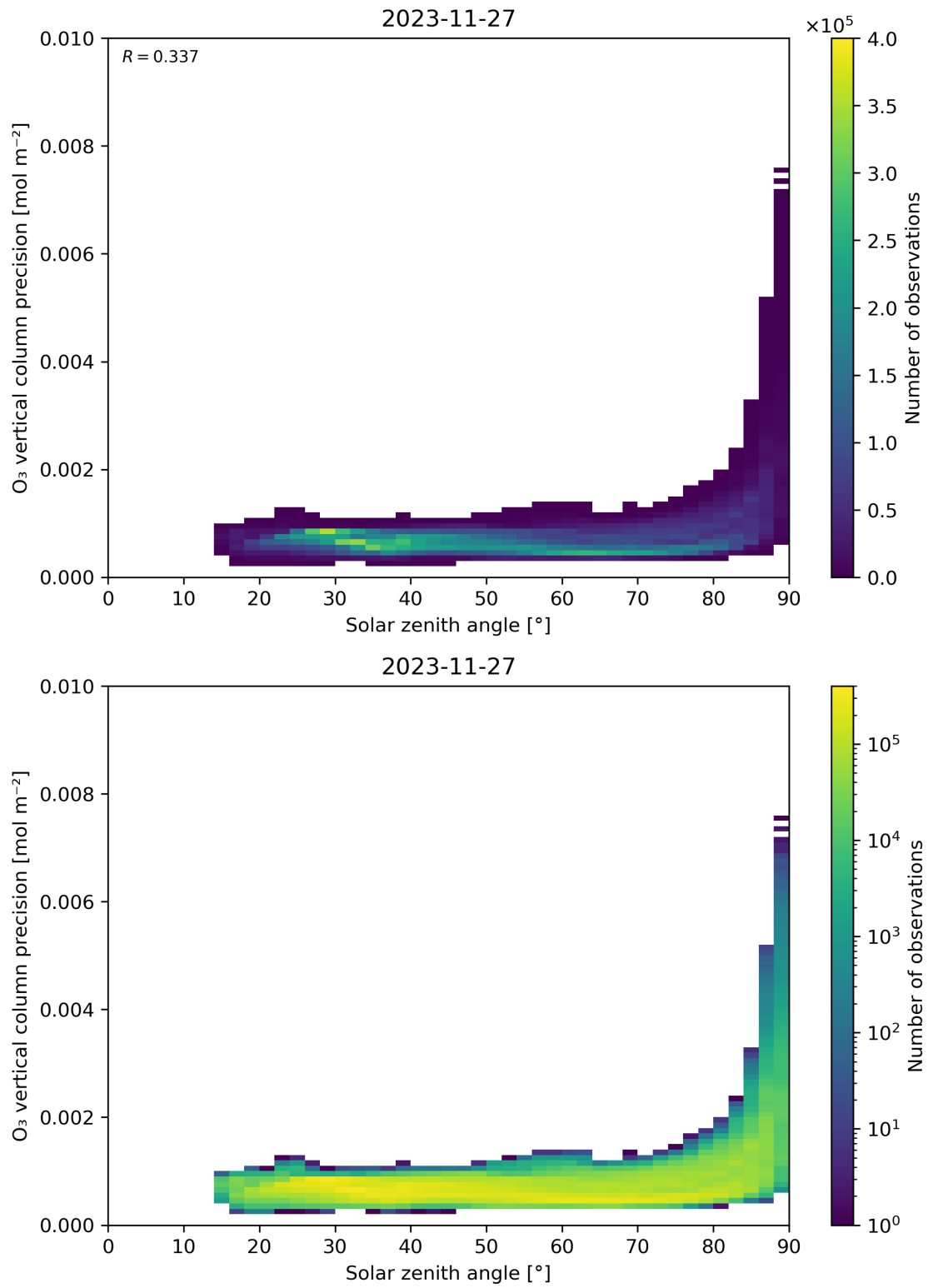
Figure 48: Scatter density plot of “Solar zenith angle” against “O 3 vertical column precision” for 2023-11-26 to 2023-11-28.
