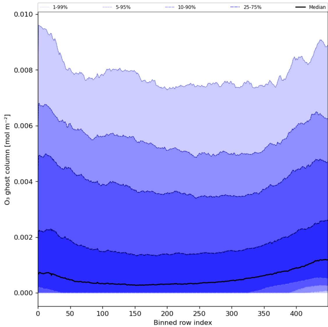
Figure 32: Along track statistics of “O 3 ghost column” for 2023-11-26 to 2023-11-28
