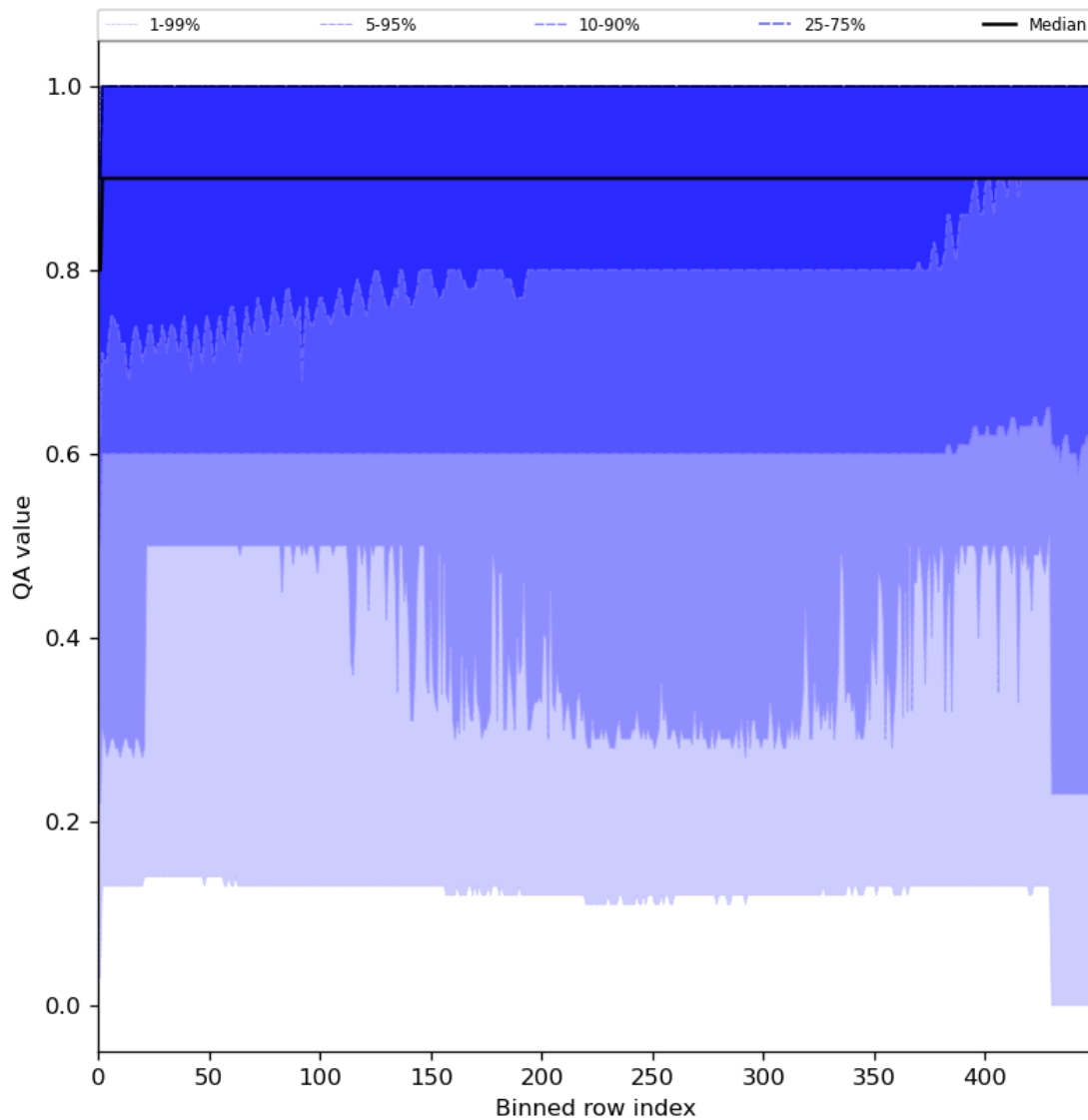
Figure 27: Along track statistics of “QA value” for 2023-11-26 to 2023-11-28
