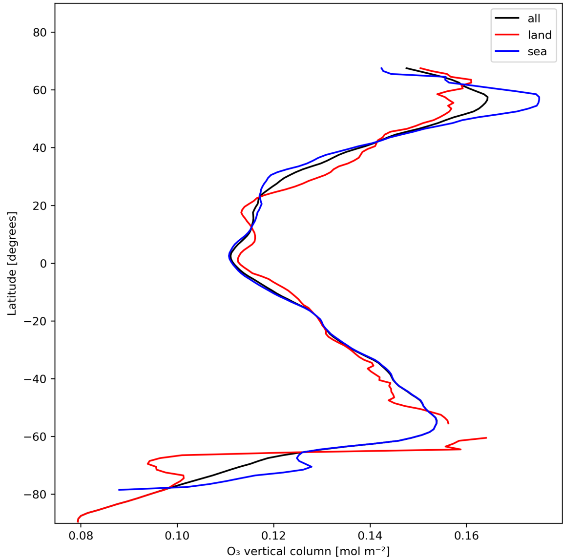
Figure 14: Zonal average of “O 3 vertical column” for 2023-11-26 to 2023-11-28.
