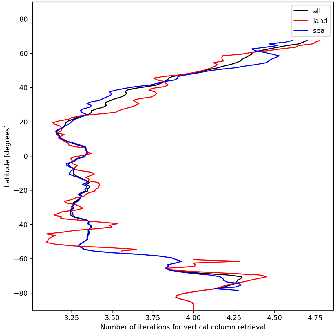
Figure 19: Zonal average of “Number of iterations for vertical column retrieval” for 2023-11-26 to 2023-11-28.
