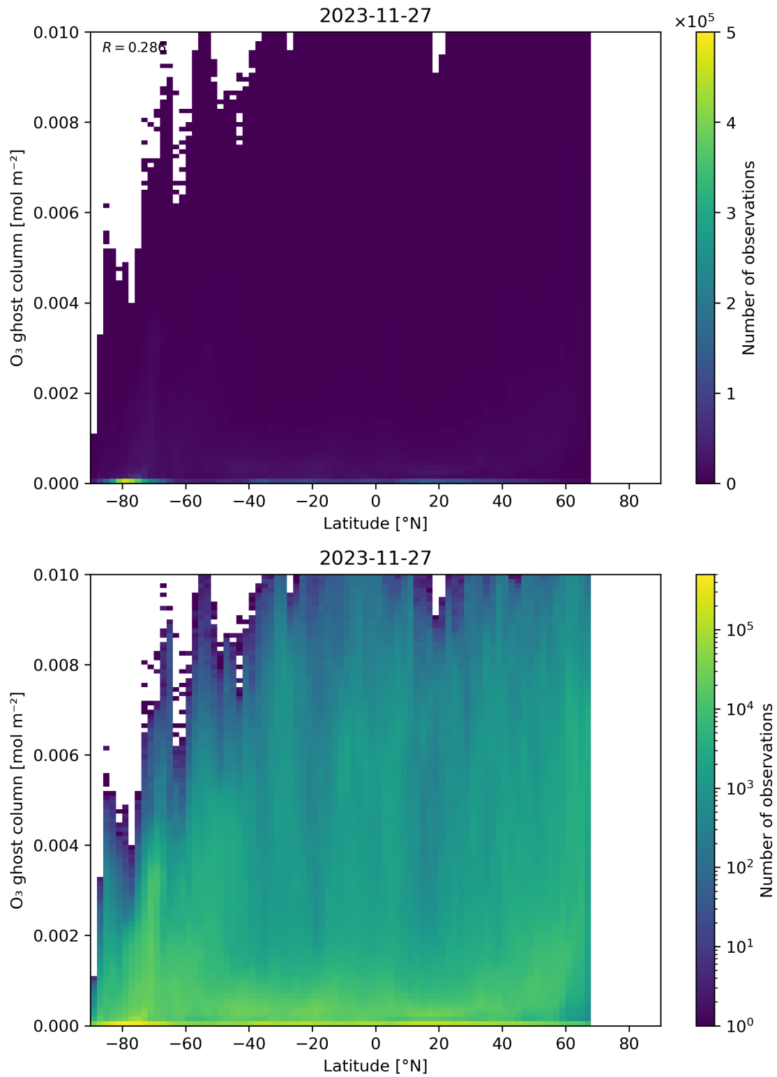
Figure 35: Scatter density plot of “Latitude” against “O 3 ghost column” for 2023-11-26 to 2023-11-28.
