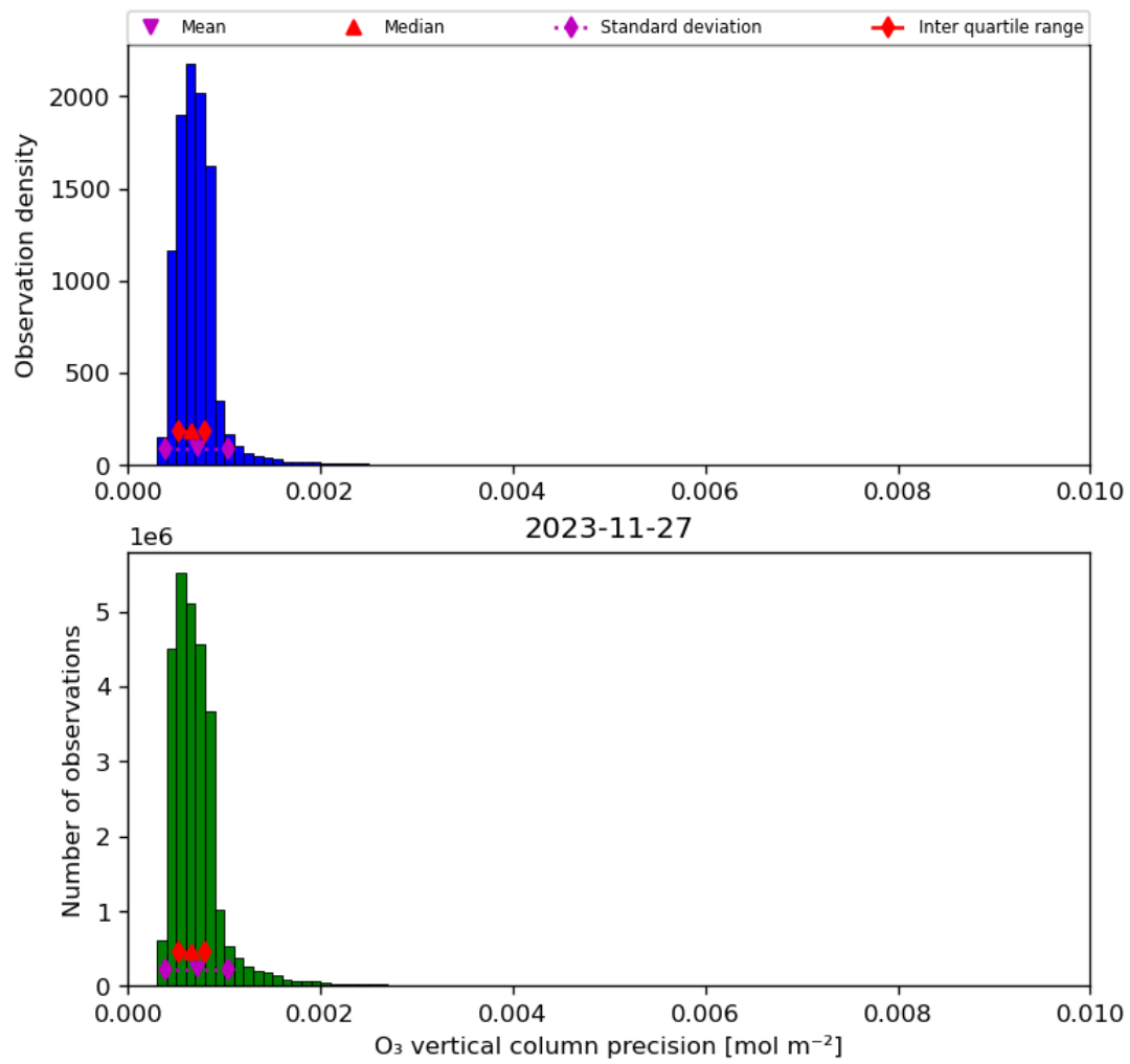
Figure 22: Histogram of “O 3 vertical column precision” for 2023-11-26 to 2023-11-28
