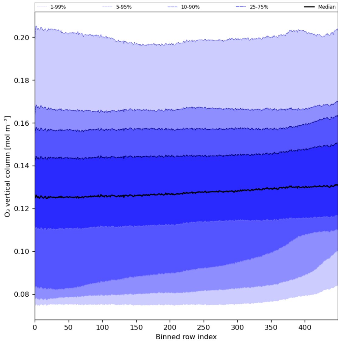
Figure 28: Along track statistics of "O 3 vertical column" for 2023-11-26 to 2023-11-28
