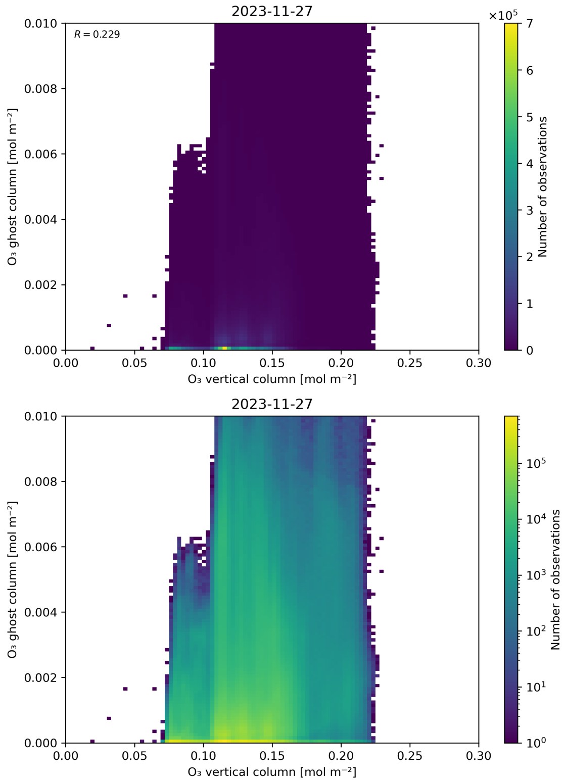
Figure 40: Scatter density plot of “O 3 vertical column” against “O 3 ghost column” for 2023-11-26 to 2023-11-28.
