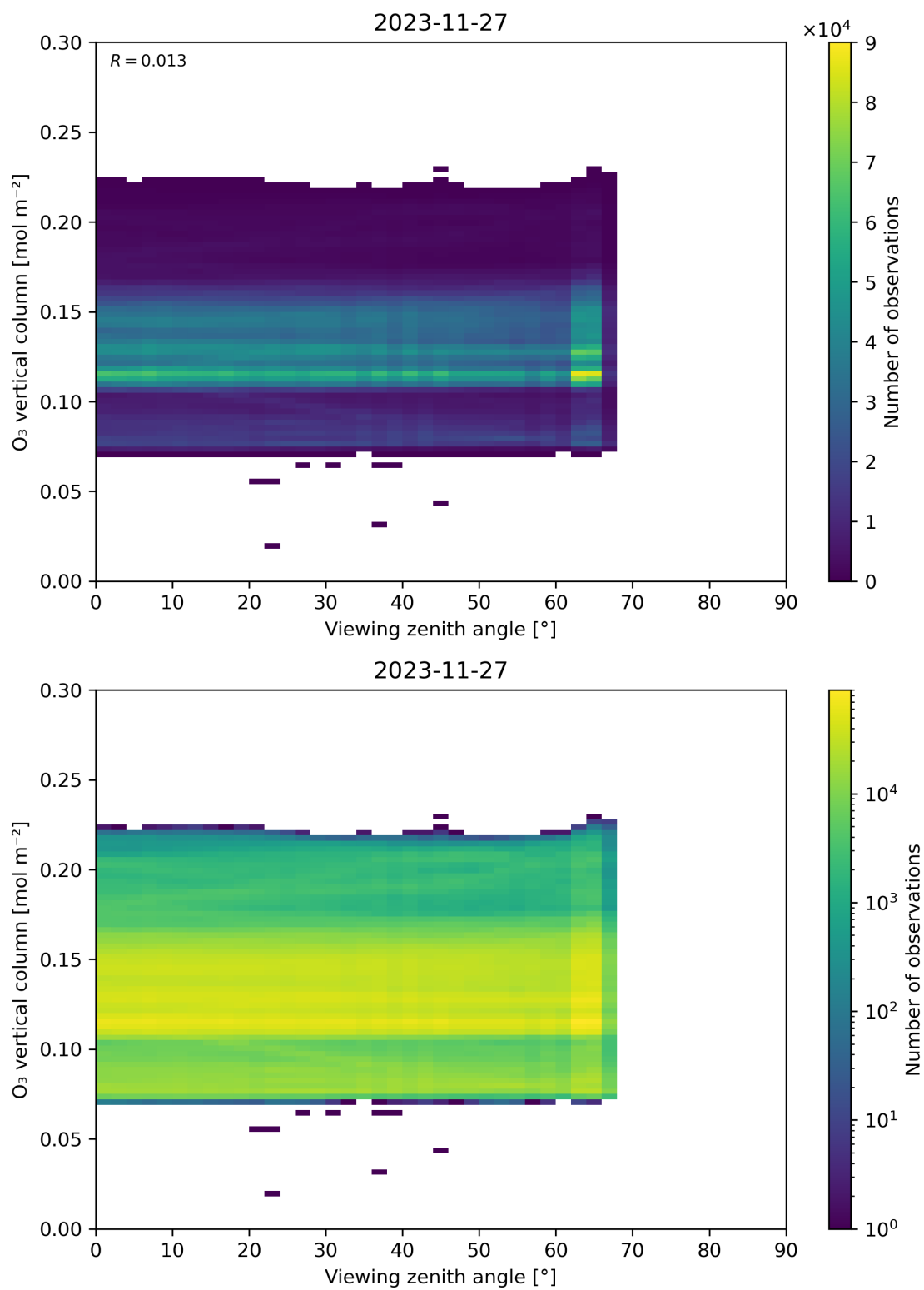
Figure 52: Scatter density plot of “Viewing zenith angle” against “O 3 vertical column” for 2023-11-26 to 2023-11-28.
