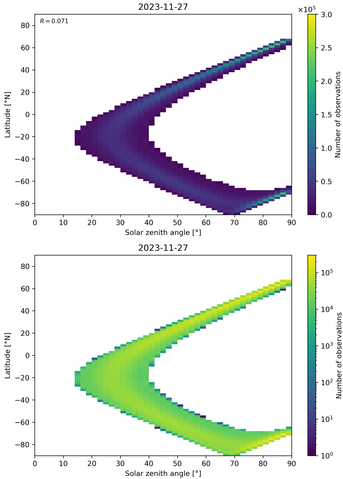
Figure 44: Scatter density plot of “Solar zenith angle” against “Latitude” for 2023-11-26 to 2023-11-28.
