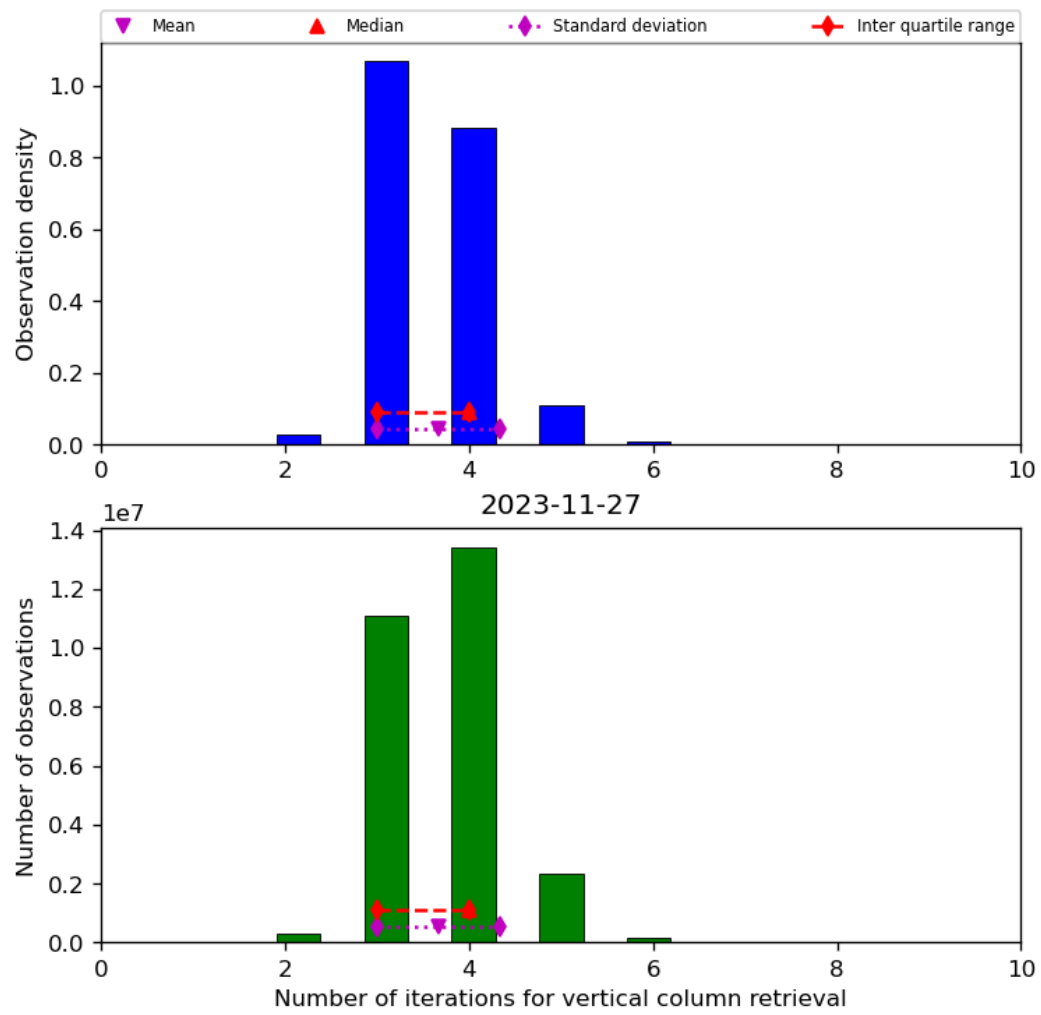
Figure 26: Histogram of “Number of iterations for vertical column retrieval” for 2023-11-26 to 2023-11-28
