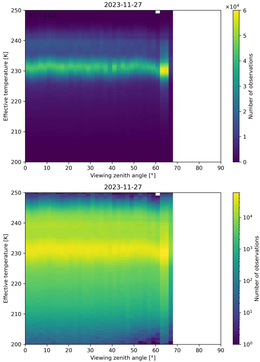
Figure 50: Scatter density plot of “Viewing zenith angle” against “Effective temperature” for 2023-11-26 to 2023-11-28.
