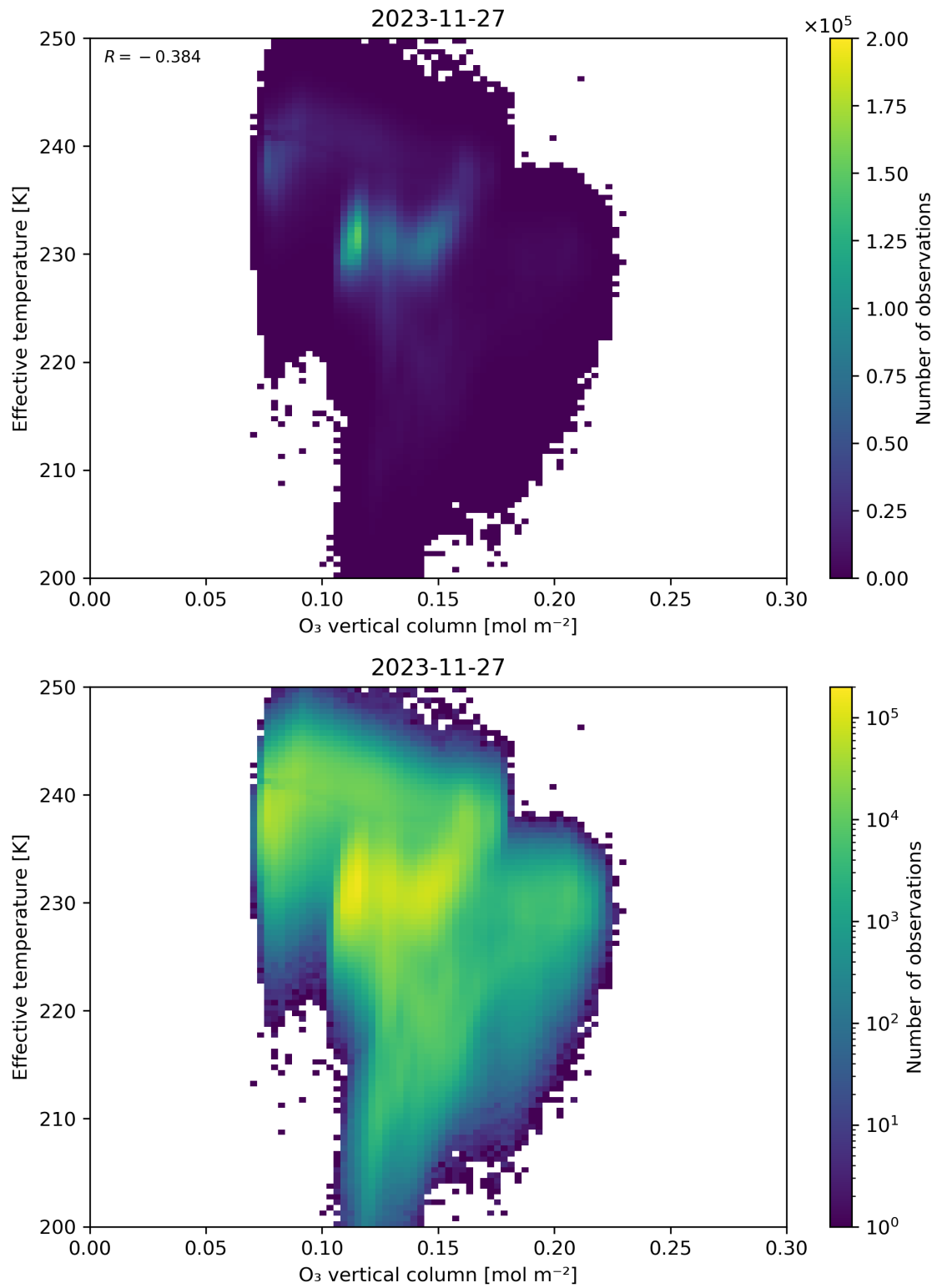
Figure 39: Scatter density plot of “O 3 vertical column” against “Effective temperature” for 2023-11-26 to 2023-11-28.
