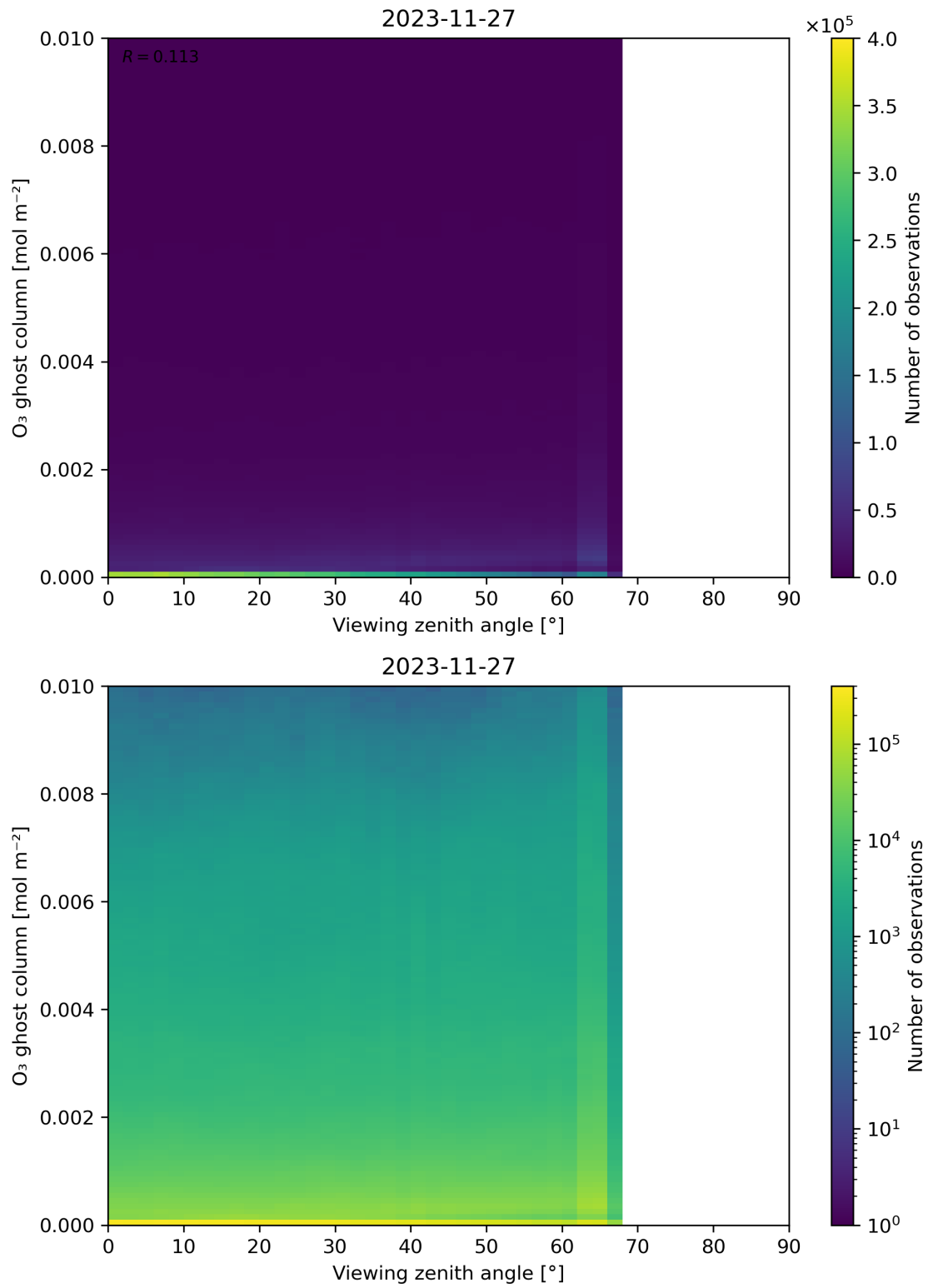
Figure 51: Scatter density plot of “Viewing zenith angle” against “O 3 ghost column” for 2023-11-26 to 2023-11-28.
