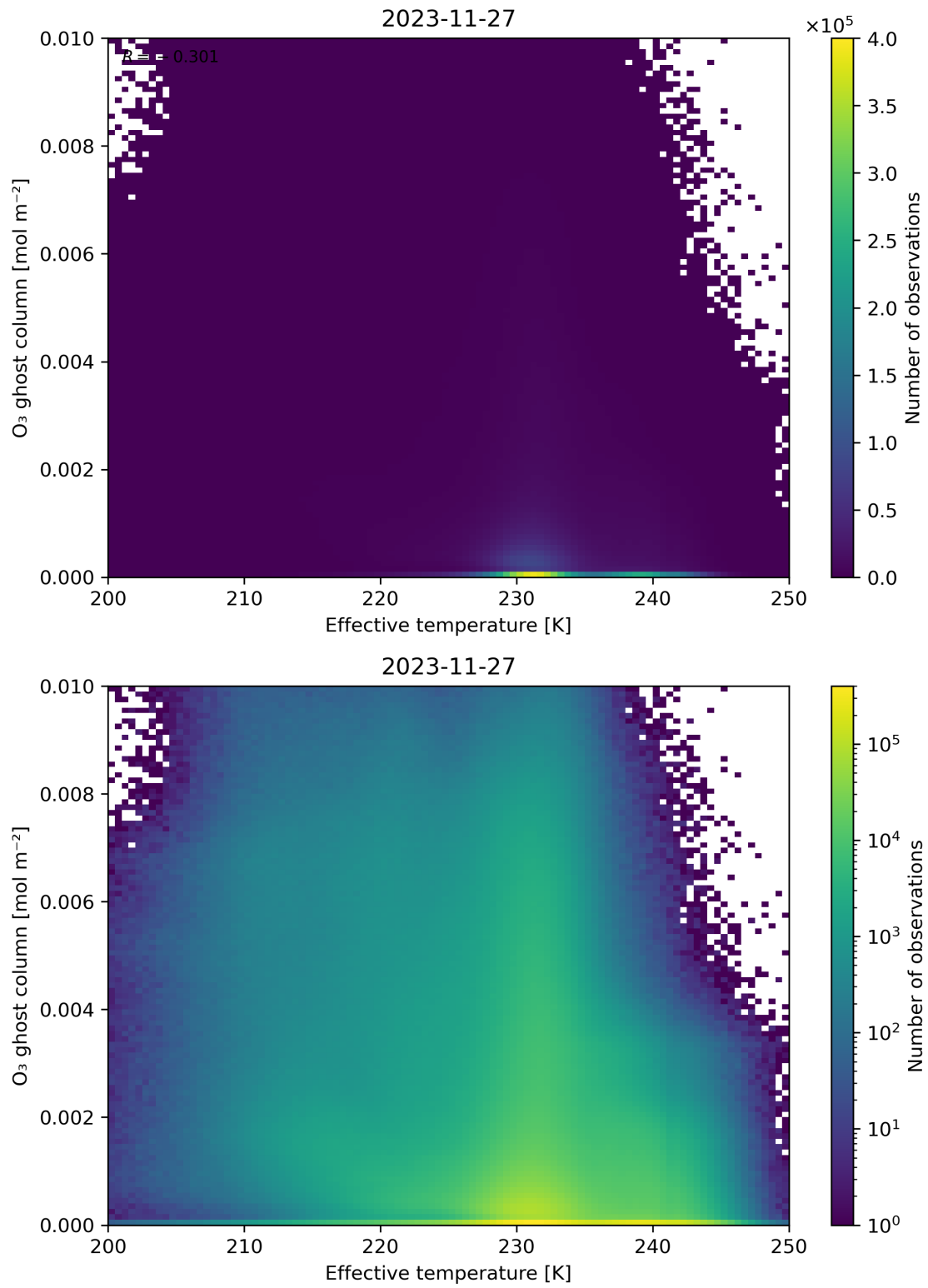
Figure 38: Scatter density plot of “Effective temperature” against “O 3 ghost column” for 2023-11-26 to 2023-11-28.
