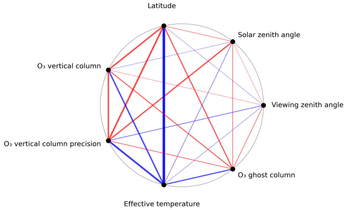
Figure 1: Map of correlation graph for 2023-11-26 to 2023-11-28.
