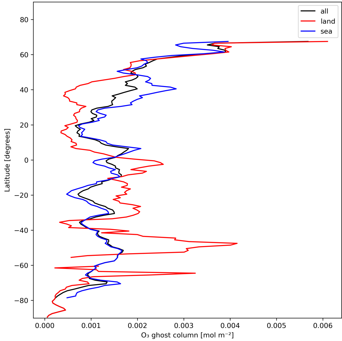
Figure 18: Zonal average of "O 3 ghost column" for 2023-11-26 to 2023-11-28.
