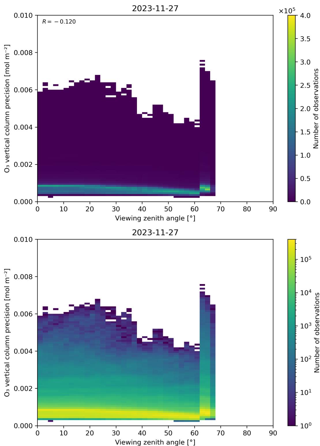
Figure 53: Scatter density plot of “Viewing zenith angle” against “O 3 vertical column precision” for 2023-11-26 to 2023-11-28.
