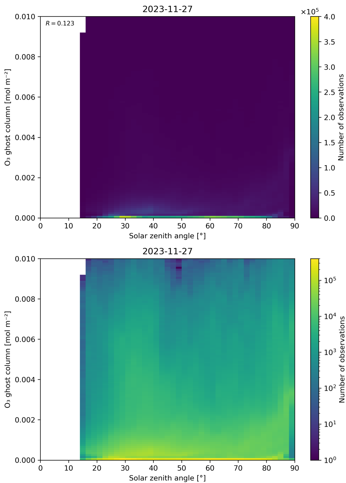
Figure 46: Scatter density plot of “Solar zenith angle” against “O 3 ghost column” for 2023-11-26 to 2023-11-28.
