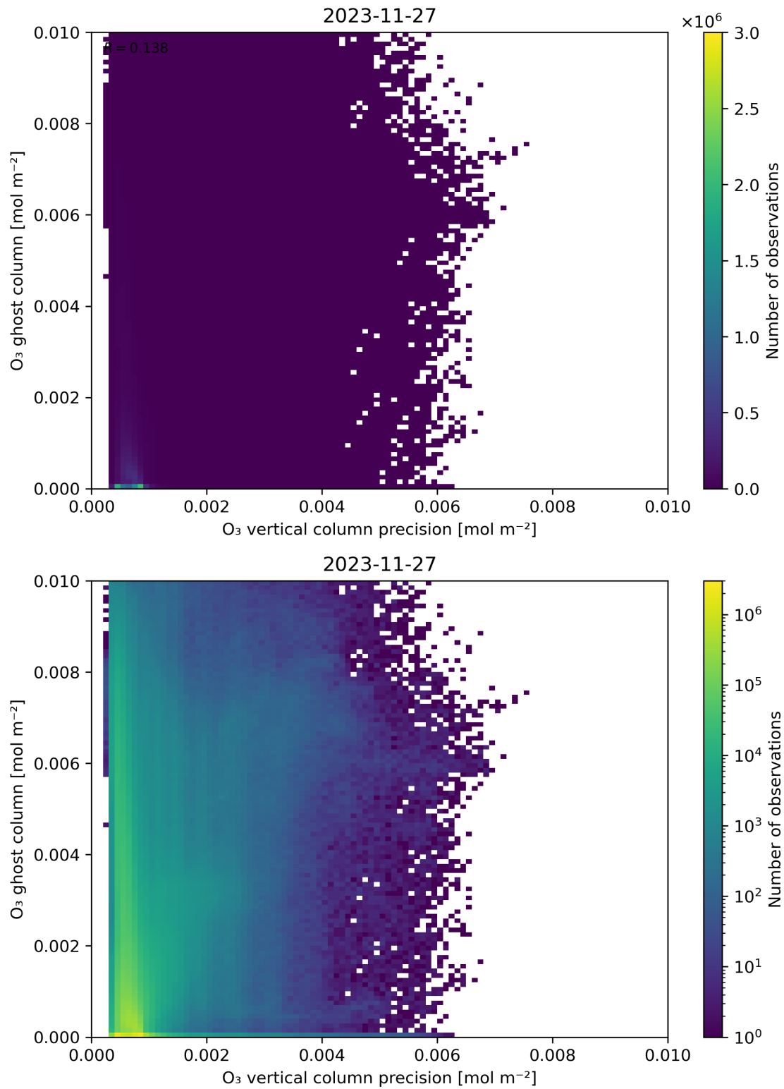
Figure 43: Scatter density plot of “O 3 vertical column precision” against “O 3 ghost column” for 2023-11-26 to 2023-11-28.
