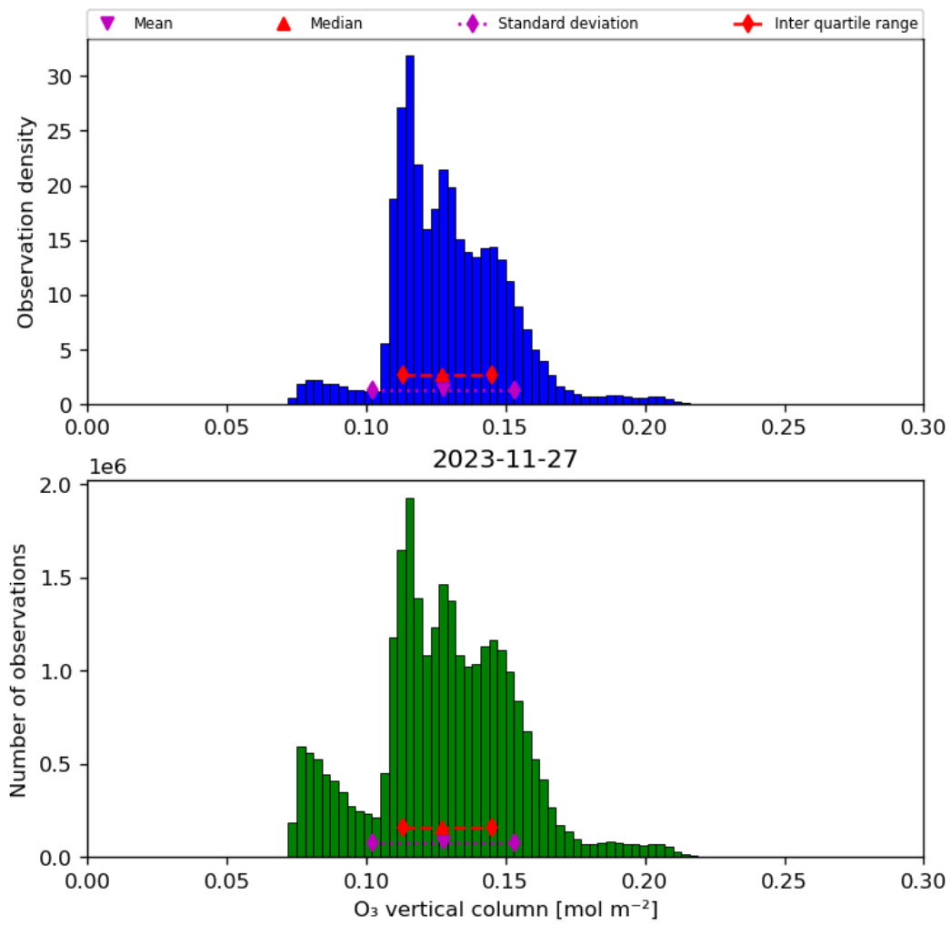
Figure 21: Histogram of “O 3 vertical column” for 2023-11-26 to 2023-11-28
