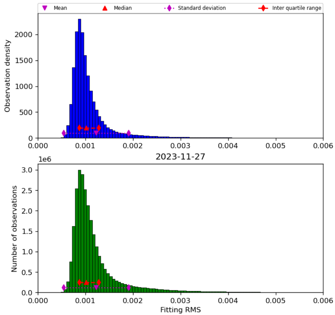
Figure 23: Histogram of “Fitting RMS” for 2023-11-26 to 2023-11-28
