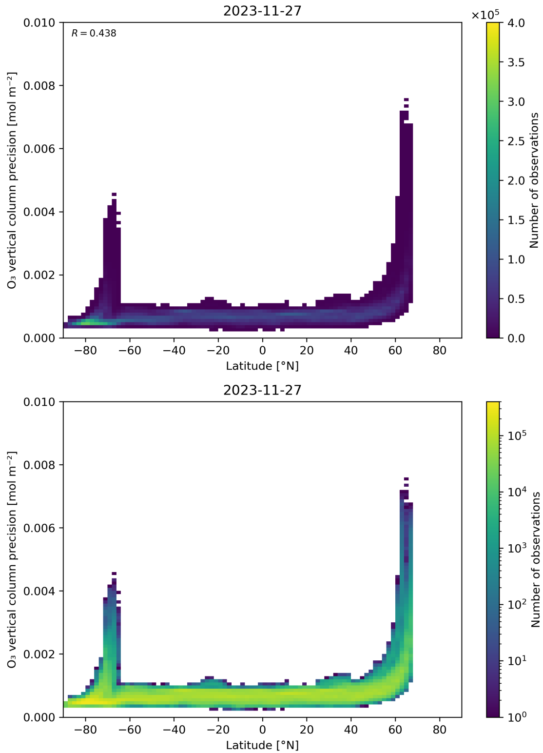
Figure 37: Scatter density plot of “Latitude” against “O 3 vertical column precision” for 2023-11-26 to 2023-11-28.
