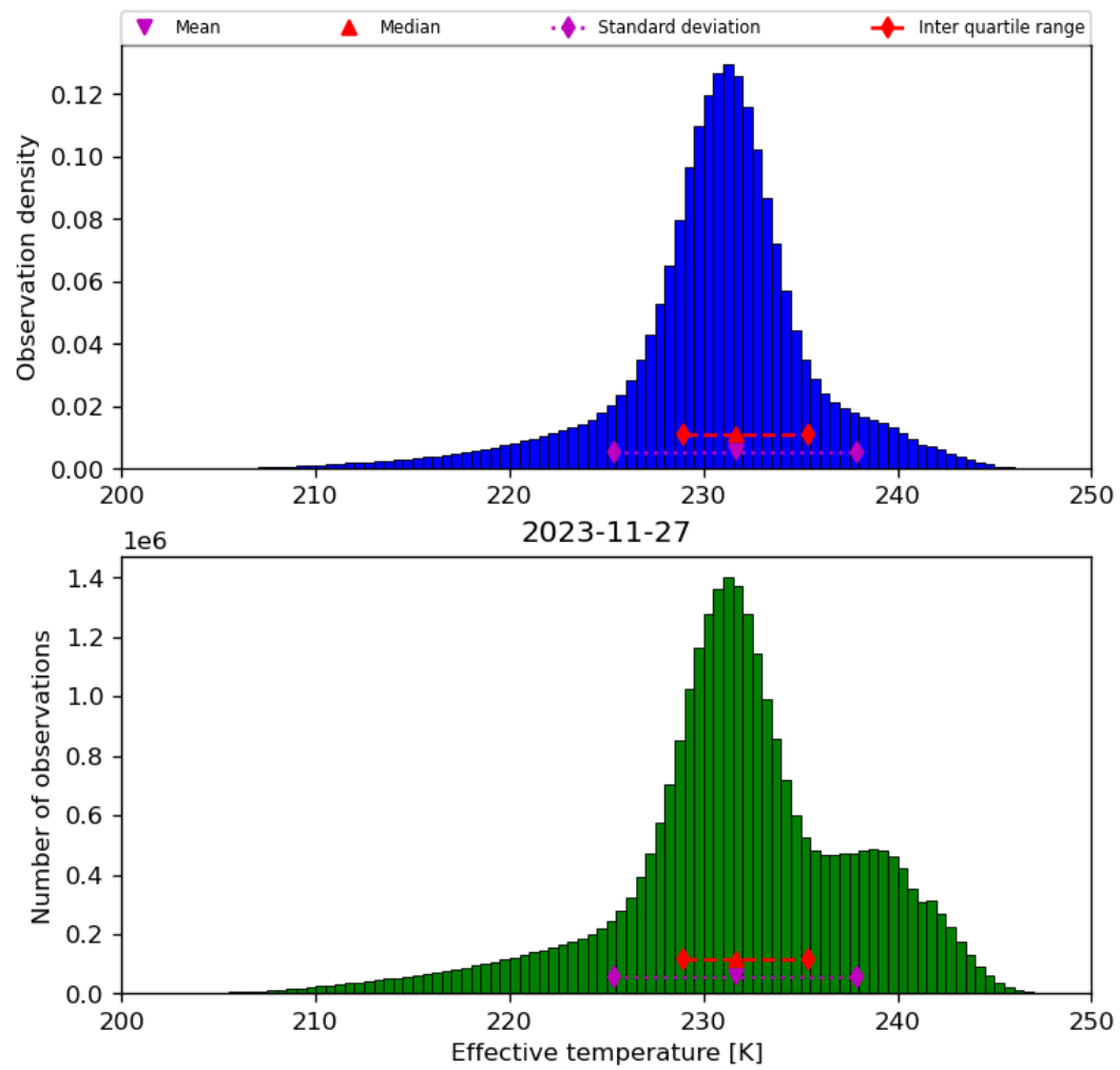
Figure 24: Histogram of “Effective temperature” for 2023-11-26 to 2023-11-28
