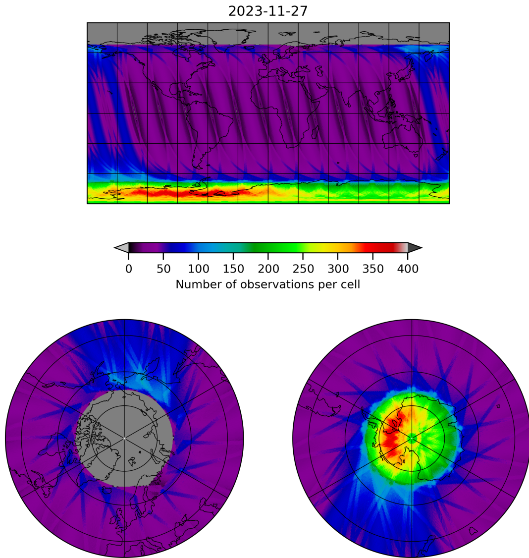
Figure 12: Map of the number of observations for 2023-11-26 to 2023-11-28
