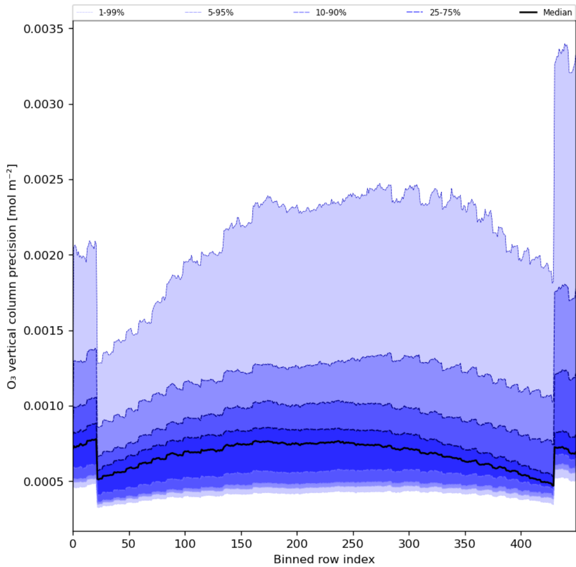
Figure 29: Along track statistics of “O 3 vertical column precision” for 2023-11-26 to 2023-11-28
