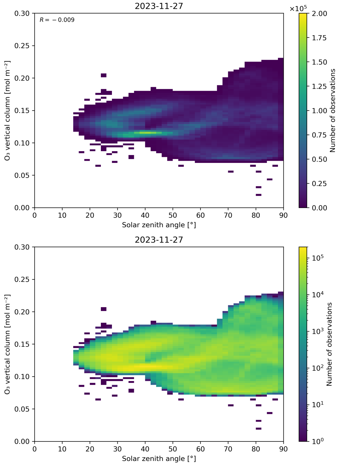
Figure 47: Scatter density plot of “Solar zenith angle” against “O 3 vertical column” for 2023-11-26 to 2023-11-28.
