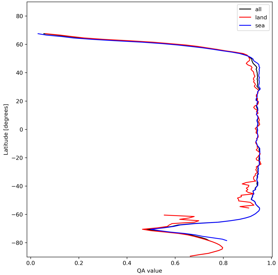
Figure 13: Zonal average of “QA value” for 2023-11-26 to 2023-11-28.
