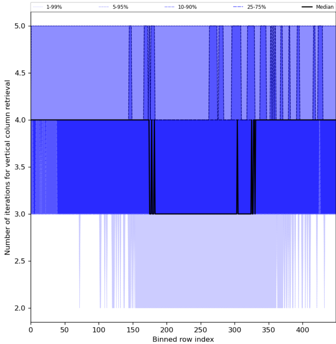
Figure 33: Along track statistics of “Number of iterations for vertical column retrieval” for 2023-11-26 to 2023-11-28
