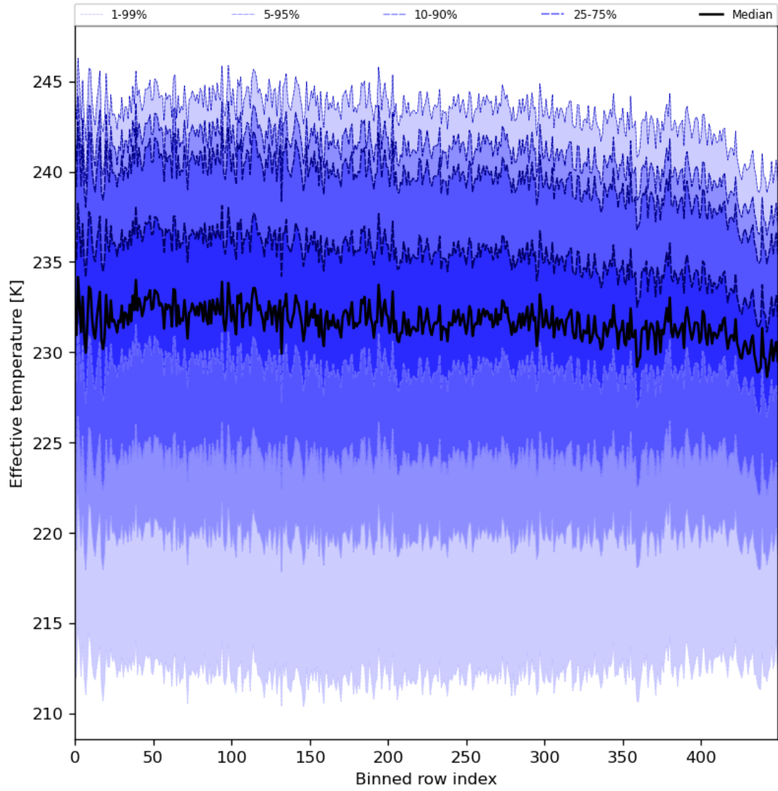
Figure 31: Along track statistics of “Effective temperature” for 2023-11-26 to 2023-11-28
