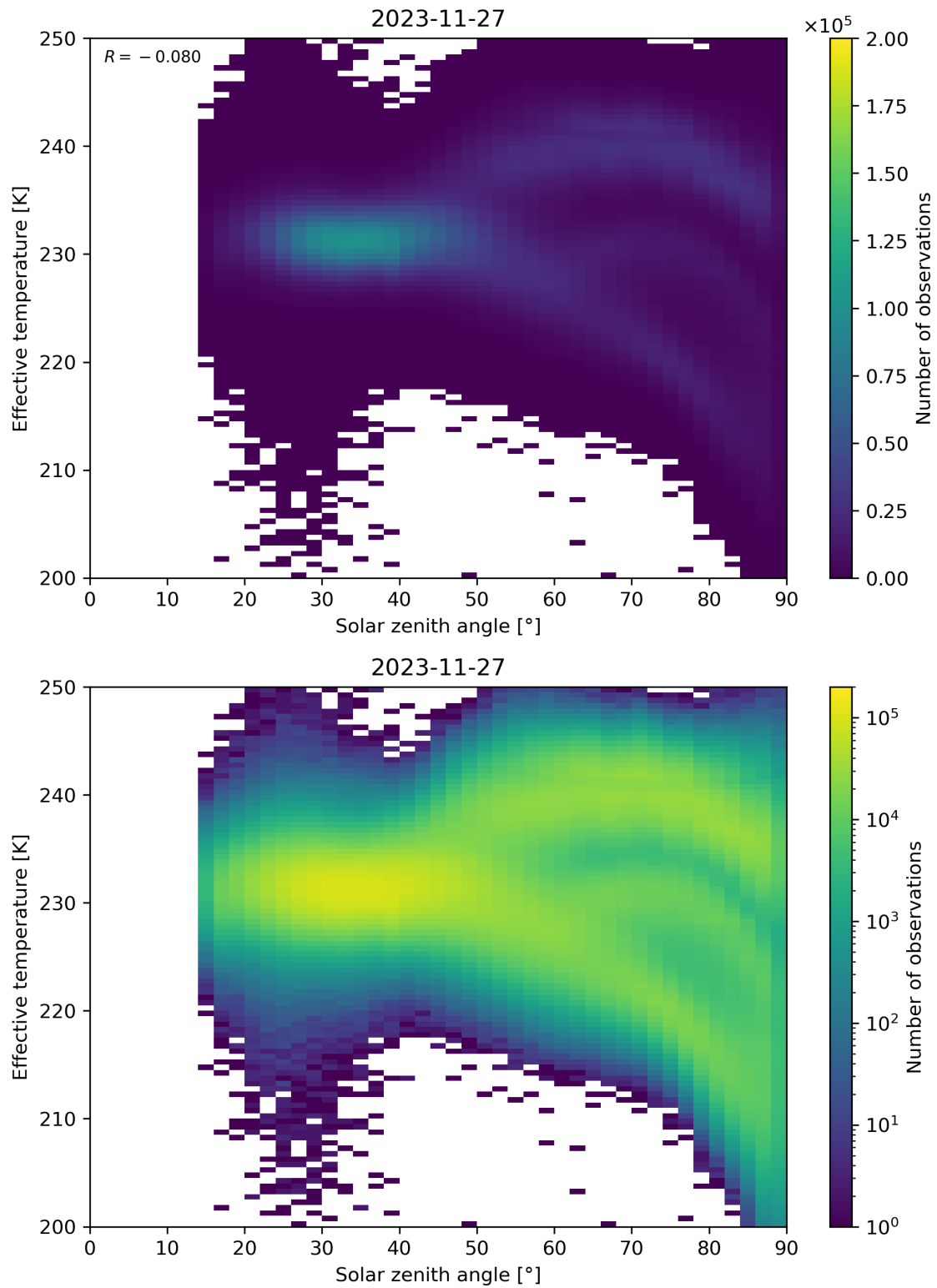
Figure 45: Scatter density plot of “Solar zenith angle” against “Effective temperature” for 2023-11-26 to 2023-11-28.
