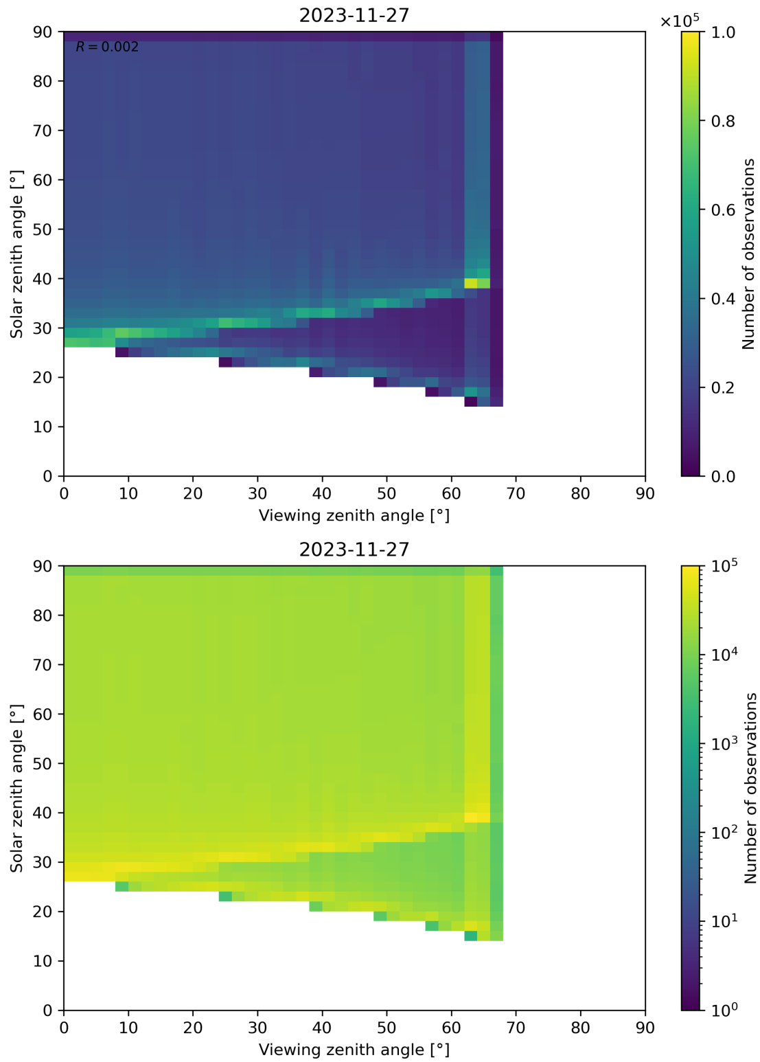
Figure 54: Scatter density plot of “Viewing zenith angle” against “Solar zenith angle” for 2023-11-26 to 2023-11-28.
