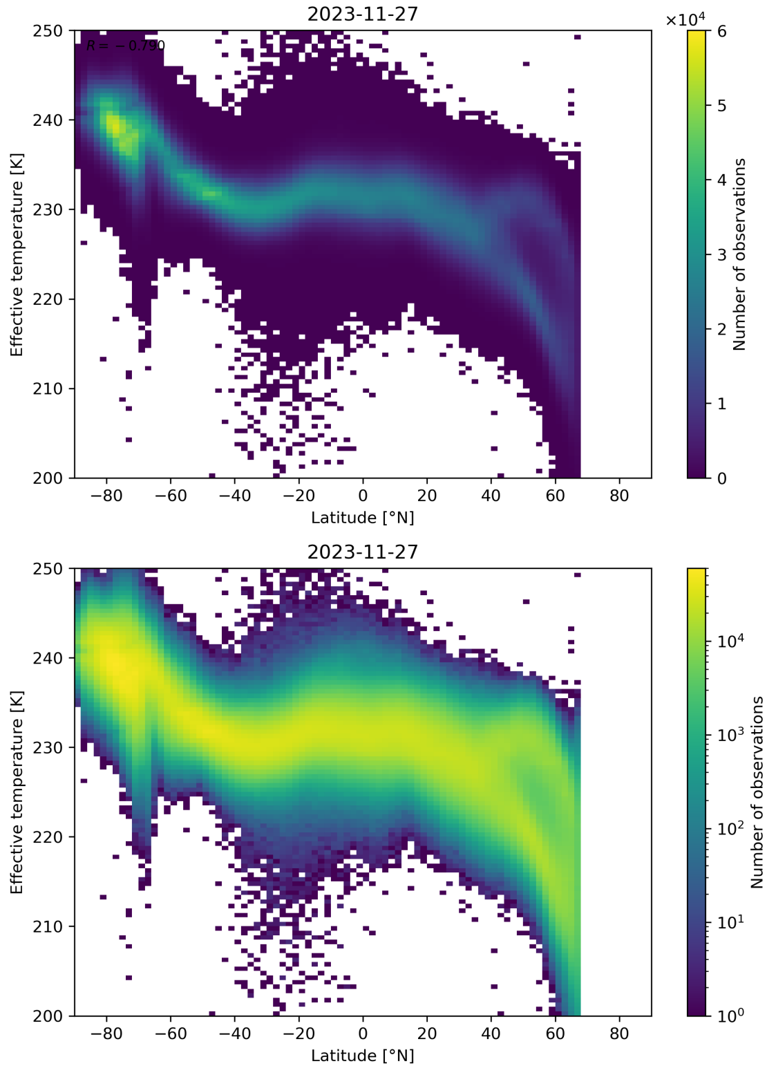
Figure 34: Scatter density plot of “Latitude” against “Effective temperature” for 2023-11-26 to 2023-11-28.
