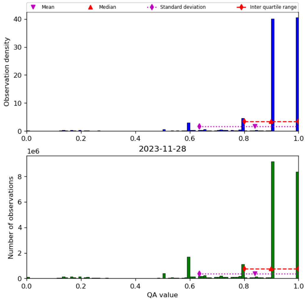
Figure 20: Histogram of “QA value” for 2023-11-28 to 2023-11-29
