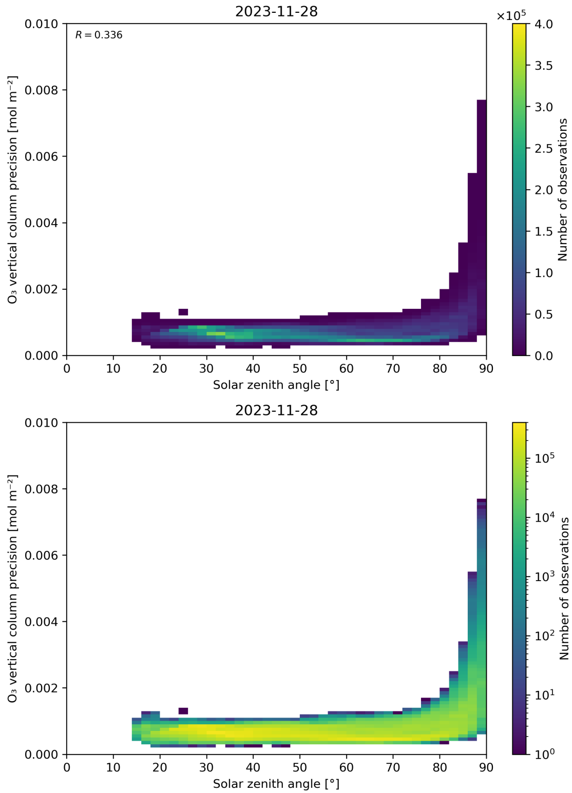
Figure 48: Scatter density plot of “Solar zenith angle” against “O 3 vertical column precision” for 2023-11-28 to 2023-11-29.
