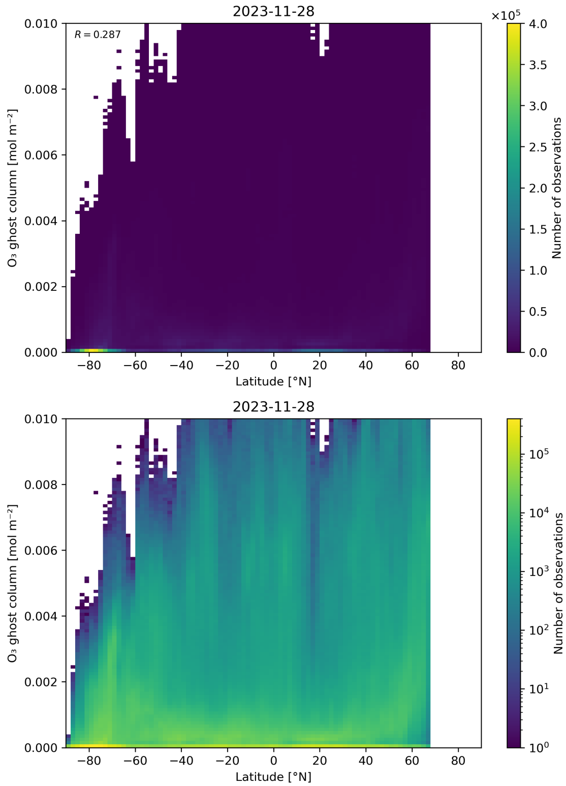
Figure 35: Scatter density plot of “Latitude” against “O 3 ghost column” for 2023-11-28 to 2023-11-29.
