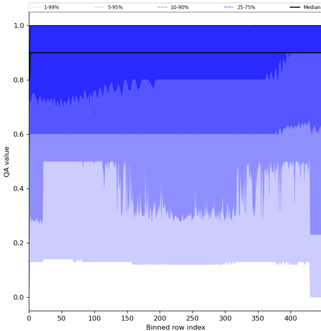
Figure 27: Along track statistics of “QA value” for 2023-11-28 to 2023-11-29
