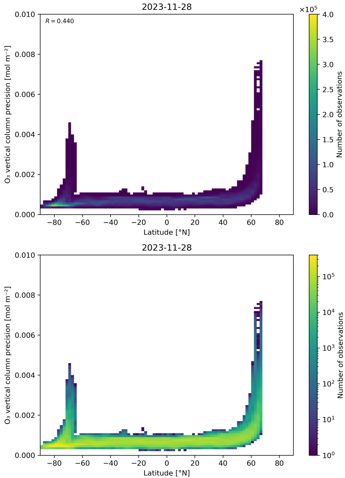
Figure 37: Scatter density plot of “Latitude” against “O 3 vertical column precision” for 2023-11-28 to 2023-11-29.
