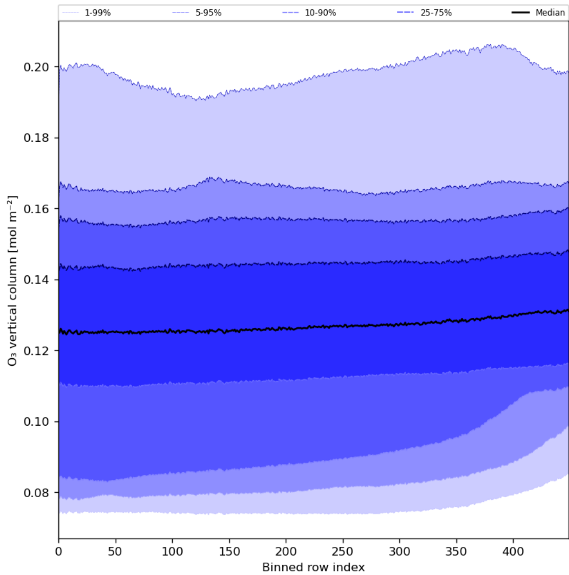
Figure 28: Along track statistics of “ O_3 vertical column” for 2023-11-28 to 2023-11-29
