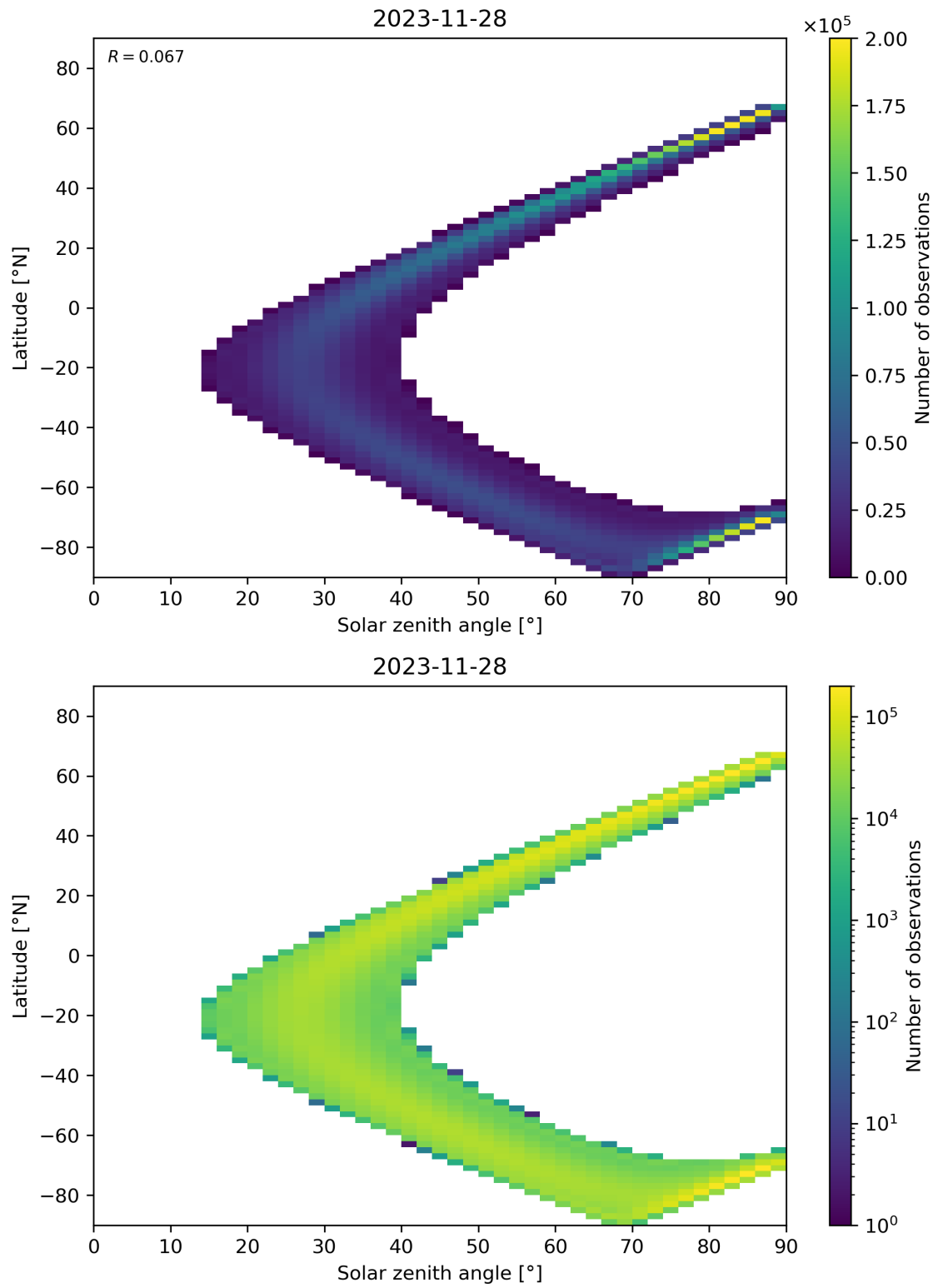
Figure 44: Scatter density plot of “Solar zenith angle” against “Latitude” for 2023-11-28 to 2023-11-29.
