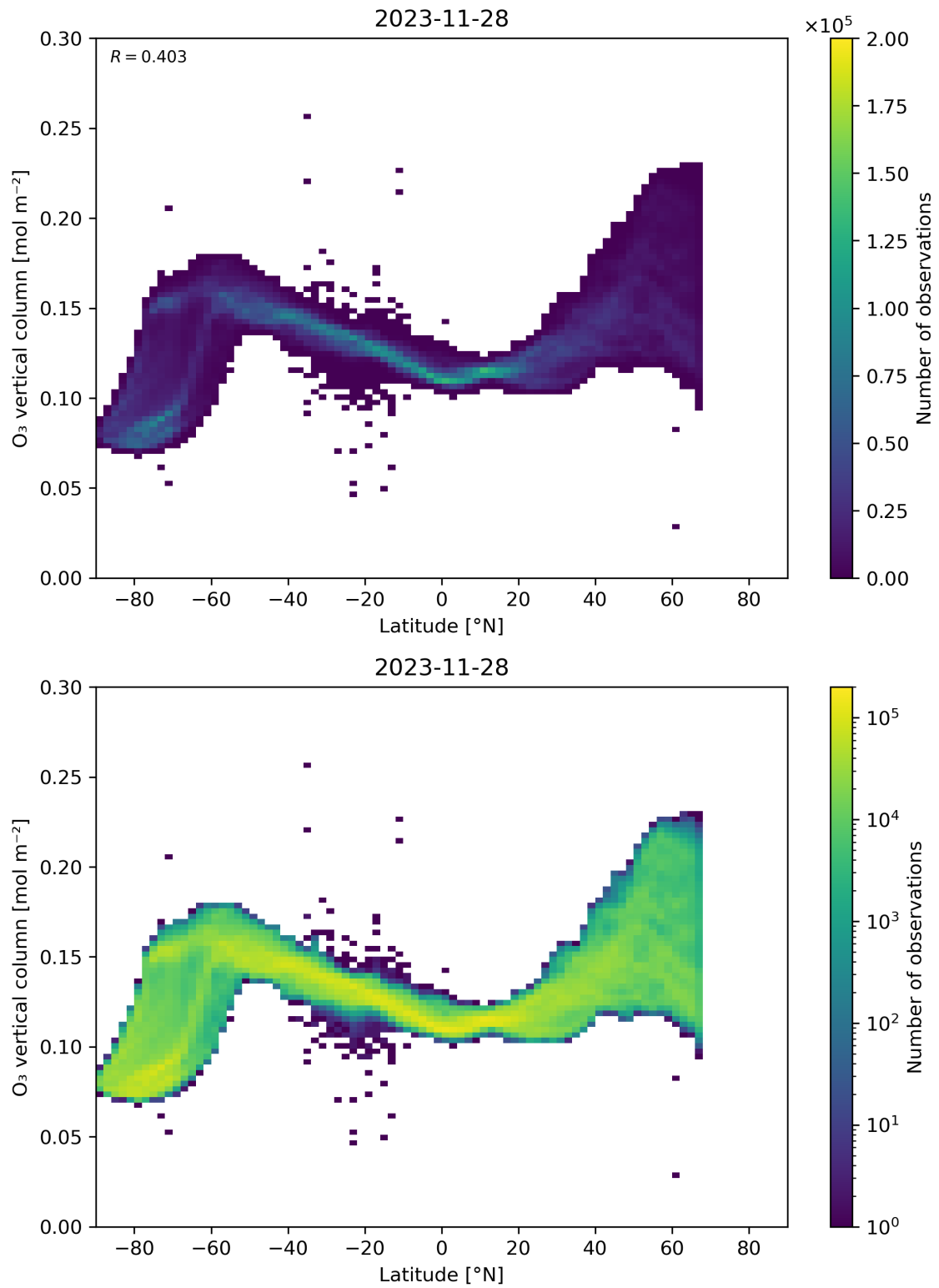
Figure 36: Scatter density plot of “Latitude” against “O 3 vertical column” for 2023-11-28 to 2023-11-29.
