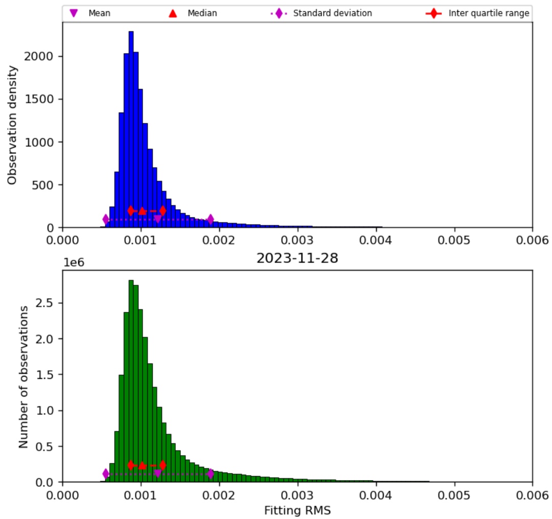
Figure 23: Histogram of “Fitting RMS” for 2023-11-28 to 2023-11-29
