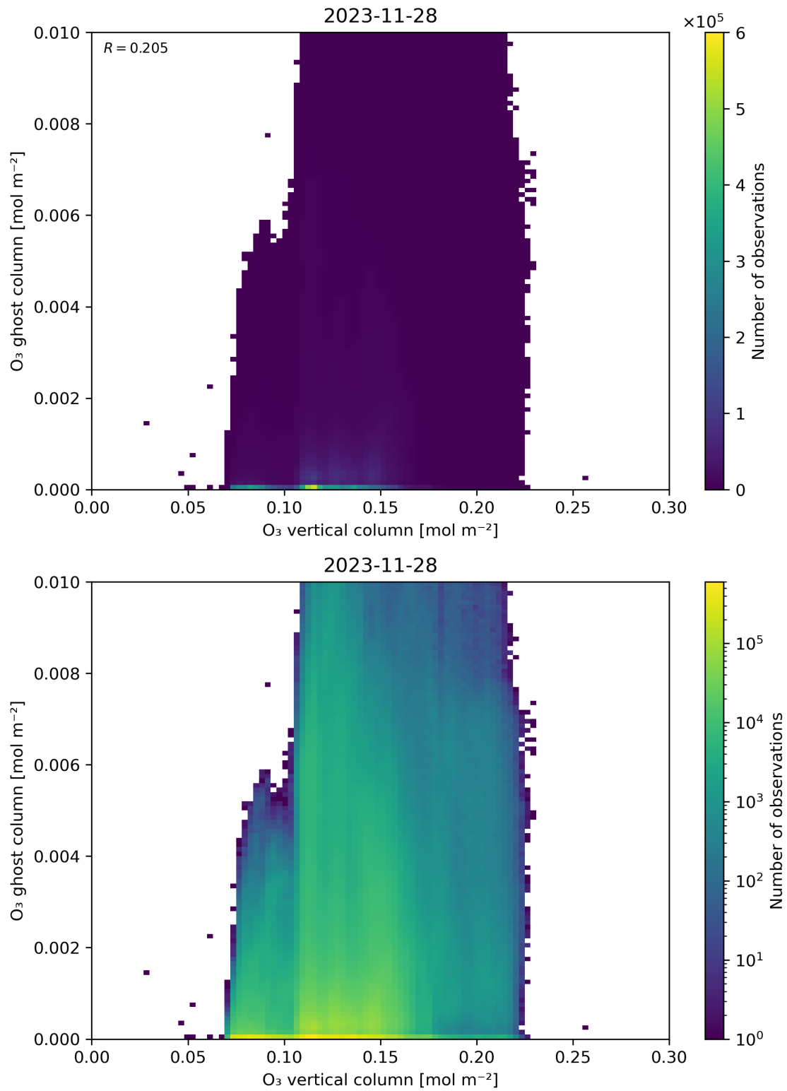
Figure 40: Scatter density plot of “O 3 vertical column” against “O 3 ghost column” for 2023-11-28 to 2023-11-29.
