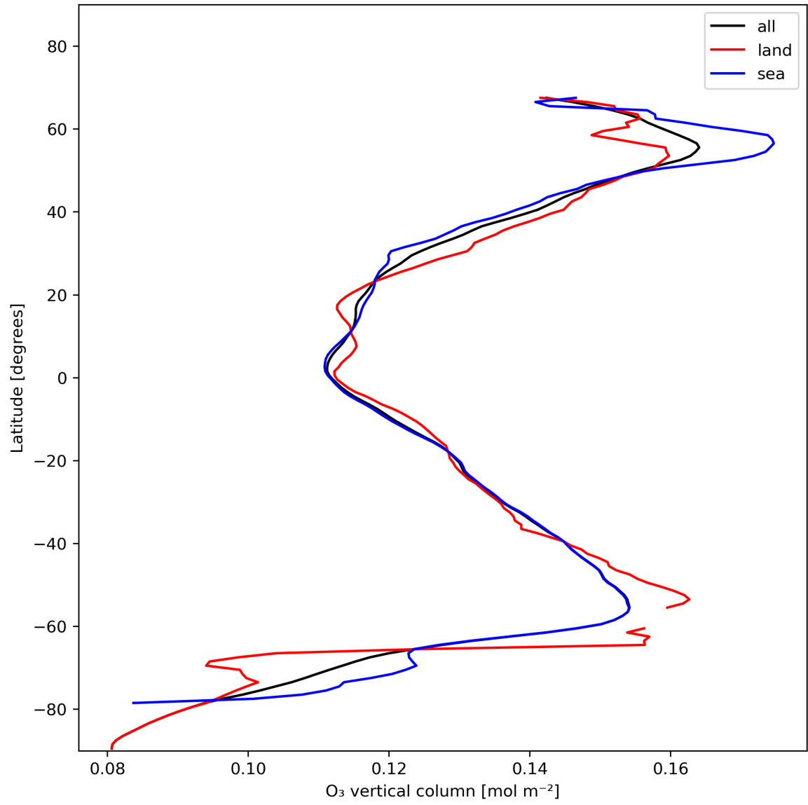
Figure 14: Zonal average of “O 3 vertical column” for 2023-11-28 to 2023-11-29.
