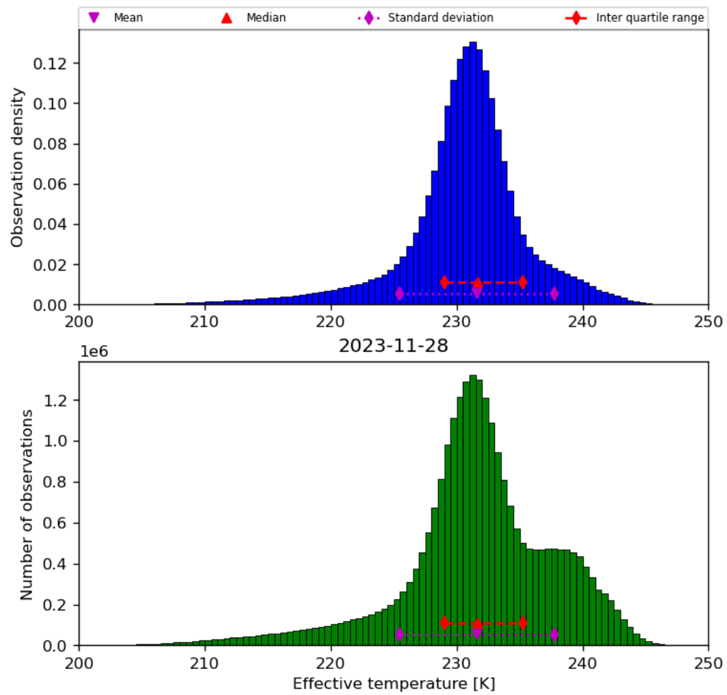
Figure 24: Histogram of “Effective temperature” for 2023-11-28 to 2023-11-29
