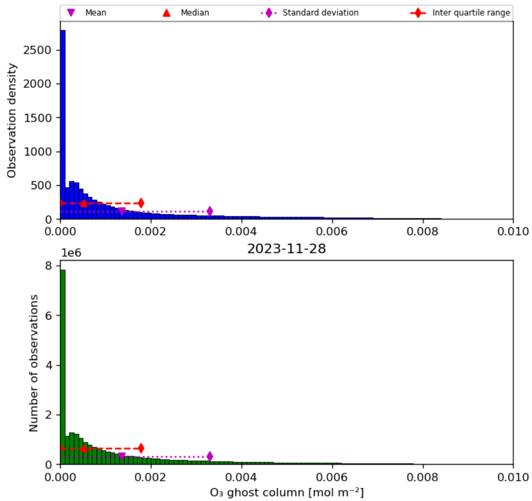
Figure 25: Histogram of “O 3 ghost column” for 2023-11-28 to 2023-11-29
