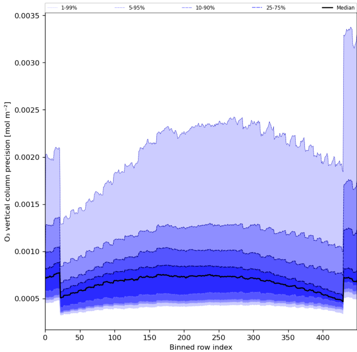
Figure 29: Along track statistics of “O 3 vertical column precision” for 2023-11-28 to 2023-11-29
