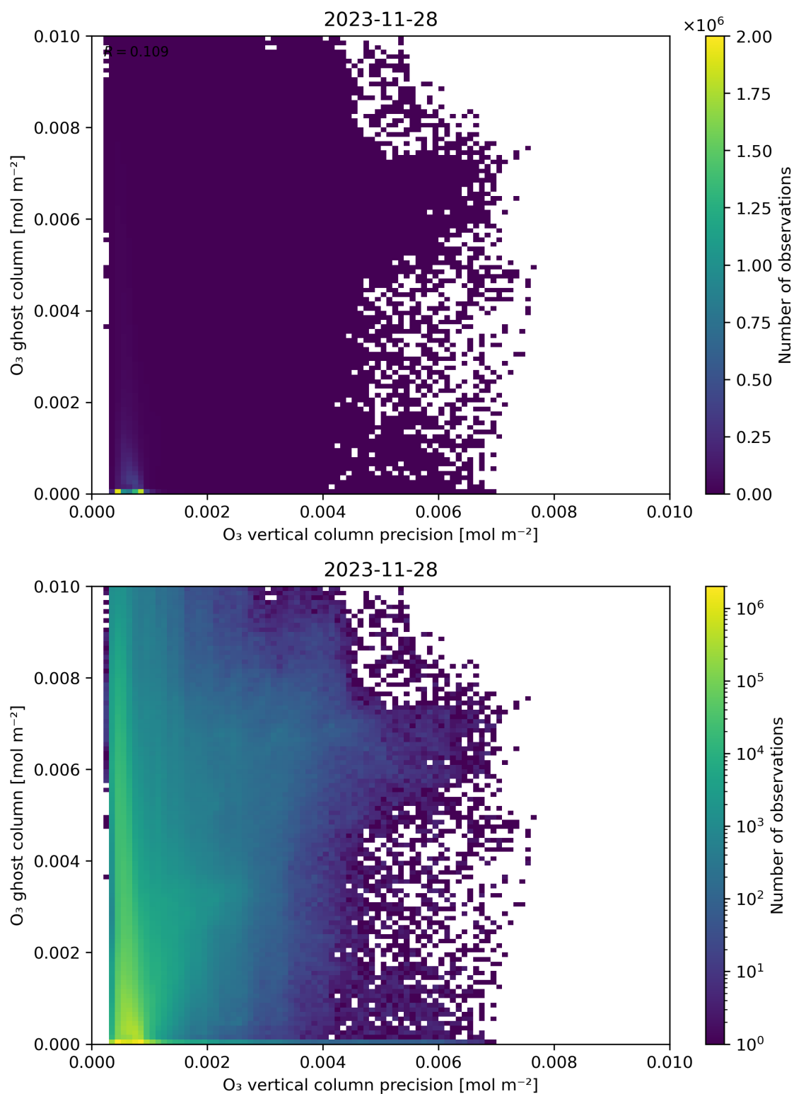
Figure 43: Scatter density plot of “O 3 vertical column precision” against “O 3 ghost column” for 2023-11-28 to 2023-11-29.
