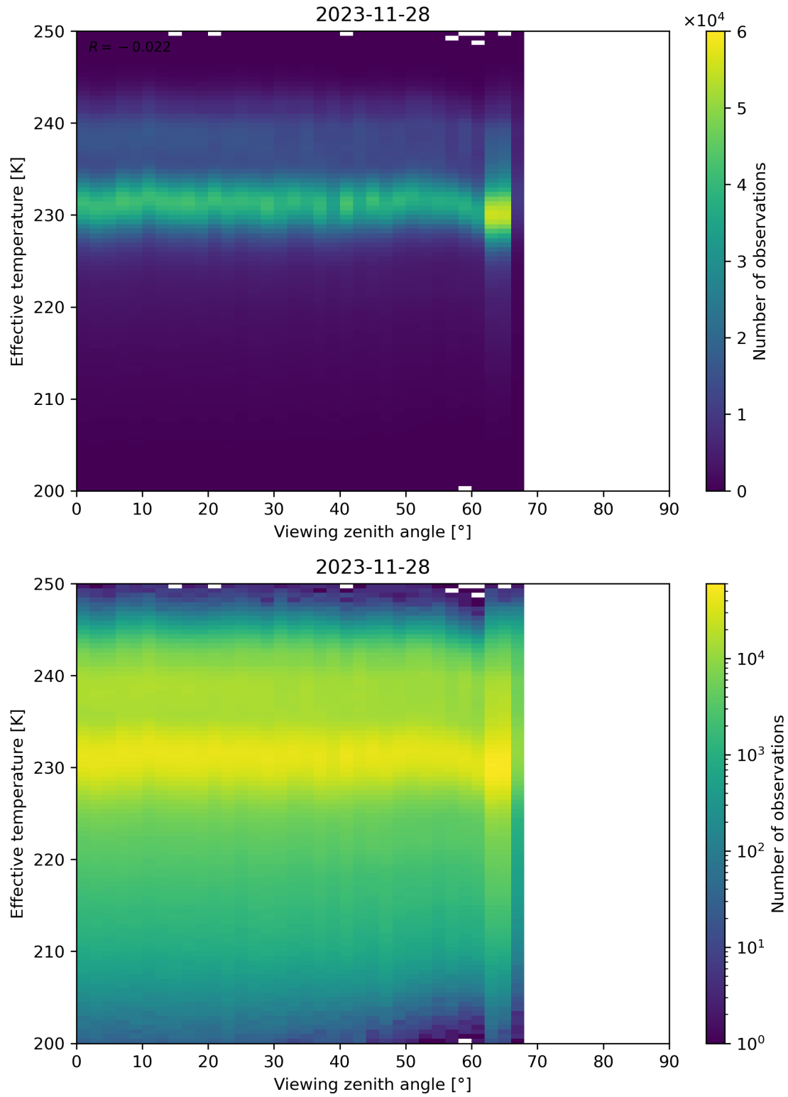
Figure 50: Scatter density plot of “Viewing zenith angle” against “Effective temperature” for 2023-11-28 to 2023-11-29.
