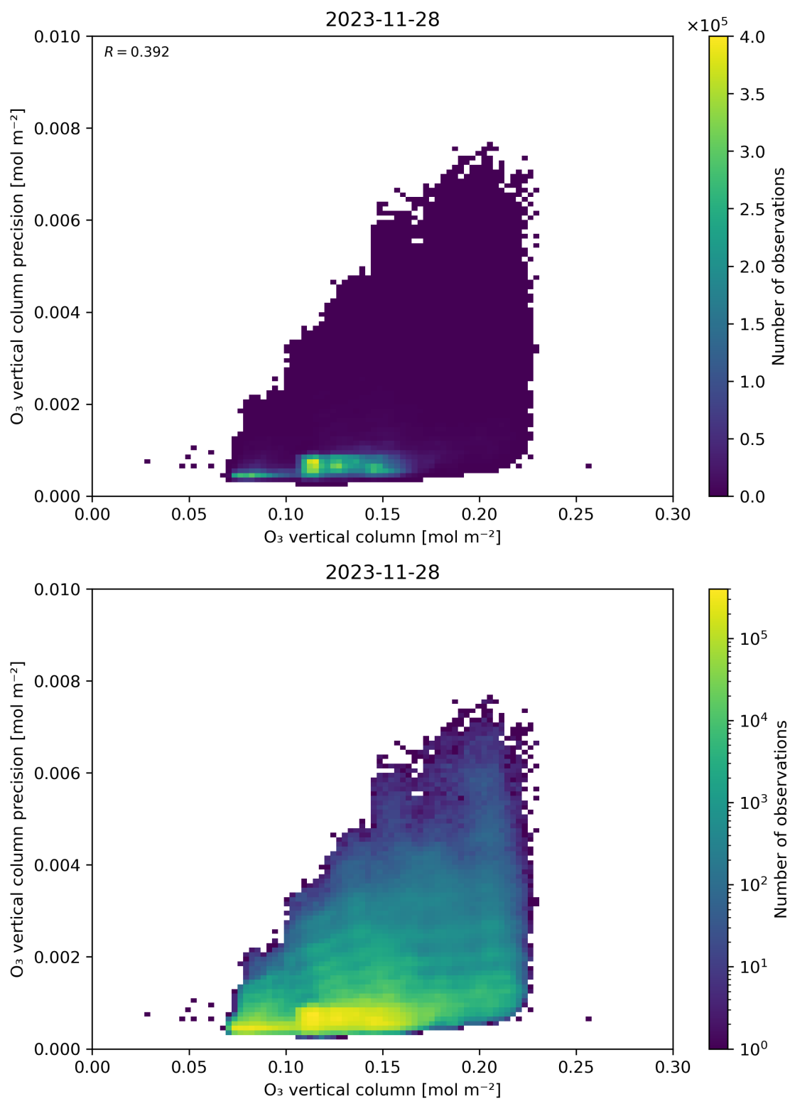
Figure 41: Scatter density plot of “O 3 vertical column” against “O 3 vertical column precision” for 2023-11-28 to 2023-11-29.
