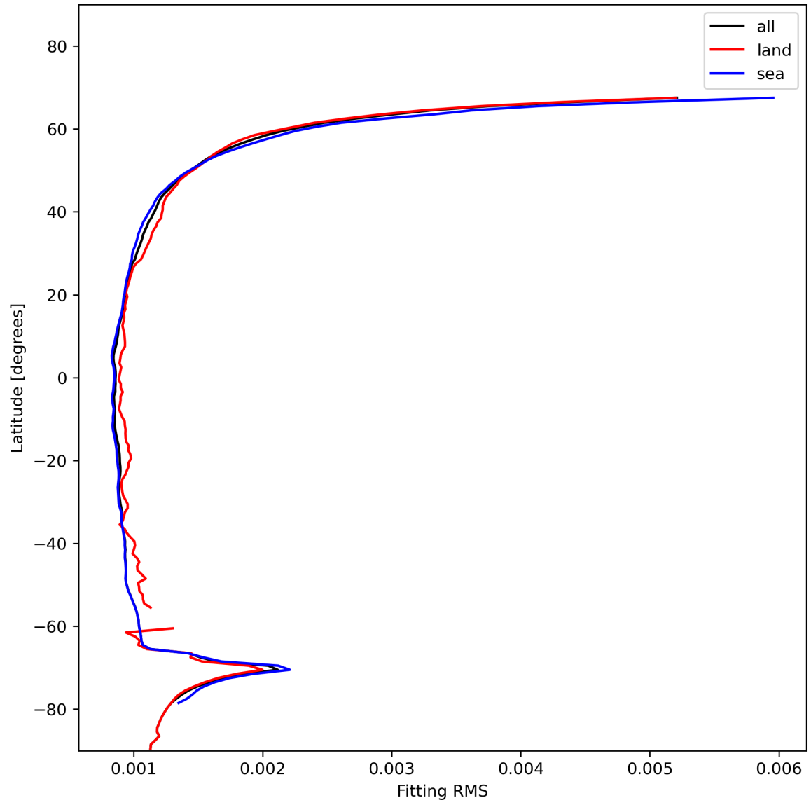
Figure 16: Zonal average of “Fitting RMS” for 2023-11-28 to 2023-11-29.
