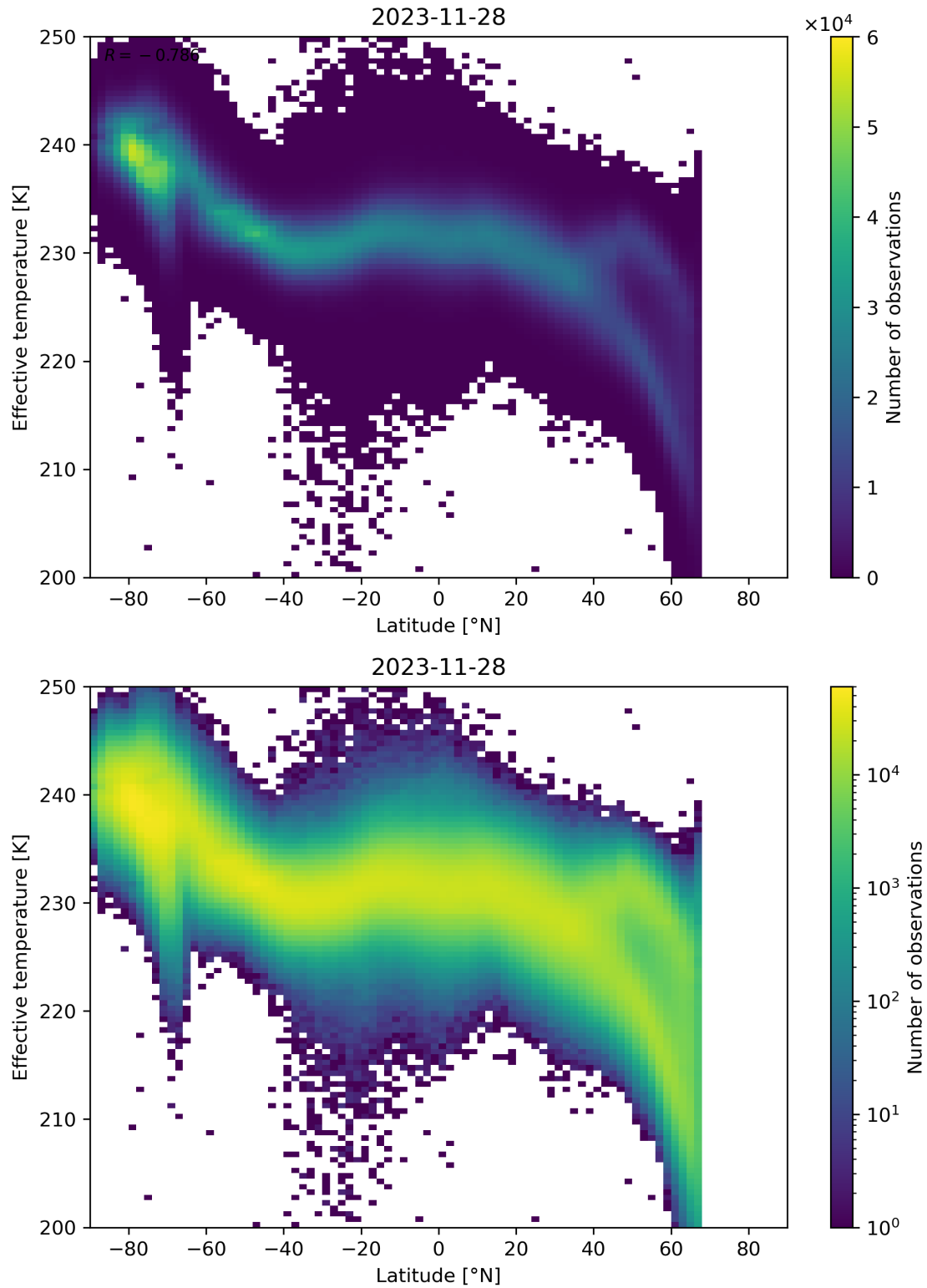
Figure 34: Scatter density plot of “Latitude” against “Effective temperature” for 2023-11-28 to 2023-11-29.
