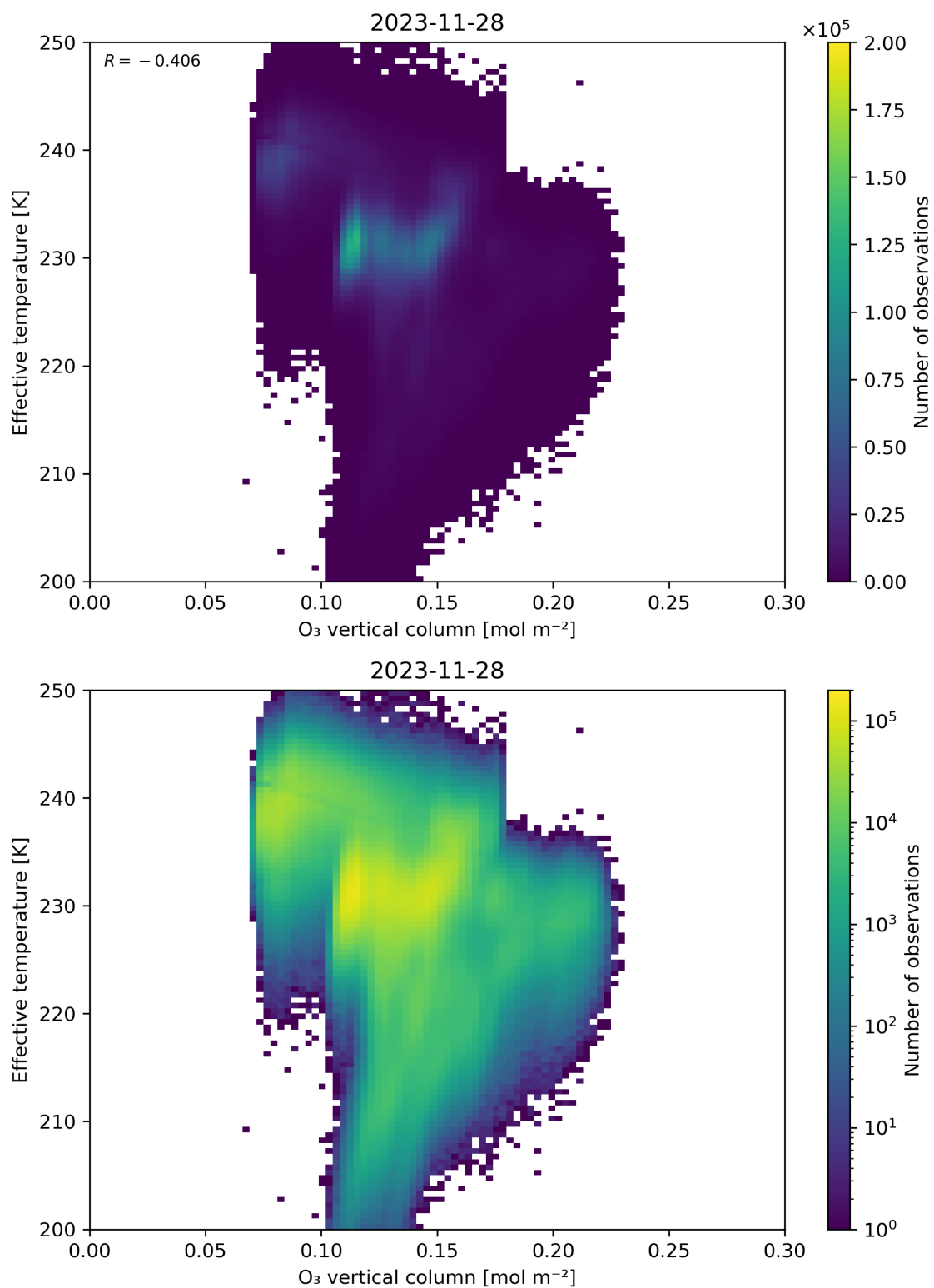
Figure 39: Scatter density plot of “O 3 vertical column” against “Effective temperature” for 2023-11-28 to 2023-11-29.
