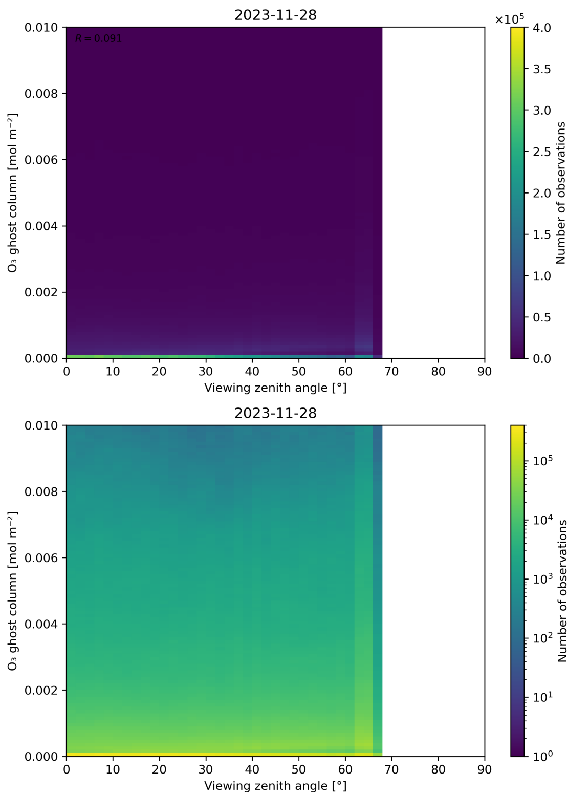
Figure 51: Scatter density plot of “Viewing zenith angle” against “O 3 ghost column” for 2023-11-28 to 2023-11-29.
