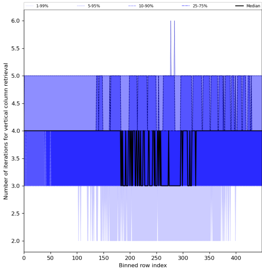
Figure 33: Along track statistics of “Number of iterations for vertical column retrieval” for 2023-11-28 to 2023-11-29
