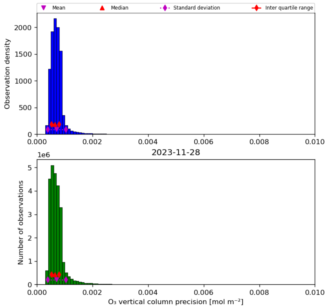
Figure 22: Histogram of “O 3 vertical column precision” for 2023-11-28 to 2023-11-29
