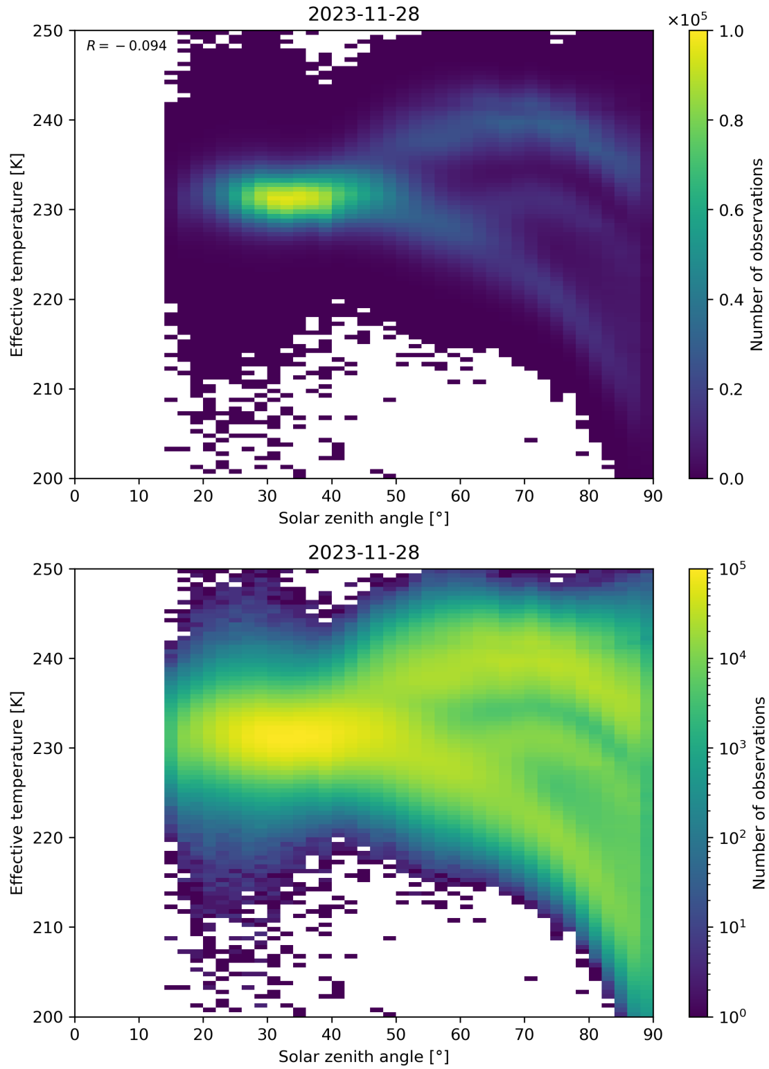
Figure 45: Scatter density plot of “Solar zenith angle” against “Effective temperature” for 2023-11-28 to 2023-11-29.
