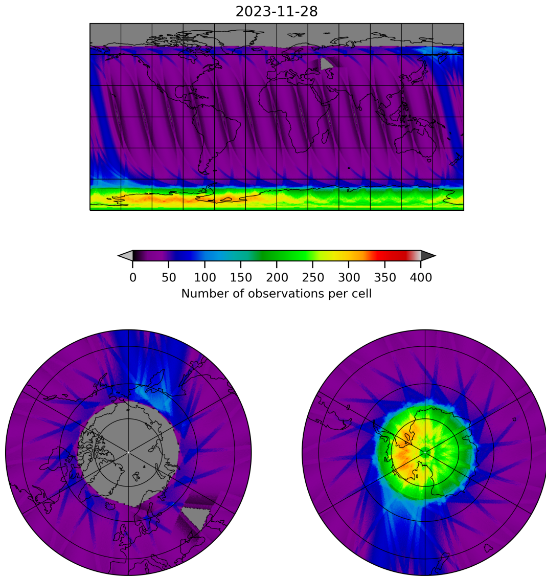
Figure 12: Map of the number of observations for 2023-11-28 to 2023-11-29
