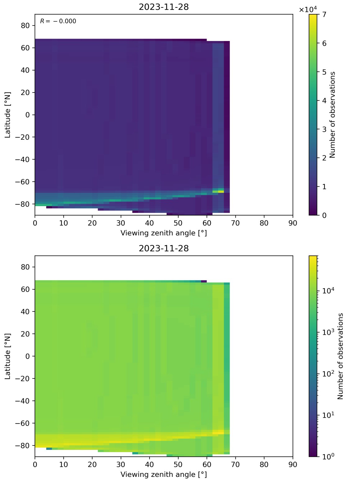
Figure 49: Scatter density plot of “Viewing zenith angle” against “Latitude” for 2023-11-28 to 2023-11-29.
