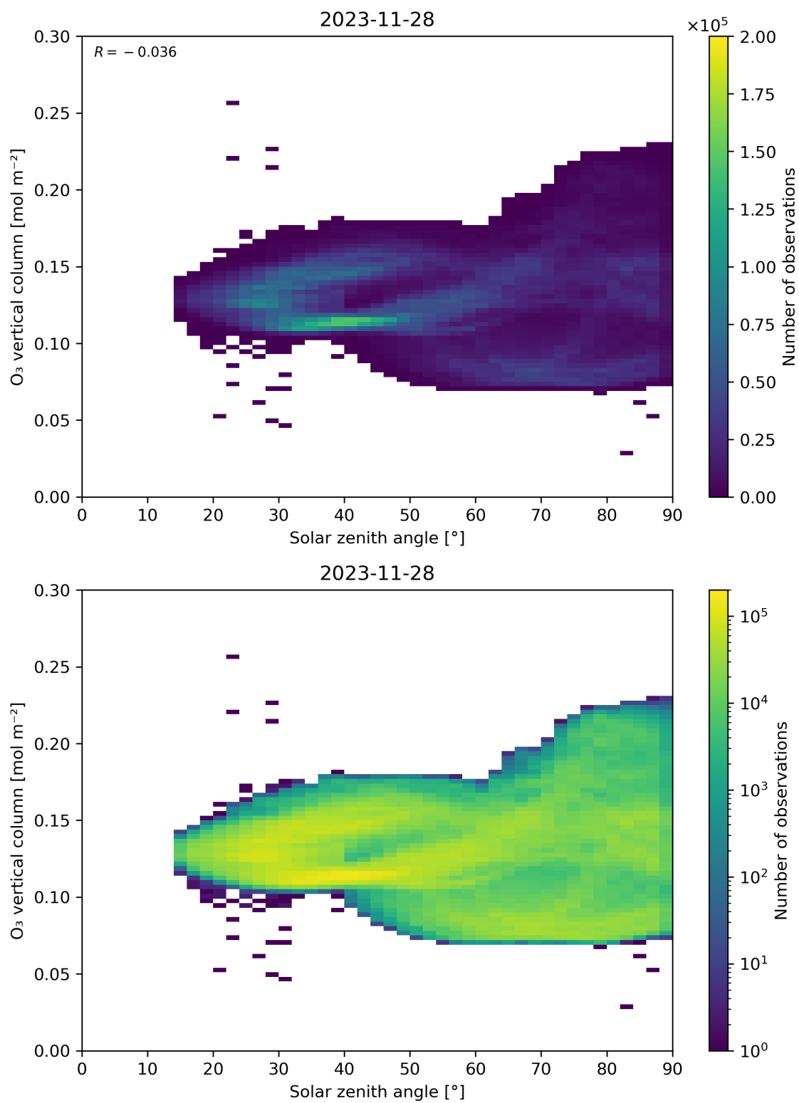
Figure 47: Scatter density plot of “Solar zenith angle” against “O 3 vertical column” for 2023-11-28 to 2023-11-29.
