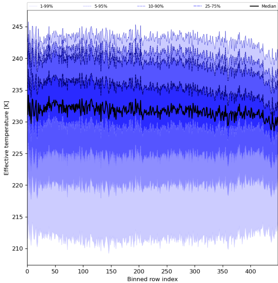
Figure 31: Along track statistics of “Effective temperature” for 2023-11-28 to 2023-11-29
