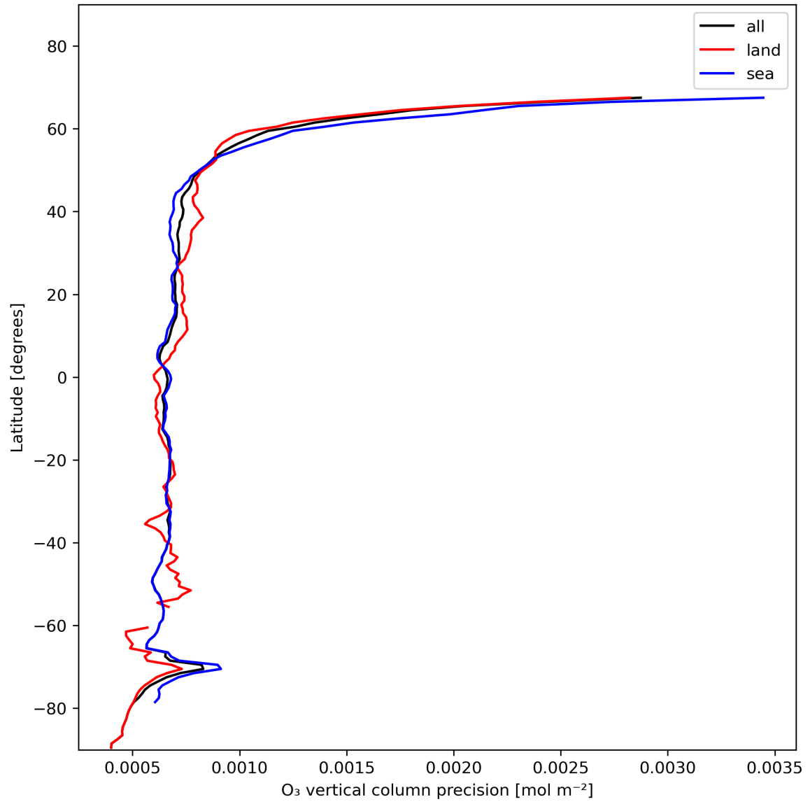
Figure 15: Zonal average of “O 3 vertical column precision” for 2023-11-28 to 2023-11-29.
