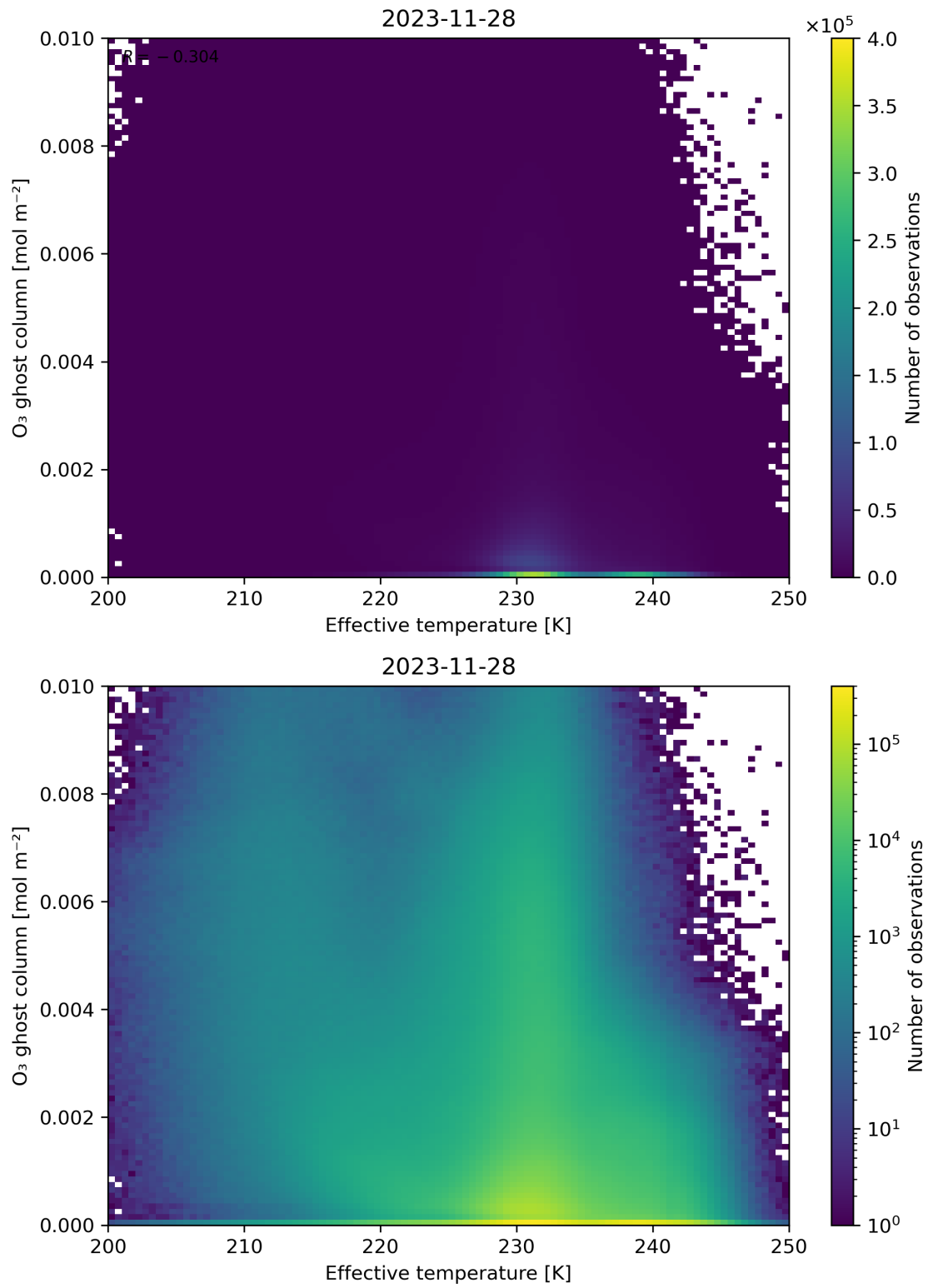
Figure 38: Scatter density plot of “Effective temperature” against “O 3 ghost column” for 2023-11-28 to 2023-11-29.
