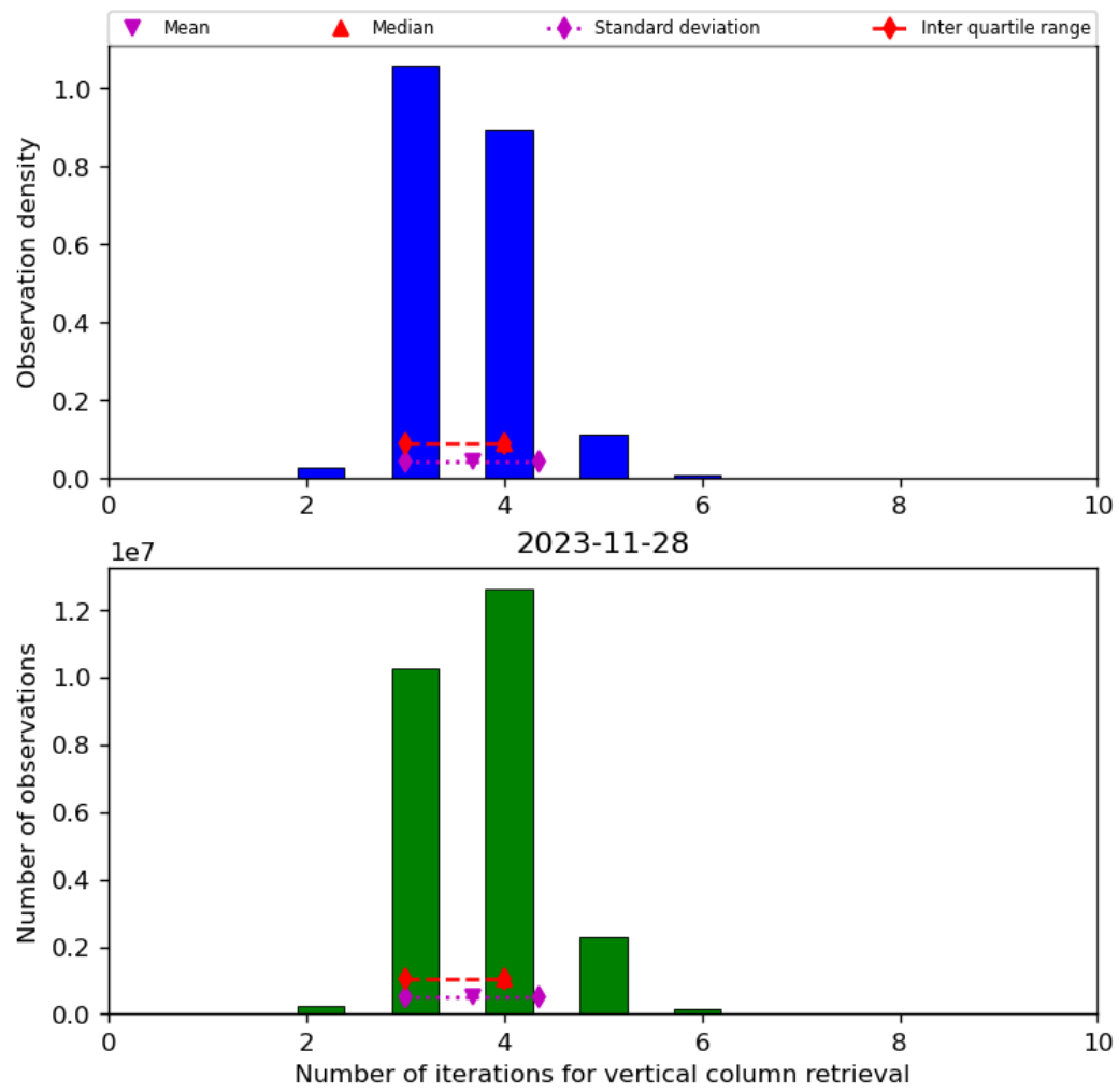
Figure 26: Histogram of “Number of iterations for vertical column retrieval” for 2023-11-28 to 2023-11-29
