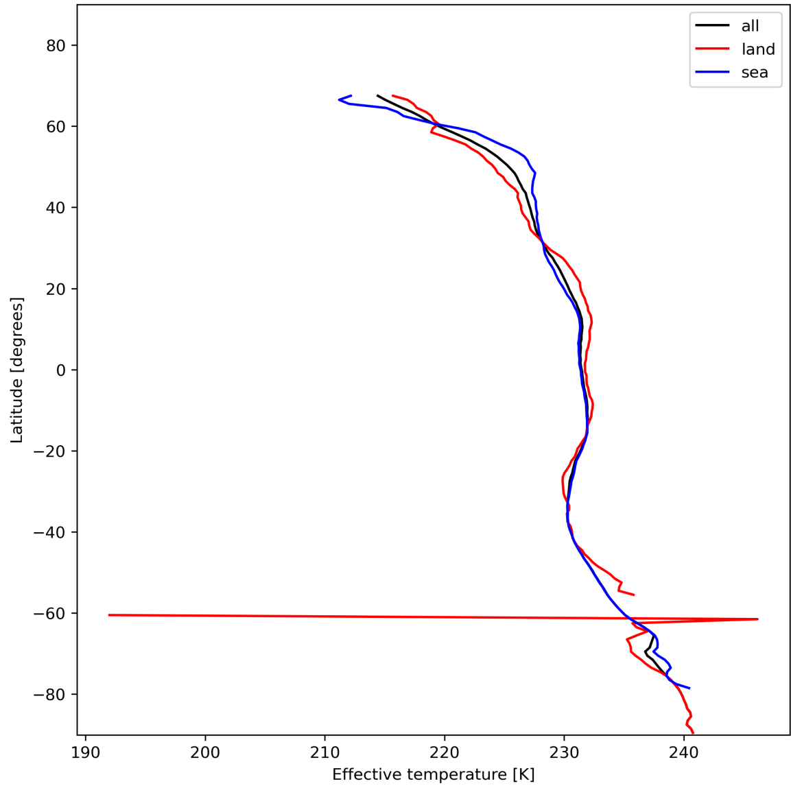
Figure 17: Zonal average of “Effective temperature” for 2023-11-28 to 2023-11-29.
