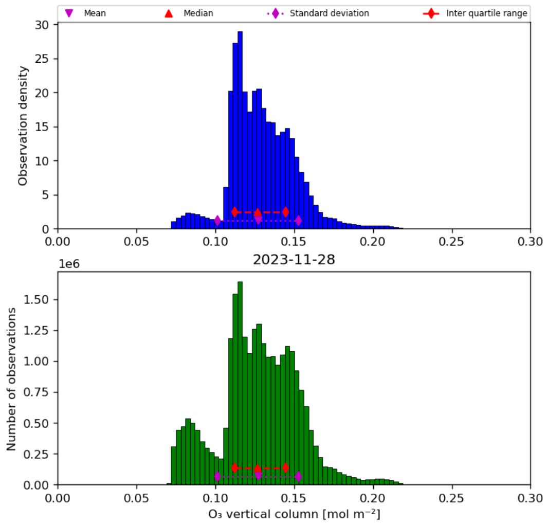
Figure 21: Histogram of “O 3 vertical column” for 2023-11-28 to 2023-11-29
