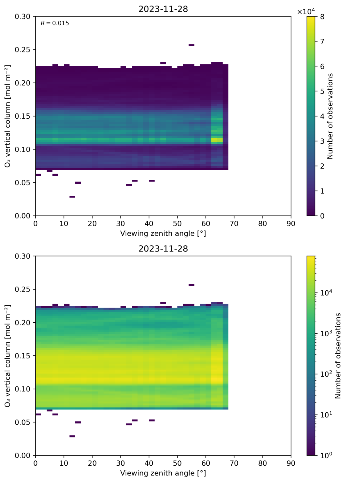
Figure 52: Scatter density plot of “Viewing zenith angle” against “O 3 vertical column” for 2023-11-28 to 2023-11-29.
