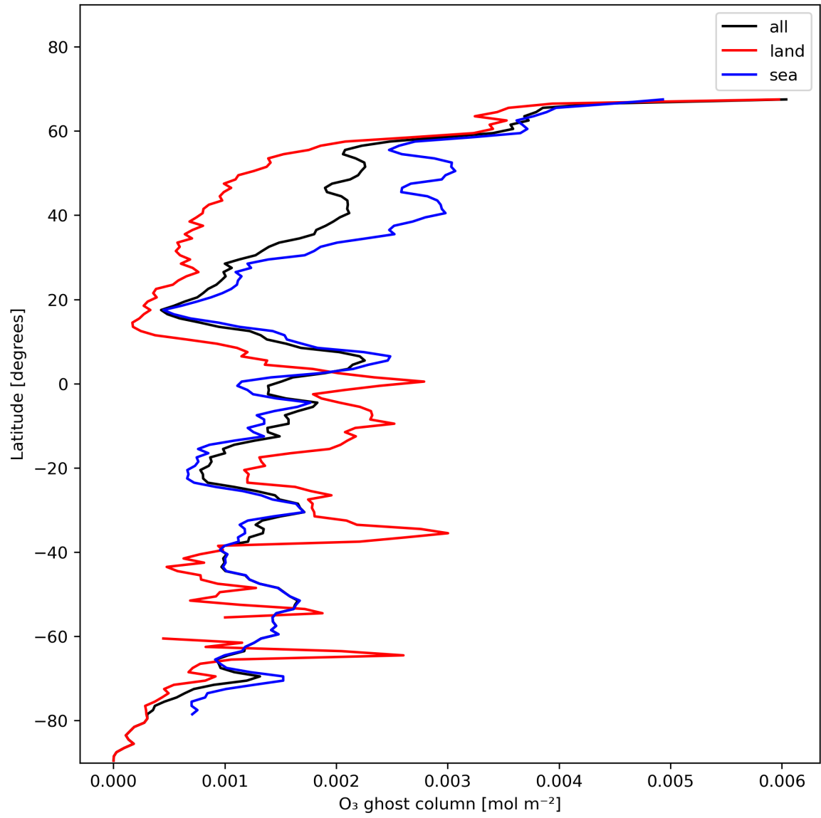
Figure 18: Zonal average of "O 3 ghost column" for 2023-11-28 to 2023-11-29.
