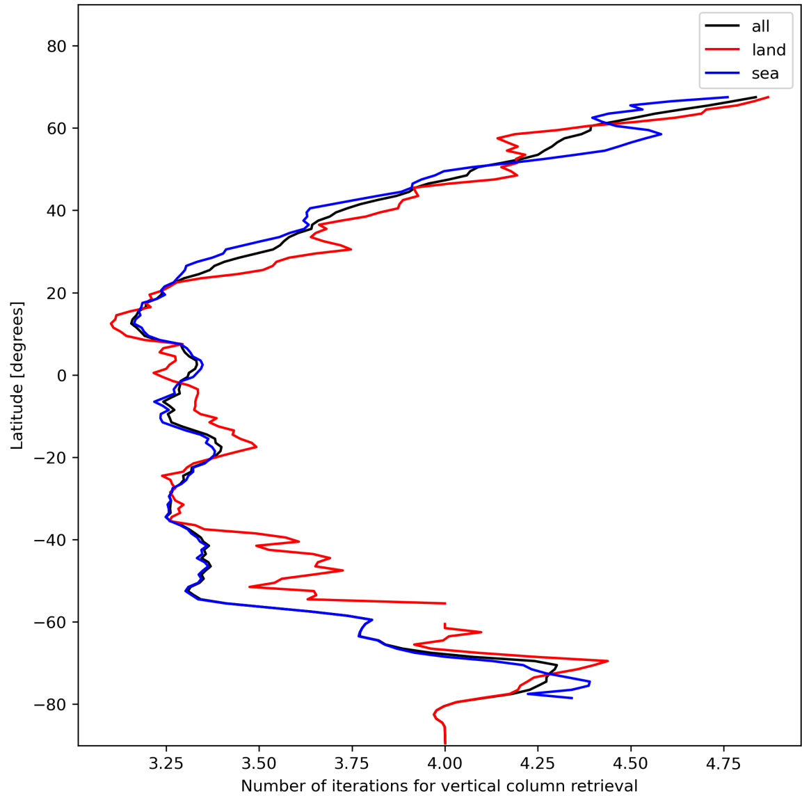
Figure 19: Zonal average of “Number of iterations for vertical column retrieval” for 2023-11-28 to 2023-11-29.
