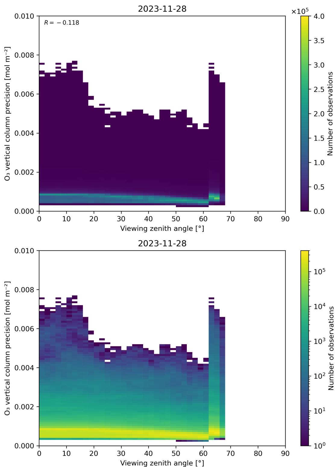
Figure 53: Scatter density plot of “Viewing zenith angle” against “O 3 vertical column precision” for 2023-11-28 to 2023-11-29.
