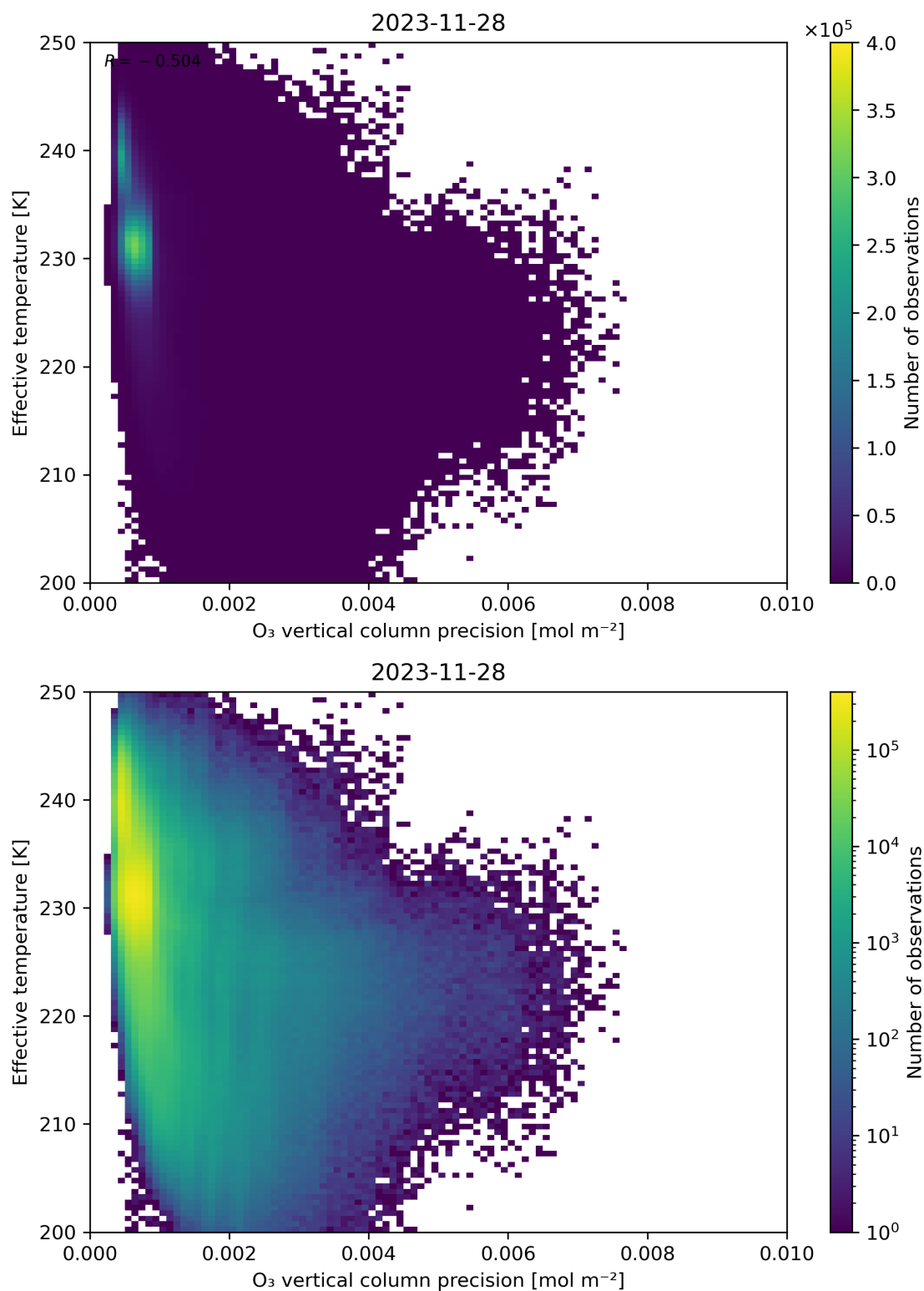
Figure 42: Scatter density plot of “O 3 vertical column precision” against “Effective temperature” for 2023-11-28 to 2023-11-29.
