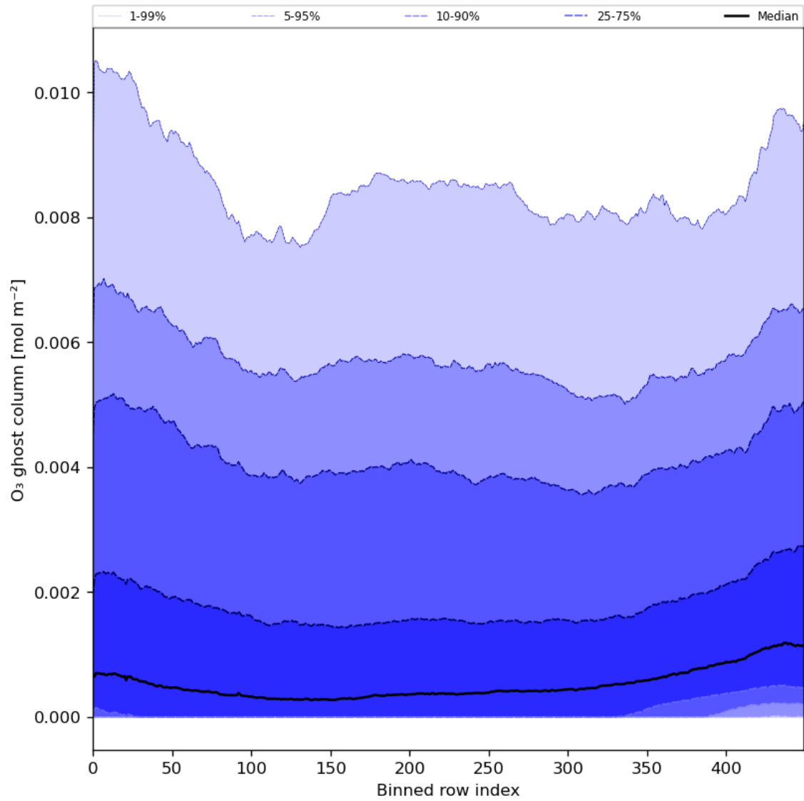
Figure 32: Along track statistics of “O 3 ghost column” for 2023-11-28 to 2023-11-29
