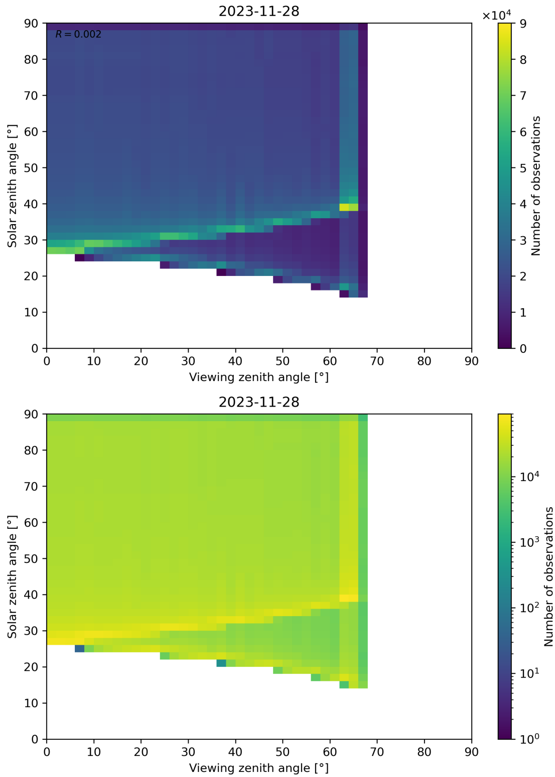
Figure 54: Scatter density plot of “Viewing zenith angle” against “Solar zenith angle” for 2023-11-28 to 2023-11-29.
