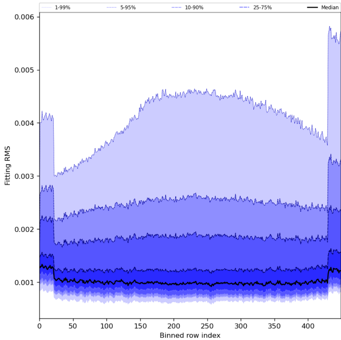
Figure 30: Along track statistics of “Fitting RMS” for 2023-11-28 to 2023-11-29
