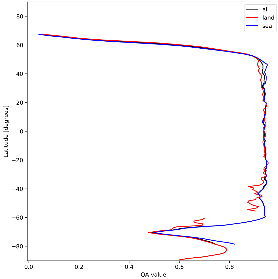
Figure 13: Zonal average of “QA value” for 2023-11-28 to 2023-11-29.
