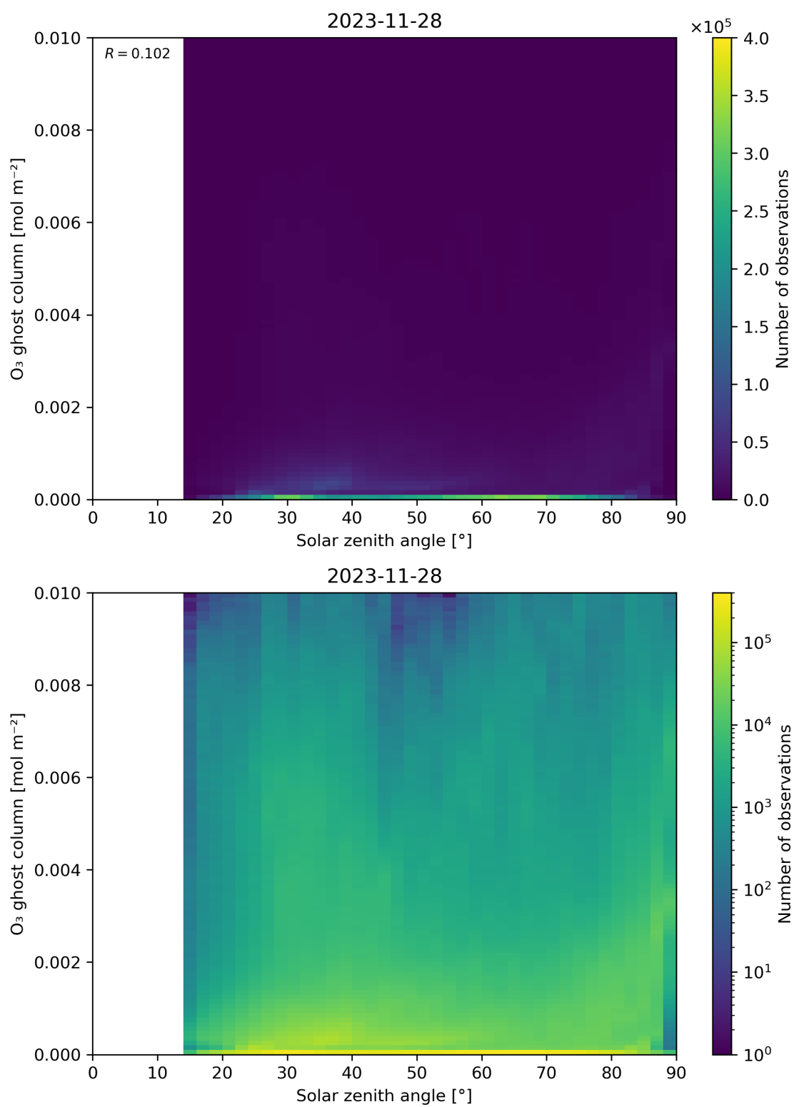
Figure 46: Scatter density plot of “Solar zenith angle” against “O 3 ghost column” for 2023-11-28 to 2023-11-29.
