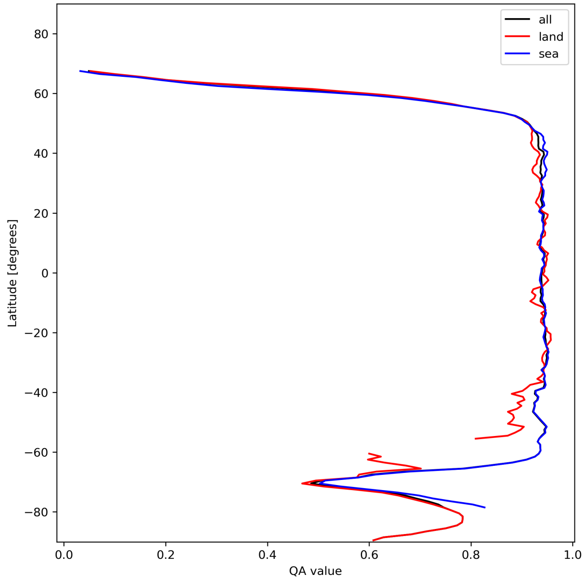
Figure 13: Zonal average of “QA value” for 2023-11-28 to 2023-11-30.
