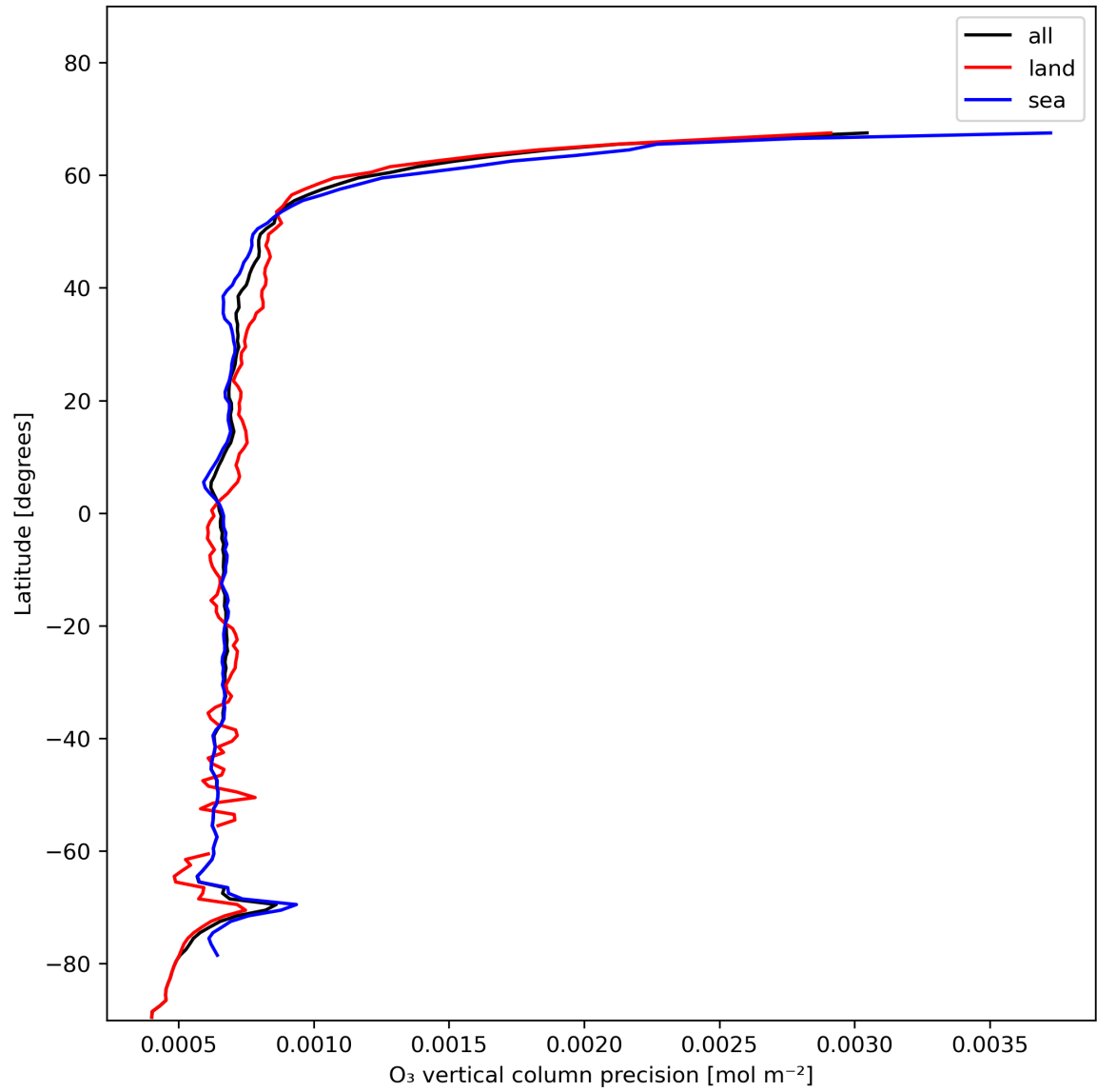
Figure 15: Zonal average of “O 3 vertical column precision” for 2023-11-28 to 2023-11-30.
