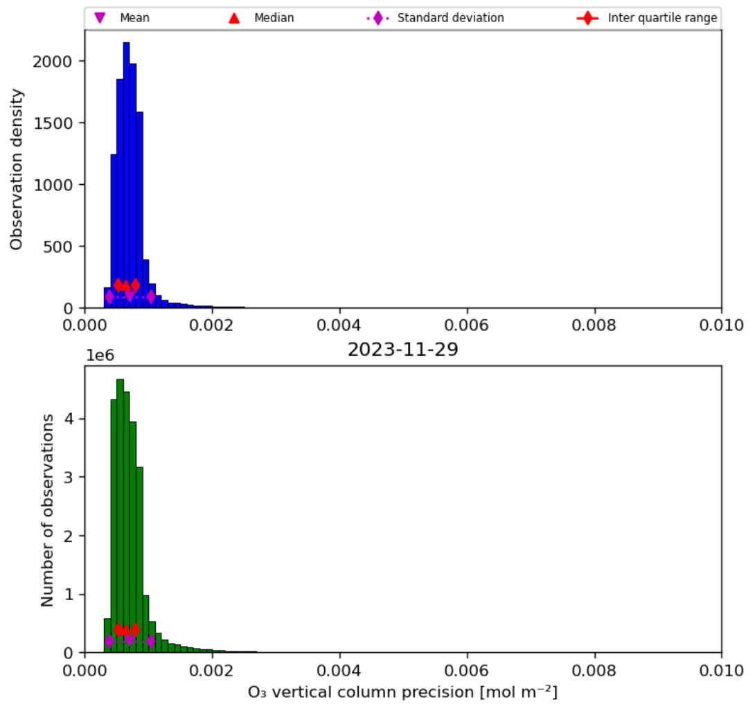
Figure 22: Histogram of “O 3 vertical column precision” for 2023-11-28 to 2023-11-30
