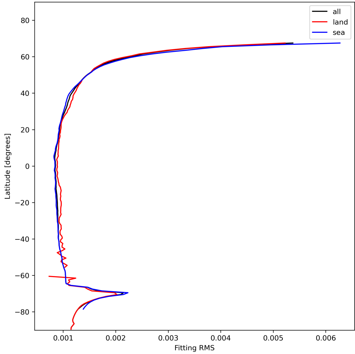
Figure 16: Zonal average of “Fitting RMS” for 2023-11-28 to 2023-11-30.
