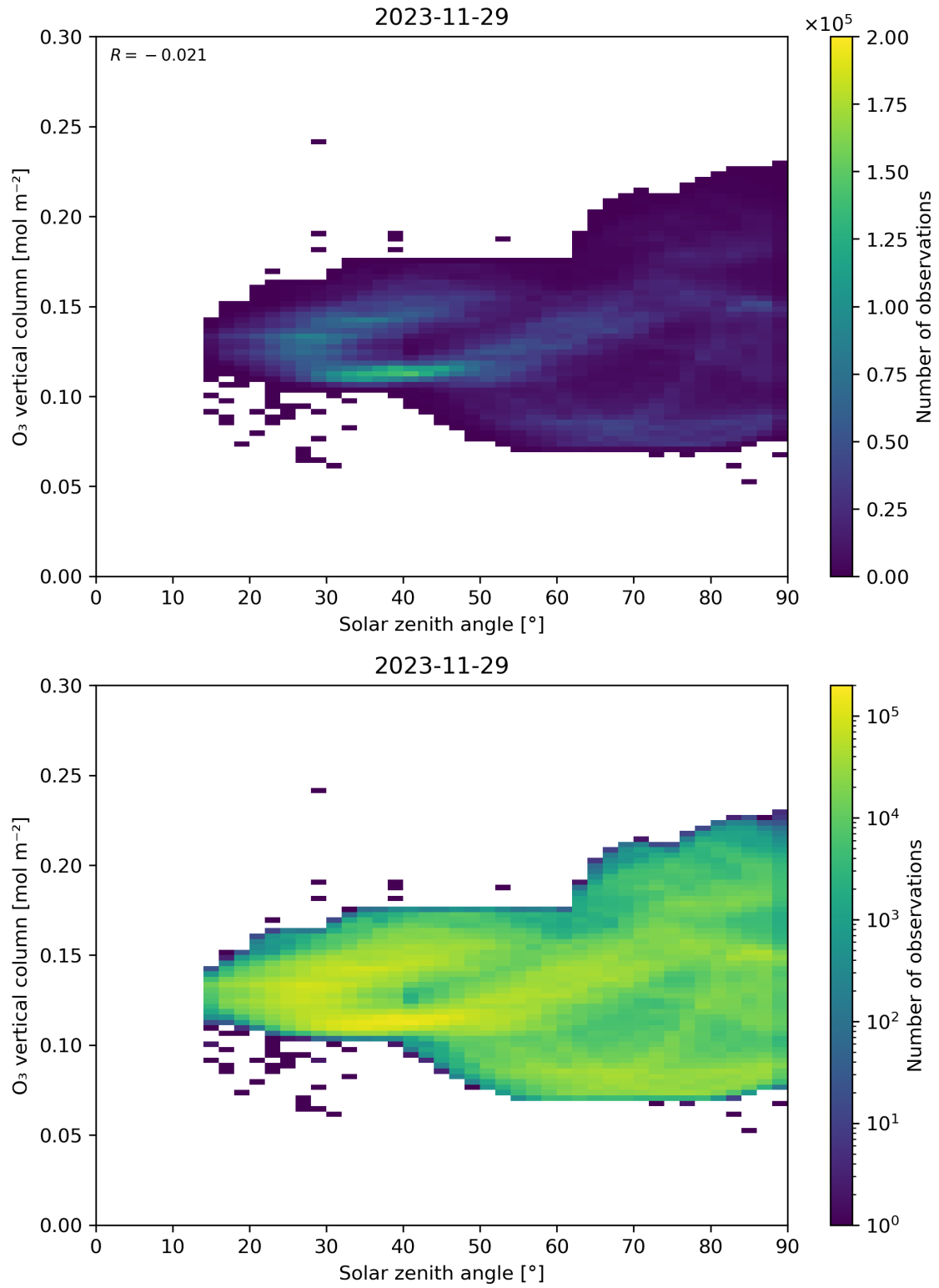
Figure 47: Scatter density plot of “Solar zenith angle” against “O 3 vertical column” for 2023-11-28 to 2023-11-30.
