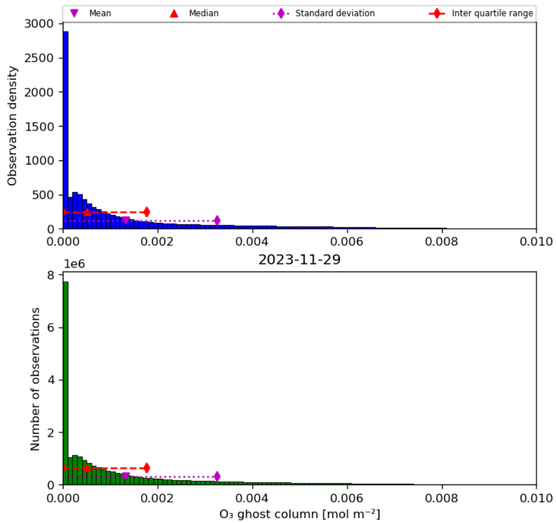
Figure 25: Histogram of “O 3 ghost column” for 2023-11-28 to 2023-11-30
