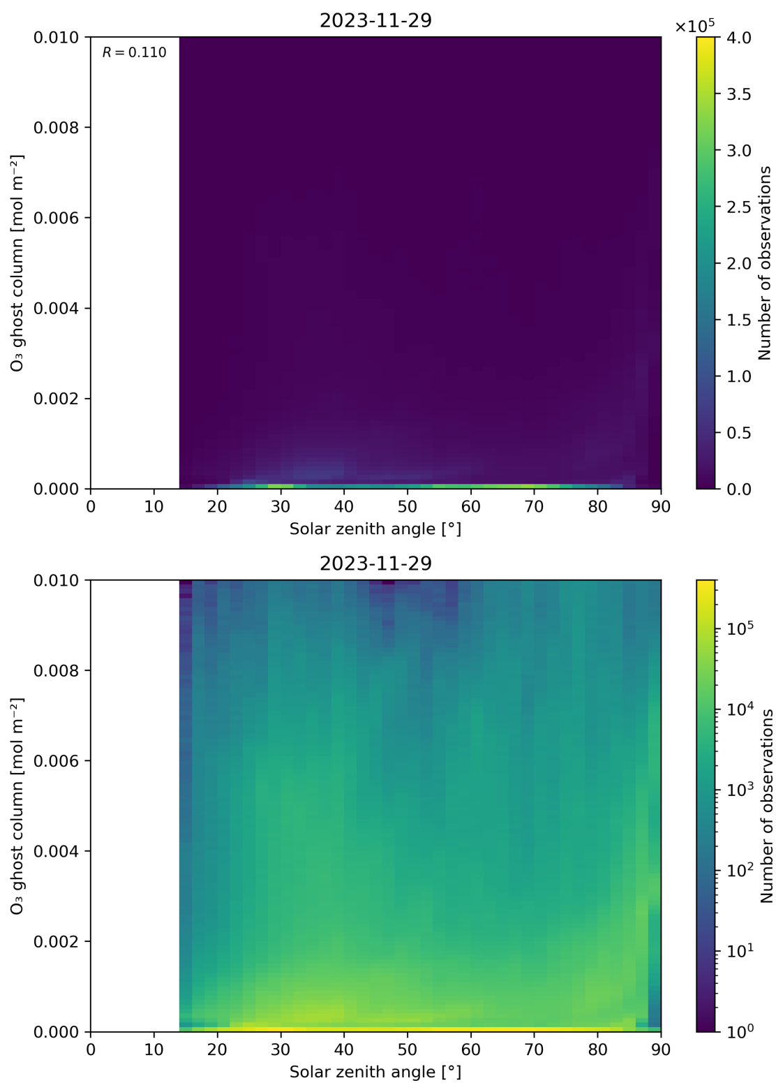
Figure 46: Scatter density plot of “Solar zenith angle” against “O 3 ghost column” for 2023-11-28 to 2023-11-30.
