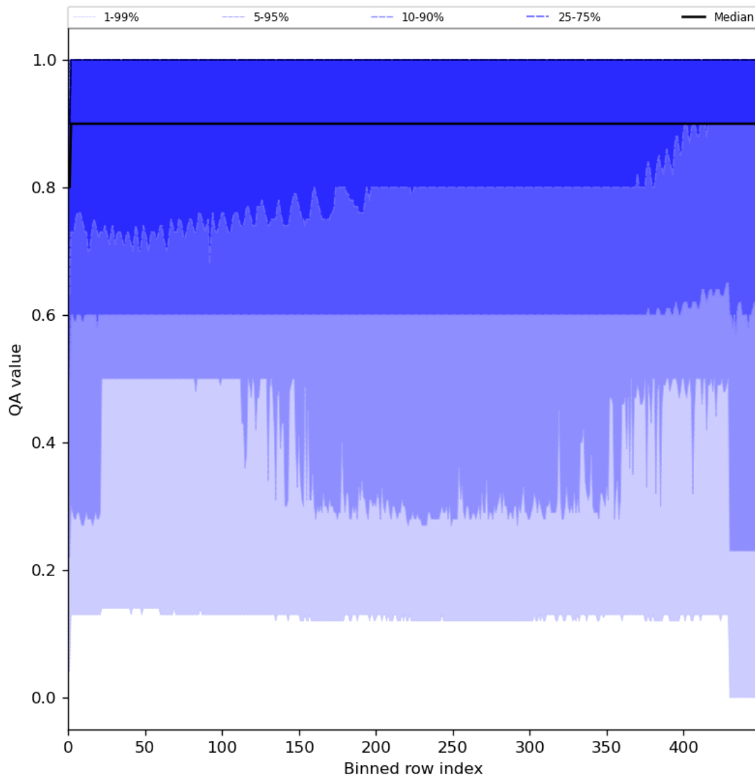
Figure 27: Along track statistics of “QA value” for 2023-11-28 to 2023-11-30
