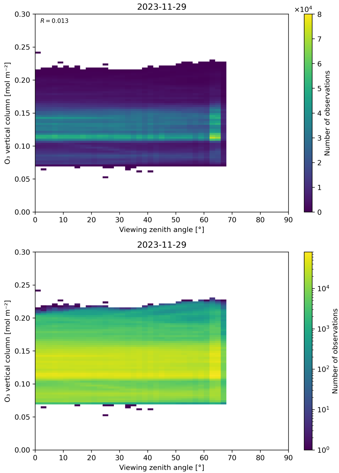
Figure 52: Scatter density plot of “Viewing zenith angle” against “O 3 vertical column” for 2023-11-28 to 2023-11-30.
