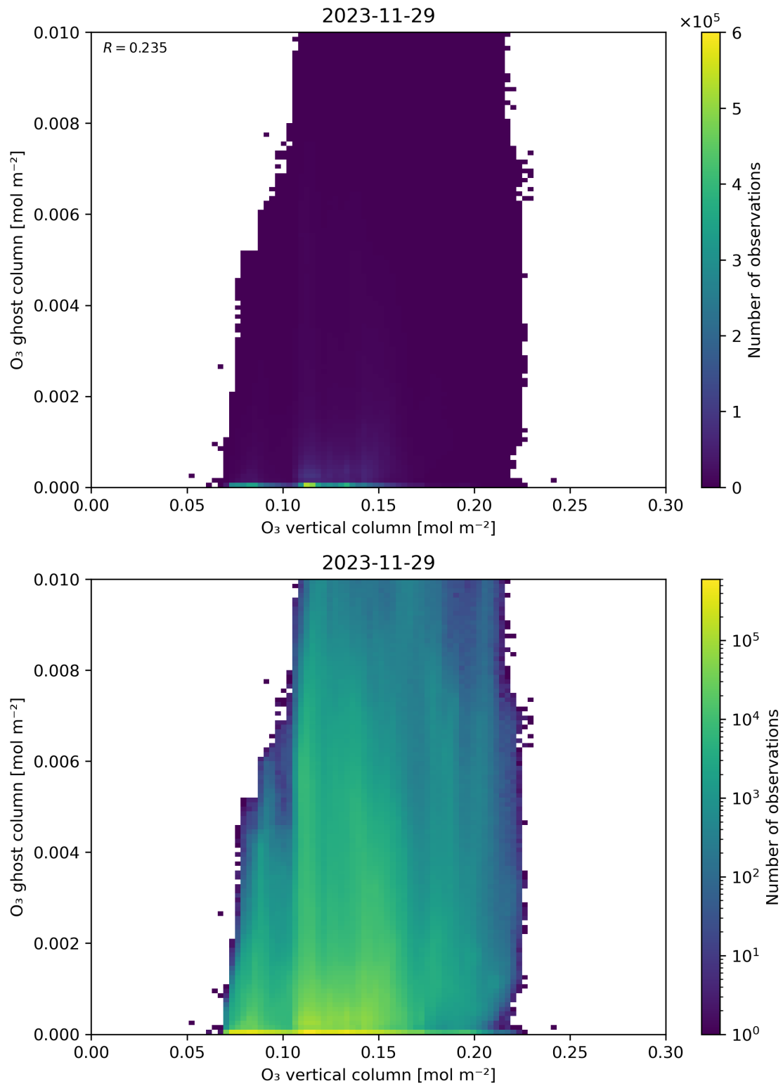
Figure 40: Scatter density plot of “O 3 vertical column” against “O 3 ghost column” for 2023-11-28 to 2023-11-30.
