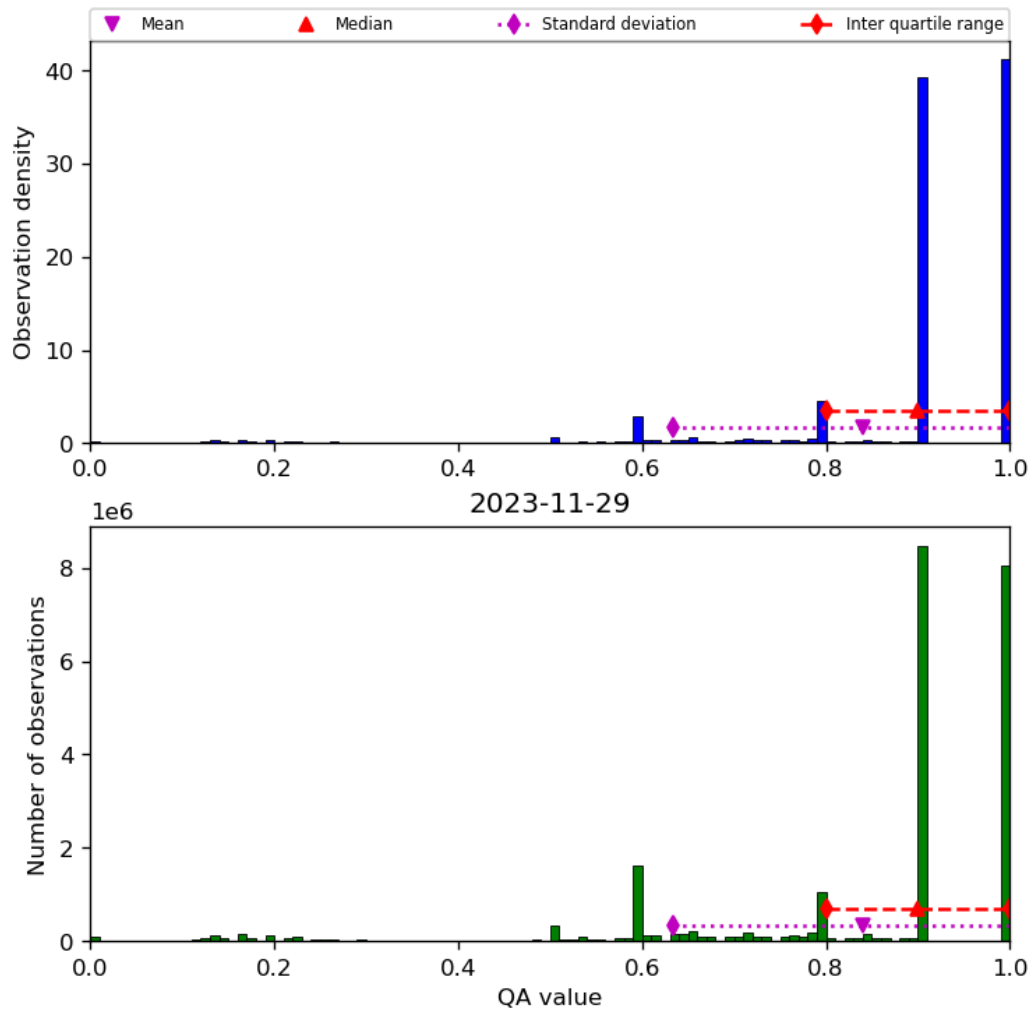
Figure 20: Histogram of “QA value” for 2023-11-28 to 2023-11-30
