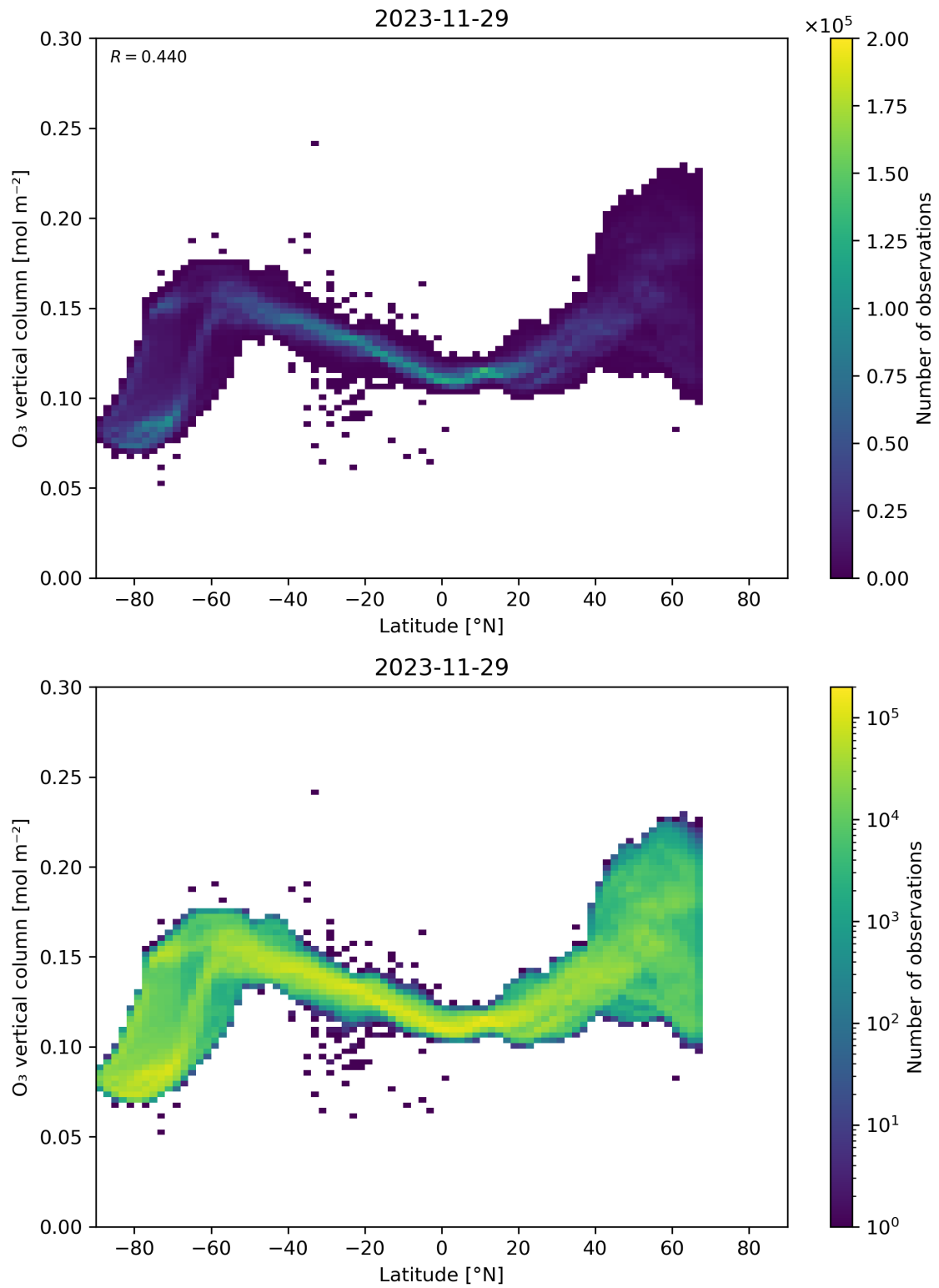
Figure 36: Scatter density plot of “Latitude” against “O 3 vertical column” for 2023-11-28 to 2023-11-30.
