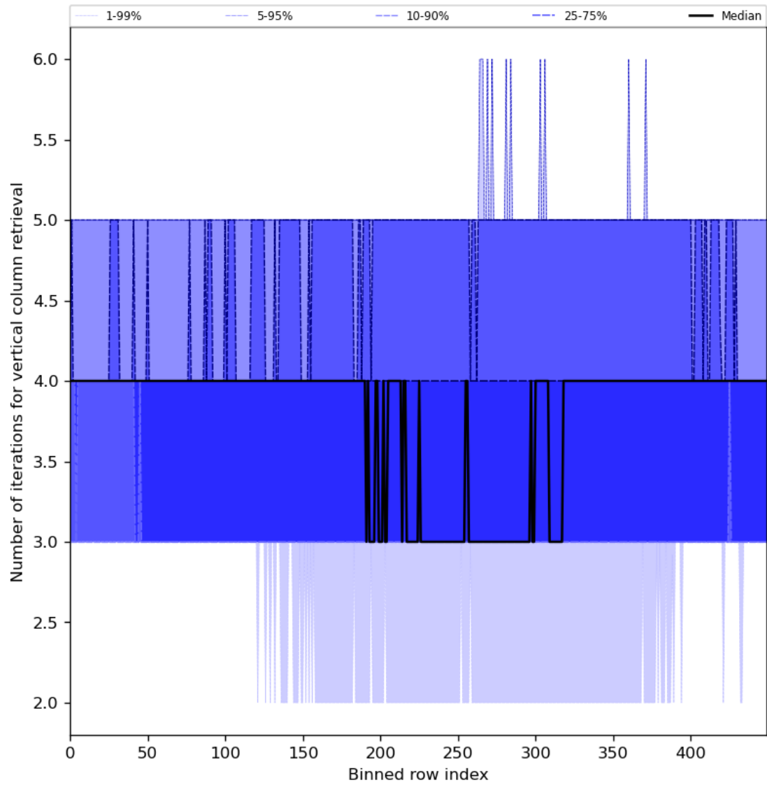
Figure 33: Along track statistics of “Number of iterations for vertical column retrieval” for 2023-11-28 to 2023-11-30
