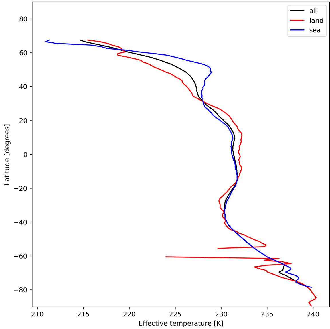
Figure 17: Zonal average of “Effective temperature” for 2023-11-28 to 2023-11-30.
