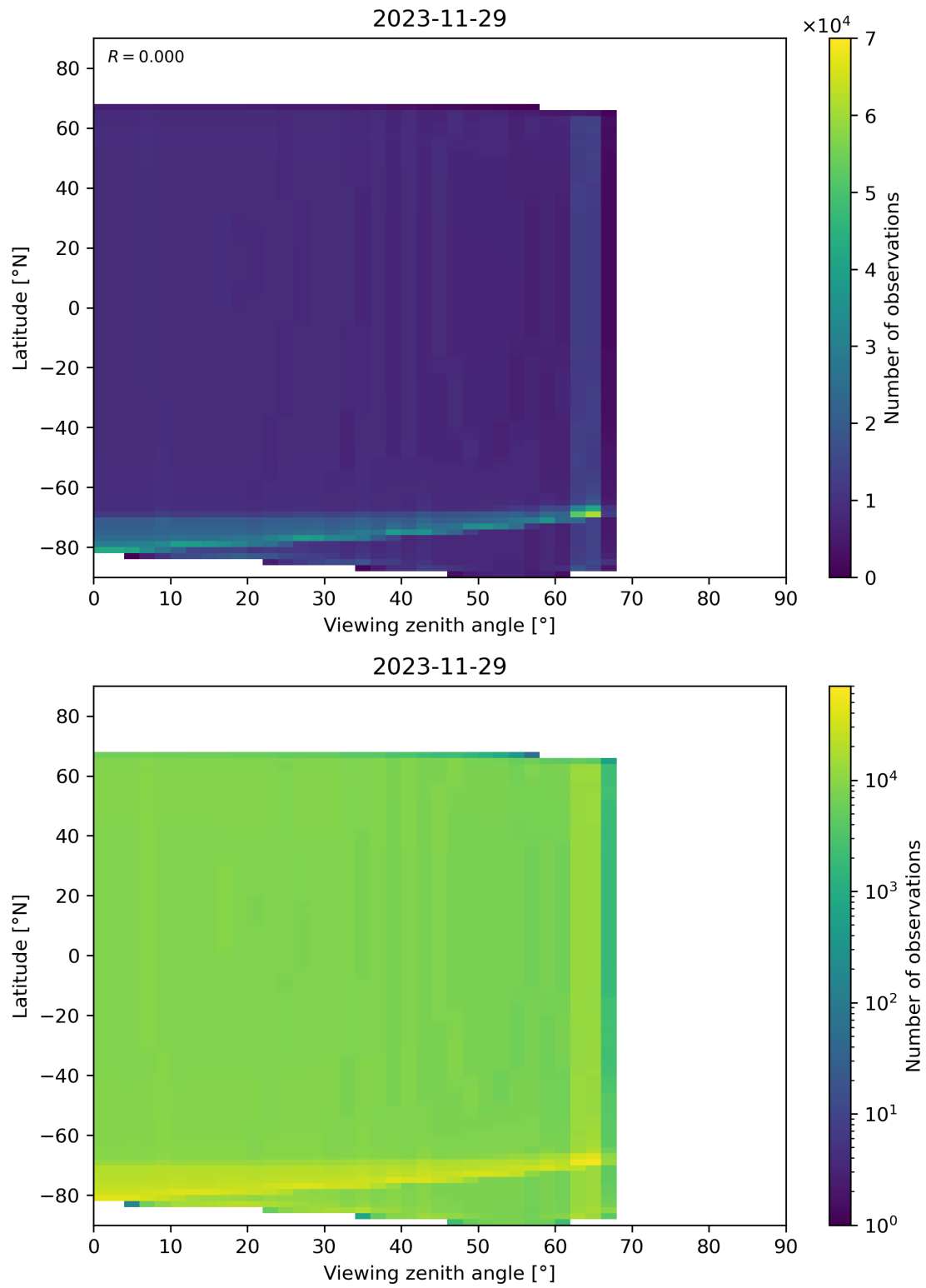
Figure 49: Scatter density plot of “Viewing zenith angle” against “Latitude” for 2023-11-28 to 2023-11-30.
