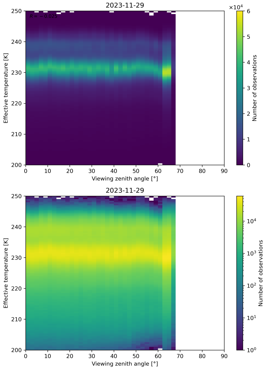
Figure 50: Scatter density plot of “Viewing zenith angle” against “Effective temperature” for 2023-11-28 to 2023-11-30.
