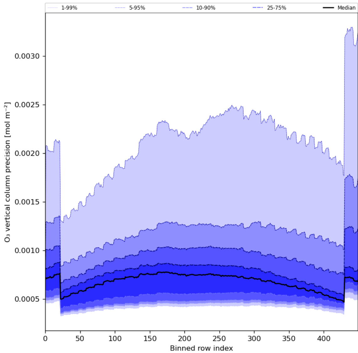
Figure 29: Along track statistics of “O 3 vertical column precision” for 2023-11-28 to 2023-11-30
