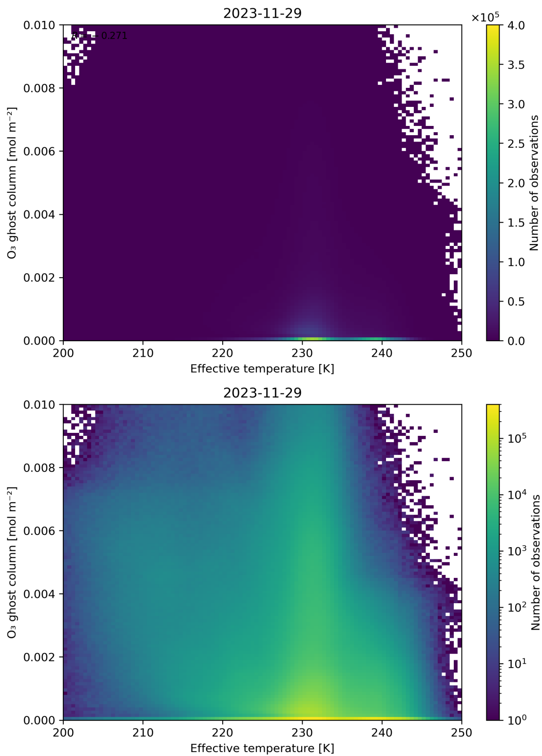
Figure 38: Scatter density plot of “Effective temperature” against “O 3 ghost column” for 2023-11-28 to 2023-11-30.
