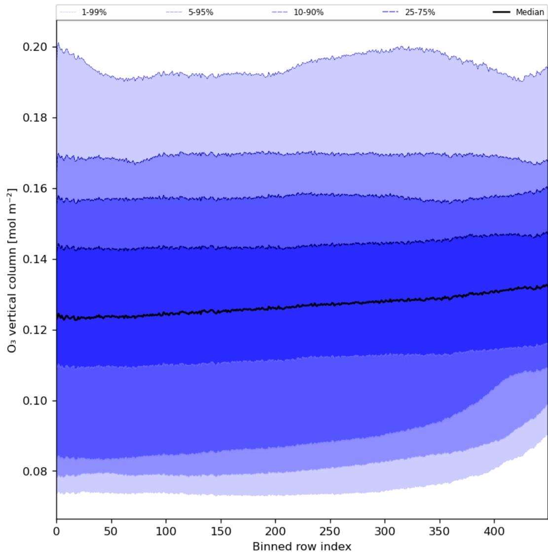
Figure 28: Along track statistics of “O 3 vertical column” for 2023-11-28 to 2023-11-30
