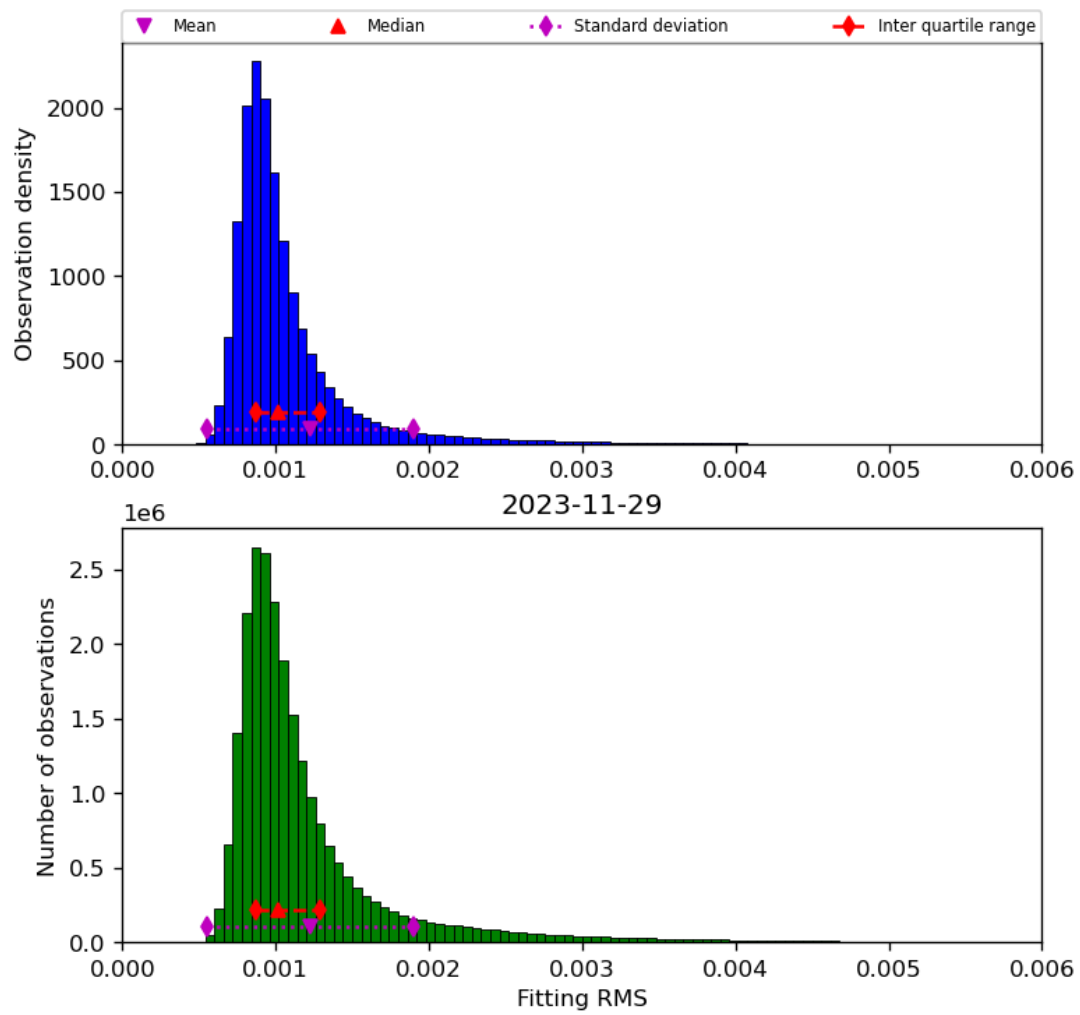
Figure 23: Histogram of “Fitting RMS” for 2023-11-28 to 2023-11-30
