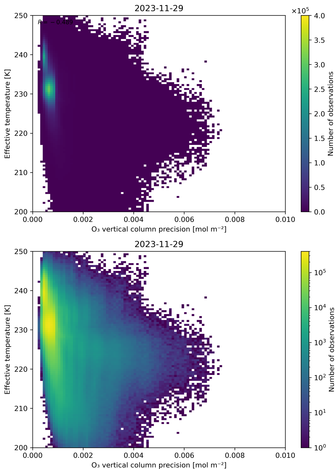
Figure 42: Scatter density plot of “O 3 vertical column precision” against “Effective temperature” for 2023-11-28 to 2023-11-30.
