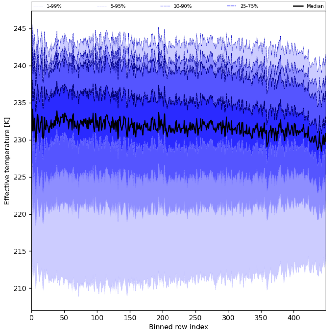
Figure 31: Along track statistics of “Effective temperature” for 2023-11-28 to 2023-11-30
