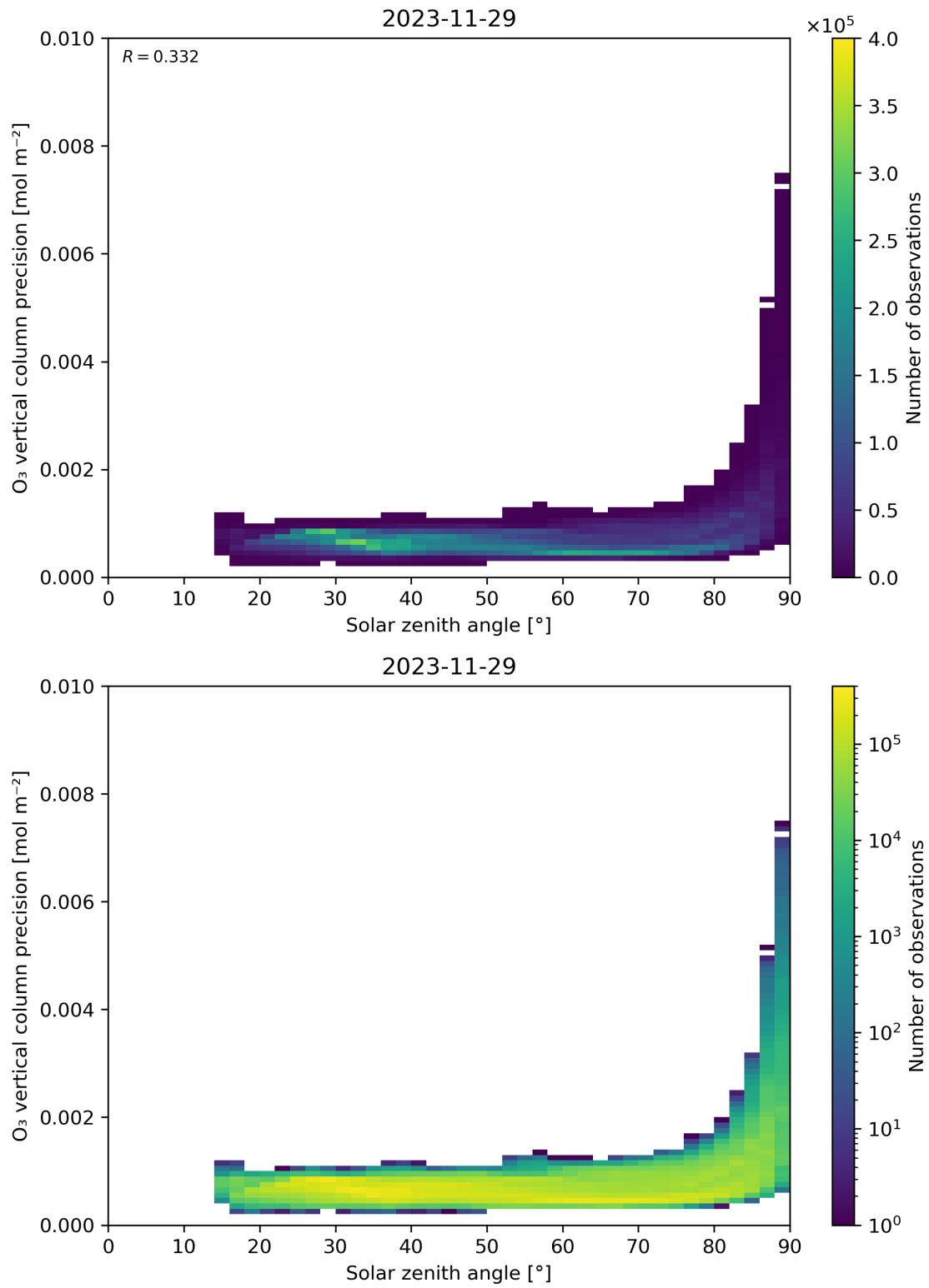
Figure 48: Scatter density plot of “Solar zenith angle” against “O 3 vertical column precision” for 2023-11-28 to 2023-11-30.
