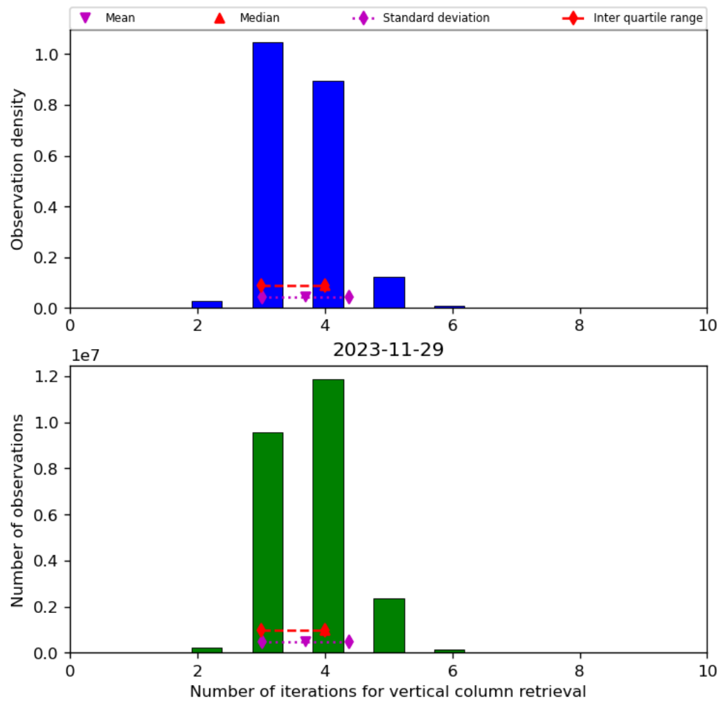
Figure 26: Histogram of “Number of iterations for vertical column retrieval” for 2023-11-28 to 2023-11-30
