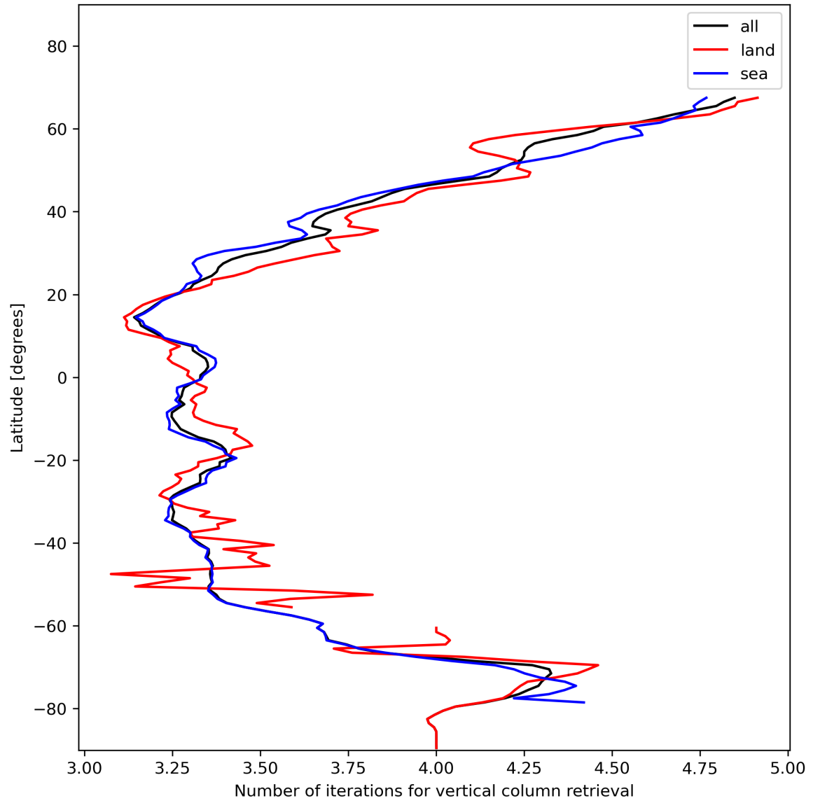
Figure 19: Zonal average of “Number of iterations for vertical column retrieval” for 2023-11-28 to 2023-11-30.
