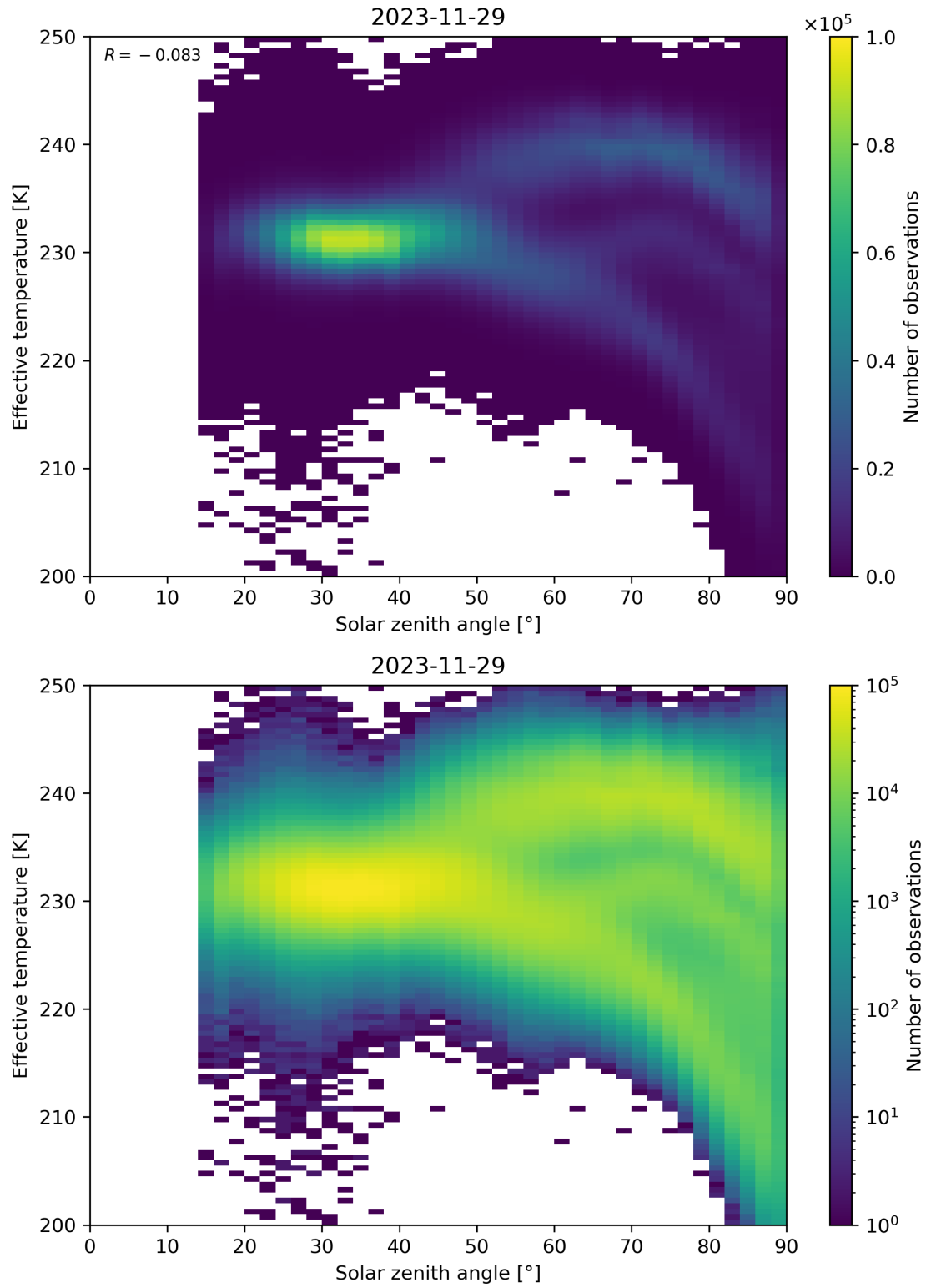
Figure 45: Scatter density plot of “Solar zenith angle” against “Effective temperature” for 2023-11-28 to 2023-11-30.
