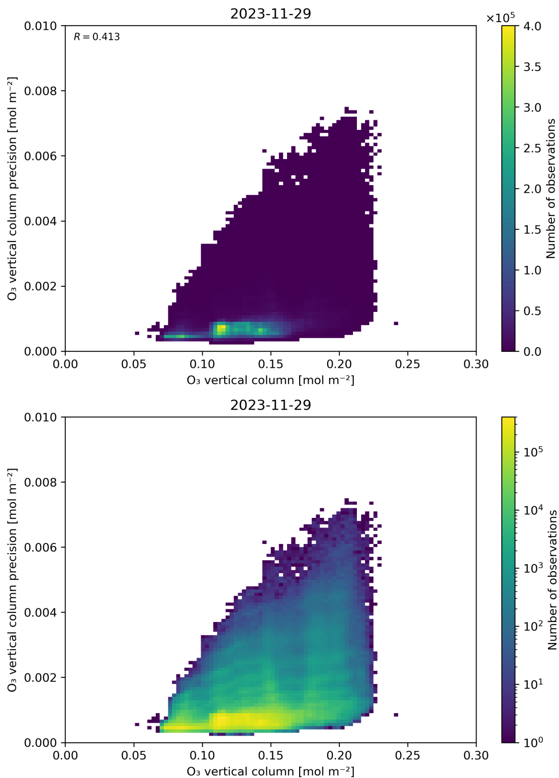
Figure 41: Scatter density plot of “O 3 vertical column” against “O 3 vertical column precision” for 2023-11-28 to 2023-11-30.
