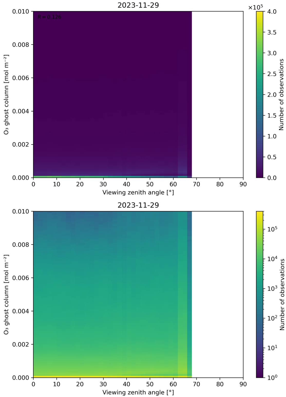
Figure 51: Scatter density plot of “Viewing zenith angle” against “O 3 ghost column” for 2023-11-28 to 2023-11-30.
