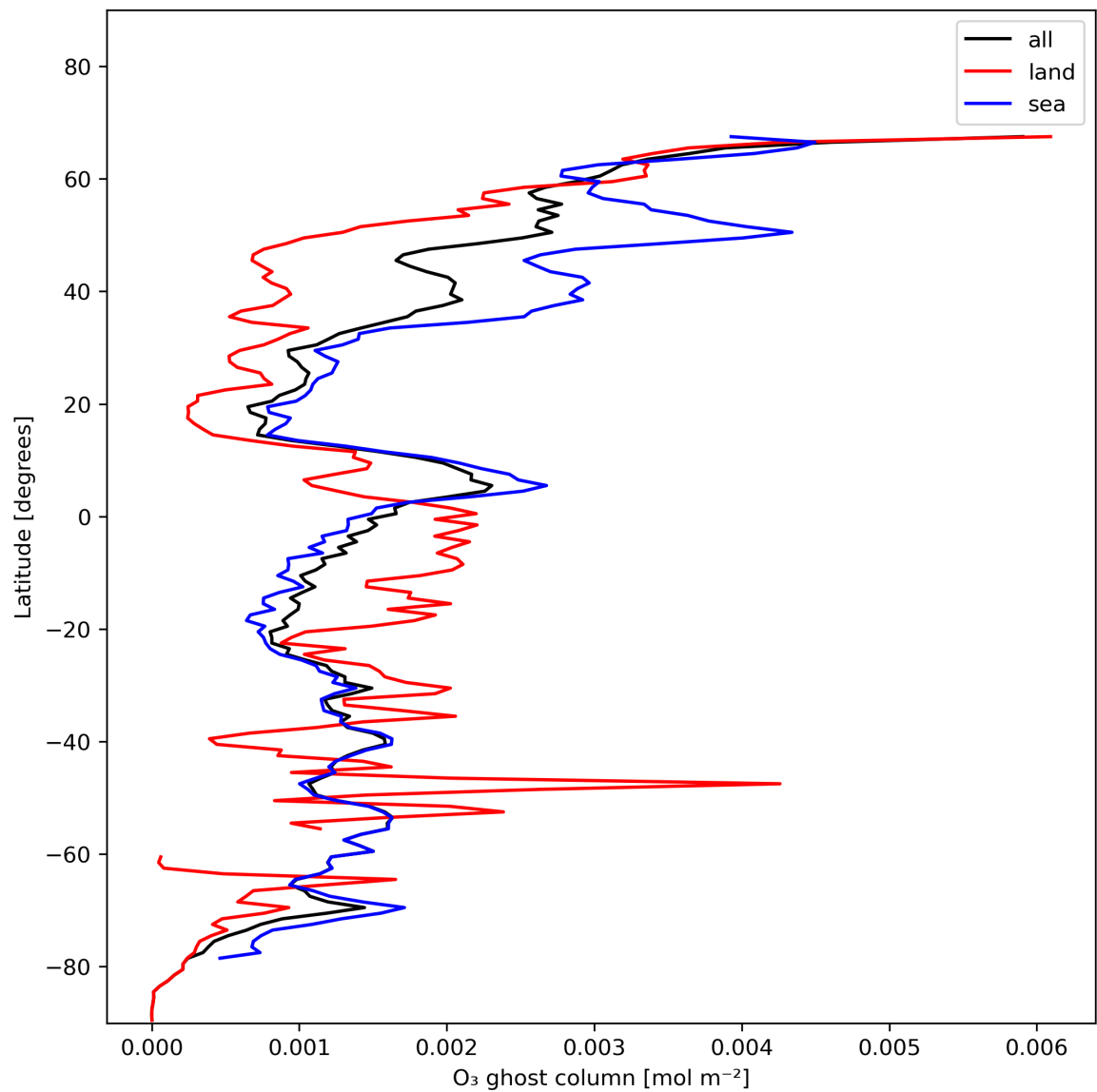
Figure 18: Zonal average of “O 3 ghost column” for 2023-11-28 to 2023-11-30.
