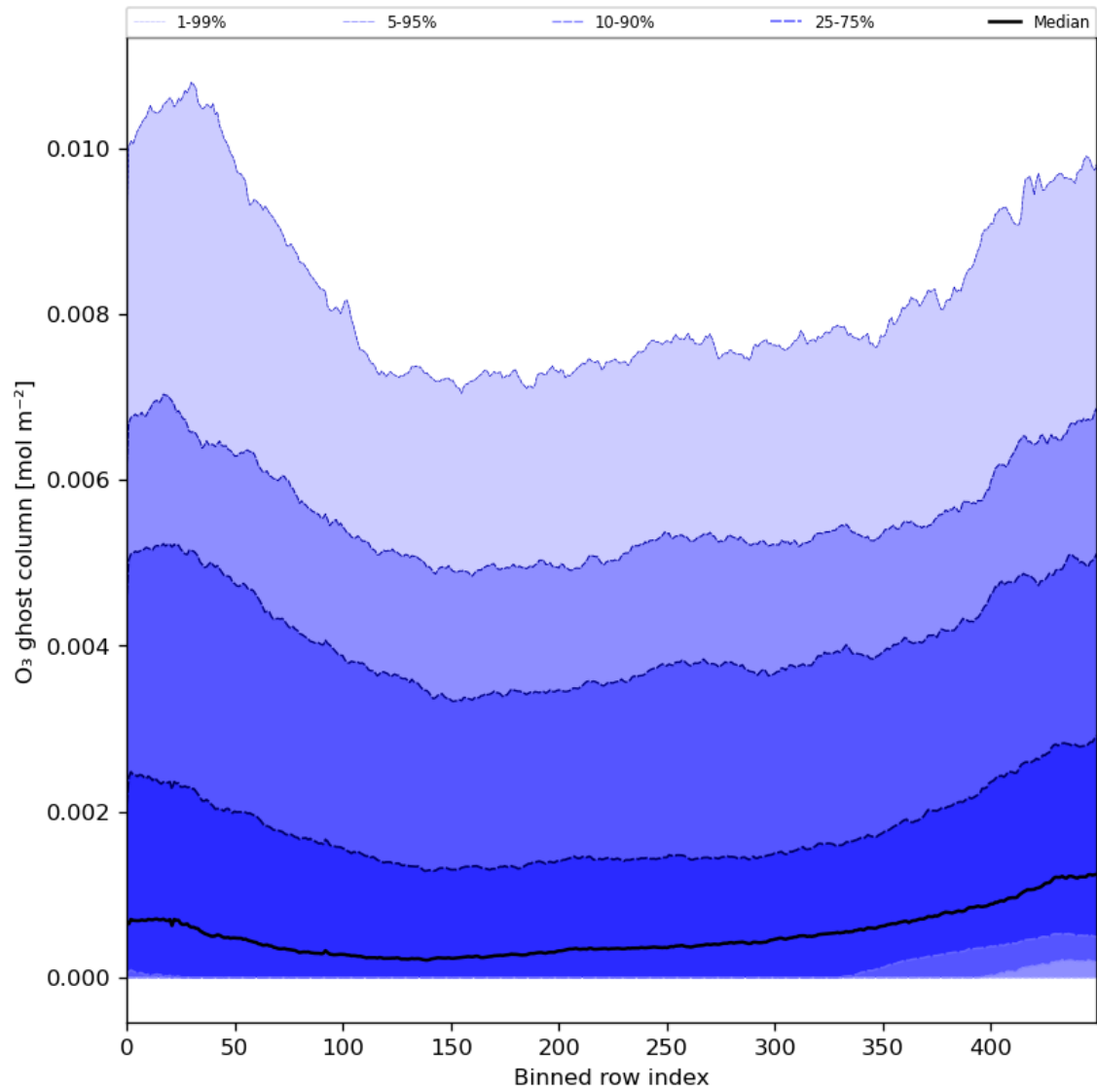
Figure 32: Along track statistics of “O 3 ghost column” for 2023-11-28 to 2023-11-30
