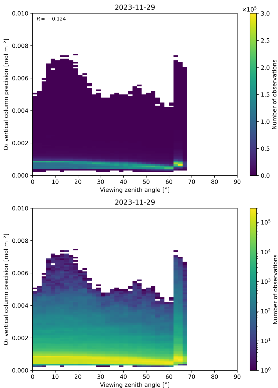
Figure 53: Scatter density plot of “Viewing zenith angle” against “O 3 vertical column precision” for 2023-11-28 to 2023-11-30.
