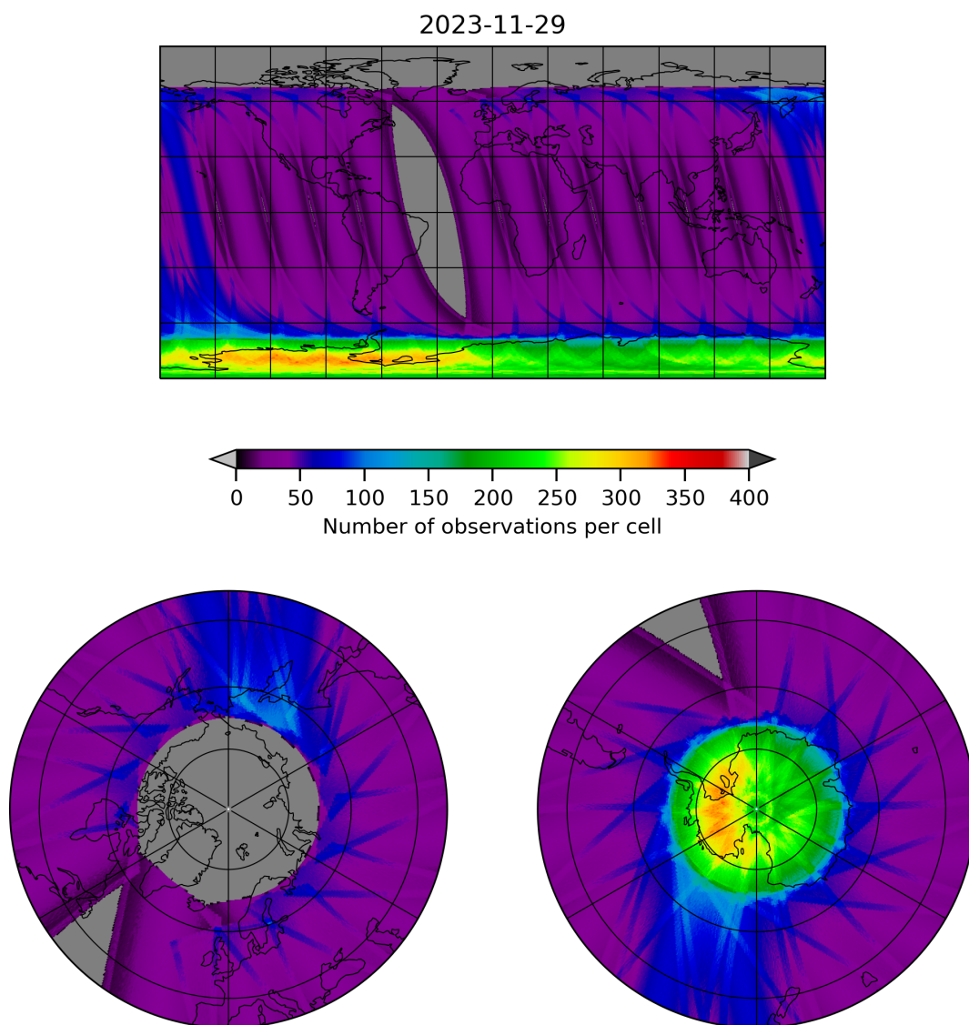
Figure 12: Map of the number of observations for 2023-11-28 to 2023-11-30
