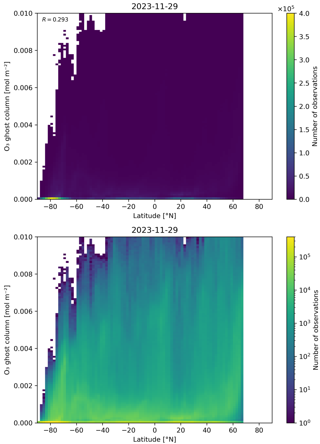
Figure 35: Scatter density plot of “Latitude” against “O 3 ghost column” for 2023-11-28 to 2023-11-30.
