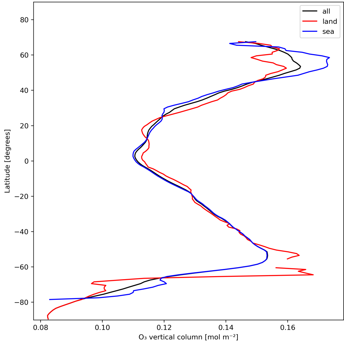
Figure 14: Zonal average of “O 3 vertical column” for 2023-11-28 to 2023-11-30.
