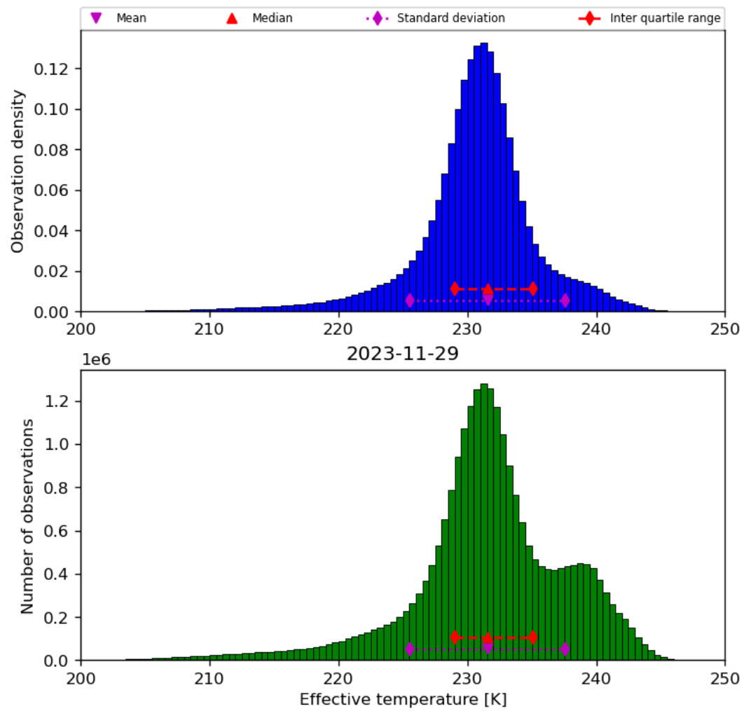
Figure 24: Histogram of “Effective temperature” for 2023-11-28 to 2023-11-30
