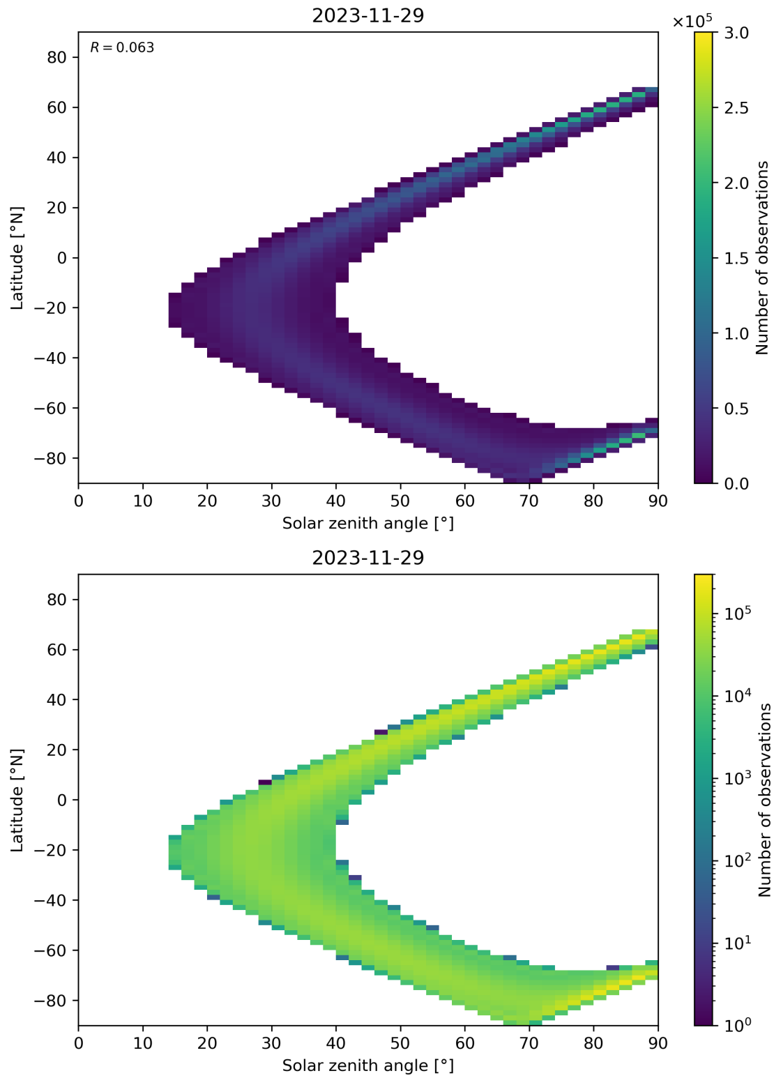
Figure 44: Scatter density plot of “Solar zenith angle” against “Latitude” for 2023-11-28 to 2023-11-30.
