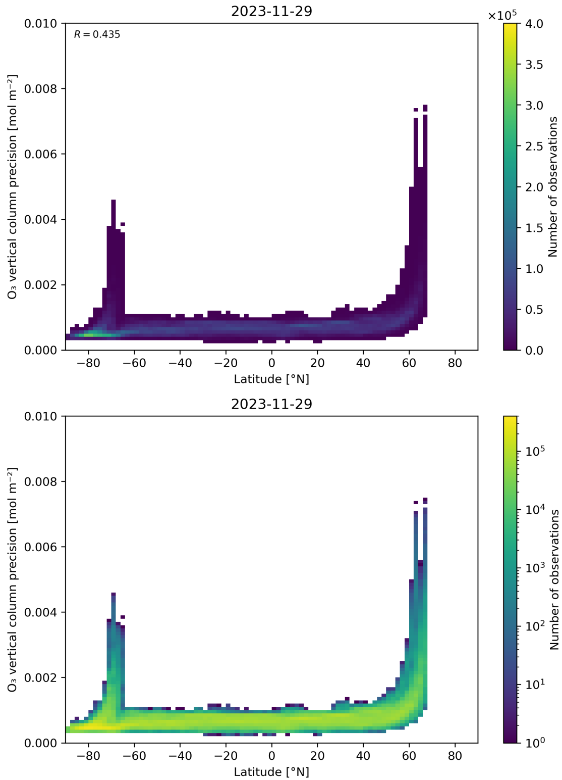
Figure 37: Scatter density plot of “Latitude” against “O 3 vertical column precision” for 2023-11-28 to 2023-11-30.
