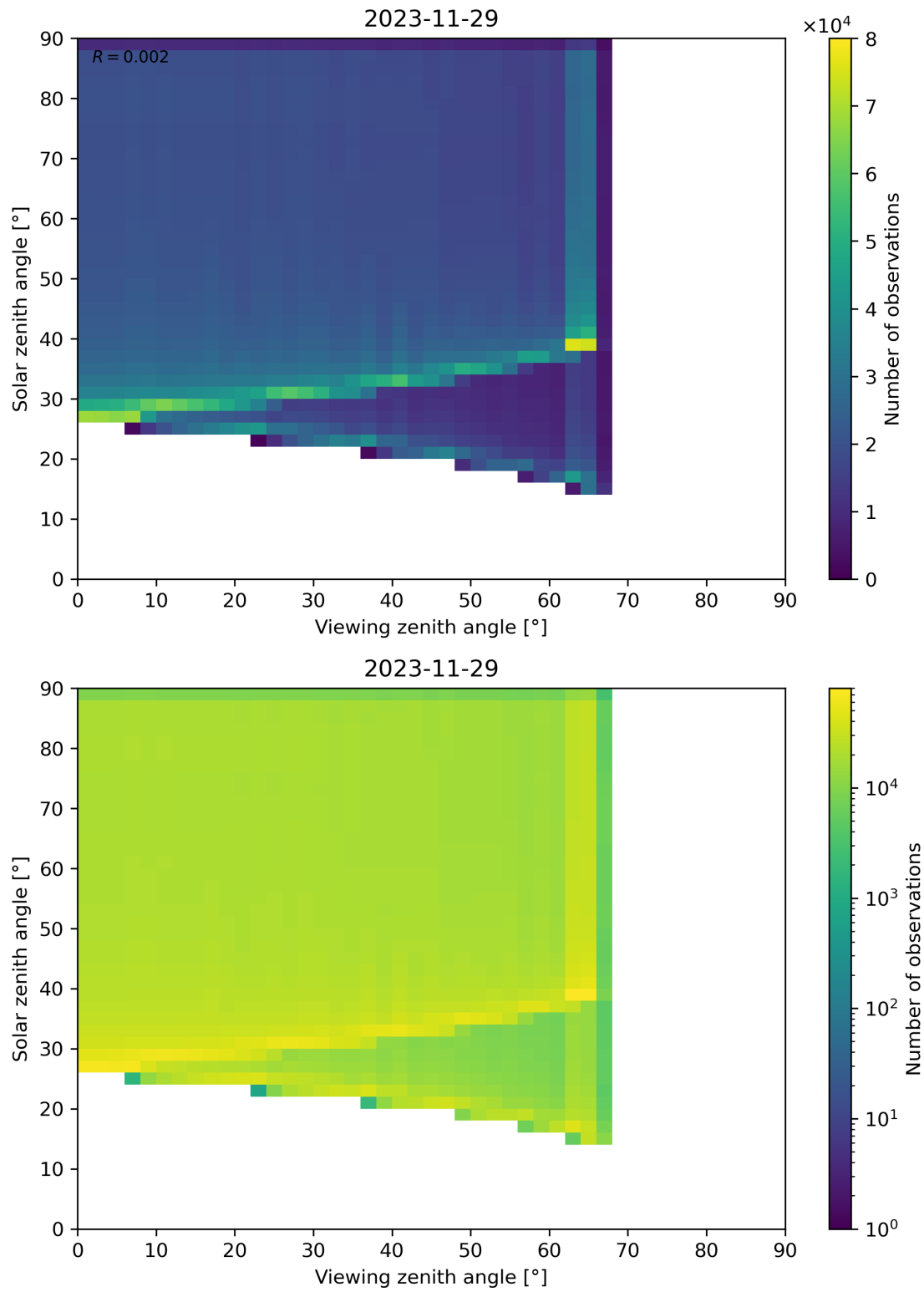
Figure 54: Scatter density plot of “Viewing zenith angle” against “Solar zenith angle” for 2023-11-28 to 2023-11-30.
