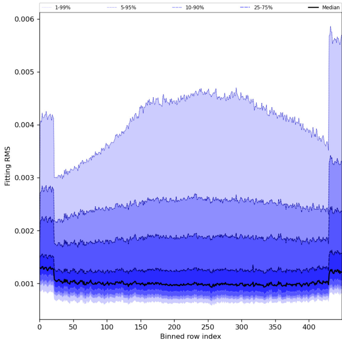
Figure 30: Along track statistics of “Fitting RMS” for 2023-11-28 to 2023-11-30
