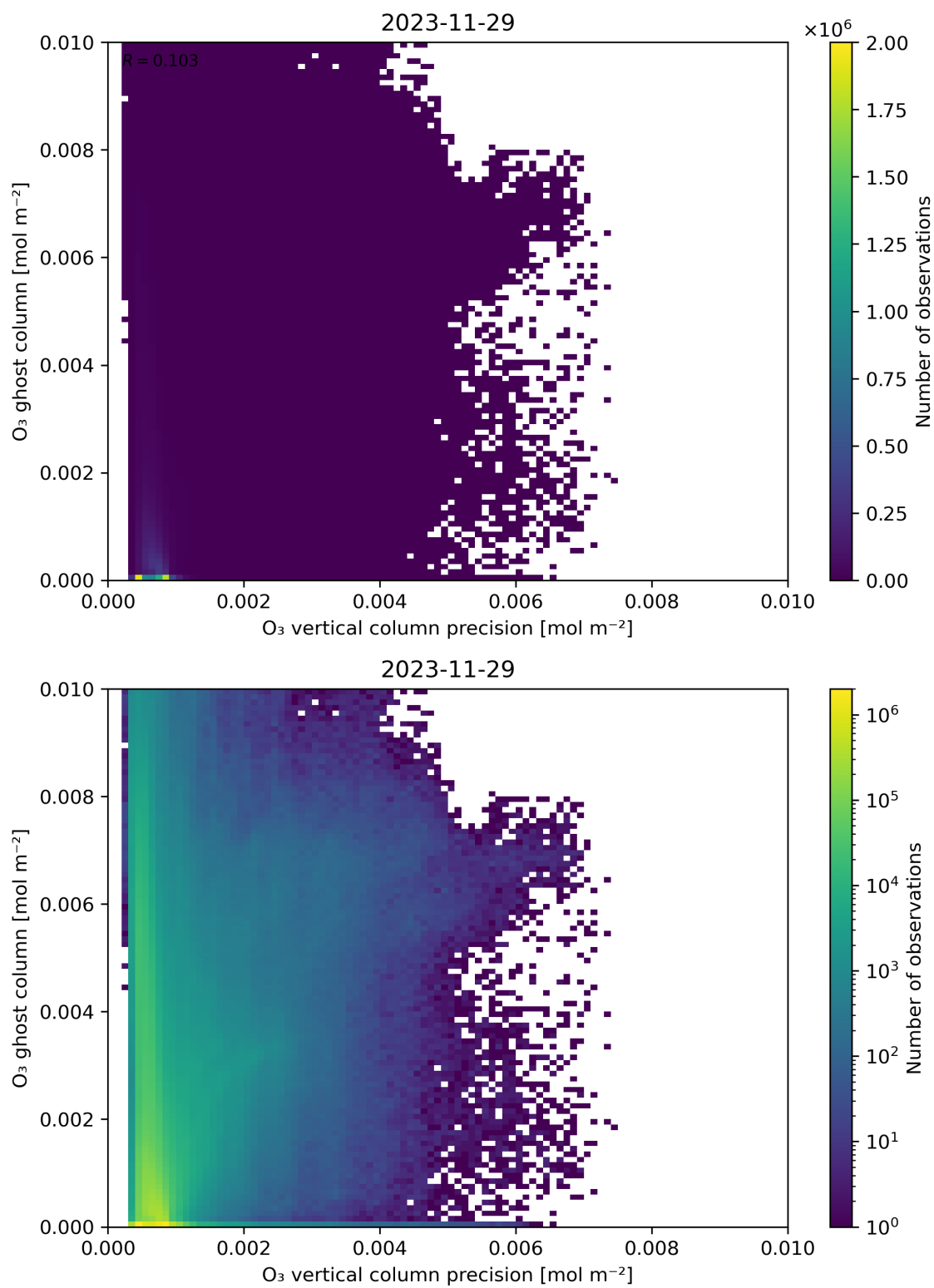
Figure 43: Scatter density plot of “ \text{O}_3 vertical column precision” against “ \text{O}_3 ghost column” for 2023-11-28 to 2023-11-30.
