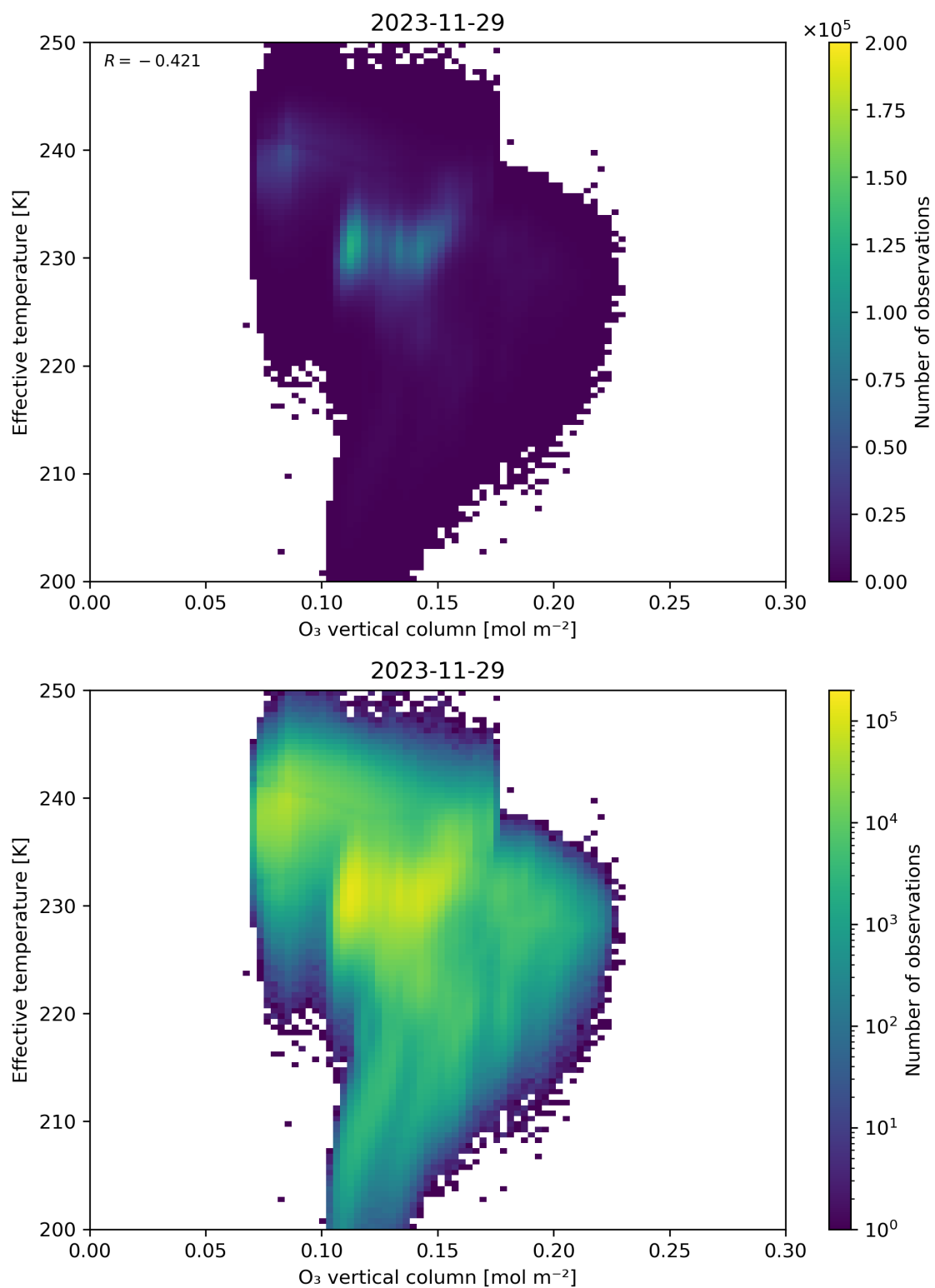
Figure 39: Scatter density plot of “O 3 vertical column” against “Effective temperature” for 2023-11-28 to 2023-11-30.
