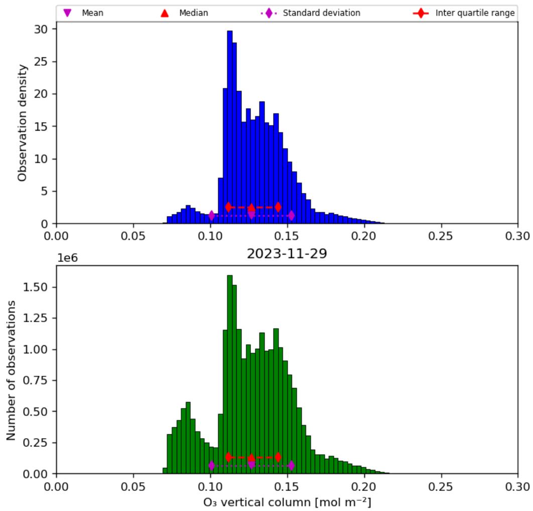
Figure 21: Histogram of “O 3 vertical column” for 2023-11-28 to 2023-11-30
