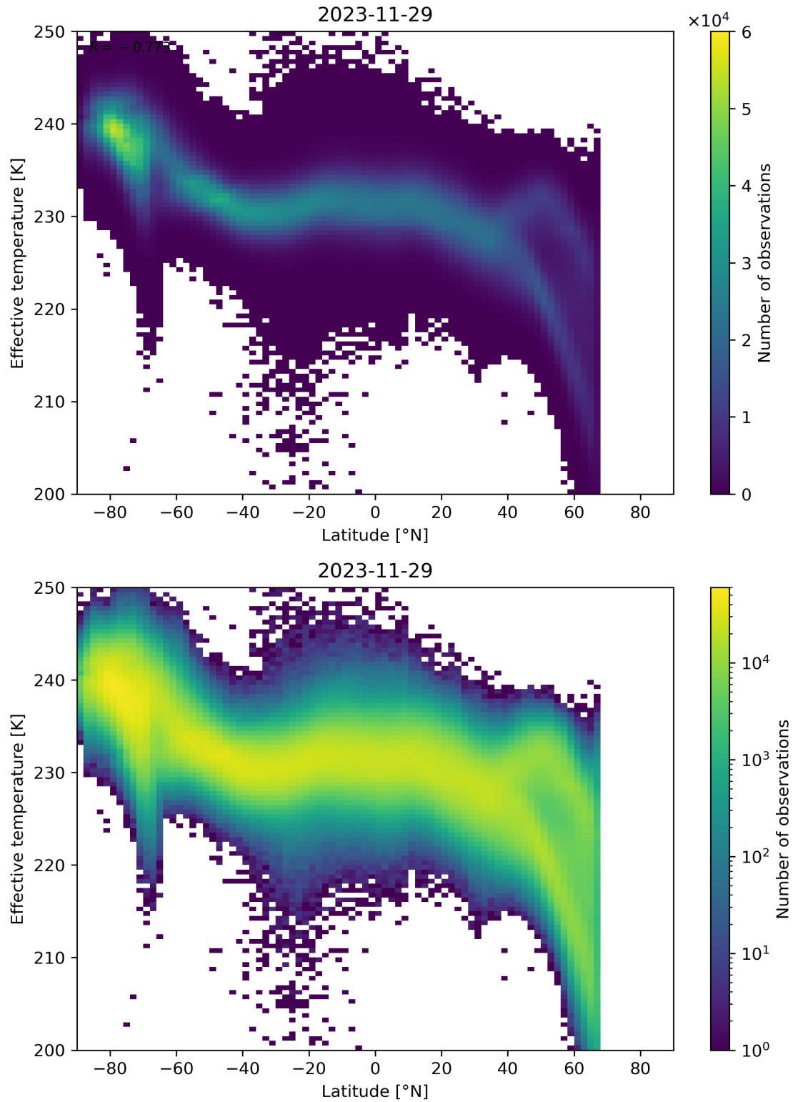
Figure 34: Scatter density plot of “Latitude” against “Effective temperature” for 2023-11-28 to 2023-11-30.
