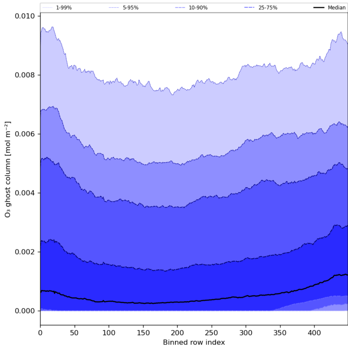
Figure 32: Along track statistics of “O 3 ghost column” for 2023-11-29 to 2023-12-01
