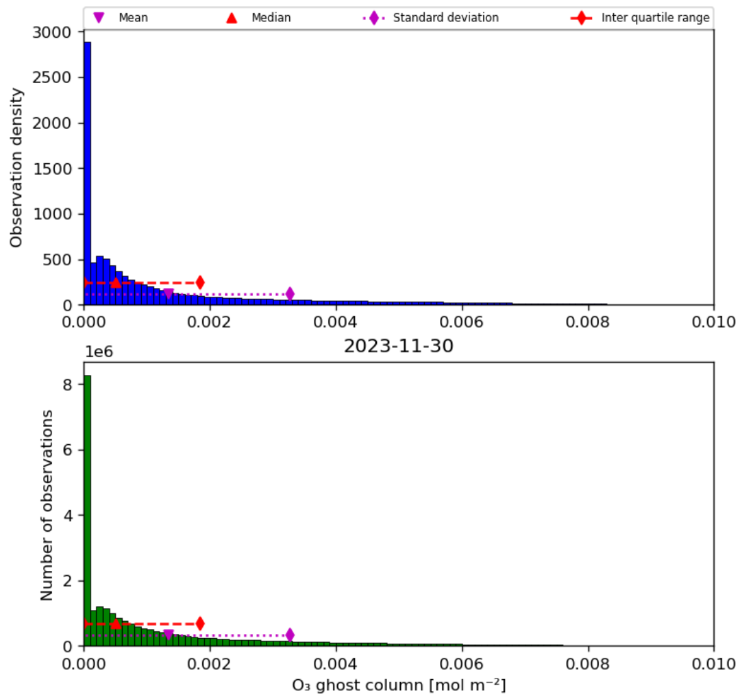
Figure 25: Histogram of “O 3 ghost column” for 2023-11-29 to 2023-12-01
