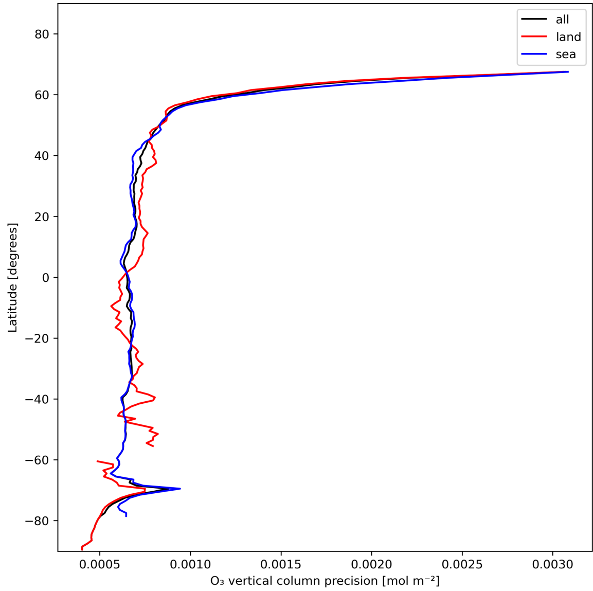
Figure 15: Zonal average of “O 3 vertical column precision” for 2023-11-29 to 2023-12-01.
