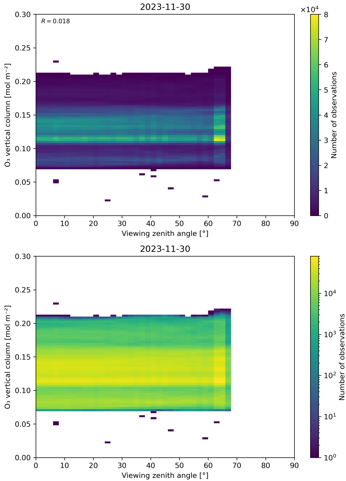
Figure 52: Scatter density plot of “Viewing zenith angle” against “O 3 vertical column” for 2023-11-29 to 2023-12-01.
