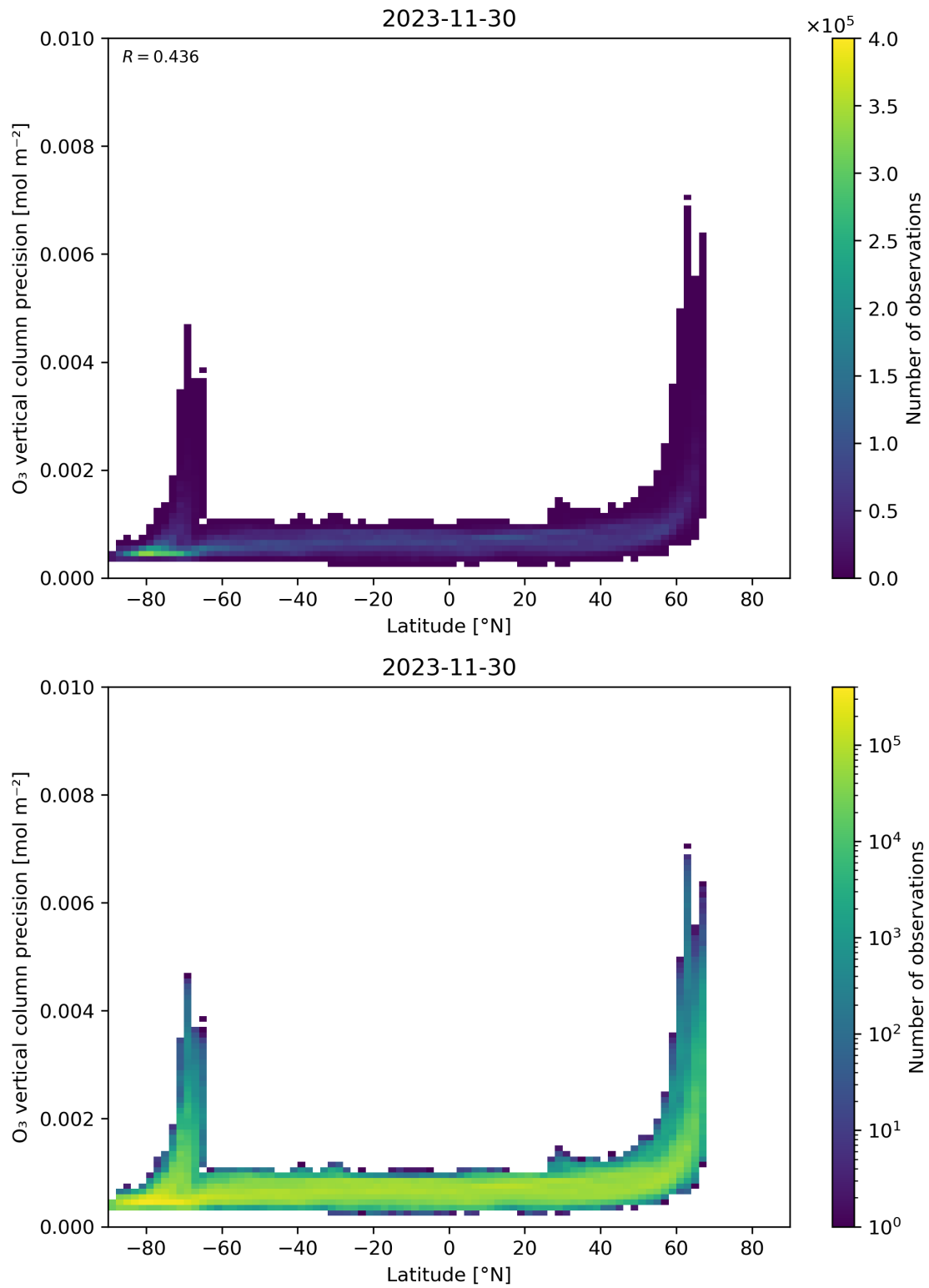
Figure 37: Scatter density plot of “Latitude” against “O 3 vertical column precision” for 2023-11-29 to 2023-12-01.
