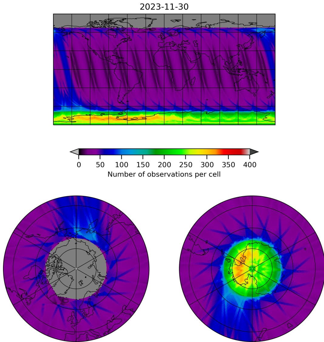
Figure 12: Map of the number of observations for 2023-11-29 to 2023-12-01
