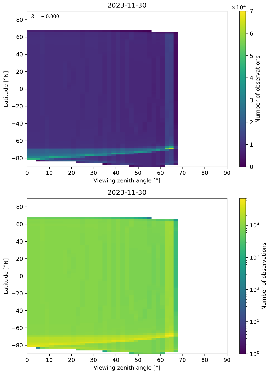
Figure 49: Scatter density plot of “Viewing zenith angle” against “Latitude” for 2023-11-29 to 2023-12-01.
