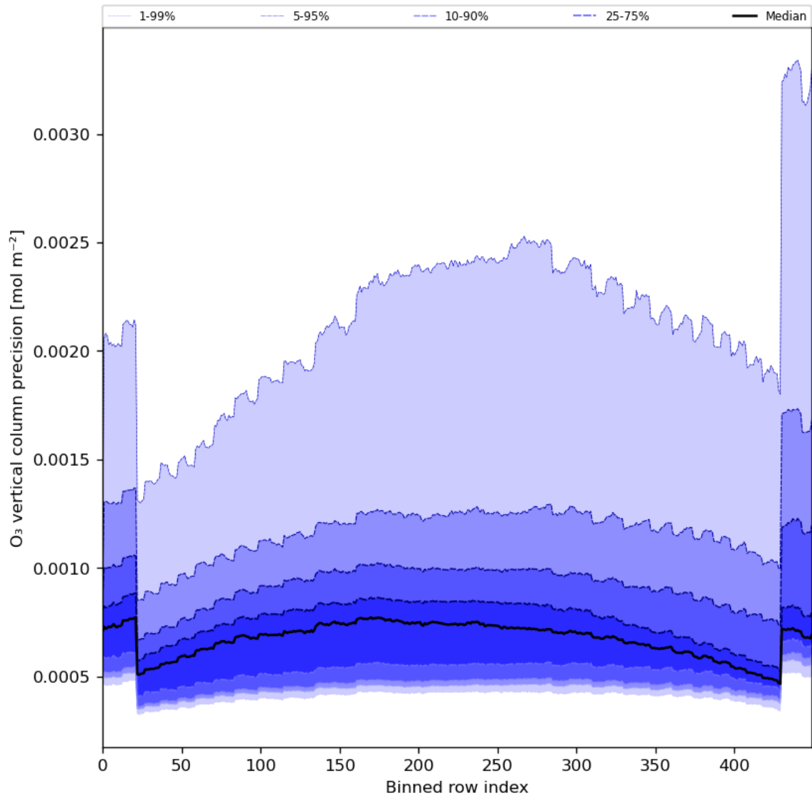
Figure 29: Along track statistics of “O 3 vertical column precision” for 2023-11-29 to 2023-12-01
