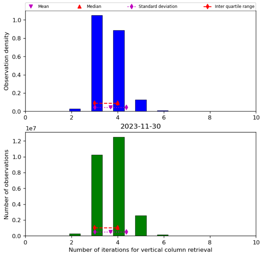
Figure 26: Histogram of “Number of iterations for vertical column retrieval” for 2023-11-29 to 2023-12-01
