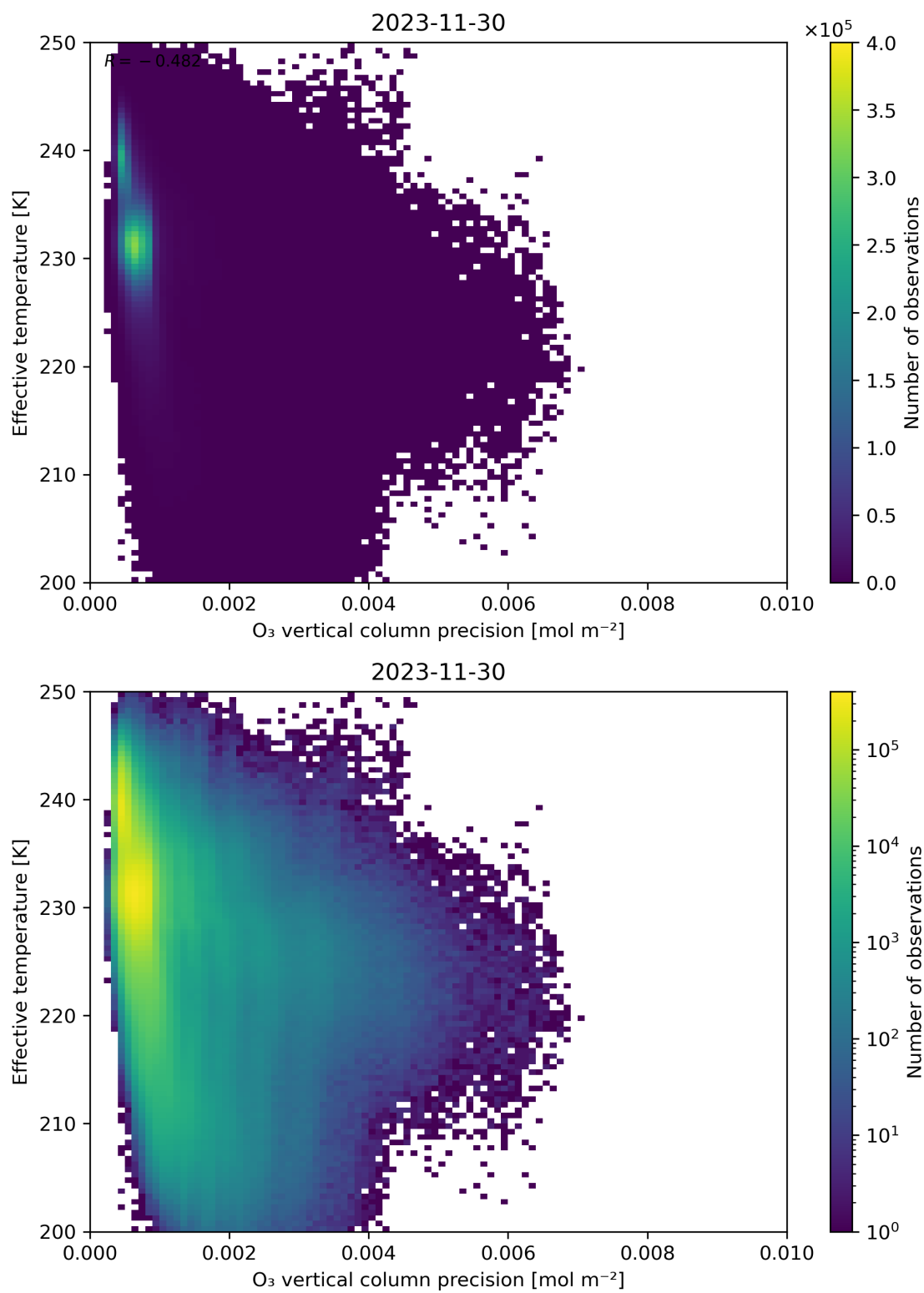
Figure 42: Scatter density plot of “O 3 vertical column precision” against “Effective temperature” for 2023-11-29 to 2023-12-01.
