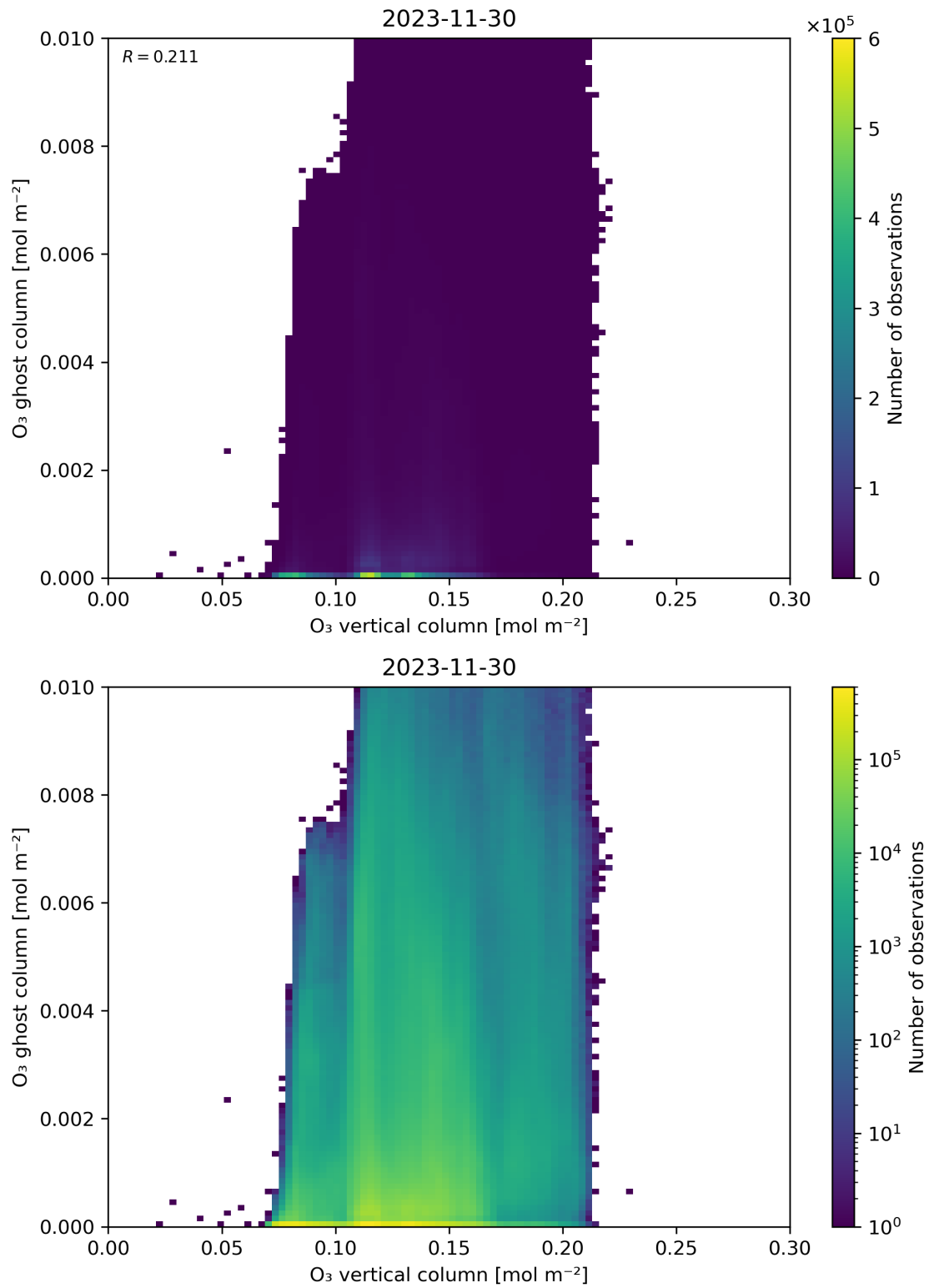
Figure 40: Scatter density plot of “O 3 vertical column” against “O 3 ghost column” for 2023-11-29 to 2023-12-01.
