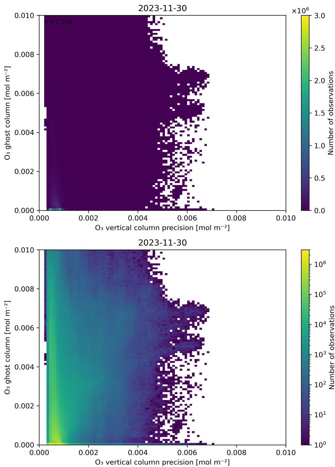
Figure 43: Scatter density plot of “ O_3 vertical column precision” against “ O_3 ghost column” for 2023-11-29 to 2023-12-01.
