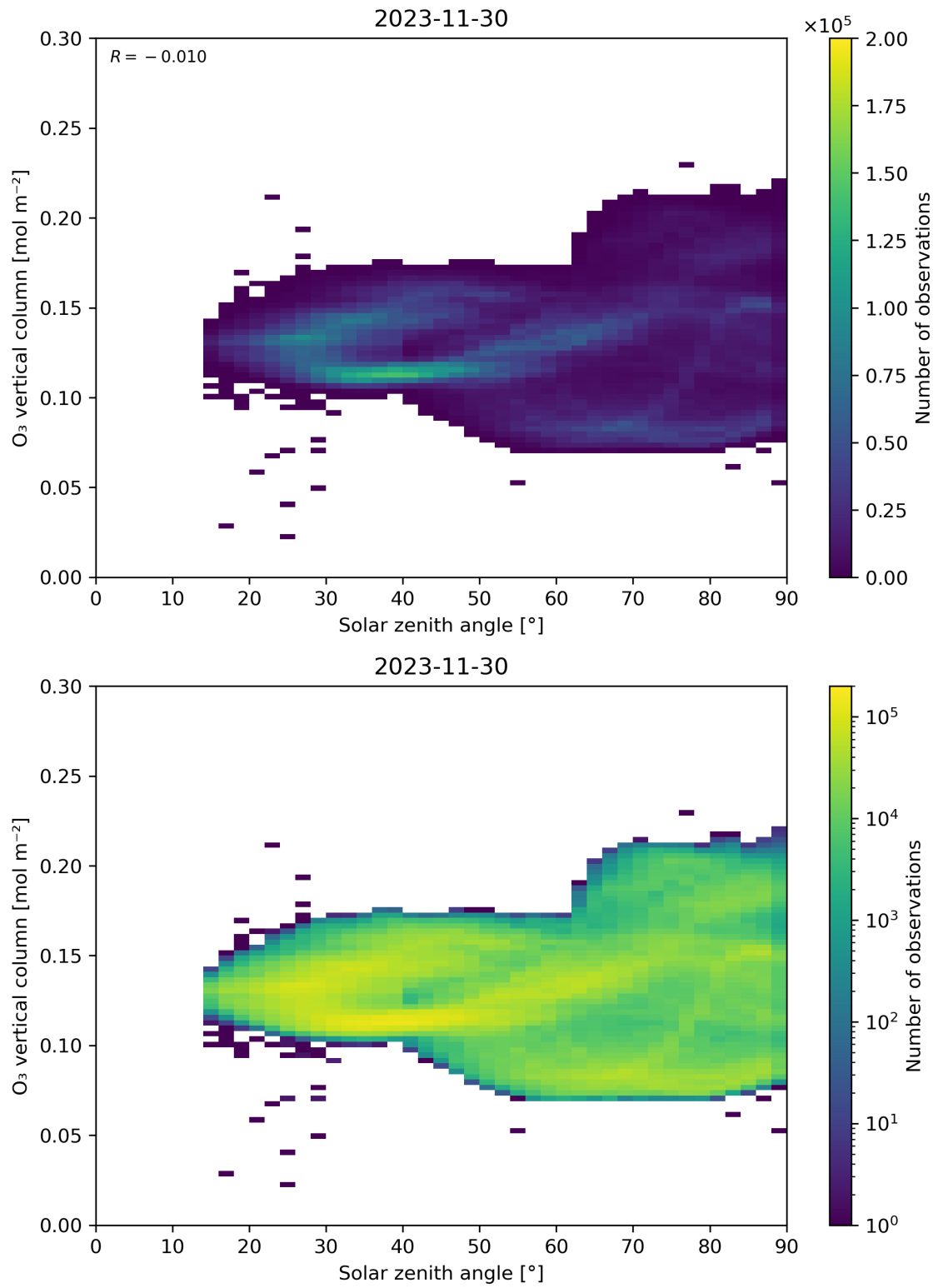
Figure 47: Scatter density plot of “Solar zenith angle” against “O 3 vertical column” for 2023-11-29 to 2023-12-01.
