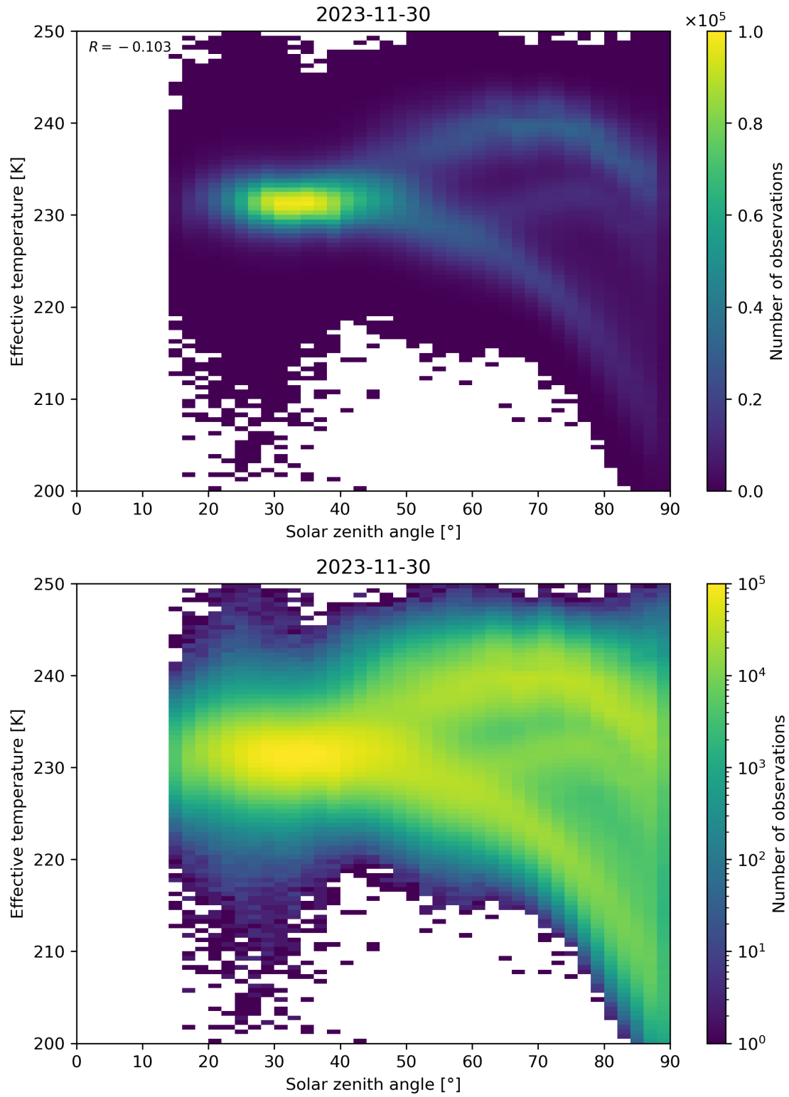
Figure 45: Scatter density plot of “Solar zenith angle” against “Effective temperature” for 2023-11-29 to 2023-12-01.
