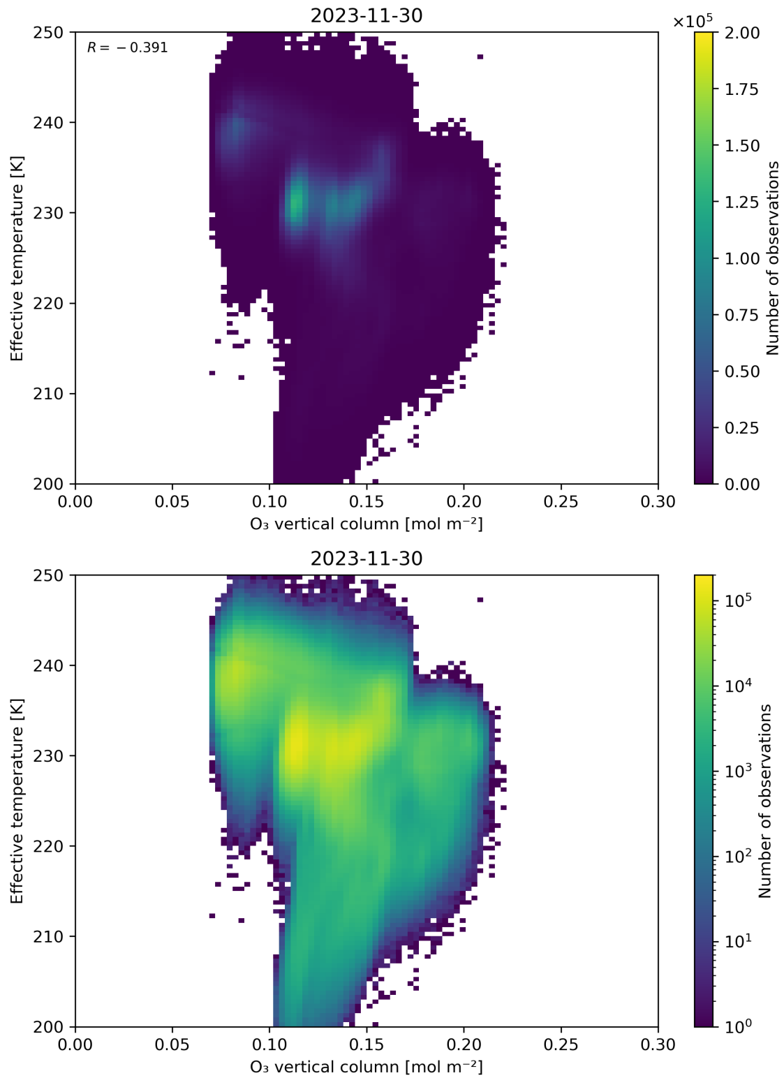
Figure 39: Scatter density plot of “O 3 vertical column” against “Effective temperature” for 2023-11-29 to 2023-12-01.
