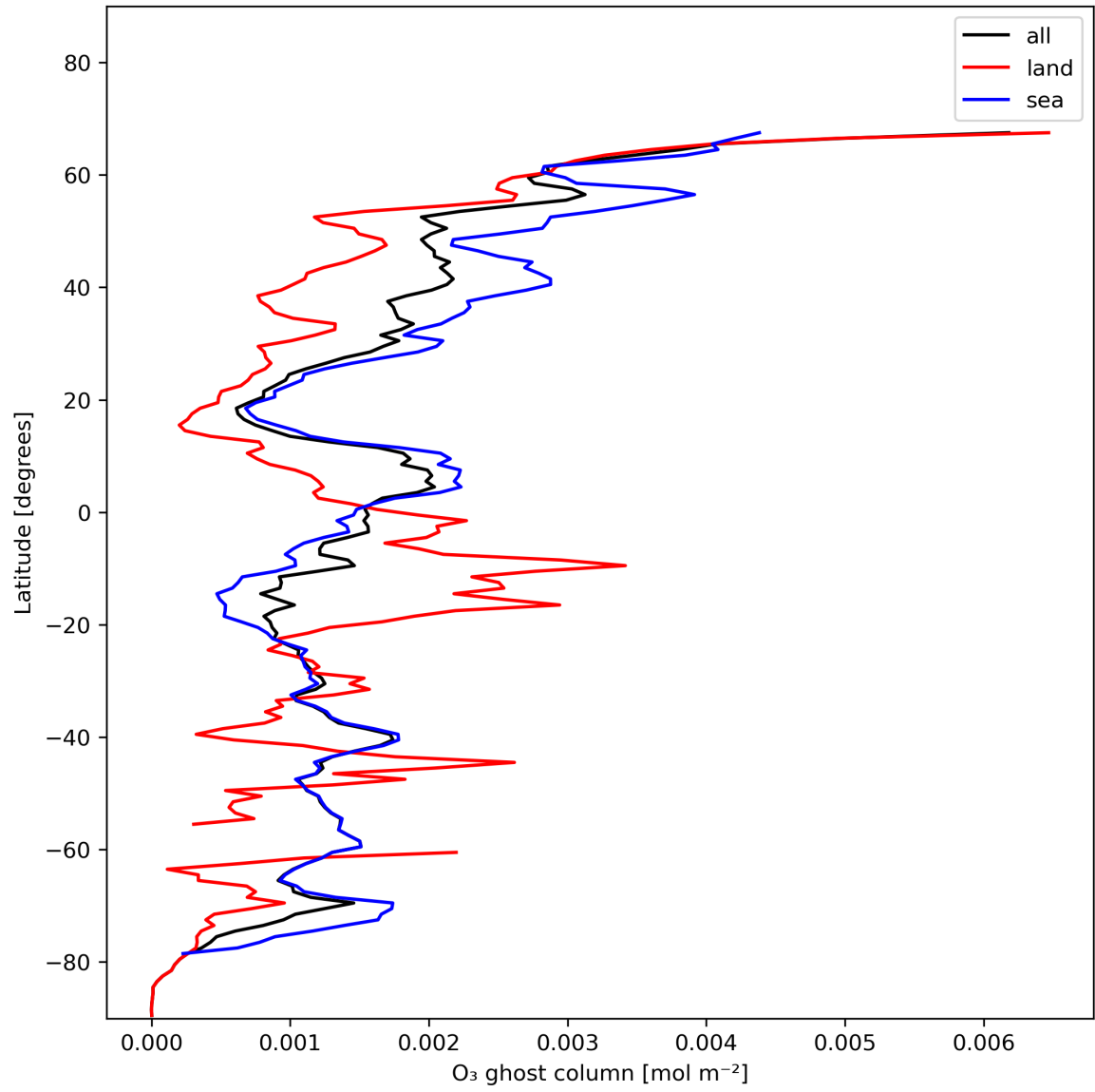
Figure 18: Zonal average of "O 3 ghost column" for 2023-11-29 to 2023-12-01.
