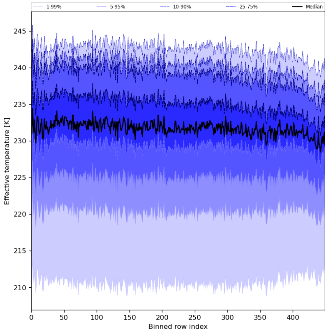
Figure 31: Along track statistics of “Effective temperature” for 2023-11-29 to 2023-12-01
