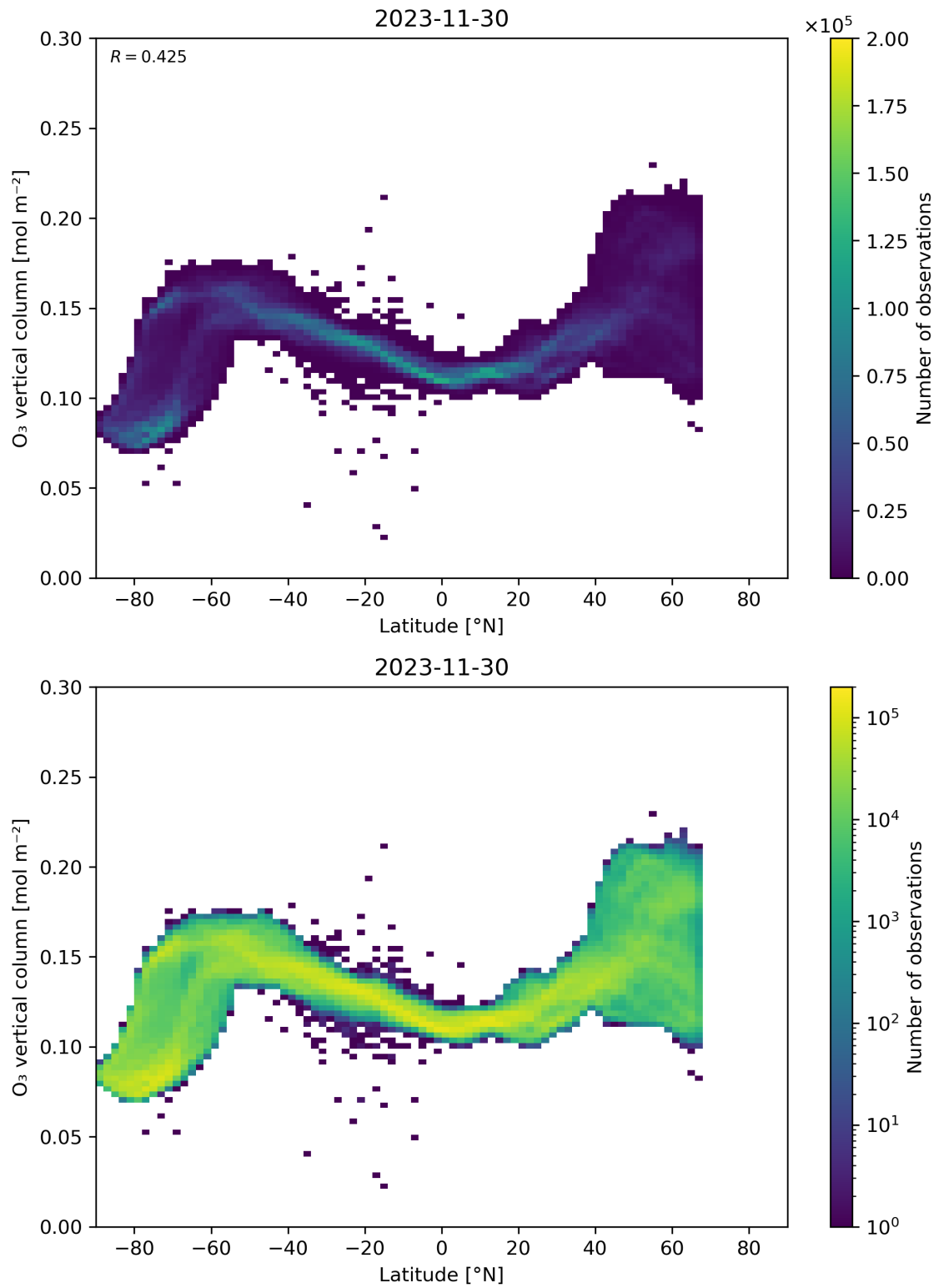
Figure 36: Scatter density plot of “Latitude” against “O 3 vertical column” for 2023-11-29 to 2023-12-01.
