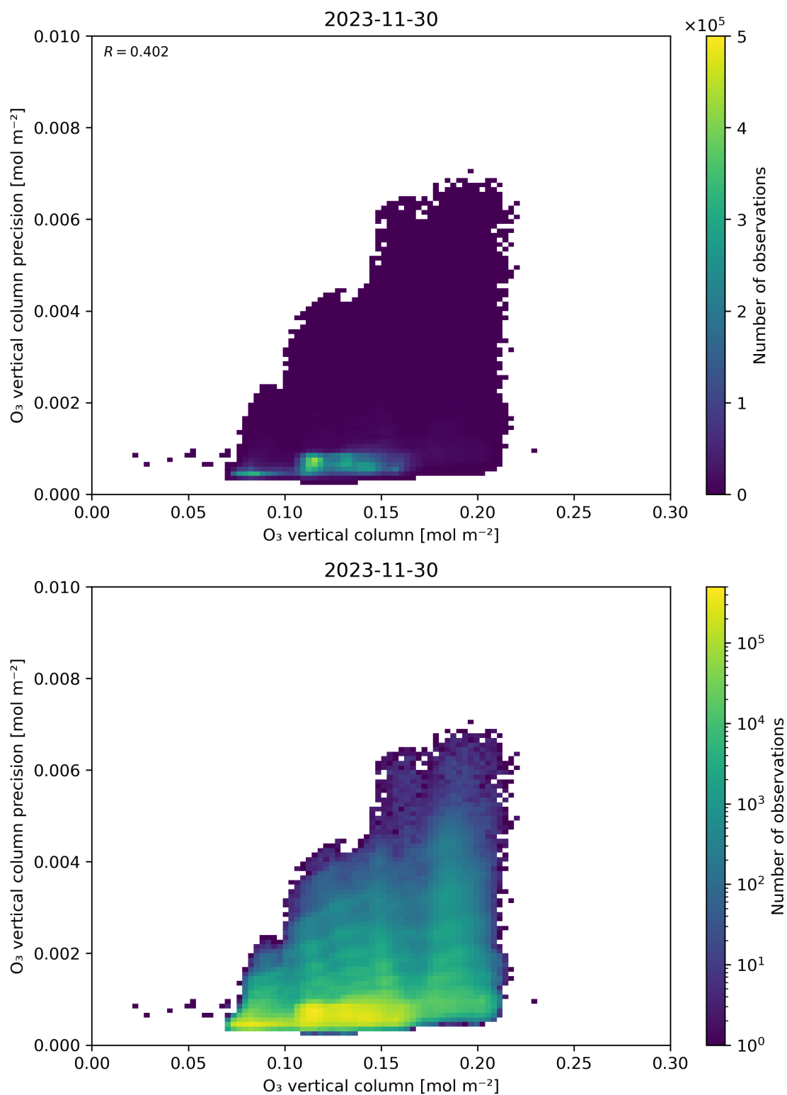
Figure 41: Scatter density plot of “O 3 vertical column” against “O 3 vertical column precision” for 2023-11-29 to 2023-12-01.
