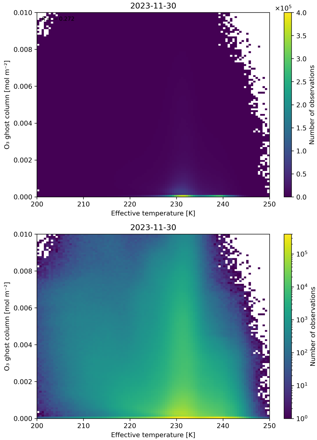
Figure 38: Scatter density plot of “Effective temperature” against “O 3 ghost column” for 2023-11-29 to 2023-12-01.
