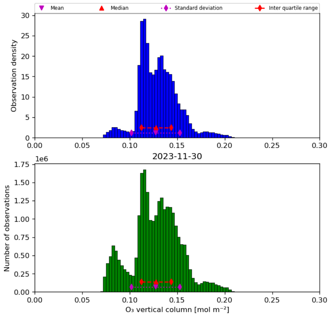
Figure 21: Histogram of “O 3 vertical column” for 2023-11-29 to 2023-12-01
