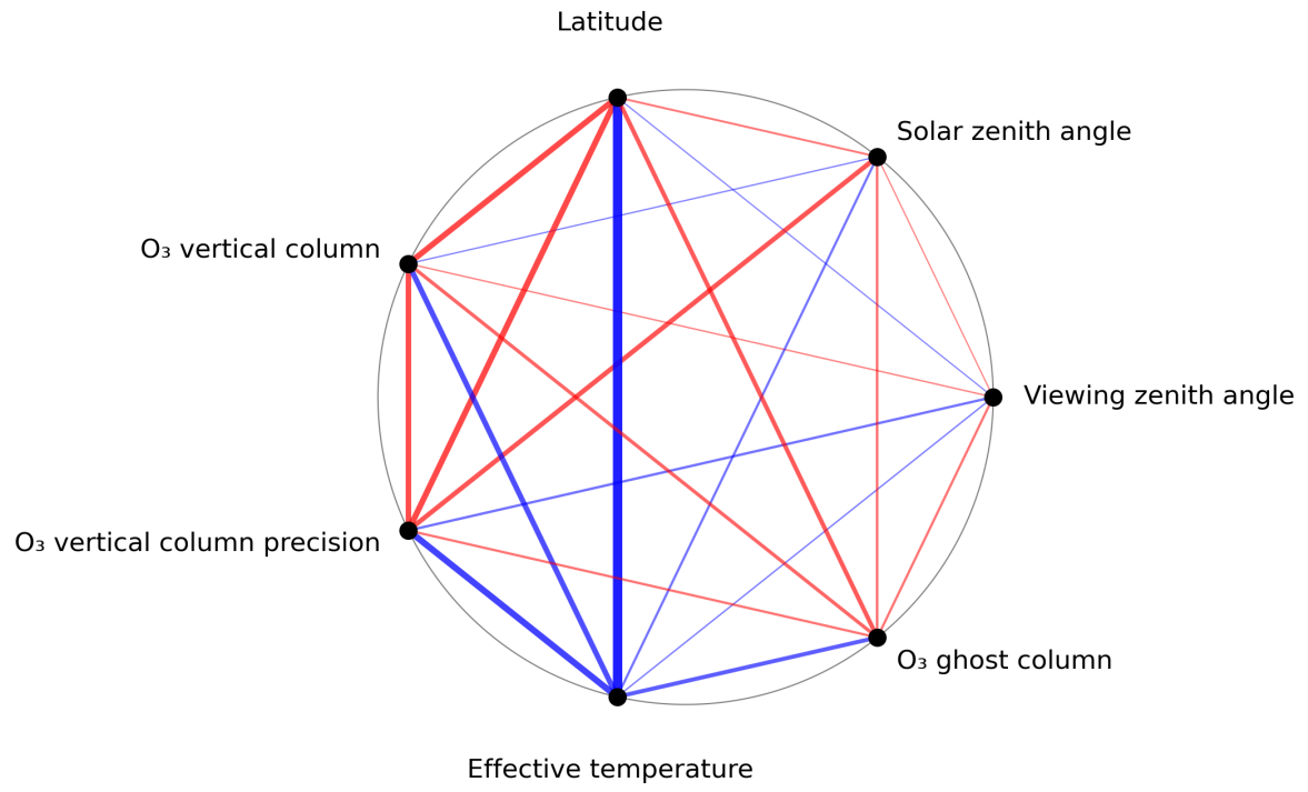
Figure 1: Map of correlation graph for 2023-11-29 to 2023-12-01.
