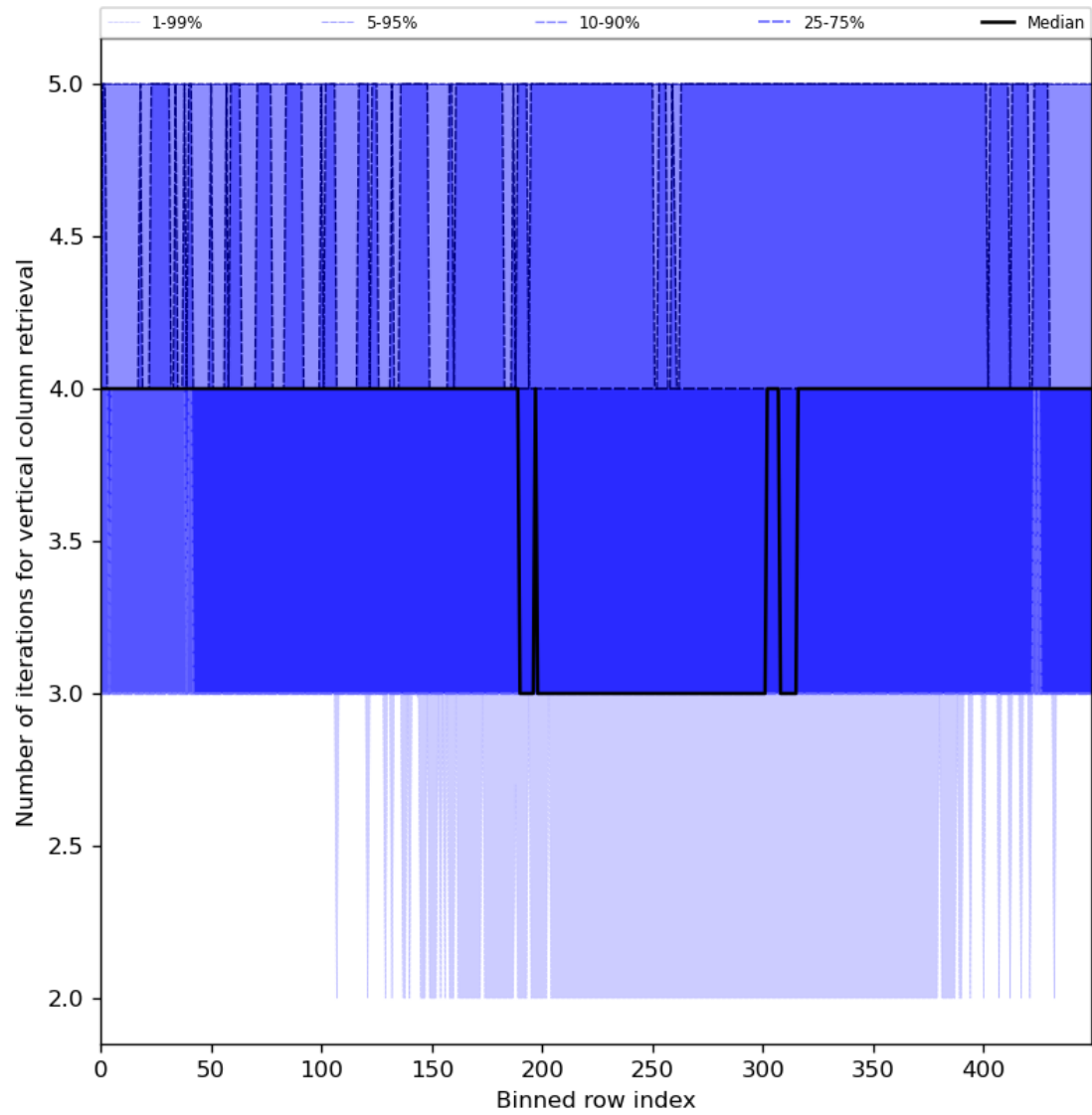
Figure 33: Along track statistics of “Number of iterations for vertical column retrieval” for 2023-11-29 to 2023-12-01
