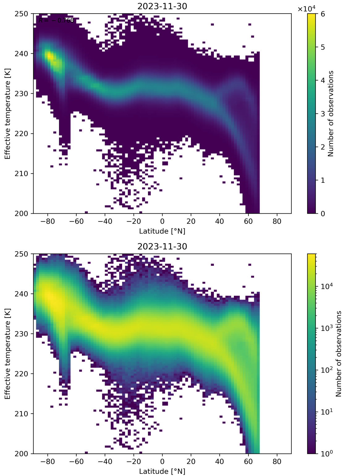
Figure 34: Scatter density plot of “Latitude” against “Effective temperature” for 2023-11-29 to 2023-12-01.
