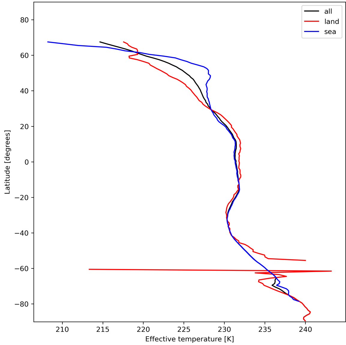
Figure 17: Zonal average of “Effective temperature” for 2023-11-29 to 2023-12-01.
