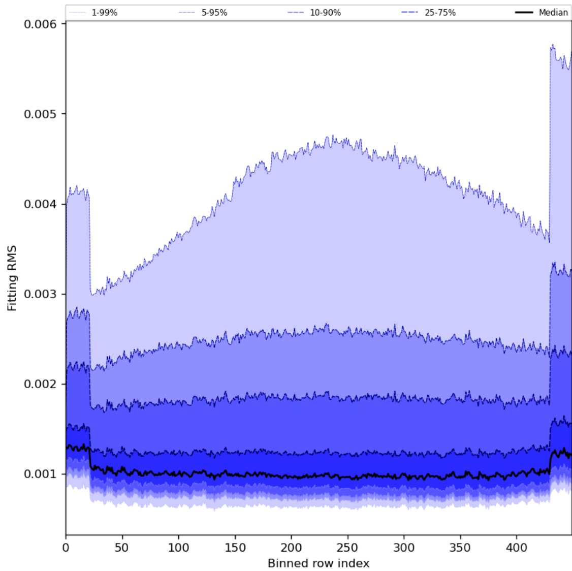
Figure 30: Along track statistics of “Fitting RMS” for 2023-11-29 to 2023-12-01
