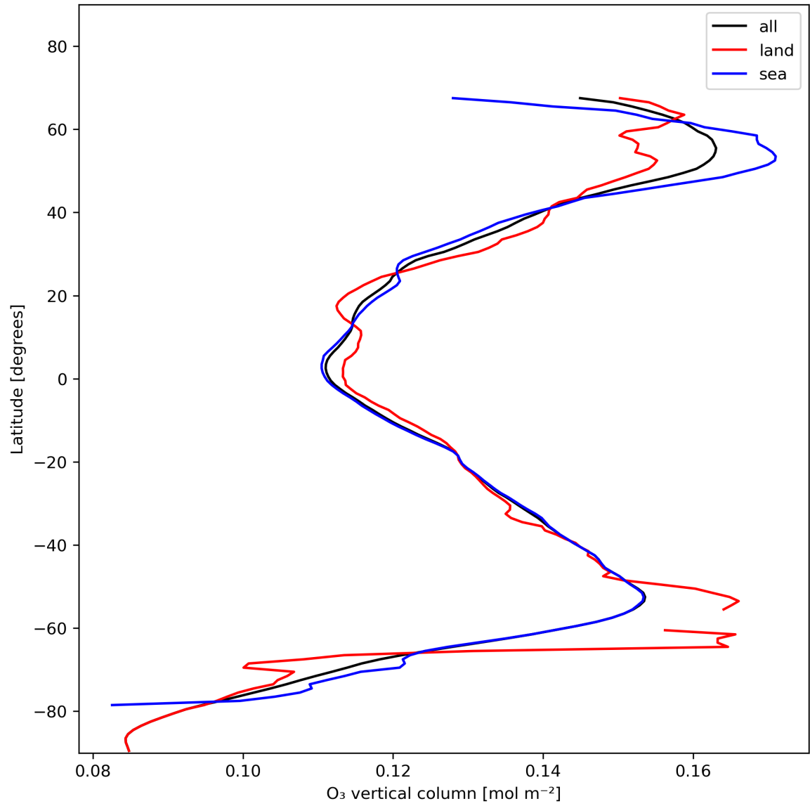
Figure 14: Zonal average of “O 3 vertical column” for 2023-11-29 to 2023-12-01.
