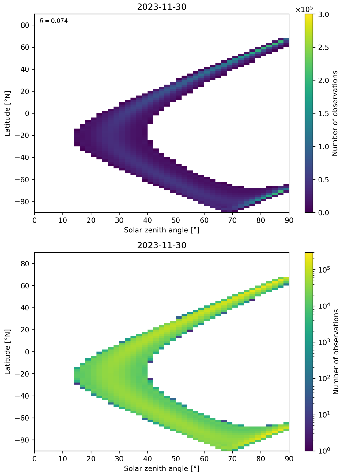
Figure 44: Scatter density plot of “Solar zenith angle” against “Latitude” for 2023-11-29 to 2023-12-01.
