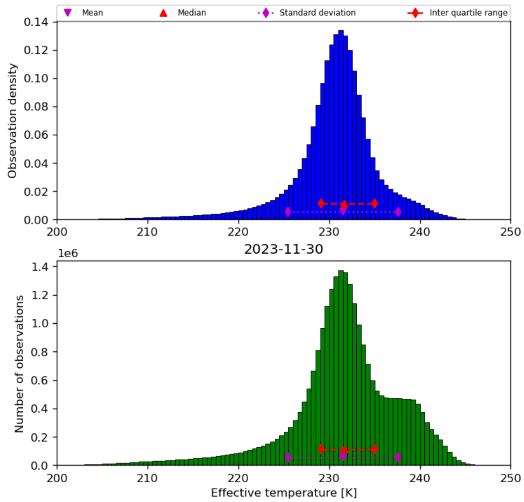
Figure 24: Histogram of “Effective temperature” for 2023-11-29 to 2023-12-01
