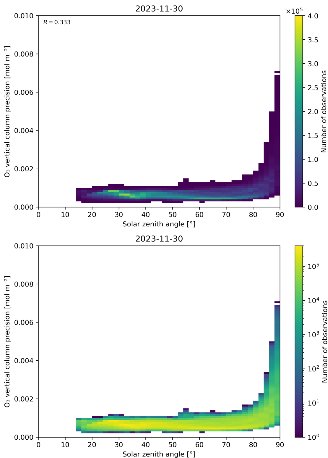
Figure 48: Scatter density plot of “Solar zenith angle” against “O 3 vertical column precision” for 2023-11-29 to 2023-12-01.
