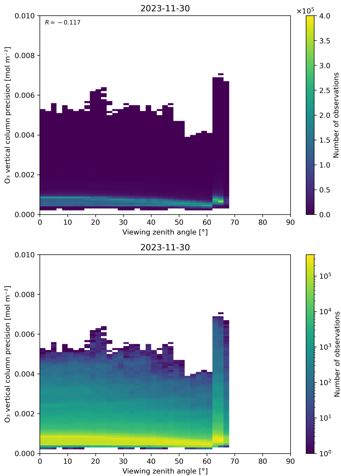
Figure 53: Scatter density plot of “Viewing zenith angle” against “O 3 vertical column precision” for 2023-11-29 to 2023-12-01.
