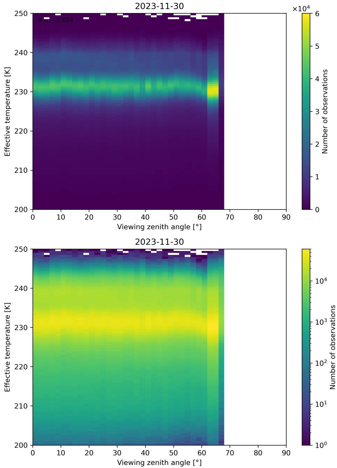
Figure 50: Scatter density plot of “Viewing zenith angle” against “Effective temperature” for 2023-11-29 to 2023-12-01.
