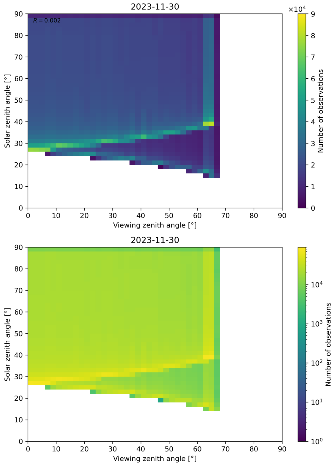
Figure 54: Scatter density plot of “Viewing zenith angle” against “Solar zenith angle” for 2023-11-29 to 2023-12-01.
