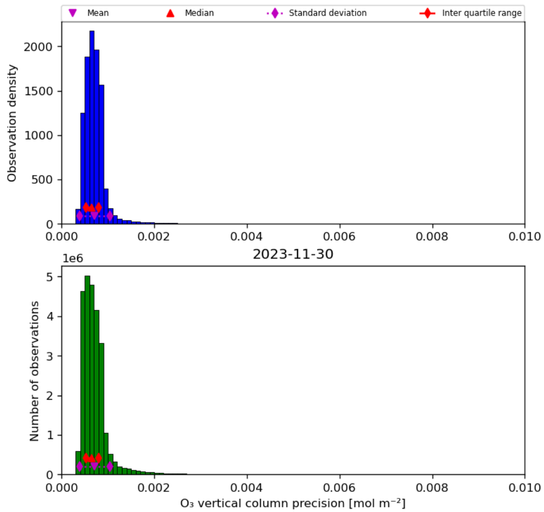
Figure 22: Histogram of "O 3 vertical column precision" for 2023-11-29 to 2023-12-01
