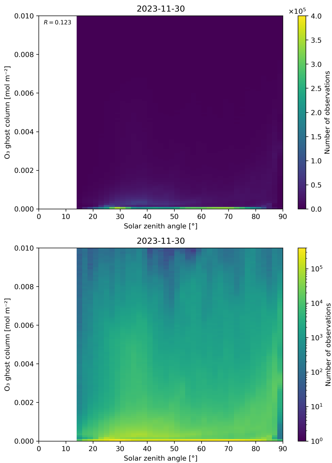
Figure 46: Scatter density plot of “Solar zenith angle” against “O 3 ghost column” for 2023-11-29 to 2023-12-01.
