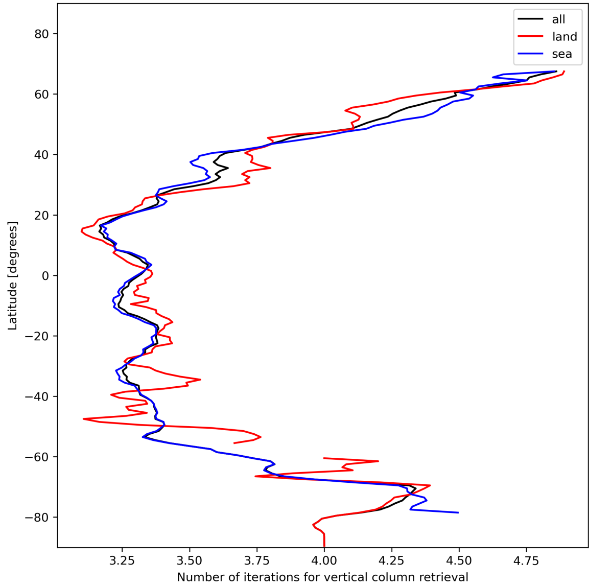
Figure 19: Zonal average of “Number of iterations for vertical column retrieval” for 2023-11-29 to 2023-12-01.
