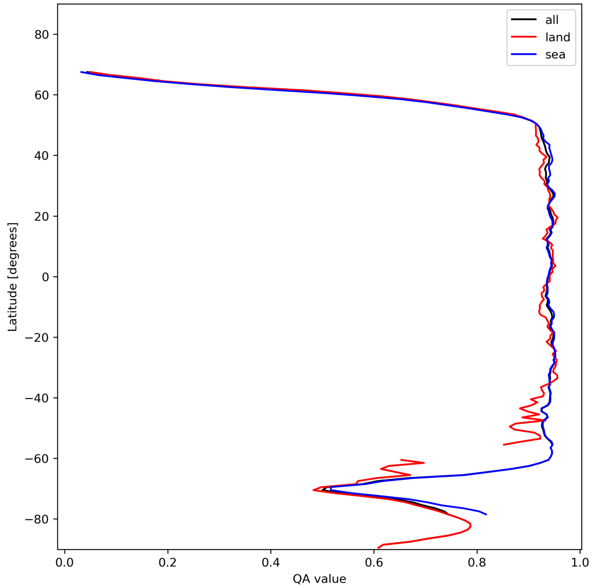
Figure 13: Zonal average of “QA value” for 2023-11-29 to 2023-12-01.
