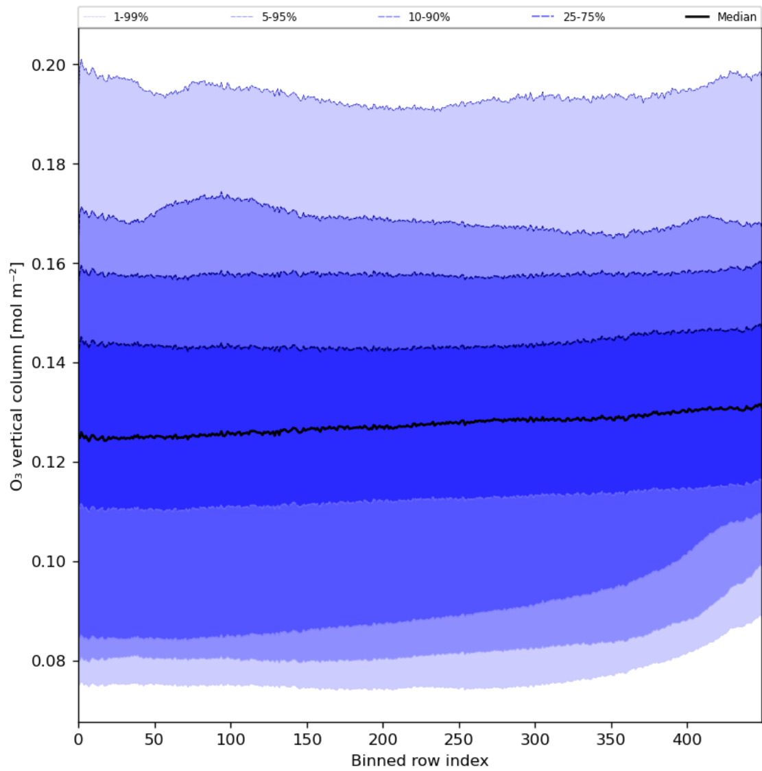
Figure 28: Along track statistics of “O 3 vertical column” for 2023-11-29 to 2023-12-01
