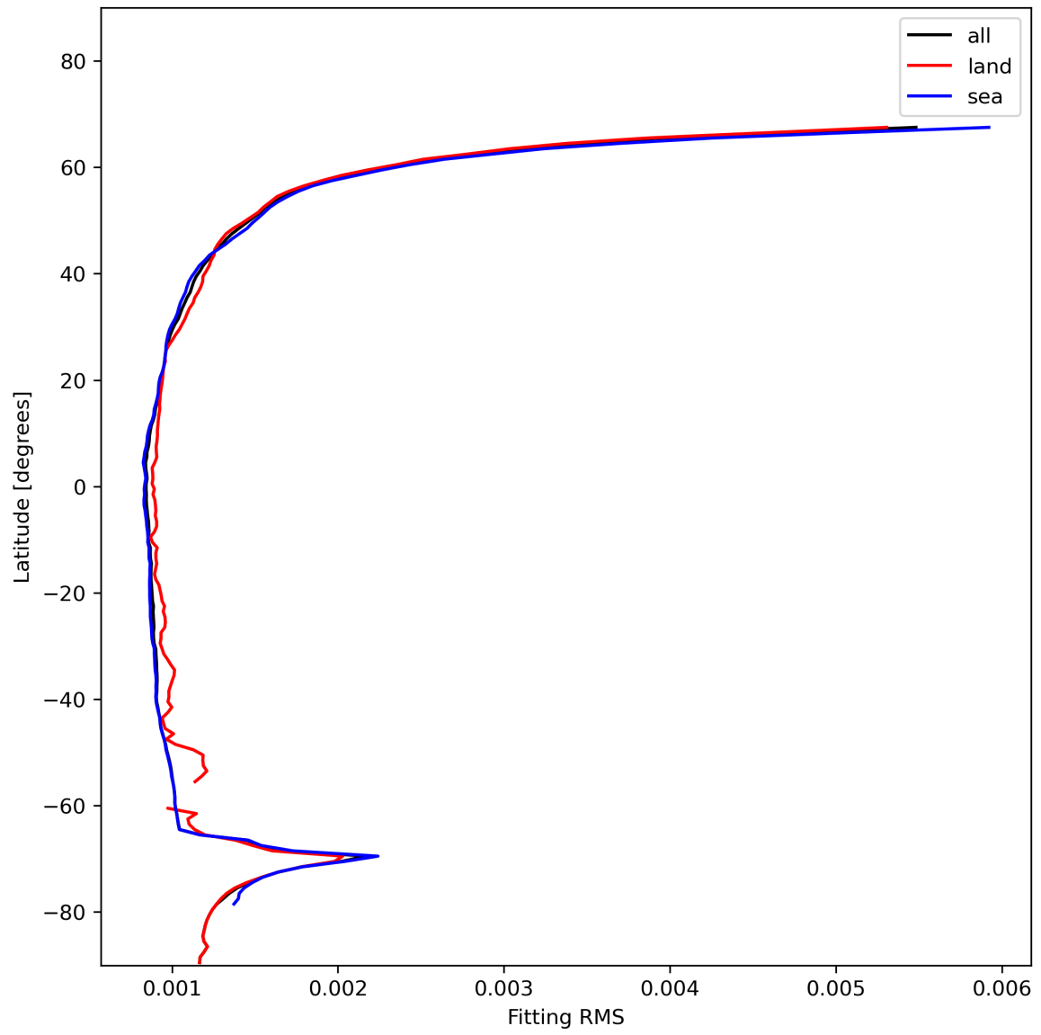
Figure 16: Zonal average of “Fitting RMS” for 2023-11-29 to 2023-12-01.
