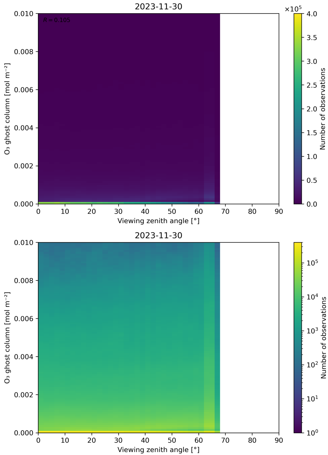
Figure 51: Scatter density plot of “Viewing zenith angle” against “O 3 ghost column” for 2023-11-29 to 2023-12-01.
