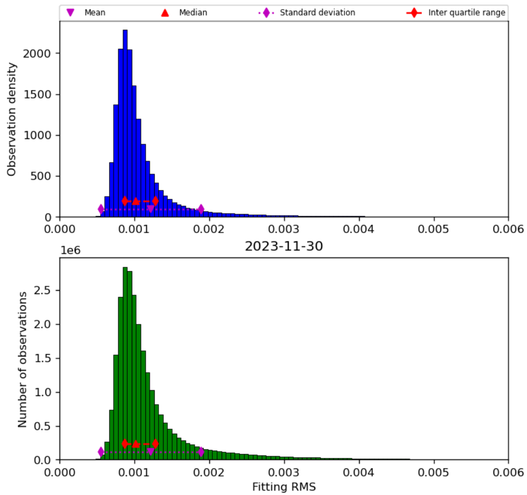
Figure 23: Histogram of “Fitting RMS” for 2023-11-29 to 2023-12-01
