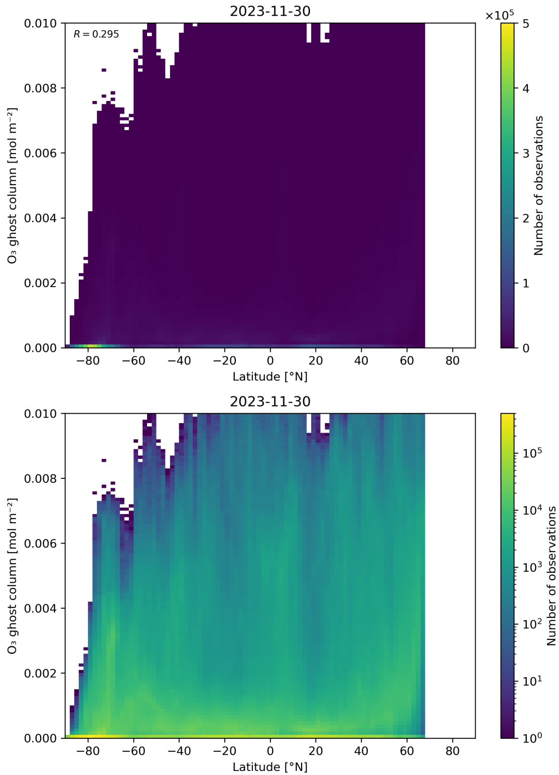
Figure 35: Scatter density plot of “Latitude” against “O 3 ghost column” for 2023-11-29 to 2023-12-01.
