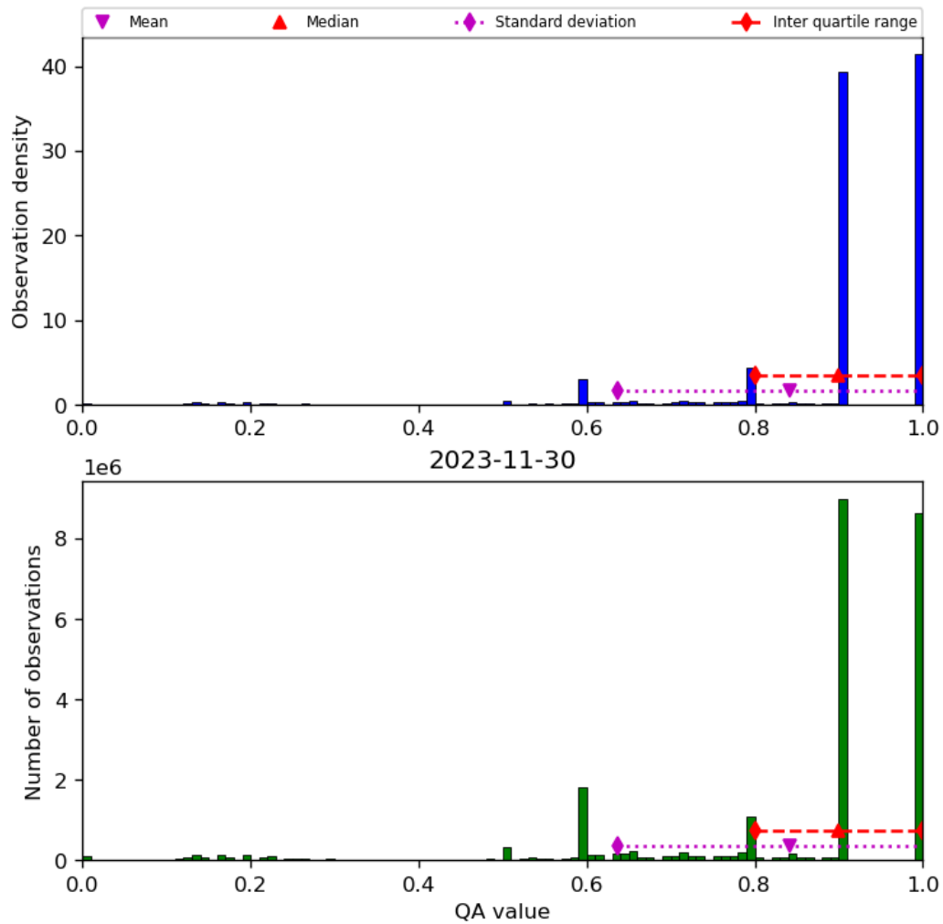
Figure 20: Histogram of “QA value” for 2023-11-29 to 2023-12-01
