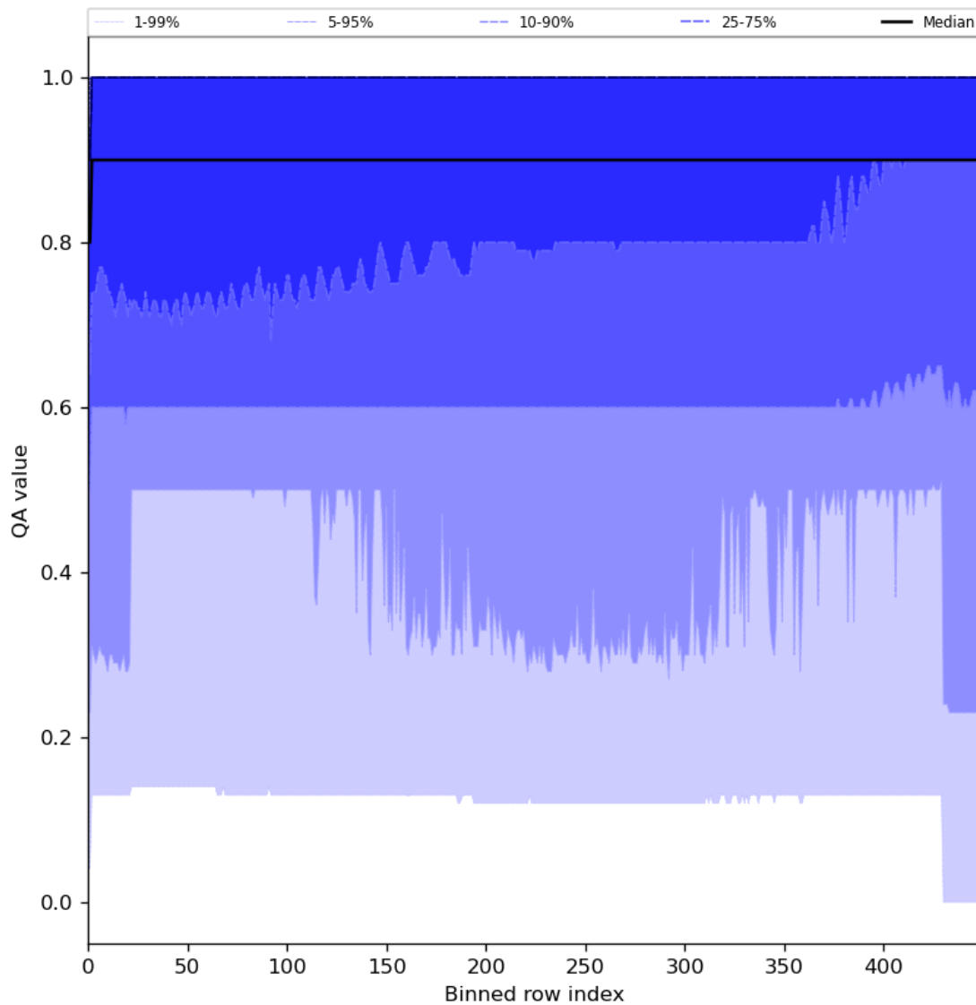
Figure 27: Along track statistics of “QA value” for 2023-11-29 to 2023-12-01
