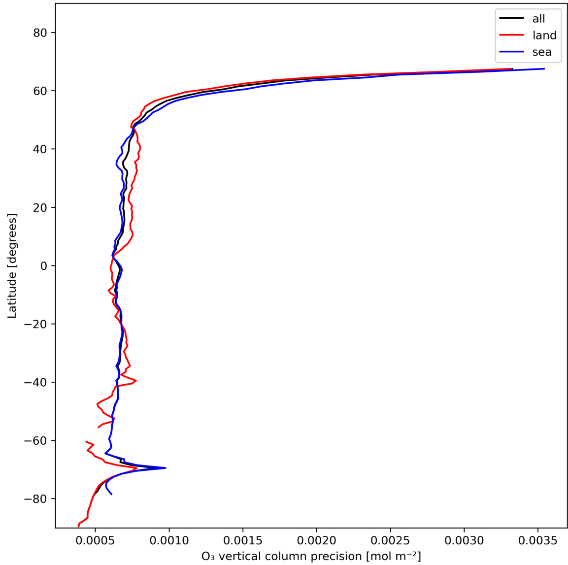
Figure 15: Zonal average of “O 3 vertical column precision” for 2023-12-01 to 2023-12-03.
