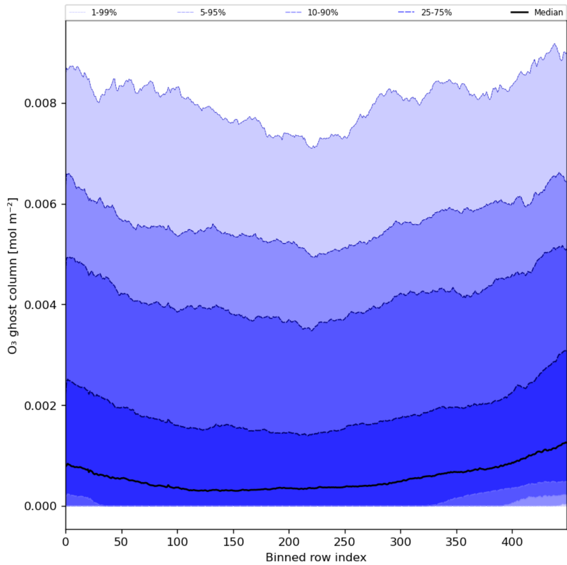
Figure 32: Along track statistics of “O 3 ghost column” for 2023-12-01 to 2023-12-03
