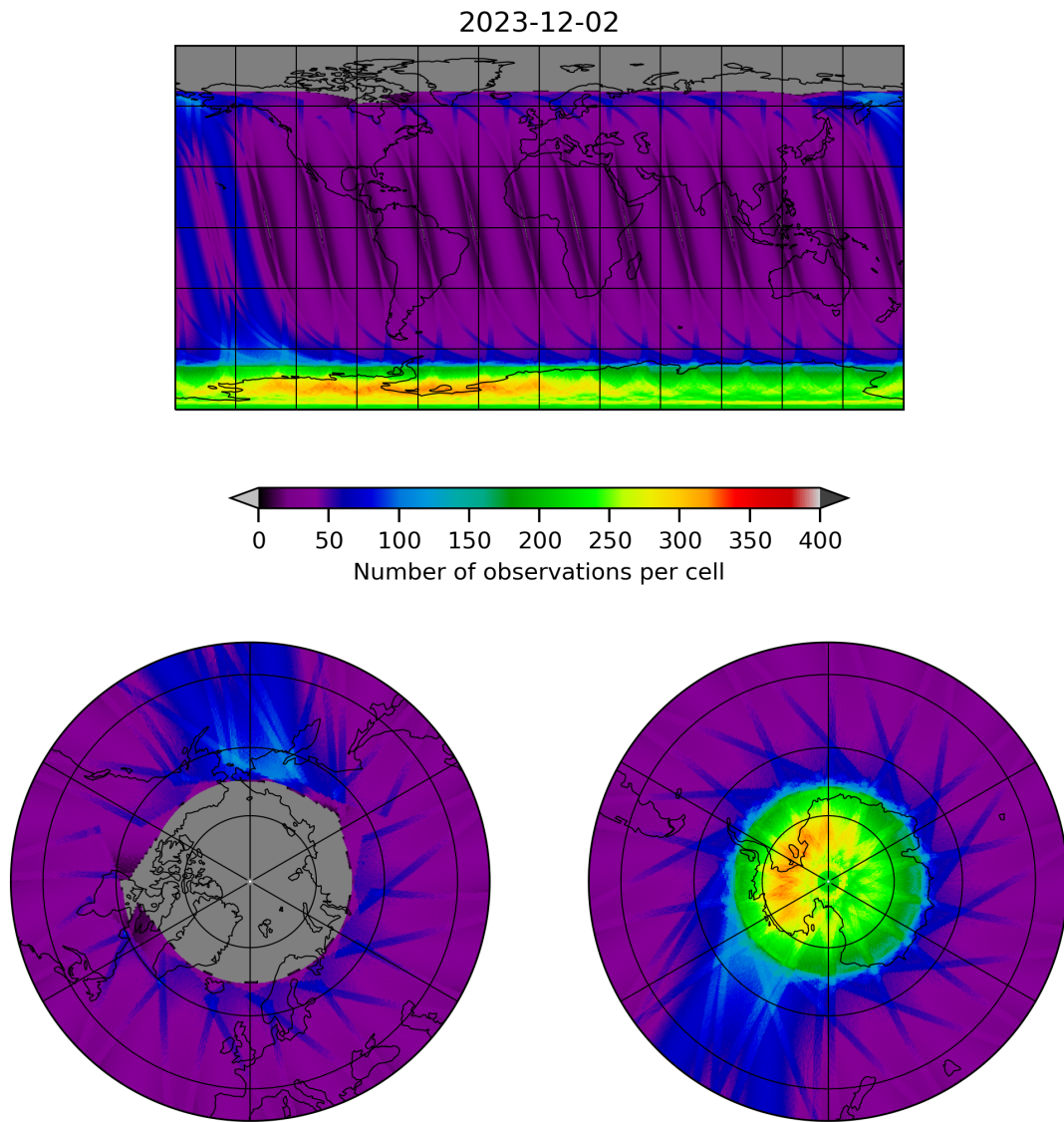
Figure 12: Map of the number of observations for 2023-12-01 to 2023-12-03
