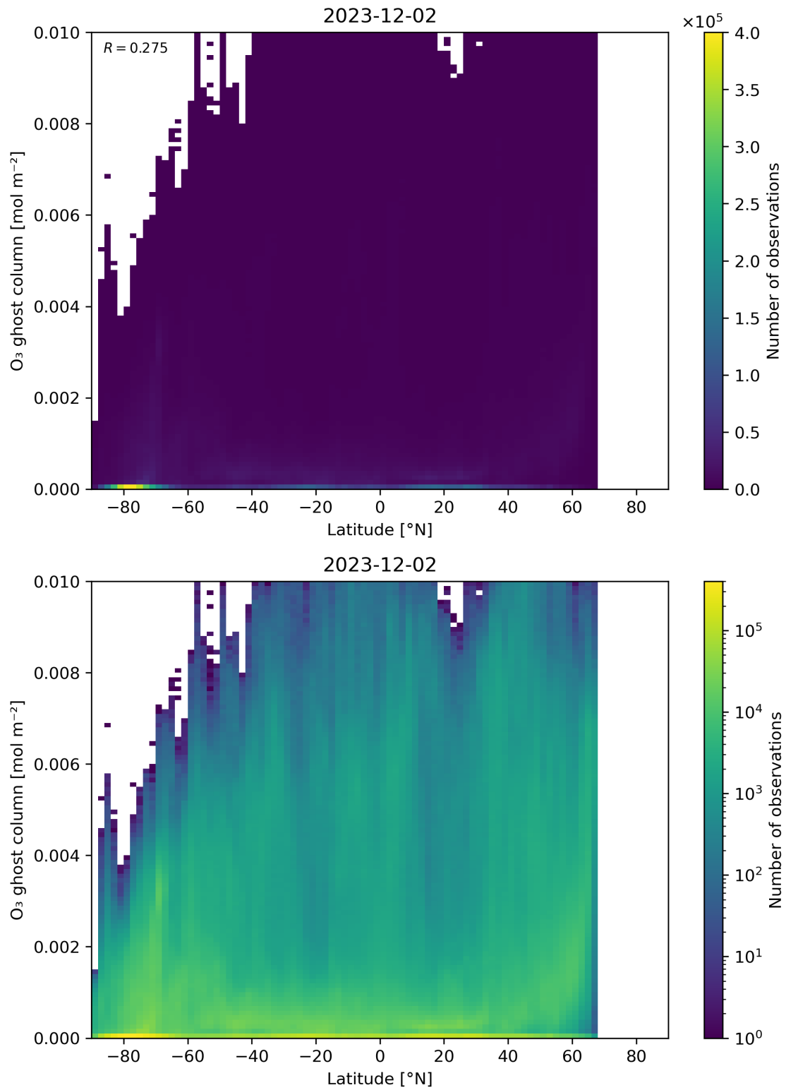
Figure 35: Scatter density plot of “Latitude” against “O 3 ghost column” for 2023-12-01 to 2023-12-03.
