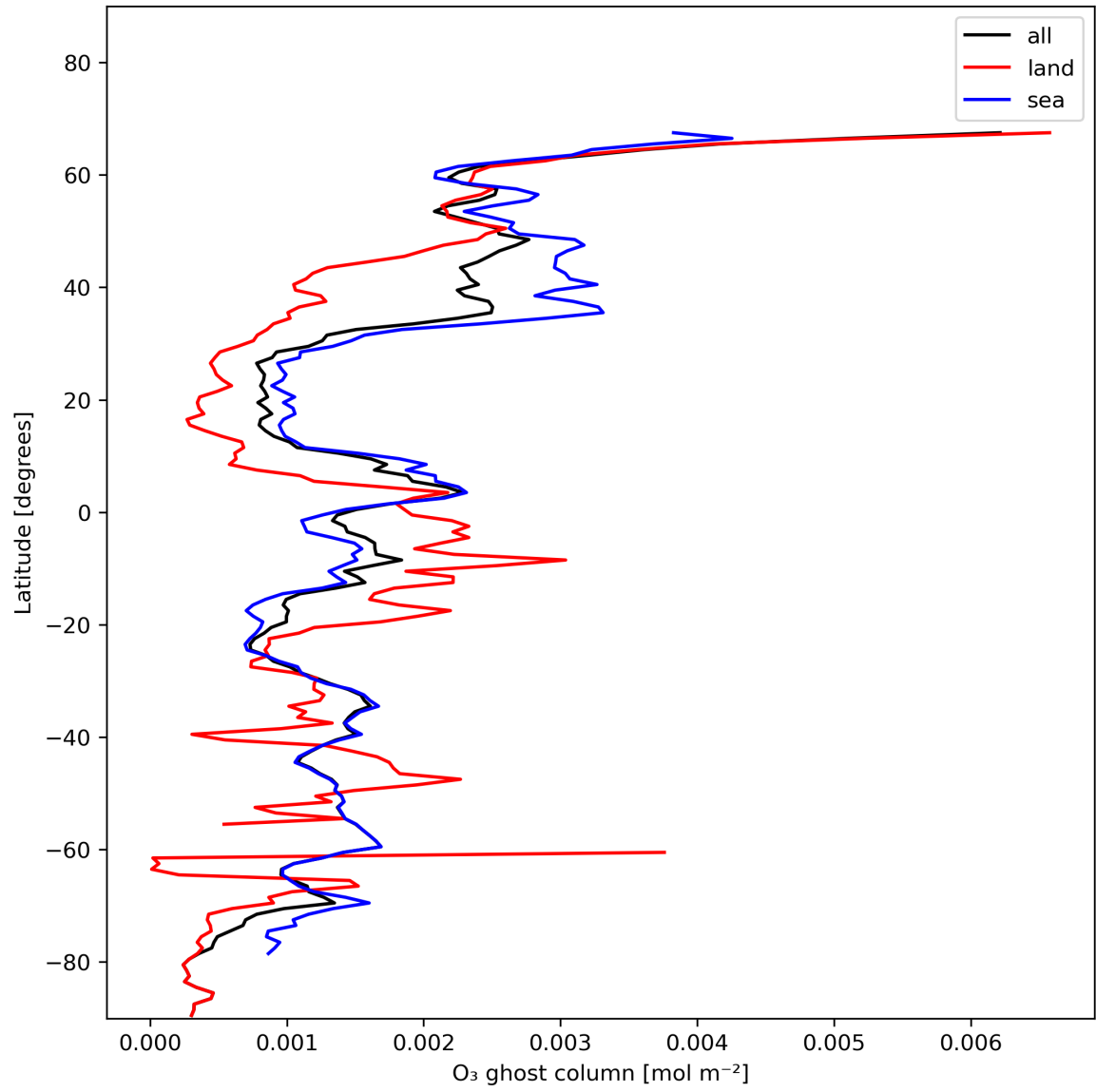
Figure 18: Zonal average of "O 3 ghost column" for 2023-12-01 to 2023-12-03.
