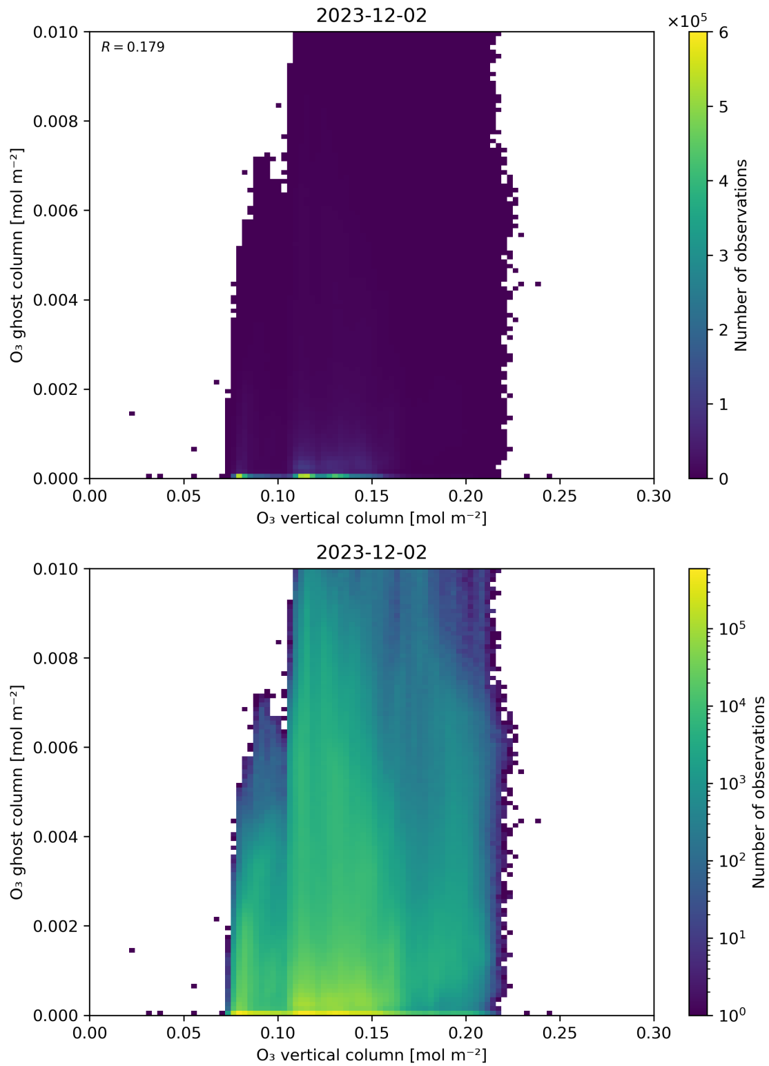
Figure 40: Scatter density plot of “O 3 vertical column” against “O 3 ghost column” for 2023-12-01 to 2023-12-03.
