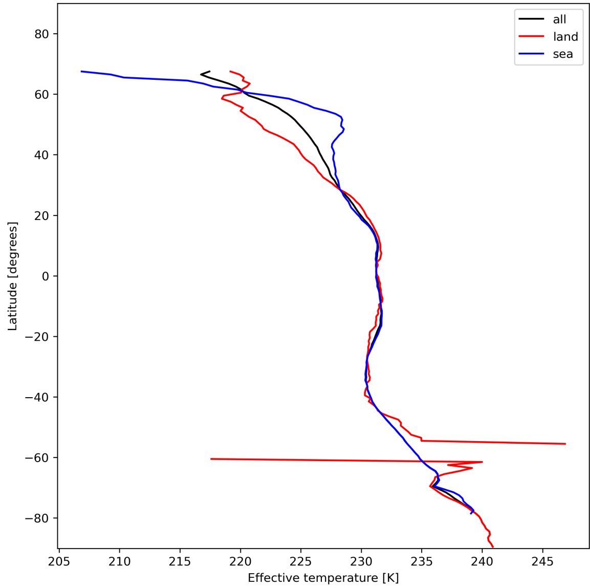
Figure 17: Zonal average of “Effective temperature” for 2023-12-01 to 2023-12-03.
