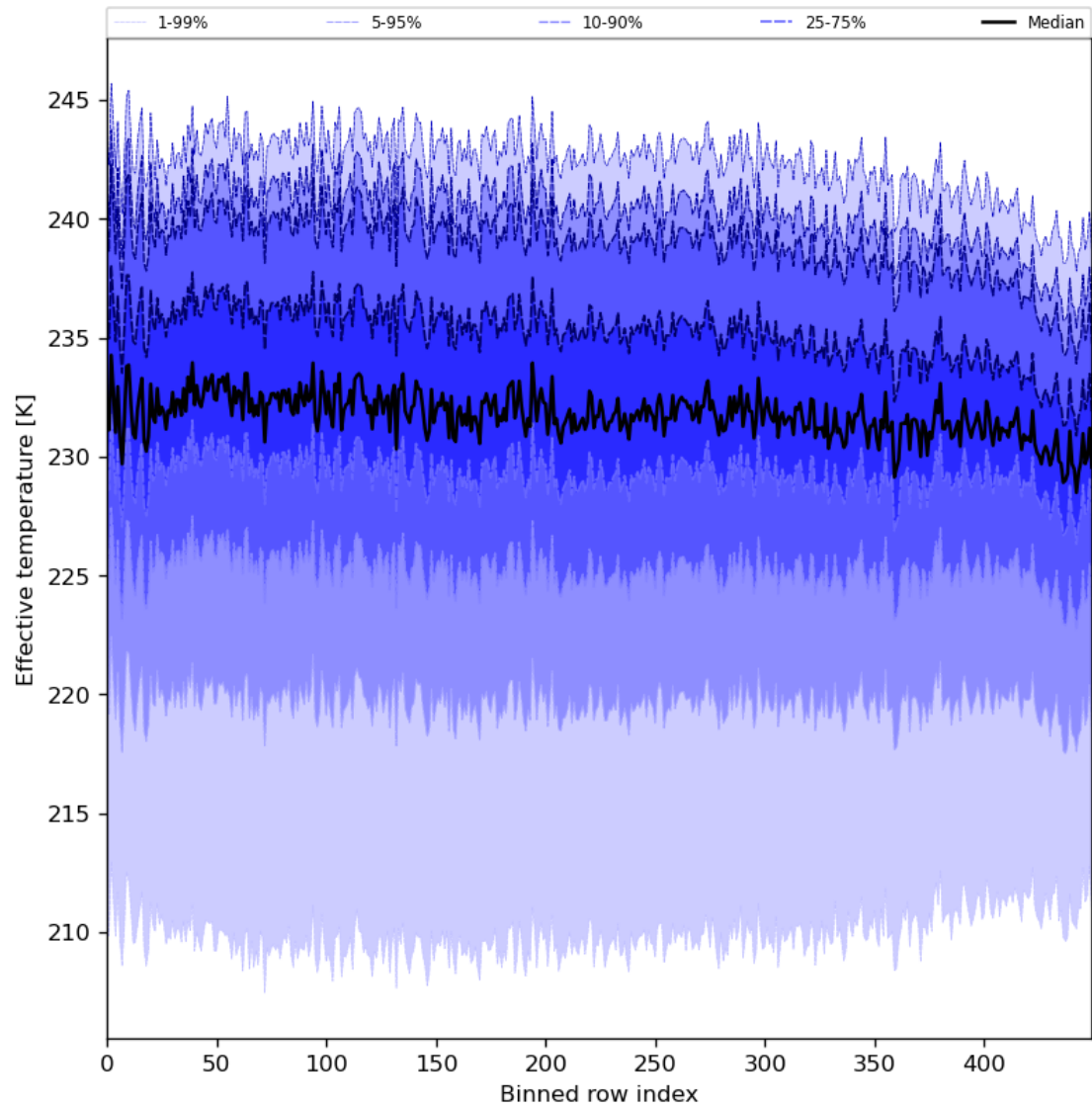
Figure 31: Along track statistics of “Effective temperature” for 2023-12-01 to 2023-12-03
