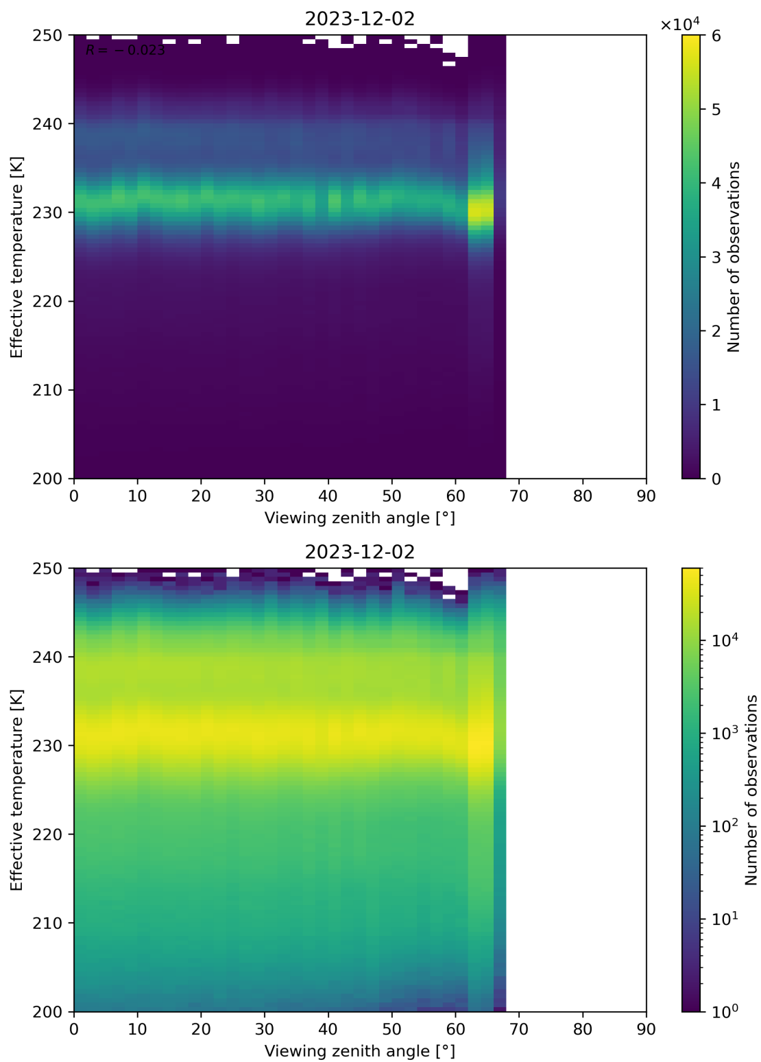
Figure 50: Scatter density plot of “Viewing zenith angle” against “Effective temperature” for 2023-12-01 to 2023-12-03.
