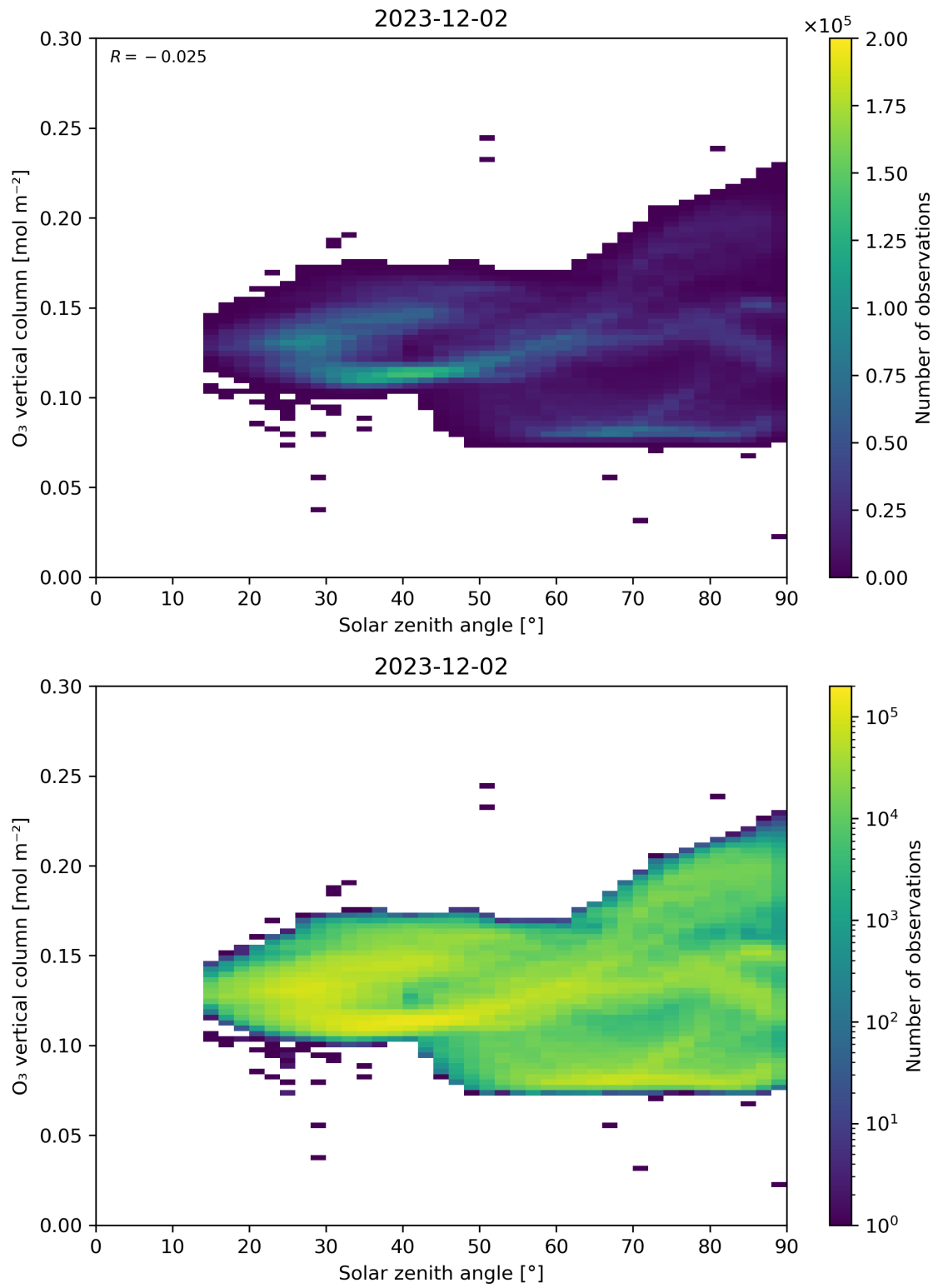
Figure 47: Scatter density plot of “Solar zenith angle” against “O 3 vertical column” for 2023-12-01 to 2023-12-03.
