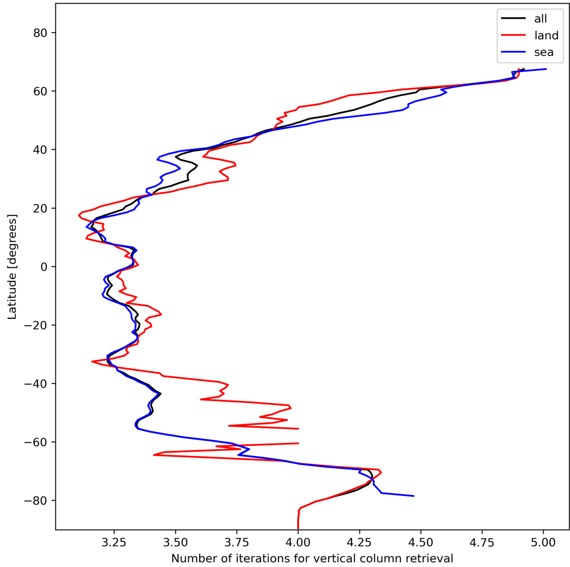
Figure 19: Zonal average of “Number of iterations for vertical column retrieval” for 2023-12-01 to 2023-12-03.
