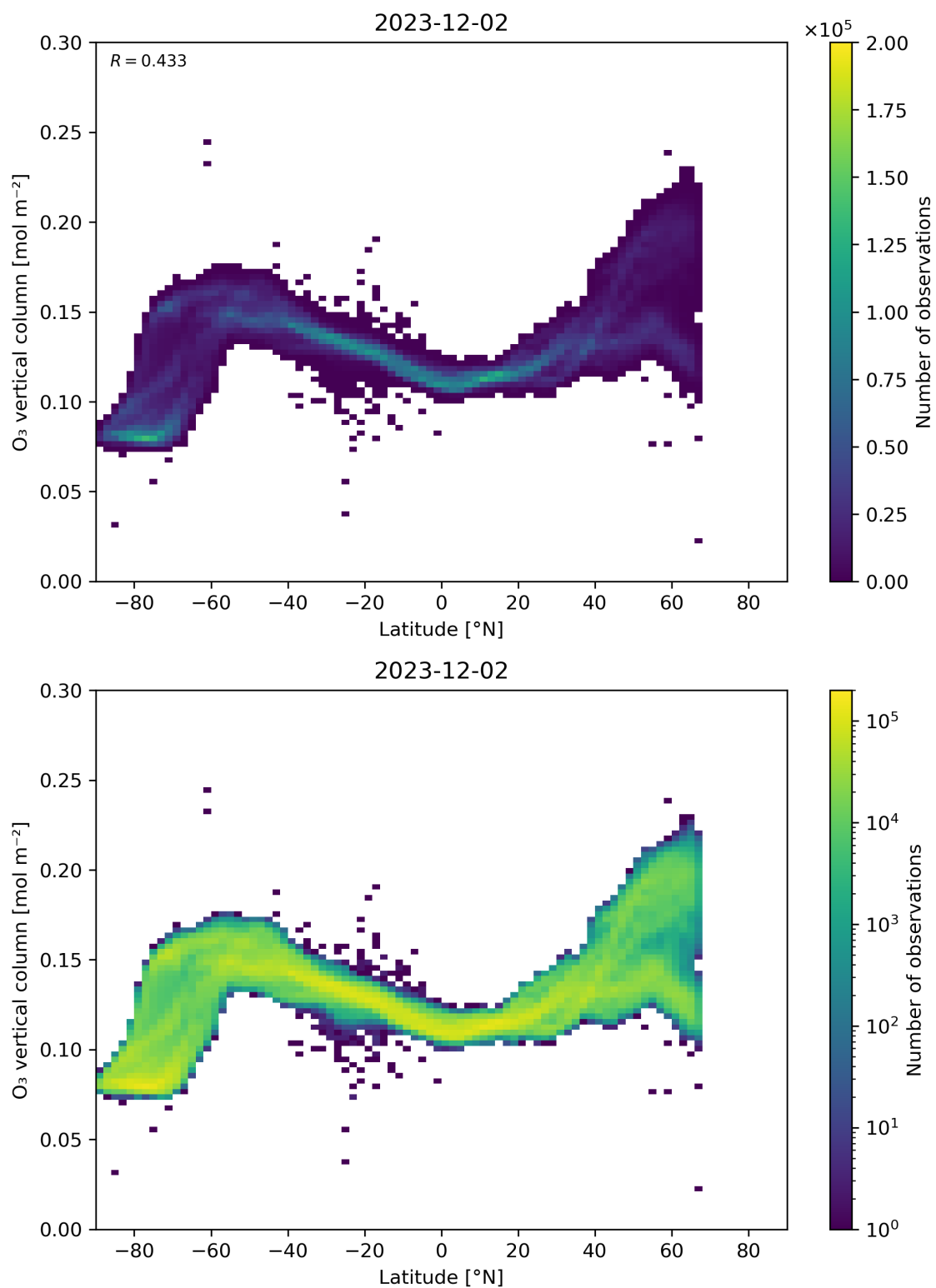
Figure 36: Scatter density plot of “Latitude” against “O 3 vertical column” for 2023-12-01 to 2023-12-03.
