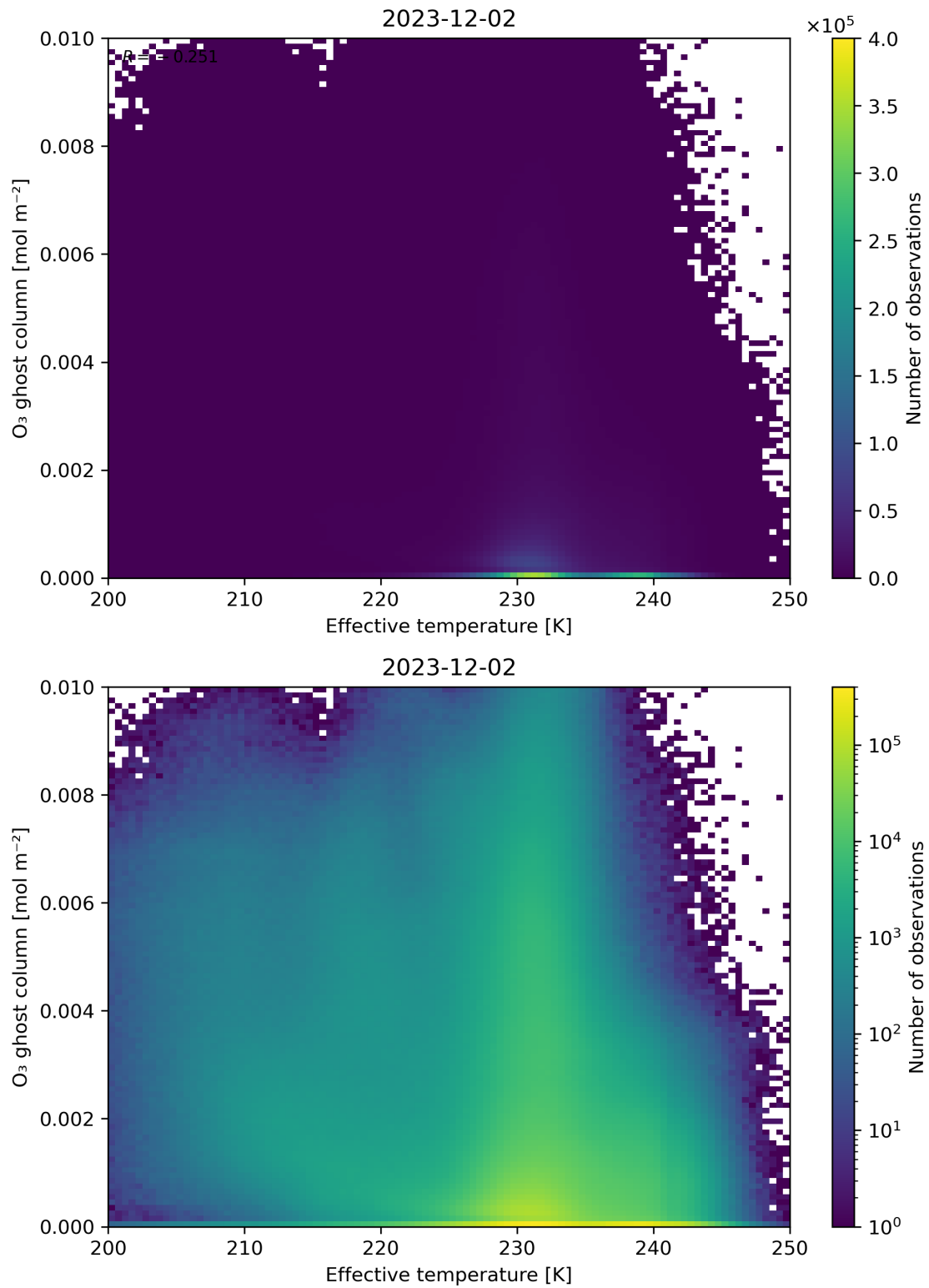
Figure 38: Scatter density plot of “Effective temperature” against “O 3 ghost column” for 2023-12-01 to 2023-12-03.
