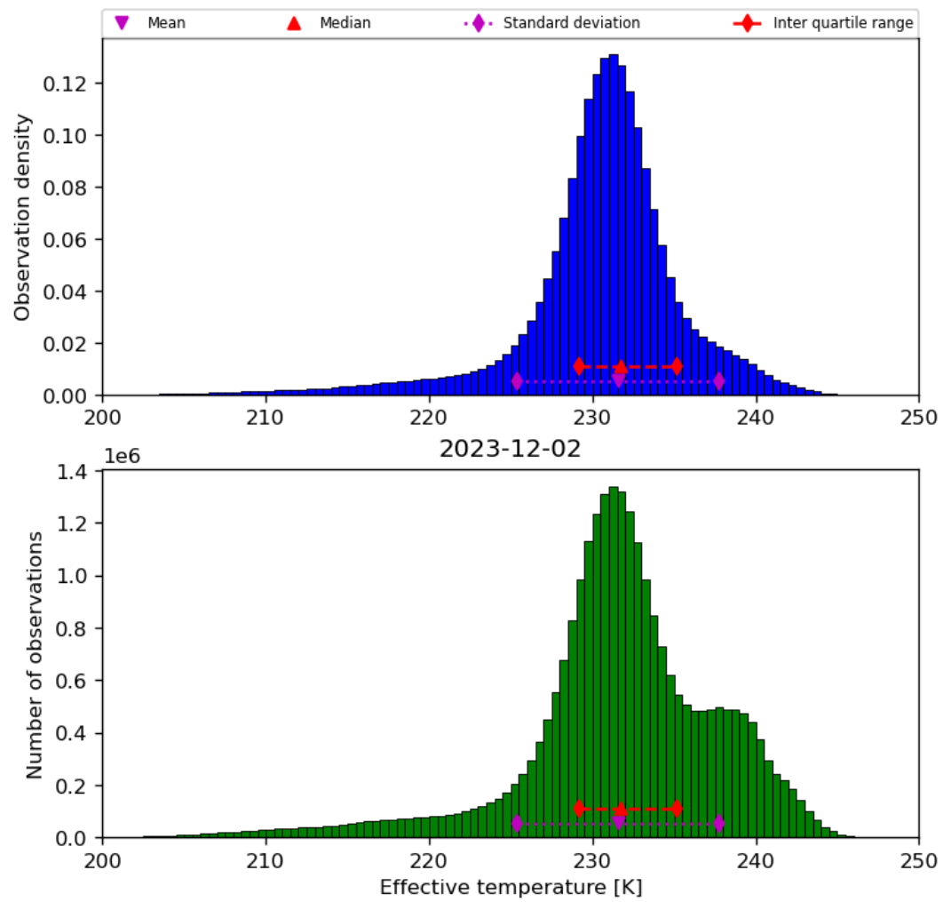
Figure 24: Histogram of “Effective temperature” for 2023-12-01 to 2023-12-03
