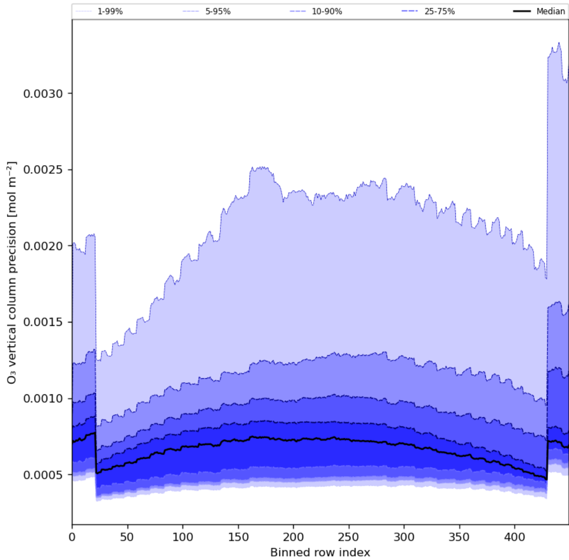
Figure 29: Along track statistics of “O 3 vertical column precision” for 2023-12-01 to 2023-12-03
