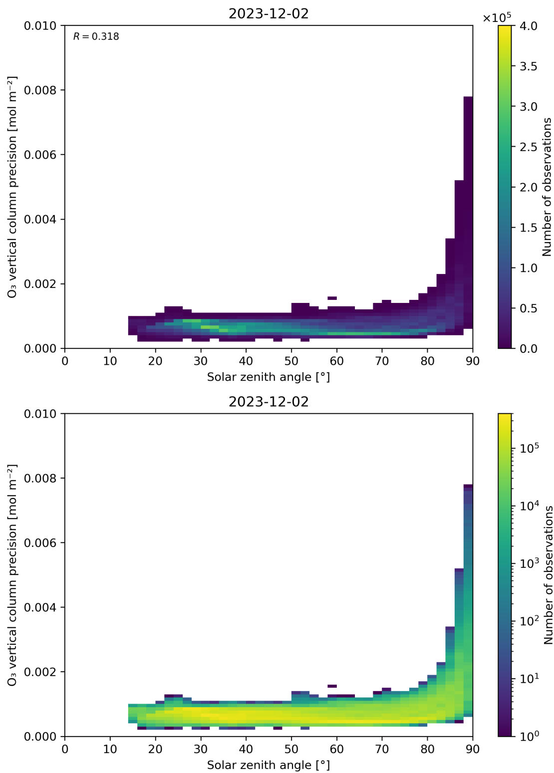
Figure 48: Scatter density plot of “Solar zenith angle” against “O 3 vertical column precision” for 2023-12-01 to 2023-12-03.
