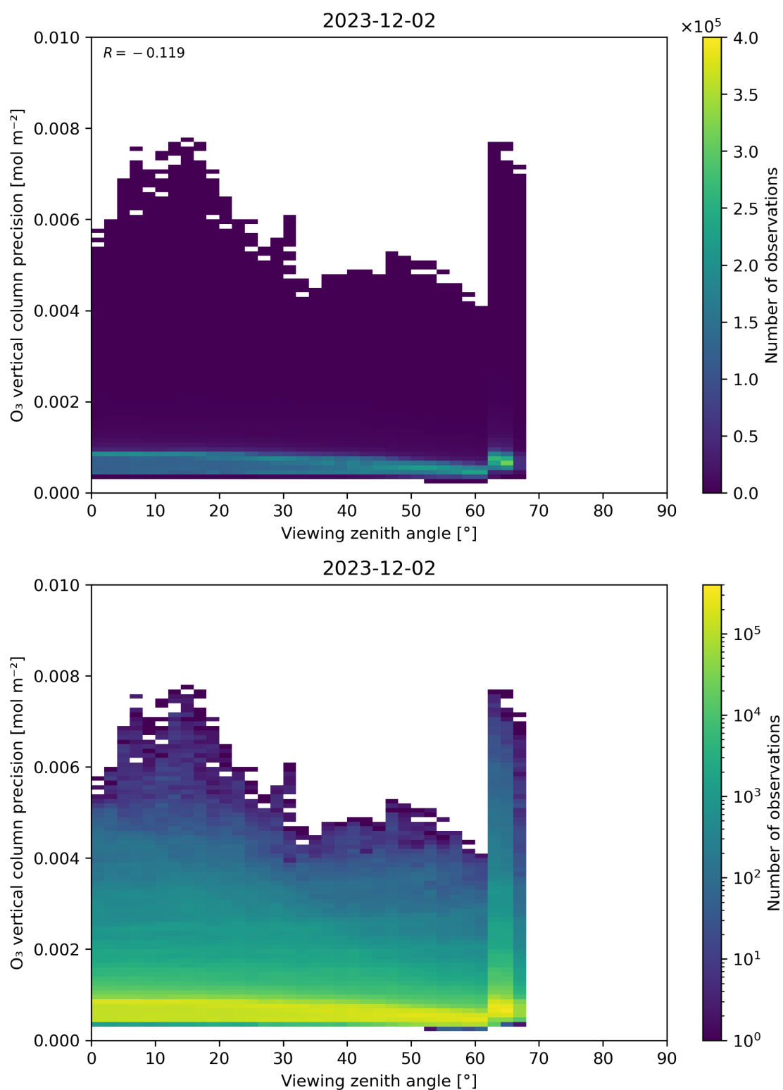
Figure 53: Scatter density plot of “Viewing zenith angle” against “O 3 vertical column precision” for 2023-12-01 to 2023-12-03.
