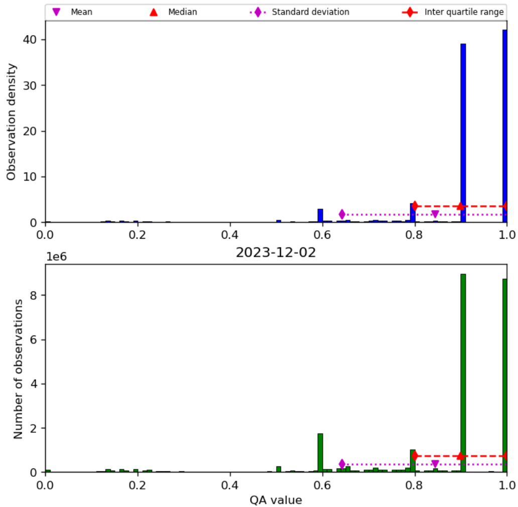
Figure 20: Histogram of “QA value” for 2023-12-01 to 2023-12-03
