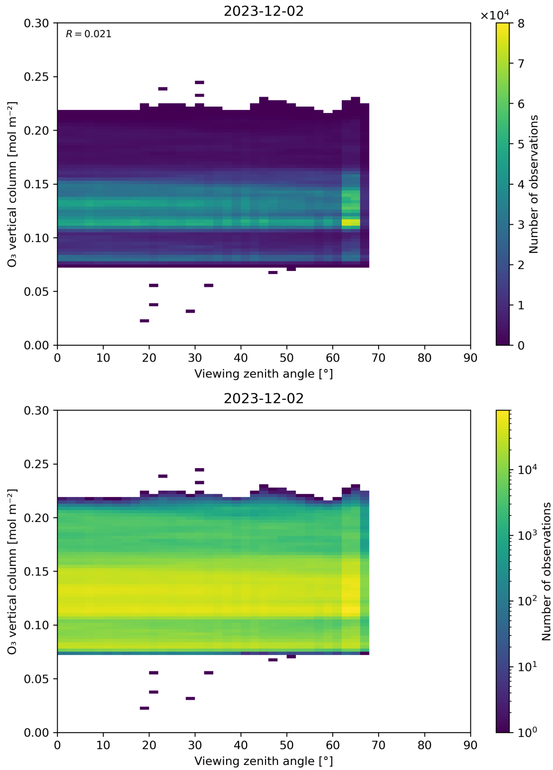
Figure 52: Scatter density plot of “Viewing zenith angle” against “O 3 vertical column” for 2023-12-01 to 2023-12-03.
