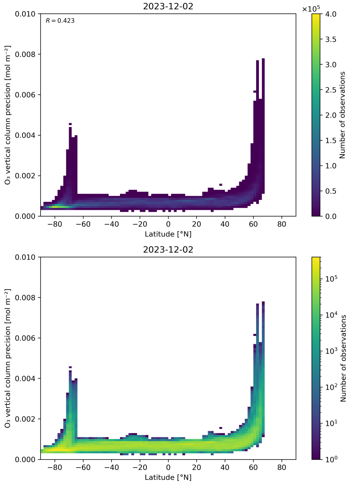
Figure 37: Scatter density plot of “Latitude” against “O 3 vertical column precision” for 2023-12-01 to 2023-12-03.
