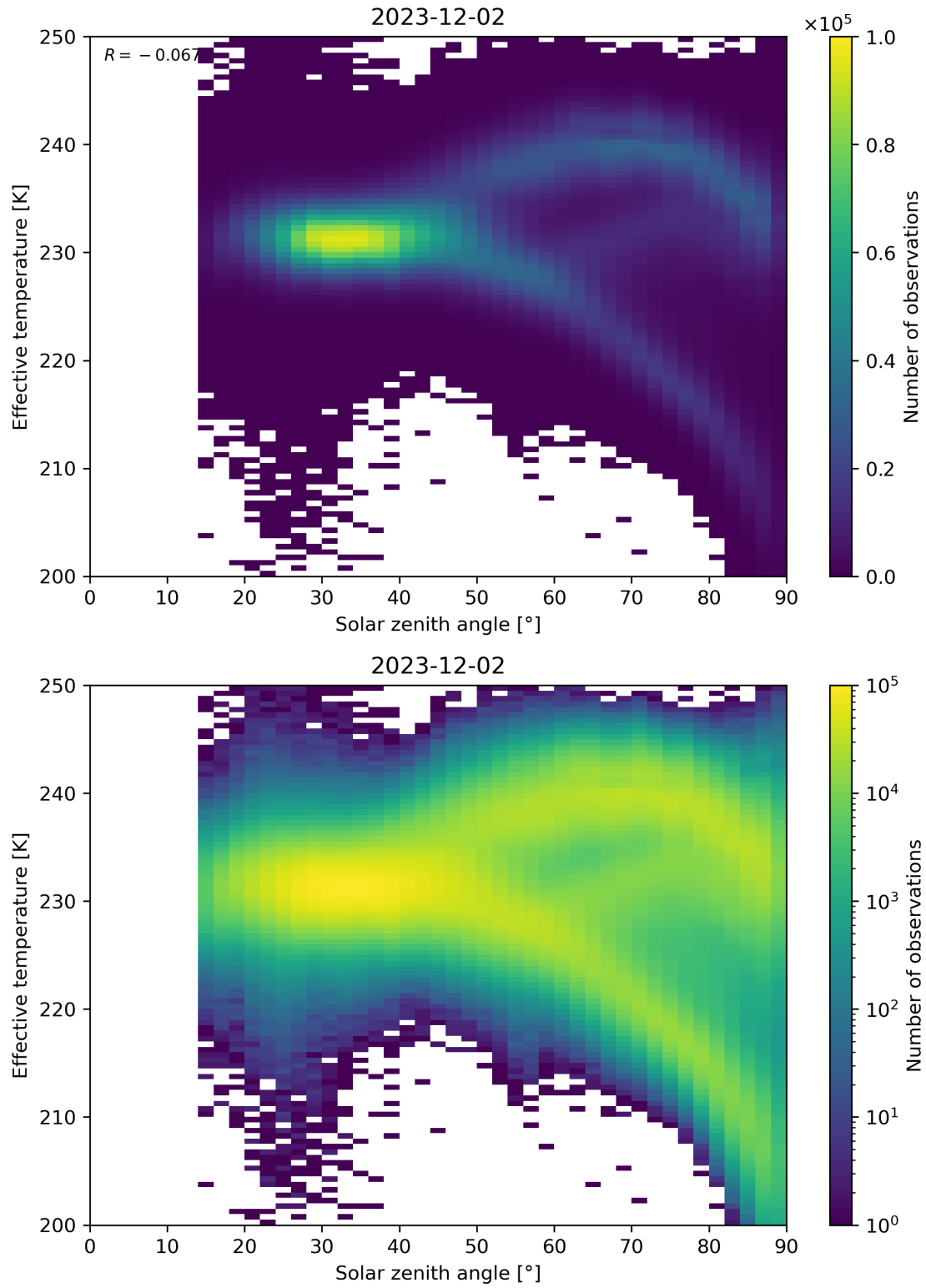
Figure 45: Scatter density plot of “Solar zenith angle” against “Effective temperature” for 2023-12-01 to 2023-12-03.
