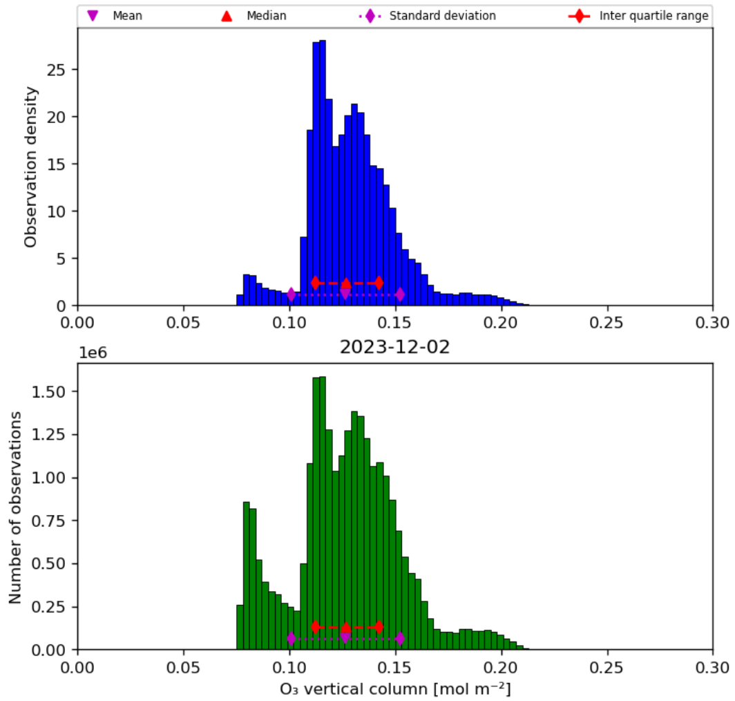
Figure 21: Histogram of “O 3 vertical column” for 2023-12-01 to 2023-12-03
