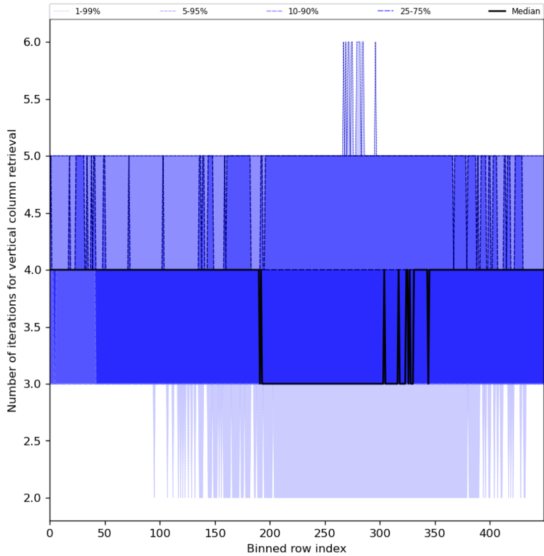
Figure 33: Along track statistics of “Number of iterations for vertical column retrieval” for 2023-12-01 to 2023-12-03
