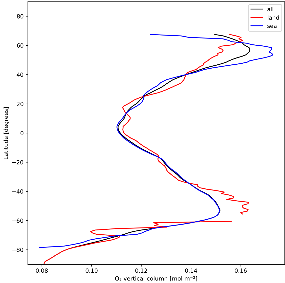
Figure 14: Zonal average of “O 3 vertical column” for 2023-12-01 to 2023-12-03.
