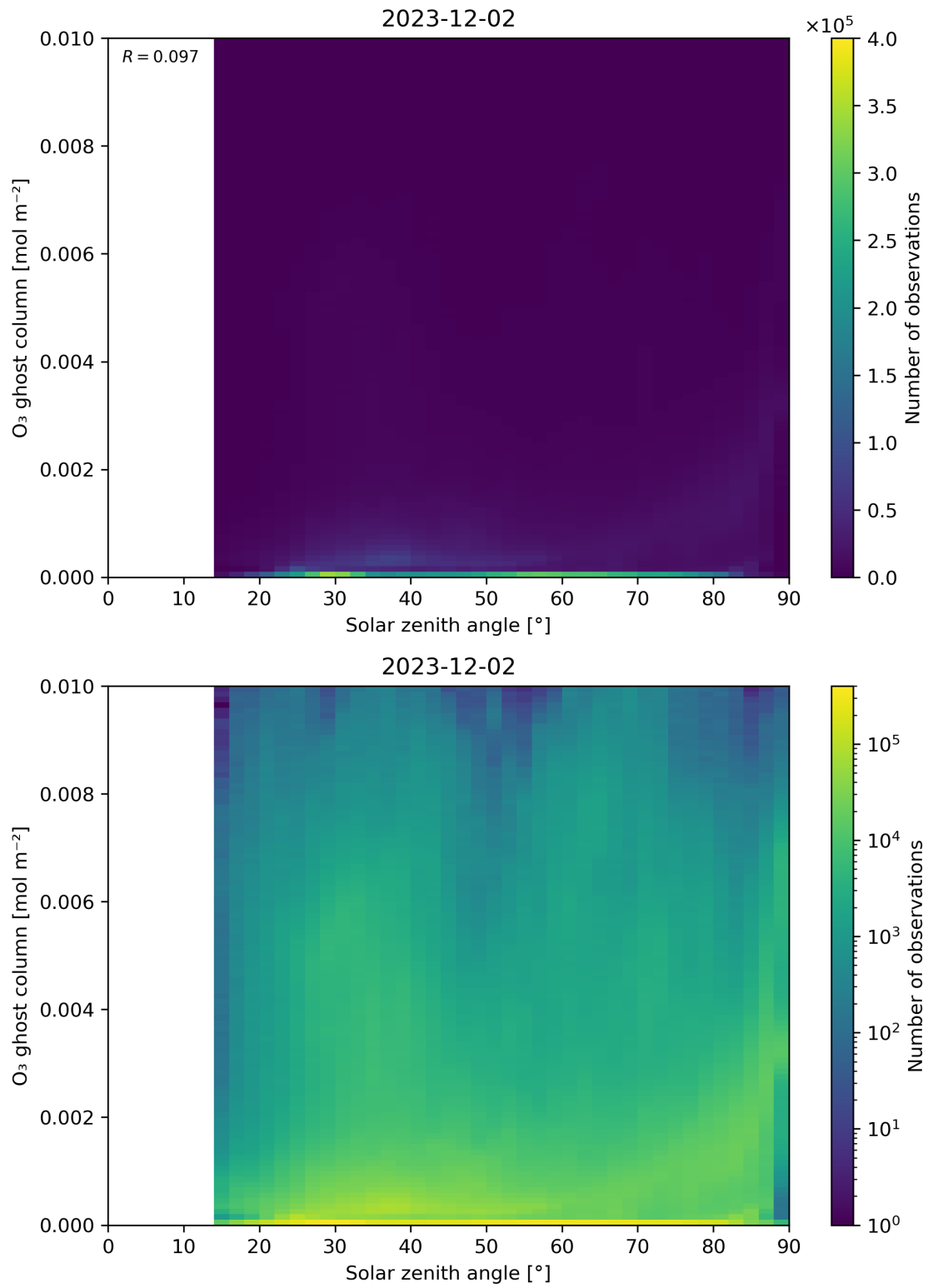
Figure 46: Scatter density plot of “Solar zenith angle” against “O 3 ghost column” for 2023-12-01 to 2023-12-03.
