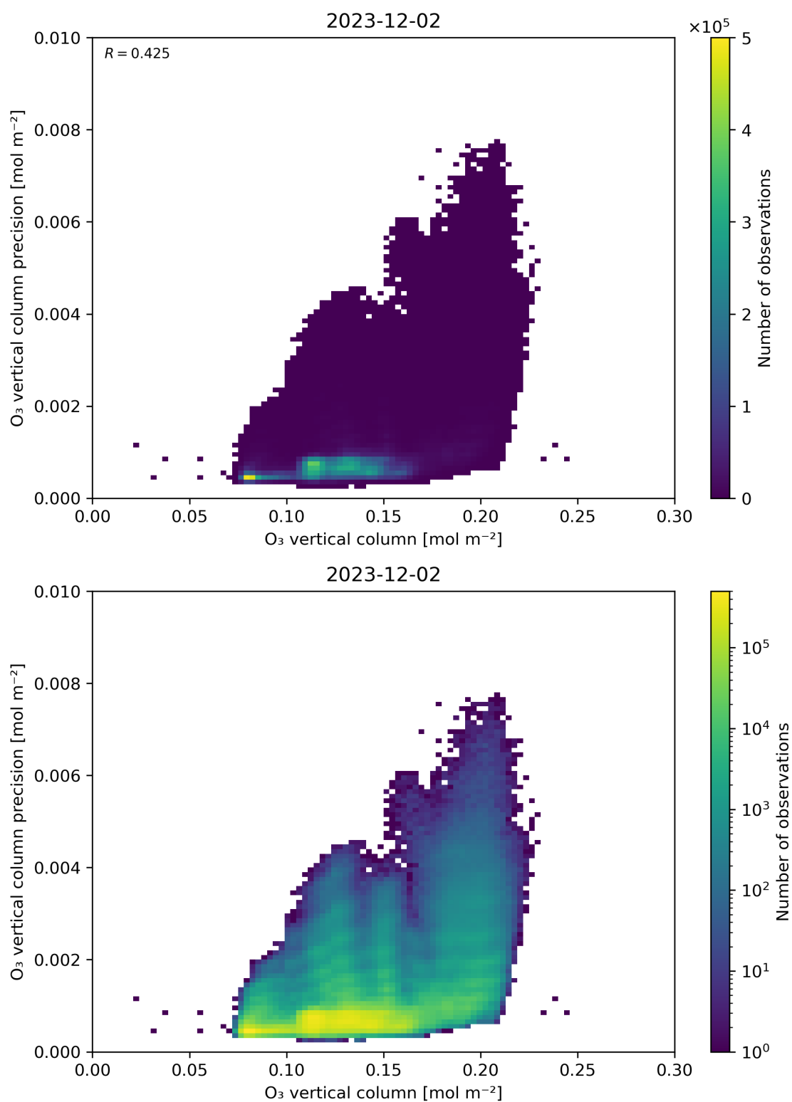
Figure 41: Scatter density plot of “O 3 vertical column” against “O 3 vertical column precision” for 2023-12-01 to 2023-12-03.
