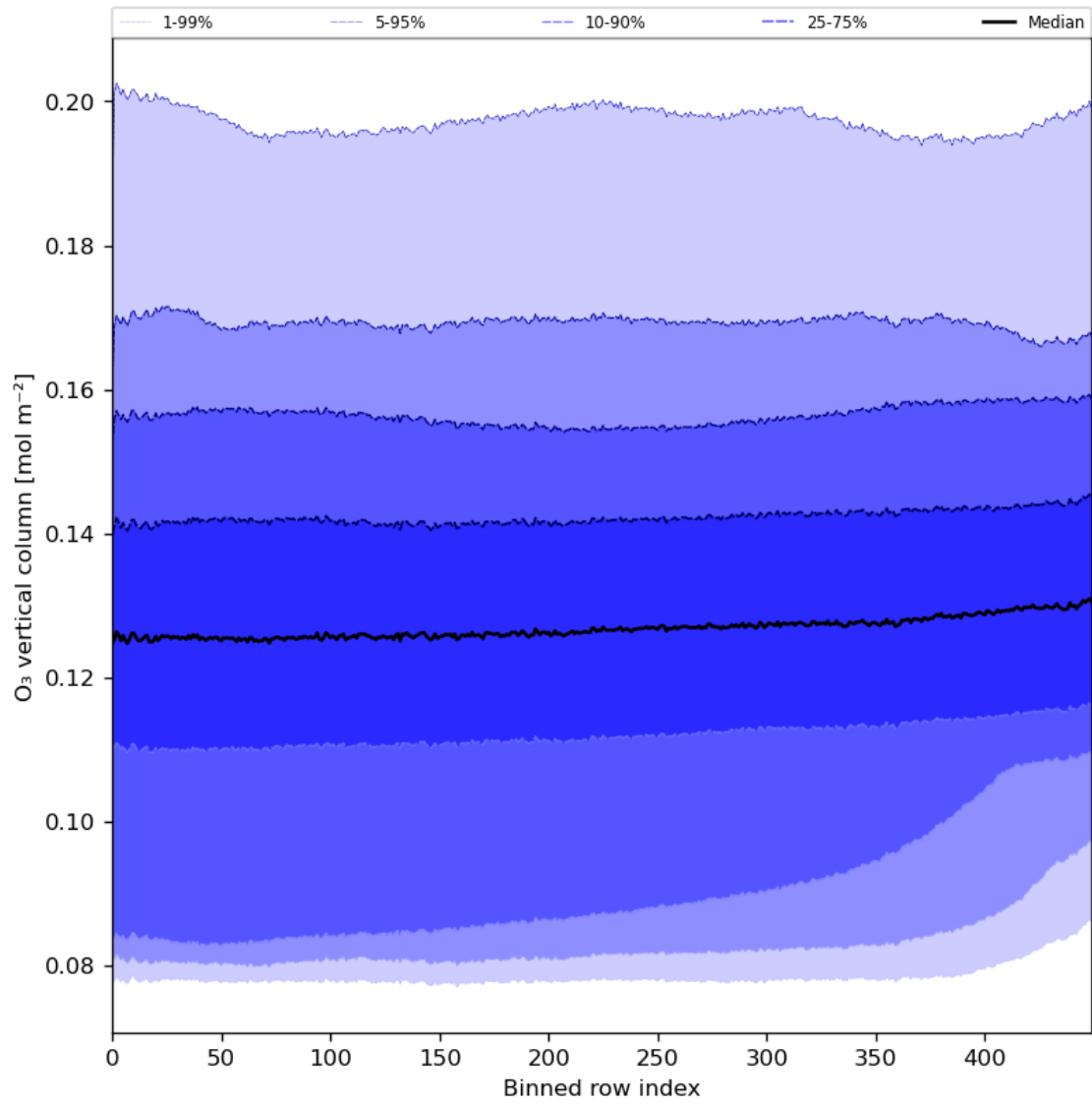
Figure 28: Along track statistics of “O 3 vertical column” for 2023-12-01 to 2023-12-03
