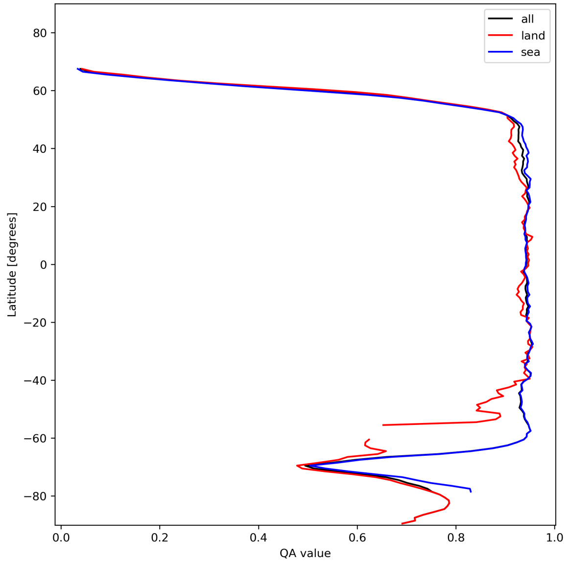
Figure 13: Zonal average of “QA value” for 2023-12-01 to 2023-12-03.
