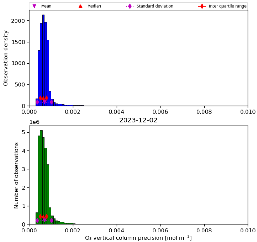
Figure 22: Histogram of “O 3 vertical column precision” for 2023-12-01 to 2023-12-03
