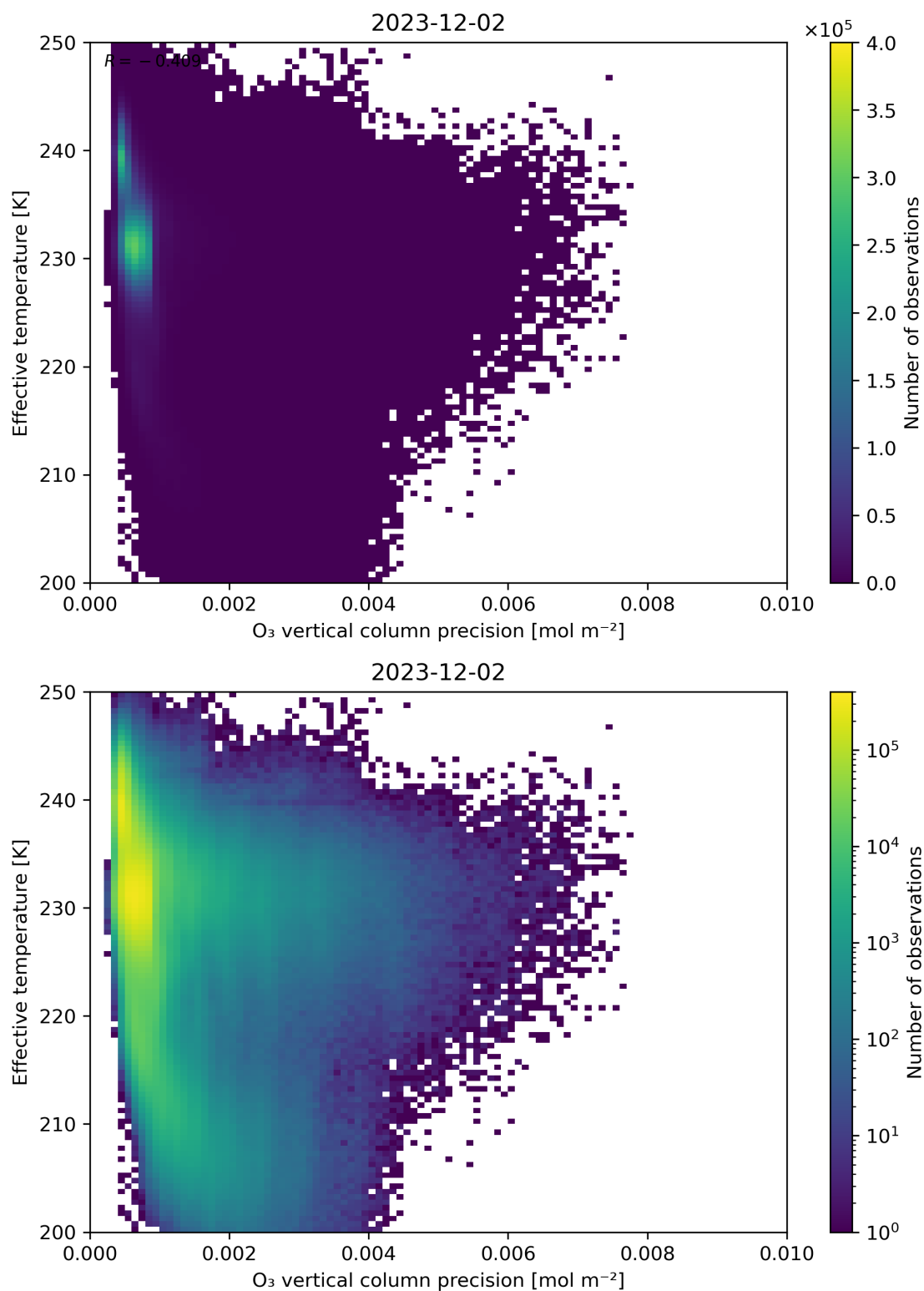
Figure 42: Scatter density plot of “O 3 vertical column precision” against “Effective temperature” for 2023-12-01 to 2023-12-03.
