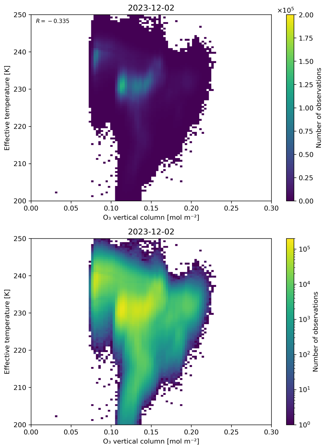
Figure 39: Scatter density plot of “O 3 vertical column” against “Effective temperature” for 2023-12-01 to 2023-12-03.
