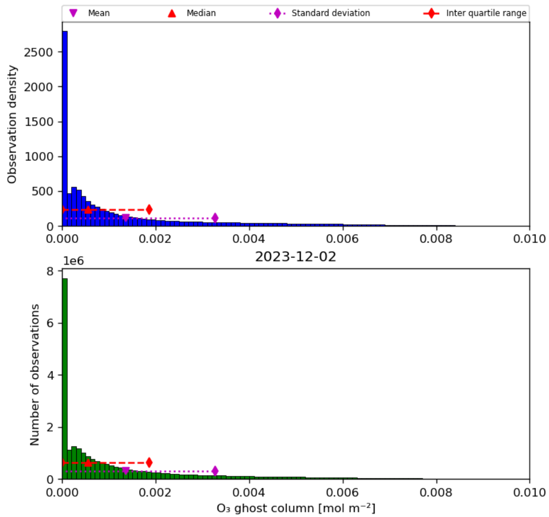
Figure 25: Histogram of "O 3 ghost column" for 2023-12-01 to 2023-12-03
