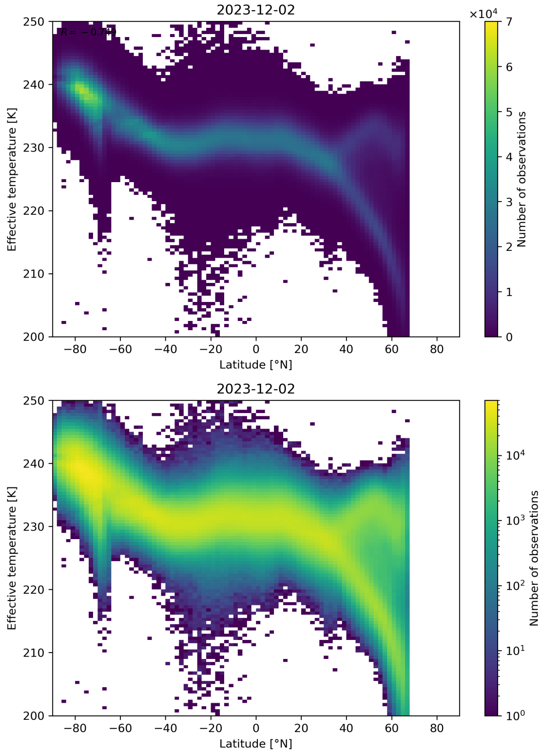
Figure 34: Scatter density plot of “Latitude” against “Effective temperature” for 2023-12-01 to 2023-12-03.
