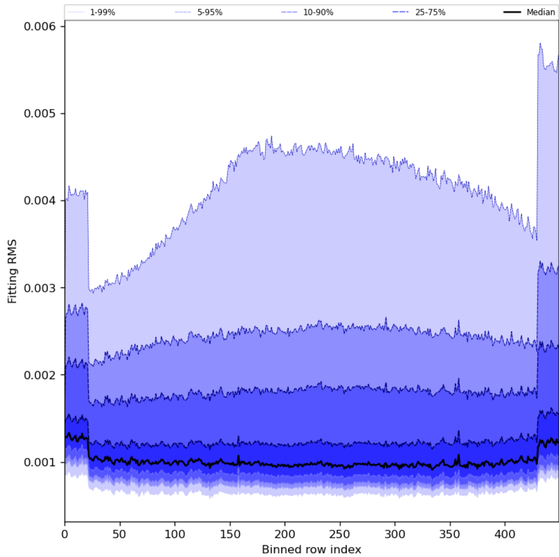
Figure 30: Along track statistics of “Fitting RMS” for 2023-12-01 to 2023-12-03
