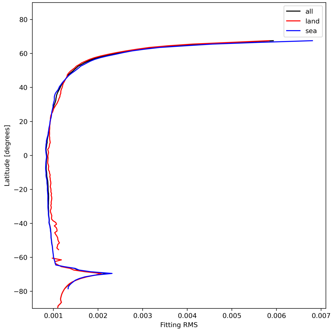
Figure 16: Zonal average of “Fitting RMS” for 2023-12-01 to 2023-12-03.
