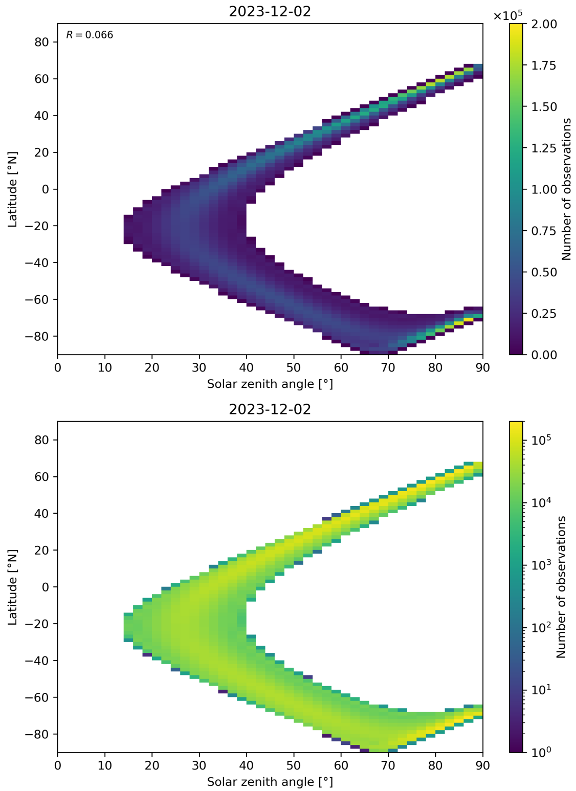
Figure 44: Scatter density plot of “Solar zenith angle” against “Latitude” for 2023-12-01 to 2023-12-03.
