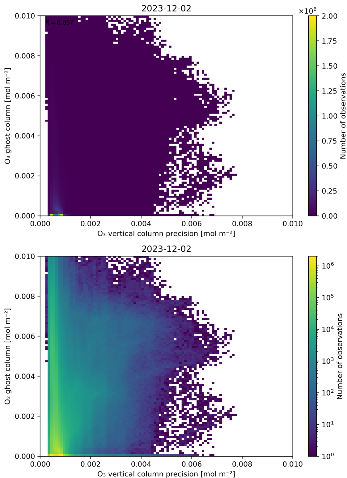
Figure 43: Scatter density plot of “ O_3 vertical column precision” against “ O_3 ghost column” for 2023-12-01 to 2023-12-03.
