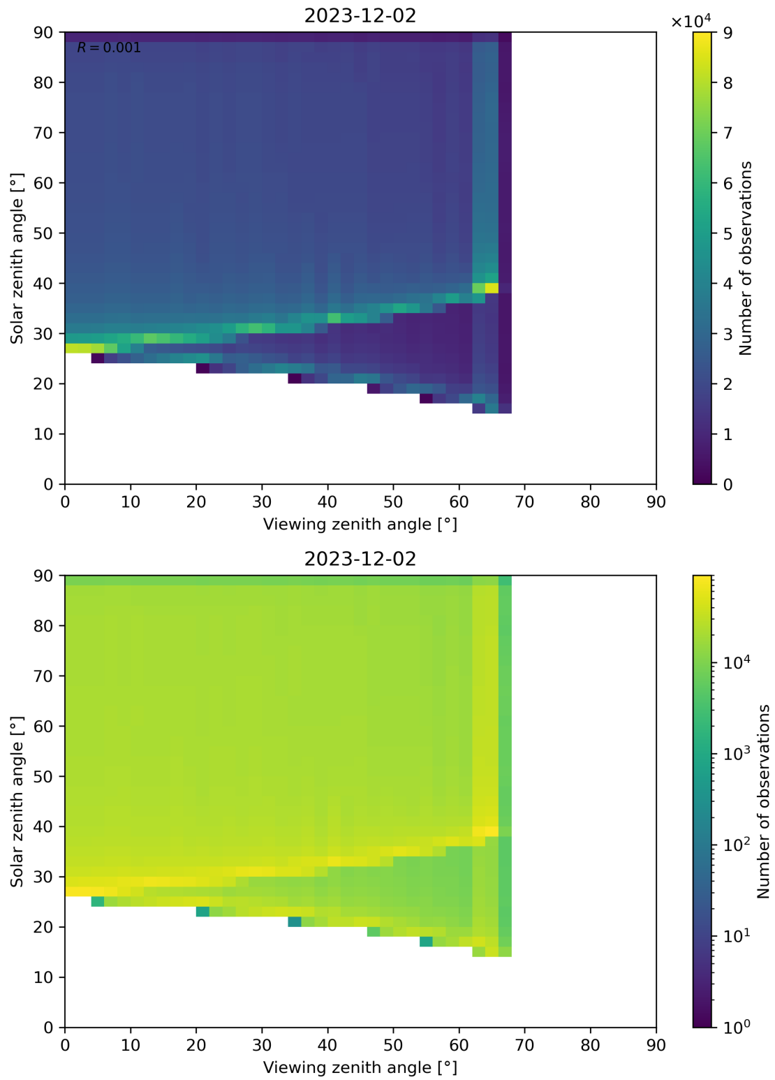
Figure 54: Scatter density plot of “Viewing zenith angle” against “Solar zenith angle” for 2023-12-01 to 2023-12-03.
