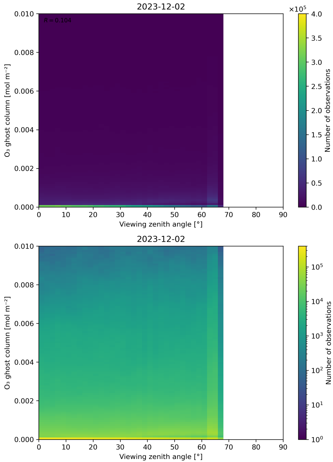
Figure 51: Scatter density plot of “Viewing zenith angle” against “O 3 ghost column” for 2023-12-01 to 2023-12-03.
