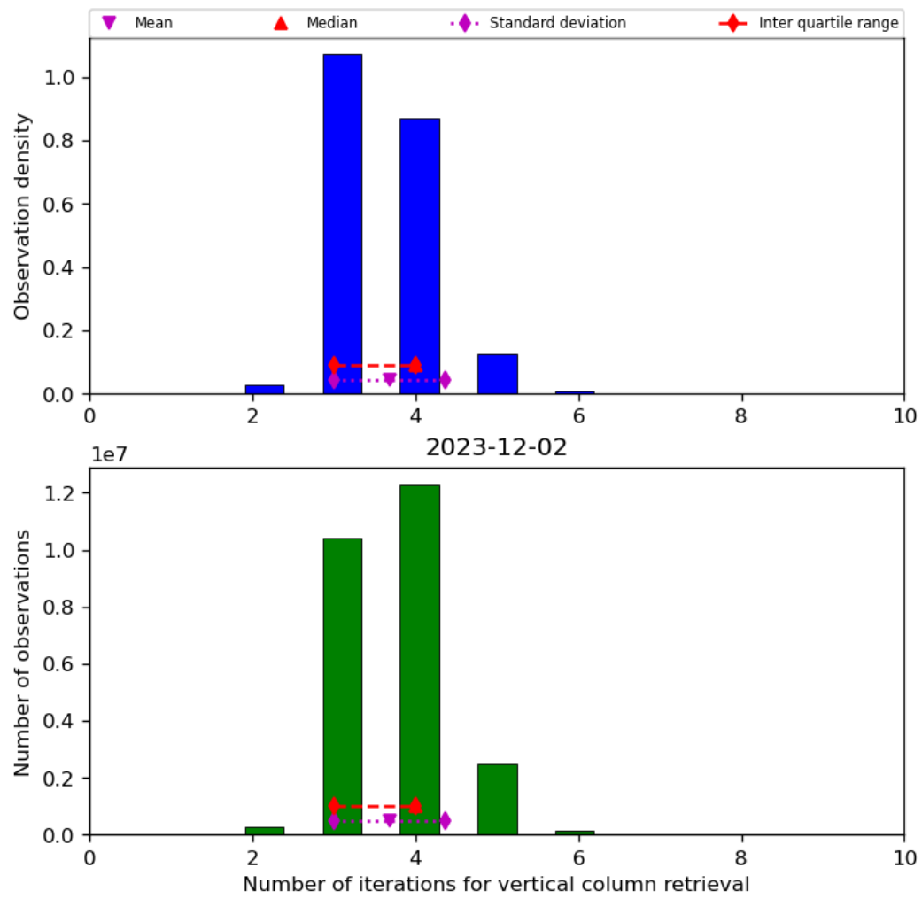
Figure 26: Histogram of “Number of iterations for vertical column retrieval” for 2023-12-01 to 2023-12-03
