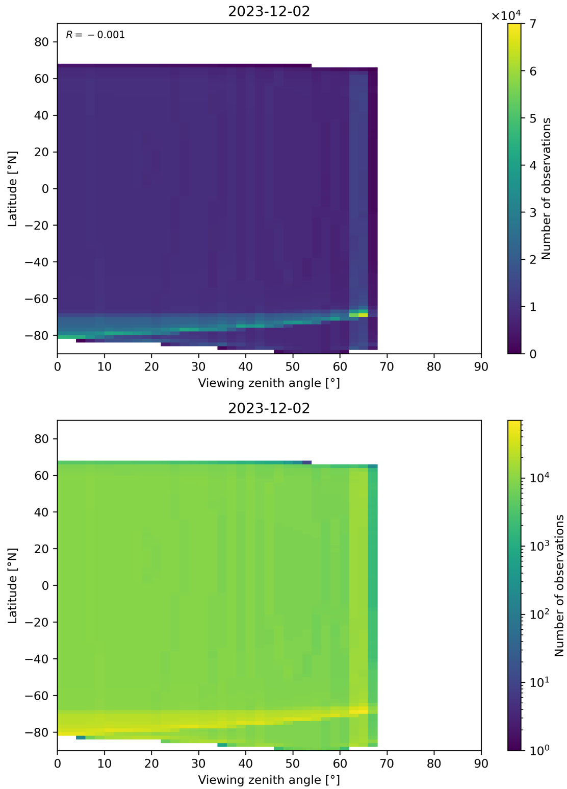
Figure 49: Scatter density plot of “Viewing zenith angle” against “Latitude” for 2023-12-01 to 2023-12-03.
