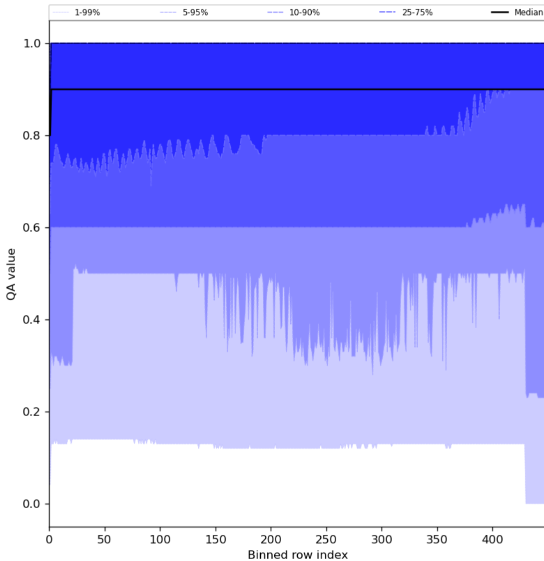
Figure 27: Along track statistics of “QA value” for 2023-12-01 to 2023-12-03
