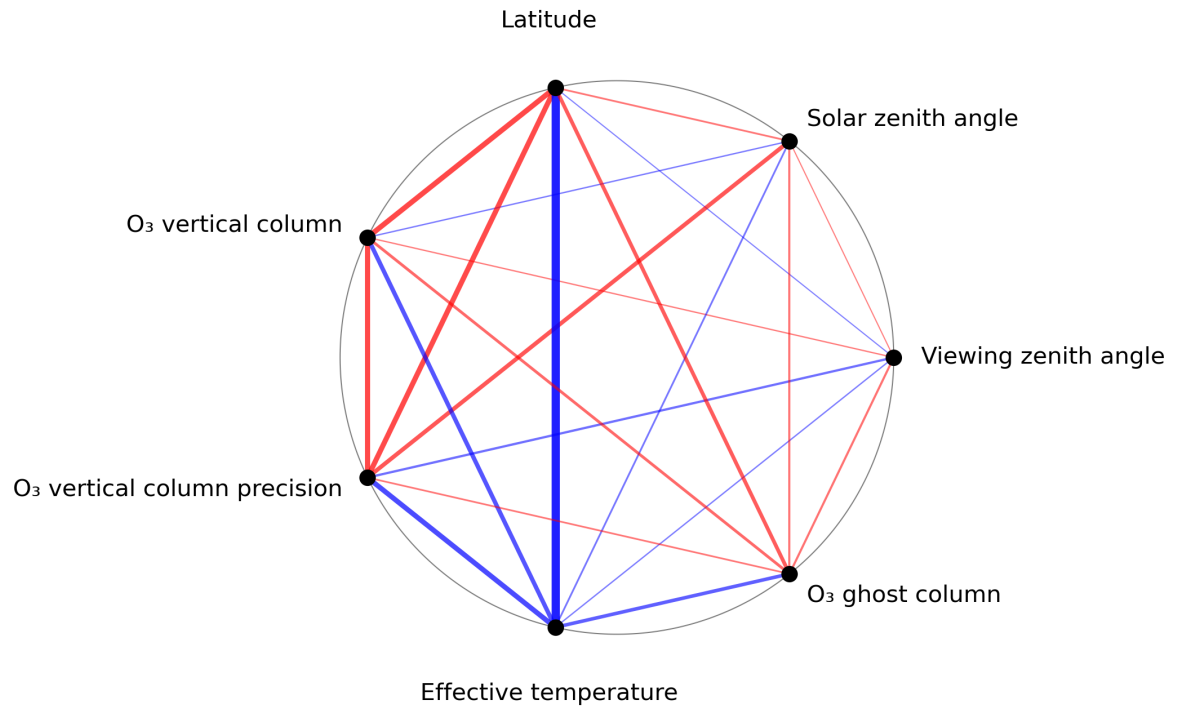
Figure 1: Map of correlation graph for 2023-12-01 to 2023-12-03.
