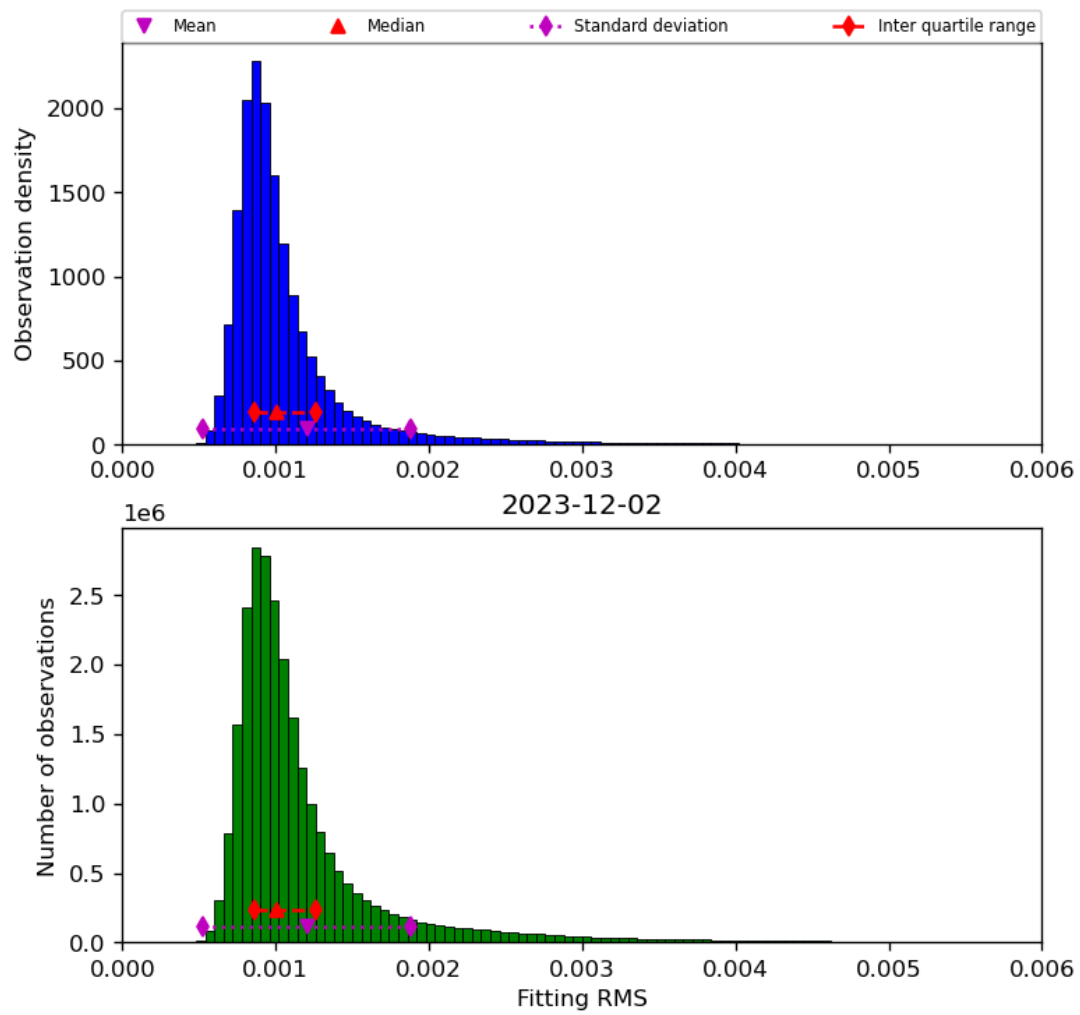
Figure 23: Histogram of “Fitting RMS” for 2023-12-01 to 2023-12-03
