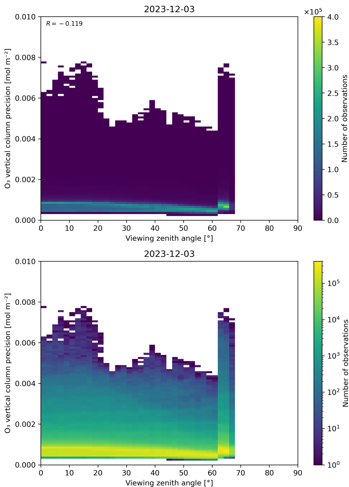
Figure 53: Scatter density plot of “Viewing zenith angle” against “O 3 vertical column precision” for 2023-12-02 to 2023-12-04.
