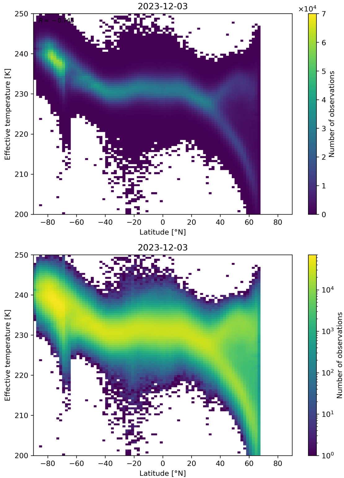
Figure 34: Scatter density plot of “Latitude” against “Effective temperature” for 2023-12-02 to 2023-12-04.
