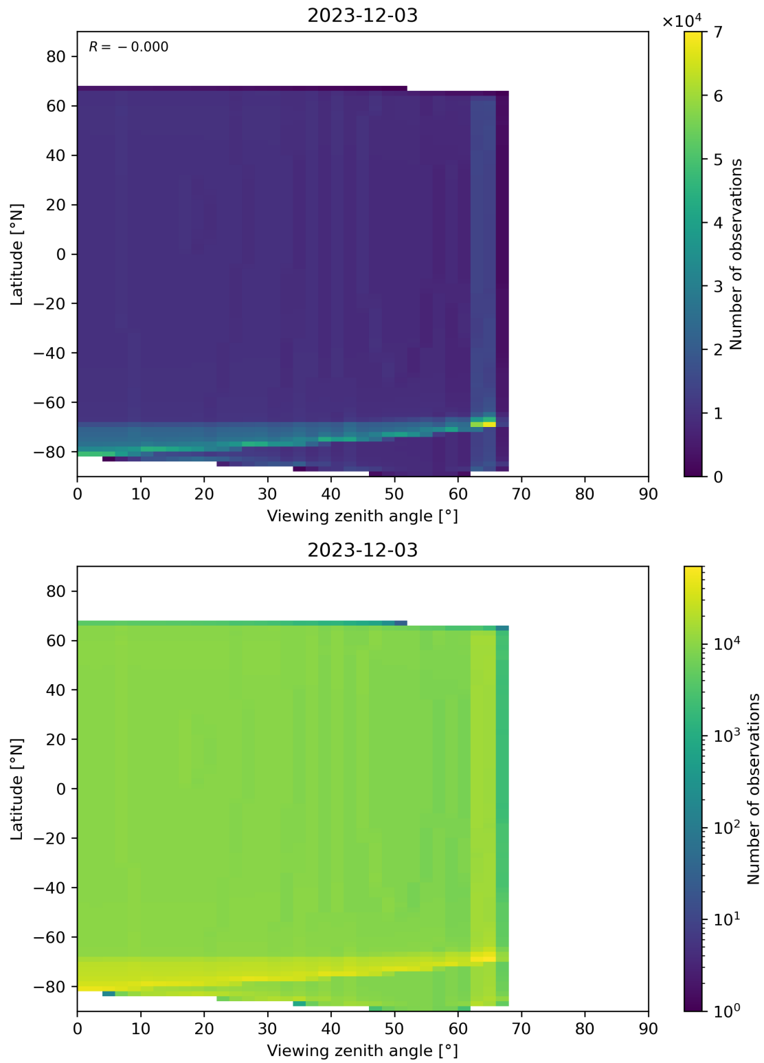
Figure 49: Scatter density plot of “Viewing zenith angle” against “Latitude” for 2023-12-02 to 2023-12-04.
