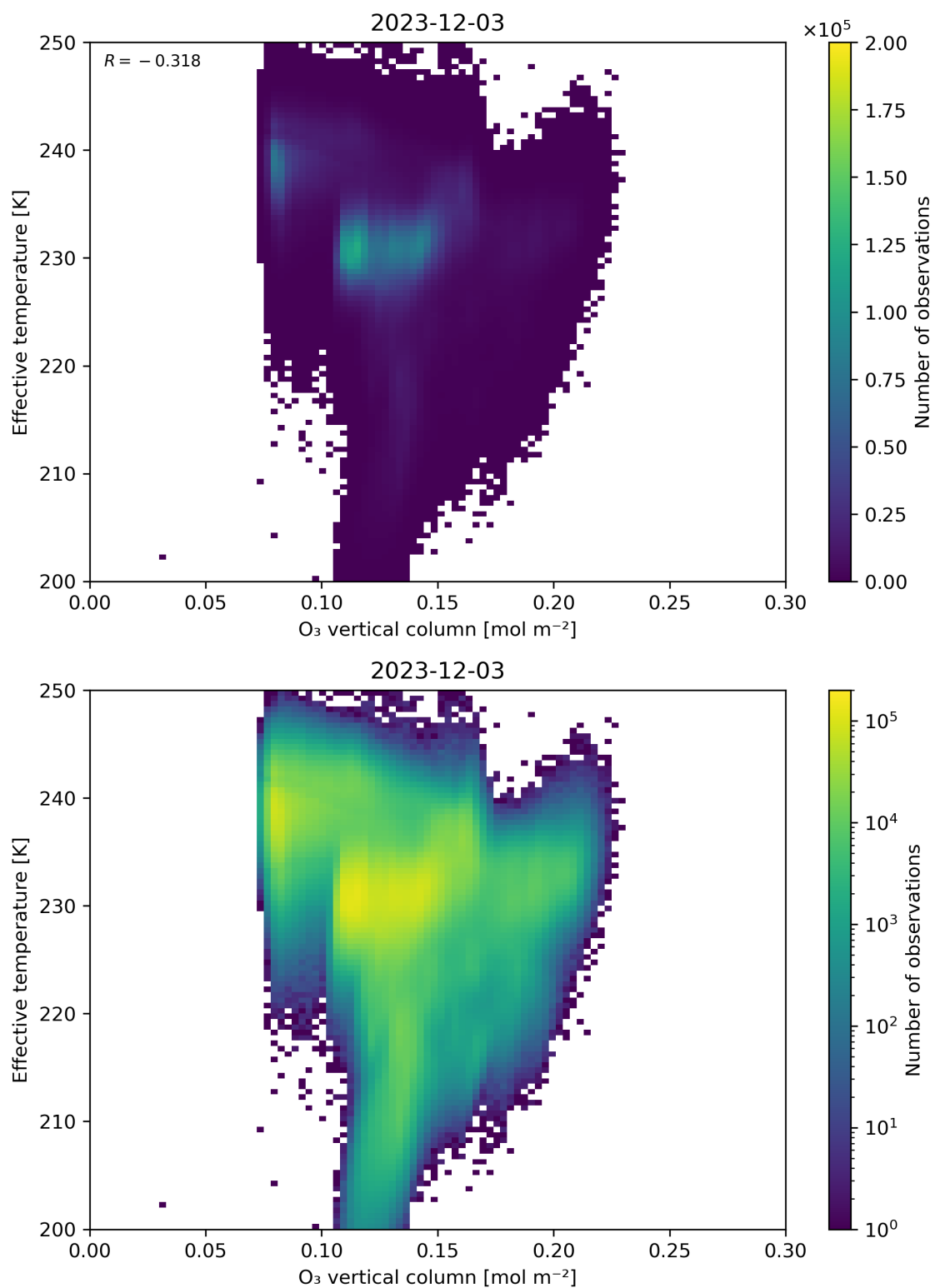
Figure 39: Scatter density plot of “O 3 vertical column” against “Effective temperature” for 2023-12-02 to 2023-12-04.
