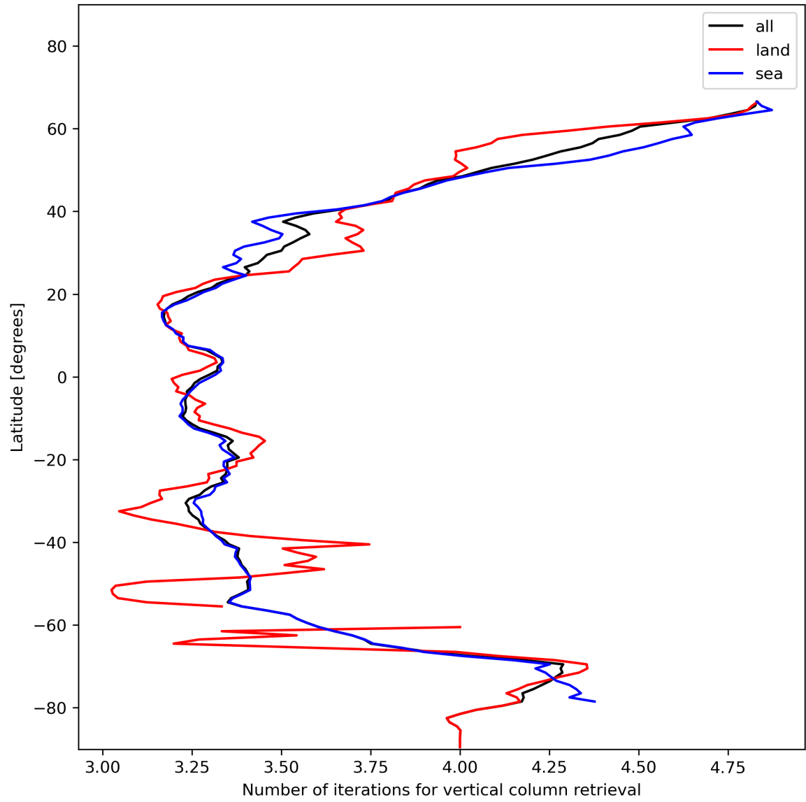
Figure 19: Zonal average of “Number of iterations for vertical column retrieval” for 2023-12-02 to 2023-12-04.
