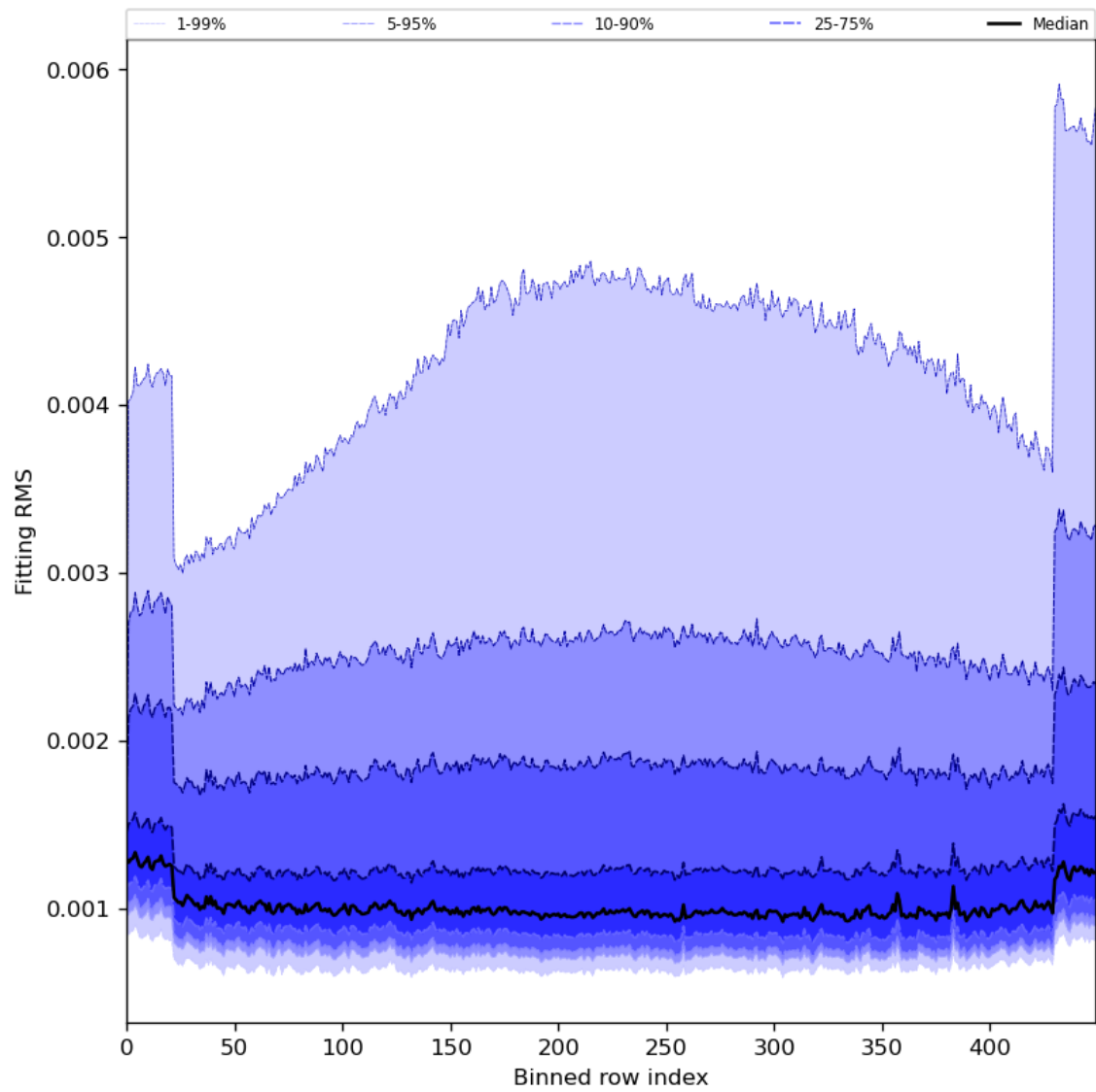
Figure 30: Along track statistics of “Fitting RMS” for 2023-12-02 to 2023-12-04
