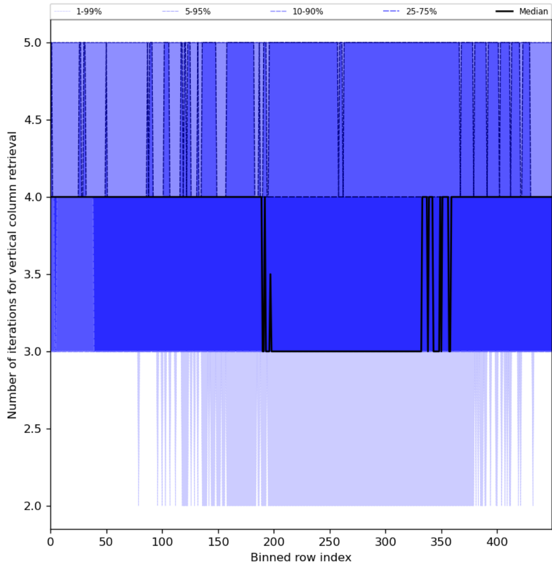
Figure 33: Along track statistics of “Number of iterations for vertical column retrieval” for 2023-12-02 to 2023-12-04
