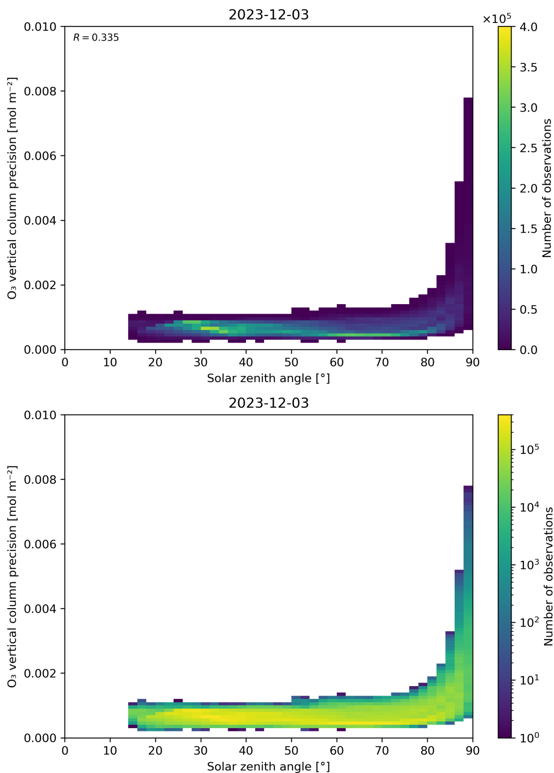
Figure 48: Scatter density plot of “Solar zenith angle” against “O 3 vertical column precision” for 2023-12-02 to 2023-12-04.
