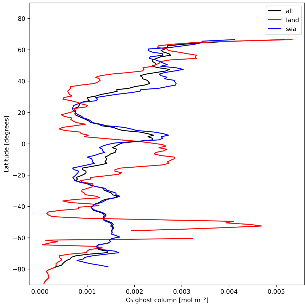
Figure 18: Zonal average of “O 3 ghost column” for 2023-12-02 to 2023-12-04.
