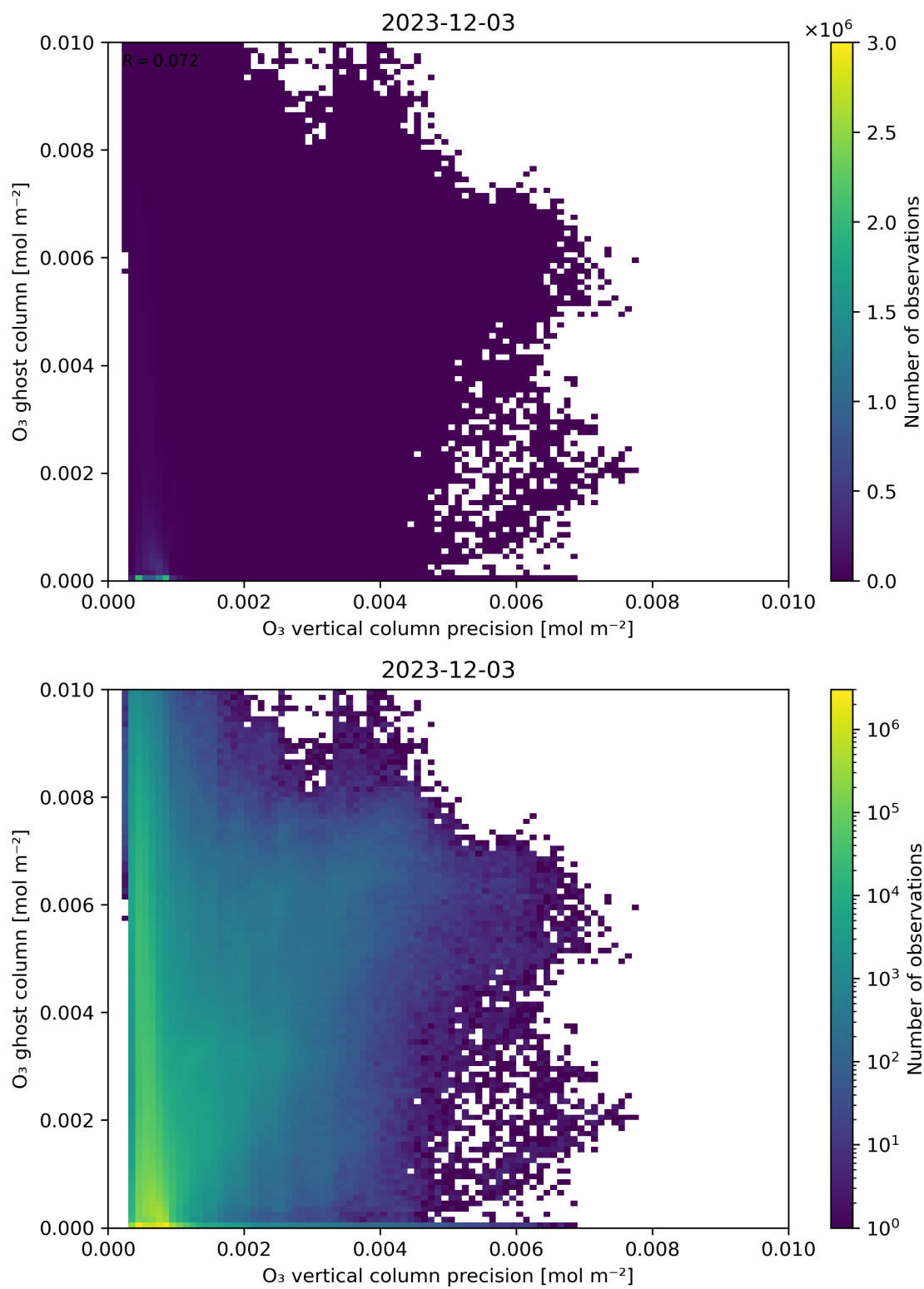
Figure 43: Scatter density plot of “O 3 vertical column precision” against “O 3 ghost column” for 2023-12-02 to 2023-12-04.
