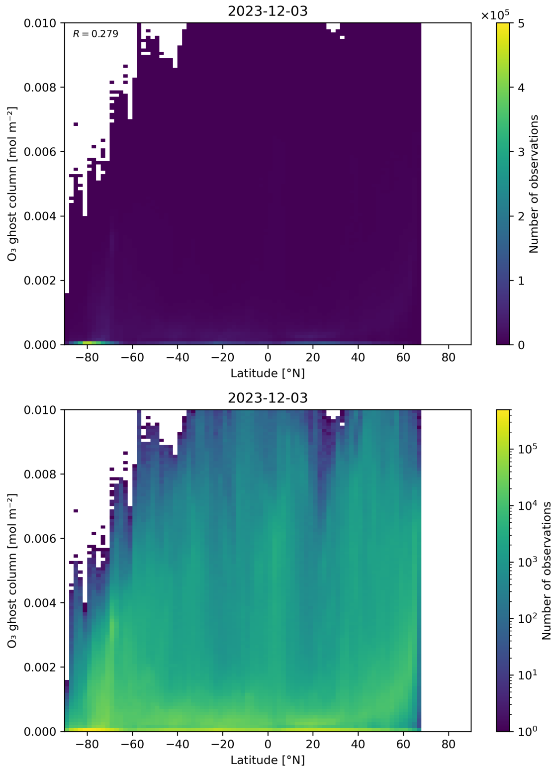
Figure 35: Scatter density plot of “Latitude” against “O 3 ghost column” for 2023-12-02 to 2023-12-04.
