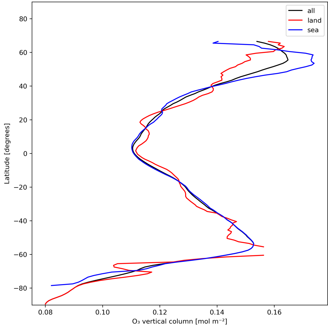
Figure 14: Zonal average of “O 3 vertical column” for 2023-12-02 to 2023-12-04.
