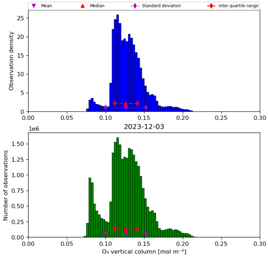
Figure 21: Histogram of “O 3 vertical column” for 2023-12-02 to 2023-12-04
