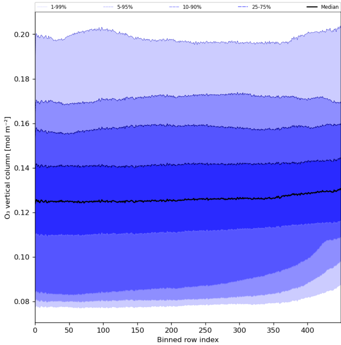
Figure 28: Along track statistics of “O 3 vertical column” for 2023-12-02 to 2023-12-04
