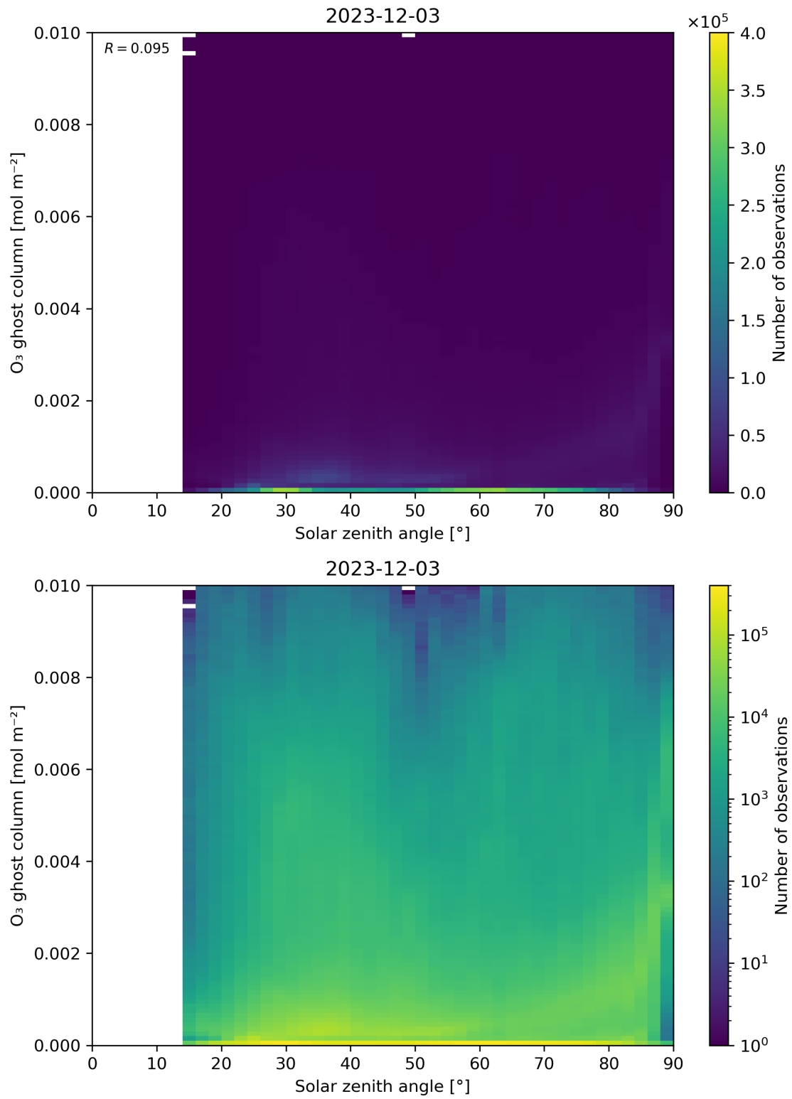
Figure 46: Scatter density plot of “Solar zenith angle” against “O 3 ghost column” for 2023-12-02 to 2023-12-04.
