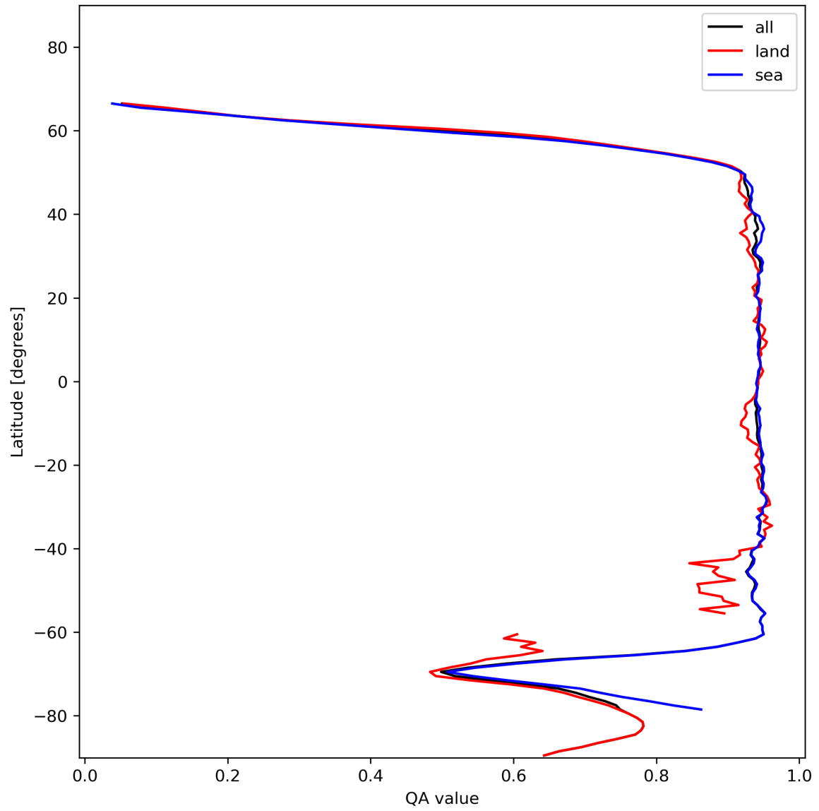
Figure 13: Zonal average of “QA value” for 2023-12-02 to 2023-12-04.
