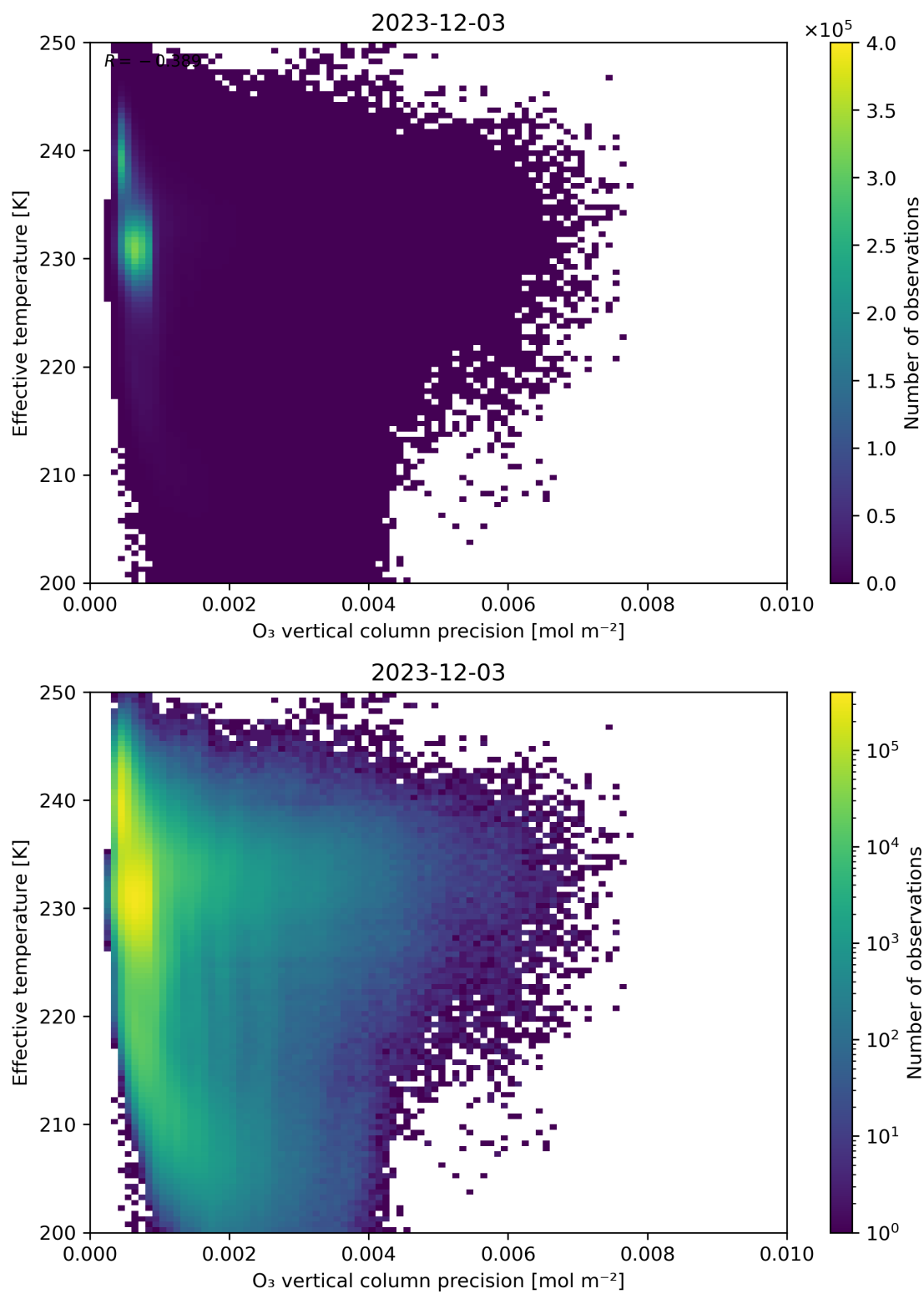
Figure 42: Scatter density plot of “O 3 vertical column precision” against “Effective temperature” for 2023-12-02 to 2023-12-04.
