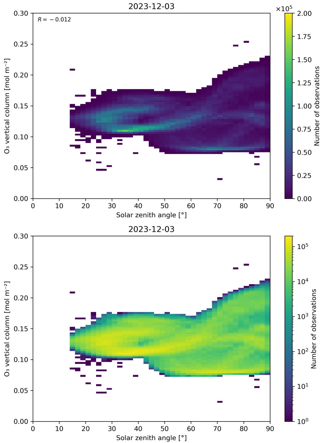
Figure 47: Scatter density plot of “Solar zenith angle” against “O 3 vertical column” for 2023-12-02 to 2023-12-04.
