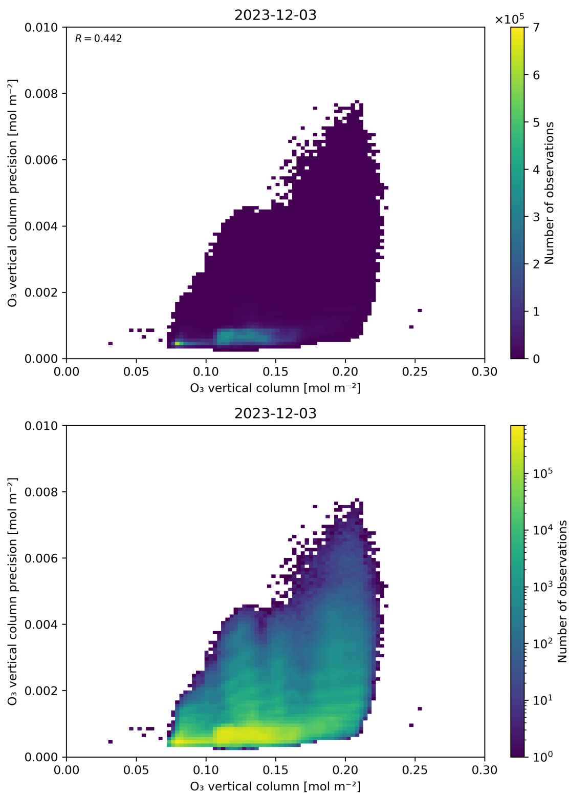
Figure 41: Scatter density plot of “O 3 vertical column” against “O 3 vertical column precision” for 2023-12-02 to 2023-12-04.
