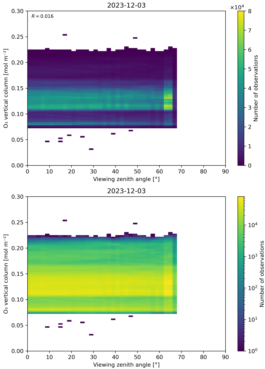
Figure 52: Scatter density plot of “Viewing zenith angle” against “O 3 vertical column” for 2023-12-02 to 2023-12-04.
