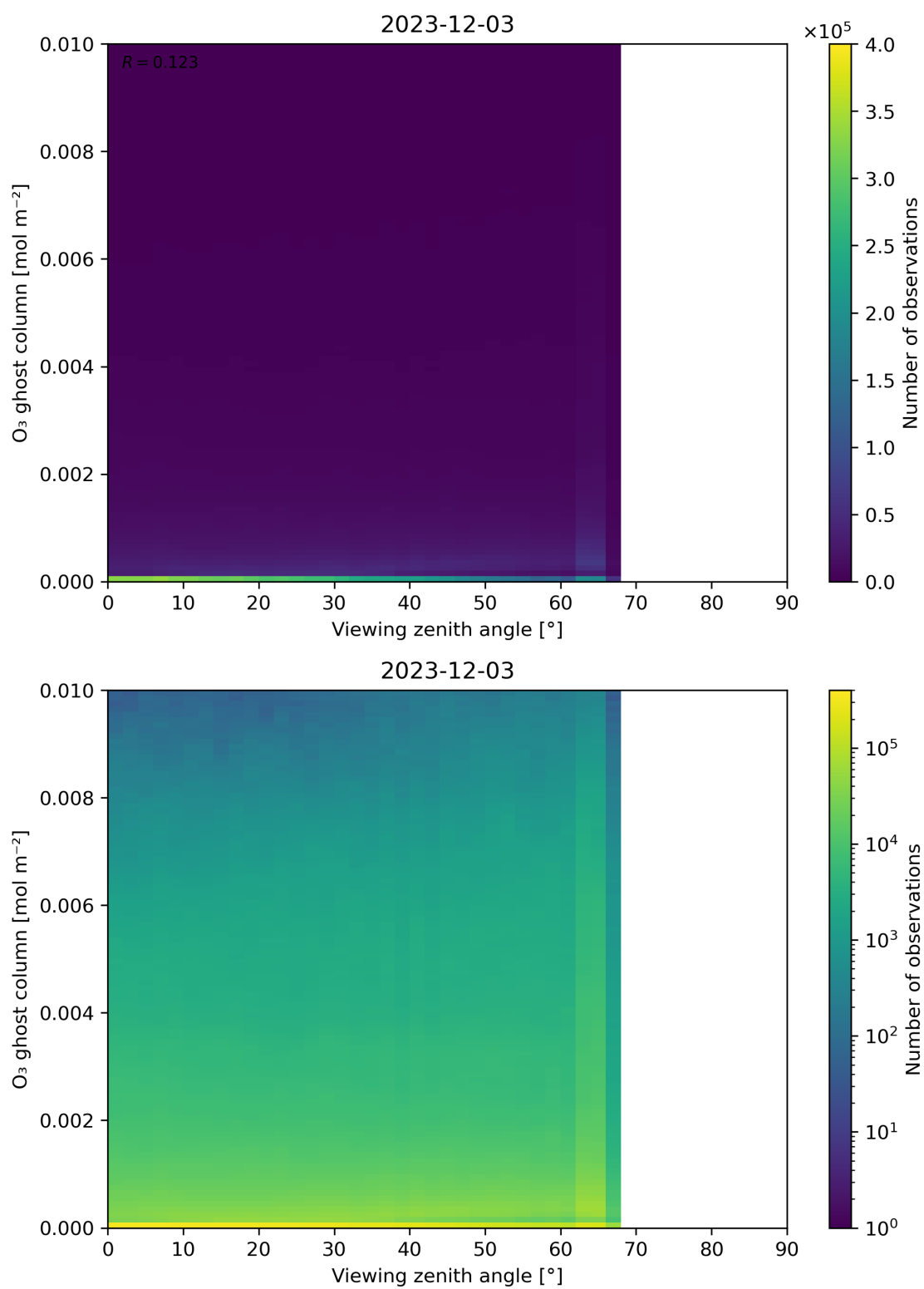
Figure 51: Scatter density plot of “Viewing zenith angle” against “O 3 ghost column” for 2023-12-02 to 2023-12-04.
