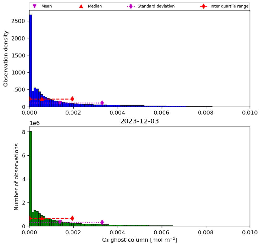
Figure 25: Histogram of “O 3 ghost column” for 2023-12-02 to 2023-12-04
