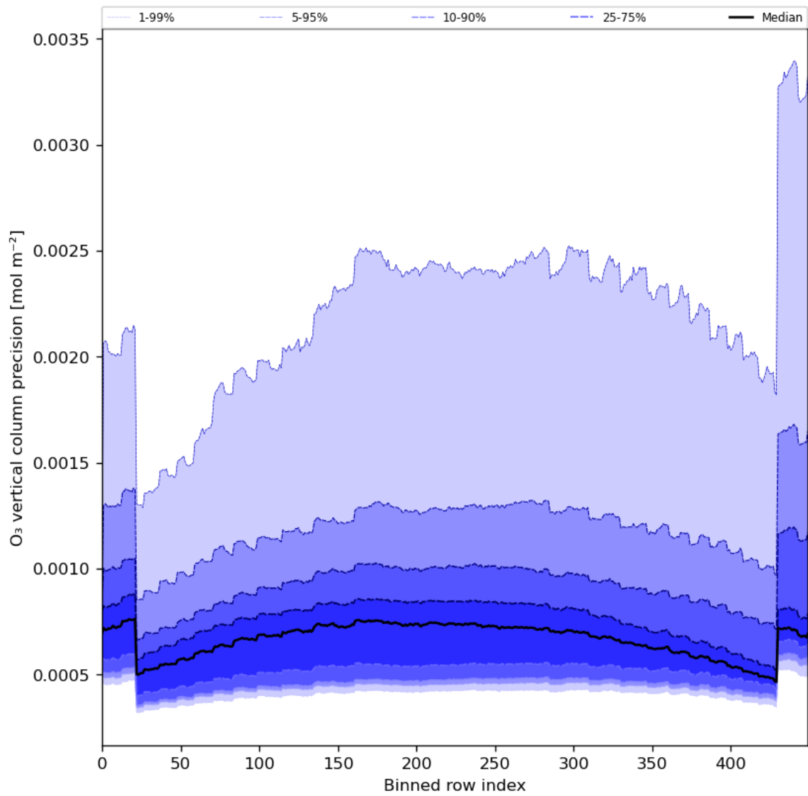
Figure 29: Along track statistics of “O 3 vertical column precision” for 2023-12-02 to 2023-12-04
