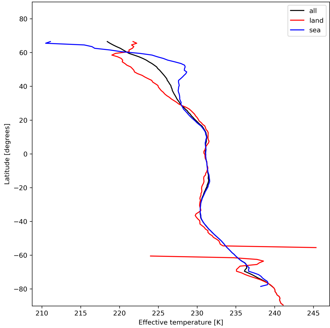
Figure 17: Zonal average of “Effective temperature” for 2023-12-02 to 2023-12-04.
