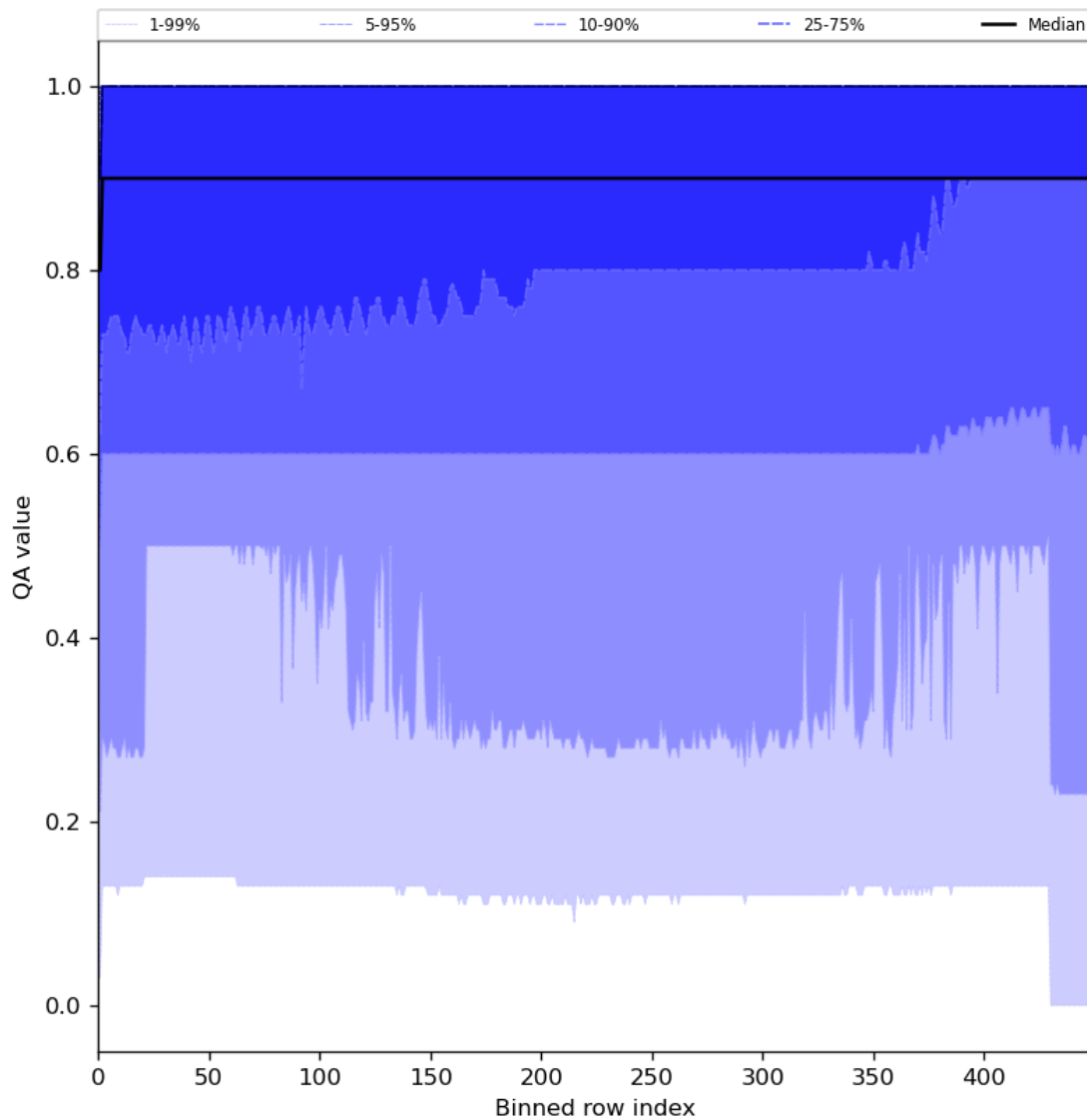
Figure 27: Along track statistics of “QA value” for 2023-12-02 to 2023-12-04
