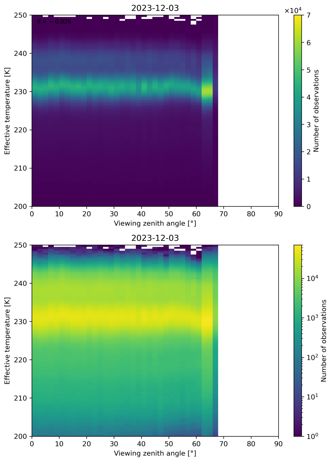
Figure 50: Scatter density plot of “Viewing zenith angle” against “Effective temperature” for 2023-12-02 to 2023-12-04.
