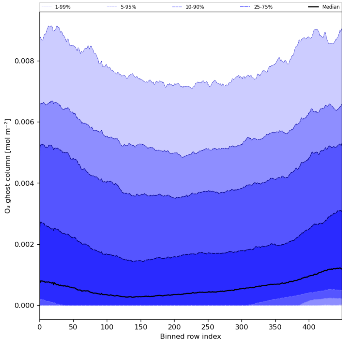
Figure 32: Along track statistics of “O 3 ghost column” for 2023-12-02 to 2023-12-04
