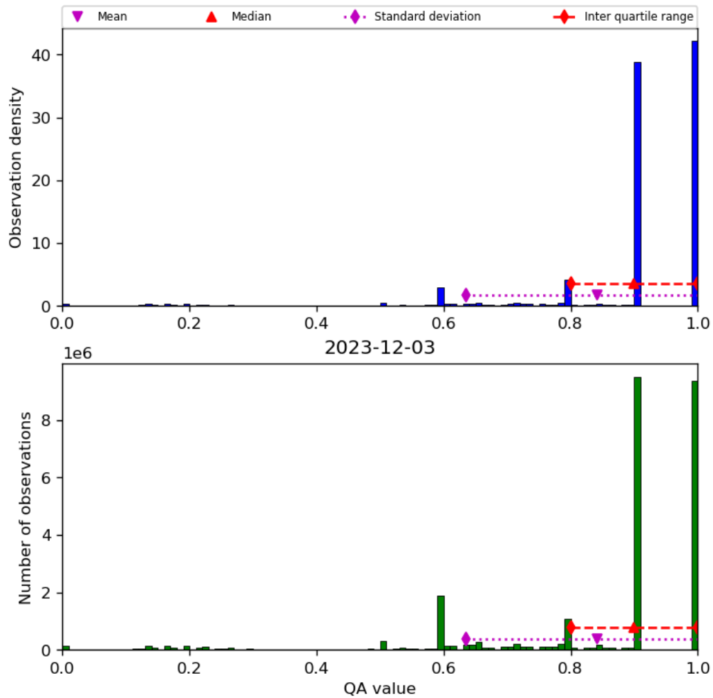
Figure 20: Histogram of “QA value” for 2023-12-02 to 2023-12-04
