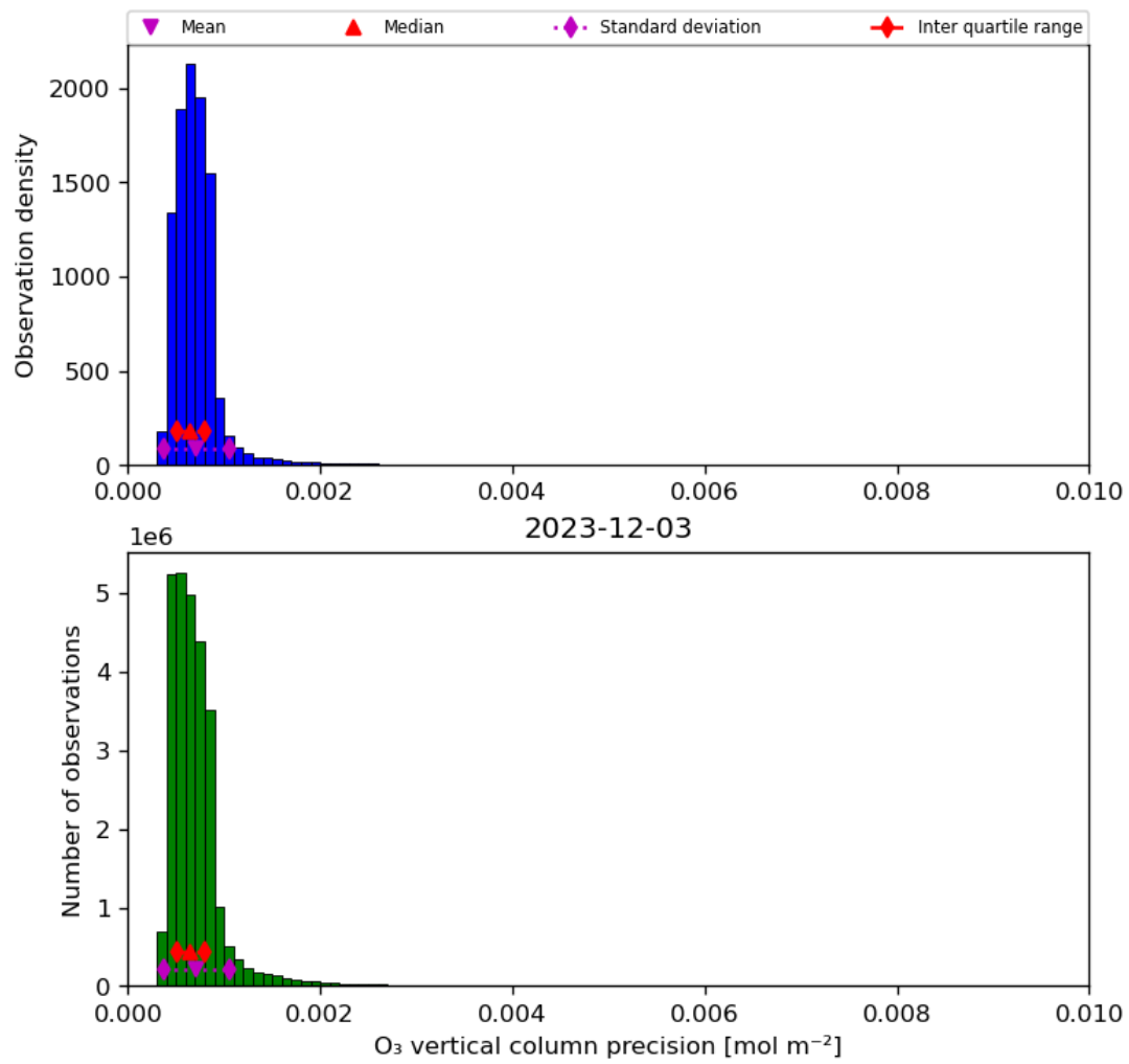
Figure 22: Histogram of “O 3 vertical column precision” for 2023-12-02 to 2023-12-04
