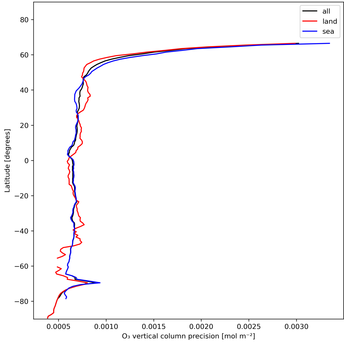
Figure 15: Zonal average of “O 3 vertical column precision” for 2023-12-02 to 2023-12-04.
