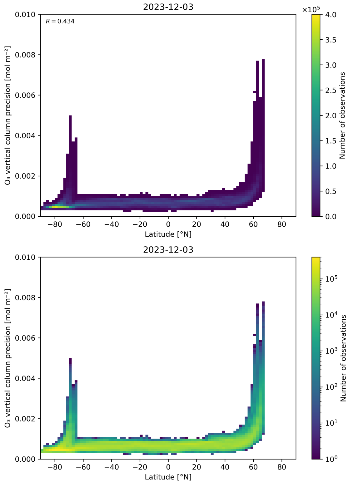
Figure 37: Scatter density plot of “Latitude” against “O 3 vertical column precision” for 2023-12-02 to 2023-12-04.
