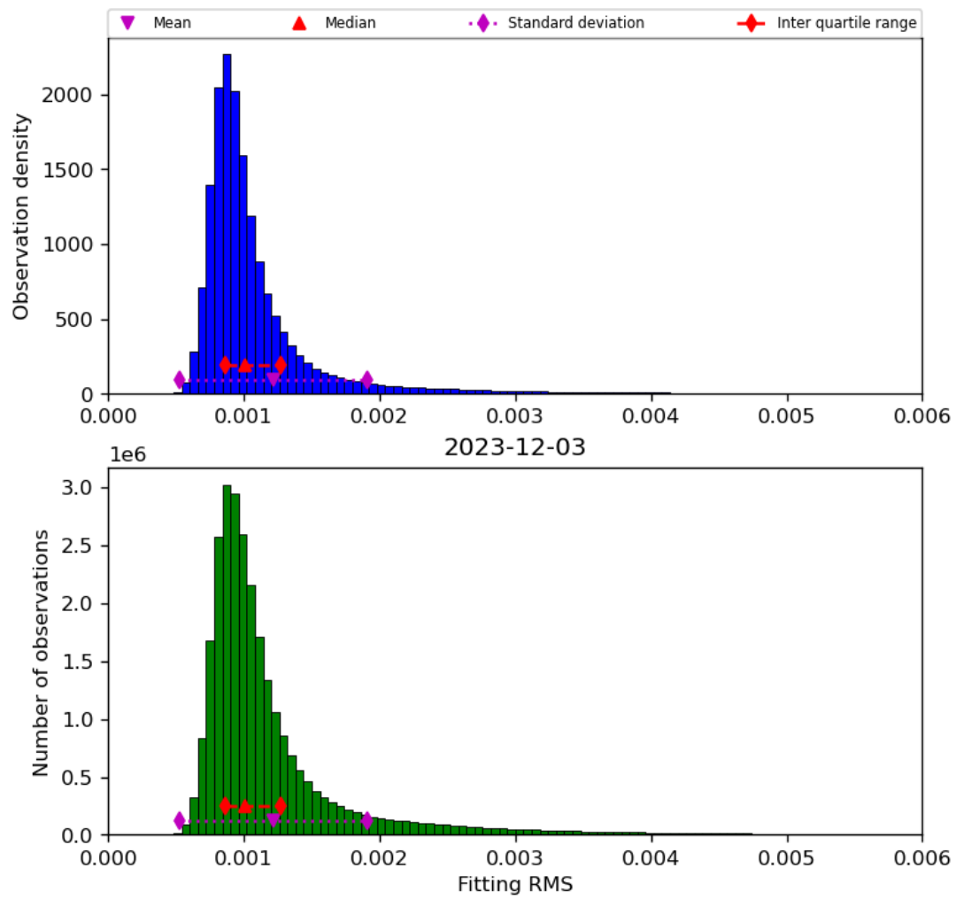
Figure 23: Histogram of “Fitting RMS” for 2023-12-02 to 2023-12-04
