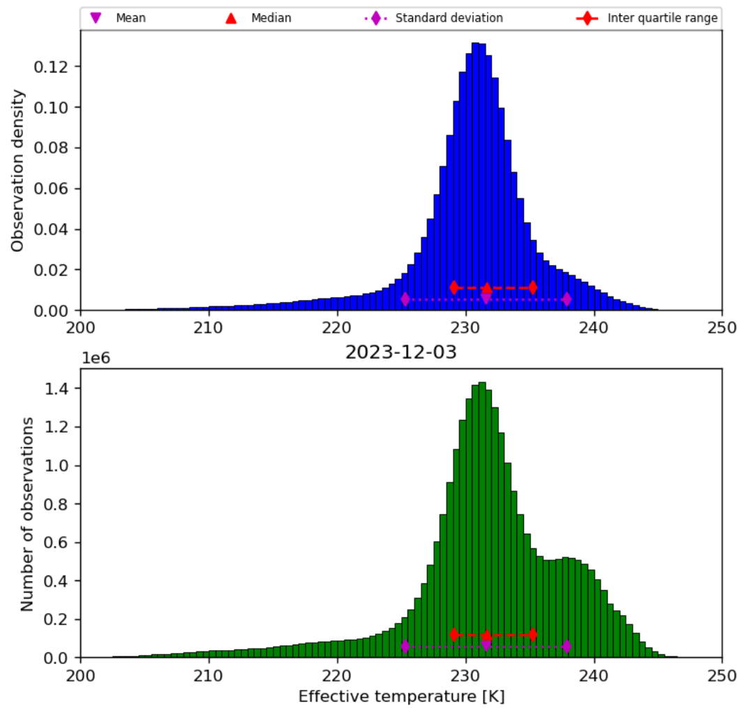
Figure 24: Histogram of “Effective temperature” for 2023-12-02 to 2023-12-04
