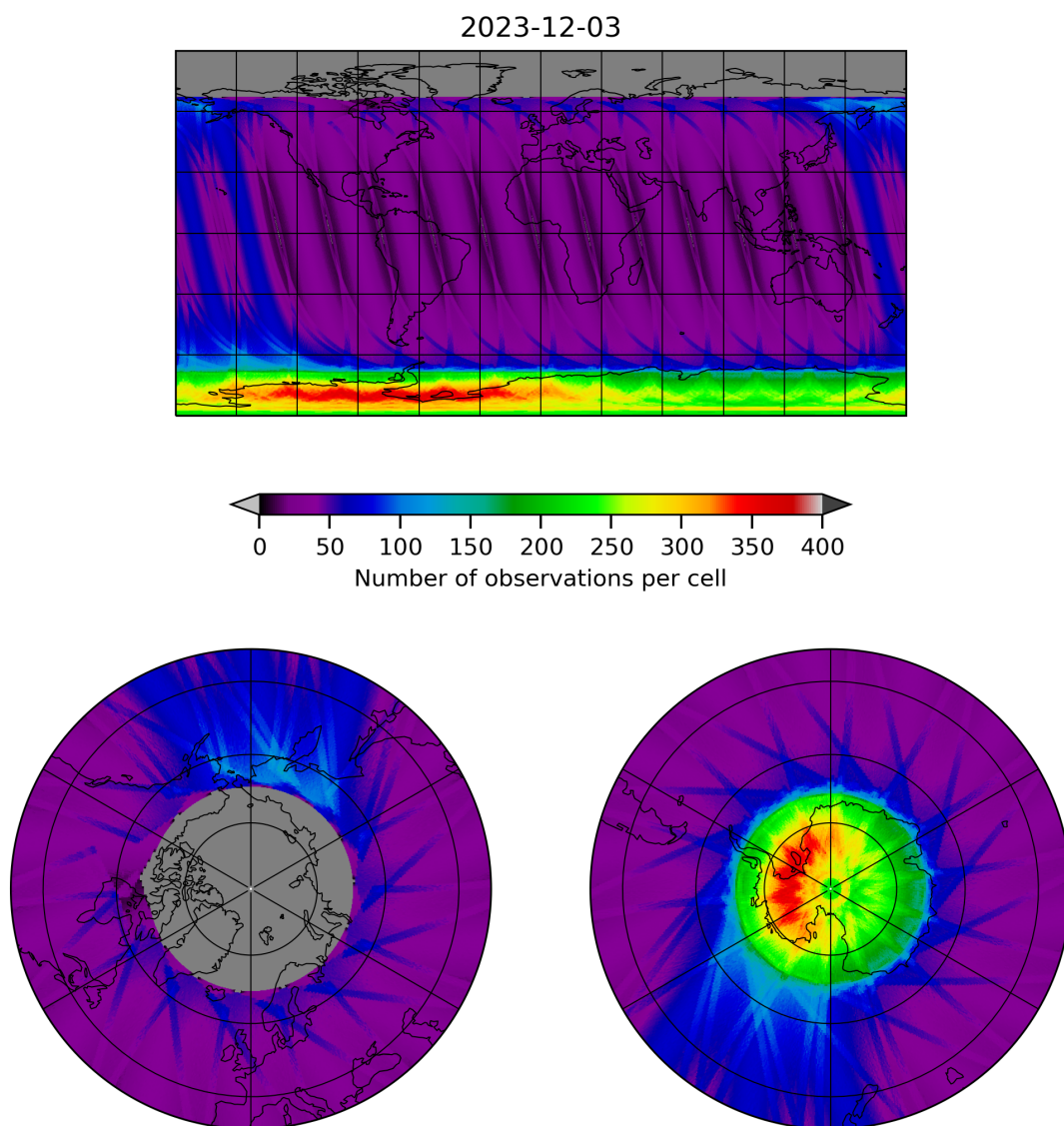
Figure 12: Map of the number of observations for 2023-12-02 to 2023-12-04
