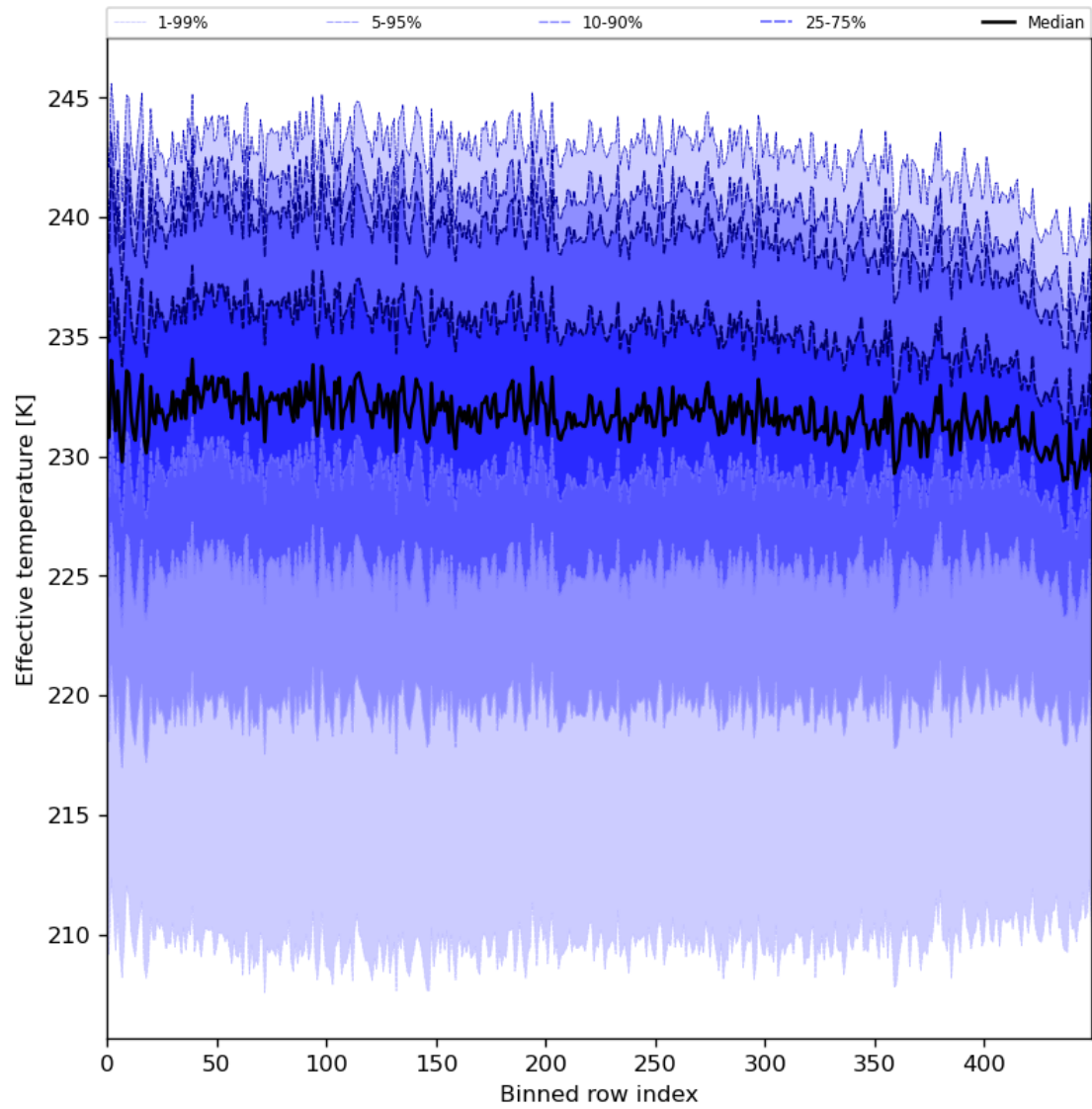
Figure 31: Along track statistics of “Effective temperature” for 2023-12-02 to 2023-12-04
