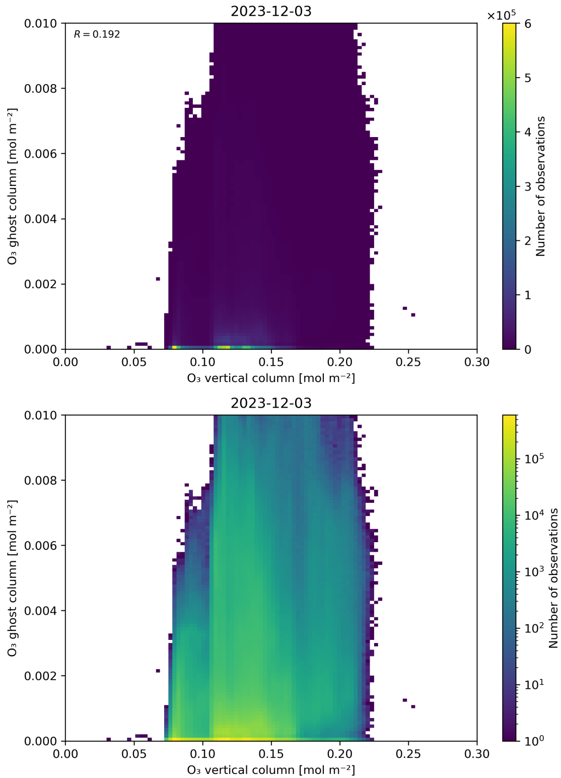
Figure 40: Scatter density plot of “O 3 vertical column” against “O 3 ghost column” for 2023-12-02 to 2023-12-04.
