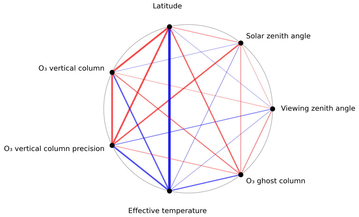
Figure 1: Map of correlation graph for 2023-12-02 to 2023-12-04.
