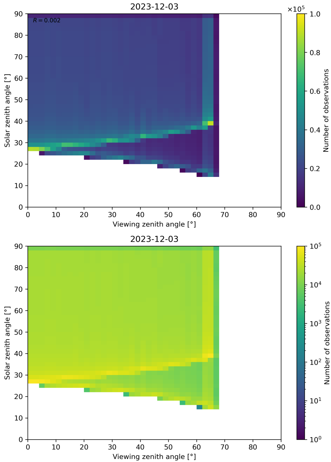
Figure 54: Scatter density plot of “Viewing zenith angle” against “Solar zenith angle” for 2023-12-02 to 2023-12-04.
