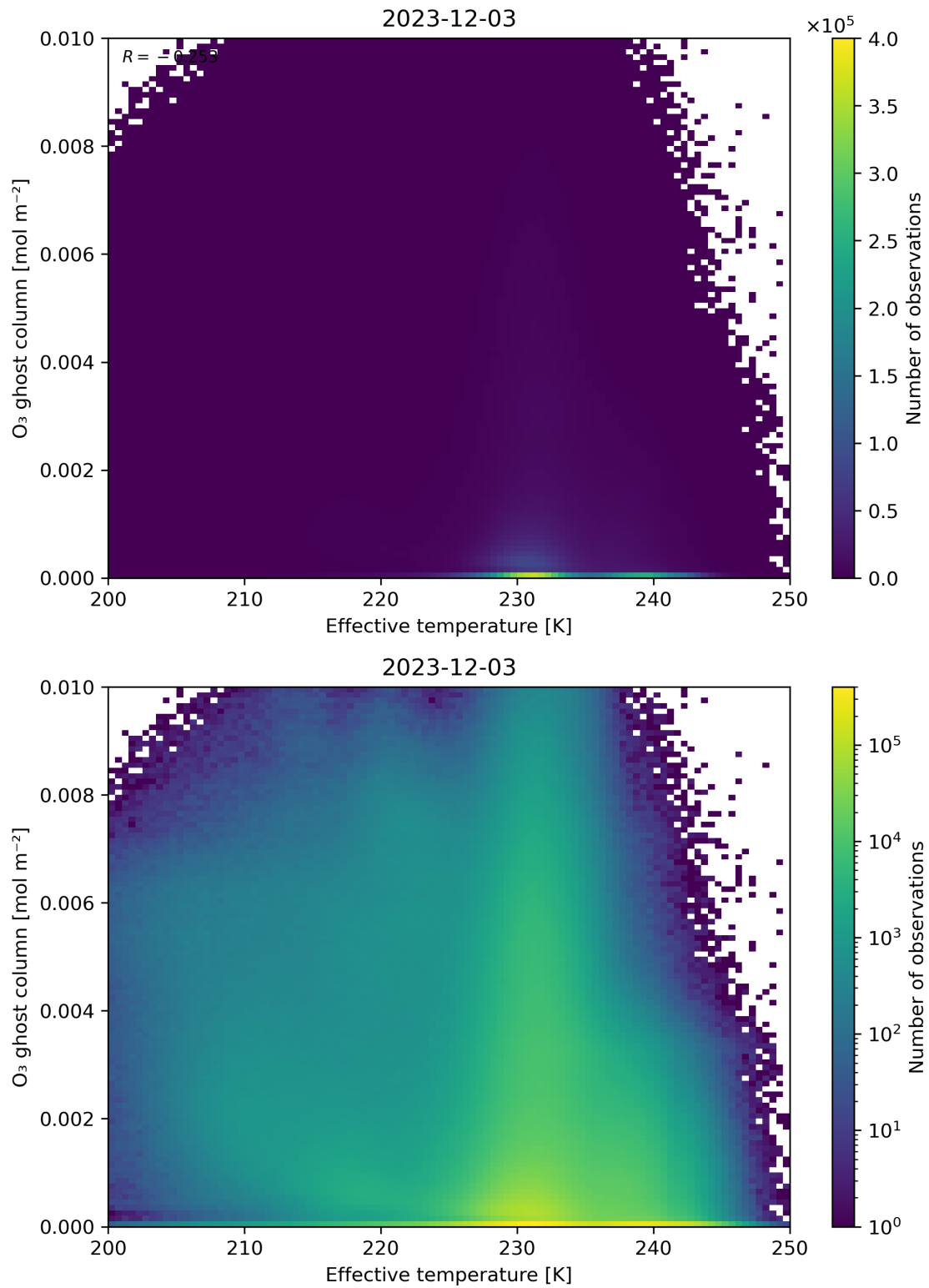
Figure 38: Scatter density plot of “Effective temperature” against “O 3 ghost column” for 2023-12-02 to 2023-12-04.
