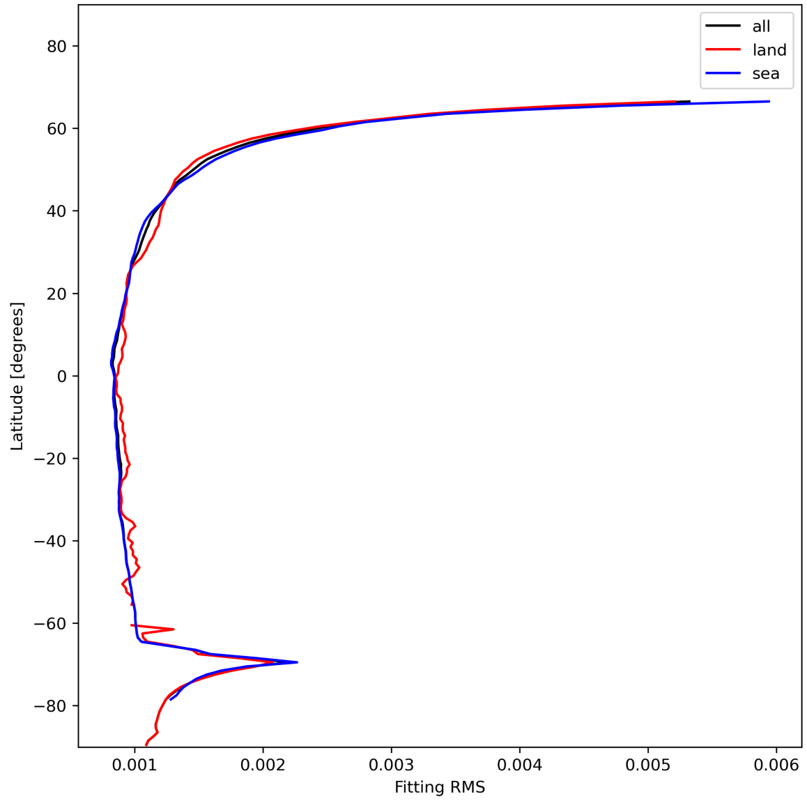
Figure 16: Zonal average of “Fitting RMS” for 2023-12-02 to 2023-12-04.
