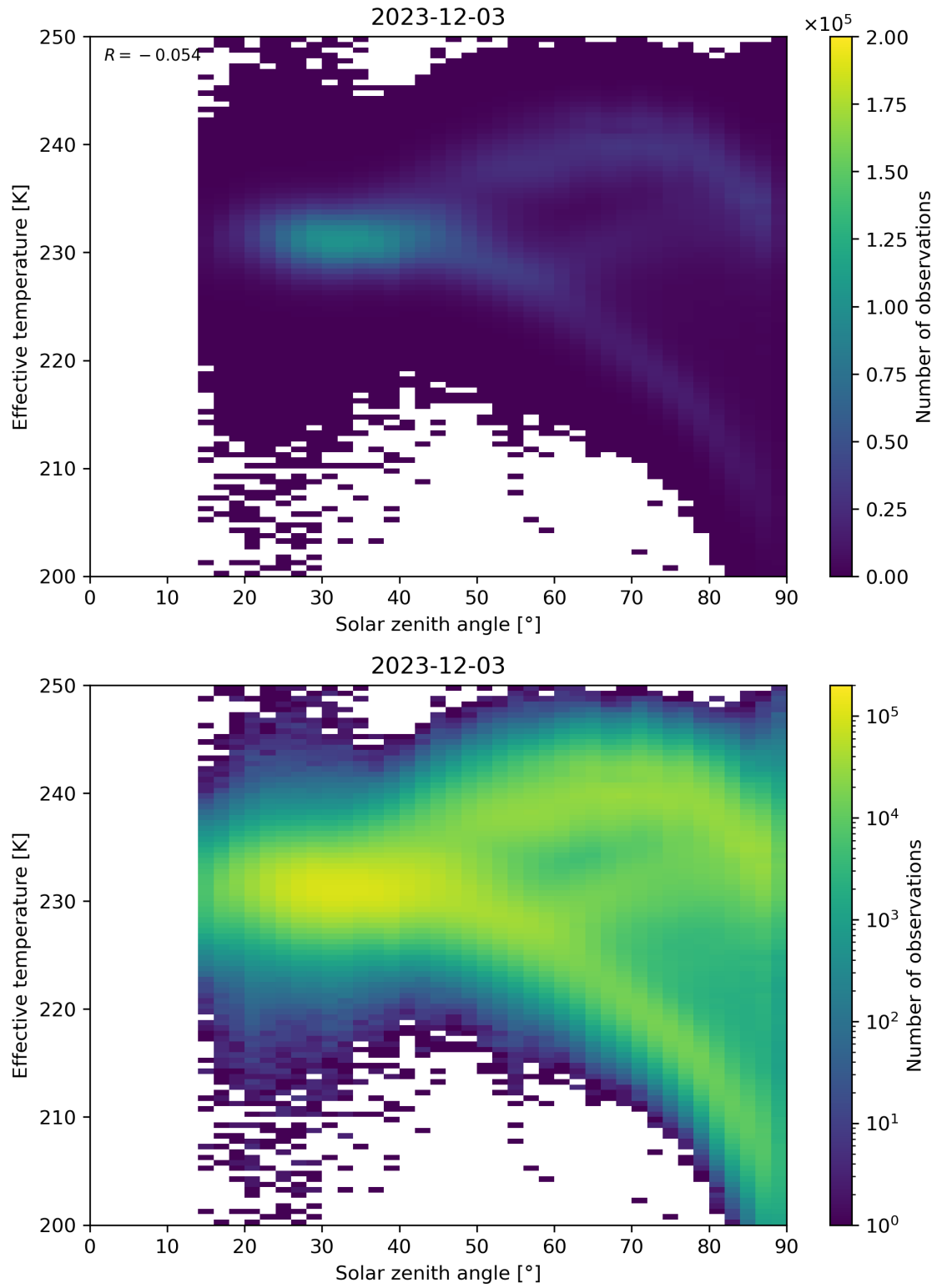
Figure 45: Scatter density plot of “Solar zenith angle” against “Effective temperature” for 2023-12-02 to 2023-12-04.
