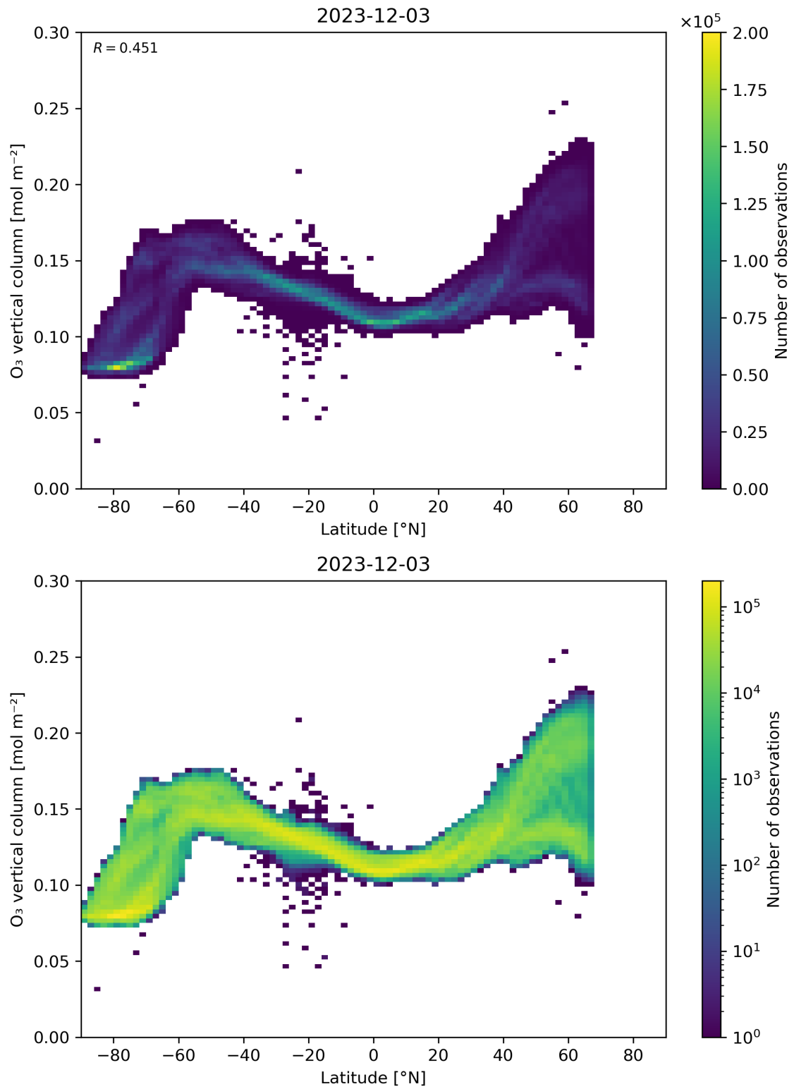
Figure 36: Scatter density plot of “Latitude” against “O 3 vertical column” for 2023-12-02 to 2023-12-04.
