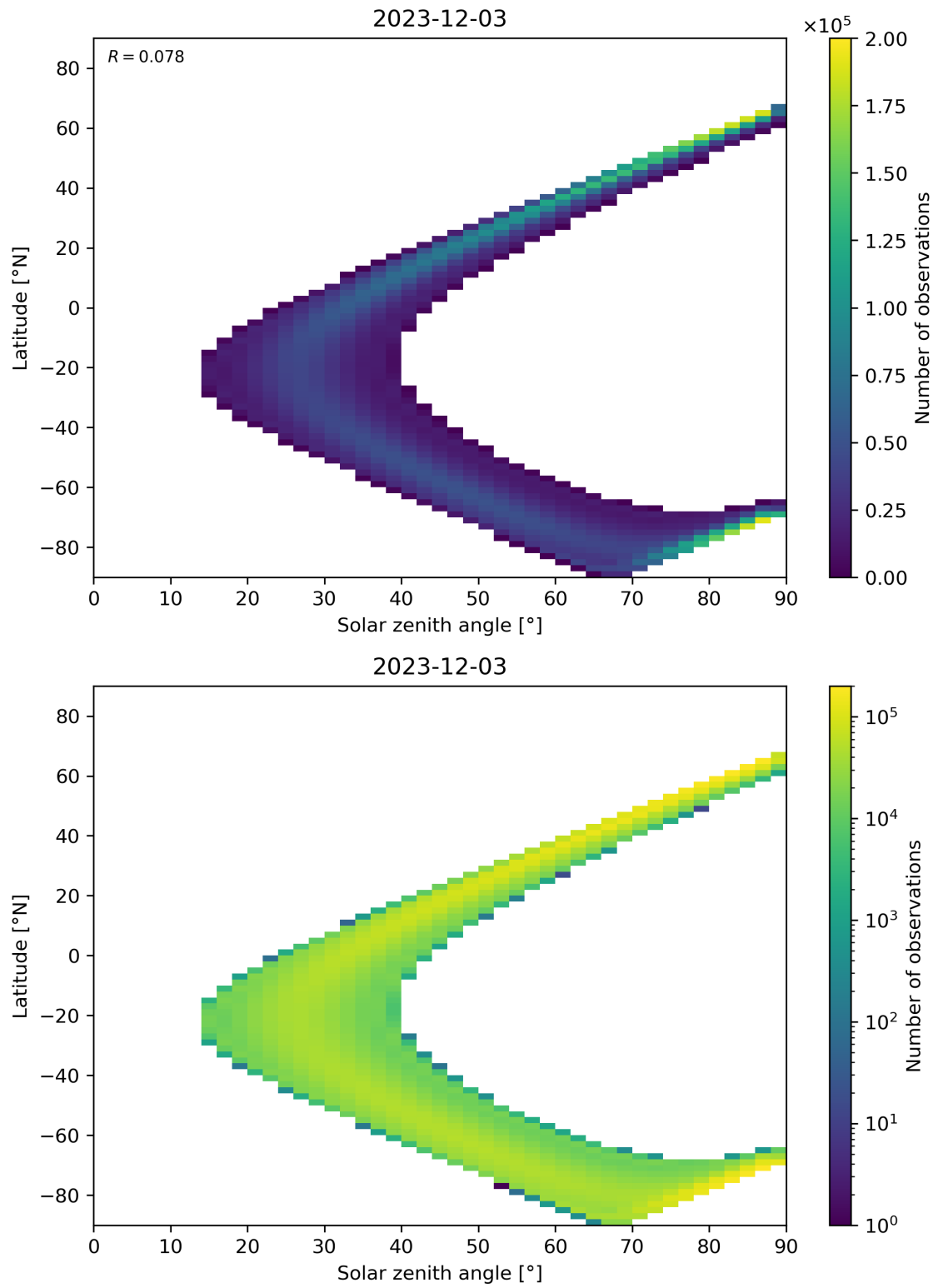
Figure 44: Scatter density plot of “Solar zenith angle” against “Latitude” for 2023-12-02 to 2023-12-04.
