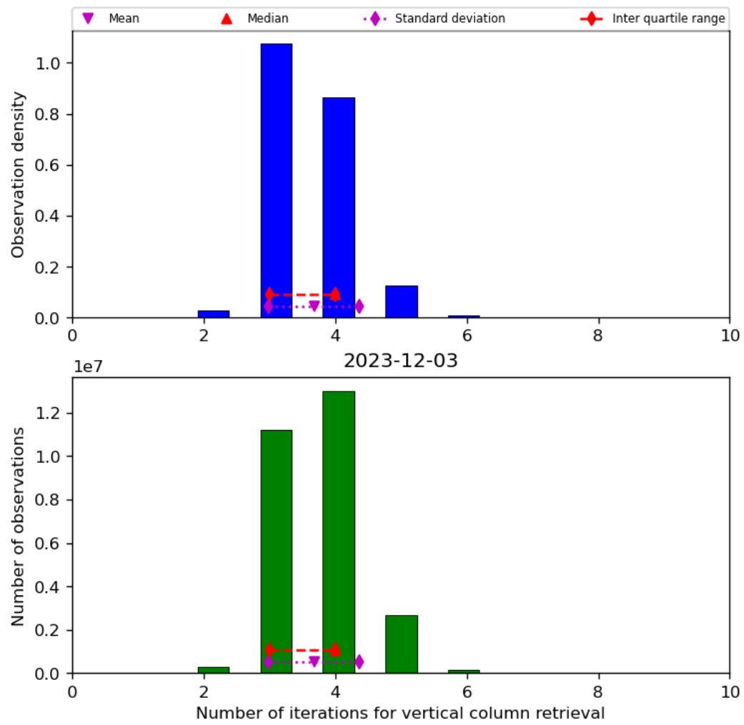
Figure 26: Histogram of “Number of iterations for vertical column retrieval” for 2023-12-02 to 2023-12-04
