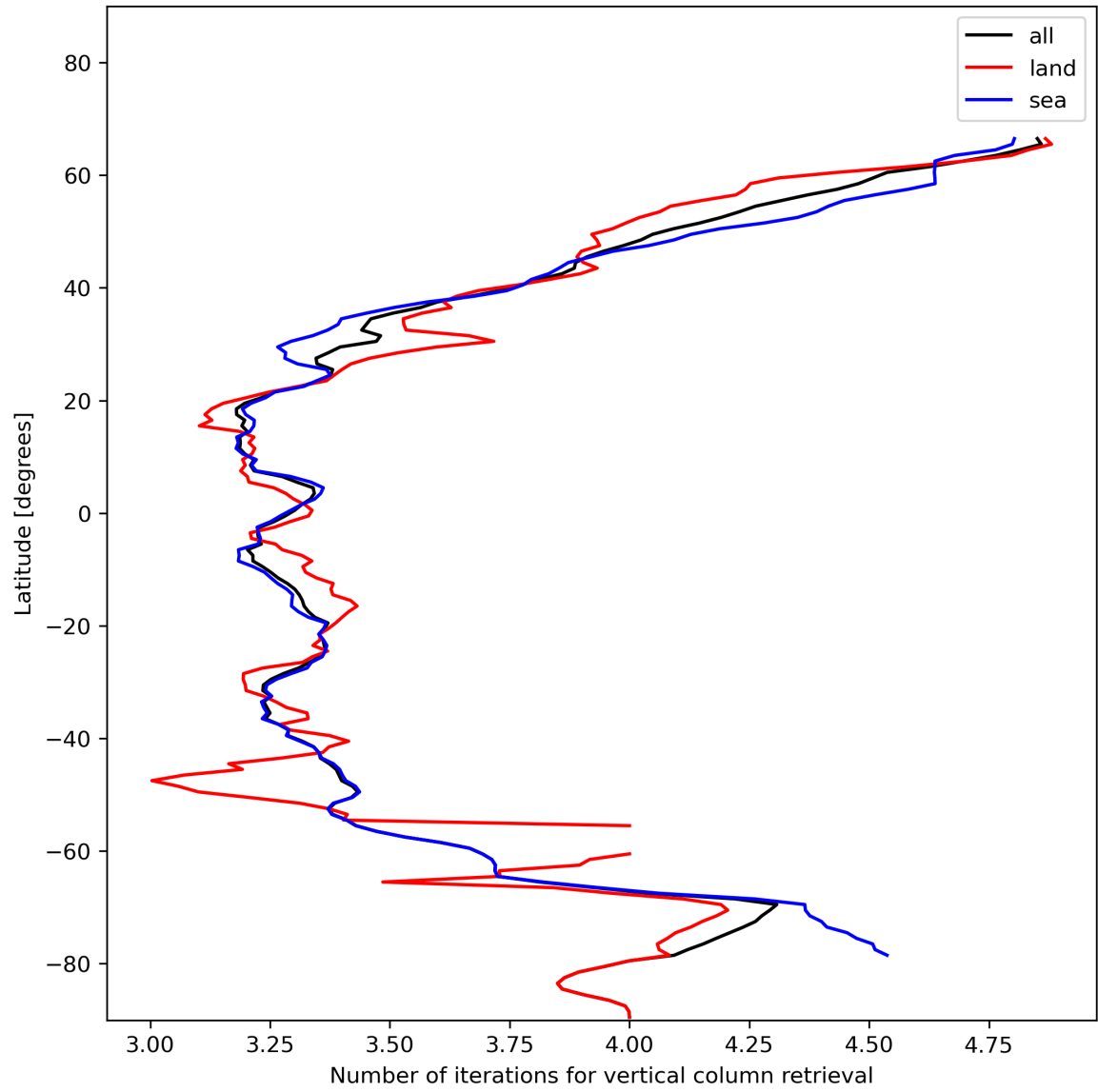
Figure 19: Zonal average of “Number of iterations for vertical column retrieval” for 2023-12-04 to 2023-12-06.
