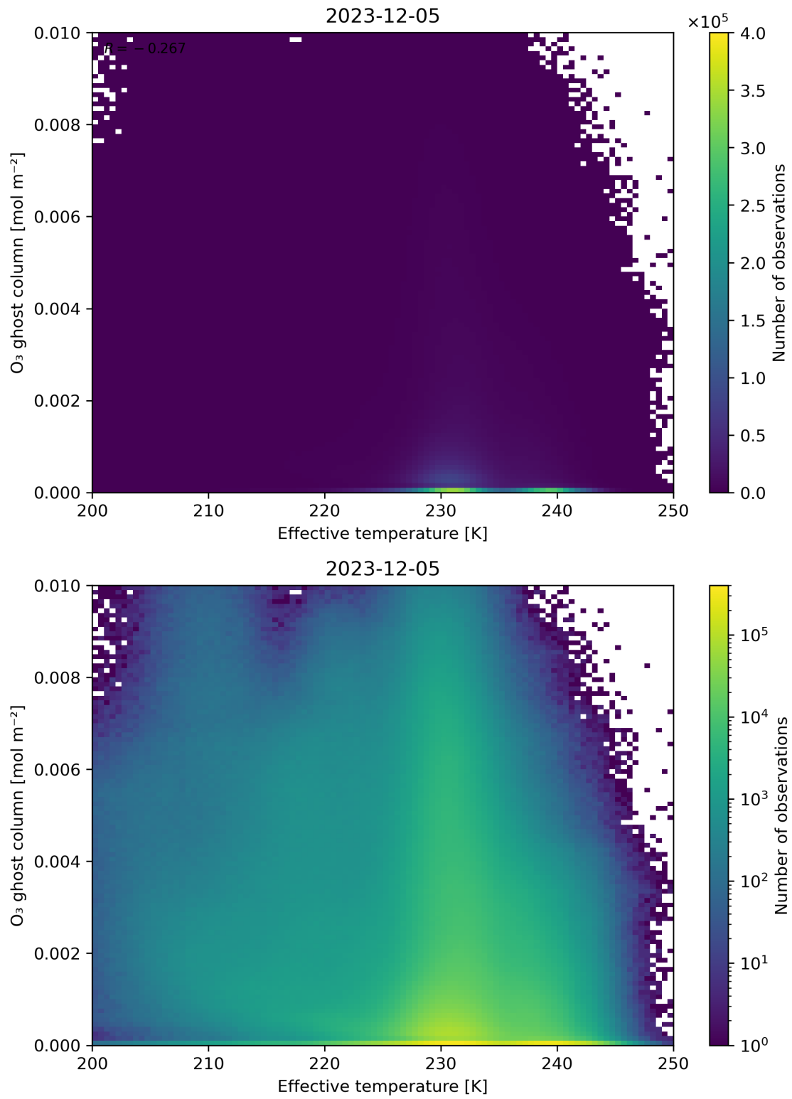
Figure 38: Scatter density plot of “Effective temperature” against “O 3 ghost column” for 2023-12-04 to 2023-12-06.
