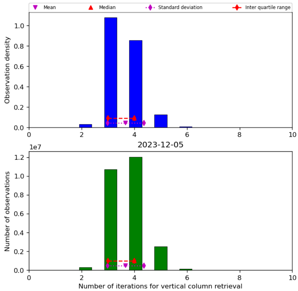
Figure 26: Histogram of “Number of iterations for vertical column retrieval” for 2023-12-04 to 2023-12-06
