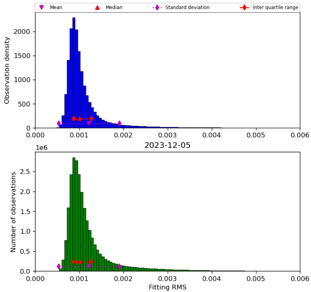
Figure 23: Histogram of “Fitting RMS” for 2023-12-04 to 2023-12-06
