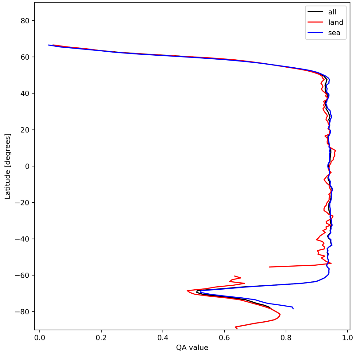
Figure 13: Zonal average of “QA value” for 2023-12-04 to 2023-12-06.
