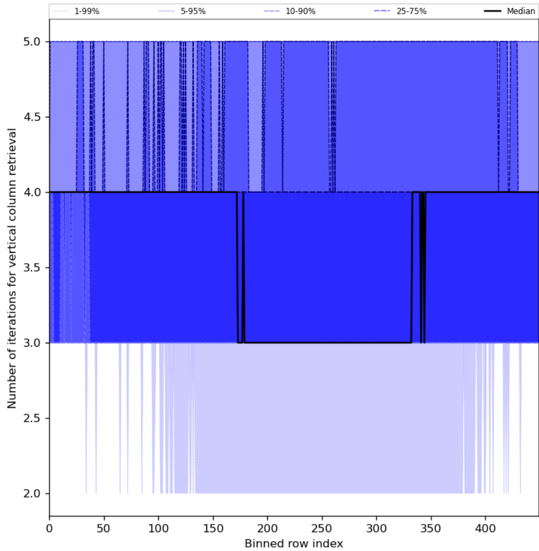
Figure 33: Along track statistics of “Number of iterations for vertical column retrieval” for 2023-12-04 to 2023-12-06
