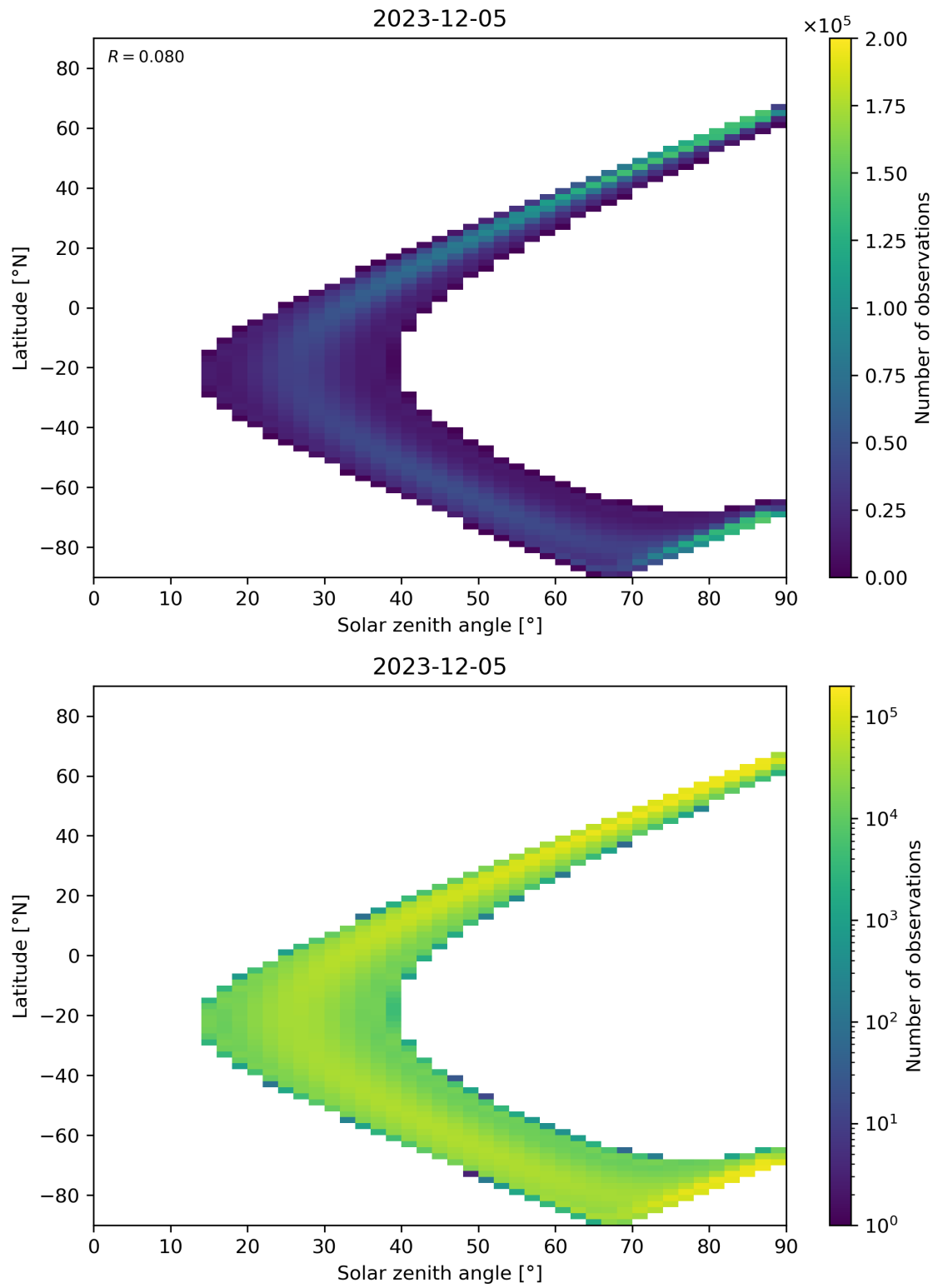
Figure 44: Scatter density plot of “Solar zenith angle” against “Latitude” for 2023-12-04 to 2023-12-06.
