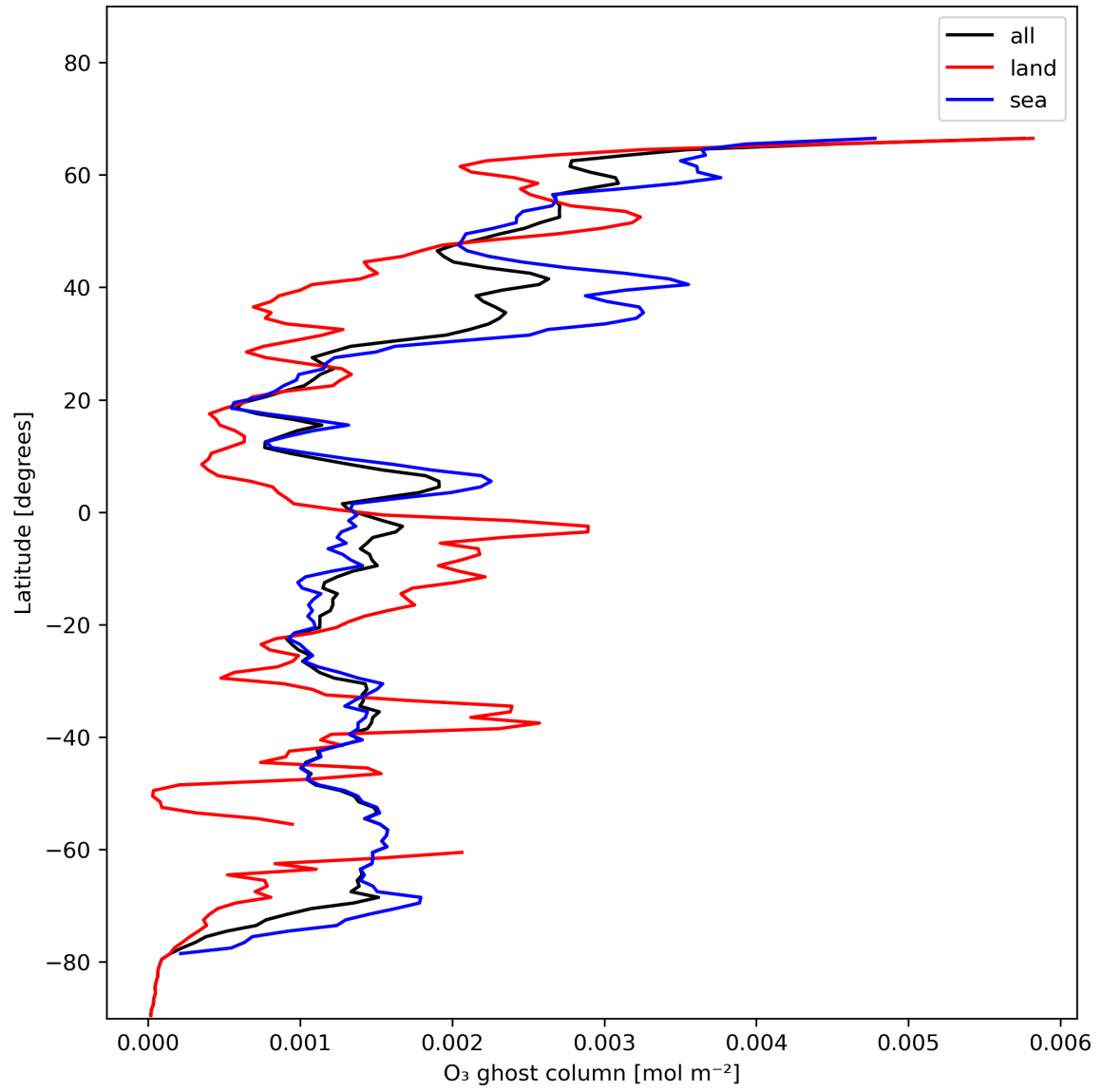
Figure 18: Zonal average of "O 3 ghost column" for 2023-12-04 to 2023-12-06.
