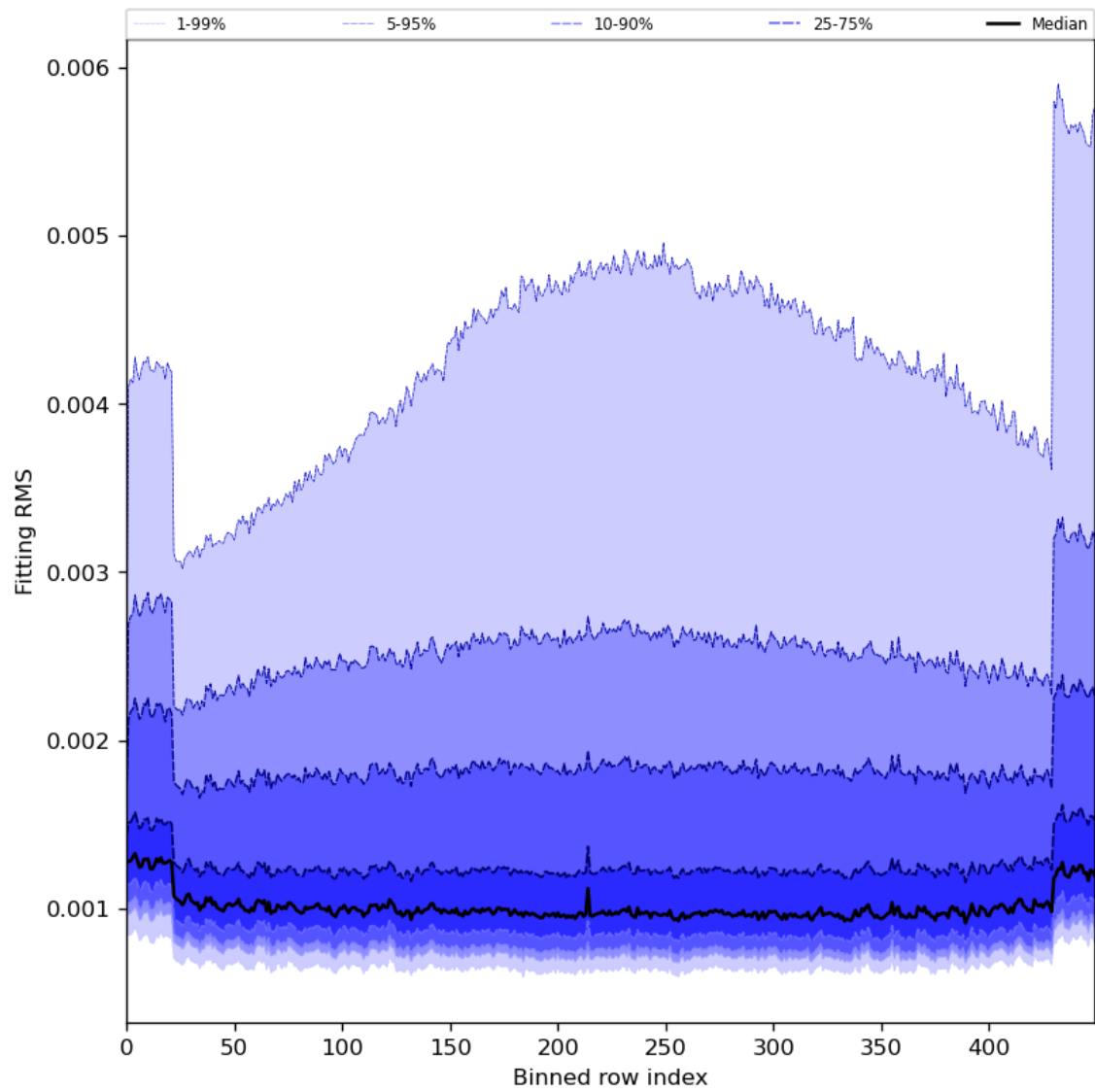
Figure 30: Along track statistics of “Fitting RMS” for 2023-12-04 to 2023-12-06
