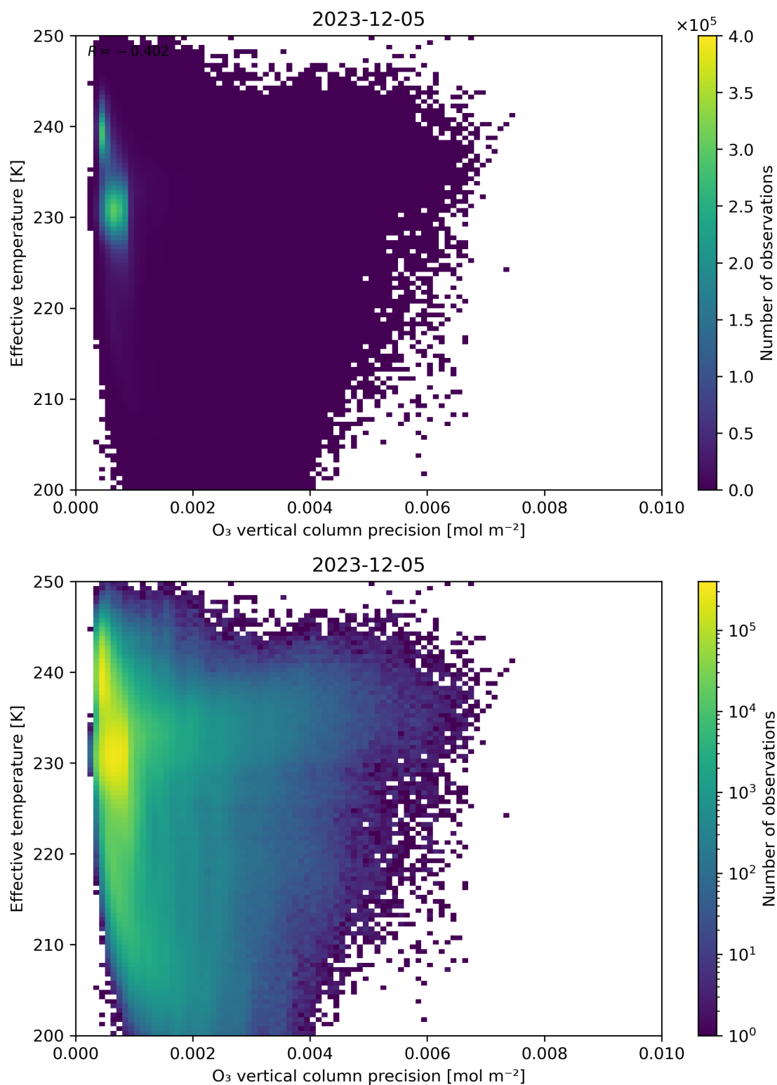
Figure 42: Scatter density plot of “O 3 vertical column precision” against “Effective temperature” for 2023-12-04 to 2023-12-06.
