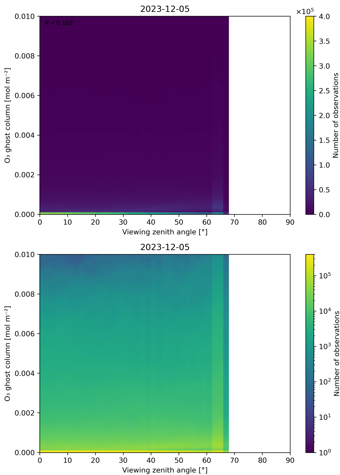
Figure 51: Scatter density plot of “Viewing zenith angle” against “O 3 ghost column” for 2023-12-04 to 2023-12-06.
