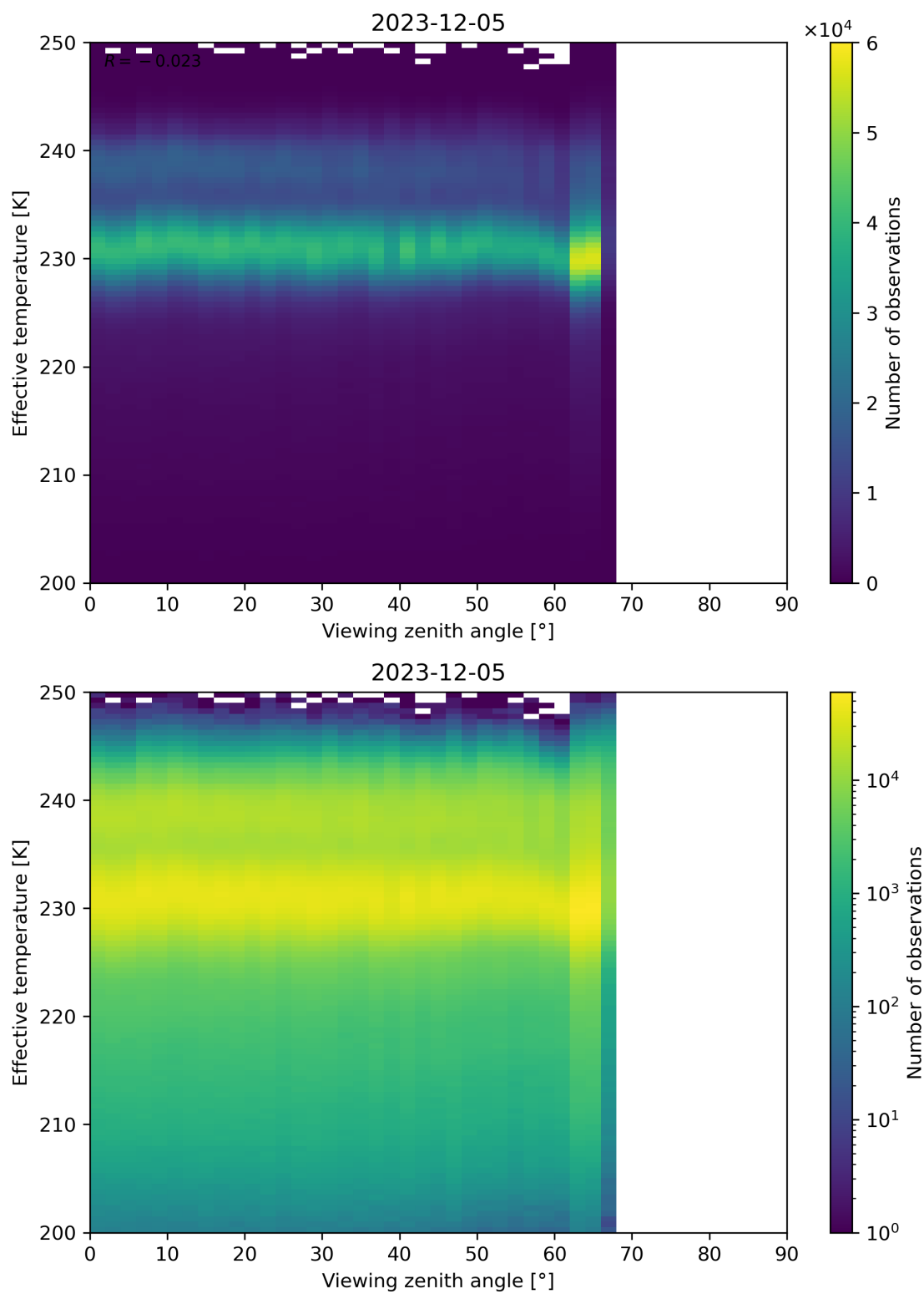
Figure 50: Scatter density plot of “Viewing zenith angle” against “Effective temperature” for 2023-12-04 to 2023-12-06.
