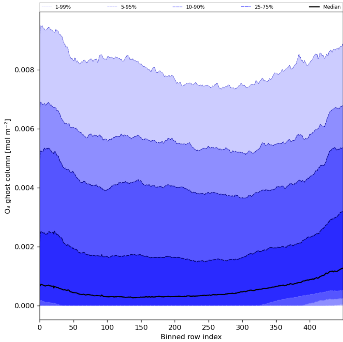
Figure 32: Along track statistics of “O 3 ghost column” for 2023-12-04 to 2023-12-06
