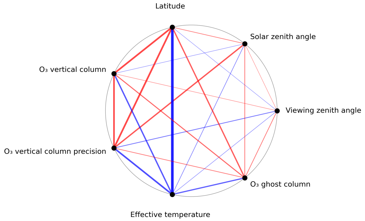
Figure 1: Map of correlation graph for 2023-12-04 to 2023-12-06.
