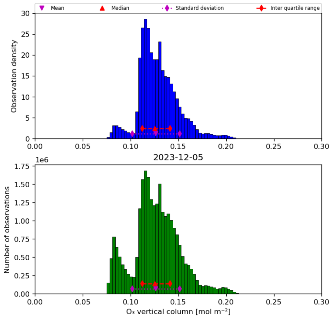
Figure 21: Histogram of “O 3 vertical column” for 2023-12-04 to 2023-12-06
