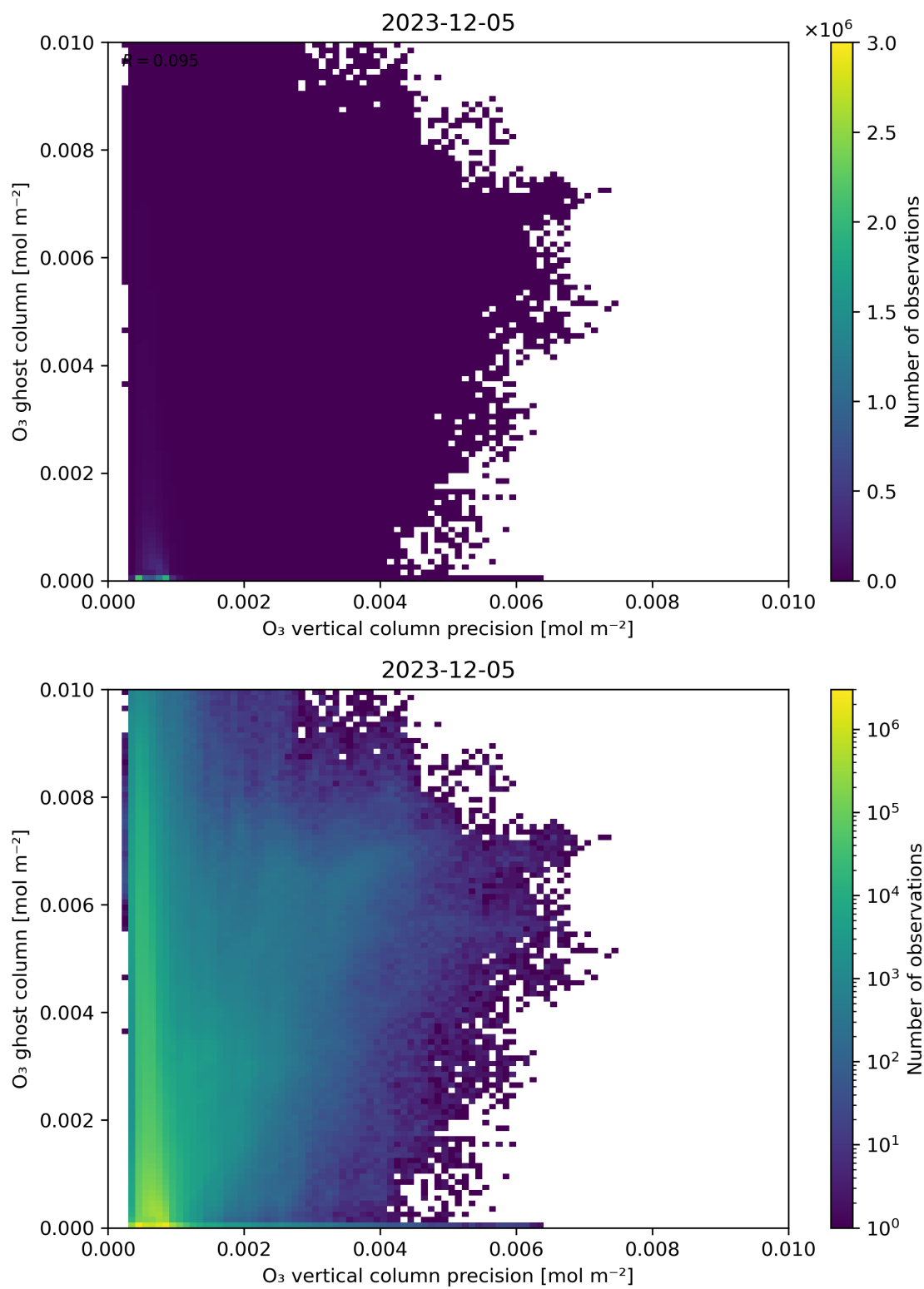
Figure 43: Scatter density plot of “O 3 vertical column precision” against “O 3 ghost column” for 2023-12-04 to 2023-12-06.
