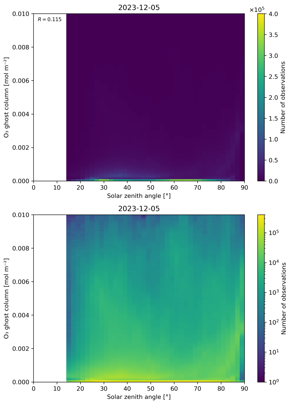
Figure 46: Scatter density plot of “Solar zenith angle” against “O 3 ghost column” for 2023-12-04 to 2023-12-06.
