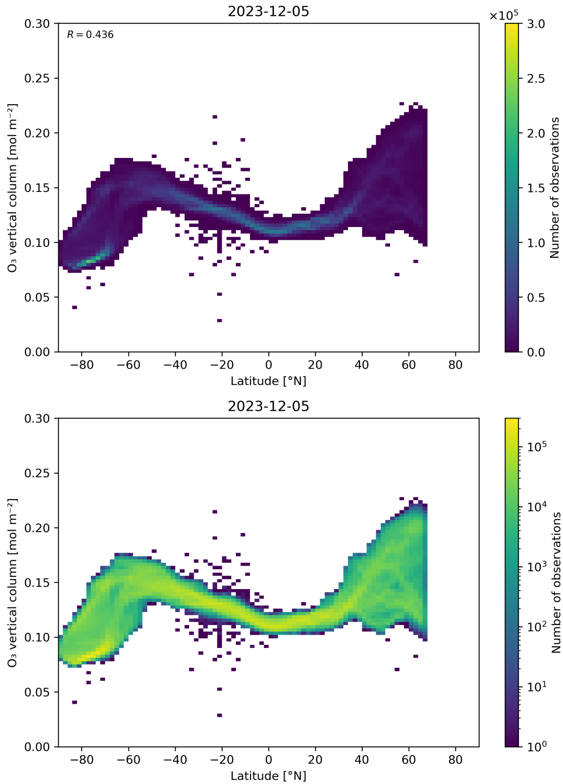
Figure 36: Scatter density plot of “Latitude” against “O 3 vertical column” for 2023-12-04 to 2023-12-06.
