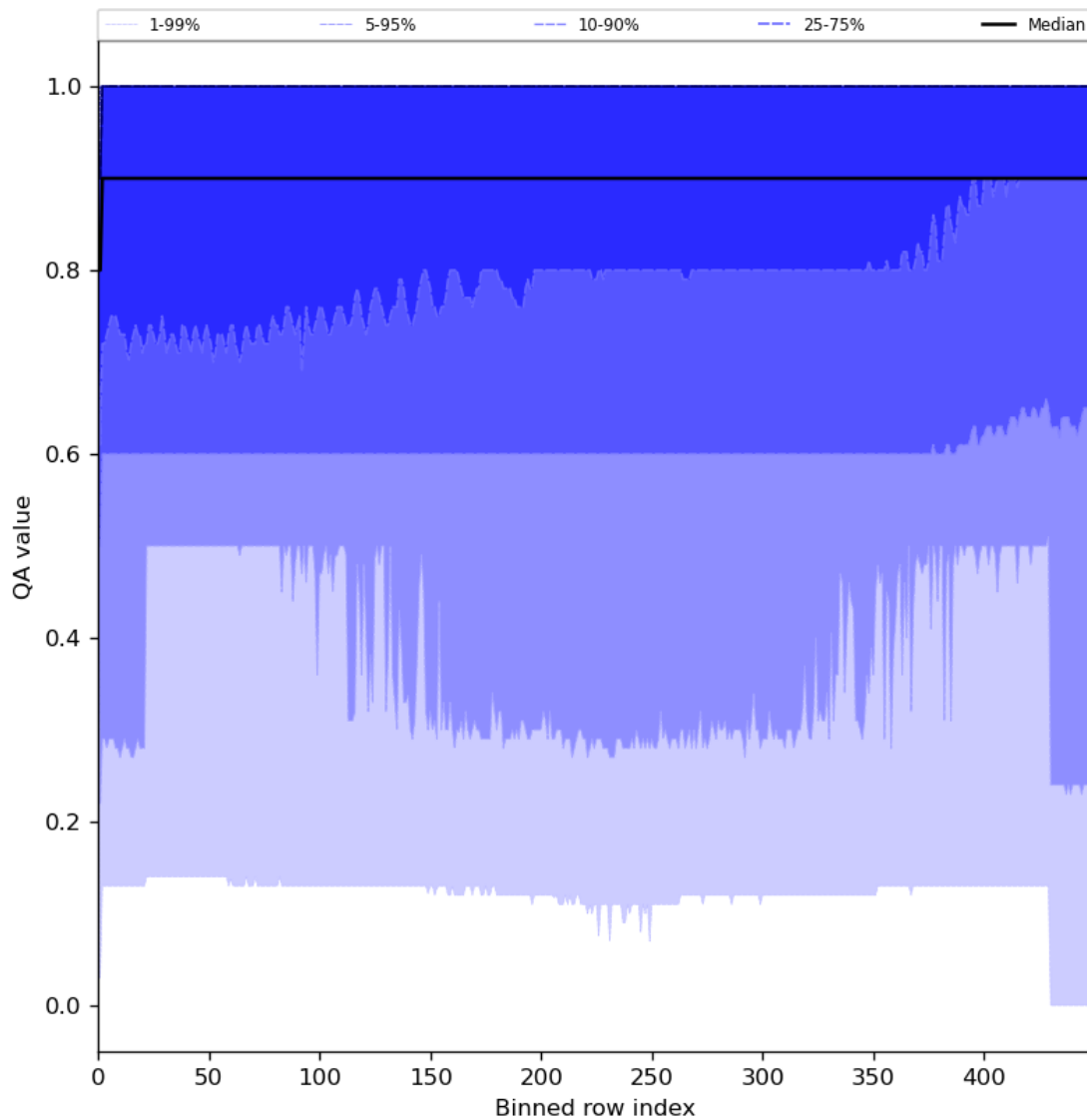
Figure 27: Along track statistics of “QA value” for 2023-12-04 to 2023-12-06
