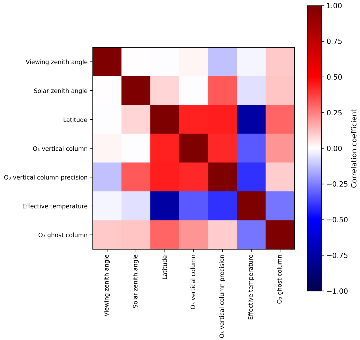
Figure 2: Map of correlation matrix for 2023-12-04 to 2023-12-06.
