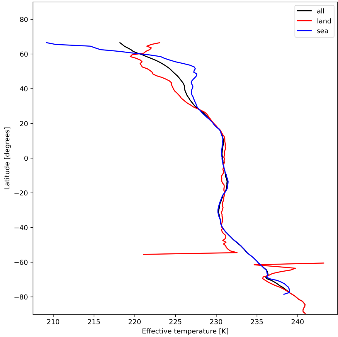
Figure 17: Zonal average of “Effective temperature” for 2023-12-04 to 2023-12-06.
