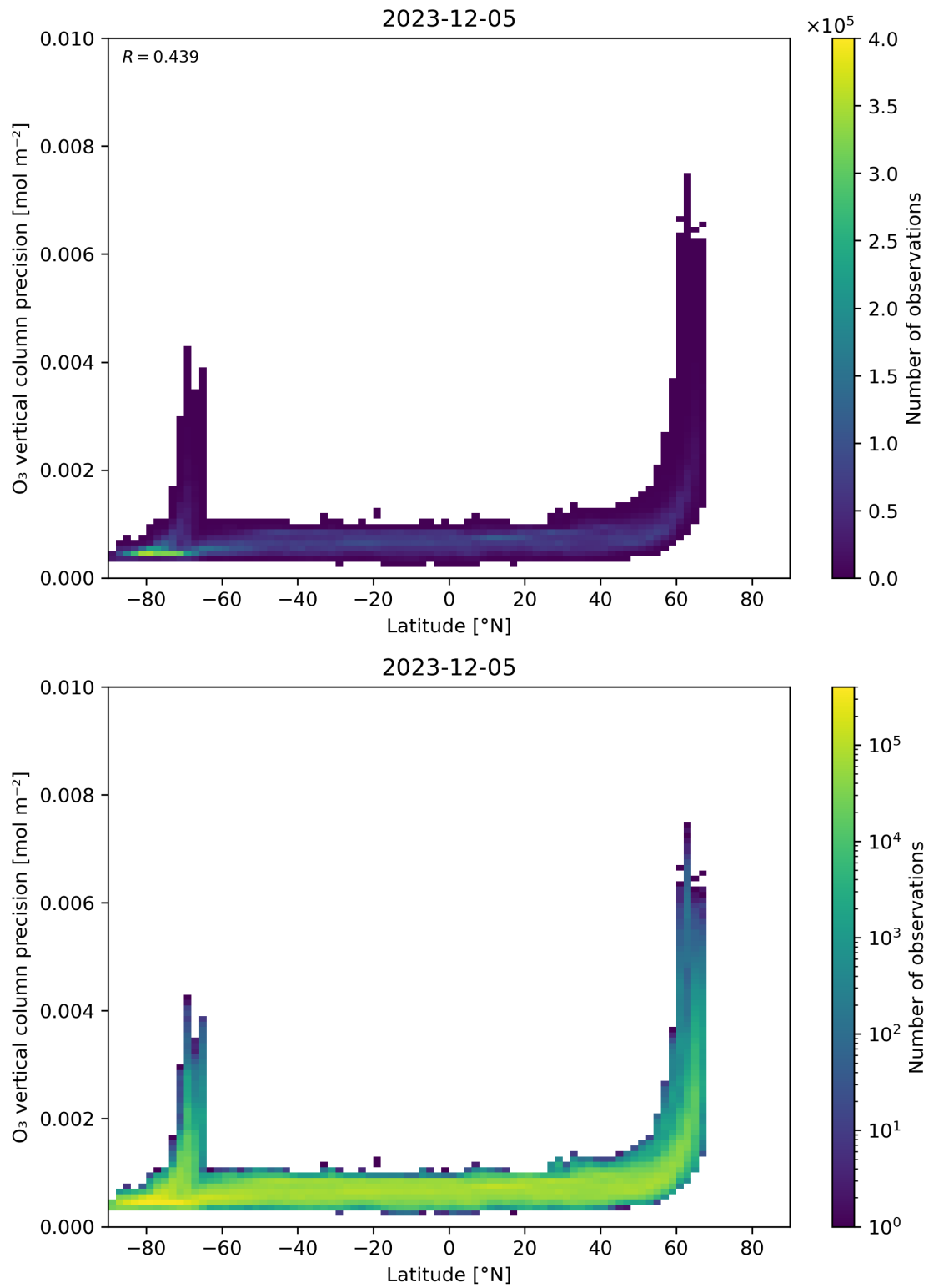
Figure 37: Scatter density plot of “Latitude” against “O 3 vertical column precision” for 2023-12-04 to 2023-12-06.
