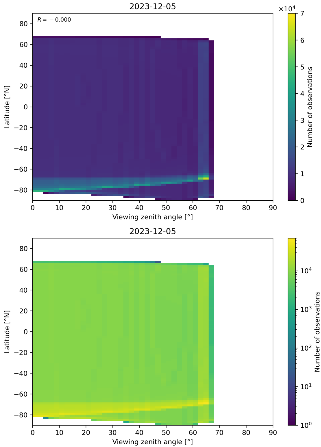
Figure 49: Scatter density plot of “Viewing zenith angle” against “Latitude” for 2023-12-04 to 2023-12-06.
