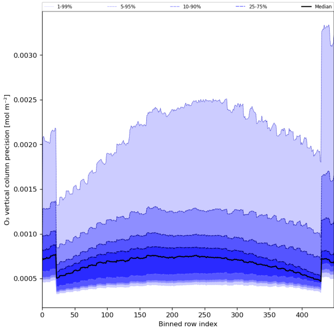
Figure 29: Along track statistics of “O 3 vertical column precision” for 2023-12-04 to 2023-12-06
