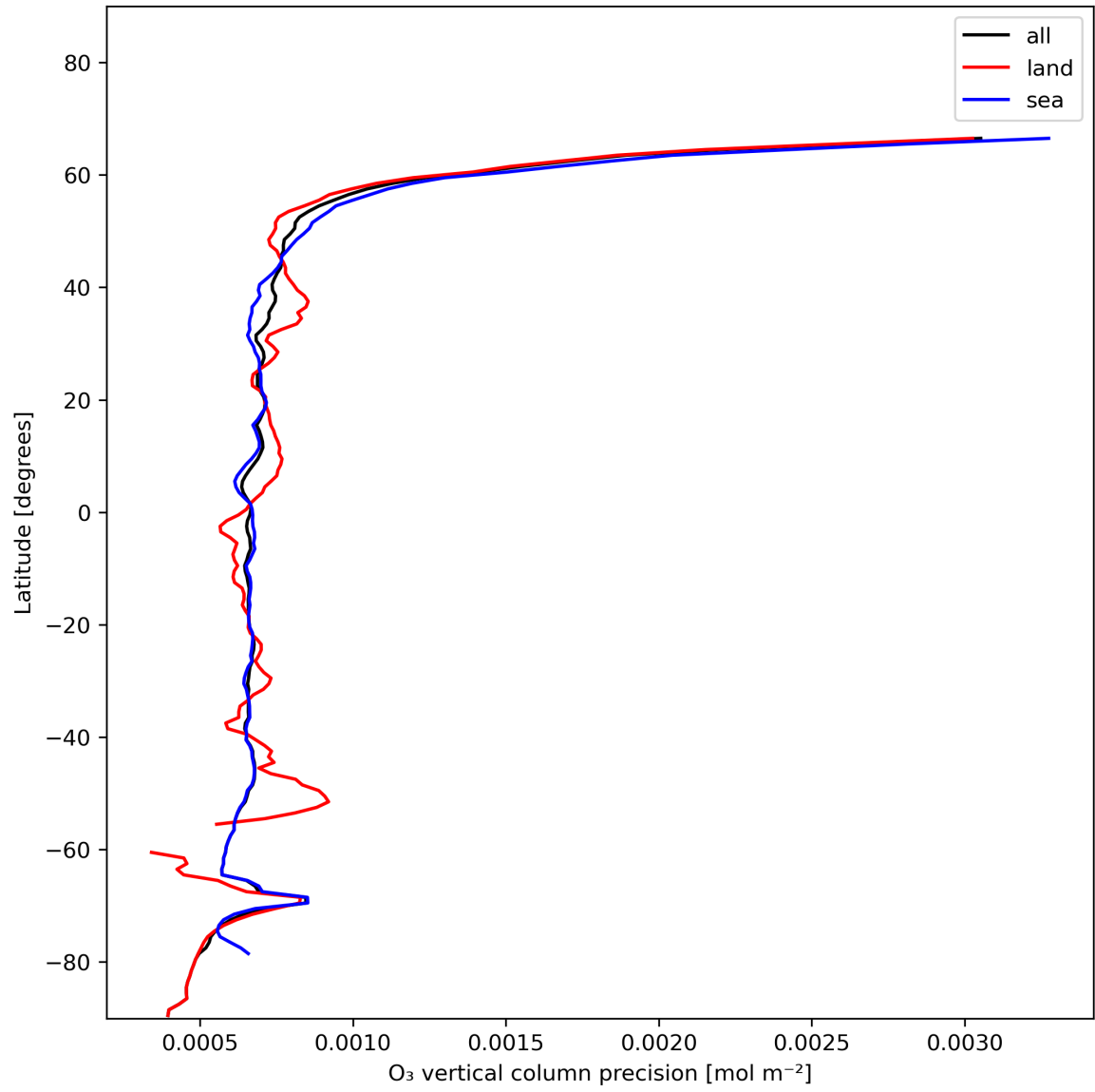
Figure 15: Zonal average of “O 3 vertical column precision” for 2023-12-04 to 2023-12-06.
