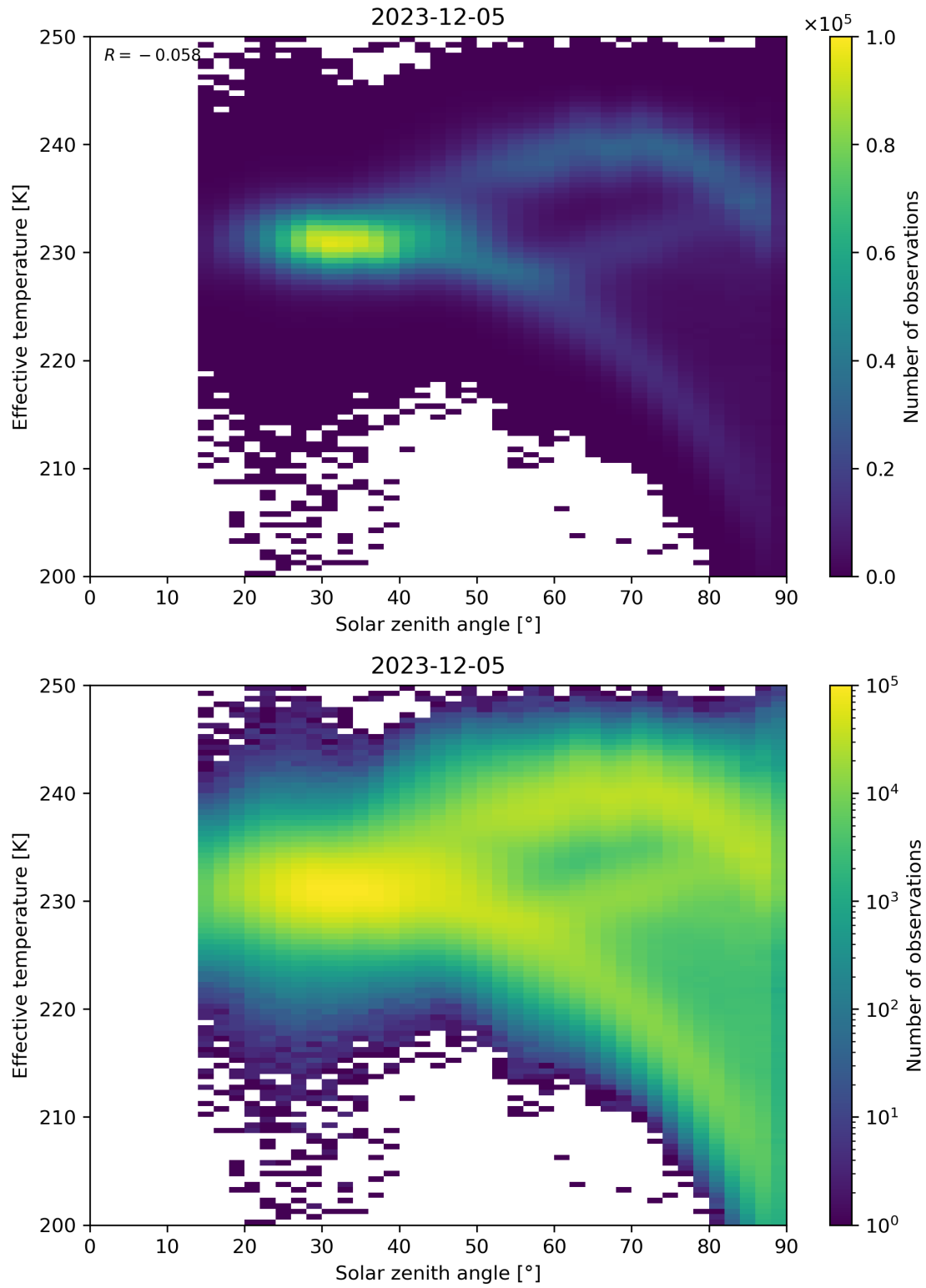
Figure 45: Scatter density plot of “Solar zenith angle” against “Effective temperature” for 2023-12-04 to 2023-12-06.
