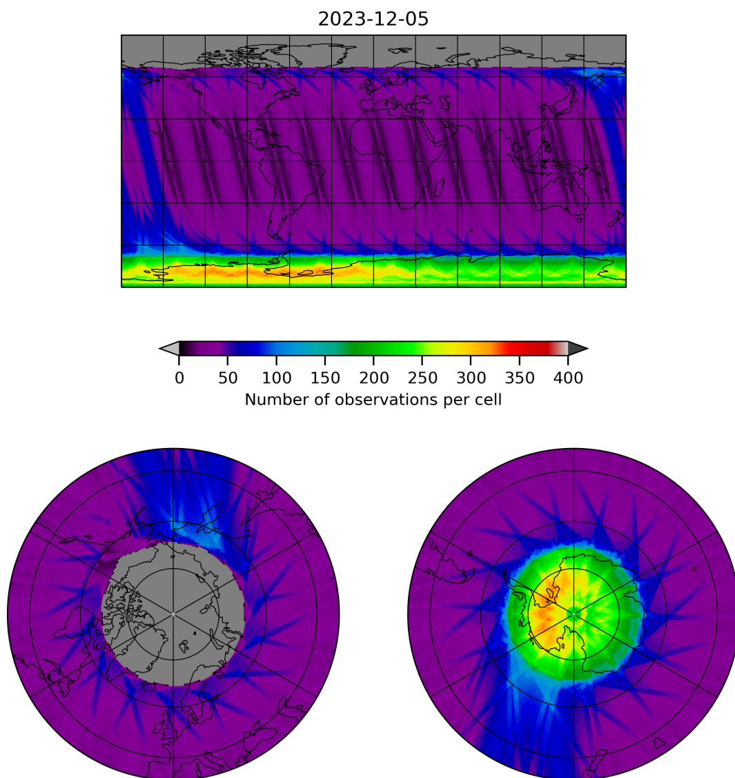
Figure 12: Map of the number of observations for 2023-12-04 to 2023-12-06
