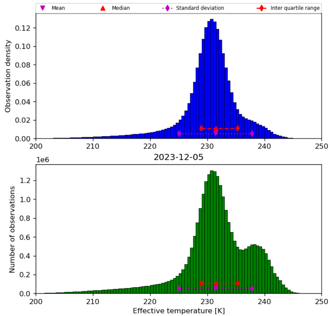
Figure 24: Histogram of “Effective temperature” for 2023-12-04 to 2023-12-06
