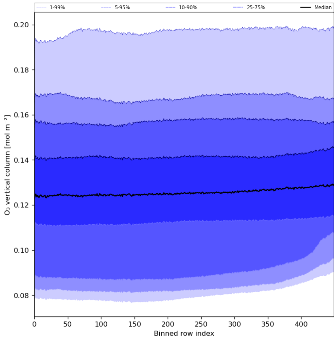
Figure 28: Along track statistics of “O 3 vertical column” for 2023-12-04 to 2023-12-06
