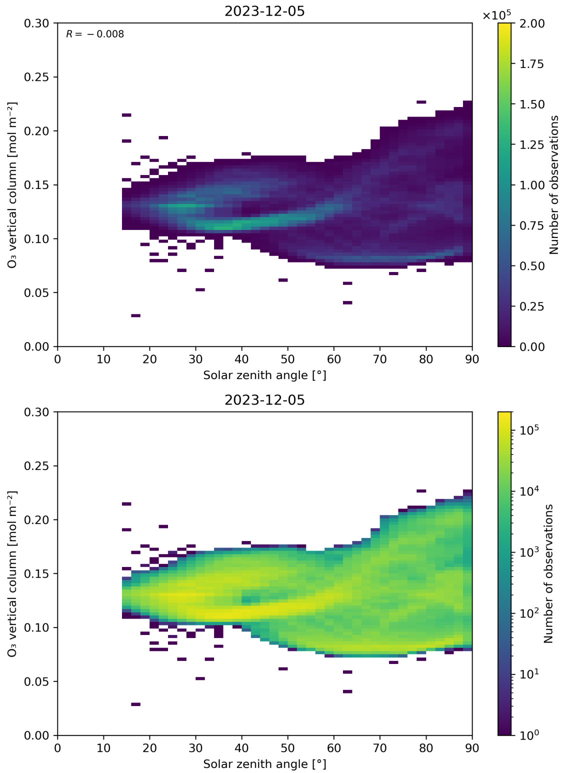
Figure 47: Scatter density plot of “Solar zenith angle” against “O 3 vertical column” for 2023-12-04 to 2023-12-06.
