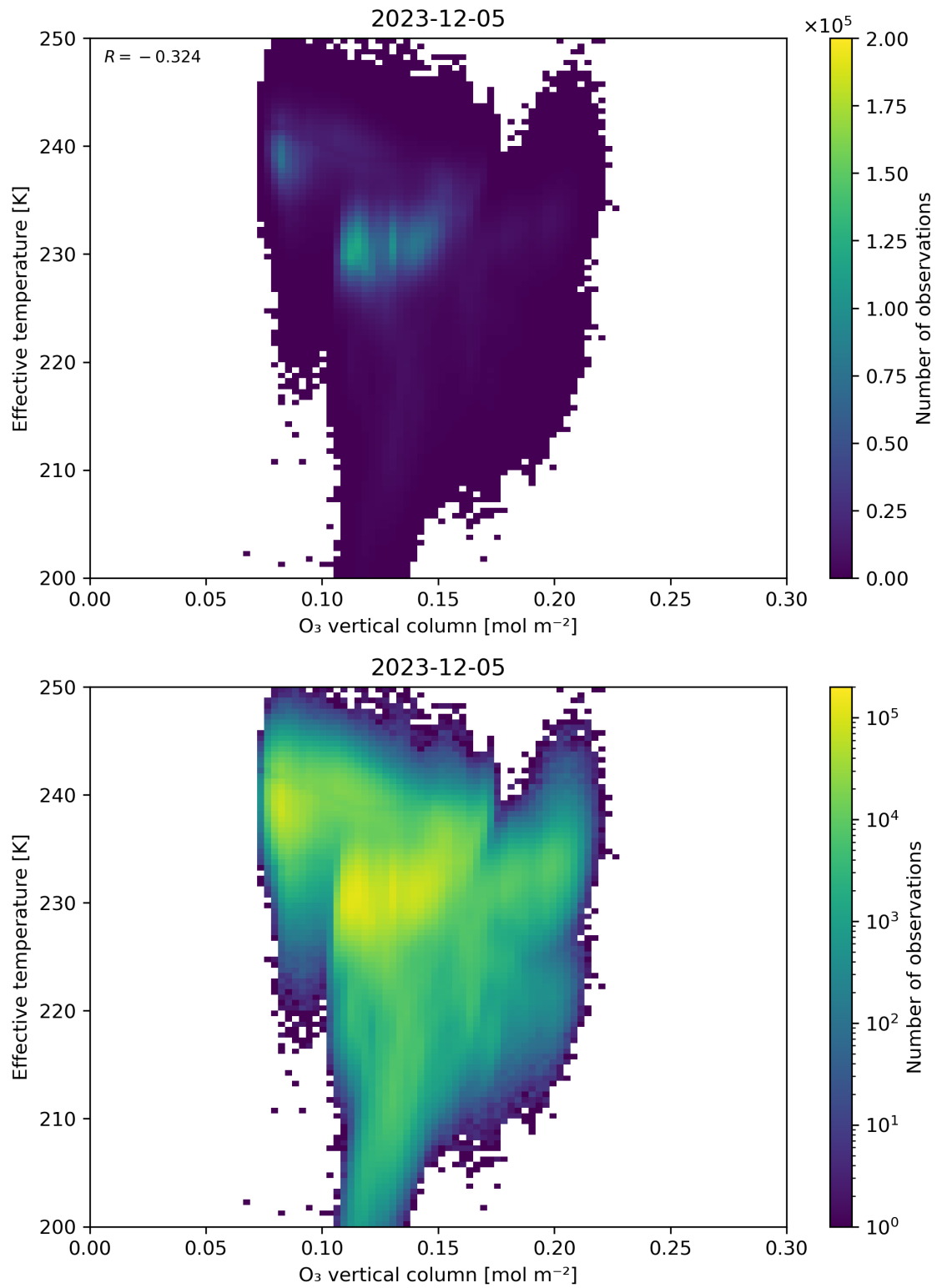
Figure 39: Scatter density plot of “O 3 vertical column” against “Effective temperature” for 2023-12-04 to 2023-12-06.
