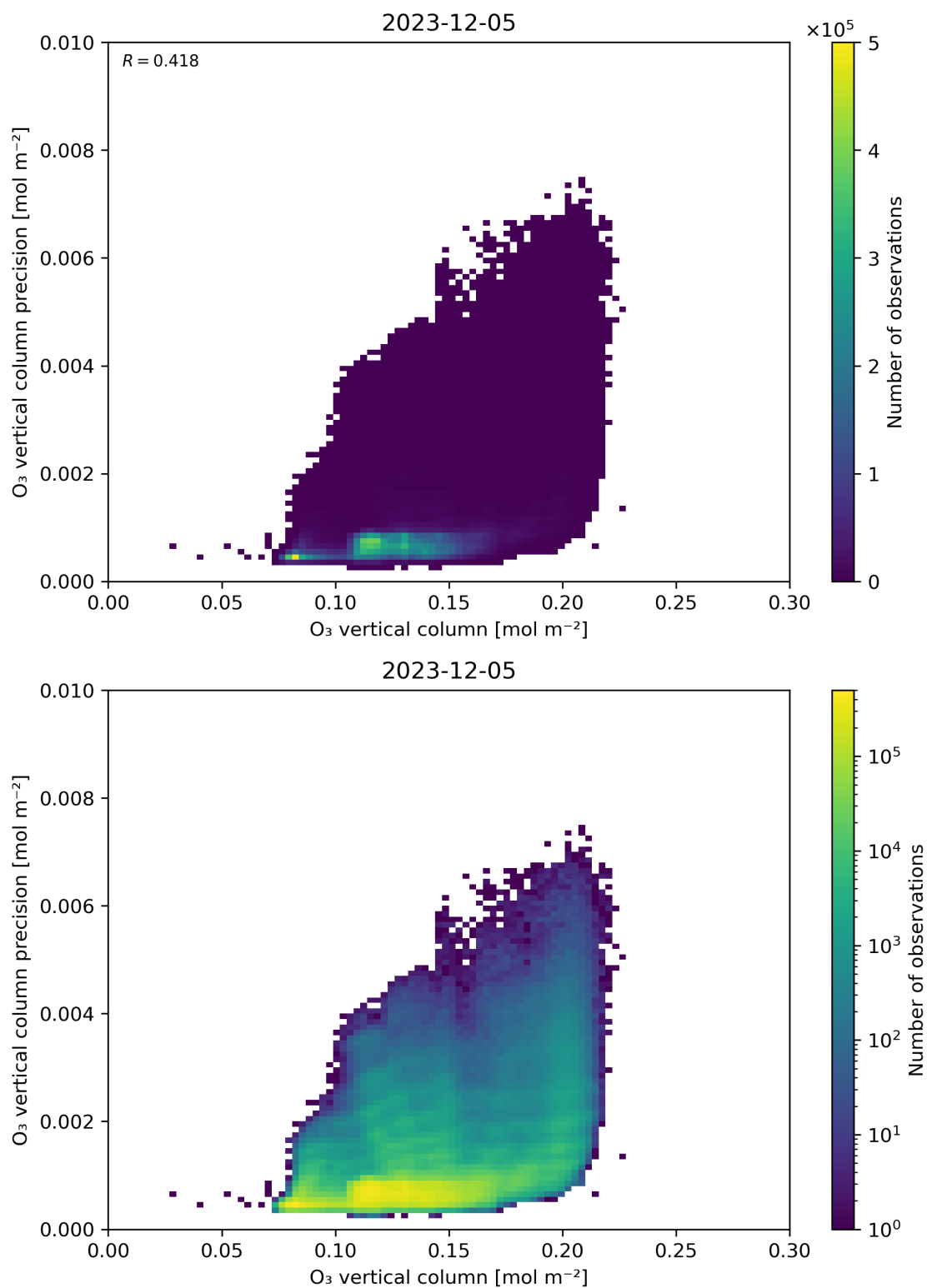
Figure 41: Scatter density plot of “O 3 vertical column” against “O 3 vertical column precision” for 2023-12-04 to 2023-12-06.
