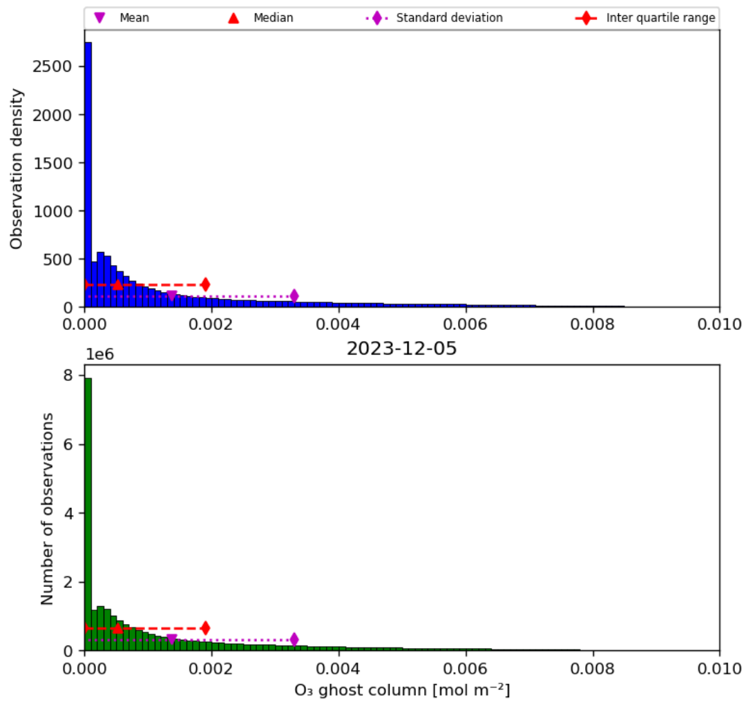
Figure 25: Histogram of “O 3 ghost column” for 2023-12-04 to 2023-12-06
