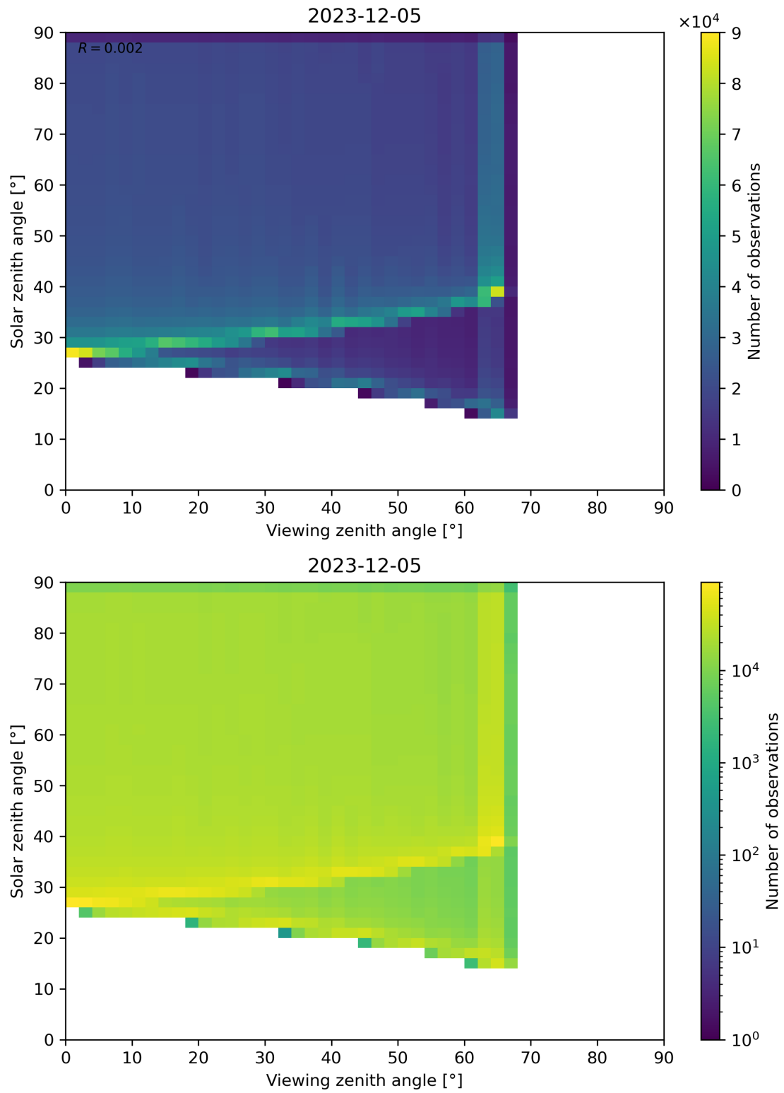
Figure 54: Scatter density plot of “Viewing zenith angle” against “Solar zenith angle” for 2023-12-04 to 2023-12-06.
