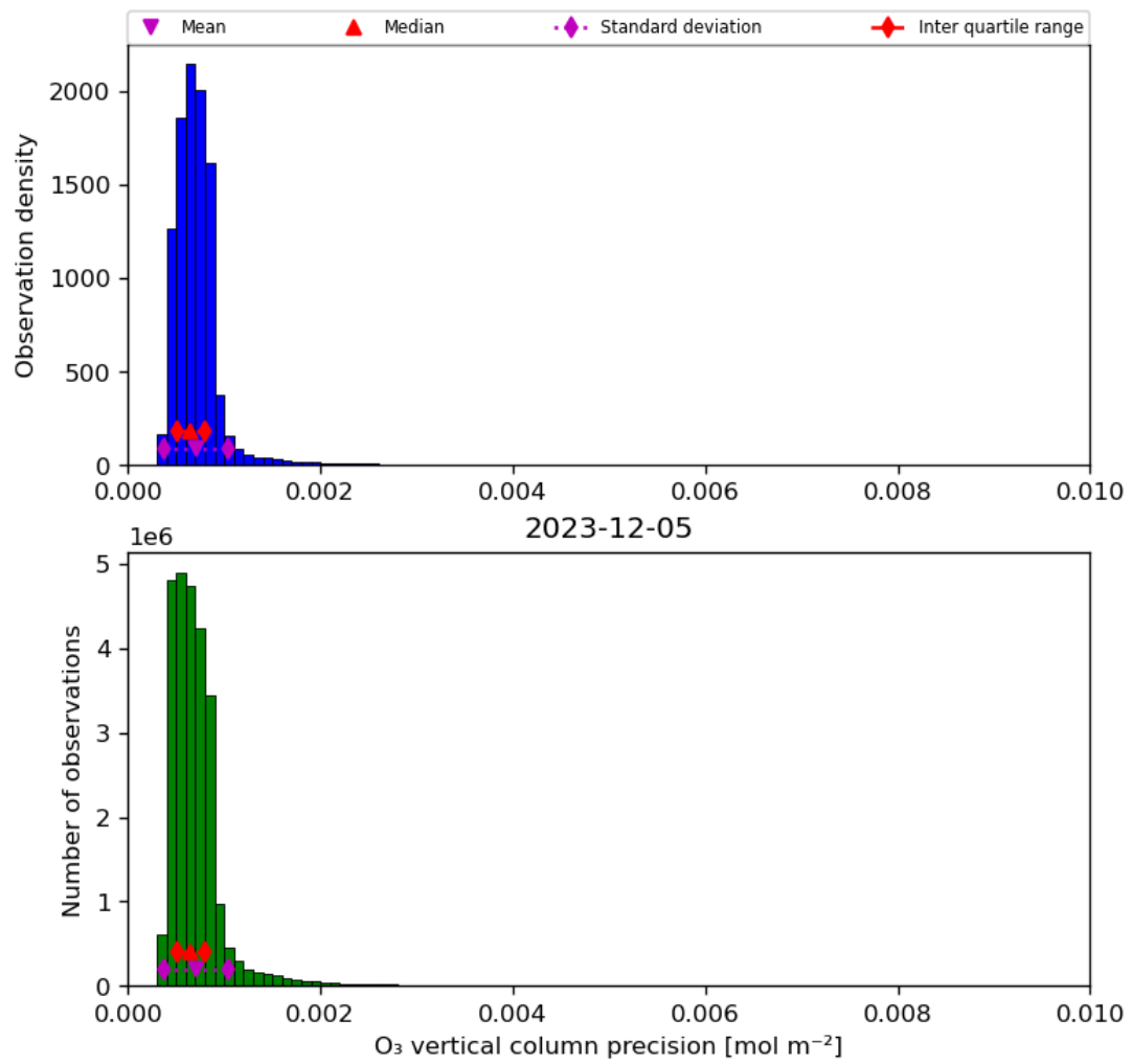
Figure 22: Histogram of “O 3 vertical column precision” for 2023-12-04 to 2023-12-06
