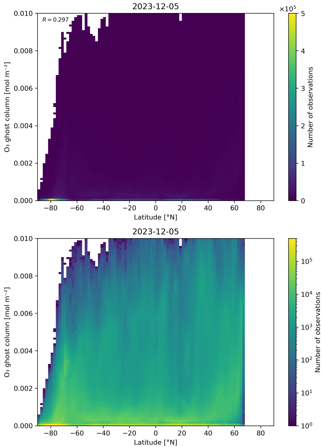
Figure 35: Scatter density plot of “Latitude” against “O 3 ghost column” for 2023-12-04 to 2023-12-06.
