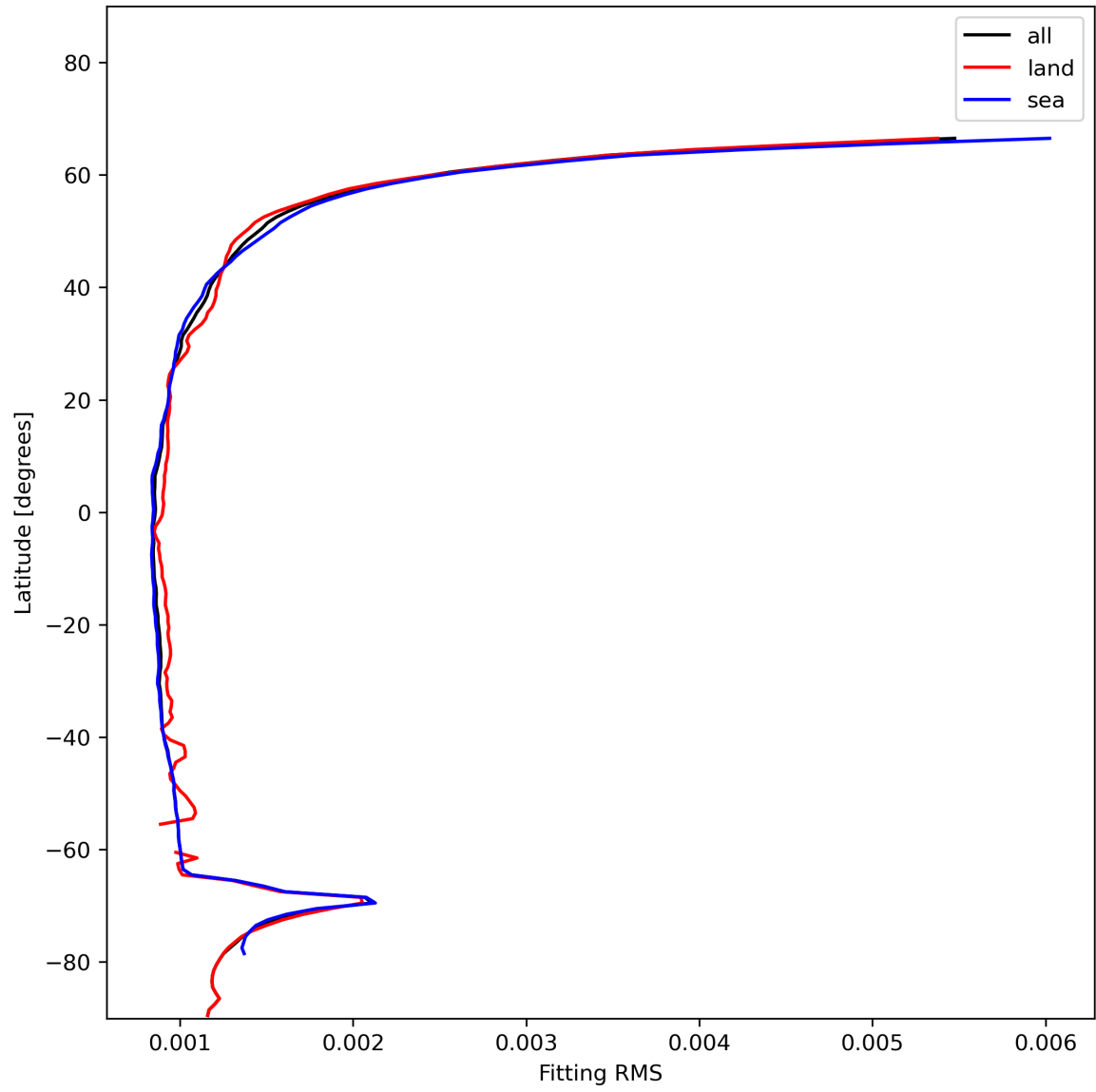
Figure 16: Zonal average of “Fitting RMS” for 2023-12-04 to 2023-12-06.
