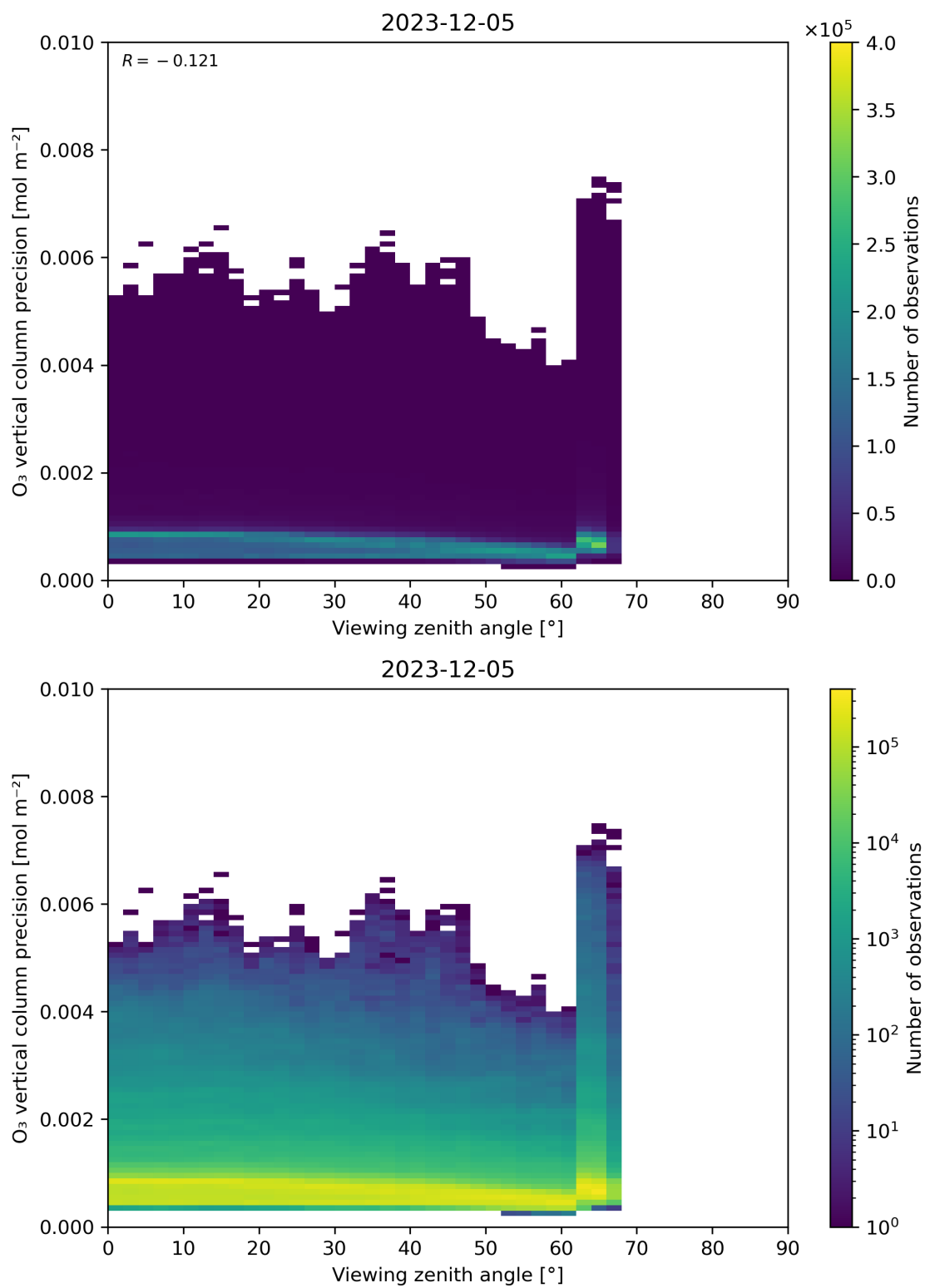
Figure 53: Scatter density plot of “Viewing zenith angle” against “O 3 vertical column precision” for 2023-12-04 to 2023-12-06.
