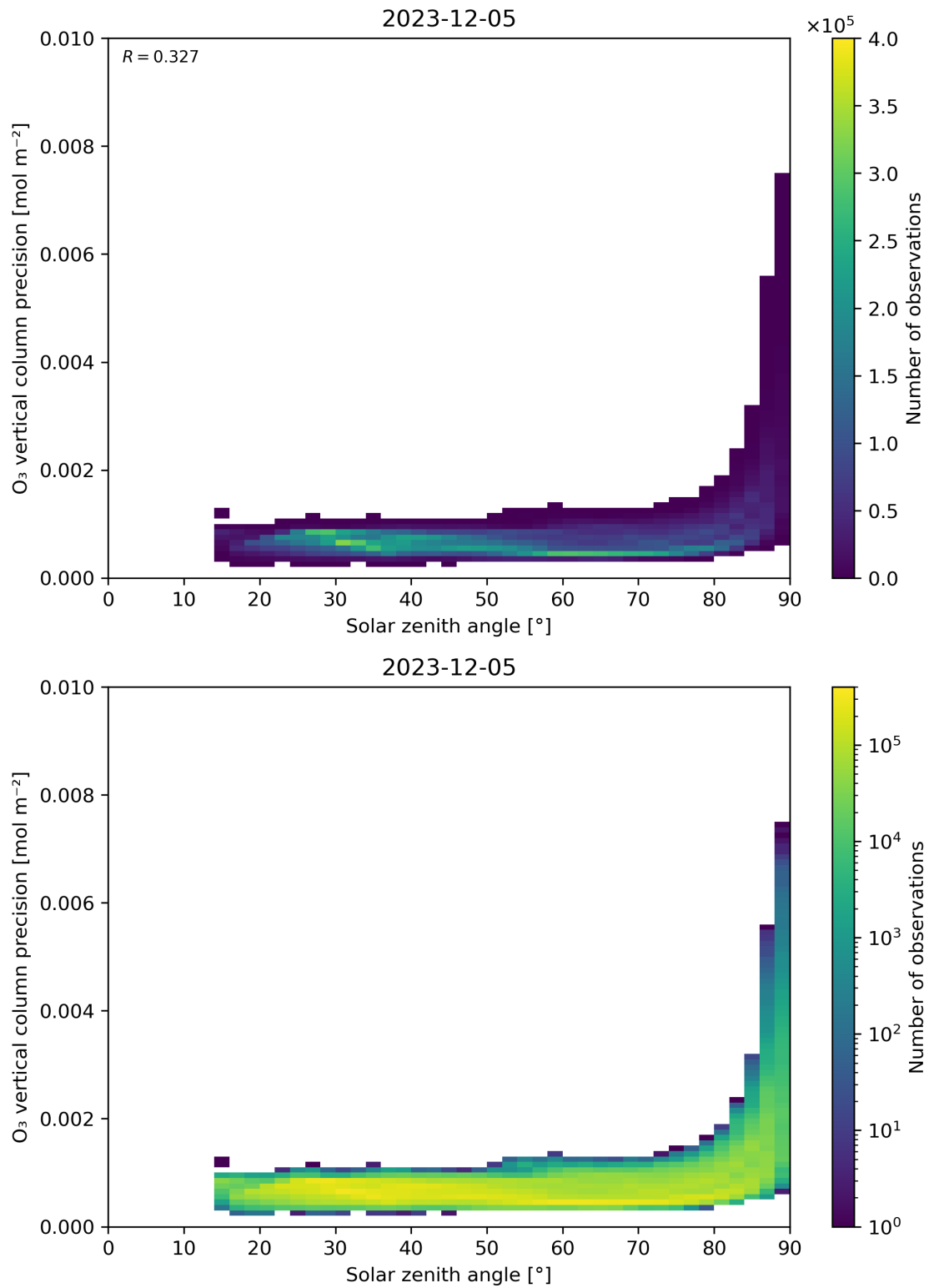
Figure 48: Scatter density plot of “Solar zenith angle” against “O 3 vertical column precision” for 2023-12-04 to 2023-12-06.
