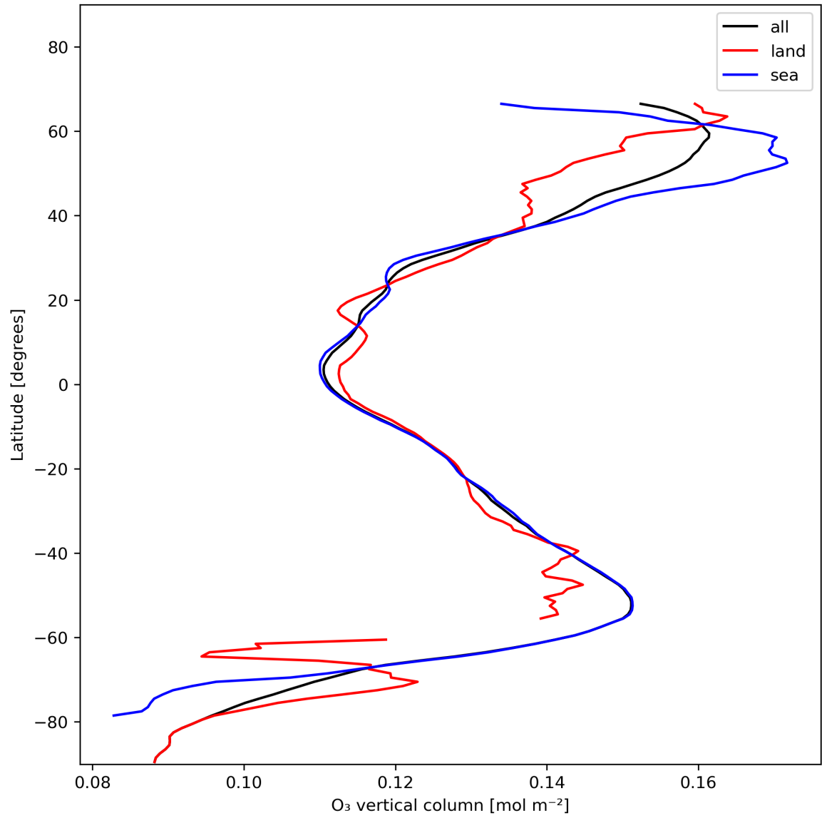
Figure 14: Zonal average of “O 3 vertical column” for 2023-12-04 to 2023-12-06.
