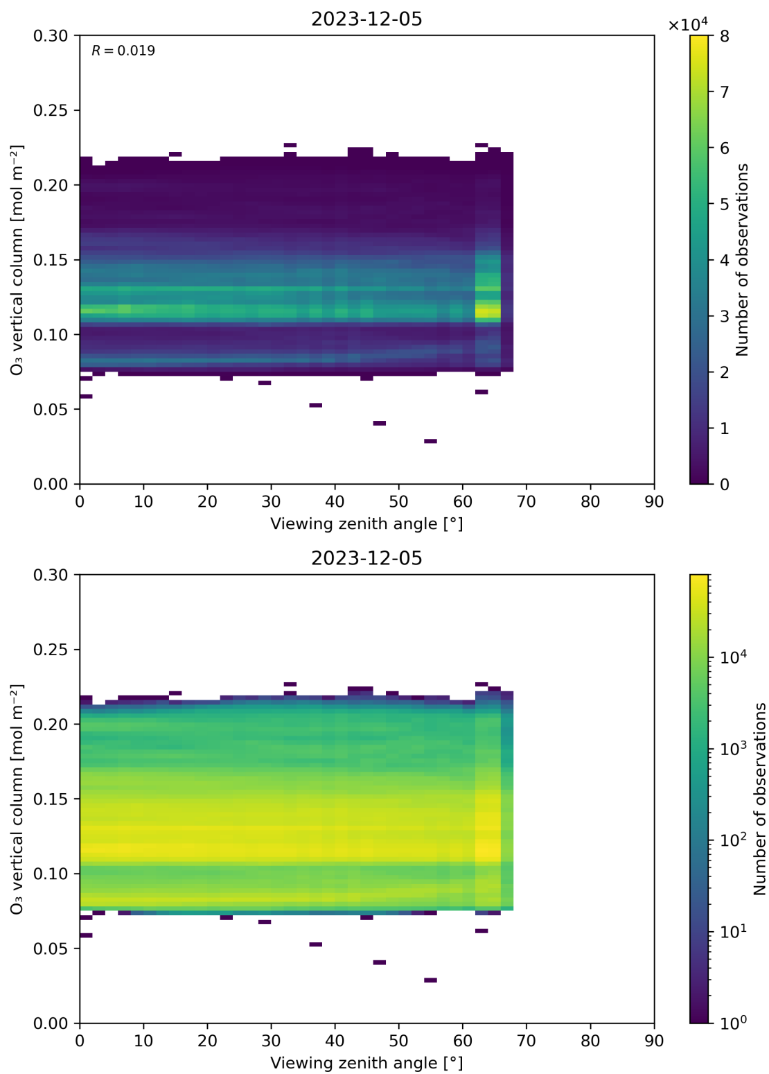
Figure 52: Scatter density plot of “Viewing zenith angle” against “O 3 vertical column” for 2023-12-04 to 2023-12-06.
