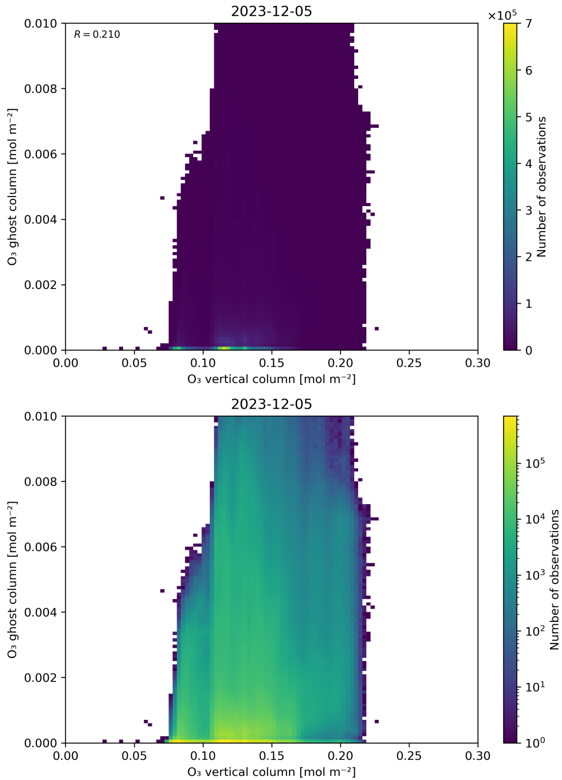
Figure 40: Scatter density plot of “O 3 vertical column” against “O 3 ghost column” for 2023-12-04 to 2023-12-06.
