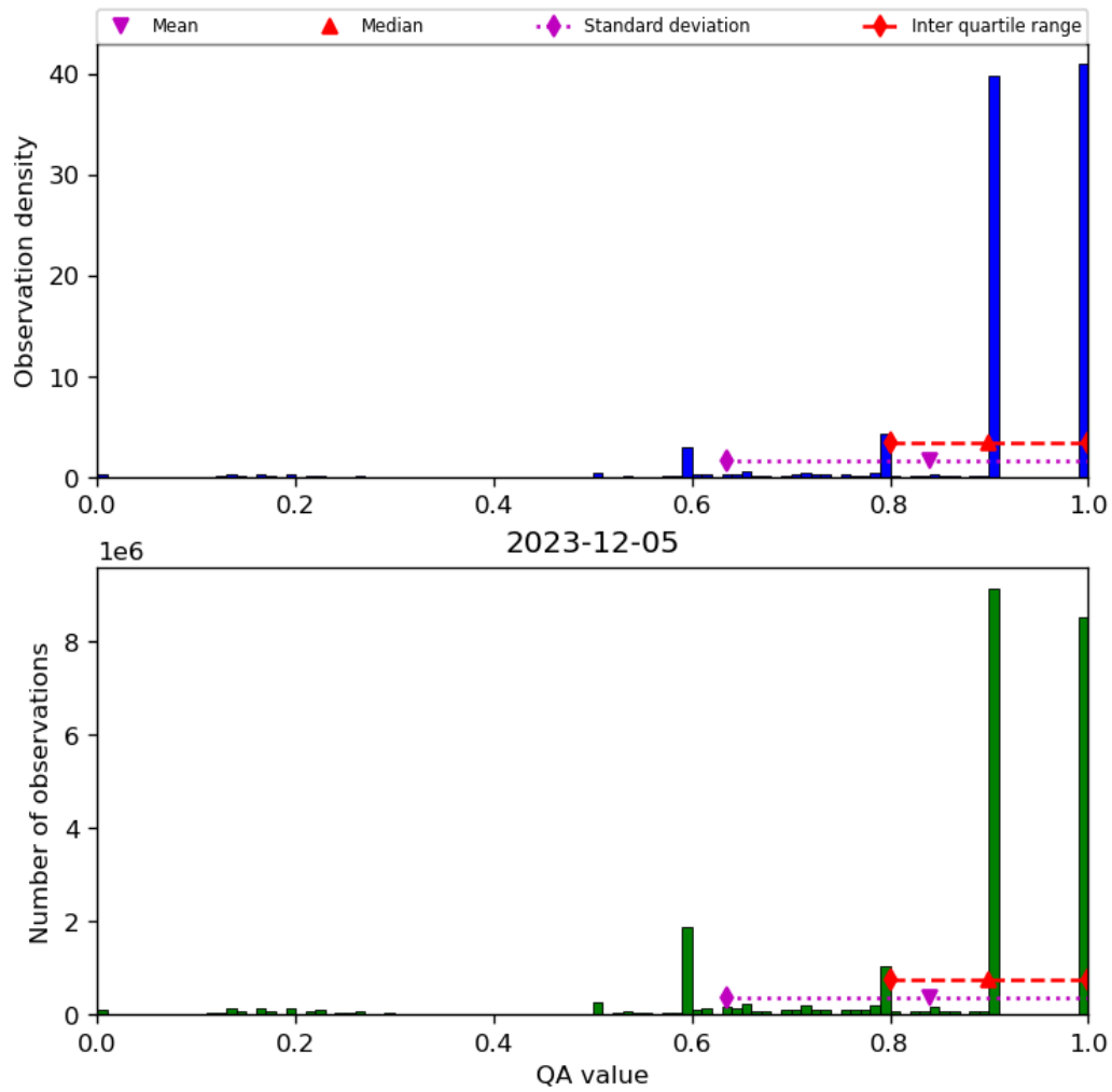
Figure 20: Histogram of “QA value” for 2023-12-04 to 2023-12-06
