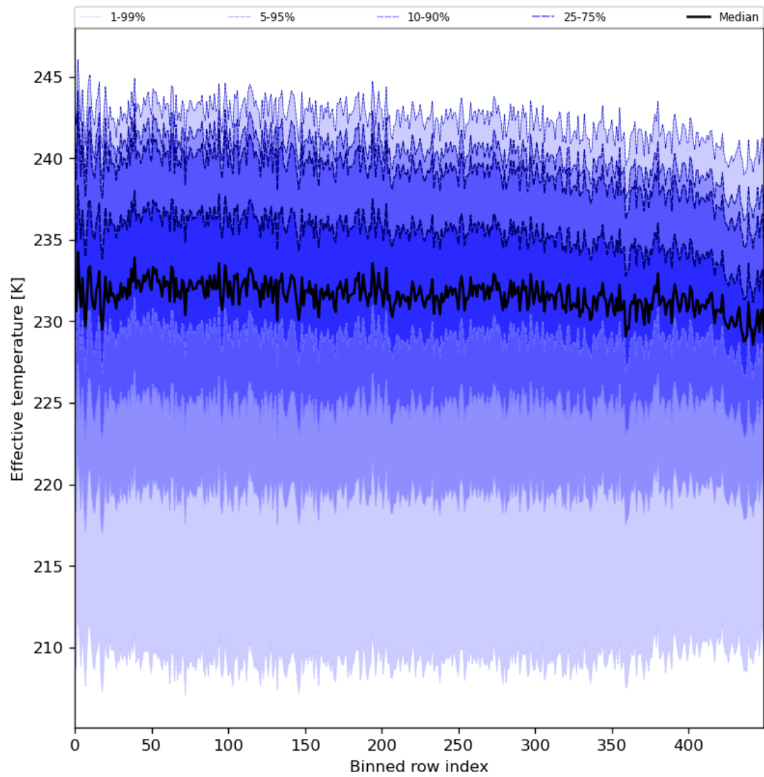
Figure 31: Along track statistics of “Effective temperature” for 2023-12-04 to 2023-12-06
