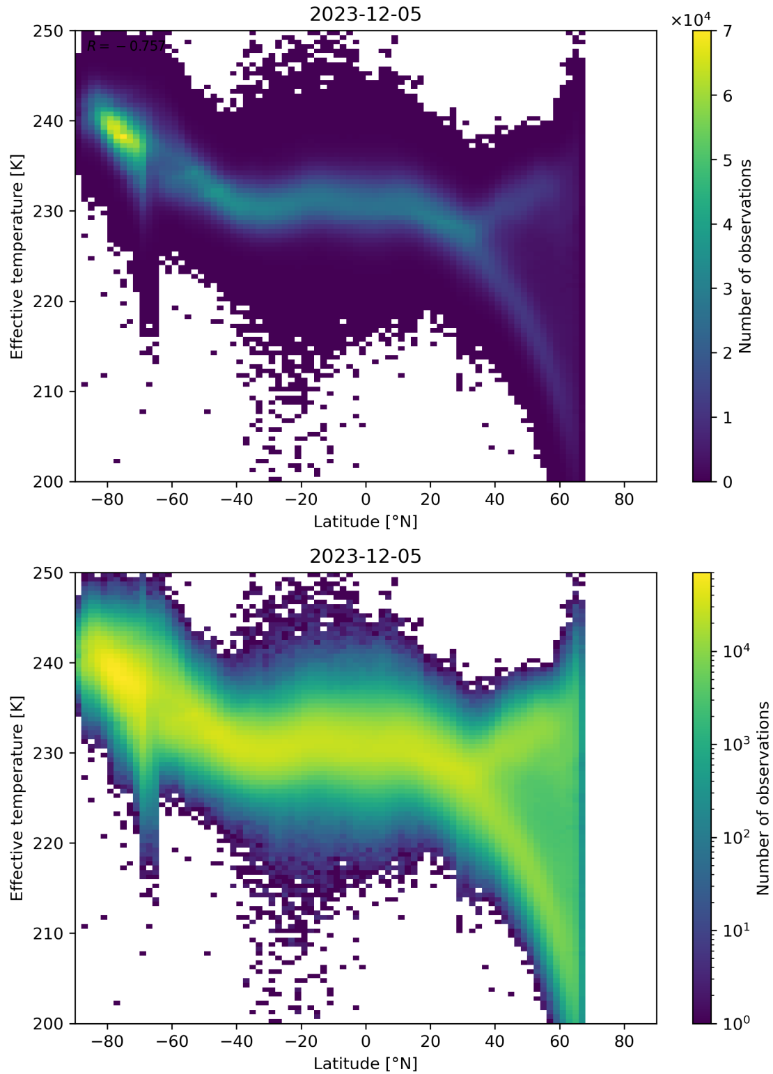
Figure 34: Scatter density plot of “Latitude” against “Effective temperature” for 2023-12-04 to 2023-12-06.
