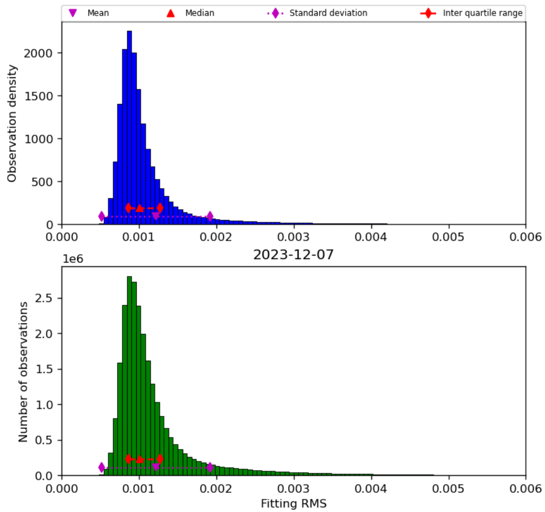
Figure 23: Histogram of “Fitting RMS” for 2023-12-06 to 2023-12-08
