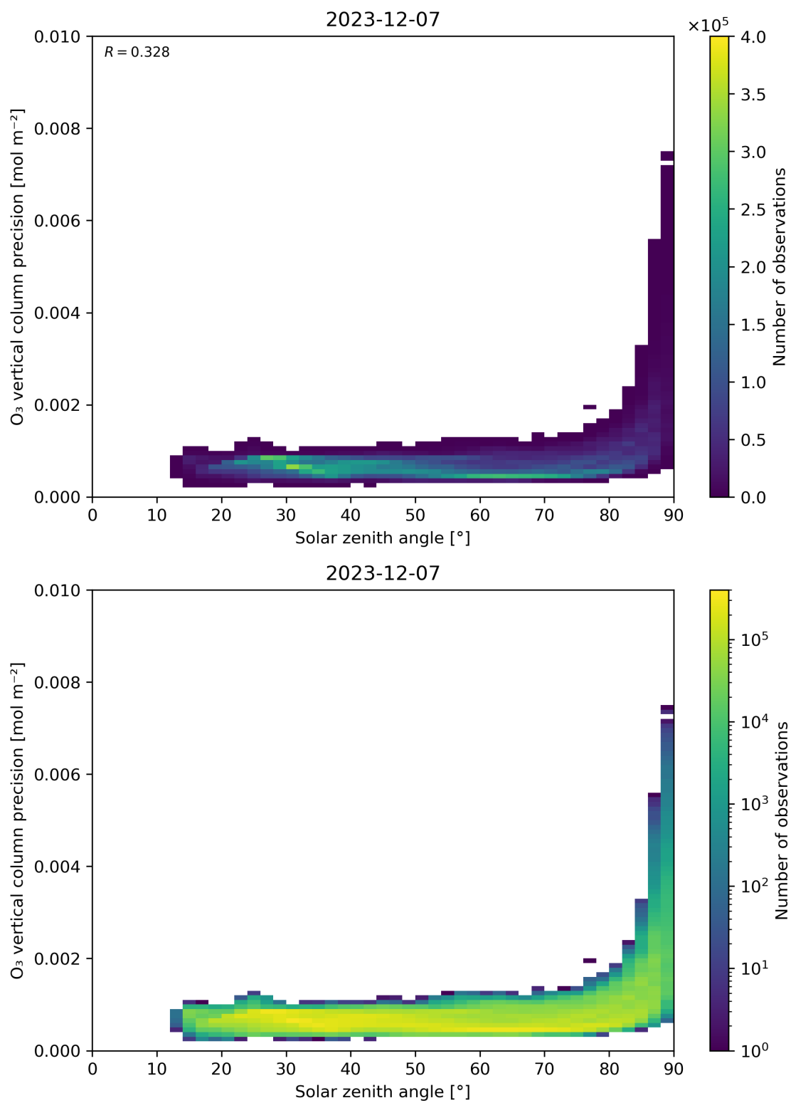
Figure 48: Scatter density plot of “Solar zenith angle” against “O 3 vertical column precision” for 2023-12-06 to 2023-12-08.
