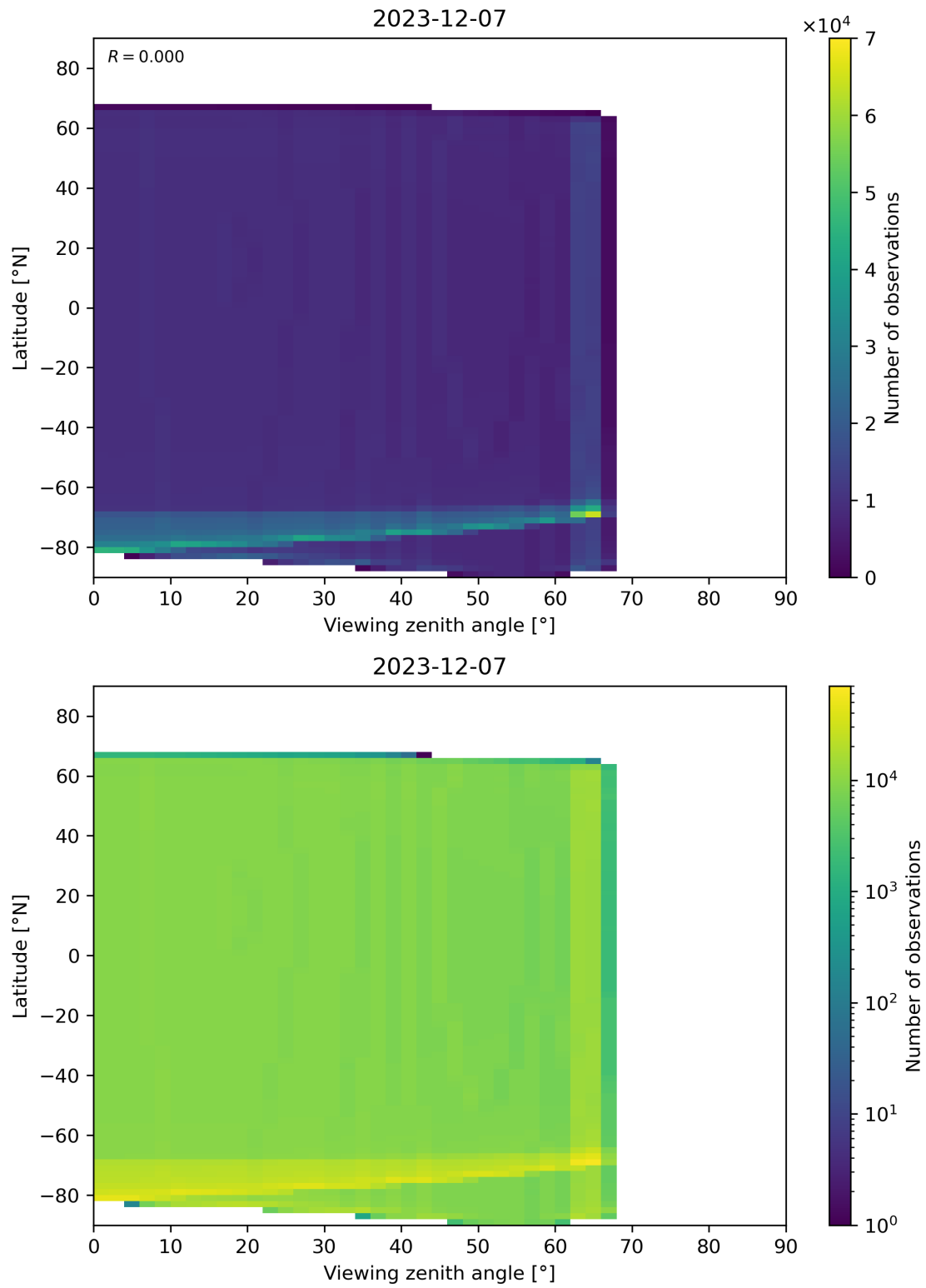
Figure 49: Scatter density plot of “Viewing zenith angle” against “Latitude” for 2023-12-06 to 2023-12-08.
