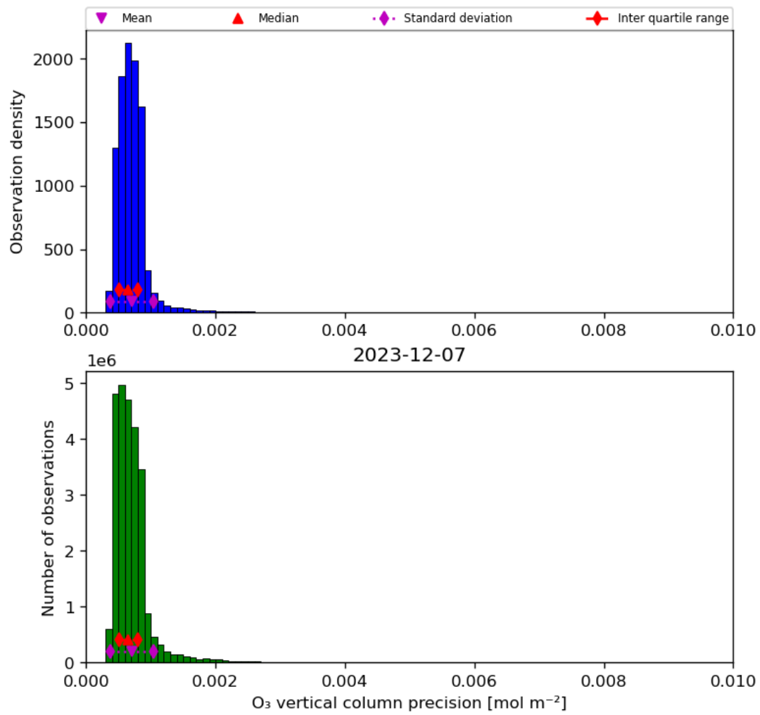
Figure 22: Histogram of “O 3 vertical column precision” for 2023-12-06 to 2023-12-08
