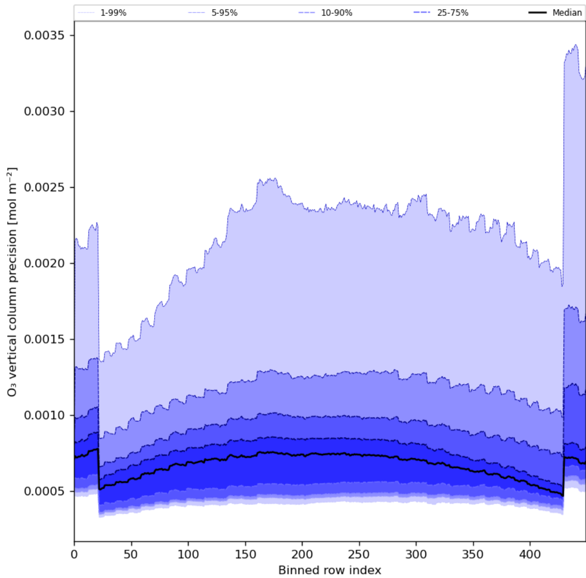
Figure 29: Along track statistics of “O 3 vertical column precision” for 2023-12-06 to 2023-12-08
