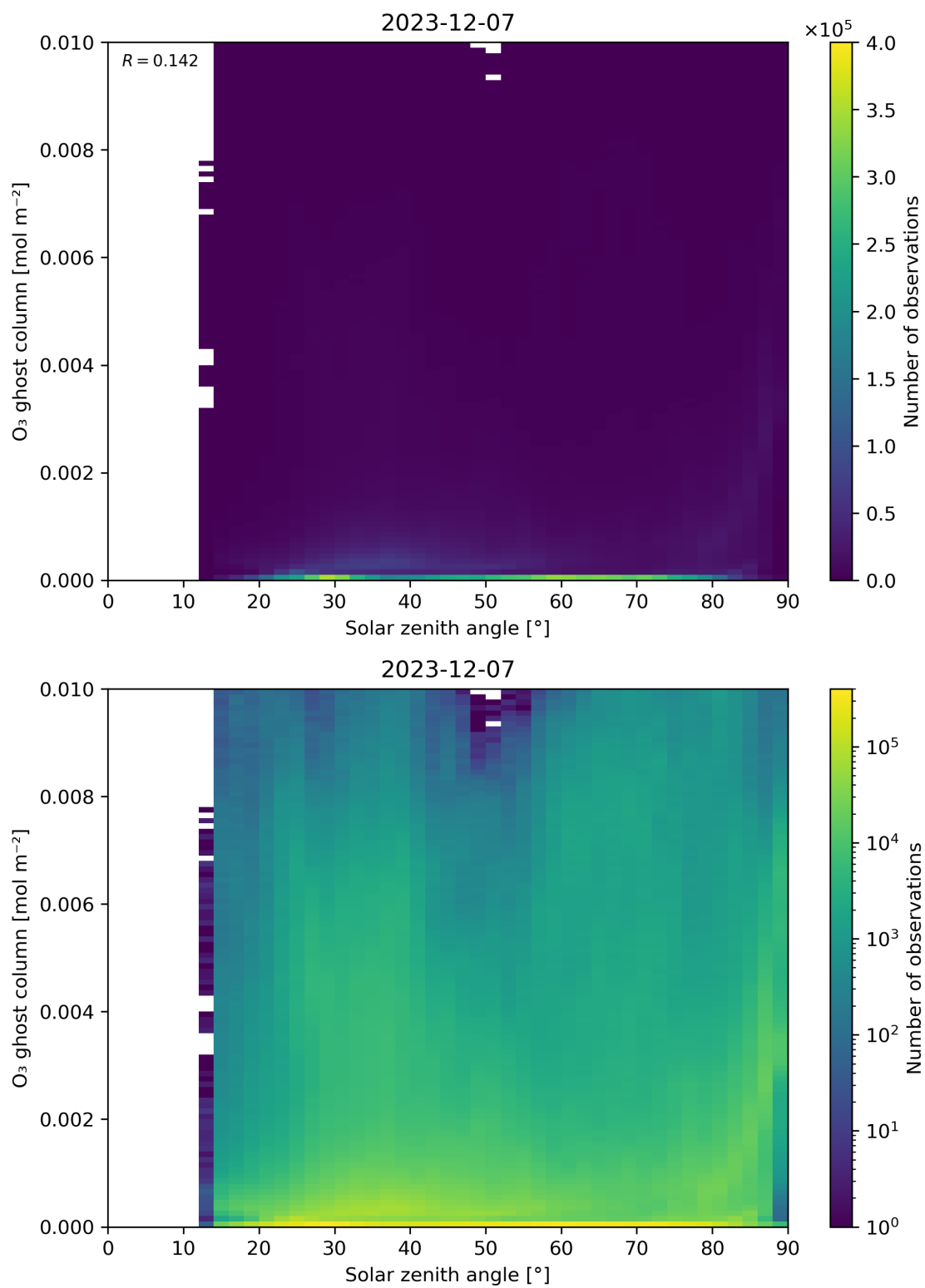
Figure 46: Scatter density plot of “Solar zenith angle” against “O 3 ghost column” for 2023-12-06 to 2023-12-08.
