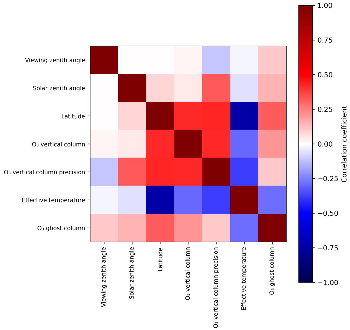
Figure 2: Map of correlation matrix for 2023-12-06 to 2023-12-08.
