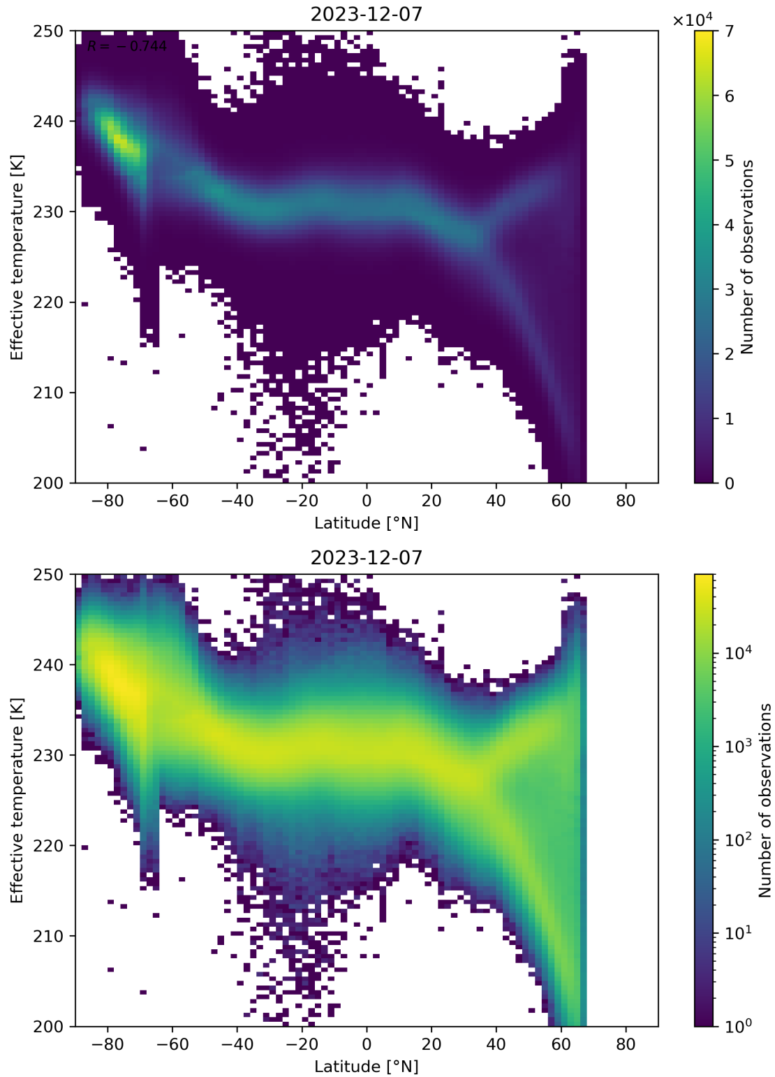
Figure 34: Scatter density plot of “Latitude” against “Effective temperature” for 2023-12-06 to 2023-12-08.
