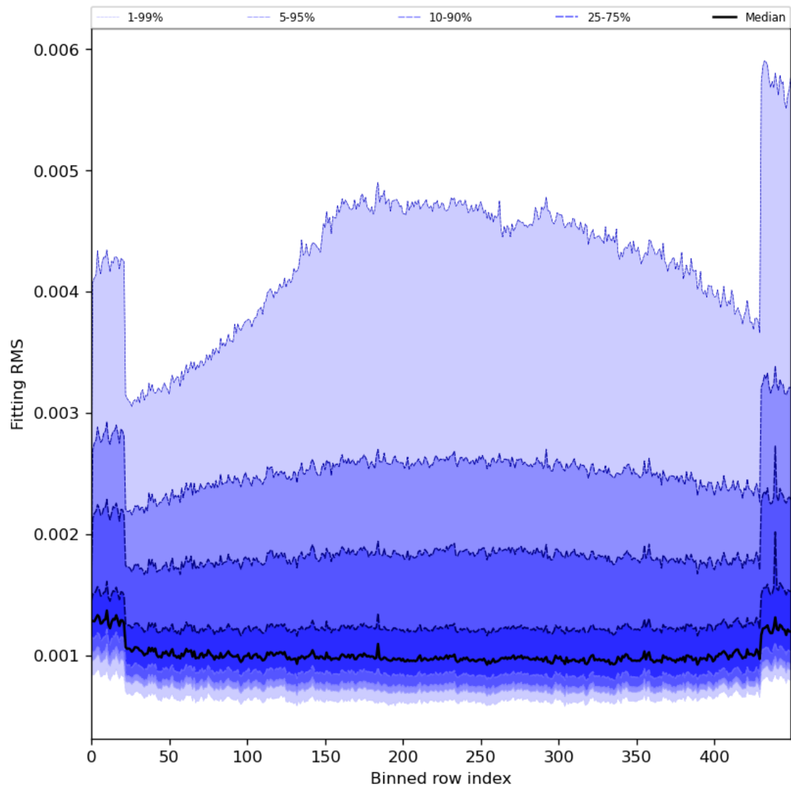
Figure 30: Along track statistics of “Fitting RMS” for 2023-12-06 to 2023-12-08
