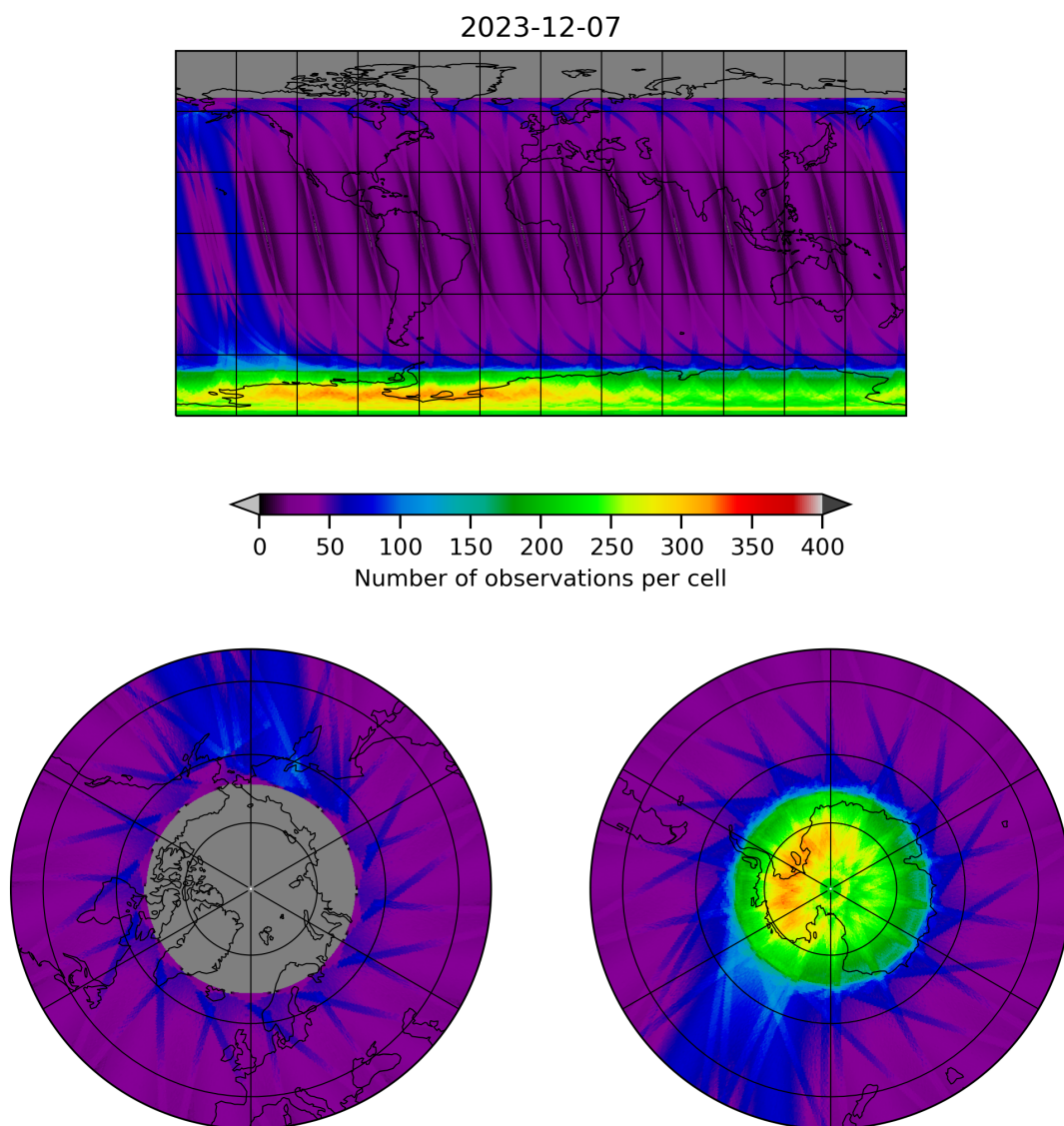
Figure 12: Map of the number of observations for 2023-12-06 to 2023-12-08
