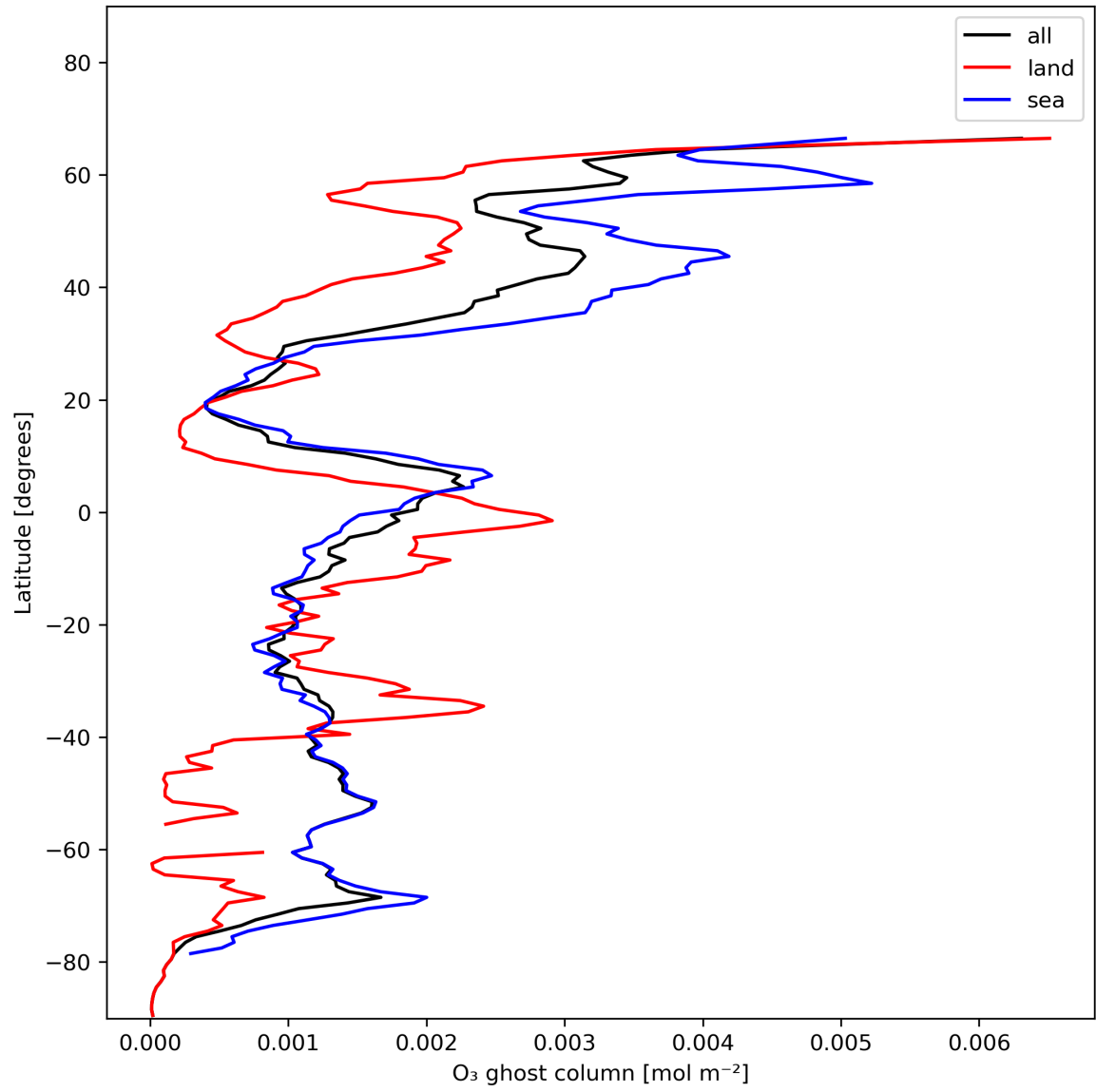
Figure 18: Zonal average of “O 3 ghost column” for 2023-12-06 to 2023-12-08.
