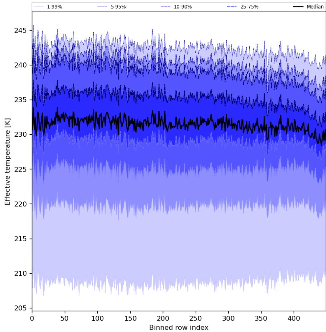
Figure 31: Along track statistics of “Effective temperature” for 2023-12-06 to 2023-12-08
