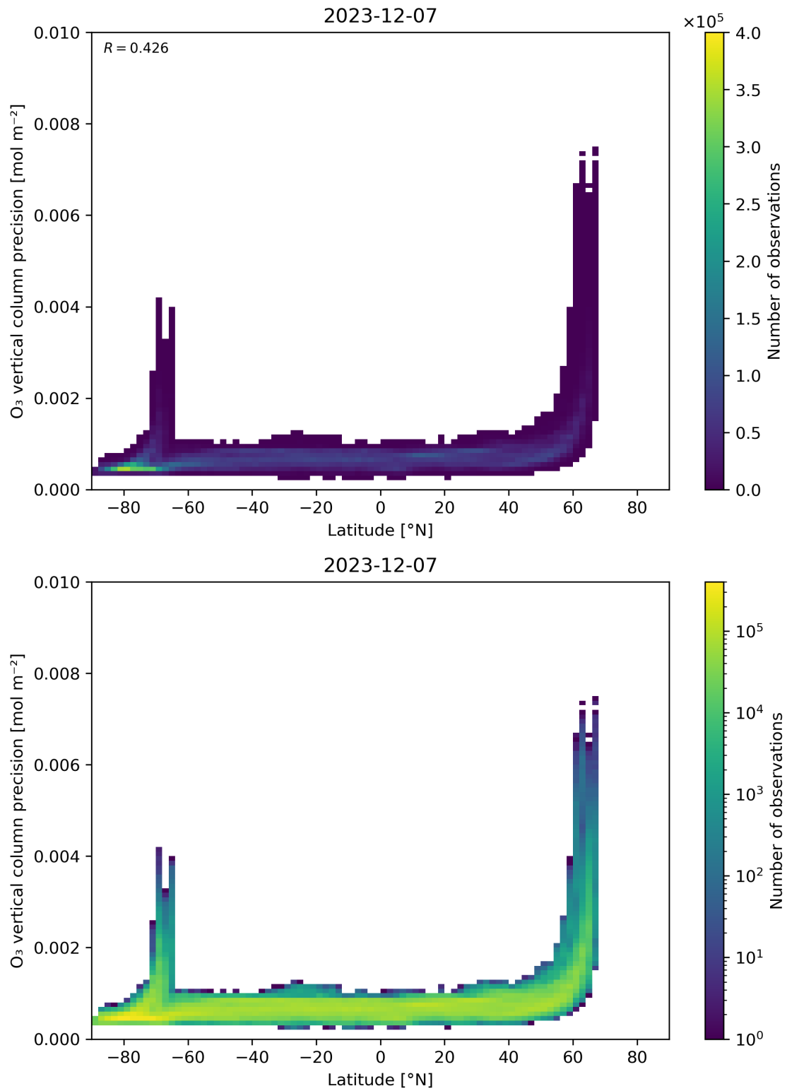
Figure 37: Scatter density plot of “Latitude” against “O 3 vertical column precision” for 2023-12-06 to 2023-12-08.
