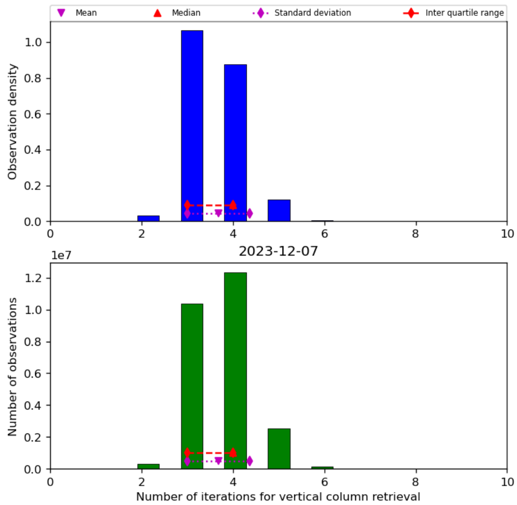
Figure 26: Histogram of “Number of iterations for vertical column retrieval” for 2023-12-06 to 2023-12-08
