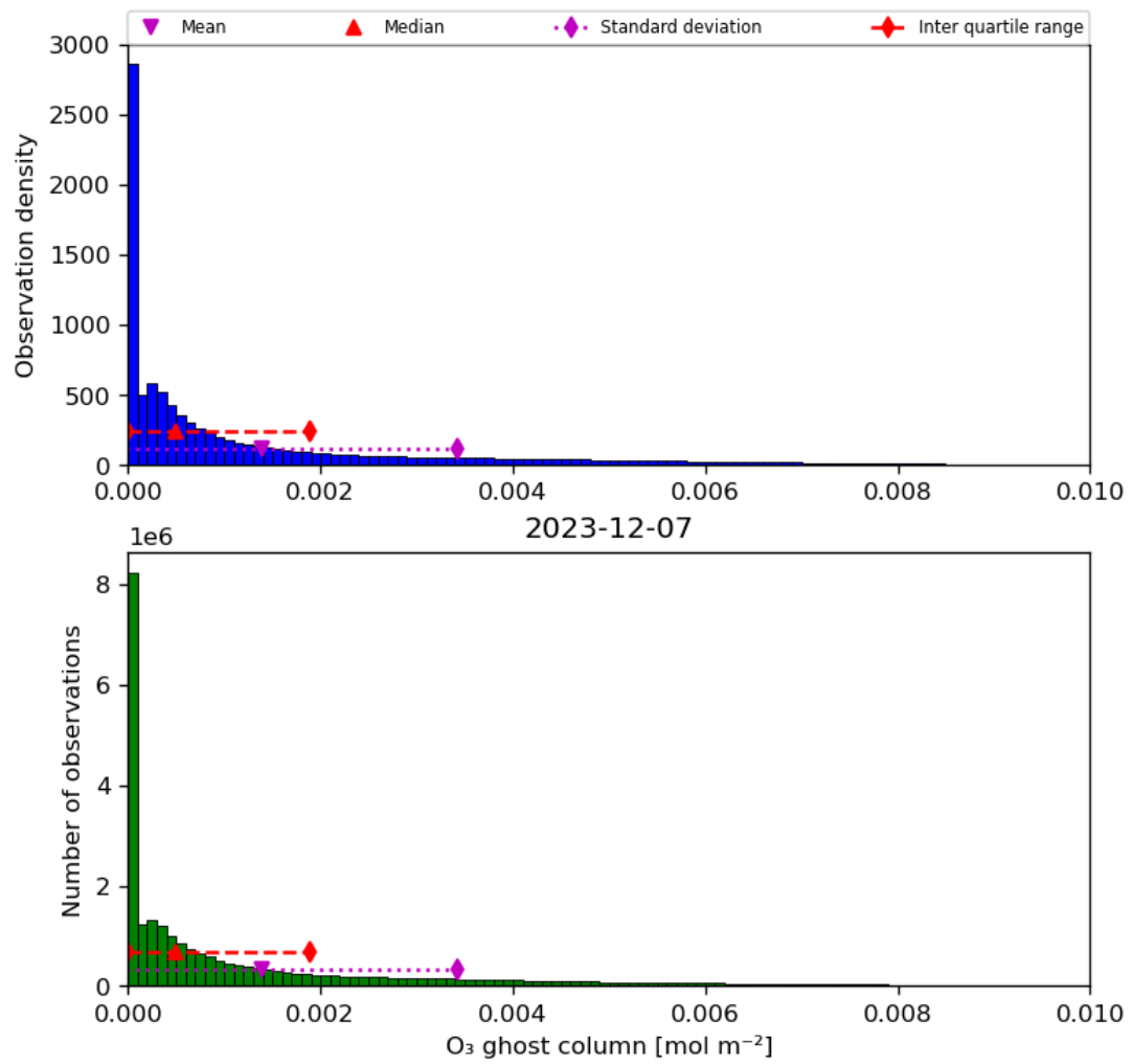
Figure 25: Histogram of “O 3 ghost column” for 2023-12-06 to 2023-12-08
