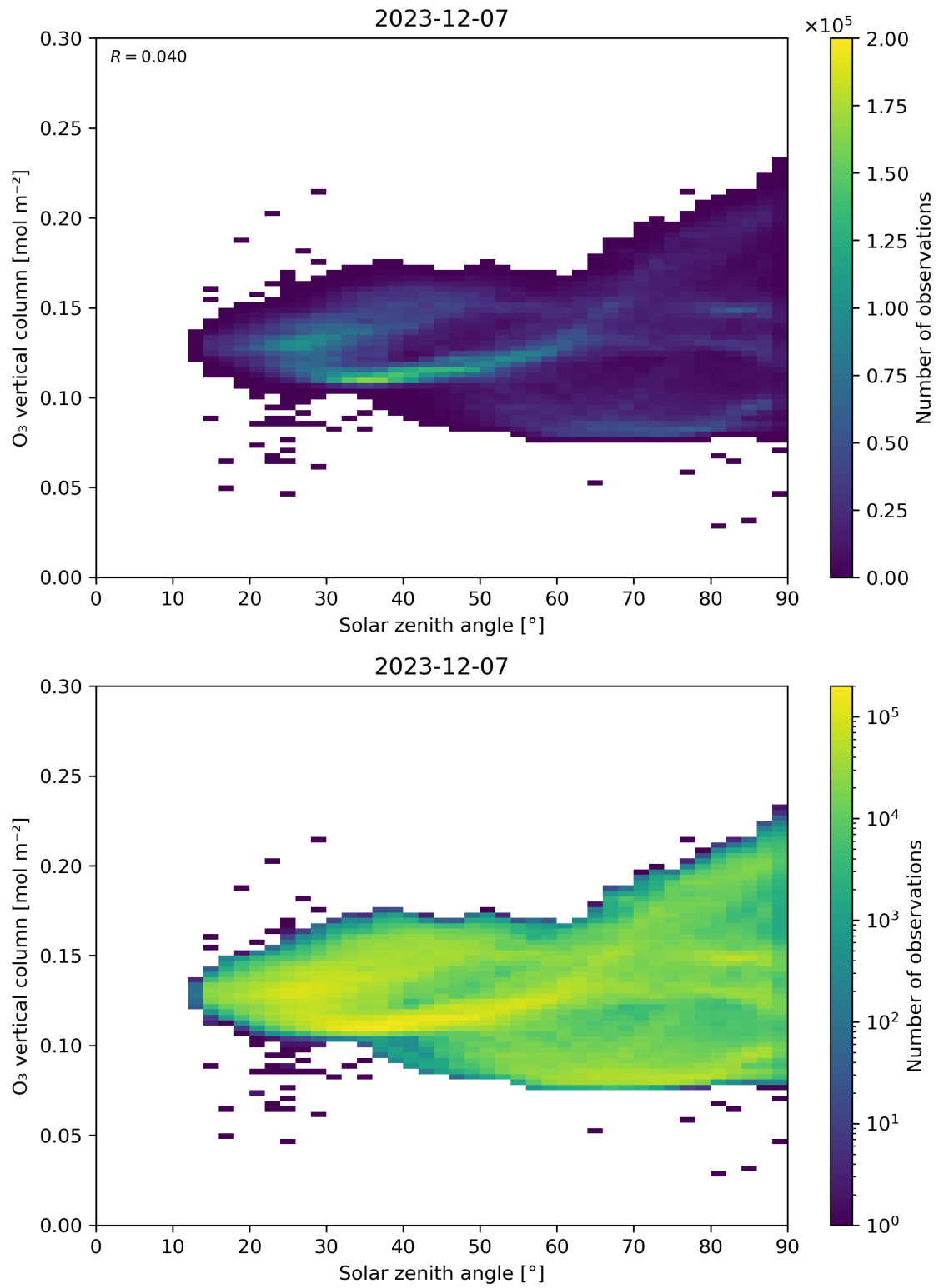
Figure 47: Scatter density plot of “Solar zenith angle” against “O 3 vertical column” for 2023-12-06 to 2023-12-08.
