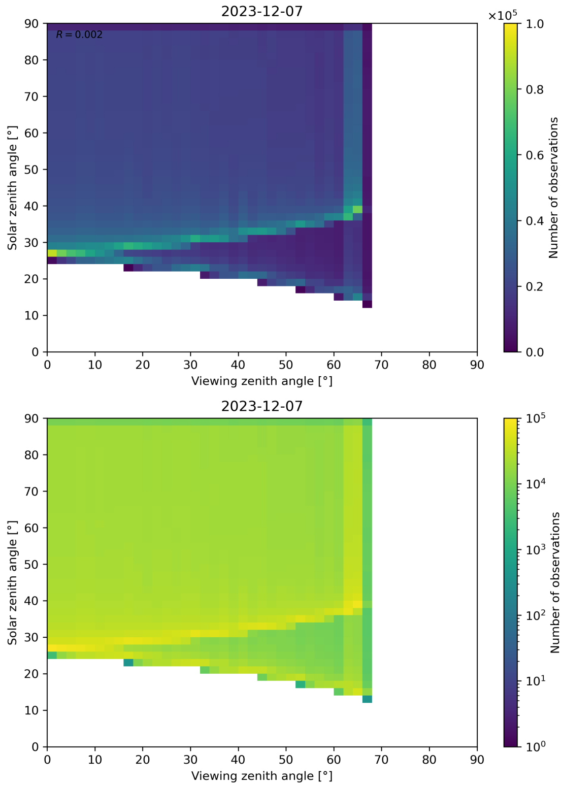
Figure 54: Scatter density plot of “Viewing zenith angle” against “Solar zenith angle” for 2023-12-06 to 2023-12-08.
