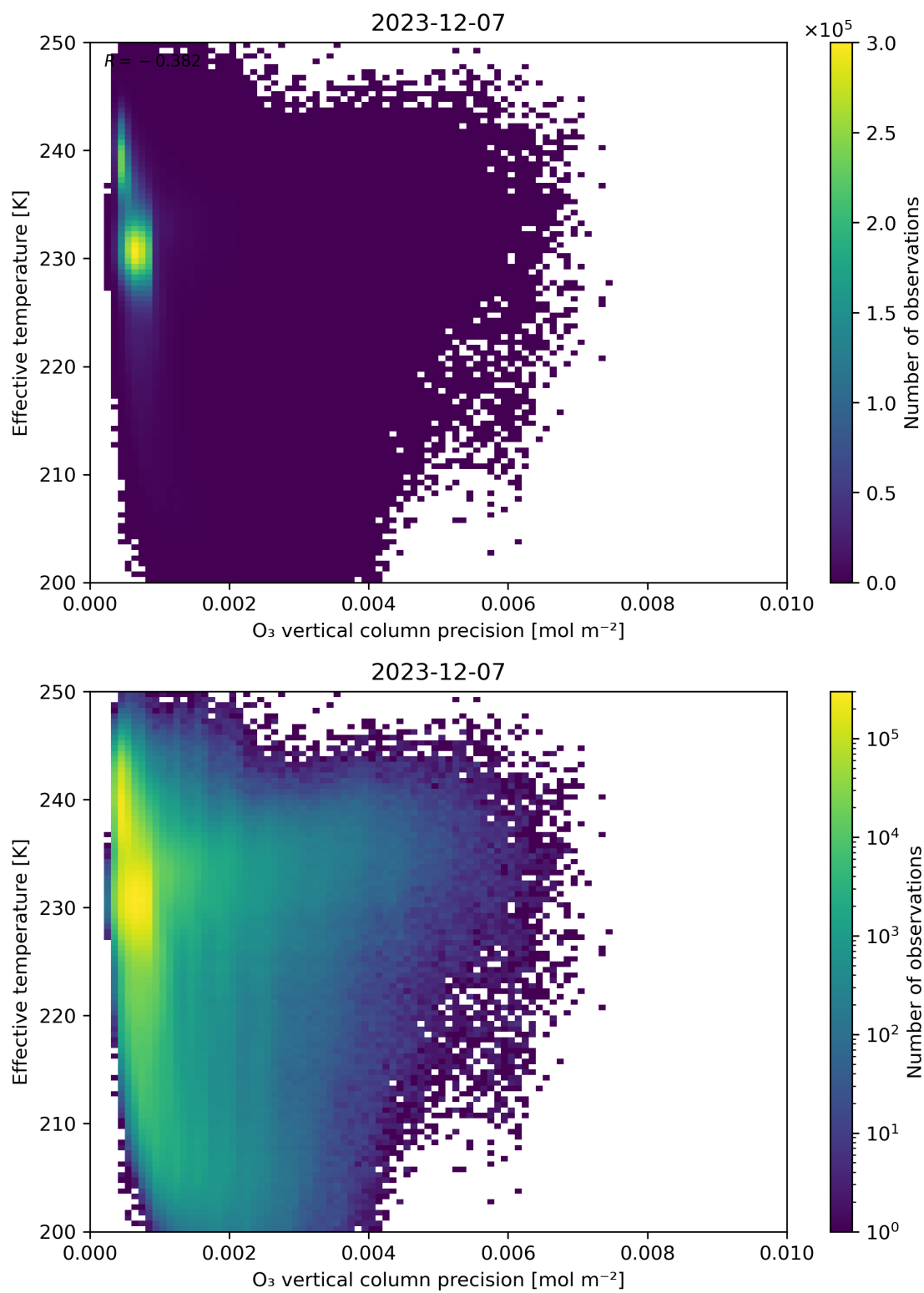
Figure 42: Scatter density plot of “O 3 vertical column precision” against “Effective temperature” for 2023-12-06 to 2023-12-08.
