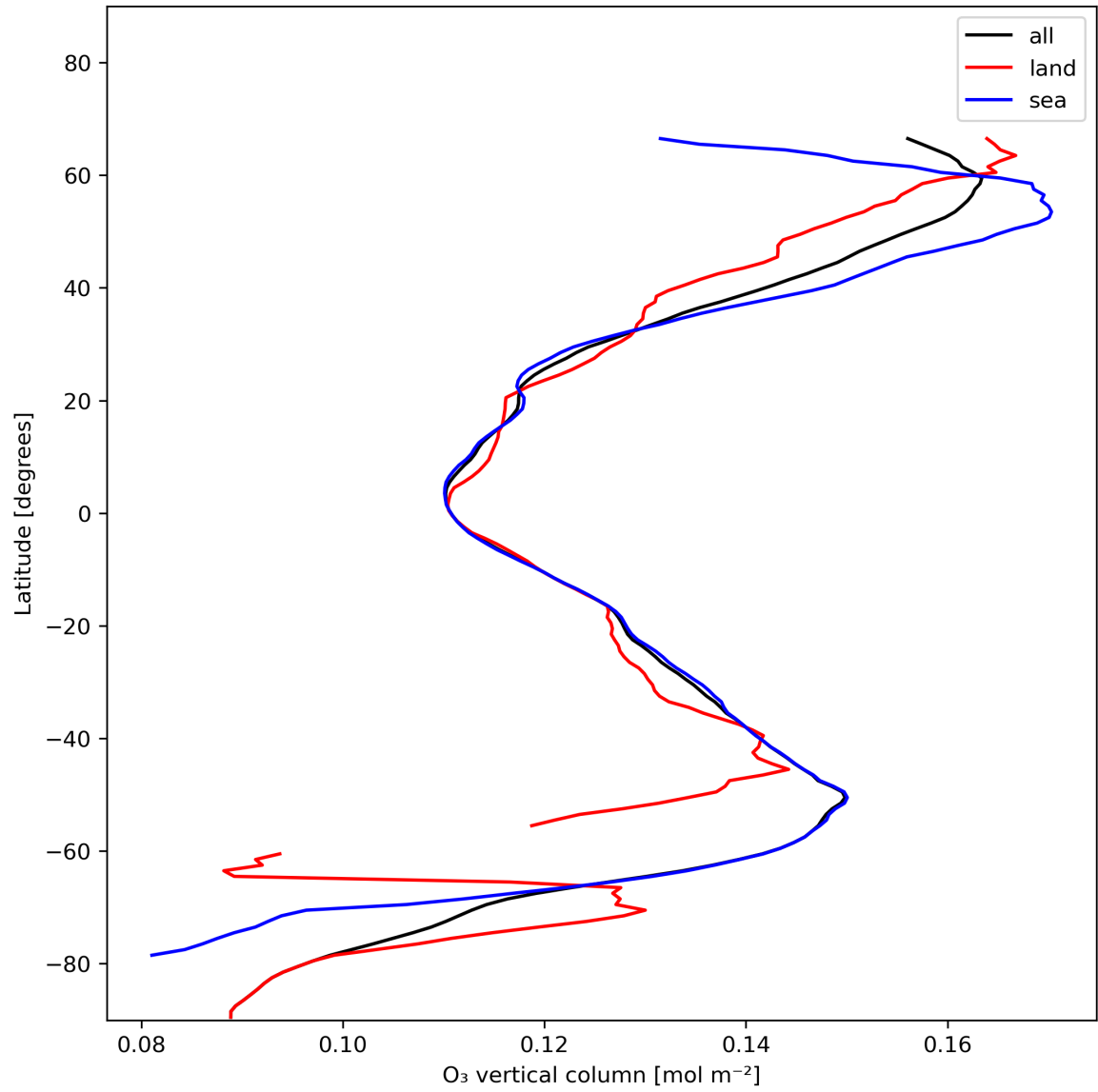
Figure 14: Zonal average of “O 3 vertical column” for 2023-12-06 to 2023-12-08.
