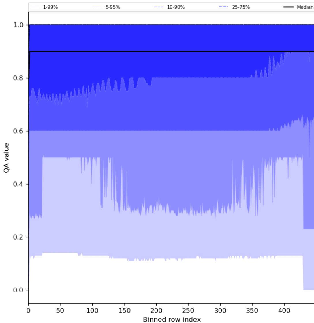
Figure 27: Along track statistics of “QA value” for 2023-12-06 to 2023-12-08
