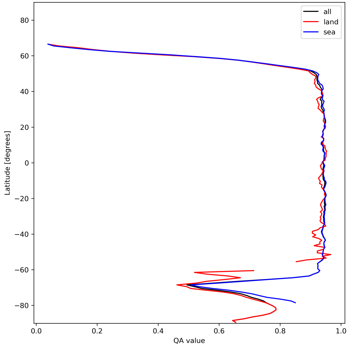
Figure 13: Zonal average of “QA value” for 2023-12-06 to 2023-12-08.
