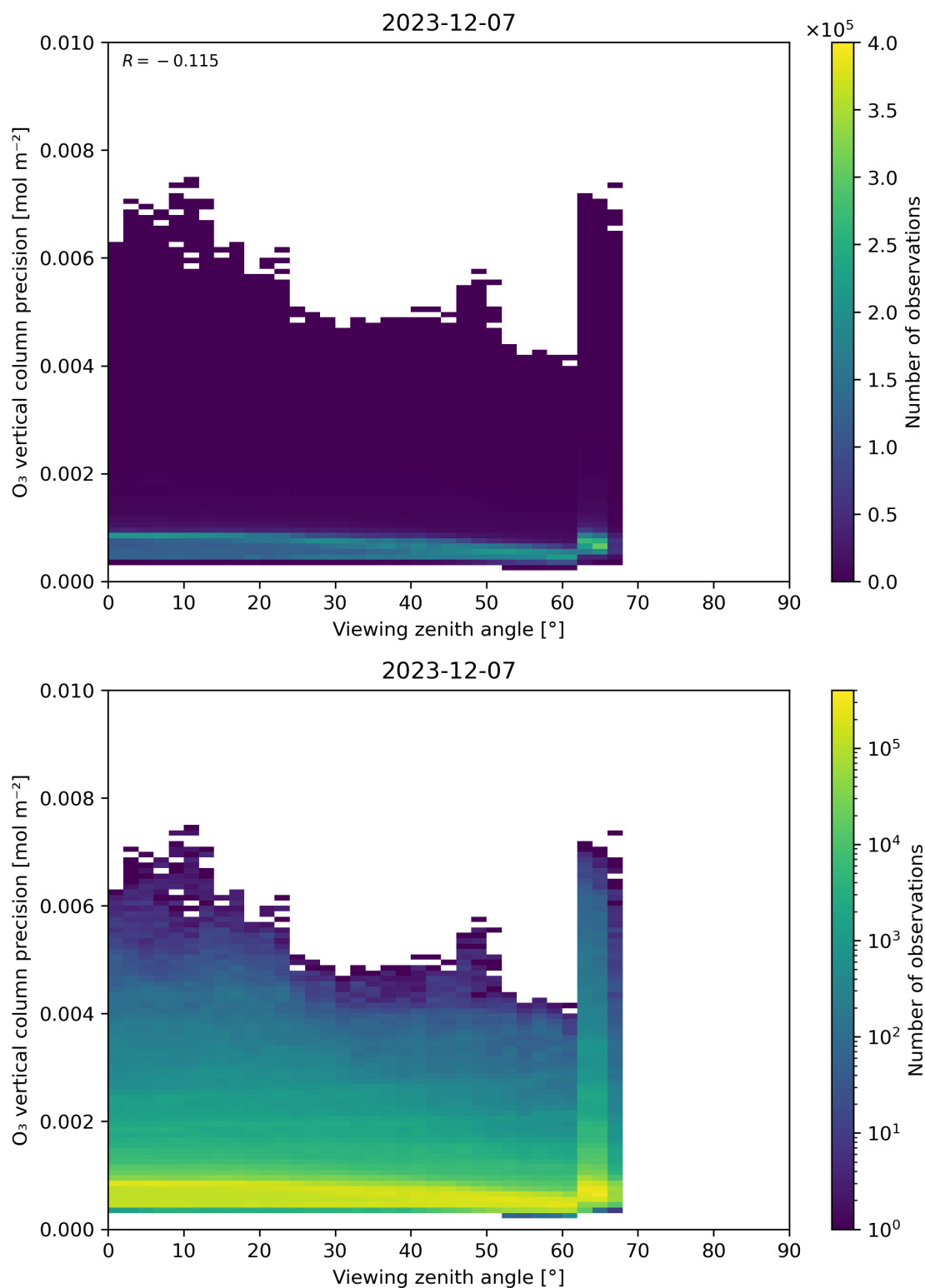
Figure 53: Scatter density plot of “Viewing zenith angle” against “O 3 vertical column precision” for 2023-12-06 to 2023-12-08.
