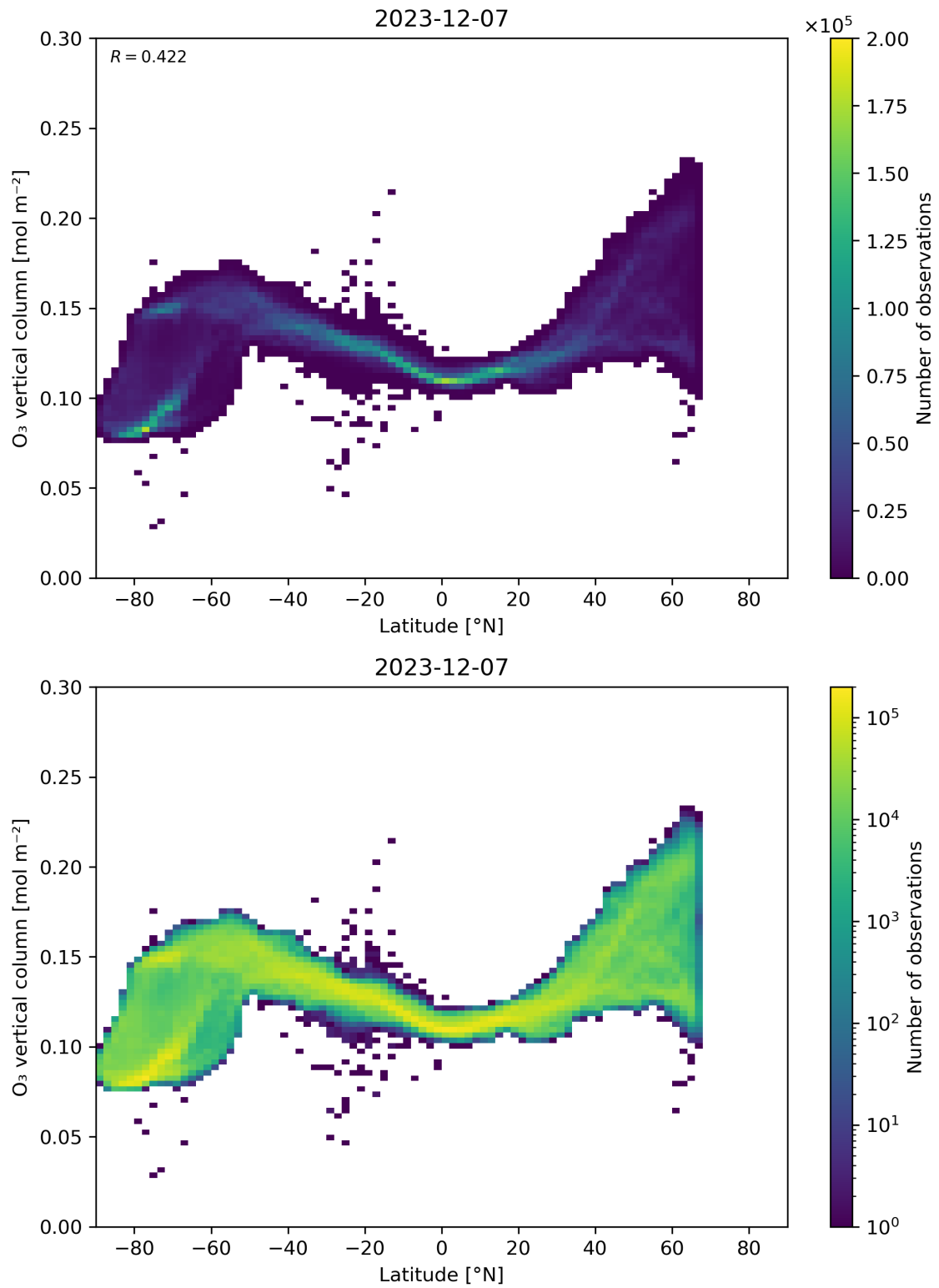
Figure 36: Scatter density plot of “Latitude” against “O 3 vertical column” for 2023-12-06 to 2023-12-08.
