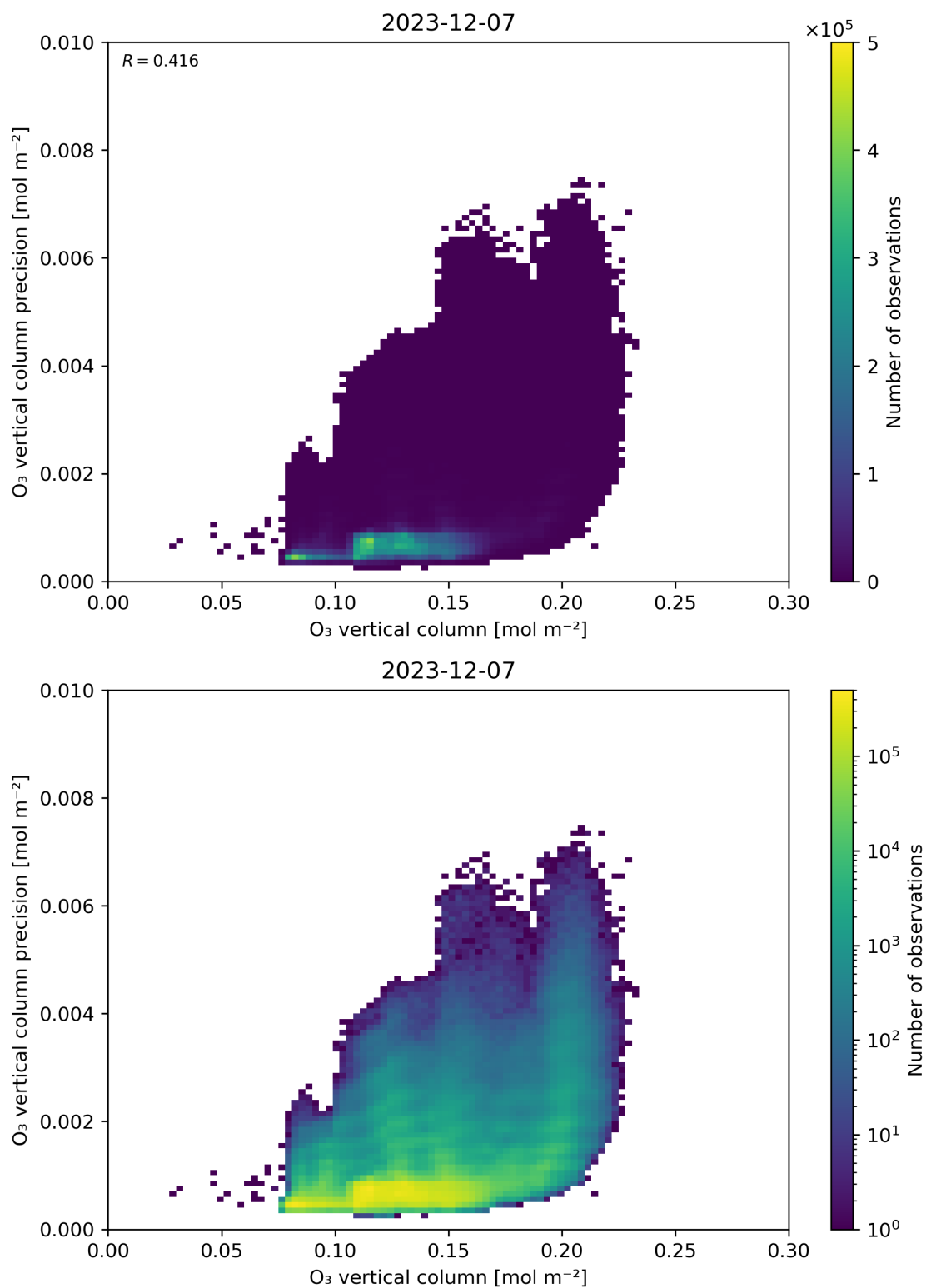
Figure 41: Scatter density plot of “O 3 vertical column” against “O 3 vertical column precision” for 2023-12-06 to 2023-12-08.
