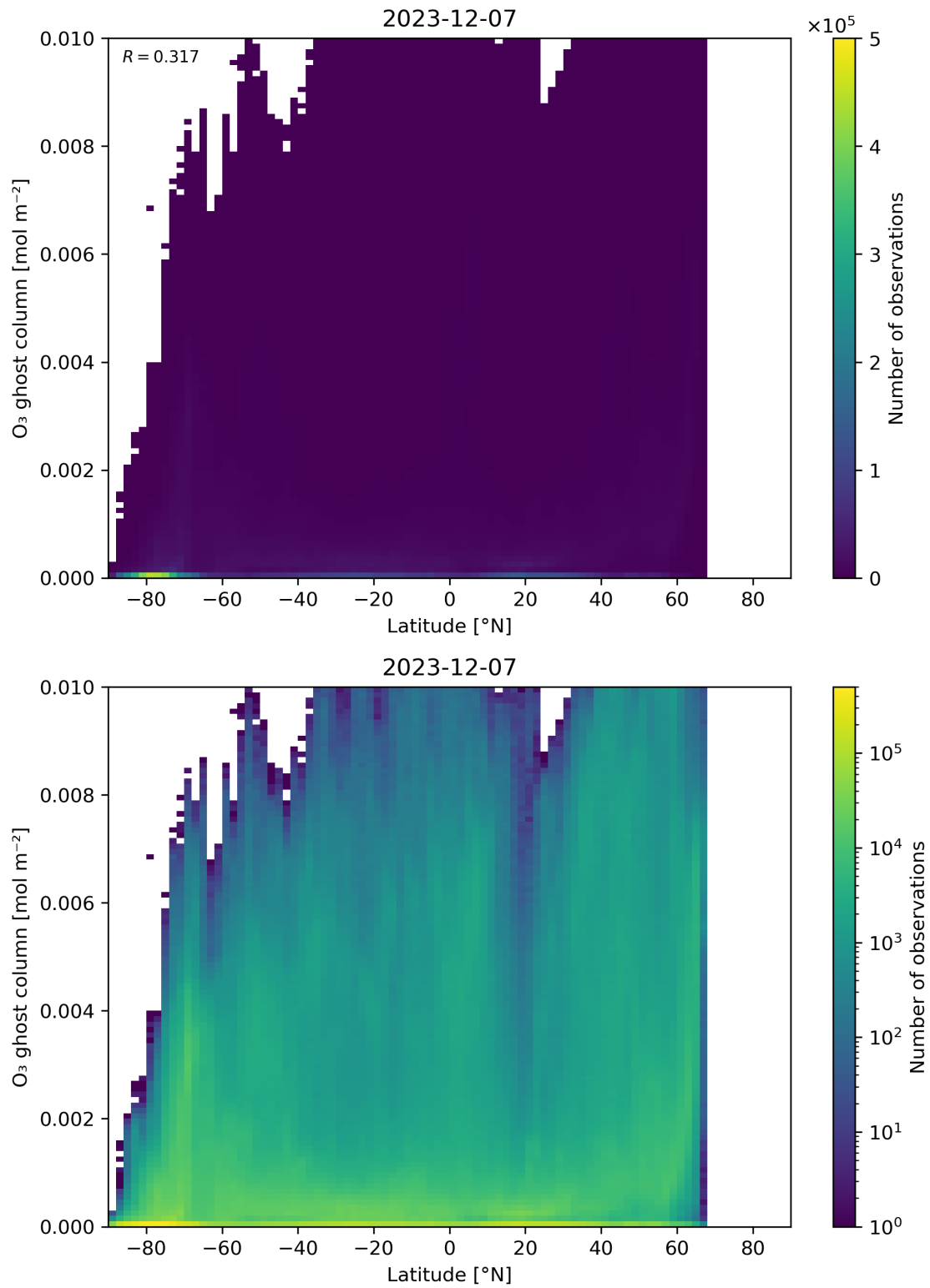
Figure 35: Scatter density plot of “Latitude” against “O 3 ghost column” for 2023-12-06 to 2023-12-08.
