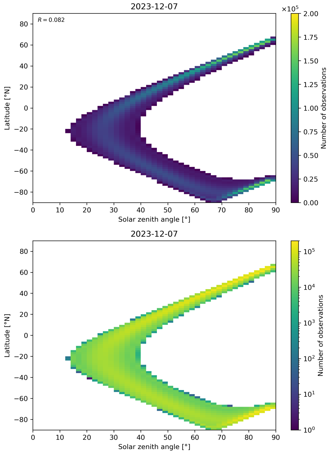
Figure 44: Scatter density plot of “Solar zenith angle” against “Latitude” for 2023-12-06 to 2023-12-08.
