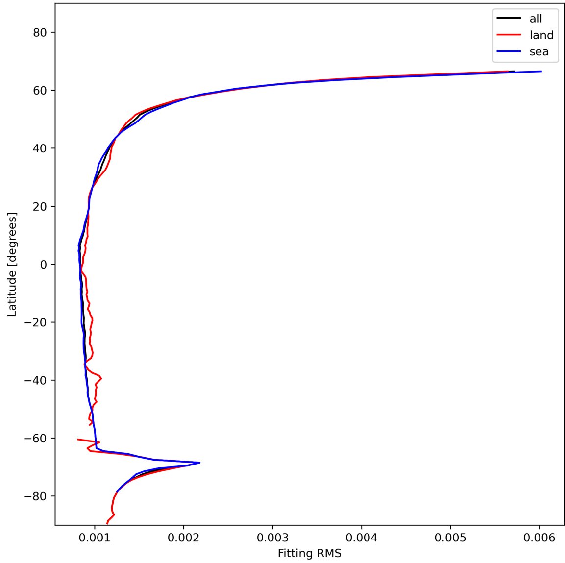
Figure 16: Zonal average of “Fitting RMS” for 2023-12-06 to 2023-12-08.
