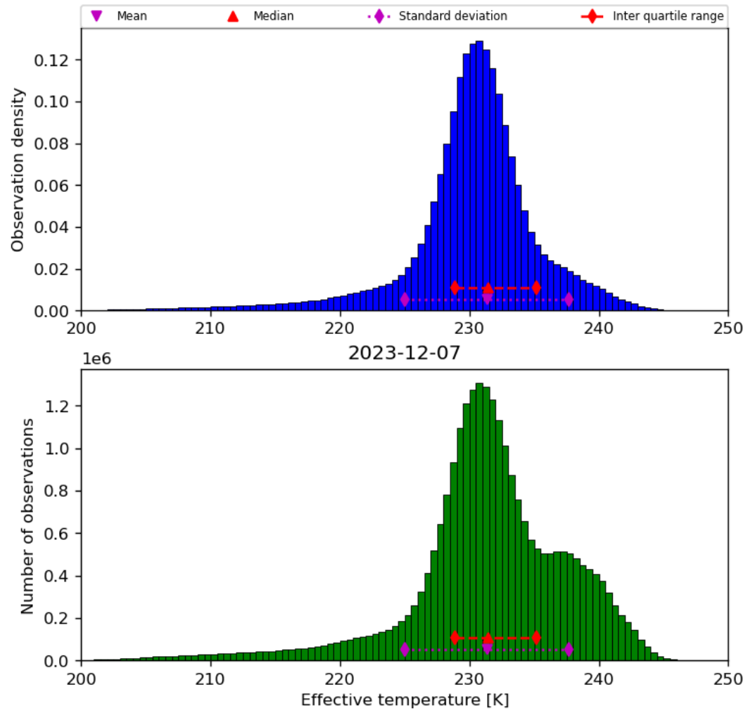
Figure 24: Histogram of “Effective temperature” for 2023-12-06 to 2023-12-08
