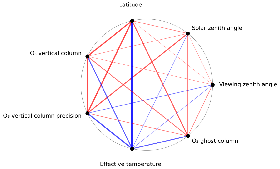
Figure 1: Map of correlation graph for 2023-12-06 to 2023-12-08.
