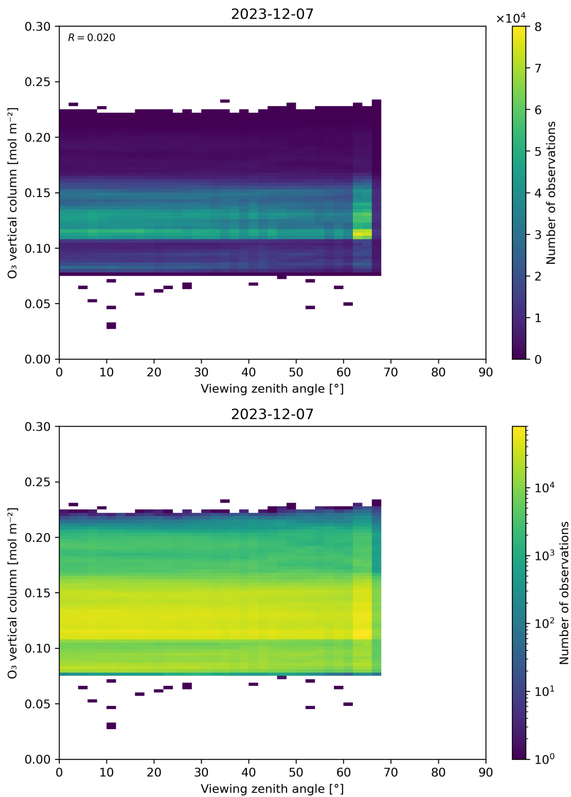
Figure 52: Scatter density plot of “Viewing zenith angle” against “O 3 vertical column” for 2023-12-06 to 2023-12-08.
