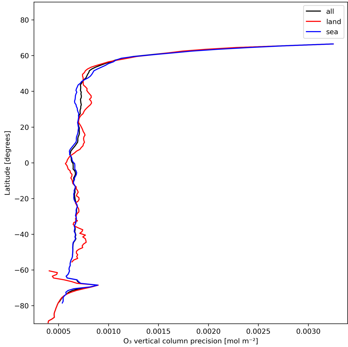
Figure 15: Zonal average of “O 3 vertical column precision” for 2023-12-06 to 2023-12-08.
