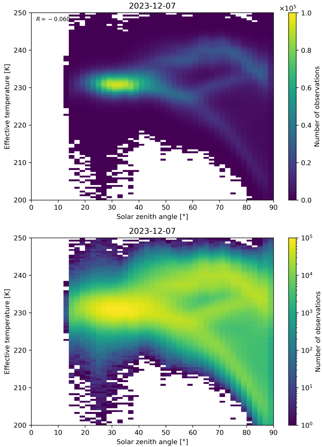
Figure 45: Scatter density plot of “Solar zenith angle” against “Effective temperature” for 2023-12-06 to 2023-12-08.
