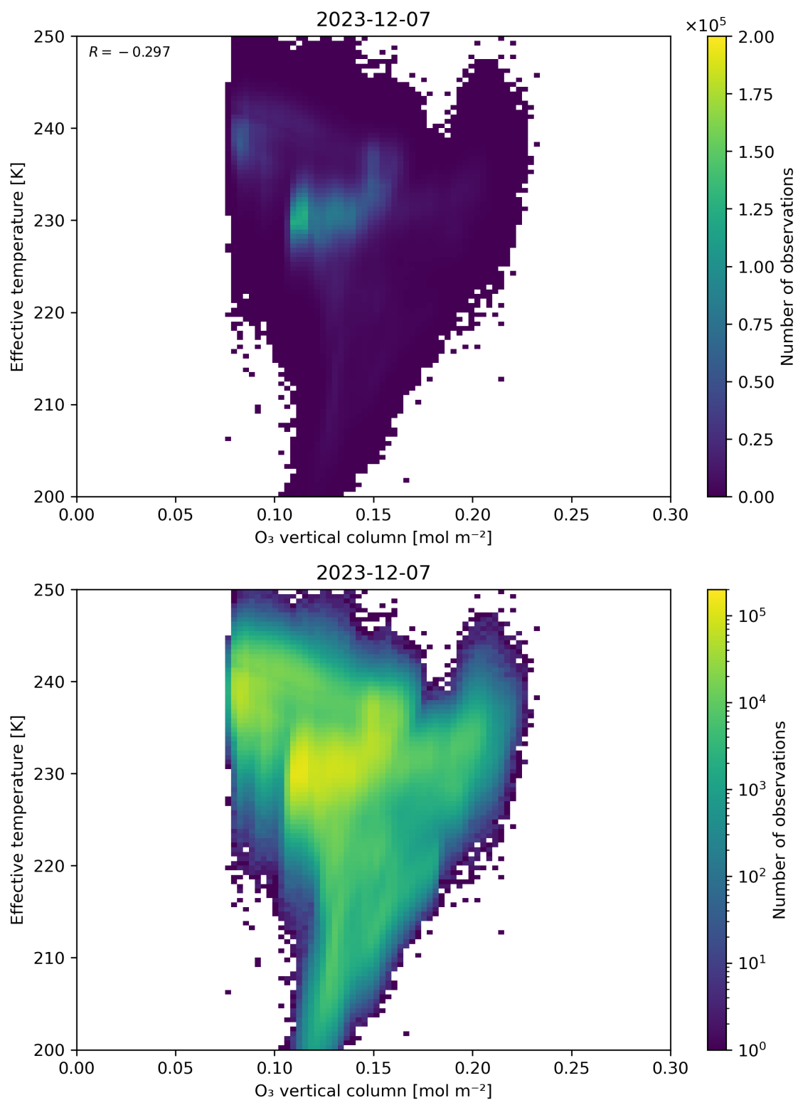
Figure 39: Scatter density plot of “O 3 vertical column” against “Effective temperature” for 2023-12-06 to 2023-12-08.
