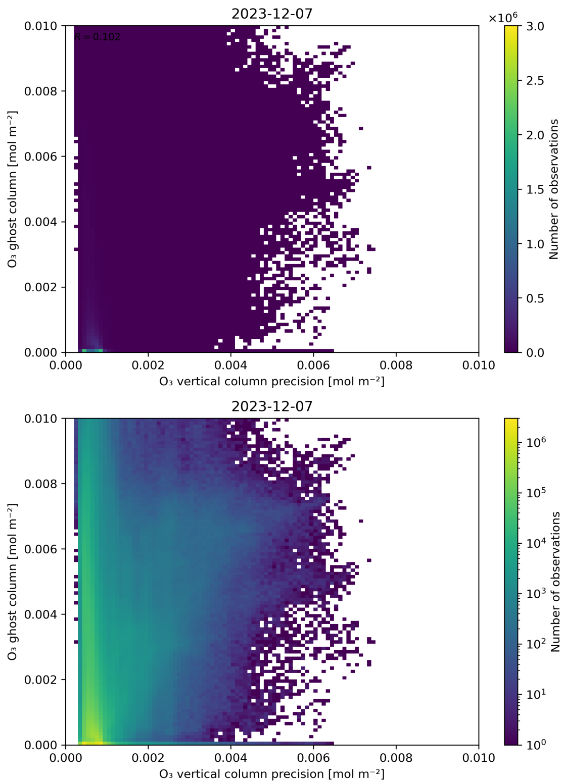
Figure 43: Scatter density plot of “ \text{O}_3 vertical column precision” against “ \text{O}_3 ghost column” for 2023-12-06 to 2023-12-08.
