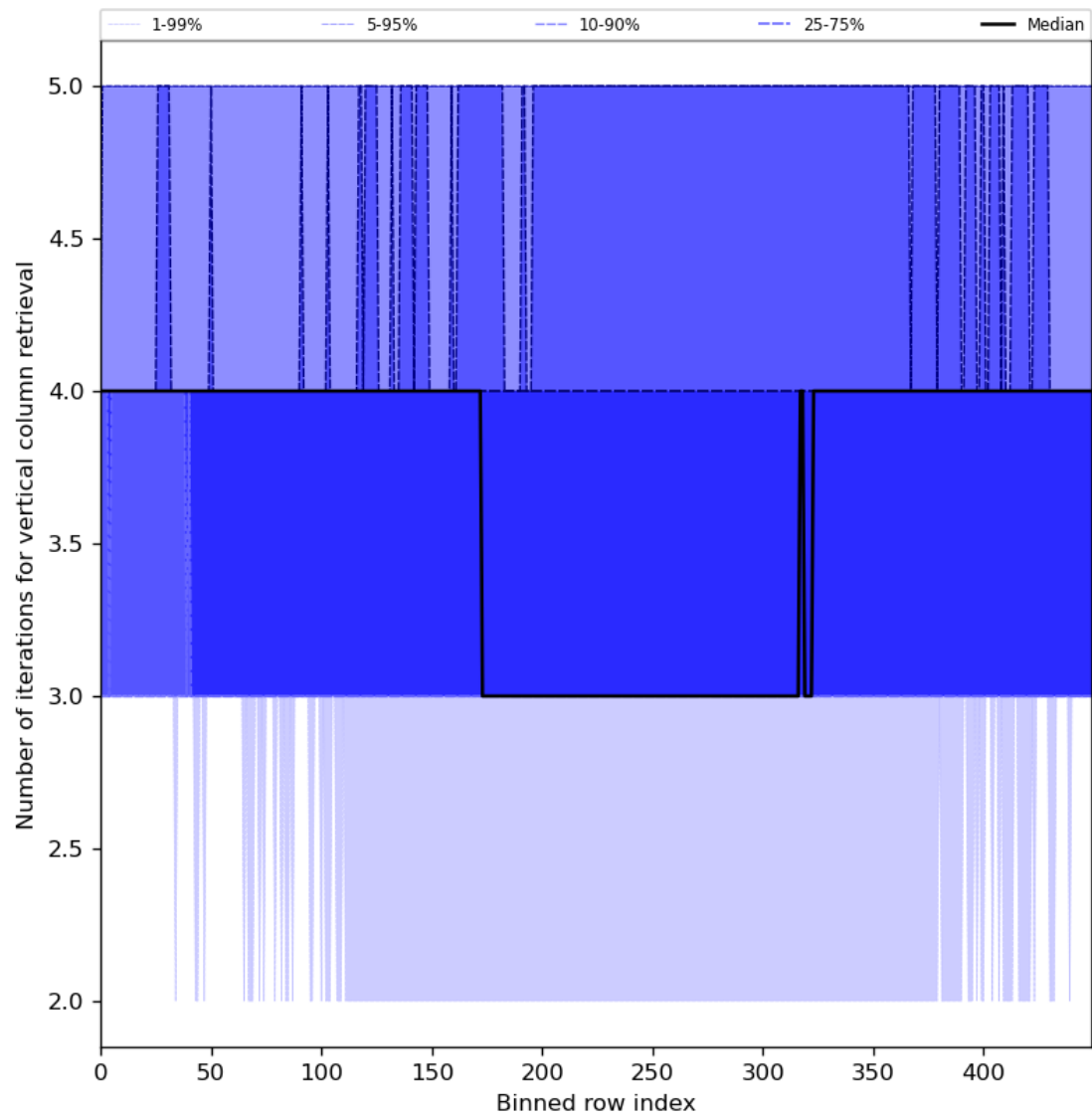
Figure 33: Along track statistics of “Number of iterations for vertical column retrieval” for 2023-12-06 to 2023-12-08
