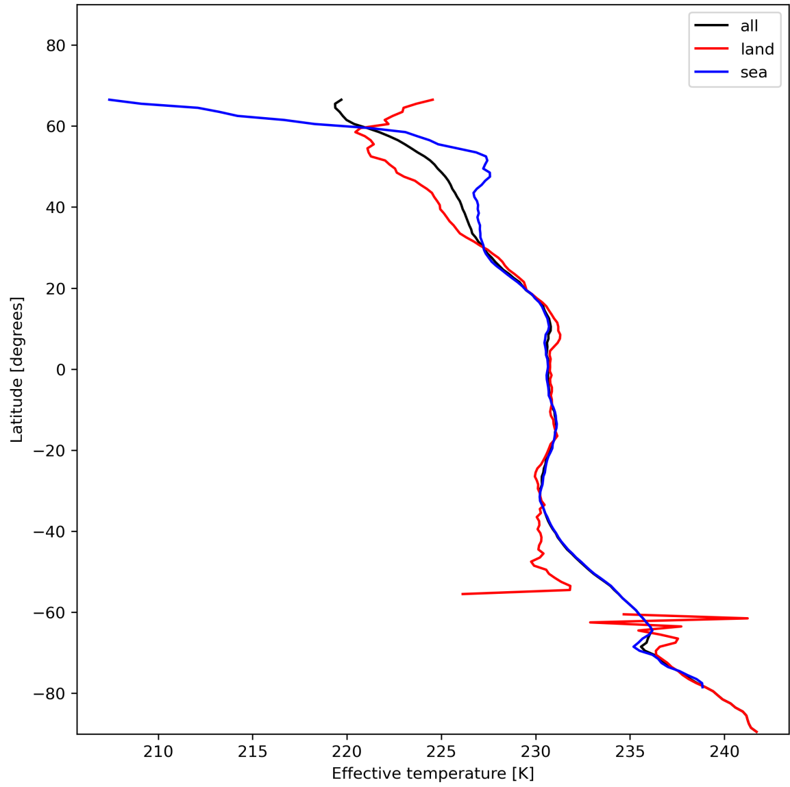
Figure 17: Zonal average of "Effective temperature" for 2023-12-06 to 2023-12-08.
