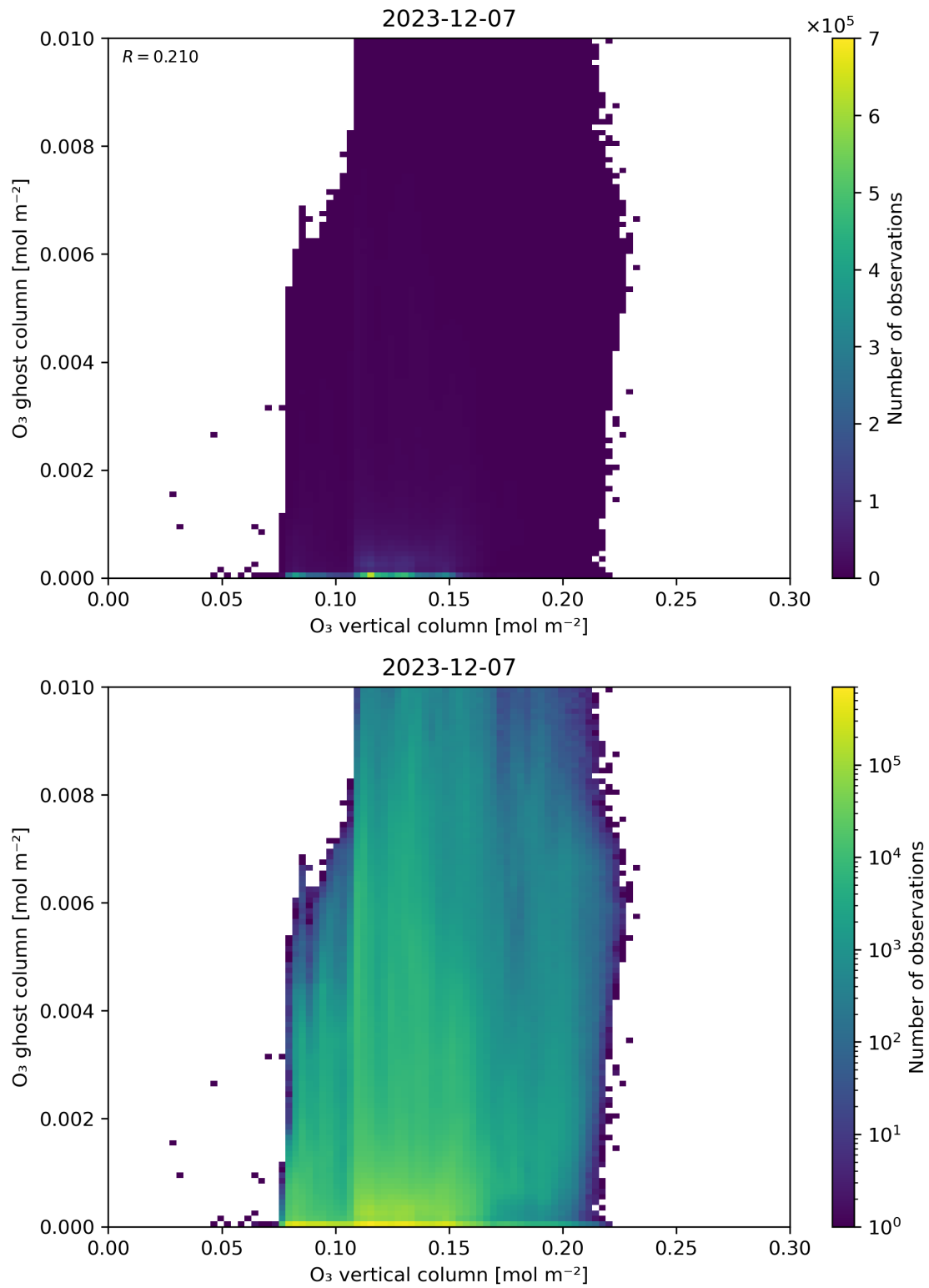
Figure 40: Scatter density plot of “O 3 vertical column” against “O 3 ghost column” for 2023-12-06 to 2023-12-08.
