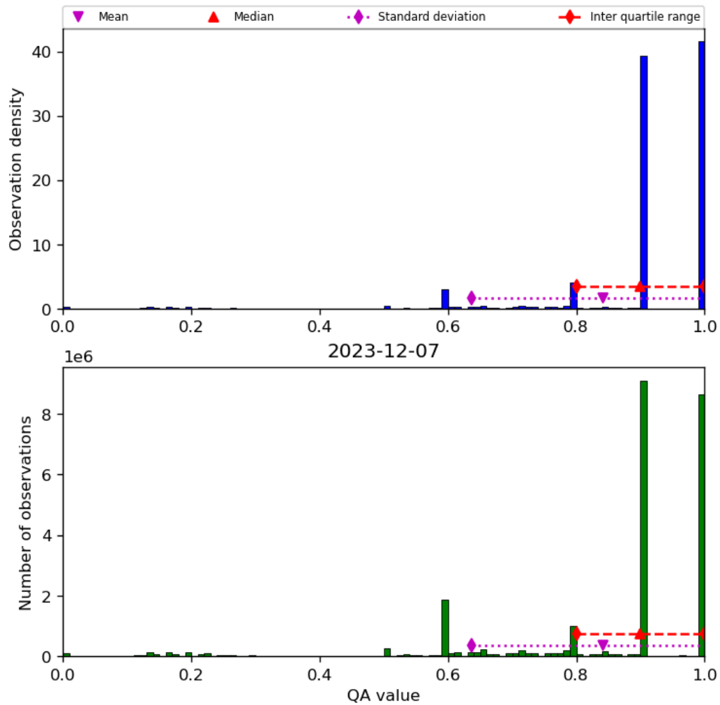
Figure 20: Histogram of “QA value” for 2023-12-06 to 2023-12-08
