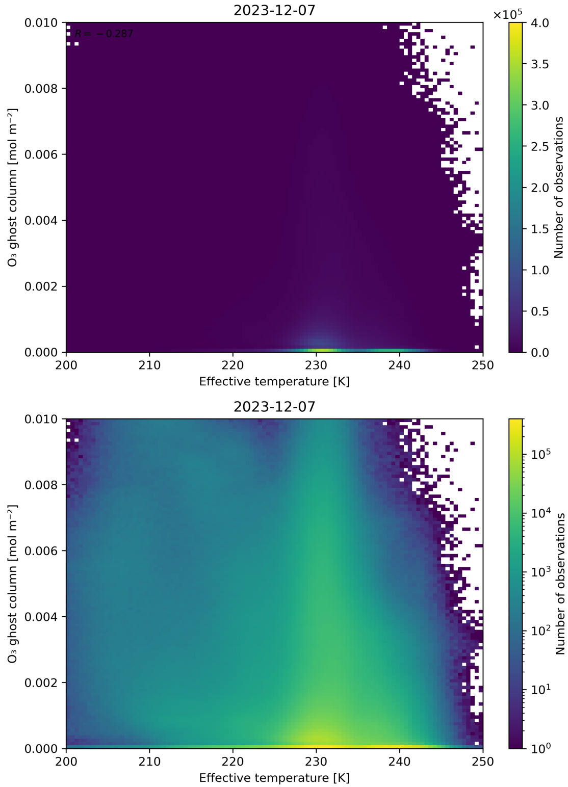
Figure 38: Scatter density plot of “Effective temperature” against “O 3 ghost column” for 2023-12-06 to 2023-12-08.
