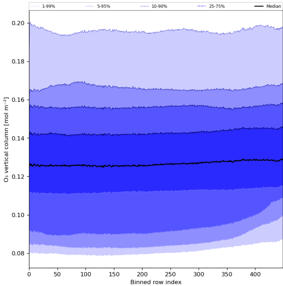
Figure 28: Along track statistics of “O 3 vertical column” for 2023-12-06 to 2023-12-08
