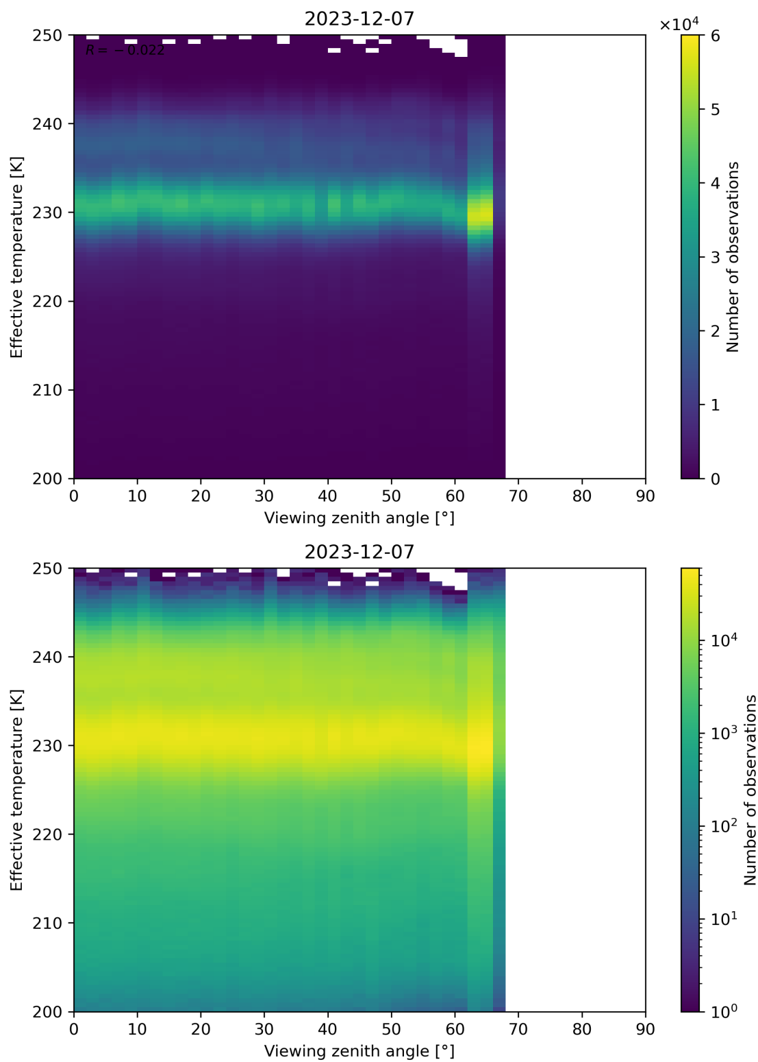
Figure 50: Scatter density plot of “Viewing zenith angle” against “Effective temperature” for 2023-12-06 to 2023-12-08.
