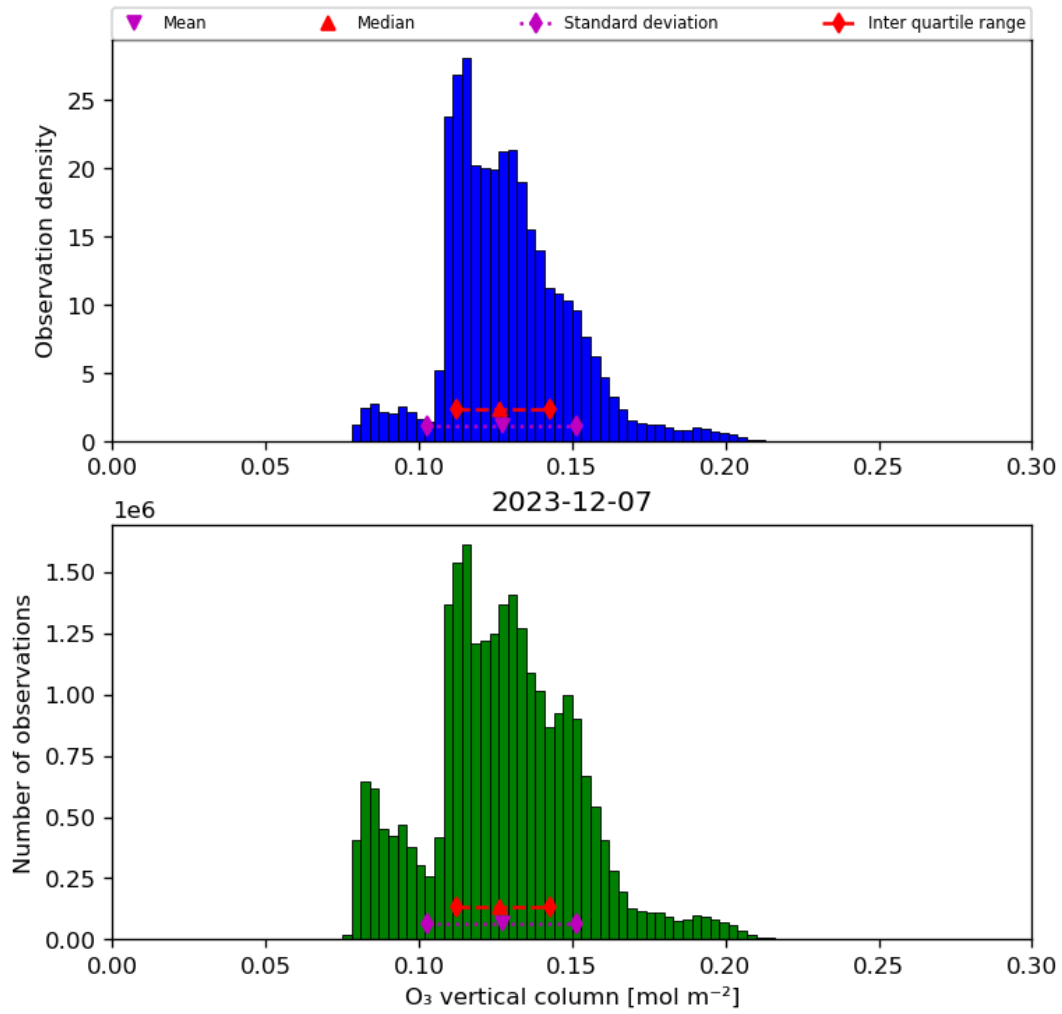
Figure 21: Histogram of “O 3 vertical column” for 2023-12-06 to 2023-12-08
