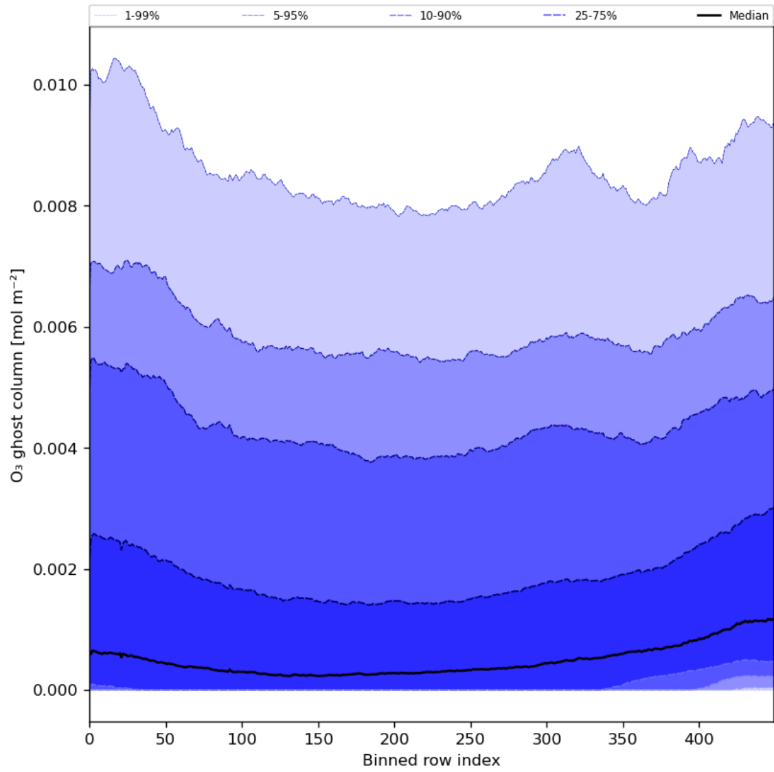
Figure 32: Along track statistics of "O 3 ghost column" for 2023-12-06 to 2023-12-08
