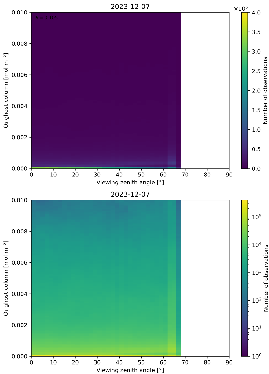
Figure 51: Scatter density plot of “Viewing zenith angle” against “O 3 ghost column” for 2023-12-06 to 2023-12-08.
