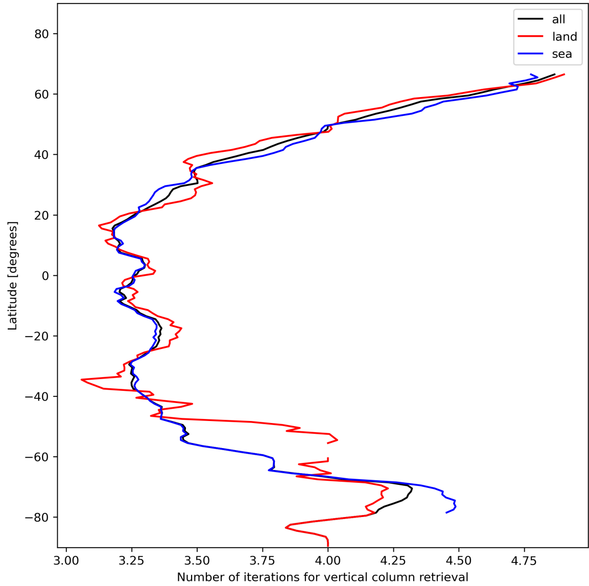
Figure 19: Zonal average of “Number of iterations for vertical column retrieval” for 2023-12-06 to 2023-12-08.
