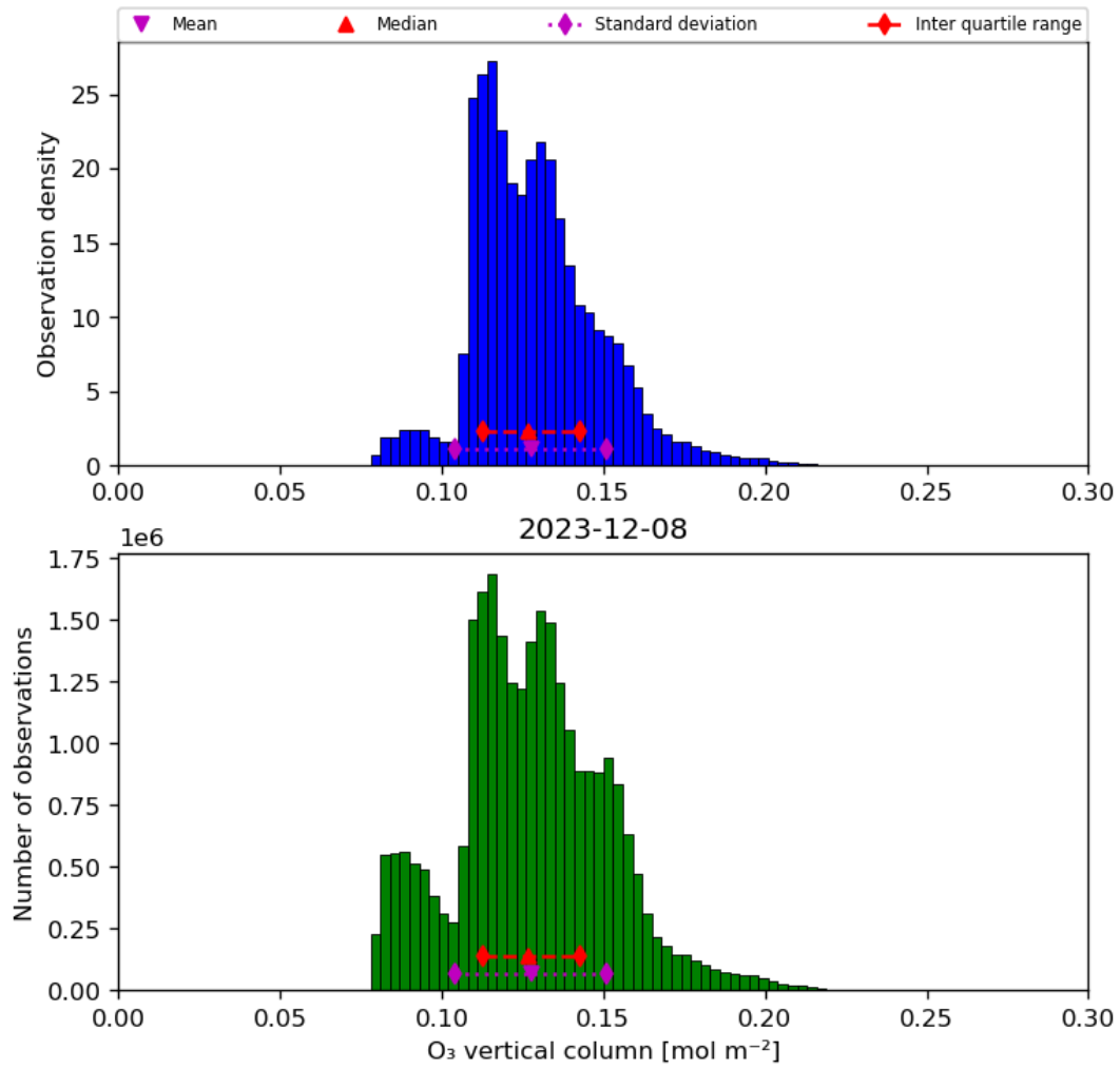
Figure 21: Histogram of “O 3 vertical column” for 2023-12-07 to 2023-12-09
