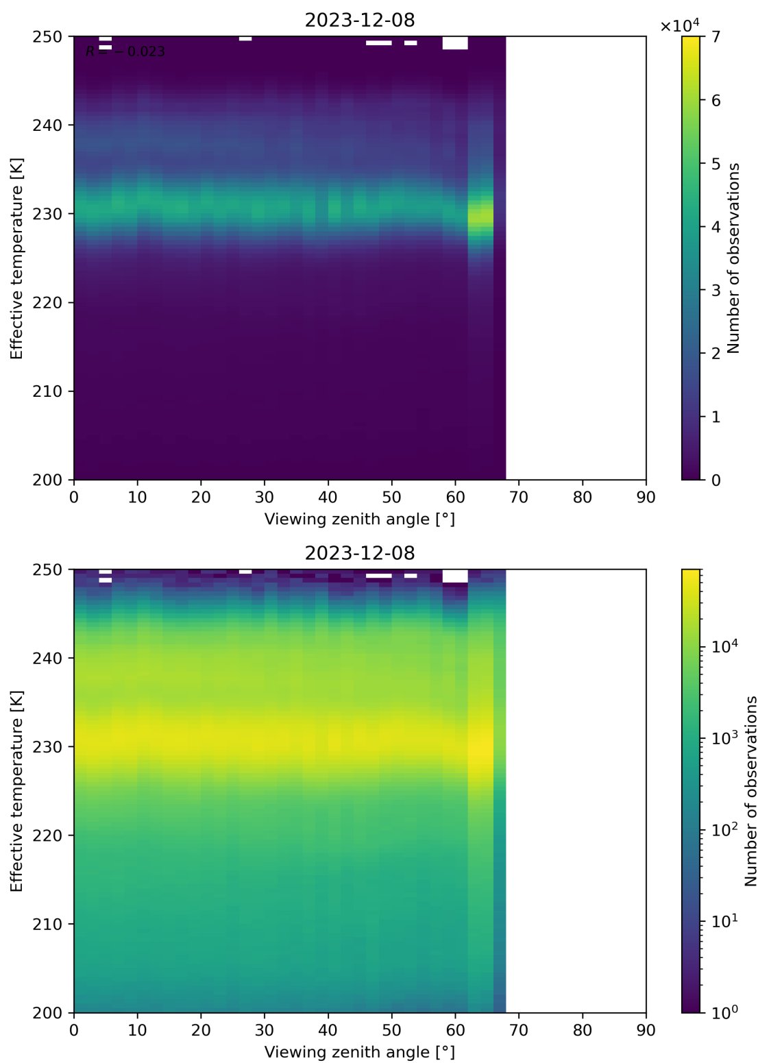
Figure 50: Scatter density plot of “Viewing zenith angle” against “Effective temperature” for 2023-12-07 to 2023-12-09.
