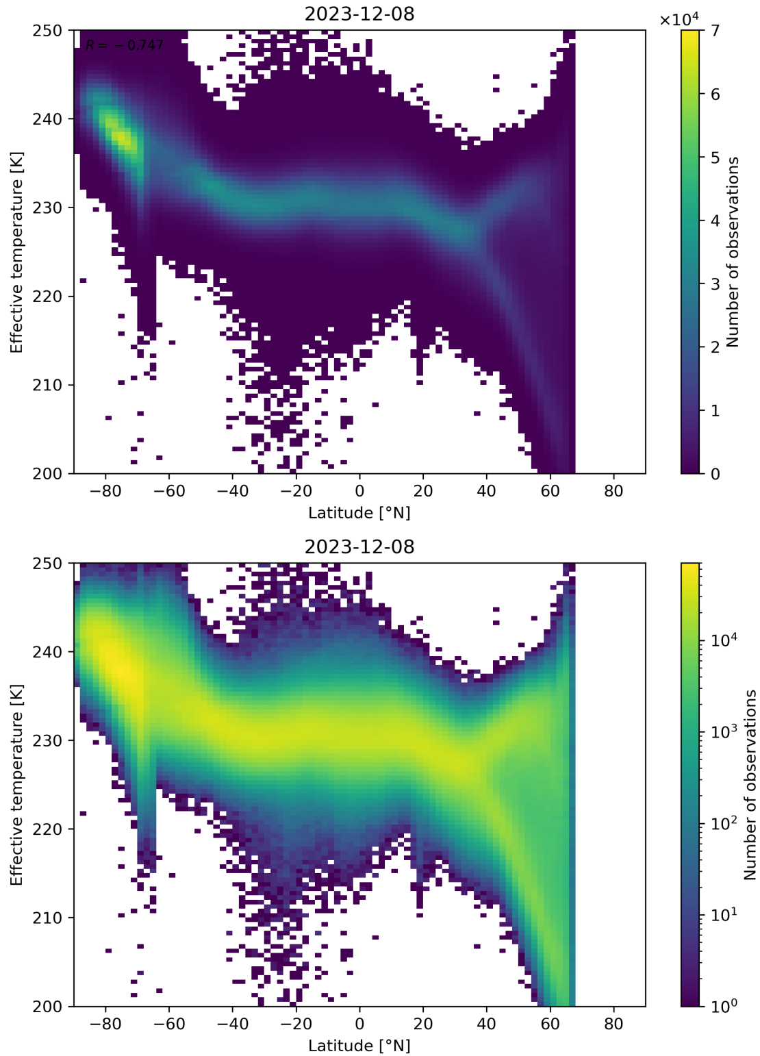
Figure 34: Scatter density plot of “Latitude” against “Effective temperature” for 2023-12-07 to 2023-12-09.
