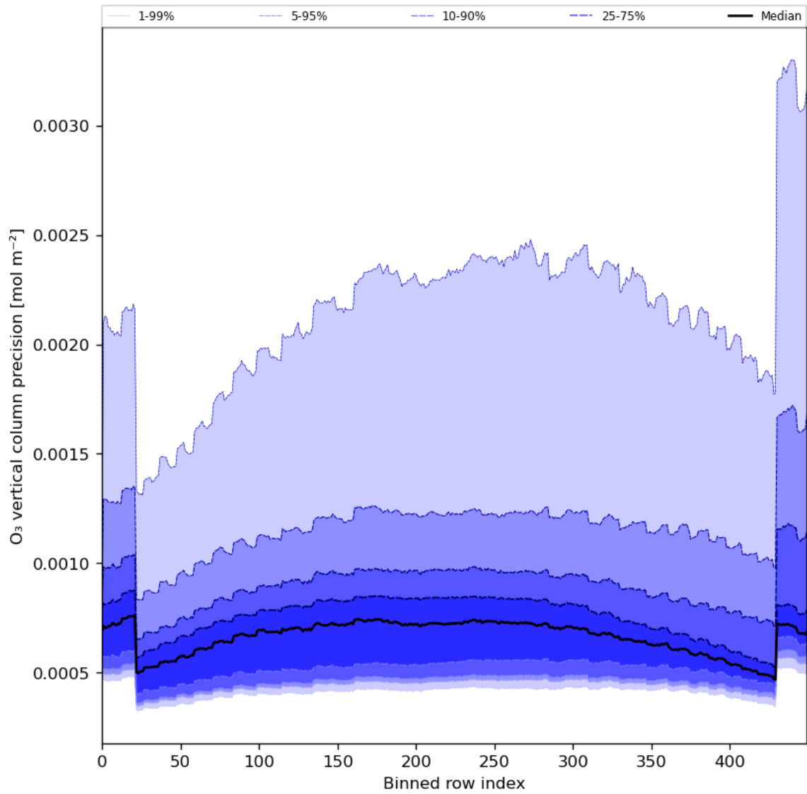
Figure 29: Along track statistics of “O 3 vertical column precision” for 2023-12-07 to 2023-12-09
