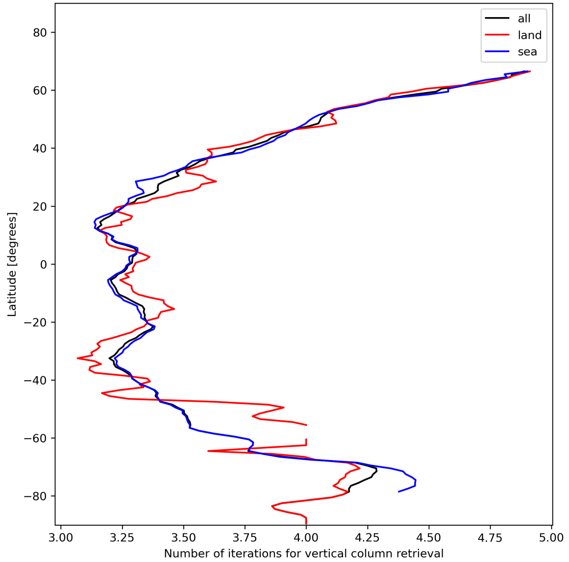
Figure 19: Zonal average of “Number of iterations for vertical column retrieval” for 2023-12-07 to 2023-12-09.
