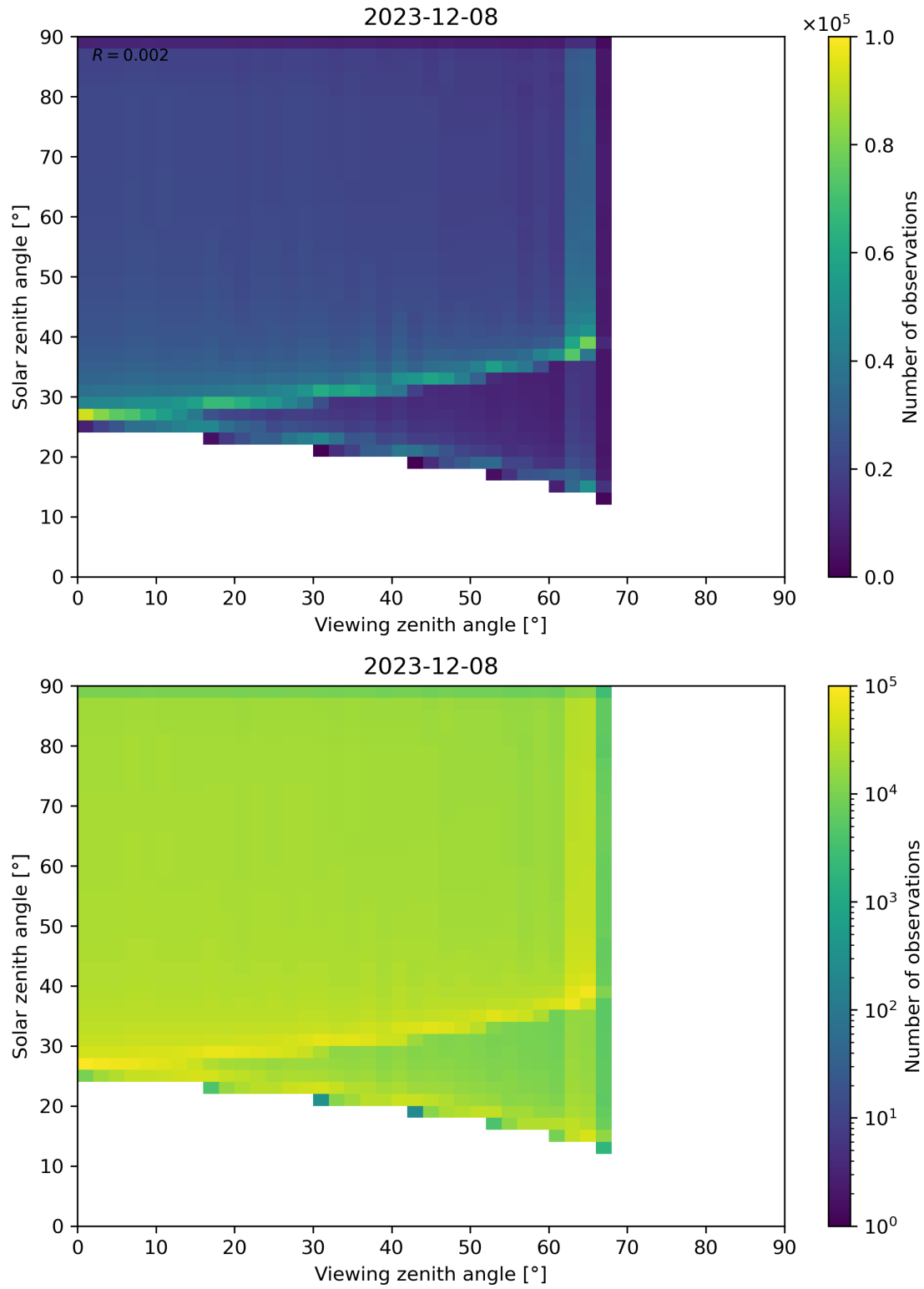
Figure 54: Scatter density plot of “Viewing zenith angle” against “Solar zenith angle” for 2023-12-07 to 2023-12-09.
