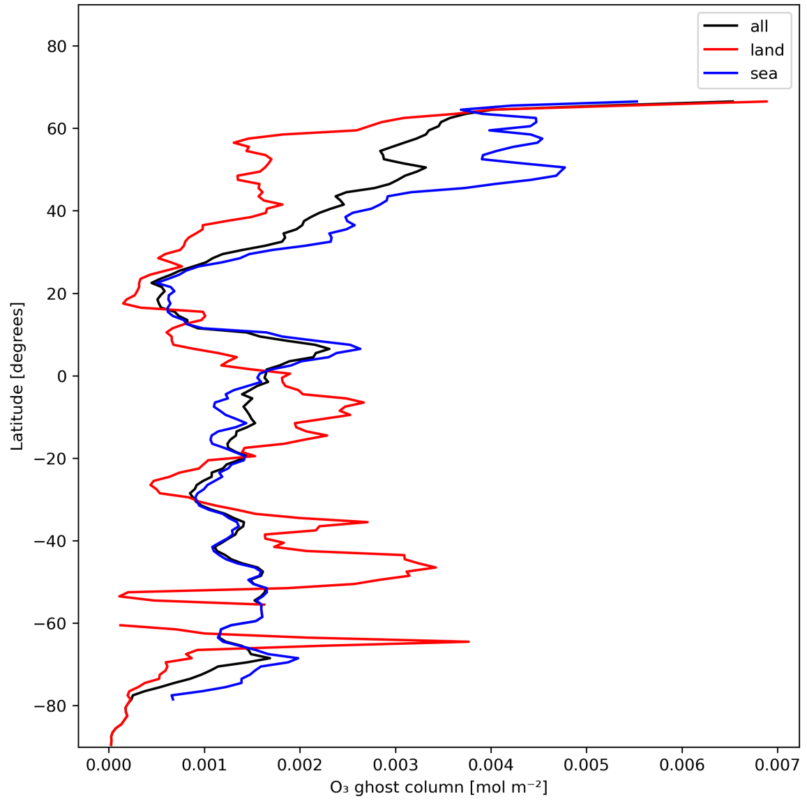
Figure 18: Zonal average of “O 3 ghost column” for 2023-12-07 to 2023-12-09.
