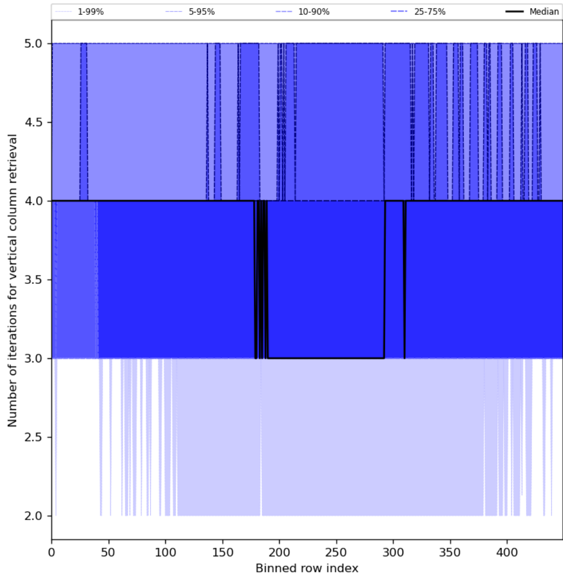
Figure 33: Along track statistics of “Number of iterations for vertical column retrieval” for 2023-12-07 to 2023-12-09
