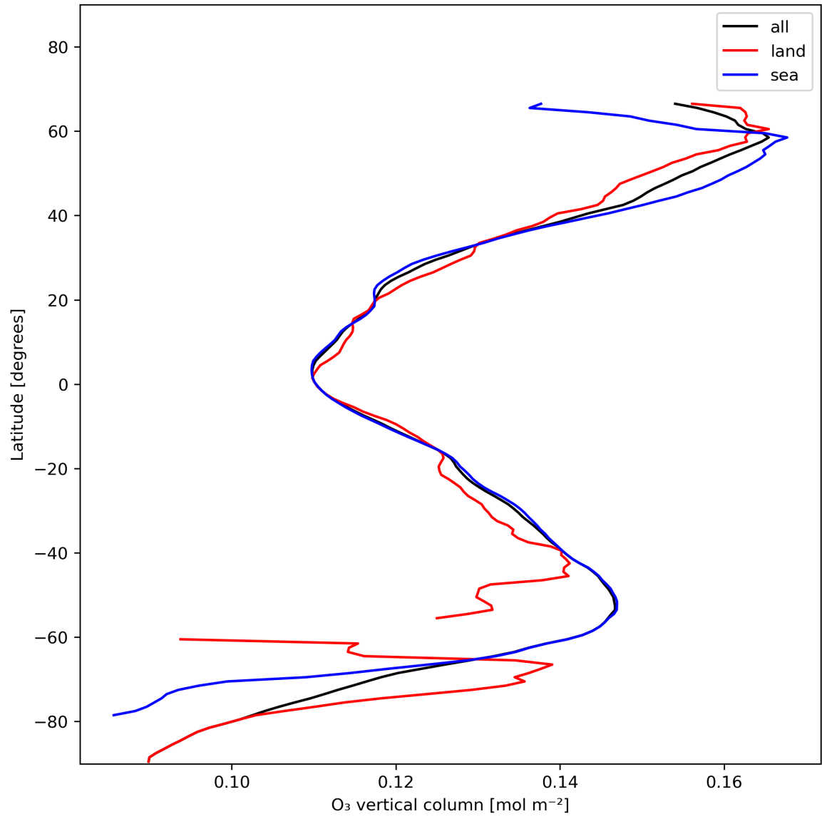
Figure 14: Zonal average of “O 3 vertical column” for 2023-12-07 to 2023-12-09.
