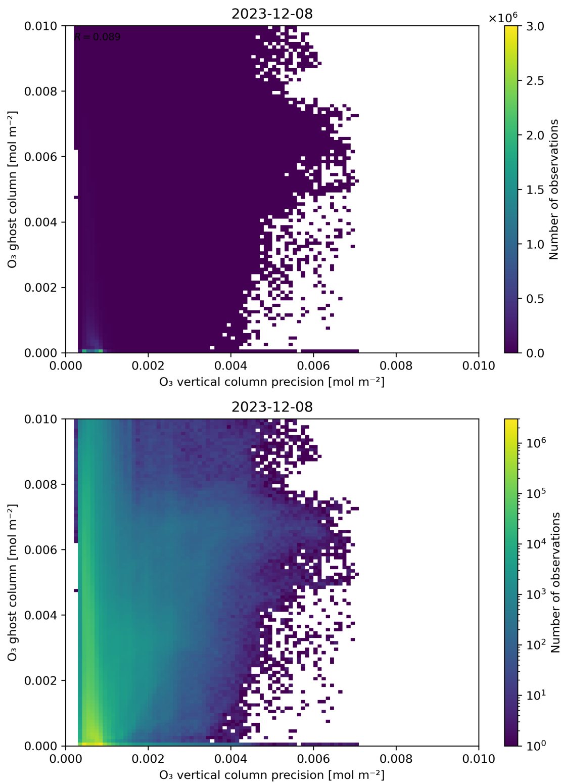
Figure 43: Scatter density plot of “ \text{O}_3 vertical column precision” against “ \text{O}_3 ghost column” for 2023-12-07 to 2023-12-09.
