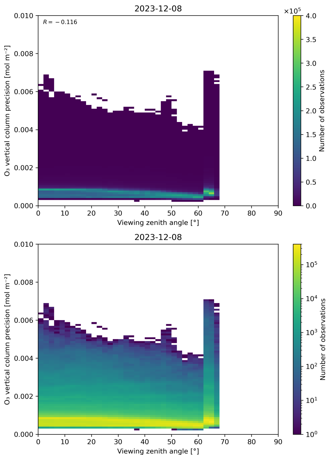
Figure 53: Scatter density plot of “Viewing zenith angle” against “O 3 vertical column precision” for 2023-12-07 to 2023-12-09.
