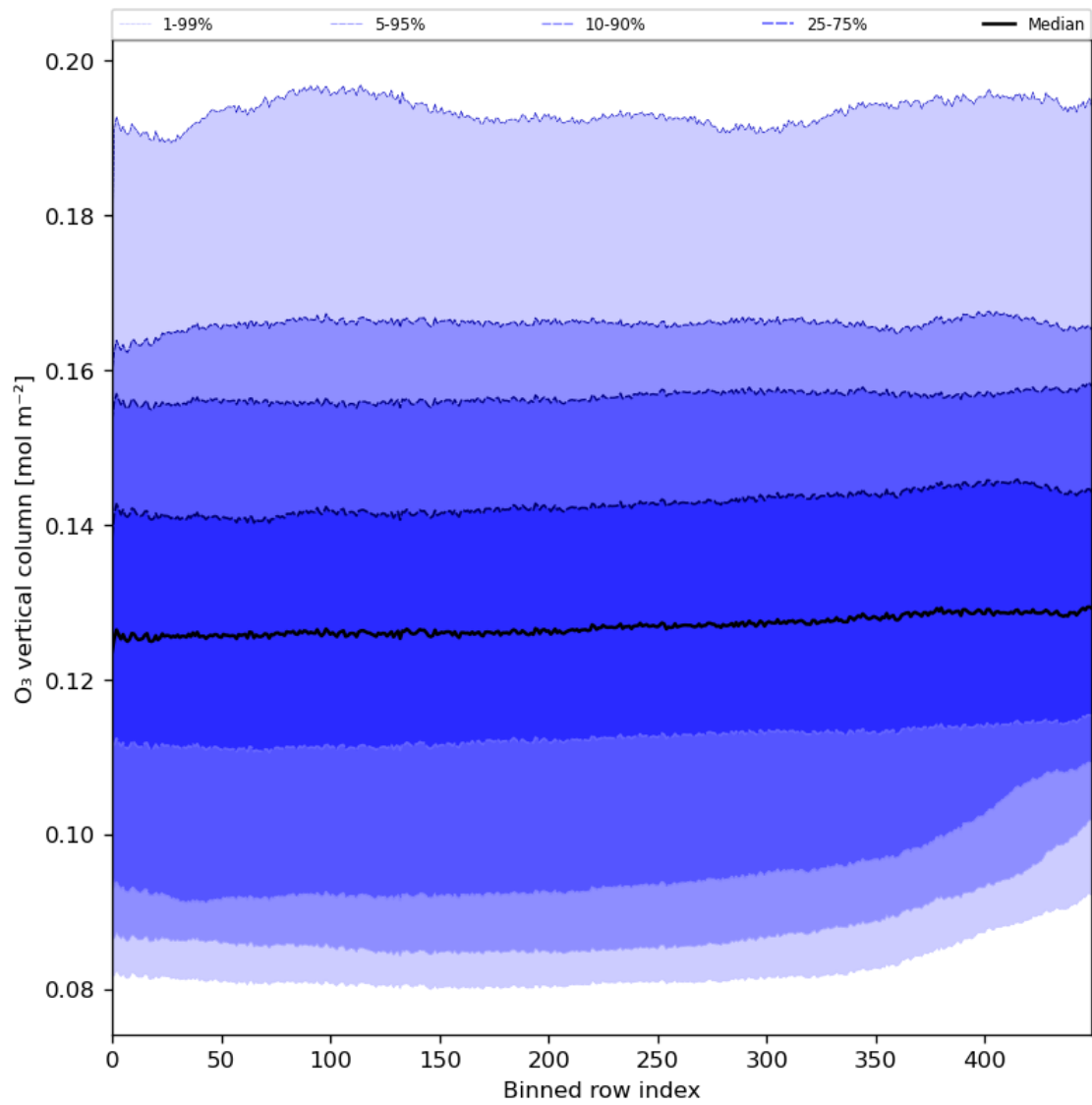
Figure 28: Along track statistics of “O 3 vertical column” for 2023-12-07 to 2023-12-09
