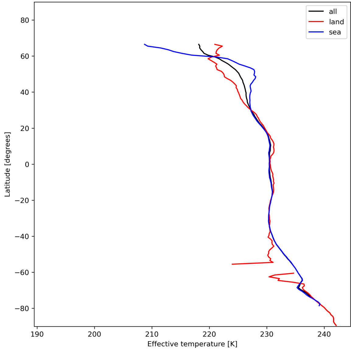
Figure 17: Zonal average of "Effective temperature" for 2023-12-07 to 2023-12-09.
