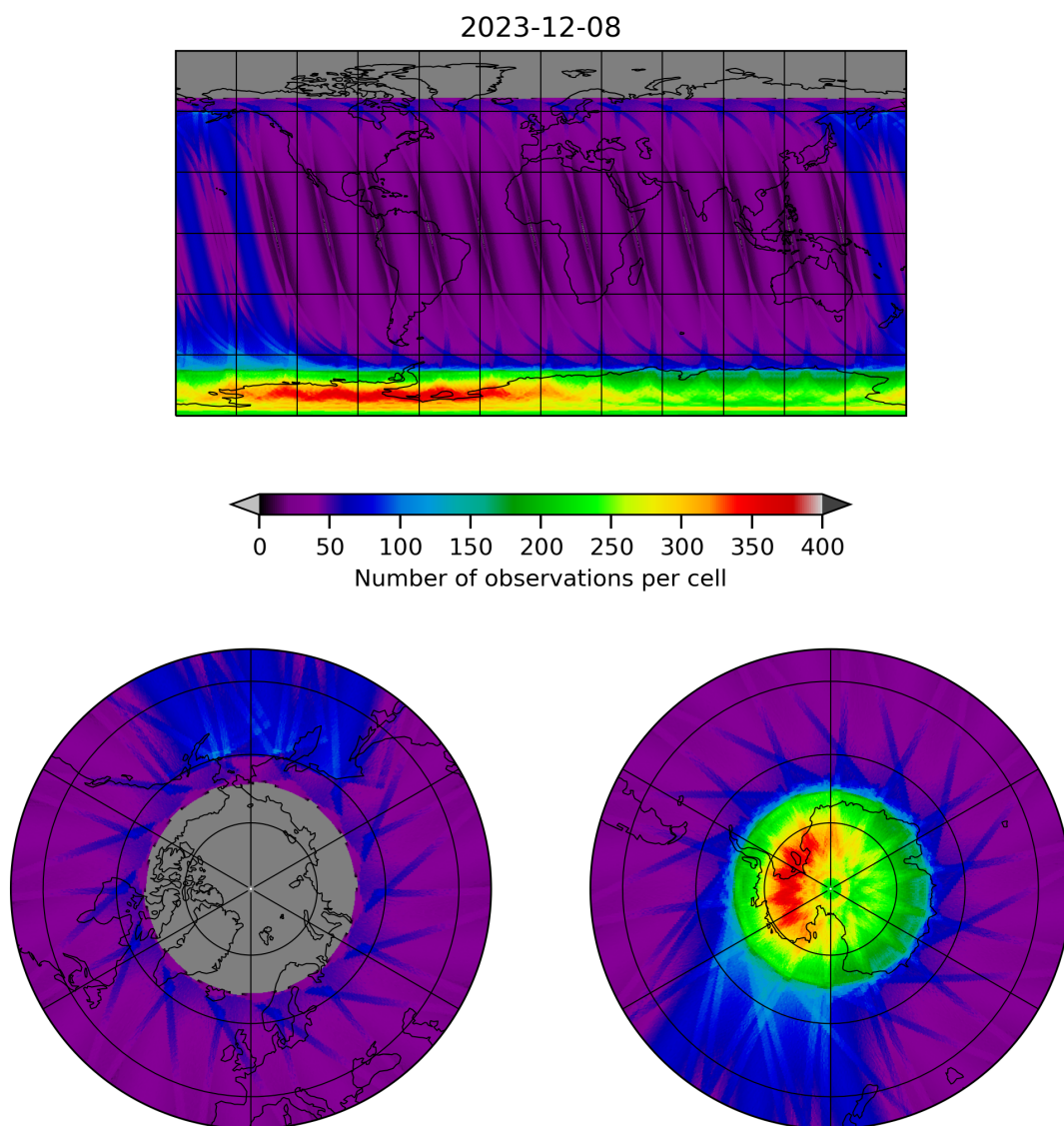
Figure 12: Map of the number of observations for 2023-12-07 to 2023-12-09
