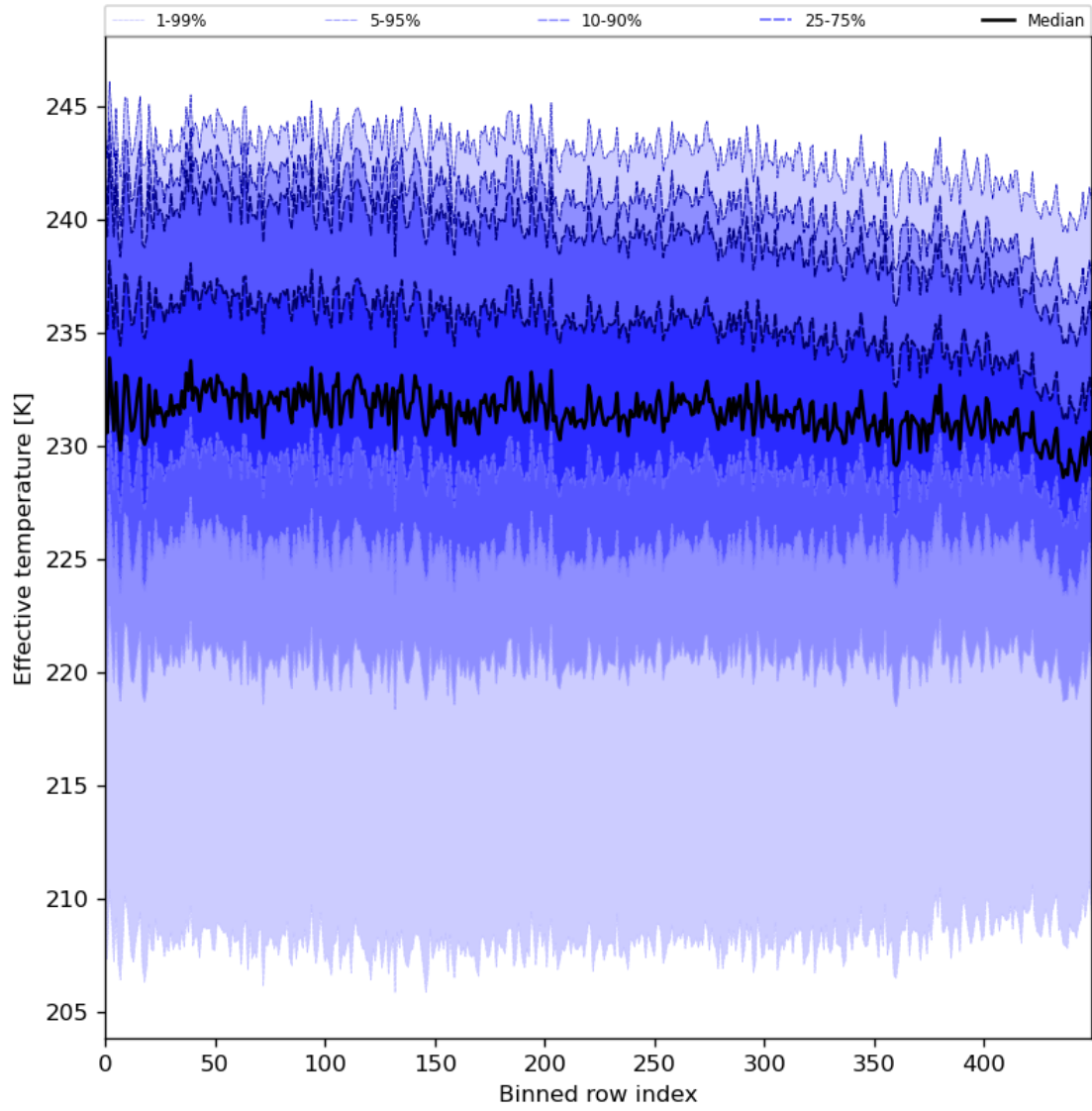
Figure 31: Along track statistics of “Effective temperature” for 2023-12-07 to 2023-12-09
