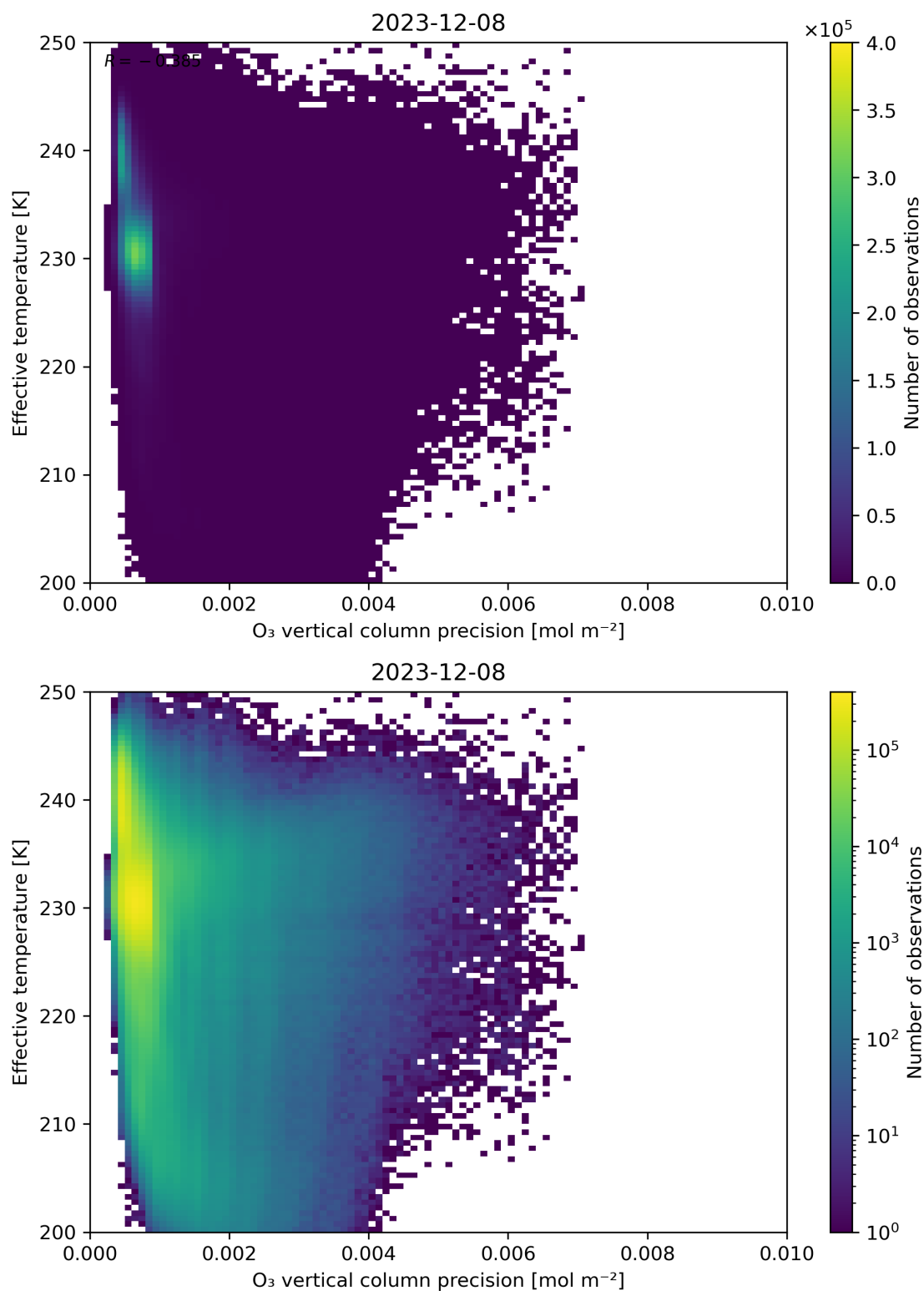
Figure 42: Scatter density plot of “O 3 vertical column precision” against “Effective temperature” for 2023-12-07 to 2023-12-09.
