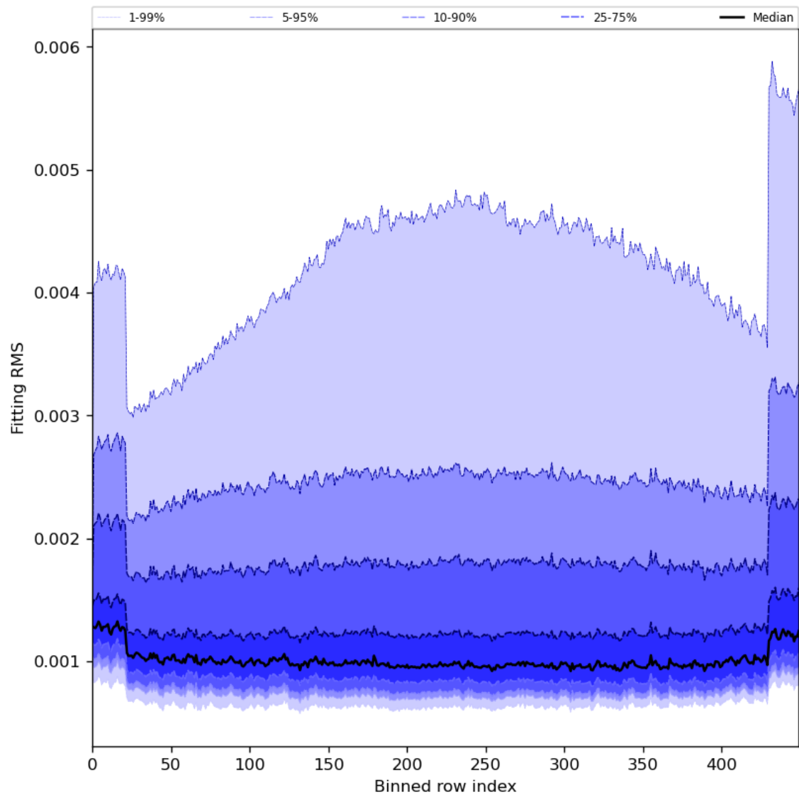
Figure 30: Along track statistics of “Fitting RMS” for 2023-12-07 to 2023-12-09
