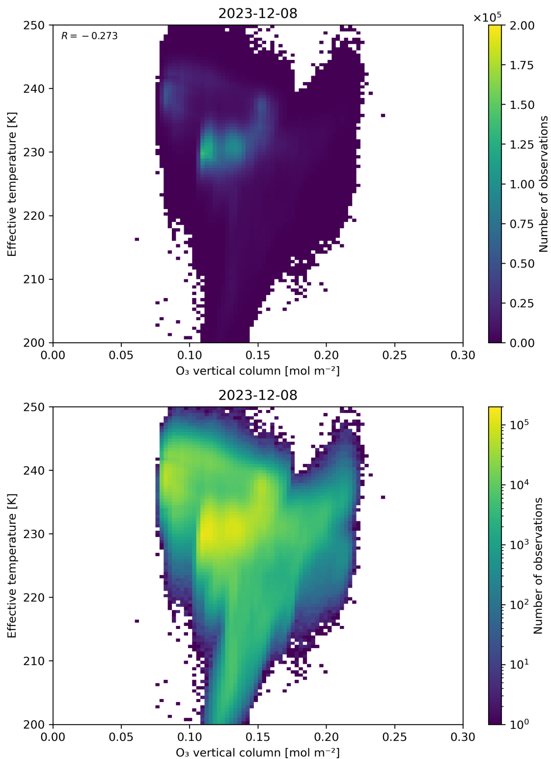
Figure 39: Scatter density plot of “O 3 vertical column” against “Effective temperature” for 2023-12-07 to 2023-12-09.
