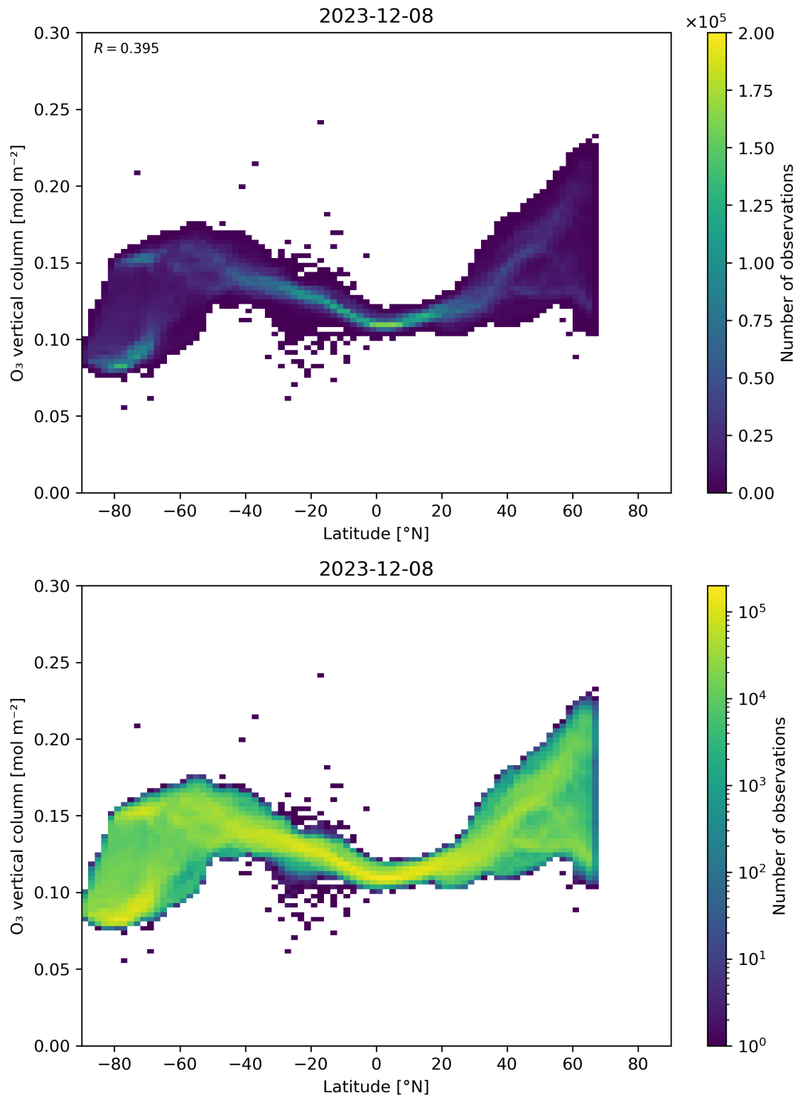
Figure 36: Scatter density plot of “Latitude” against “O 3 vertical column” for 2023-12-07 to 2023-12-09.
