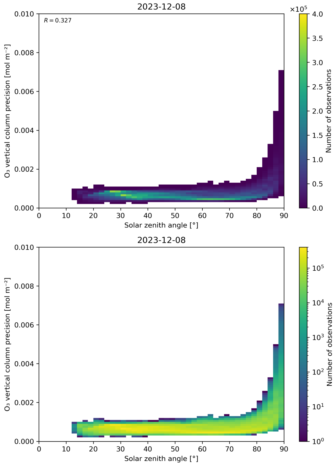
Figure 48: Scatter density plot of “Solar zenith angle” against “O 3 vertical column precision” for 2023-12-07 to 2023-12-09.
