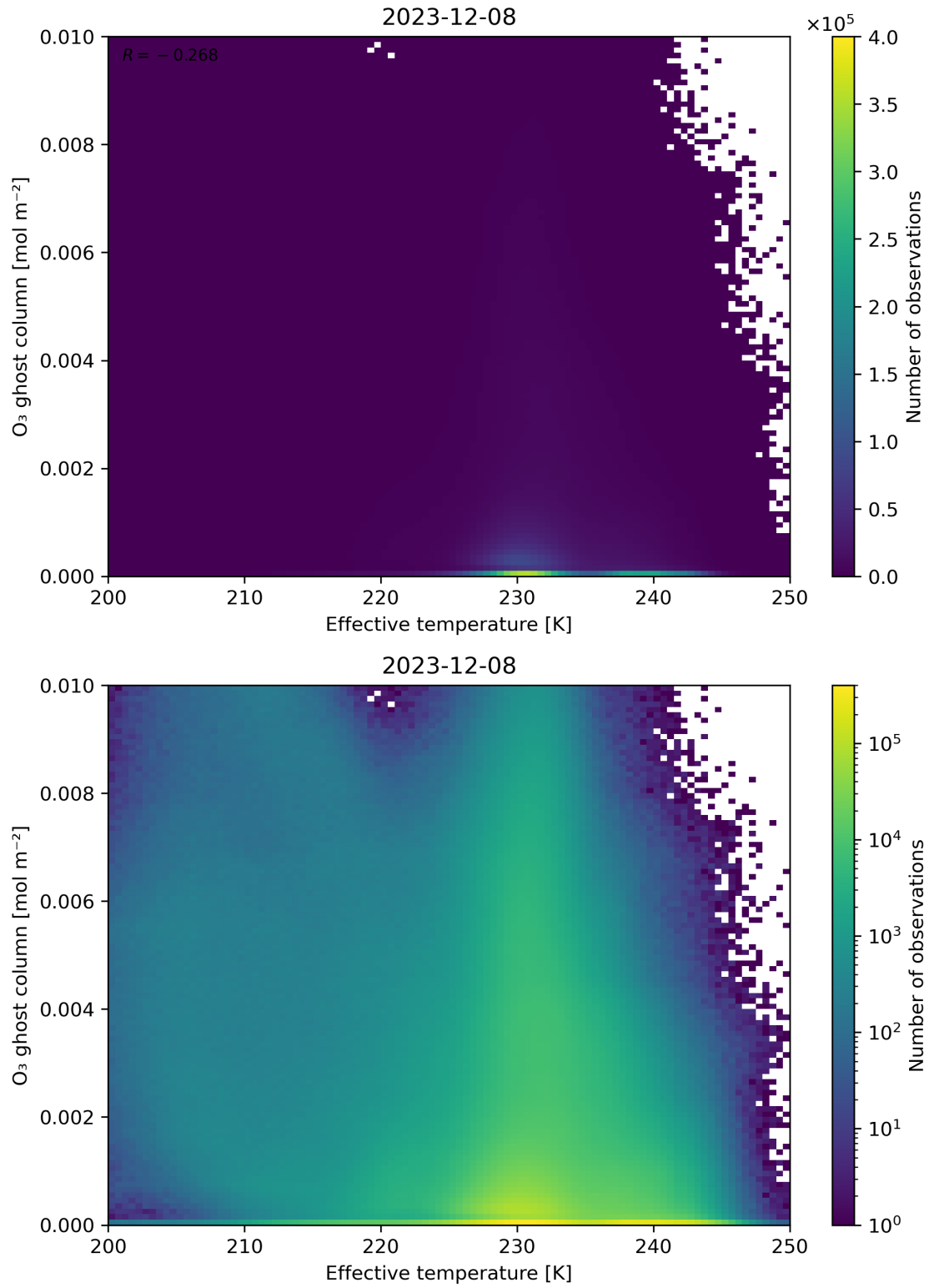
Figure 38: Scatter density plot of “Effective temperature” against “O 3 ghost column” for 2023-12-07 to 2023-12-09.
