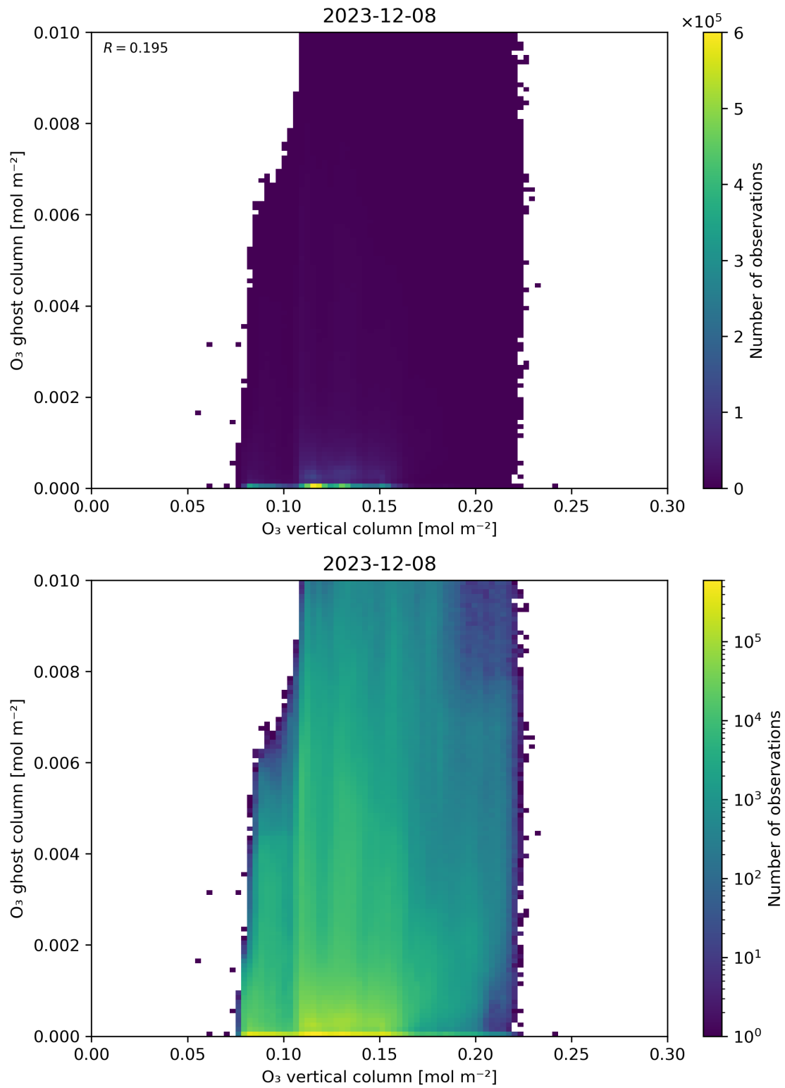
Figure 40: Scatter density plot of “O 3 vertical column” against “O 3 ghost column” for 2023-12-07 to 2023-12-09.
