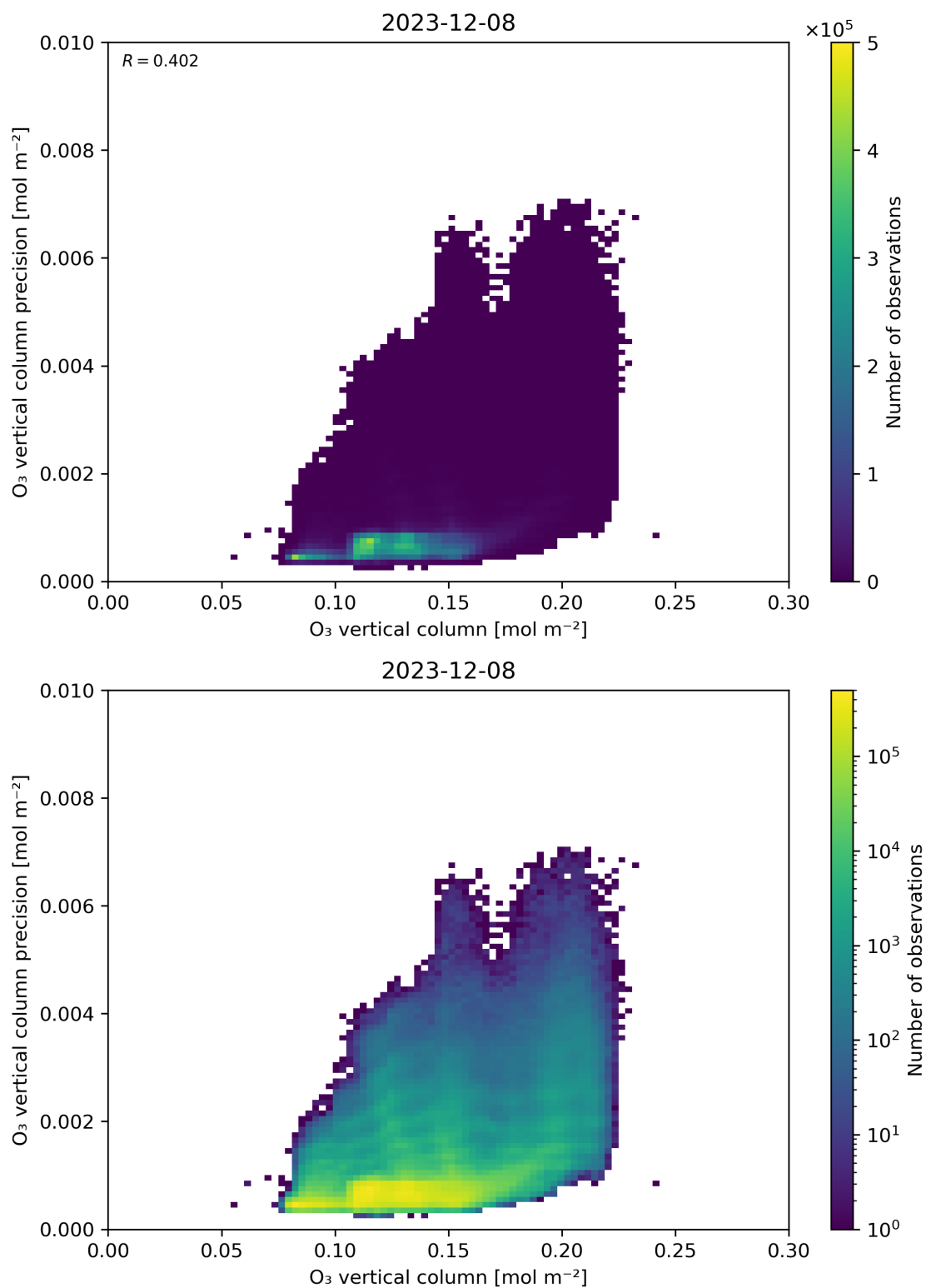
Figure 41: Scatter density plot of “O 3 vertical column” against “O 3 vertical column precision” for 2023-12-07 to 2023-12-09.
