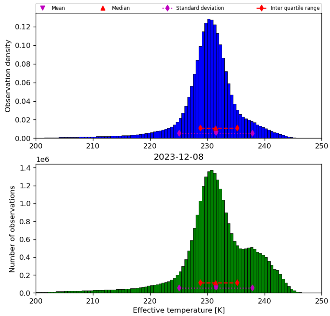
Figure 24: Histogram of “Effective temperature” for 2023-12-07 to 2023-12-09
