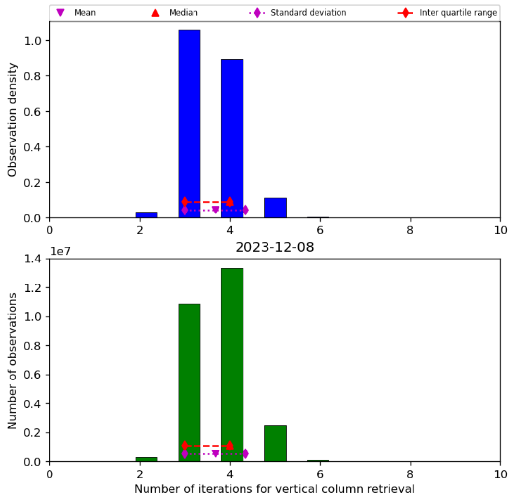
Figure 26: Histogram of “Number of iterations for vertical column retrieval” for 2023-12-07 to 2023-12-09
