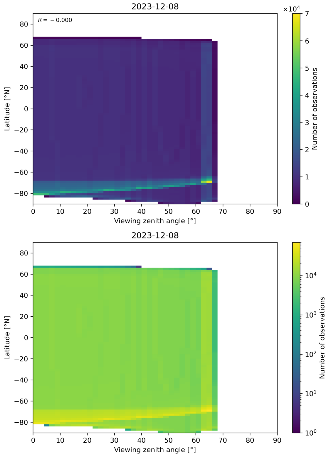
Figure 49: Scatter density plot of “Viewing zenith angle” against “Latitude” for 2023-12-07 to 2023-12-09.
