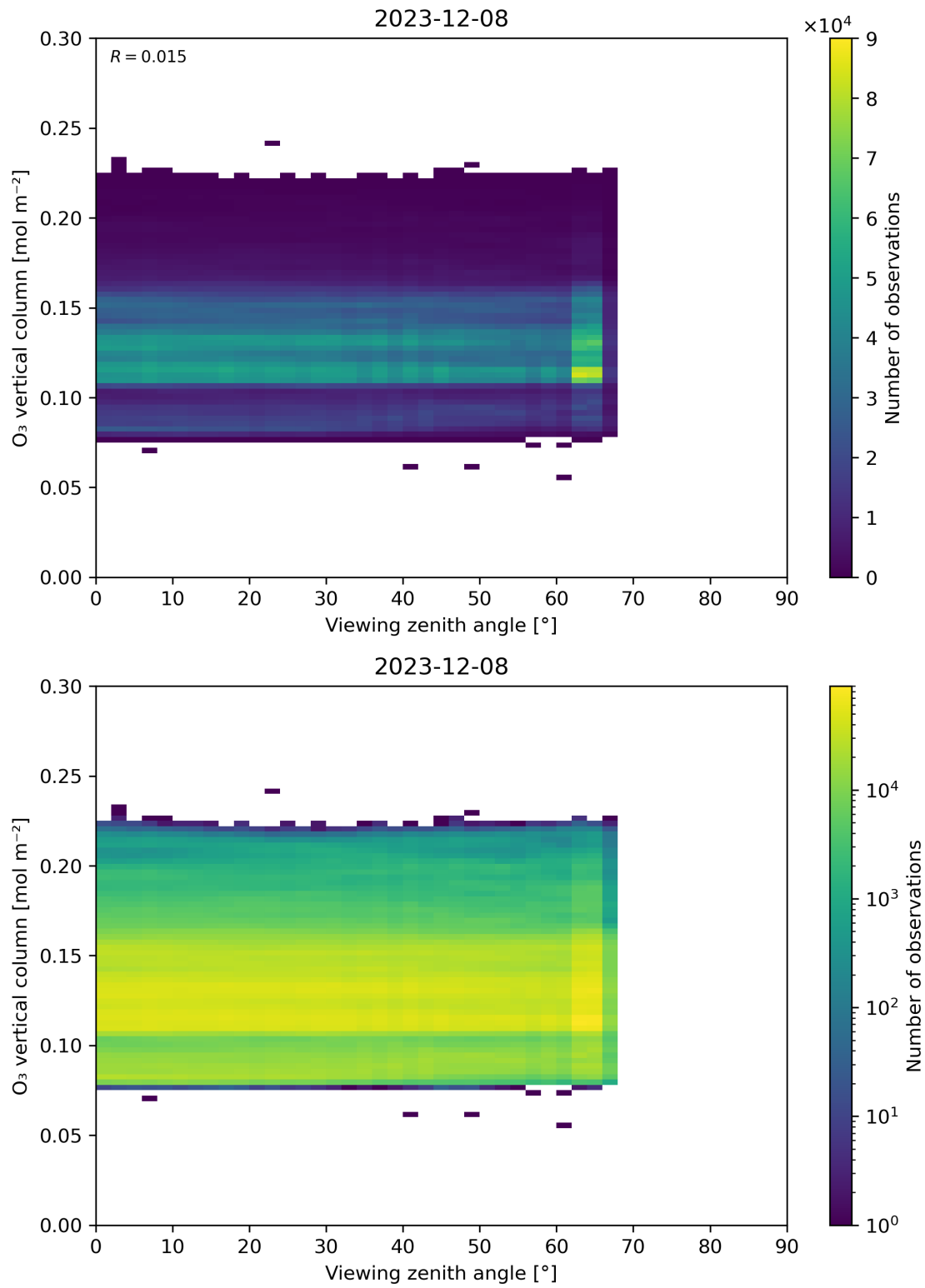
Figure 52: Scatter density plot of “Viewing zenith angle” against “O 3 vertical column” for 2023-12-07 to 2023-12-09.
