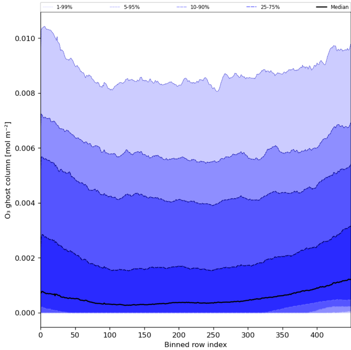
Figure 32: Along track statistics of “O 3 ghost column” for 2023-12-07 to 2023-12-09
