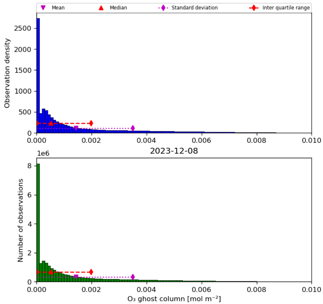
Figure 25: Histogram of “O 3 ghost column” for 2023-12-07 to 2023-12-09
