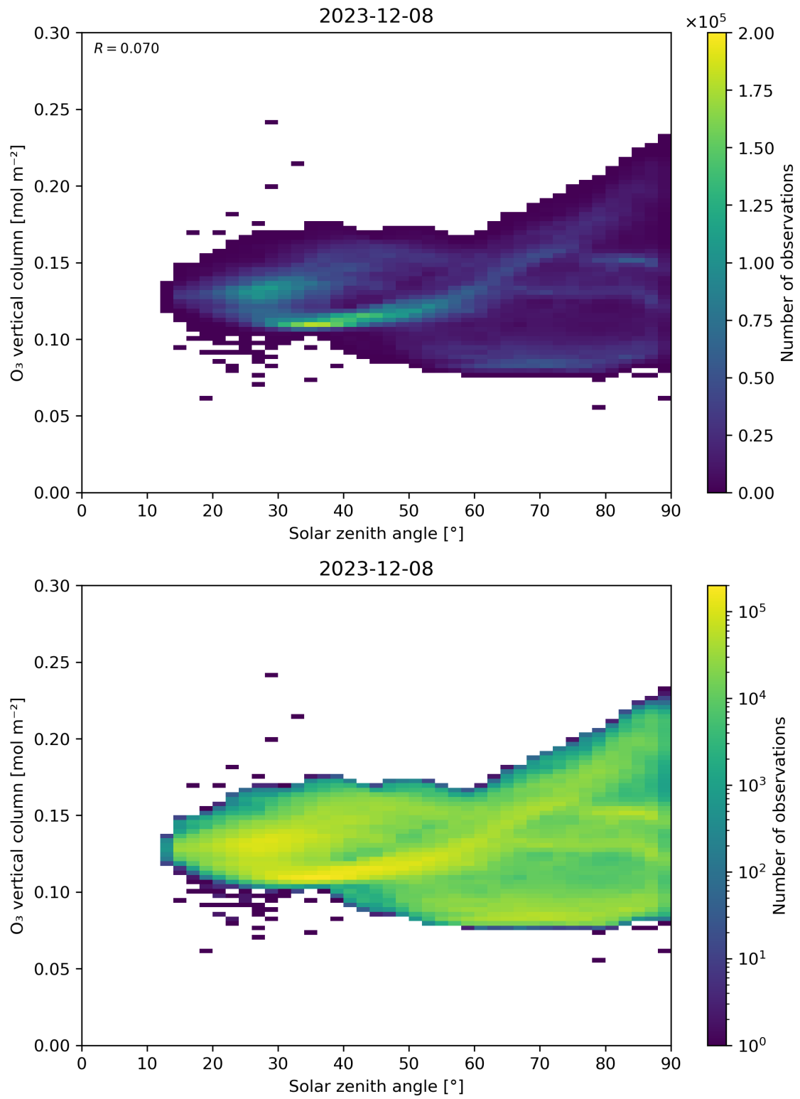
Figure 47: Scatter density plot of “Solar zenith angle” against “O 3 vertical column” for 2023-12-07 to 2023-12-09.
