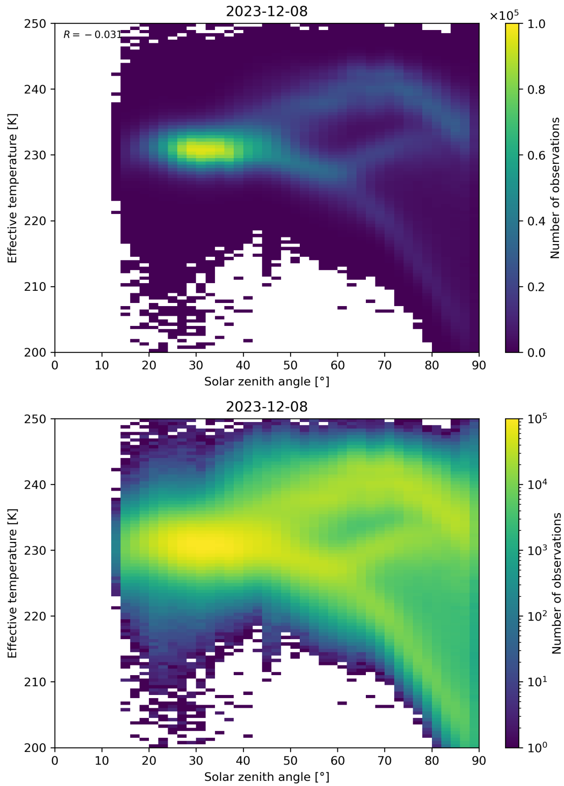
Figure 45: Scatter density plot of “Solar zenith angle” against “Effective temperature” for 2023-12-07 to 2023-12-09.
