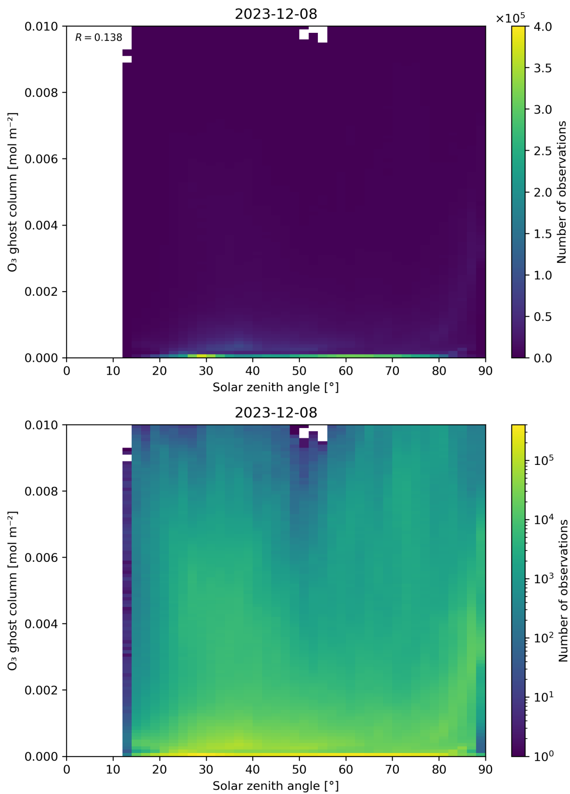
Figure 46: Scatter density plot of “Solar zenith angle” against “O 3 ghost column” for 2023-12-07 to 2023-12-09.
