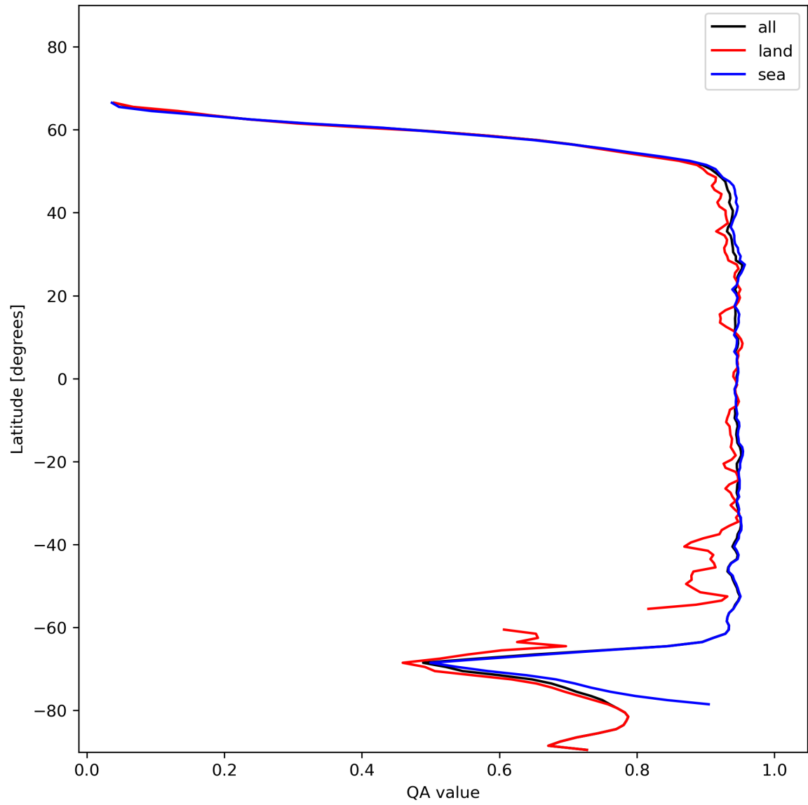
Figure 13: Zonal average of “QA value” for 2023-12-07 to 2023-12-09.
