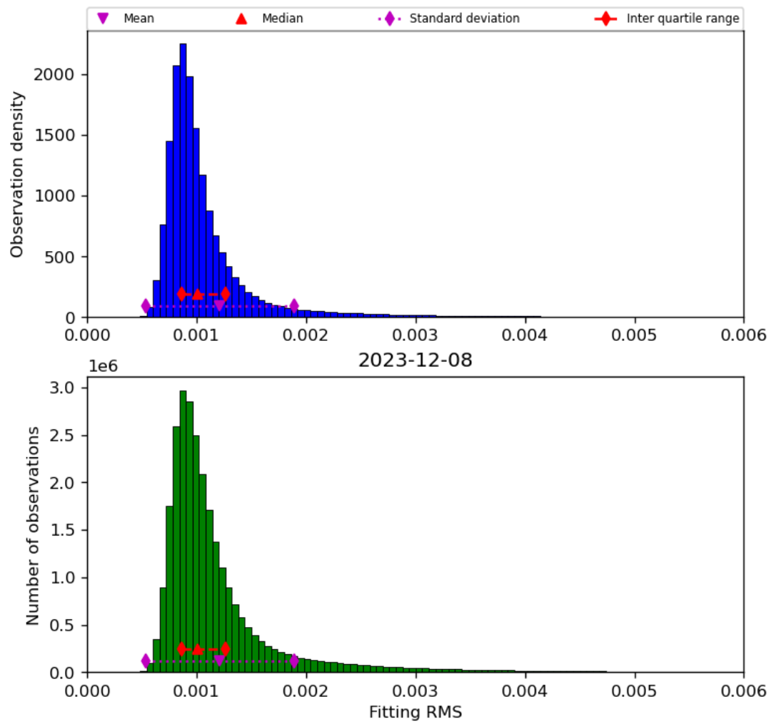
Figure 23: Histogram of “Fitting RMS” for 2023-12-07 to 2023-12-09
