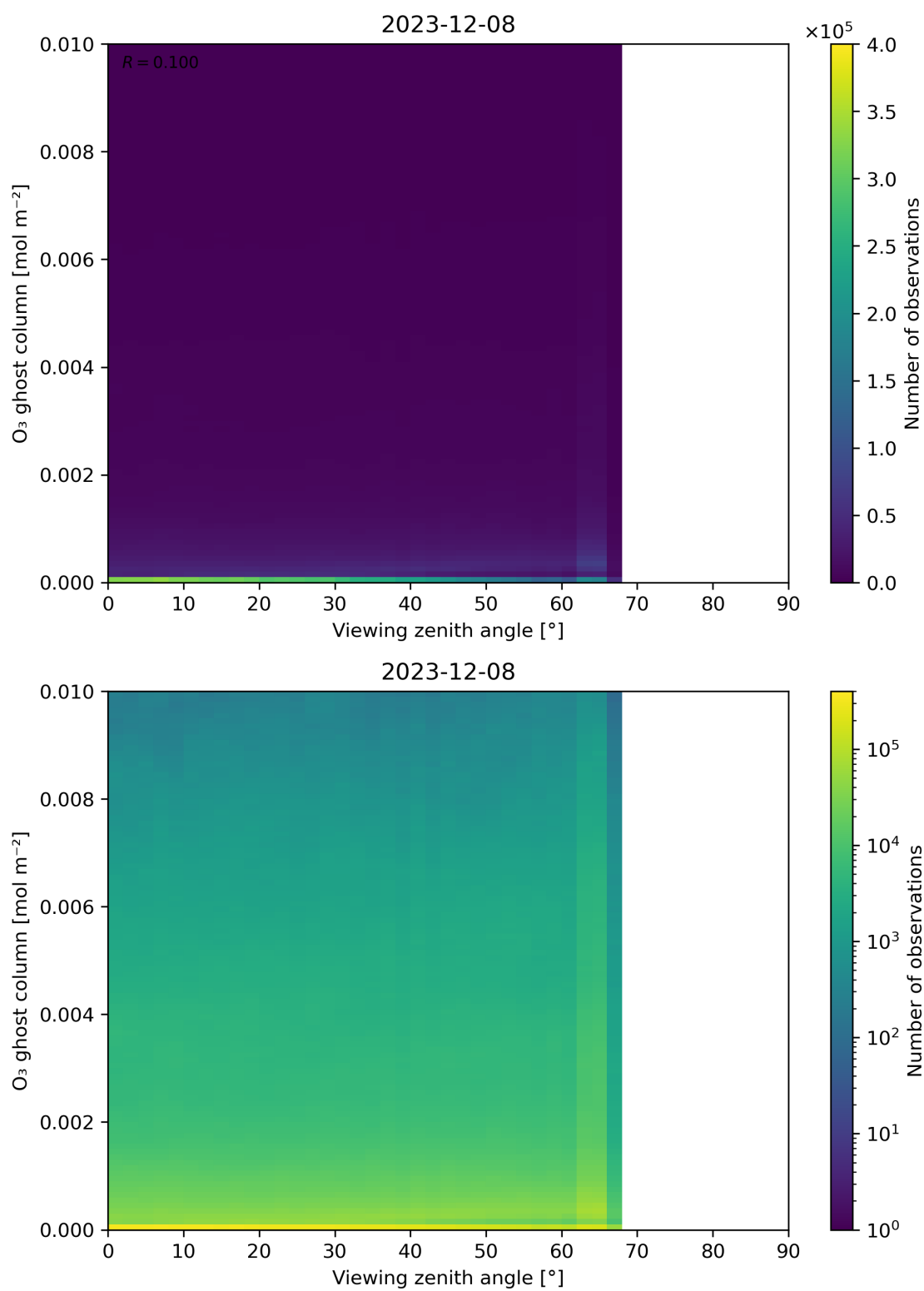
Figure 51: Scatter density plot of “Viewing zenith angle” against “O 3 ghost column” for 2023-12-07 to 2023-12-09.
