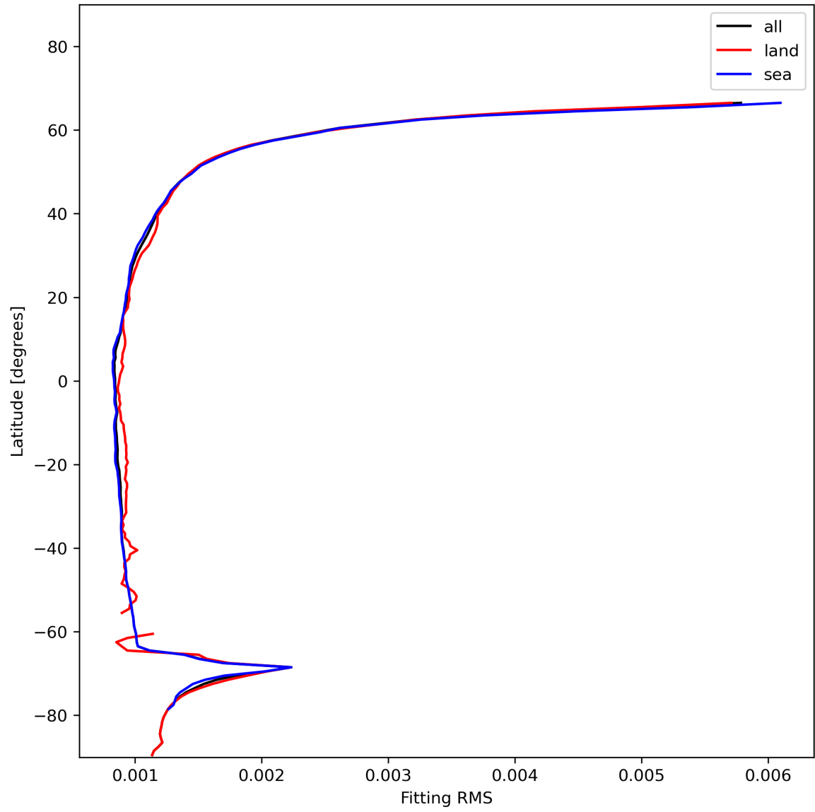
Figure 16: Zonal average of “Fitting RMS” for 2023-12-07 to 2023-12-09.
