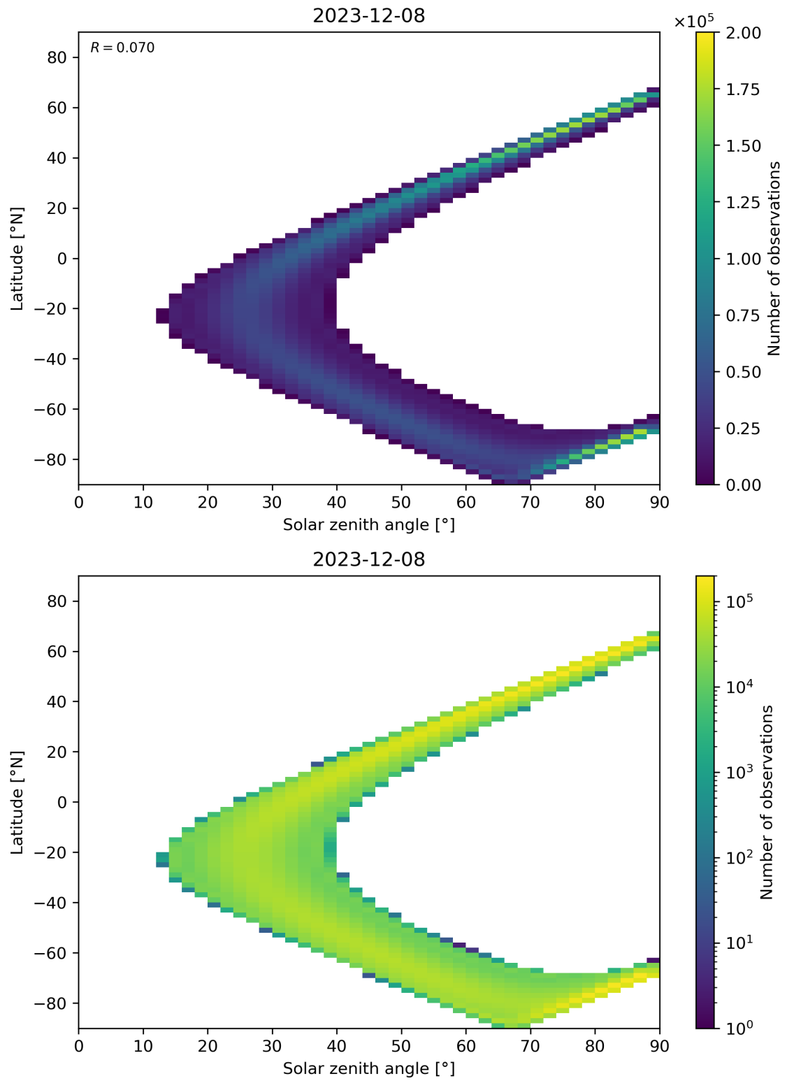
Figure 44: Scatter density plot of “Solar zenith angle” against “Latitude” for 2023-12-07 to 2023-12-09.
