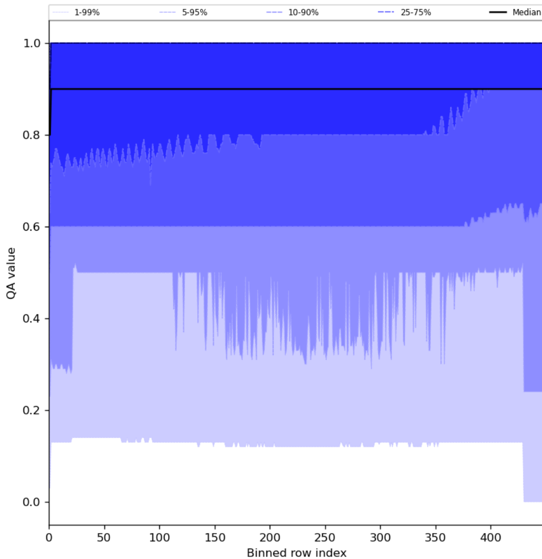
Figure 27: Along track statistics of “QA value” for 2023-12-07 to 2023-12-09
