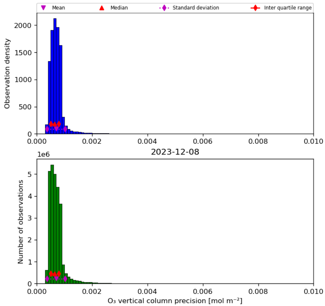
Figure 22: Histogram of “O 3 vertical column precision” for 2023-12-07 to 2023-12-09
