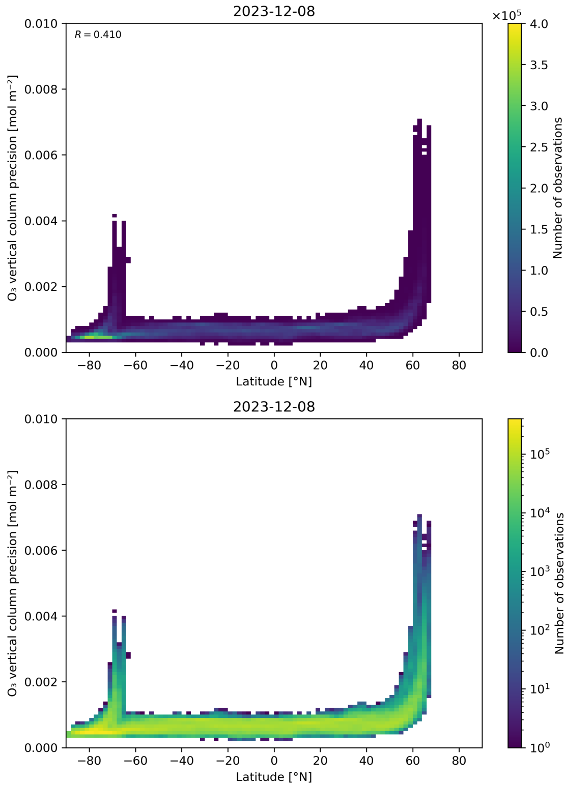
Figure 37: Scatter density plot of “Latitude” against “O 3 vertical column precision” for 2023-12-07 to 2023-12-09.
