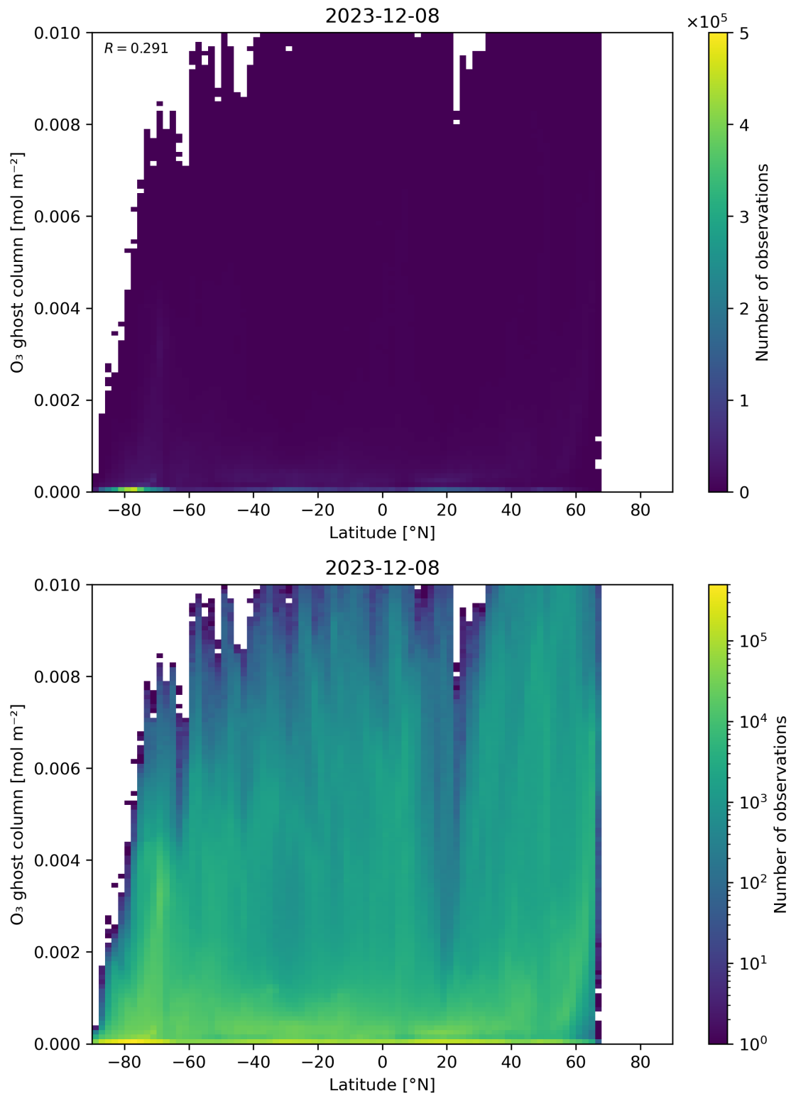
Figure 35: Scatter density plot of “Latitude” against “O 3 ghost column” for 2023-12-07 to 2023-12-09.
