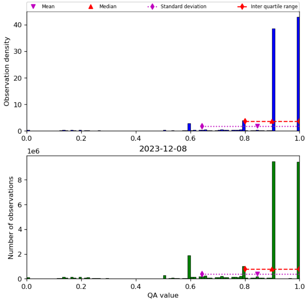
Figure 20: Histogram of “QA value” for 2023-12-07 to 2023-12-09
