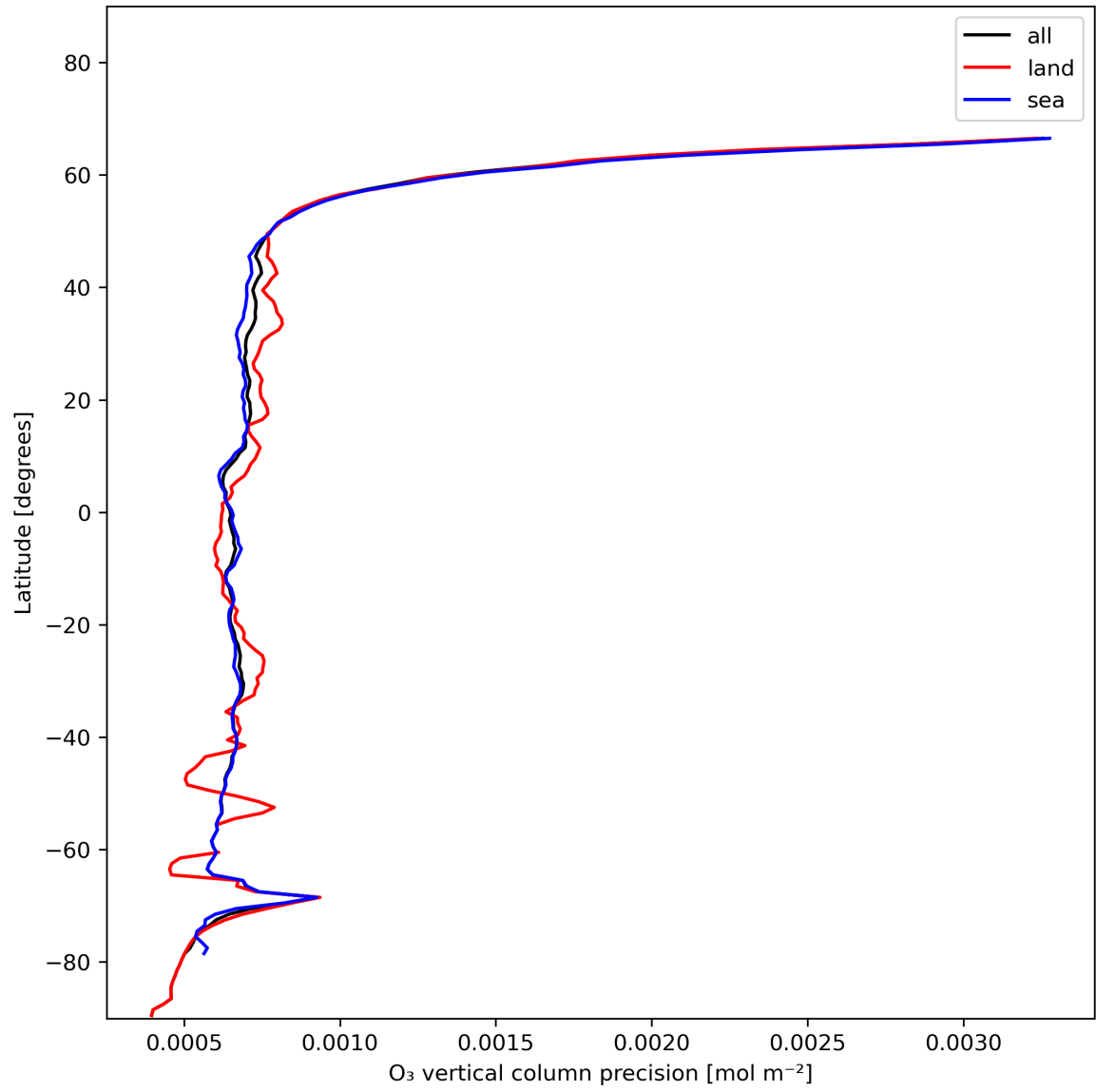
Figure 15: Zonal average of “O 3 vertical column precision” for 2023-12-07 to 2023-12-09.
