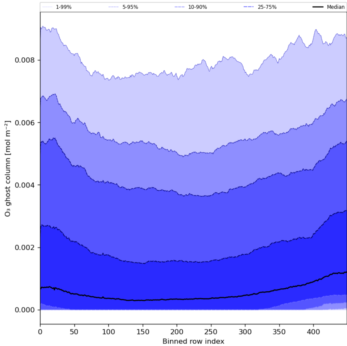
Figure 32: Along track statistics of “O 3 ghost column” for 2023-12-09 to 2023-12-10
