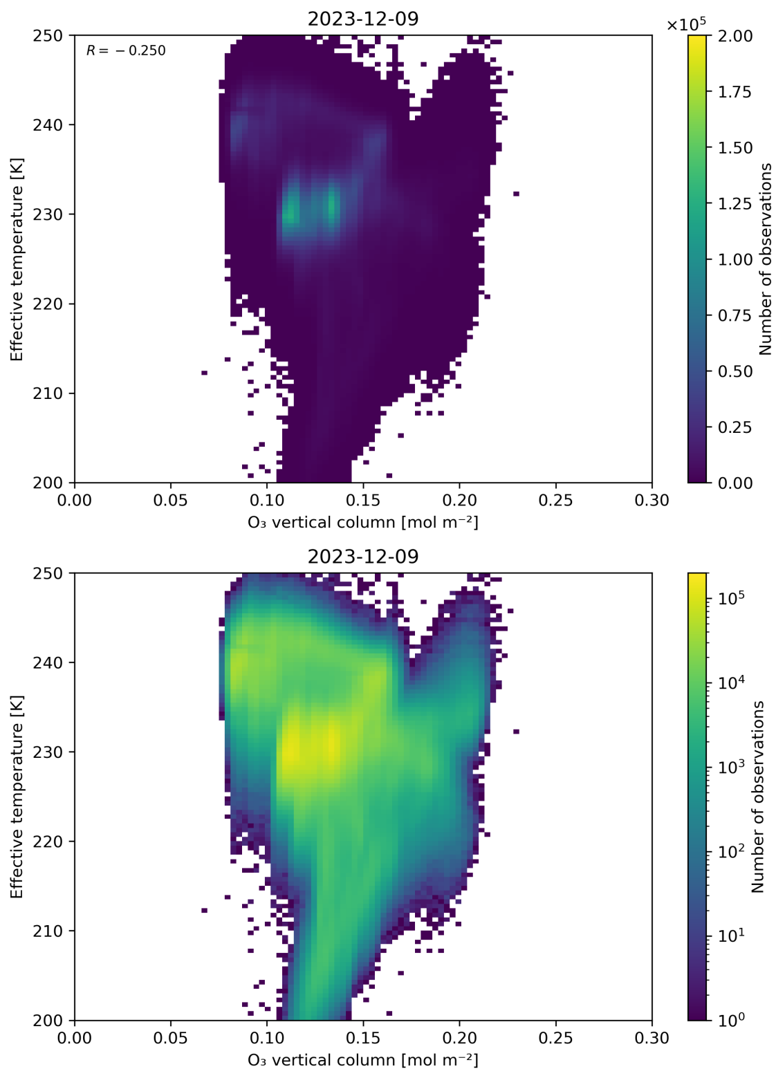
Figure 39: Scatter density plot of “O 3 vertical column” against “Effective temperature” for 2023-12-09 to 2023-12-10.
