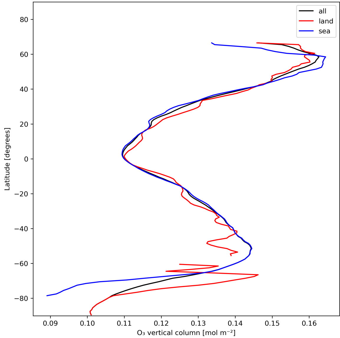
Figure 14: Zonal average of “O 3 vertical column” for 2023-12-09 to 2023-12-10.
