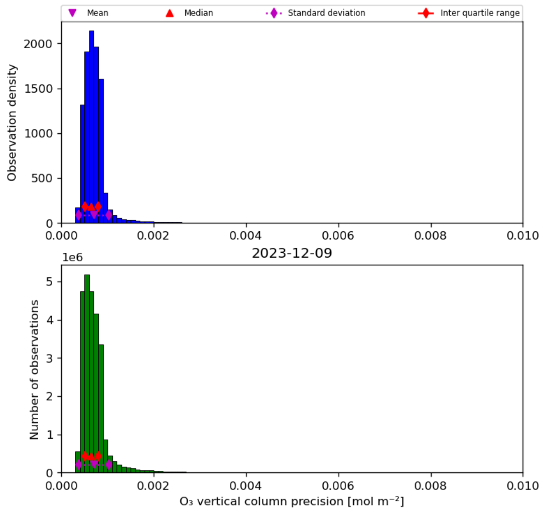
Figure 22: Histogram of “O 3 vertical column precision” for 2023-12-09 to 2023-12-10
