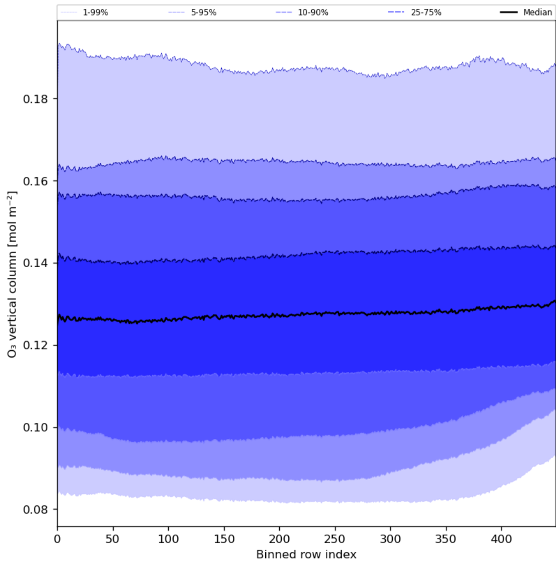
Figure 28: Along track statistics of “O 3 vertical column” for 2023-12-09 to 2023-12-10
