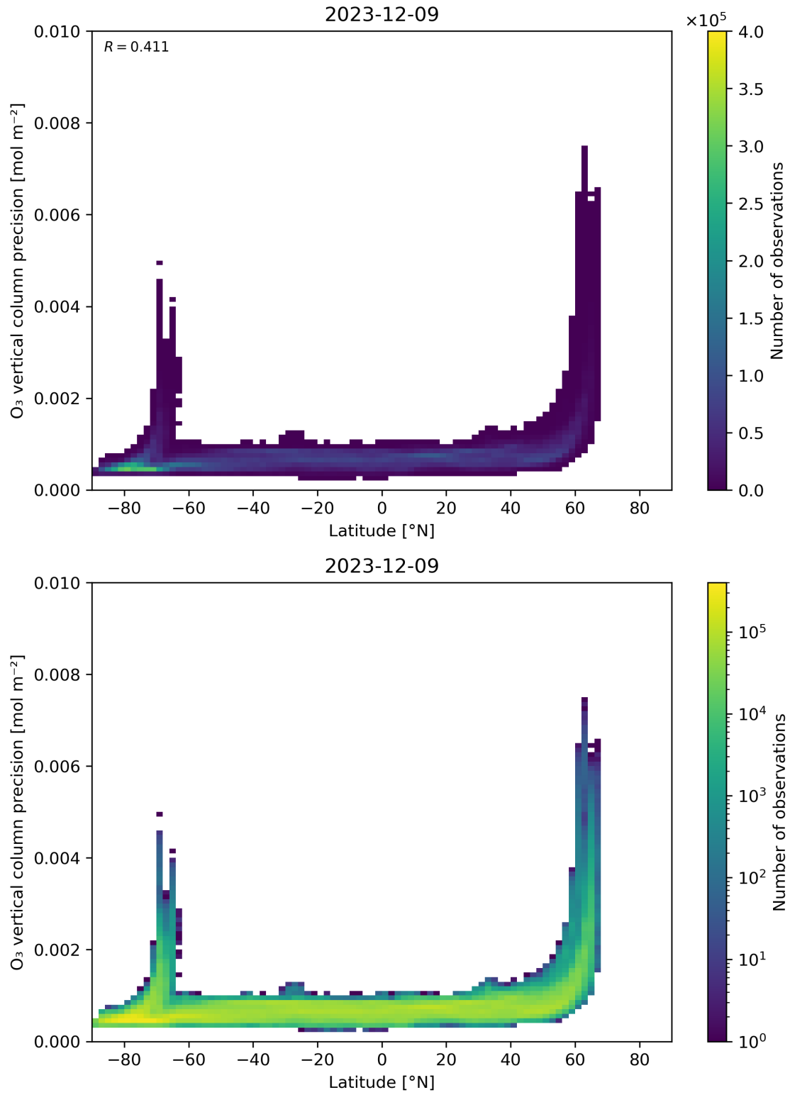
Figure 37: Scatter density plot of “Latitude” against “O 3 vertical column precision” for 2023-12-09 to 2023-12-10.
