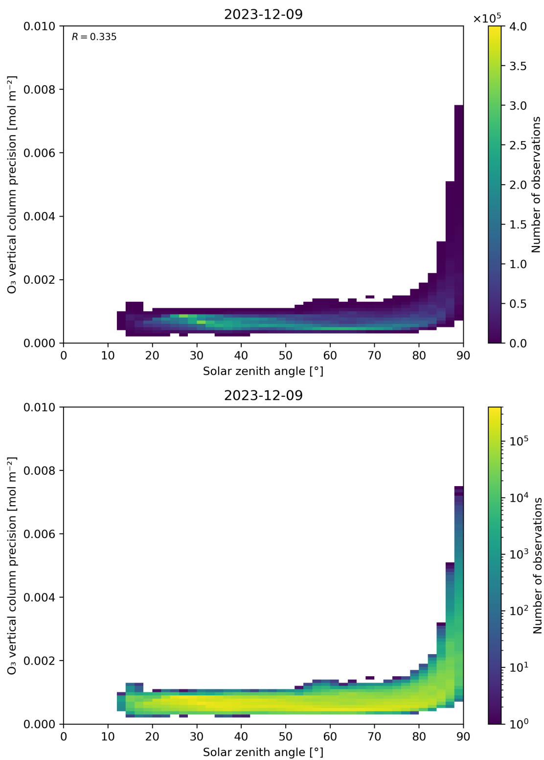
Figure 48: Scatter density plot of “Solar zenith angle” against “O 3 vertical column precision” for 2023-12-09 to 2023-12-10.
