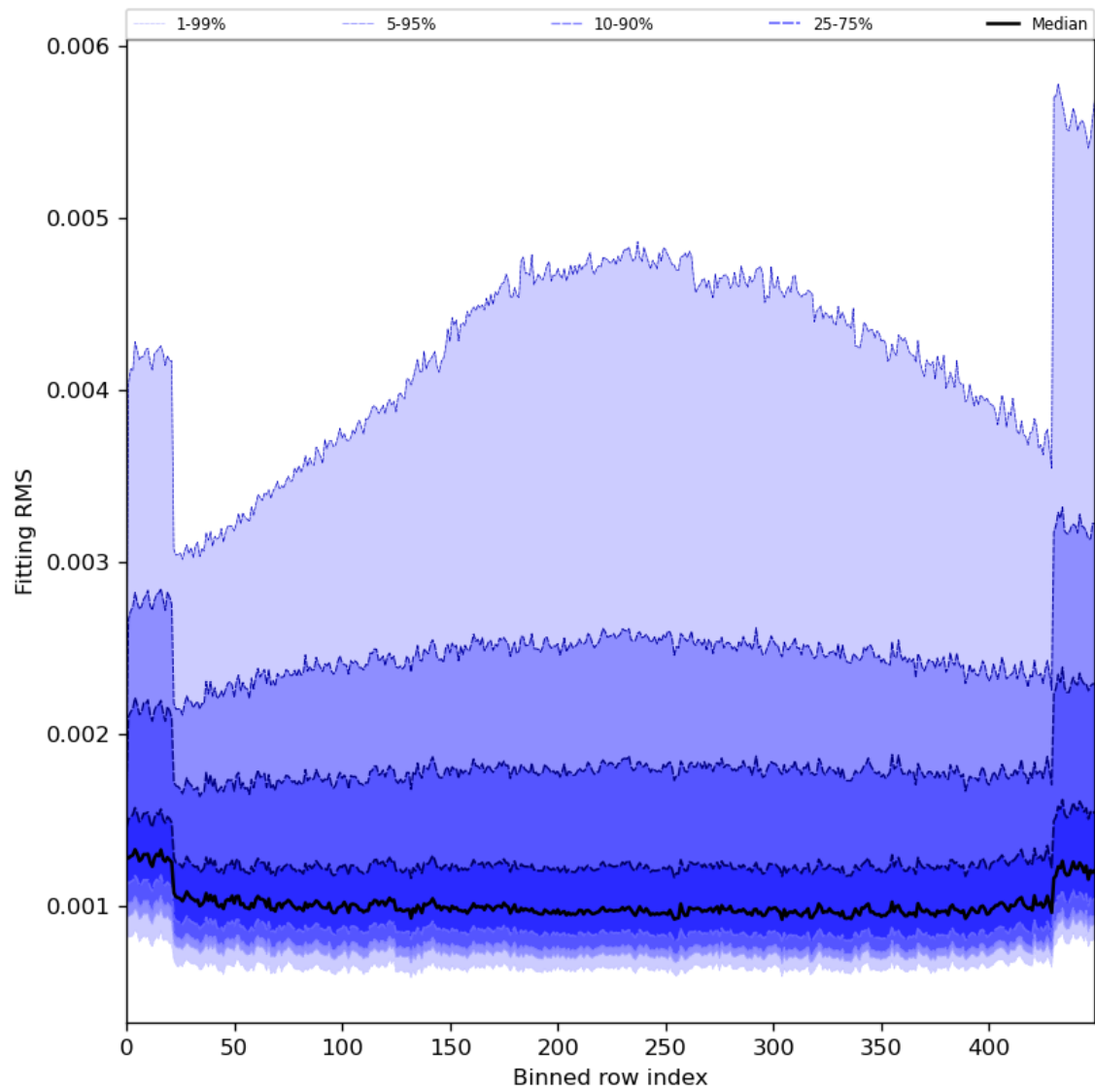
Figure 30: Along track statistics of “Fitting RMS” for 2023-12-09 to 2023-12-10
