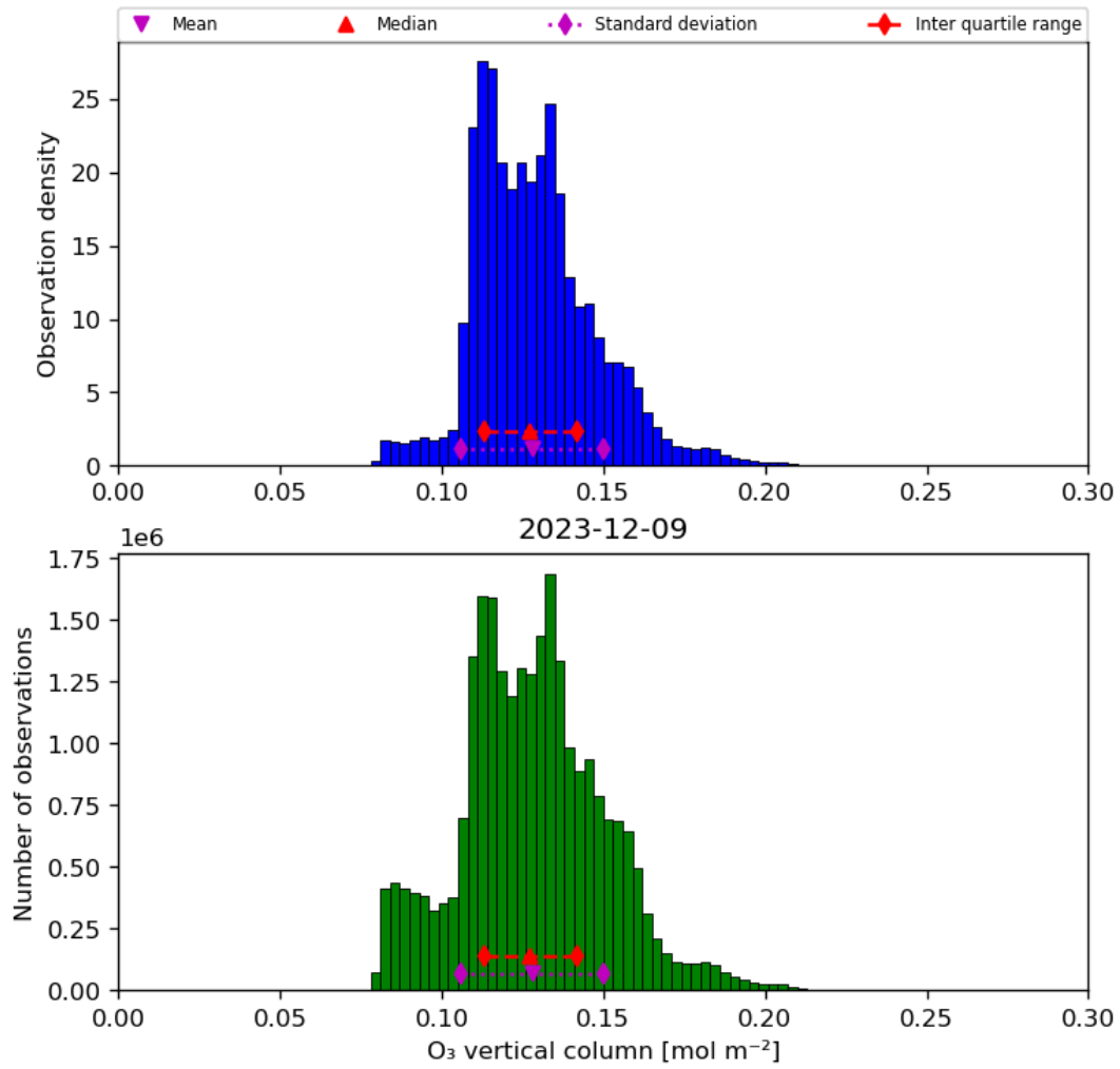
Figure 21: Histogram of “O 3 vertical column” for 2023-12-09 to 2023-12-10
