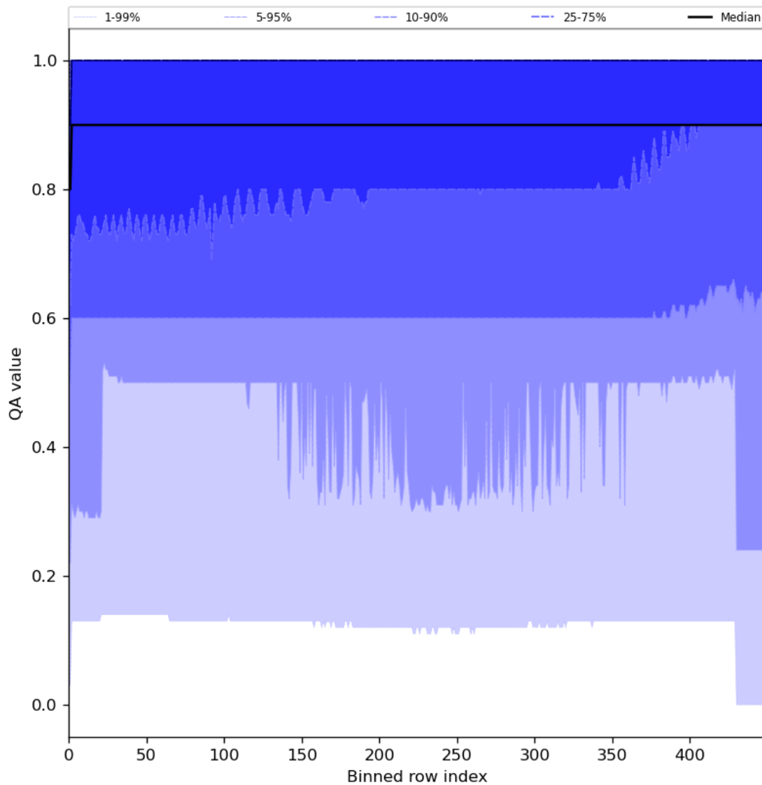
Figure 27: Along track statistics of “QA value” for 2023-12-09 to 2023-12-10
