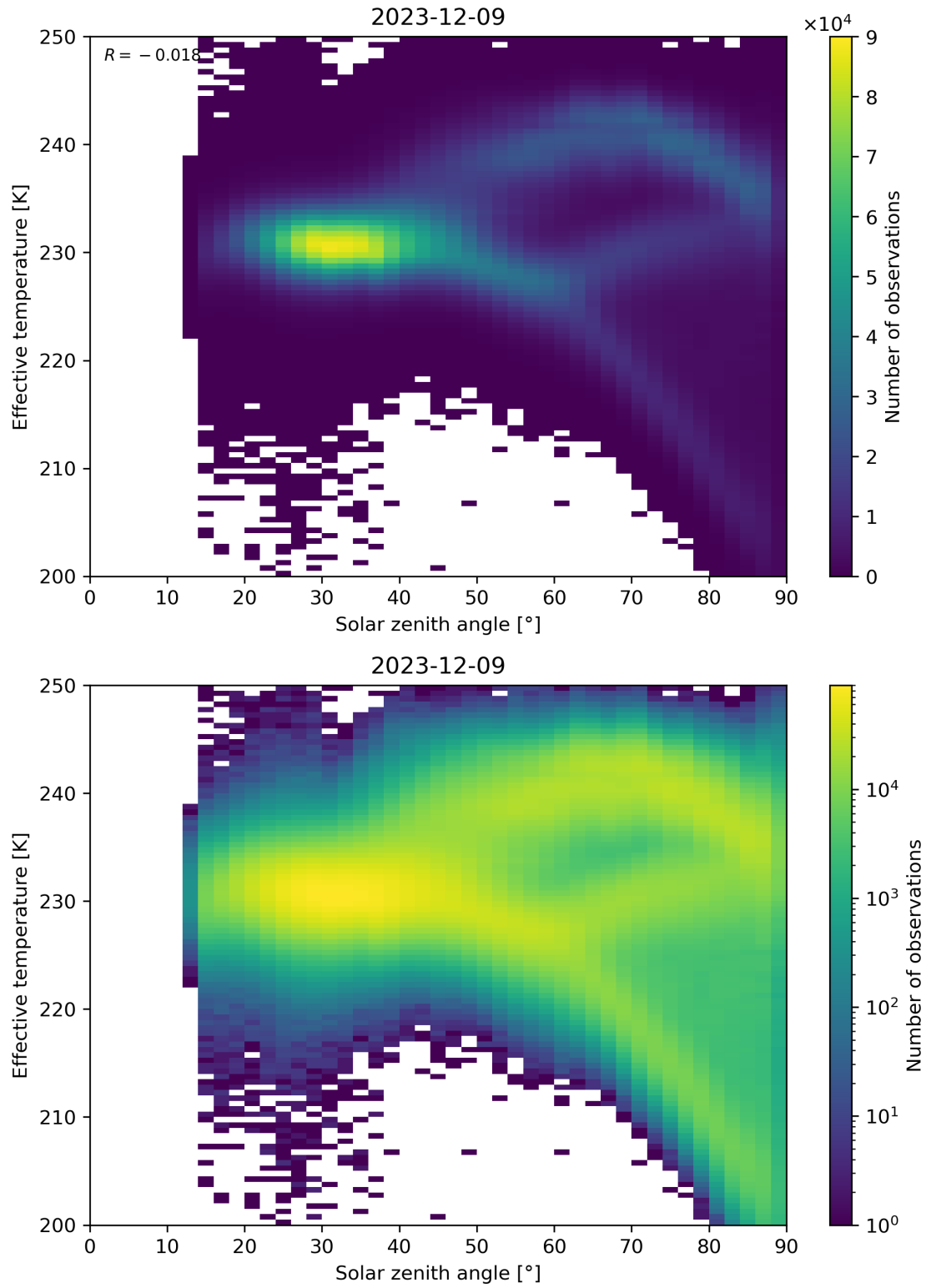
Figure 45: Scatter density plot of “Solar zenith angle” against “Effective temperature” for 2023-12-09 to 2023-12-10.
