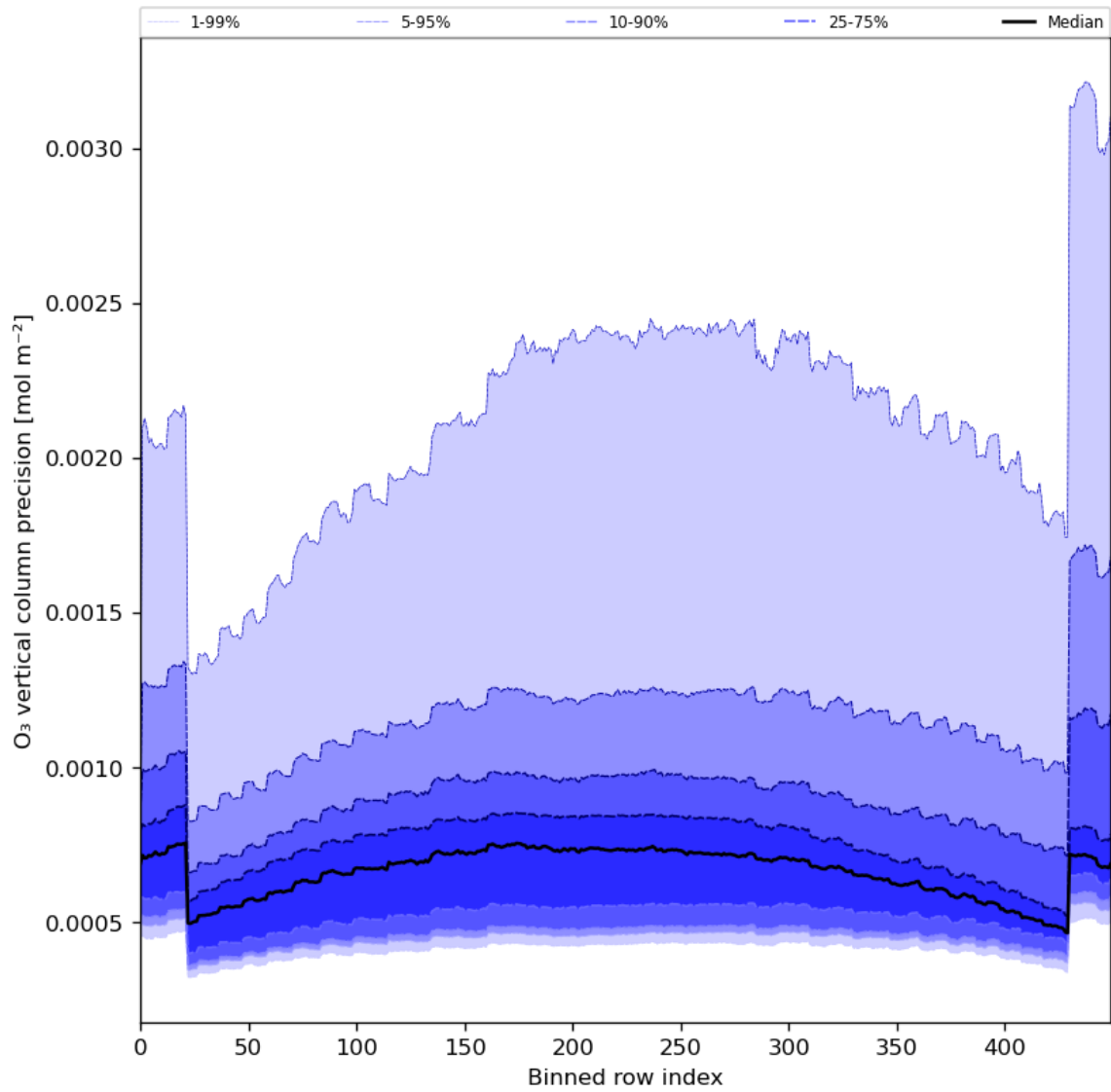
Figure 29: Along track statistics of “O 3 vertical column precision” for 2023-12-09 to 2023-12-10
