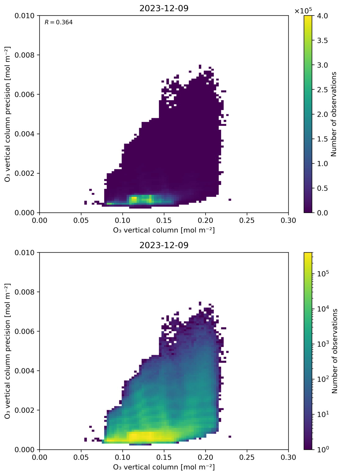
Figure 41: Scatter density plot of “O 3 vertical column” against “O 3 vertical column precision” for 2023-12-09 to 2023-12-10.
