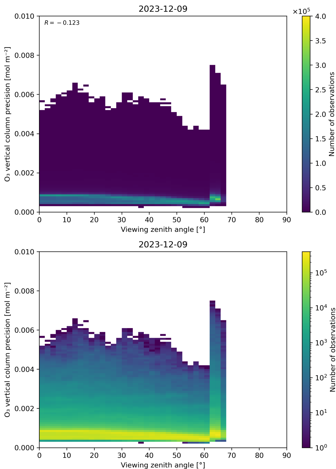
Figure 53: Scatter density plot of “Viewing zenith angle” against “O 3 vertical column precision” for 2023-12-09 to 2023-12-10.
