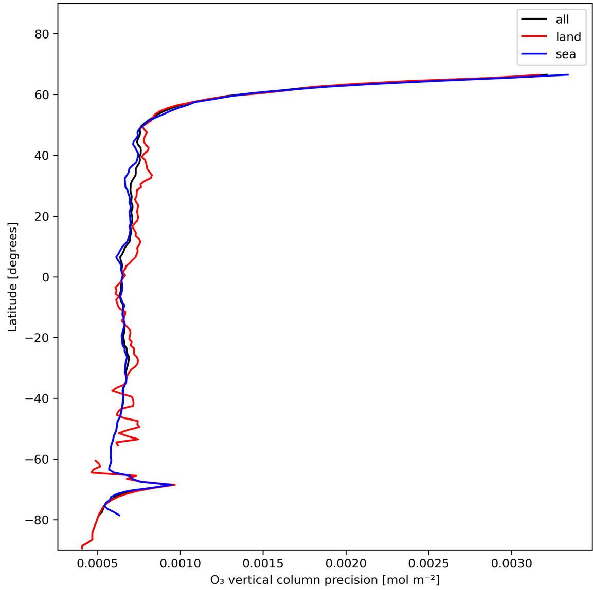
Figure 15: Zonal average of “O 3 vertical column precision” for 2023-12-09 to 2023-12-10.
