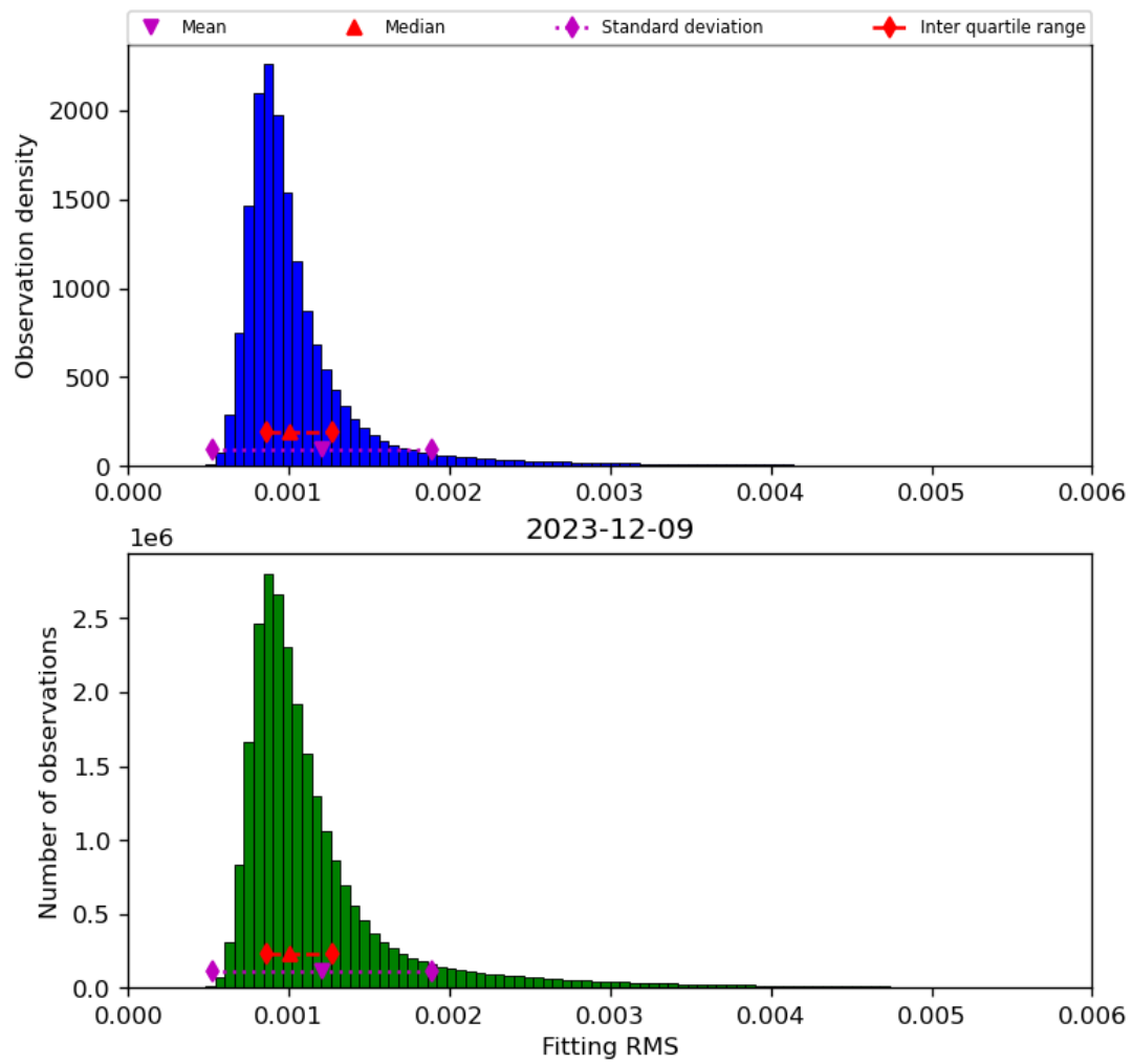
Figure 23: Histogram of “Fitting RMS” for 2023-12-09 to 2023-12-10
