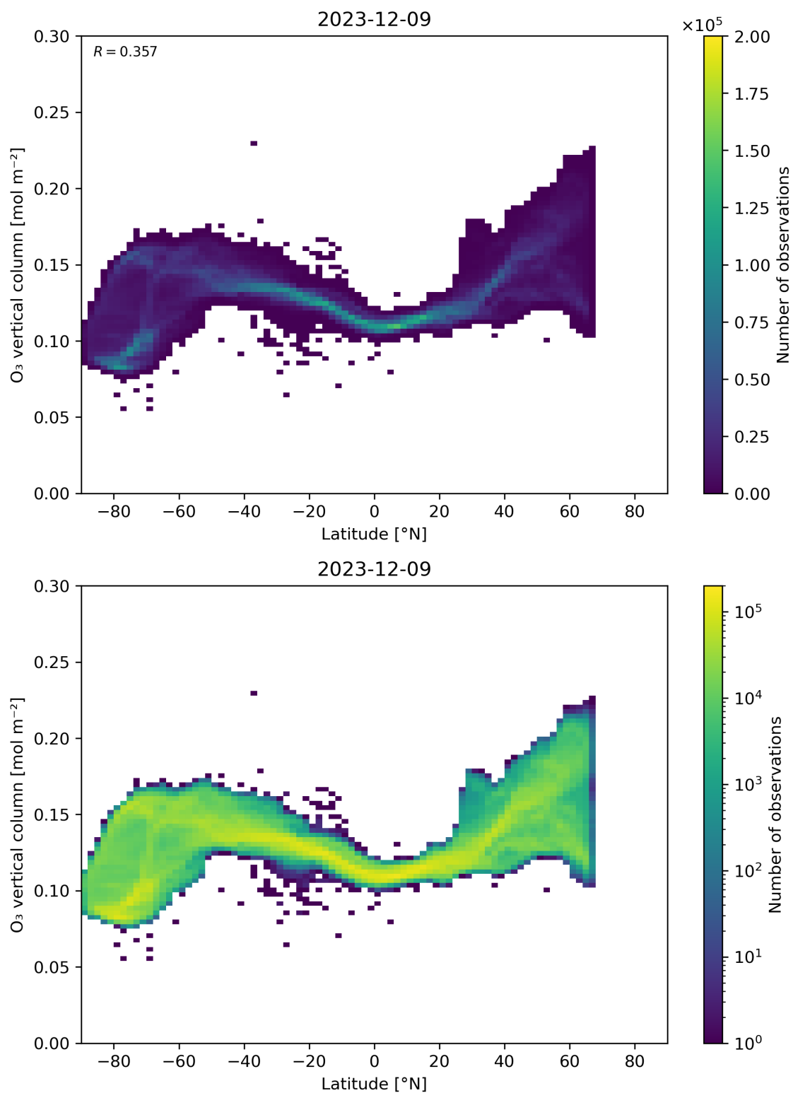
Figure 36: Scatter density plot of “Latitude” against “O 3 vertical column” for 2023-12-09 to 2023-12-10.
