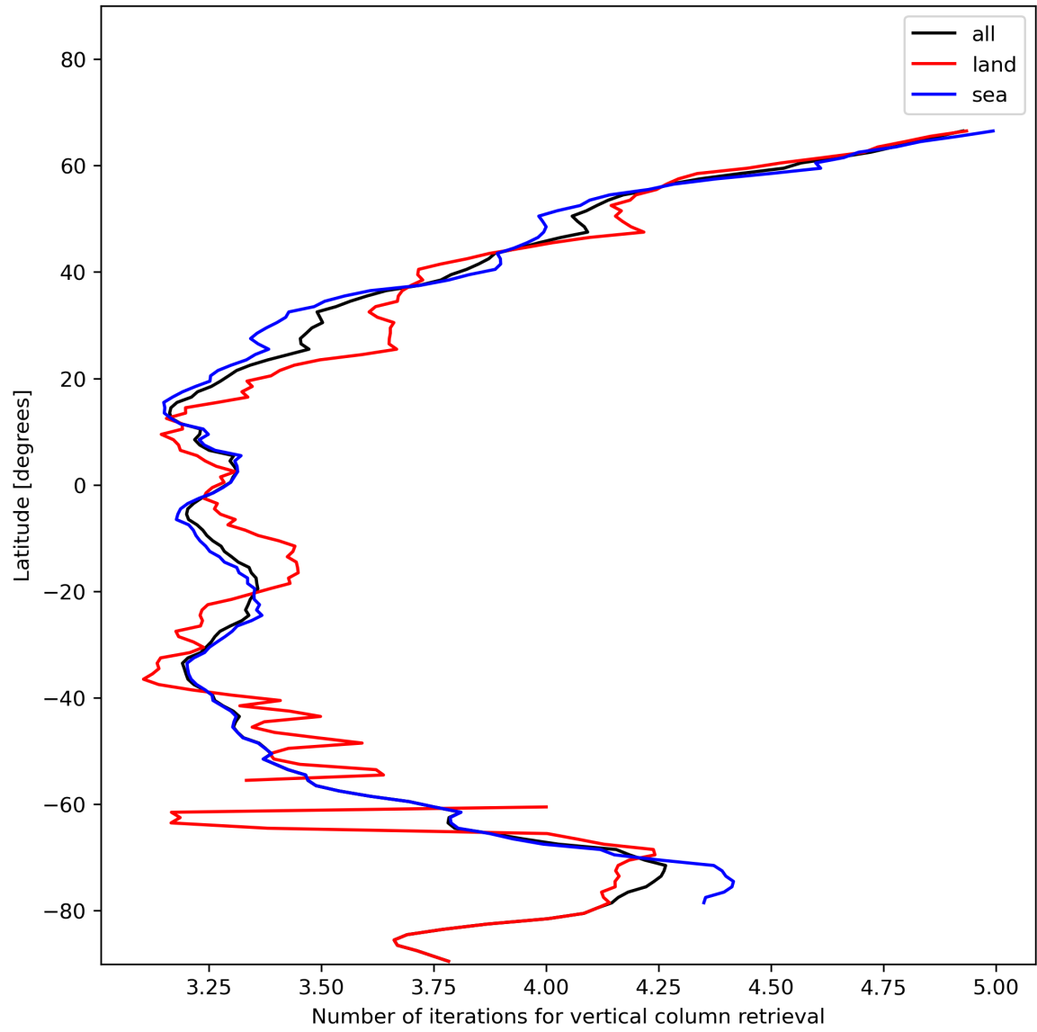
Figure 19: Zonal average of “Number of iterations for vertical column retrieval” for 2023-12-09 to 2023-12-10.
