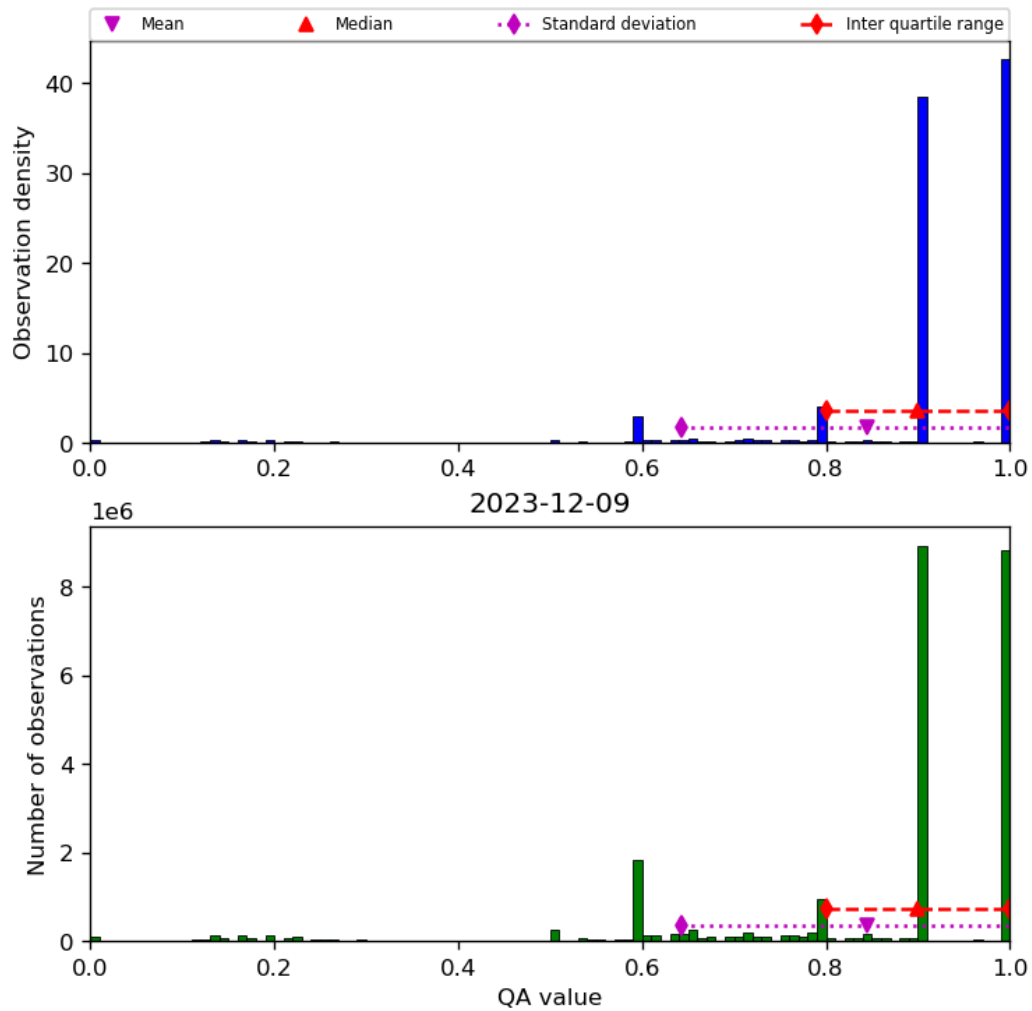
Figure 20: Histogram of “QA value” for 2023-12-09 to 2023-12-10
