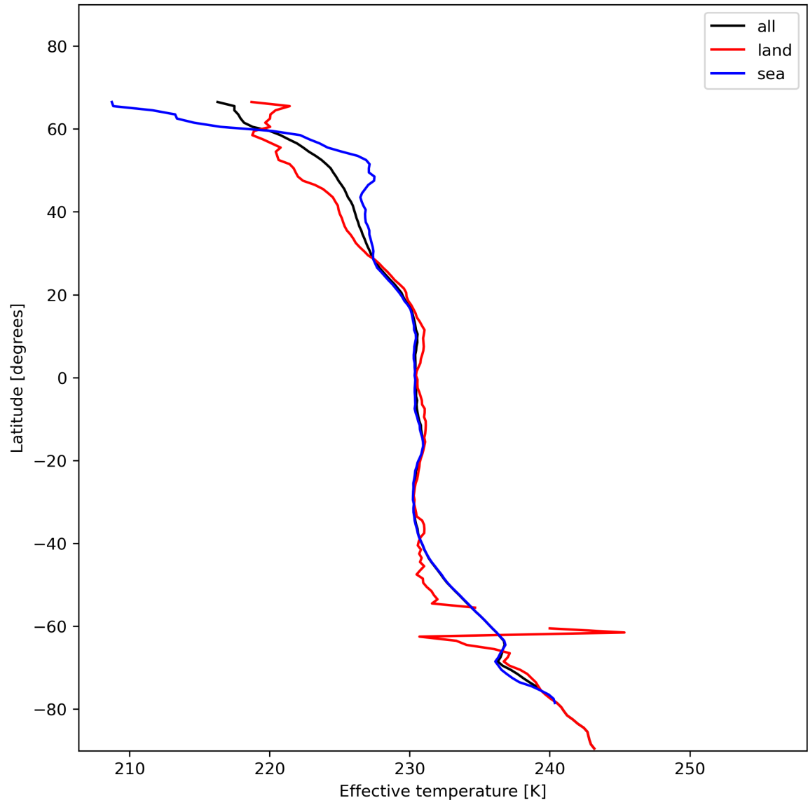
Figure 17: Zonal average of “Effective temperature” for 2023-12-09 to 2023-12-10.
