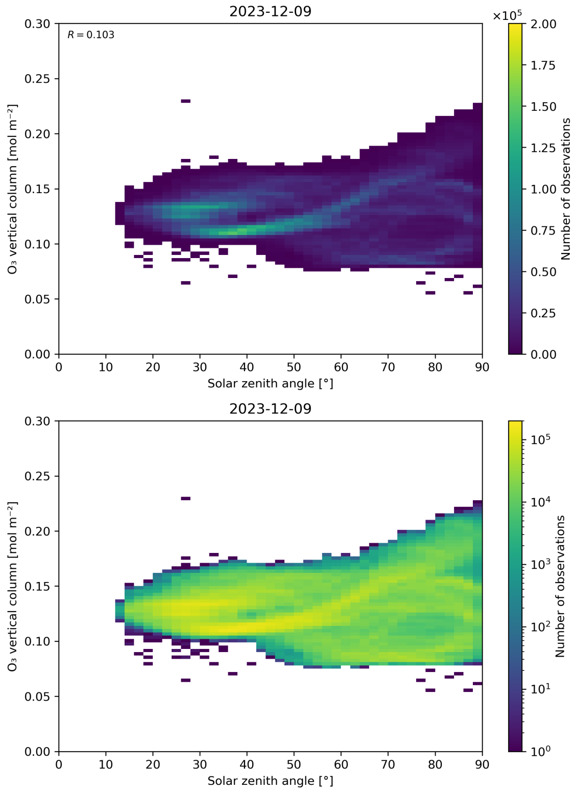
Figure 47: Scatter density plot of “Solar zenith angle” against “O 3 vertical column” for 2023-12-09 to 2023-12-10.
