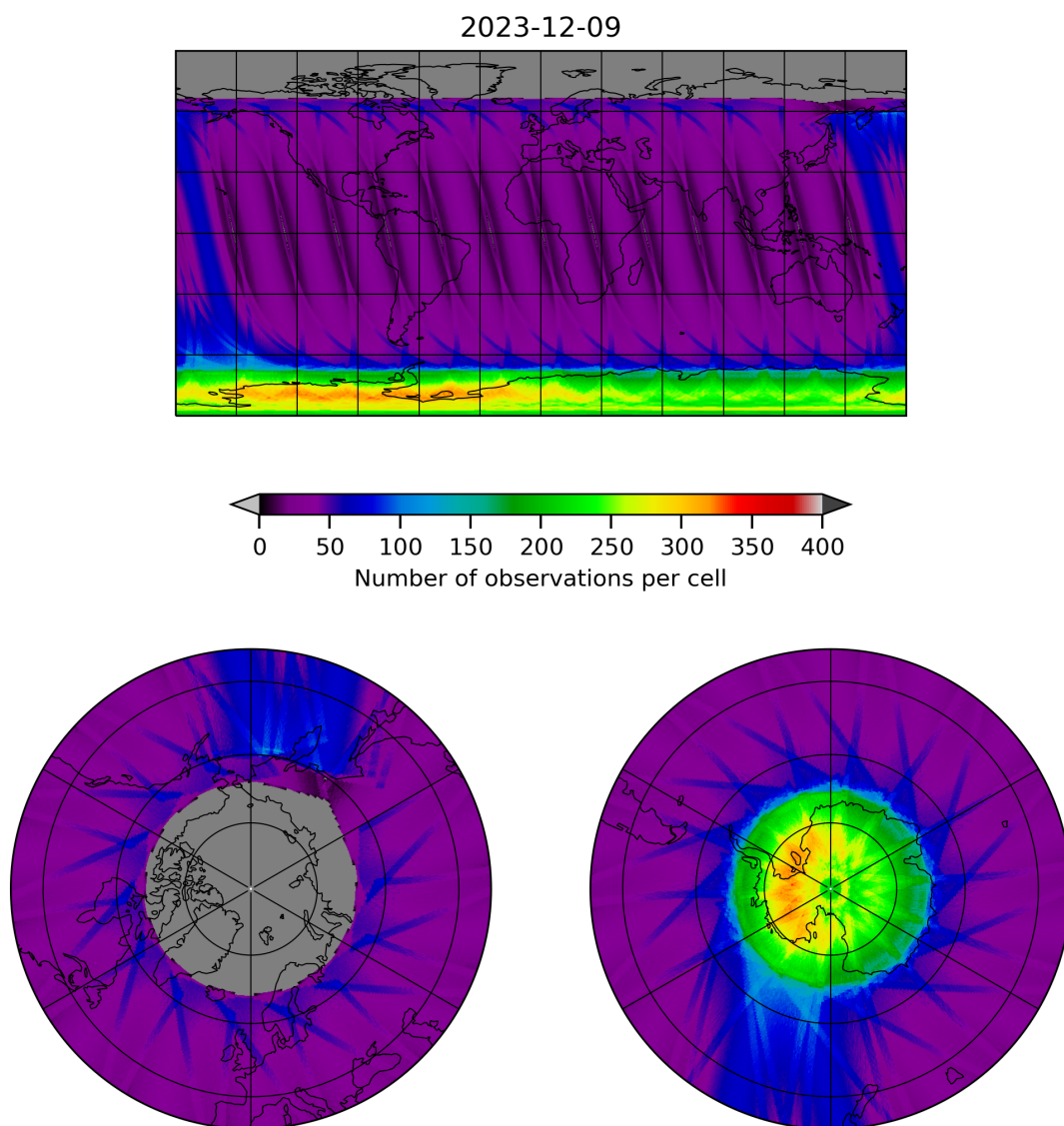
Figure 12: Map of the number of observations for 2023-12-09 to 2023-12-10
