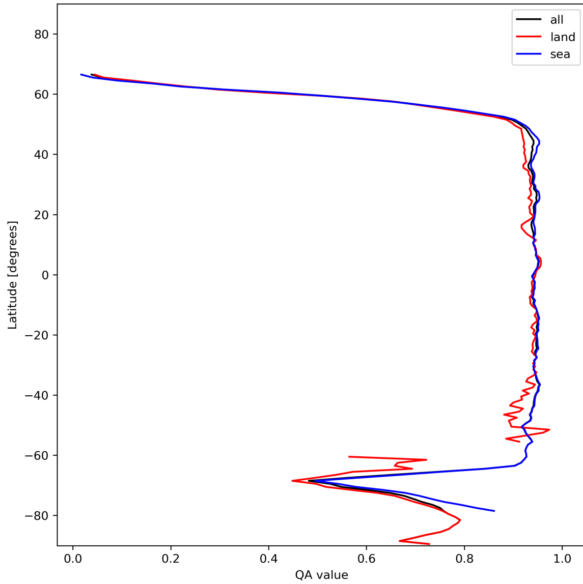
Figure 13: Zonal average of “QA value” for 2023-12-09 to 2023-12-10.
