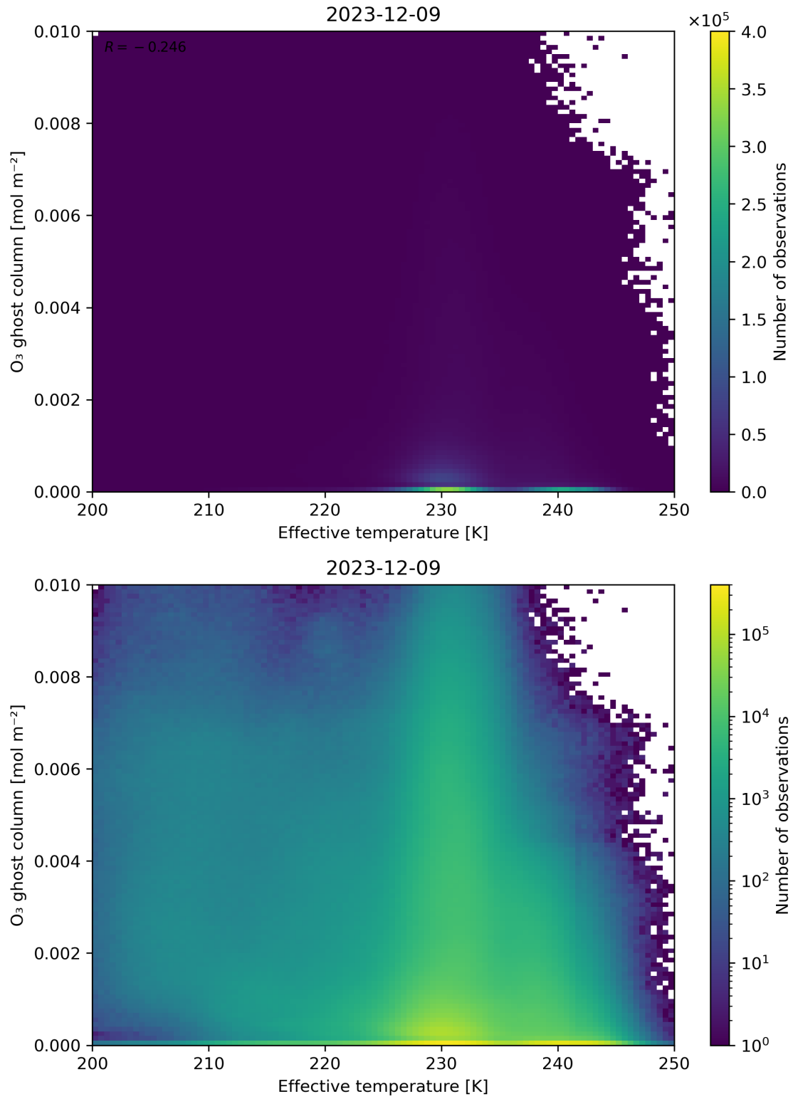
Figure 38: Scatter density plot of “Effective temperature” against “O 3 ghost column” for 2023-12-09 to 2023-12-10.
