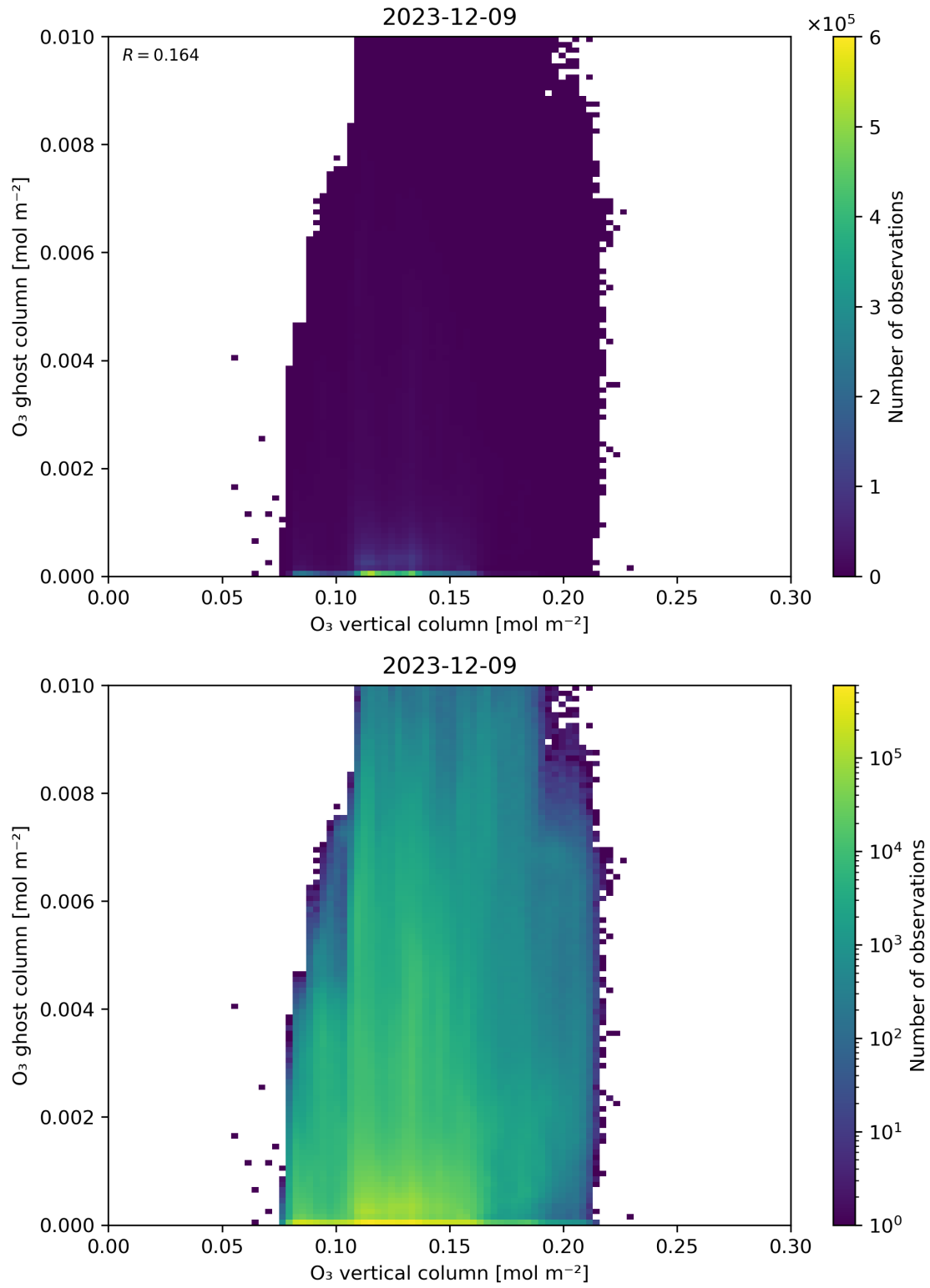
Figure 40: Scatter density plot of “O 3 vertical column” against “O 3 ghost column” for 2023-12-09 to 2023-12-10.
