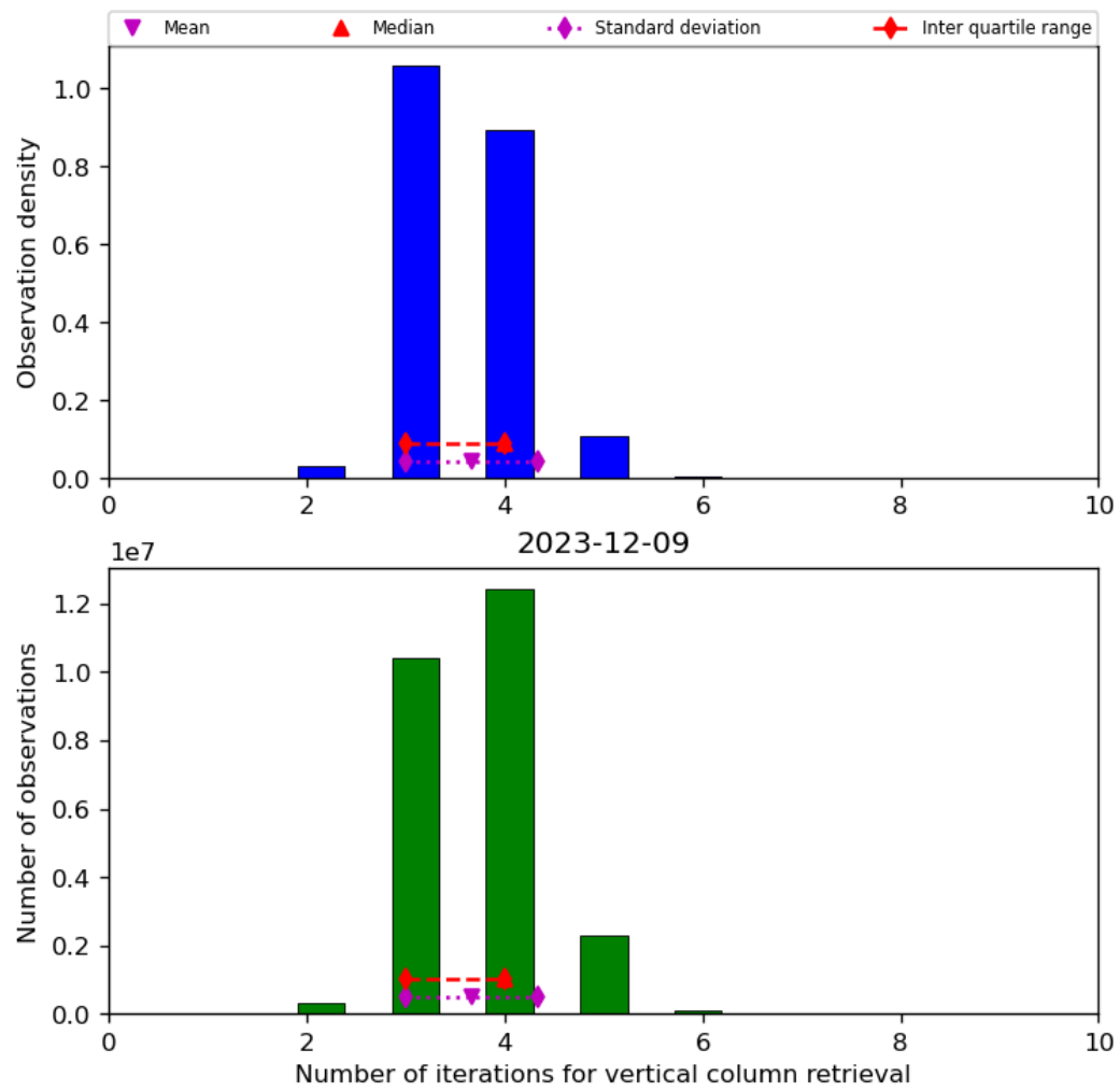
Figure 26: Histogram of “Number of iterations for vertical column retrieval” for 2023-12-09 to 2023-12-10
