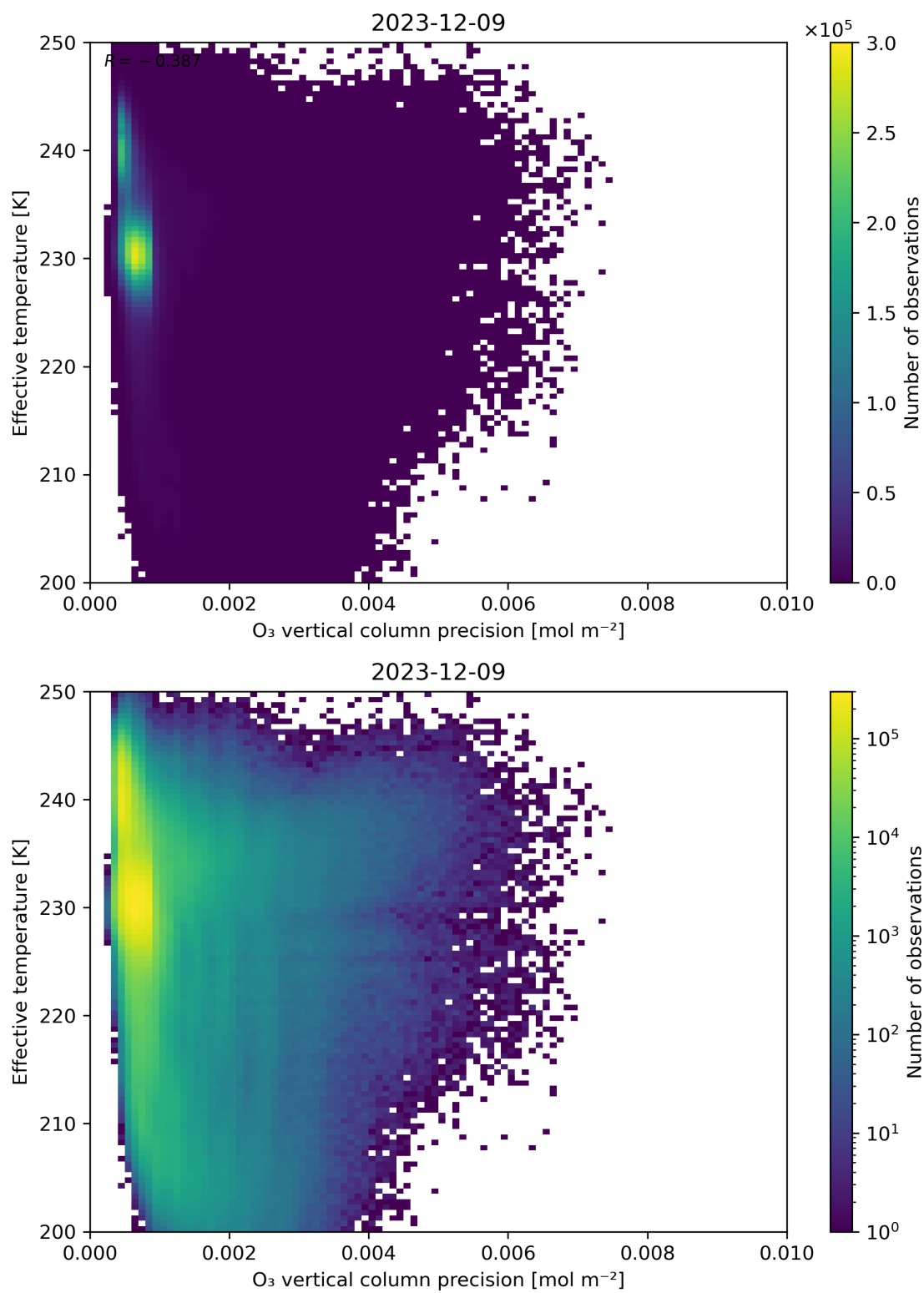
Figure 42: Scatter density plot of “O 3 vertical column precision” against “Effective temperature” for 2023-12-09 to 2023-12-10.
