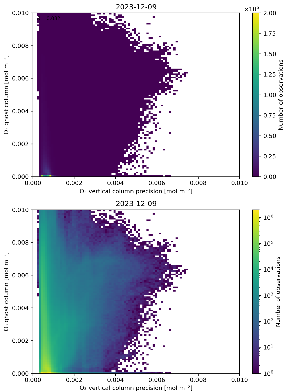
Figure 43: Scatter density plot of “O 3 vertical column precision” against “O 3 ghost column” for 2023-12-09 to 2023-12-10.
