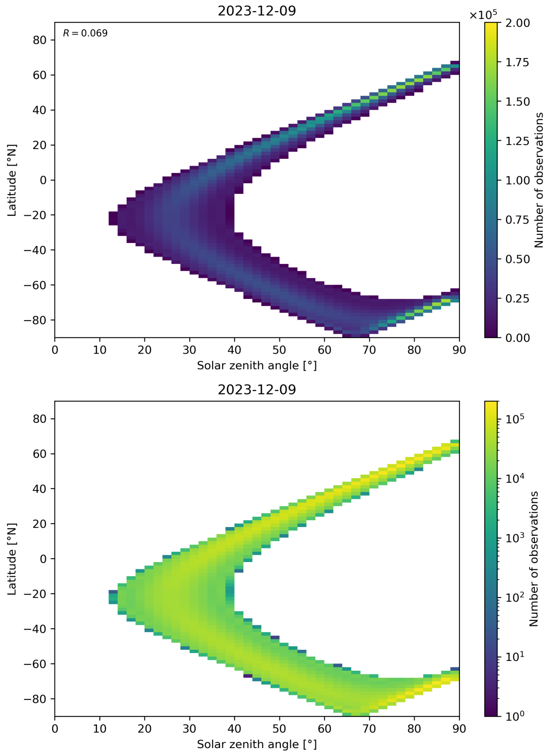
Figure 44: Scatter density plot of “Solar zenith angle” against “Latitude” for 2023-12-09 to 2023-12-10.
