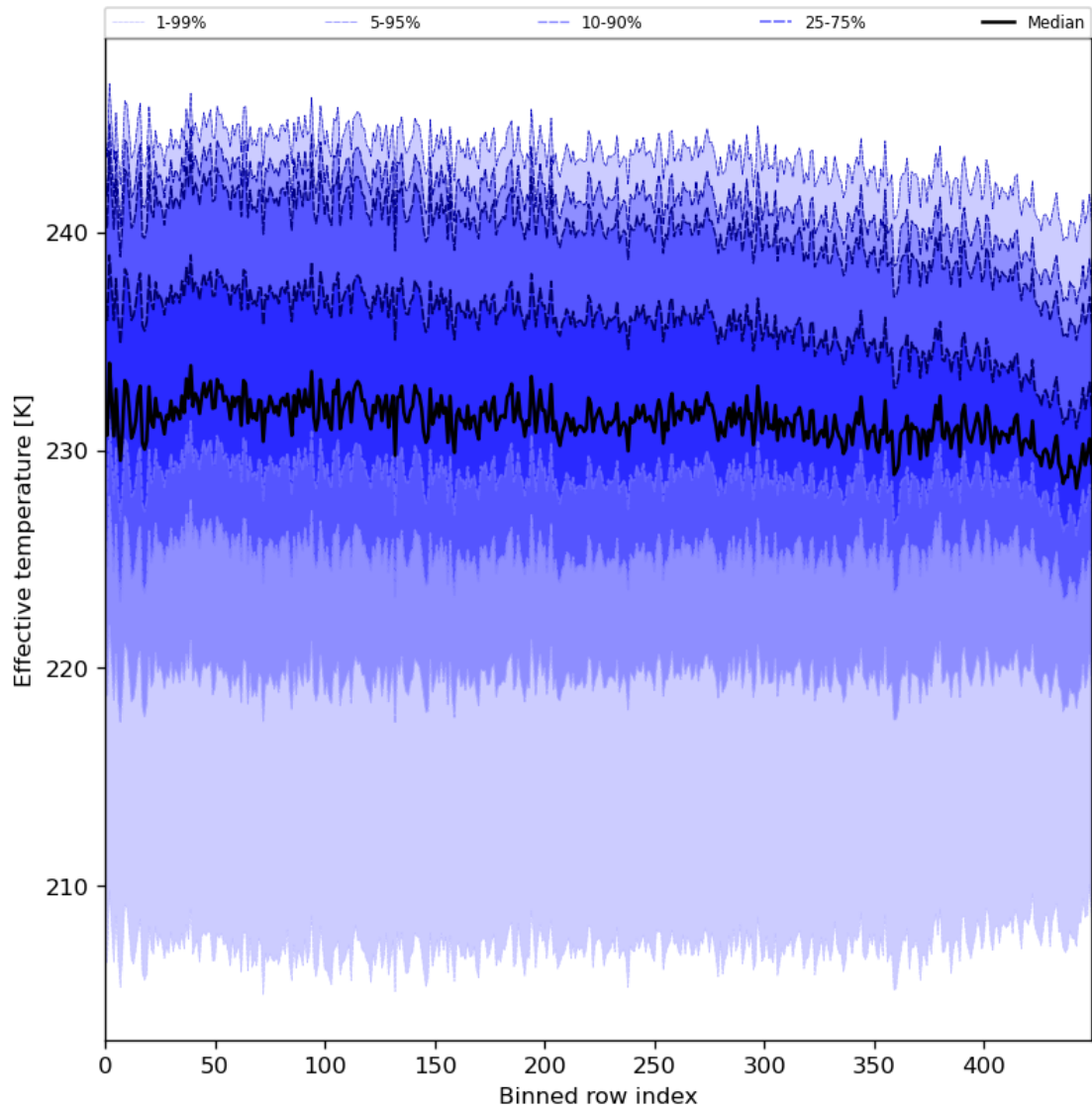
Figure 31: Along track statistics of “Effective temperature” for 2023-12-09 to 2023-12-10
