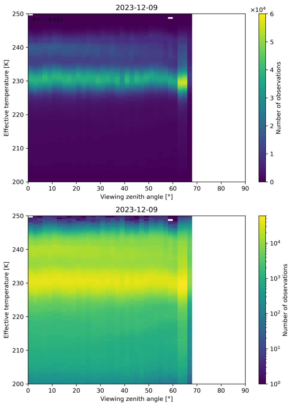
Figure 50: Scatter density plot of “Viewing zenith angle” against “Effective temperature” for 2023-12-09 to 2023-12-10.
