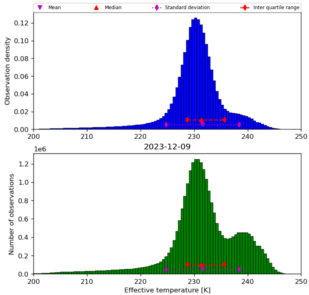
Figure 24: Histogram of “Effective temperature” for 2023-12-09 to 2023-12-10
