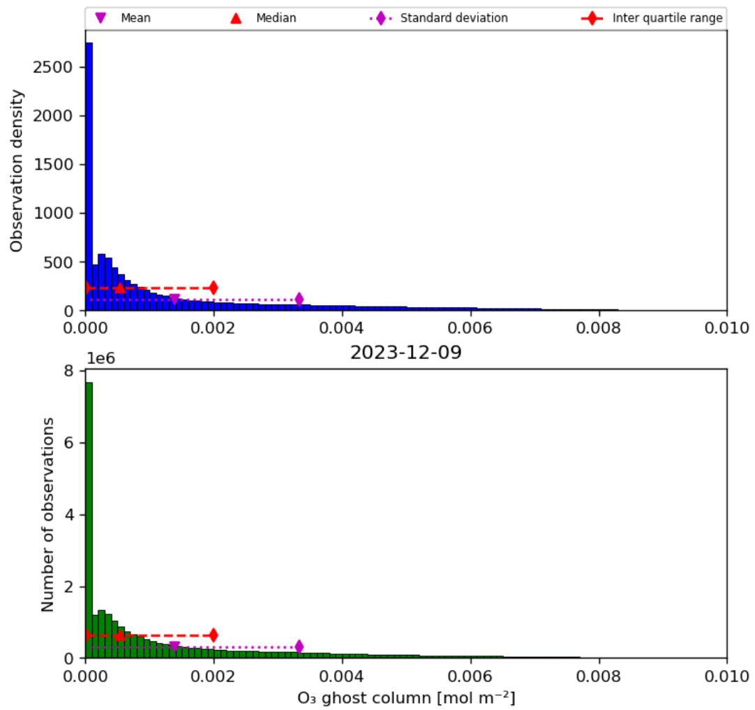
Figure 25: Histogram of “O 3 ghost column” for 2023-12-09 to 2023-12-10
