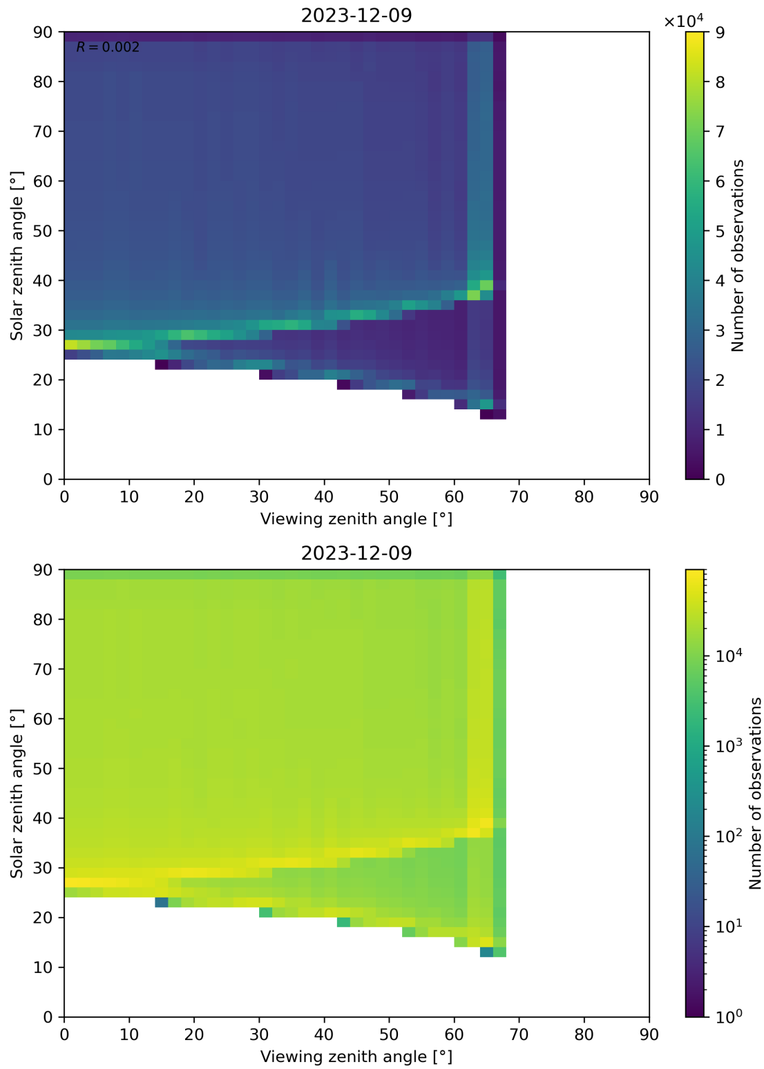
Figure 54: Scatter density plot of “Viewing zenith angle” against “Solar zenith angle” for 2023-12-09 to 2023-12-10.
