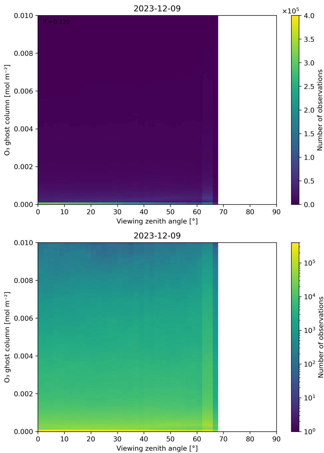
Figure 51: Scatter density plot of “Viewing zenith angle” against “O 3 ghost column” for 2023-12-09 to 2023-12-10.
