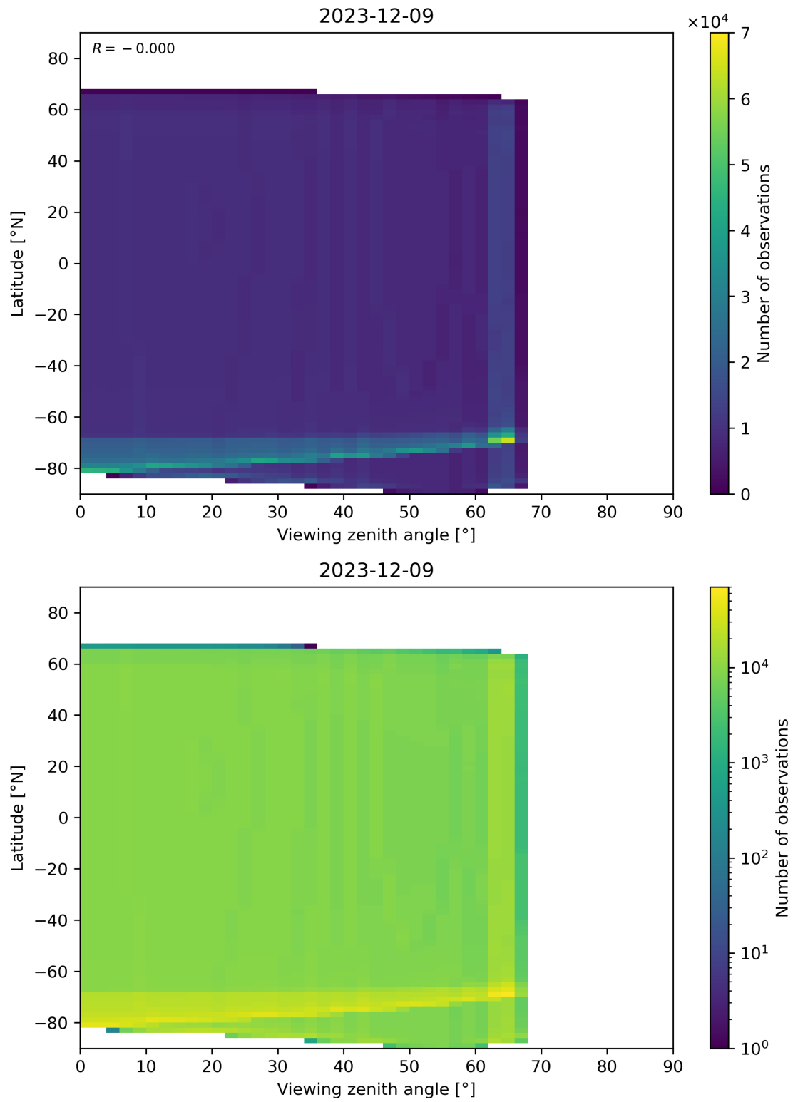
Figure 49: Scatter density plot of “Viewing zenith angle” against “Latitude” for 2023-12-09 to 2023-12-10.
