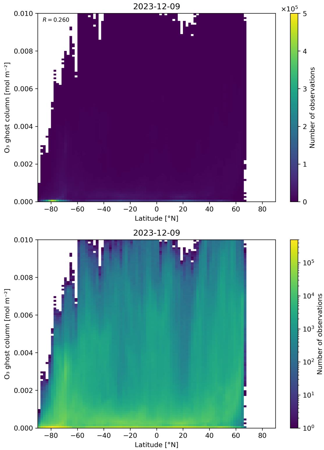
Figure 35: Scatter density plot of “Latitude” against “O 3 ghost column” for 2023-12-09 to 2023-12-10.
