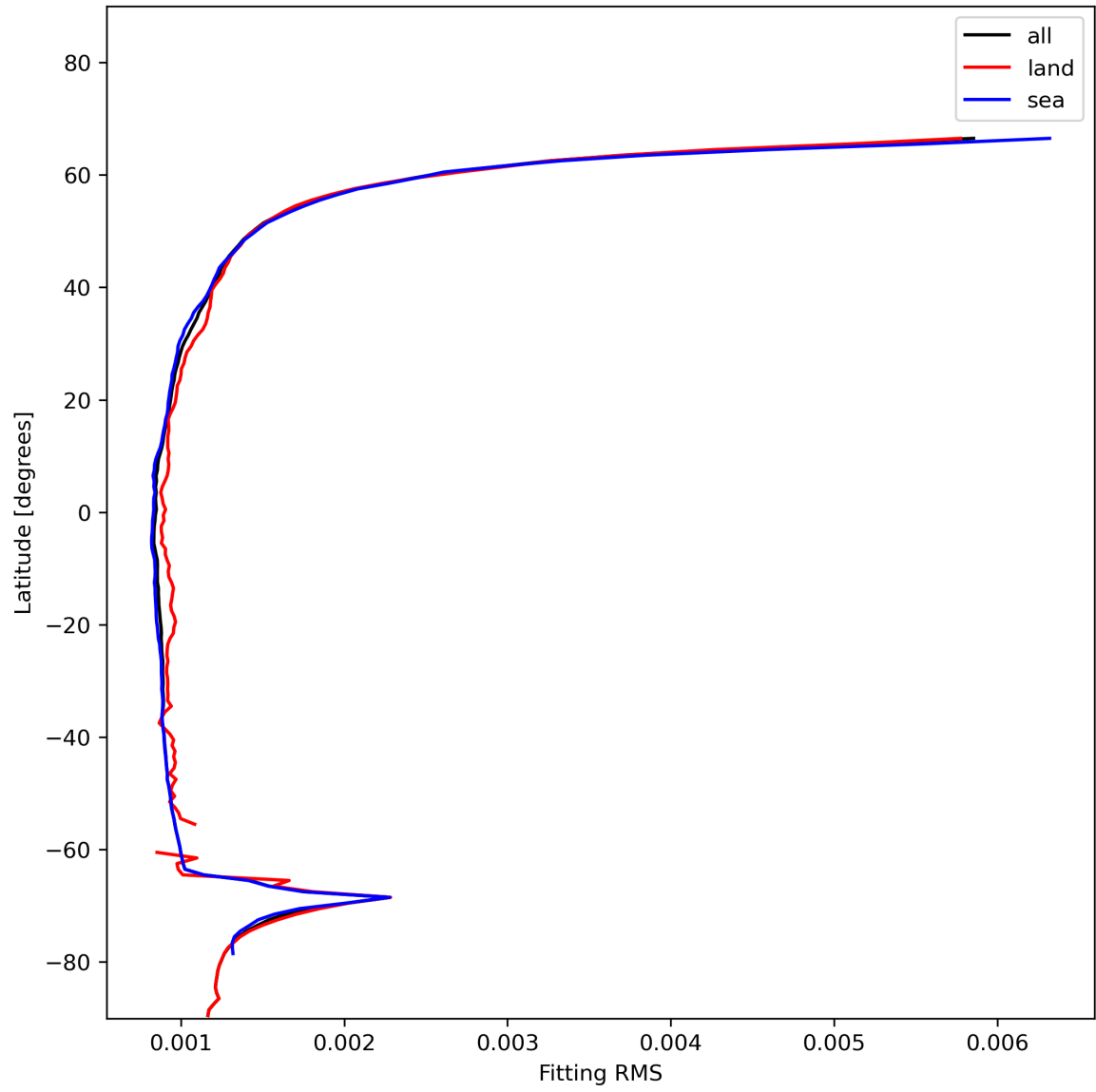
Figure 16: Zonal average of “Fitting RMS” for 2023-12-09 to 2023-12-10.
