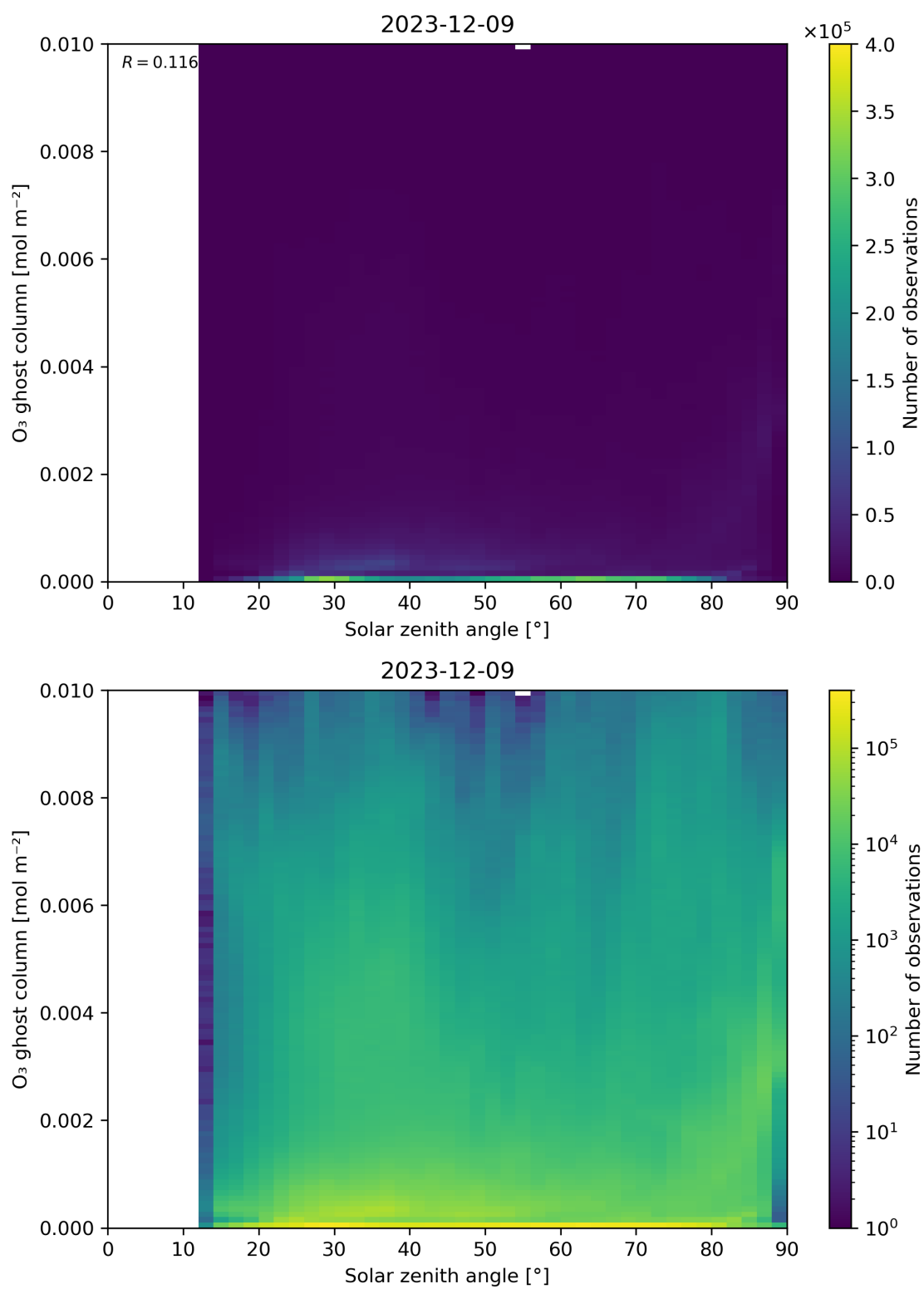
Figure 46: Scatter density plot of “Solar zenith angle” against “O 3 ghost column” for 2023-12-09 to 2023-12-10.
