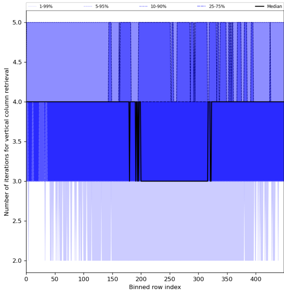
Figure 33: Along track statistics of “Number of iterations for vertical column retrieval” for 2023-12-09 to 2023-12-10
