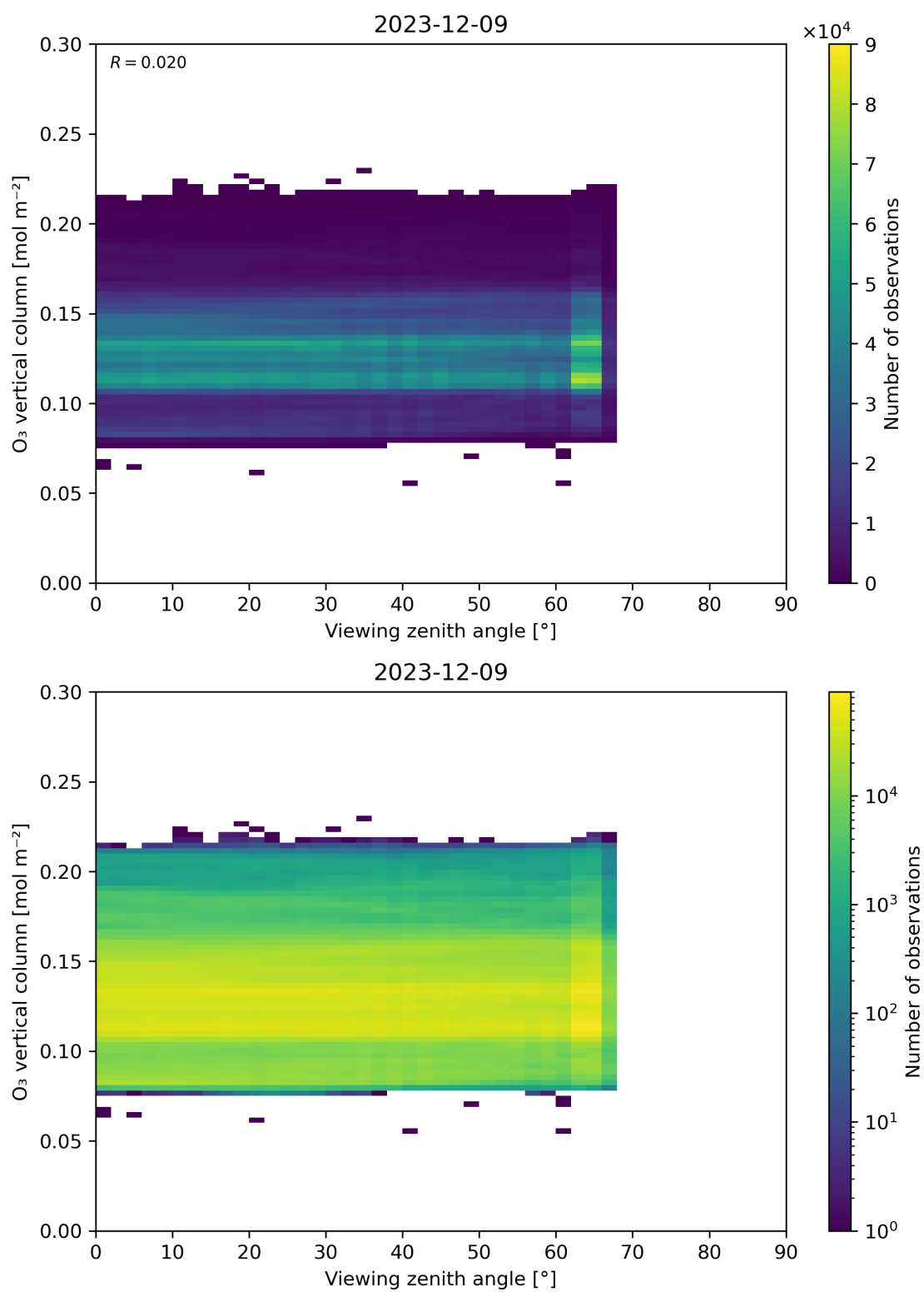
Figure 52: Scatter density plot of “Viewing zenith angle” against “O 3 vertical column” for 2023-12-09 to 2023-12-10.
