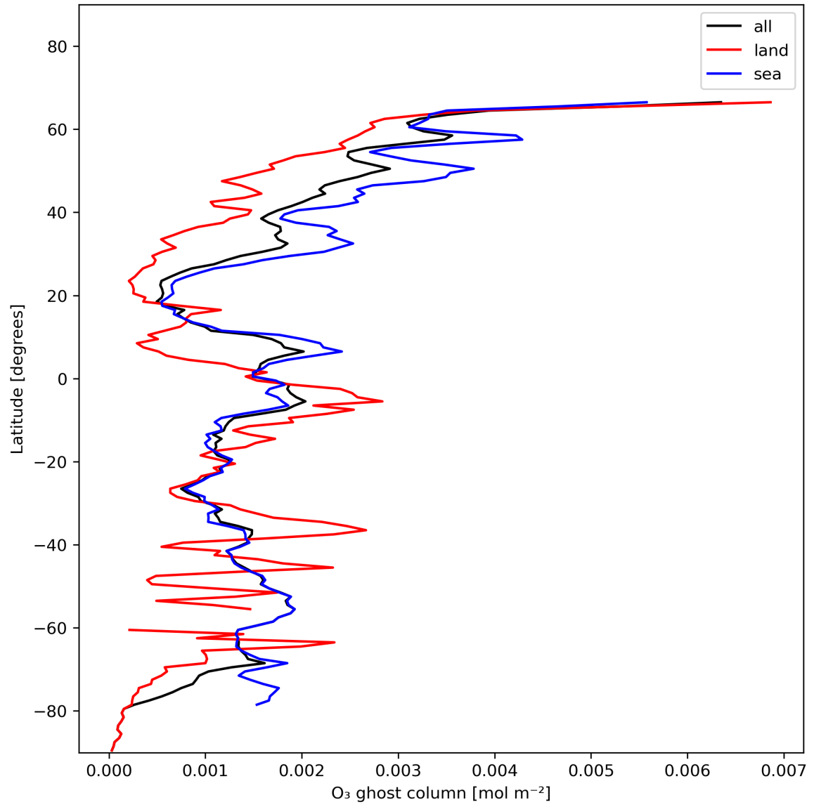
Figure 18: Zonal average of "O 3 ghost column" for 2023-12-09 to 2023-12-10.
