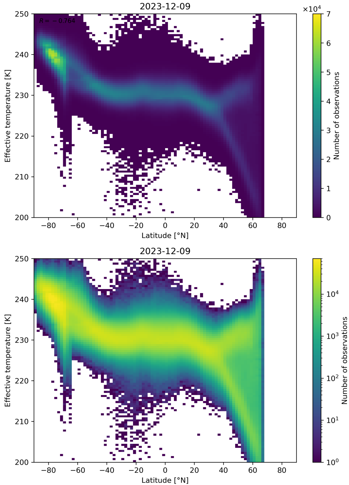
Figure 34: Scatter density plot of “Latitude” against “Effective temperature” for 2023-12-09 to 2023-12-10.
