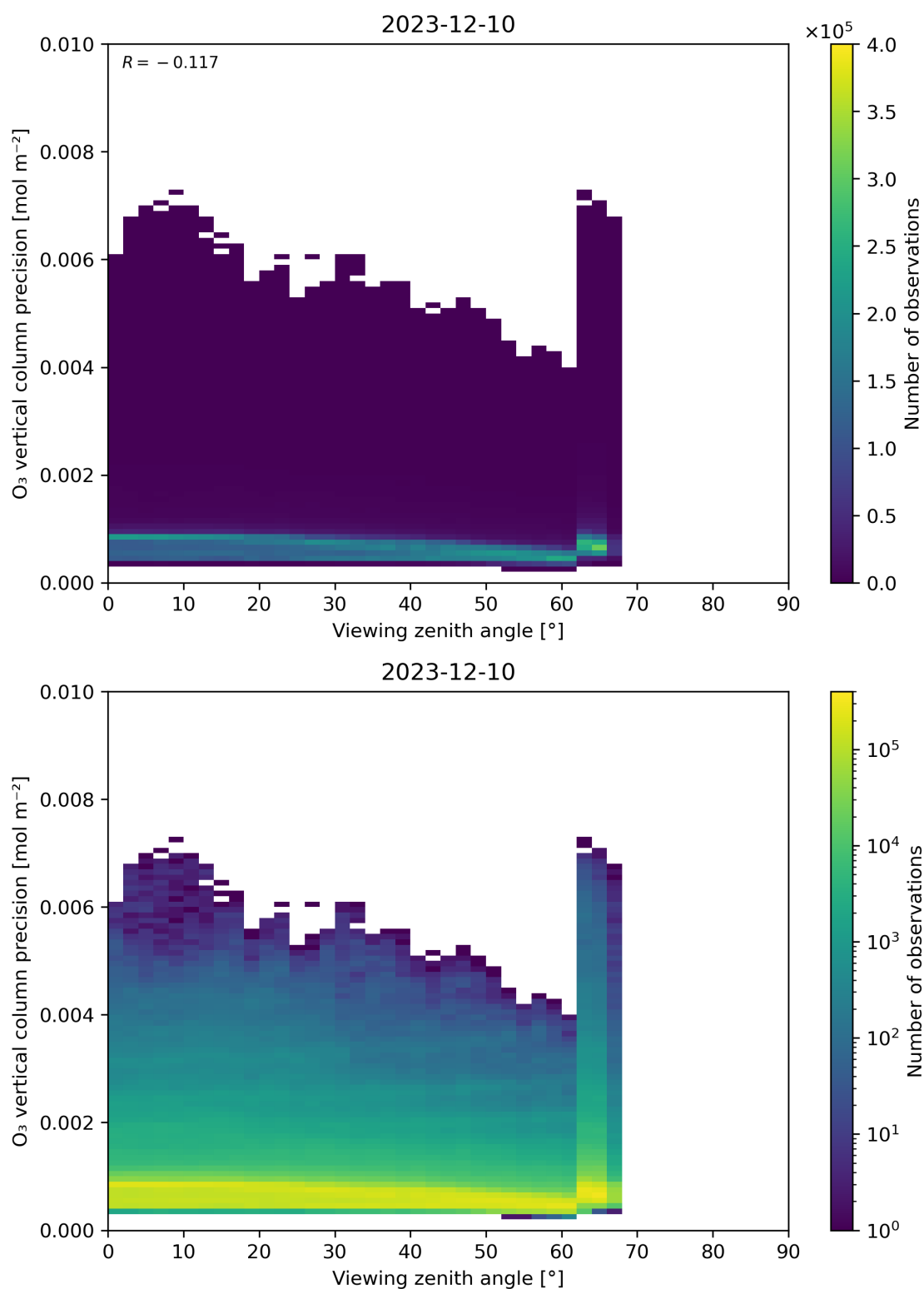
Figure 53: Scatter density plot of “Viewing zenith angle” against “O 3 vertical column precision” for 2023-12-09 to 2023-12-11.
