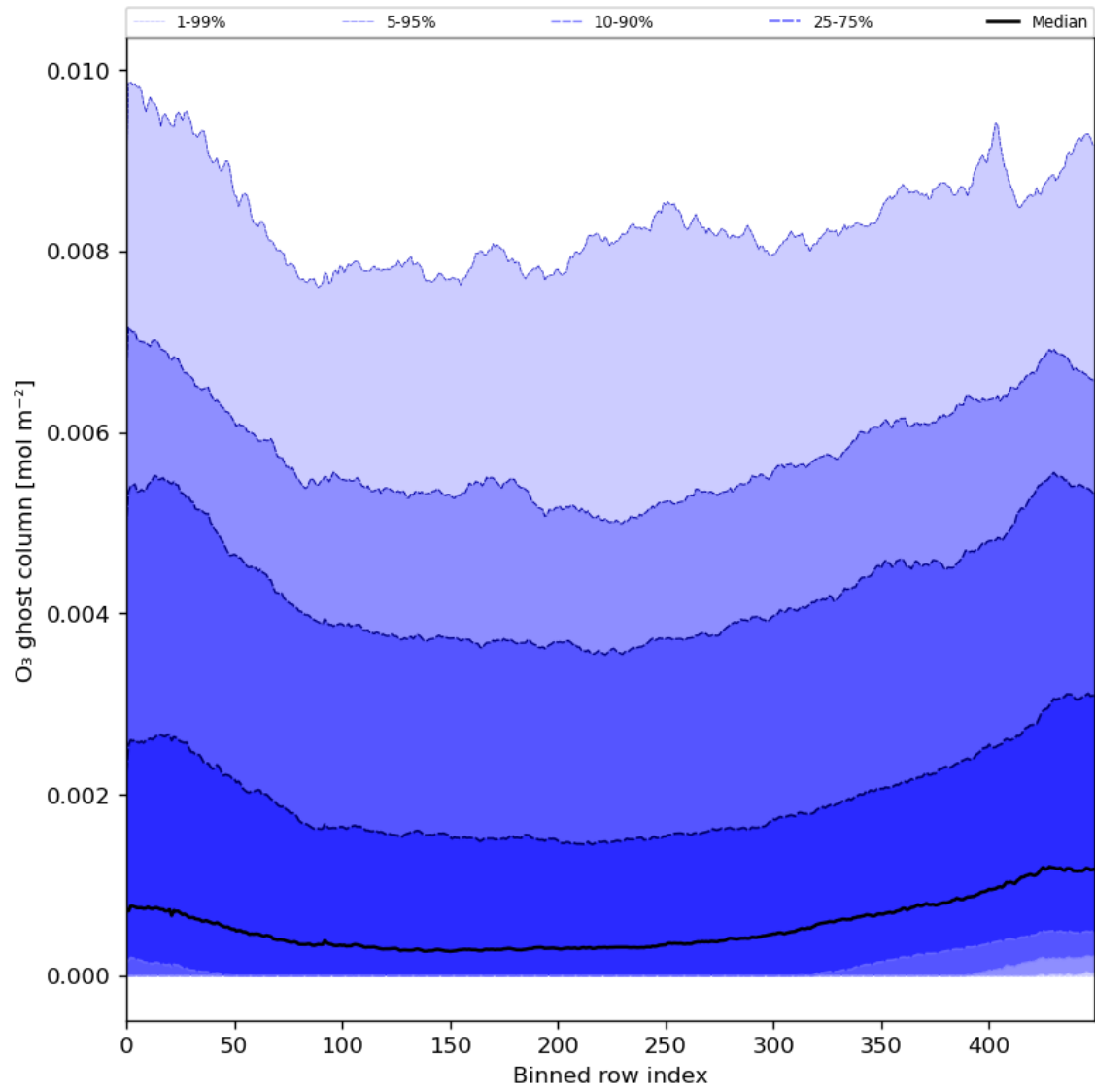
Figure 32: Along track statistics of “O 3 ghost column” for 2023-12-09 to 2023-12-11
