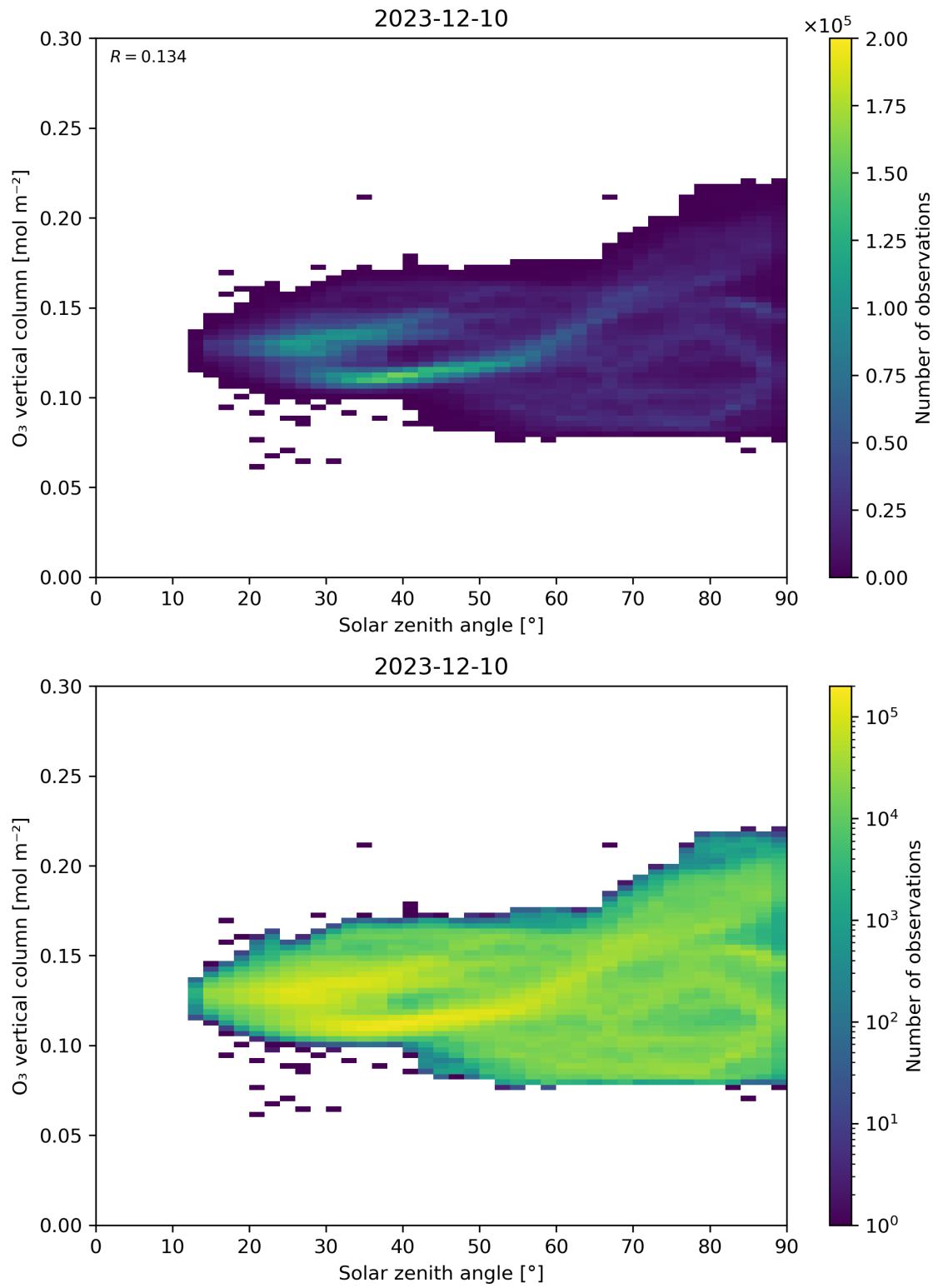
Figure 47: Scatter density plot of “Solar zenith angle” against “O 3 vertical column” for 2023-12-09 to 2023-12-11.
