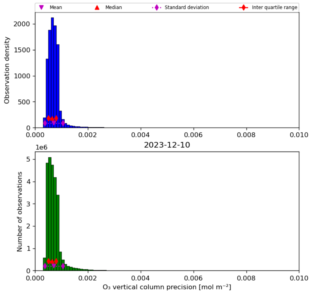
Figure 22: Histogram of “O 3 vertical column precision” for 2023-12-09 to 2023-12-11
