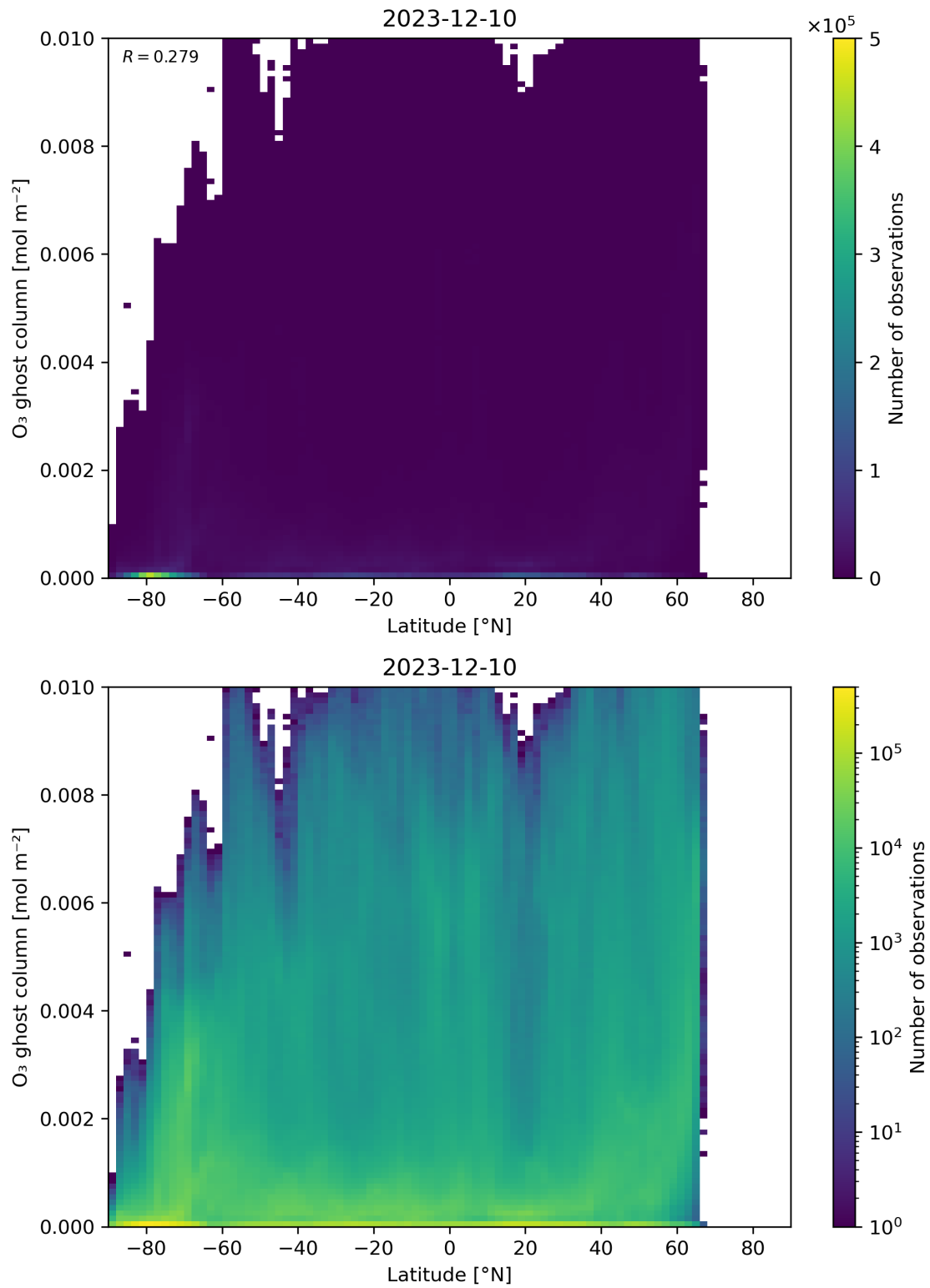
Figure 35: Scatter density plot of “Latitude” against “O 3 ghost column” for 2023-12-09 to 2023-12-11.
