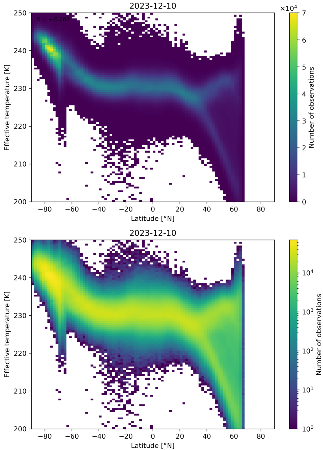
Figure 34: Scatter density plot of “Latitude” against “Effective temperature” for 2023-12-09 to 2023-12-11.
