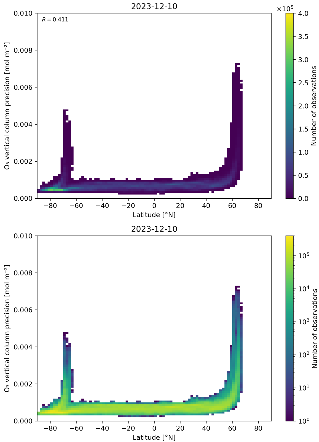
Figure 37: Scatter density plot of “Latitude” against “O 3 vertical column precision” for 2023-12-09 to 2023-12-11.
