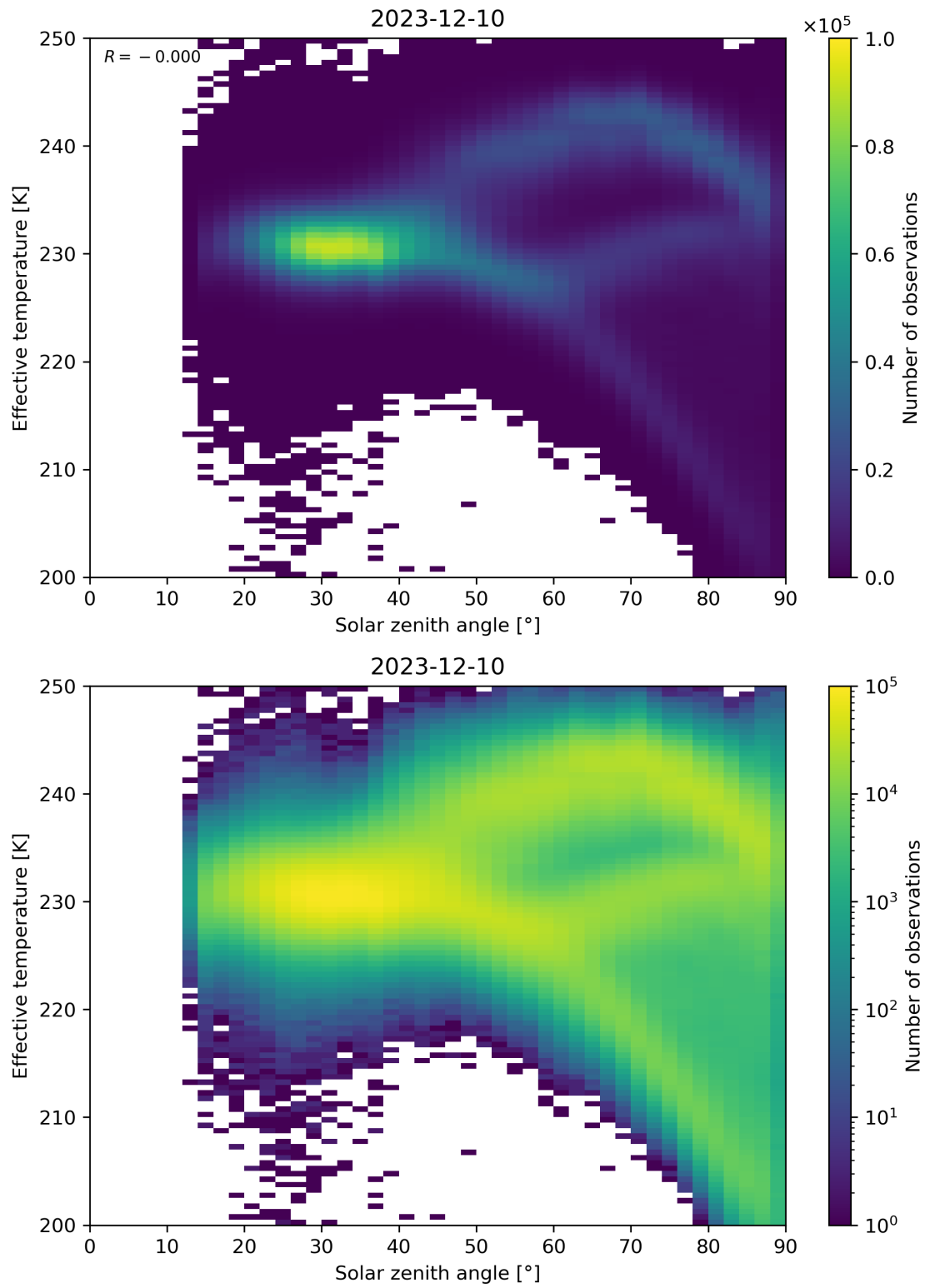
Figure 45: Scatter density plot of “Solar zenith angle” against “Effective temperature” for 2023-12-09 to 2023-12-11.
