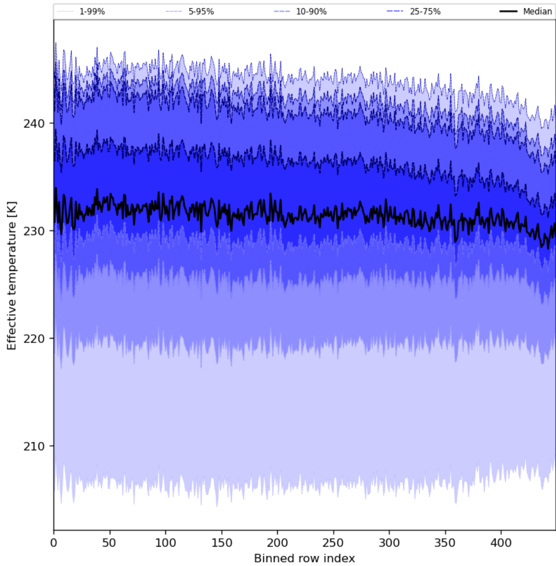
Figure 31: Along track statistics of “Effective temperature” for 2023-12-09 to 2023-12-11
