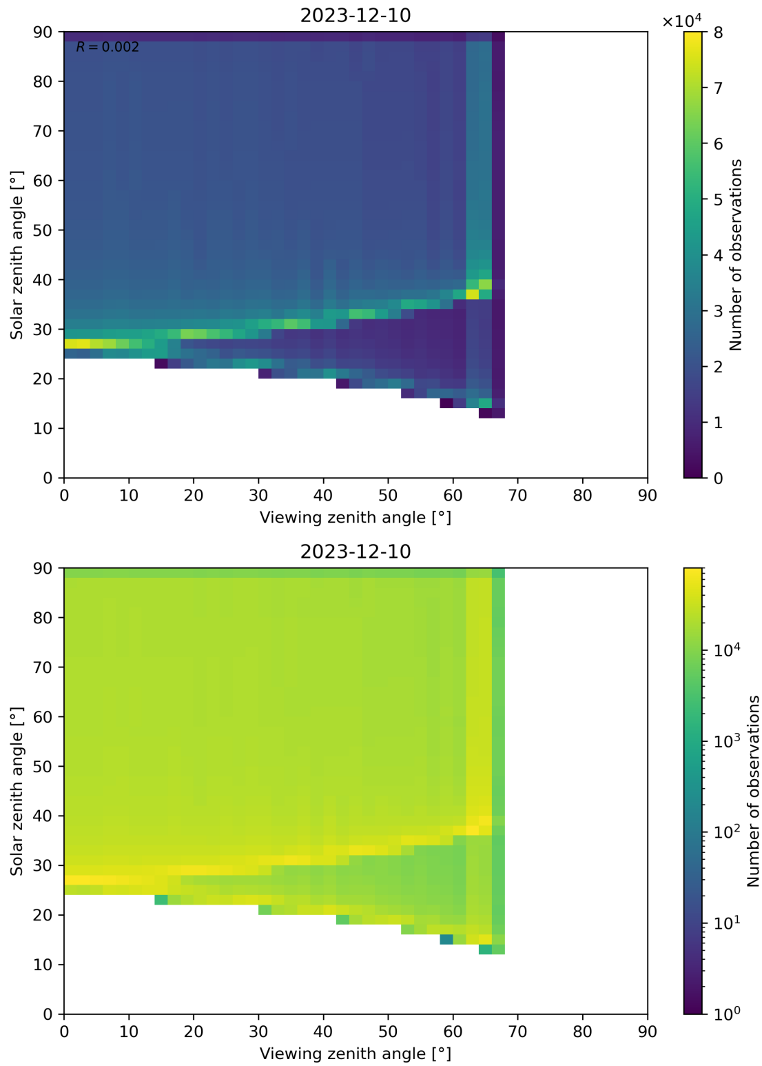
Figure 54: Scatter density plot of “Viewing zenith angle” against “Solar zenith angle” for 2023-12-09 to 2023-12-11.
