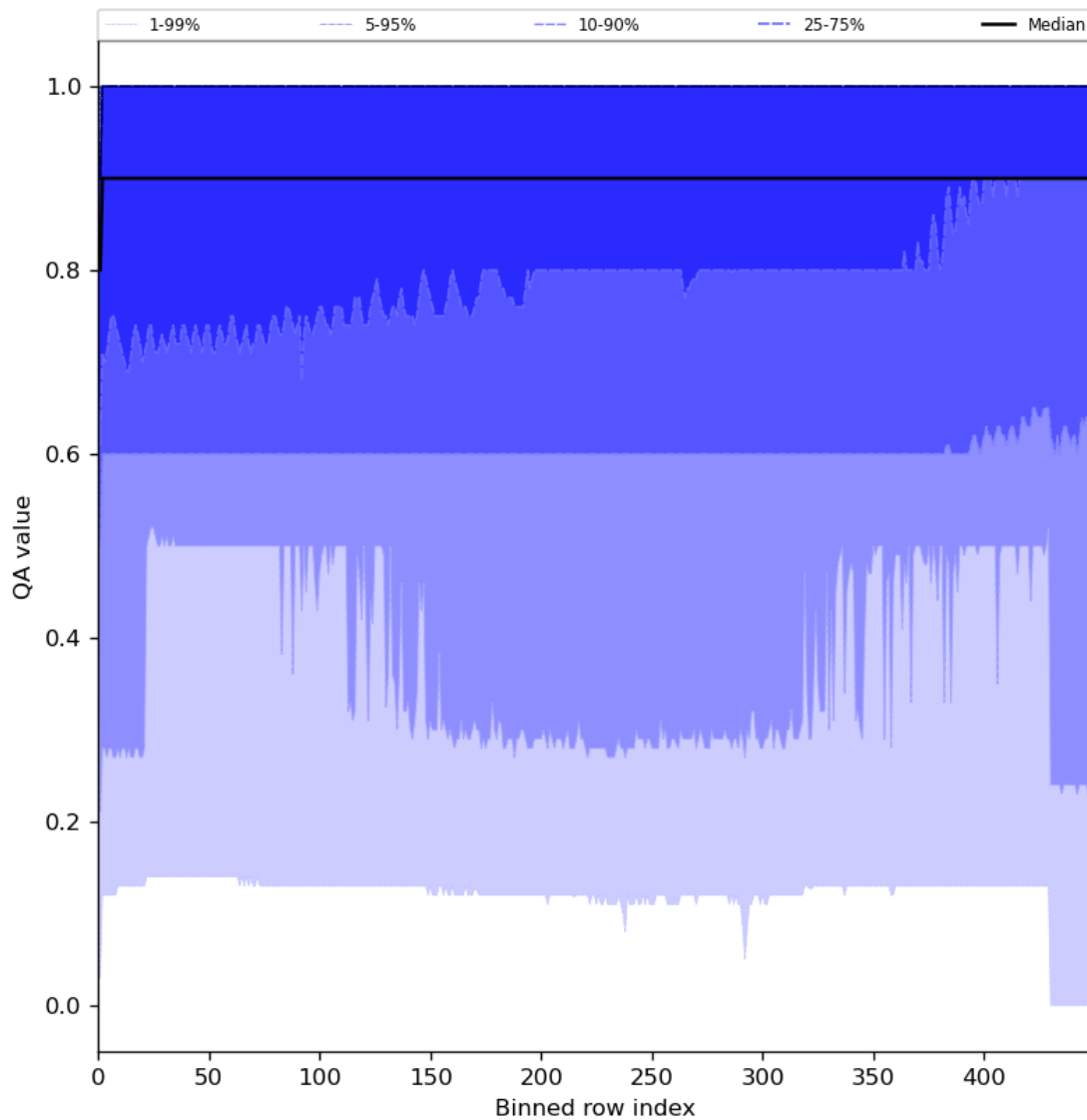
Figure 27: Along track statistics of “QA value” for 2023-12-09 to 2023-12-11
