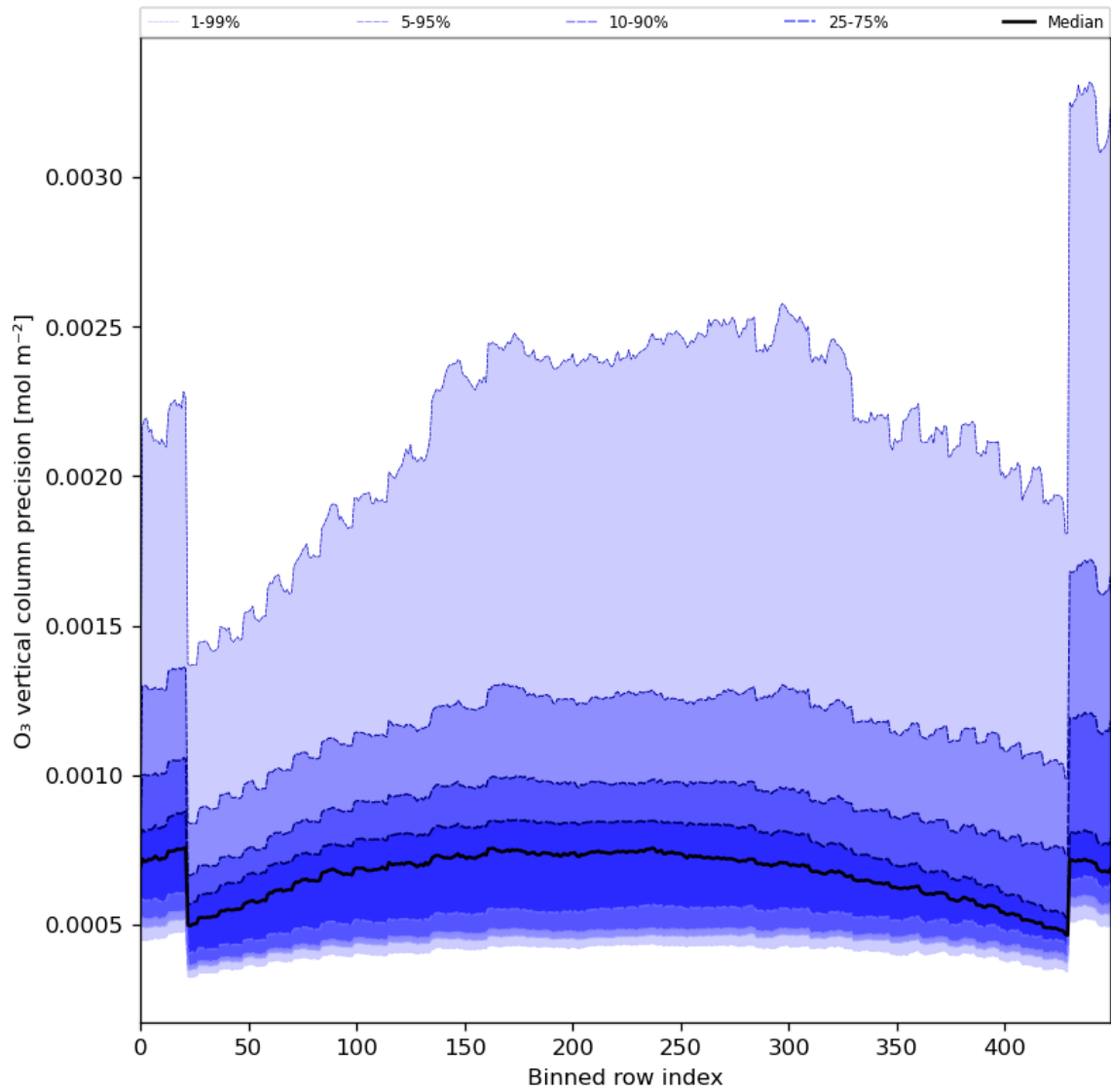
Figure 29: Along track statistics of “O 3 vertical column precision” for 2023-12-09 to 2023-12-11
