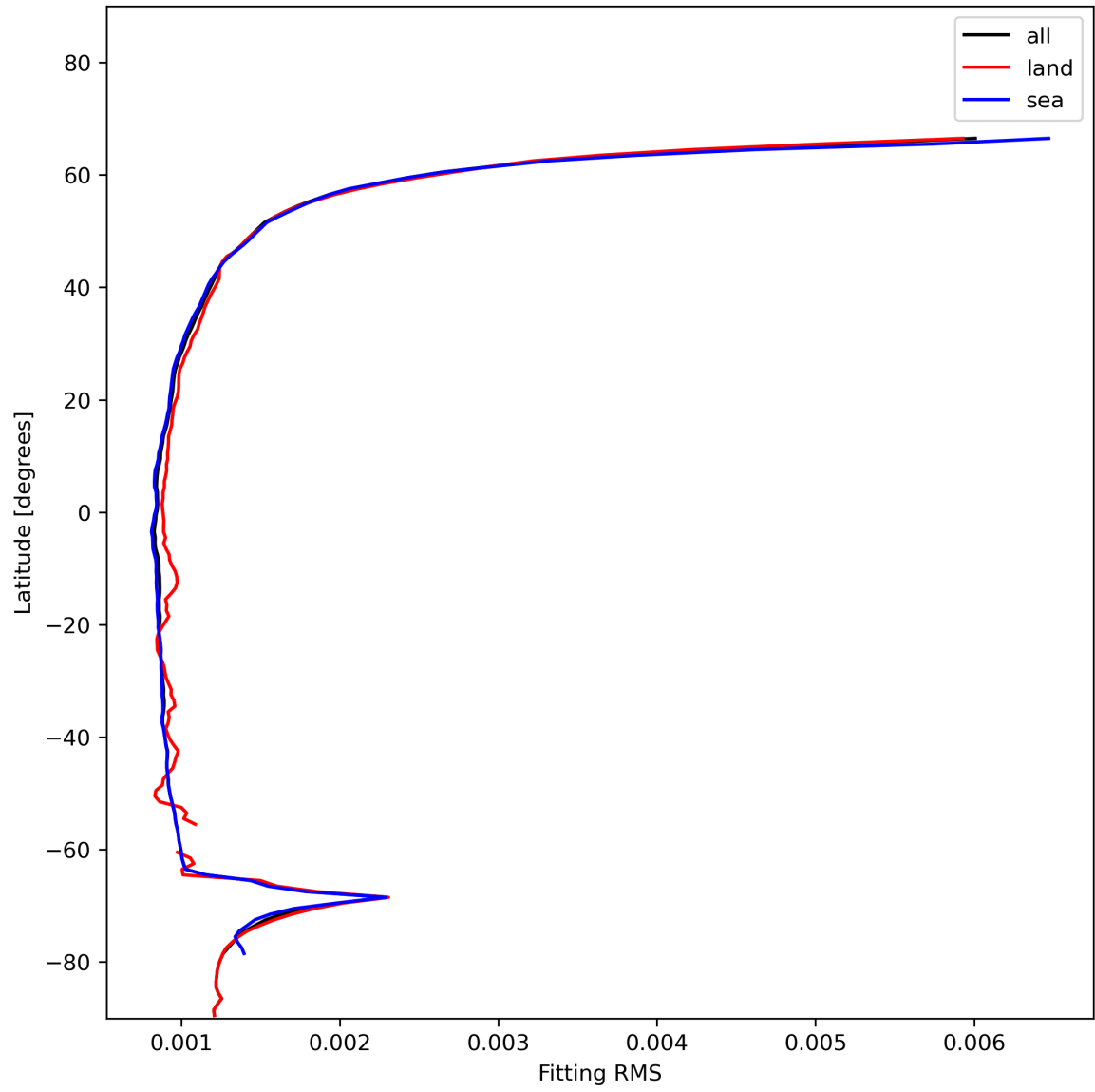
Figure 16: Zonal average of “Fitting RMS” for 2023-12-09 to 2023-12-11.
