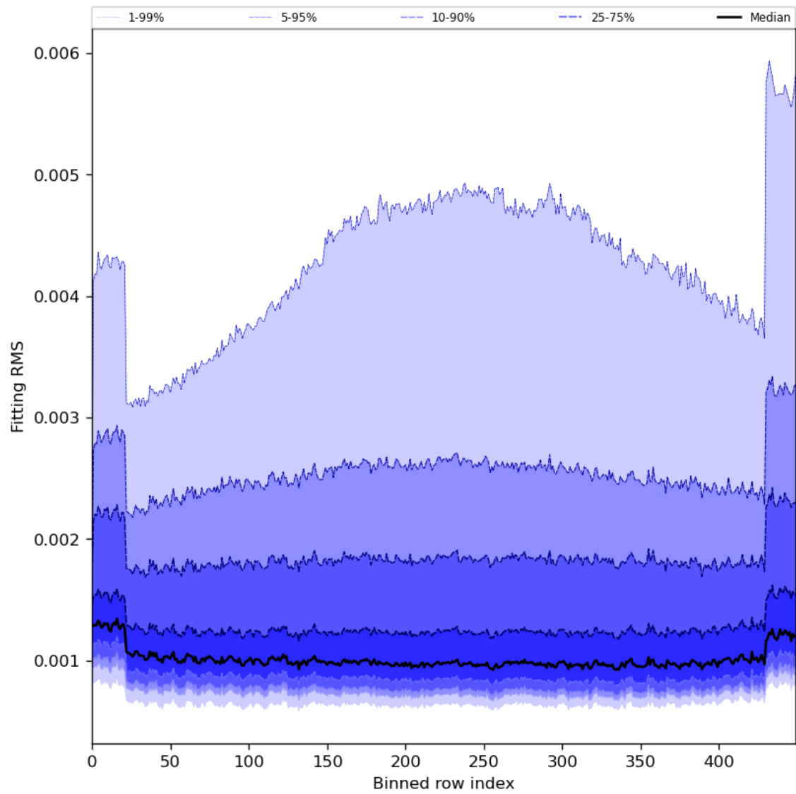
Figure 30: Along track statistics of “Fitting RMS” for 2023-12-09 to 2023-12-11
