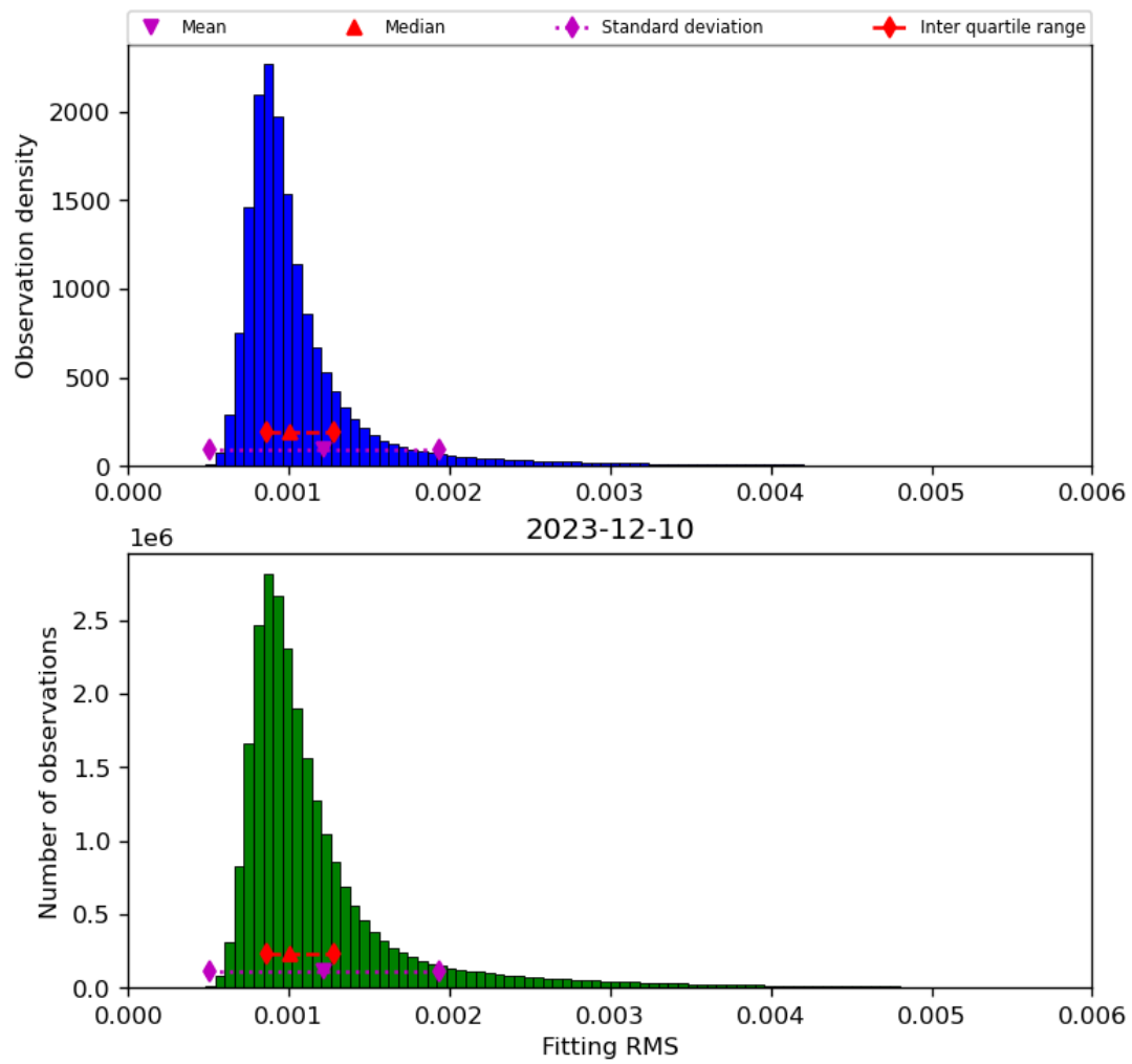
Figure 23: Histogram of “Fitting RMS” for 2023-12-09 to 2023-12-11
