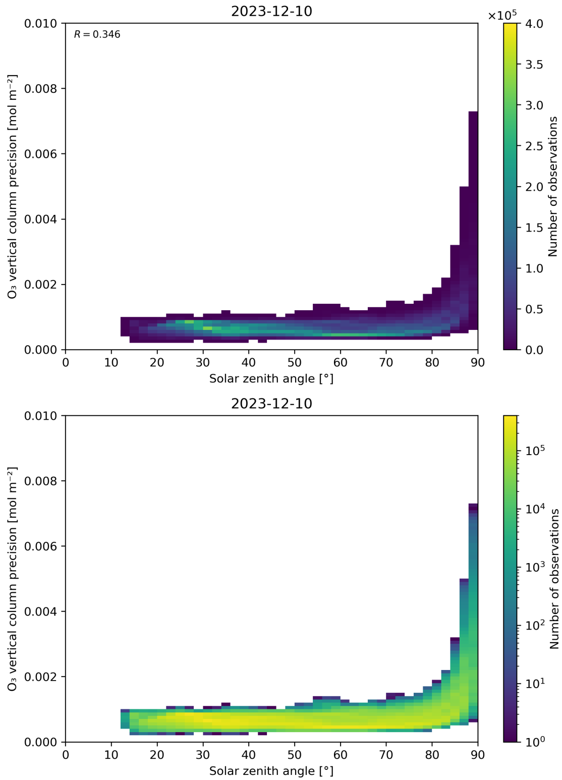
Figure 48: Scatter density plot of “Solar zenith angle” against “O 3 vertical column precision” for 2023-12-09 to 2023-12-11.
