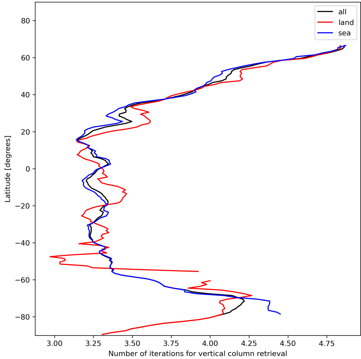
Figure 19: Zonal average of “Number of iterations for vertical column retrieval” for 2023-12-09 to 2023-12-11.
