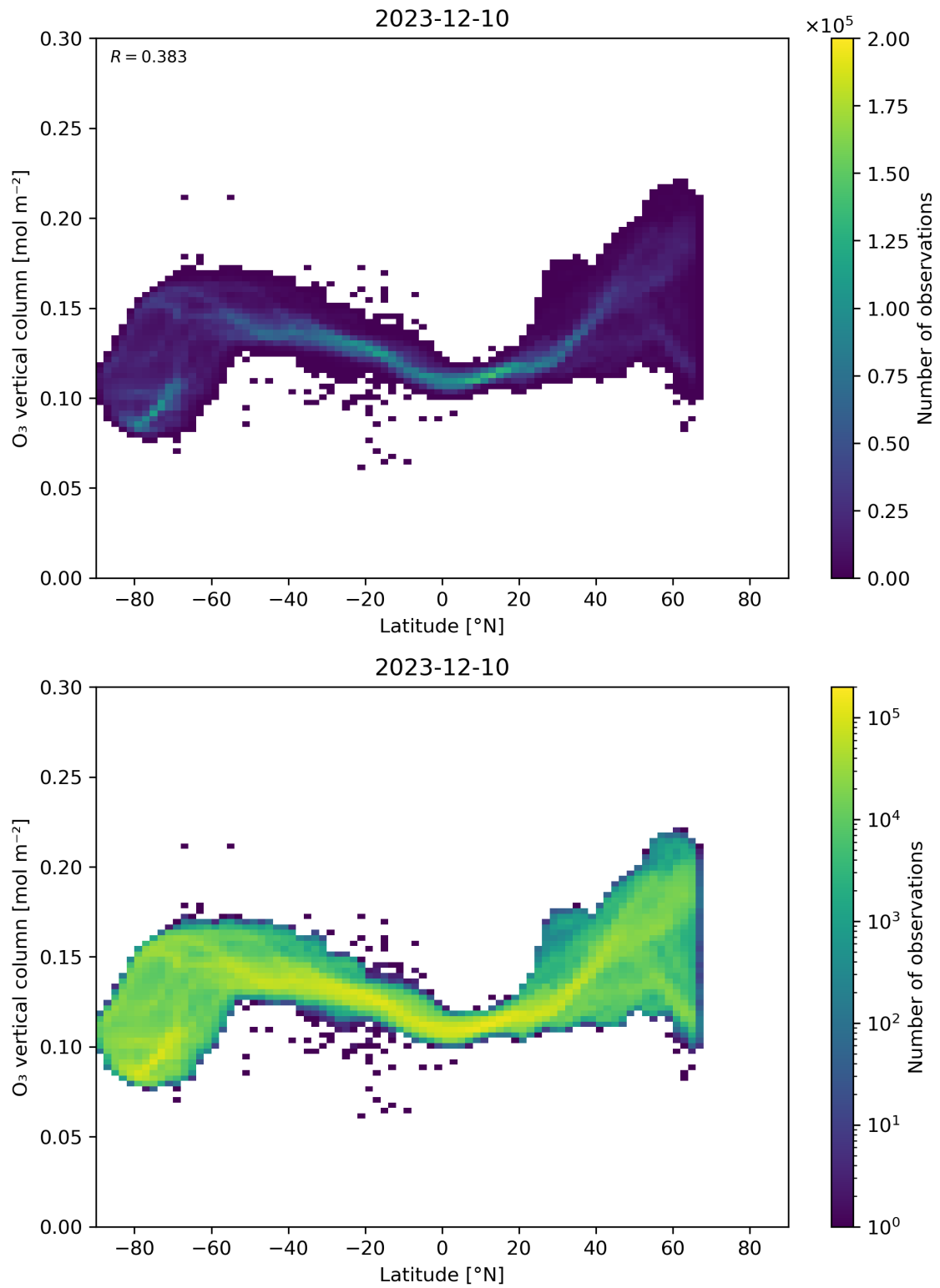
Figure 36: Scatter density plot of “Latitude” against “O 3 vertical column” for 2023-12-09 to 2023-12-11.
