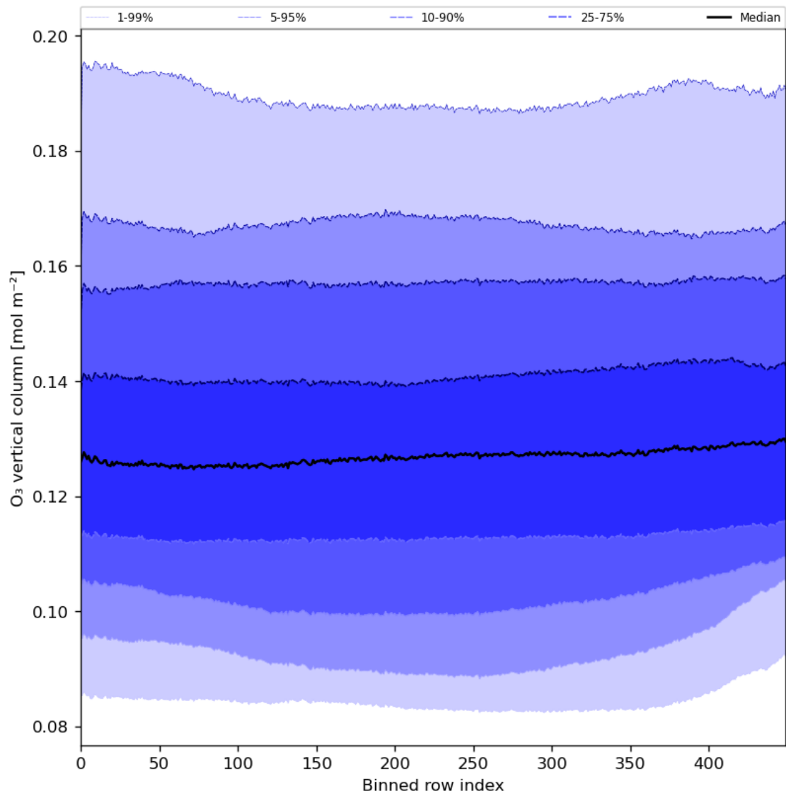
Figure 28: Along track statistics of “O 3 vertical column” for 2023-12-09 to 2023-12-11
