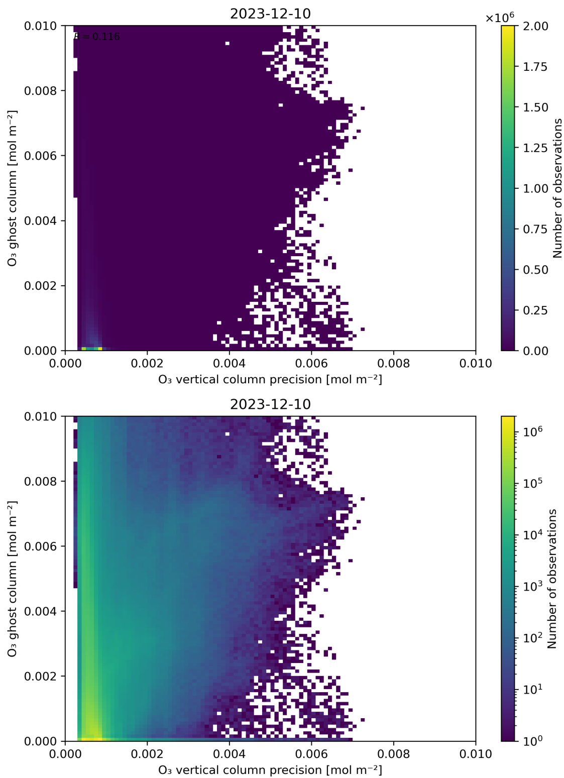
Figure 43: Scatter density plot of “ \text{O}_3 vertical column precision” against “ \text{O}_3 ghost column” for 2023-12-09 to 2023-12-11.
