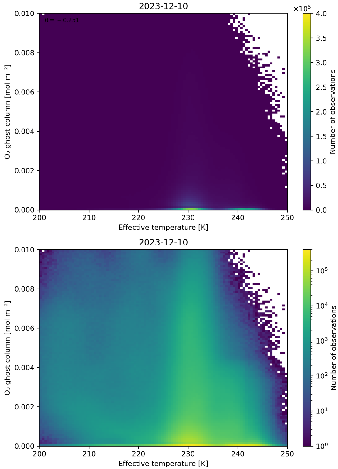
Figure 38: Scatter density plot of “Effective temperature” against “O 3 ghost column” for 2023-12-09 to 2023-12-11.
