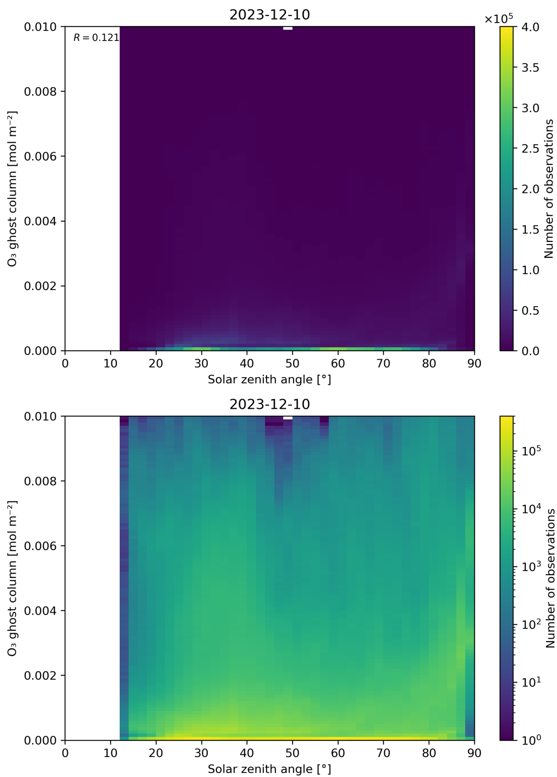
Figure 46: Scatter density plot of “Solar zenith angle” against “O 3 ghost column” for 2023-12-09 to 2023-12-11.
