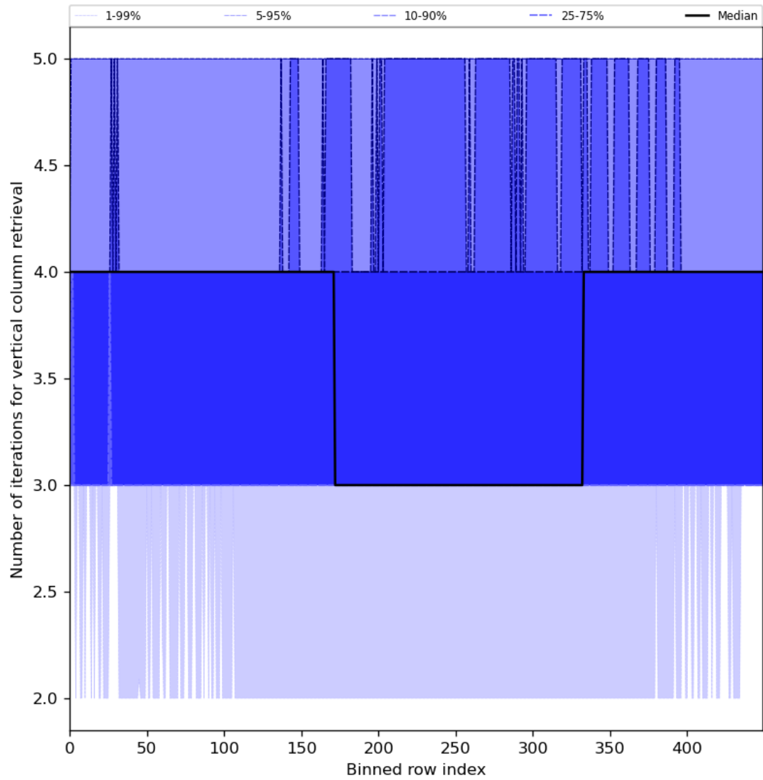
Figure 33: Along track statistics of “Number of iterations for vertical column retrieval” for 2023-12-09 to 2023-12-11
