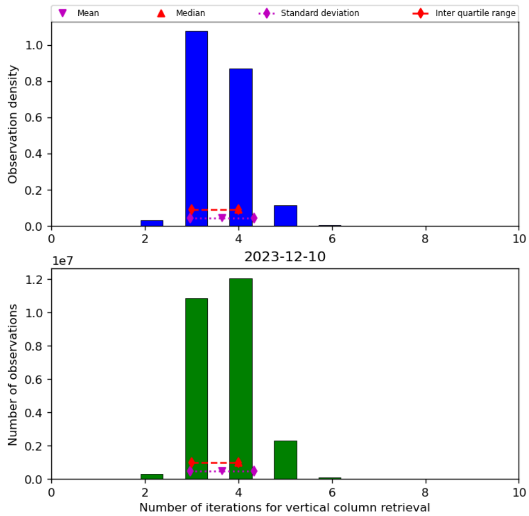
Figure 26: Histogram of “Number of iterations for vertical column retrieval” for 2023-12-09 to 2023-12-11
