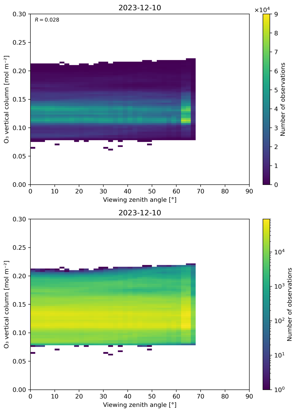
Figure 52: Scatter density plot of “Viewing zenith angle” against “O 3 vertical column” for 2023-12-09 to 2023-12-11.
