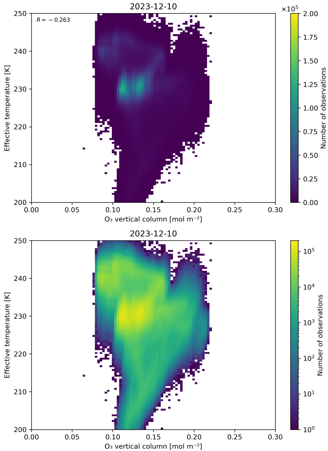
Figure 39: Scatter density plot of “O 3 vertical column” against “Effective temperature” for 2023-12-09 to 2023-12-11.
