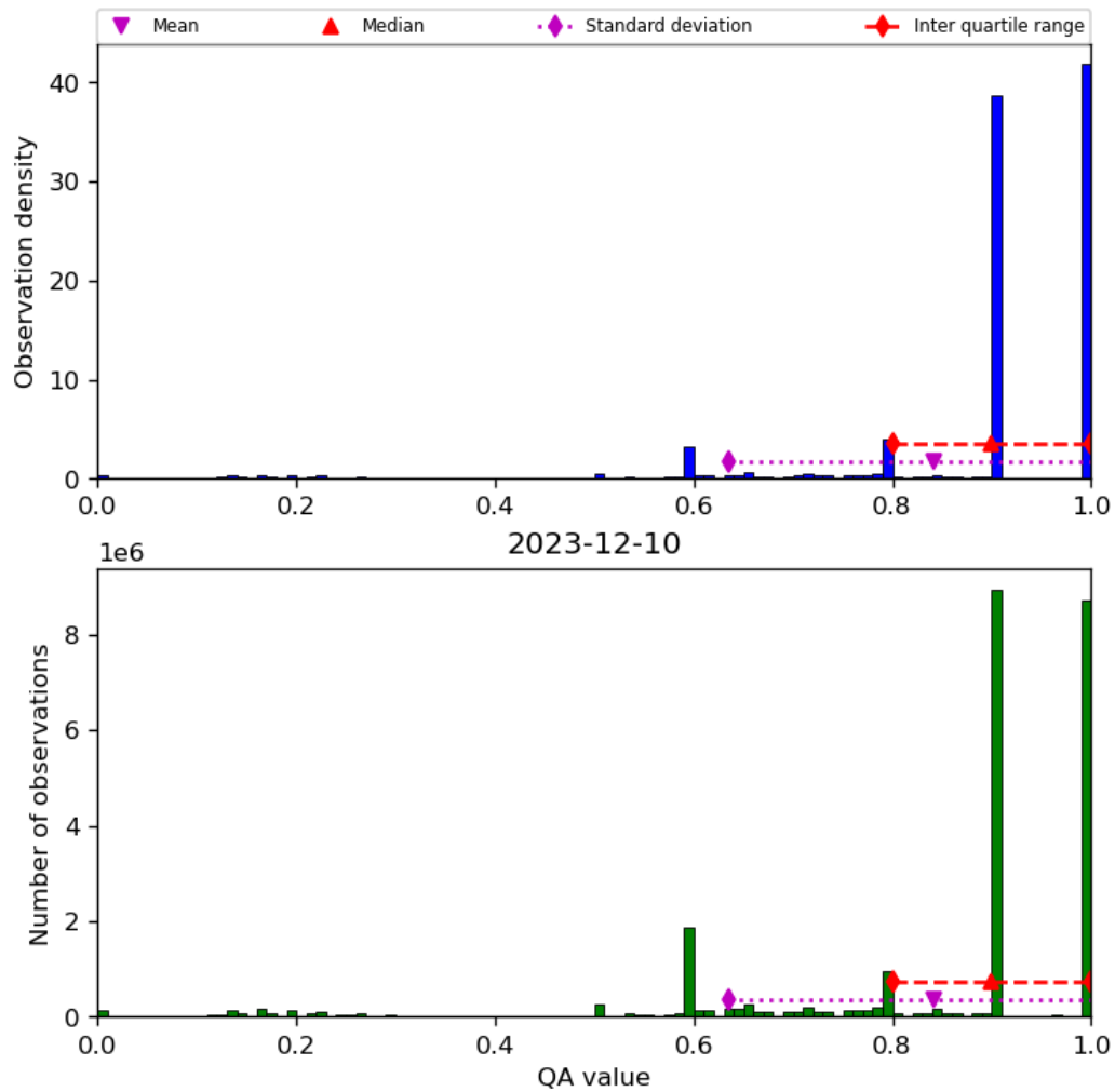
Figure 20: Histogram of “QA value” for 2023-12-09 to 2023-12-11
