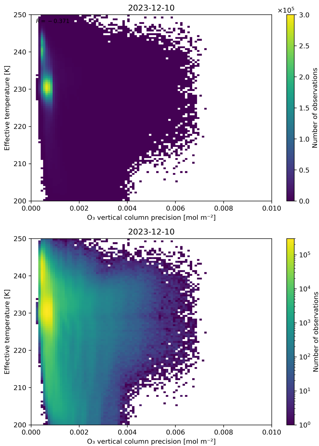
Figure 42: Scatter density plot of “O 3 vertical column precision” against “Effective temperature” for 2023-12-09 to 2023-12-11.
