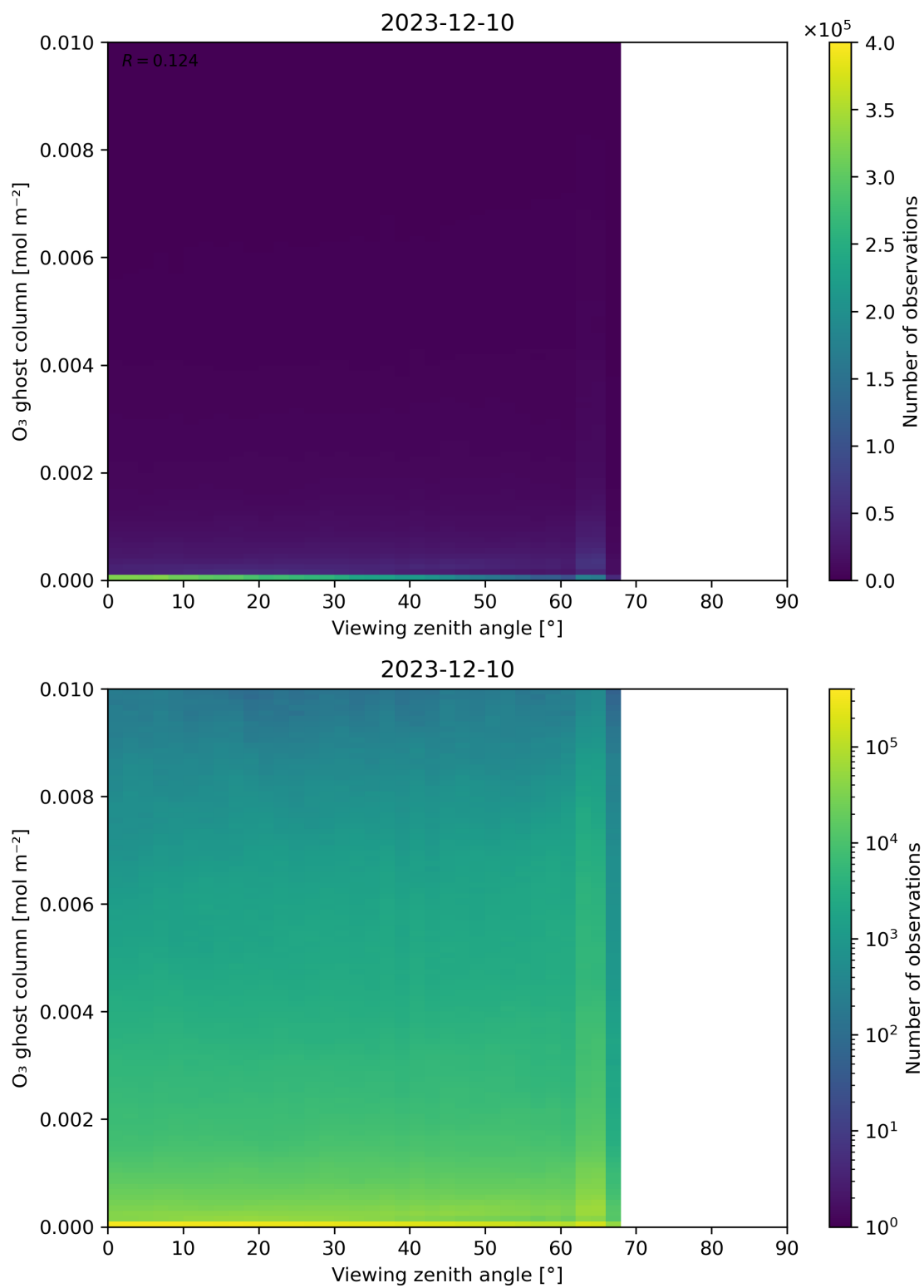
Figure 51: Scatter density plot of “Viewing zenith angle” against “O 3 ghost column” for 2023-12-09 to 2023-12-11.
