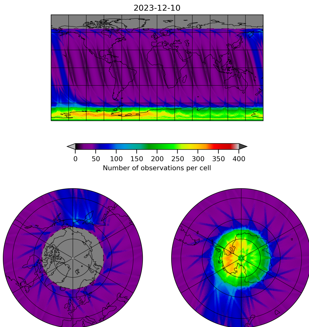
Figure 12: Map of the number of observations for 2023-12-09 to 2023-12-11
