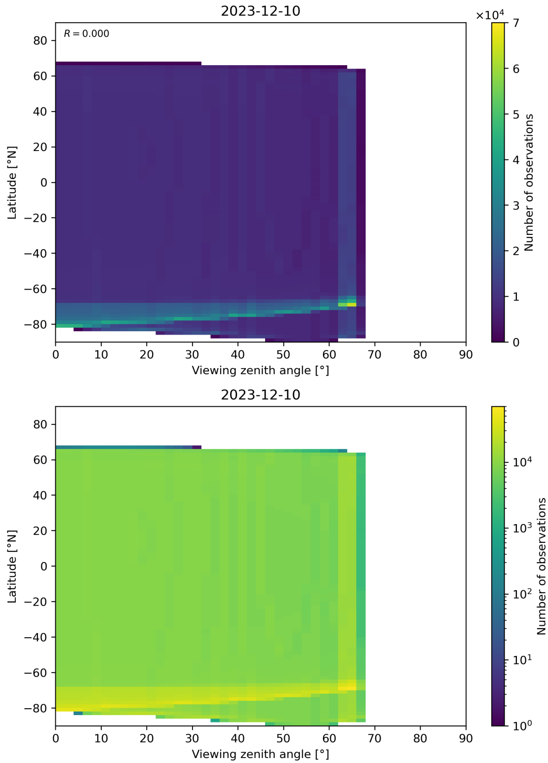
Figure 49: Scatter density plot of “Viewing zenith angle” against “Latitude” for 2023-12-09 to 2023-12-11.
