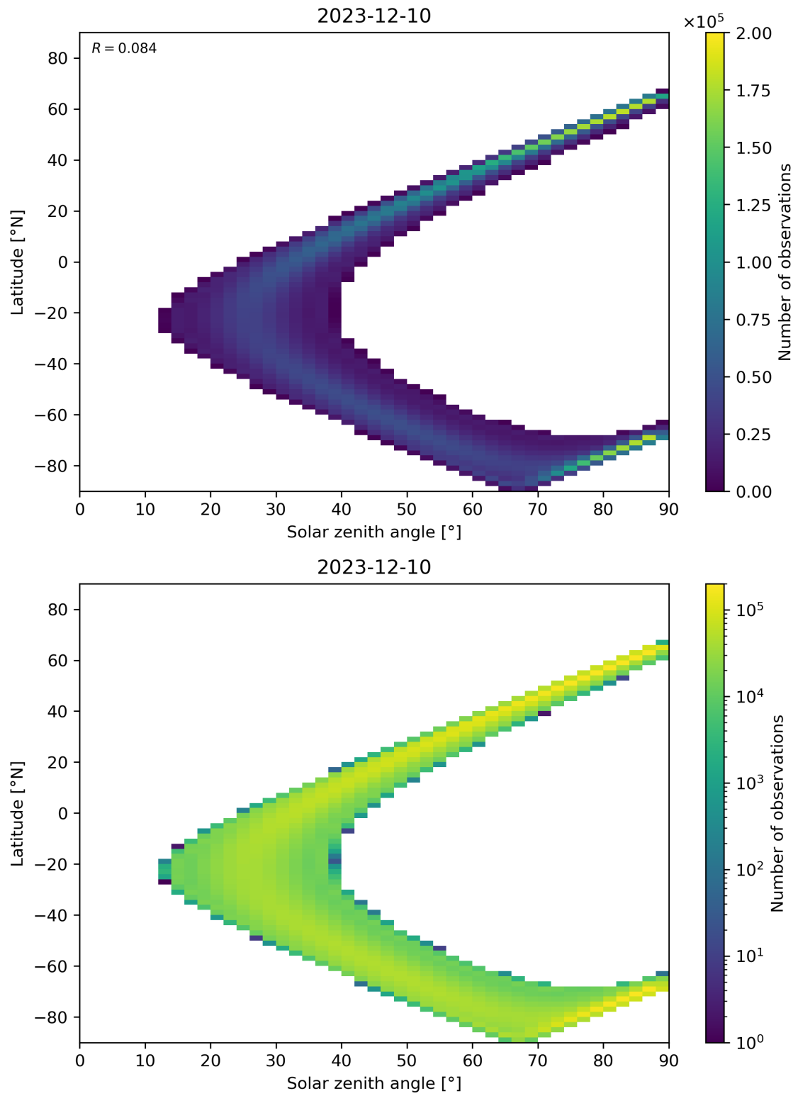
Figure 44: Scatter density plot of “Solar zenith angle” against “Latitude” for 2023-12-09 to 2023-12-11.
