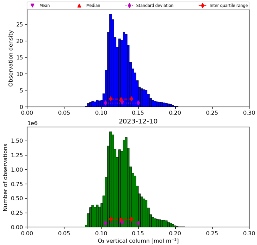
Figure 21: Histogram of “O 3 vertical column” for 2023-12-09 to 2023-12-11
