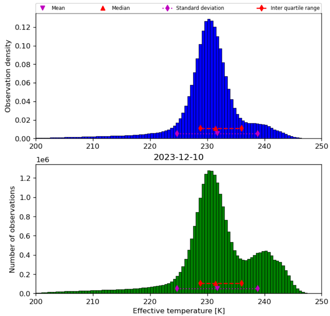
Figure 24: Histogram of “Effective temperature” for 2023-12-09 to 2023-12-11
