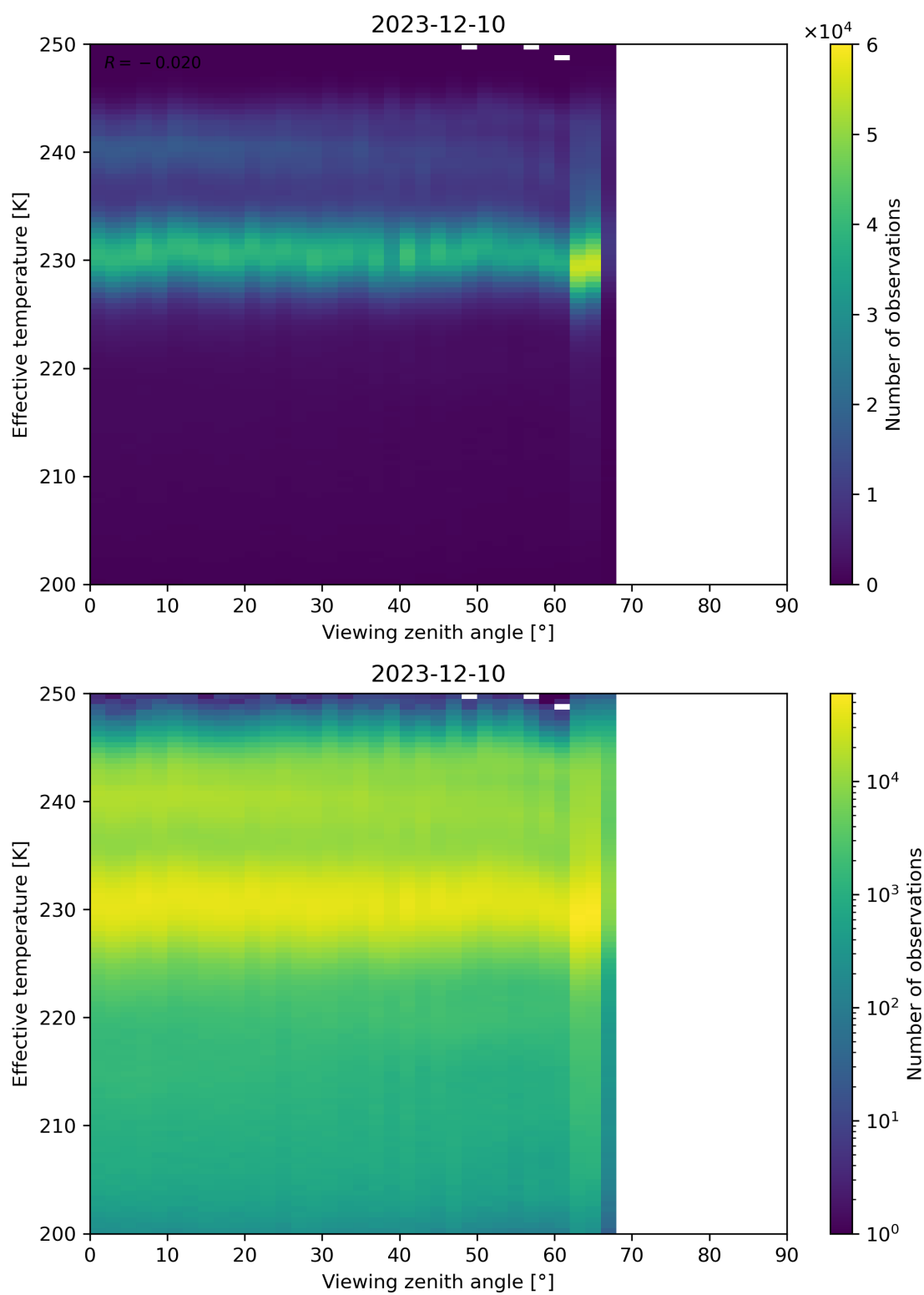
Figure 50: Scatter density plot of “Viewing zenith angle” against “Effective temperature” for 2023-12-09 to 2023-12-11.
