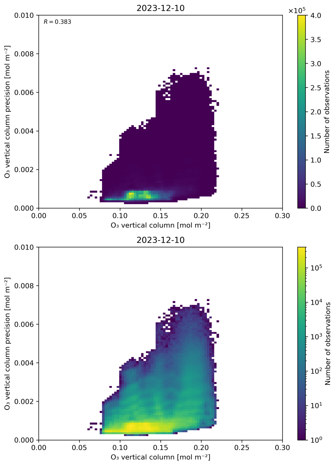
Figure 41: Scatter density plot of “O 3 vertical column” against “O 3 vertical column precision” for 2023-12-09 to 2023-12-11.
