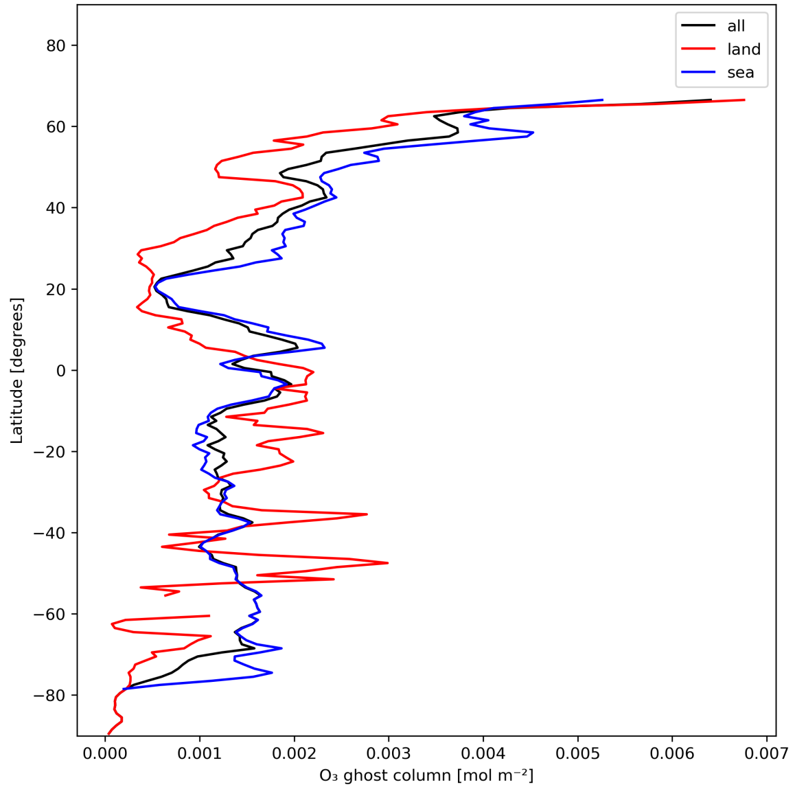
Figure 18: Zonal average of "O 3 ghost column" for 2023-12-09 to 2023-12-11.
