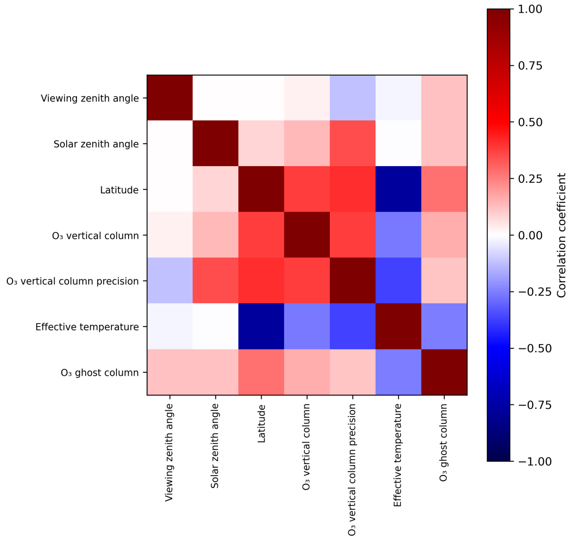
Figure 2: Map of correlation matrix for 2023-12-09 to 2023-12-11.
