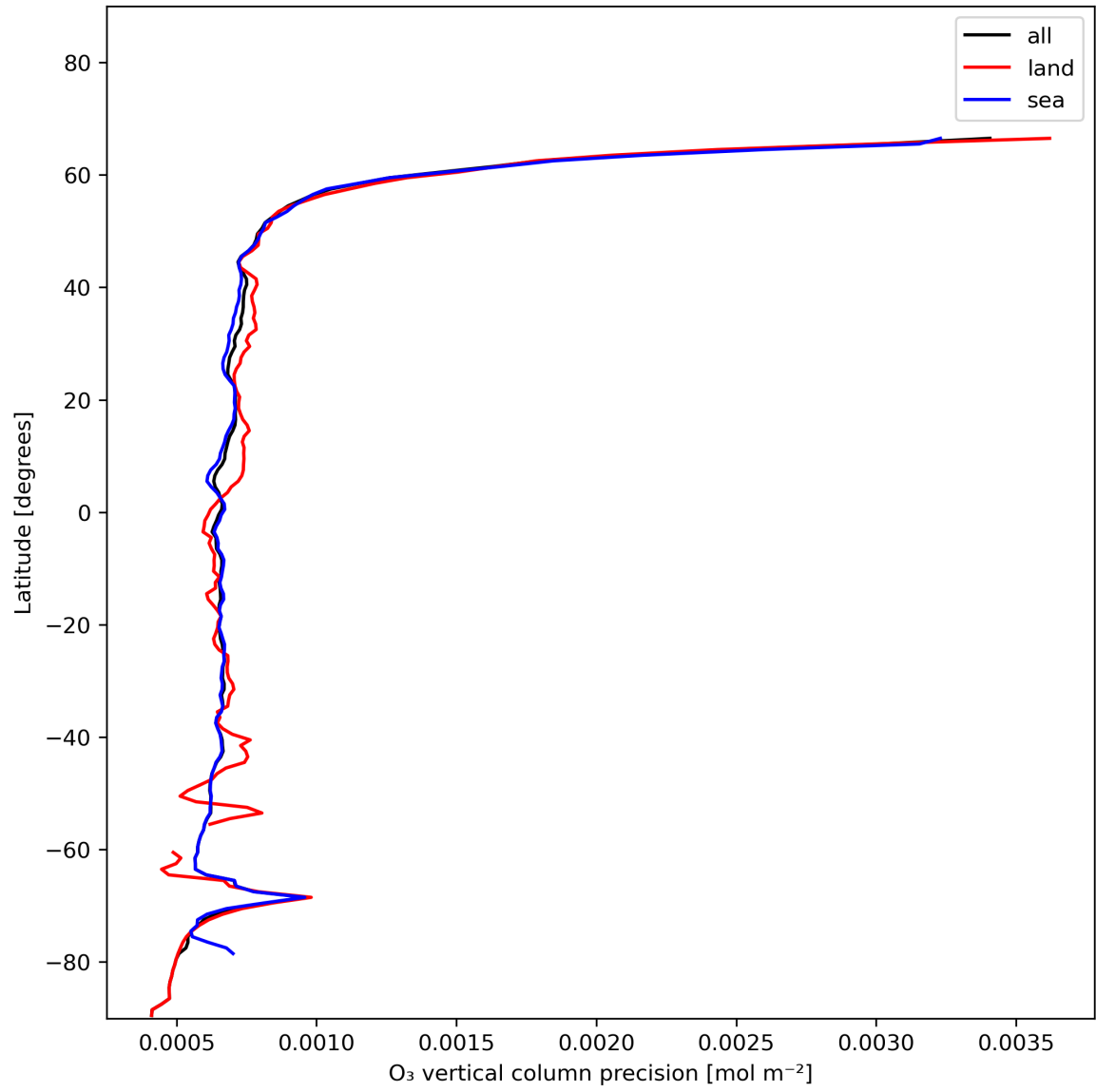
Figure 15: Zonal average of “O 3 vertical column precision” for 2023-12-09 to 2023-12-11.
