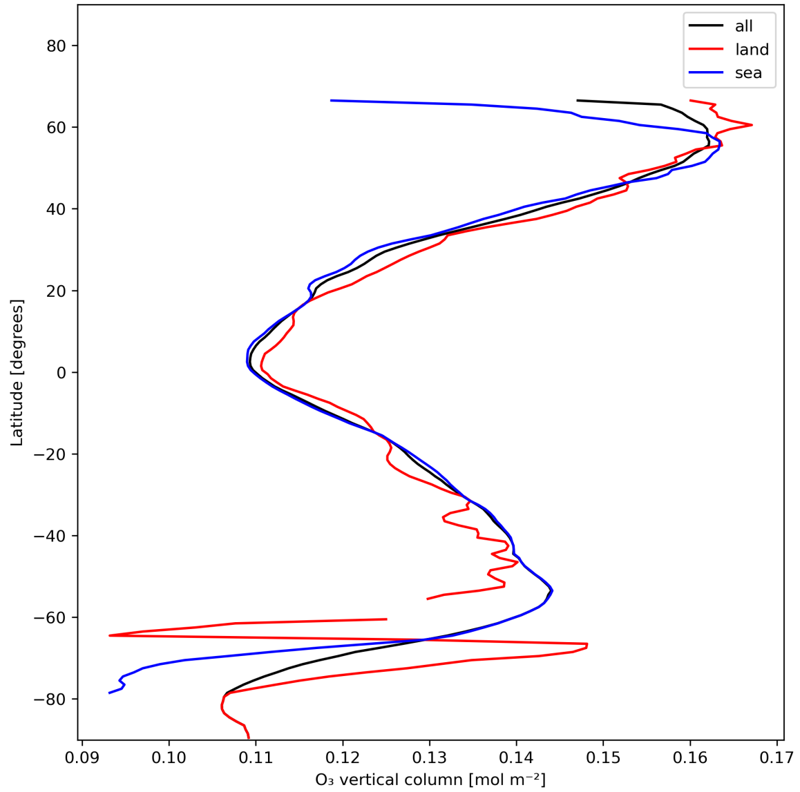
Figure 14: Zonal average of “O 3 vertical column” for 2023-12-09 to 2023-12-11.
