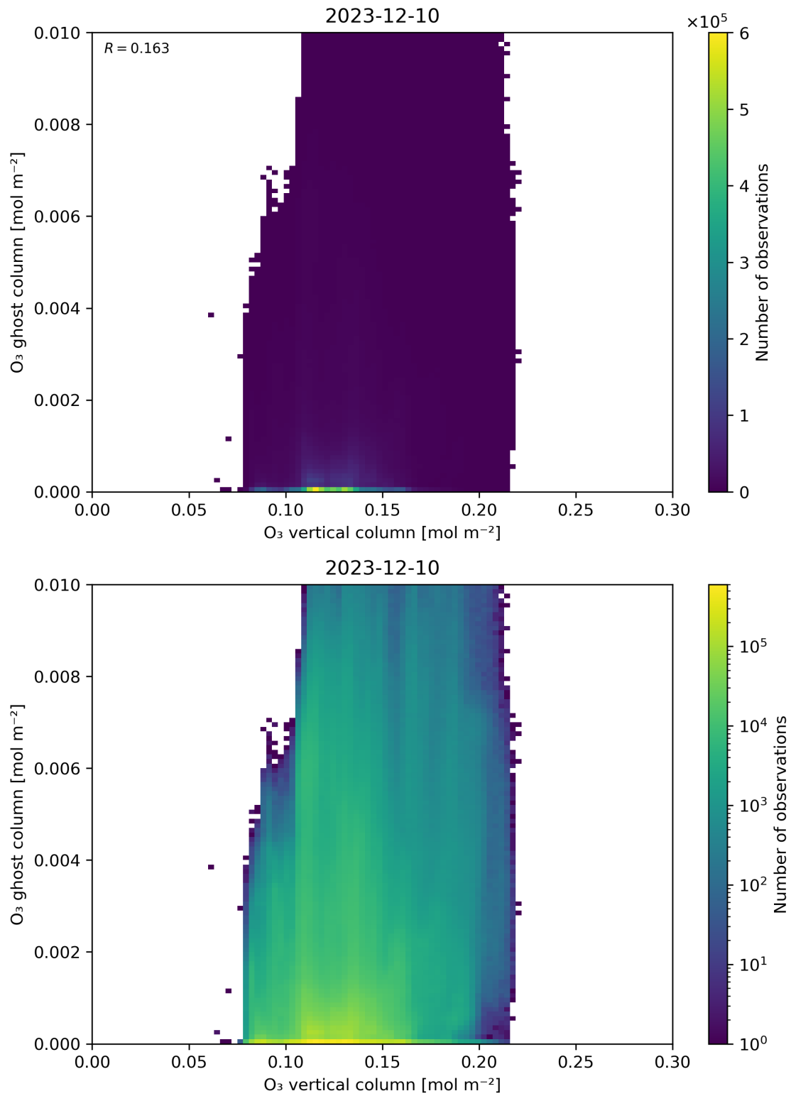
Figure 40: Scatter density plot of “O 3 vertical column” against “O 3 ghost column” for 2023-12-09 to 2023-12-11.
