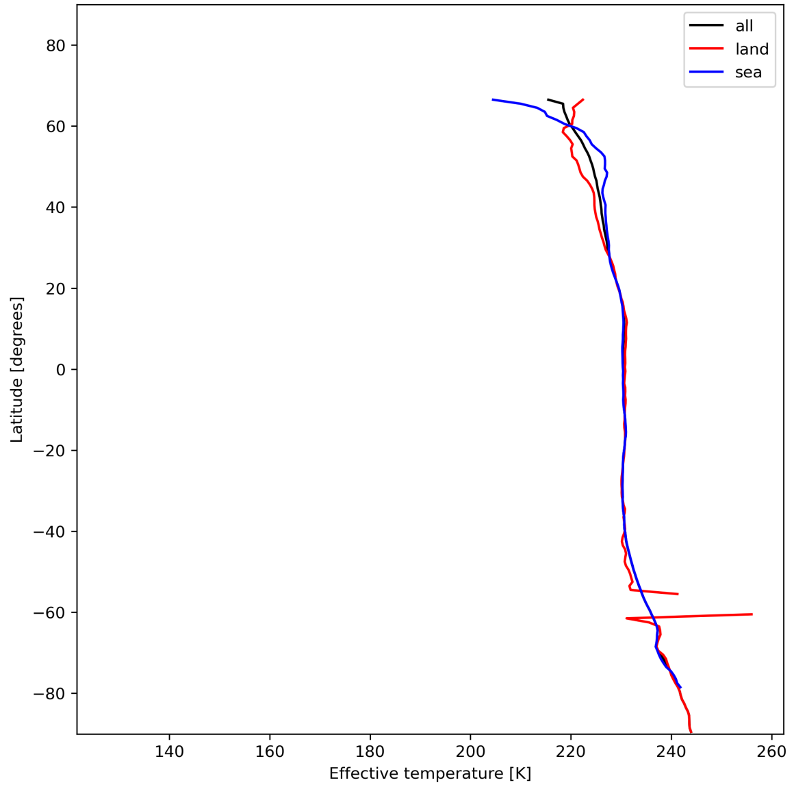
Figure 17: Zonal average of "Effective temperature" for 2023-12-09 to 2023-12-11.
