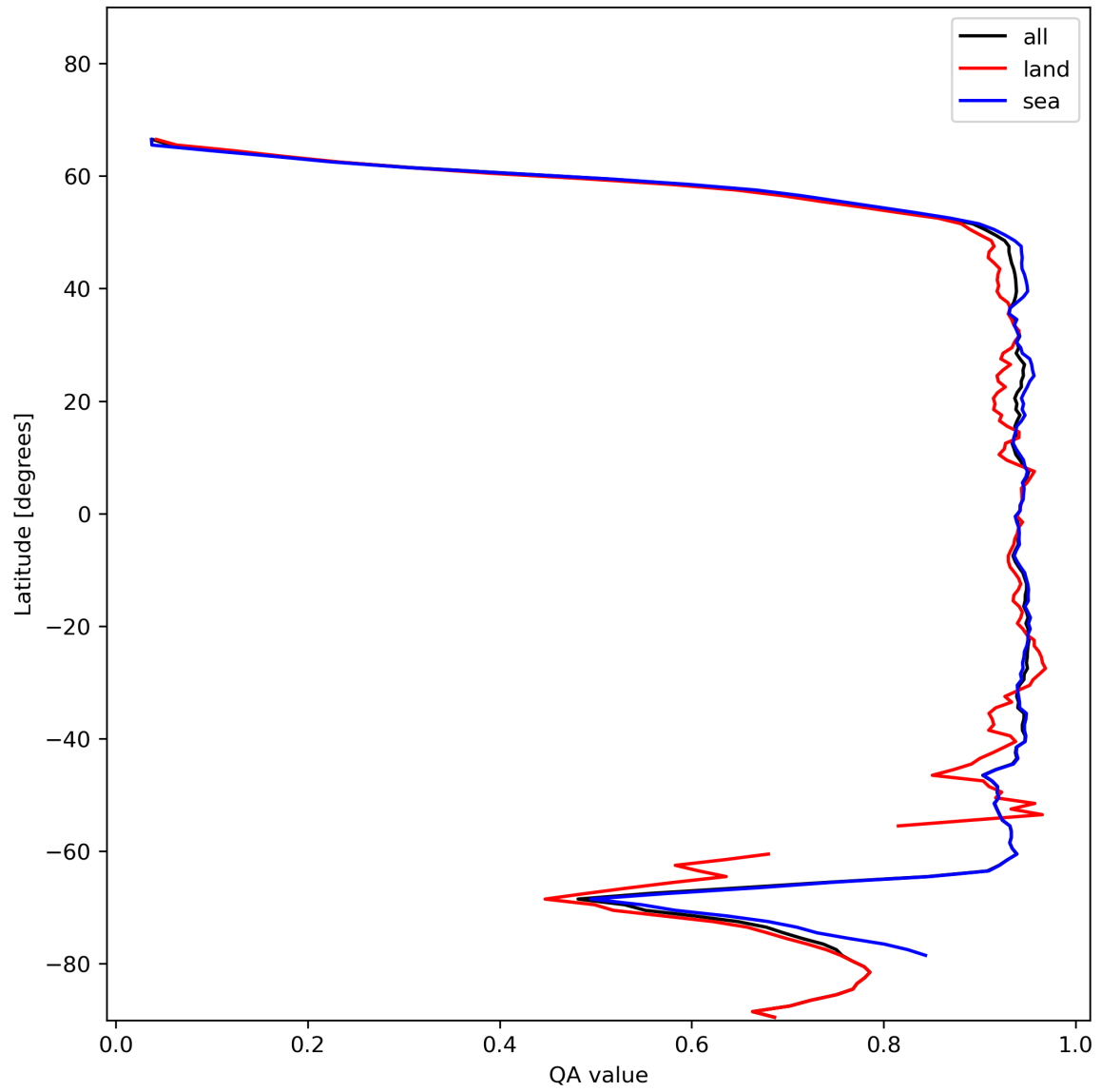
Figure 13: Zonal average of “QA value” for 2023-12-09 to 2023-12-11.
