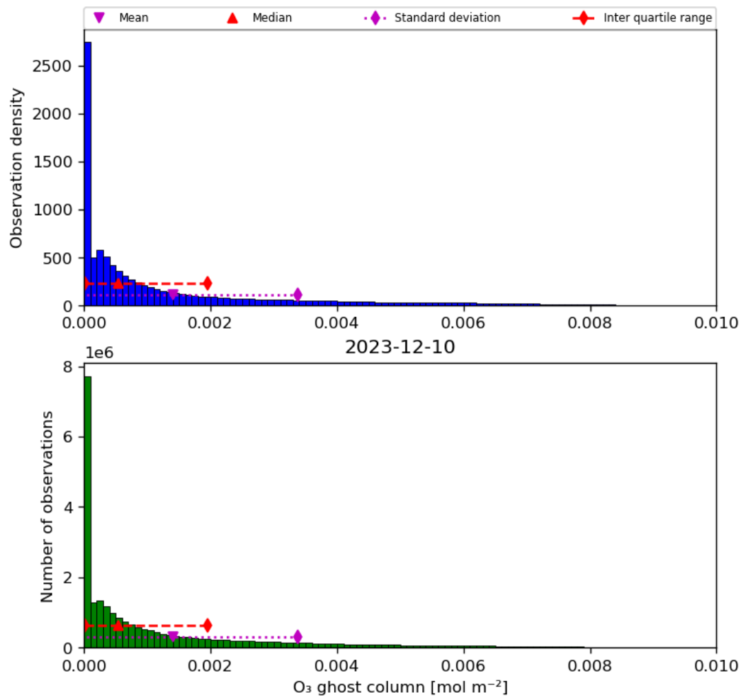
Figure 25: Histogram of “O 3 ghost column” for 2023-12-09 to 2023-12-11
