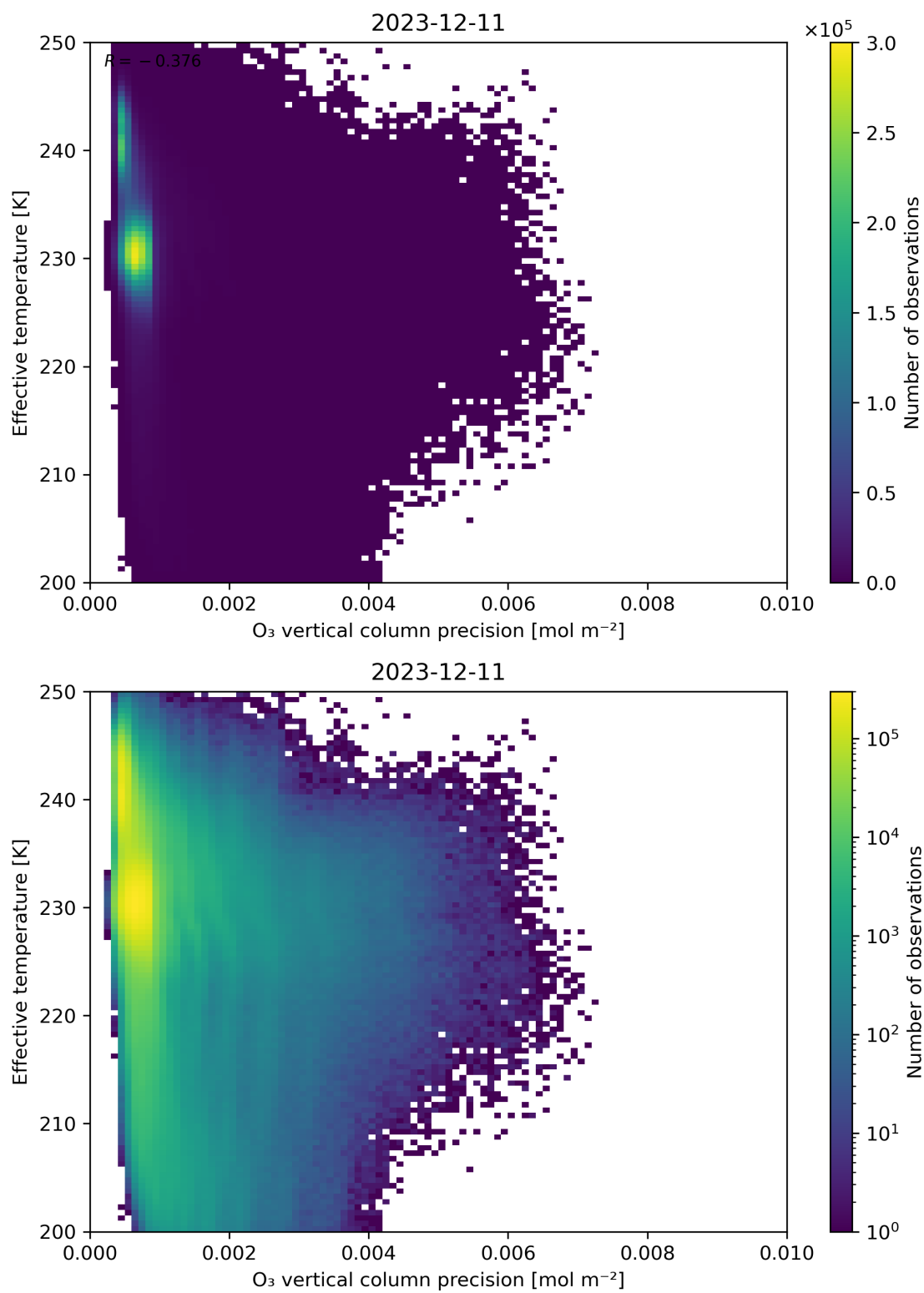
Figure 42: Scatter density plot of “O 3 vertical column precision” against “Effective temperature” for 2023-12-10 to 2023-12-12.
