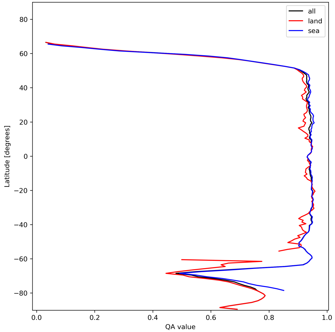
Figure 13: Zonal average of “QA value” for 2023-12-10 to 2023-12-12.
