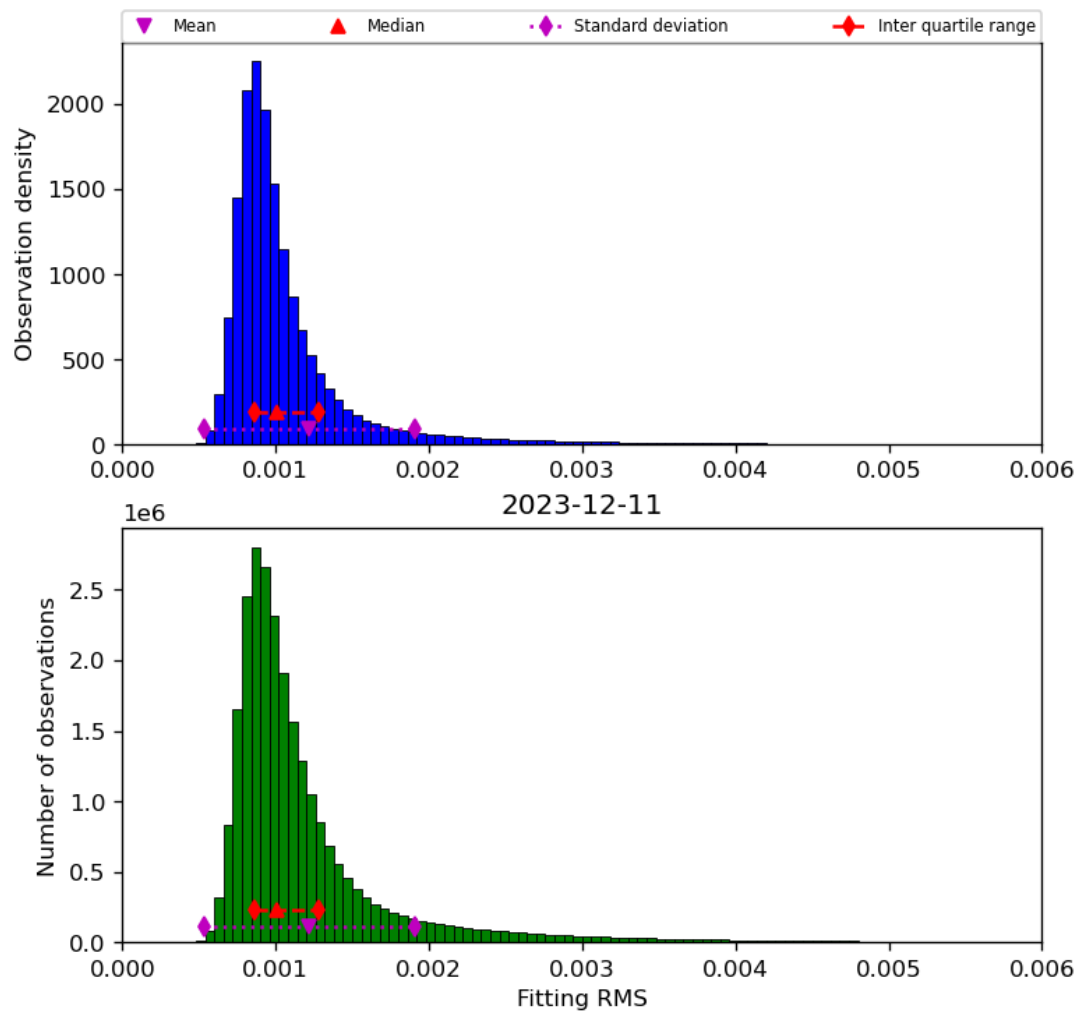
Figure 23: Histogram of “Fitting RMS” for 2023-12-10 to 2023-12-12
