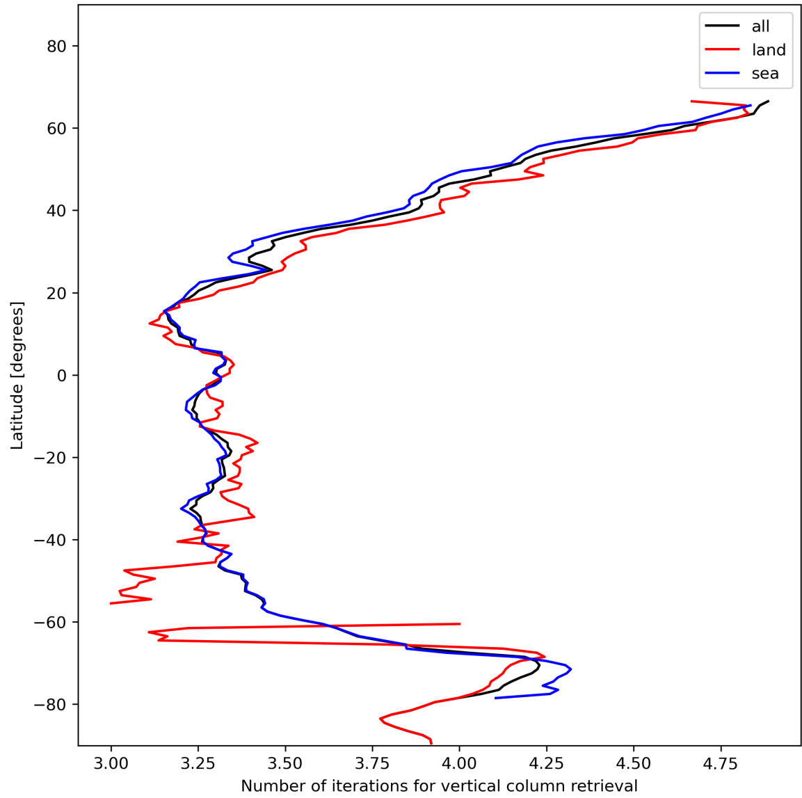
Figure 19: Zonal average of “Number of iterations for vertical column retrieval” for 2023-12-10 to 2023-12-12.
