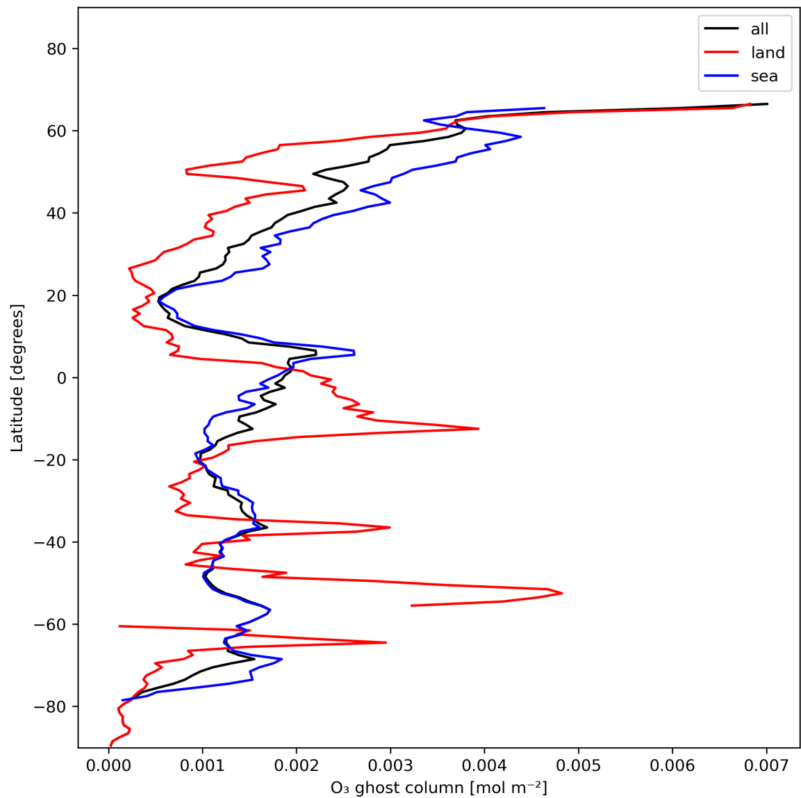
Figure 18: Zonal average of “O 3 ghost column” for 2023-12-10 to 2023-12-12.
