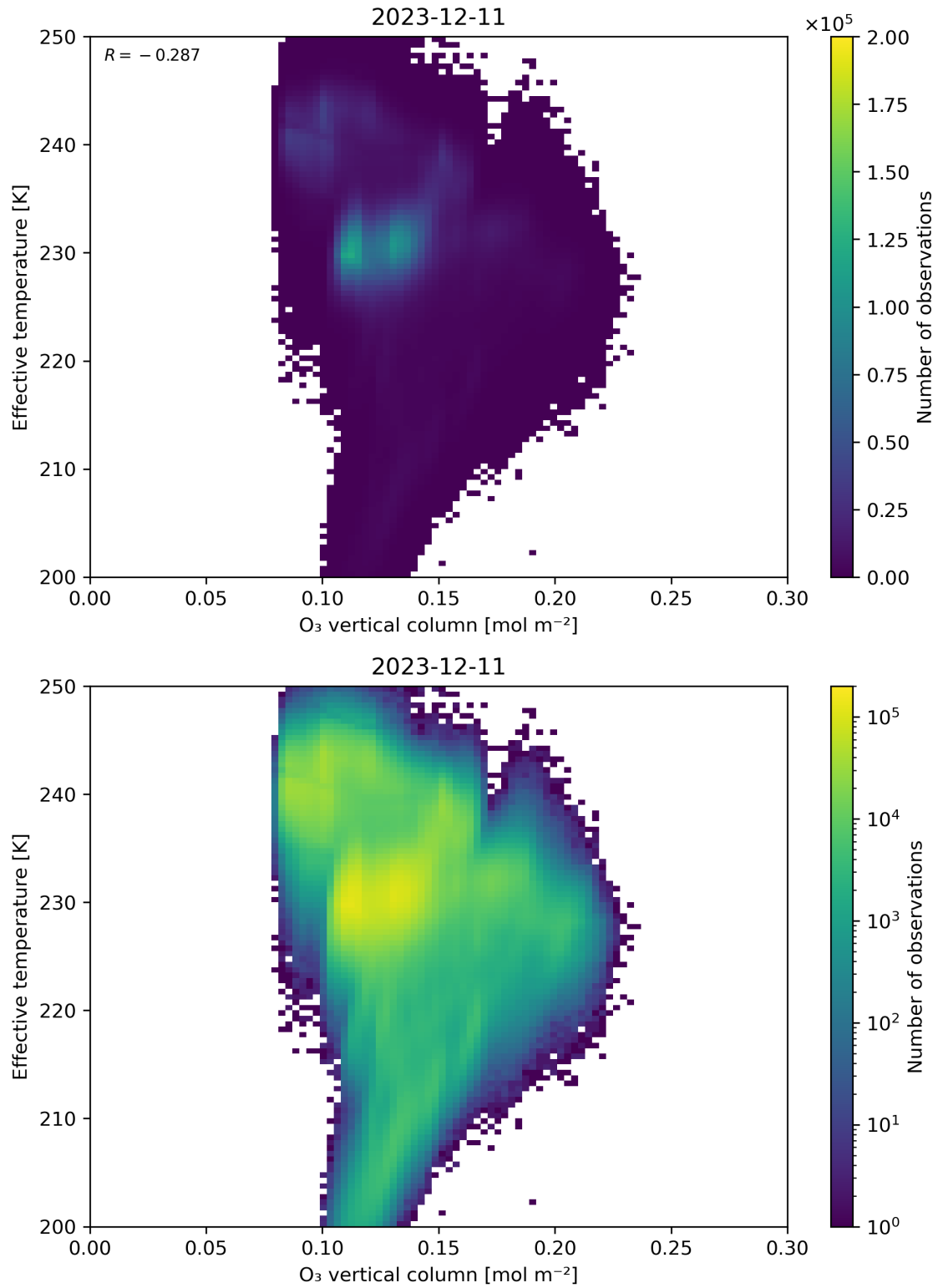
Figure 39: Scatter density plot of “O 3 vertical column” against “Effective temperature” for 2023-12-10 to 2023-12-12.
