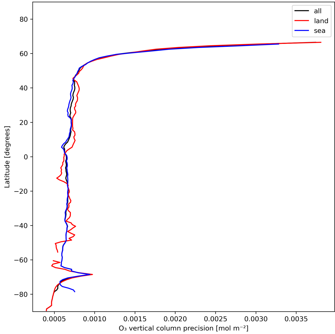
Figure 15: Zonal average of “O 3 vertical column precision” for 2023-12-10 to 2023-12-12.
