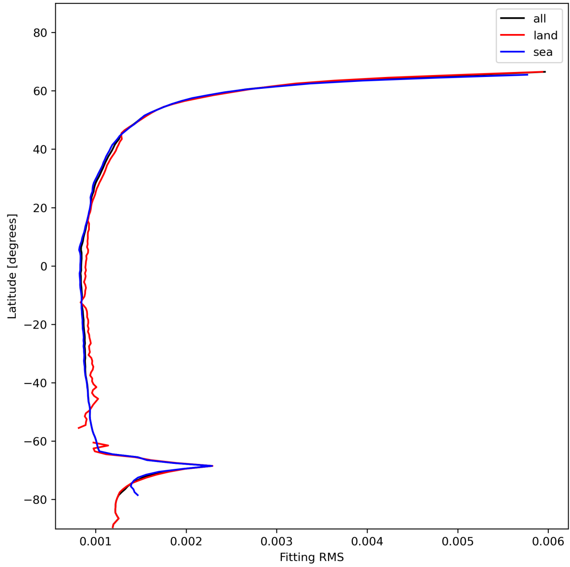
Figure 16: Zonal average of “Fitting RMS” for 2023-12-10 to 2023-12-12.
