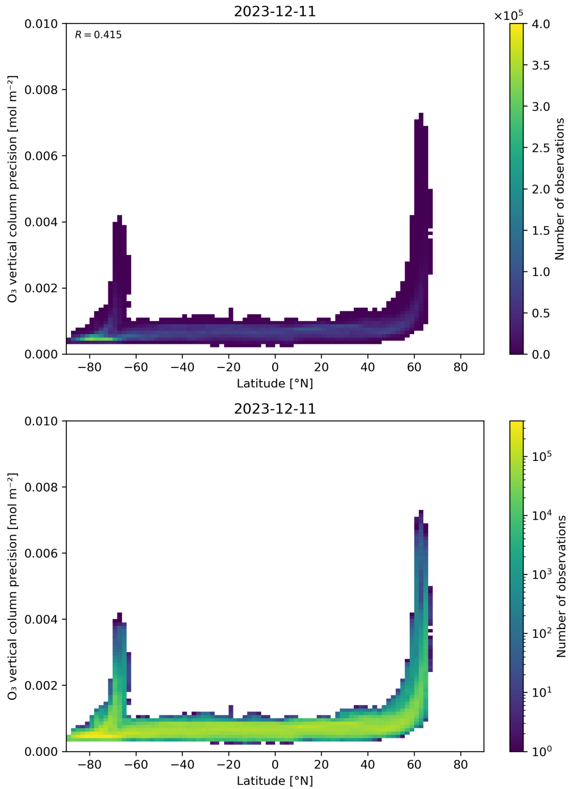
Figure 37: Scatter density plot of “Latitude” against “O 3 vertical column precision” for 2023-12-10 to 2023-12-12.
