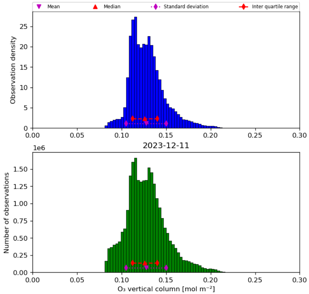
Figure 21: Histogram of “O 3 vertical column” for 2023-12-10 to 2023-12-12
