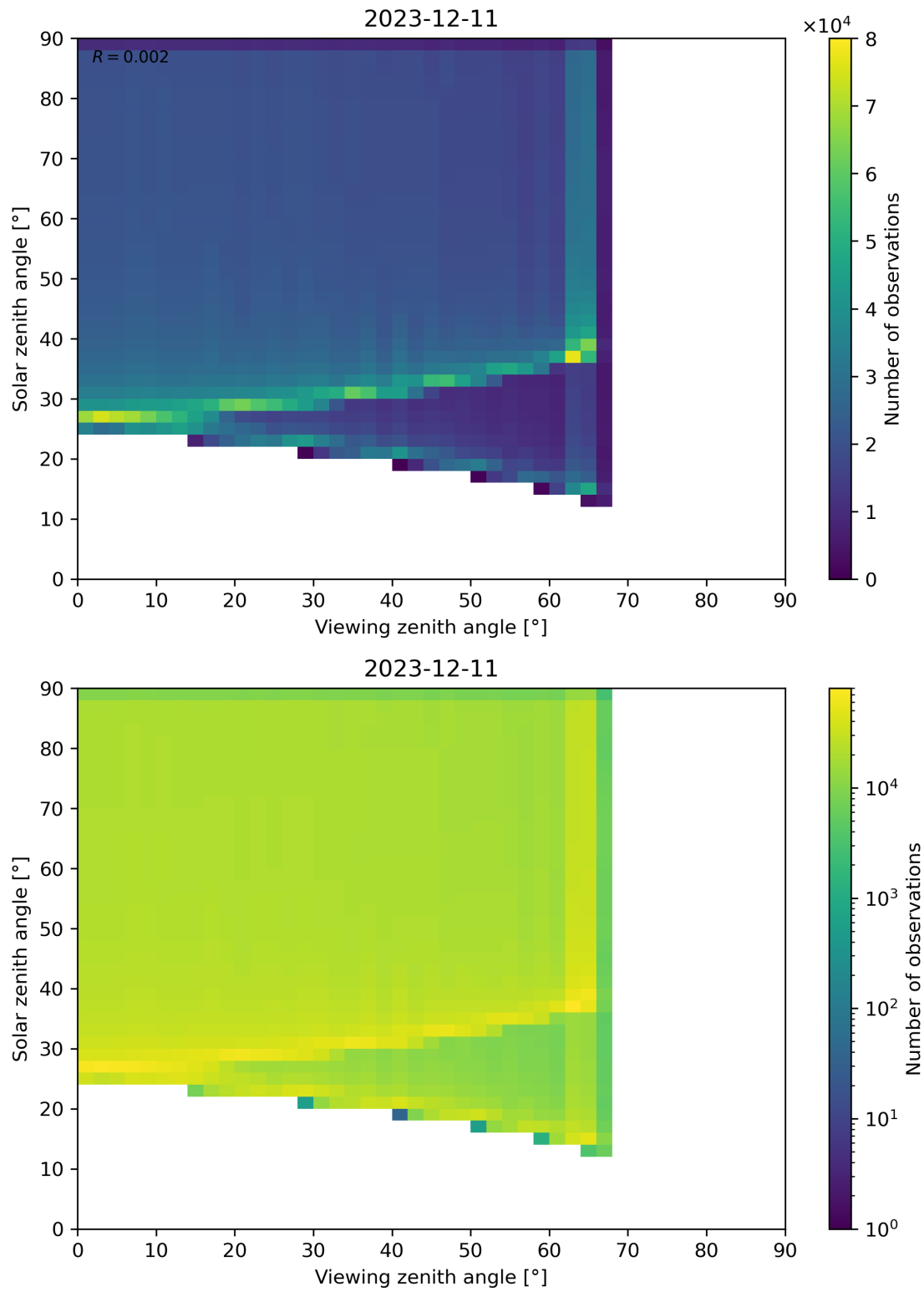
Figure 54: Scatter density plot of “Viewing zenith angle” against “Solar zenith angle” for 2023-12-10 to 2023-12-12.
