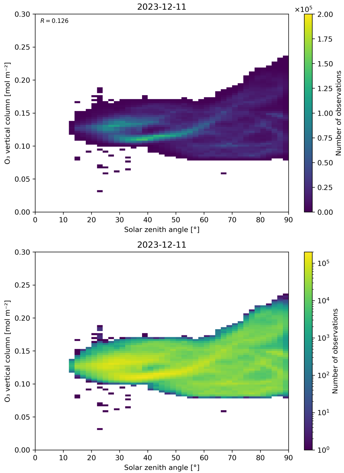
Figure 47: Scatter density plot of “Solar zenith angle” against “O 3 vertical column” for 2023-12-10 to 2023-12-12.
