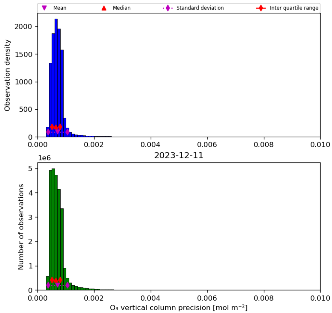
Figure 22: Histogram of “O 3 vertical column precision” for 2023-12-10 to 2023-12-12
