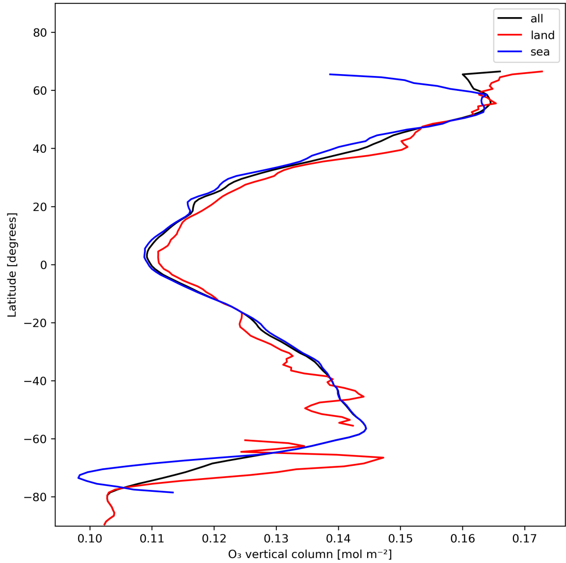
Figure 14: Zonal average of “O 3 vertical column” for 2023-12-10 to 2023-12-12.
