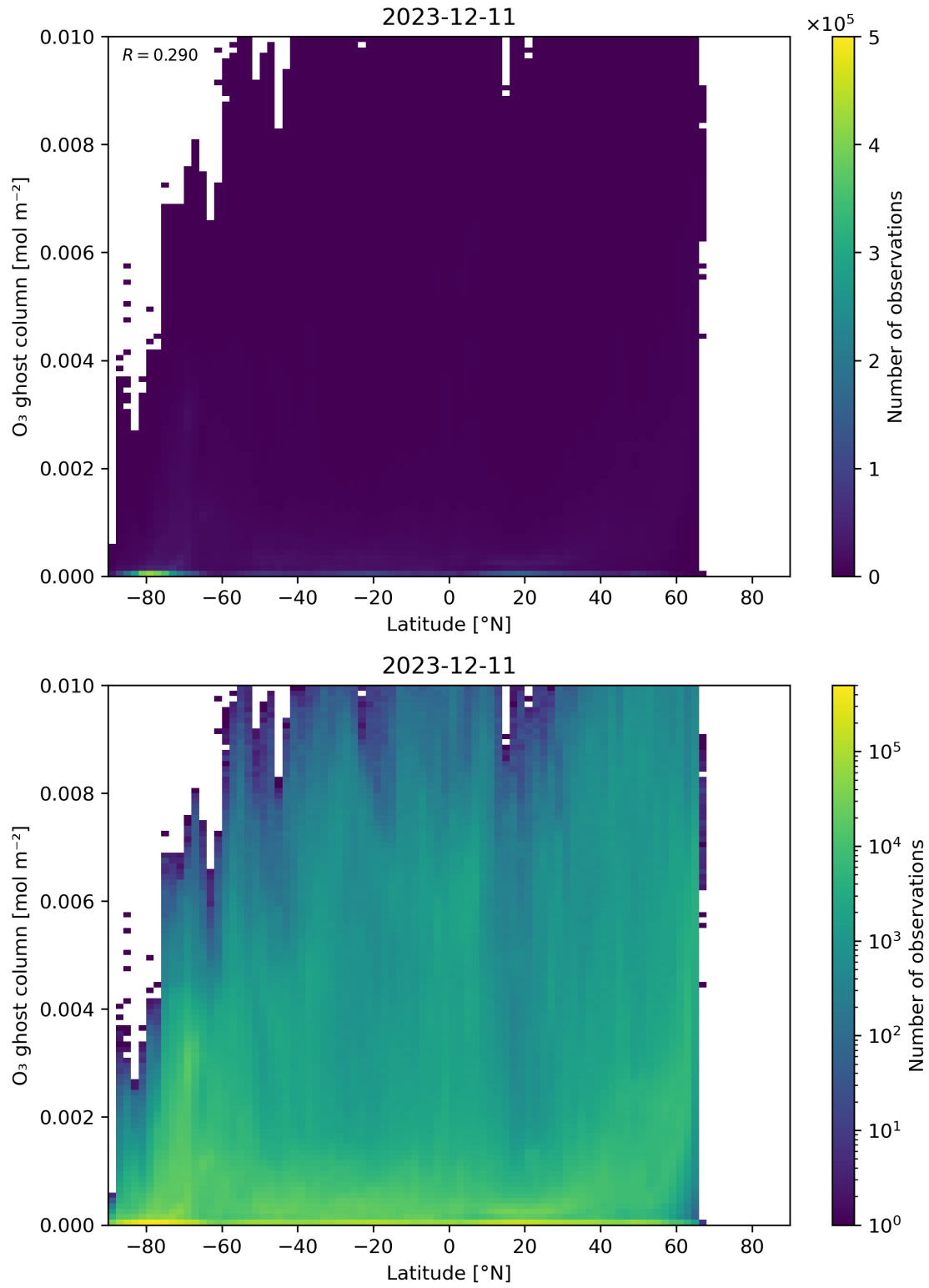
Figure 35: Scatter density plot of “Latitude” against “O 3 ghost column” for 2023-12-10 to 2023-12-12.
