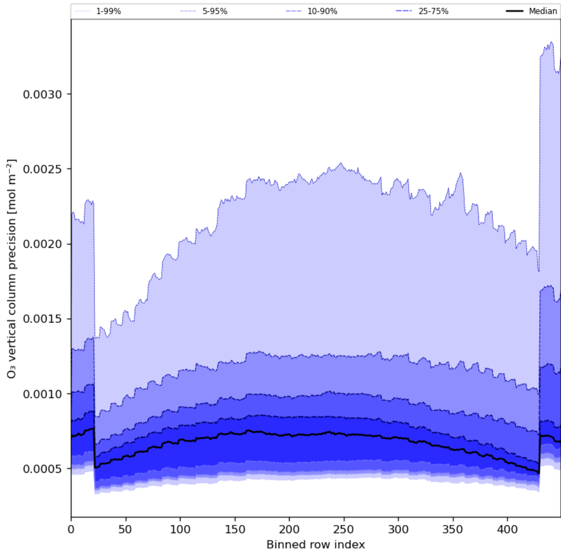
Figure 29: Along track statistics of “O 3 vertical column precision” for 2023-12-10 to 2023-12-12
