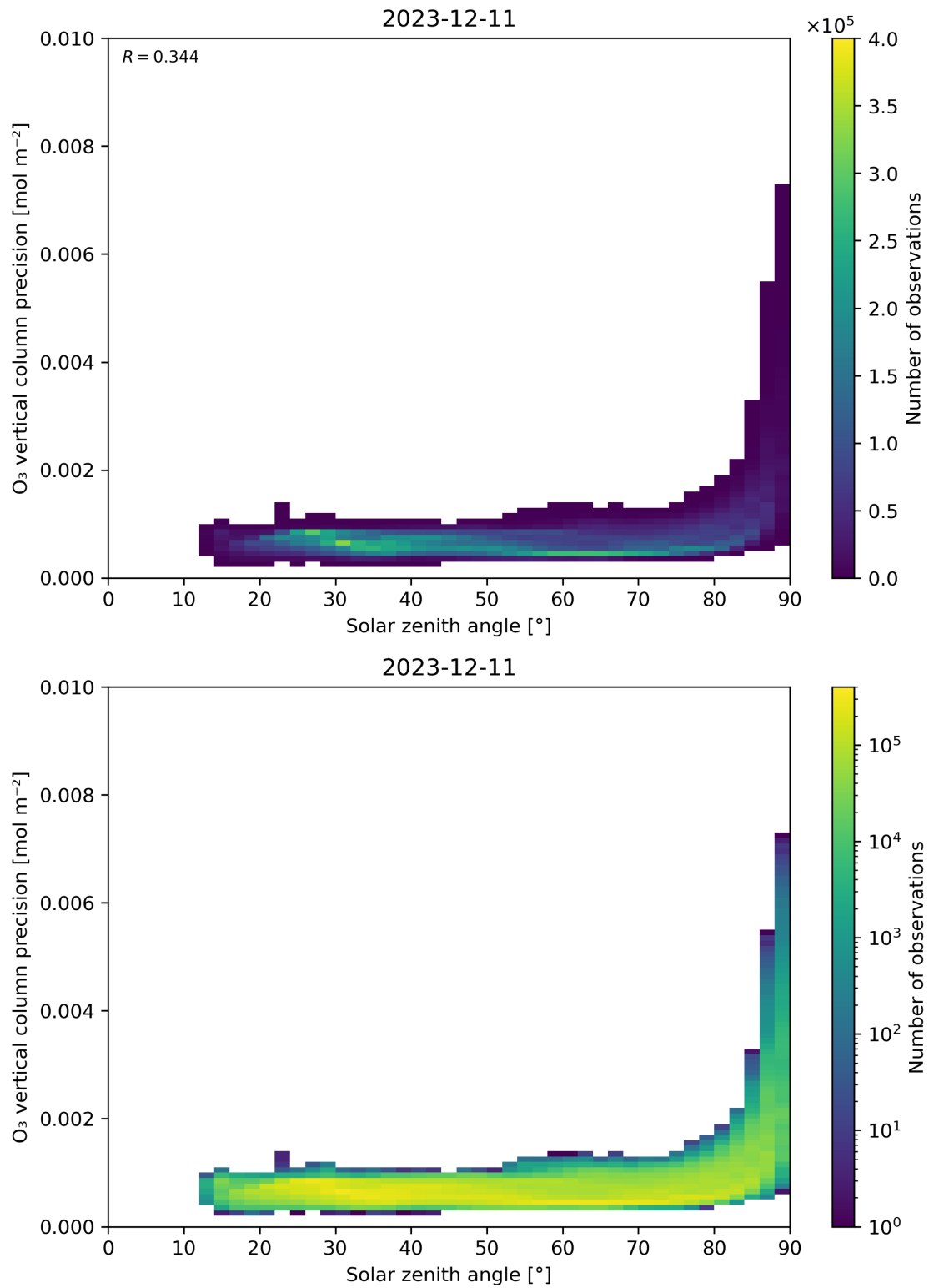
Figure 48: Scatter density plot of “Solar zenith angle” against “O 3 vertical column precision” for 2023-12-10 to 2023-12-12.
