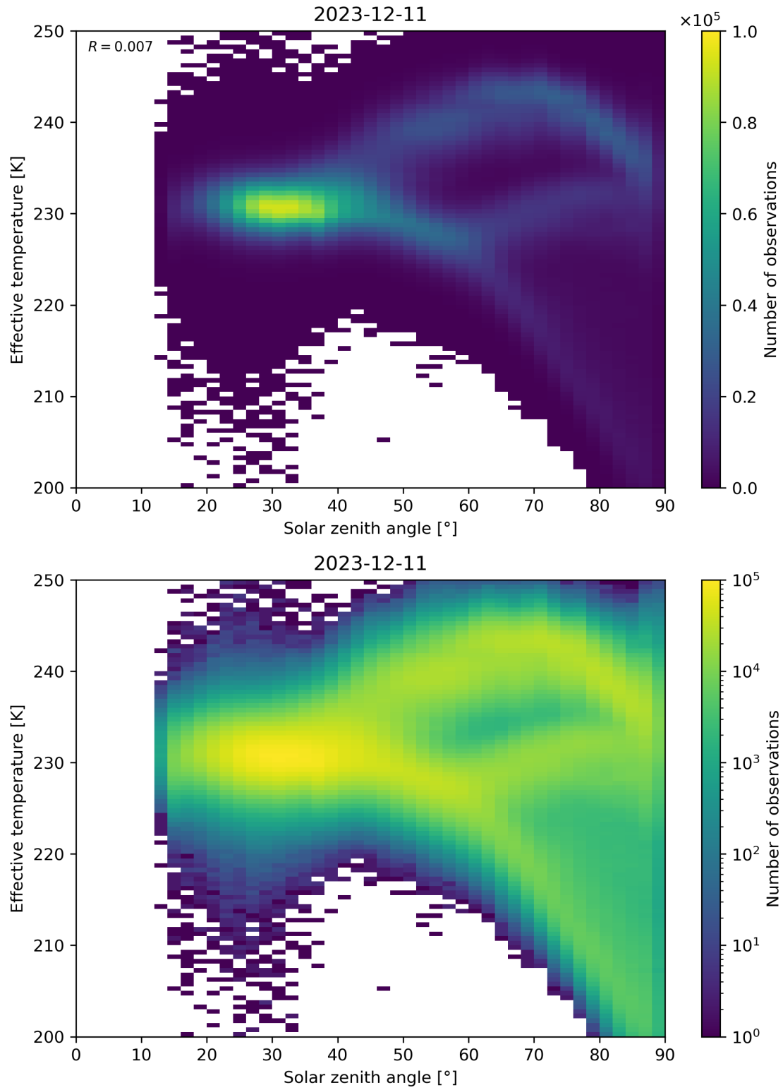
Figure 45: Scatter density plot of “Solar zenith angle” against “Effective temperature” for 2023-12-10 to 2023-12-12.
