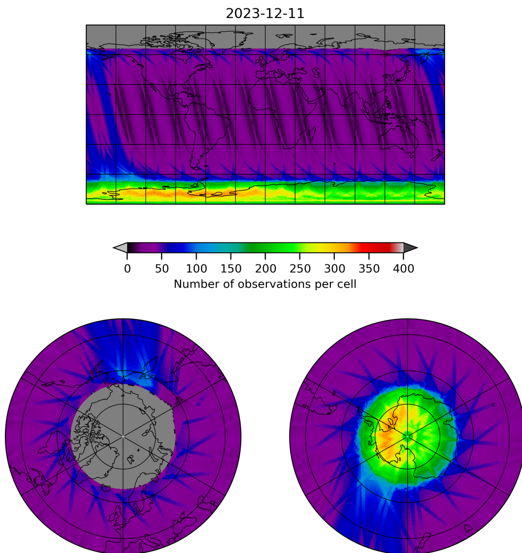
Figure 12: Map of the number of observations for 2023-12-10 to 2023-12-12
