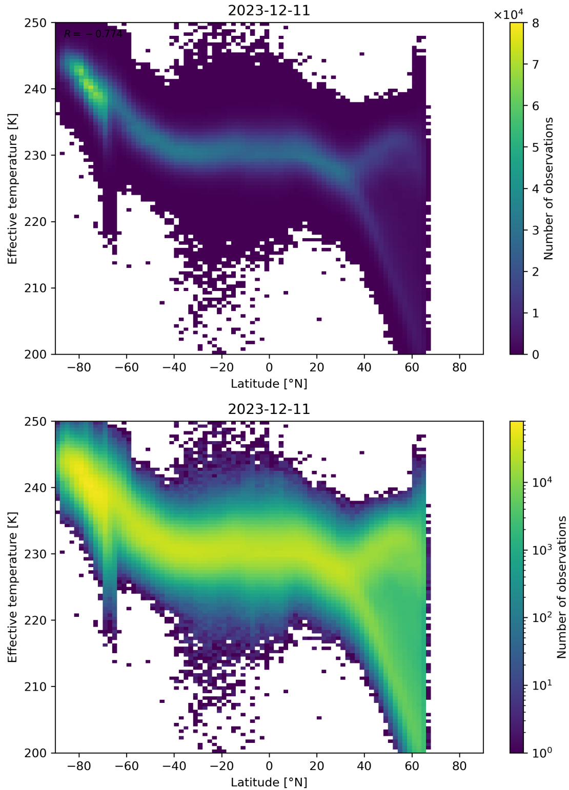
Figure 34: Scatter density plot of “Latitude” against “Effective temperature” for 2023-12-10 to 2023-12-12.
