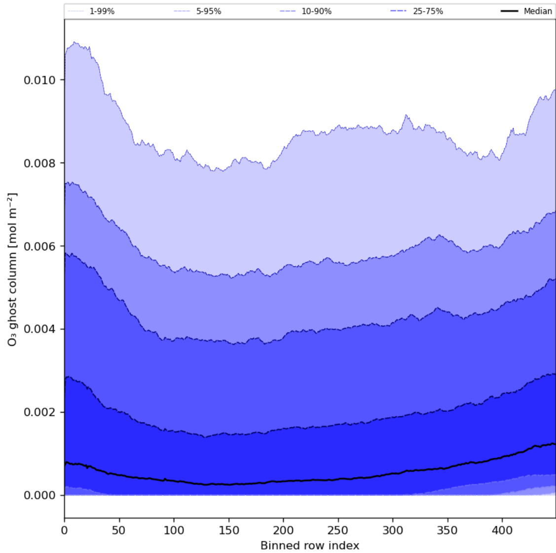
Figure 32: Along track statistics of “O 3 ghost column” for 2023-12-10 to 2023-12-12
