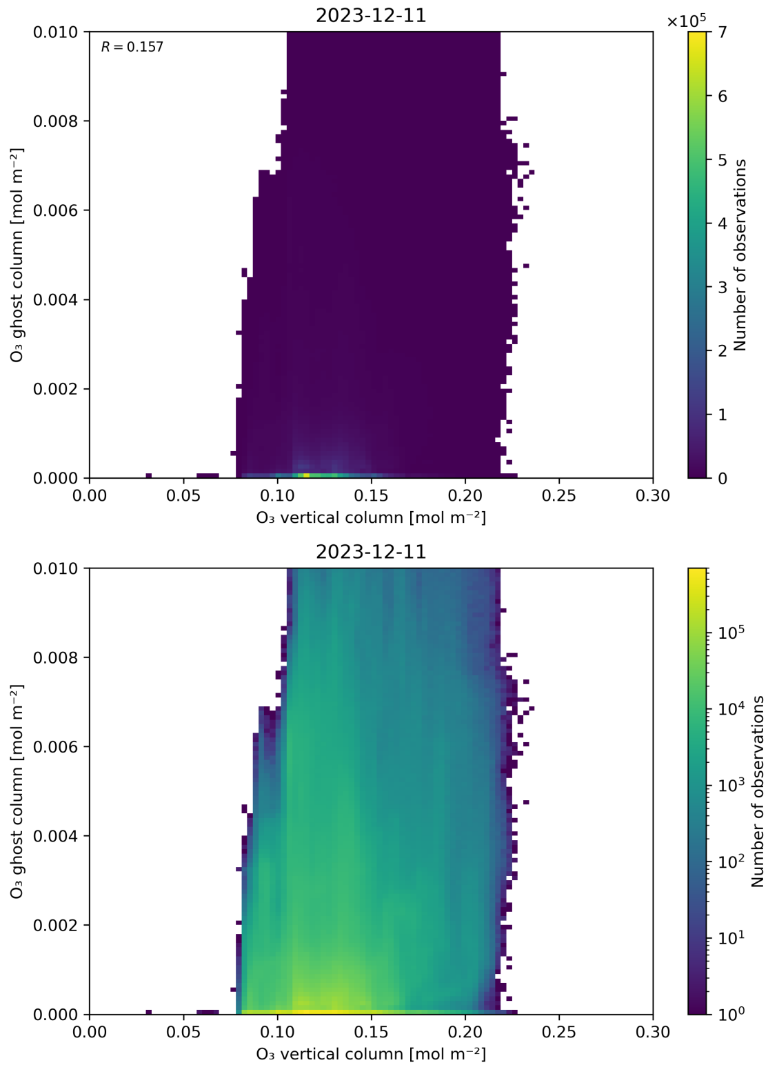
Figure 40: Scatter density plot of “O 3 vertical column” against “O 3 ghost column” for 2023-12-10 to 2023-12-12.
