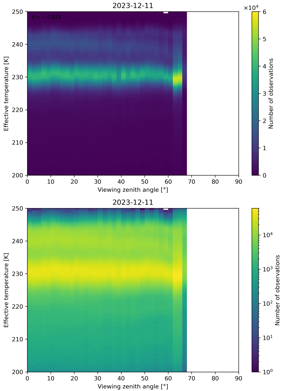
Figure 50: Scatter density plot of “Viewing zenith angle” against “Effective temperature” for 2023-12-10 to 2023-12-12.
