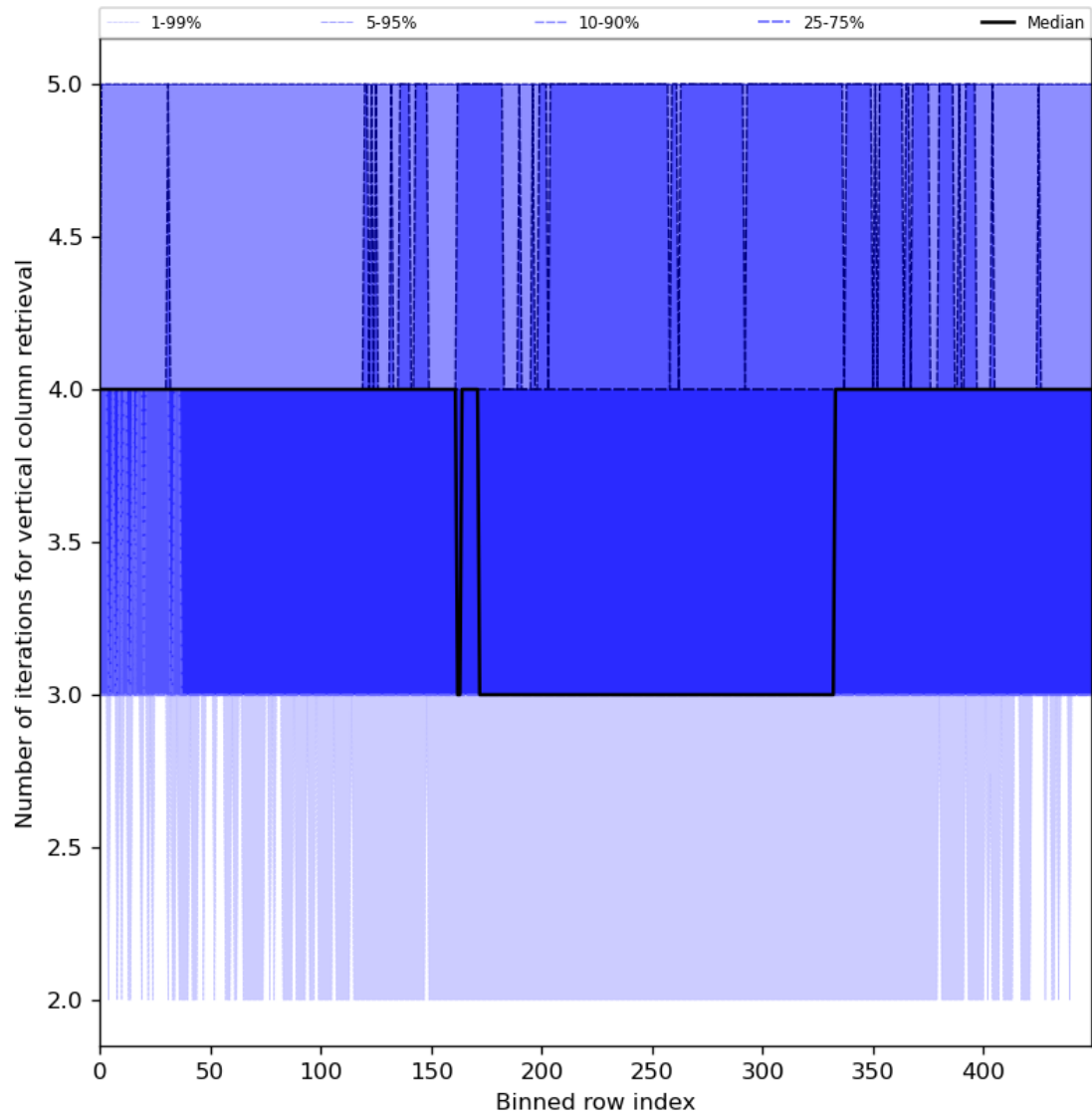
Figure 33: Along track statistics of “Number of iterations for vertical column retrieval” for 2023-12-10 to 2023-12-12
