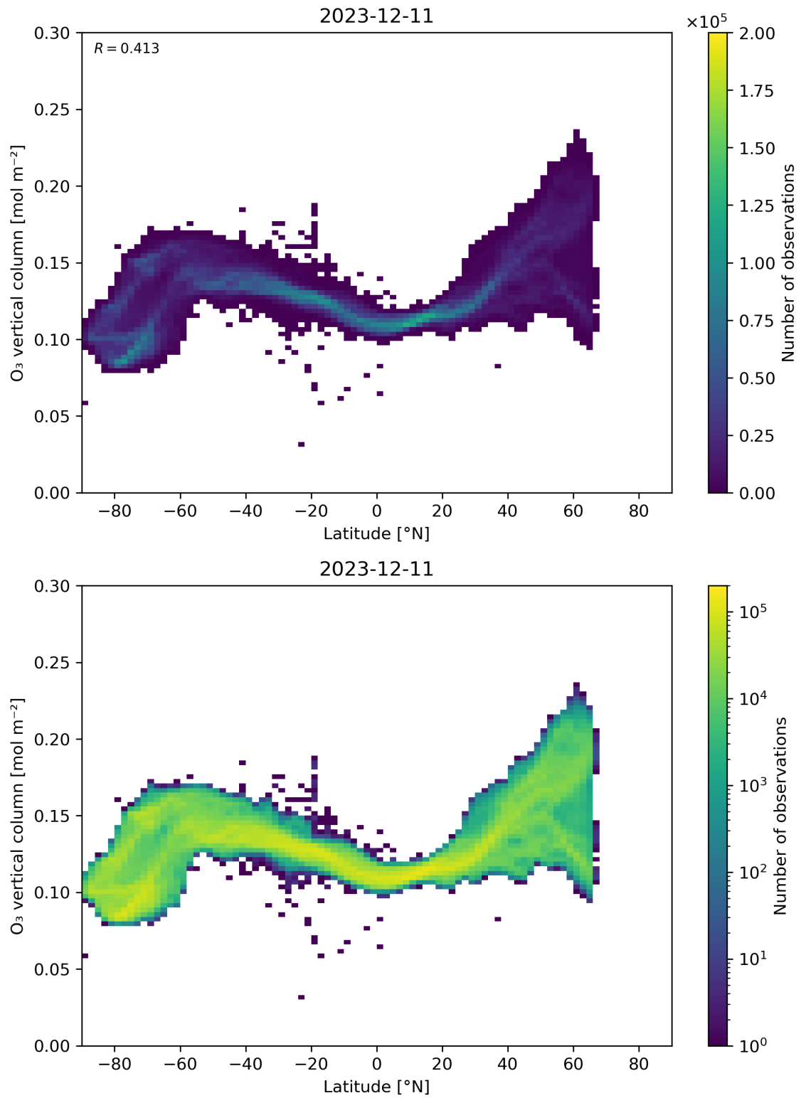
Figure 36: Scatter density plot of “Latitude” against “O 3 vertical column” for 2023-12-10 to 2023-12-12.
