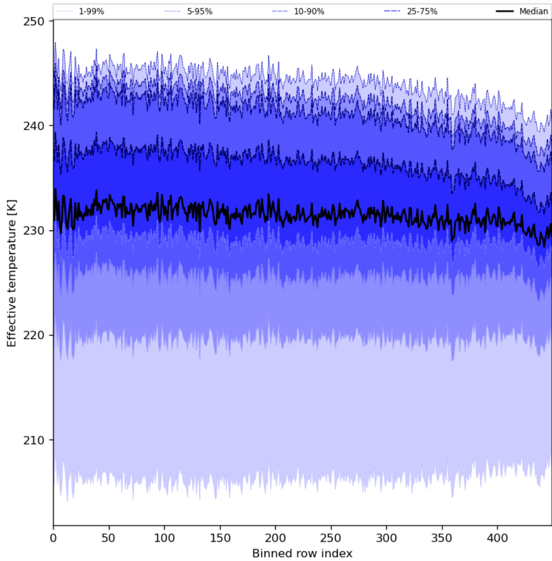
Figure 31: Along track statistics of “Effective temperature” for 2023-12-10 to 2023-12-12
