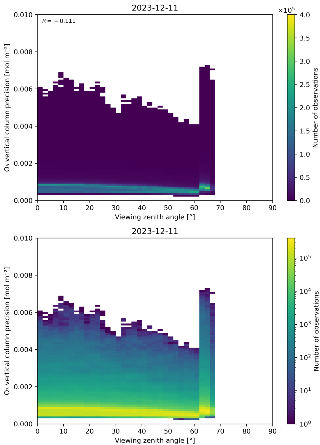
Figure 53: Scatter density plot of “Viewing zenith angle” against “O 3 vertical column precision” for 2023-12-10 to 2023-12-12.
