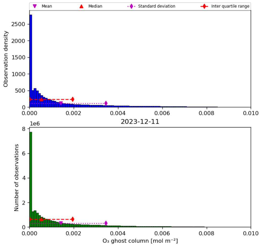
Figure 25: Histogram of “O 3 ghost column” for 2023-12-10 to 2023-12-12
