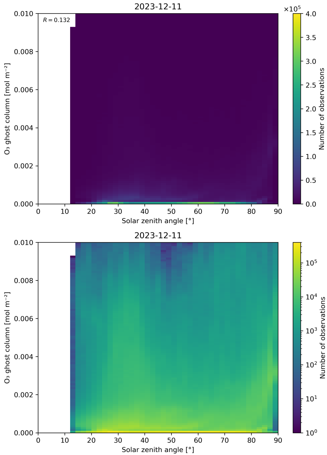
Figure 46: Scatter density plot of “Solar zenith angle” against “O 3 ghost column” for 2023-12-10 to 2023-12-12.
