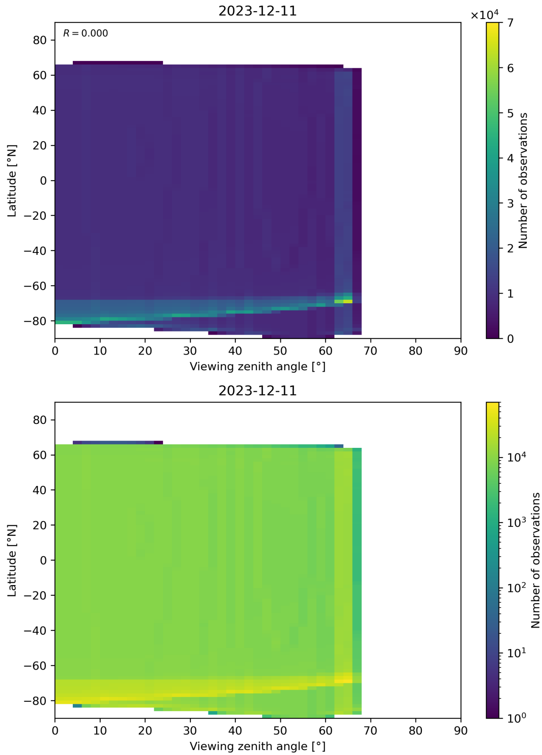
Figure 49: Scatter density plot of “Viewing zenith angle” against “Latitude” for 2023-12-10 to 2023-12-12.
