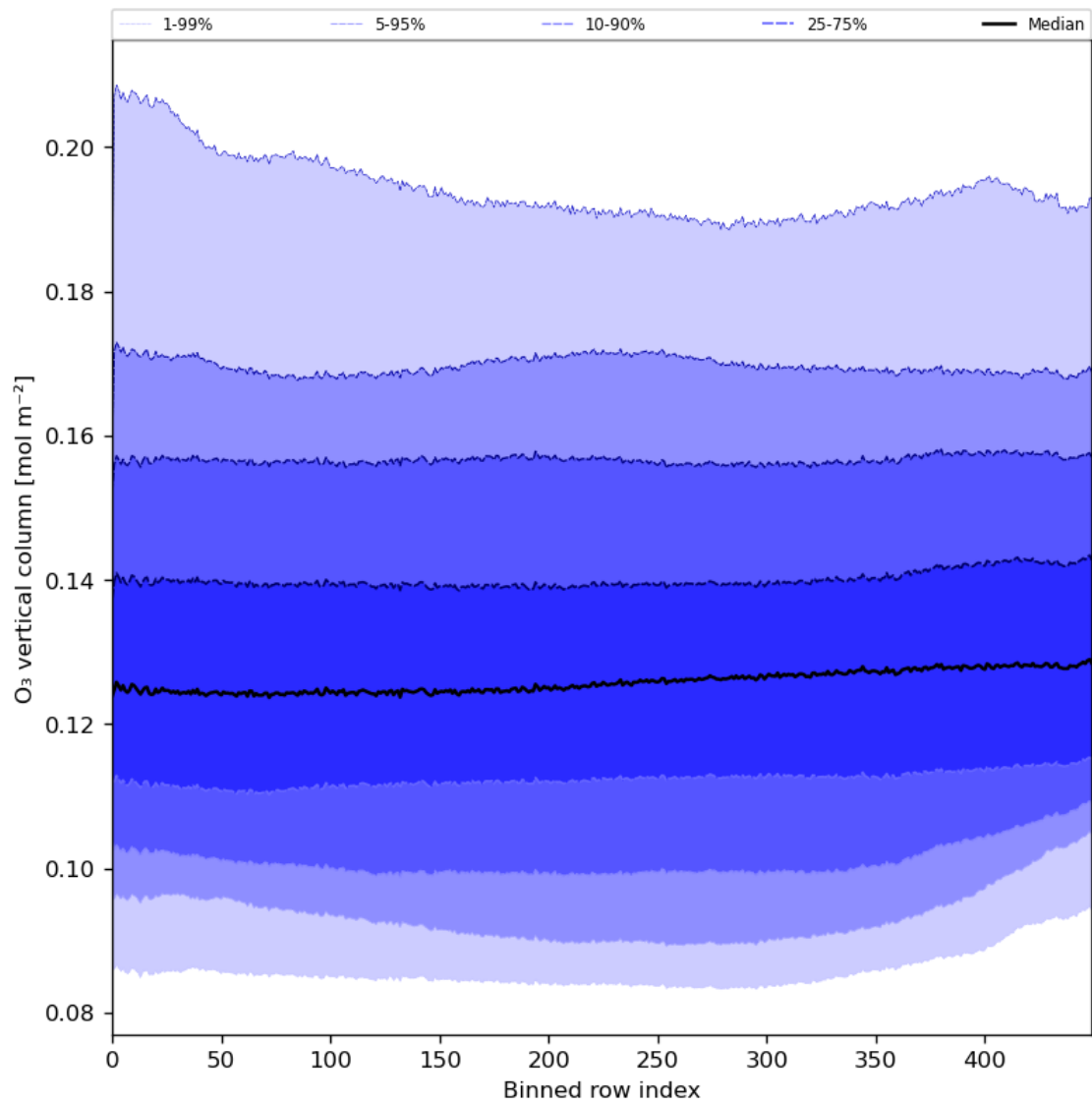
Figure 28: Along track statistics of “O 3 vertical column” for 2023-12-10 to 2023-12-12
