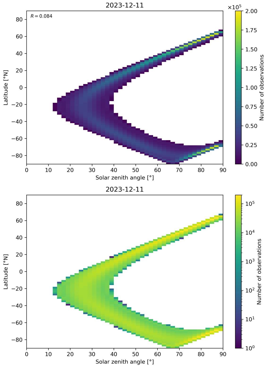
Figure 44: Scatter density plot of “Solar zenith angle” against “Latitude” for 2023-12-10 to 2023-12-12.
