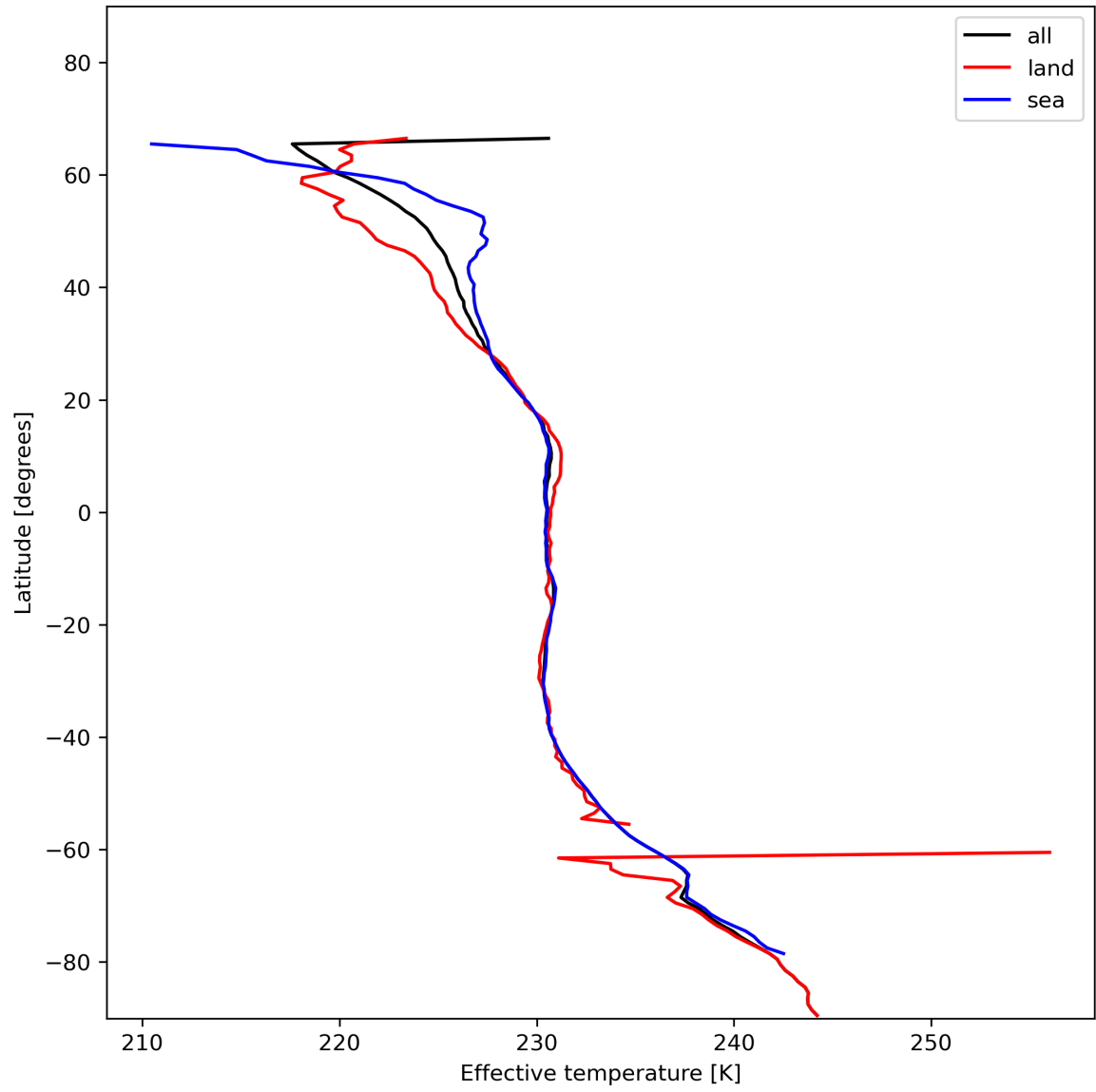
Figure 17: Zonal average of “Effective temperature” for 2023-12-10 to 2023-12-12.
