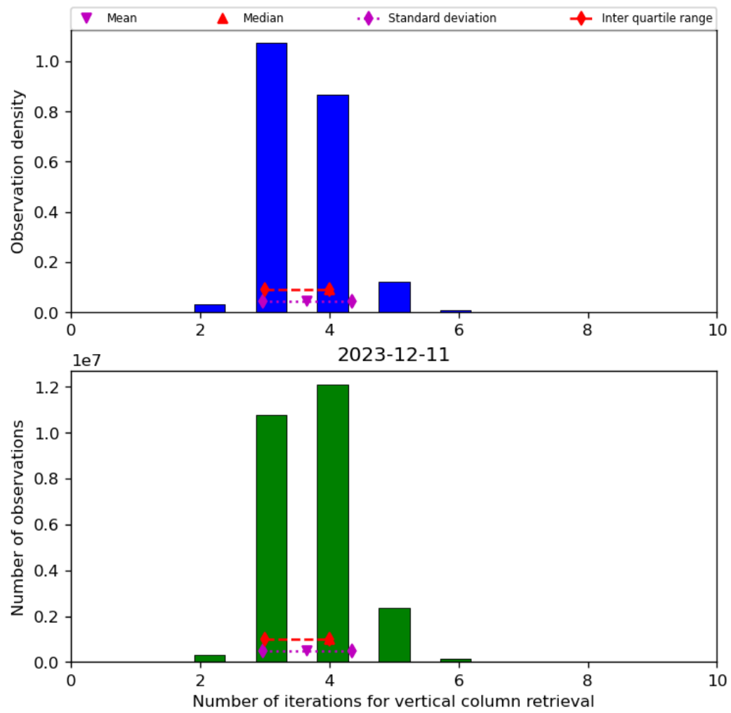
Figure 26: Histogram of “Number of iterations for vertical column retrieval” for 2023-12-10 to 2023-12-12
