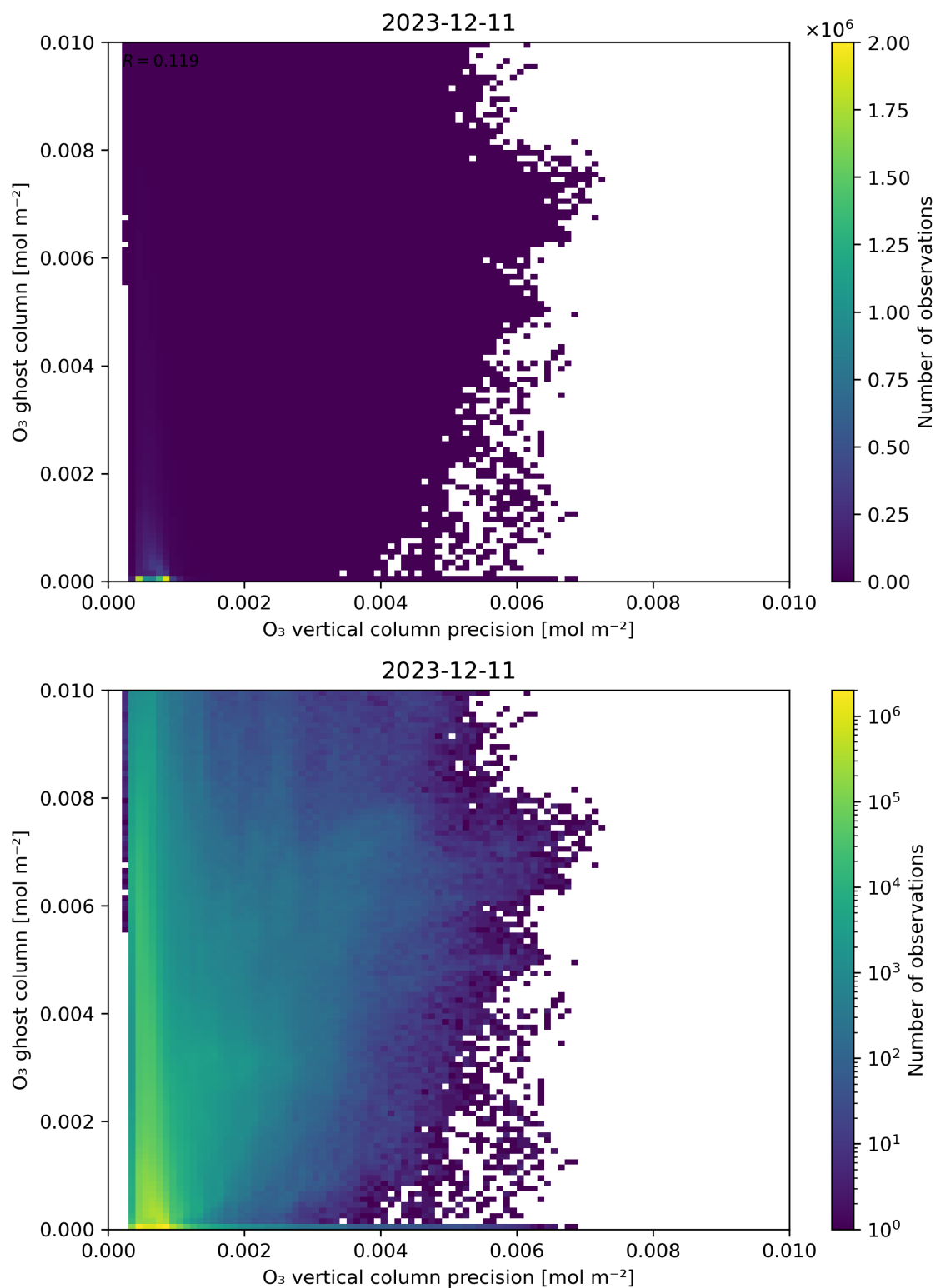
Figure 43: Scatter density plot of “ O_3 vertical column precision” against “ O_3 ghost column” for 2023-12-10 to 2023-12-12.
