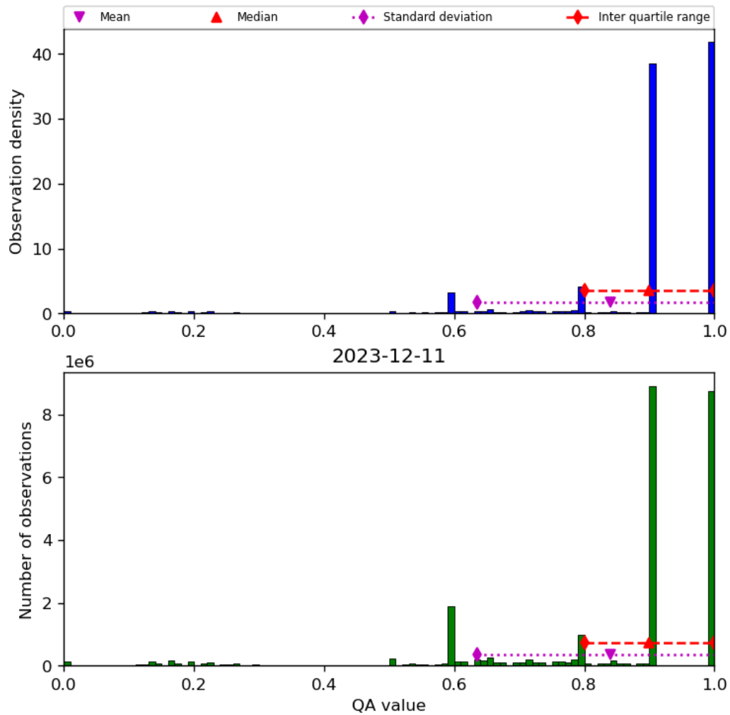
Figure 20: Histogram of “QA value” for 2023-12-10 to 2023-12-12
