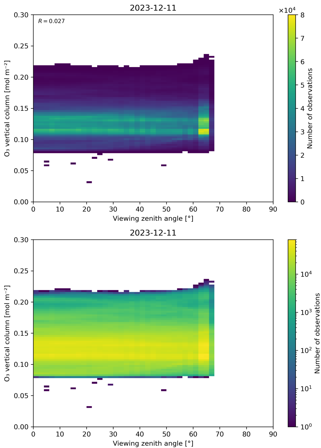
Figure 52: Scatter density plot of “Viewing zenith angle” against “O 3 vertical column” for 2023-12-10 to 2023-12-12.
