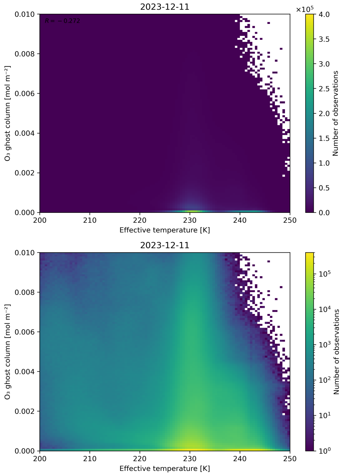
Figure 38: Scatter density plot of “Effective temperature” against “O 3 ghost column” for 2023-12-10 to 2023-12-12.
