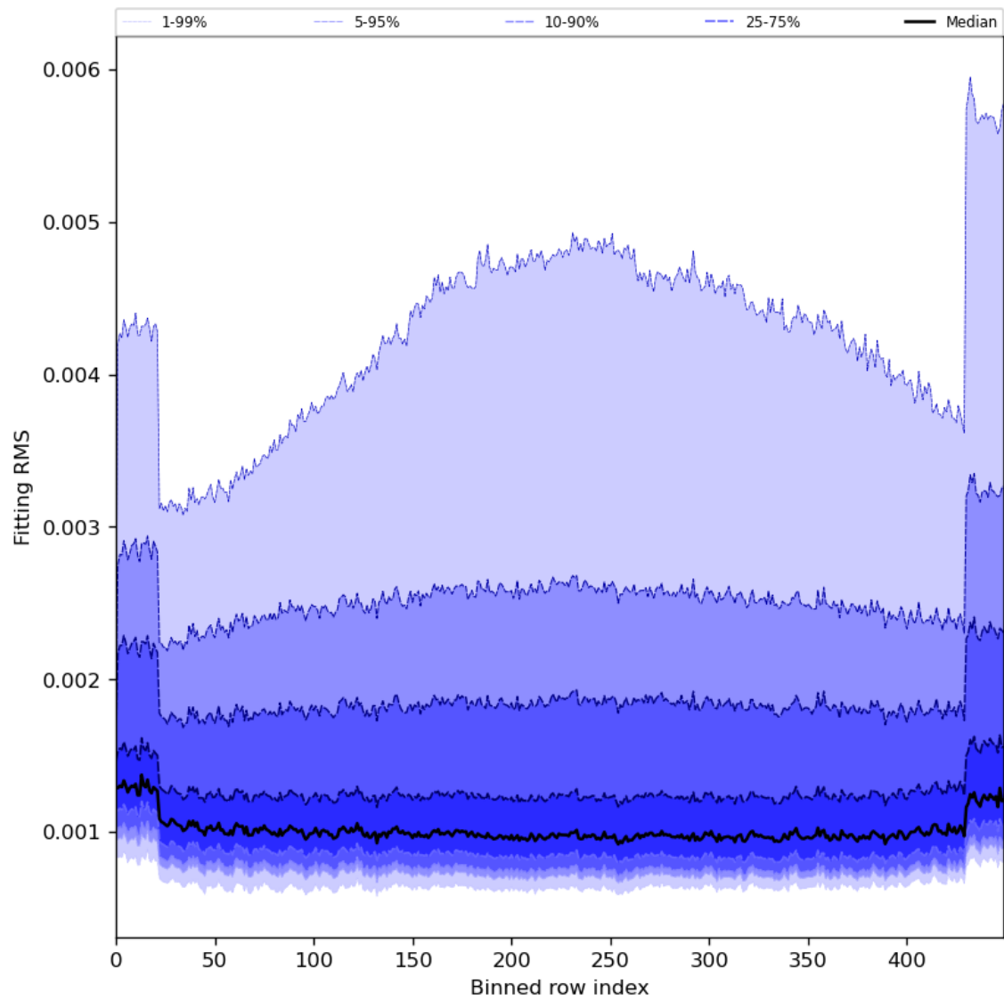
Figure 30: Along track statistics of “Fitting RMS” for 2023-12-10 to 2023-12-12
