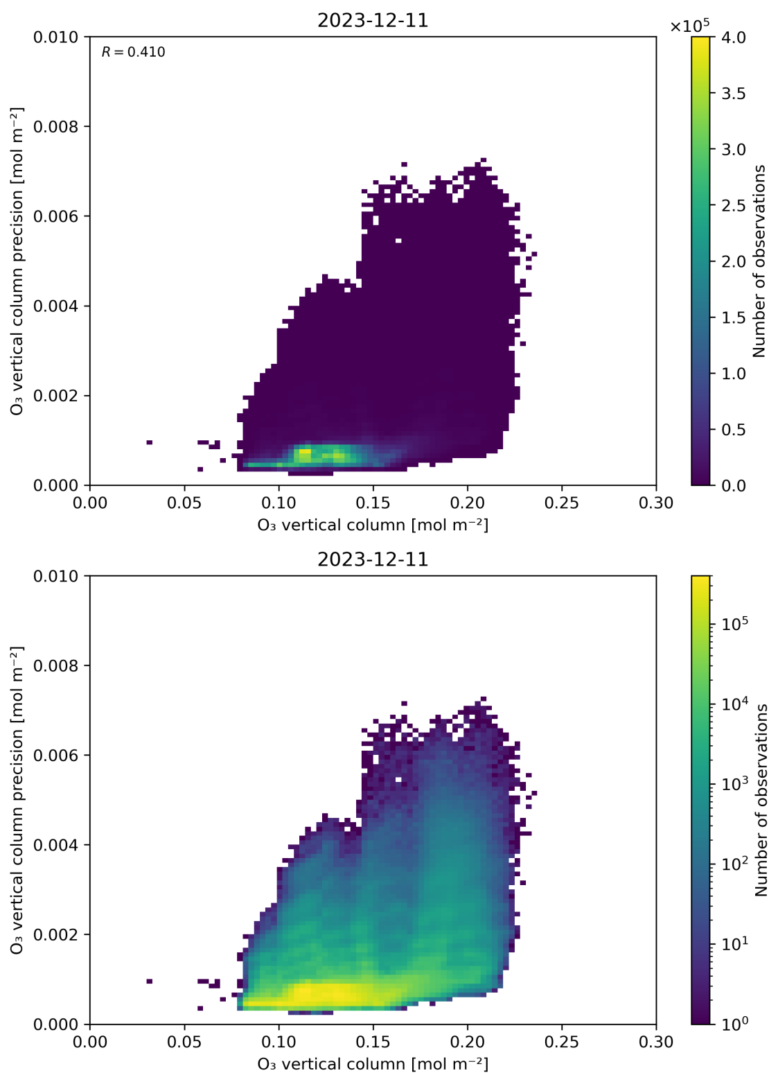
Figure 41: Scatter density plot of “O 3 vertical column” against “O 3 vertical column precision” for 2023-12-10 to 2023-12-12.
