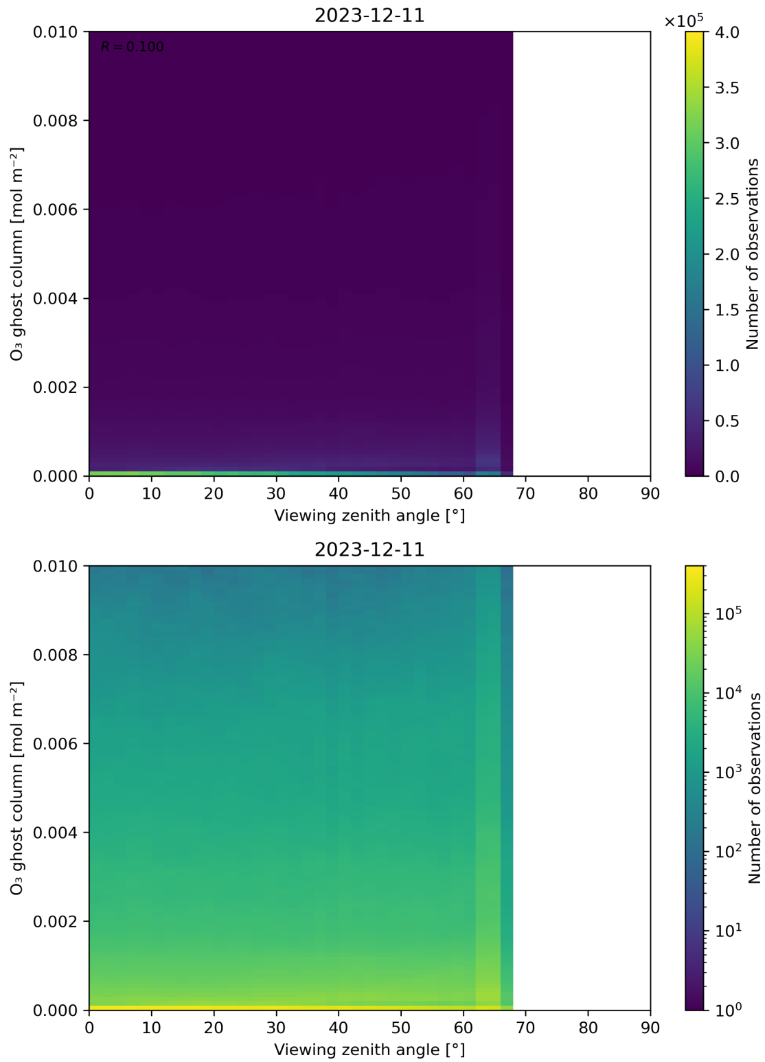
Figure 51: Scatter density plot of “Viewing zenith angle” against “O 3 ghost column” for 2023-12-10 to 2023-12-12.
