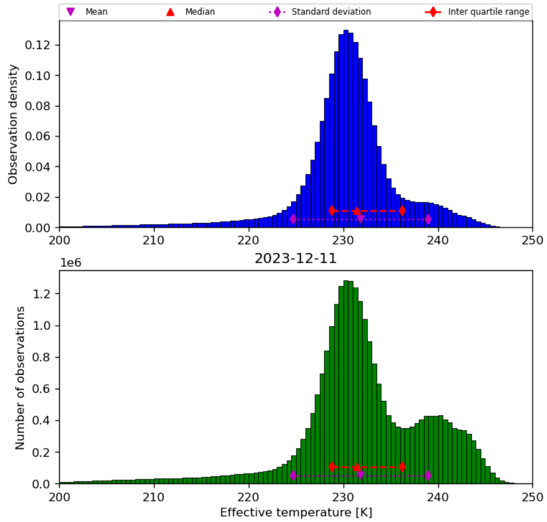
Figure 24: Histogram of “Effective temperature” for 2023-12-10 to 2023-12-12
