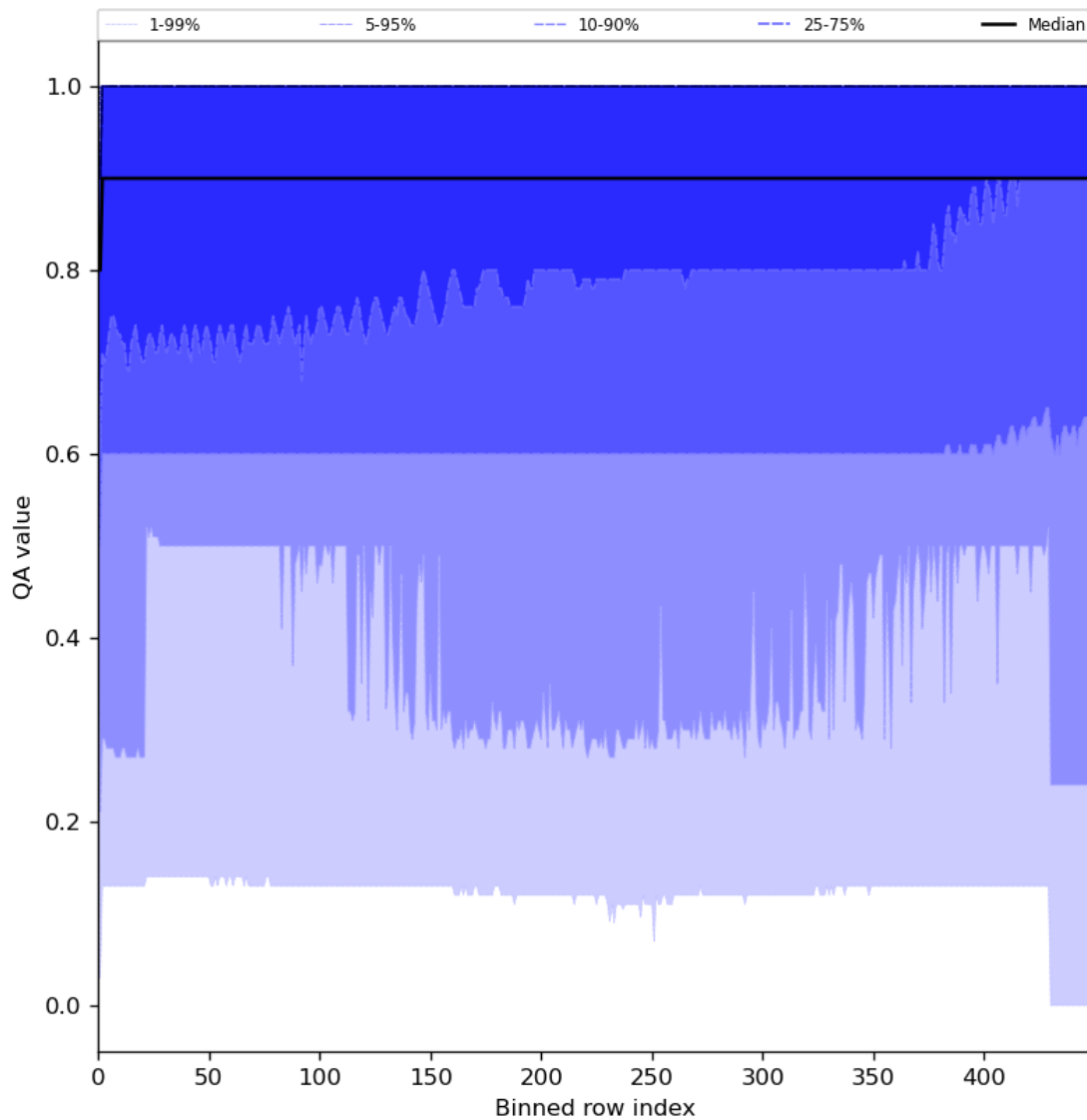
Figure 27: Along track statistics of “QA value” for 2023-12-10 to 2023-12-12
